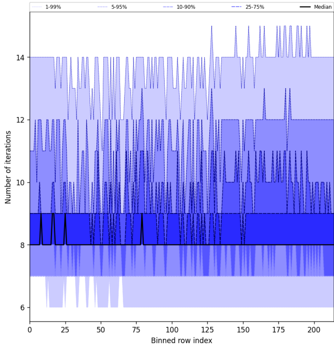
Figure 32: Along track statistics of “Number of iterations” for 2025-09-22 to 2025-09-24
