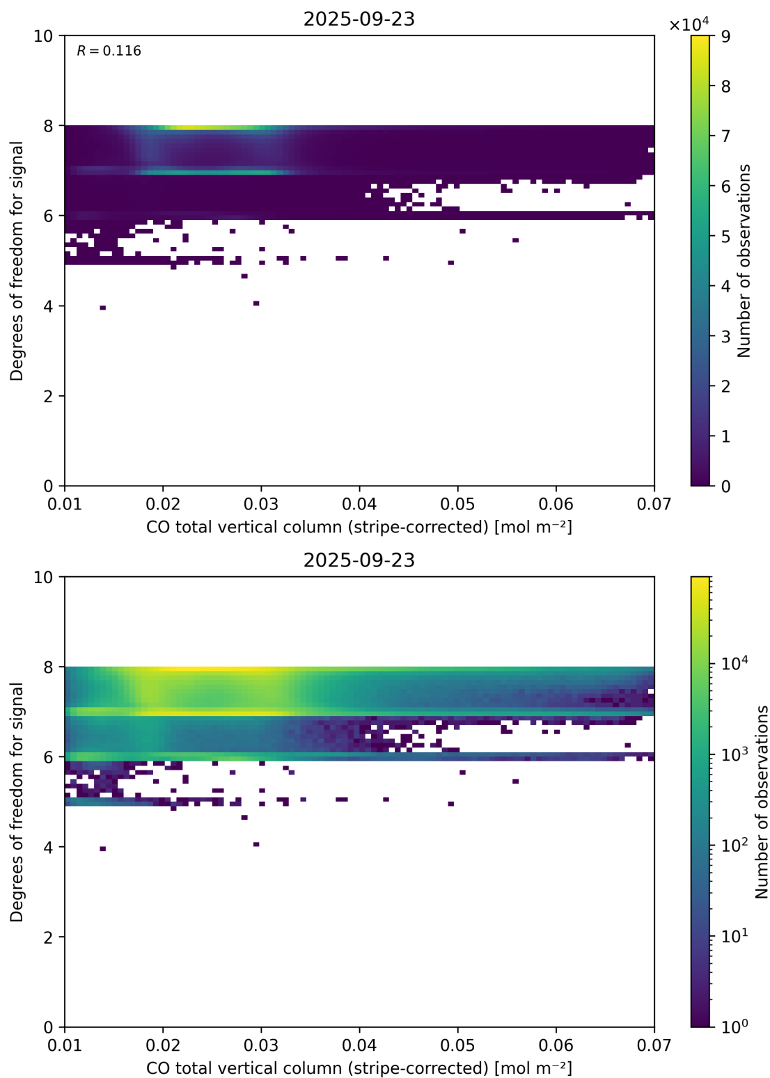
Figure 38: Scatter density plot of “CO total vertical column (stripe-corrected)” against “Degrees of freedom for signal” for 2025-09-22 to 2025-09-24.
