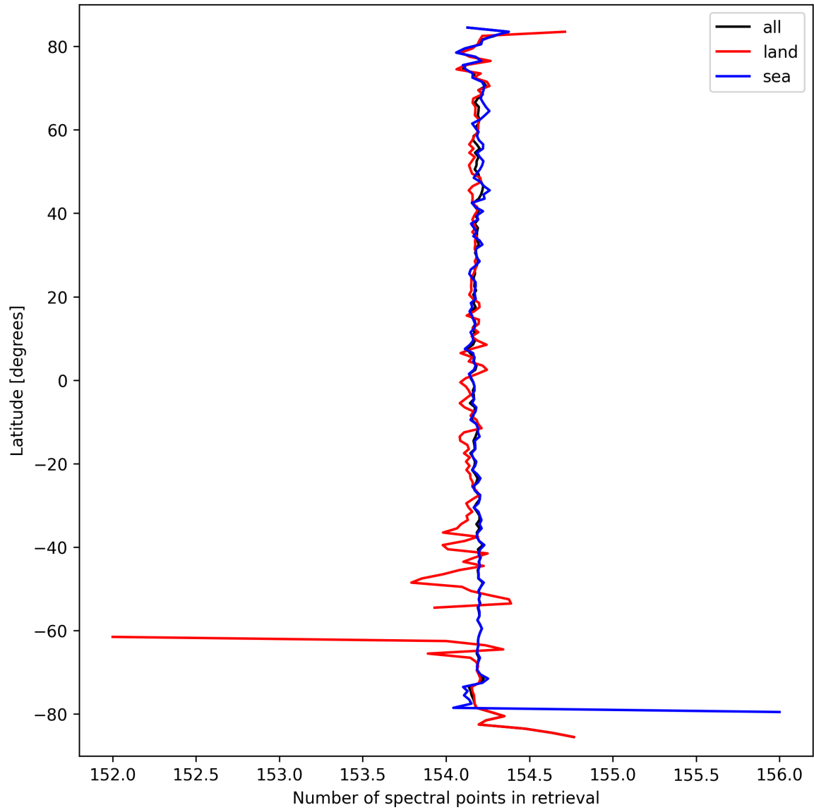
Figure 13: Zonal average of “Number of spectral points in retrieval” for 2025-09-22 to 2025-09-24.
