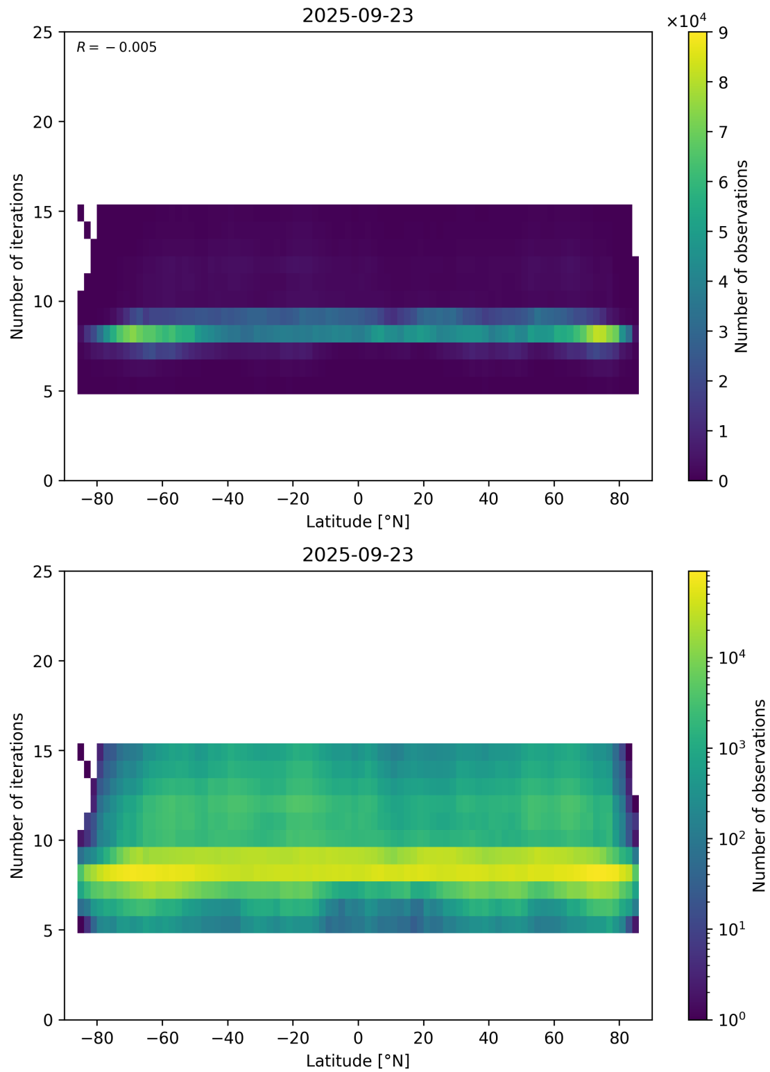
Figure 56: Scatter density plot of “Latitude” against “Number of iterations” for 2025-09-22 to 2025-09-24.
