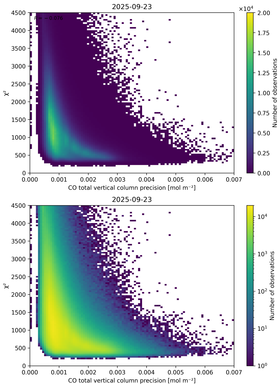
Figure 44: Scatter density plot of “CO total vertical column precision” against “ \chi^2 ” for 2025-09-22 to 2025-09-24.
