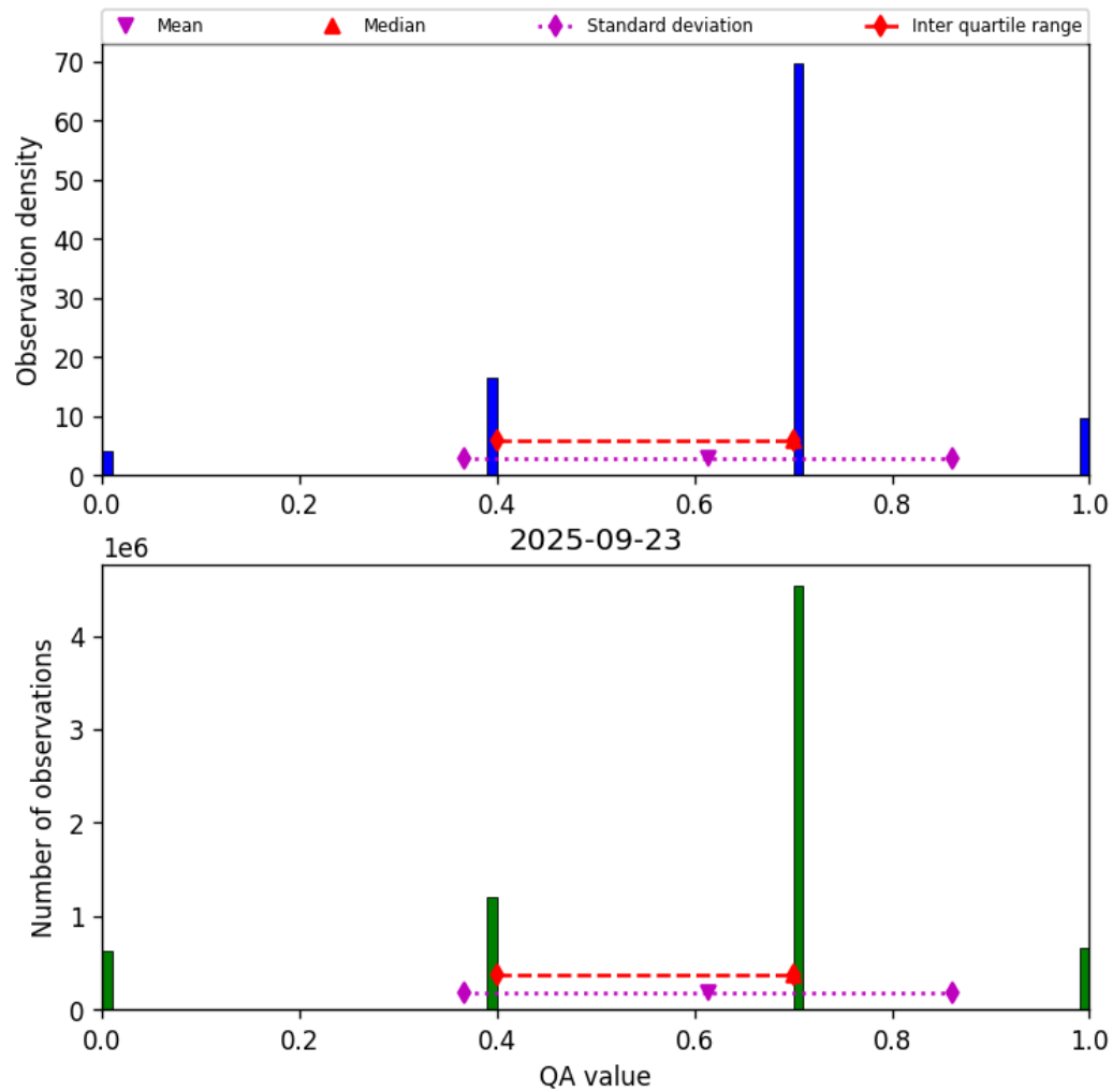
Figure 17: Histogram of “QA value” for 2025-09-22 to 2025-09-24
