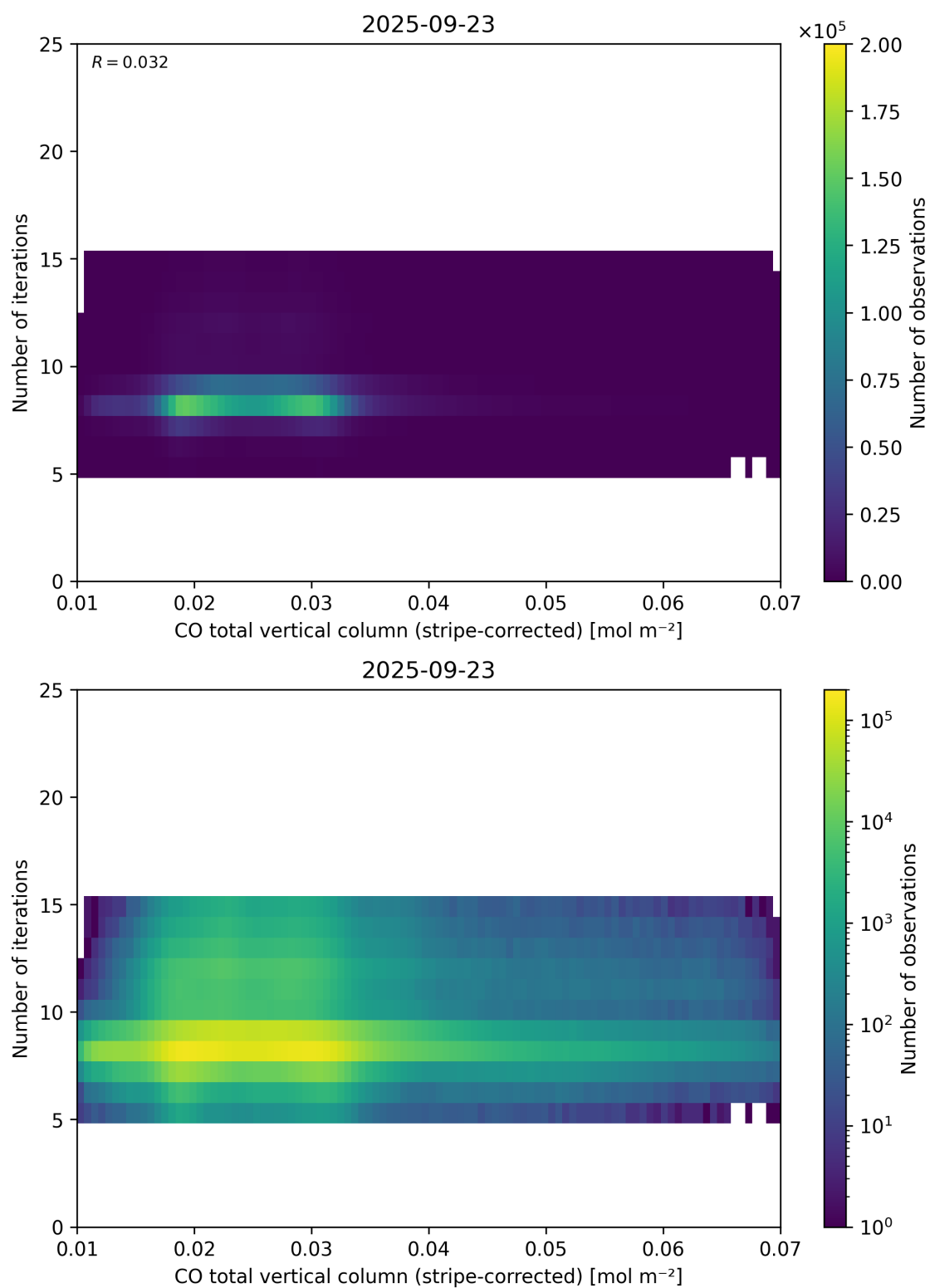
Figure 39: Scatter density plot of “CO total vertical column (stripe-corrected)” against “Number of iterations” for 2025-09-22 to 2025-09-24.
