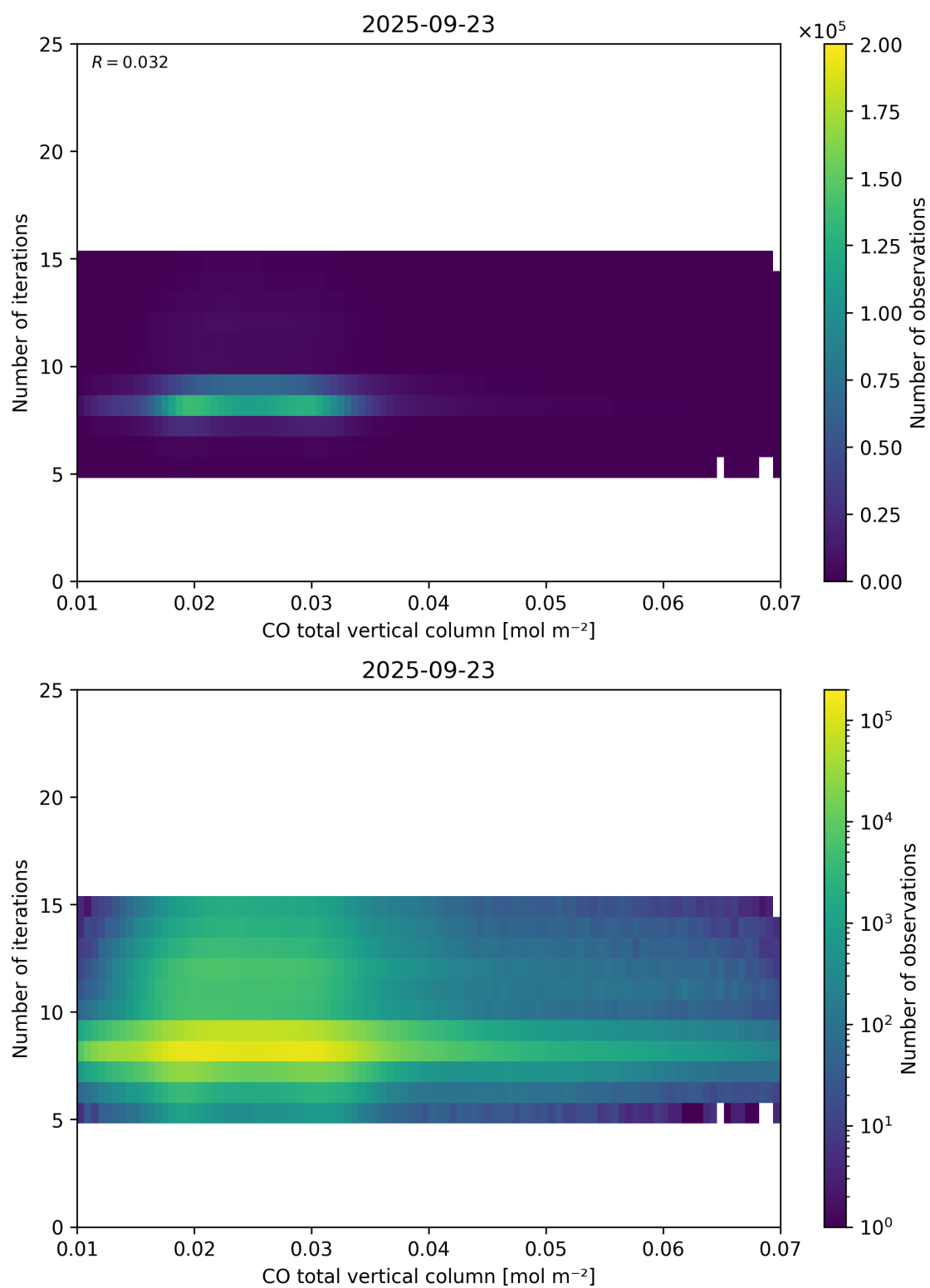
Figure 42: Scatter density plot of “CO total vertical column” against “Number of iterations” for 2025-09-22 to 2025-09-24.
