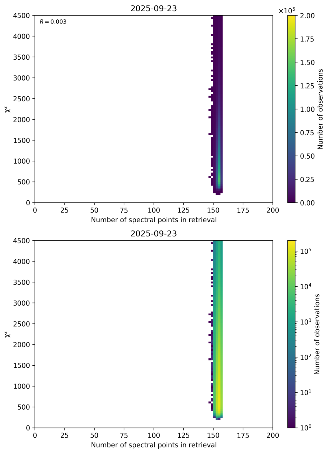
Figure 58: Scatter density plot of “Number of spectral points in retrieval” against “ \chi^2 ” for 2025-09-22 to 2025-09-24.
