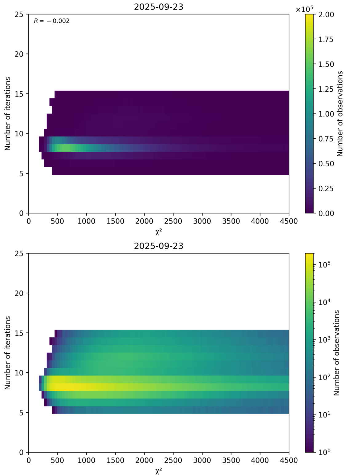
Figure 49: Scatter density plot of “ \chi^2 ” against “Number of iterations” for 2025-09-22 to 2025-09-24.
