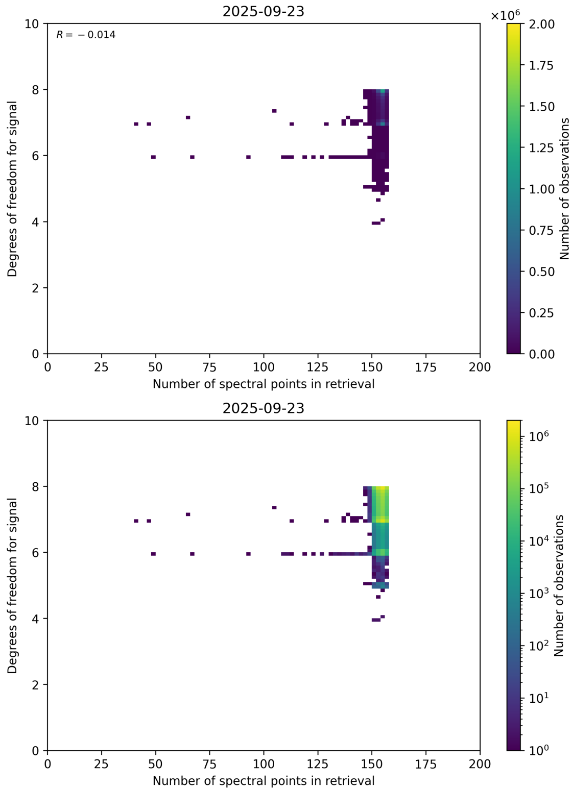
Figure 59: Scatter density plot of “Number of spectral points in retrieval” against “Degrees of freedom for signal” for 2025-09-22 to 2025-09-24.
