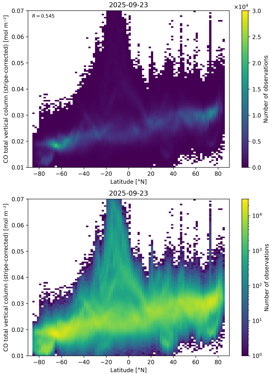
Figure 52: Scatter density plot of “Latitude” against “CO total vertical column (stripe-corrected)” for 2025-09-22 to 2025-09-24.
