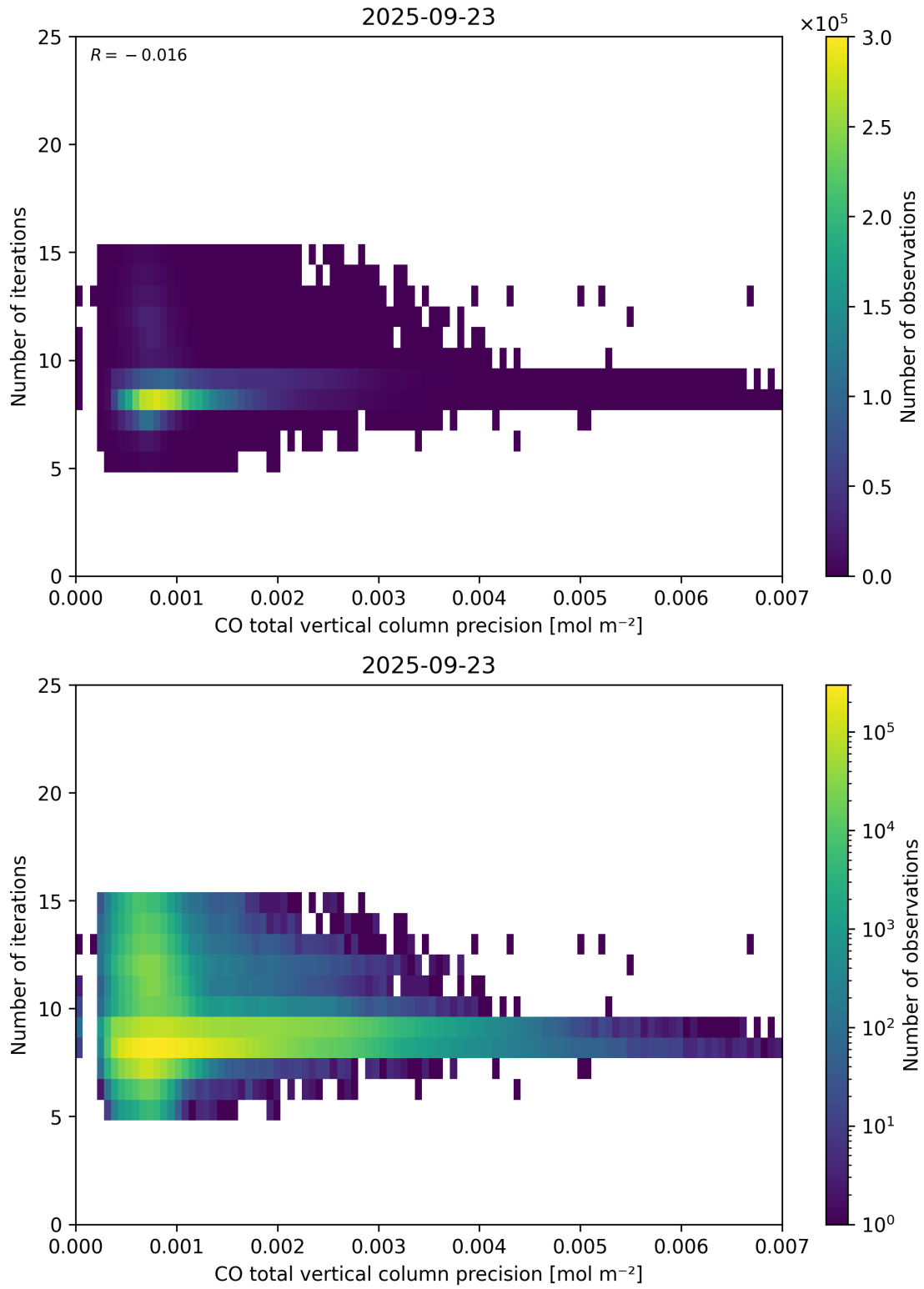
Figure 46: Scatter density plot of “CO total vertical column precision” against “Number of iterations” for 2025-09-22 to 2025-09-24.
