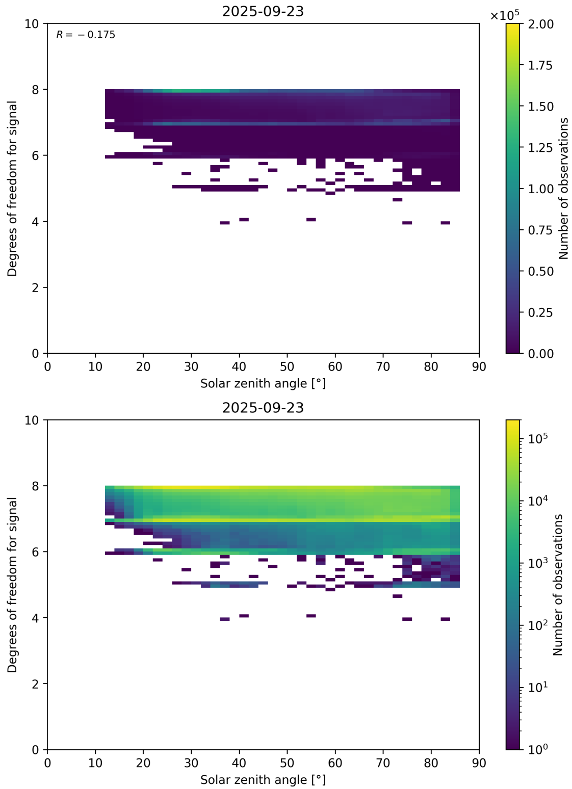
Figure 65: Scatter density plot of “Solar zenith angle” against “Degrees of freedom for signal” for 2025-09-22 to 2025-09-24.
