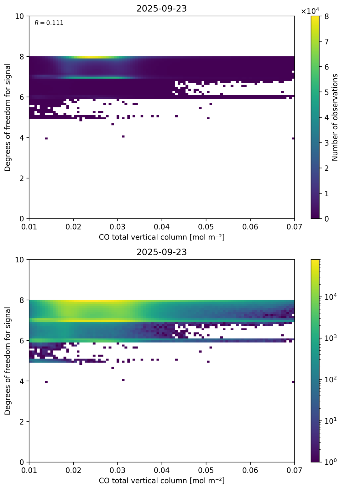
Figure 41: Scatter density plot of “CO total vertical column” against “Degrees of freedom for signal” for 2025-09-22 to 2025-09-24.
