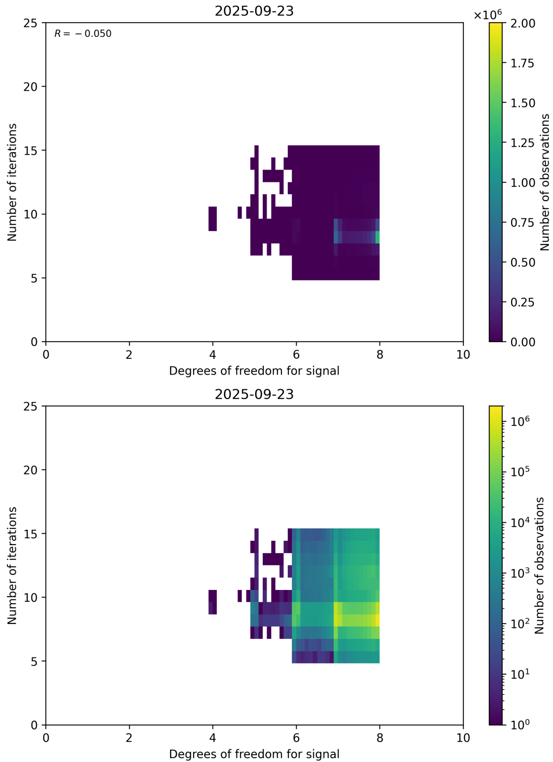
Figure 50: Scatter density plot of “Degrees of freedom for signal” against “Number of iterations” for 2025-09-22 to 2025-09-24.
