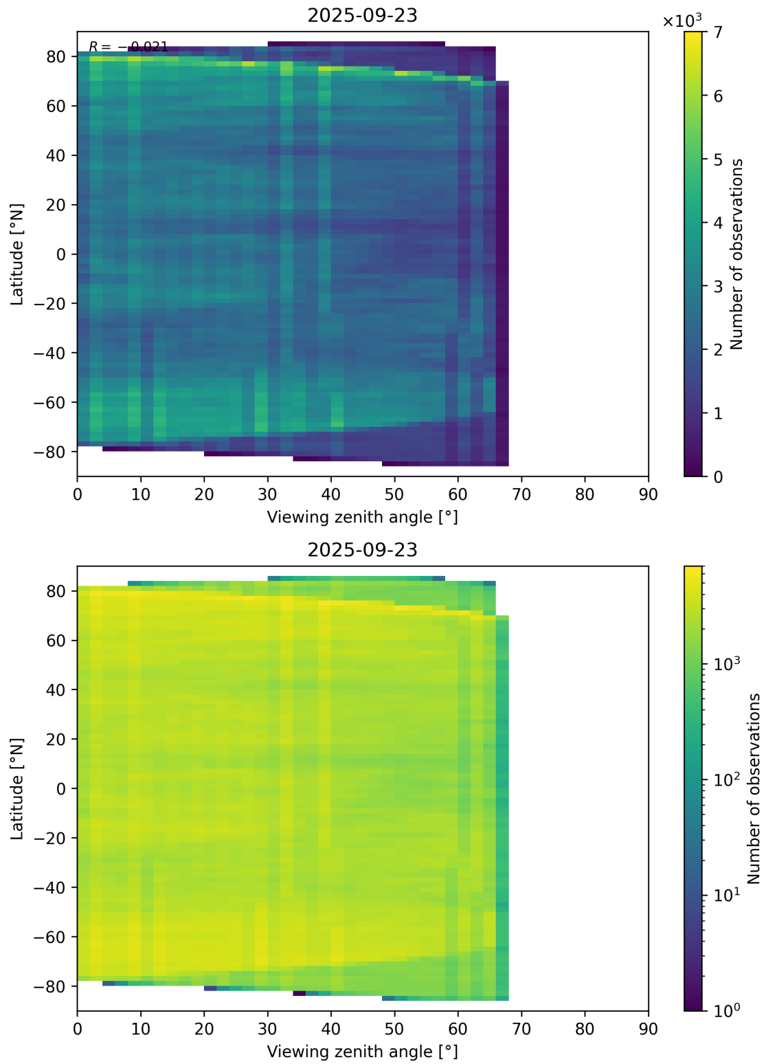
Figure 74: Scatter density plot of “Viewing zenith angle” against “Latitude” for 2025-09-22 to 2025-09-24.
