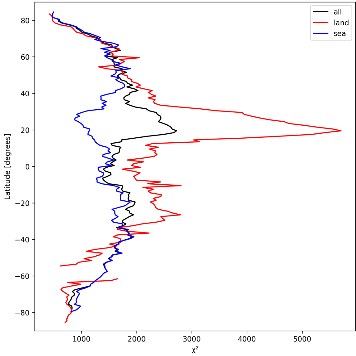
Figure 14: Zonal average of “ \chi^2 ” for 2025-09-22 to 2025-09-24.
