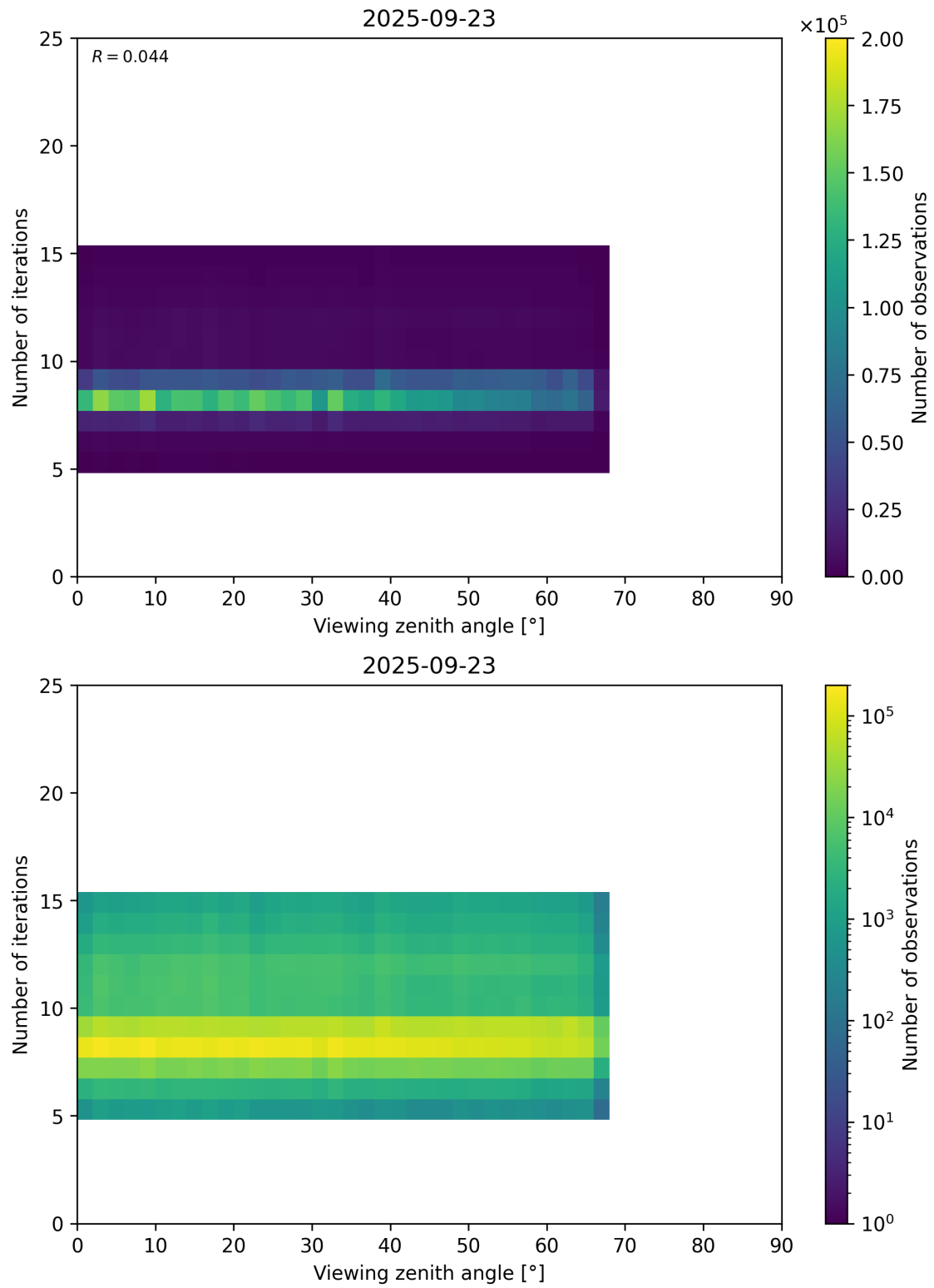
Figure 75: Scatter density plot of “Viewing zenith angle” against “Number of iterations” for 2025-09-22 to 2025-09-24.
