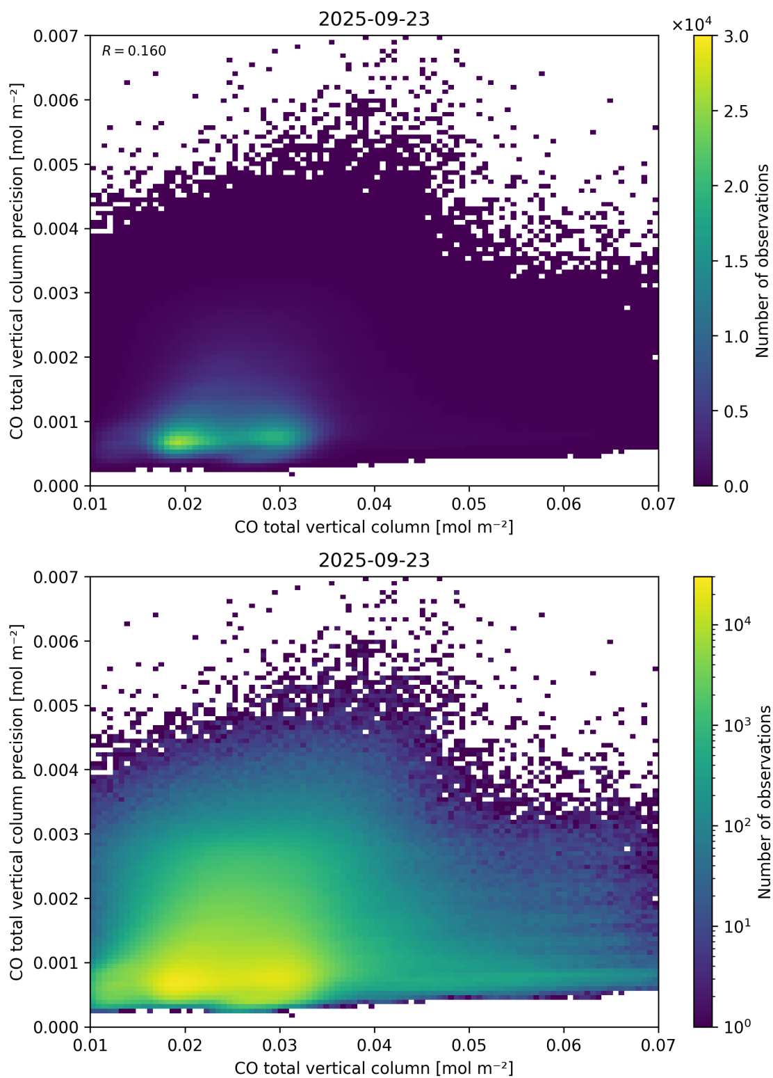
Figure 34: Scatter density plot of “CO total vertical column” against “CO total vertical column precision” for 2025-09-22 to 2025-09-24.
