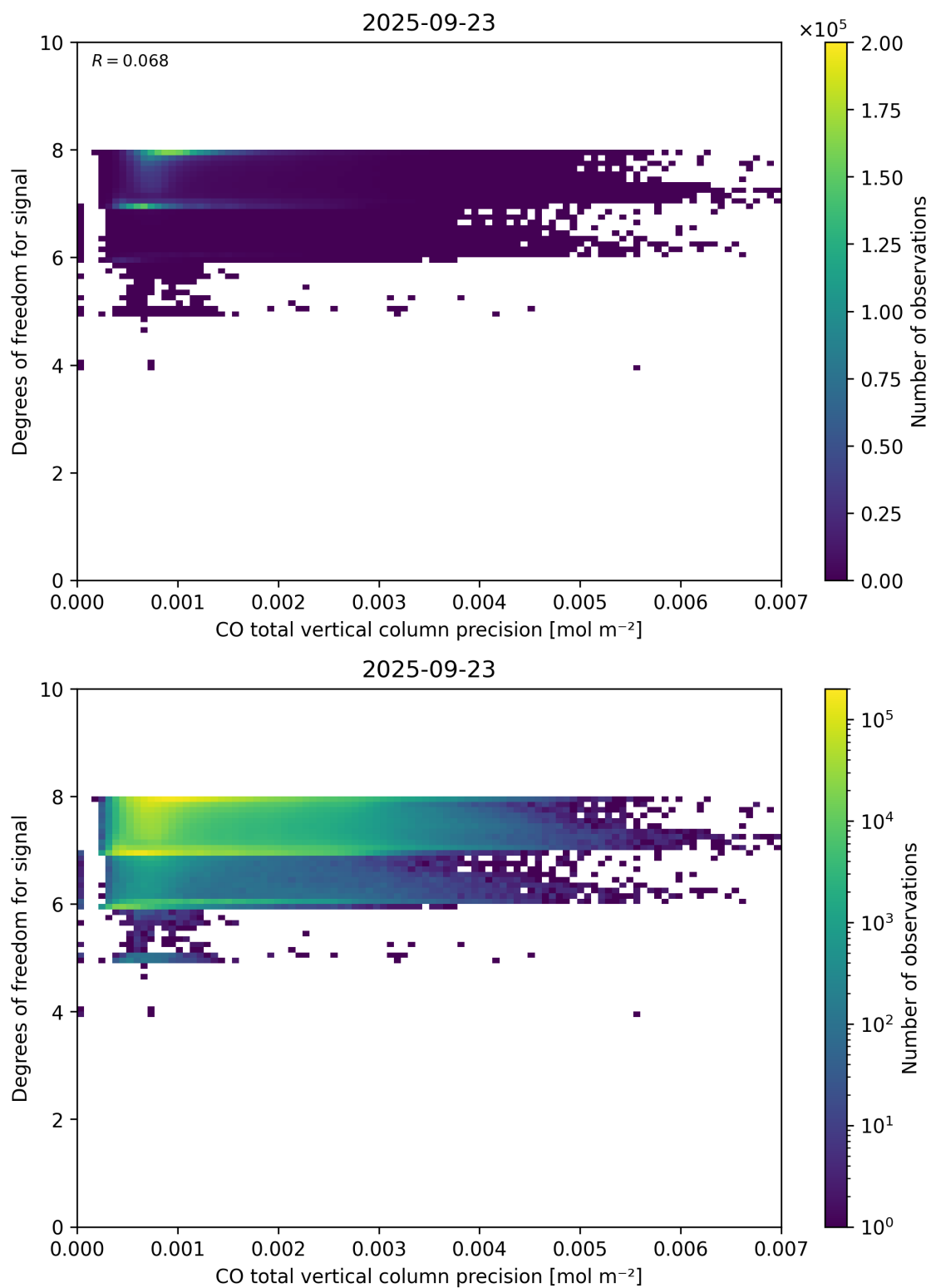
Figure 45: Scatter density plot of “CO total vertical column precision” against “Degrees of freedom for signal” for 2025-09-22 to 2025-09-24.
