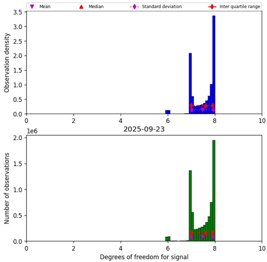
Figure 23: Histogram of “Degrees of freedom for signal” for 2025-09-22 to 2025-09-24
