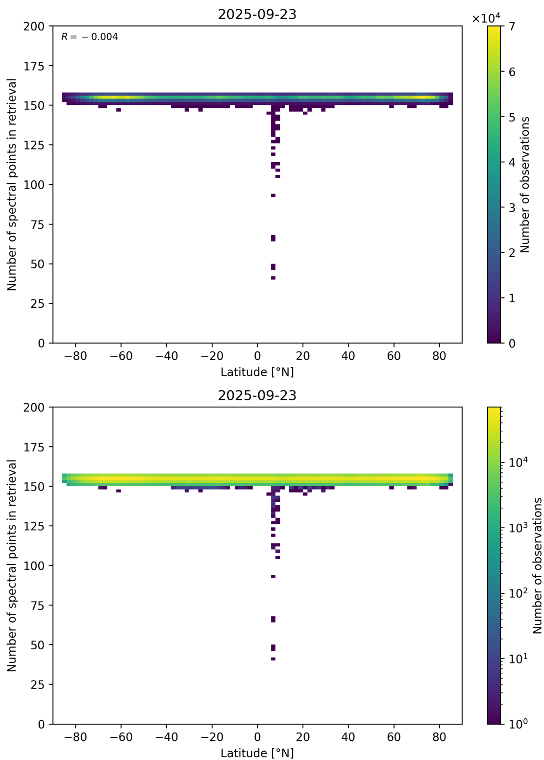
Figure 57: Scatter density plot of “Latitude” against “Number of spectral points in retrieval” for 2025-09-22 to 2025-09-24.
