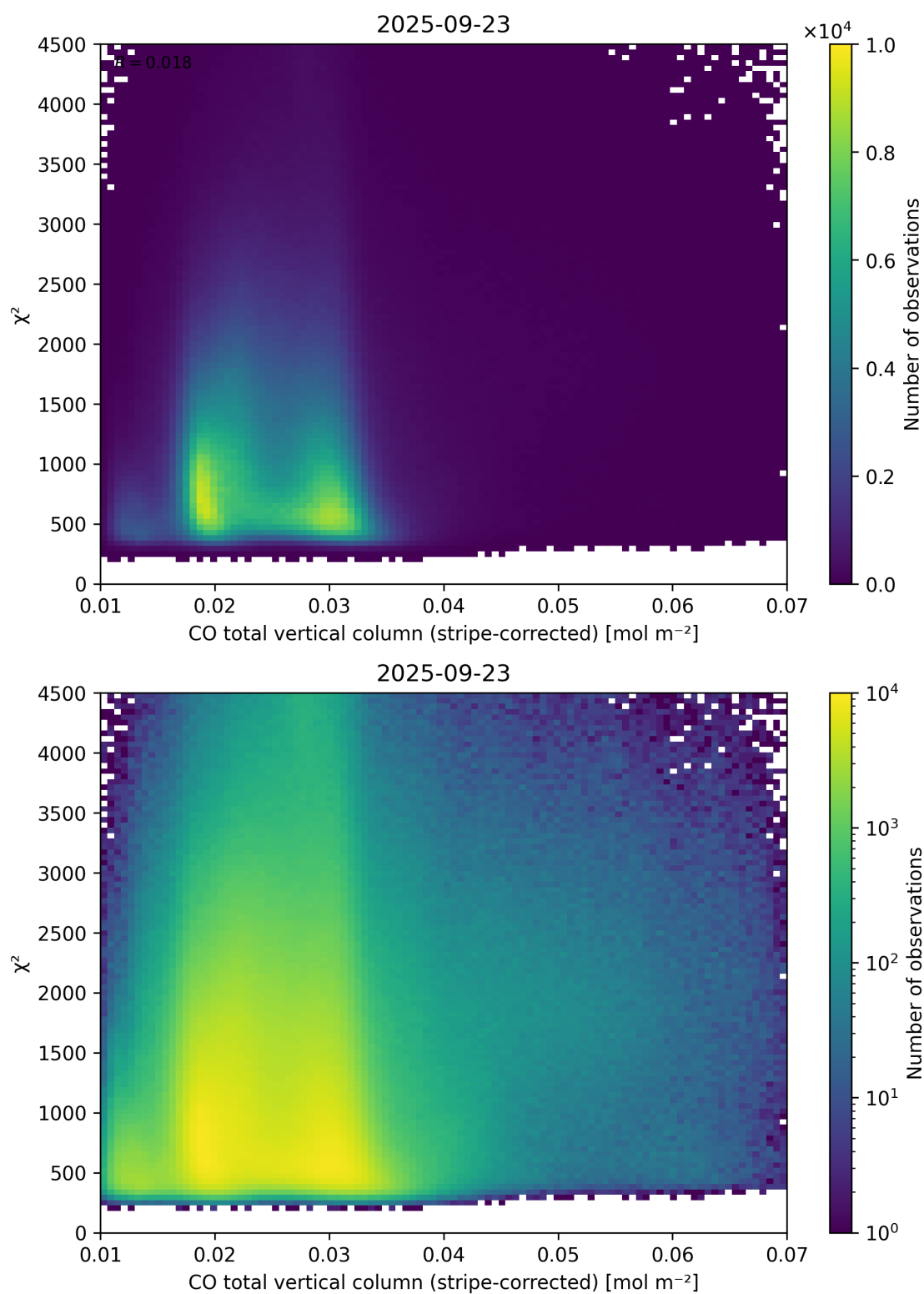
Figure 37: Scatter density plot of “CO total vertical column (stripe-corrected)” against “ \chi^2 ” for 2025-09-22 to 2025-09-24.
