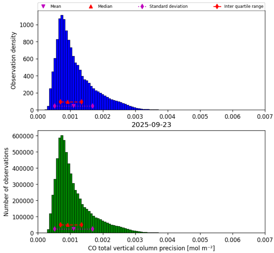
Figure 20: Histogram of “CO total vertical column precision” for 2025-09-22 to 2025-09-24
