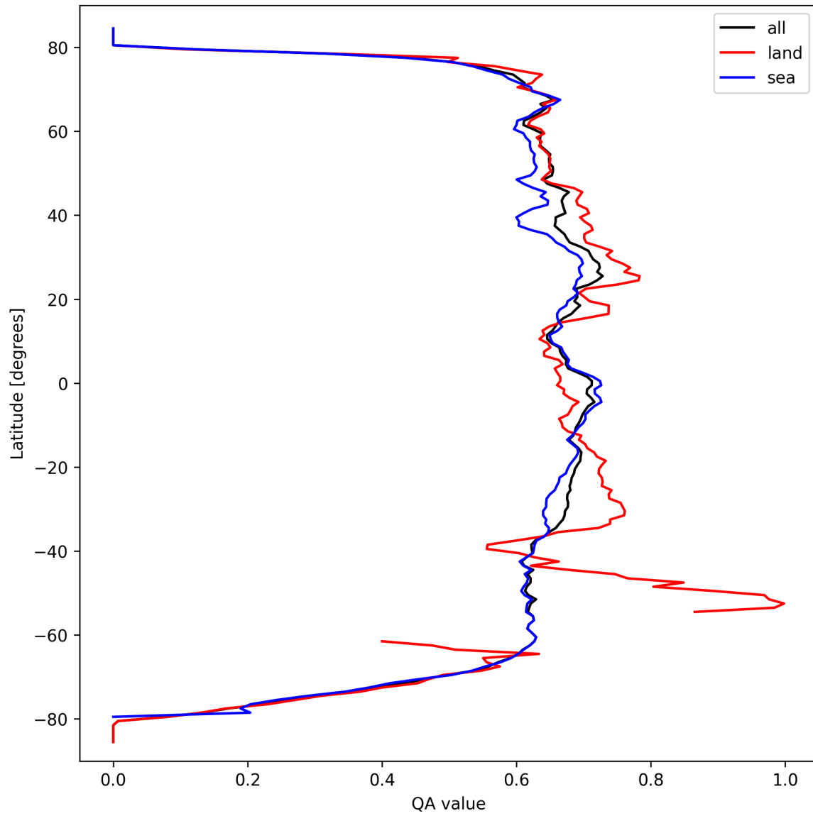
Figure 9: Zonal average of “QA value” for 2025-09-22 to 2025-09-24.
