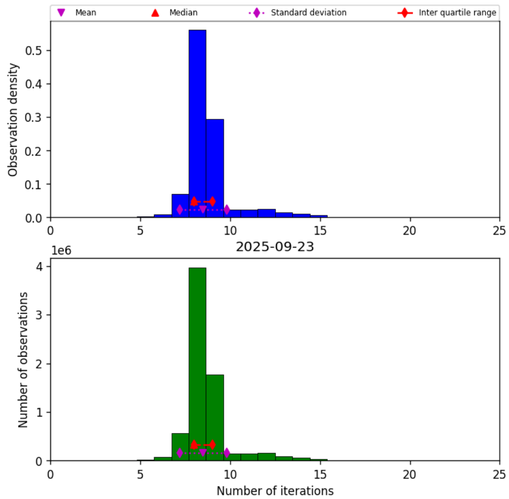
Figure 24: Histogram of “Number of iterations” for 2025-09-22 to 2025-09-24
