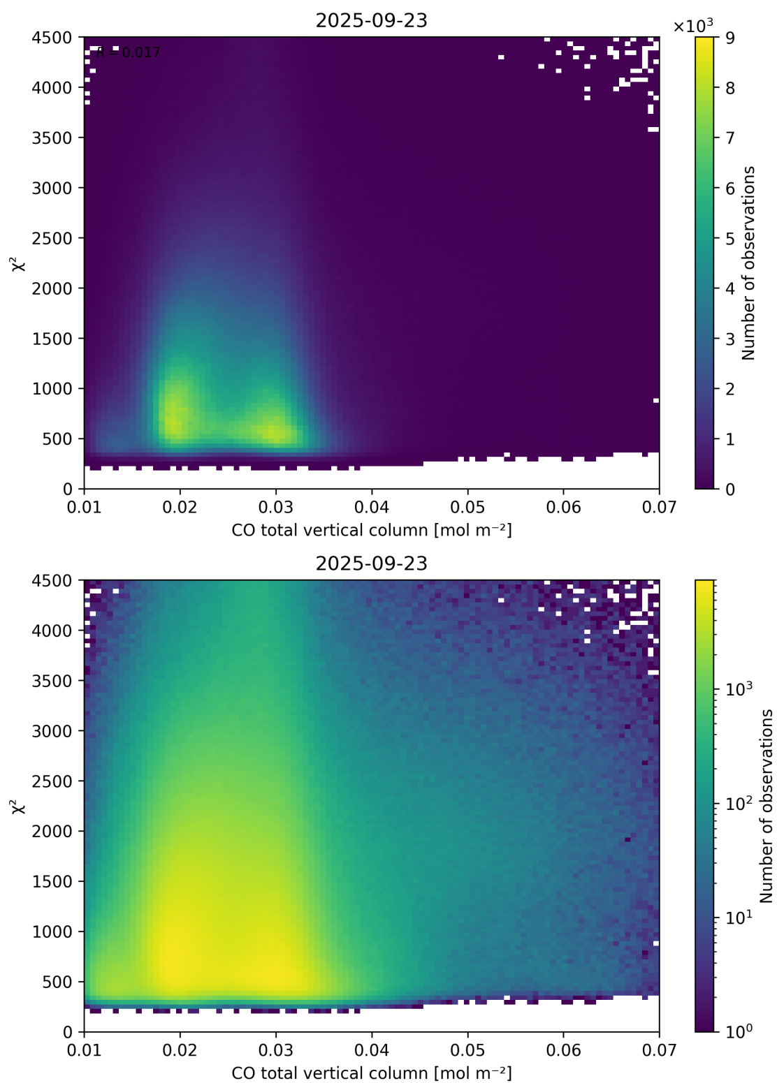
Figure 35: Scatter density plot of “CO total vertical column” against “ \chi^2 ” for 2025-09-22 to 2025-09-24.
