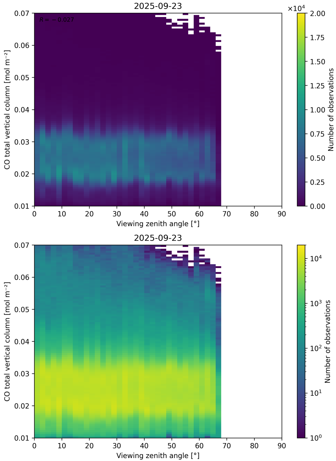
Figure 69: Scatter density plot of “Viewing zenith angle” against “CO total vertical column” for 2025-09-22 to 2025-09-24.
