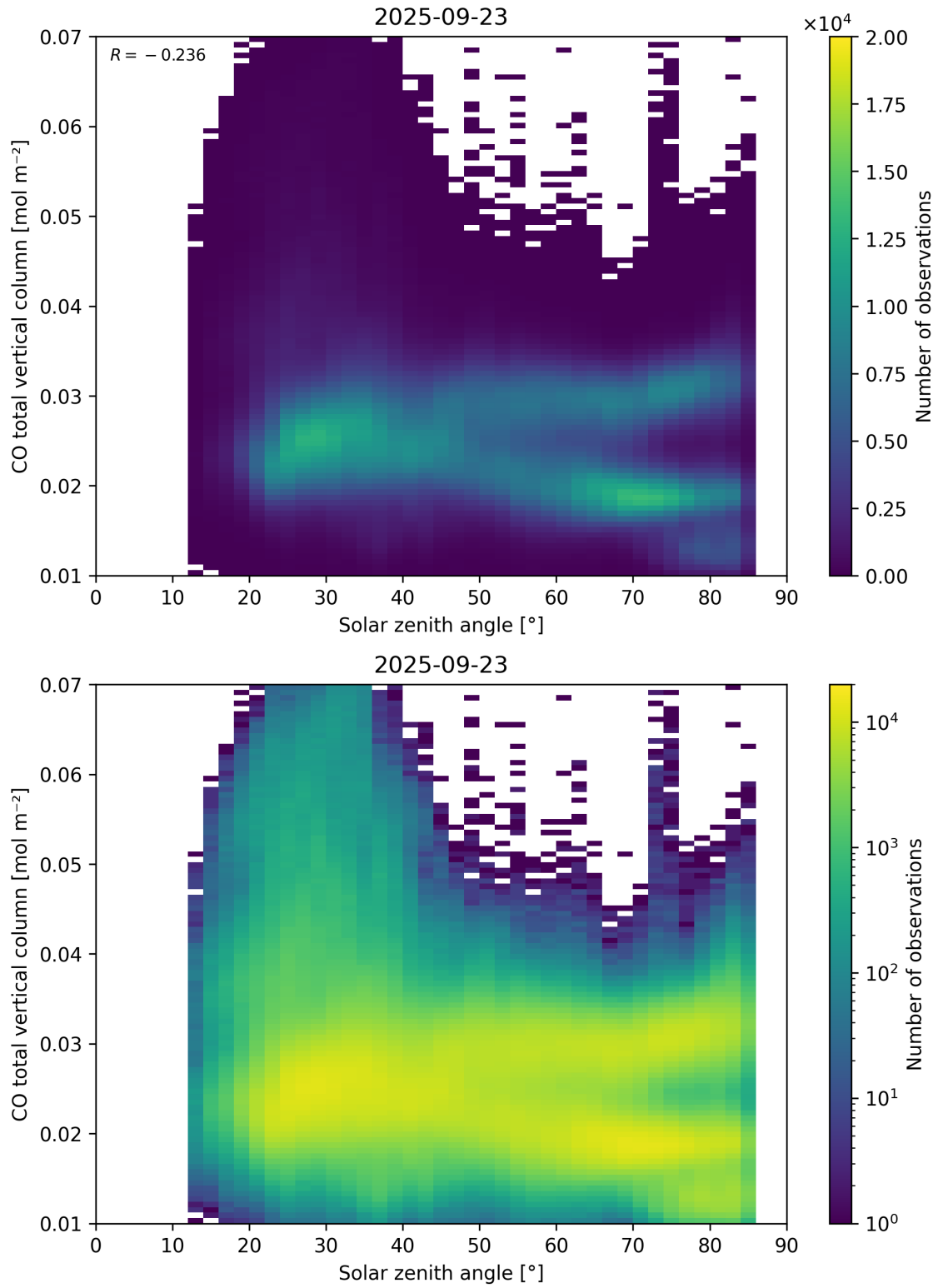
Figure 61: Scatter density plot of “Solar zenith angle” against “CO total vertical column” for 2025-09-22 to 2025-09-24.
