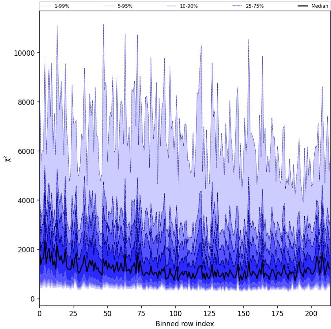
Figure 30: Along track statistics of “ \chi^2 ” for 2025-09-22 to 2025-09-24
