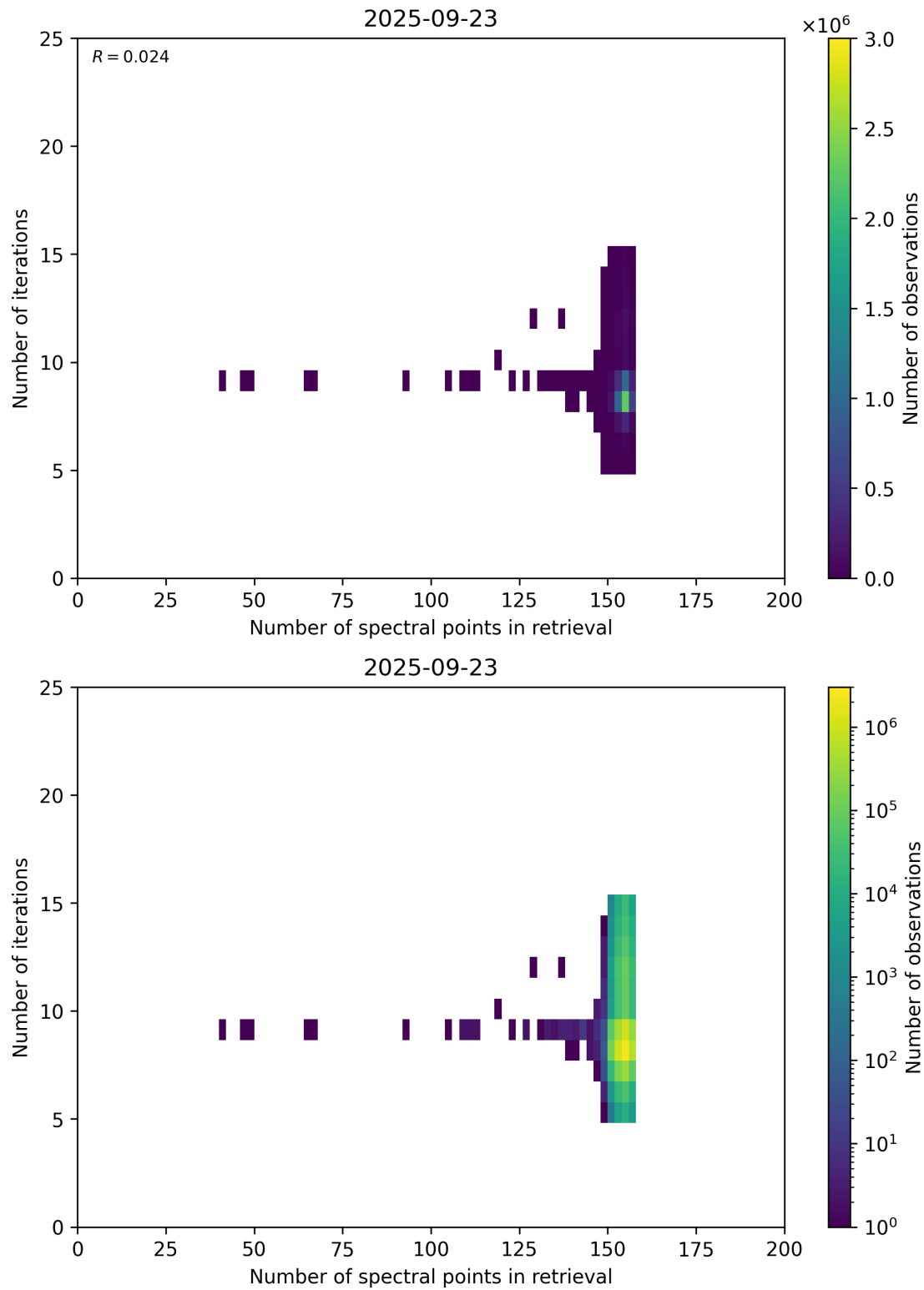
Figure 60: Scatter density plot of “Number of spectral points in retrieval” against “Number of iterations” for 2025-09-22 to 2025-09-24.
