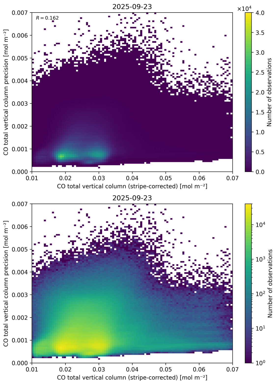
Figure 36: Scatter density plot of “CO total vertical column (stripe-corrected)” against “CO total vertical column precision” for 2025-09-22 to 2025-09-24.
