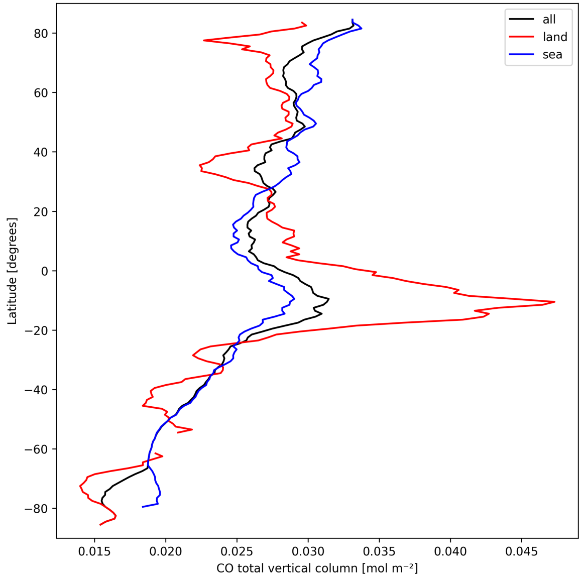
Figure 10: Zonal average of “CO total vertical column” for 2025-09-22 to 2025-09-24.
