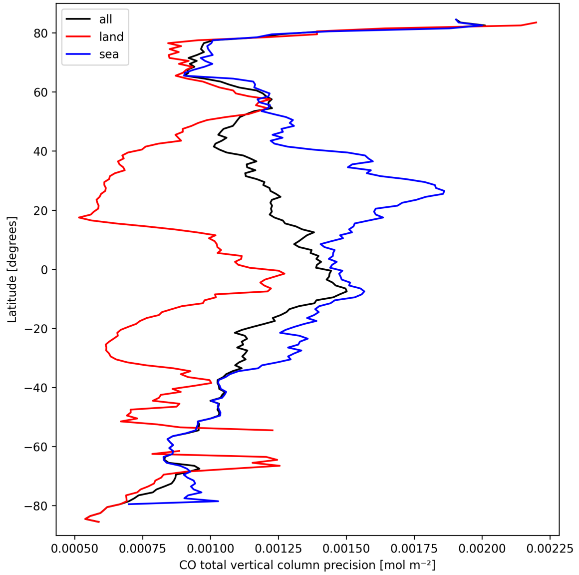
Figure 12: Zonal average of “CO total vertical column precision” for 2025-09-22 to 2025-09-24.
