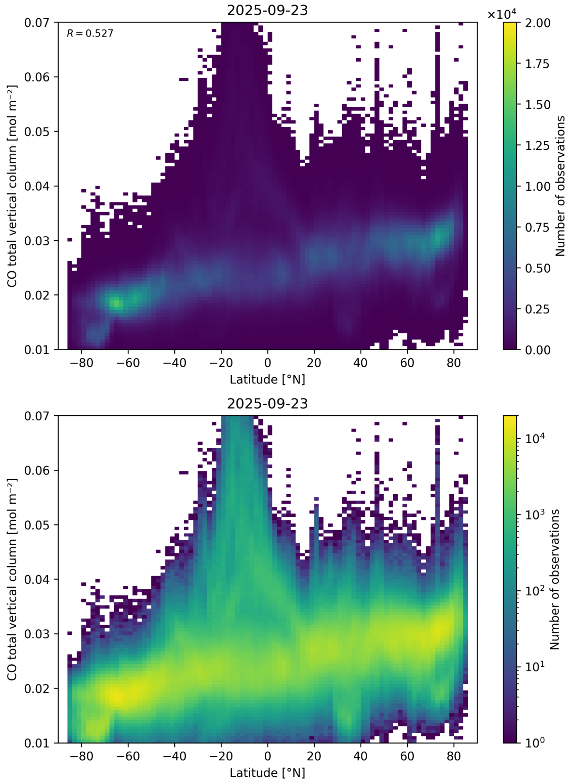
Figure 51: Scatter density plot of “Latitude” against “CO total vertical column” for 2025-09-22 to 2025-09-24.
