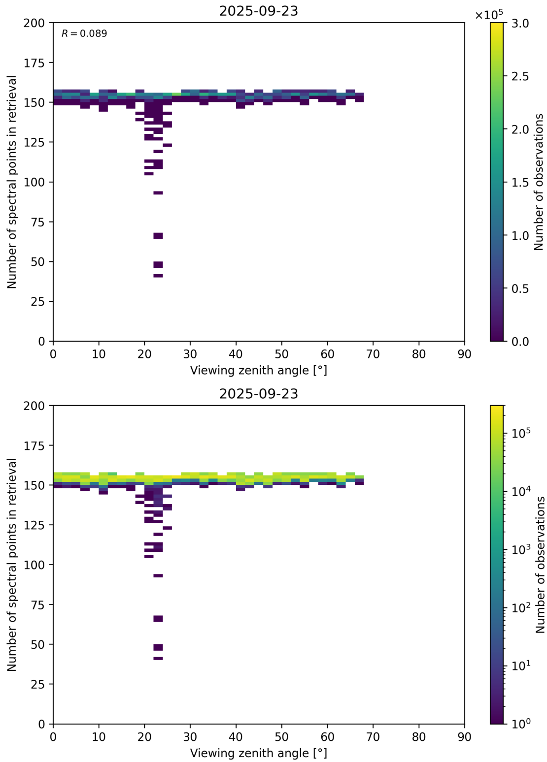
Figure 76: Scatter density plot of “Viewing zenith angle” against “Number of spectral points in retrieval” for 2025-09-22 to 2025-09-24.
