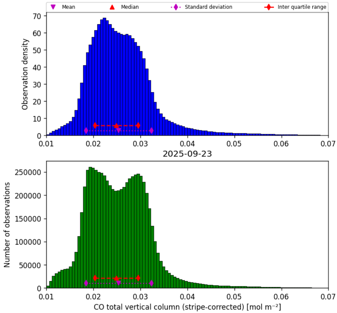
Figure 19: Histogram of “CO total vertical column (stripe-corrected)” for 2025-09-22 to 2025-09-24
