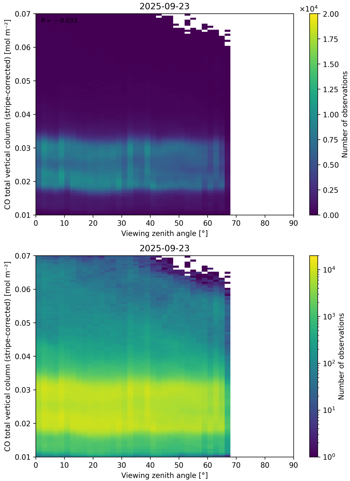
Figure 70: Scatter density plot of “Viewing zenith angle” against “CO total vertical column (stripe-corrected)” for 2025-09-22 to 2025-09-24.
