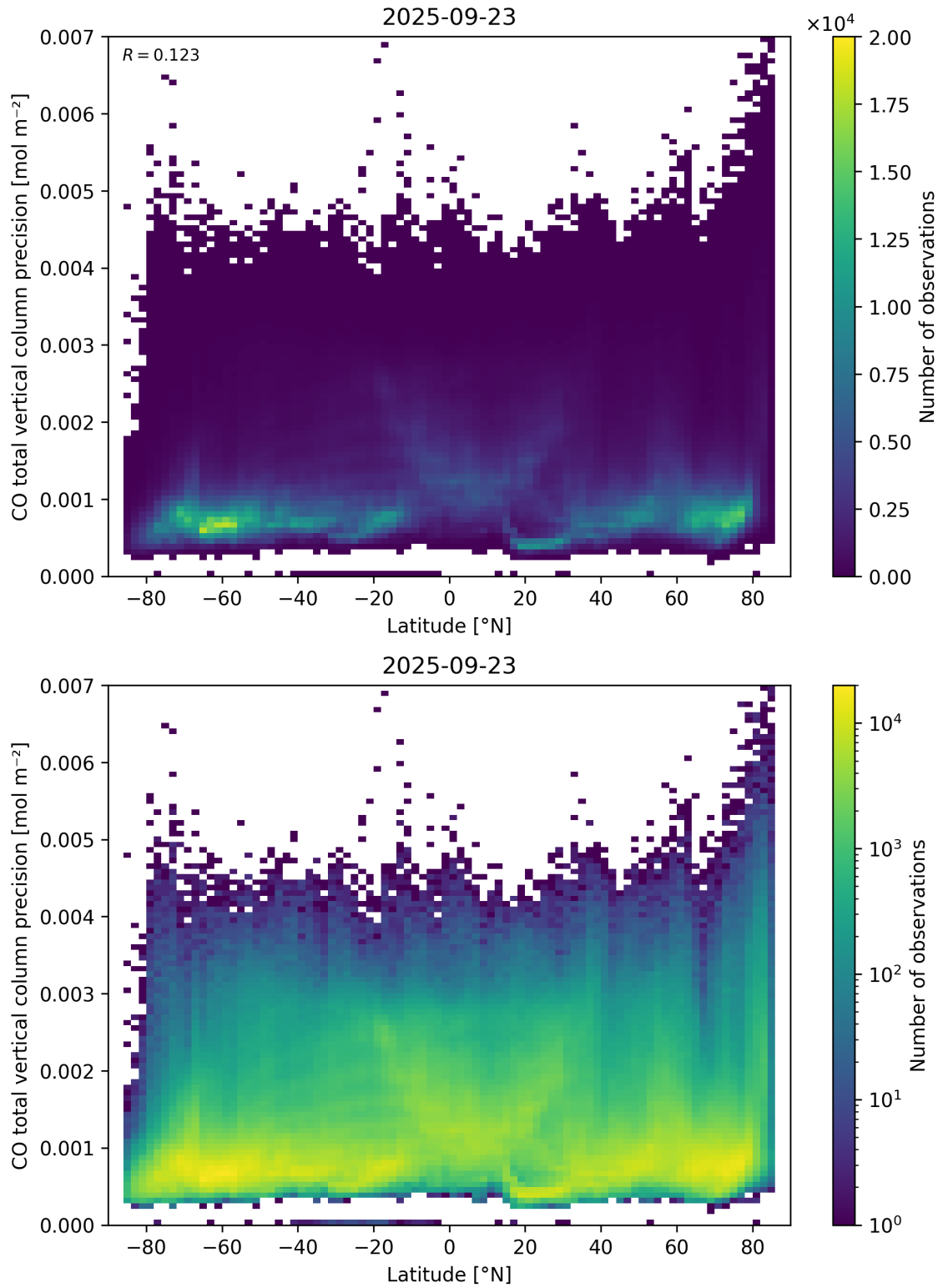
Figure 53: Scatter density plot of “Latitude” against “CO total vertical column precision” for 2025-09-22 to 2025-09-24.
