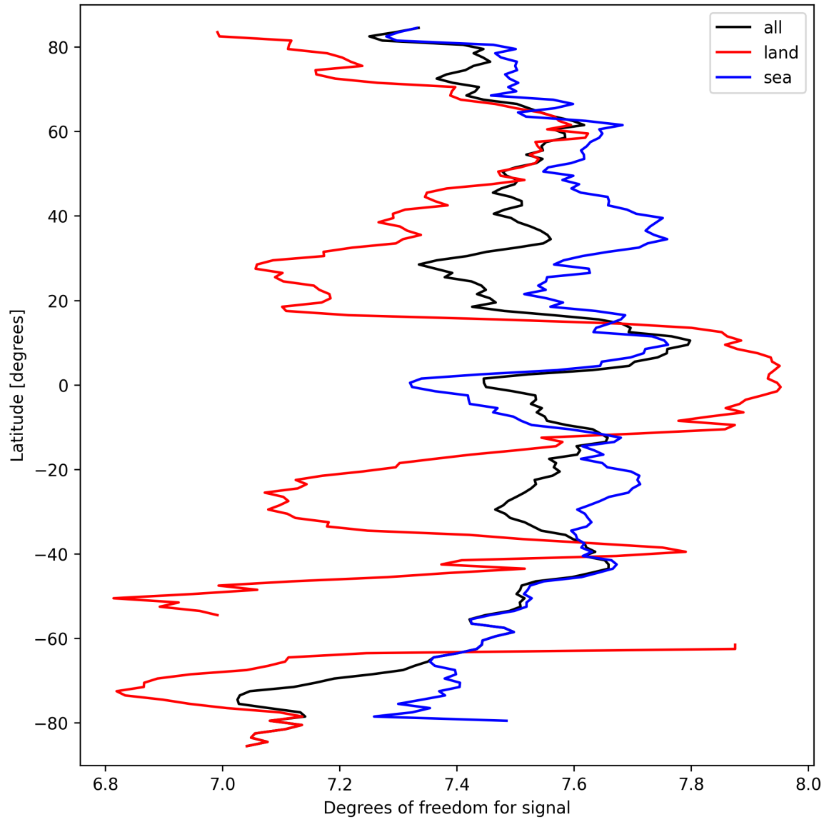
Figure 15: Zonal average of “Degrees of freedom for signal” for 2025-09-22 to 2025-09-24.
