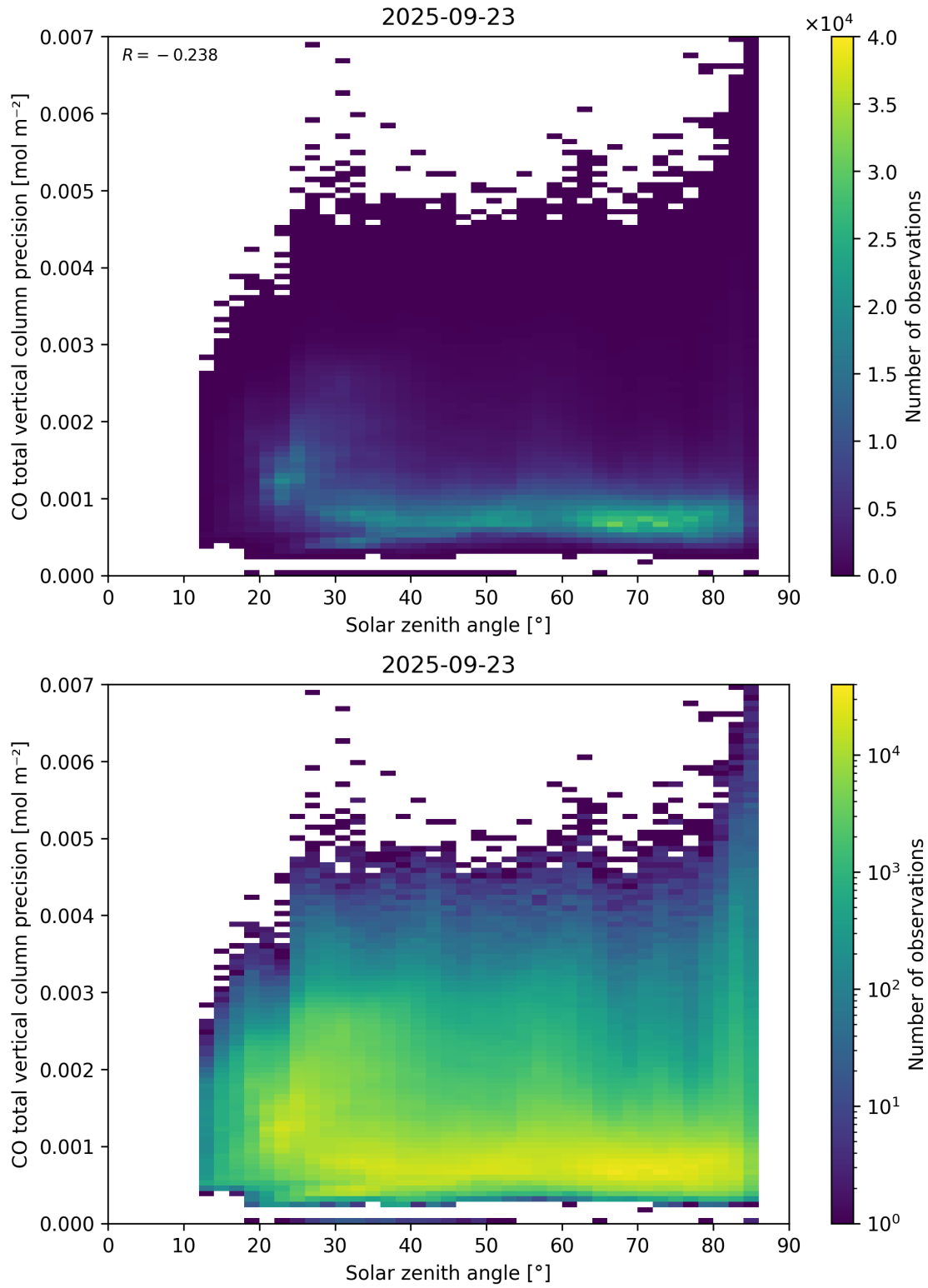
Figure 63: Scatter density plot of “Solar zenith angle” against “CO total vertical column precision” for 2025-09-22 to 2025-09-24.
