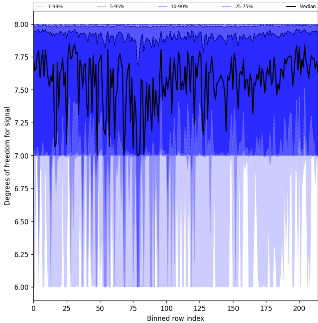
Figure 31: Along track statistics of “Degrees of freedom for signal” for 2025-09-22 to 2025-09-24
