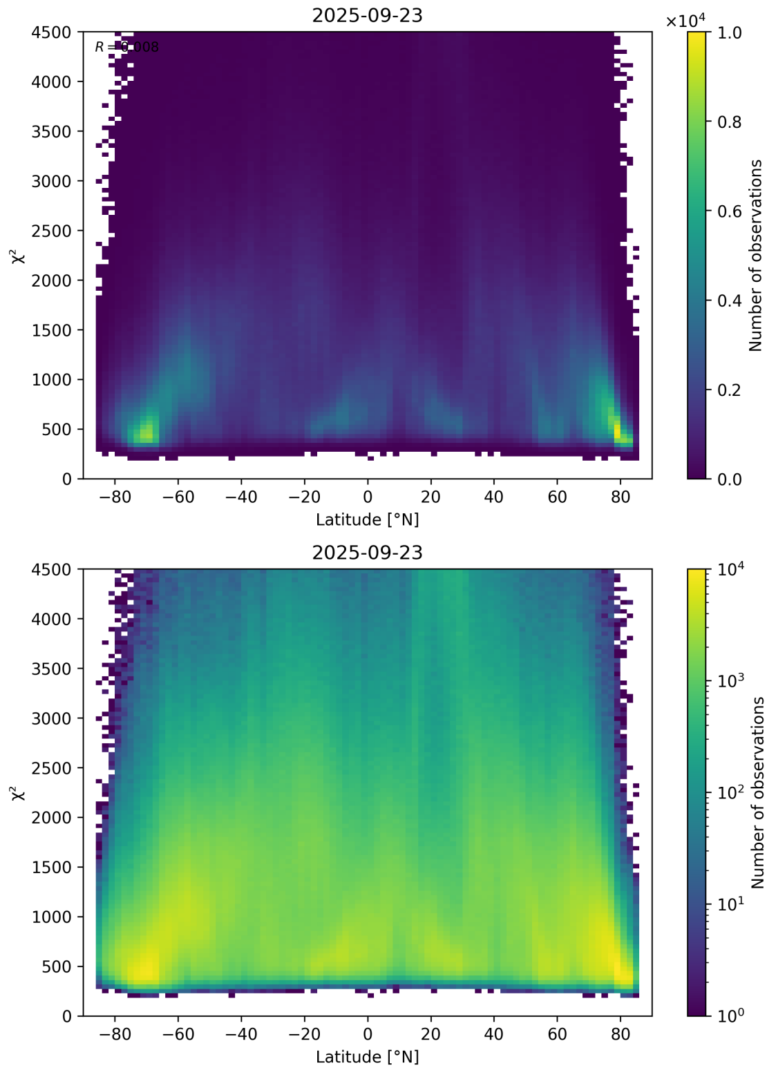
Figure 54: Scatter density plot of “Latitude” against “ \chi^2 ” for 2025-09-22 to 2025-09-24.
