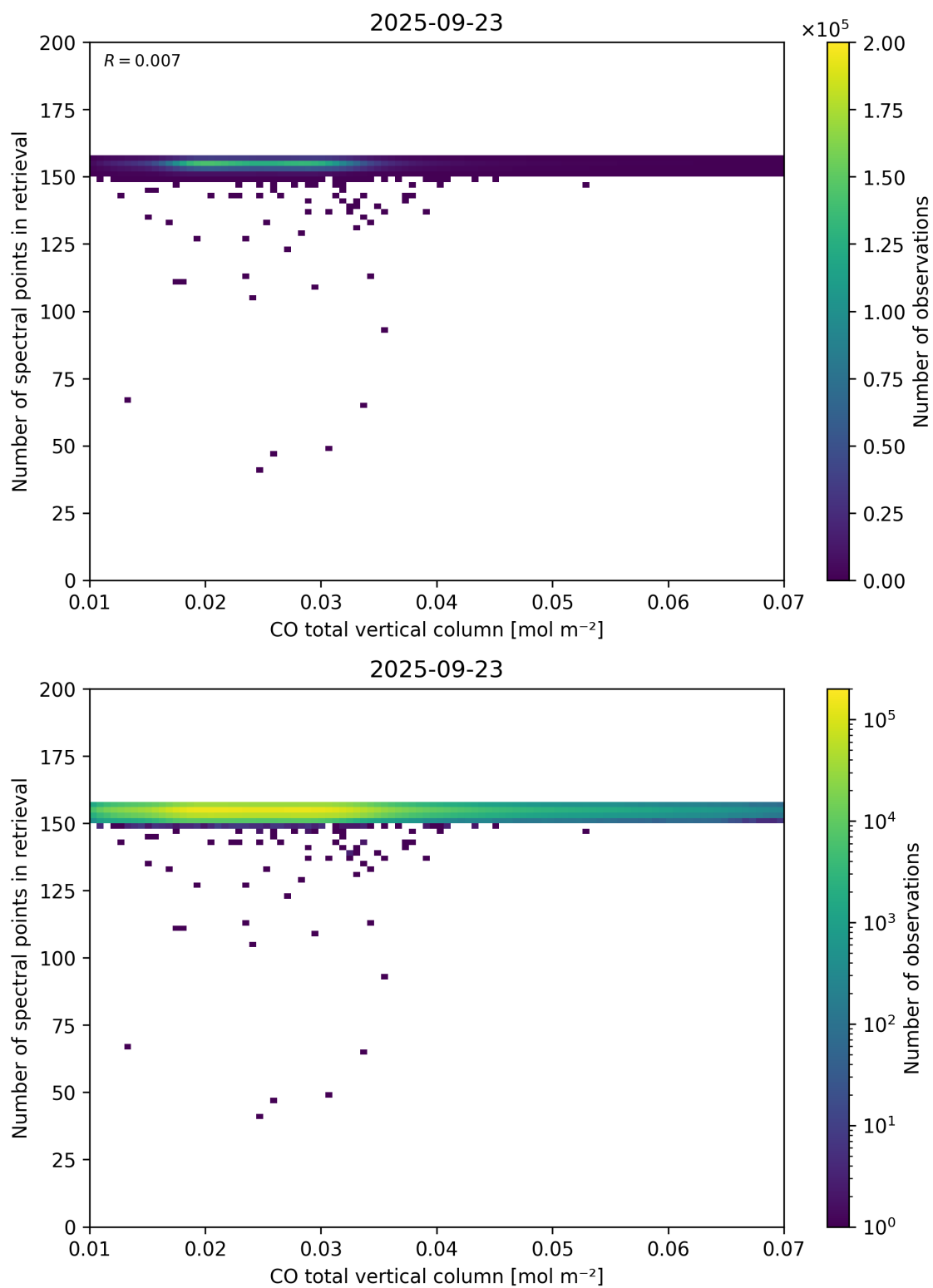
Figure 43: Scatter density plot of “CO total vertical column” against “Number of spectral points in retrieval” for 2025-09-22 to 2025-09-24.
