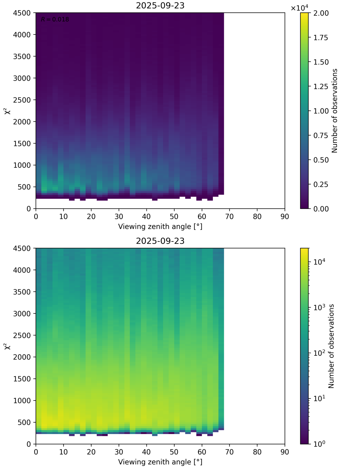
Figure 72: Scatter density plot of “Viewing zenith angle” against “ \chi^2 ” for 2025-09-22 to 2025-09-24.
