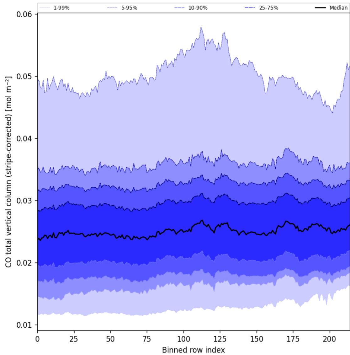
Figure 27: Along track statistics of “CO total vertical column (stripe-corrected)” for 2025-09-22 to 2025-09-24
