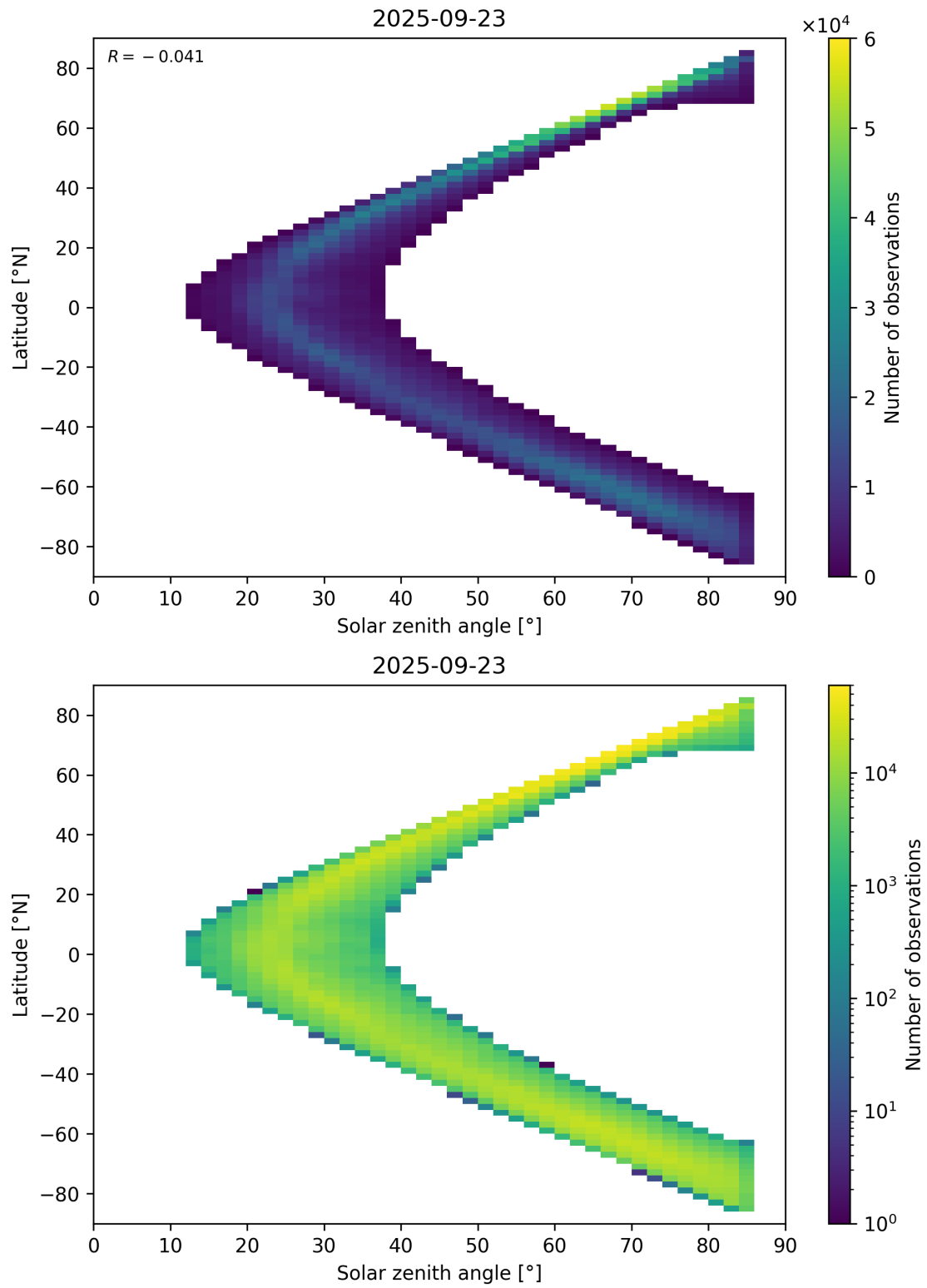
Figure 66: Scatter density plot of “Solar zenith angle” against “Latitude” for 2025-09-22 to 2025-09-24.
