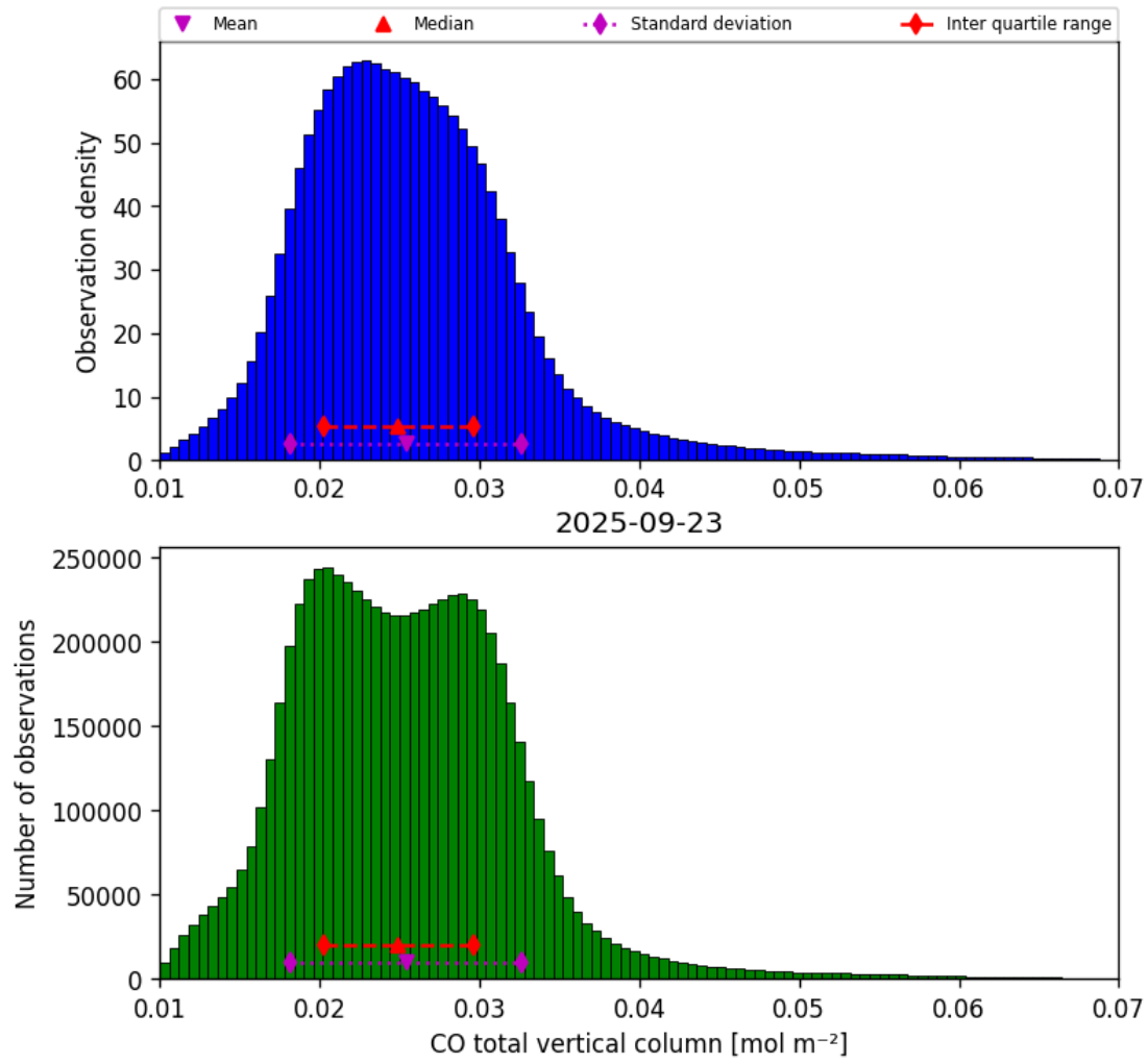
Figure 18: Histogram of “CO total vertical column” for 2025-09-22 to 2025-09-24
