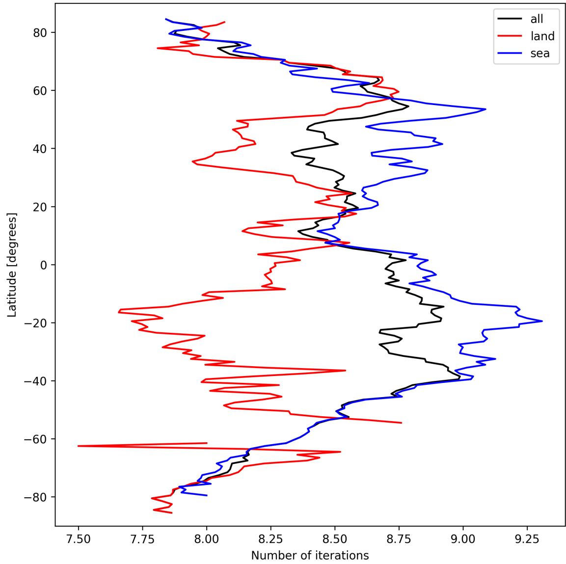
Figure 16: Zonal average of “Number of iterations” for 2025-09-22 to 2025-09-24.
