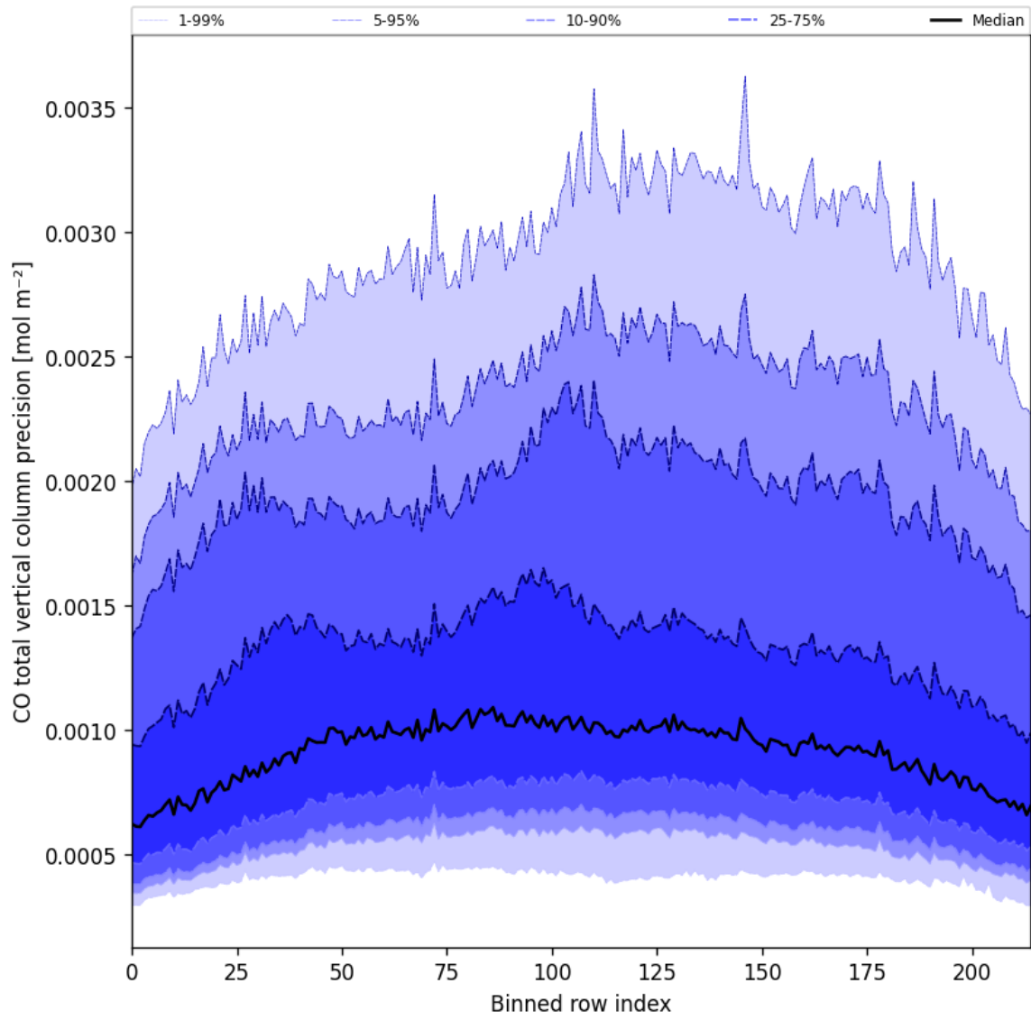
Figure 28: Along track statistics of “CO total vertical column precision” for 2025-09-22 to 2025-09-24
