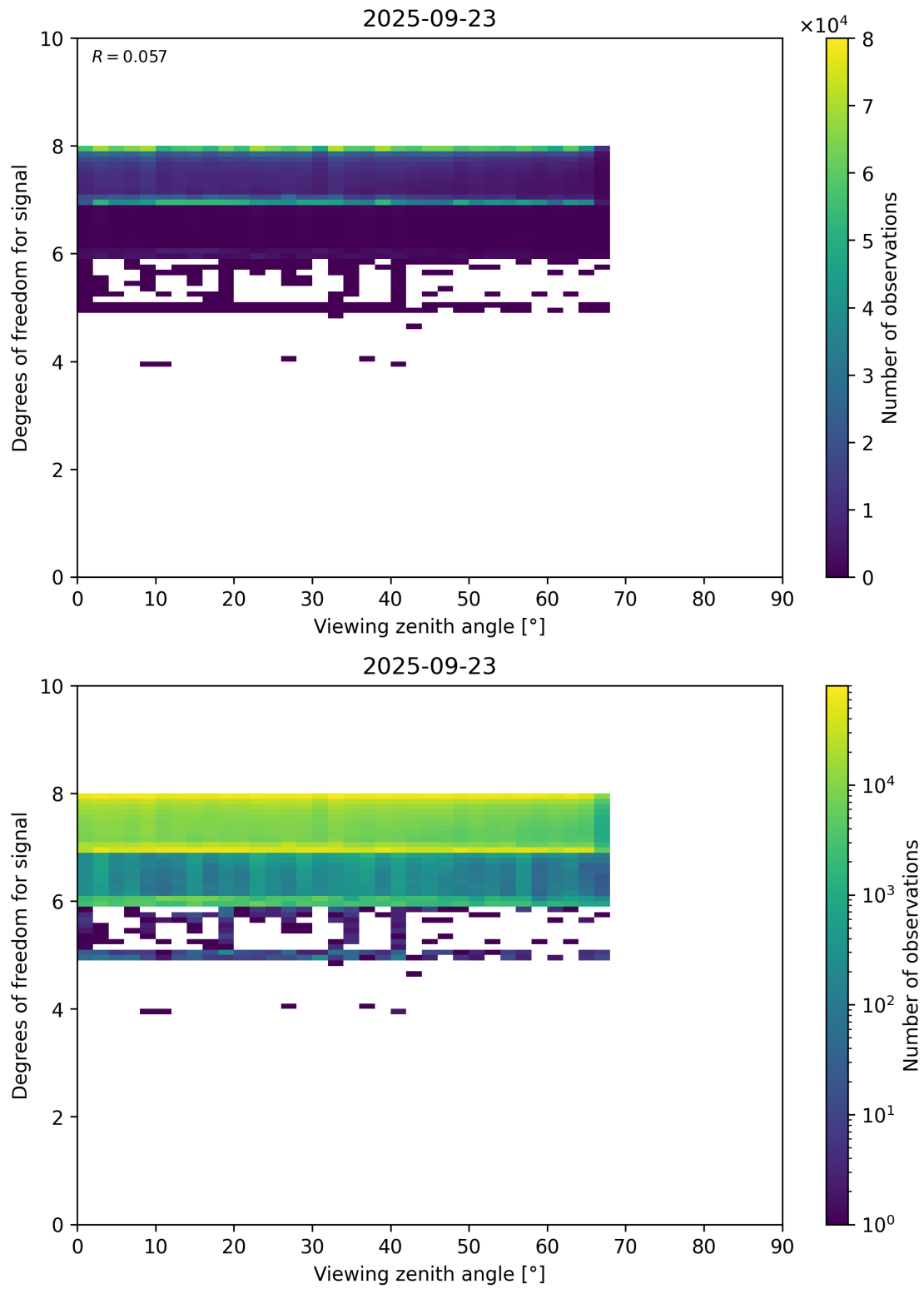
Figure 73: Scatter density plot of “Viewing zenith angle” against “Degrees of freedom for signal” for 2025-09-22 to 2025-09-24.
