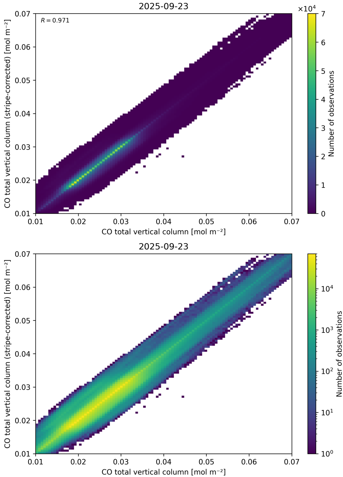
Figure 33: Scatter density plot of “CO total vertical column” against “CO total vertical column (stripe-corrected)” for 2025-09-22 to 2025-09-24.
