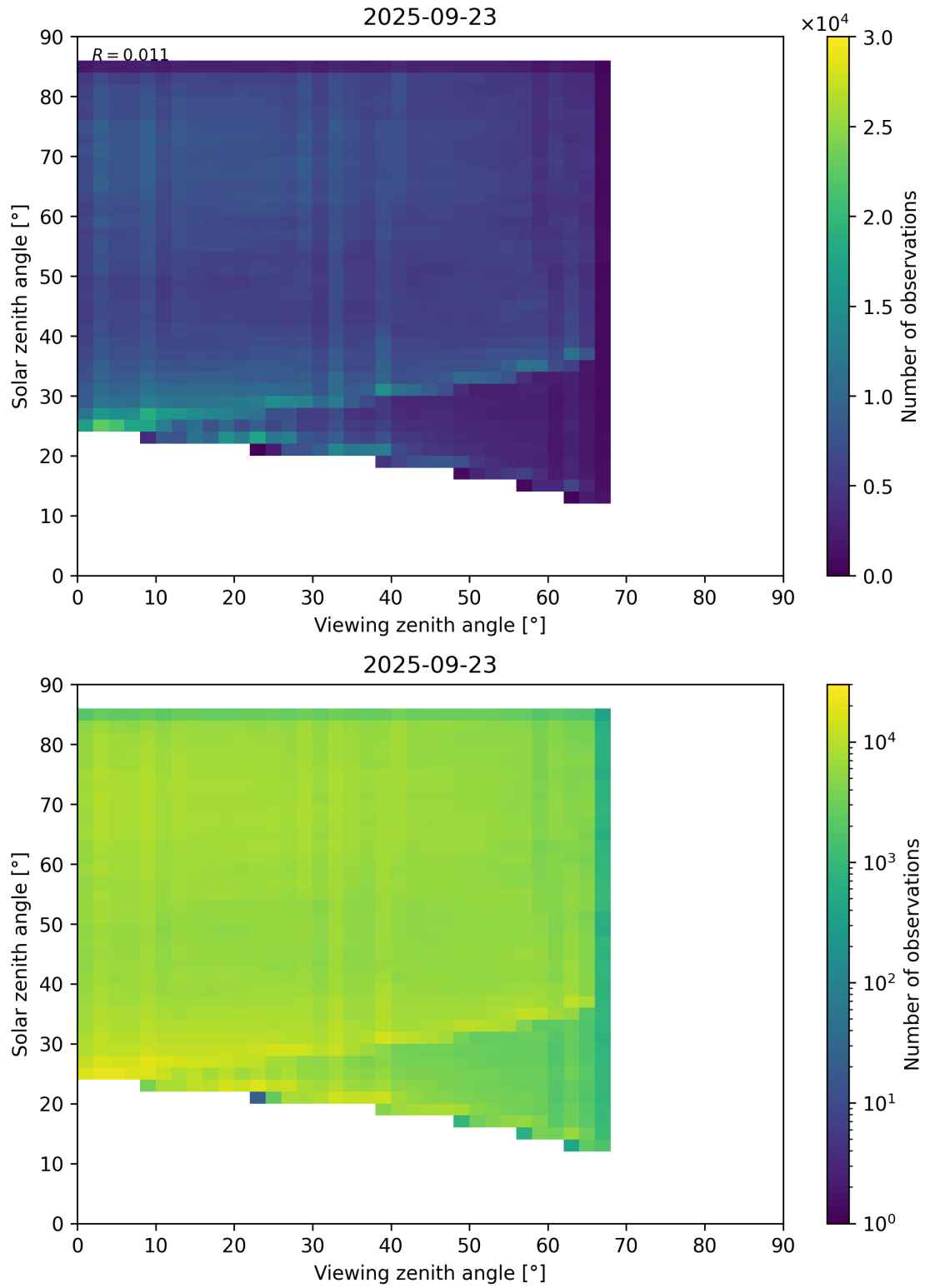
Figure 77: Scatter density plot of “Viewing zenith angle” against “Solar zenith angle” for 2025-09-22 to 2025-09-24.
