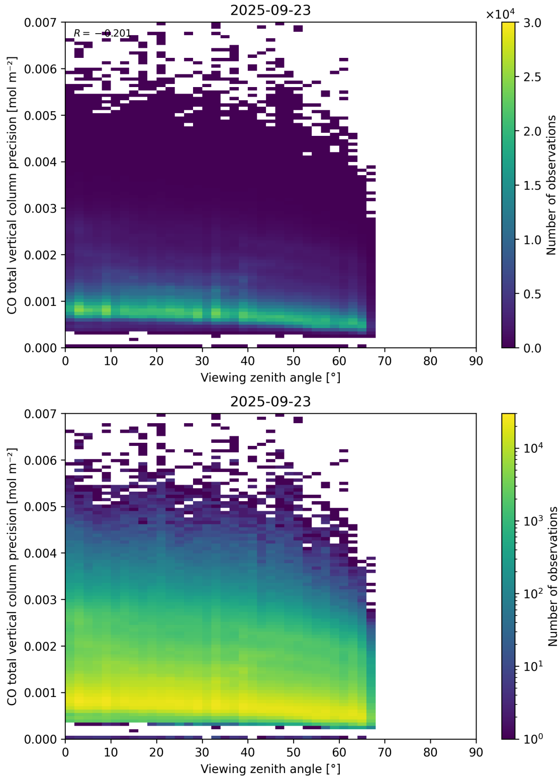
Figure 71: Scatter density plot of “Viewing zenith angle” against “CO total vertical column precision” for 2025-09-22 to 2025-09-24.
