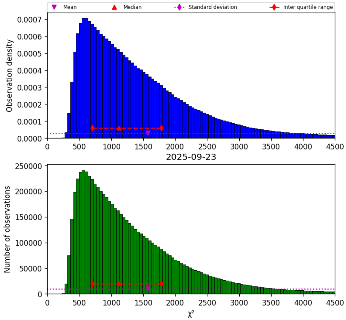
Figure 22: Histogram of “ \chi^2 ” for 2025-09-22 to 2025-09-24
