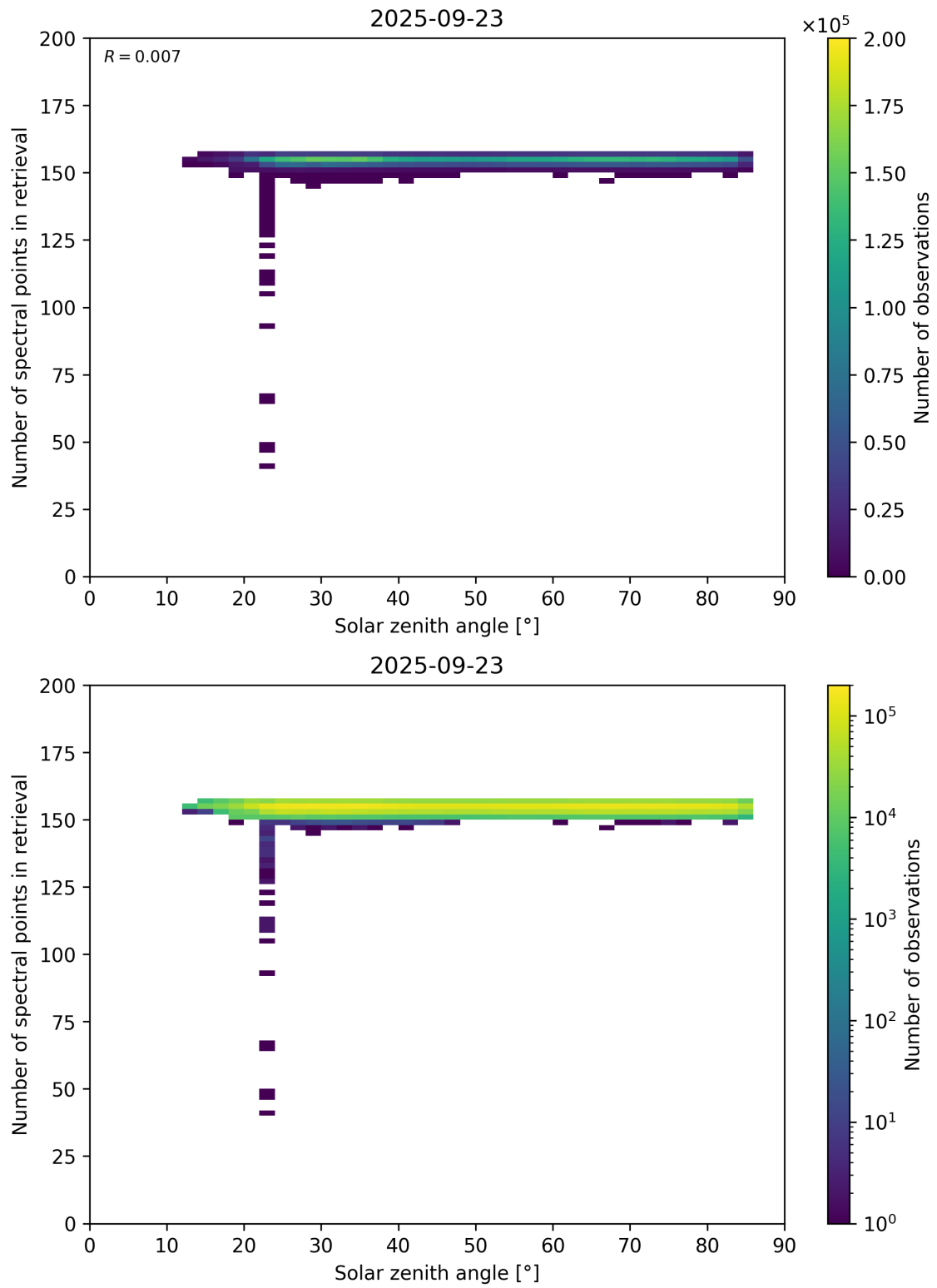
Figure 68: Scatter density plot of “Solar zenith angle” against “Number of spectral points in retrieval” for 2025-09-22 to 2025-09-24.
