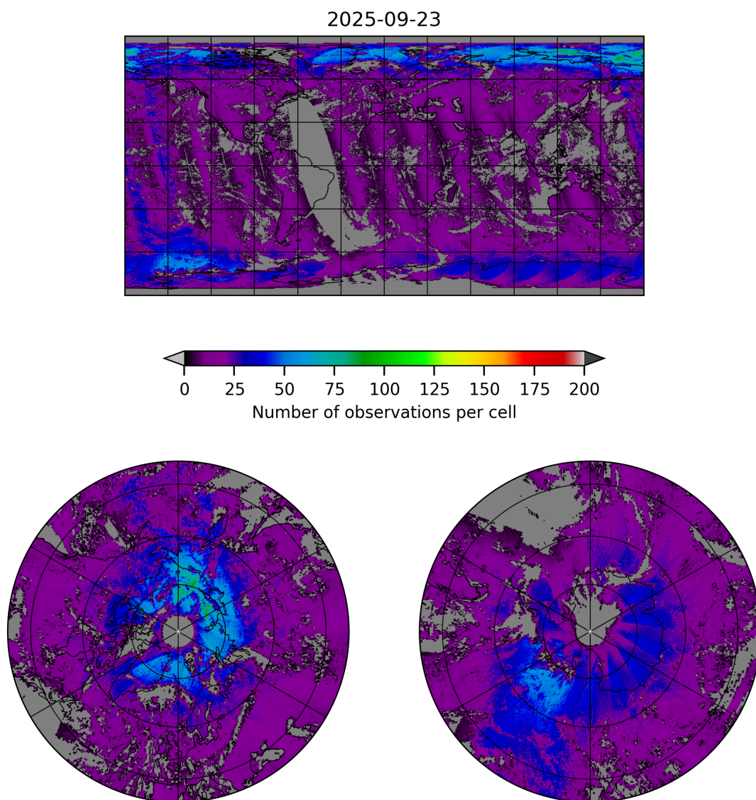
Figure 8: Map of the number of observations for 2025-09-22 to 2025-09-24
