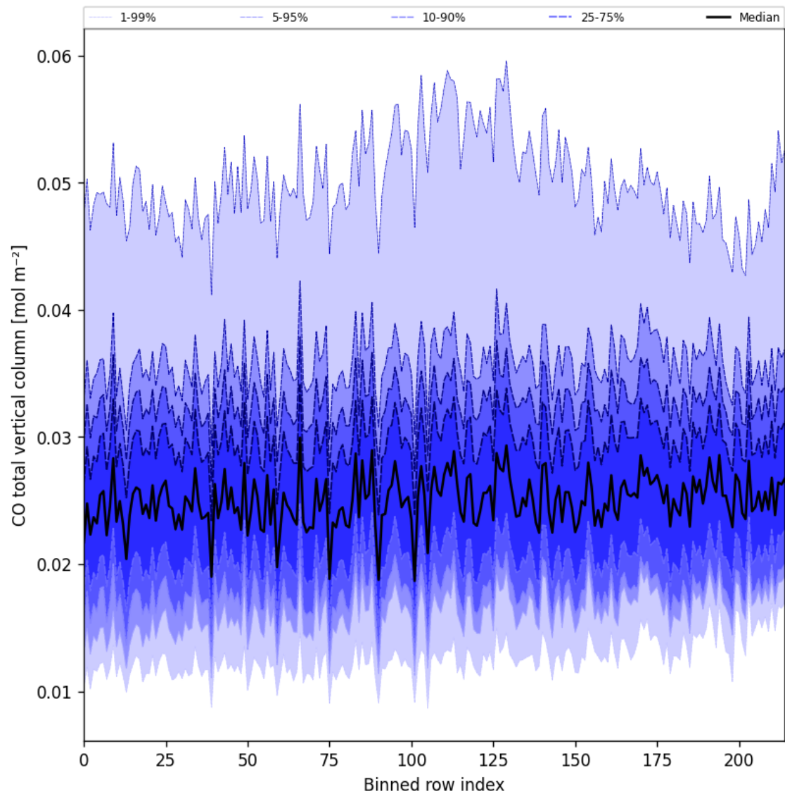
Figure 26: Along track statistics of “CO total vertical column” for 2025-09-22 to 2025-09-24
