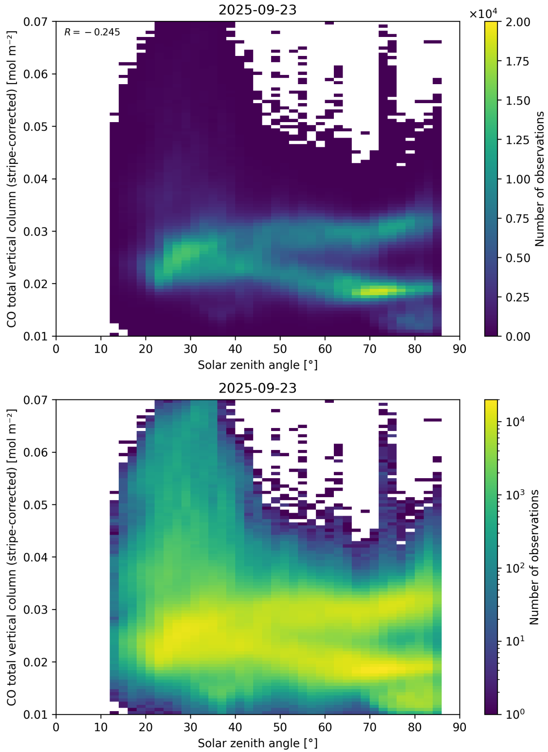
Figure 62: Scatter density plot of “Solar zenith angle” against “CO total vertical column (stripe-corrected)” for 2025-09-22 to 2025-09-24.
