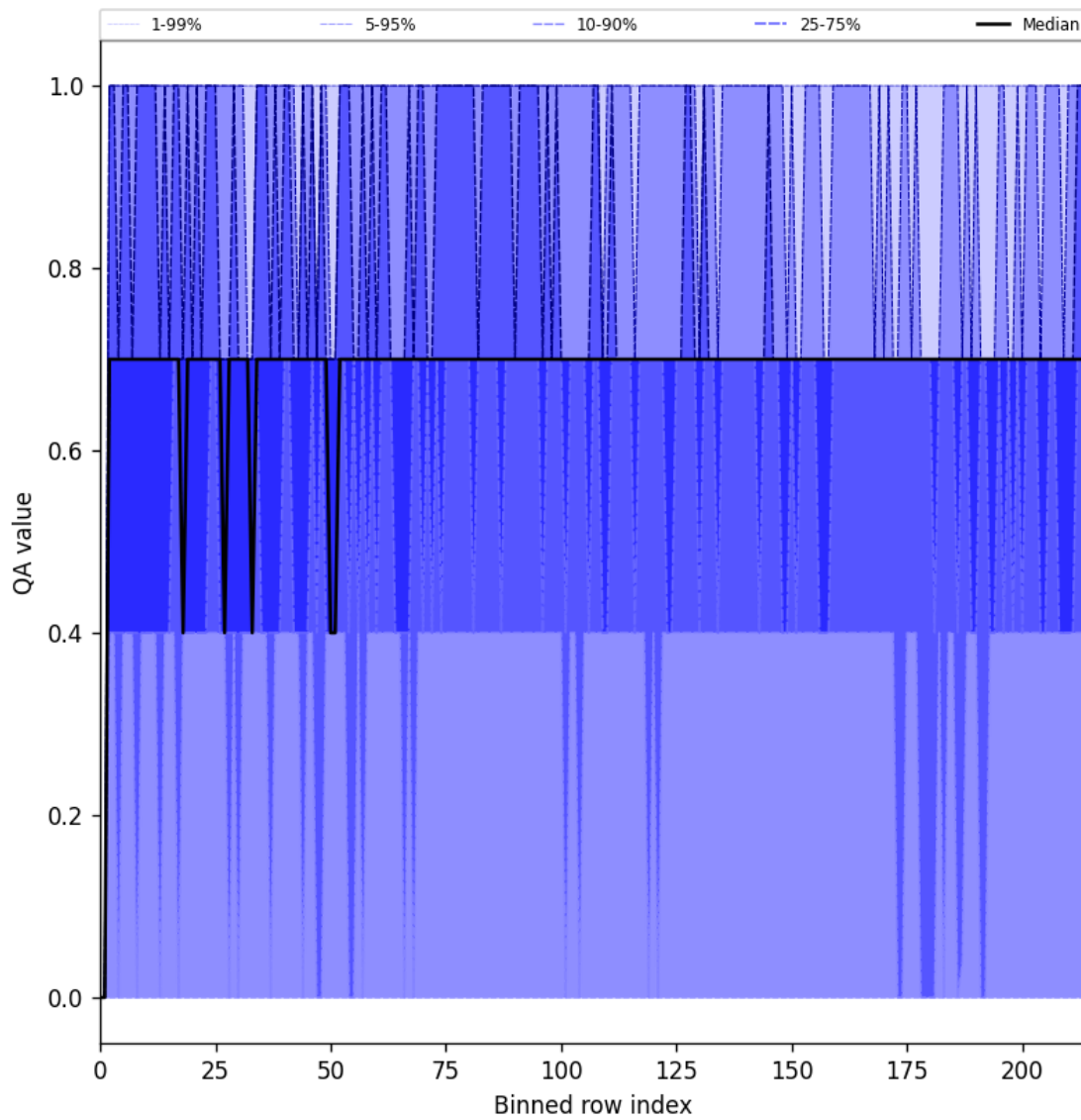
Figure 25: Along track statistics of “QA value” for 2025-09-22 to 2025-09-24
