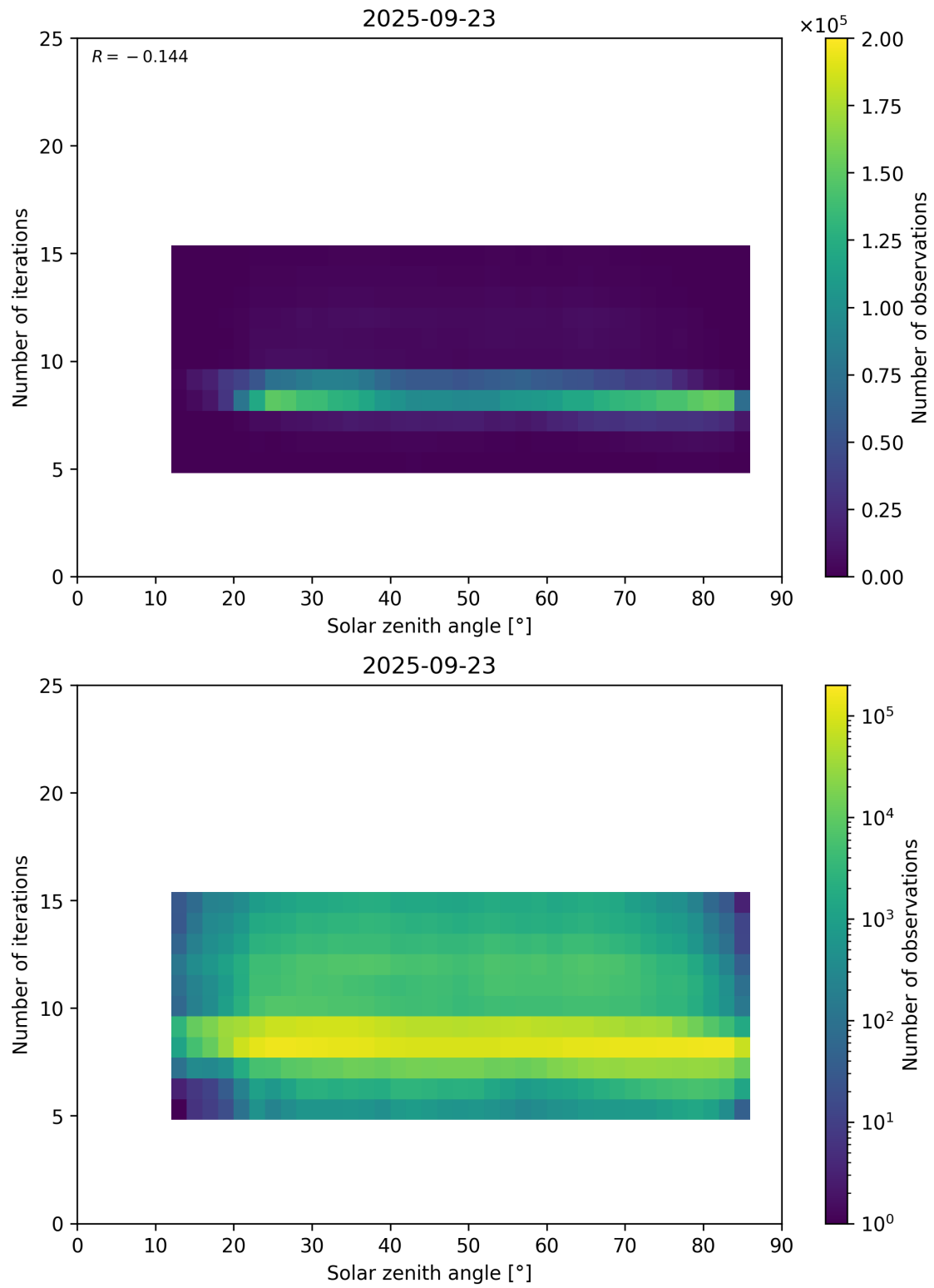
Figure 67: Scatter density plot of “Solar zenith angle” against “Number of iterations” for 2025-09-22 to 2025-09-24.
