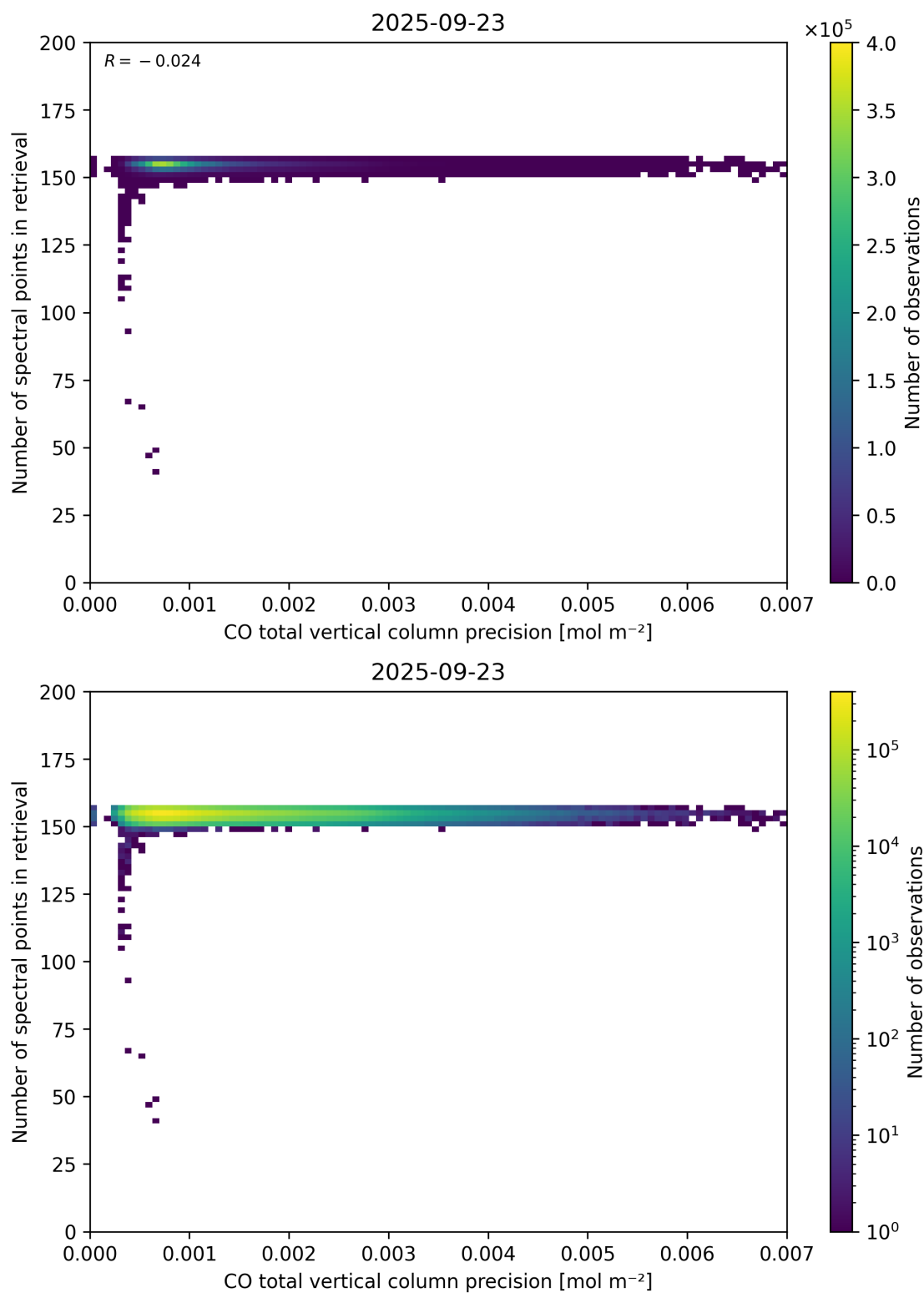
Figure 47: Scatter density plot of “CO total vertical column precision” against “Number of spectral points in retrieval” for 2025-09-22 to 2025-09-24.
