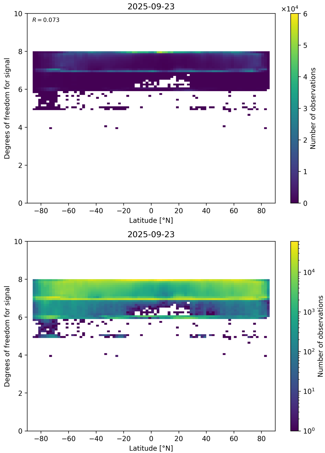
Figure 55: Scatter density plot of “Latitude” against “Degrees of freedom for signal” for 2025-09-22 to 2025-09-24.
