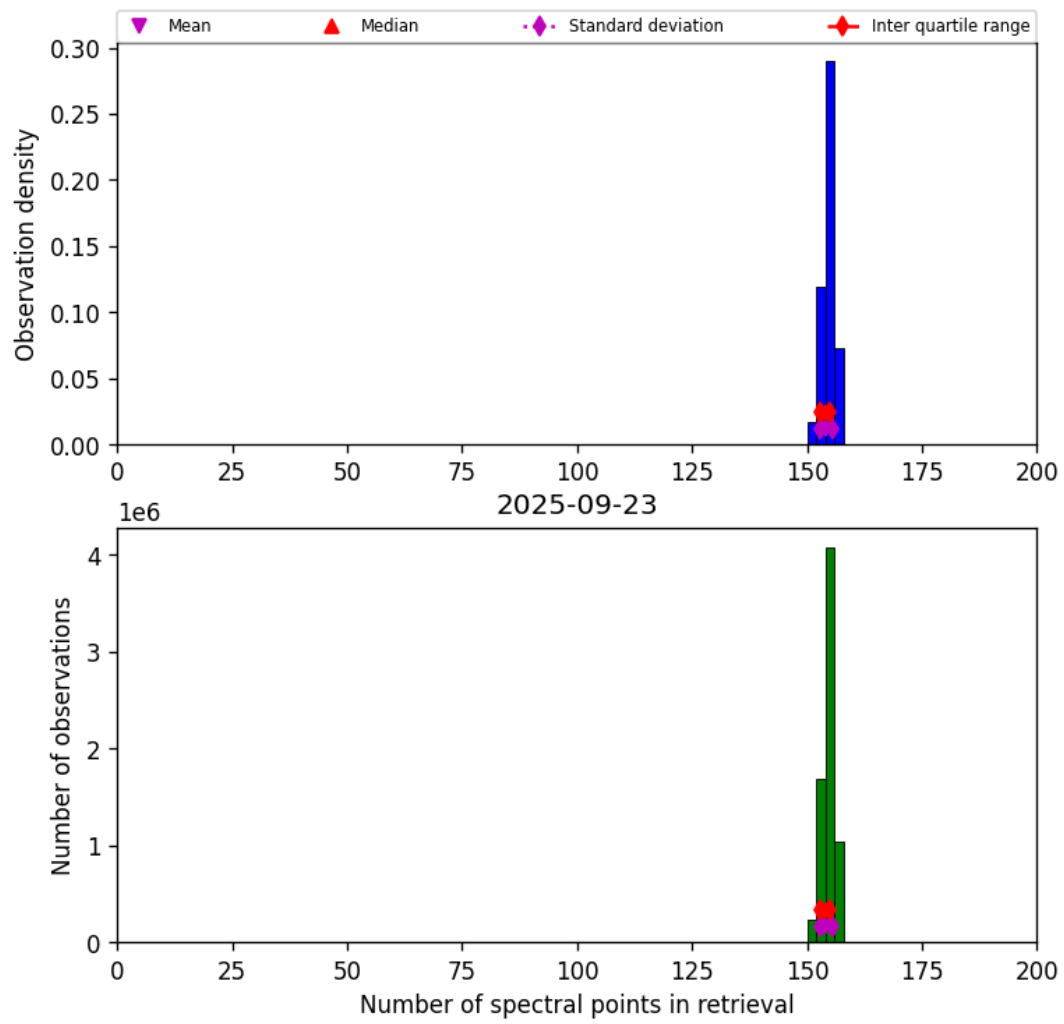
Figure 21: Histogram of “Number of spectral points in retrieval” for 2025-09-22 to 2025-09-24
