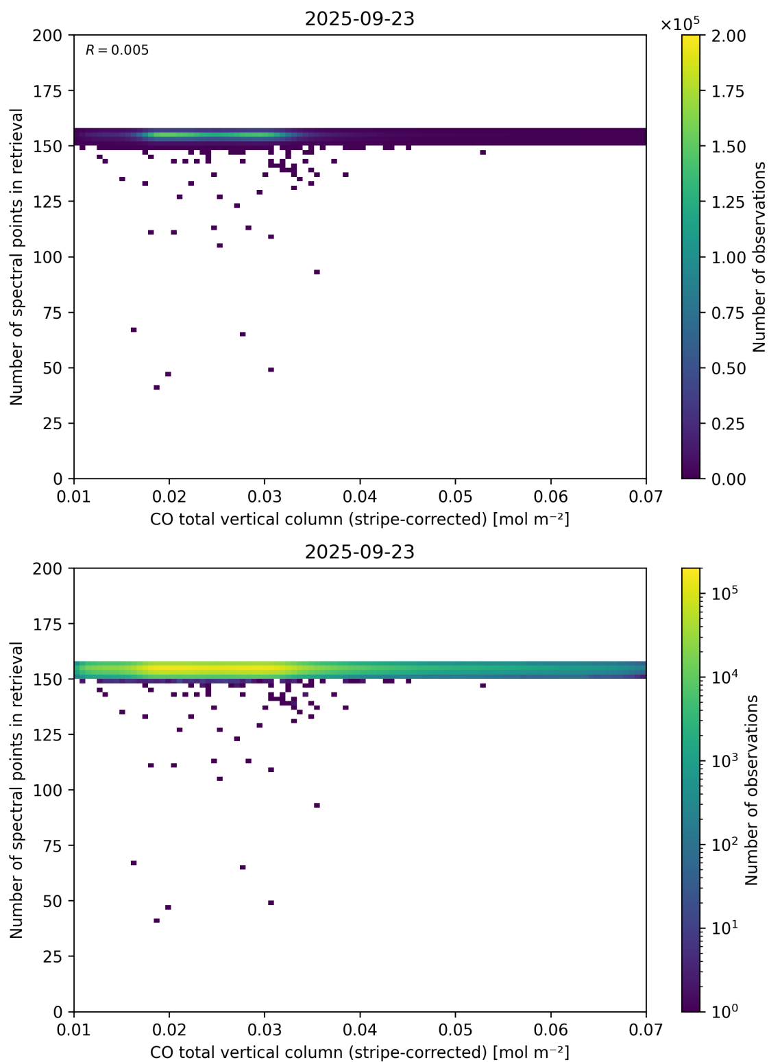
Figure 40: Scatter density plot of “CO total vertical column (stripe-corrected)” against “Number of spectral points in retrieval” for 2025-09-22 to 2025-09-24.
