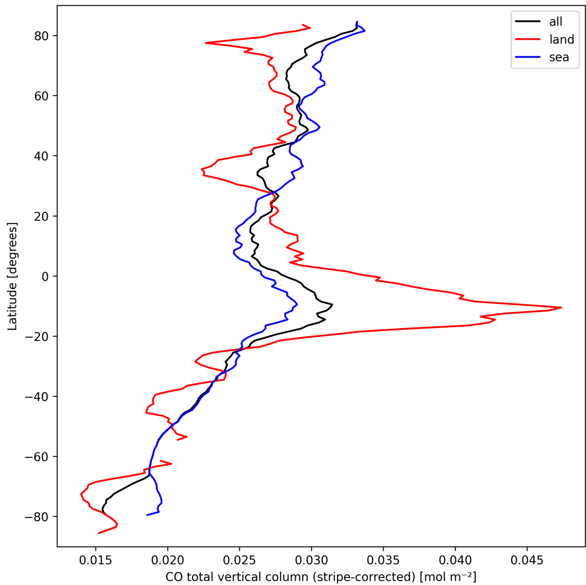
Figure 11: Zonal average of “CO total vertical column (stripe-corrected)” for 2025-09-22 to 2025-09-24.
