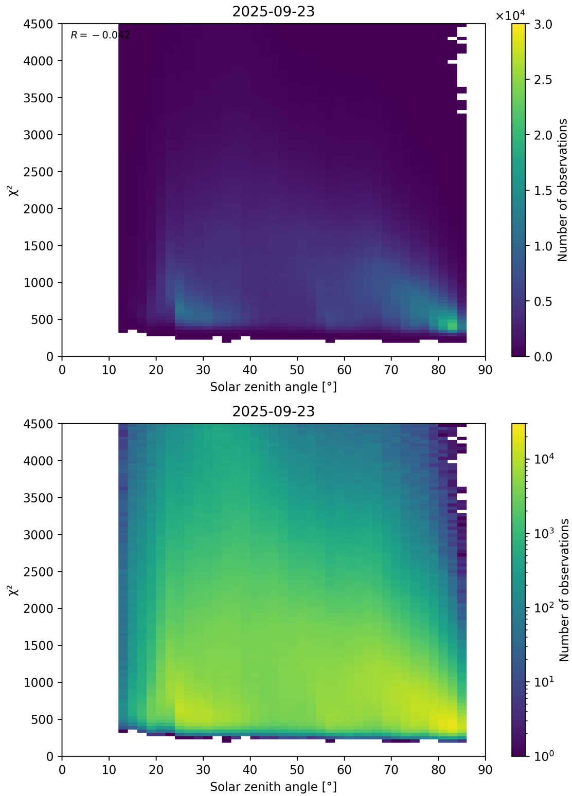
Figure 64: Scatter density plot of “Solar zenith angle” against “ \chi^2 ” for 2025-09-22 to 2025-09-24.
