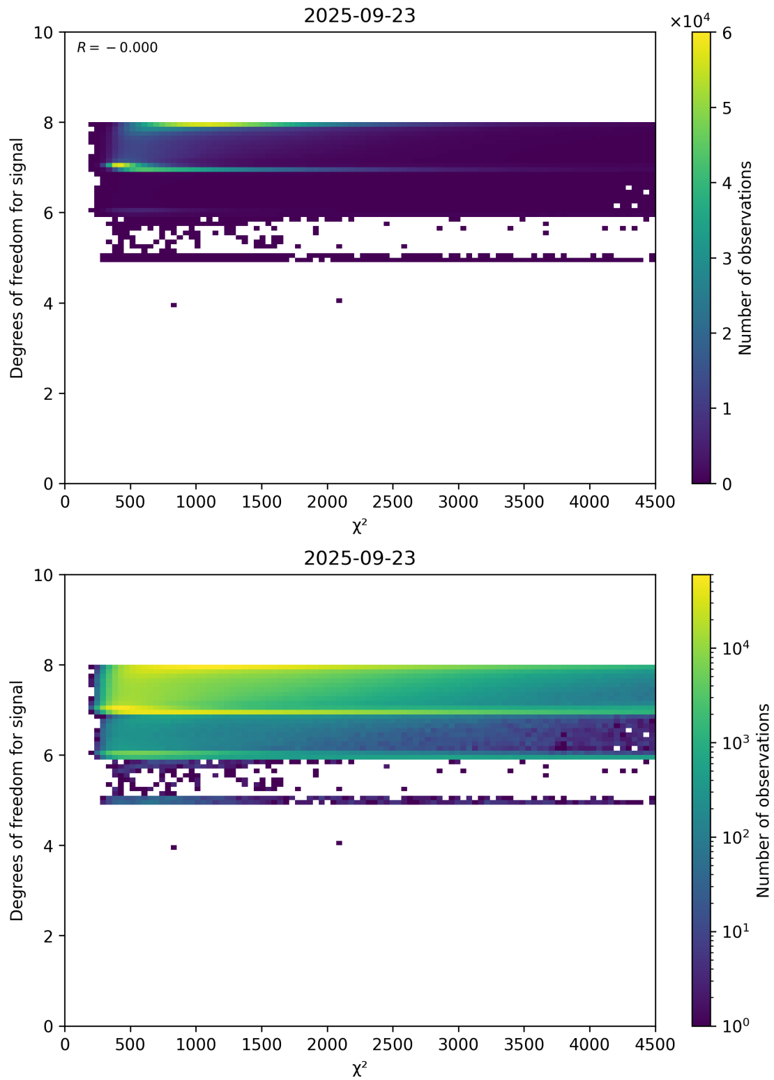
Figure 48: Scatter density plot of “ \chi^2 ” against “Degrees of freedom for signal” for 2025-09-22 to 2025-09-24.
