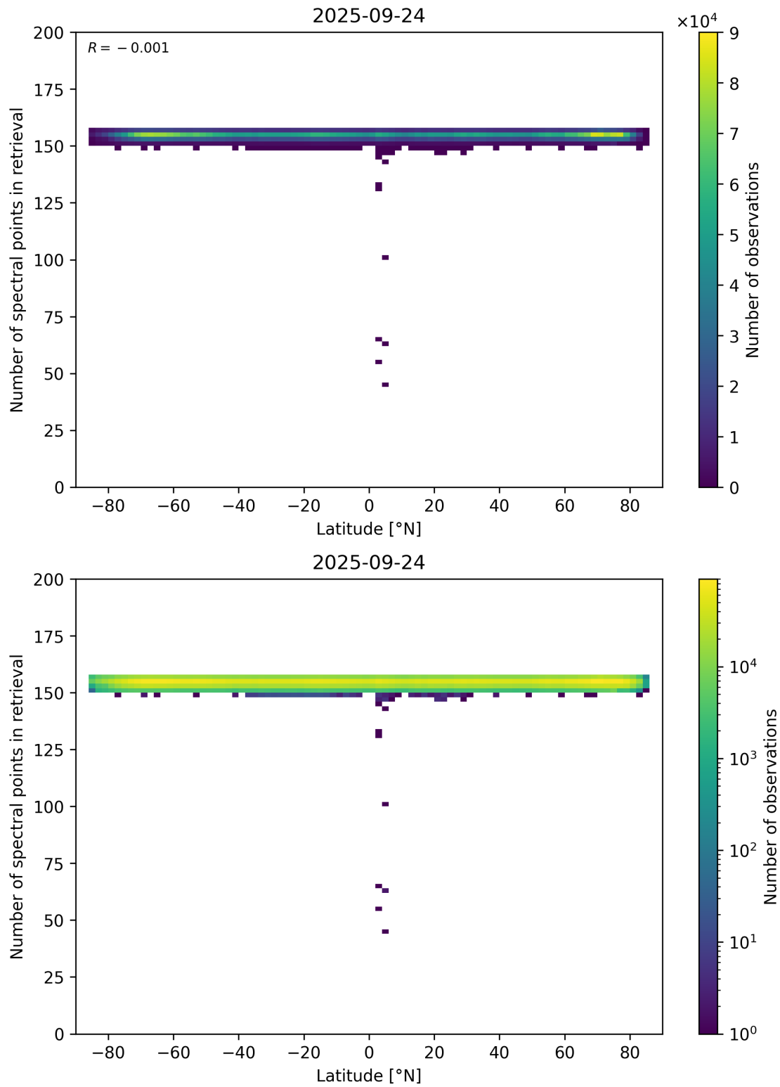
Figure 57: Scatter density plot of “Latitude” against “Number of spectral points in retrieval” for 2025-09-23 to 2025-09-25.
