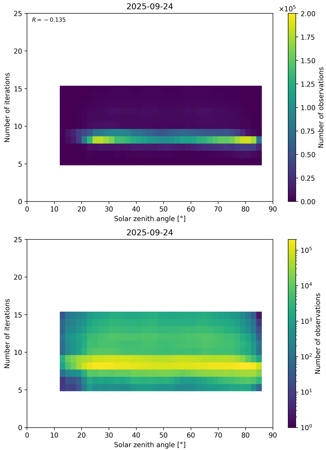
Figure 67: Scatter density plot of “Solar zenith angle” against “Number of iterations” for 2025-09-23 to 2025-09-25.
