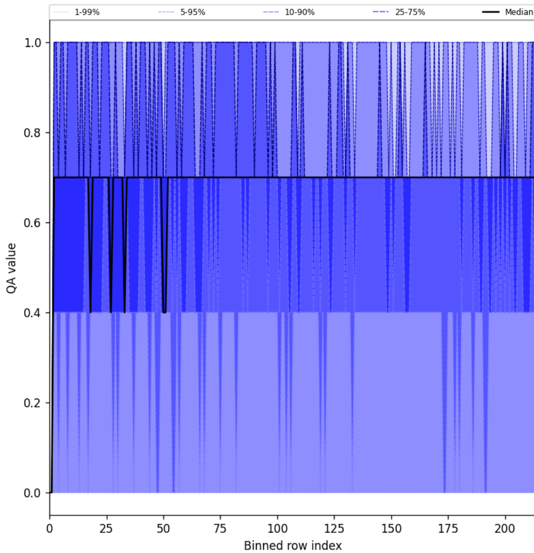
Figure 25: Along track statistics of “QA value” for 2025-09-23 to 2025-09-25
