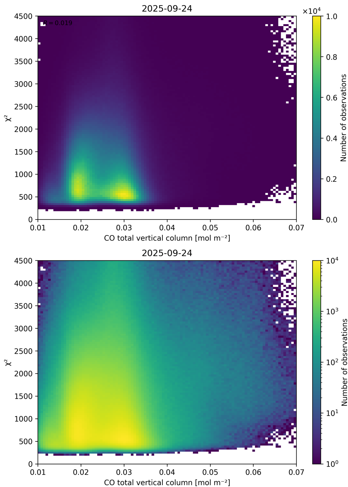
Figure 35: Scatter density plot of “CO total vertical column” against “ \chi^2 ” for 2025-09-23 to 2025-09-25.
