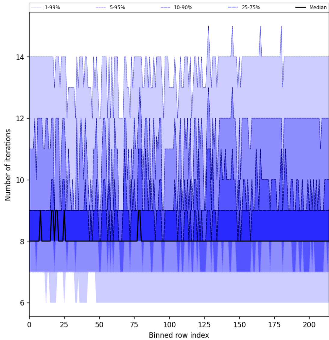
Figure 32: Along track statistics of “Number of iterations” for 2025-09-23 to 2025-09-25
