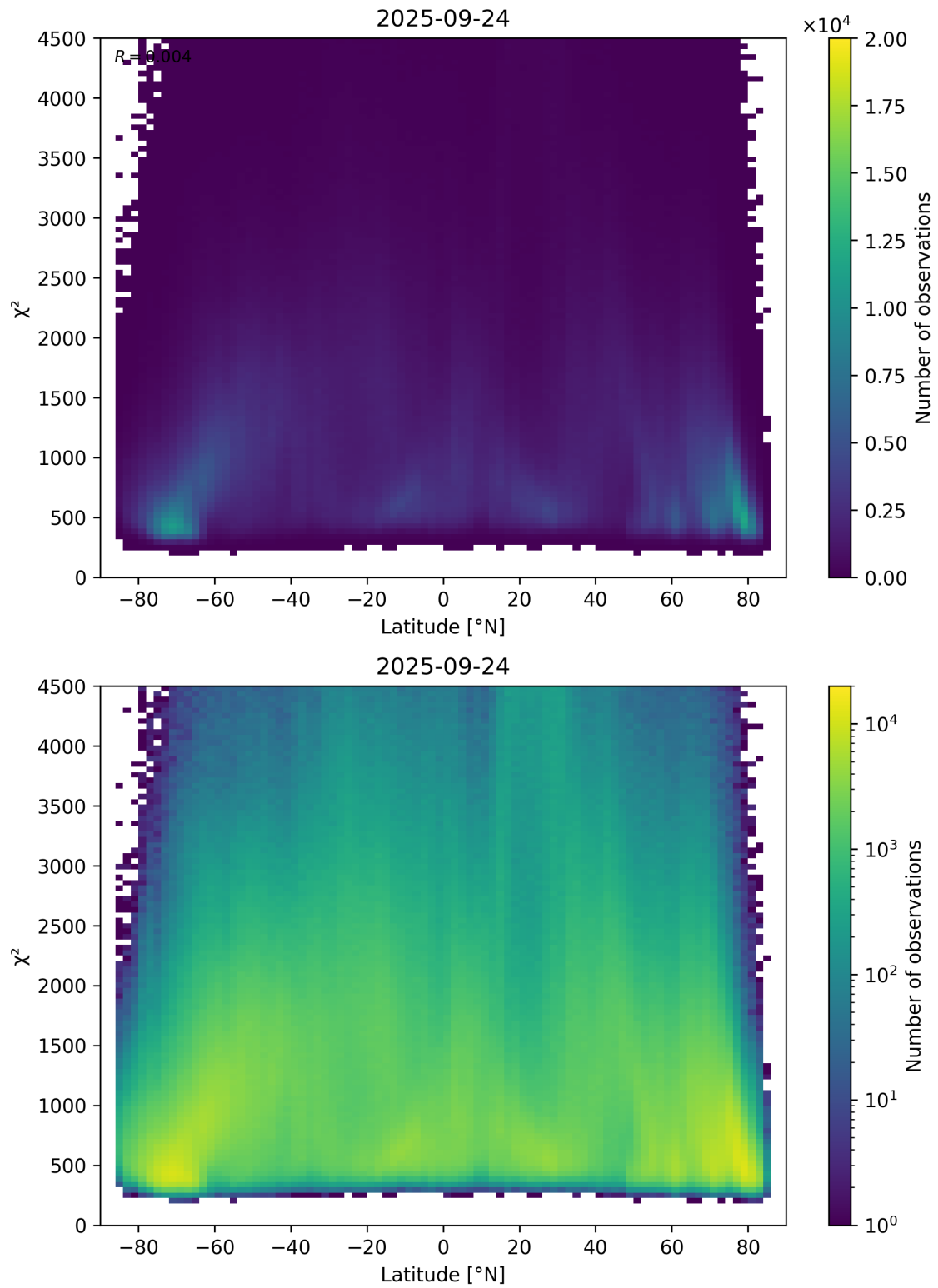
Figure 54: Scatter density plot of “Latitude” against “ \chi^2 ” for 2025-09-23 to 2025-09-25.
