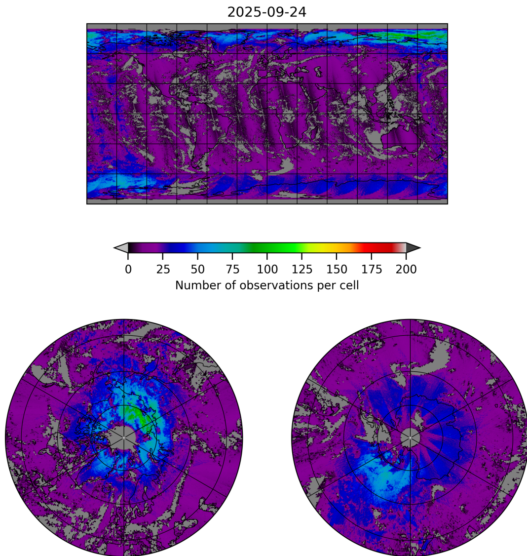
Figure 8: Map of the number of observations for 2025-09-23 to 2025-09-25
