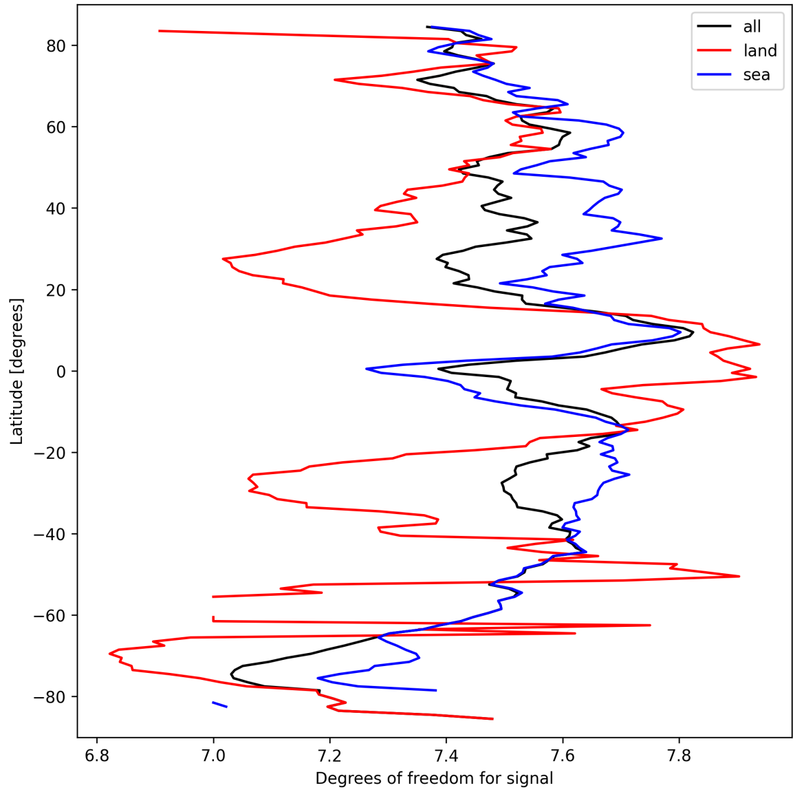
Figure 15: Zonal average of “Degrees of freedom for signal” for 2025-09-23 to 2025-09-25.
