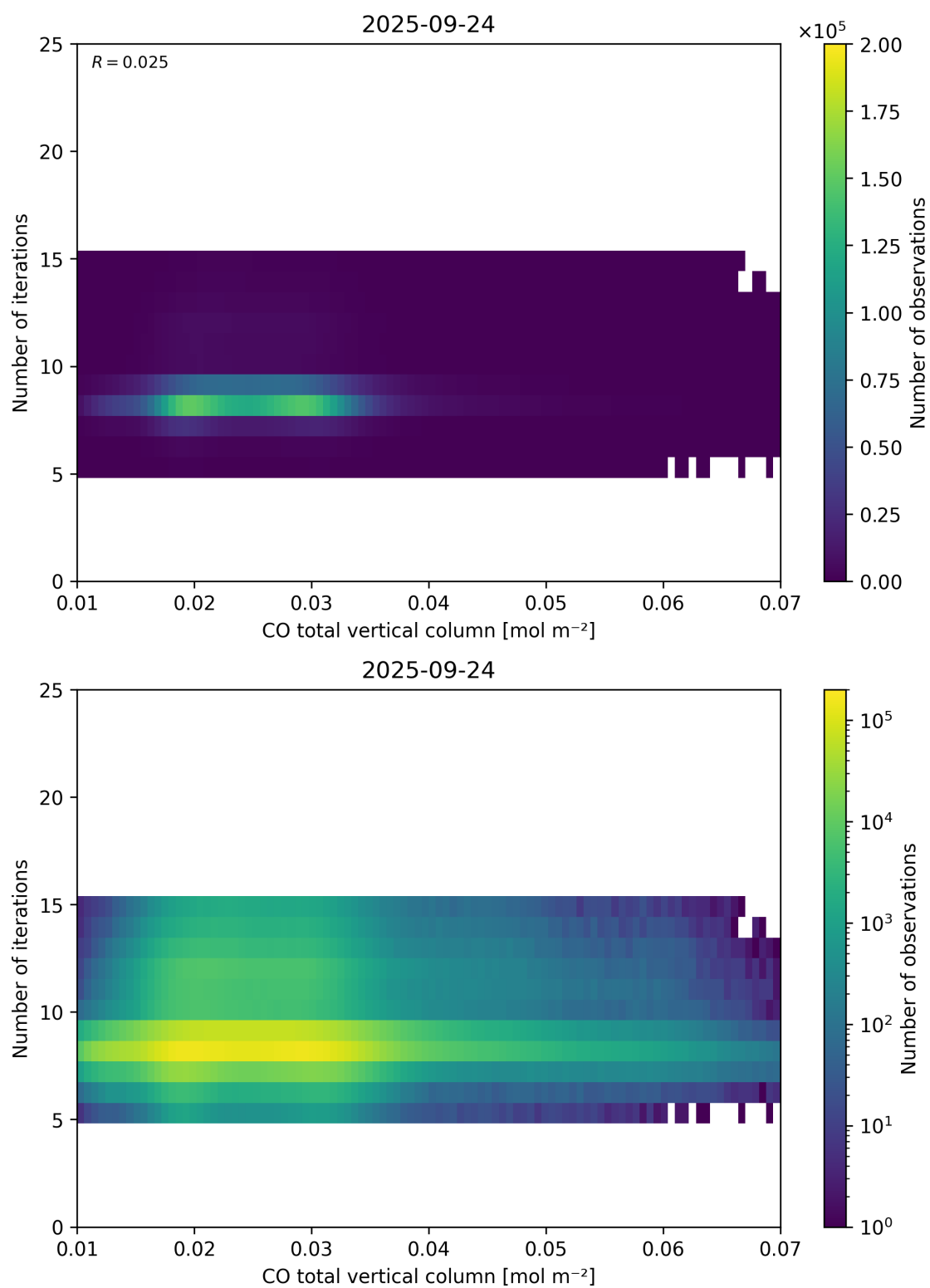
Figure 42: Scatter density plot of “CO total vertical column” against “Number of iterations” for 2025-09-23 to 2025-09-25.
