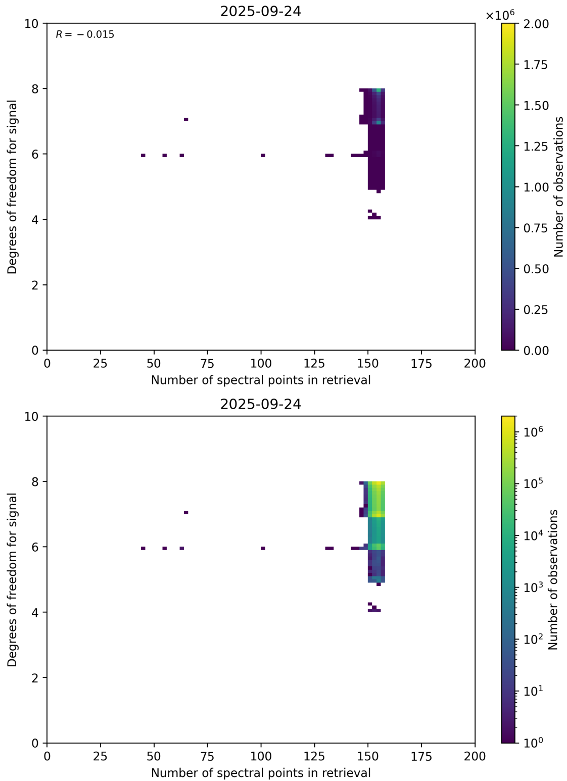
Figure 59: Scatter density plot of “Number of spectral points in retrieval” against “Degrees of freedom for signal” for 2025-09-23 to 2025-09-25.
