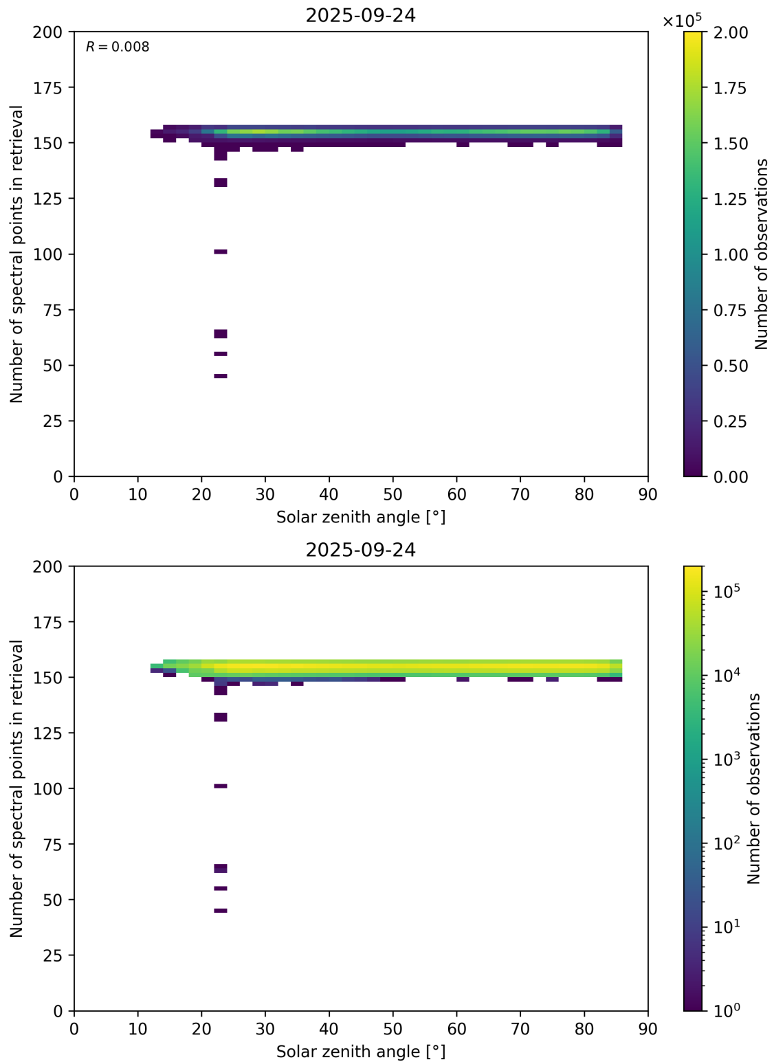
Figure 68: Scatter density plot of “Solar zenith angle” against “Number of spectral points in retrieval” for 2025-09-23 to 2025-09-25.
