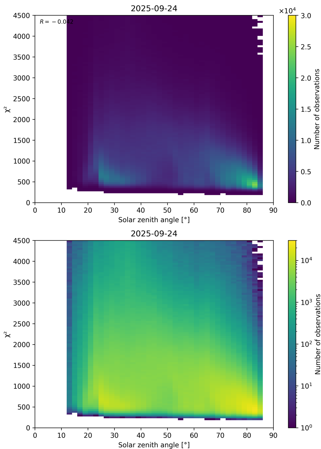
Figure 64: Scatter density plot of “Solar zenith angle” against “ \chi^2 ” for 2025-09-23 to 2025-09-25.
