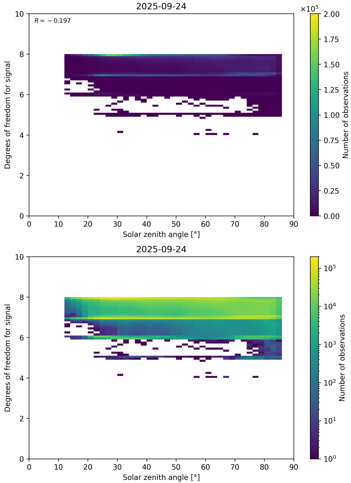
Figure 65: Scatter density plot of “Solar zenith angle” against “Degrees of freedom for signal” for 2025-09-23 to 2025-09-25.
