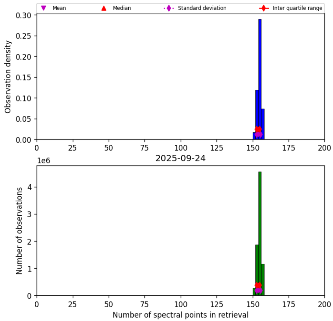
Figure 21: Histogram of “Number of spectral points in retrieval” for 2025-09-23 to 2025-09-25
