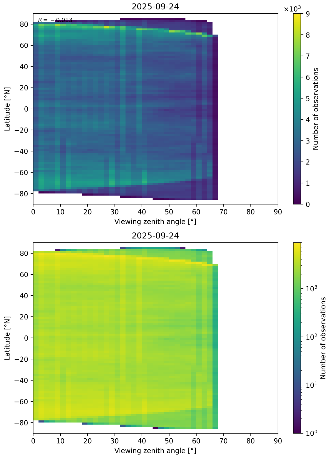
Figure 74: Scatter density plot of “Viewing zenith angle” against “Latitude” for 2025-09-23 to 2025-09-25.
