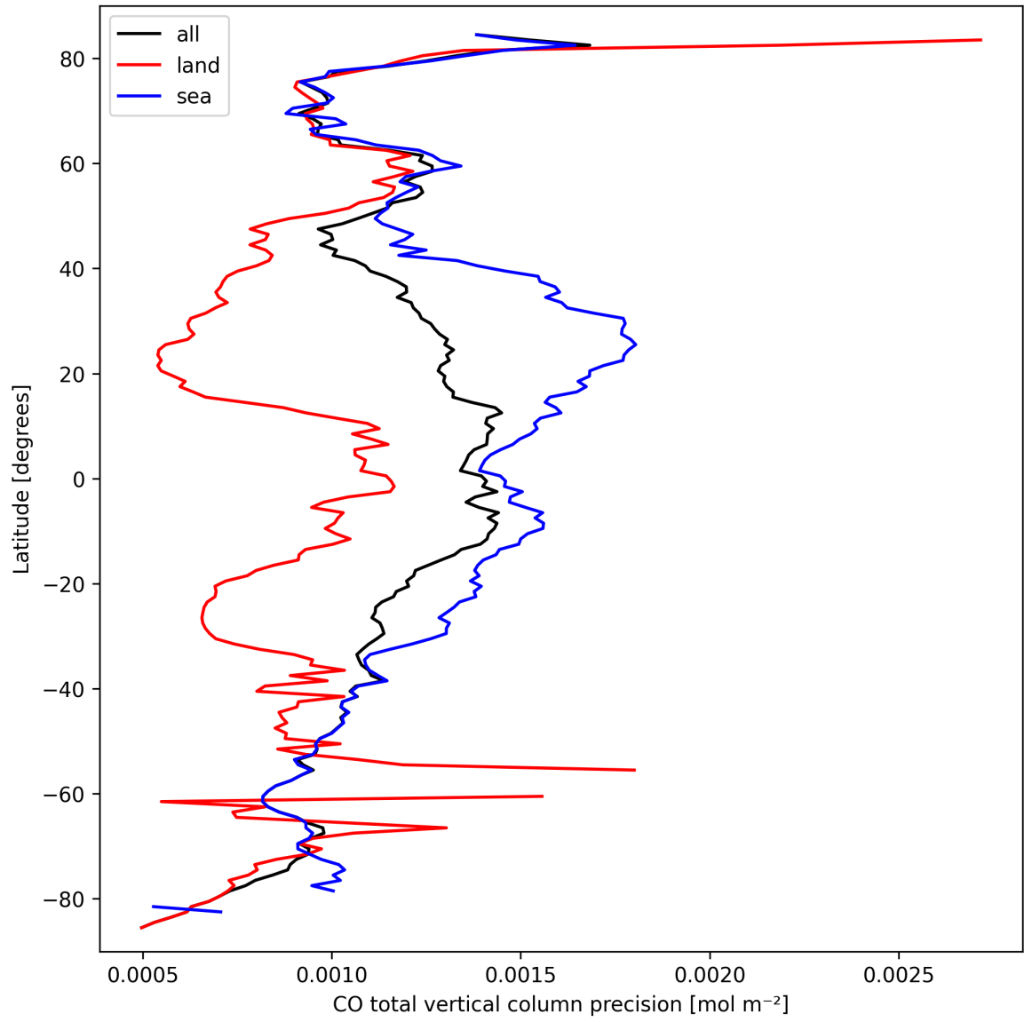
Figure 12: Zonal average of “CO total vertical column precision” for 2025-09-23 to 2025-09-25.
