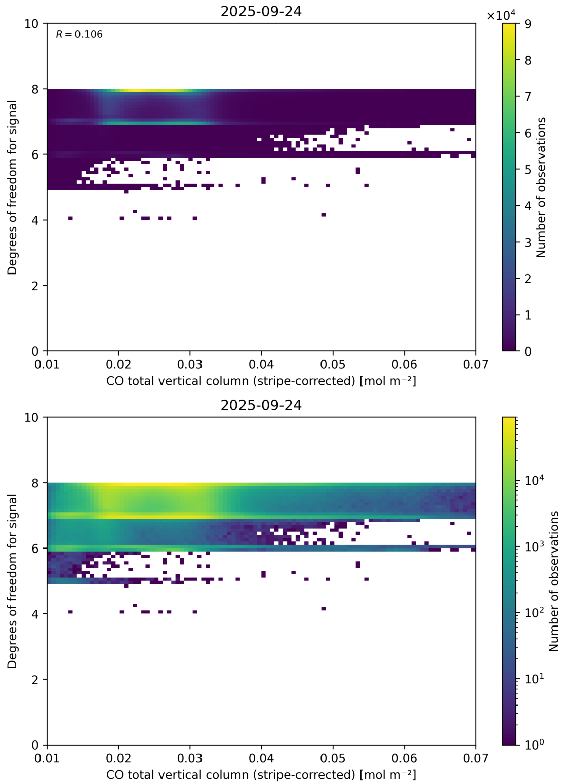
Figure 38: Scatter density plot of “CO total vertical column (stripe-corrected)” against “Degrees of freedom for signal” for 2025-09-23 to 2025-09-25.
