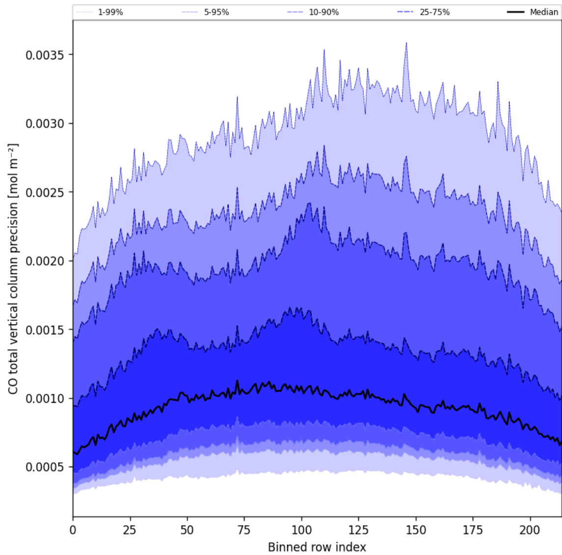
Figure 28: Along track statistics of “CO total vertical column precision” for 2025-09-23 to 2025-09-25
