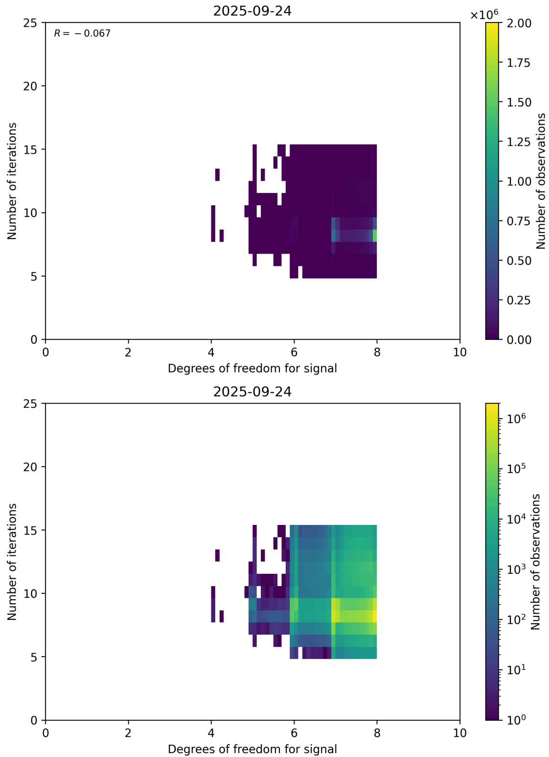
Figure 50: Scatter density plot of “Degrees of freedom for signal” against “Number of iterations” for 2025-09-23 to 2025-09-25.
