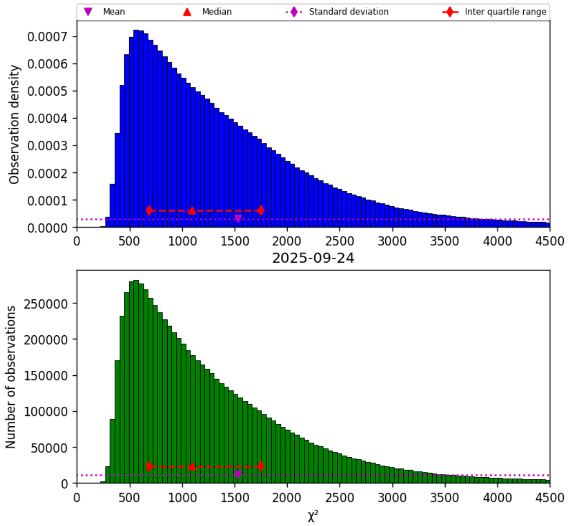
Figure 22: Histogram of “ \chi^2 ” for 2025-09-23 to 2025-09-25
