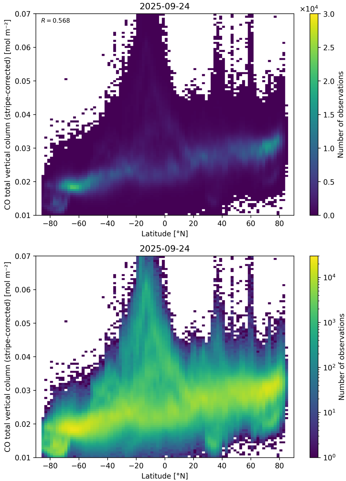
Figure 52: Scatter density plot of “Latitude” against “CO total vertical column (stripe-corrected)” for 2025-09-23 to 2025-09-25.
