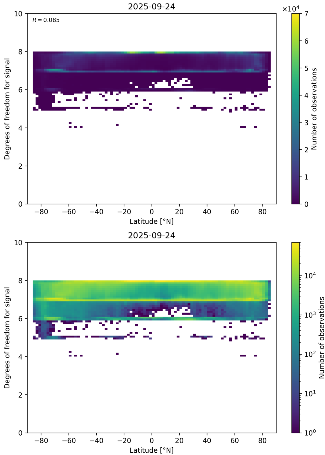
Figure 55: Scatter density plot of “Latitude” against “Degrees of freedom for signal” for 2025-09-23 to 2025-09-25.
