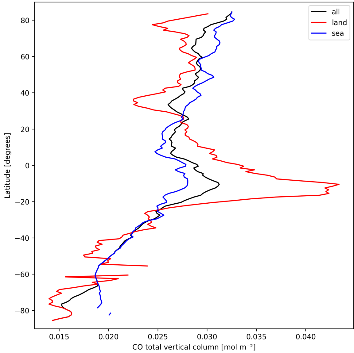
Figure 10: Zonal average of “CO total vertical column” for 2025-09-23 to 2025-09-25.
