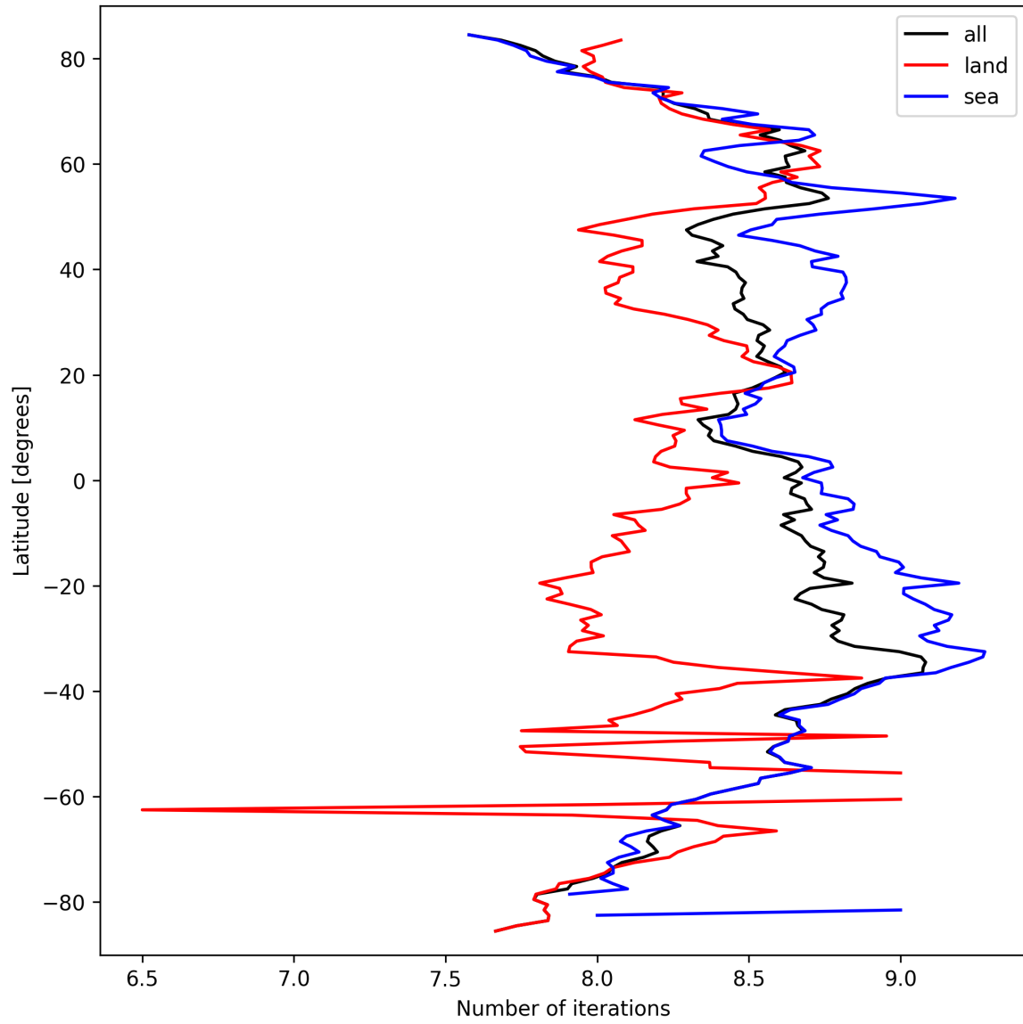
Figure 16: Zonal average of “Number of iterations” for 2025-09-23 to 2025-09-25.
