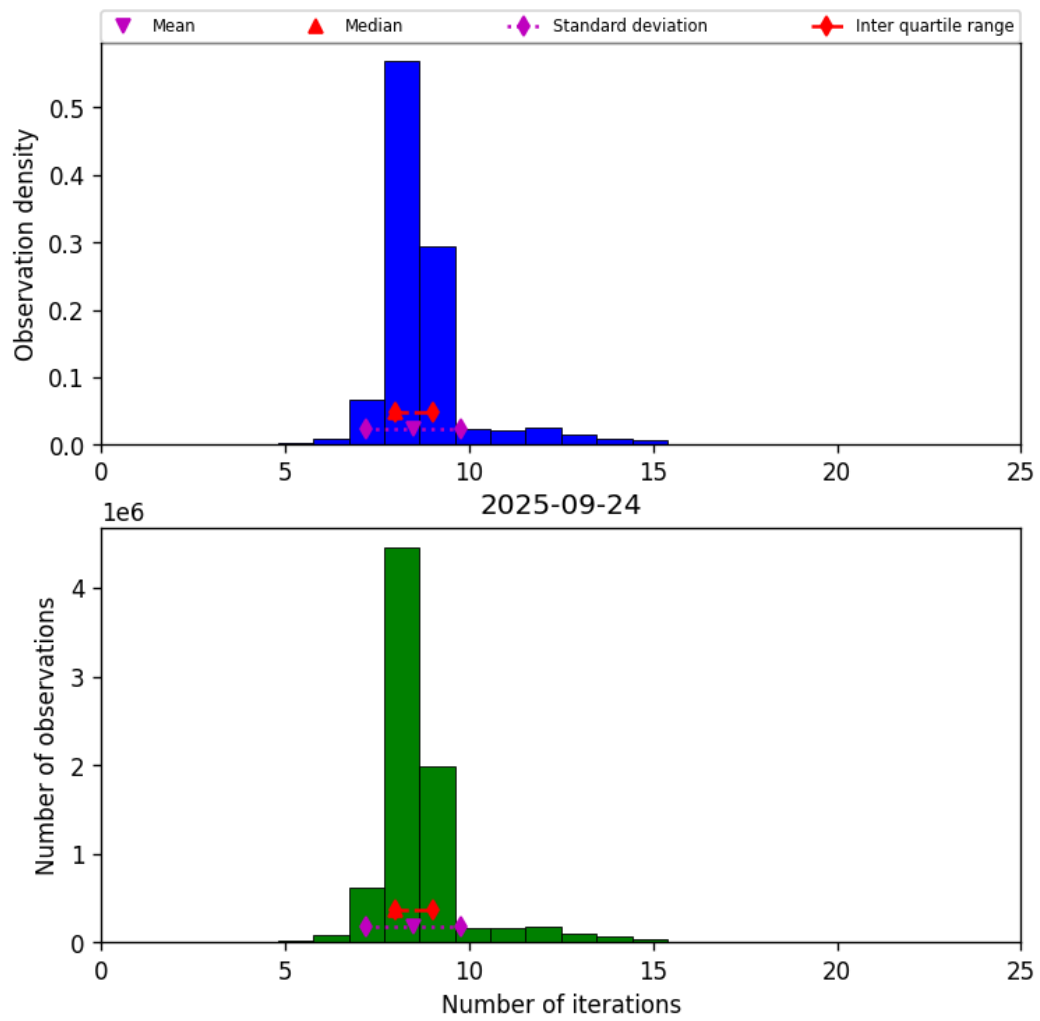
Figure 24: Histogram of “Number of iterations” for 2025-09-23 to 2025-09-25
