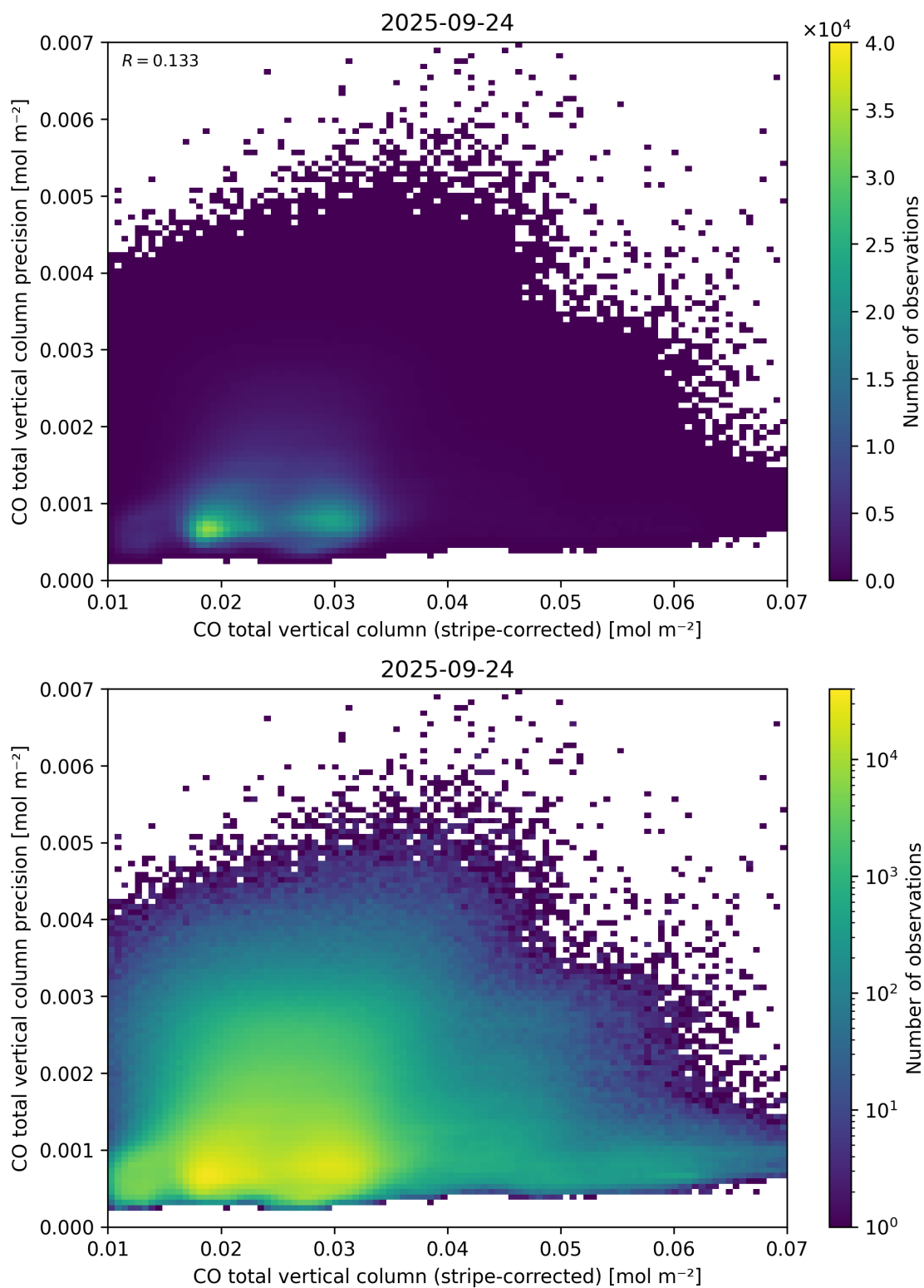
Figure 36: Scatter density plot of “CO total vertical column (stripe-corrected)” against “CO total vertical column precision” for 2025-09-23 to 2025-09-25.
