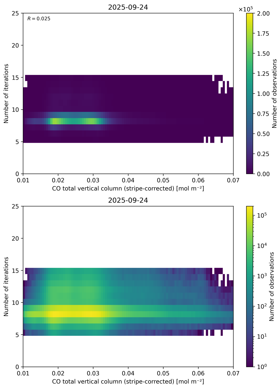
Figure 39: Scatter density plot of “CO total vertical column (stripe-corrected)” against “Number of iterations” for 2025-09-23 to 2025-09-25.
