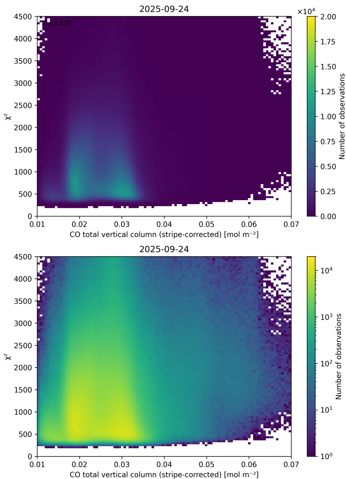
Figure 37: Scatter density plot of “CO total vertical column (stripe-corrected)” against “ \chi^2 ” for 2025-09-23 to 2025-09-25.
