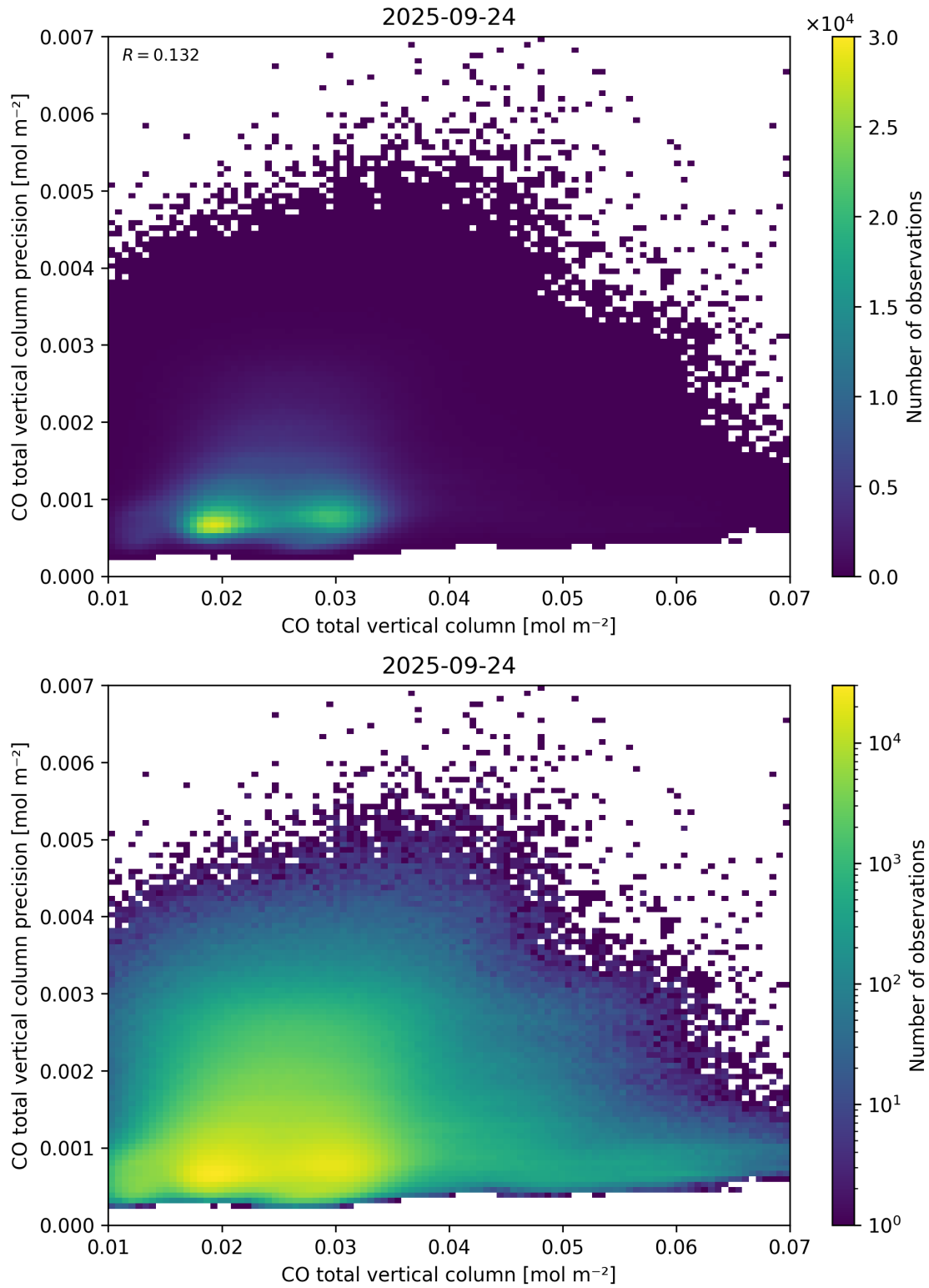
Figure 34: Scatter density plot of “CO total vertical column” against “CO total vertical column precision” for 2025-09-23 to 2025-09-25.
