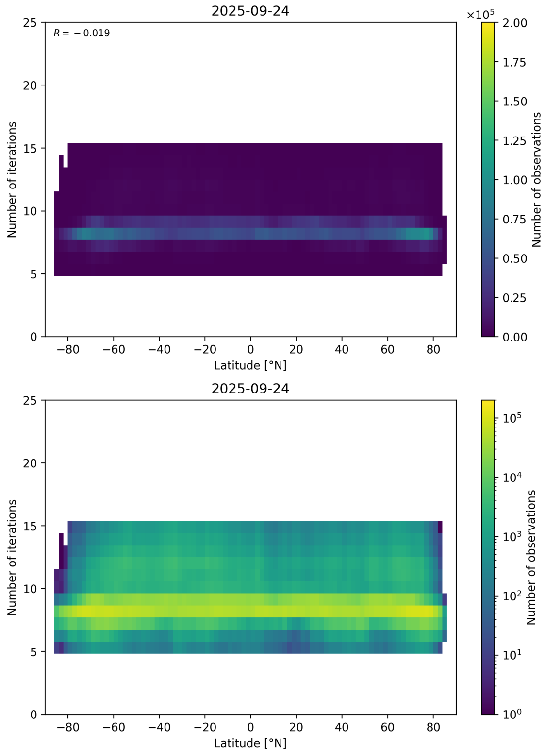
Figure 56: Scatter density plot of “Latitude” against “Number of iterations” for 2025-09-23 to 2025-09-25.
