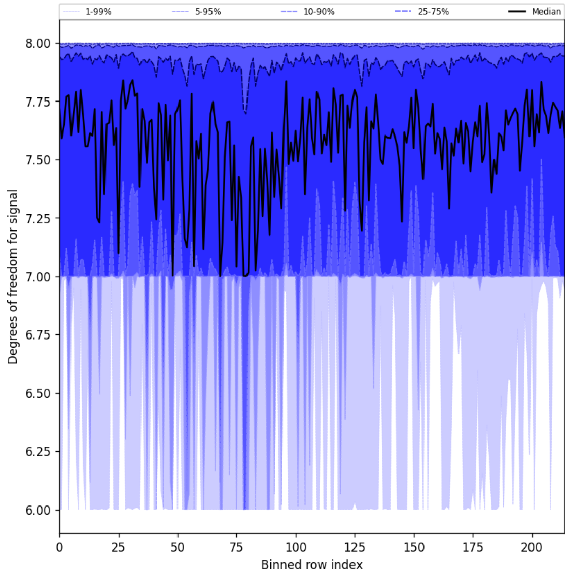
Figure 31: Along track statistics of “Degrees of freedom for signal” for 2025-09-23 to 2025-09-25
