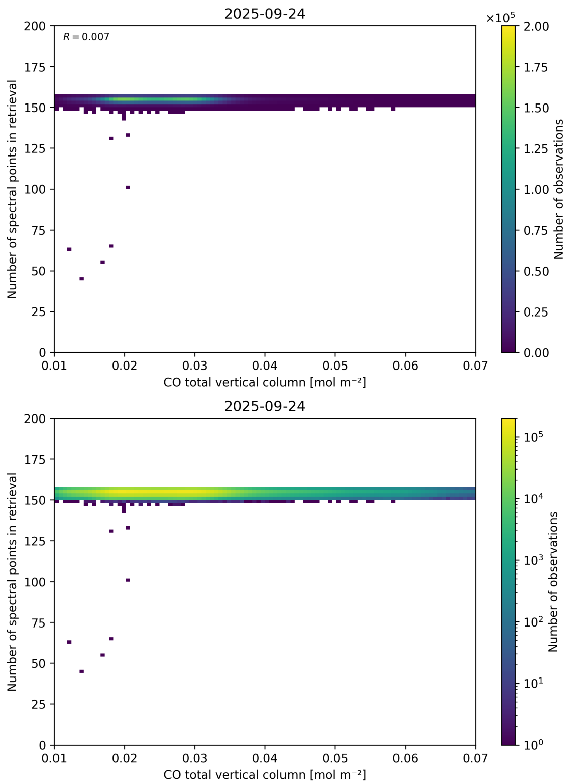
Figure 43: Scatter density plot of “CO total vertical column” against “Number of spectral points in retrieval” for 2025-09-23 to 2025-09-25.
