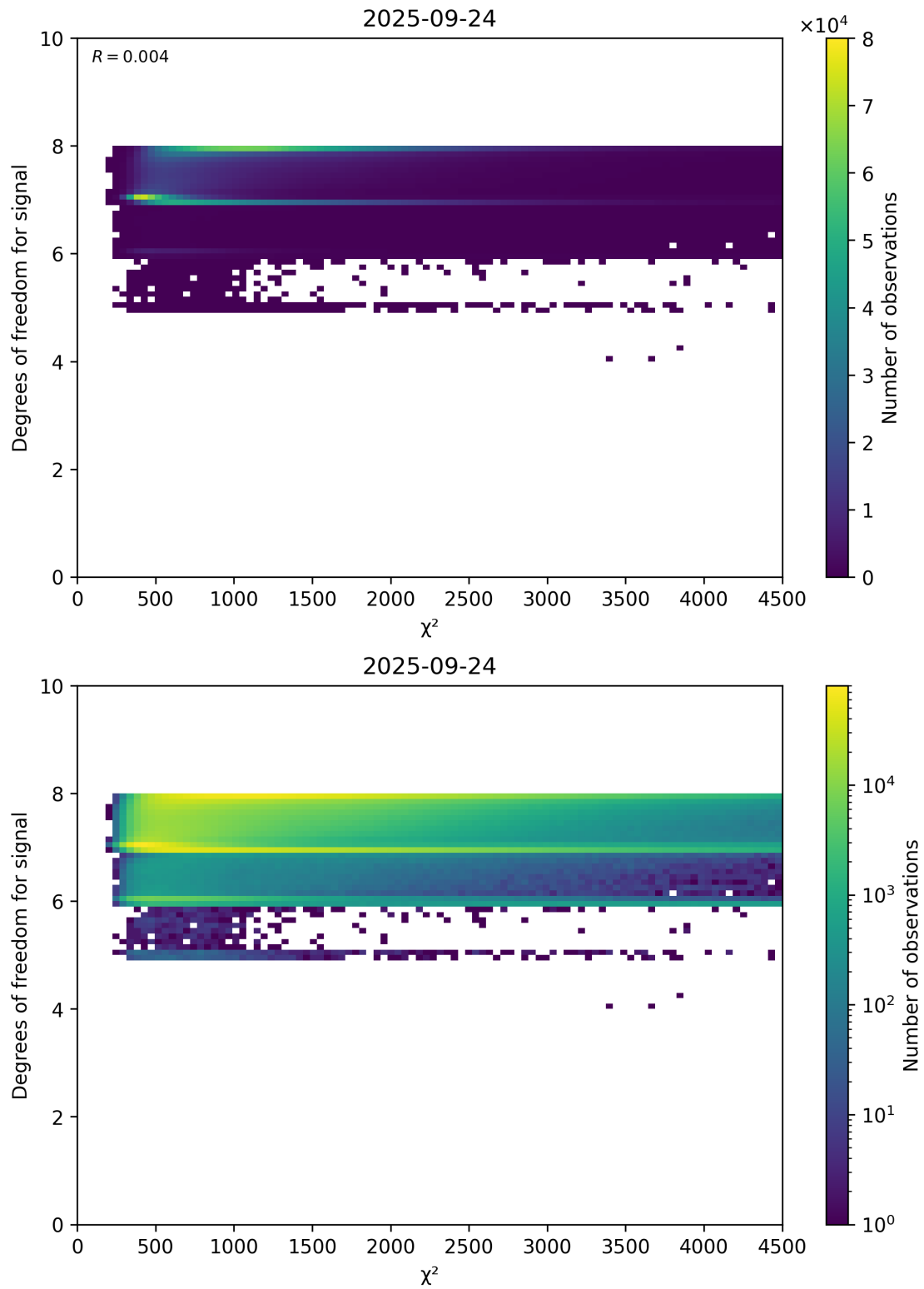
Figure 48: Scatter density plot of “ \chi^2 ” against “Degrees of freedom for signal” for 2025-09-23 to 2025-09-25.
