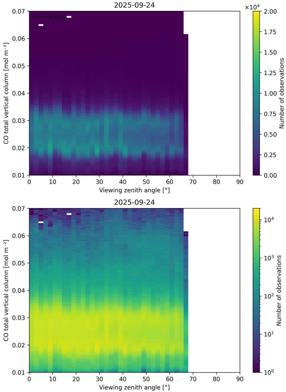
Figure 69: Scatter density plot of “Viewing zenith angle” against “CO total vertical column” for 2025-09-23 to 2025-09-25.
