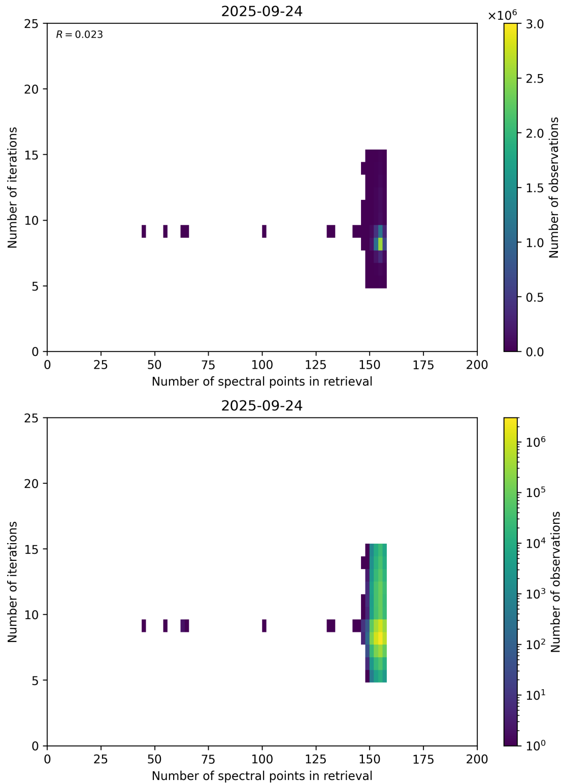
Figure 60: Scatter density plot of “Number of spectral points in retrieval” against “Number of iterations” for 2025-09-23 to 2025-09-25.
