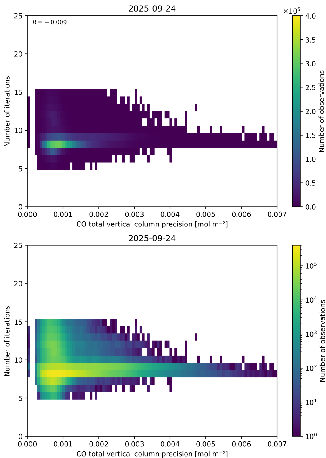
Figure 46: Scatter density plot of “CO total vertical column precision” against “Number of iterations” for 2025-09-23 to 2025-09-25.
