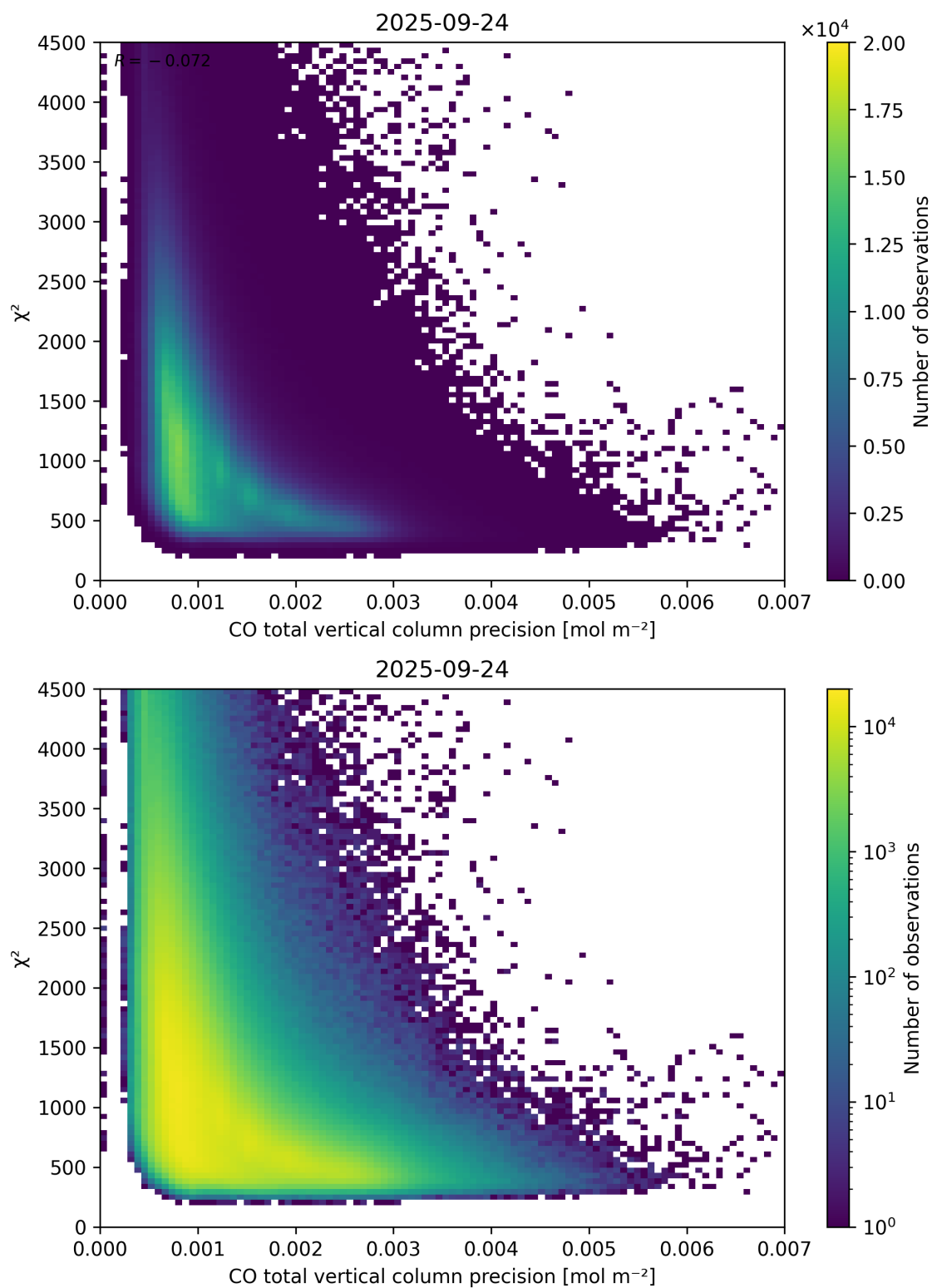
Figure 44: Scatter density plot of “CO total vertical column precision” against “ \chi^2 ” for 2025-09-23 to 2025-09-25.
