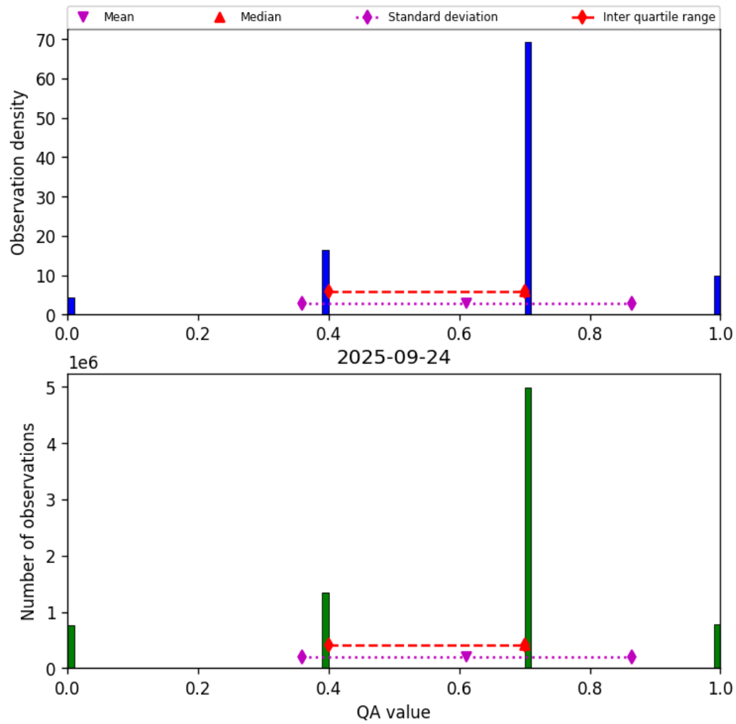
Figure 17: Histogram of “QA value” for 2025-09-23 to 2025-09-25
