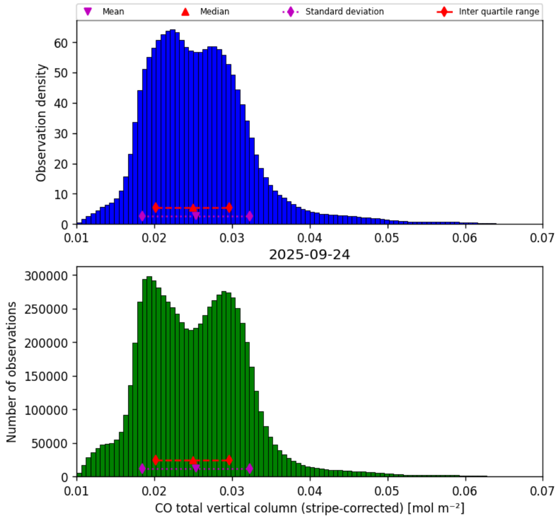
Figure 19: Histogram of “CO total vertical column (stripe-corrected)” for 2025-09-23 to 2025-09-25
