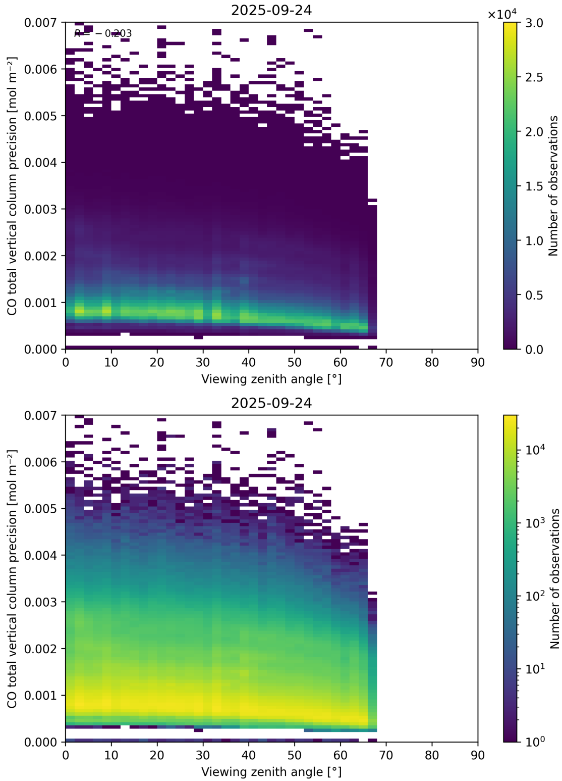
Figure 71: Scatter density plot of “Viewing zenith angle” against “CO total vertical column precision” for 2025-09-23 to 2025-09-25.
