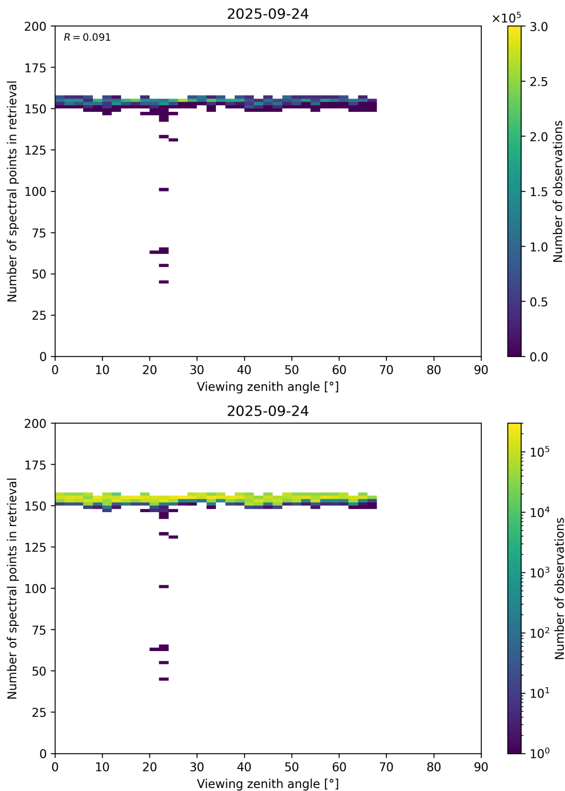
Figure 76: Scatter density plot of “Viewing zenith angle” against “Number of spectral points in retrieval” for 2025-09-23 to 2025-09-25.
