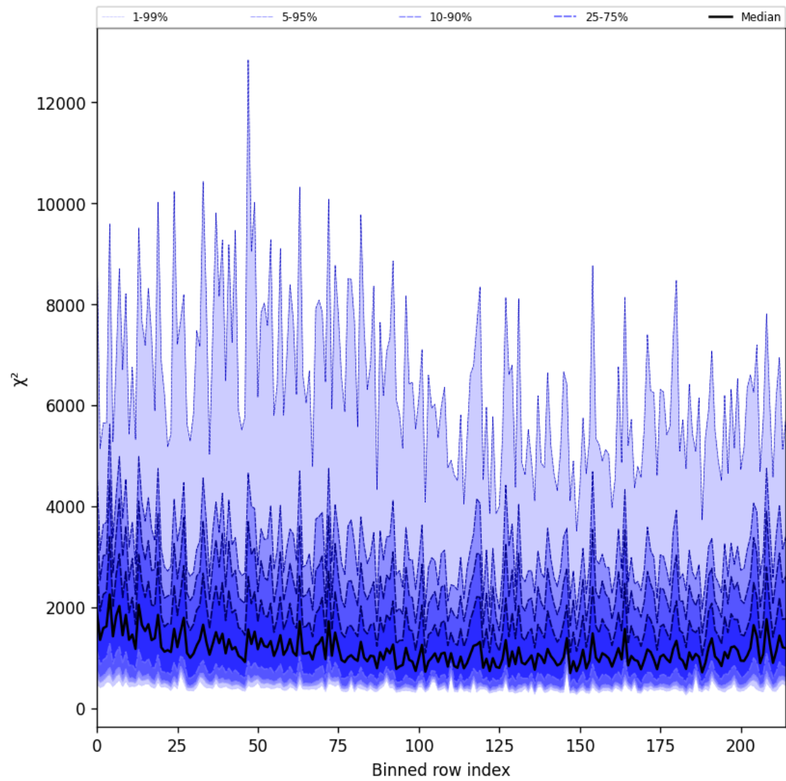
Figure 30: Along track statistics of “ \chi^2 ” for 2025-09-23 to 2025-09-25
