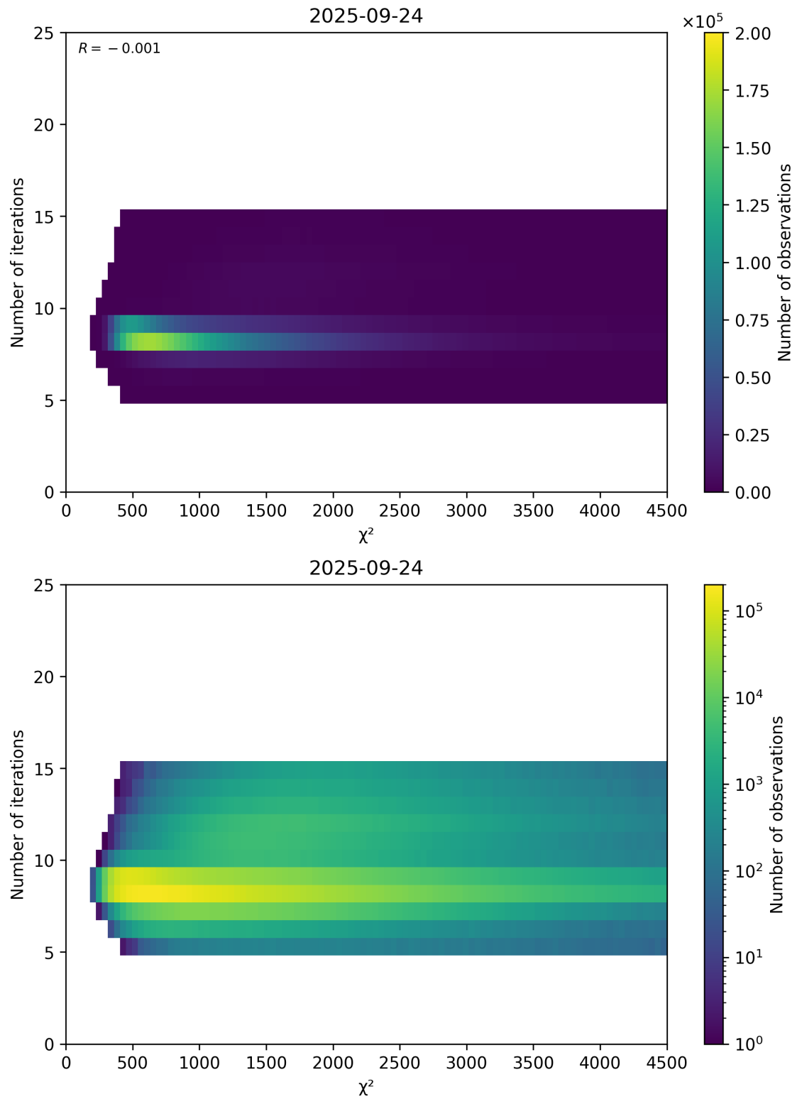
Figure 49: Scatter density plot of “ \chi^2 ” against “Number of iterations” for 2025-09-23 to 2025-09-25.
