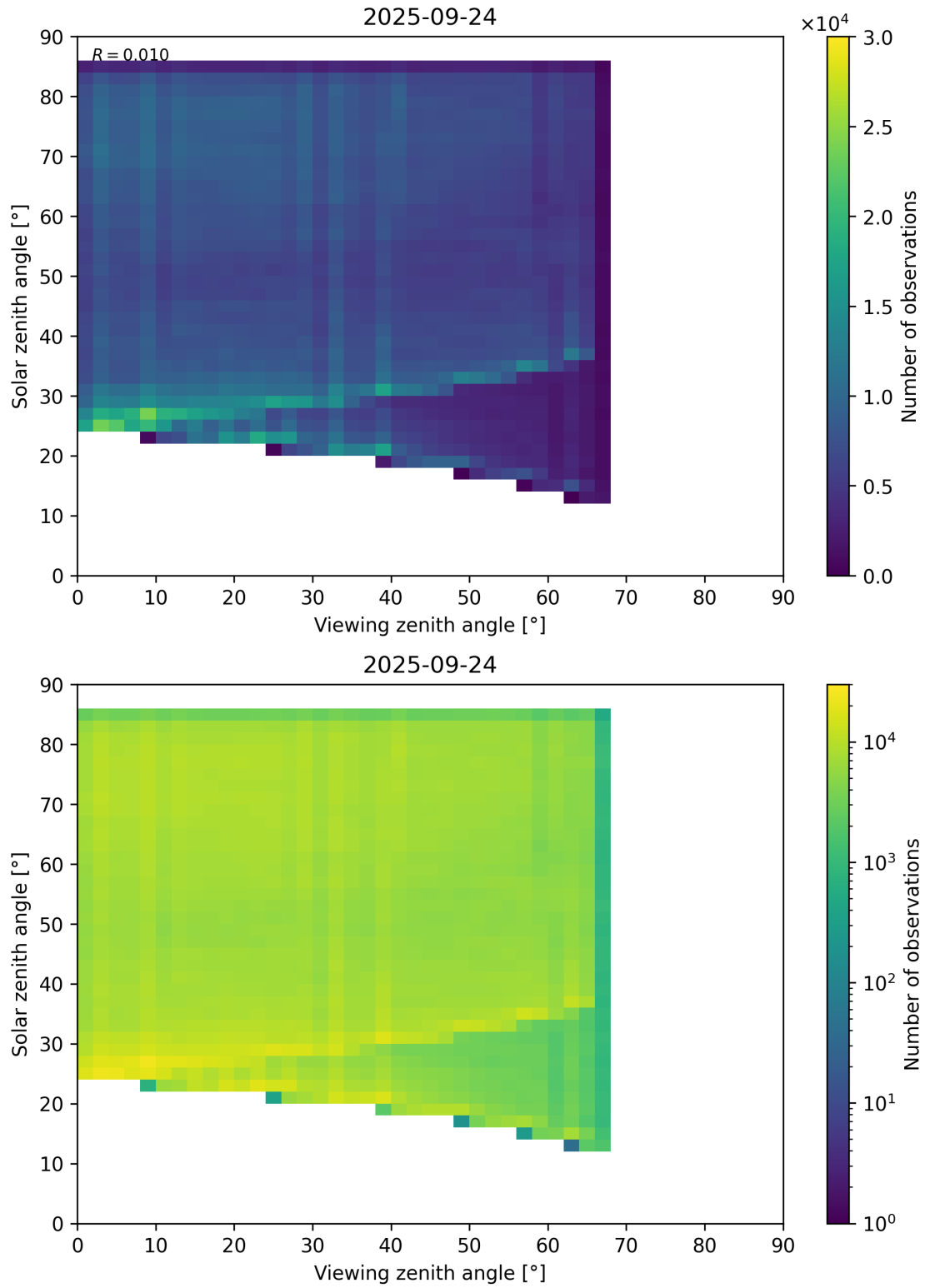
Figure 77: Scatter density plot of “Viewing zenith angle” against “Solar zenith angle” for 2025-09-23 to 2025-09-25.
