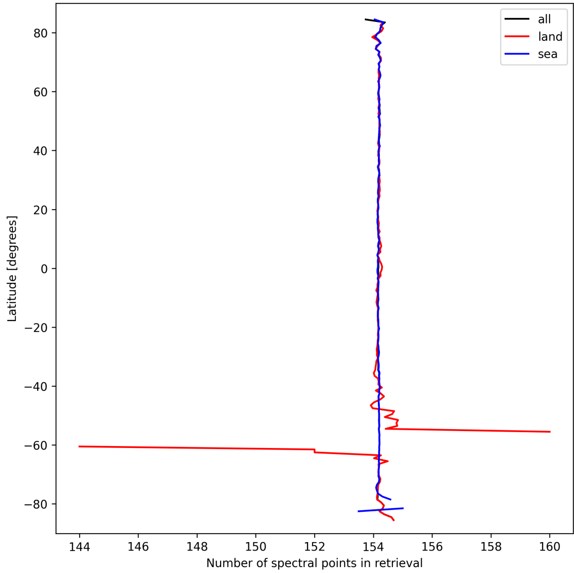
Figure 13: Zonal average of “Number of spectral points in retrieval” for 2025-09-23 to 2025-09-25.
