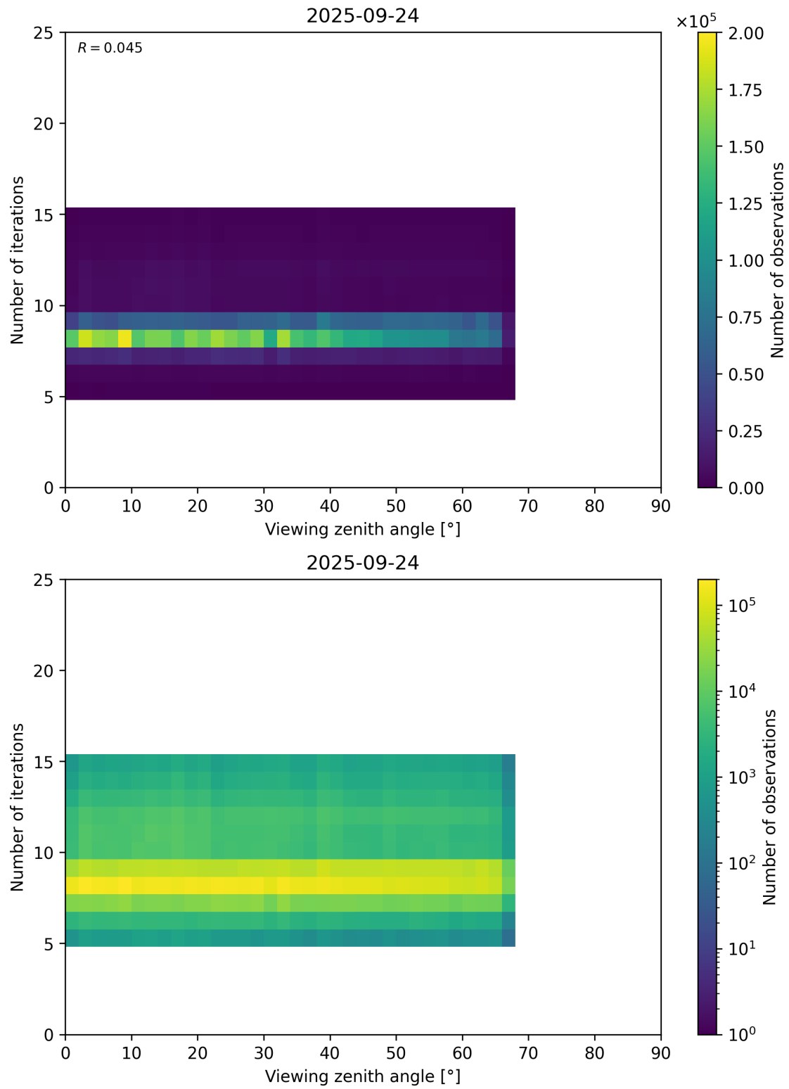
Figure 75: Scatter density plot of “Viewing zenith angle” against “Number of iterations” for 2025-09-23 to 2025-09-25.
