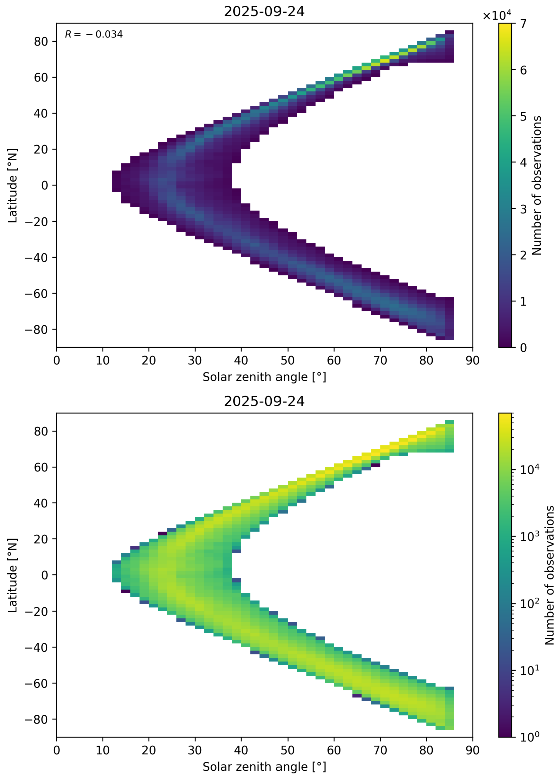
Figure 66: Scatter density plot of “Solar zenith angle” against “Latitude” for 2025-09-23 to 2025-09-25.
