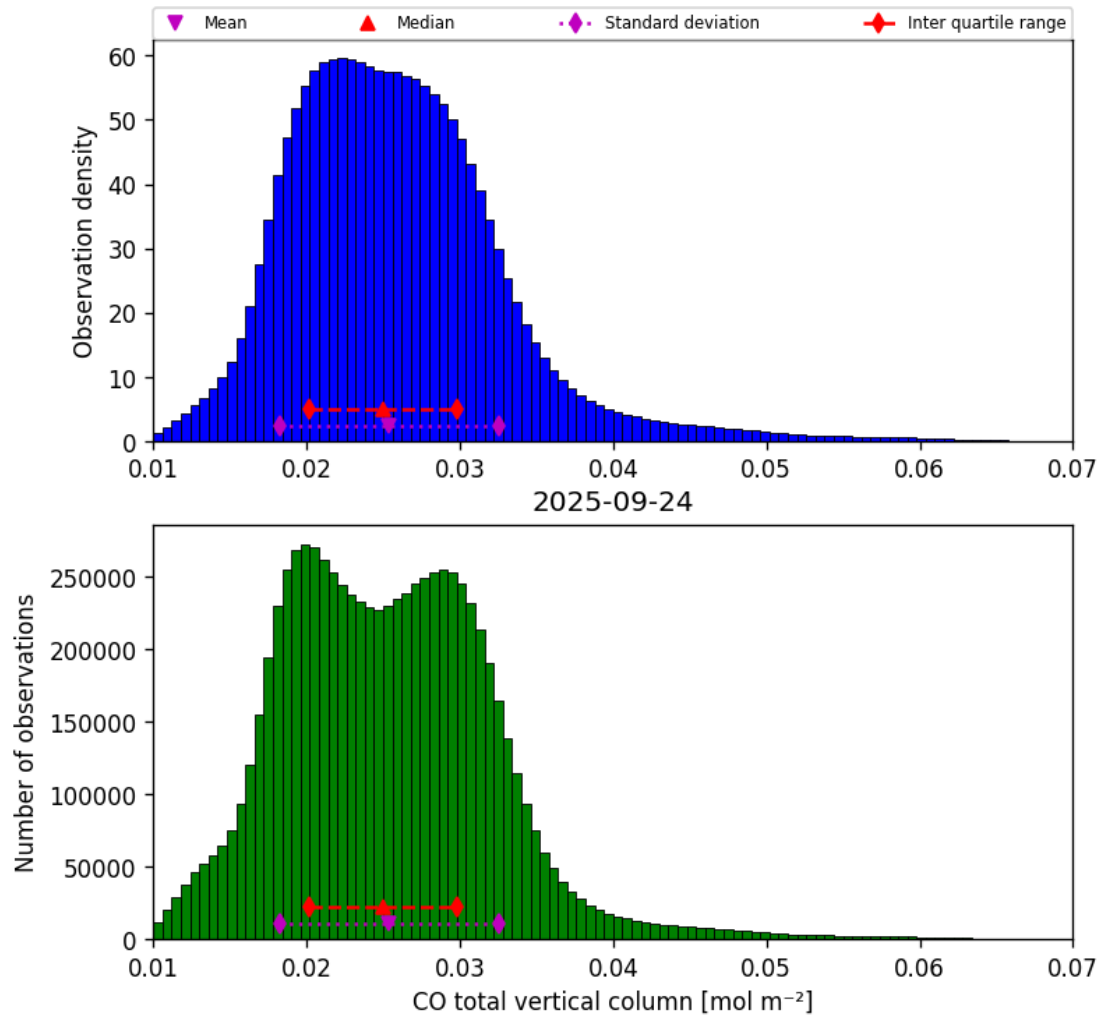
Figure 18: Histogram of “CO total vertical column” for 2025-09-23 to 2025-09-25
