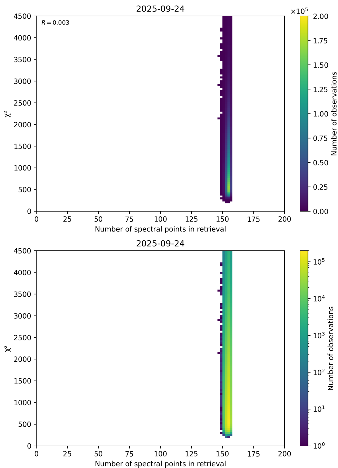
Figure 58: Scatter density plot of “Number of spectral points in retrieval” against “ \chi^2 ” for 2025-09-23 to 2025-09-25.
