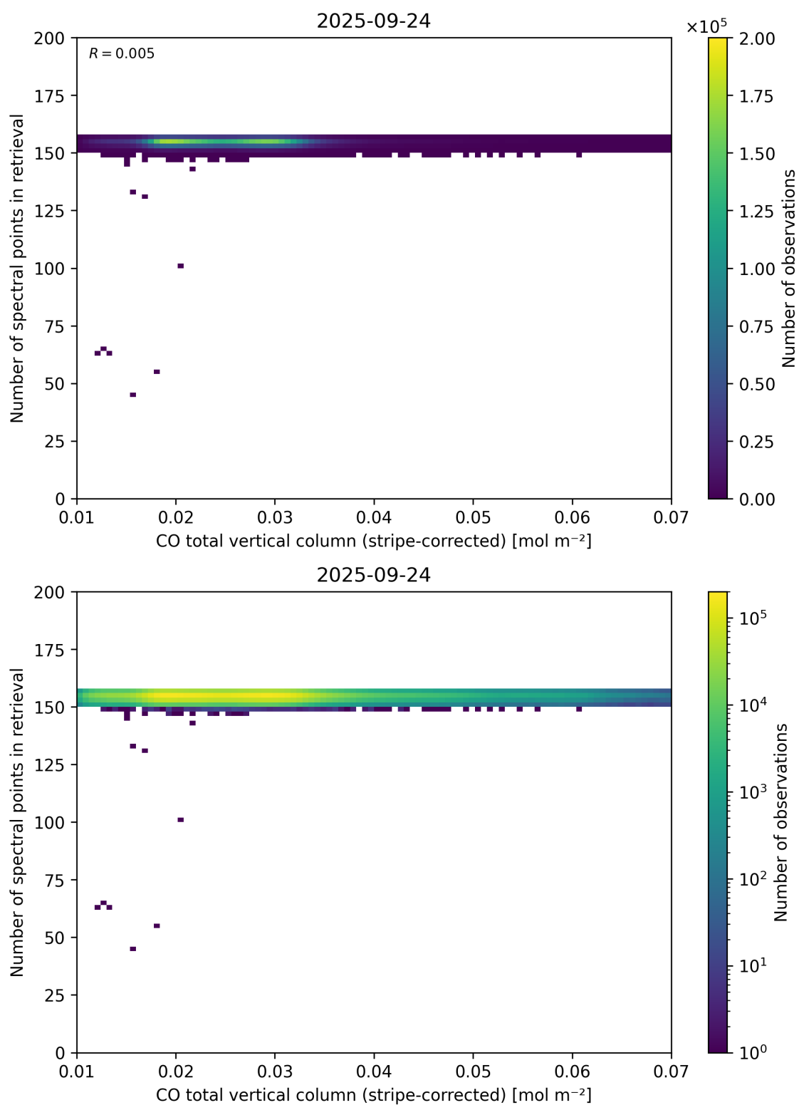
Figure 40: Scatter density plot of “CO total vertical column (stripe-corrected)” against “Number of spectral points in retrieval” for 2025-09-23 to 2025-09-25.
