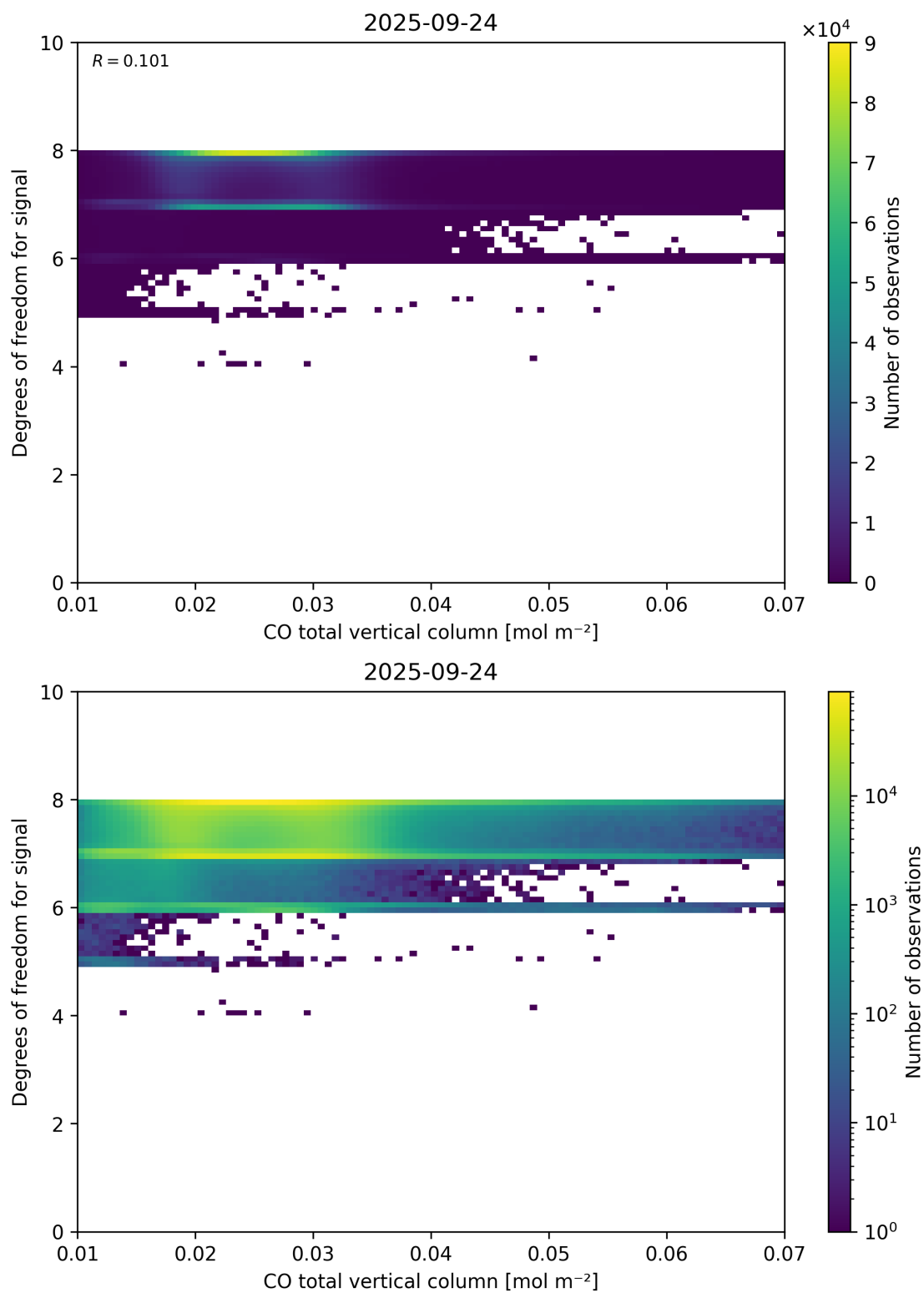
Figure 41: Scatter density plot of “CO total vertical column” against “Degrees of freedom for signal” for 2025-09-23 to 2025-09-25.
