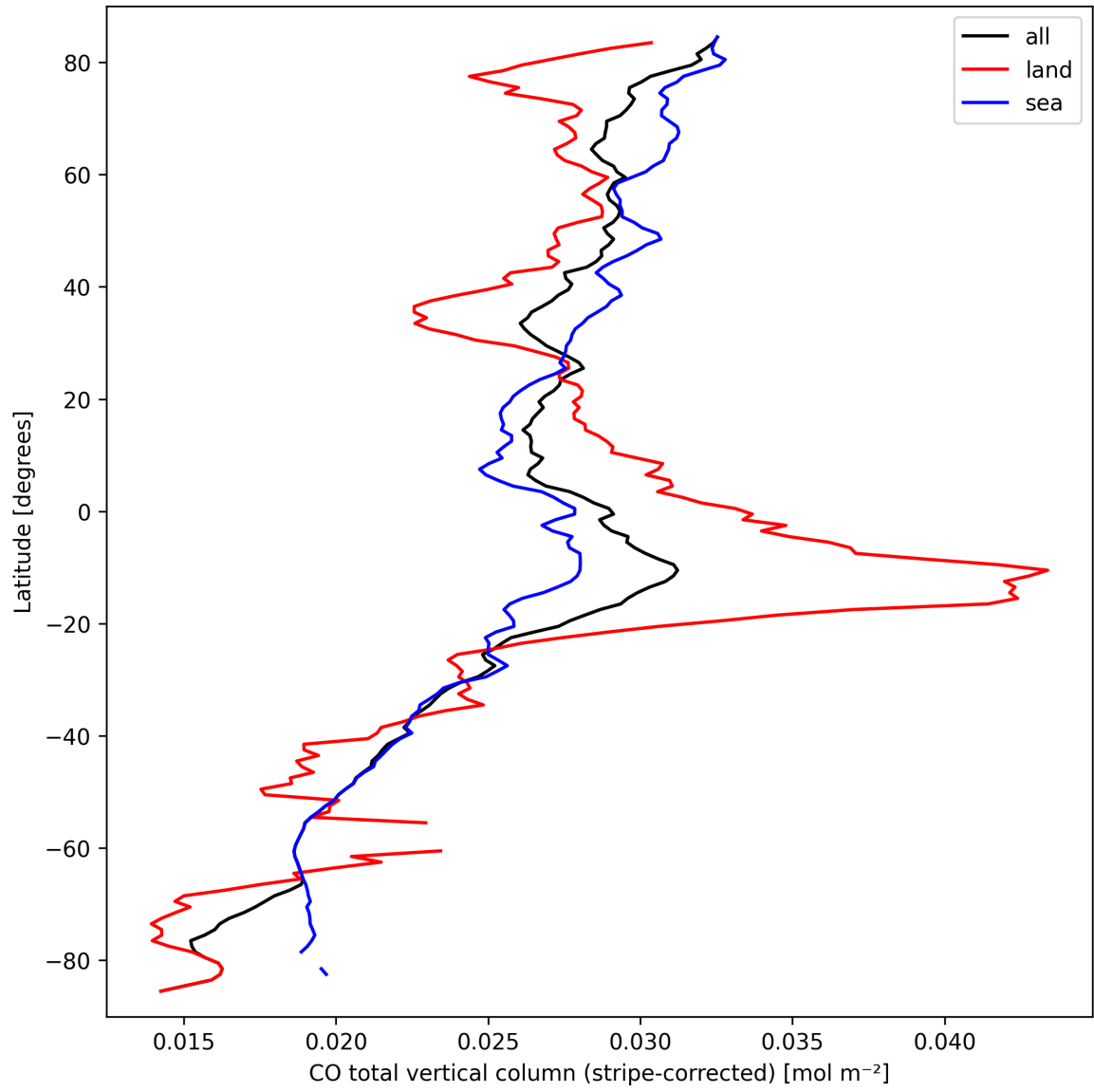
Figure 11: Zonal average of “CO total vertical column (stripe-corrected)” for 2025-09-23 to 2025-09-25.
