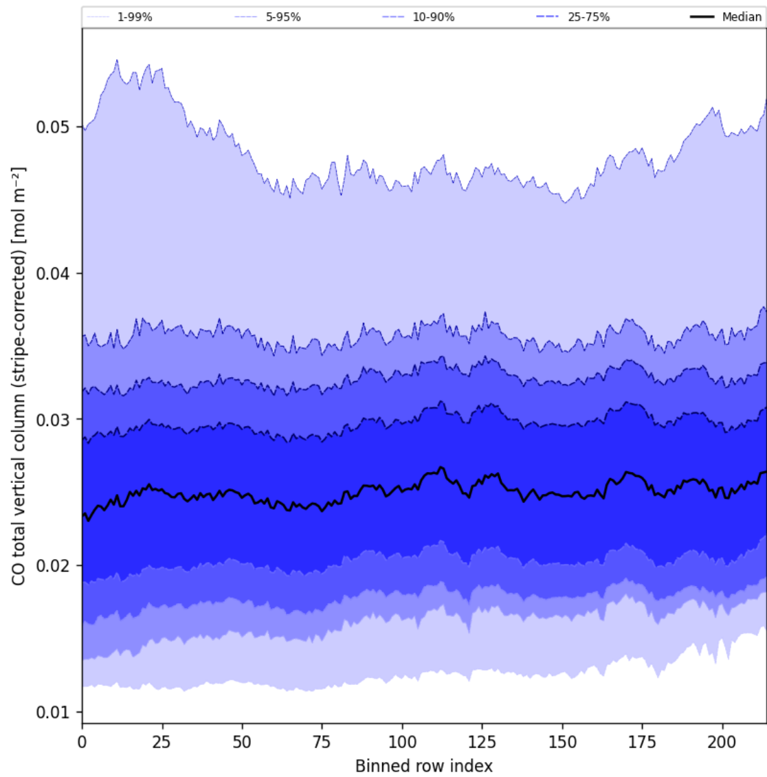
Figure 27: Along track statistics of “CO total vertical column (stripe-corrected)” for 2025-09-23 to 2025-09-25
