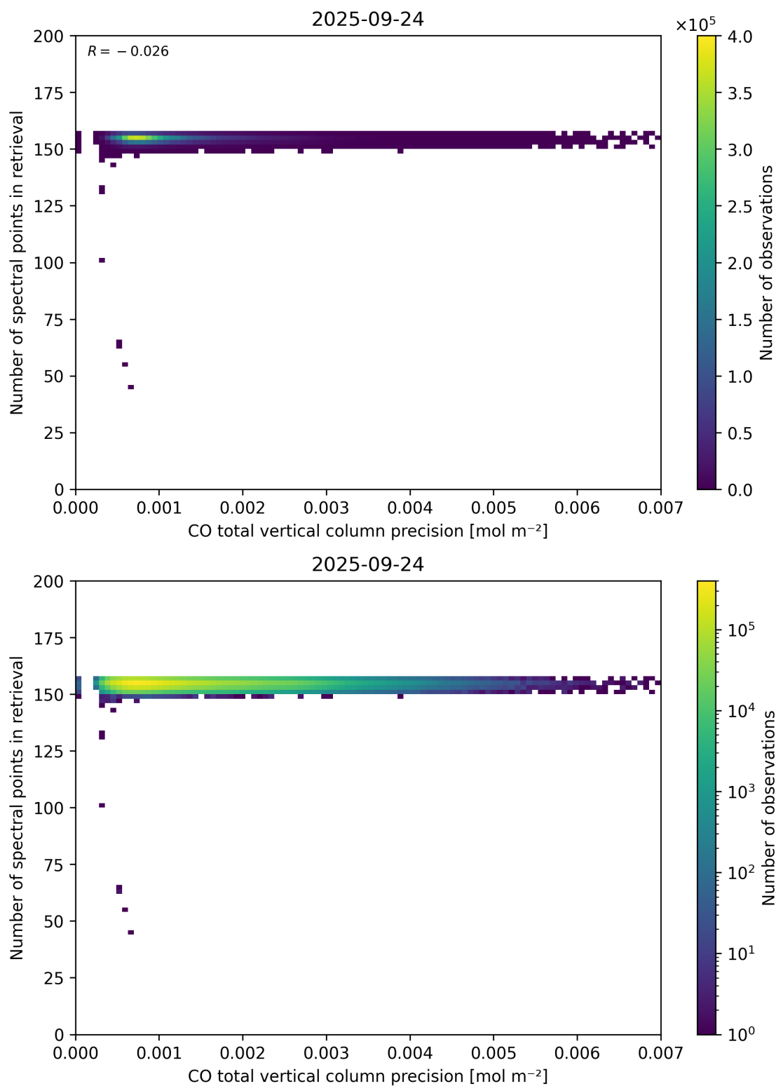
Figure 47: Scatter density plot of “CO total vertical column precision” against “Number of spectral points in retrieval” for 2025-09-23 to 2025-09-25.
