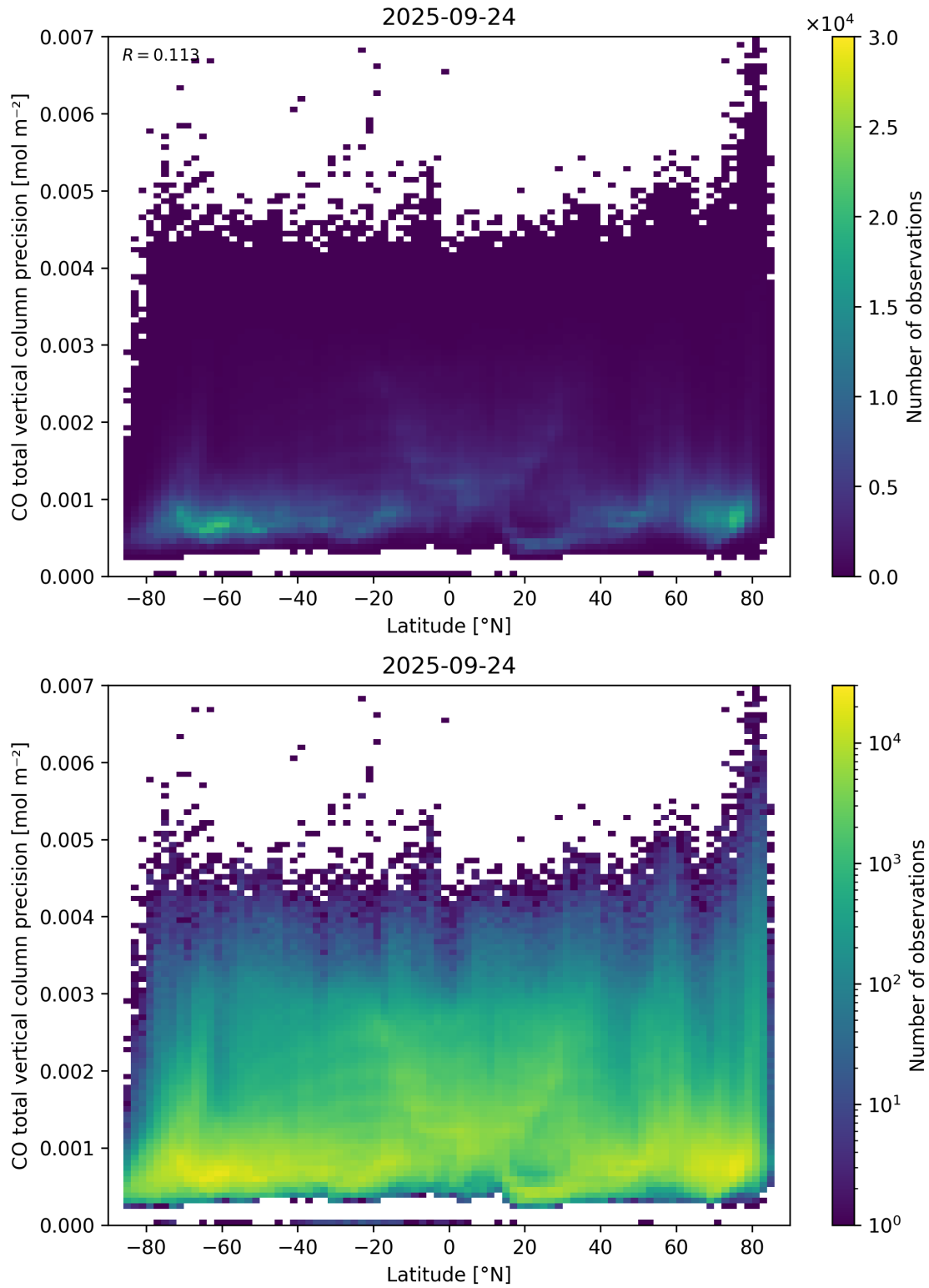
Figure 53: Scatter density plot of “Latitude” against “CO total vertical column precision” for 2025-09-23 to 2025-09-25.
