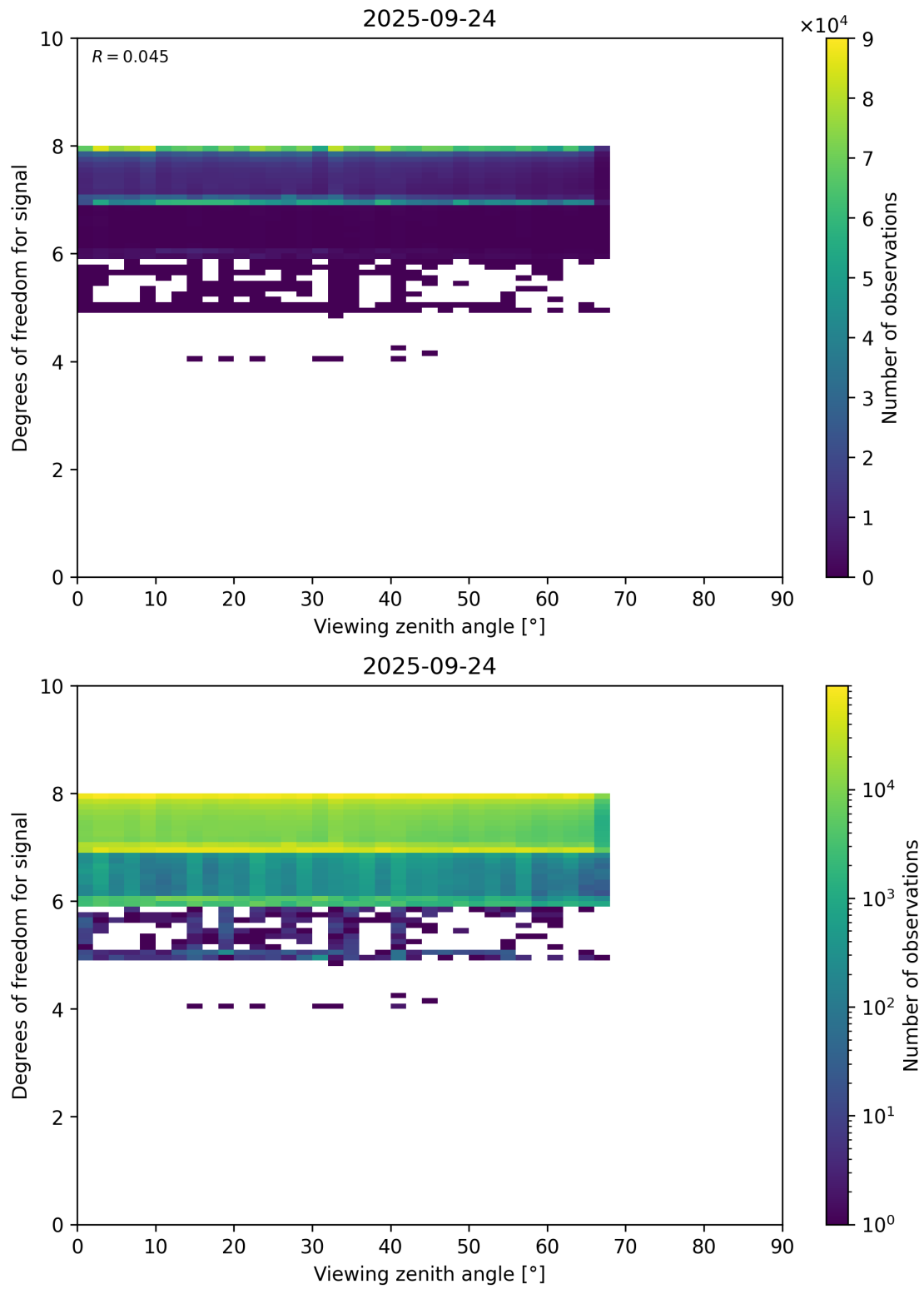
Figure 73: Scatter density plot of “Viewing zenith angle” against “Degrees of freedom for signal” for 2025-09-23 to 2025-09-25.
