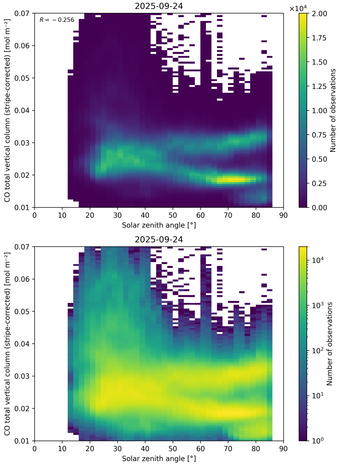
Figure 62: Scatter density plot of “Solar zenith angle” against “CO total vertical column (stripe-corrected)” for 2025-09-23 to 2025-09-25.
