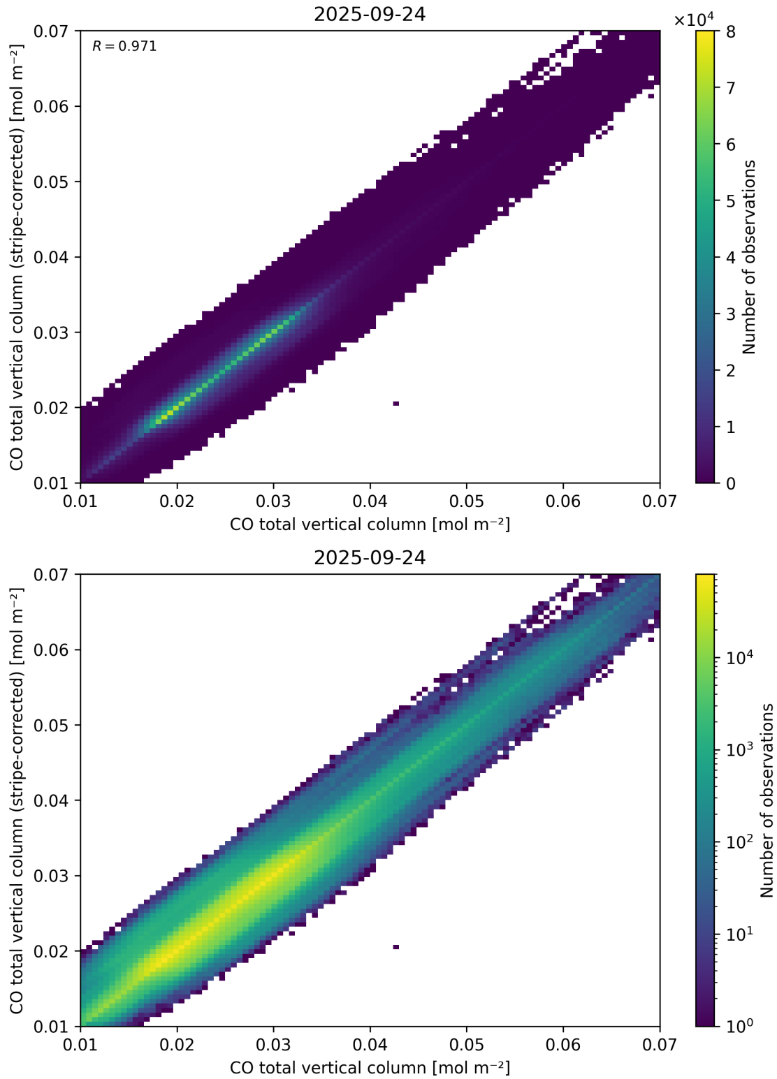
Figure 33: Scatter density plot of “CO total vertical column” against “CO total vertical column (stripe-corrected)” for 2025-09-23 to 2025-09-25.
