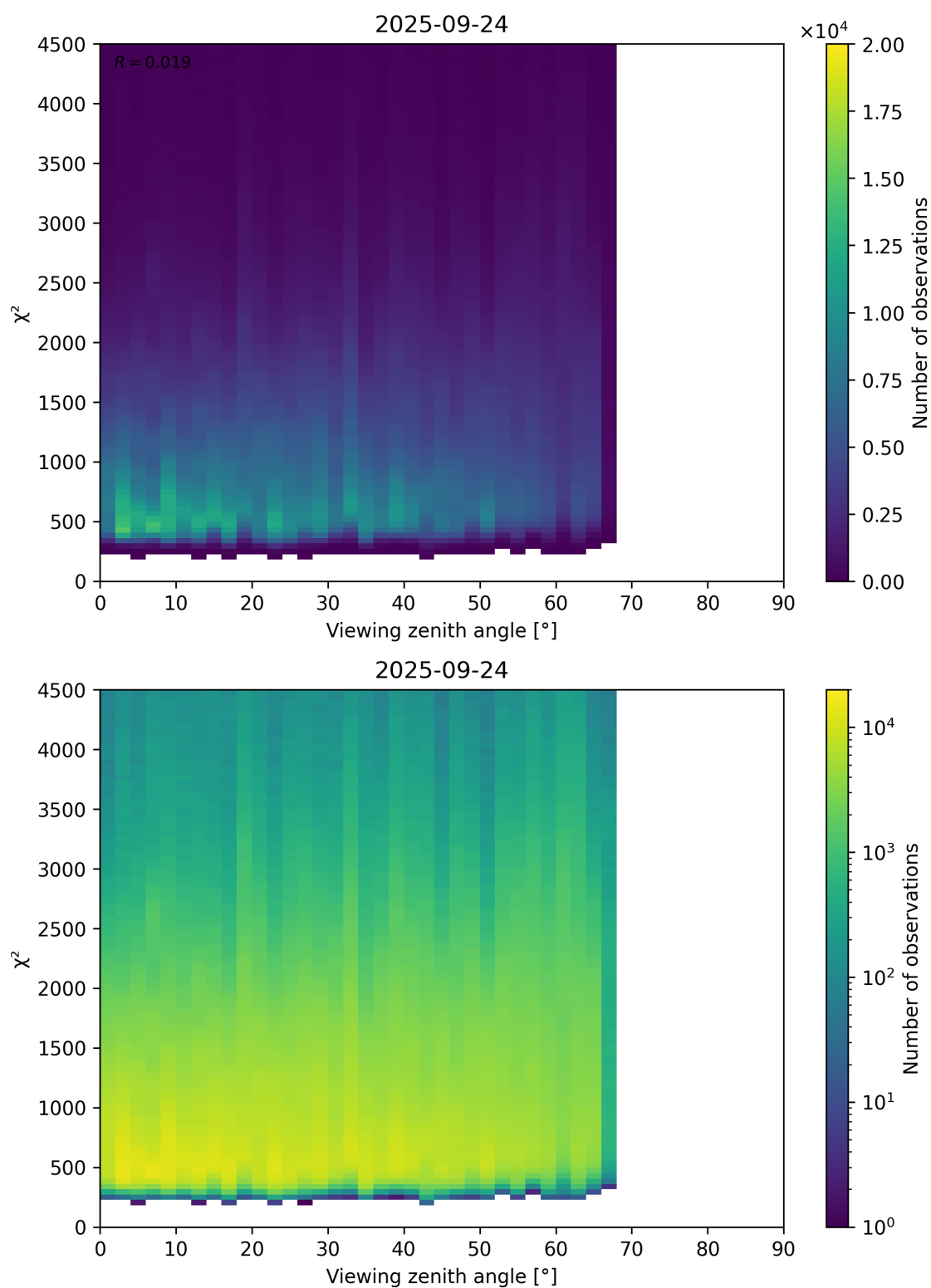
Figure 72: Scatter density plot of “Viewing zenith angle” against “ \chi^2 ” for 2025-09-23 to 2025-09-25.
