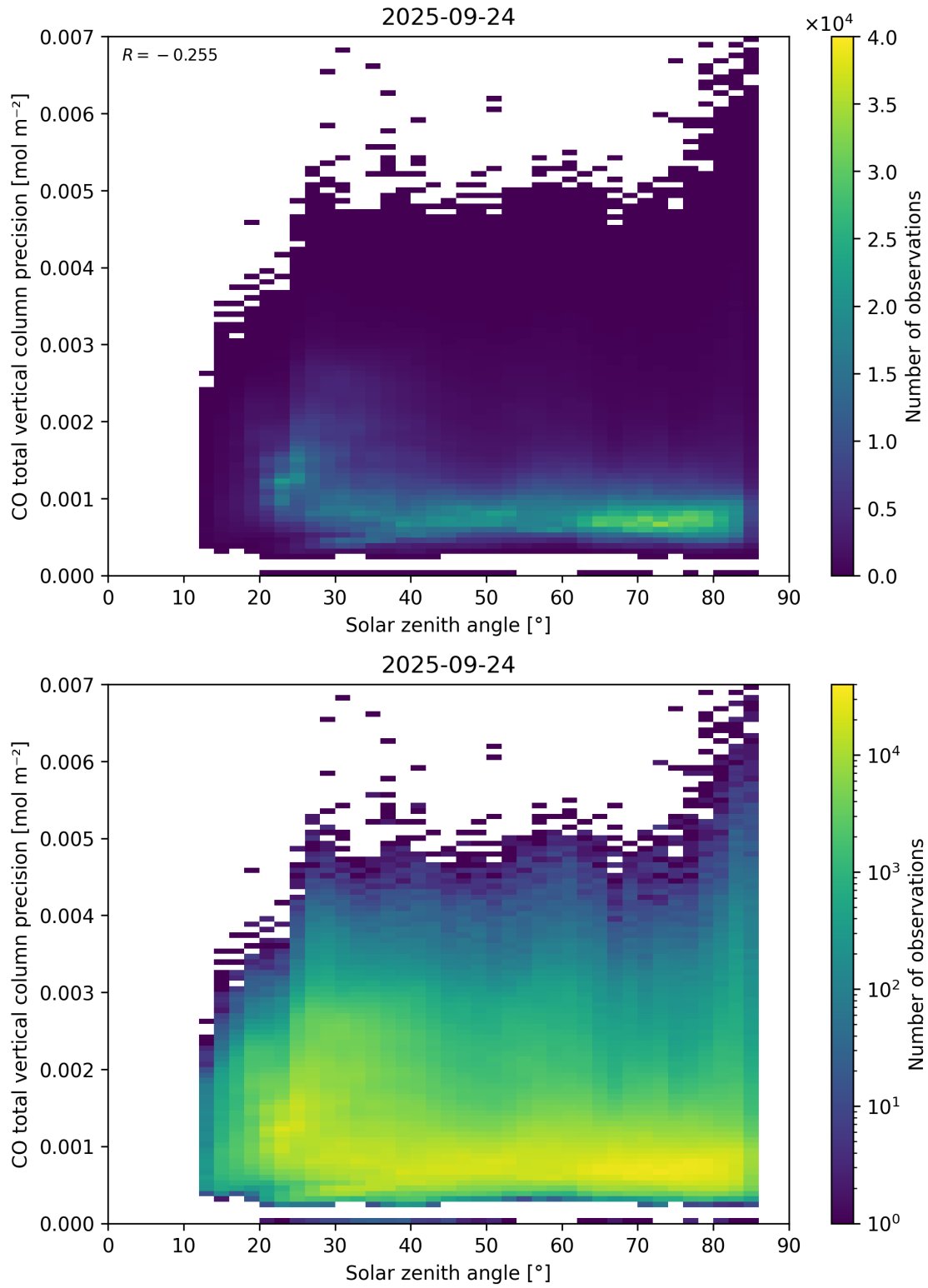
Figure 63: Scatter density plot of “Solar zenith angle” against “CO total vertical column precision” for 2025-09-23 to 2025-09-25.
