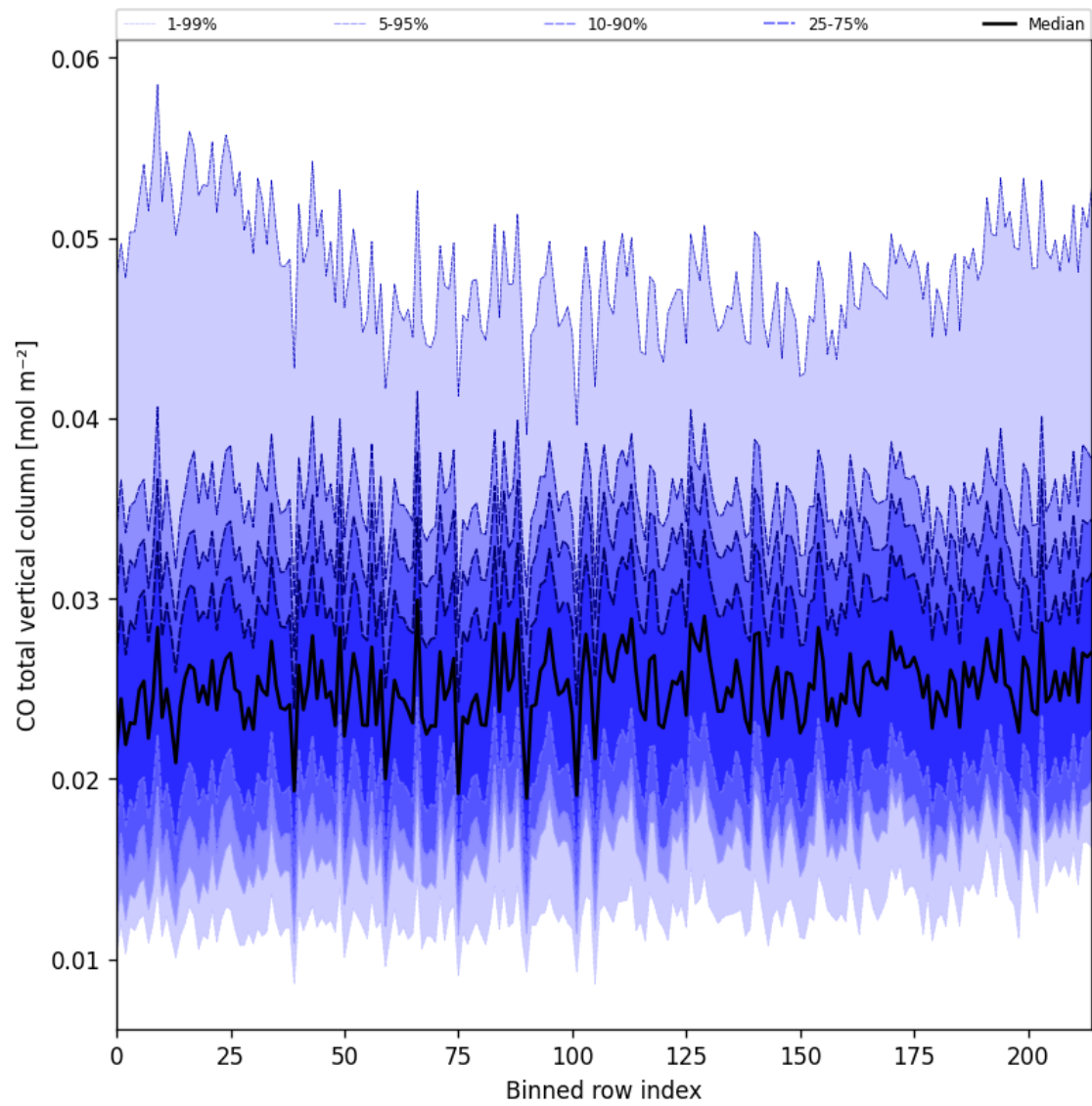
Figure 26: Along track statistics of “CO total vertical column” for 2025-09-23 to 2025-09-25
