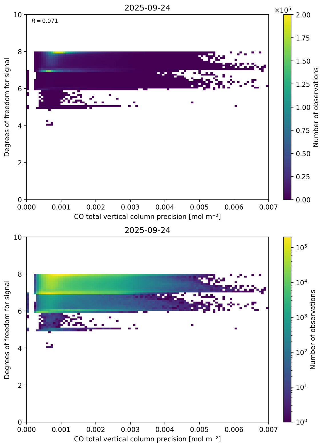
Figure 45: Scatter density plot of “CO total vertical column precision” against “Degrees of freedom for signal” for 2025-09-23 to 2025-09-25.
