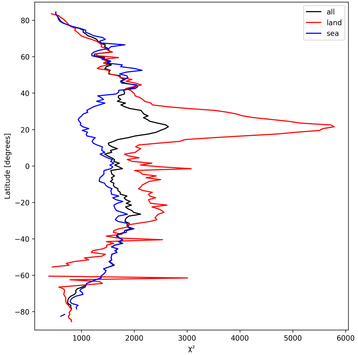
Figure 14: Zonal average of “ \chi^2 ” for 2025-09-23 to 2025-09-25.
