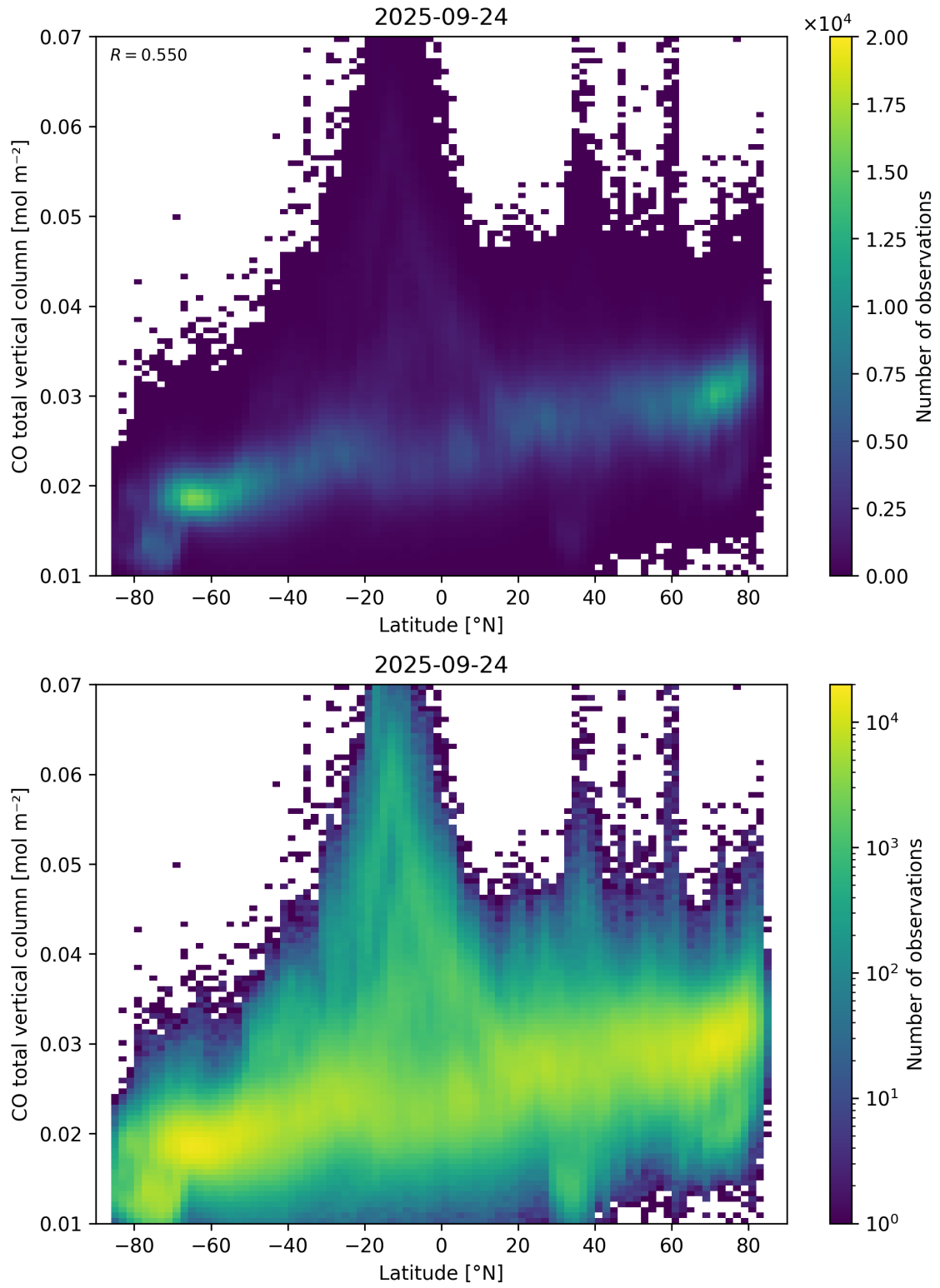
Figure 51: Scatter density plot of “Latitude” against “CO total vertical column” for 2025-09-23 to 2025-09-25.
