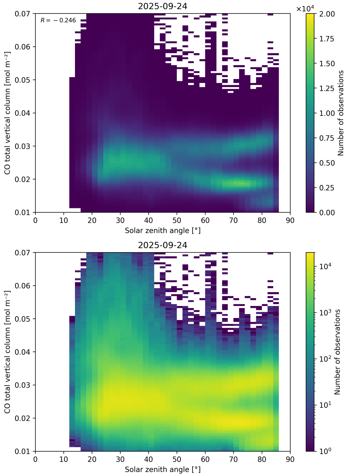
Figure 61: Scatter density plot of “Solar zenith angle” against “CO total vertical column” for 2025-09-23 to 2025-09-25.
