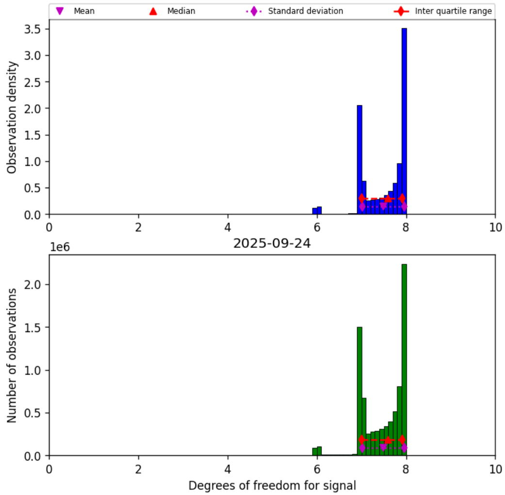
Figure 23: Histogram of “Degrees of freedom for signal” for 2025-09-23 to 2025-09-25
