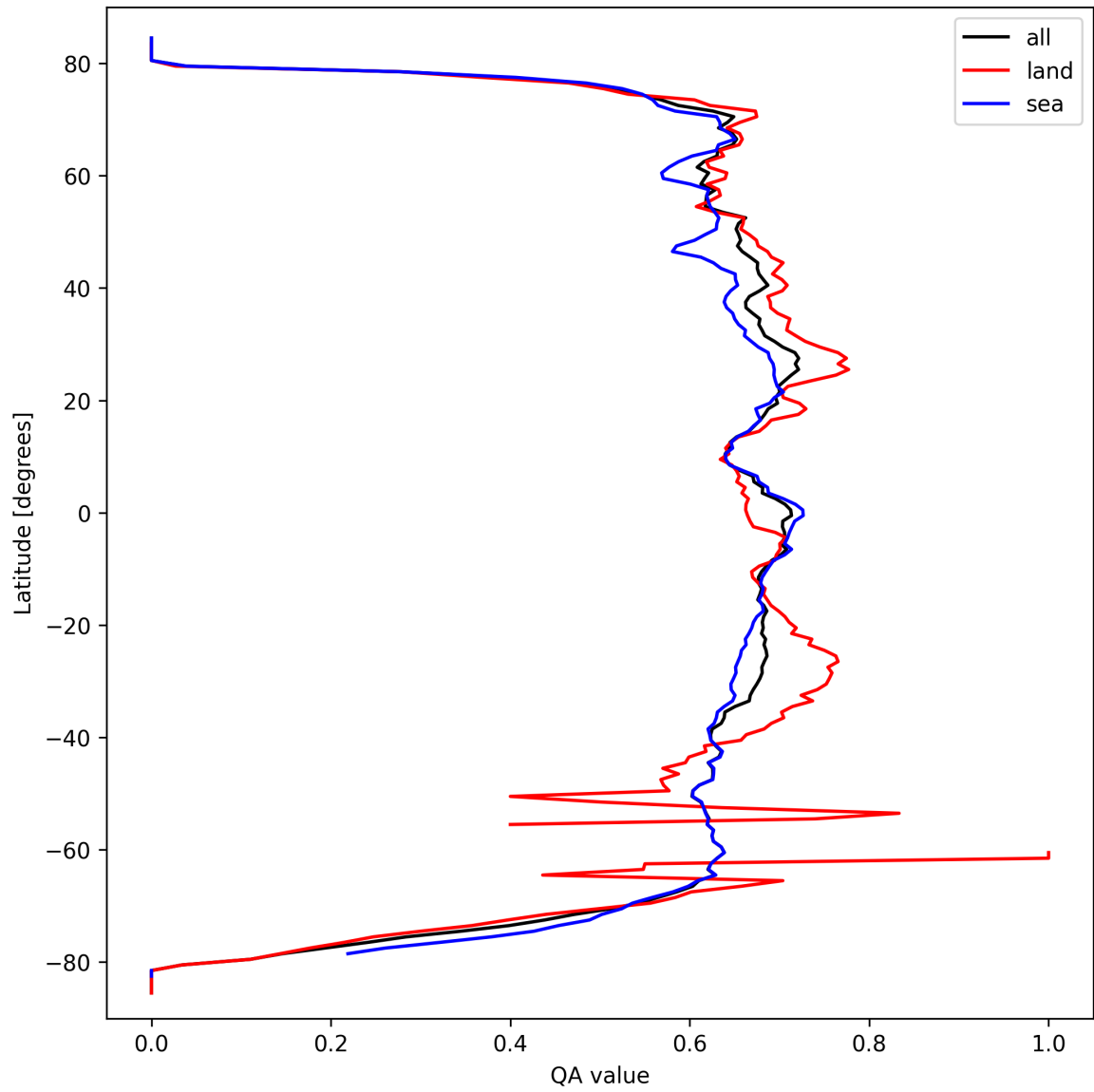
Figure 9: Zonal average of “QA value” for 2025-09-23 to 2025-09-25.
