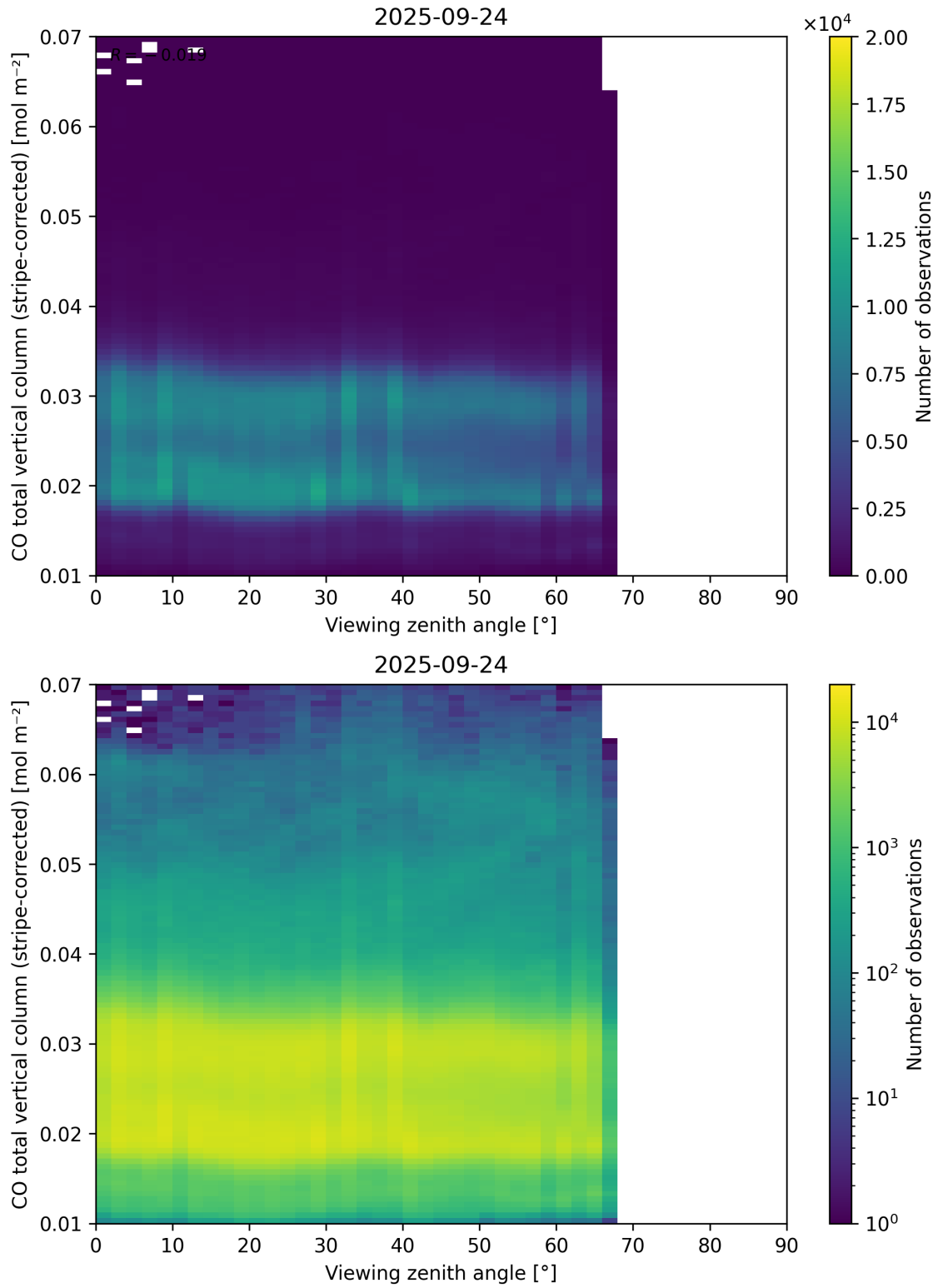
Figure 70: Scatter density plot of “Viewing zenith angle” against “CO total vertical column (stripe-corrected)” for 2025-09-23 to 2025-09-25.
