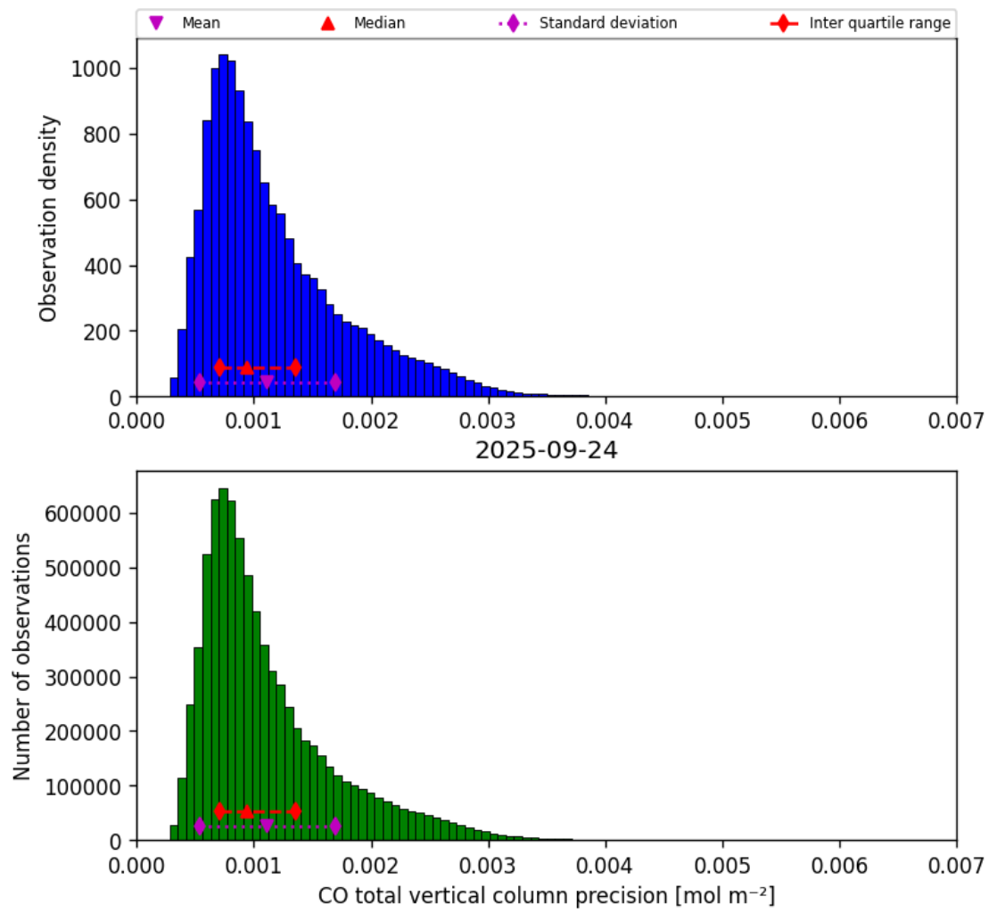
Figure 20: Histogram of “CO total vertical column precision” for 2025-09-23 to 2025-09-25
