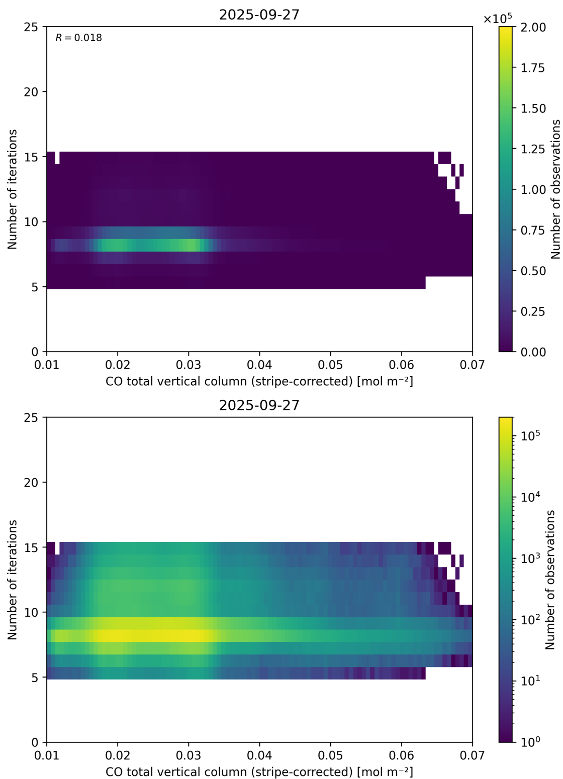
Figure 39: Scatter density plot of “CO total vertical column (stripe-corrected)” against “Number of iterations” for 2025-09-26 to 2025-09-28.
