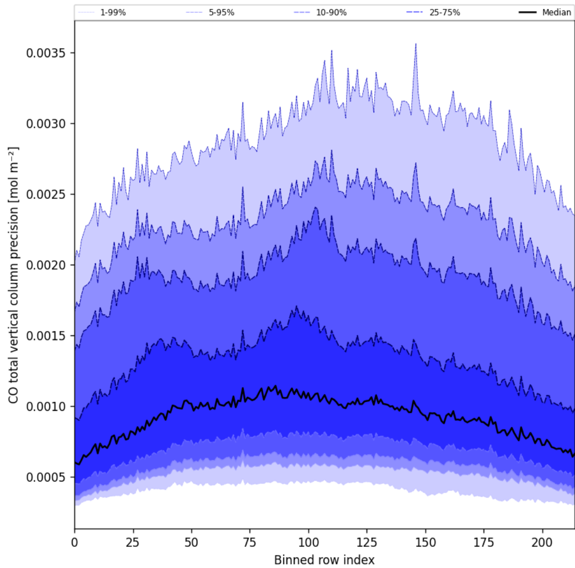
Figure 28: Along track statistics of “CO total vertical column precision” for 2025-09-26 to 2025-09-28
