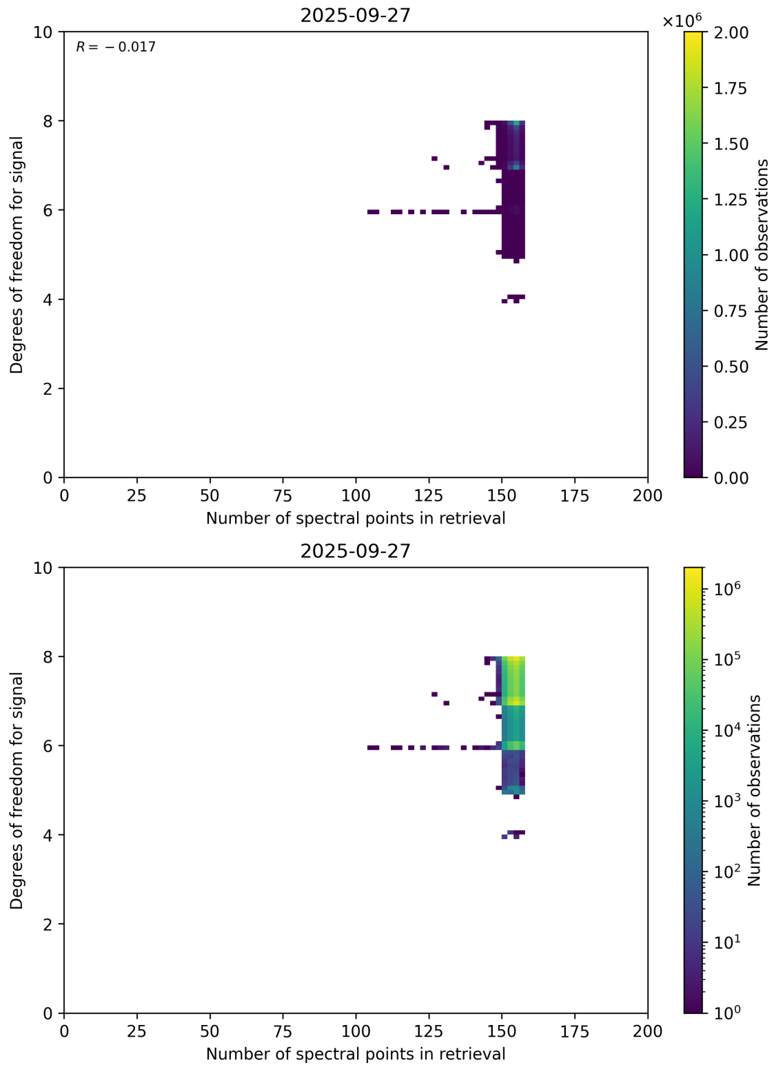
Figure 59: Scatter density plot of “Number of spectral points in retrieval” against “Degrees of freedom for signal” for 2025-09-26 to 2025-09-28.
