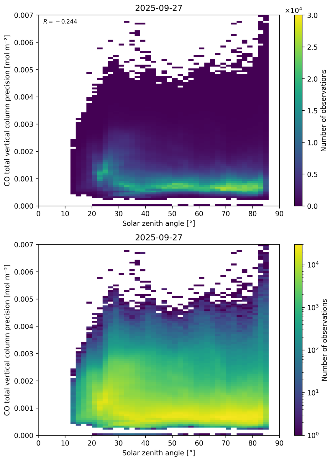
Figure 63: Scatter density plot of “Solar zenith angle” against “CO total vertical column precision” for 2025-09-26 to 2025-09-28.
