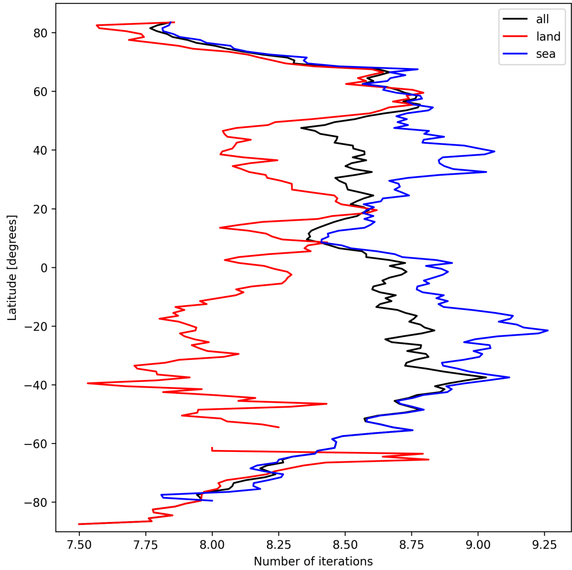
Figure 16: Zonal average of “Number of iterations” for 2025-09-26 to 2025-09-28.
