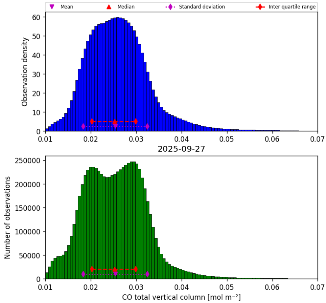
Figure 18: Histogram of “CO total vertical column” for 2025-09-26 to 2025-09-28
