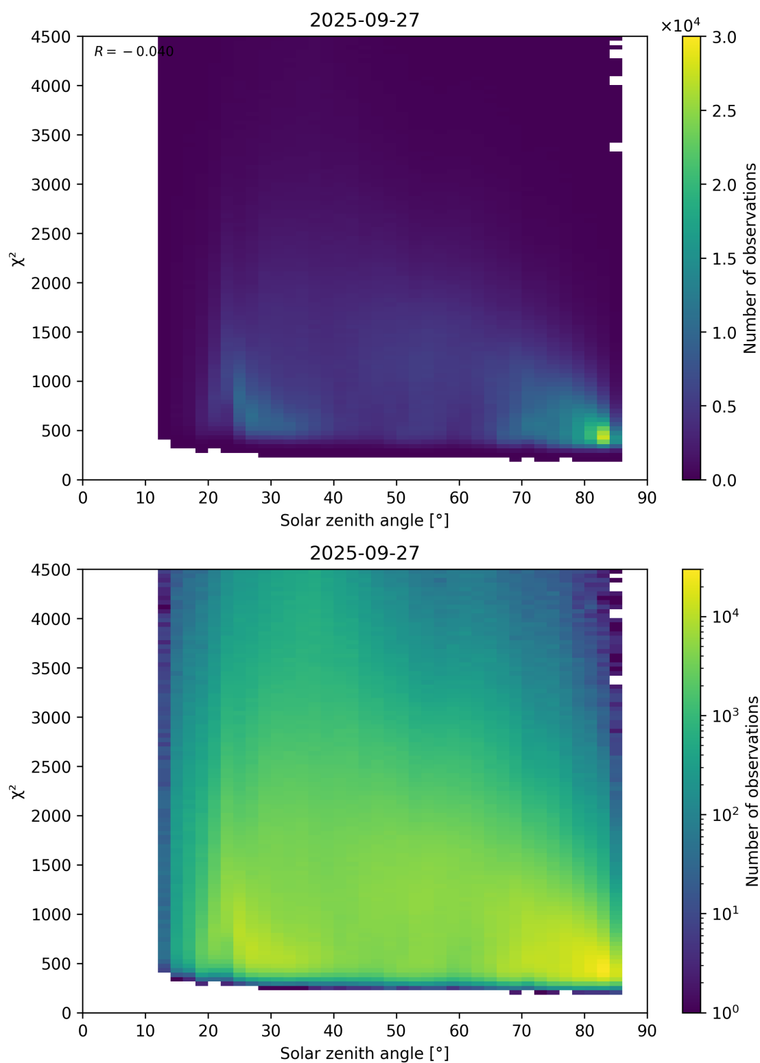
Figure 64: Scatter density plot of “Solar zenith angle” against “ \chi^2 ” for 2025-09-26 to 2025-09-28.
