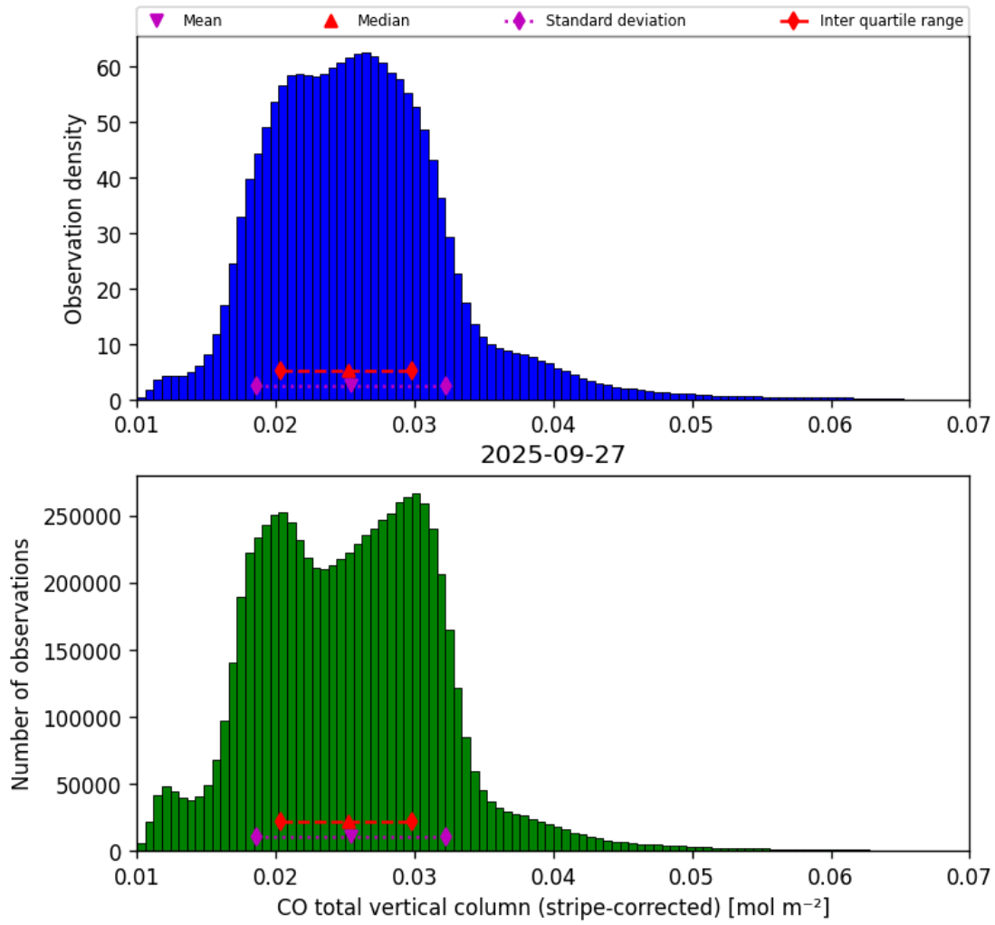
Figure 19: Histogram of “CO total vertical column (stripe-corrected)” for 2025-09-26 to 2025-09-28
