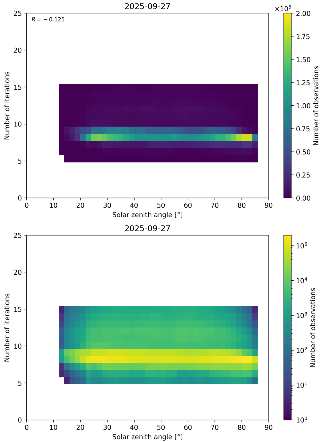
Figure 67: Scatter density plot of “Solar zenith angle” against “Number of iterations” for 2025-09-26 to 2025-09-28.
