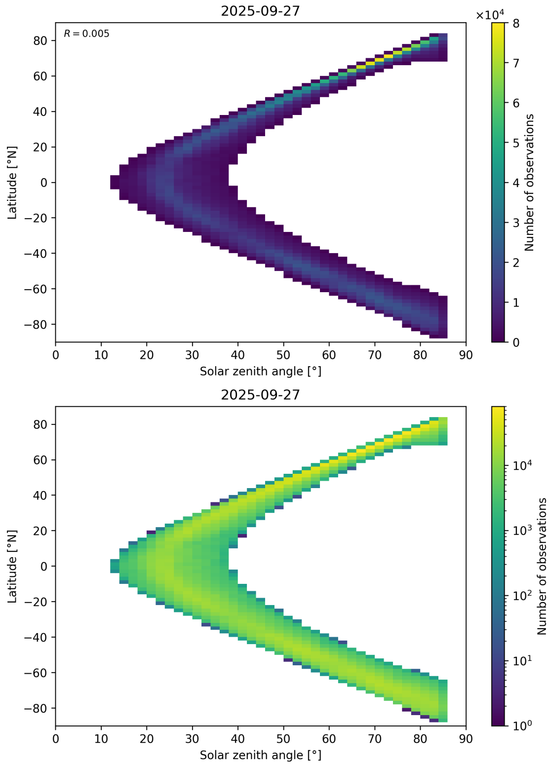
Figure 66: Scatter density plot of “Solar zenith angle” against “Latitude” for 2025-09-26 to 2025-09-28.
