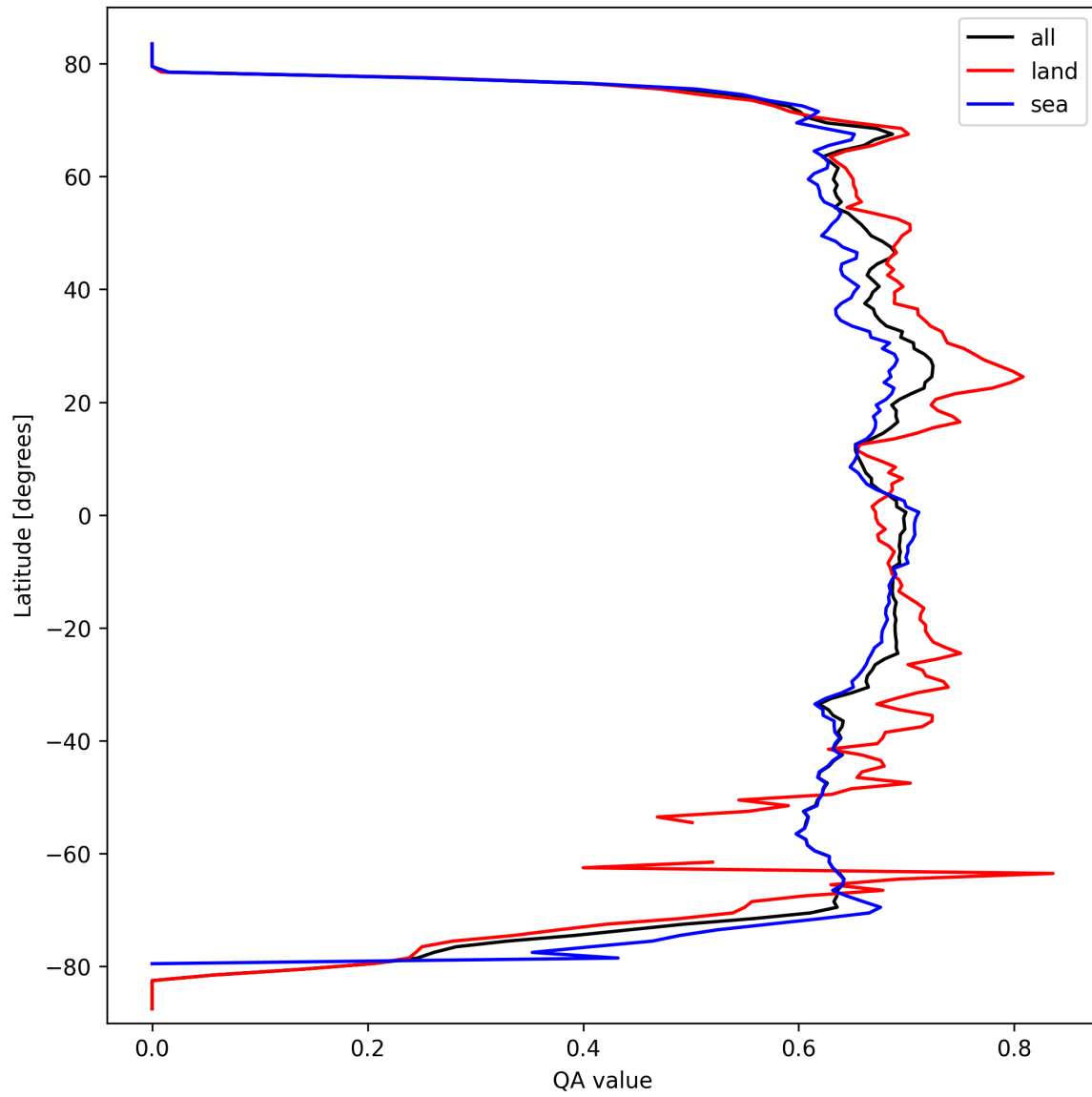
Figure 9: Zonal average of “QA value” for 2025-09-26 to 2025-09-28.
