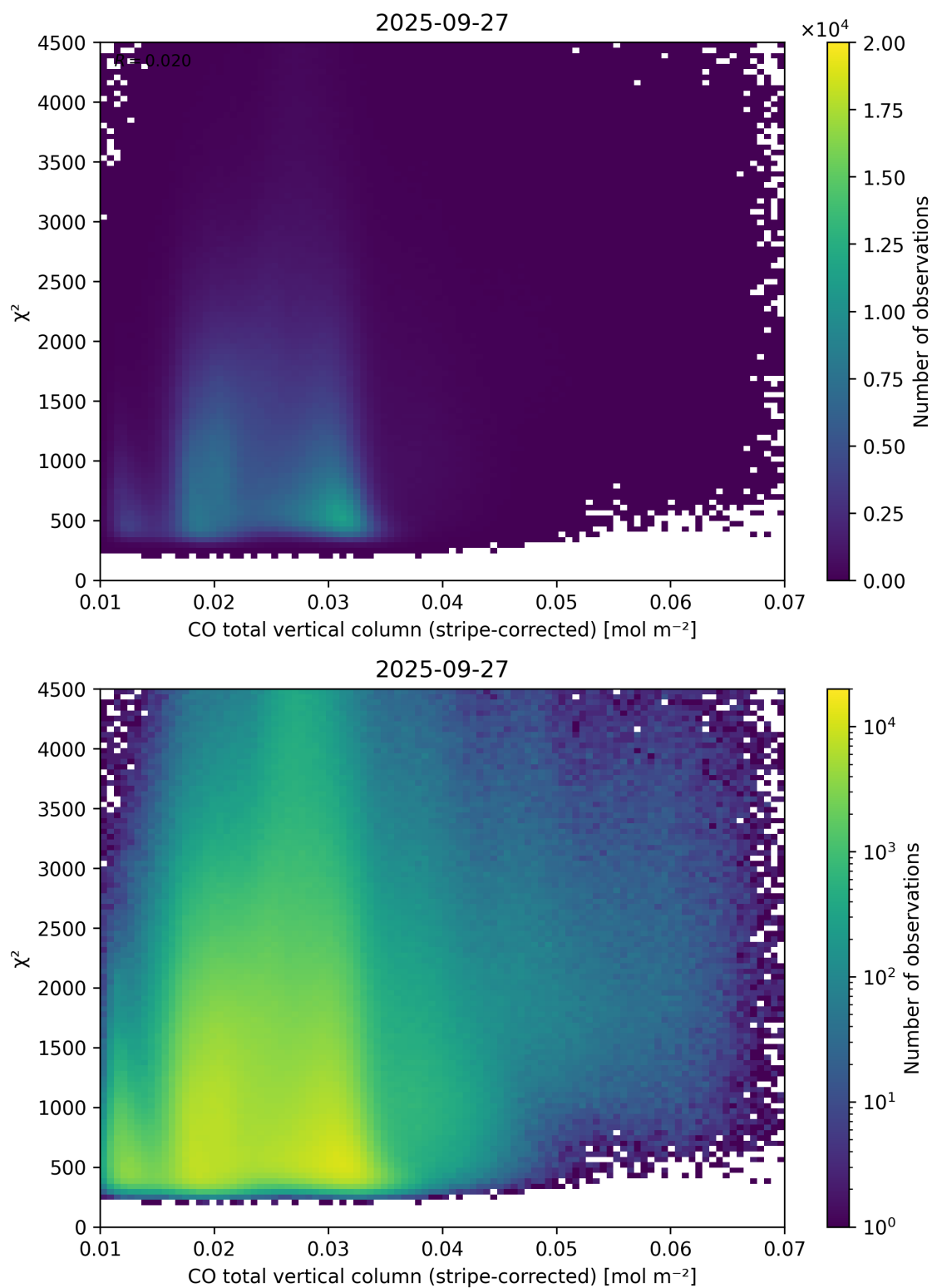
Figure 37: Scatter density plot of “CO total vertical column (stripe-corrected)” against “ \chi^2 ” for 2025-09-26 to 2025-09-28.
