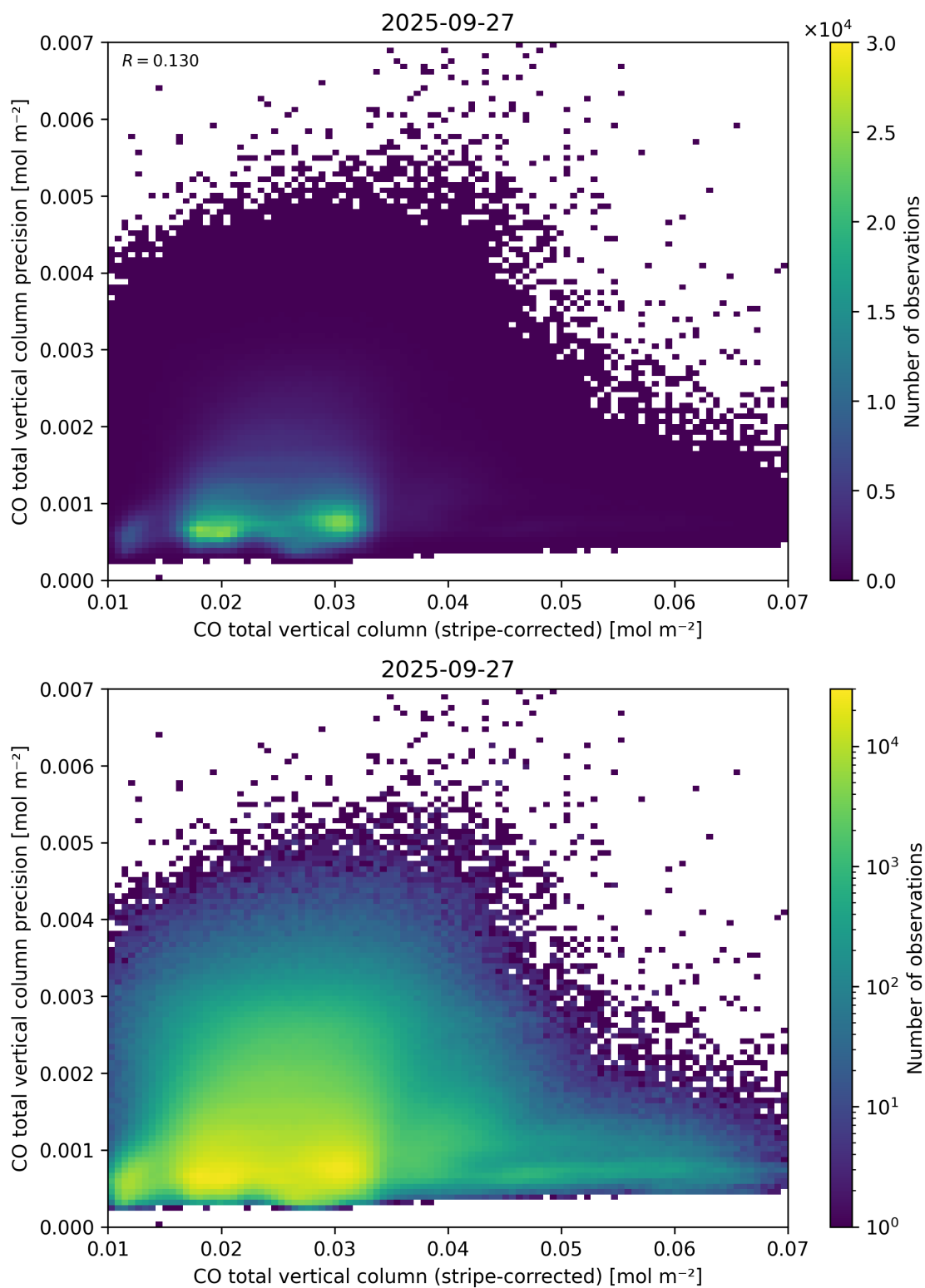
Figure 36: Scatter density plot of “CO total vertical column (stripe-corrected)” against “CO total vertical column precision” for 2025-09-26 to 2025-09-28.
