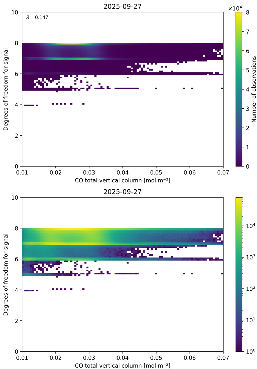
Figure 41: Scatter density plot of “CO total vertical column” against “Degrees of freedom for signal” for 2025-09-26 to 2025-09-28.
