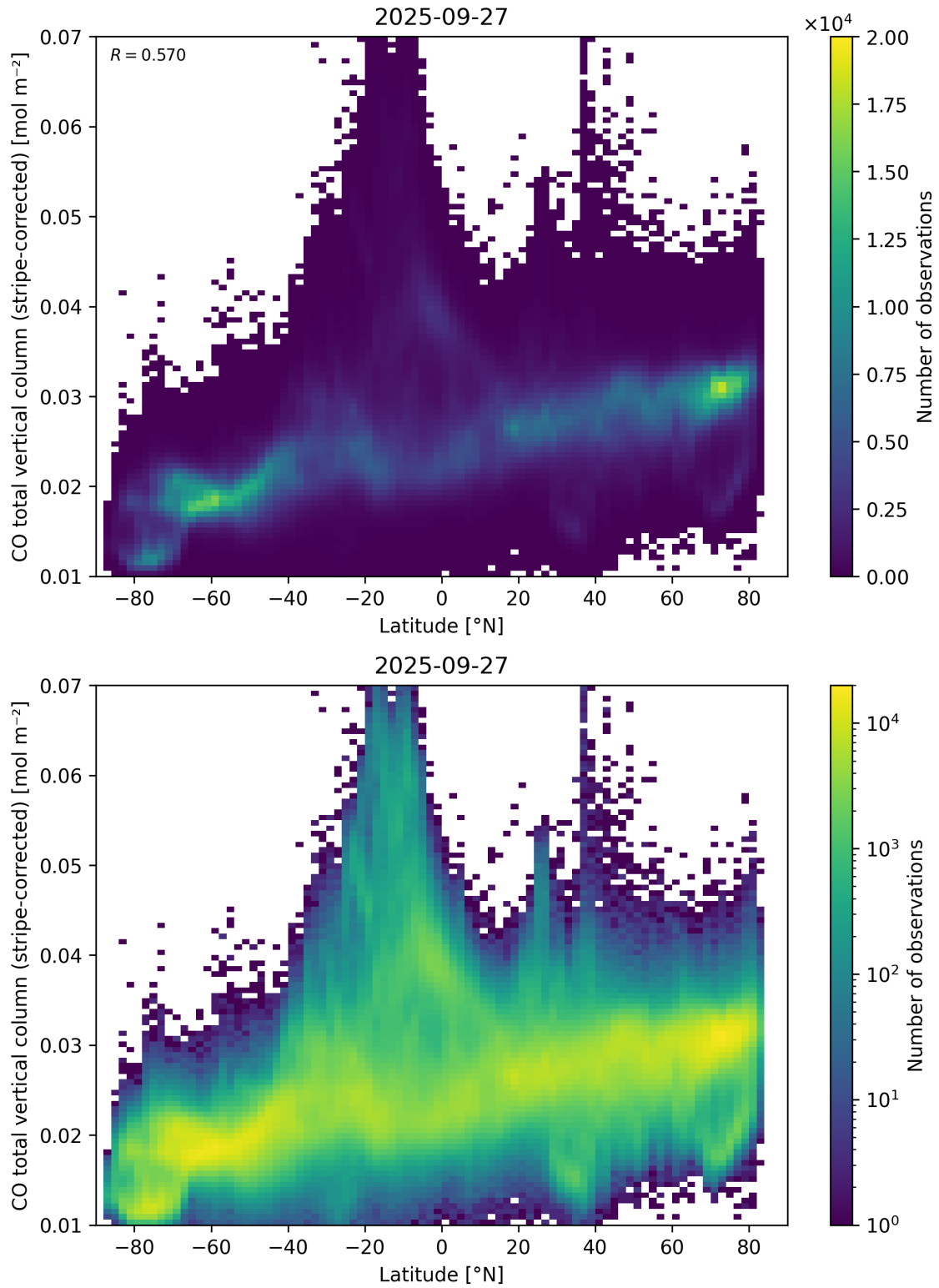
Figure 52: Scatter density plot of “Latitude” against “CO total vertical column (stripe-corrected)” for 2025-09-26 to 2025-09-28.
