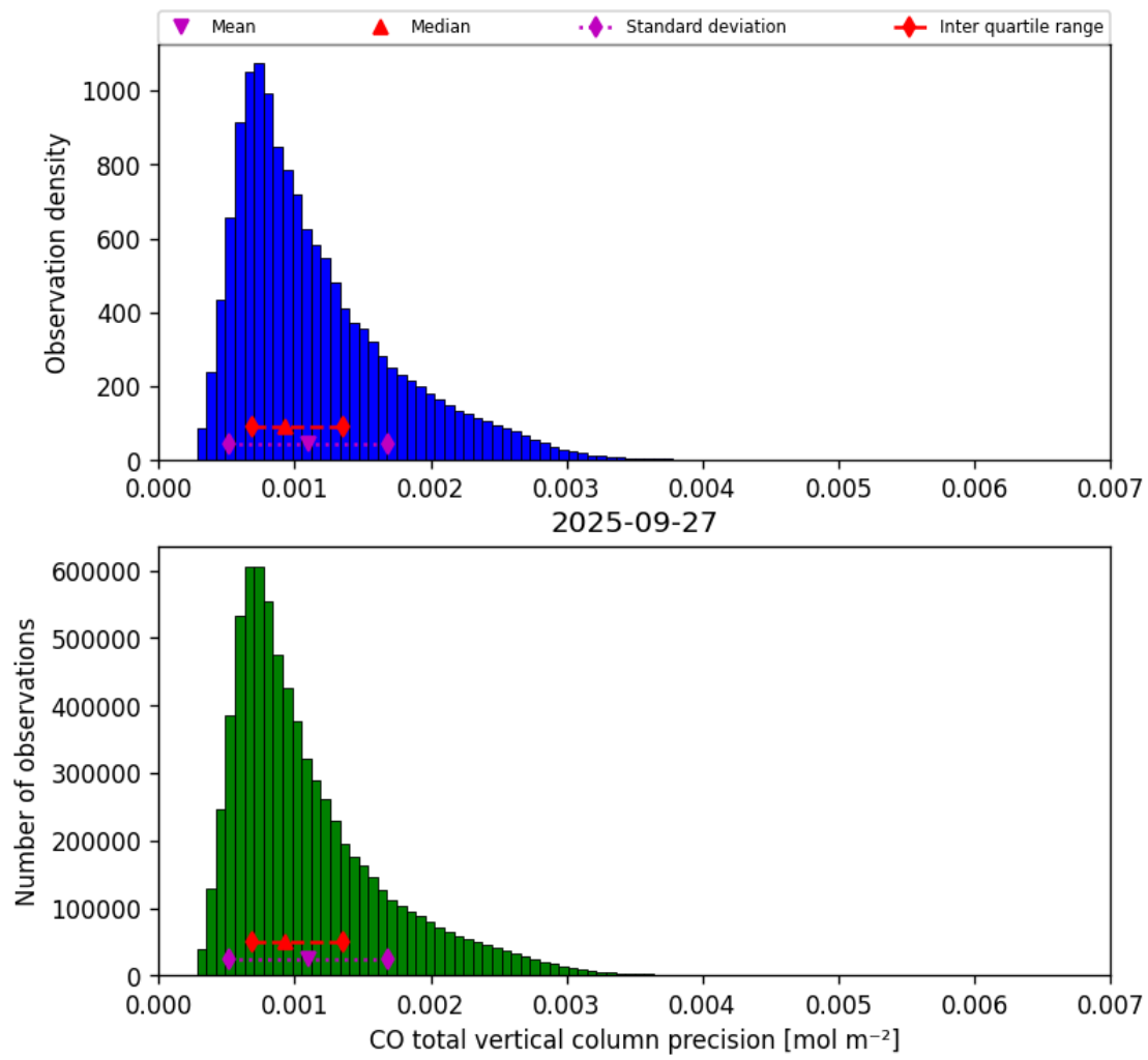
Figure 20: Histogram of “CO total vertical column precision” for 2025-09-26 to 2025-09-28
