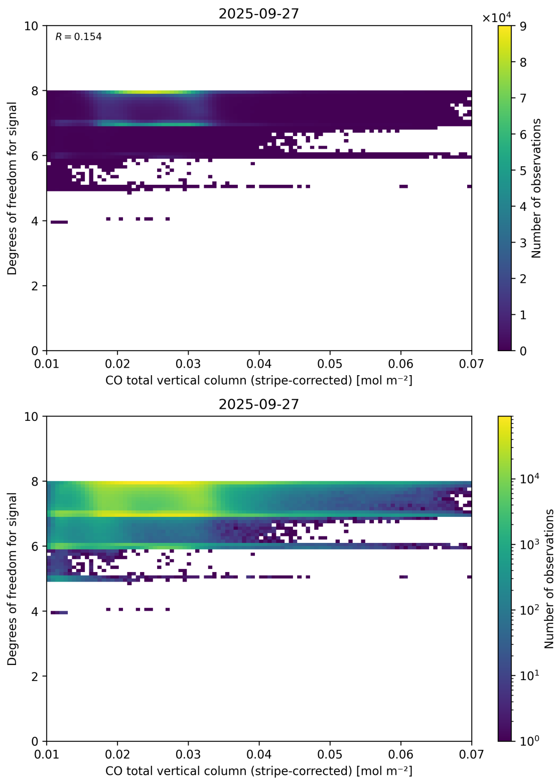
Figure 38: Scatter density plot of “CO total vertical column (stripe-corrected)” against “Degrees of freedom for signal” for 2025-09-26 to 2025-09-28.
