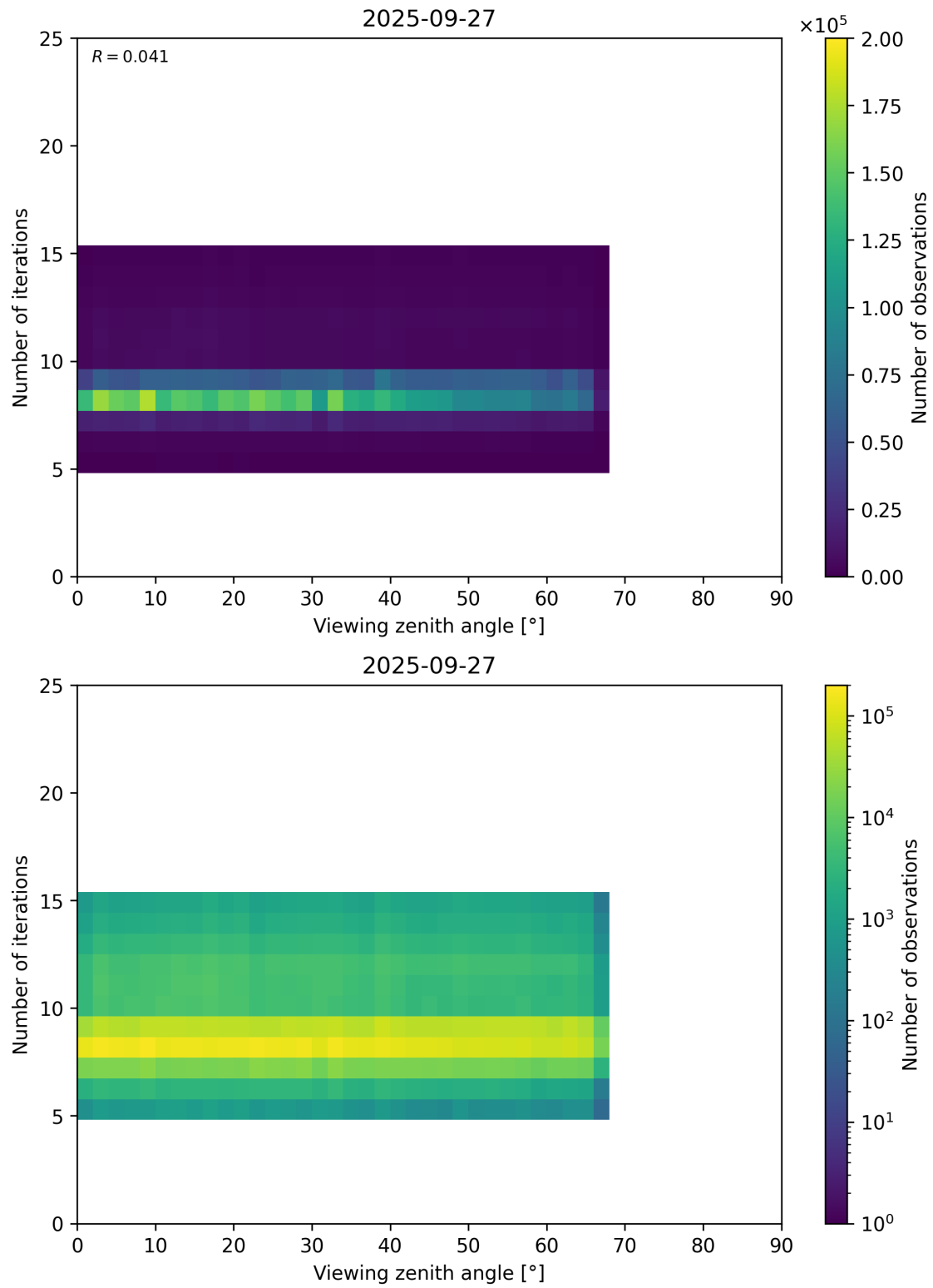
Figure 75: Scatter density plot of “Viewing zenith angle” against “Number of iterations” for 2025-09-26 to 2025-09-28.
