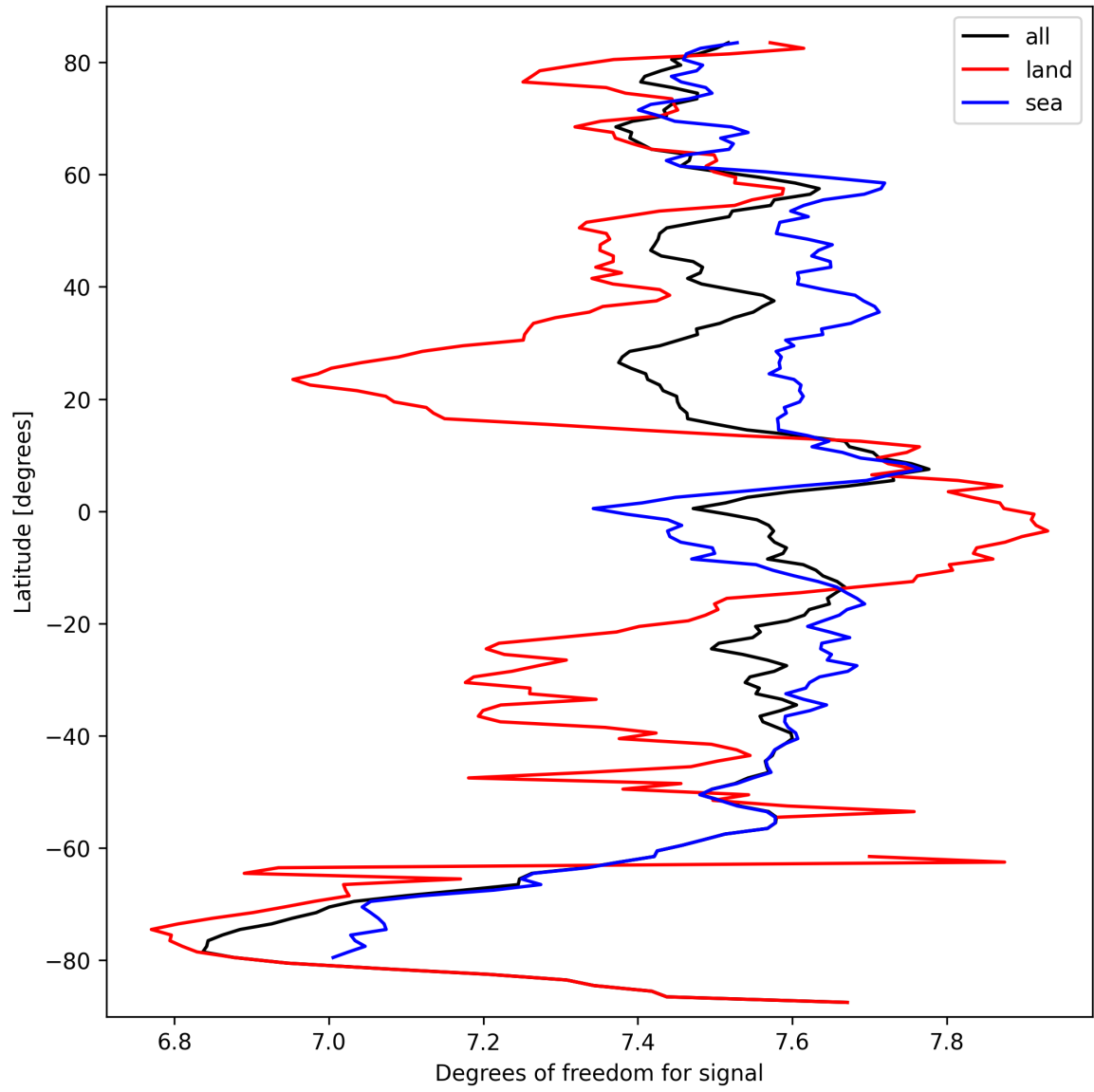
Figure 15: Zonal average of “Degrees of freedom for signal” for 2025-09-26 to 2025-09-28.
