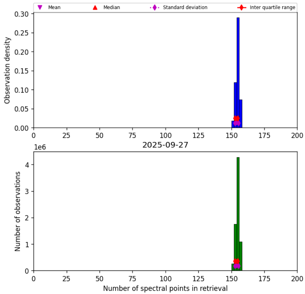
Figure 21: Histogram of “Number of spectral points in retrieval” for 2025-09-26 to 2025-09-28
