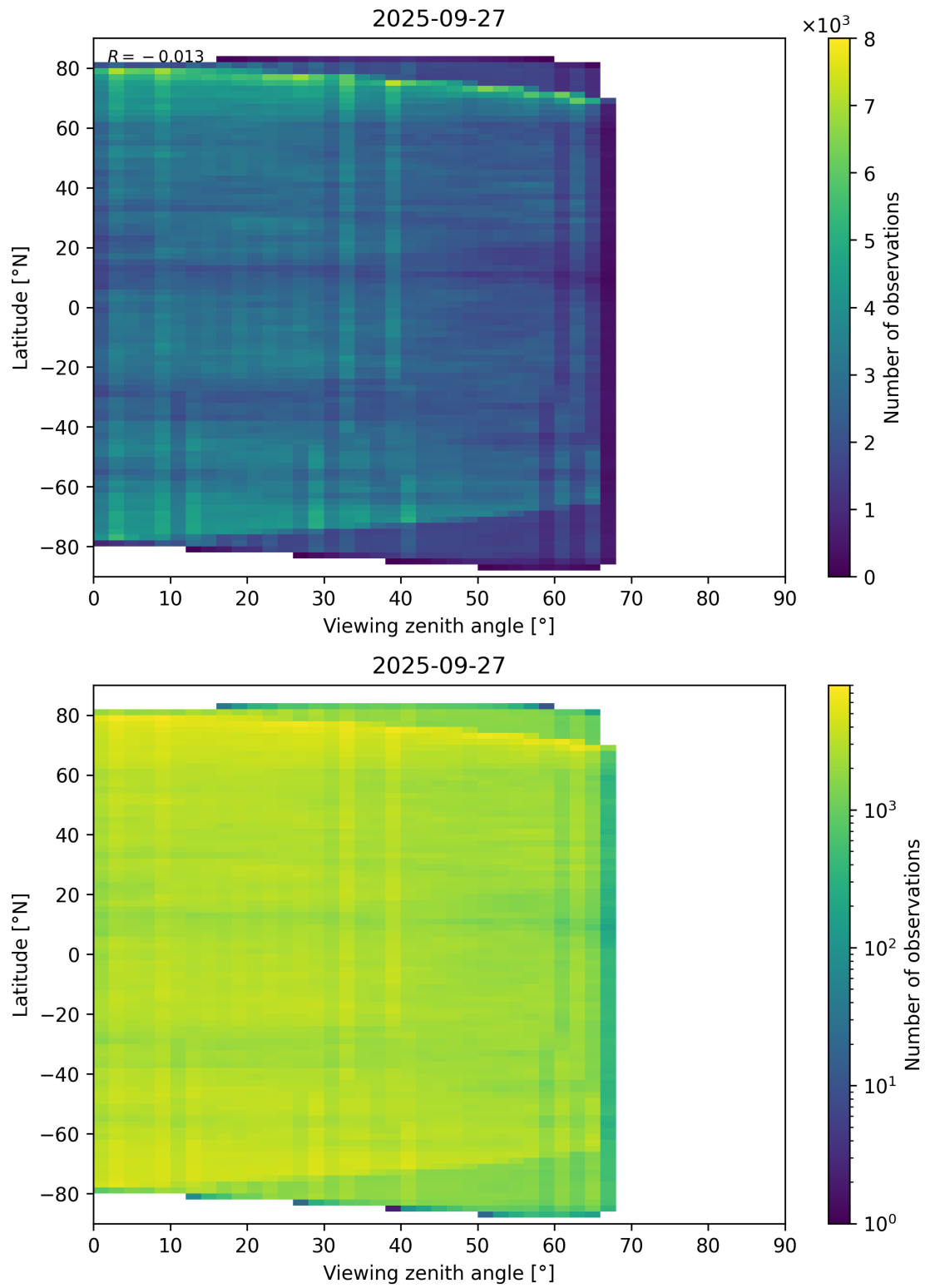
Figure 74: Scatter density plot of “Viewing zenith angle” against “Latitude” for 2025-09-26 to 2025-09-28.
