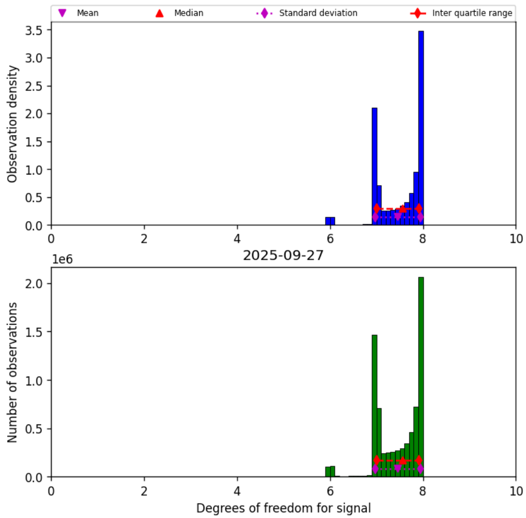
Figure 23: Histogram of “Degrees of freedom for signal” for 2025-09-26 to 2025-09-28
