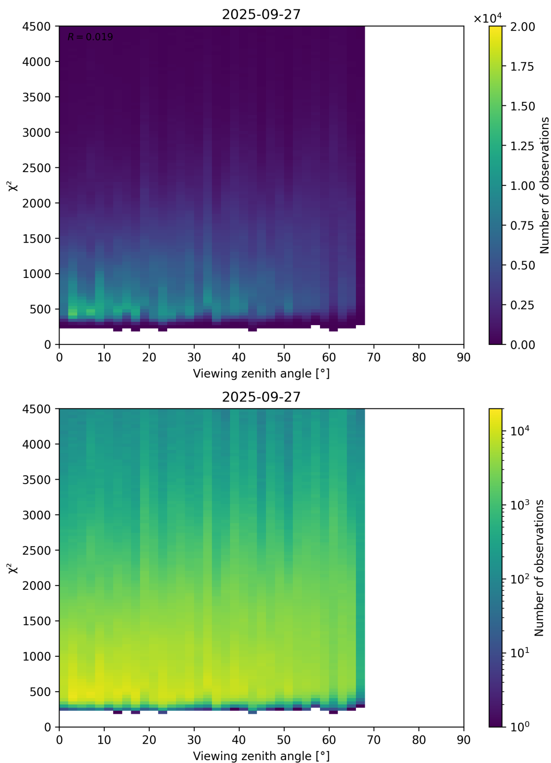
Figure 72: Scatter density plot of “Viewing zenith angle” against “ \chi^2 ” for 2025-09-26 to 2025-09-28.
