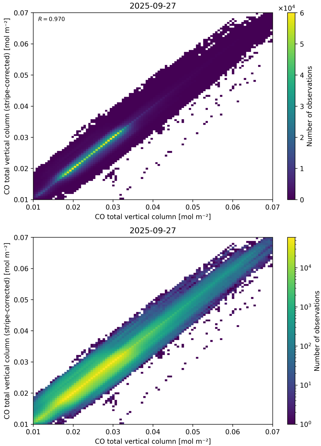
Figure 33: Scatter density plot of “CO total vertical column” against “CO total vertical column (stripe-corrected)” for 2025-09-26 to 2025-09-28.
