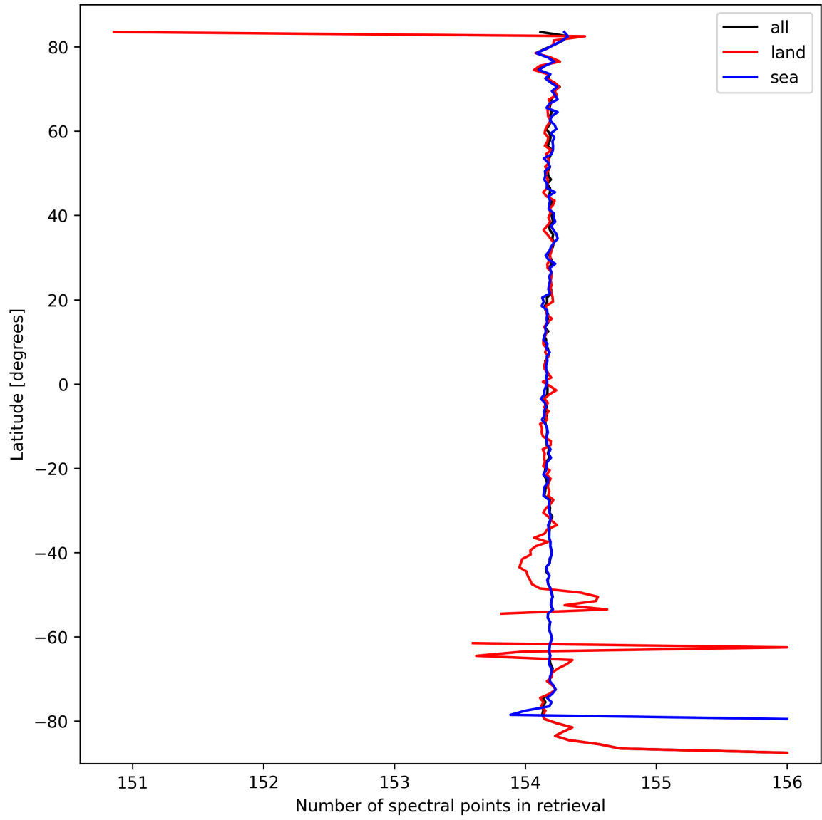
Figure 13: Zonal average of “Number of spectral points in retrieval” for 2025-09-26 to 2025-09-28.
