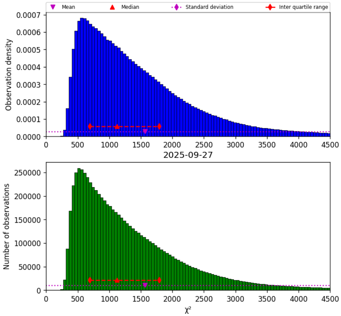
Figure 22: Histogram of " \chi^2 " for 2025-09-26 to 2025-09-28
