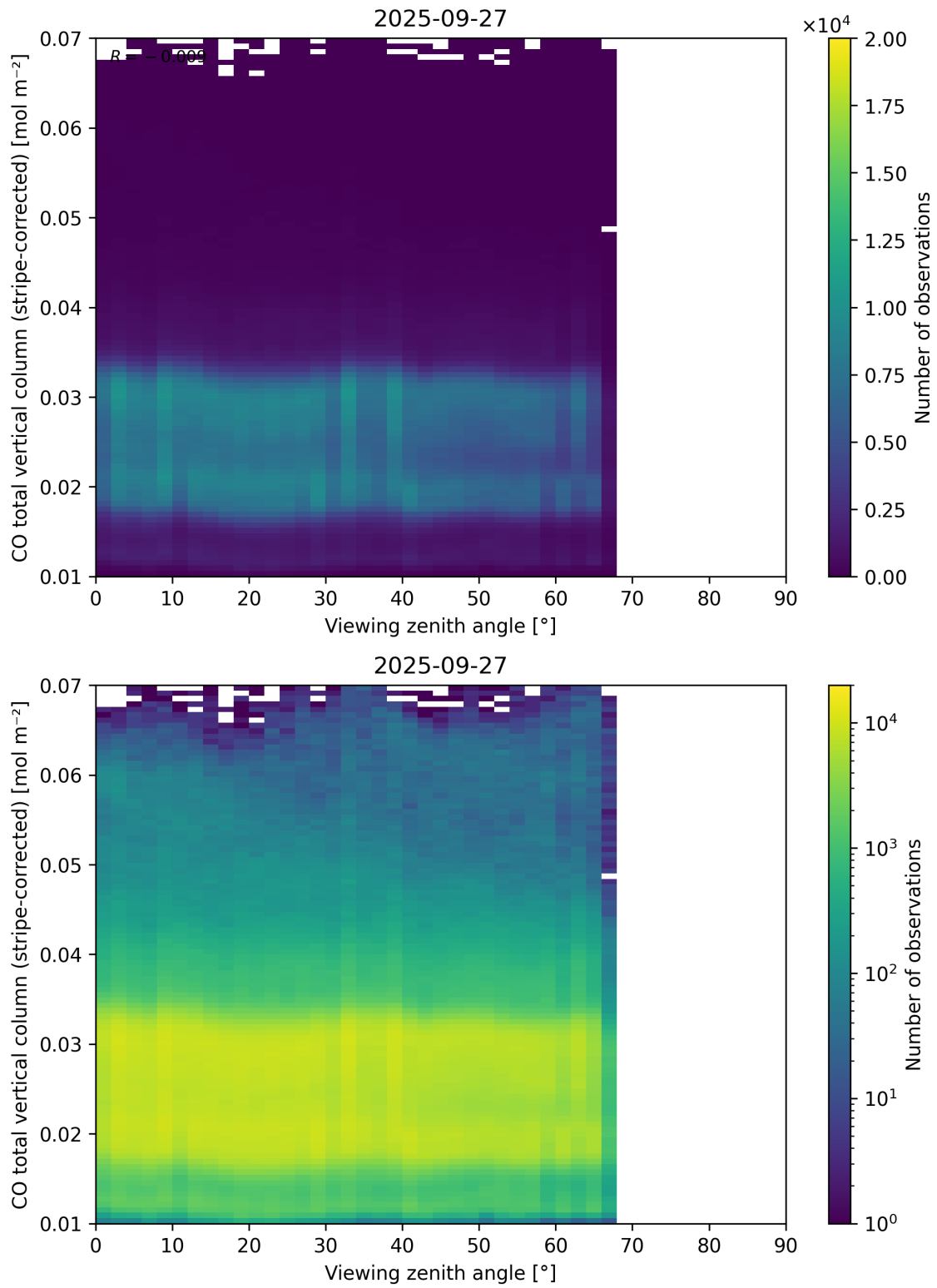
Figure 70: Scatter density plot of “Viewing zenith angle” against “CO total vertical column (stripe-corrected)” for 2025-09-26 to 2025-09-28.
