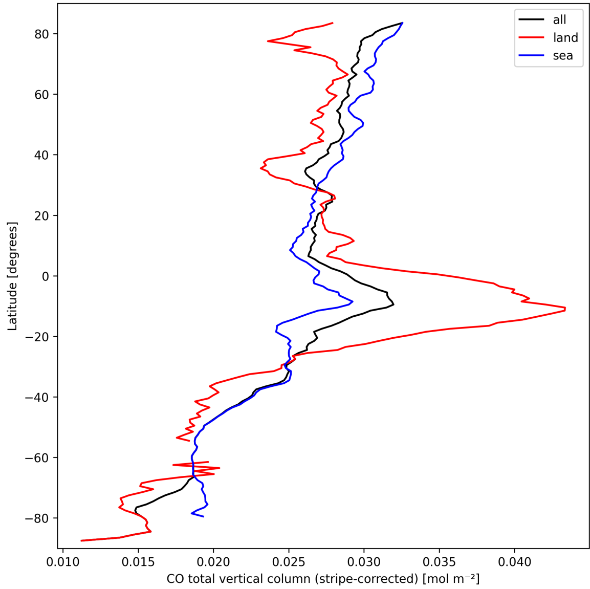
Figure 11: Zonal average of “CO total vertical column (stripe-corrected)” for 2025-09-26 to 2025-09-28.
