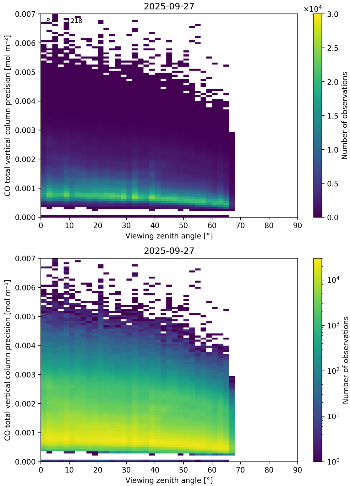
Figure 71: Scatter density plot of “Viewing zenith angle” against “CO total vertical column precision” for 2025-09-26 to 2025-09-28.
