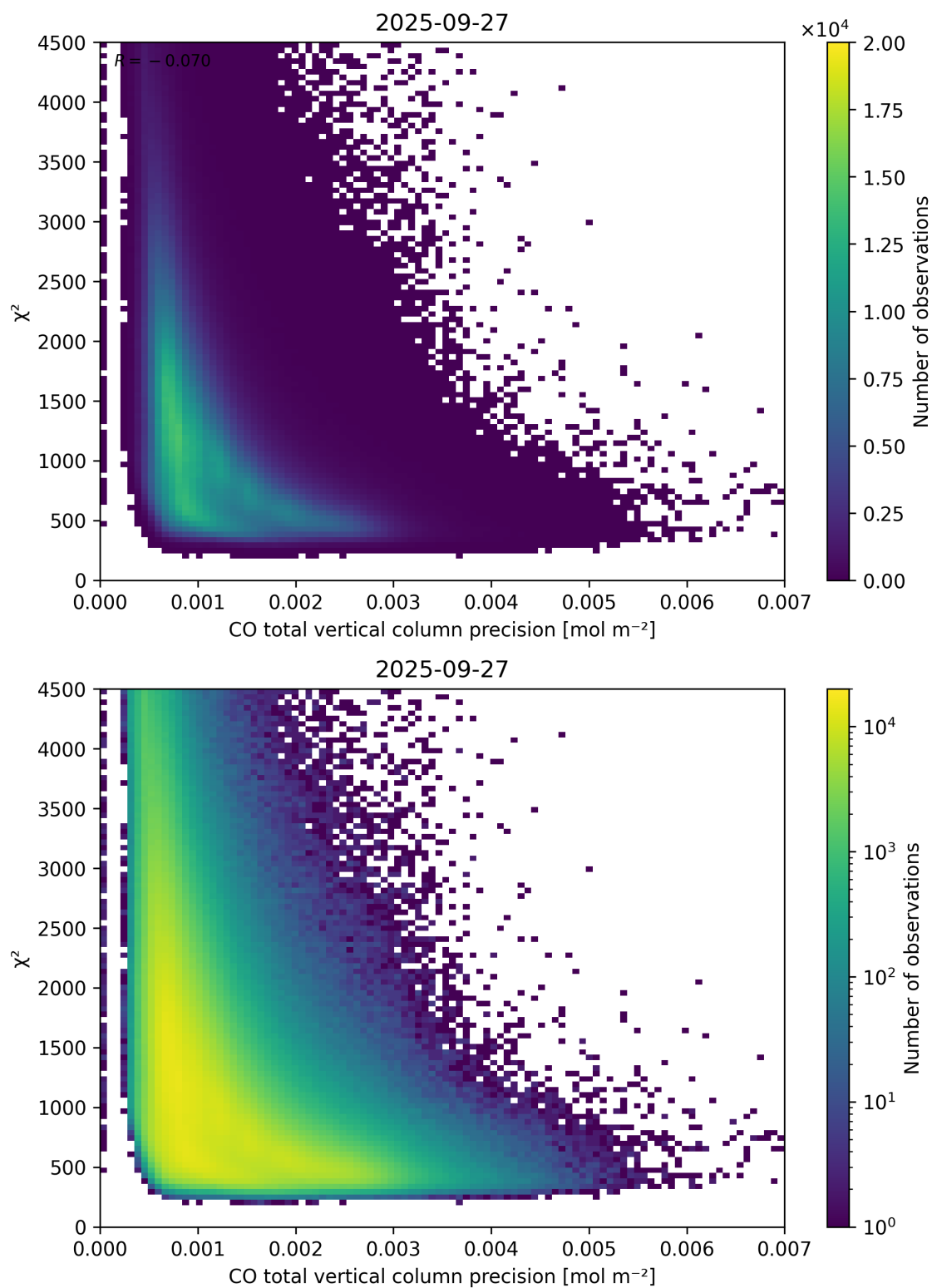
Figure 44: Scatter density plot of “CO total vertical column precision” against “ \chi^2 ” for 2025-09-26 to 2025-09-28.
