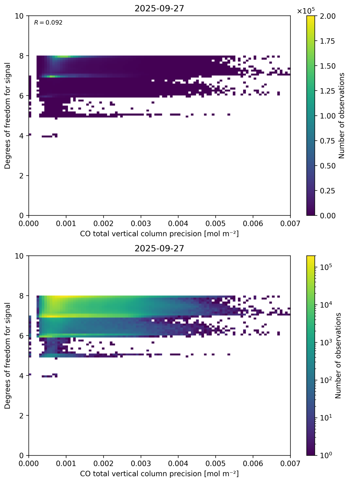
Figure 45: Scatter density plot of “CO total vertical column precision” against “Degrees of freedom for signal” for 2025-09-26 to 2025-09-28.
