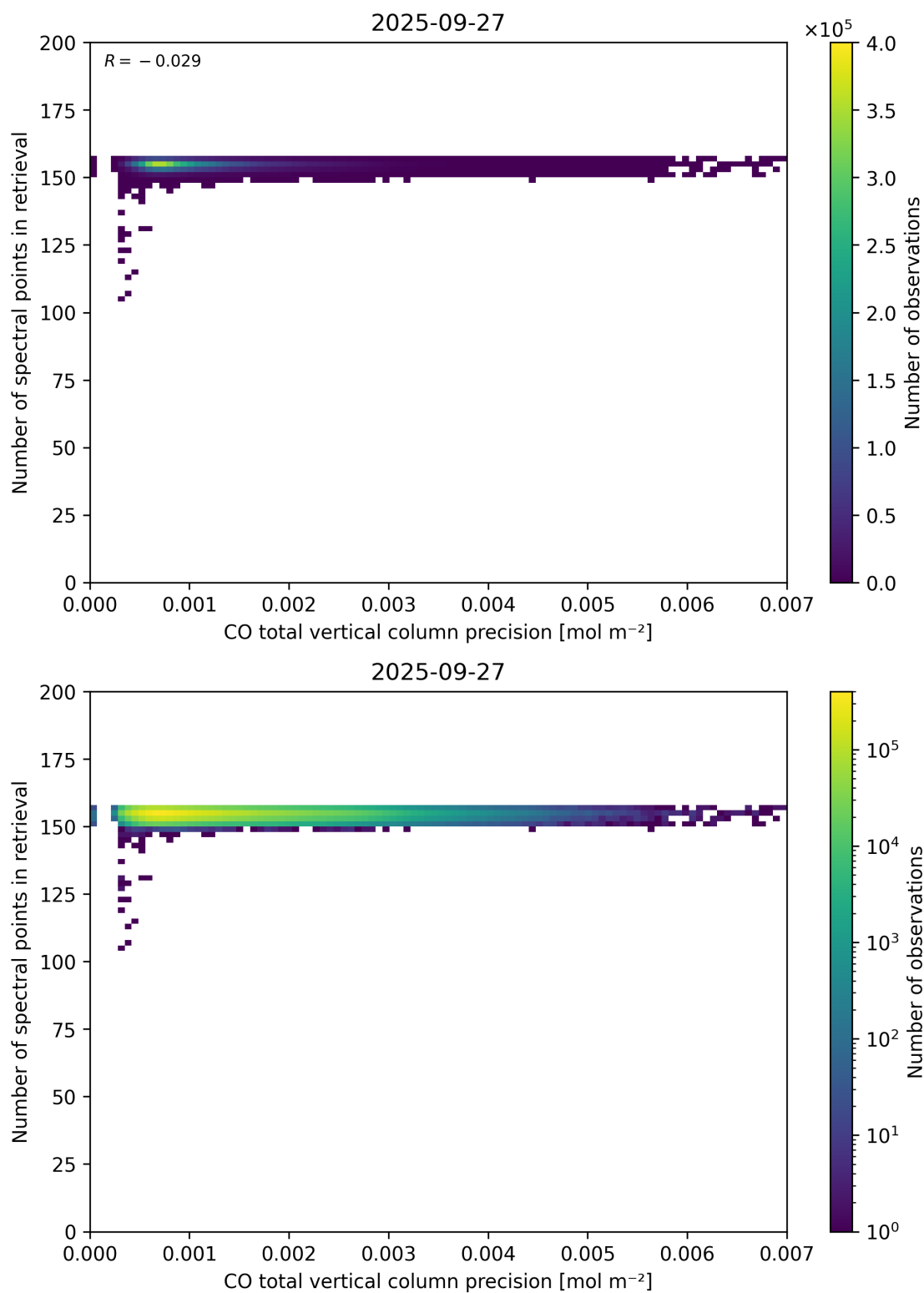
Figure 47: Scatter density plot of “CO total vertical column precision” against “Number of spectral points in retrieval” for 2025-09-26 to 2025-09-28.
