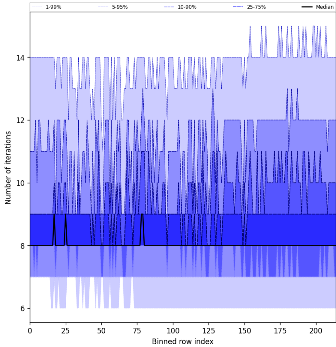
Figure 32: Along track statistics of “Number of iterations” for 2025-09-26 to 2025-09-28
