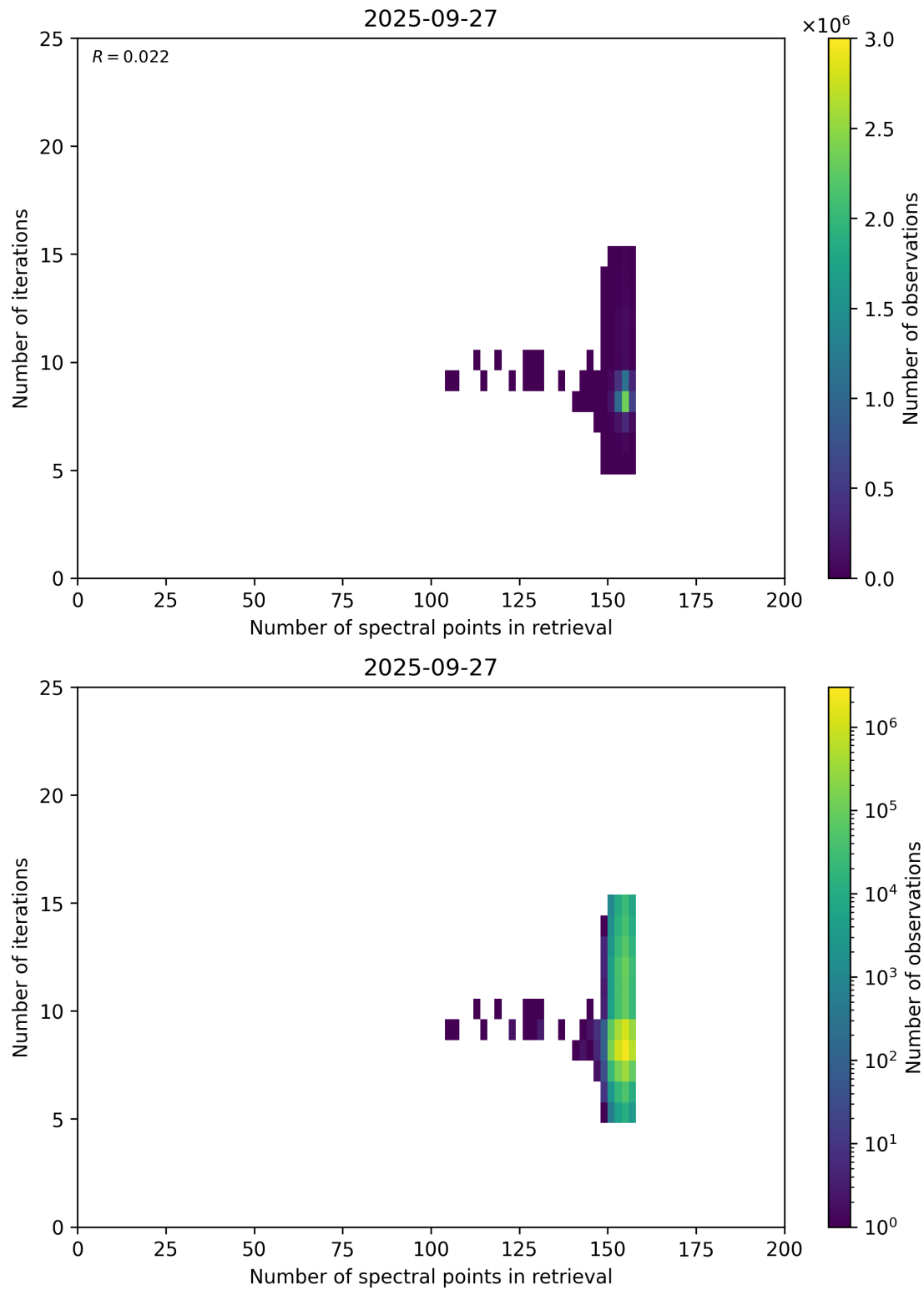
Figure 60: Scatter density plot of “Number of spectral points in retrieval” against “Number of iterations” for 2025-09-26 to 2025-09-28.
