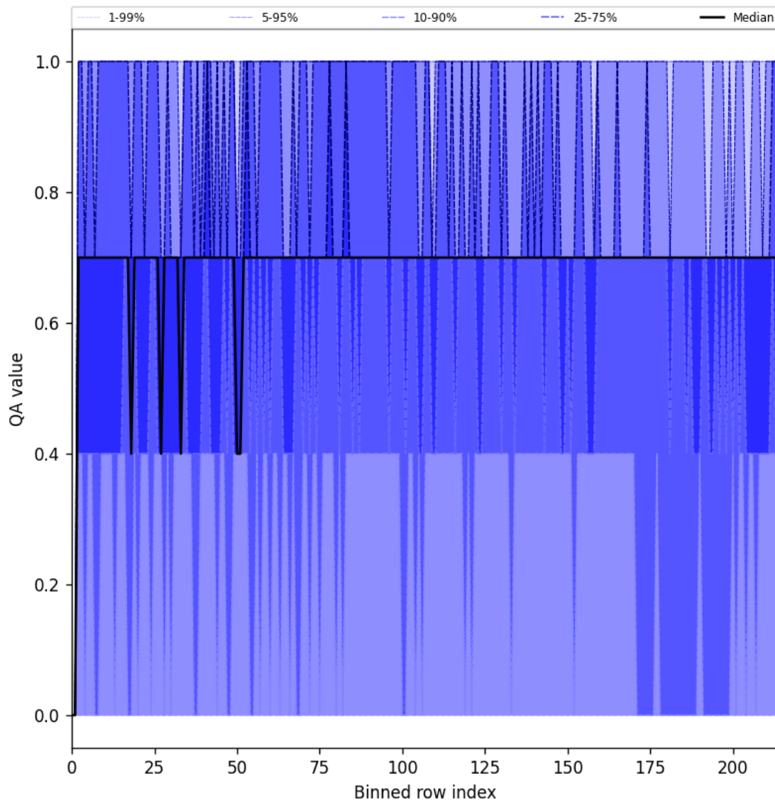
Figure 25: Along track statistics of “QA value” for 2025-09-26 to 2025-09-28
