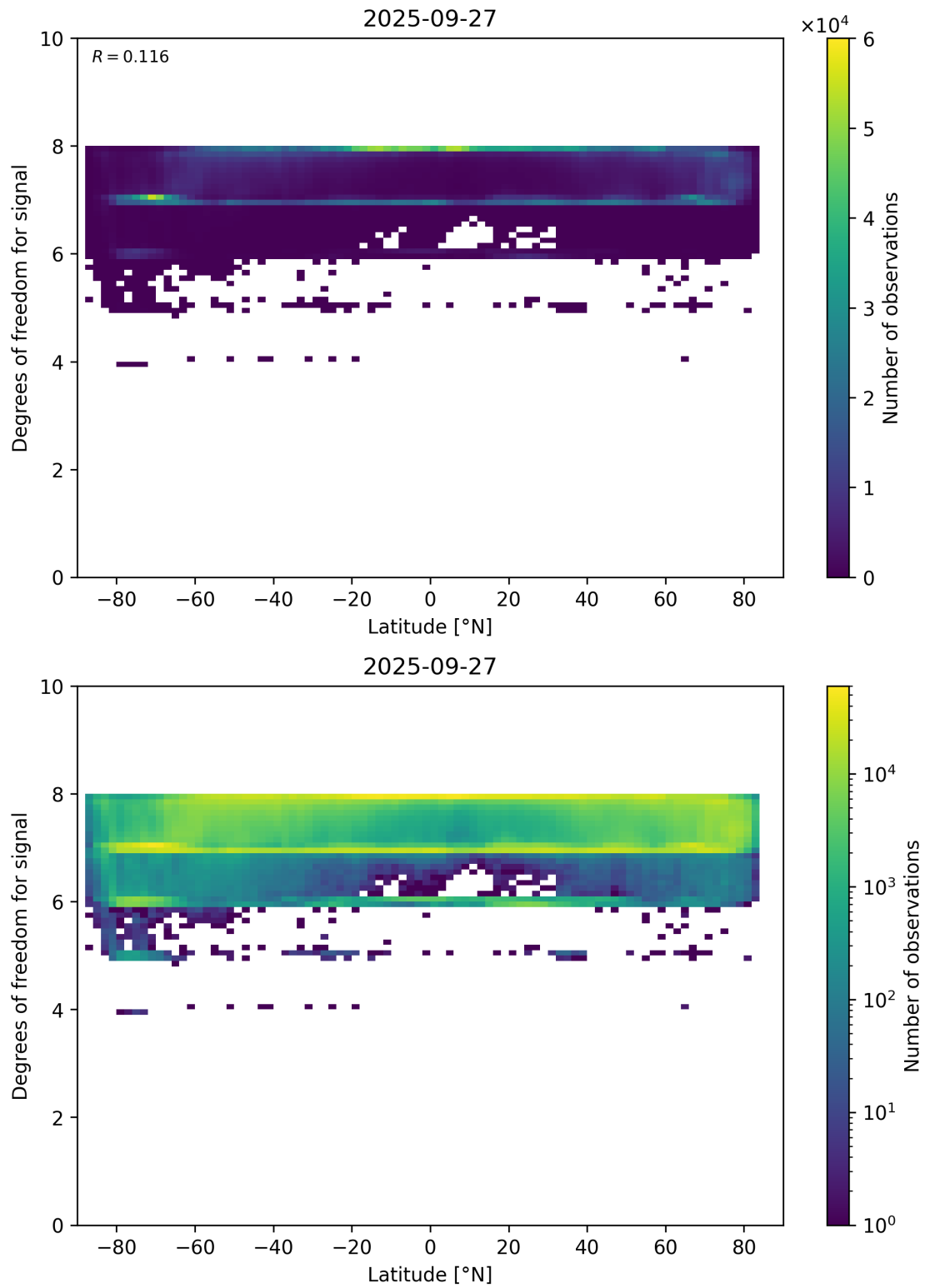
Figure 55: Scatter density plot of “Latitude” against “Degrees of freedom for signal” for 2025-09-26 to 2025-09-28.
