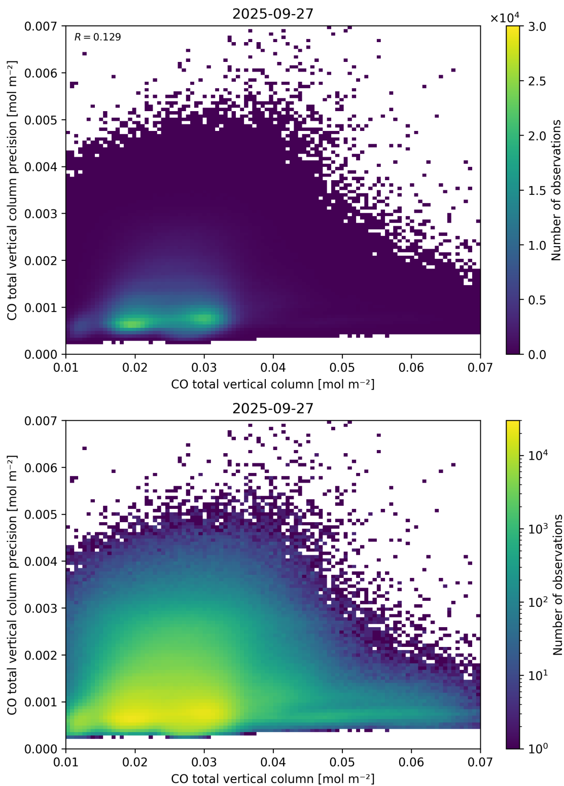
Figure 34: Scatter density plot of “CO total vertical column” against “CO total vertical column precision” for 2025-09-26 to 2025-09-28.
