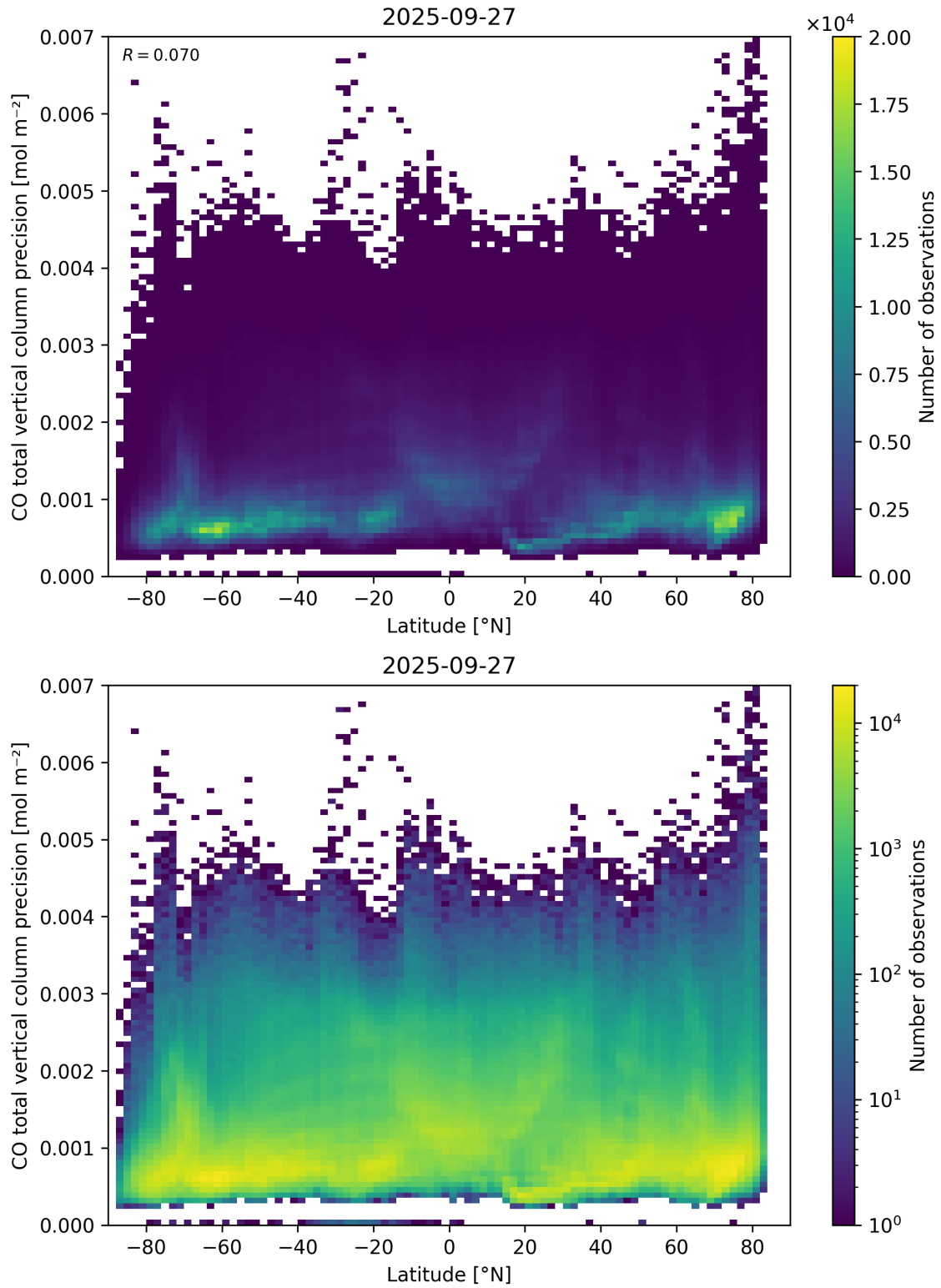
Figure 53: Scatter density plot of “Latitude” against “CO total vertical column precision” for 2025-09-26 to 2025-09-28.
