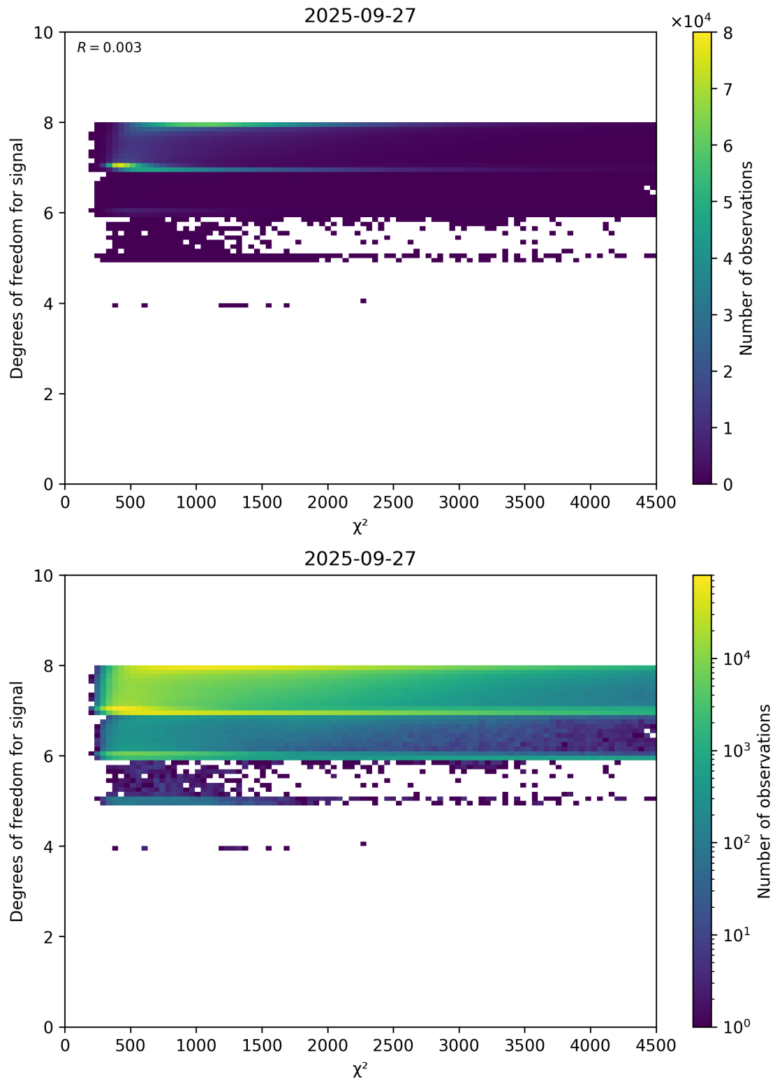
Figure 48: Scatter density plot of “ \chi^2 ” against “Degrees of freedom for signal” for 2025-09-26 to 2025-09-28.
