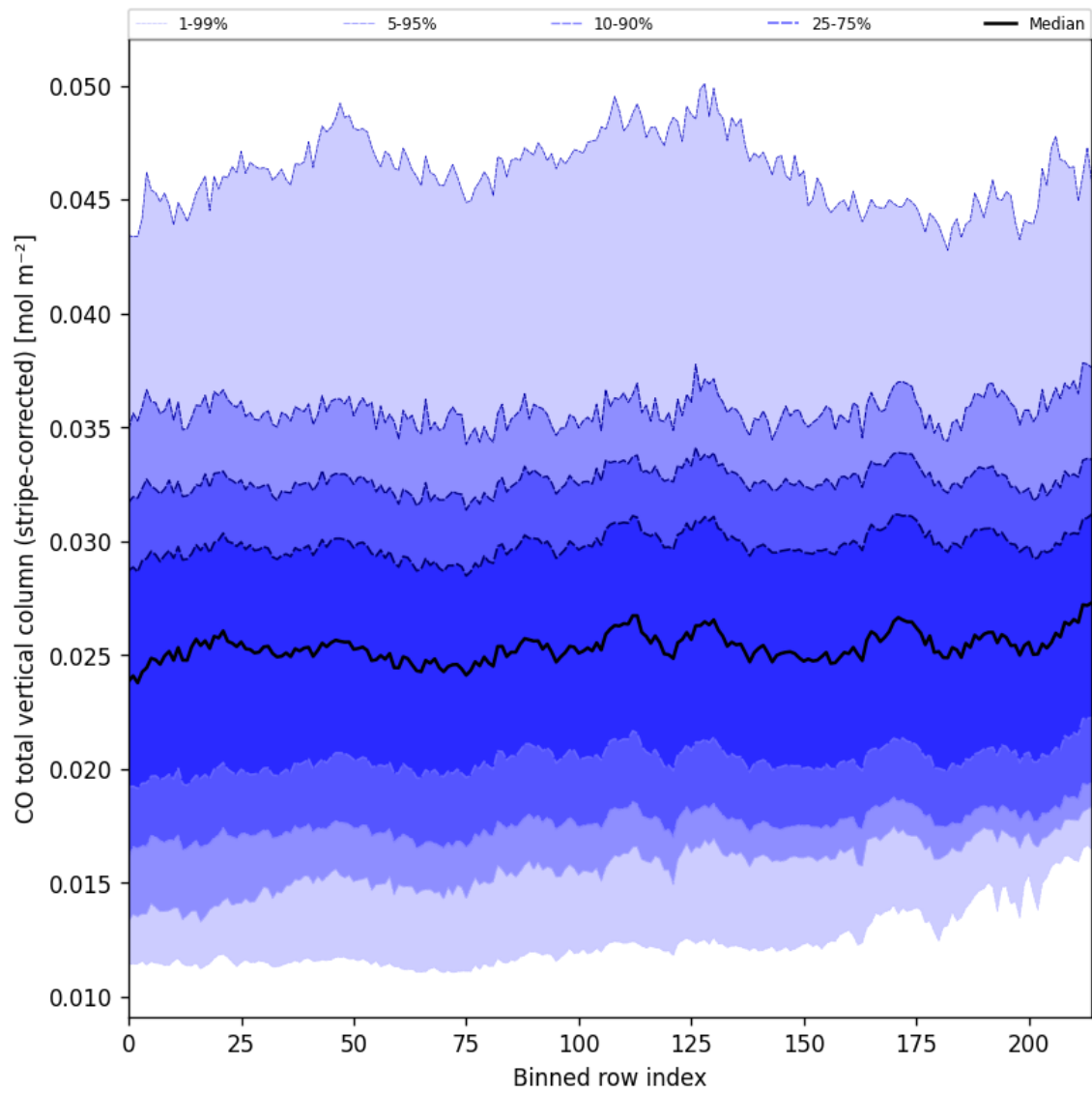
Figure 27: Along track statistics of “CO total vertical column (stripe-corrected)” for 2025-09-26 to 2025-09-28
