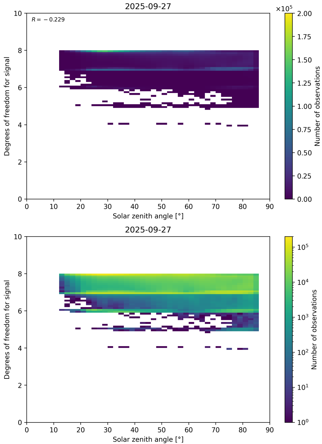
Figure 65: Scatter density plot of “Solar zenith angle” against “Degrees of freedom for signal” for 2025-09-26 to 2025-09-28.
