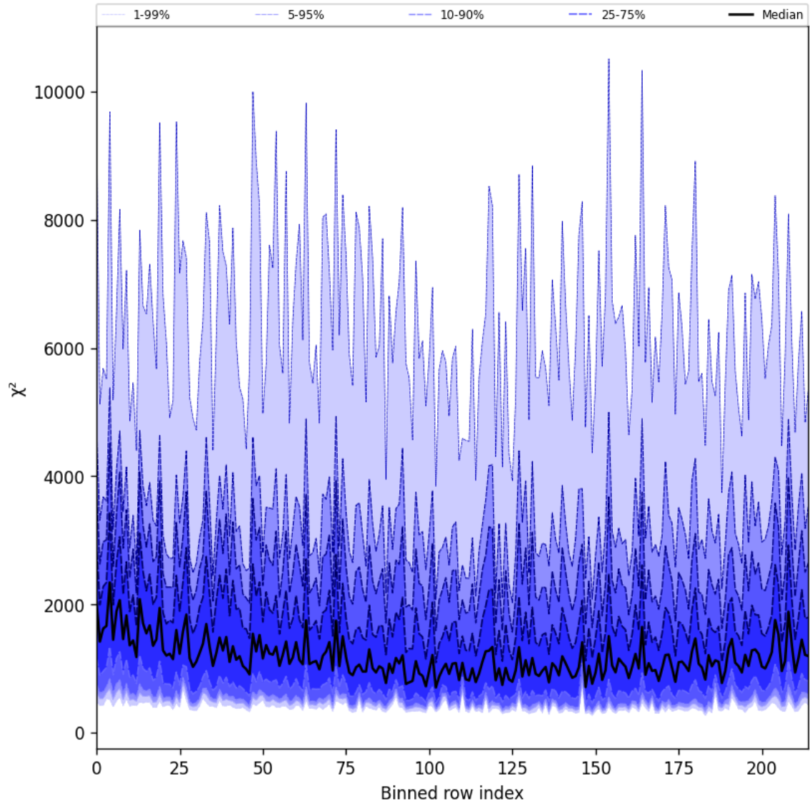
Figure 30: Along track statistics of “ \chi^2 ” for 2025-09-26 to 2025-09-28
