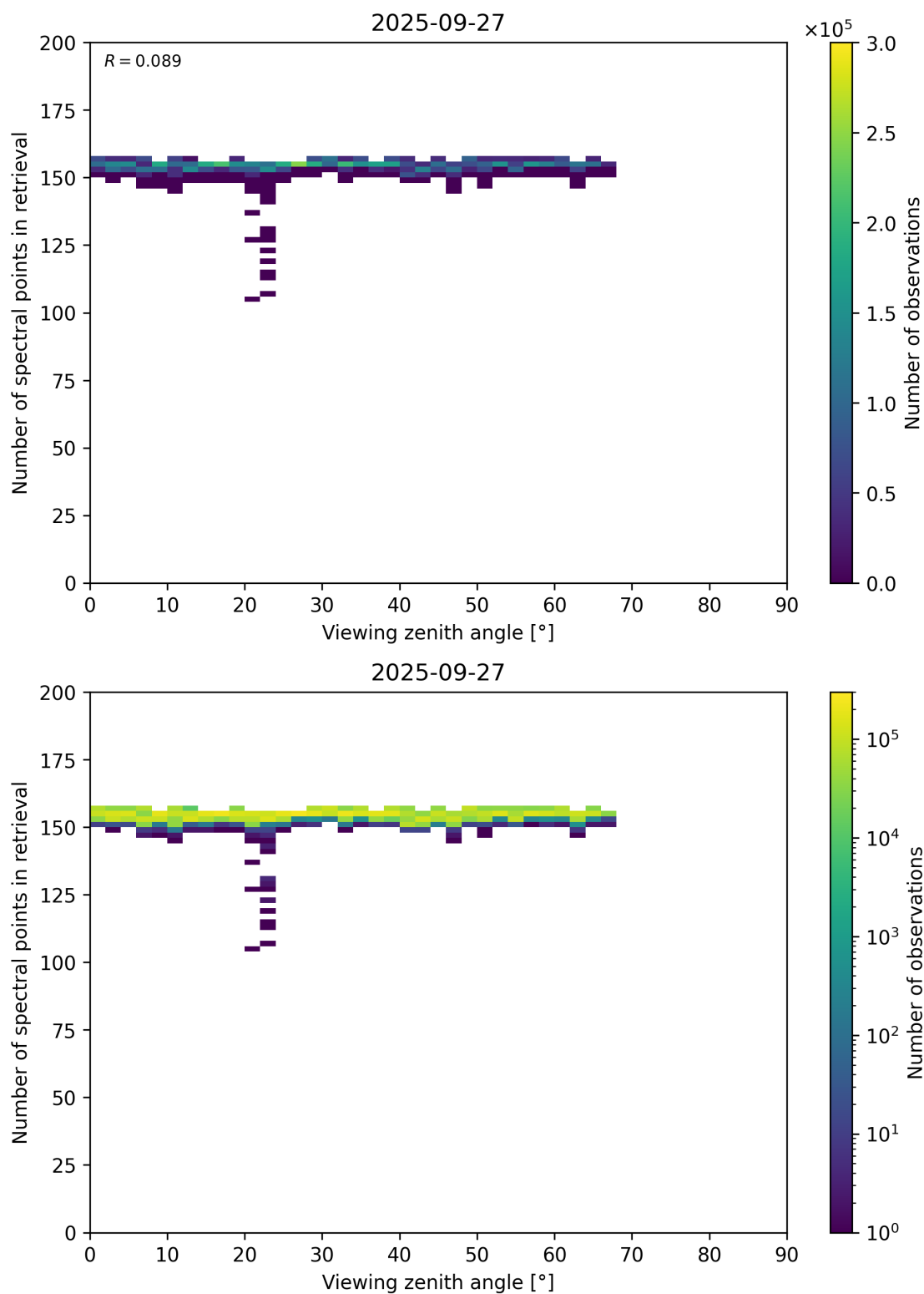
Figure 76: Scatter density plot of “Viewing zenith angle” against “Number of spectral points in retrieval” for 2025-09-26 to 2025-09-28.
