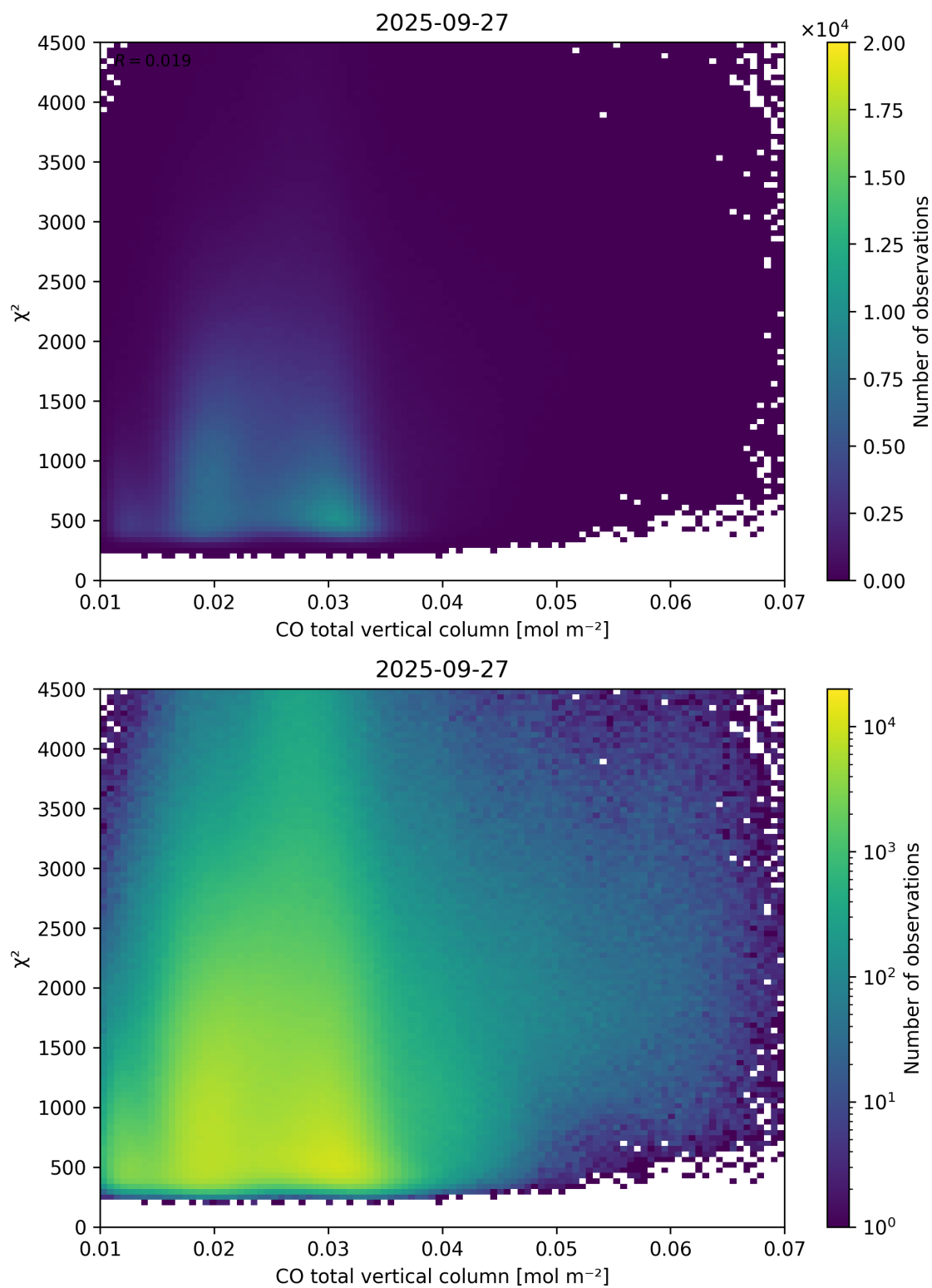
Figure 35: Scatter density plot of “CO total vertical column” against “ \chi^2 ” for 2025-09-26 to 2025-09-28.
