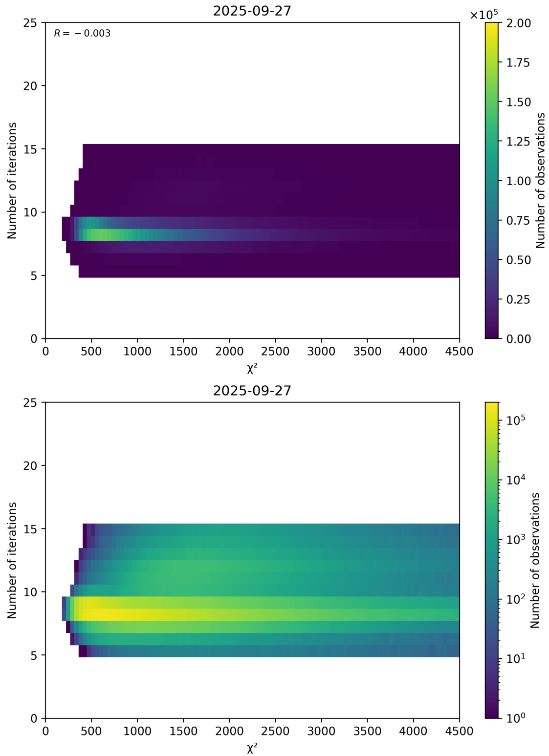
Figure 49: Scatter density plot of “ \chi^2 ” against “Number of iterations” for 2025-09-26 to 2025-09-28.
