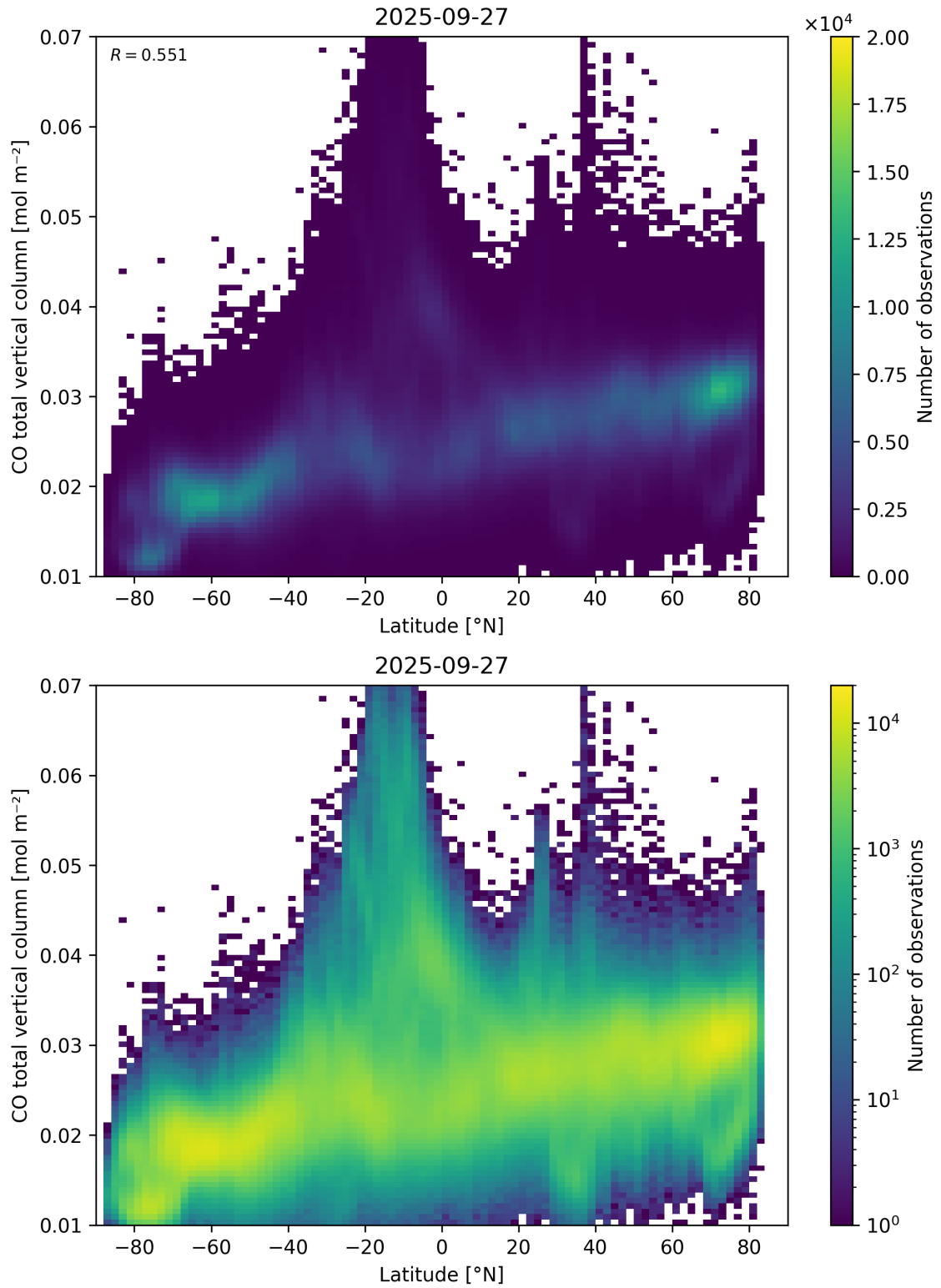
Figure 51: Scatter density plot of “Latitude” against “CO total vertical column” for 2025-09-26 to 2025-09-28.
