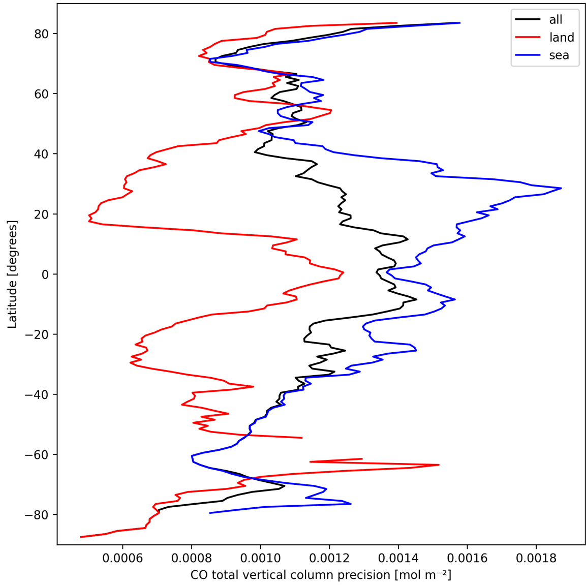
Figure 12: Zonal average of “CO total vertical column precision” for 2025-09-26 to 2025-09-28.
