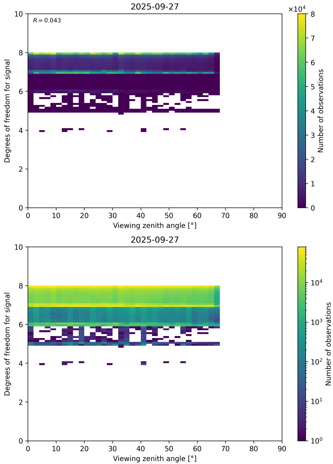
Figure 73: Scatter density plot of “Viewing zenith angle” against “Degrees of freedom for signal” for 2025-09-26 to 2025-09-28.
