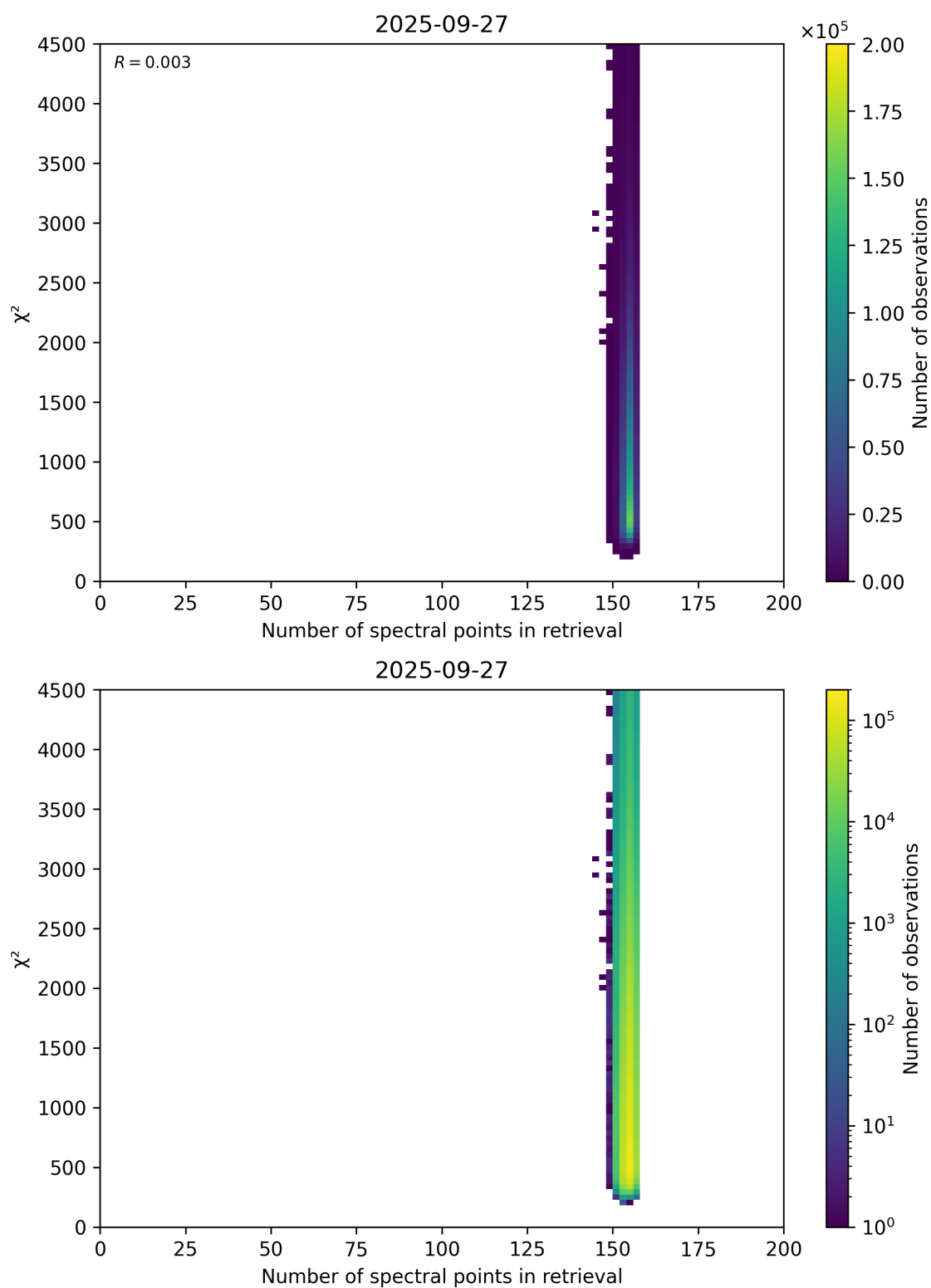
Figure 58: Scatter density plot of “Number of spectral points in retrieval” against “ \chi^2 ” for 2025-09-26 to 2025-09-28.
