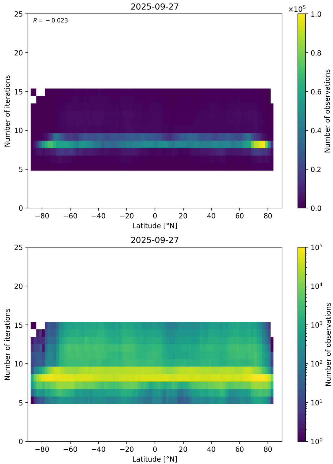
Figure 56: Scatter density plot of “Latitude” against “Number of iterations” for 2025-09-26 to 2025-09-28.
