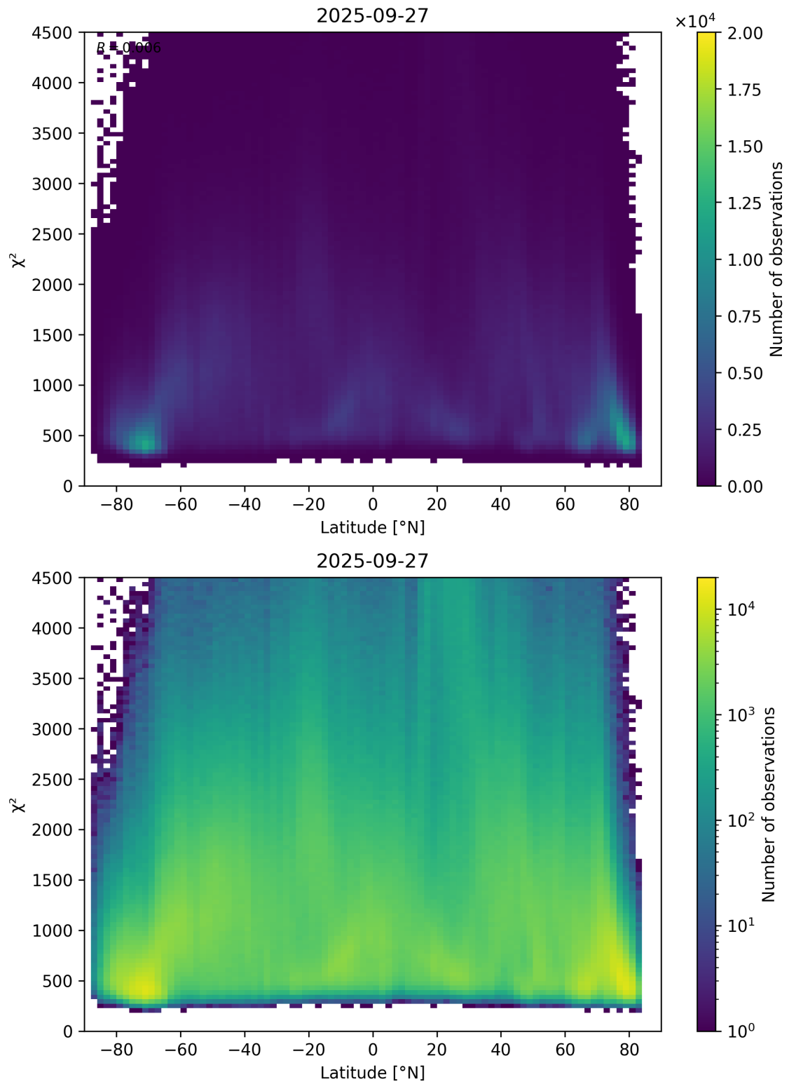
Figure 54: Scatter density plot of “Latitude” against “ \chi^2 ” for 2025-09-26 to 2025-09-28.
