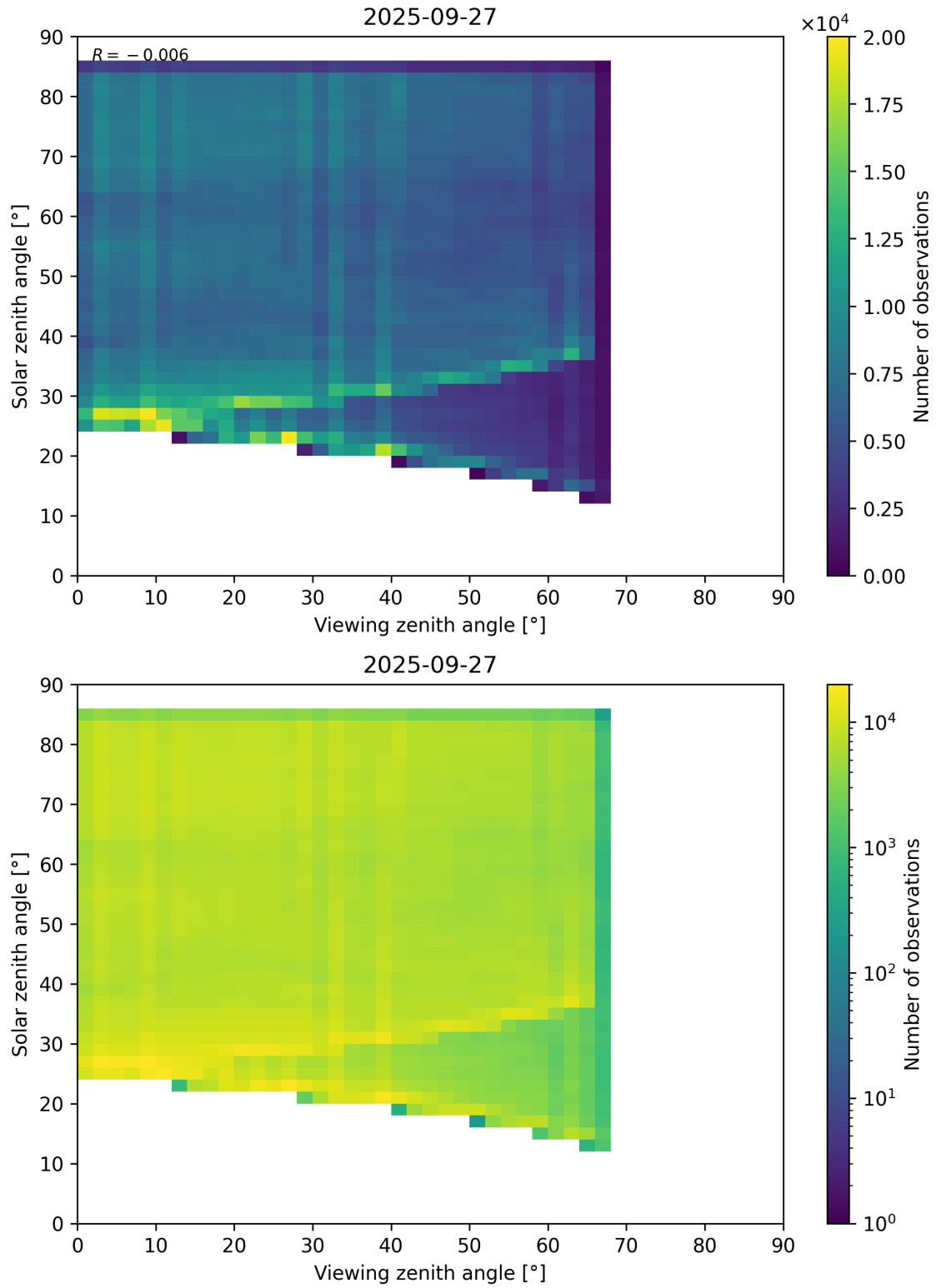
Figure 77: Scatter density plot of “Viewing zenith angle” against “Solar zenith angle” for 2025-09-26 to 2025-09-28.
