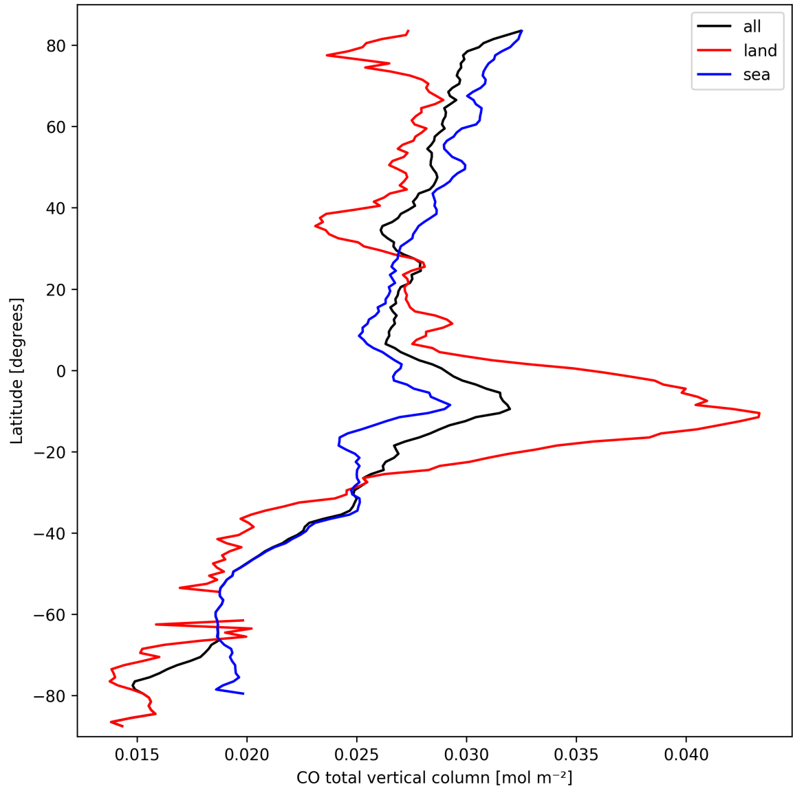
Figure 10: Zonal average of “CO total vertical column” for 2025-09-26 to 2025-09-28.
