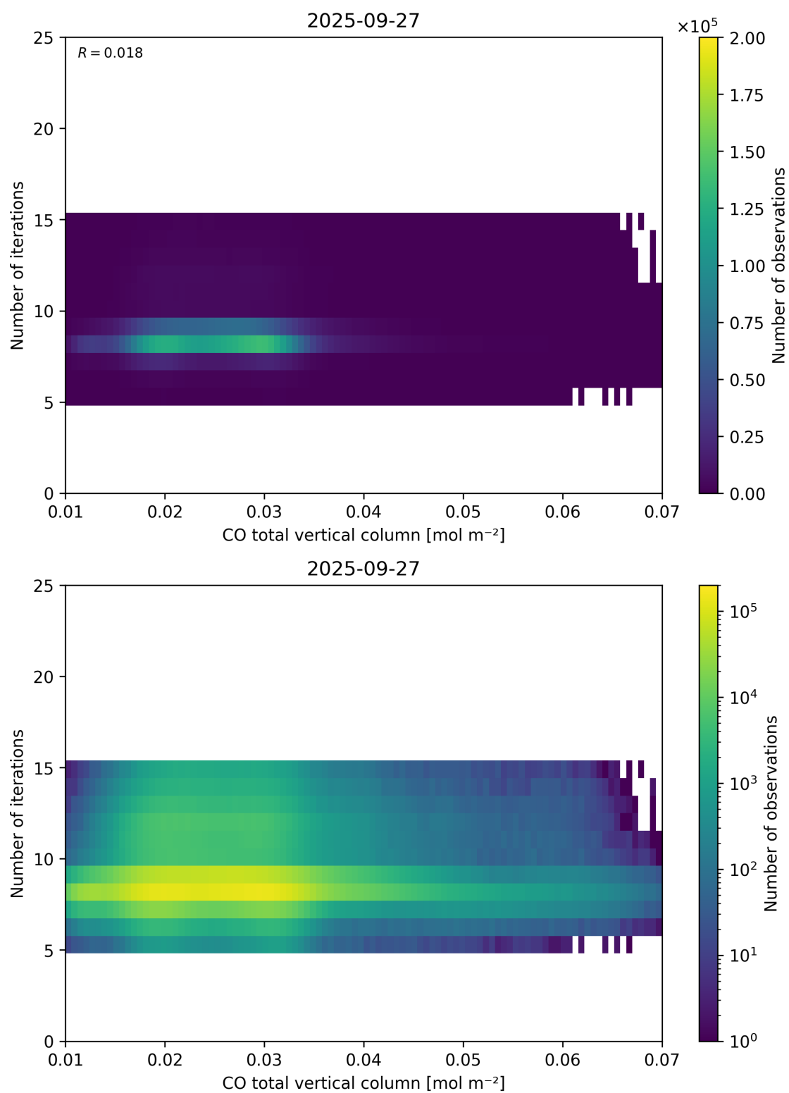
Figure 42: Scatter density plot of “CO total vertical column” against “Number of iterations” for 2025-09-26 to 2025-09-28.
