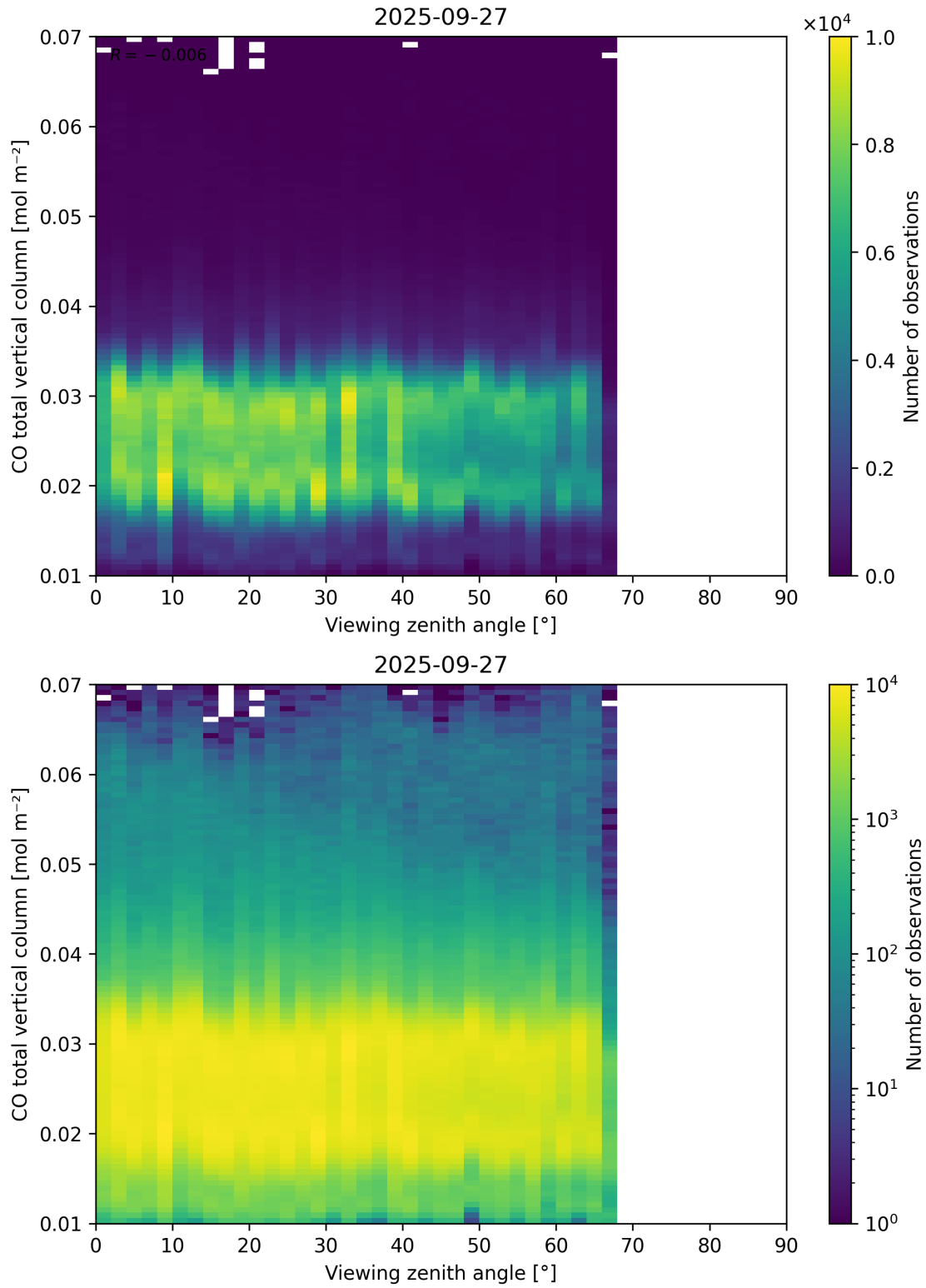
Figure 69: Scatter density plot of “Viewing zenith angle” against “CO total vertical column” for 2025-09-26 to 2025-09-28.
