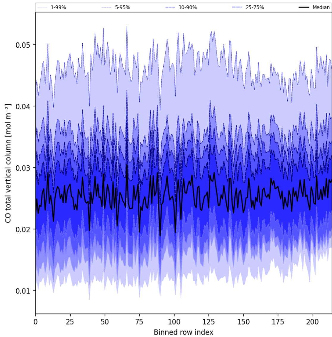
Figure 26: Along track statistics of “CO total vertical column” for 2025-09-26 to 2025-09-28
