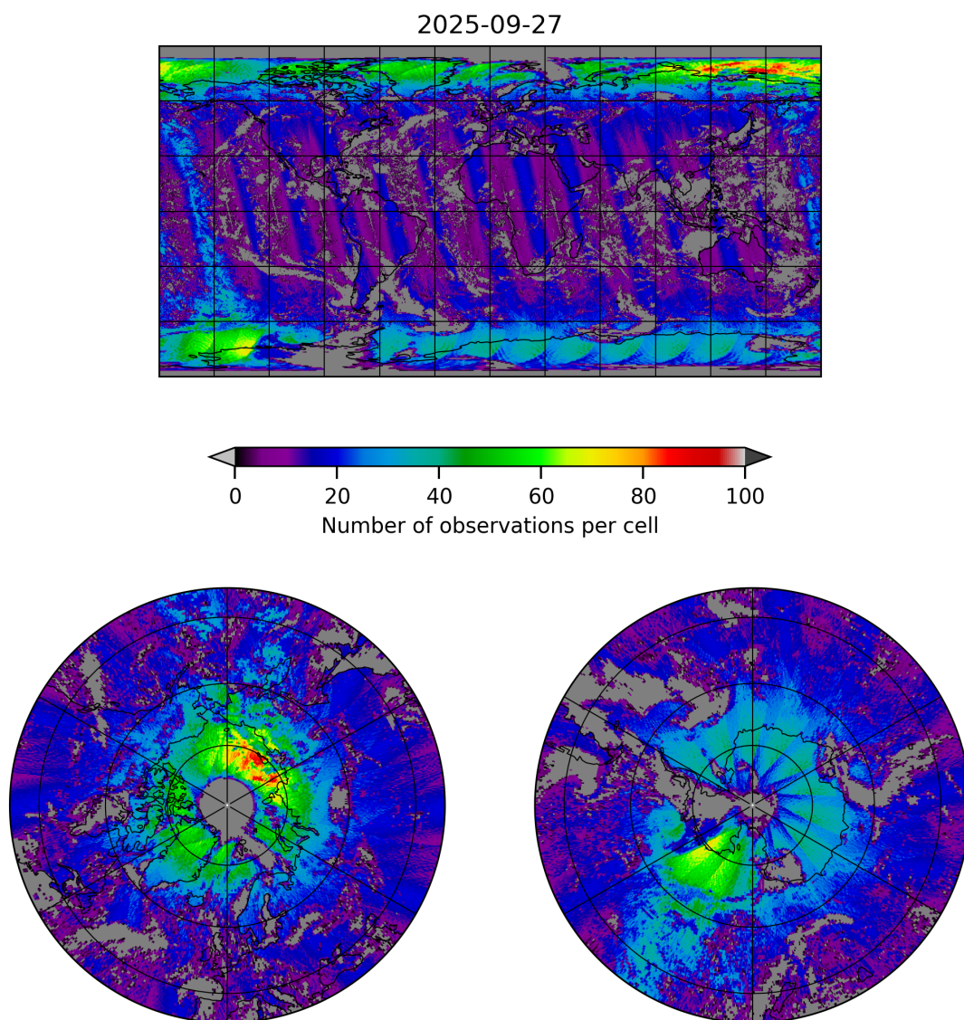
Figure 8: Map of the number of observations for 2025-09-26 to 2025-09-28
