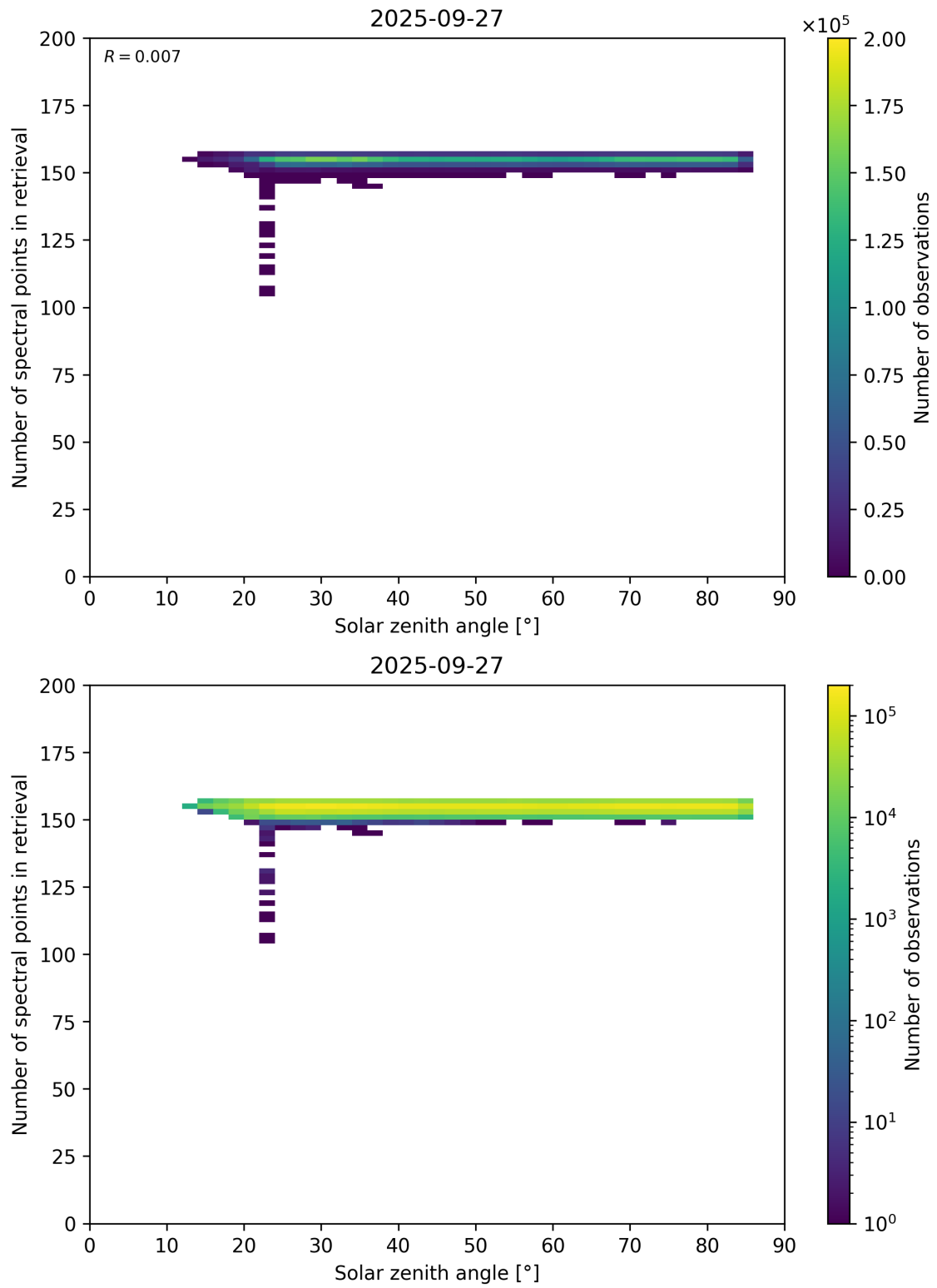
Figure 68: Scatter density plot of “Solar zenith angle” against “Number of spectral points in retrieval” for 2025-09-26 to 2025-09-28.
