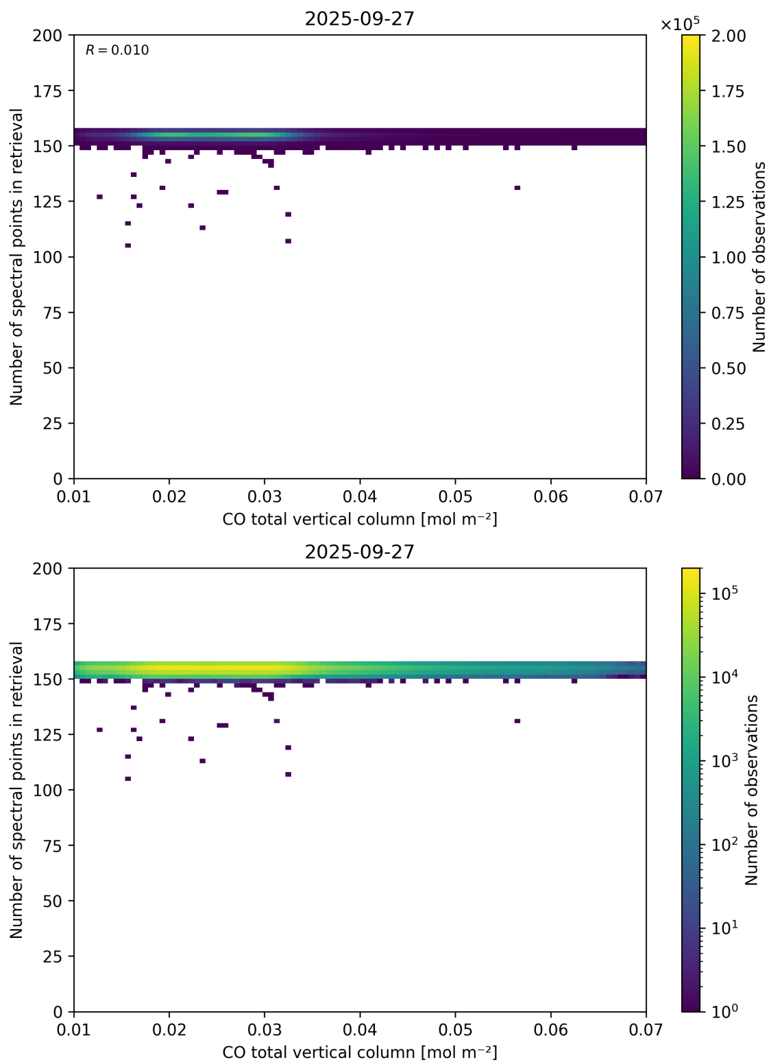
Figure 43: Scatter density plot of “CO total vertical column” against “Number of spectral points in retrieval” for 2025-09-26 to 2025-09-28.
