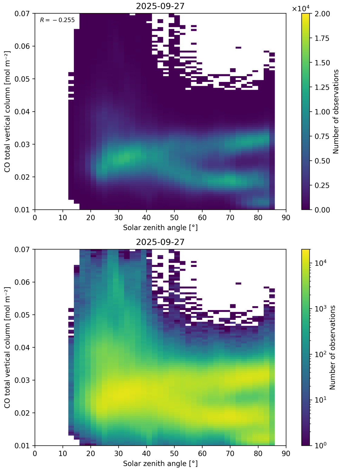
Figure 61: Scatter density plot of “Solar zenith angle” against “CO total vertical column” for 2025-09-26 to 2025-09-28.
