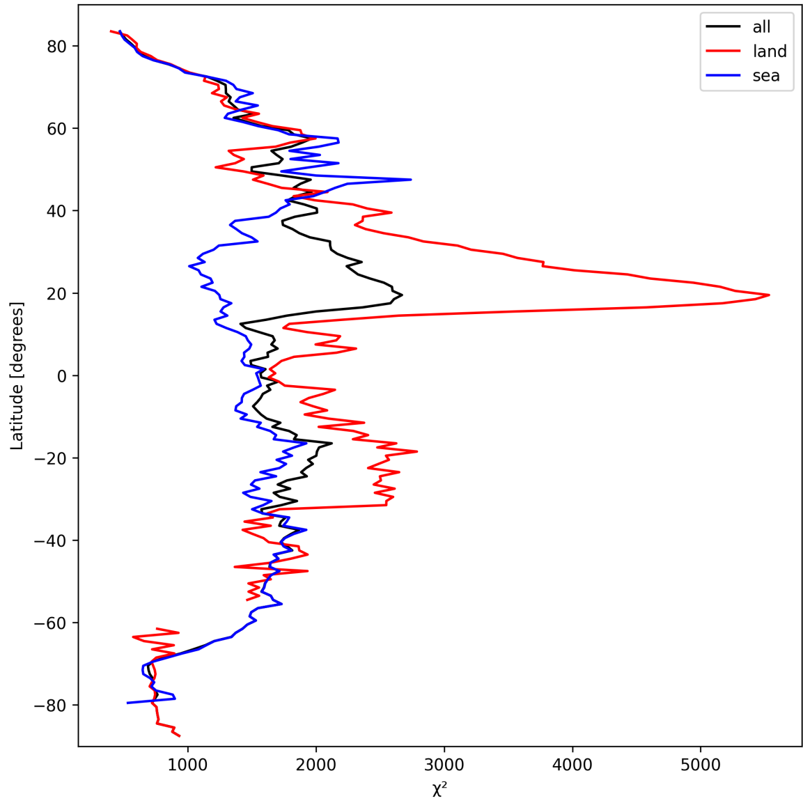
Figure 14: Zonal average of “ \chi^2 ” for 2025-09-26 to 2025-09-28.
