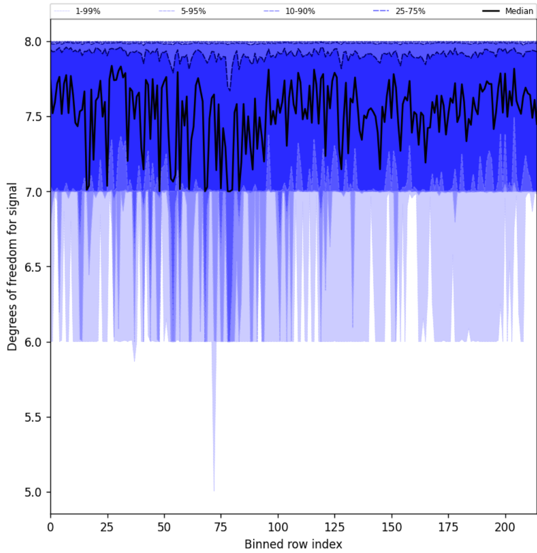
Figure 31: Along track statistics of “Degrees of freedom for signal” for 2025-09-26 to 2025-09-28
