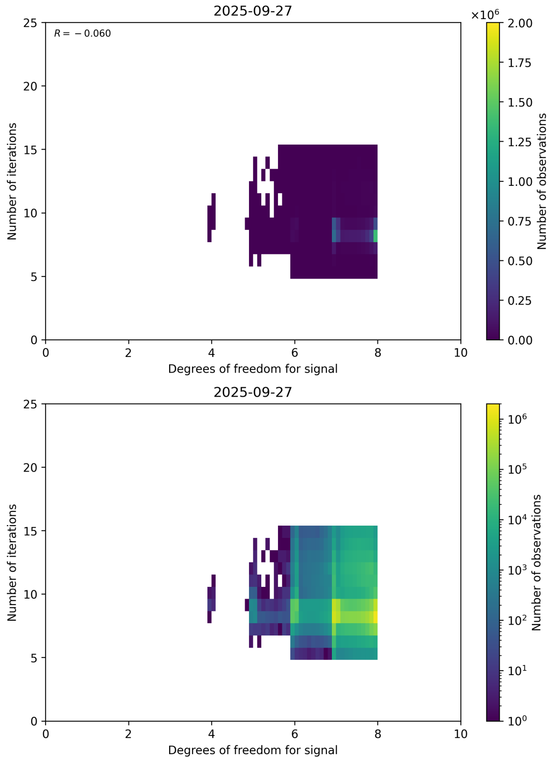
Figure 50: Scatter density plot of “Degrees of freedom for signal” against “Number of iterations” for 2025-09-26 to 2025-09-28.
