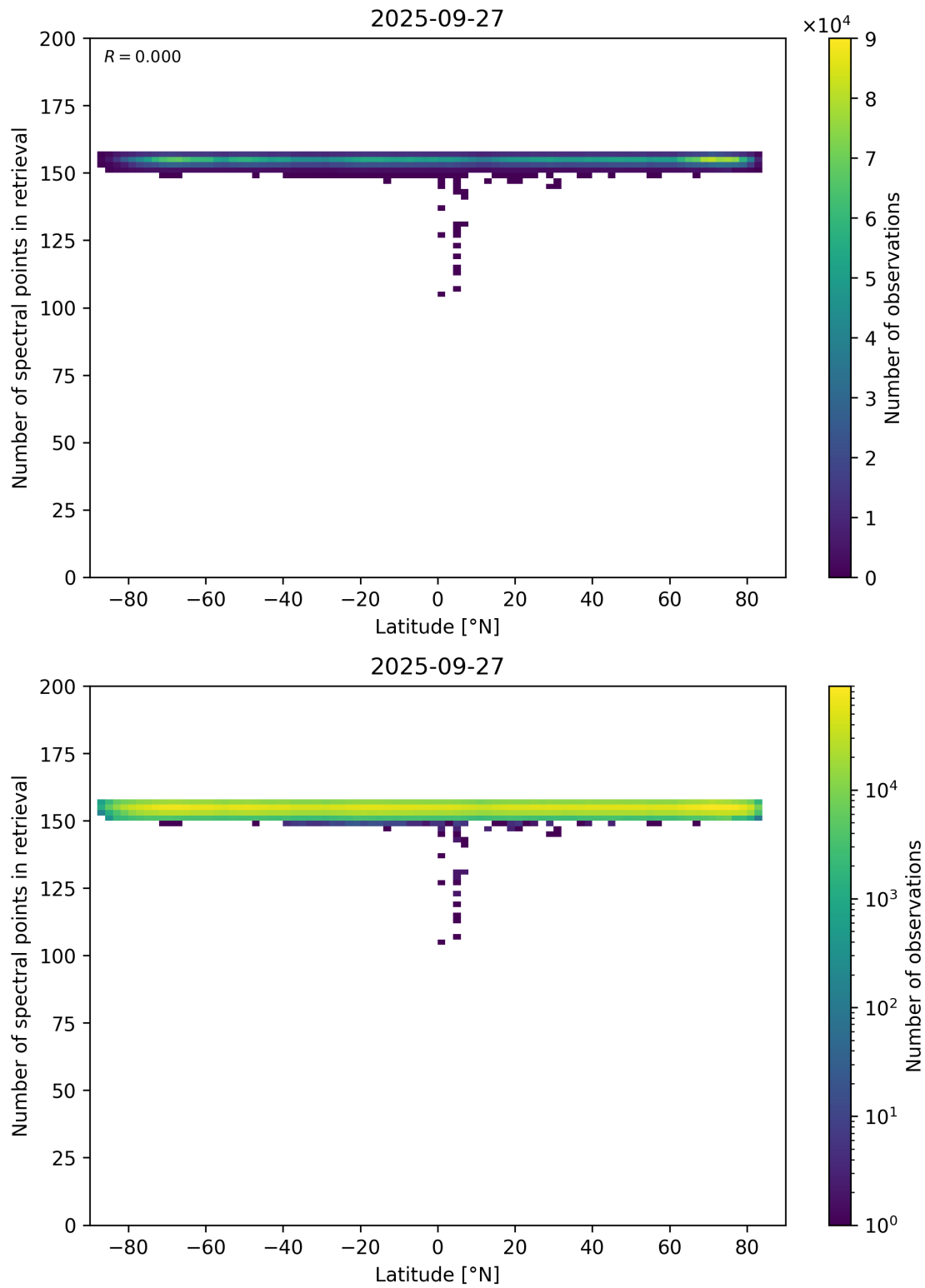
Figure 57: Scatter density plot of “Latitude” against “Number of spectral points in retrieval” for 2025-09-26 to 2025-09-28.
