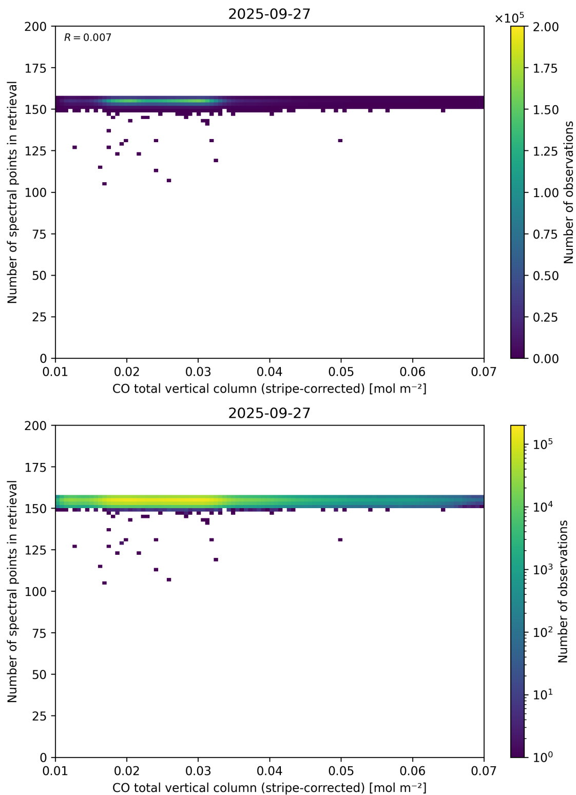
Figure 40: Scatter density plot of “CO total vertical column (stripe-corrected)” against “Number of spectral points in retrieval” for 2025-09-26 to 2025-09-28.
