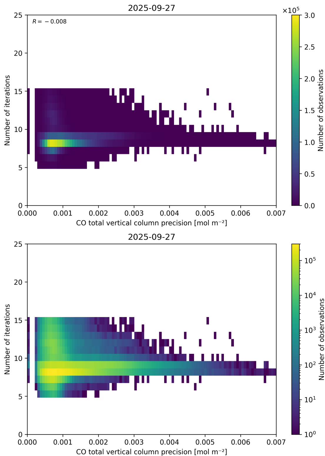
Figure 46: Scatter density plot of “CO total vertical column precision” against “Number of iterations” for 2025-09-26 to 2025-09-28.
