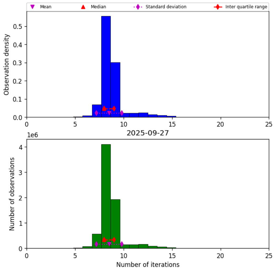
Figure 24: Histogram of “Number of iterations” for 2025-09-26 to 2025-09-28
