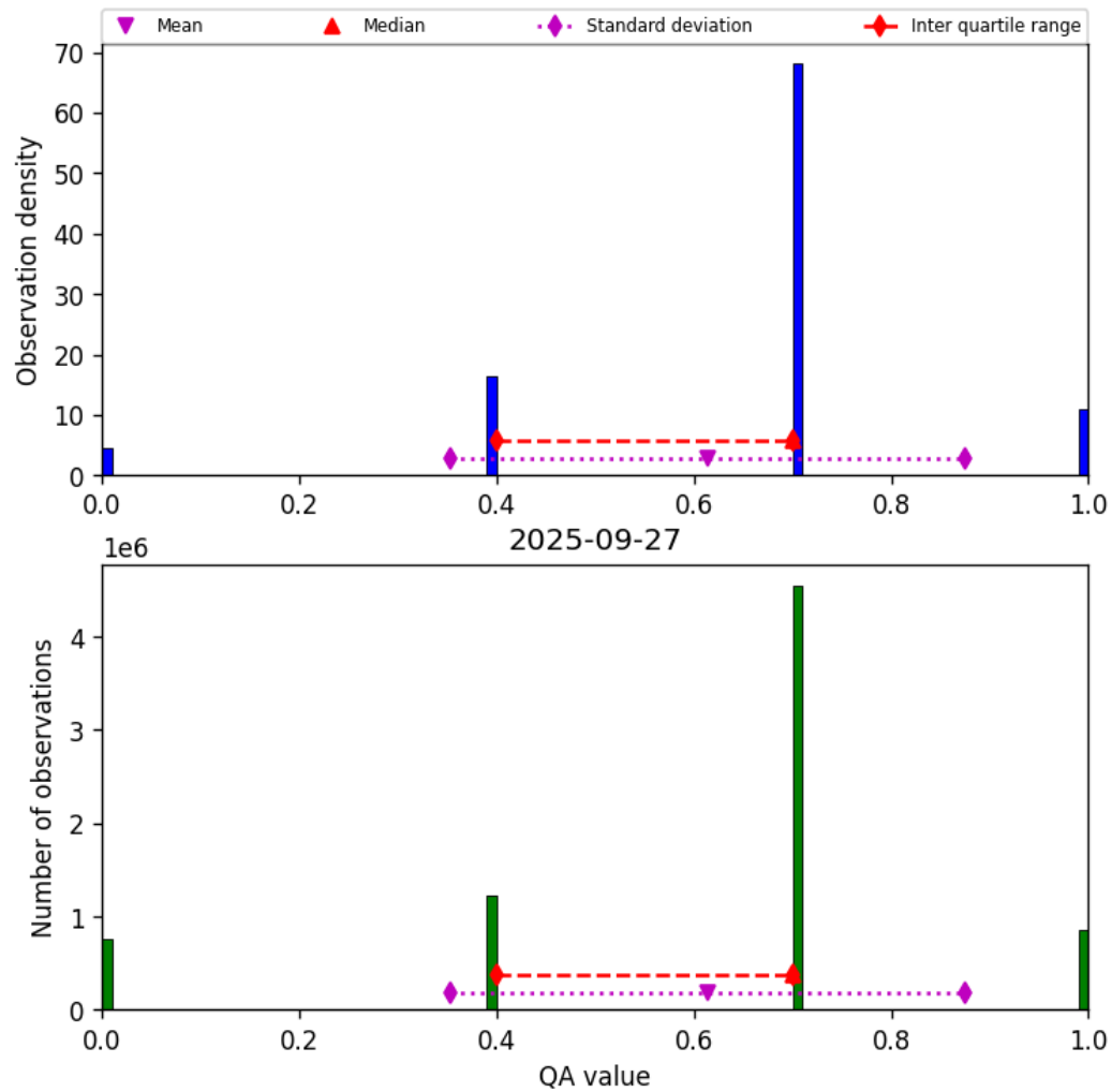
Figure 17: Histogram of “QA value” for 2025-09-26 to 2025-09-28
