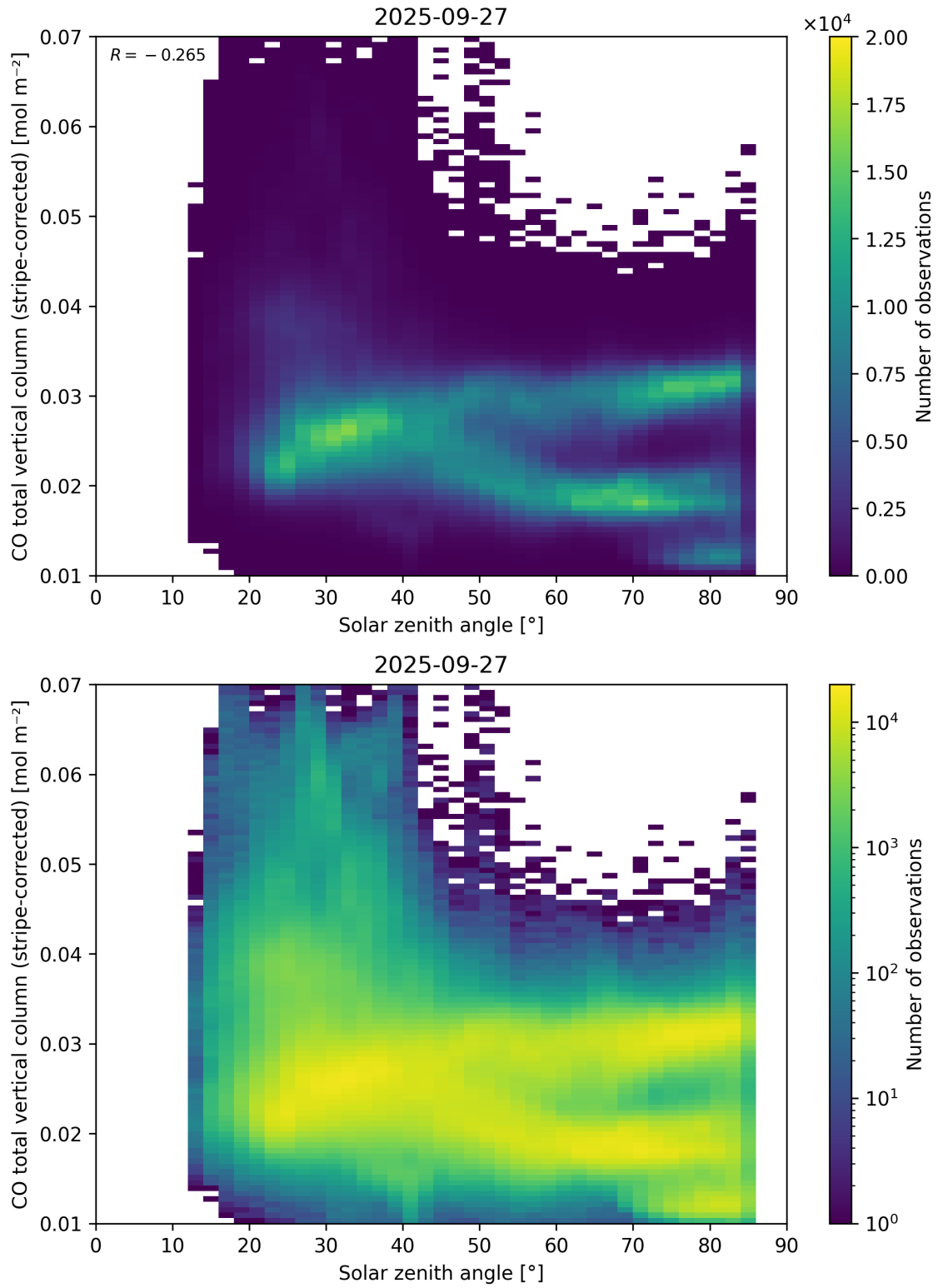
Figure 62: Scatter density plot of “Solar zenith angle” against “CO total vertical column (stripe-corrected)” for 2025-09-26 to 2025-09-28.
