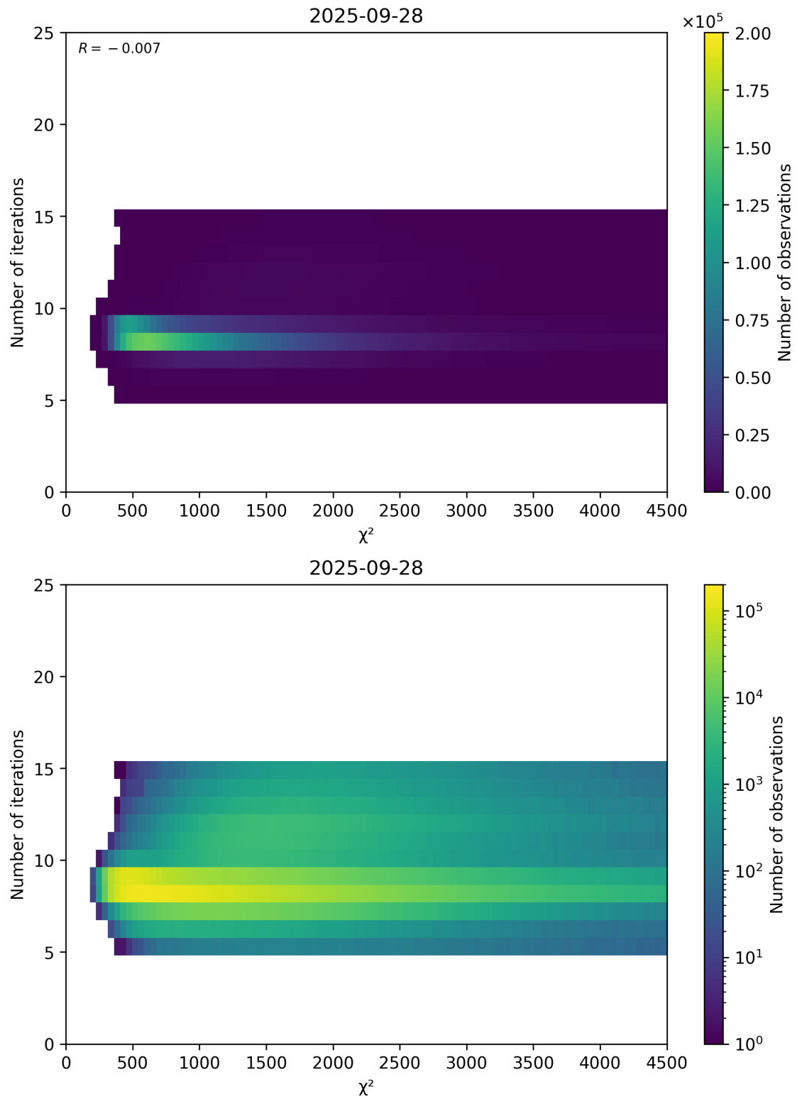
Figure 49: Scatter density plot of “ \chi^2 ” against “Number of iterations” for 2025-09-27 to 2025-09-29.
