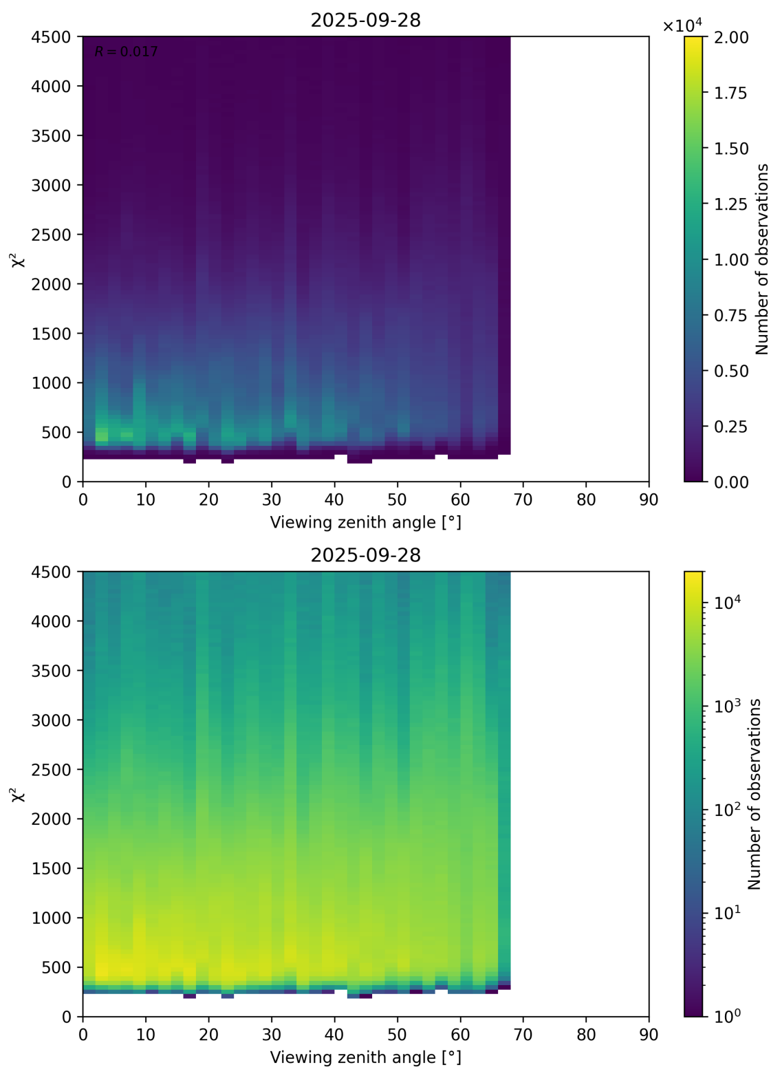
Figure 72: Scatter density plot of “Viewing zenith angle” against “ \chi^2 ” for 2025-09-27 to 2025-09-29.
