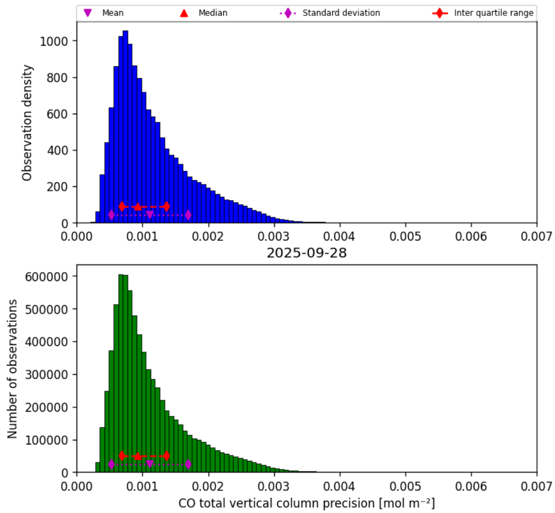
Figure 20: Histogram of “CO total vertical column precision” for 2025-09-27 to 2025-09-29
