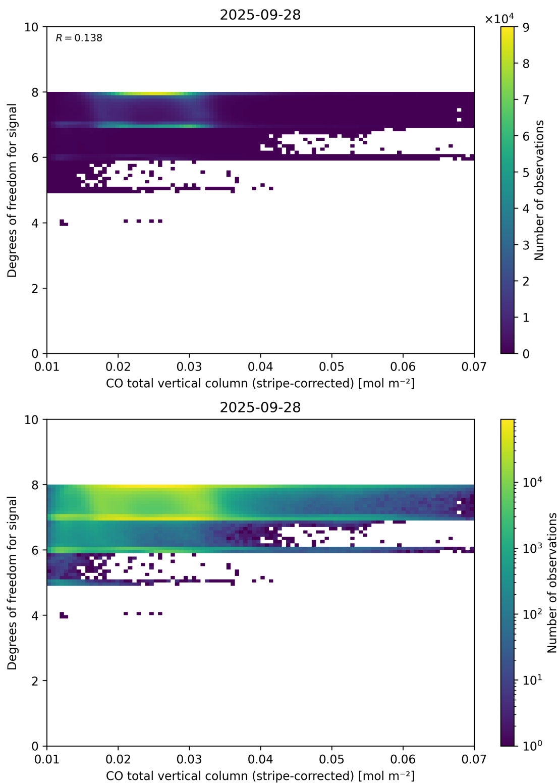
Figure 38: Scatter density plot of “CO total vertical column (stripe-corrected)” against “Degrees of freedom for signal” for 2025-09-27 to 2025-09-29.
