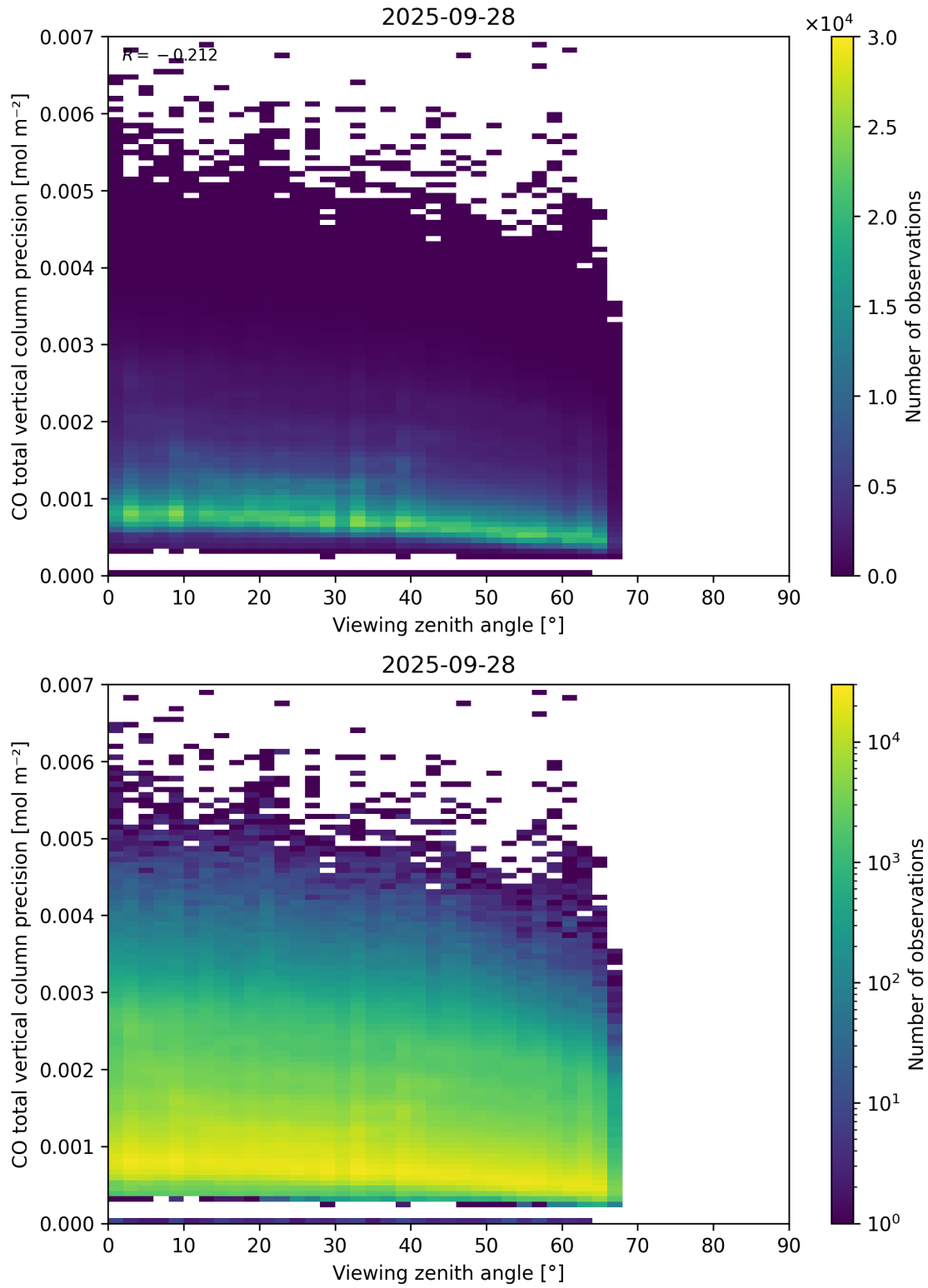
Figure 71: Scatter density plot of “Viewing zenith angle” against “CO total vertical column precision” for 2025-09-27 to 2025-09-29.
