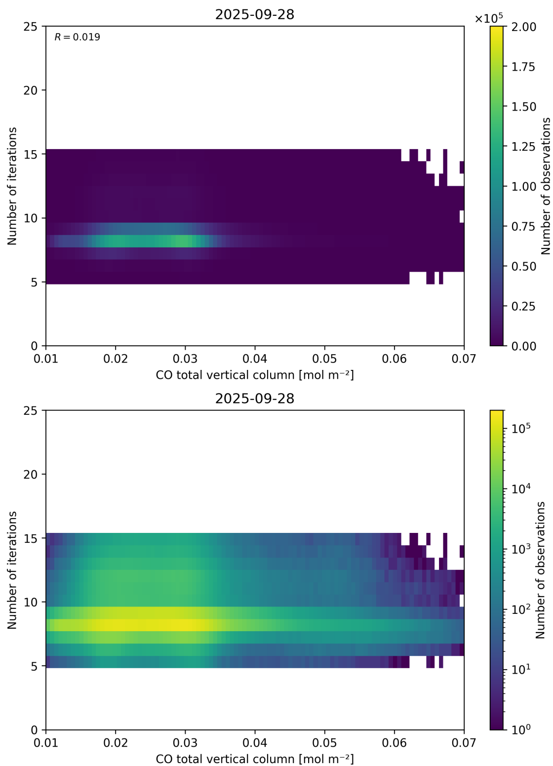
Figure 42: Scatter density plot of “CO total vertical column” against “Number of iterations” for 2025-09-27 to 2025-09-29.
