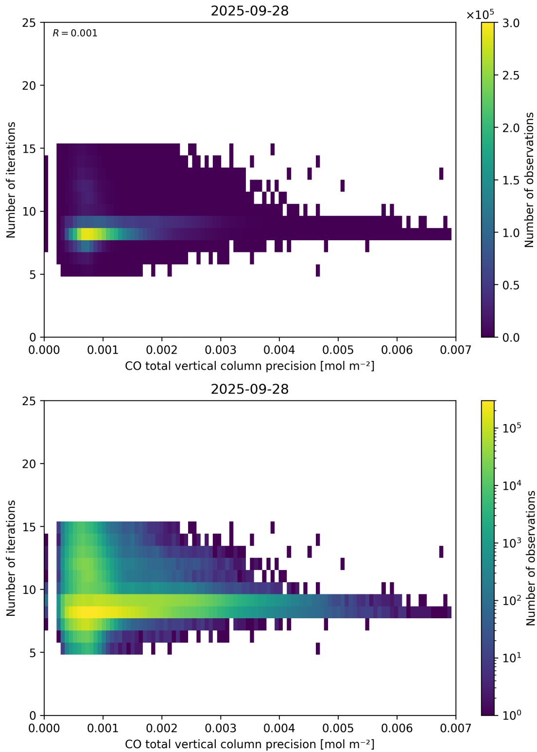
Figure 46: Scatter density plot of “CO total vertical column precision” against “Number of iterations” for 2025-09-27 to 2025-09-29.
