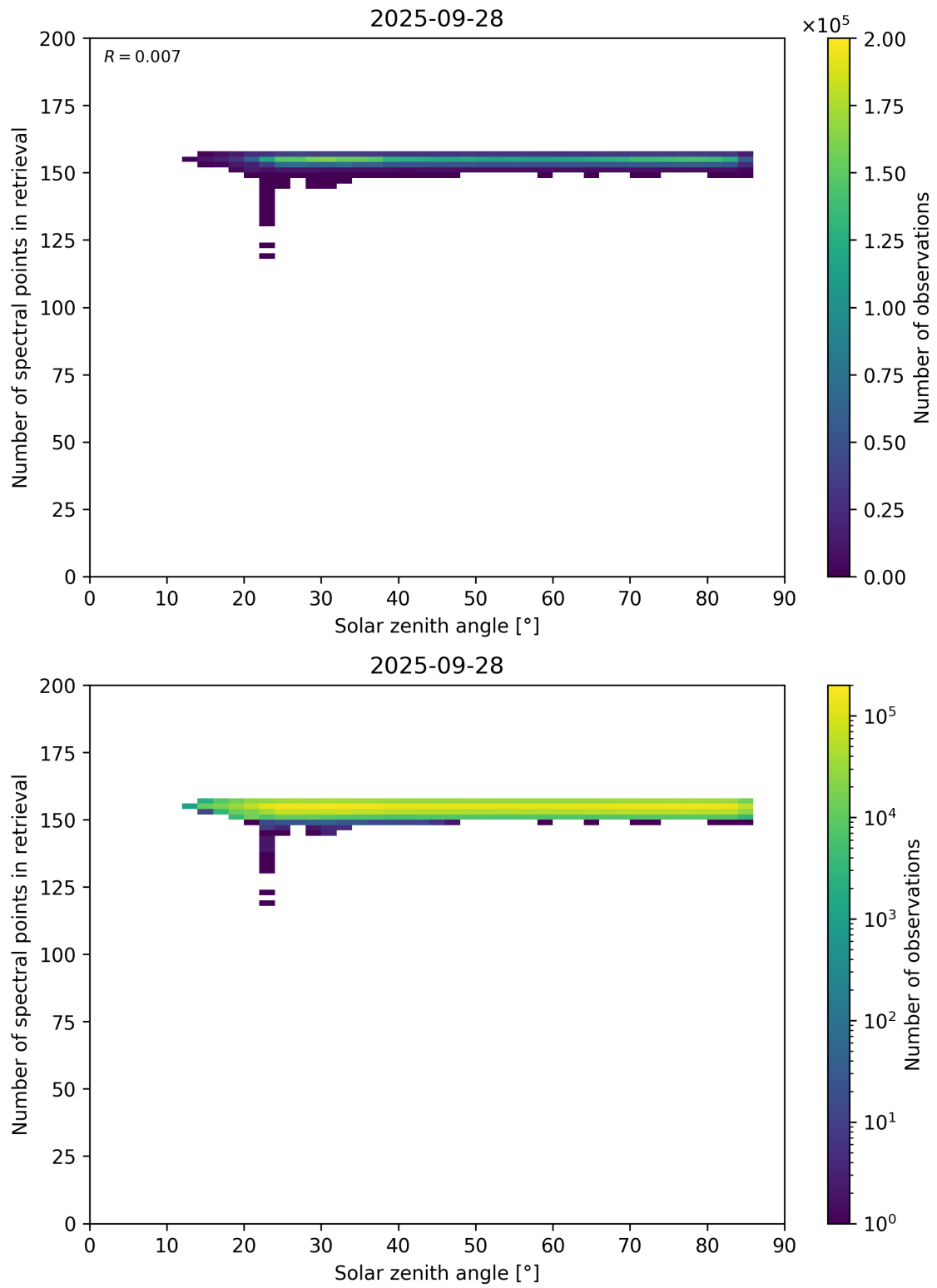
Figure 68: Scatter density plot of “Solar zenith angle” against “Number of spectral points in retrieval” for 2025-09-27 to 2025-09-29.
