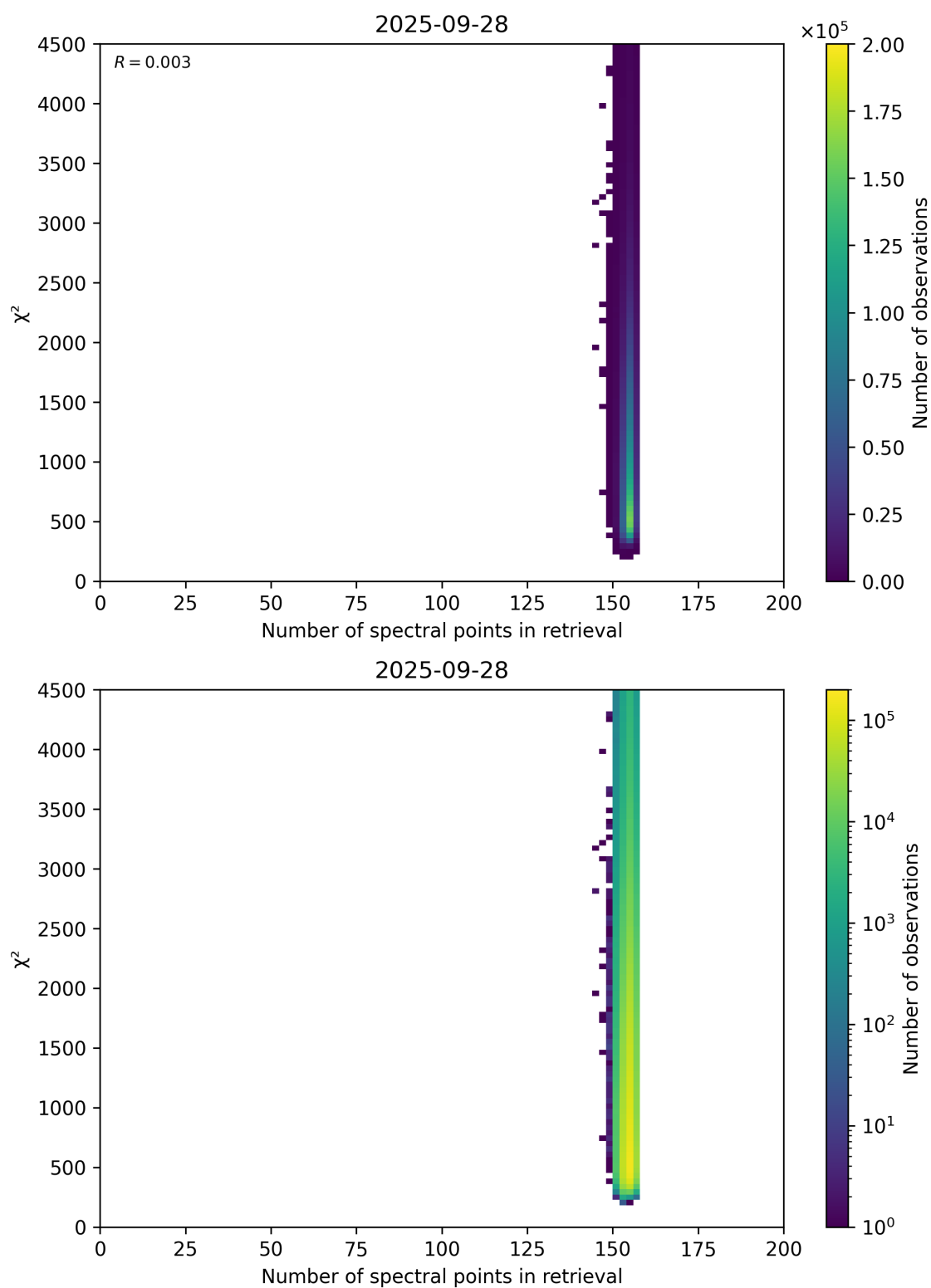
Figure 58: Scatter density plot of “Number of spectral points in retrieval” against “ \chi^2 ” for 2025-09-27 to 2025-09-29.
