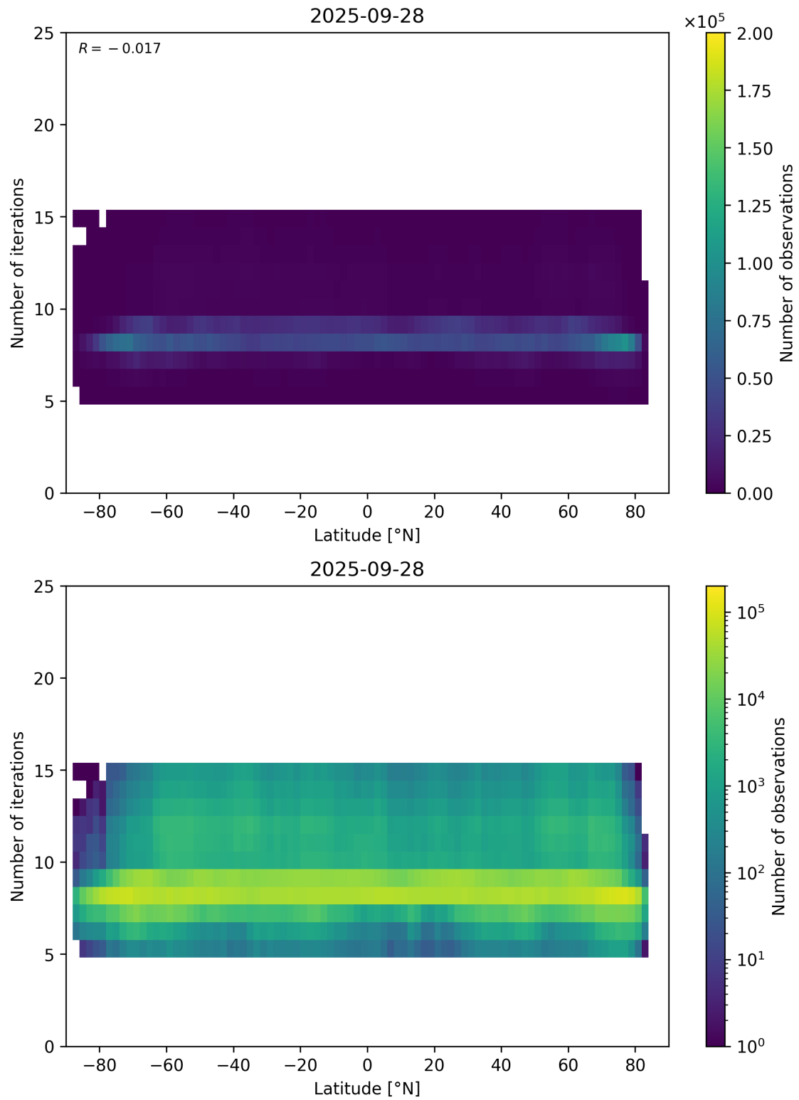
Figure 56: Scatter density plot of “Latitude” against “Number of iterations” for 2025-09-27 to 2025-09-29.
