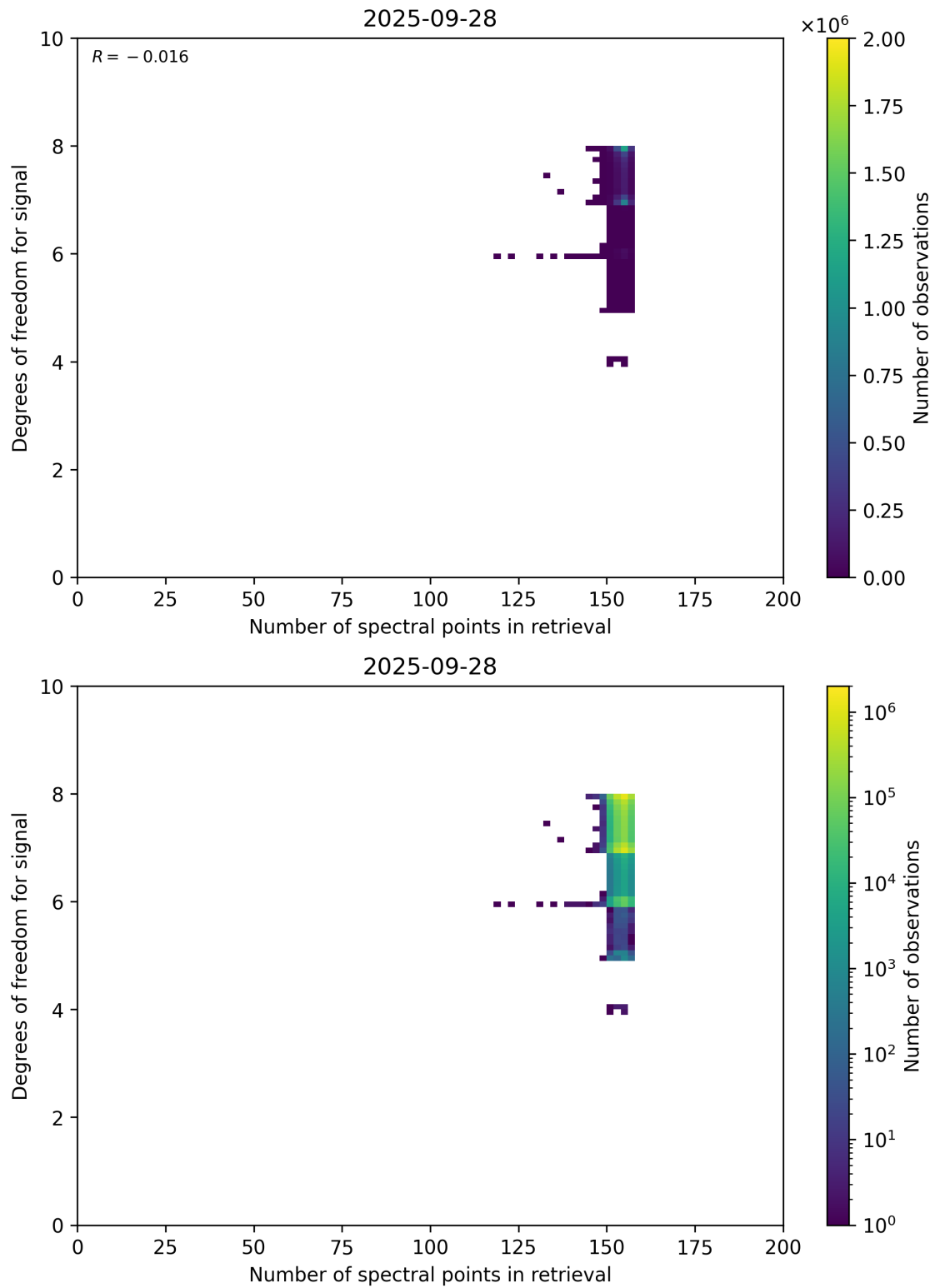
Figure 59: Scatter density plot of “Number of spectral points in retrieval” against “Degrees of freedom for signal” for 2025-09-27 to 2025-09-29.
