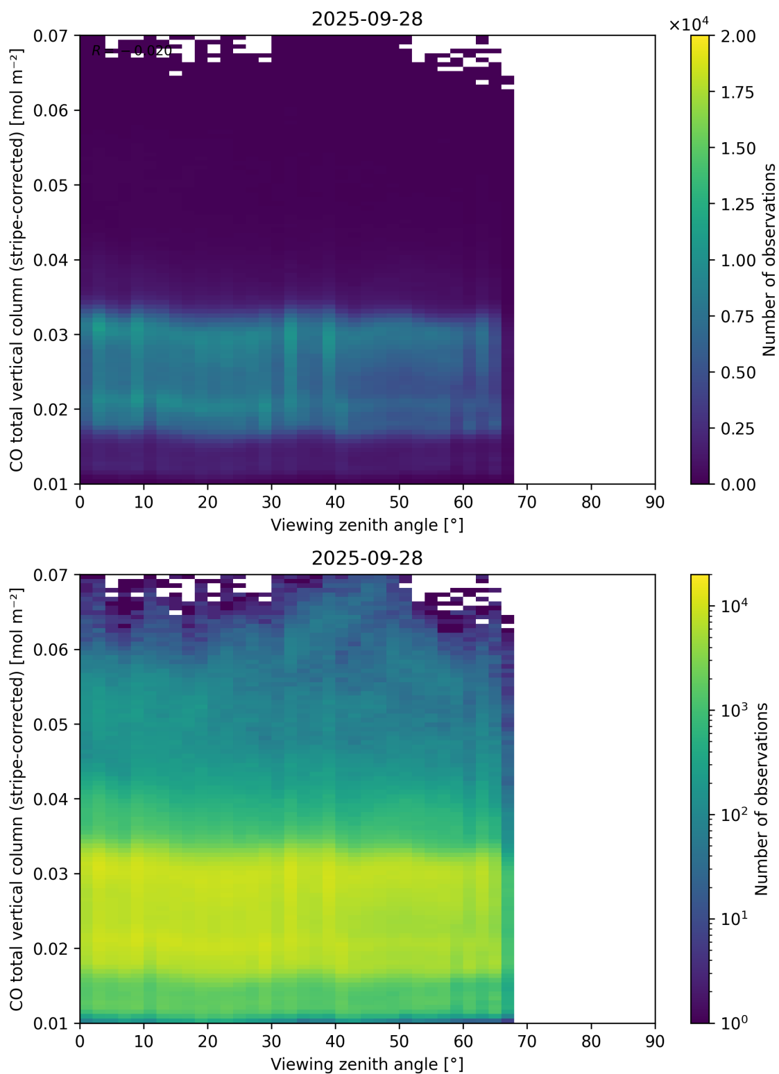
Figure 70: Scatter density plot of “Viewing zenith angle” against “CO total vertical column (stripe-corrected)” for 2025-09-27 to 2025-09-29.
