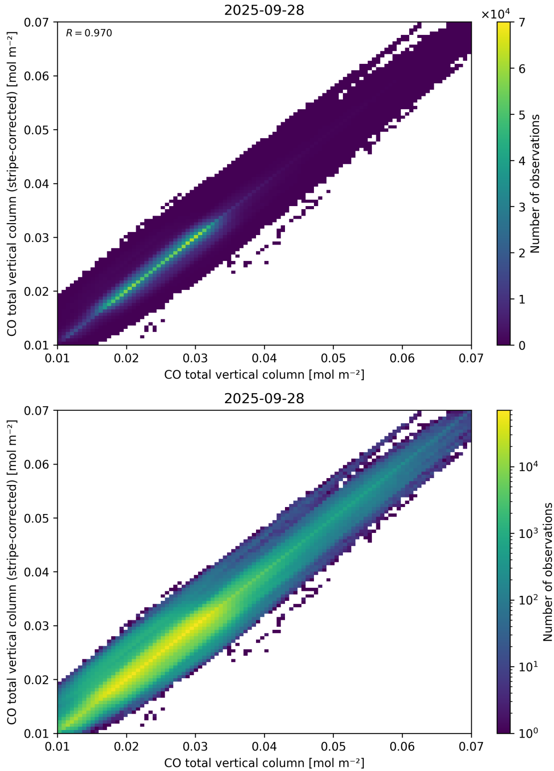
Figure 33: Scatter density plot of “CO total vertical column” against “CO total vertical column (stripe-corrected)” for 2025-09-27 to 2025-09-29.
