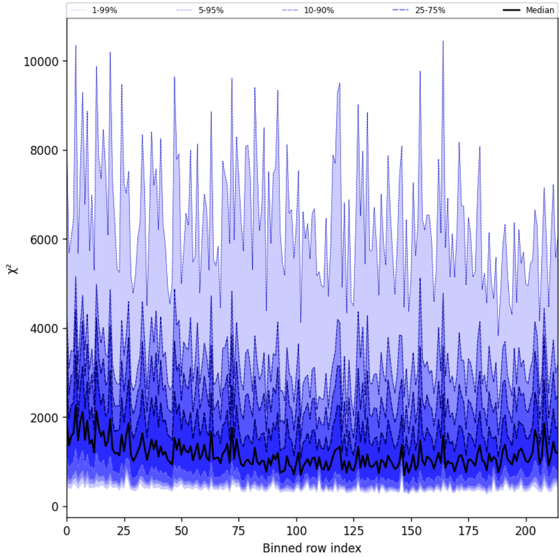
Figure 30: Along track statistics of “ \chi^2 ” for 2025-09-27 to 2025-09-29
