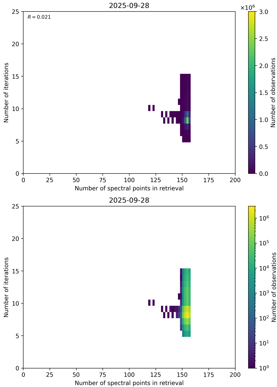
Figure 60: Scatter density plot of “Number of spectral points in retrieval” against “Number of iterations” for 2025-09-27 to 2025-09-29.
