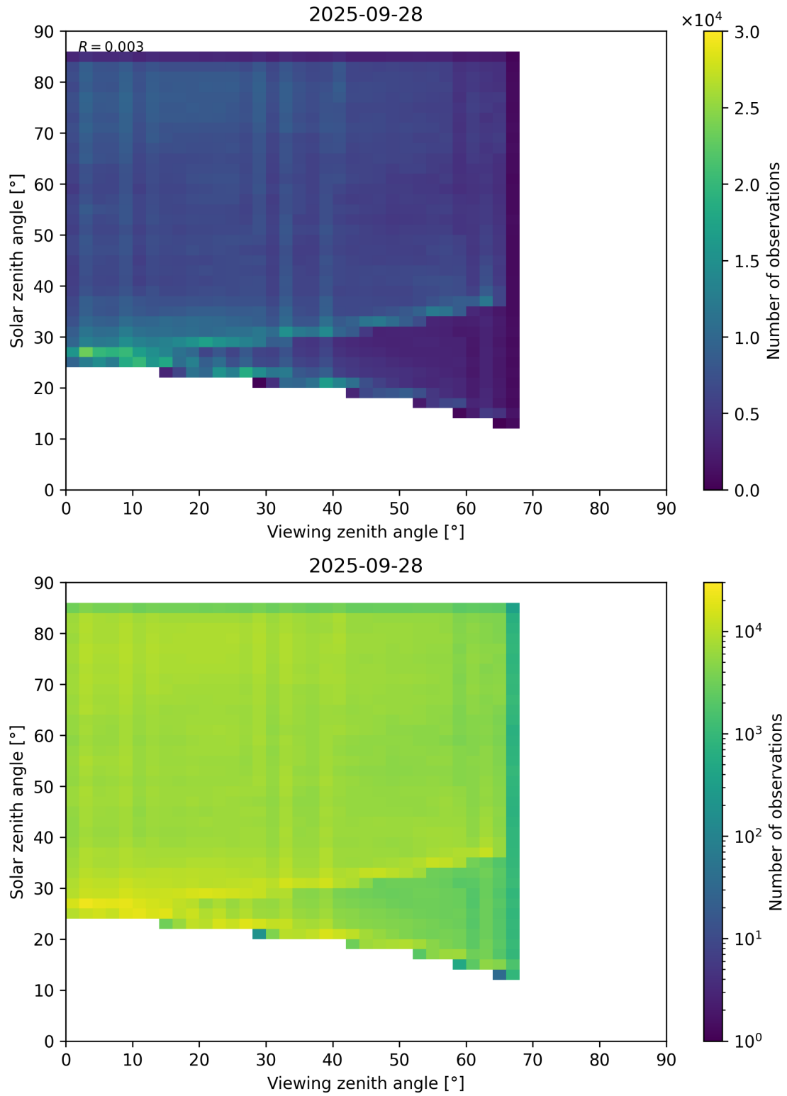
Figure 77: Scatter density plot of “Viewing zenith angle” against “Solar zenith angle” for 2025-09-27 to 2025-09-29.
