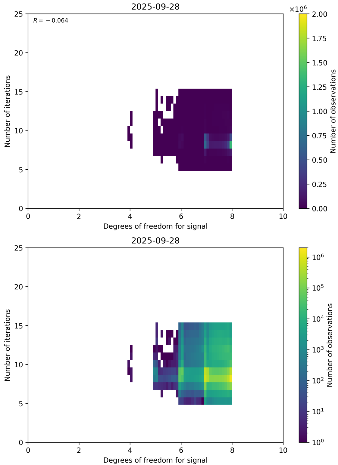
Figure 50: Scatter density plot of “Degrees of freedom for signal” against “Number of iterations” for 2025-09-27 to 2025-09-29.
