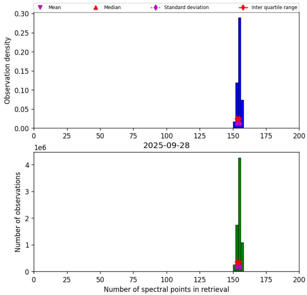
Figure 21: Histogram of “Number of spectral points in retrieval” for 2025-09-27 to 2025-09-29
