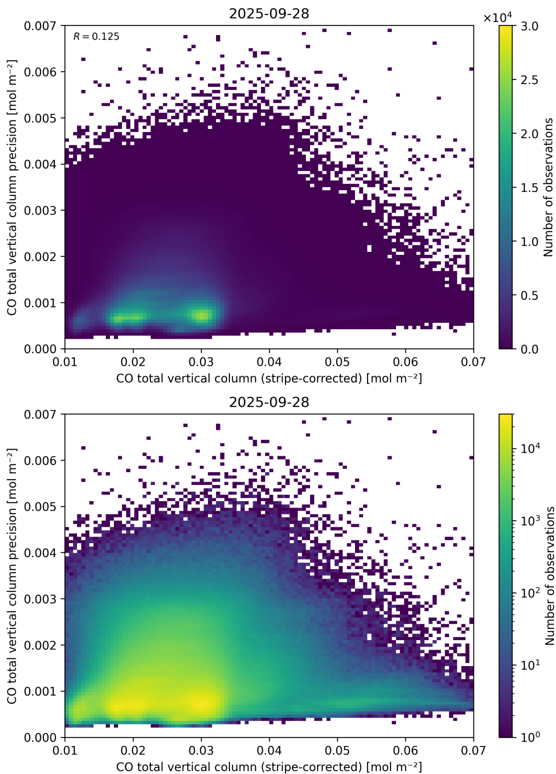
Figure 36: Scatter density plot of “CO total vertical column (stripe-corrected)” against “CO total vertical column precision” for 2025-09-27 to 2025-09-29.
