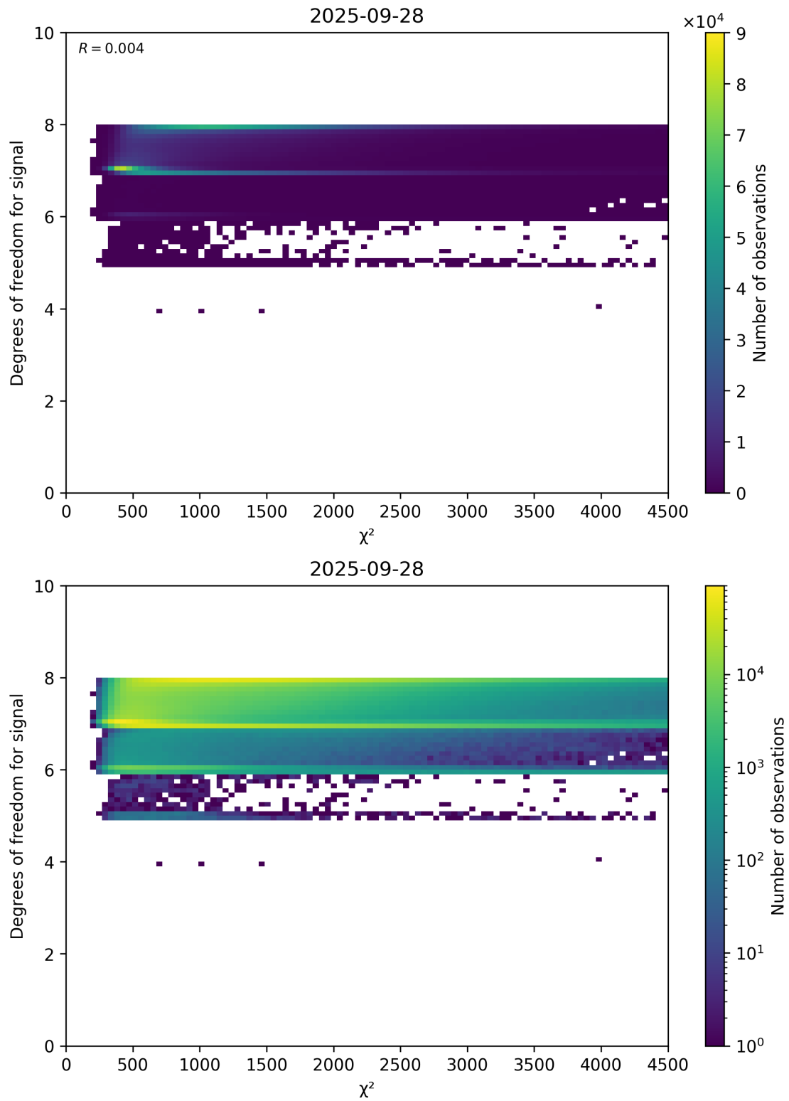
Figure 48: Scatter density plot of “ \chi^2 ” against “Degrees of freedom for signal” for 2025-09-27 to 2025-09-29.
