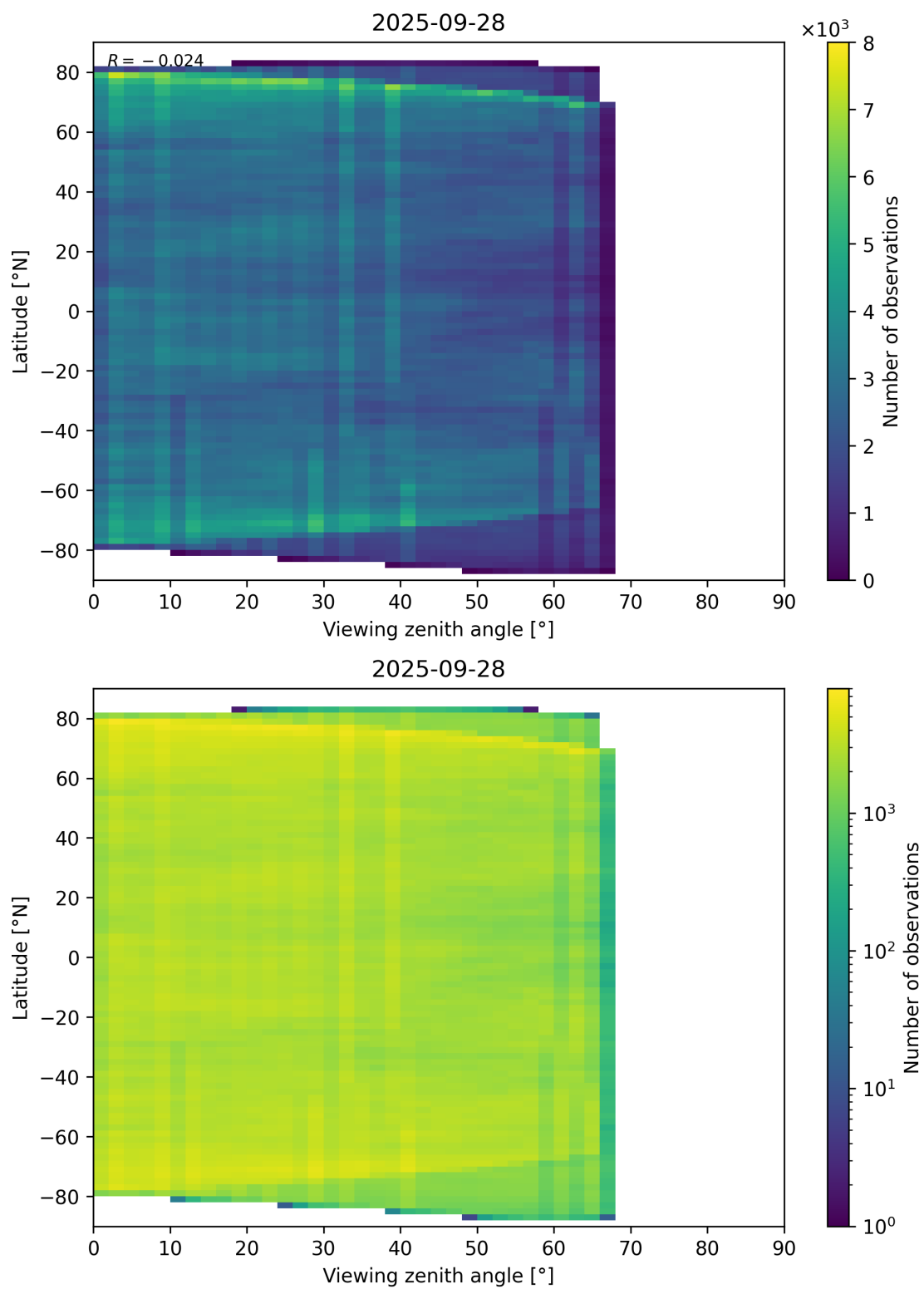
Figure 74: Scatter density plot of “Viewing zenith angle” against “Latitude” for 2025-09-27 to 2025-09-29.
