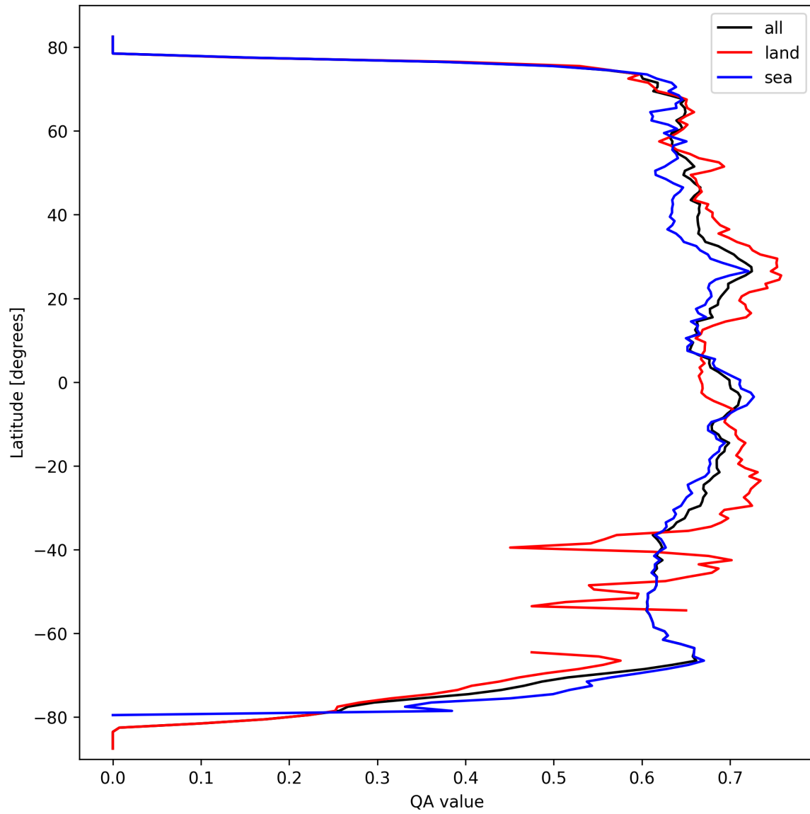
Figure 9: Zonal average of “QA value” for 2025-09-27 to 2025-09-29.
