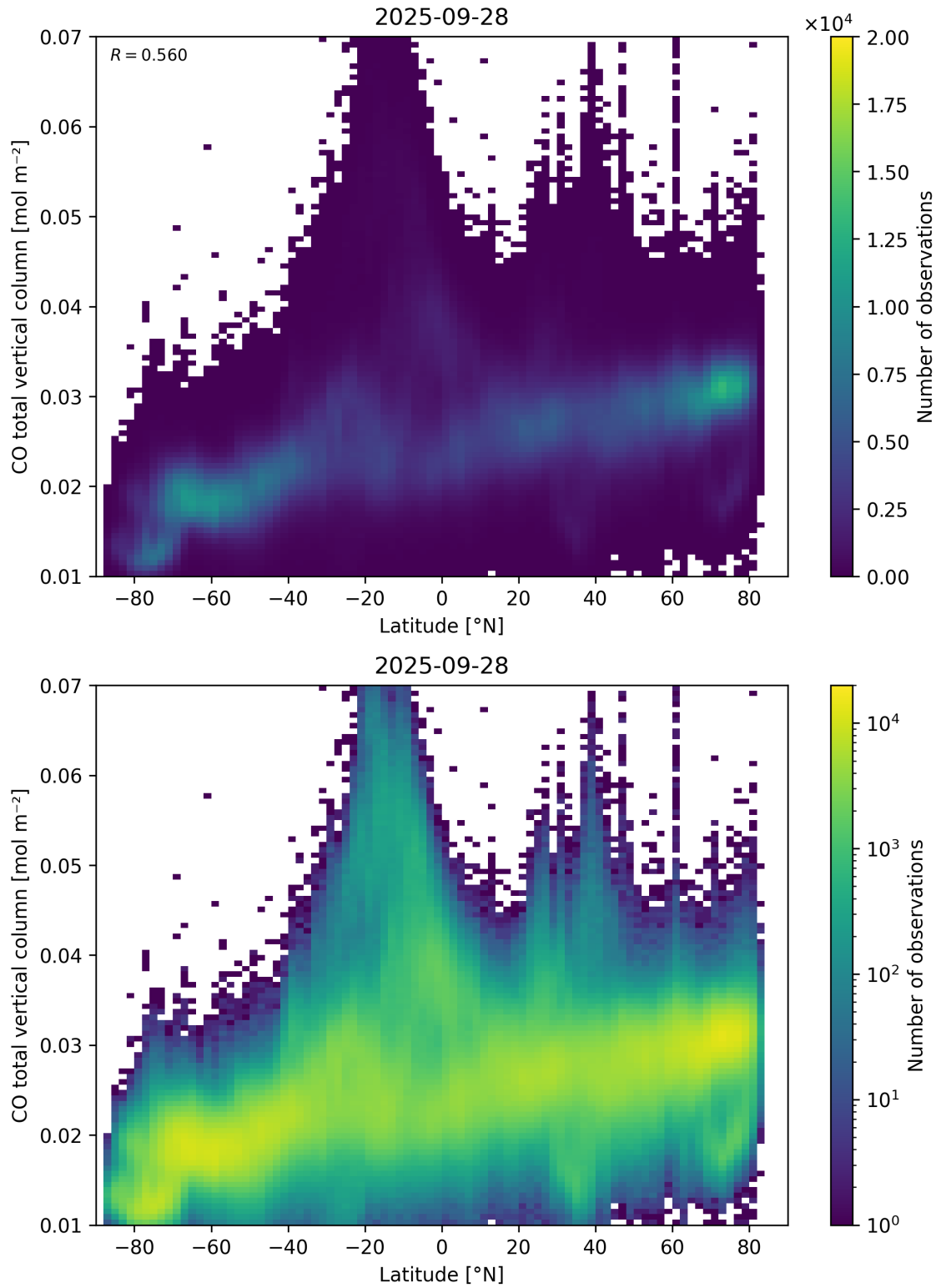
Figure 51: Scatter density plot of “Latitude” against “CO total vertical column” for 2025-09-27 to 2025-09-29.
