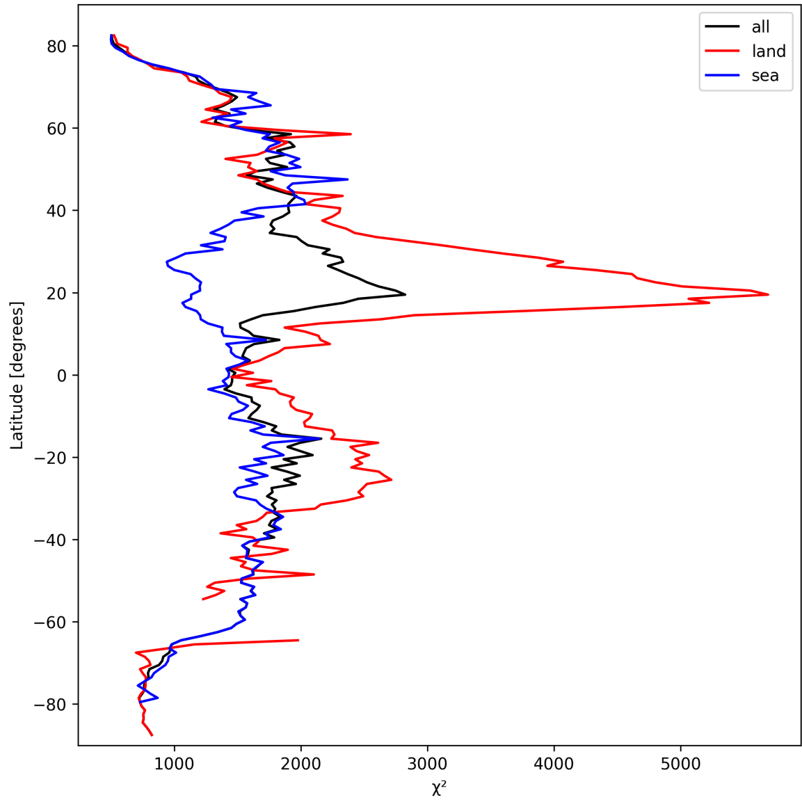
Figure 14: Zonal average of “ \chi^2 ” for 2025-09-27 to 2025-09-29.
