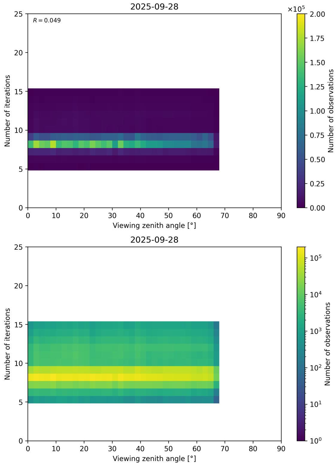
Figure 75: Scatter density plot of “Viewing zenith angle” against “Number of iterations” for 2025-09-27 to 2025-09-29.
