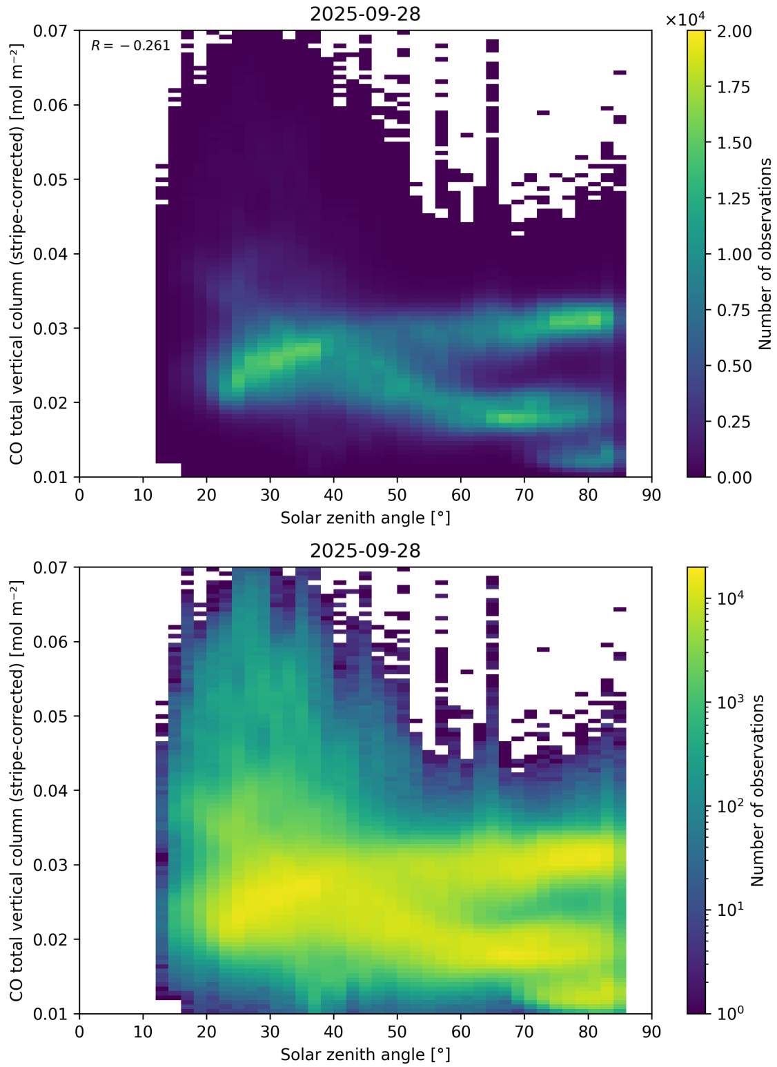
Figure 62: Scatter density plot of “Solar zenith angle” against “CO total vertical column (stripe-corrected)” for 2025-09-27 to 2025-09-29.
