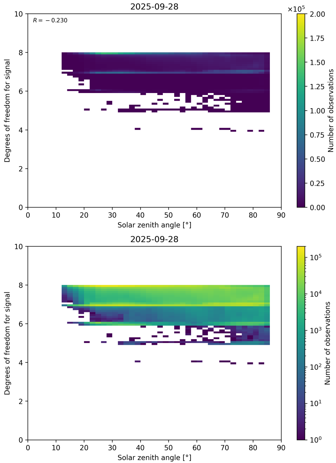
Figure 65: Scatter density plot of “Solar zenith angle” against “Degrees of freedom for signal” for 2025-09-27 to 2025-09-29.
