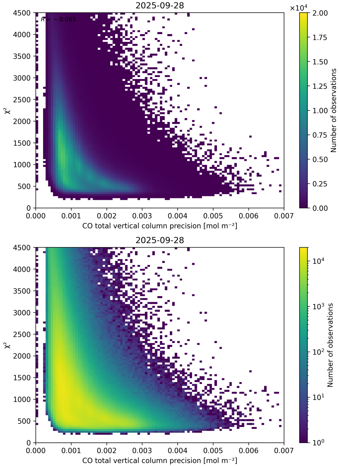
Figure 44: Scatter density plot of “CO total vertical column precision” against “ \chi^2 ” for 2025-09-27 to 2025-09-29.
