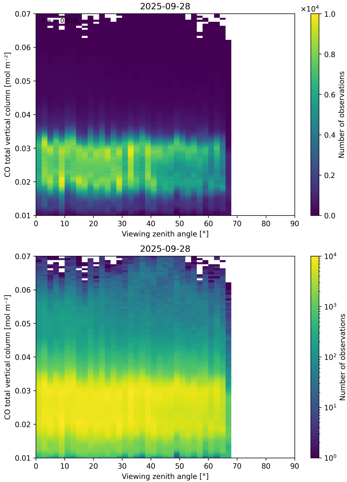
Figure 69: Scatter density plot of “Viewing zenith angle” against “CO total vertical column” for 2025-09-27 to 2025-09-29.
