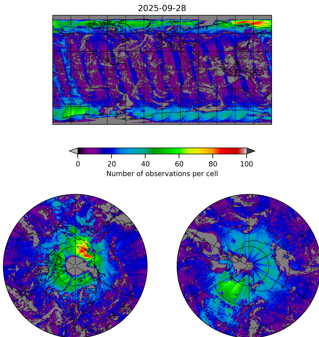
Figure 8: Map of the number of observations for 2025-09-27 to 2025-09-29
