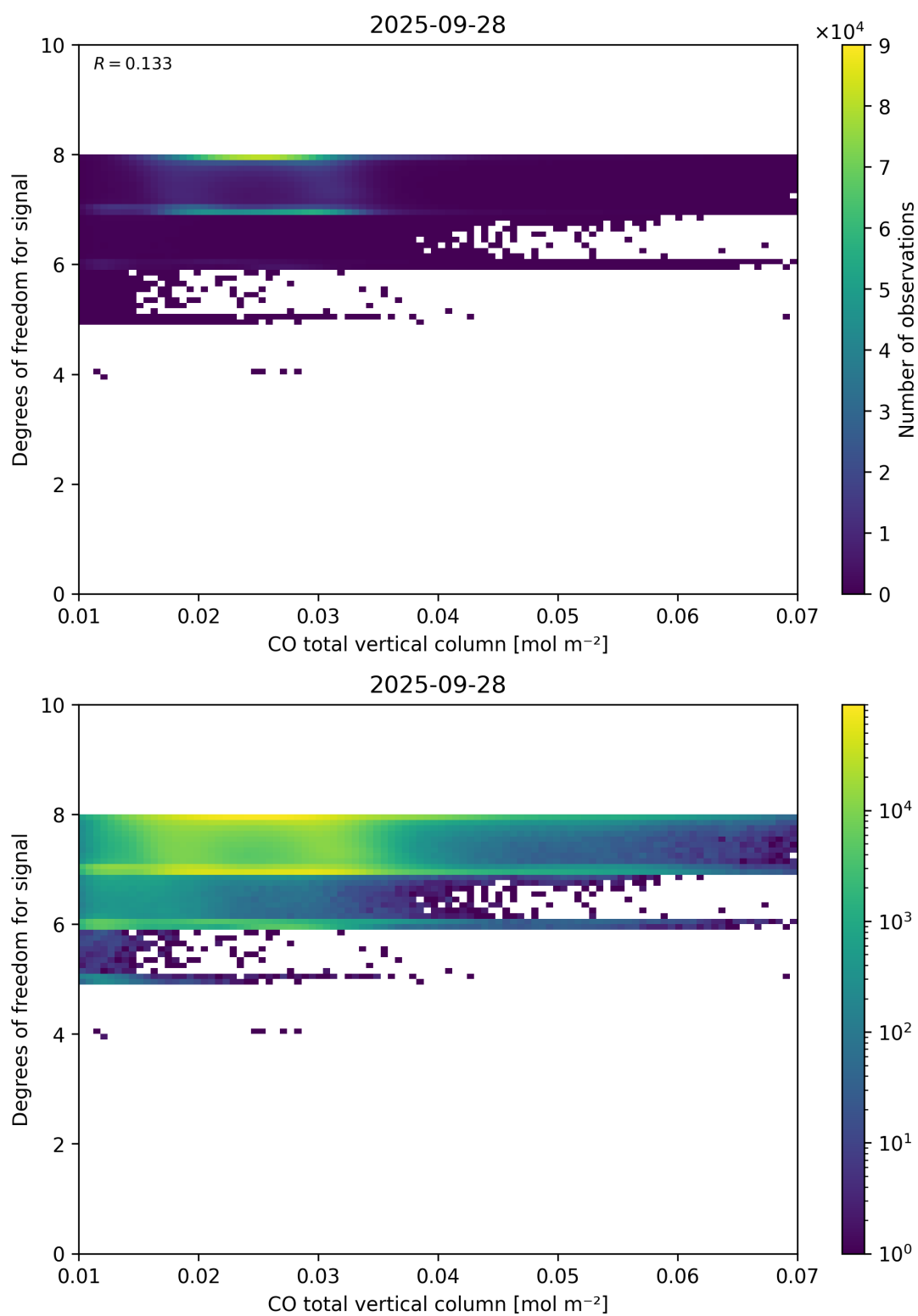
Figure 41: Scatter density plot of “CO total vertical column” against “Degrees of freedom for signal” for 2025-09-27 to 2025-09-29.
