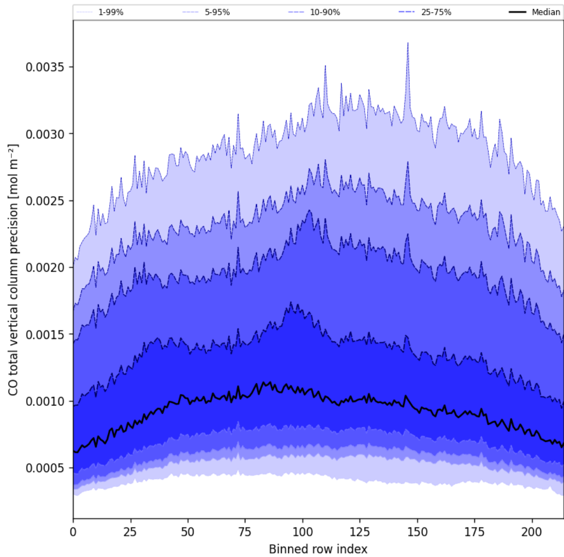
Figure 28: Along track statistics of “CO total vertical column precision” for 2025-09-27 to 2025-09-29
