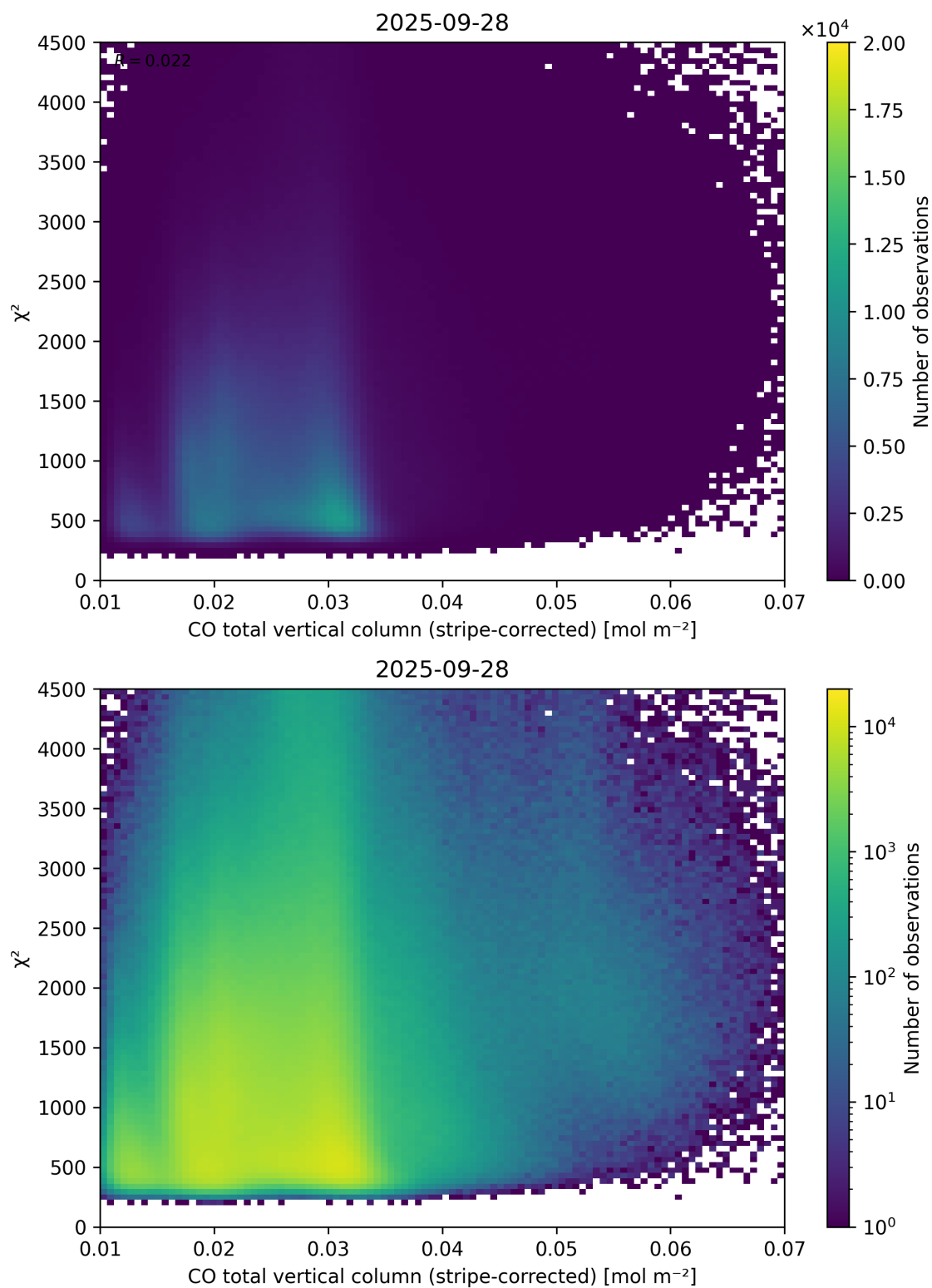
Figure 37: Scatter density plot of “CO total vertical column (stripe-corrected)” against “ \chi^2 ” for 2025-09-27 to 2025-09-29.
