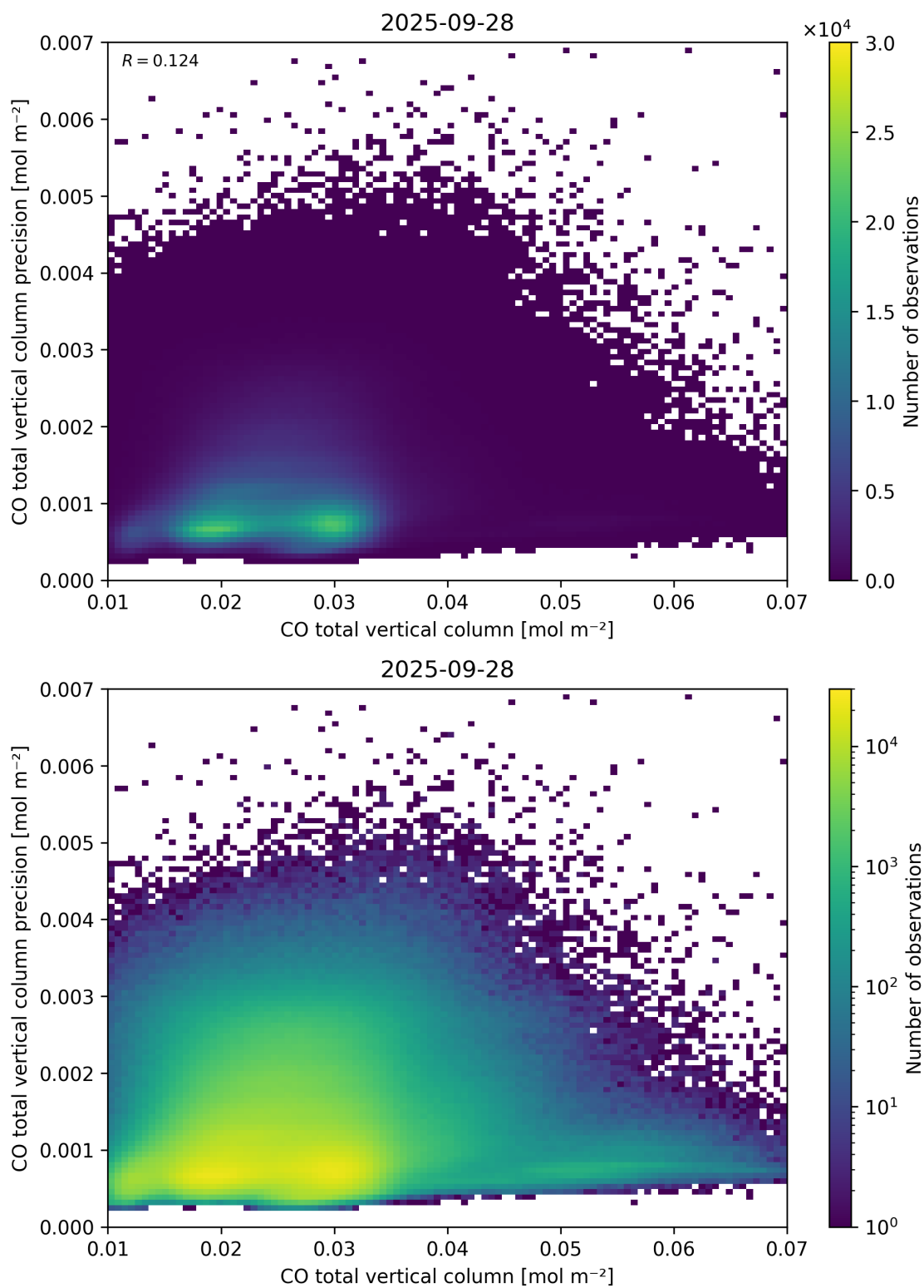
Figure 34: Scatter density plot of “CO total vertical column” against “CO total vertical column precision” for 2025-09-27 to 2025-09-29.
