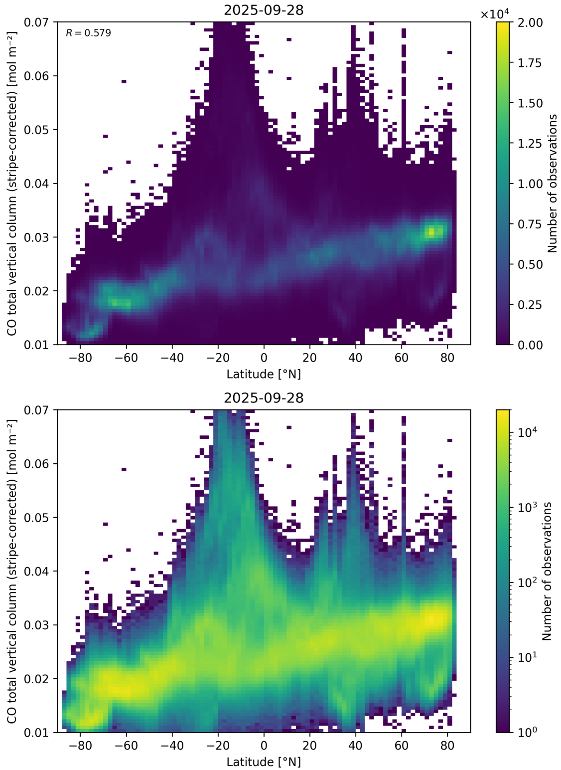
Figure 52: Scatter density plot of “Latitude” against “CO total vertical column (stripe-corrected)” for 2025-09-27 to 2025-09-29.
