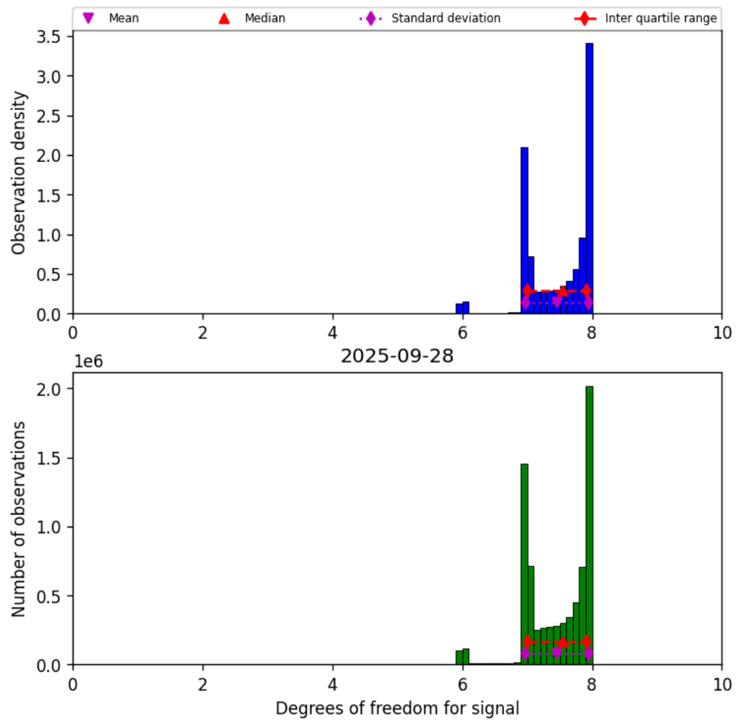
Figure 23: Histogram of “Degrees of freedom for signal” for 2025-09-27 to 2025-09-29
