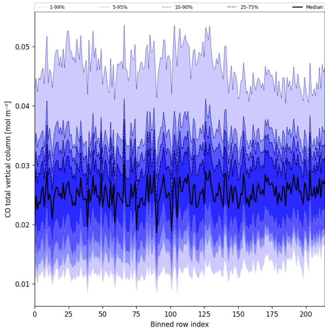
Figure 26: Along track statistics of “CO total vertical column” for 2025-09-27 to 2025-09-29
