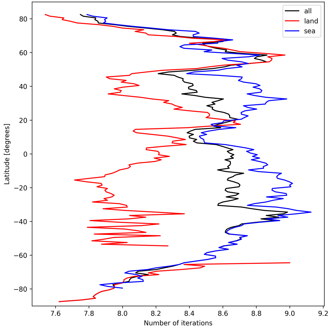
Figure 16: Zonal average of “Number of iterations” for 2025-09-27 to 2025-09-29.
