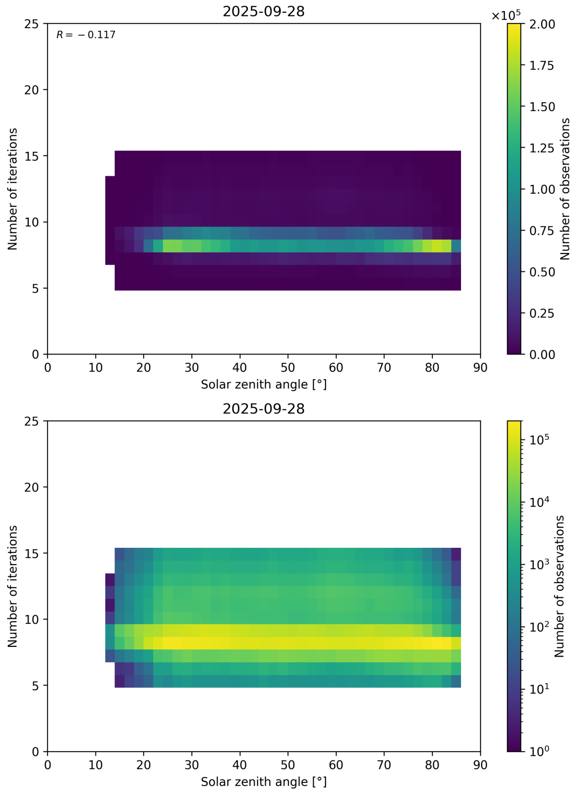
Figure 67: Scatter density plot of “Solar zenith angle” against “Number of iterations” for 2025-09-27 to 2025-09-29.
