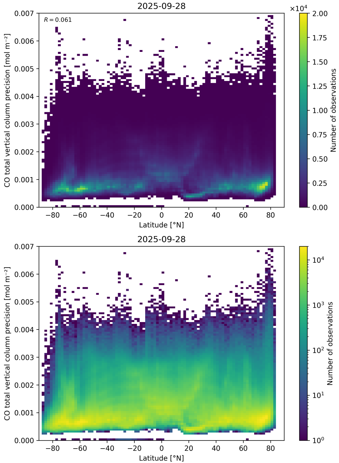
Figure 53: Scatter density plot of “Latitude” against “CO total vertical column precision” for 2025-09-27 to 2025-09-29.
