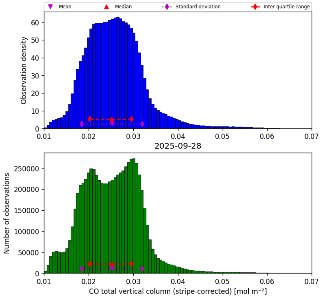
Figure 19: Histogram of “CO total vertical column (stripe-corrected)” for 2025-09-27 to 2025-09-29
