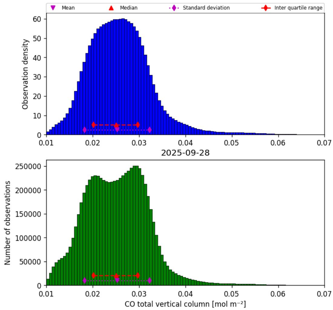
Figure 18: Histogram of “CO total vertical column” for 2025-09-27 to 2025-09-29
