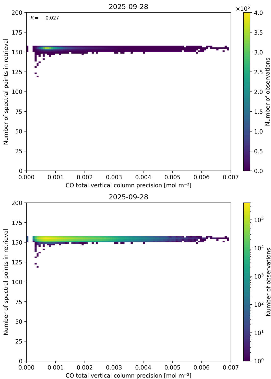
Figure 47: Scatter density plot of “CO total vertical column precision” against “Number of spectral points in retrieval” for 2025-09-27 to 2025-09-29.
