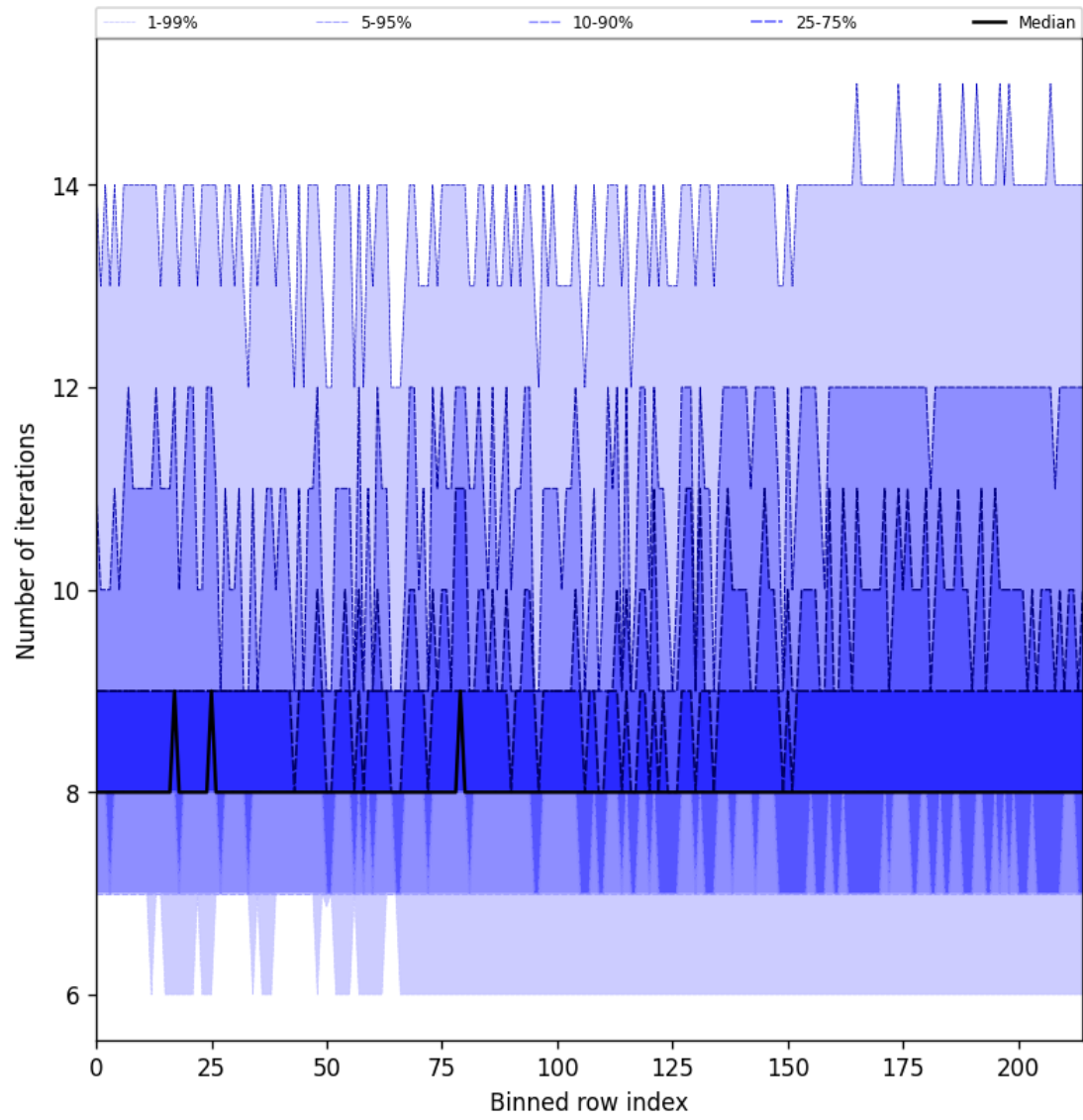
Figure 32: Along track statistics of “Number of iterations” for 2025-09-27 to 2025-09-29
