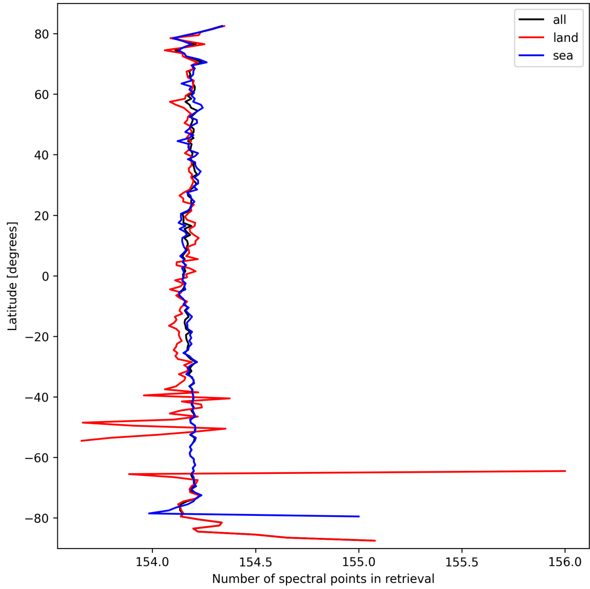
Figure 13: Zonal average of “Number of spectral points in retrieval” for 2025-09-27 to 2025-09-29.
