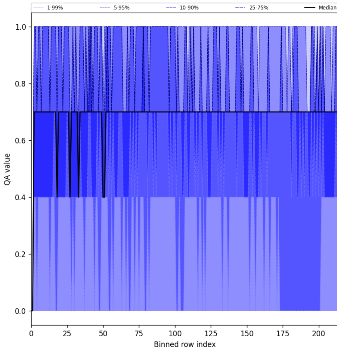
Figure 25: Along track statistics of “QA value” for 2025-09-27 to 2025-09-29
