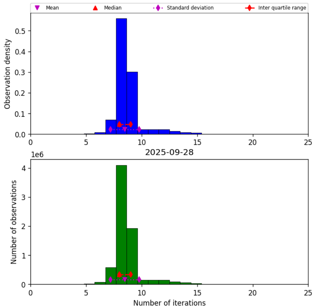
Figure 24: Histogram of “Number of iterations” for 2025-09-27 to 2025-09-29
