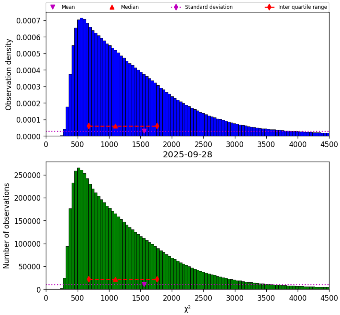
Figure 22: Histogram of “ \chi^2 ” for 2025-09-27 to 2025-09-29
