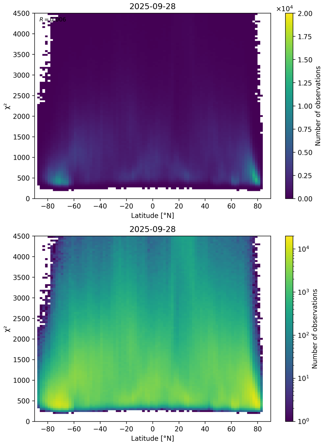
Figure 54: Scatter density plot of “Latitude” against “ \chi^2 ” for 2025-09-27 to 2025-09-29.
