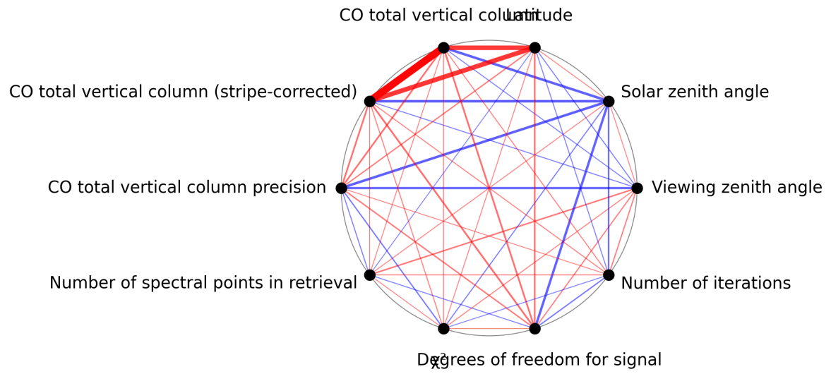
Figure 1: Map of correlation graph for 2025-09-27 to 2025-09-29.
