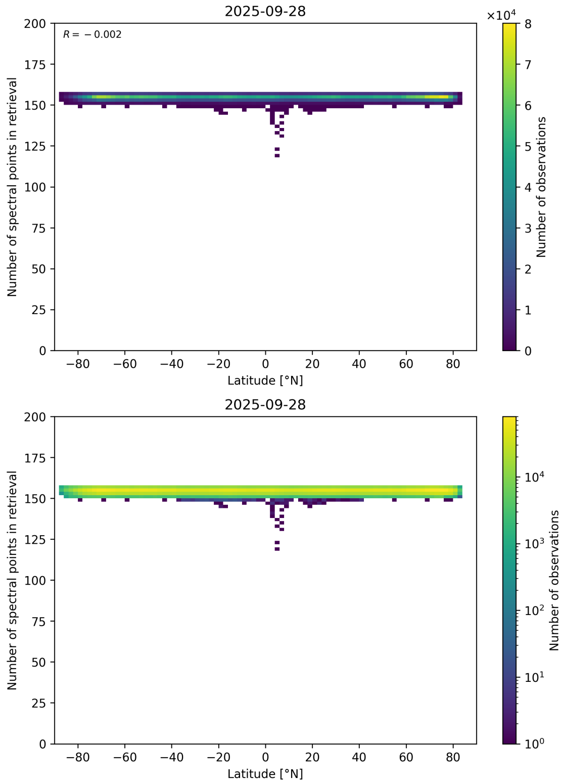
Figure 57: Scatter density plot of “Latitude” against “Number of spectral points in retrieval” for 2025-09-27 to 2025-09-29.
