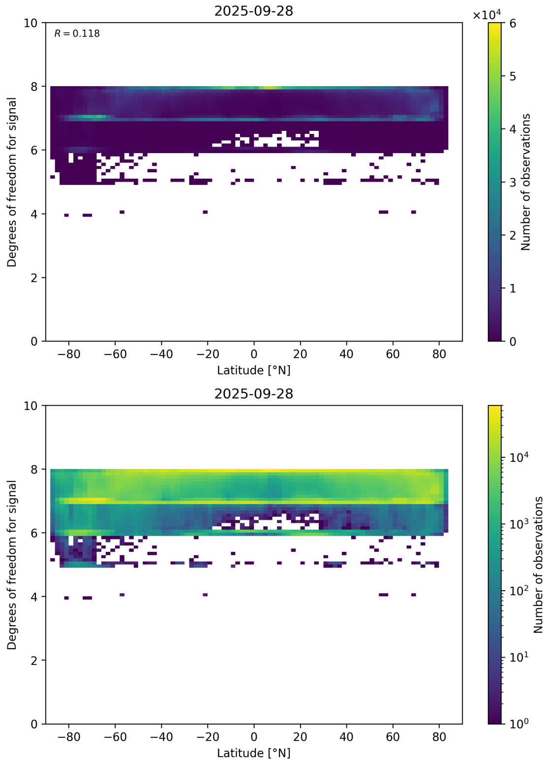
Figure 55: Scatter density plot of “Latitude” against “Degrees of freedom for signal” for 2025-09-27 to 2025-09-29.
