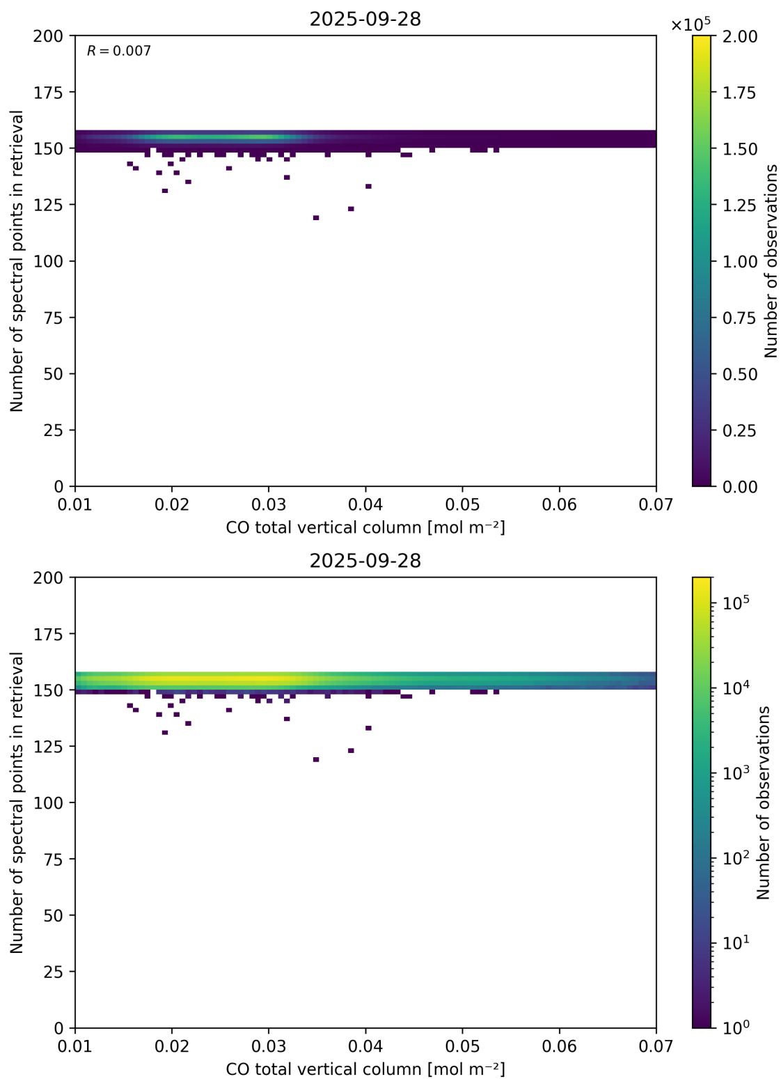
Figure 43: Scatter density plot of “CO total vertical column” against “Number of spectral points in retrieval” for 2025-09-27 to 2025-09-29.
