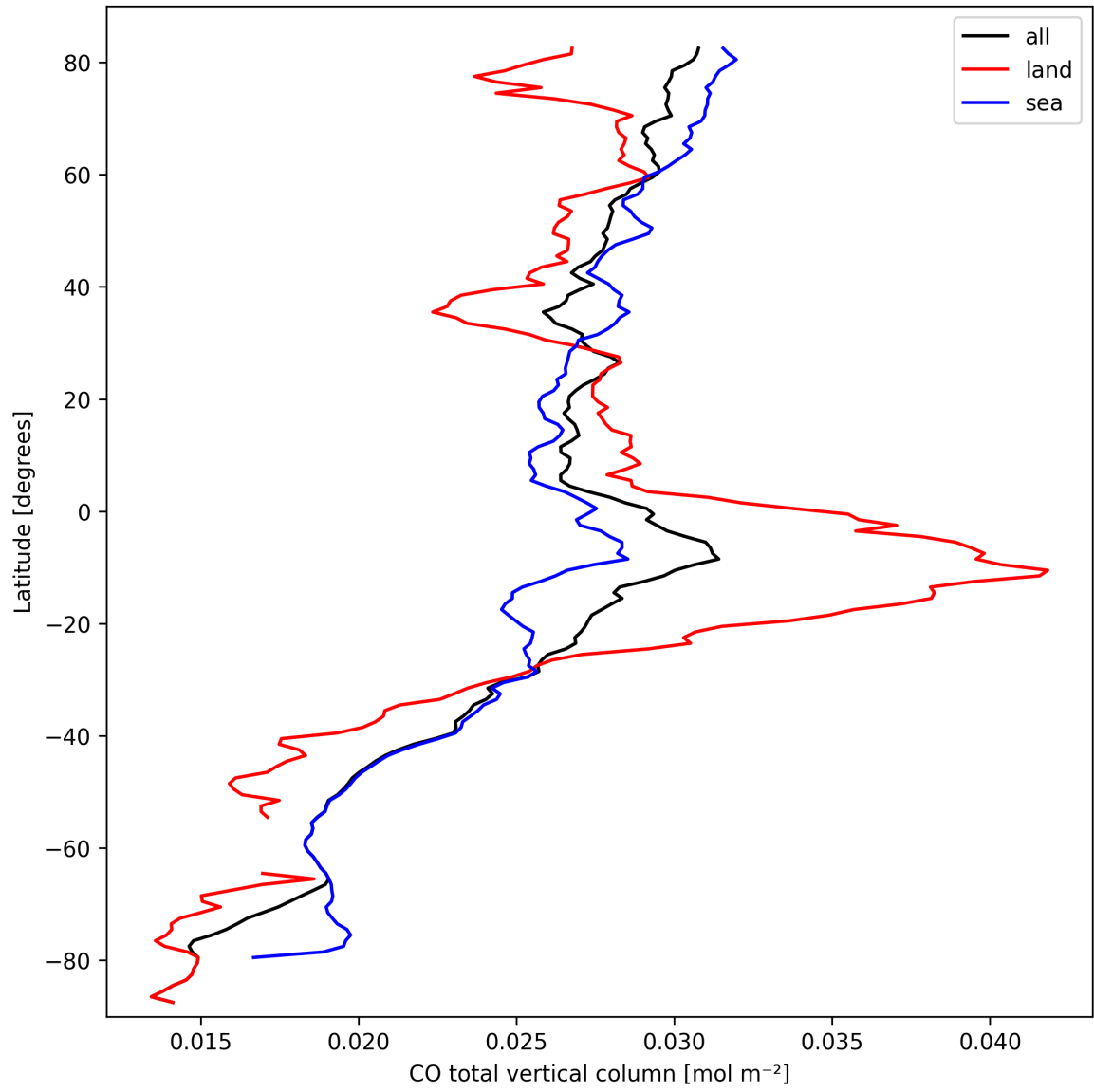
Figure 10: Zonal average of “CO total vertical column” for 2025-09-27 to 2025-09-29.
