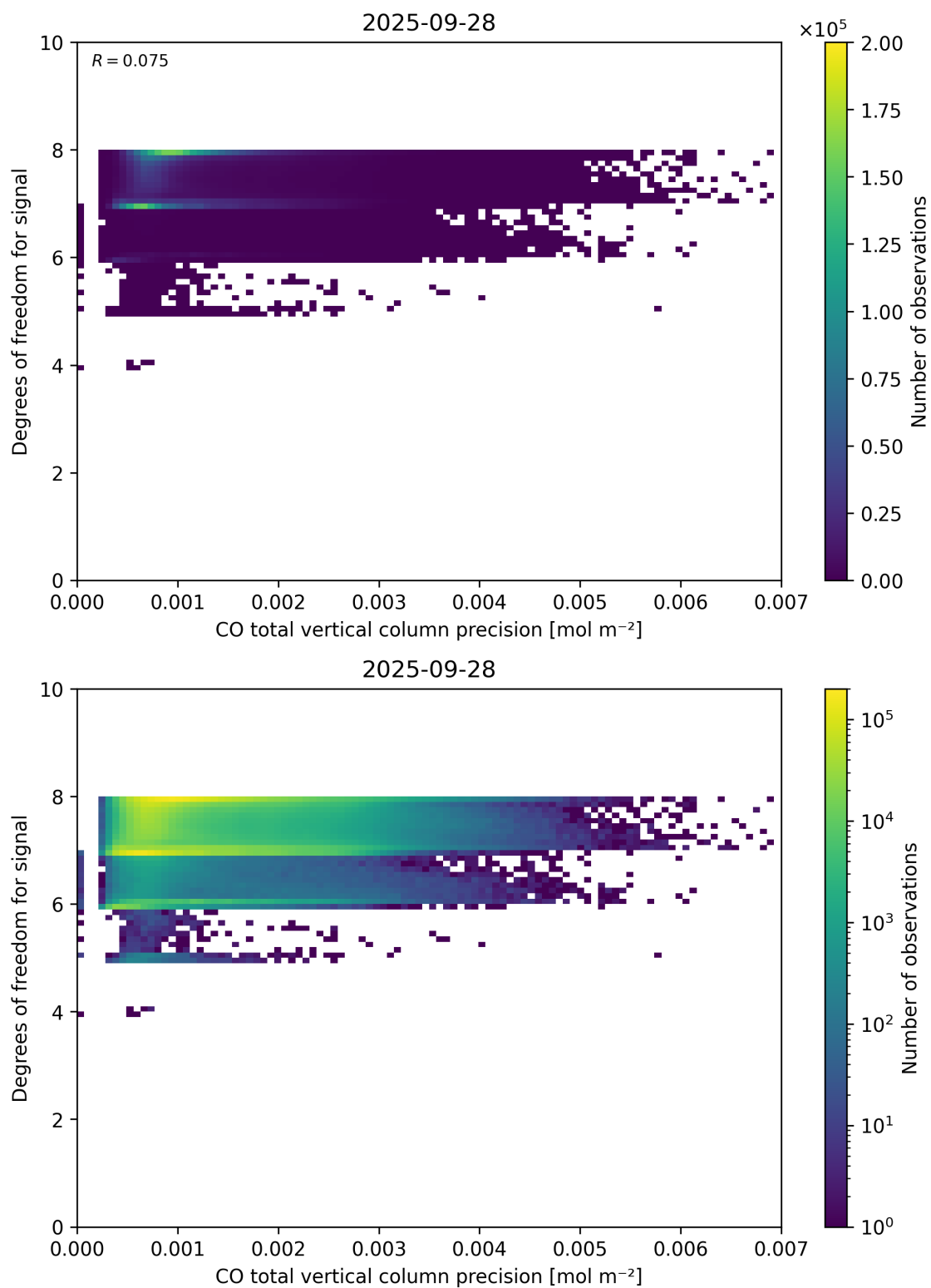
Figure 45: Scatter density plot of “CO total vertical column precision” against “Degrees of freedom for signal” for 2025-09-27 to 2025-09-29.
