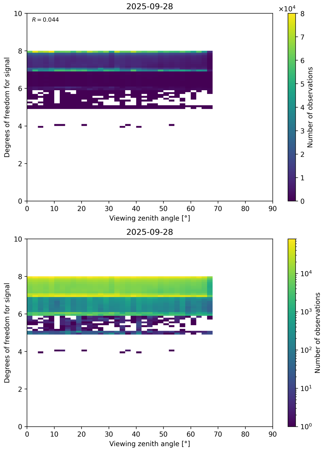
Figure 73: Scatter density plot of “Viewing zenith angle” against “Degrees of freedom for signal” for 2025-09-27 to 2025-09-29.
