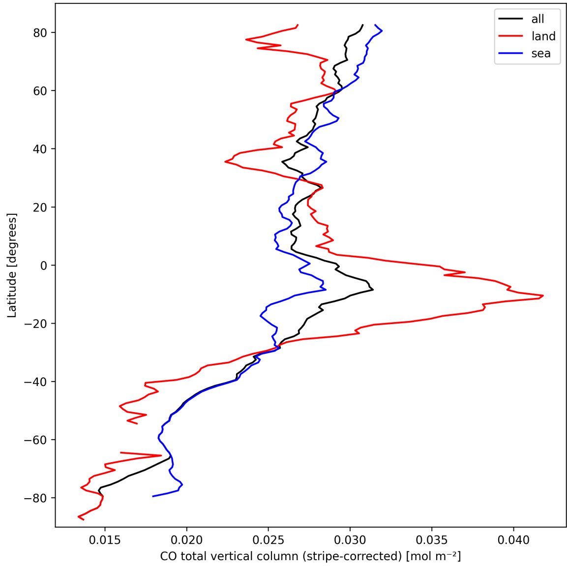
Figure 11: Zonal average of “CO total vertical column (stripe-corrected)” for 2025-09-27 to 2025-09-29.
