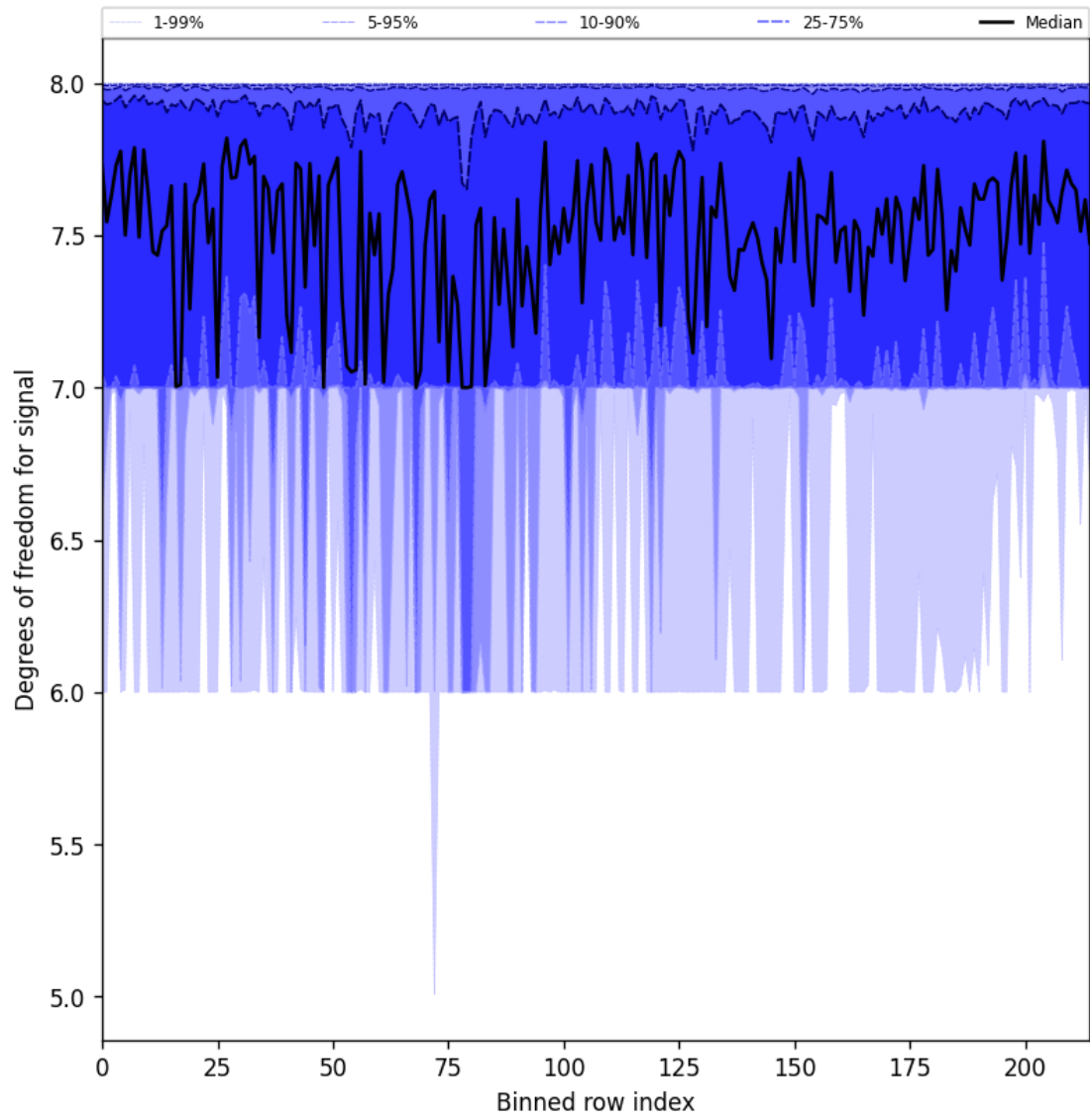
Figure 31: Along track statistics of “Degrees of freedom for signal” for 2025-09-27 to 2025-09-29
