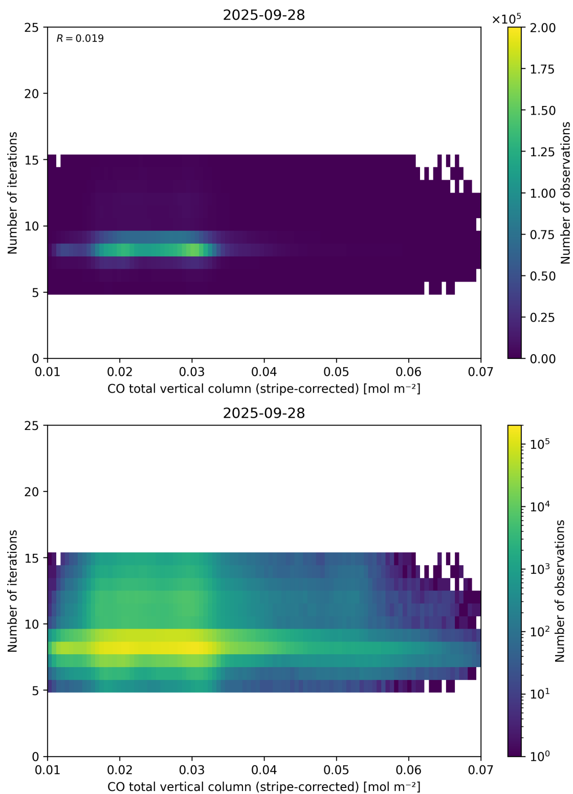
Figure 39: Scatter density plot of “CO total vertical column (stripe-corrected)” against “Number of iterations” for 2025-09-27 to 2025-09-29.
