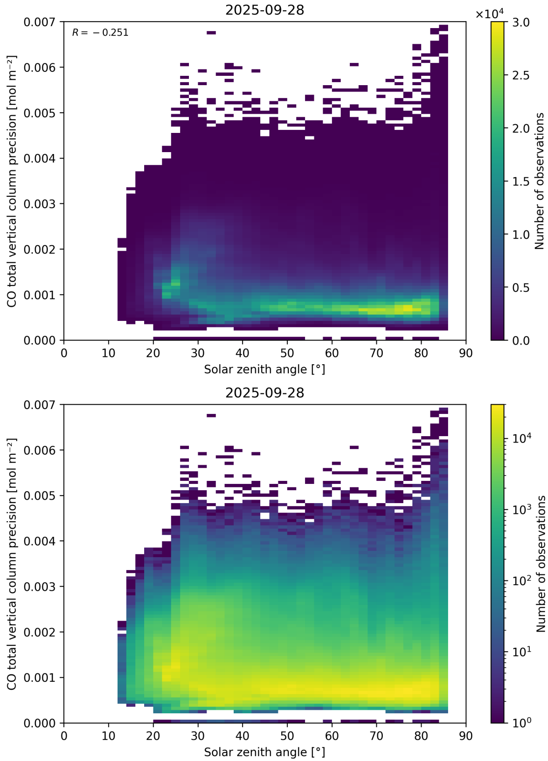
Figure 63: Scatter density plot of “Solar zenith angle” against “CO total vertical column precision” for 2025-09-27 to 2025-09-29.
