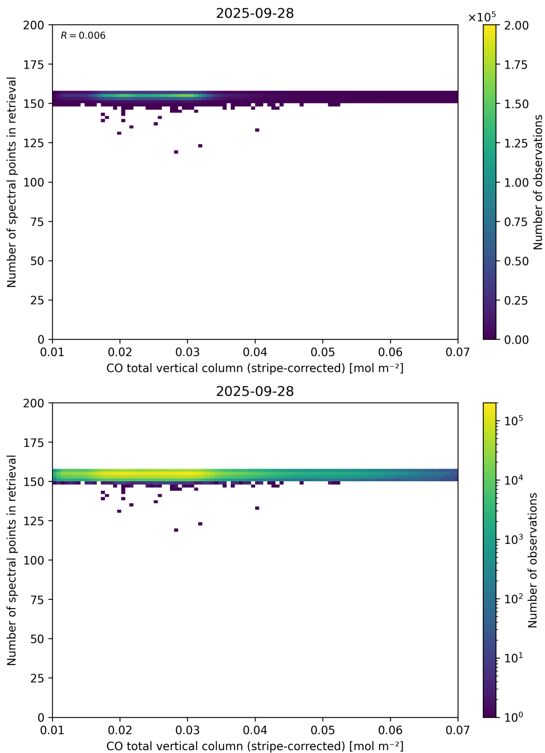
Figure 40: Scatter density plot of “CO total vertical column (stripe-corrected)” against “Number of spectral points in retrieval” for 2025-09-27 to 2025-09-29.
