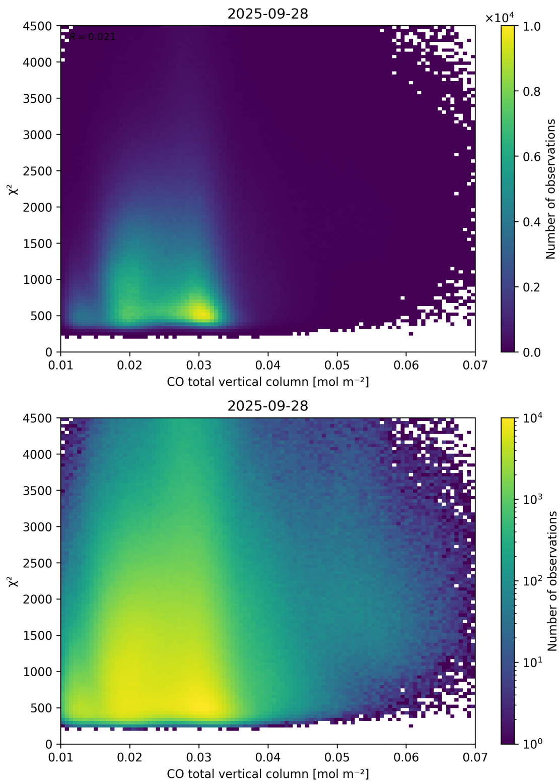
Figure 35: Scatter density plot of “CO total vertical column” against “ \chi^2 ” for 2025-09-27 to 2025-09-29.
