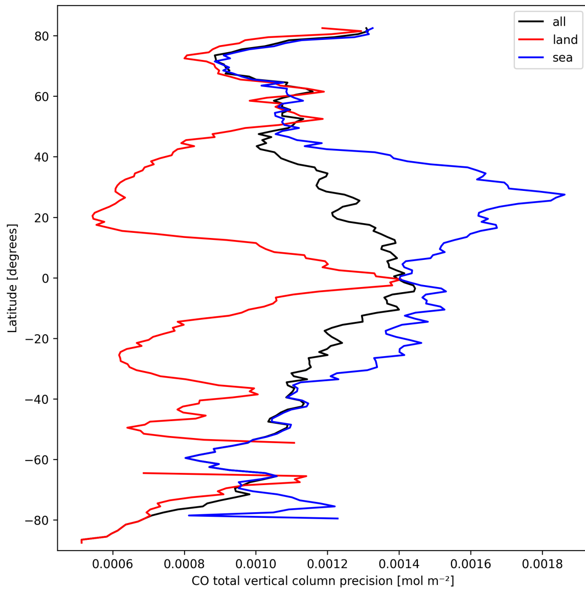
Figure 12: Zonal average of “CO total vertical column precision” for 2025-09-27 to 2025-09-29.
