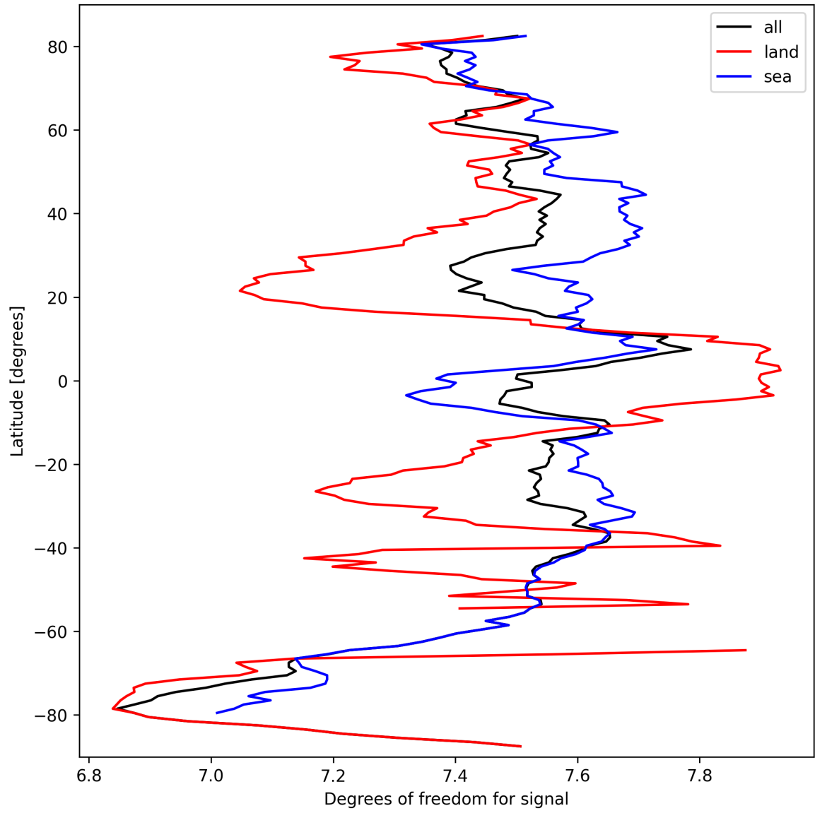
Figure 15: Zonal average of “Degrees of freedom for signal” for 2025-09-27 to 2025-09-29.
