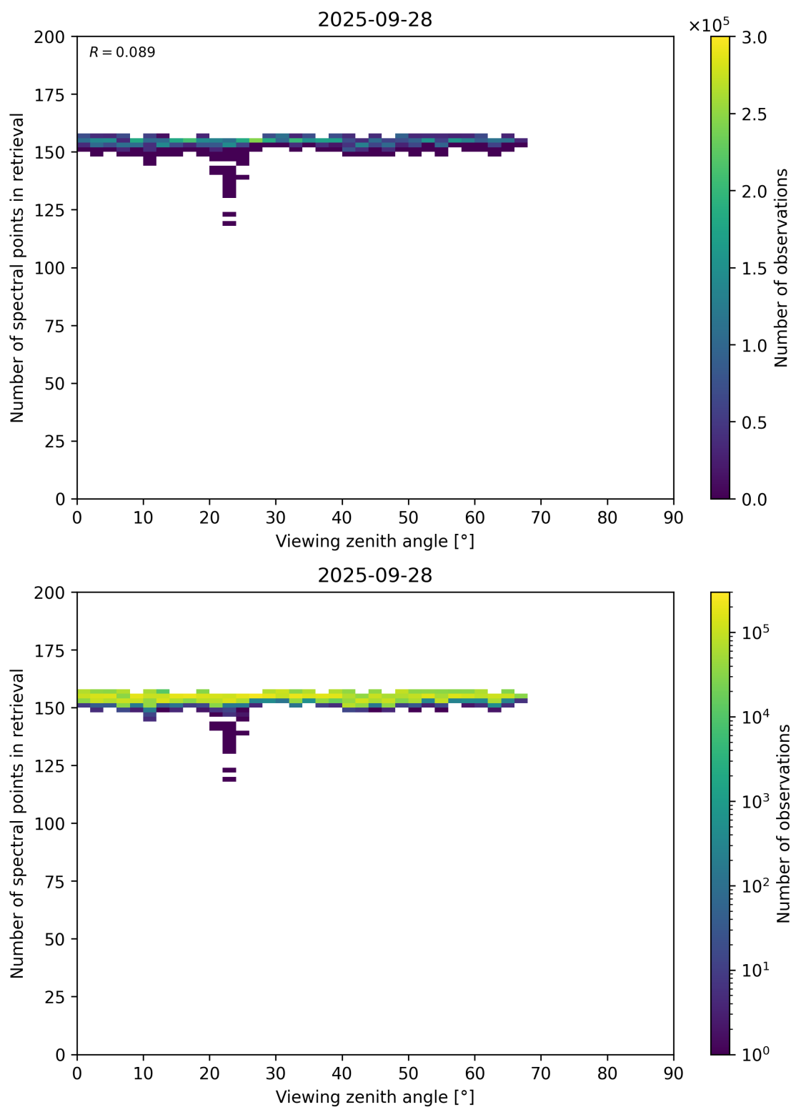
Figure 76: Scatter density plot of “Viewing zenith angle” against “Number of spectral points in retrieval” for 2025-09-27 to 2025-09-29.
