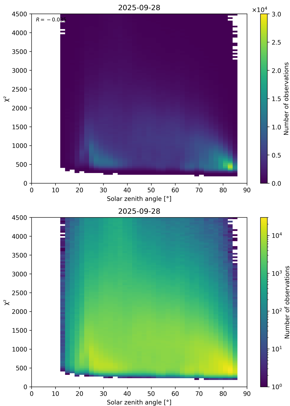
Figure 64: Scatter density plot of “Solar zenith angle” against “ \chi^2 ” for 2025-09-27 to 2025-09-29.
