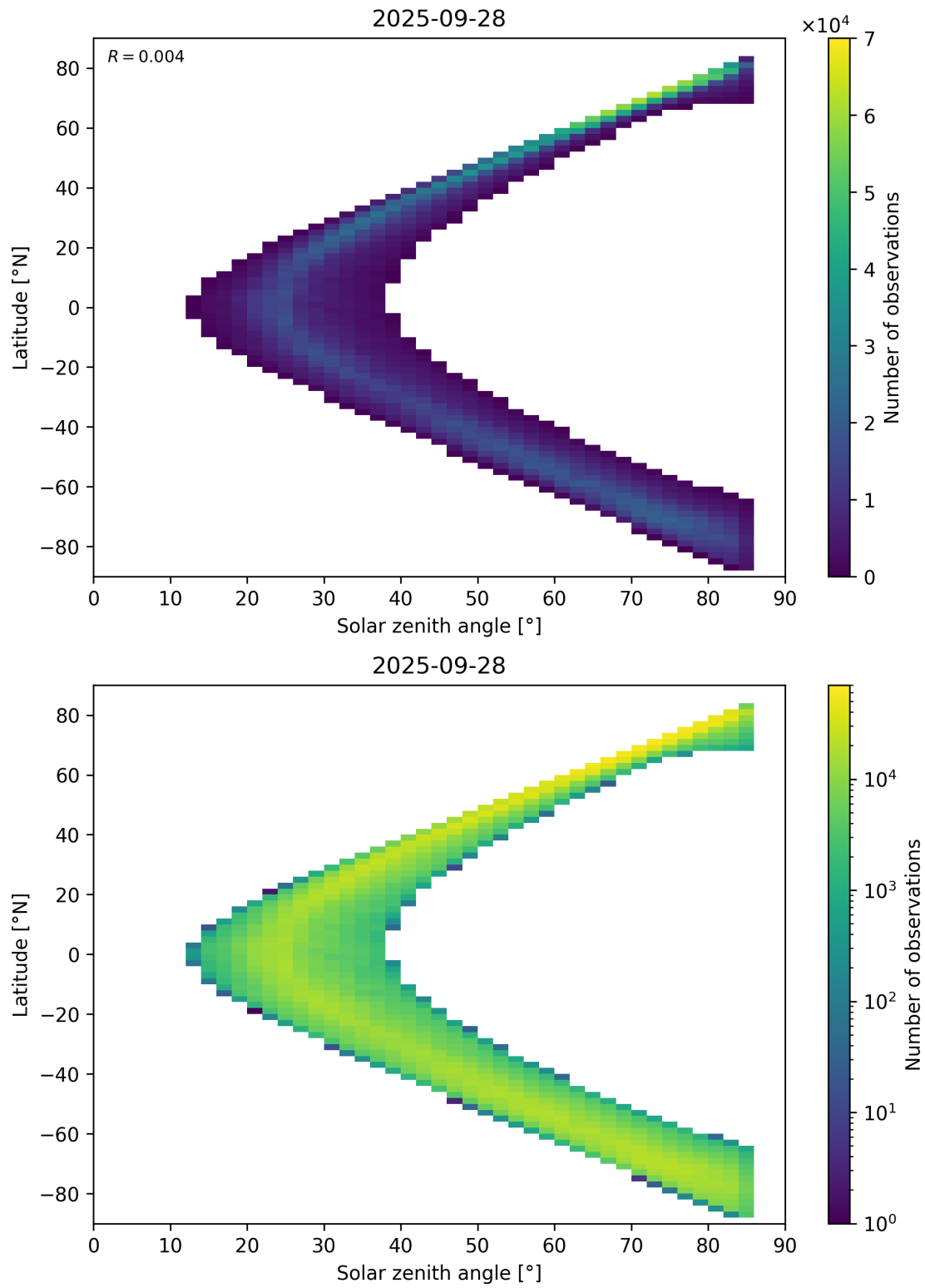
Figure 66: Scatter density plot of “Solar zenith angle” against “Latitude” for 2025-09-27 to 2025-09-29.
