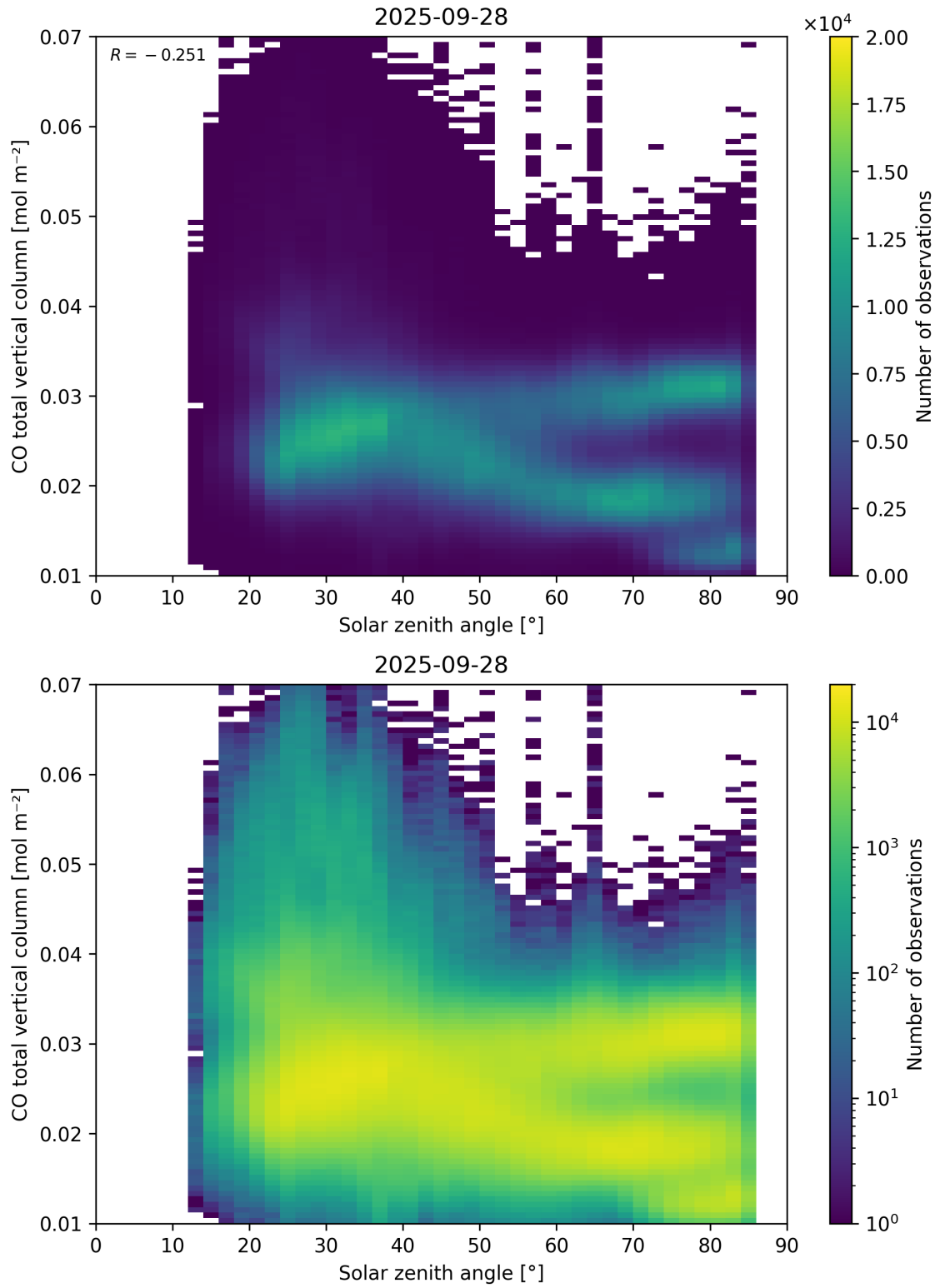
Figure 61: Scatter density plot of “Solar zenith angle” against “CO total vertical column” for 2025-09-27 to 2025-09-29.
