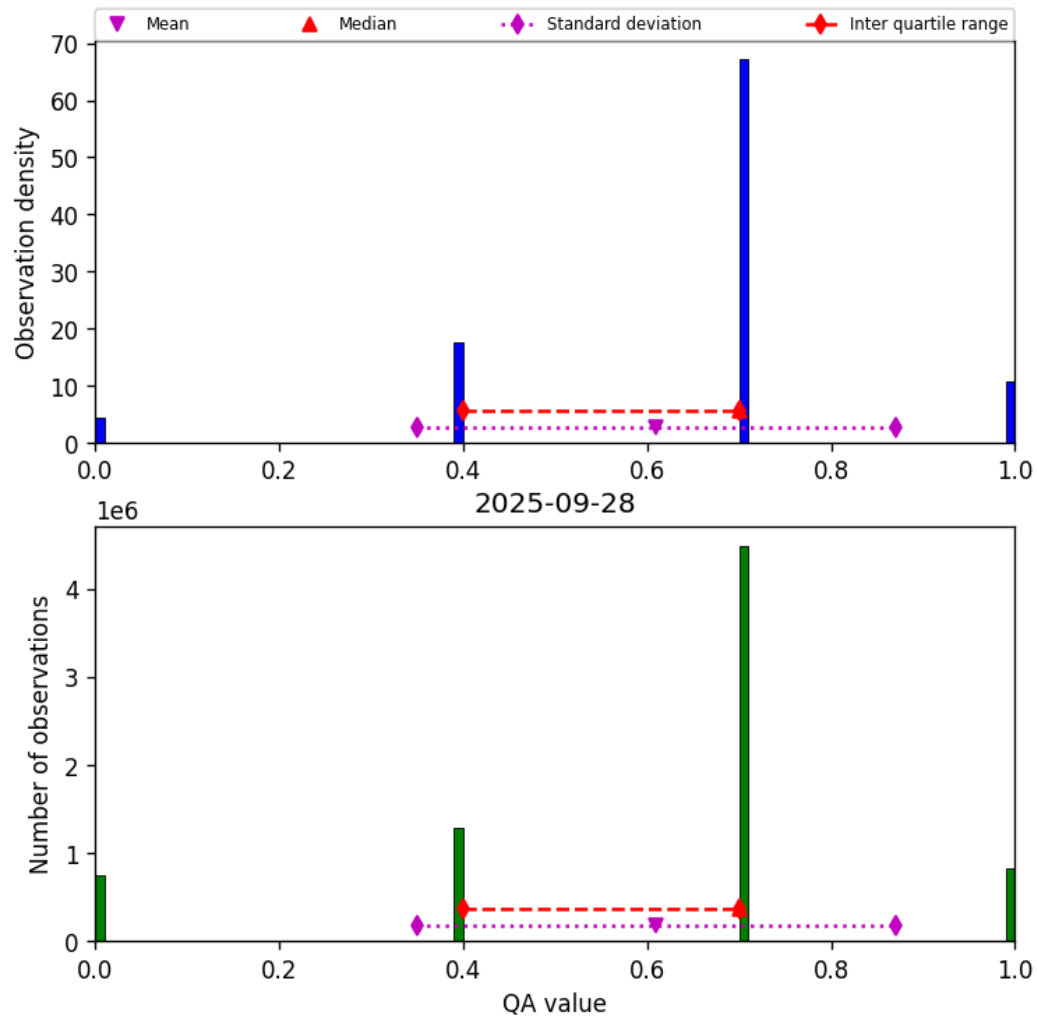
Figure 17: Histogram of “QA value” for 2025-09-27 to 2025-09-29
