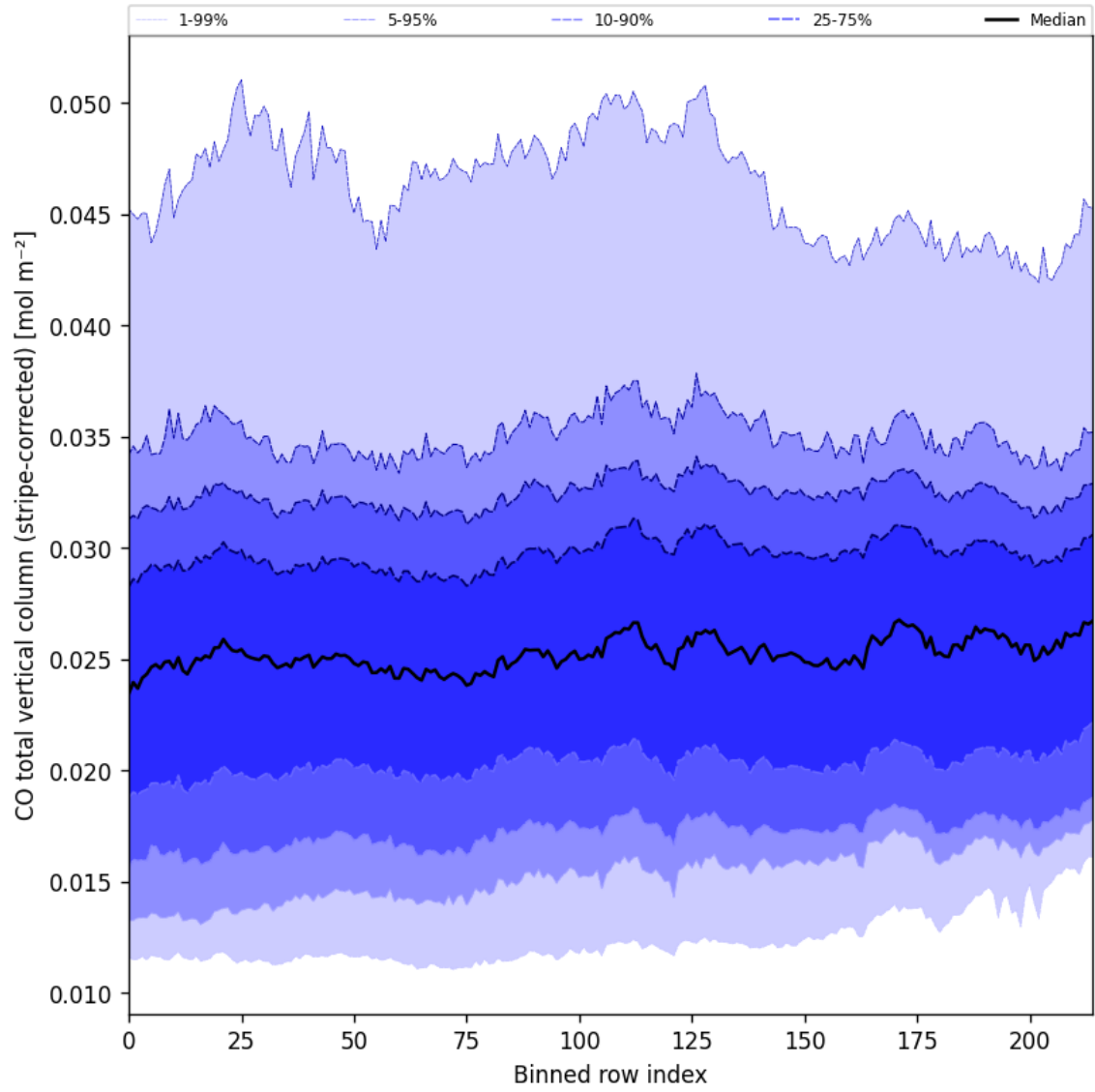
Figure 27: Along track statistics of “CO total vertical column (stripe-corrected)” for 2025-09-27 to 2025-09-29
