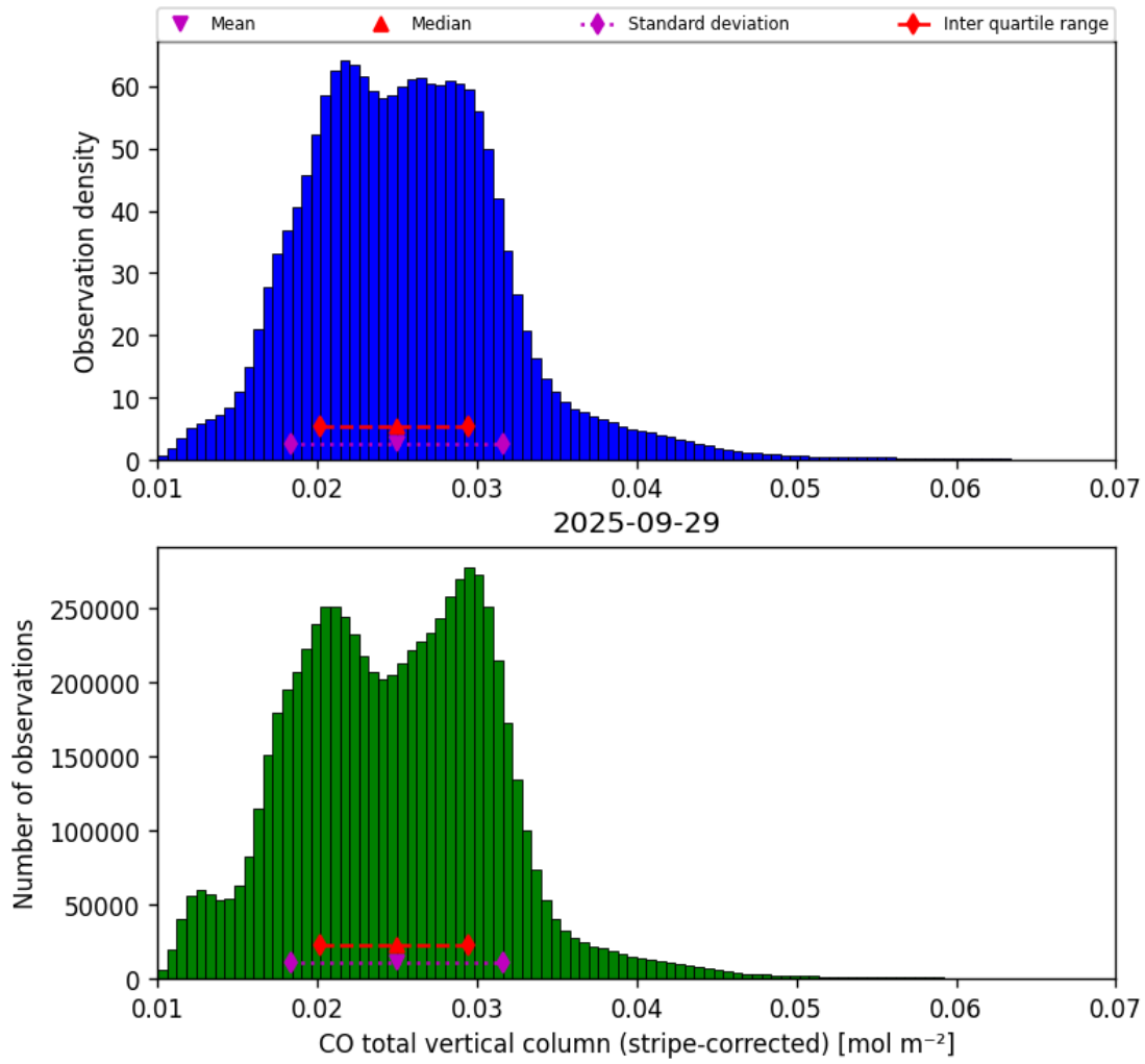
Figure 19: Histogram of “CO total vertical column (stripe-corrected)” for 2025-09-28 to 2025-09-30
