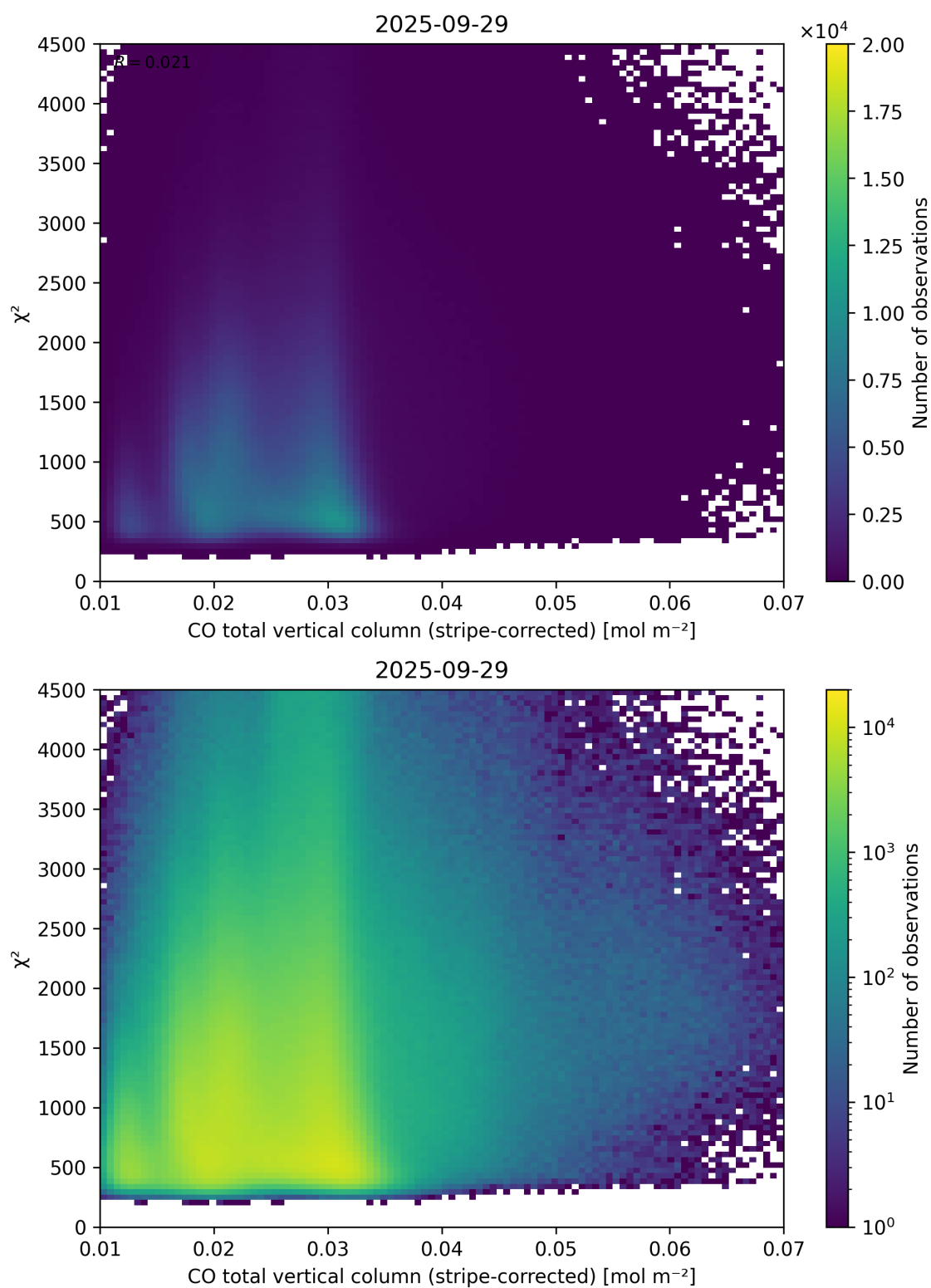
Figure 37: Scatter density plot of “CO total vertical column (stripe-corrected)” against “ \chi^2 ” for 2025-09-28 to 2025-09-30.
