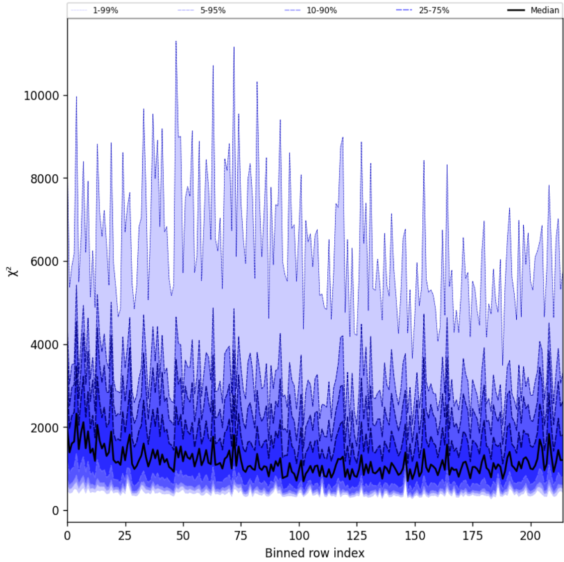
Figure 30: Along track statistics of “ \chi^2 ” for 2025-09-28 to 2025-09-30
