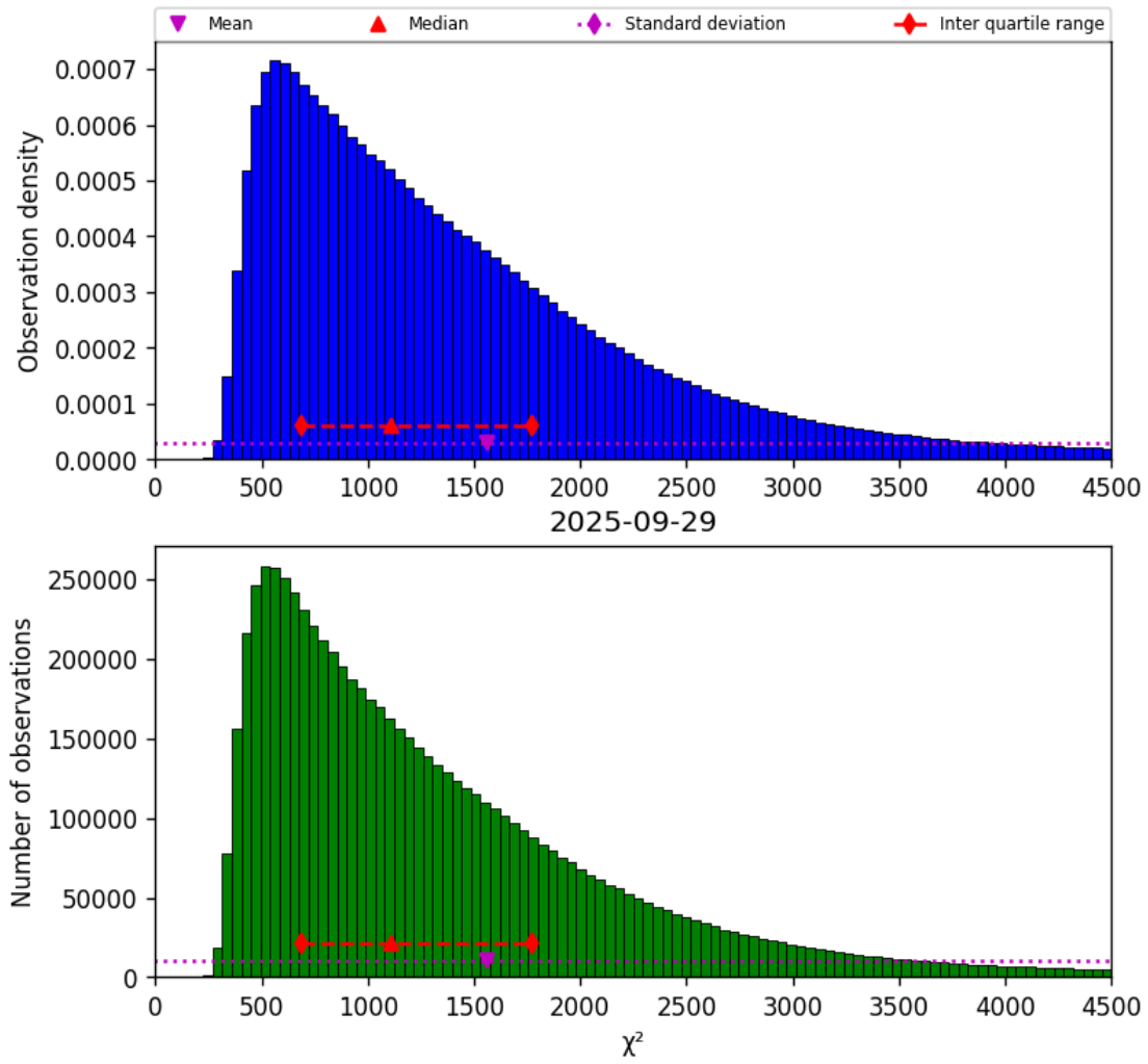
Figure 22: Histogram of “ \chi^2 ” for 2025-09-28 to 2025-09-30
