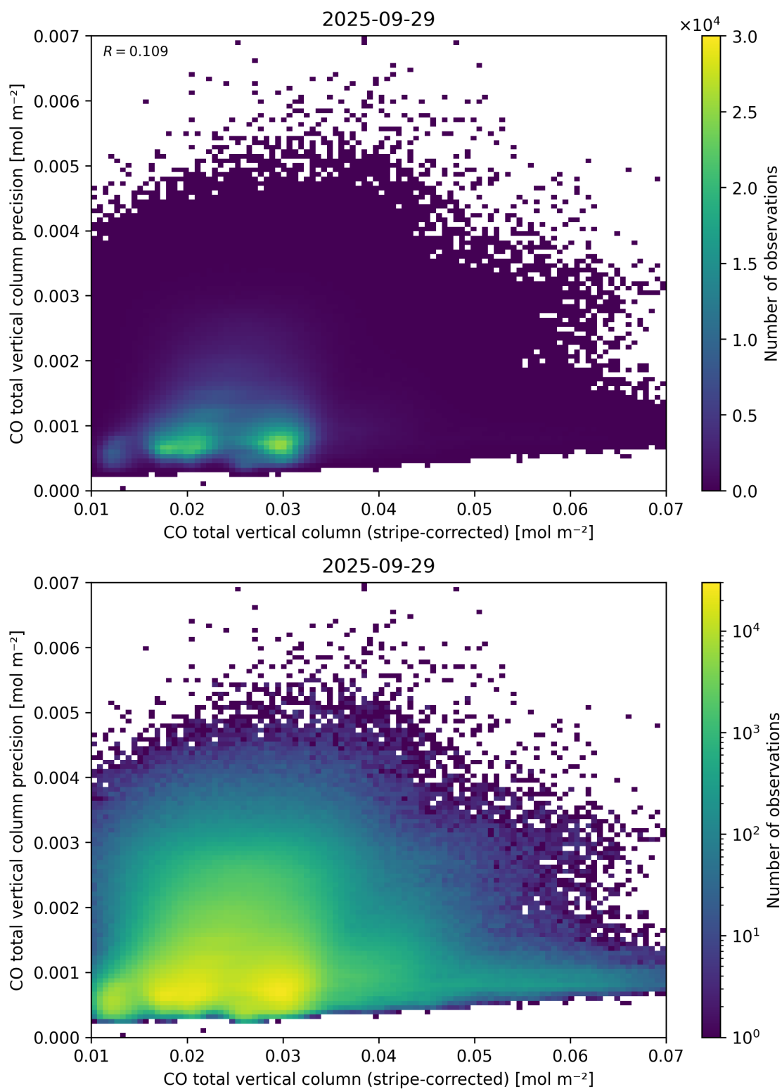
Figure 36: Scatter density plot of “CO total vertical column (stripe-corrected)” against “CO total vertical column precision” for 2025-09-28 to 2025-09-30.
