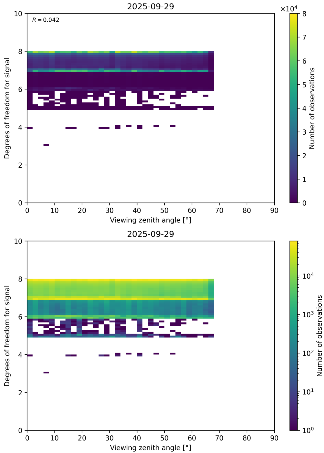
Figure 73: Scatter density plot of “Viewing zenith angle” against “Degrees of freedom for signal” for 2025-09-28 to 2025-09-30.
