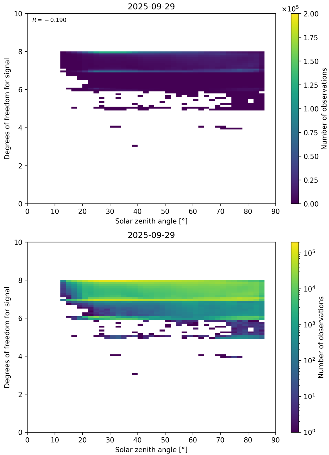
Figure 65: Scatter density plot of “Solar zenith angle” against “Degrees of freedom for signal” for 2025-09-28 to 2025-09-30.
