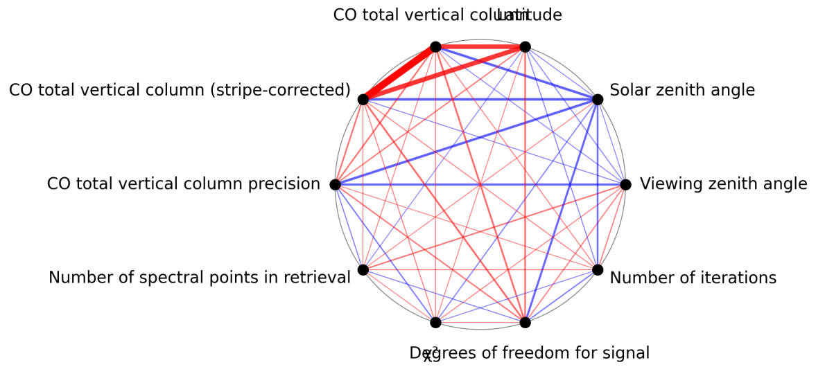
Figure 1: Map of correlation graph for 2025-09-28 to 2025-09-30.
