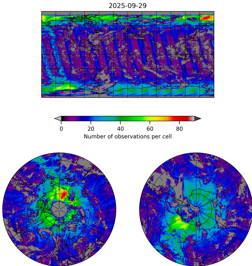
Figure 8: Map of the number of observations for 2025-09-28 to 2025-09-30
