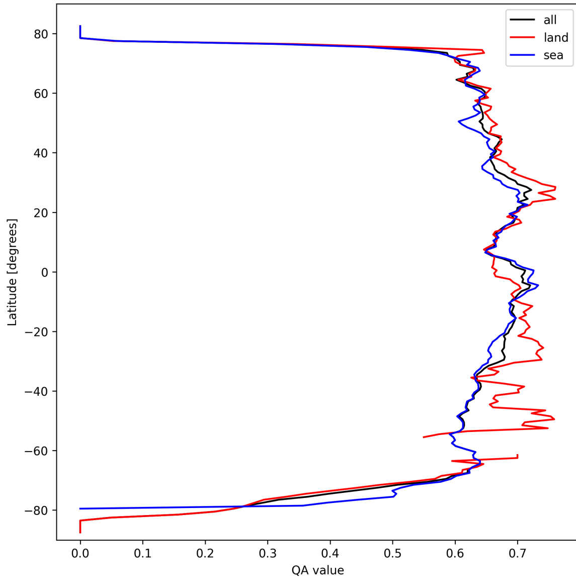
Figure 9: Zonal average of “QA value” for 2025-09-28 to 2025-09-30.
