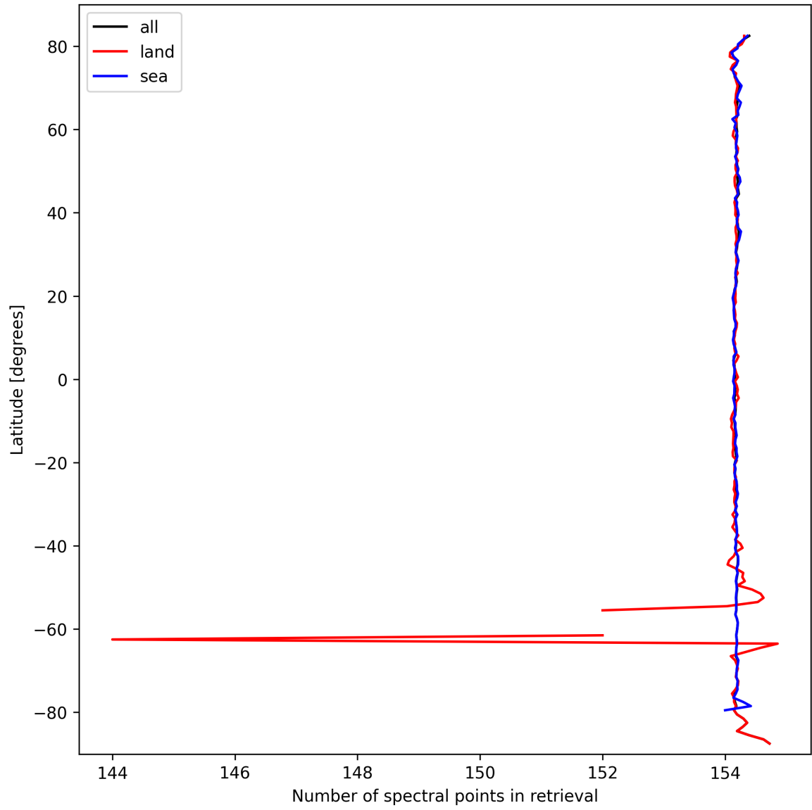
Figure 13: Zonal average of “Number of spectral points in retrieval” for 2025-09-28 to 2025-09-30.
