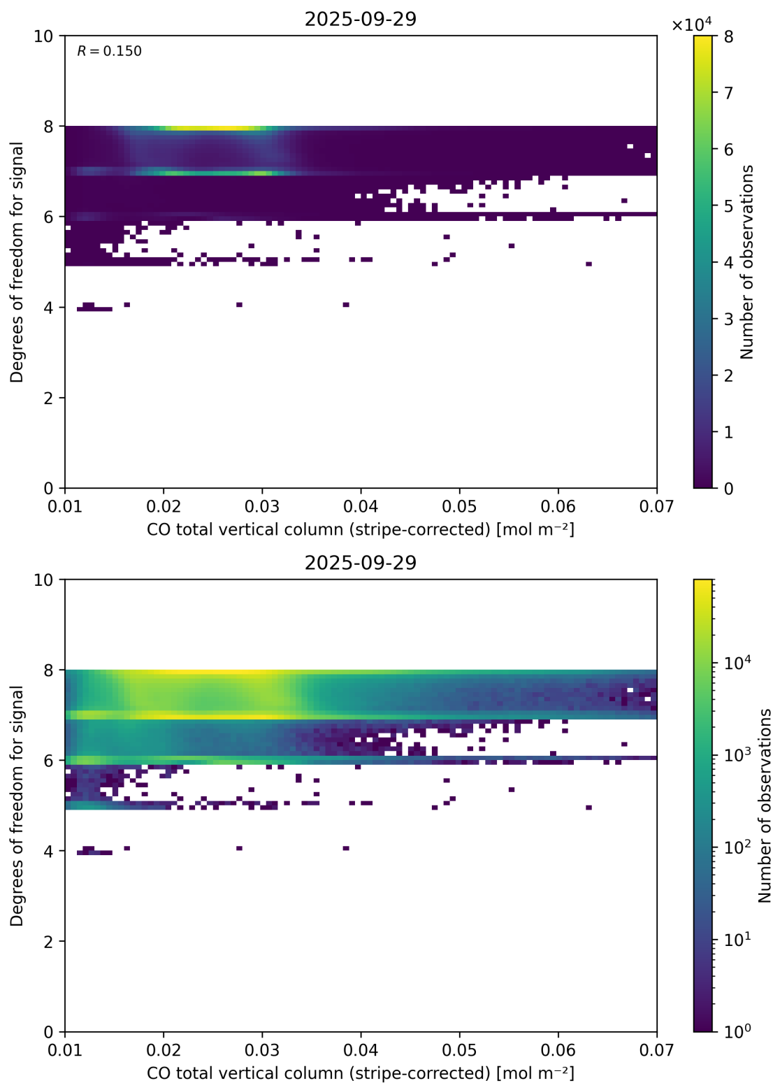
Figure 38: Scatter density plot of “CO total vertical column (stripe-corrected)” against “Degrees of freedom for signal” for 2025-09-28 to 2025-09-30.
