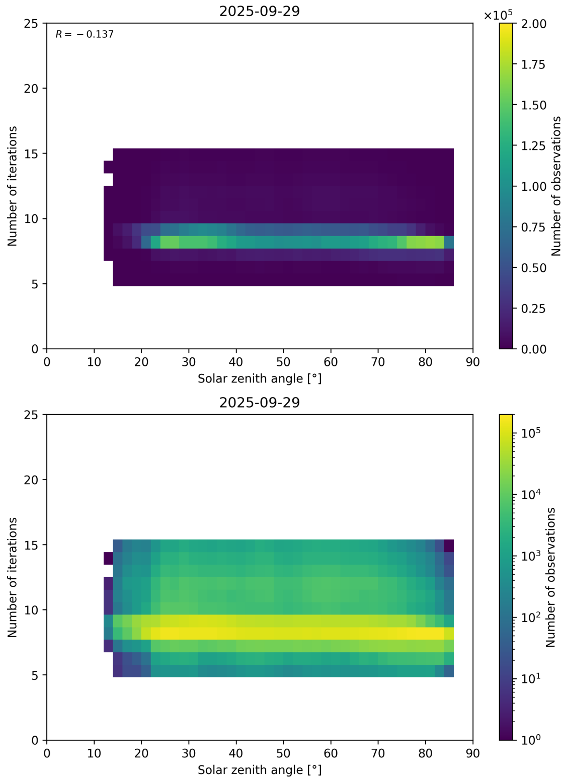
Figure 67: Scatter density plot of “Solar zenith angle” against “Number of iterations” for 2025-09-28 to 2025-09-30.
