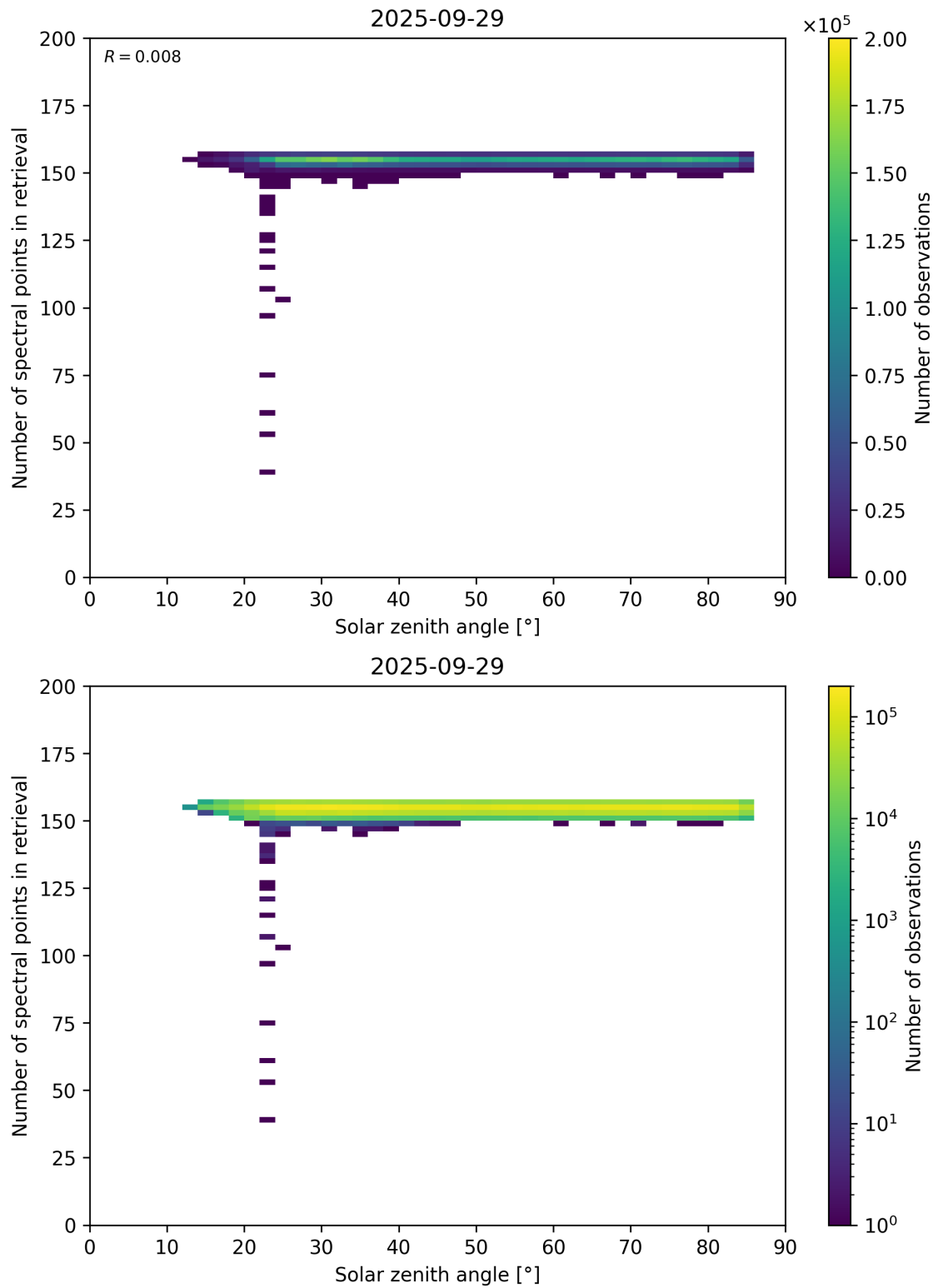
Figure 68: Scatter density plot of “Solar zenith angle” against “Number of spectral points in retrieval” for 2025-09-28 to 2025-09-30.
