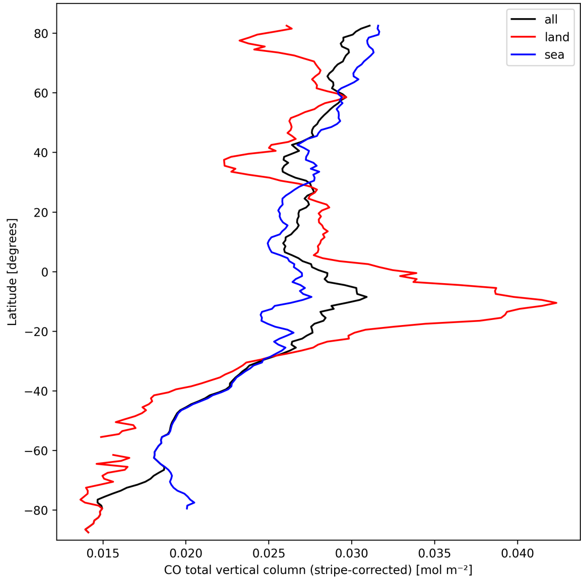
Figure 11: Zonal average of “CO total vertical column (stripe-corrected)” for 2025-09-28 to 2025-09-30.
