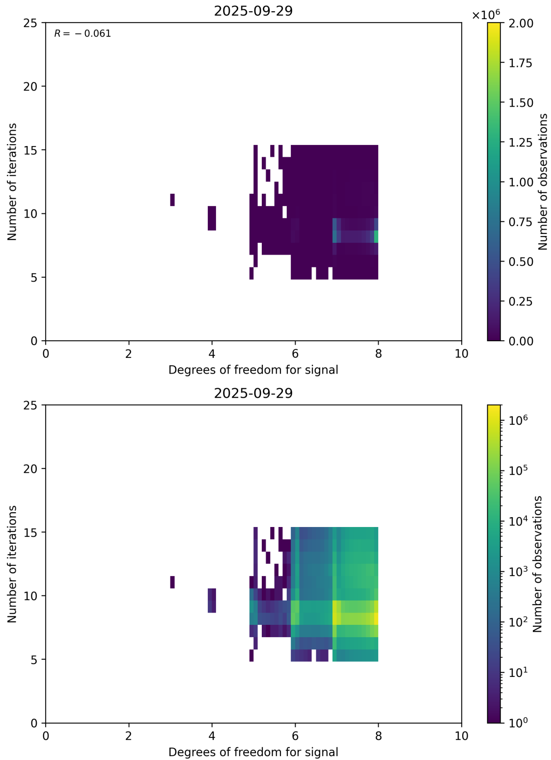
Figure 50: Scatter density plot of “Degrees of freedom for signal” against “Number of iterations” for 2025-09-28 to 2025-09-30.
