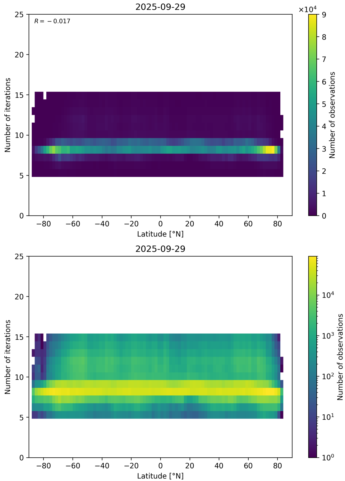
Figure 56: Scatter density plot of “Latitude” against “Number of iterations” for 2025-09-28 to 2025-09-30.
