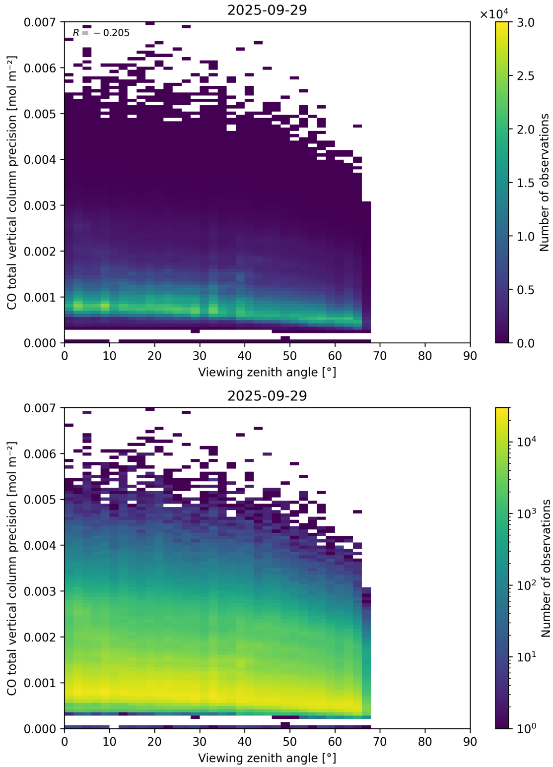
Figure 71: Scatter density plot of “Viewing zenith angle” against “CO total vertical column precision” for 2025-09-28 to 2025-09-30.
