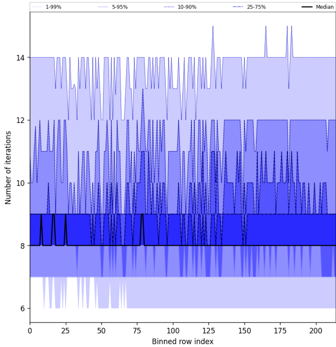
Figure 32: Along track statistics of “Number of iterations” for 2025-09-28 to 2025-09-30
