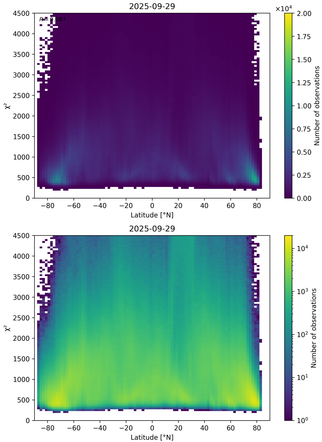
Figure 54: Scatter density plot of “Latitude” against “ \chi^2 ” for 2025-09-28 to 2025-09-30.
