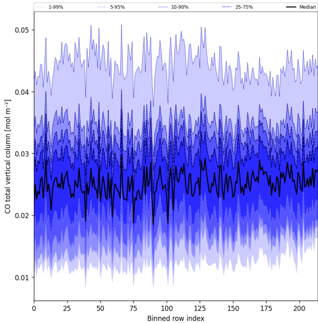
Figure 26: Along track statistics of "CO total vertical column" for 2025-09-28 to 2025-09-30
