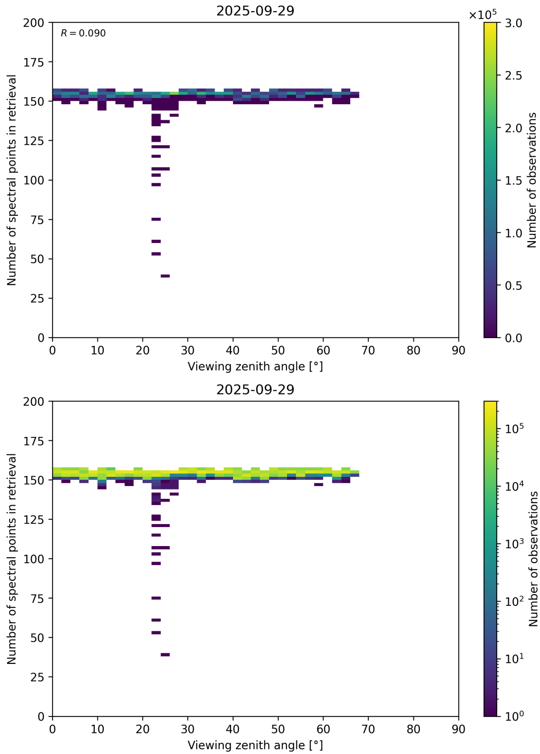
Figure 76: Scatter density plot of “Viewing zenith angle” against “Number of spectral points in retrieval” for 2025-09-28 to 2025-09-30.
