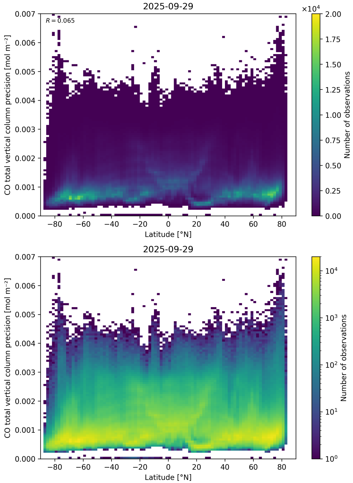
Figure 53: Scatter density plot of “Latitude” against “CO total vertical column precision” for 2025-09-28 to 2025-09-30.
