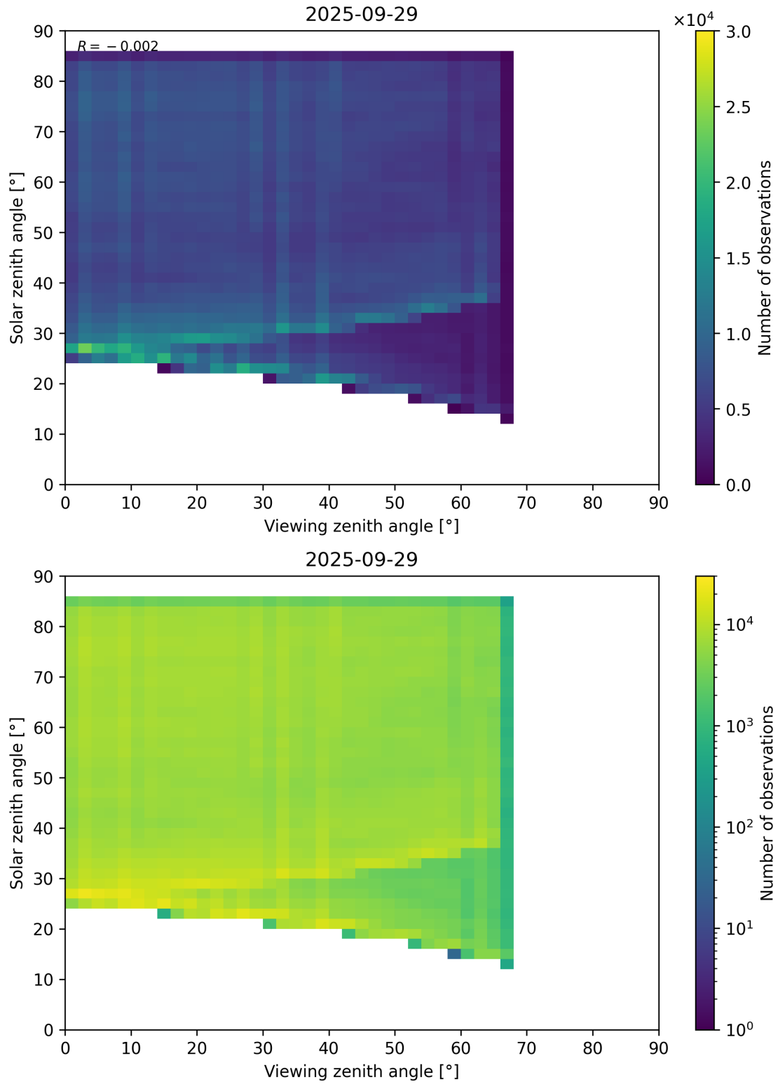
Figure 77: Scatter density plot of “Viewing zenith angle” against “Solar zenith angle” for 2025-09-28 to 2025-09-30.
