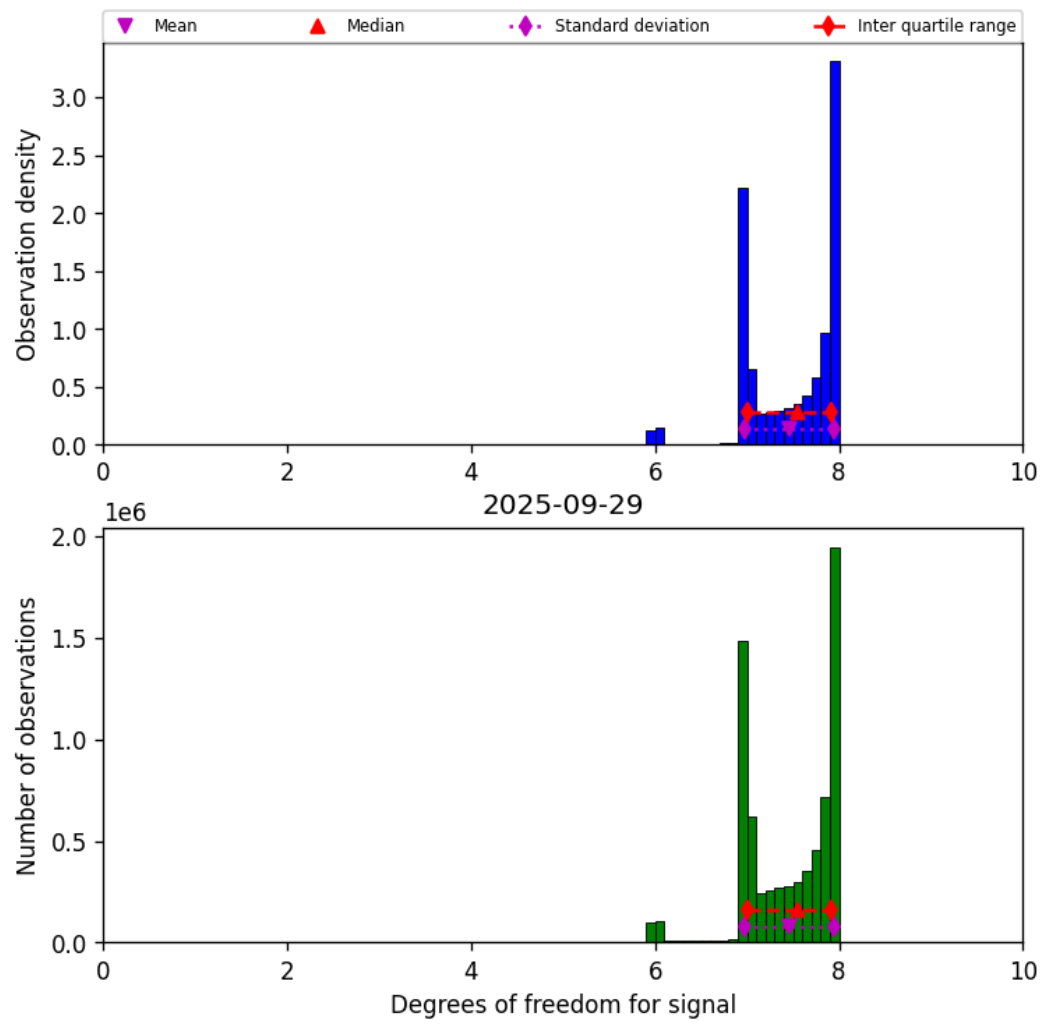
Figure 23: Histogram of “Degrees of freedom for signal” for 2025-09-28 to 2025-09-30
