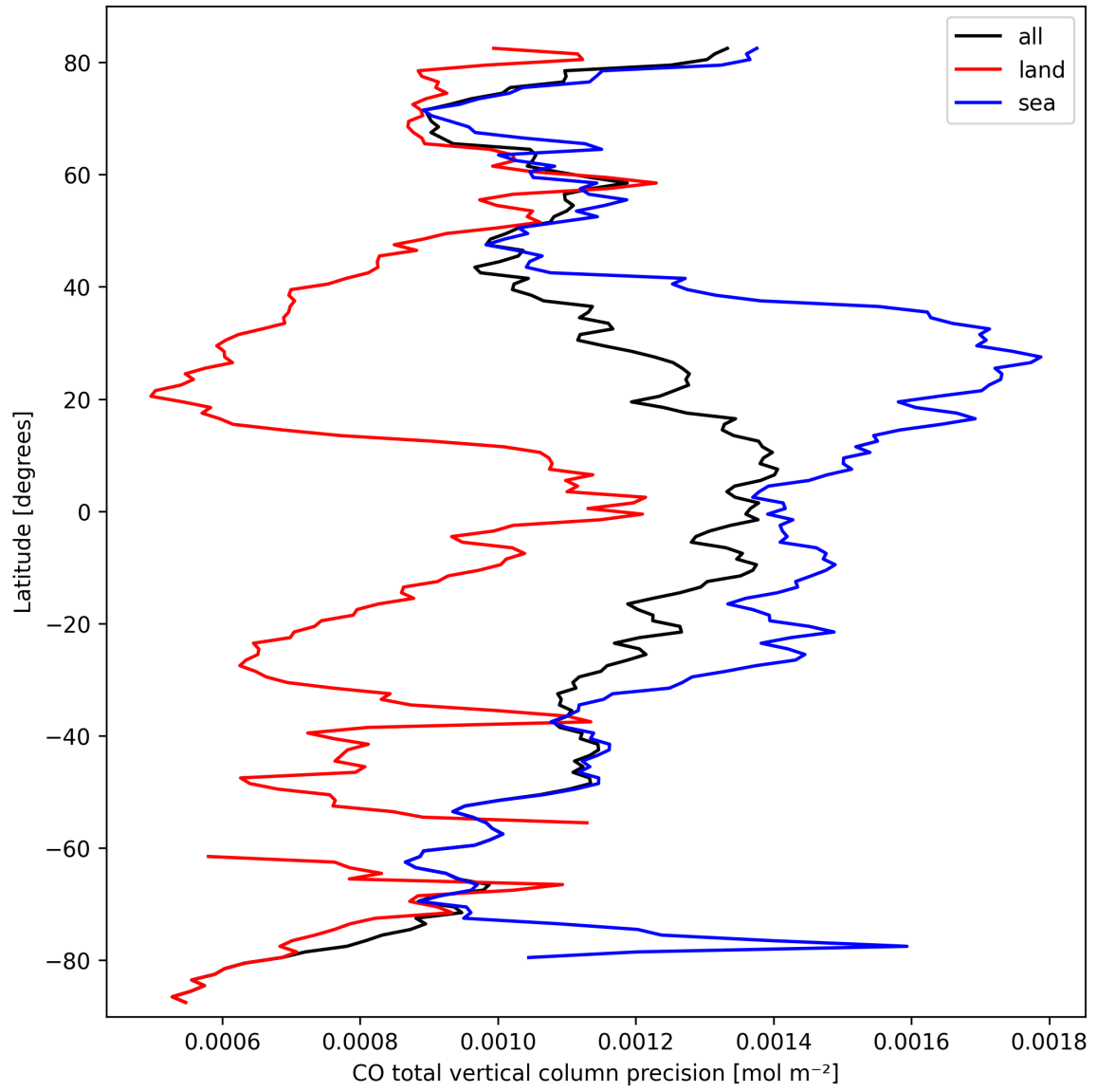
Figure 12: Zonal average of “CO total vertical column precision” for 2025-09-28 to 2025-09-30.
