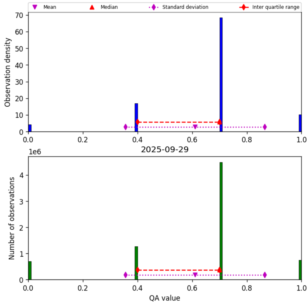
Figure 17: Histogram of “QA value” for 2025-09-28 to 2025-09-30
