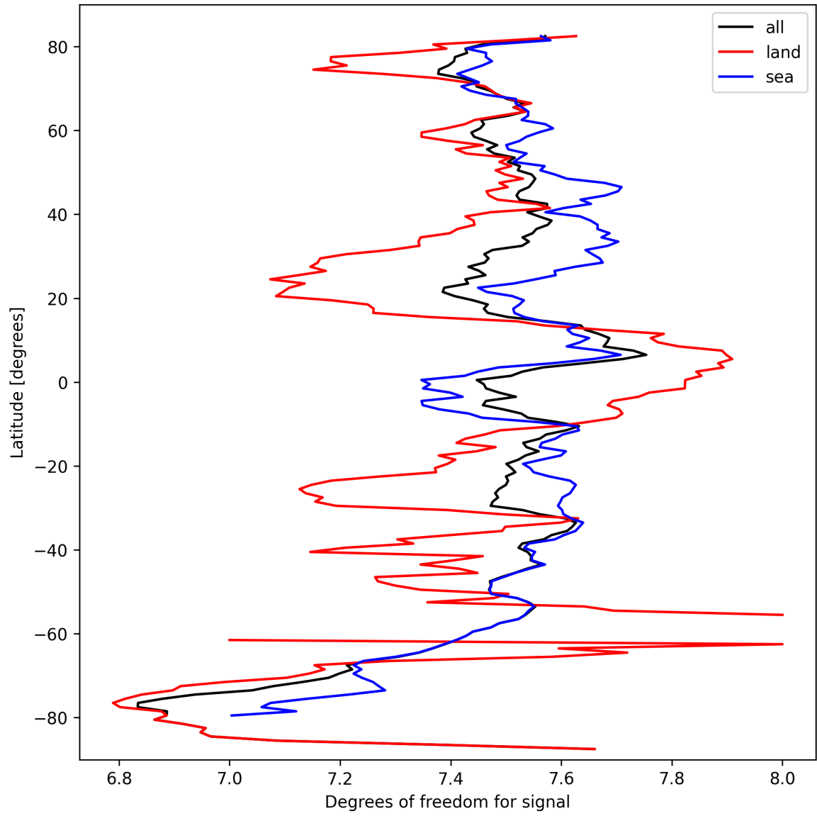
Figure 15: Zonal average of “Degrees of freedom for signal” for 2025-09-28 to 2025-09-30.
