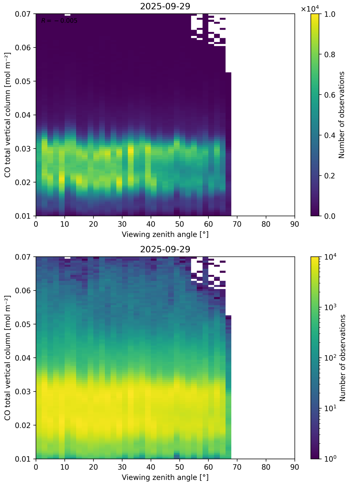
Figure 69: Scatter density plot of “Viewing zenith angle” against “CO total vertical column” for 2025-09-28 to 2025-09-30.
