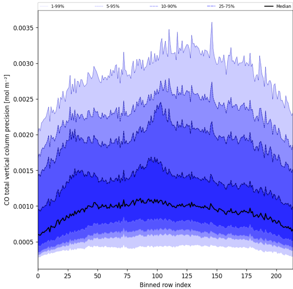
Figure 28: Along track statistics of “CO total vertical column precision” for 2025-09-28 to 2025-09-30
