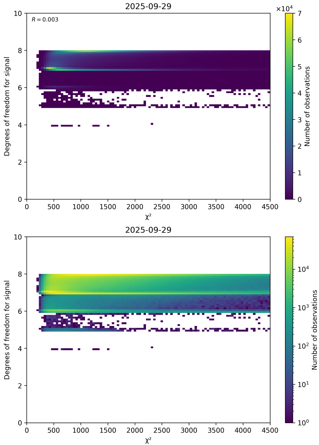
Figure 48: Scatter density plot of “ \chi^2 ” against “Degrees of freedom for signal” for 2025-09-28 to 2025-09-30.
