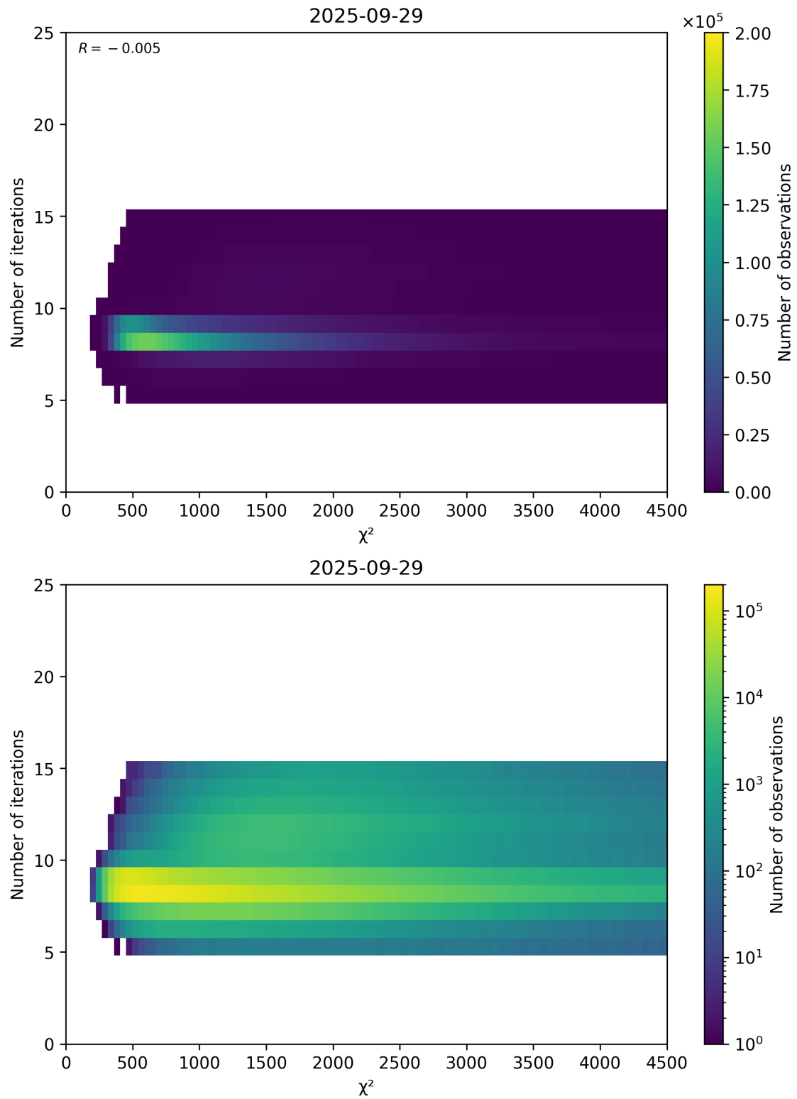
Figure 49: Scatter density plot of “ \chi^2 ” against “Number of iterations” for 2025-09-28 to 2025-09-30.
