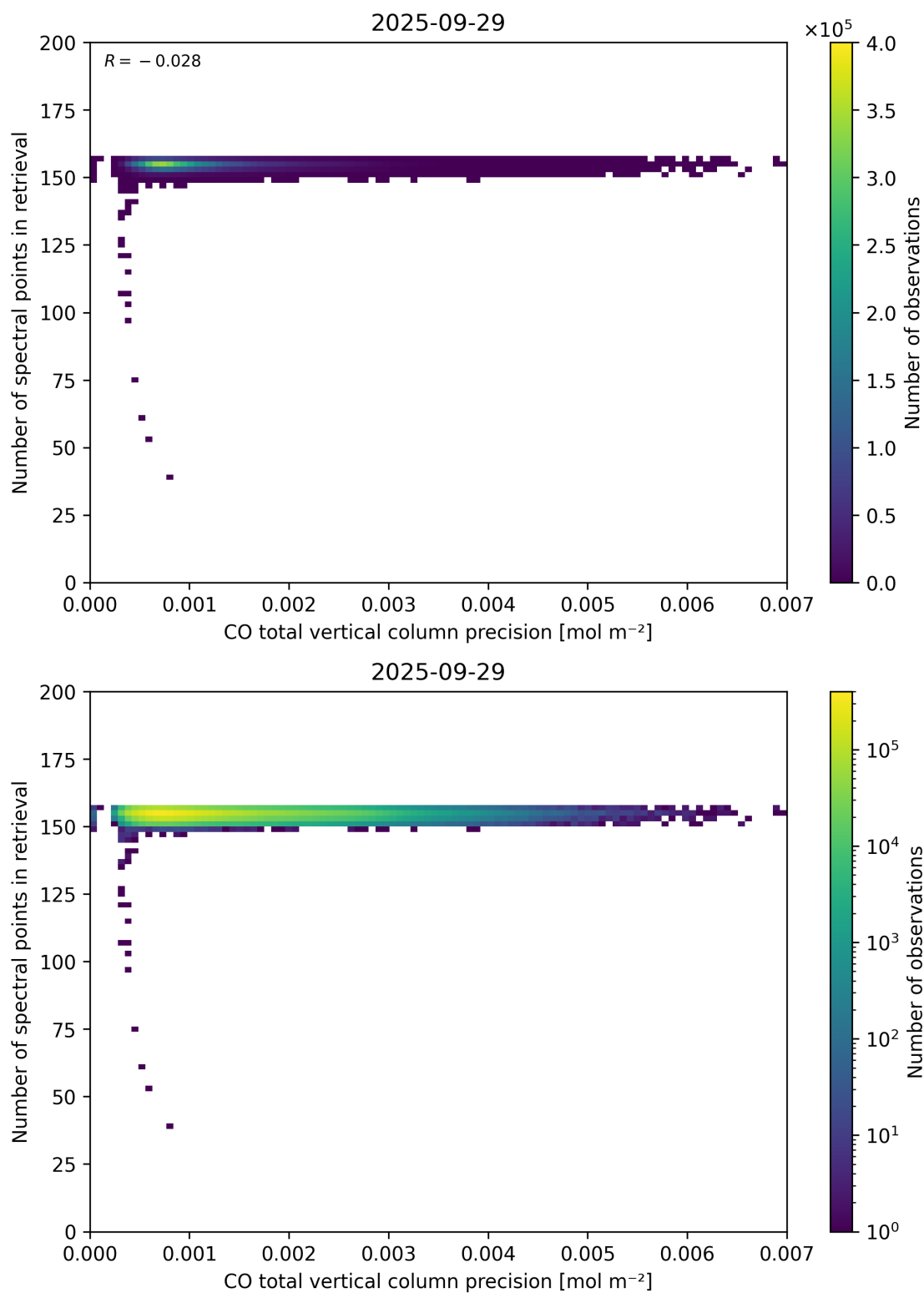
Figure 47: Scatter density plot of “CO total vertical column precision” against “Number of spectral points in retrieval” for 2025-09-28 to 2025-09-30.
