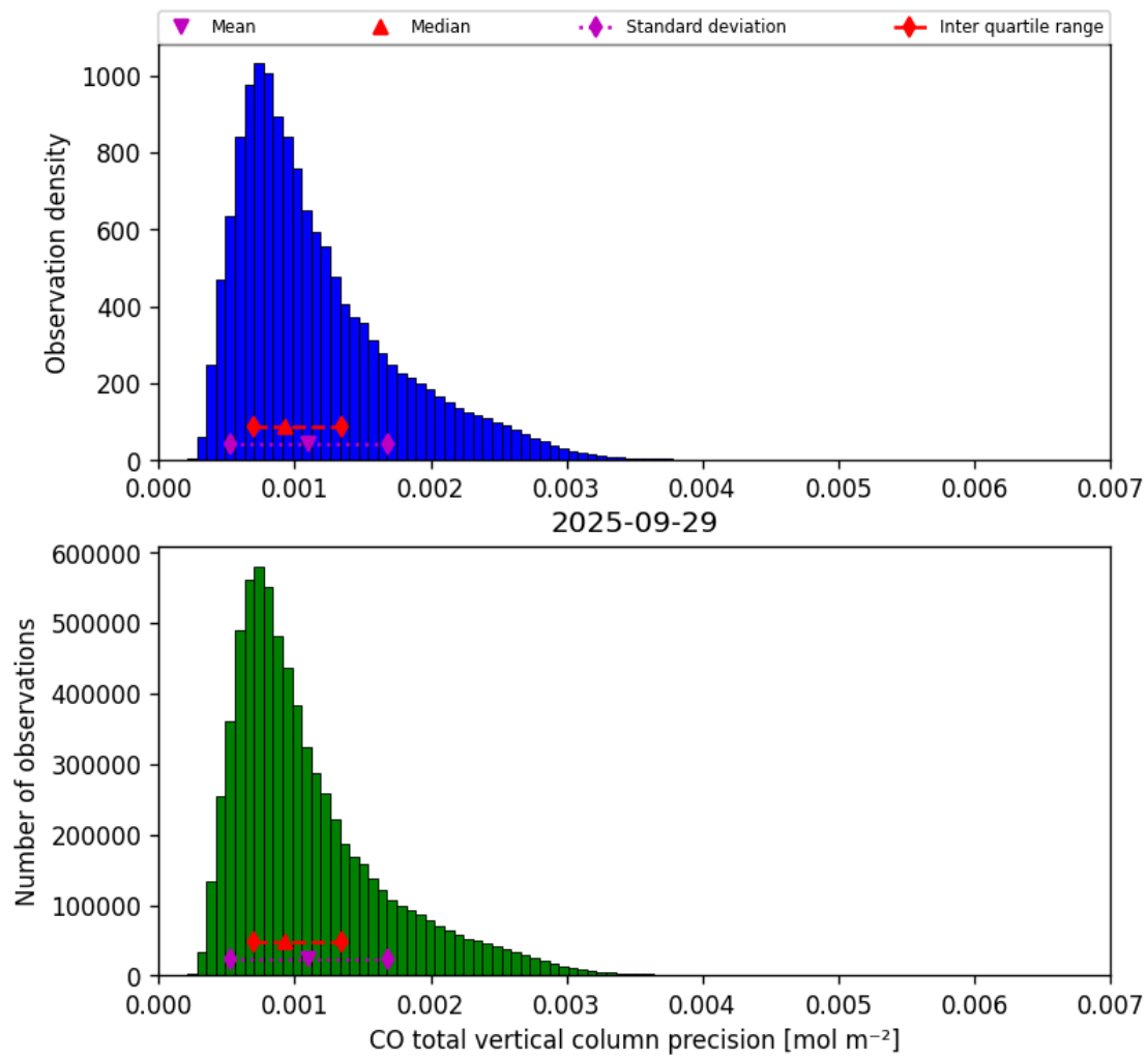
Figure 20: Histogram of “CO total vertical column precision” for 2025-09-28 to 2025-09-30
