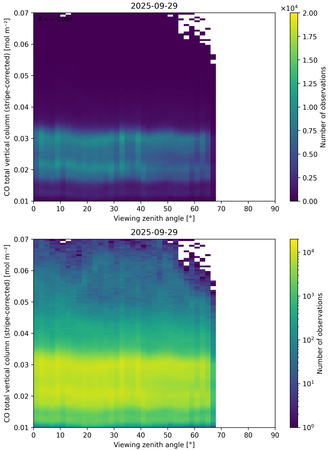
Figure 70: Scatter density plot of “Viewing zenith angle” against “CO total vertical column (stripe-corrected)” for 2025-09-28 to 2025-09-30.
