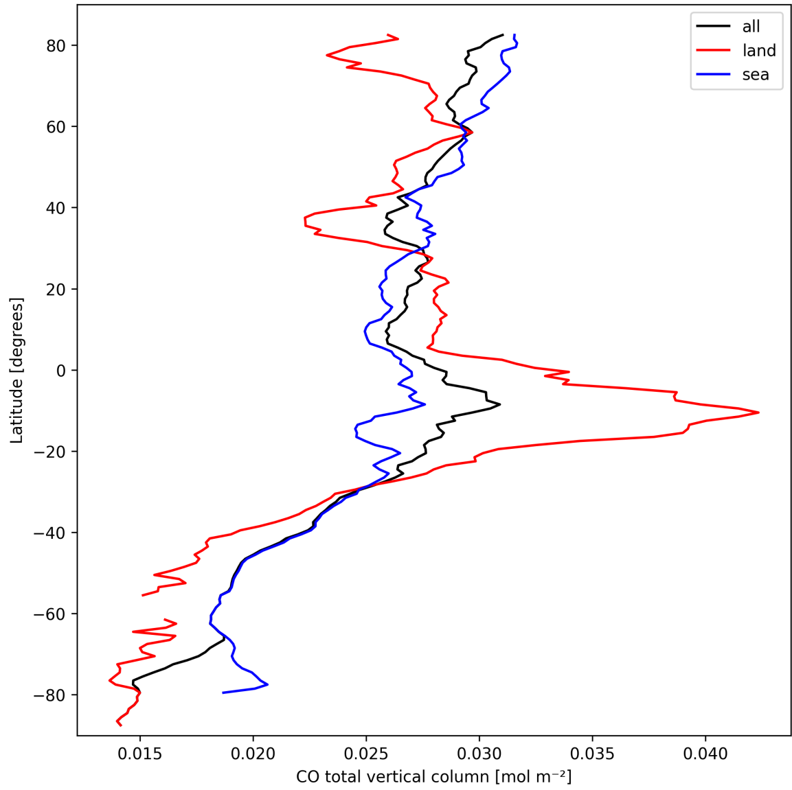
Figure 10: Zonal average of “CO total vertical column” for 2025-09-28 to 2025-09-30.
