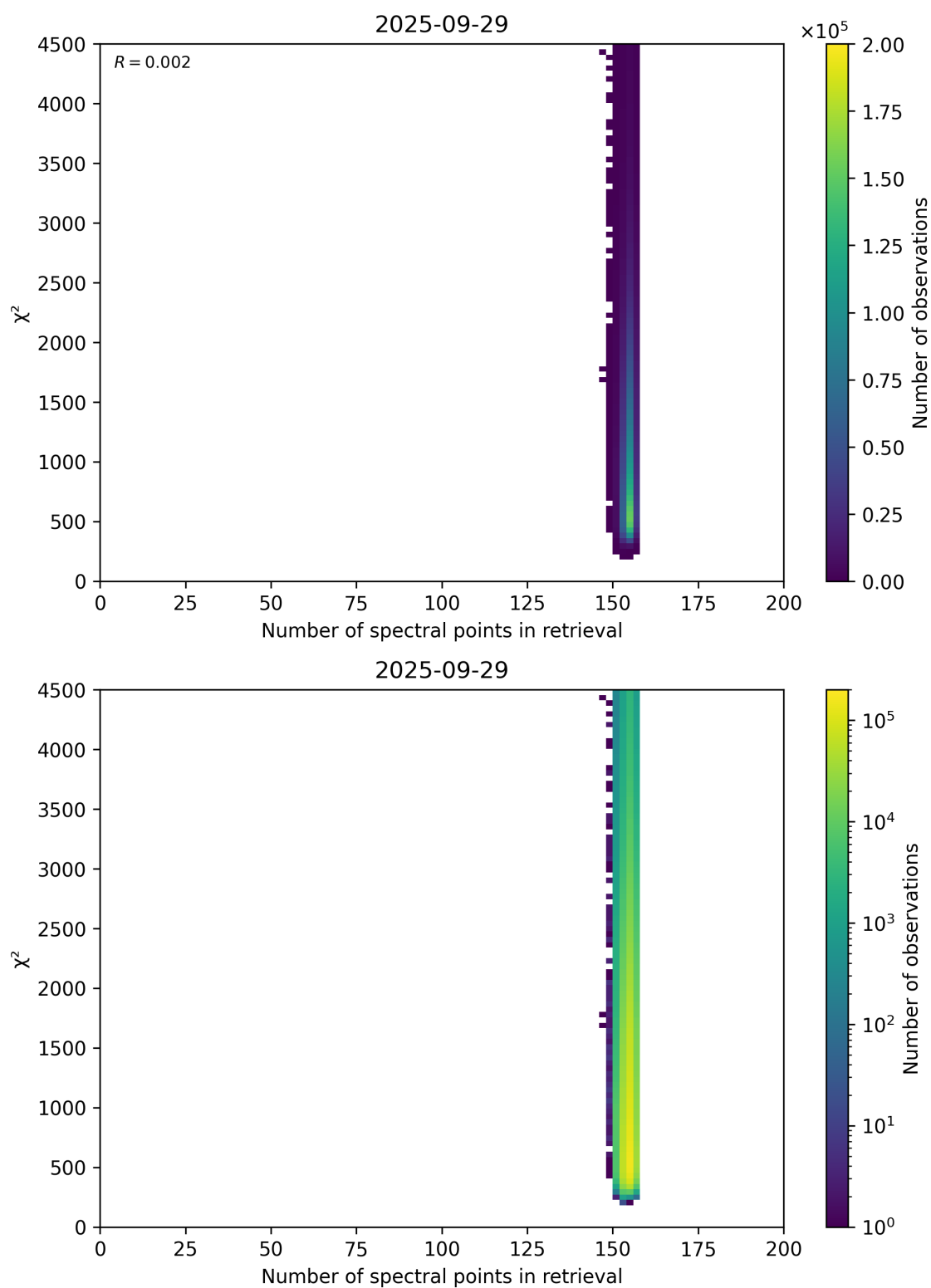
Figure 58: Scatter density plot of “Number of spectral points in retrieval” against “ \chi^2 ” for 2025-09-28 to 2025-09-30.
