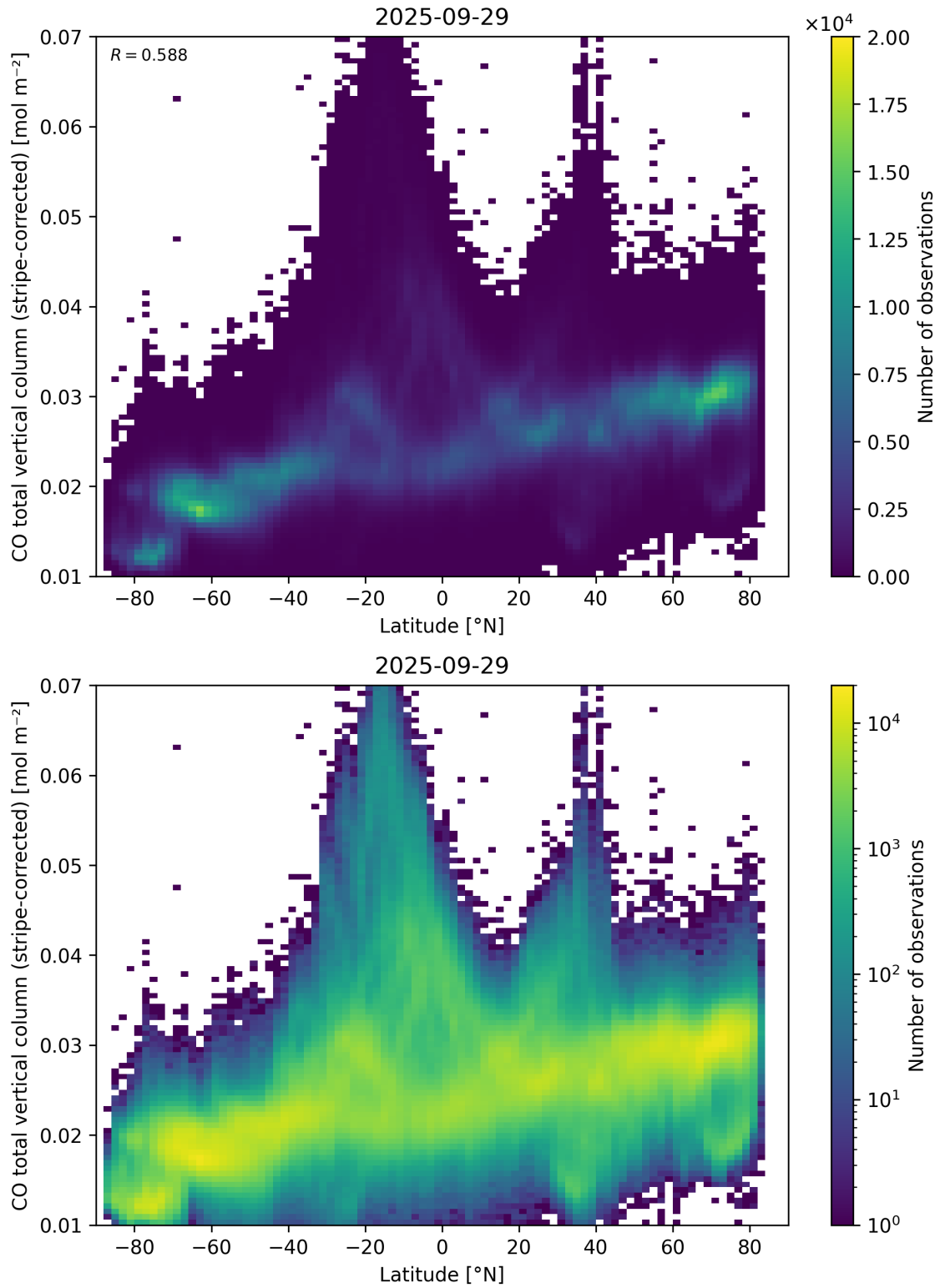
Figure 52: Scatter density plot of “Latitude” against “CO total vertical column (stripe-corrected)” for 2025-09-28 to 2025-09-30.
