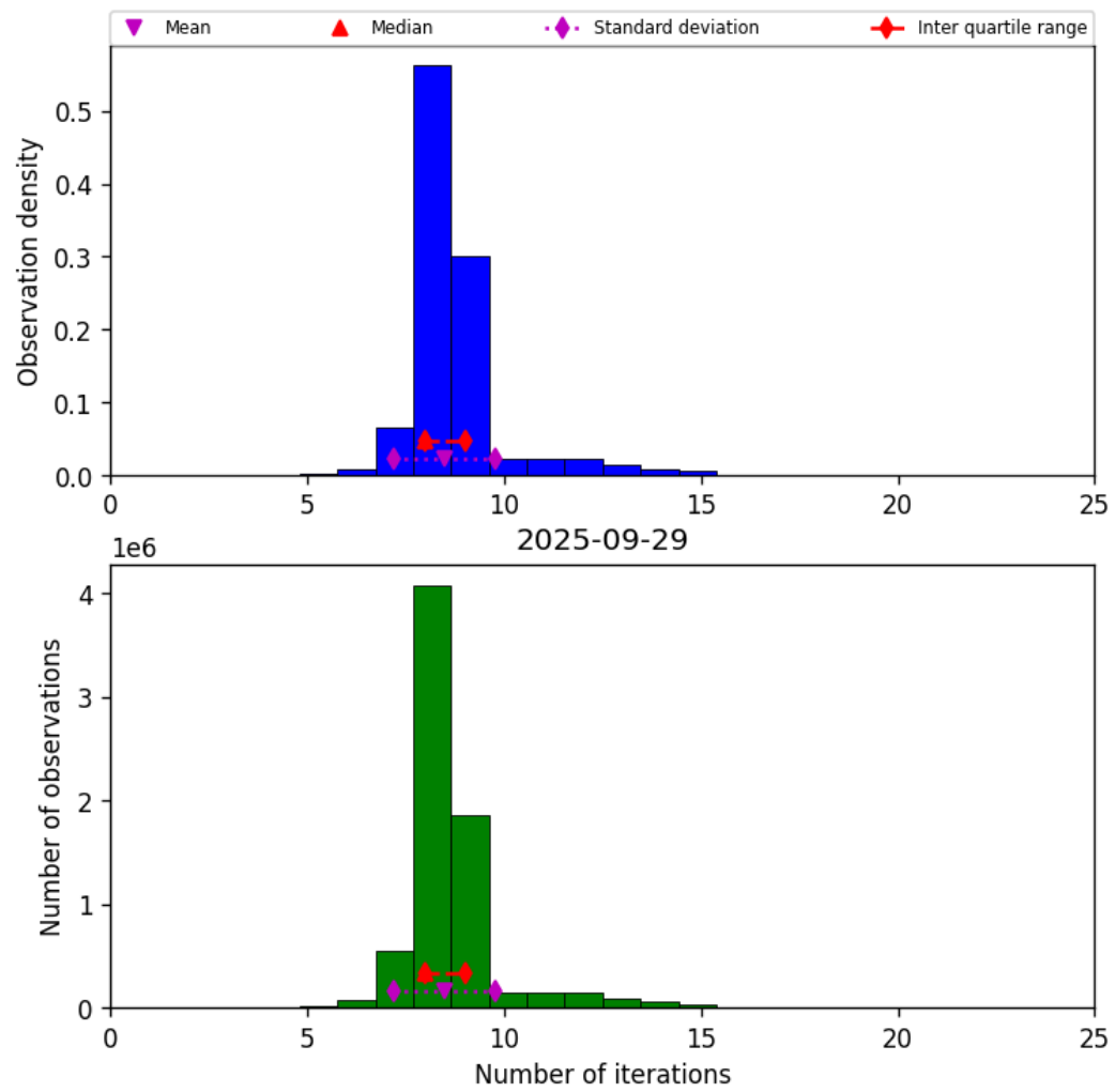
Figure 24: Histogram of “Number of iterations” for 2025-09-28 to 2025-09-30
