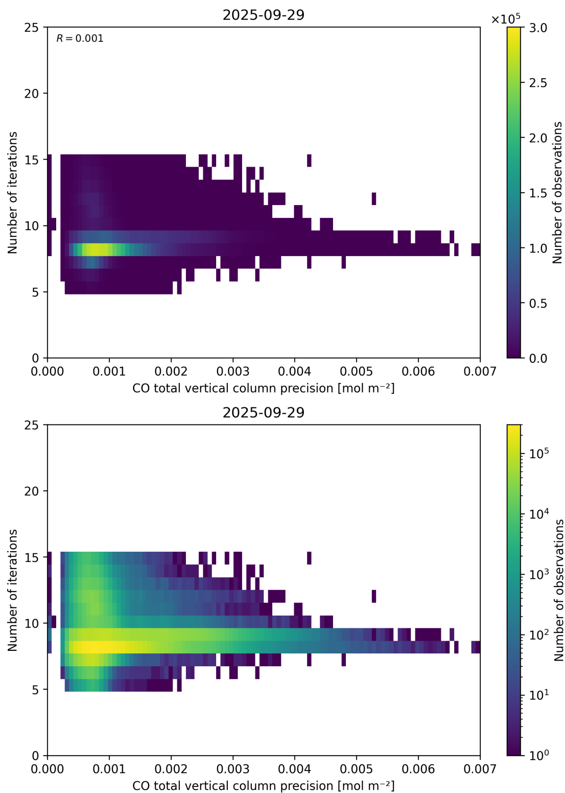
Figure 46: Scatter density plot of “CO total vertical column precision” against “Number of iterations” for 2025-09-28 to 2025-09-30.
