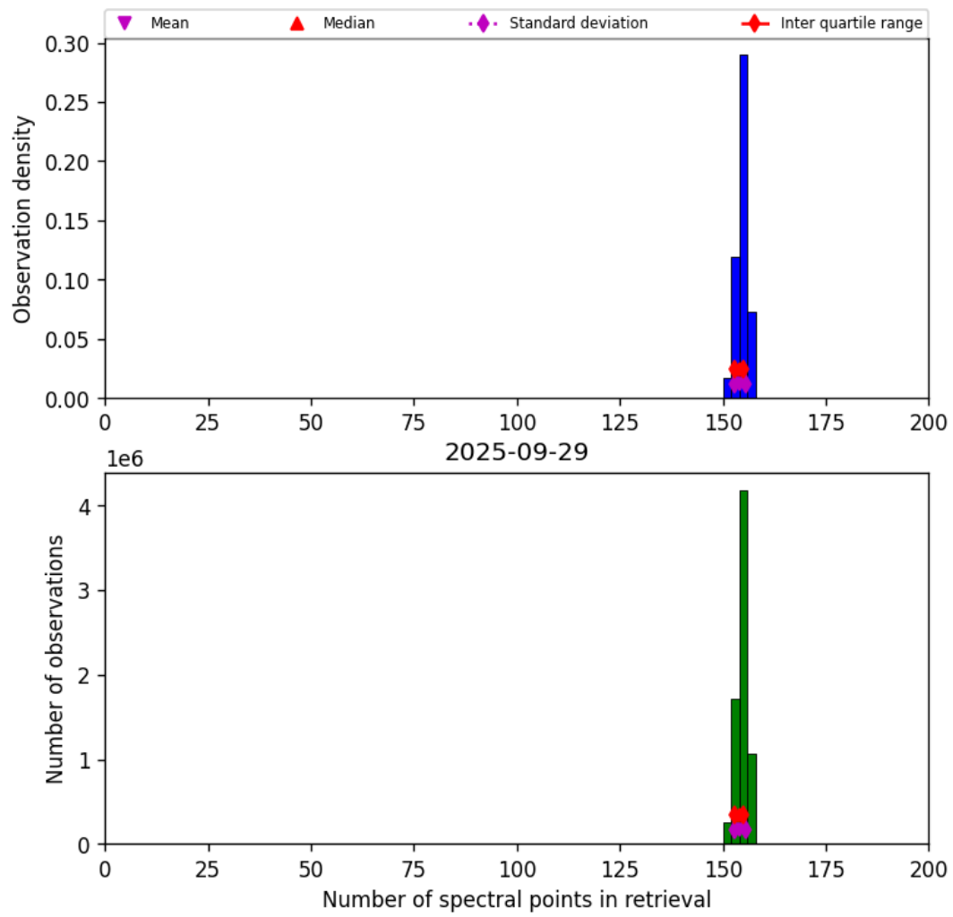
Figure 21: Histogram of “Number of spectral points in retrieval” for 2025-09-28 to 2025-09-30
