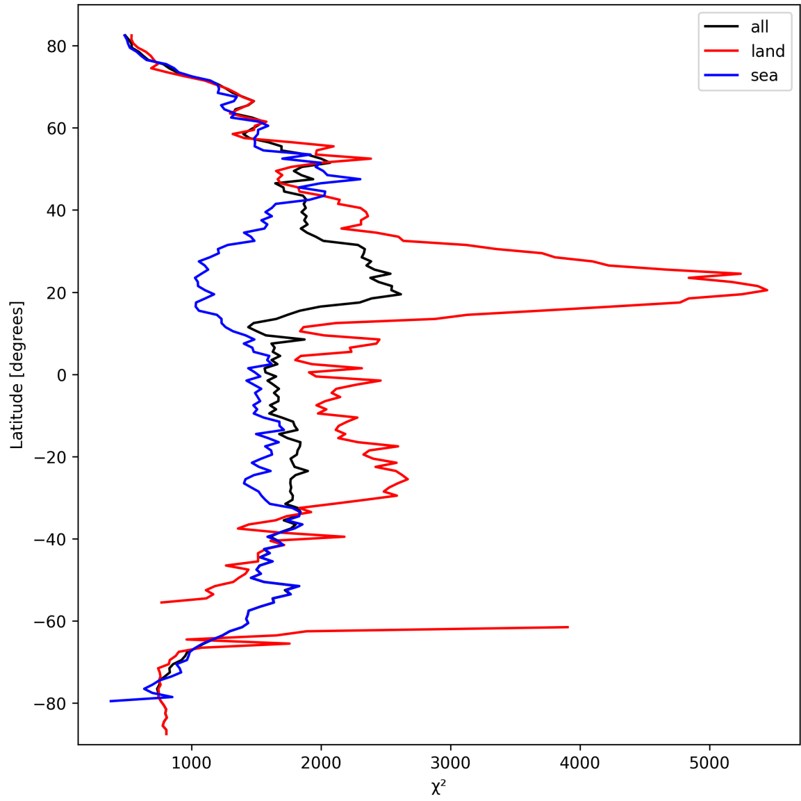
Figure 14: Zonal average of “ \chi^2 ” for 2025-09-28 to 2025-09-30.
