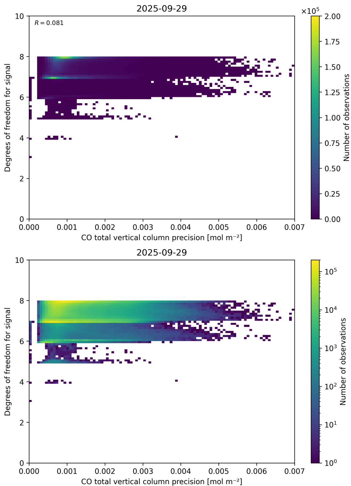
Figure 45: Scatter density plot of “CO total vertical column precision” against “Degrees of freedom for signal” for 2025-09-28 to 2025-09-30.
