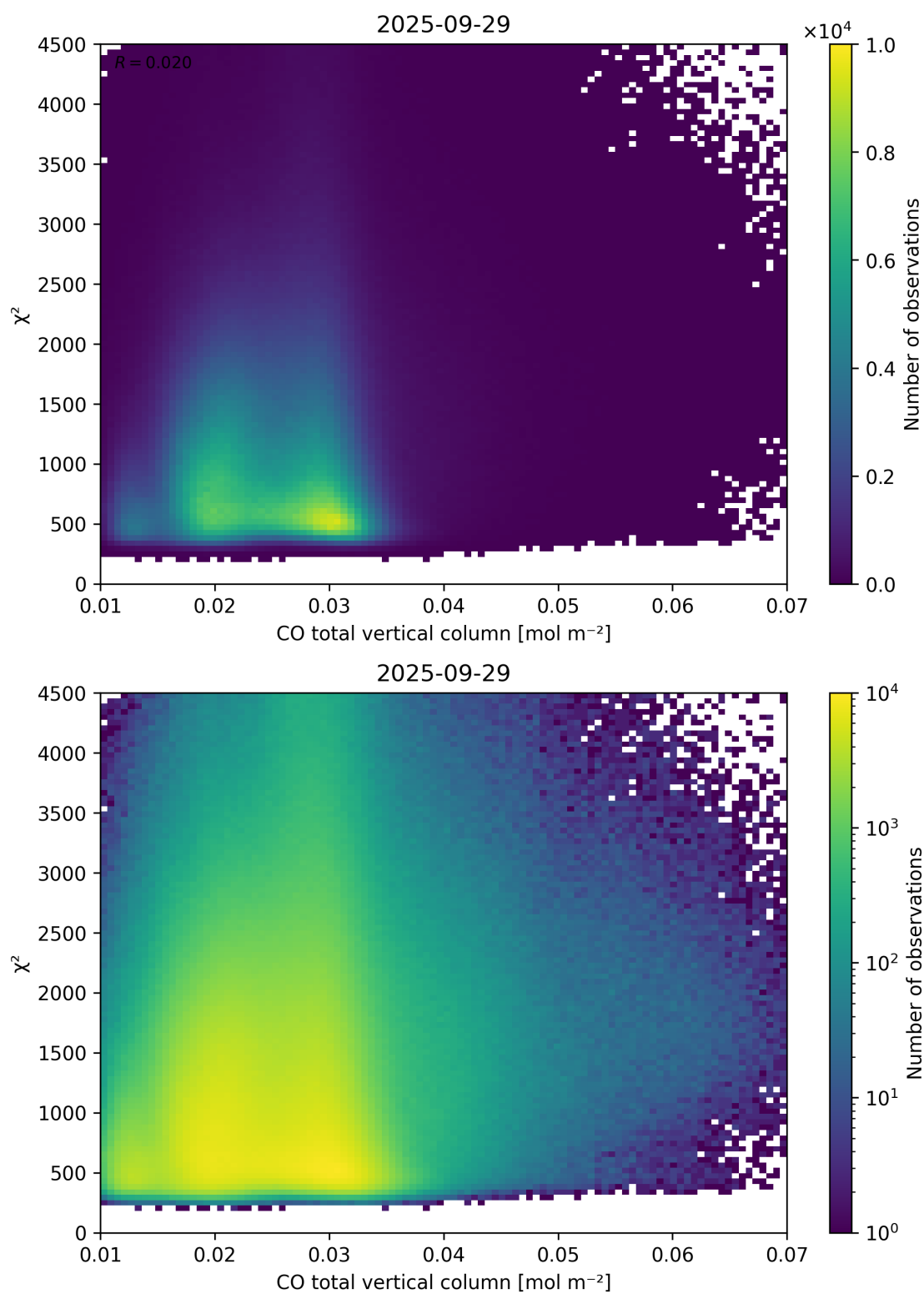
Figure 35: Scatter density plot of “CO total vertical column” against “ \chi^2 ” for 2025-09-28 to 2025-09-30.
