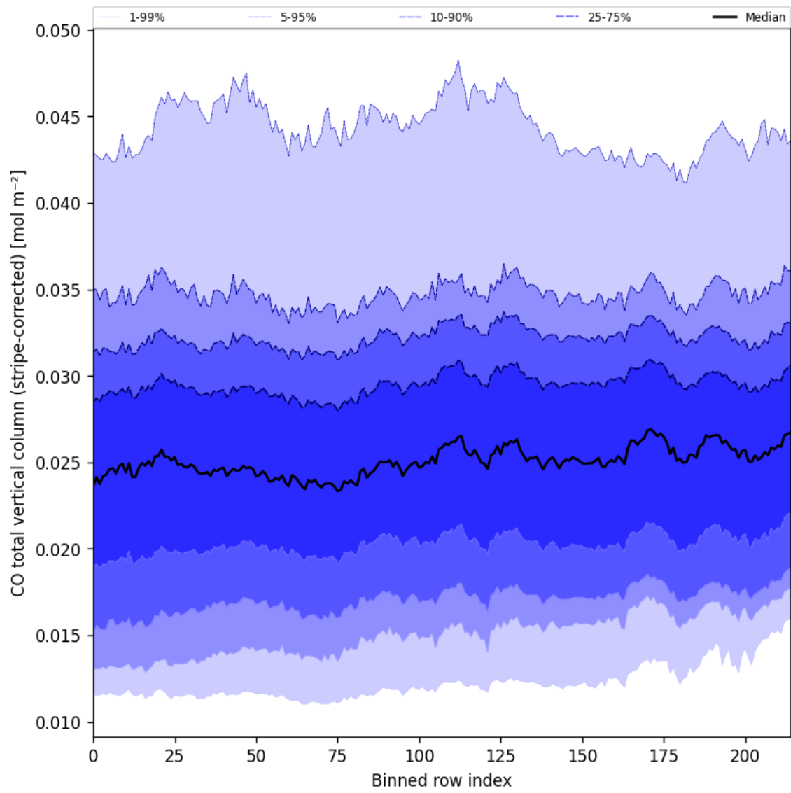
Figure 27: Along track statistics of “CO total vertical column (stripe-corrected)” for 2025-09-28 to 2025-09-30
