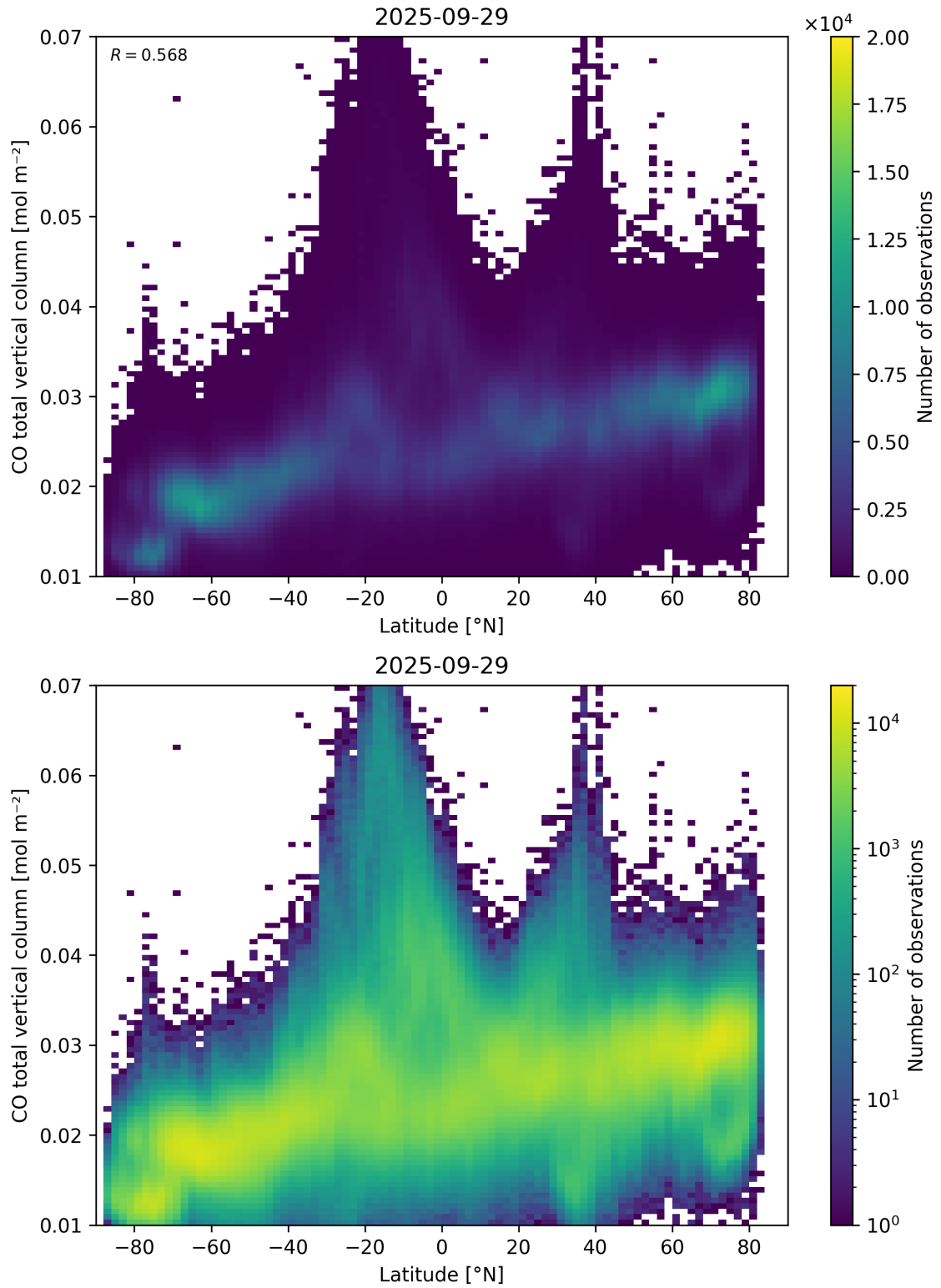
Figure 51: Scatter density plot of “Latitude” against “CO total vertical column” for 2025-09-28 to 2025-09-30.
