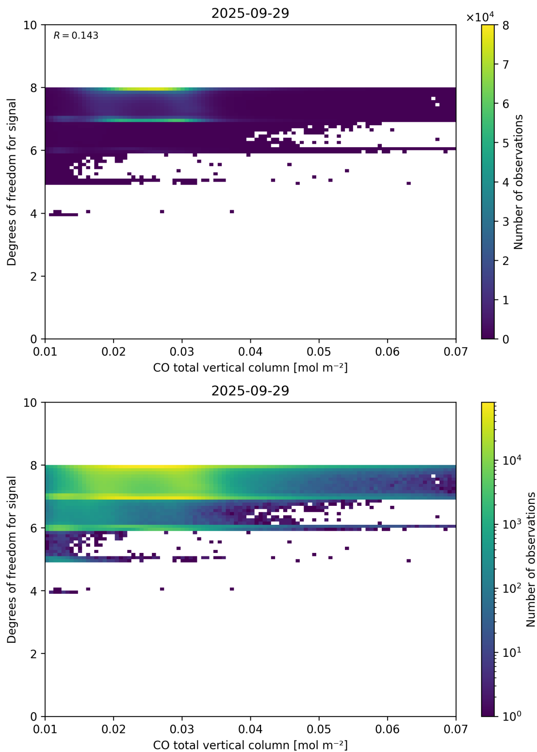
Figure 41: Scatter density plot of “CO total vertical column” against “Degrees of freedom for signal” for 2025-09-28 to 2025-09-30.
