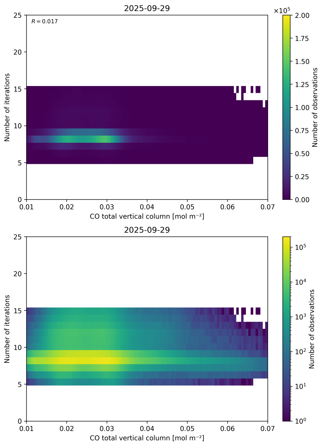
Figure 42: Scatter density plot of “CO total vertical column” against “Number of iterations” for 2025-09-28 to 2025-09-30.
