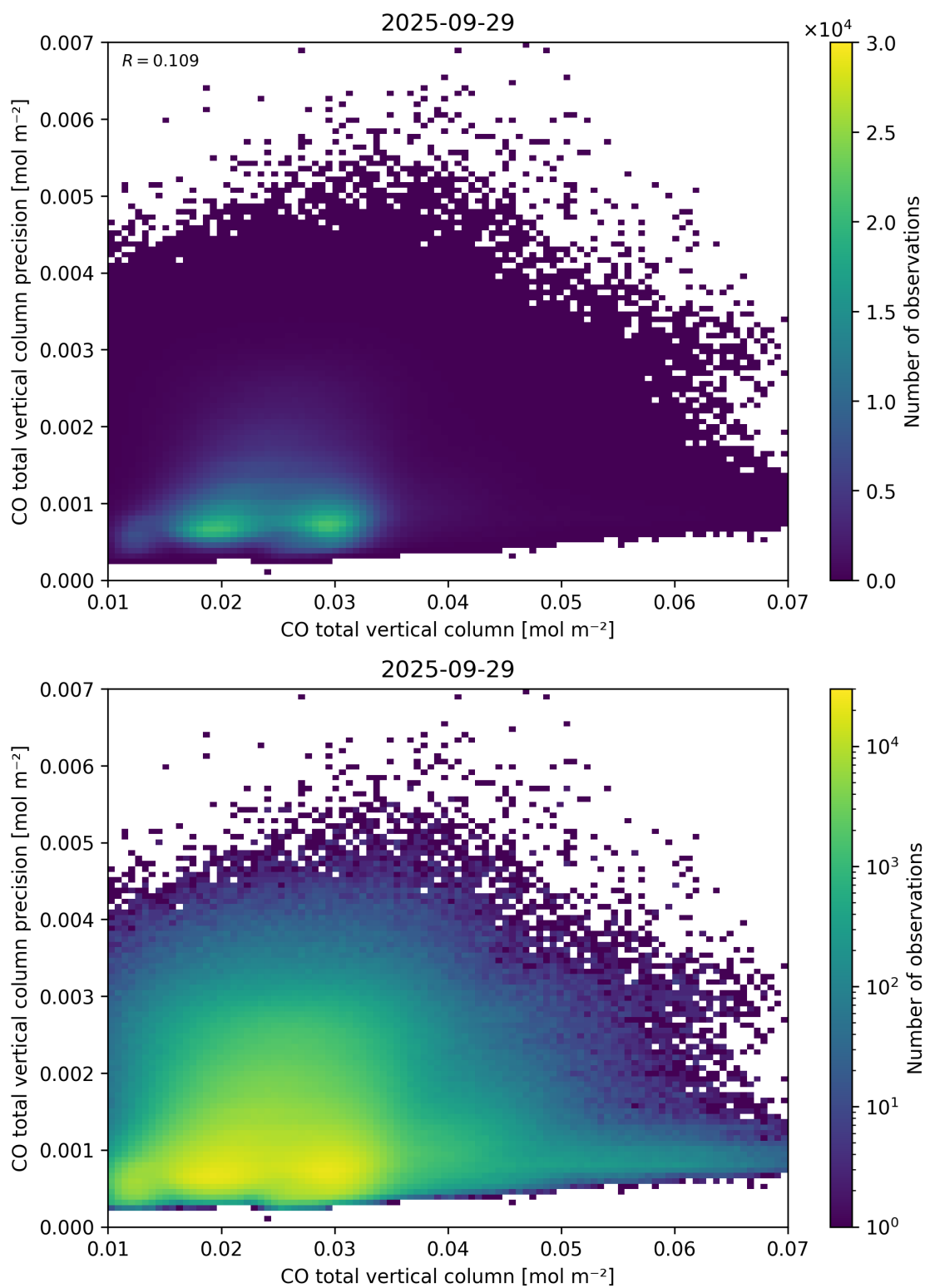
Figure 34: Scatter density plot of “CO total vertical column” against “CO total vertical column precision” for 2025-09-28 to 2025-09-30.
