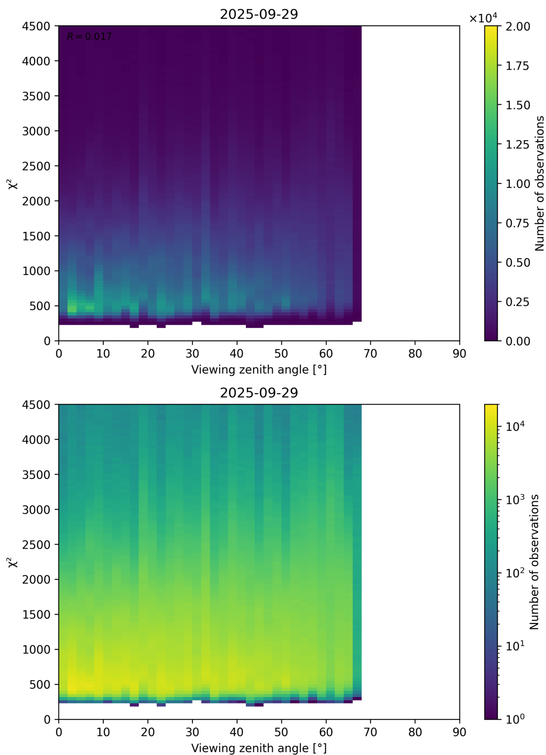
Figure 72: Scatter density plot of “Viewing zenith angle” against “ \chi^2 ” for 2025-09-28 to 2025-09-30.
