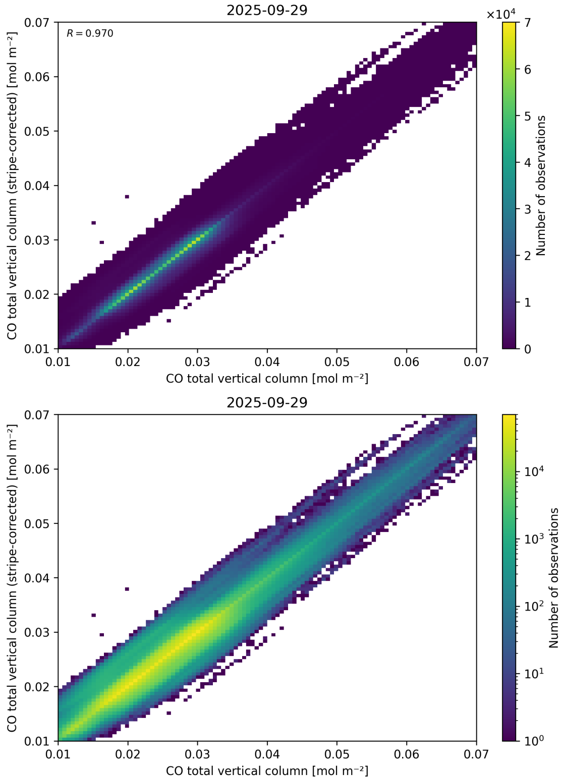
Figure 33: Scatter density plot of “CO total vertical column” against “CO total vertical column (stripe-corrected)” for 2025-09-28 to 2025-09-30.
