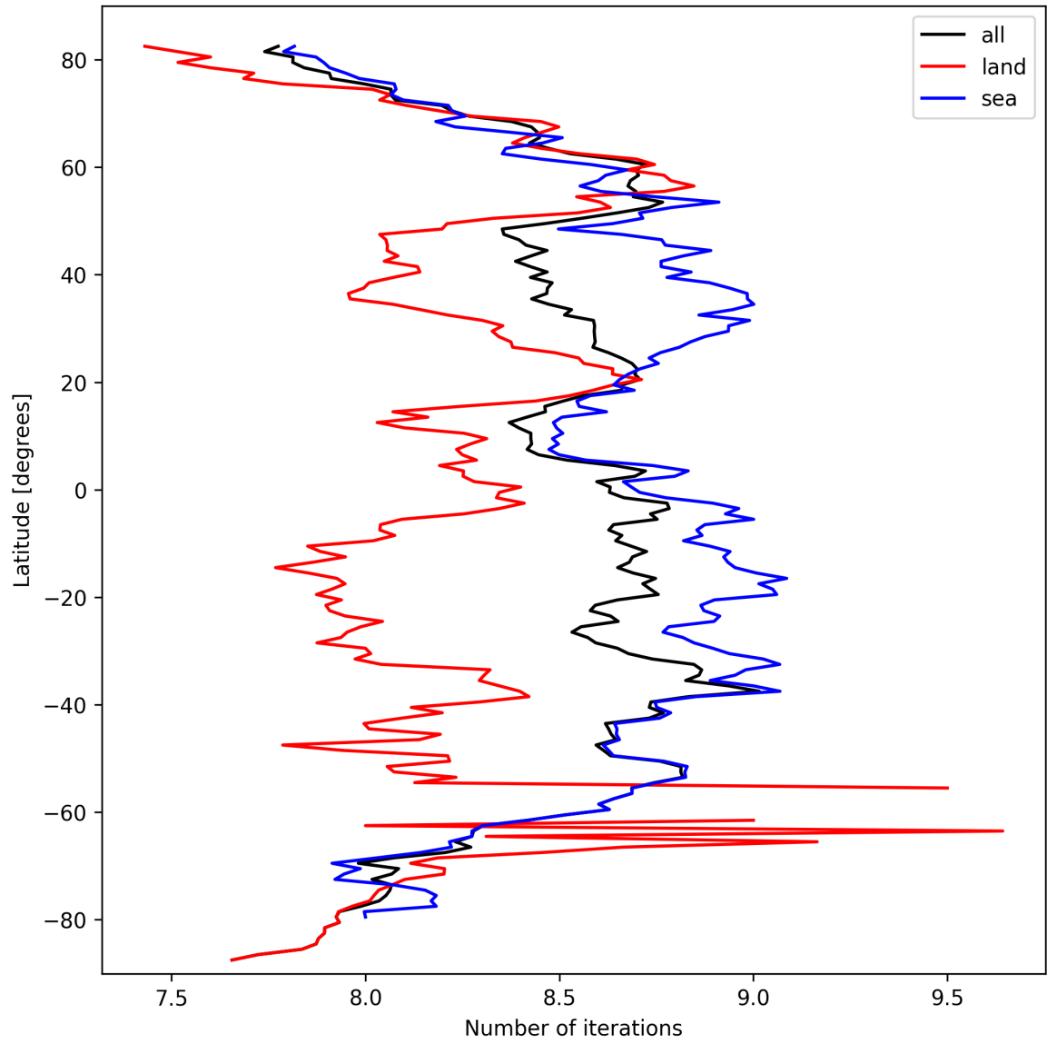
Figure 16: Zonal average of “Number of iterations” for 2025-09-28 to 2025-09-30.
