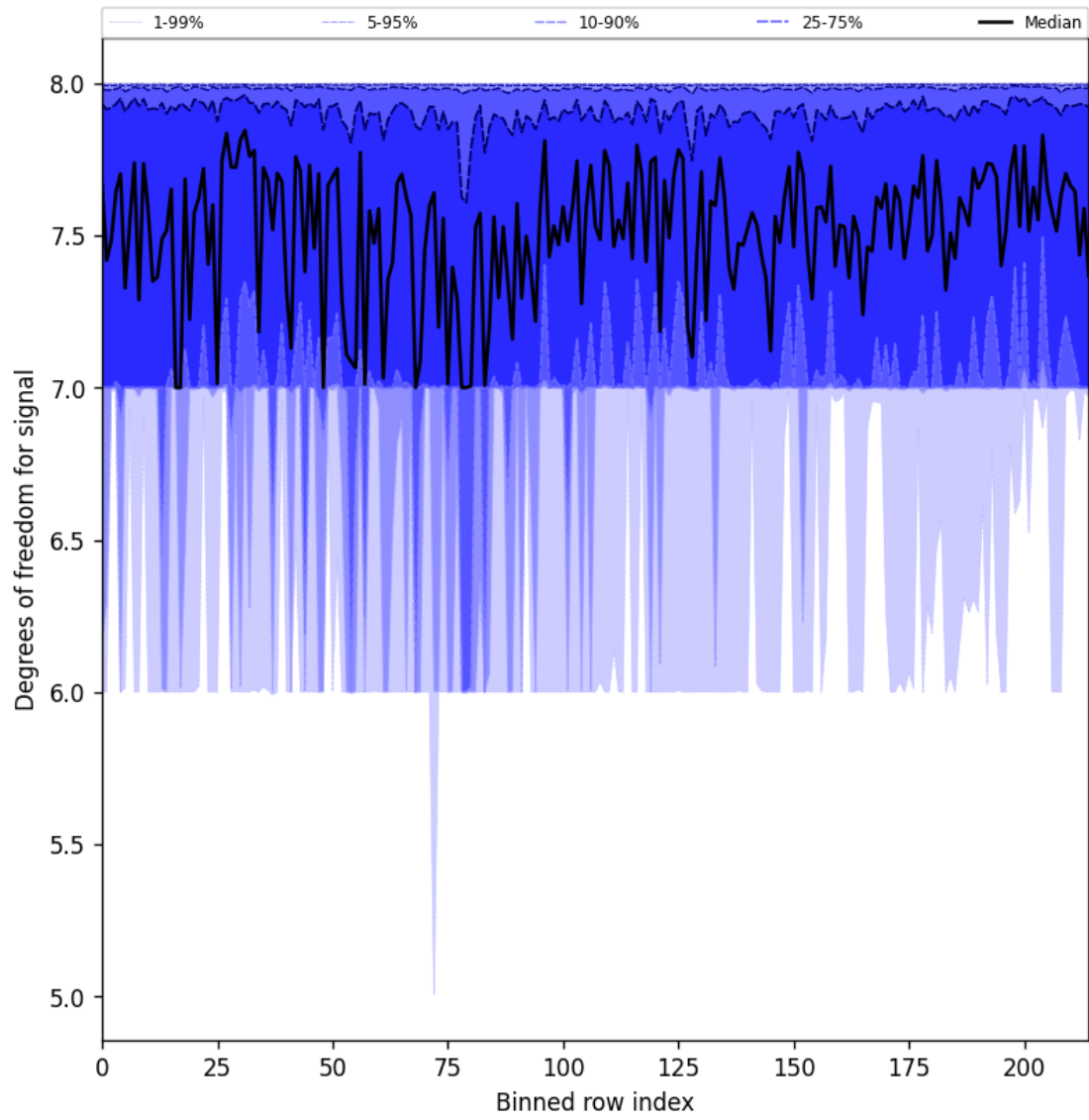
Figure 31: Along track statistics of “Degrees of freedom for signal” for 2025-09-28 to 2025-09-30
