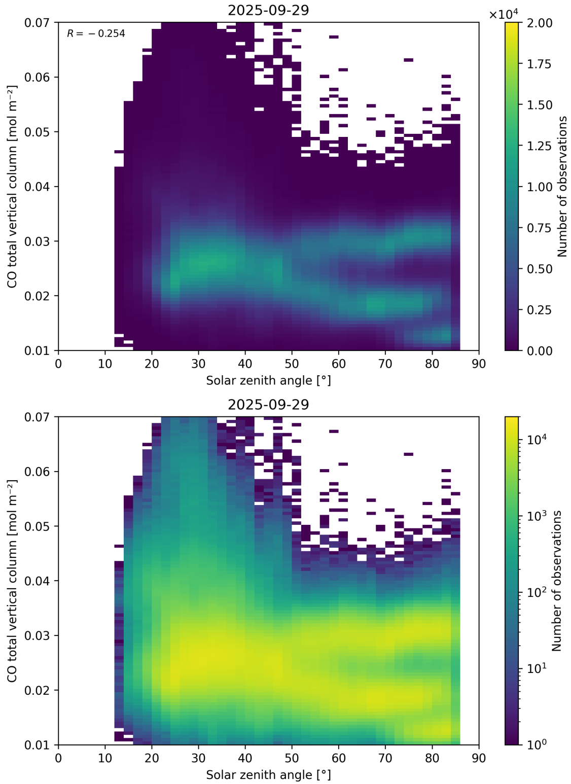
Figure 61: Scatter density plot of “Solar zenith angle” against “CO total vertical column” for 2025-09-28 to 2025-09-30.
