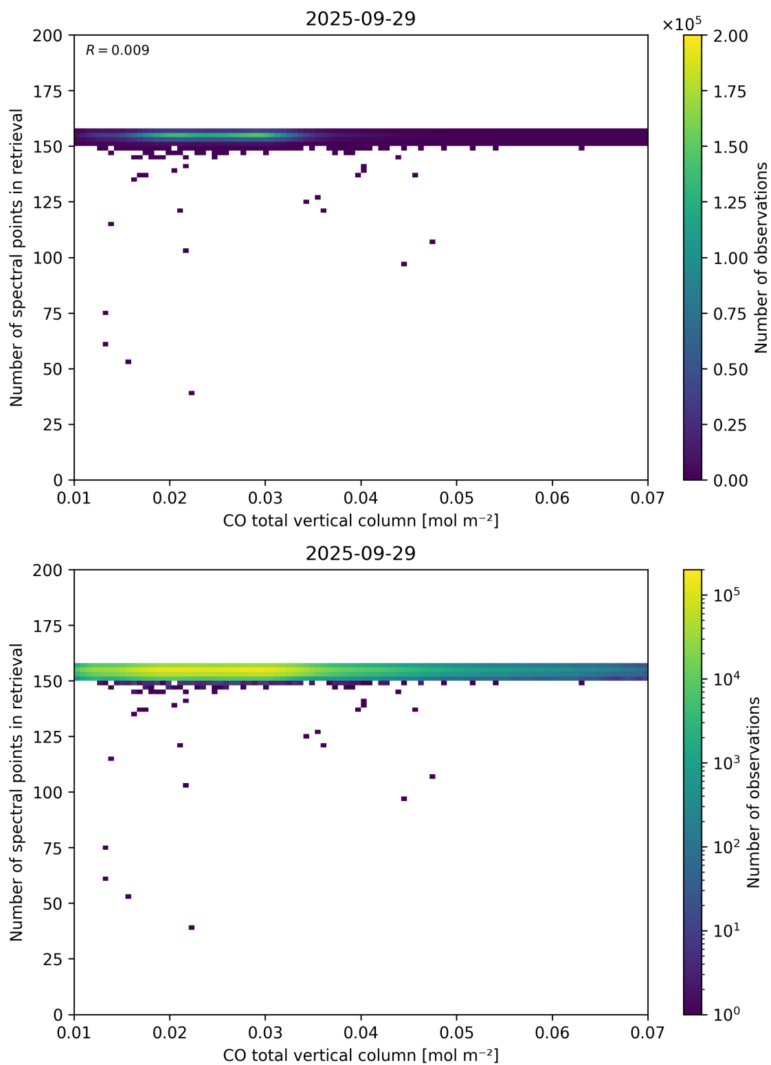
Figure 43: Scatter density plot of “CO total vertical column” against “Number of spectral points in retrieval” for 2025-09-28 to 2025-09-30.
