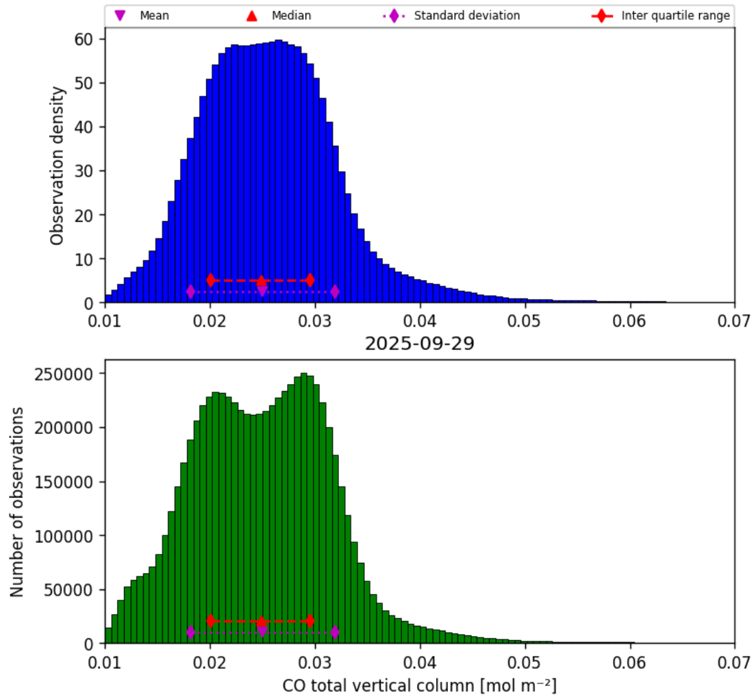
Figure 18: Histogram of “CO total vertical column” for 2025-09-28 to 2025-09-30
