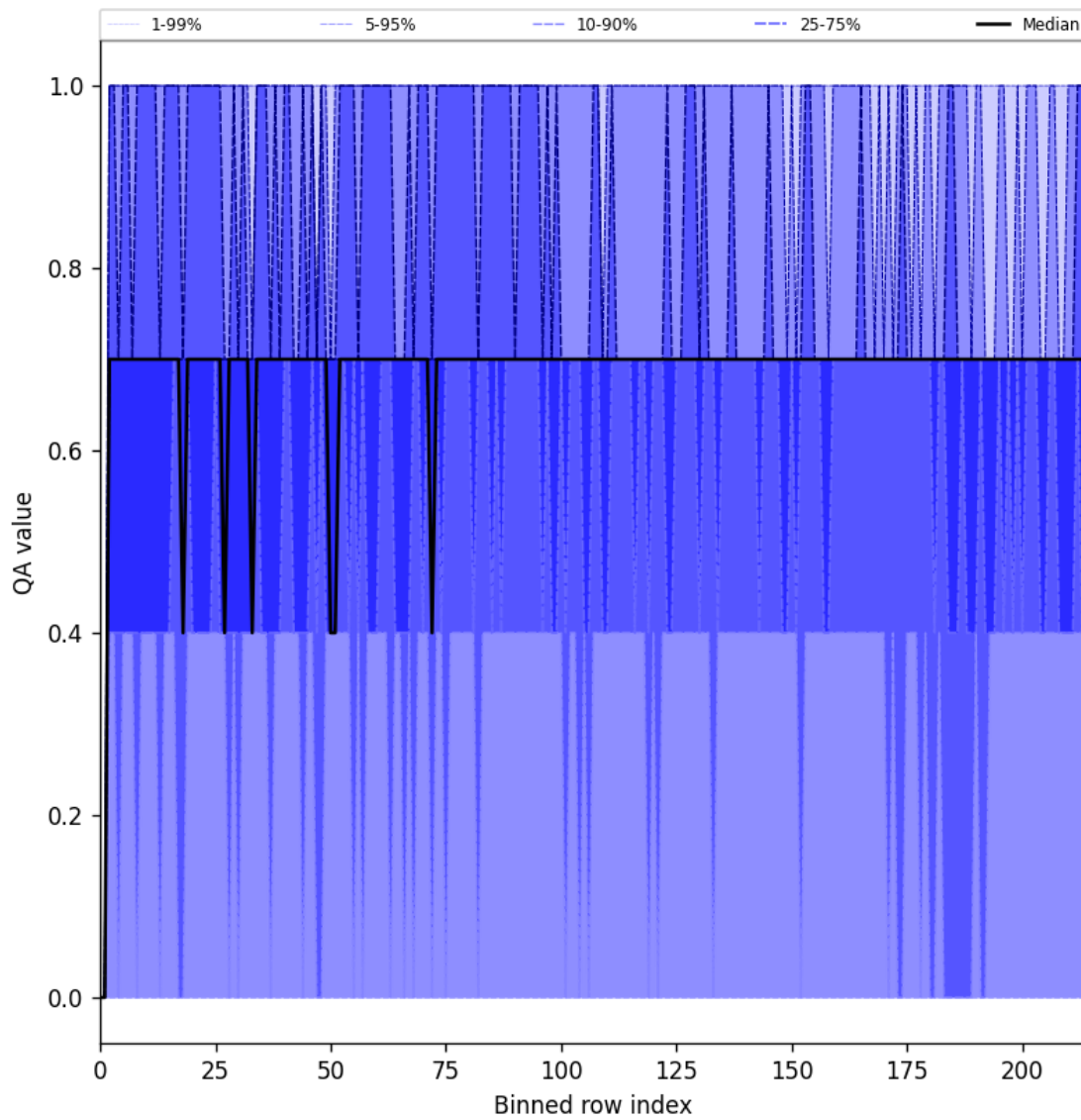
Figure 25: Along track statistics of “QA value” for 2025-09-28 to 2025-09-30
