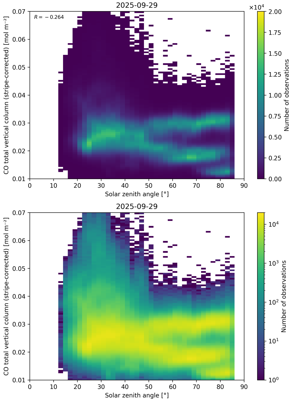
Figure 62: Scatter density plot of “Solar zenith angle” against “CO total vertical column (stripe-corrected)” for 2025-09-28 to 2025-09-30.
