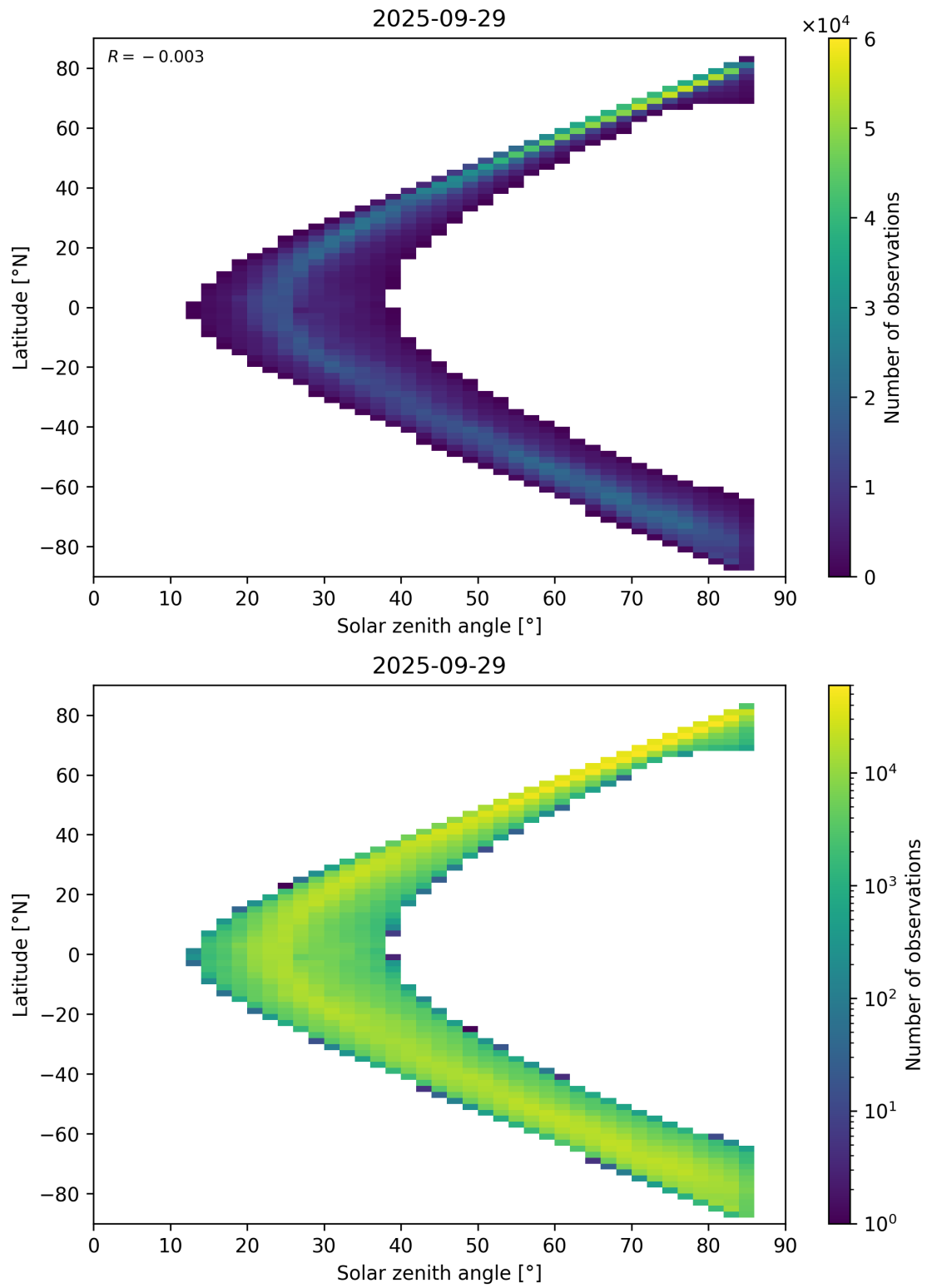
Figure 66: Scatter density plot of “Solar zenith angle” against “Latitude” for 2025-09-28 to 2025-09-30.
