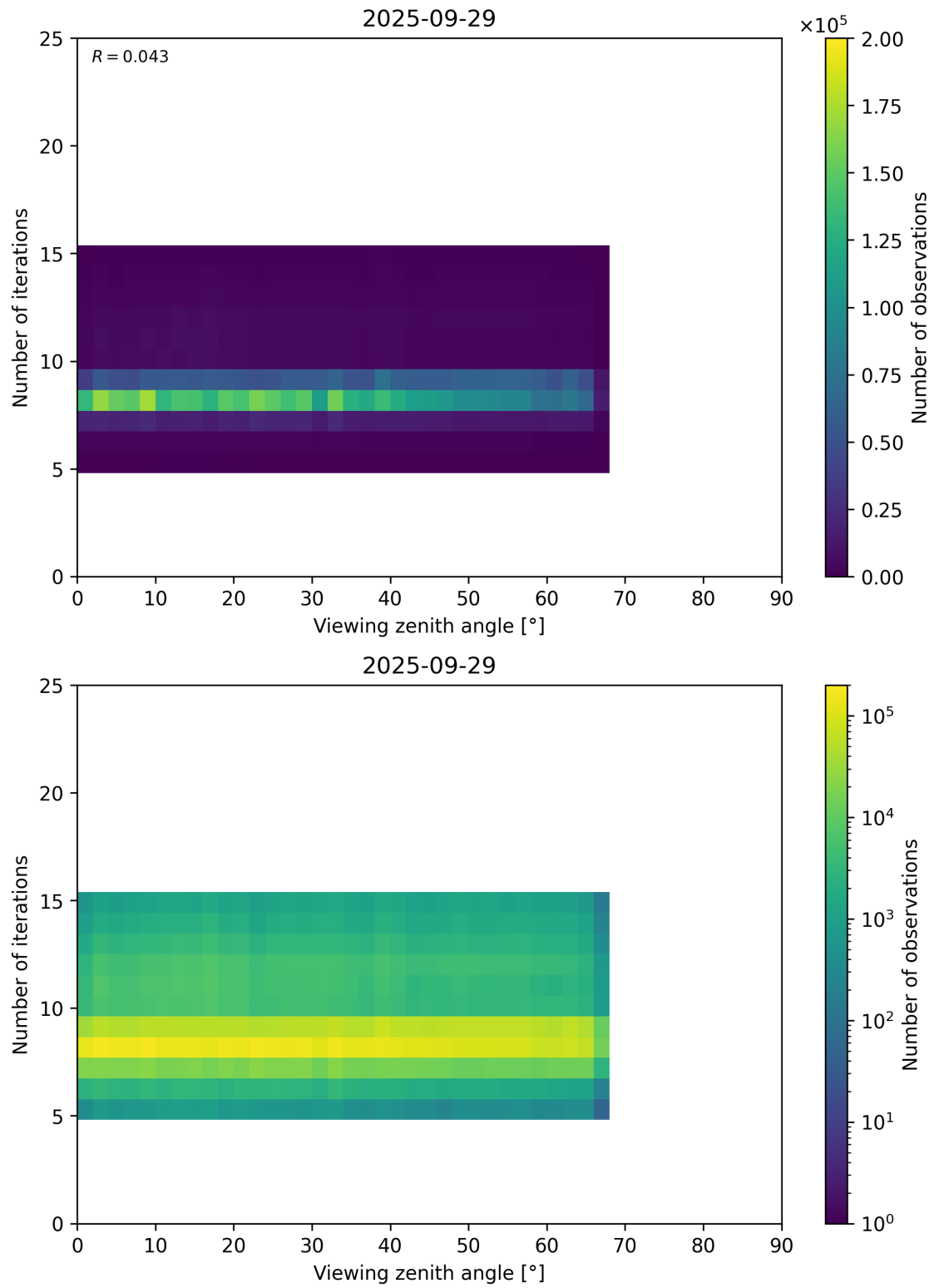
Figure 75: Scatter density plot of “Viewing zenith angle” against “Number of iterations” for 2025-09-28 to 2025-09-30.
