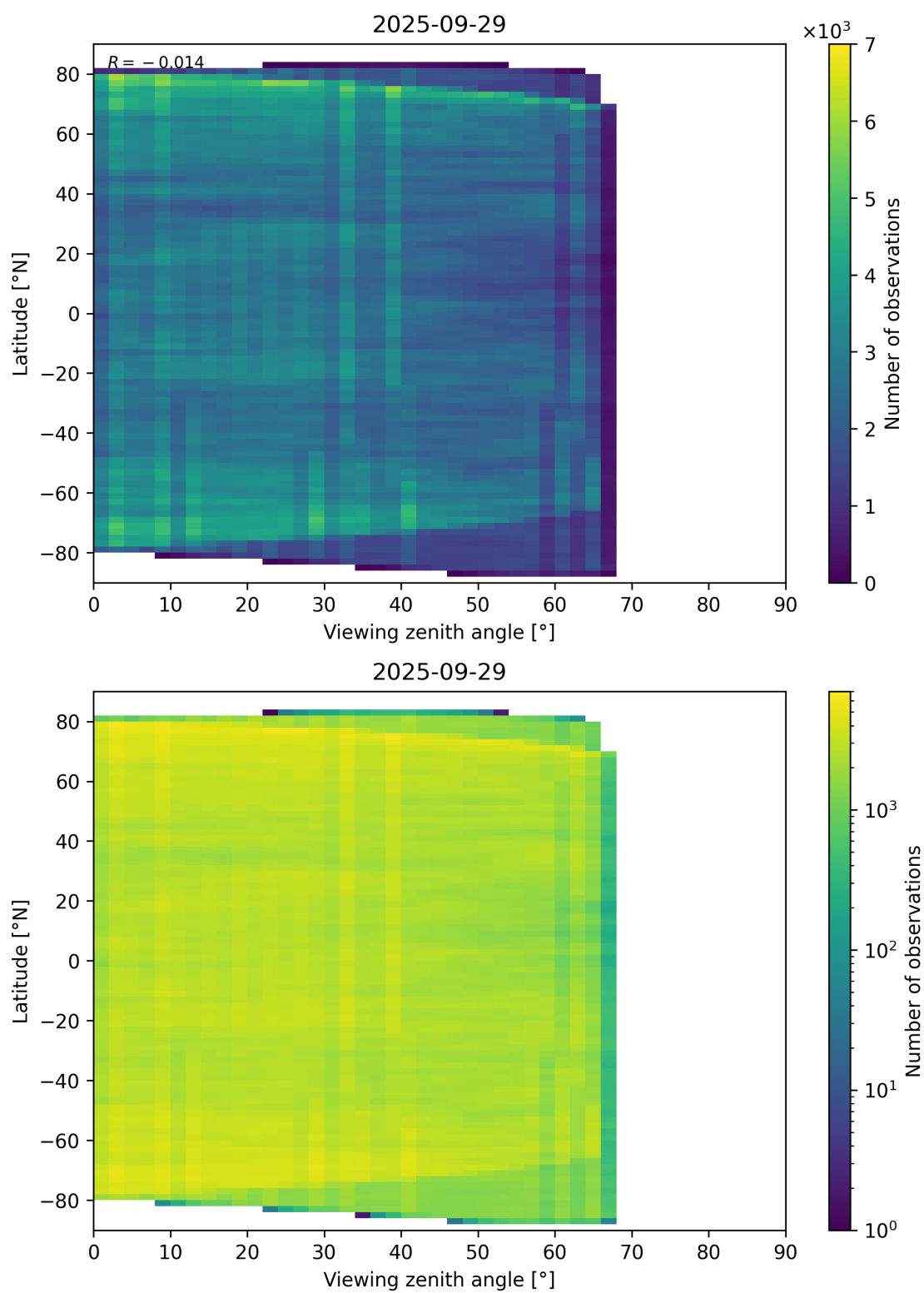
Figure 74: Scatter density plot of “Viewing zenith angle” against “Latitude” for 2025-09-28 to 2025-09-30.
