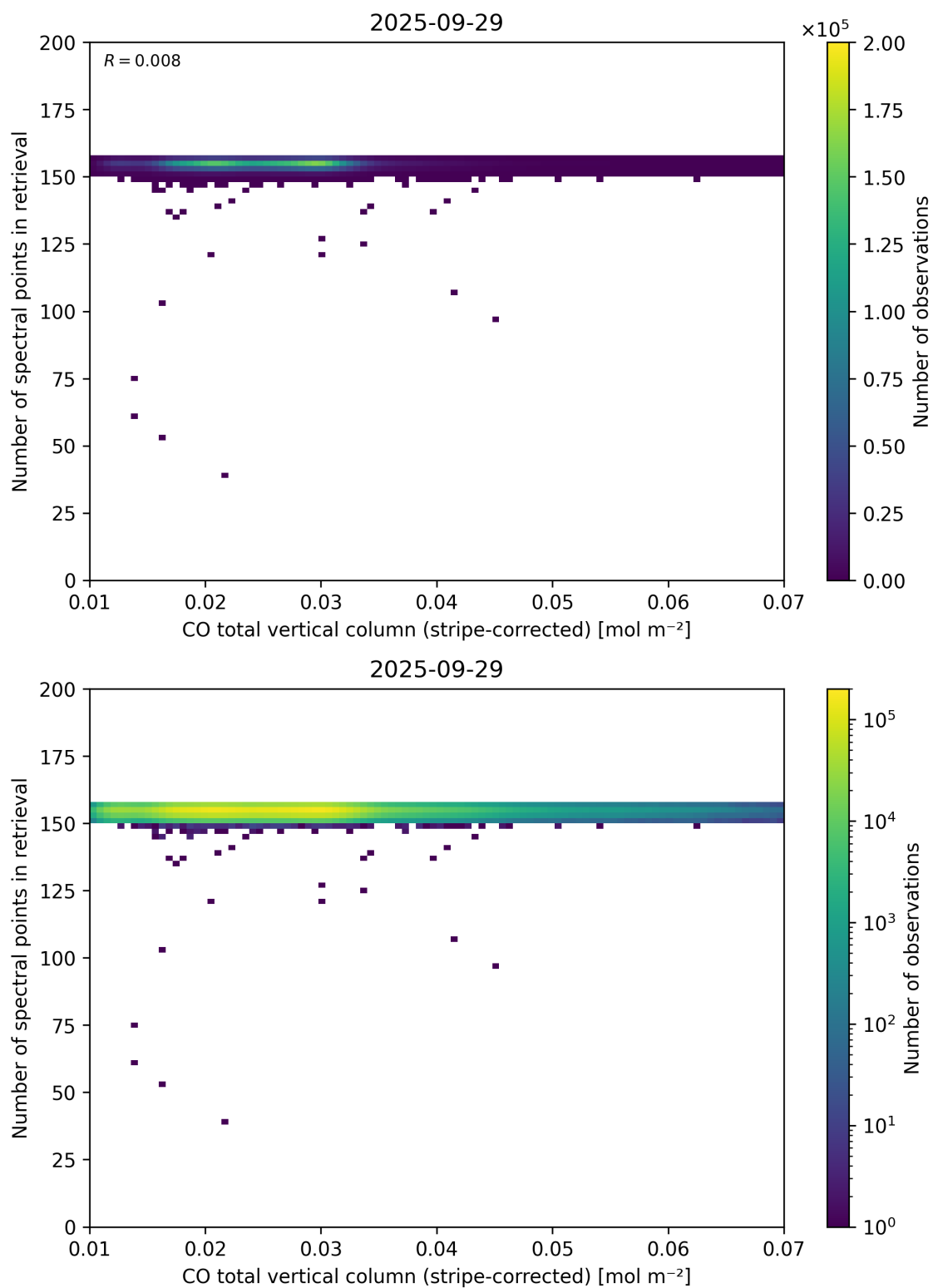
Figure 40: Scatter density plot of “CO total vertical column (stripe-corrected)” against “Number of spectral points in retrieval” for 2025-09-28 to 2025-09-30.
