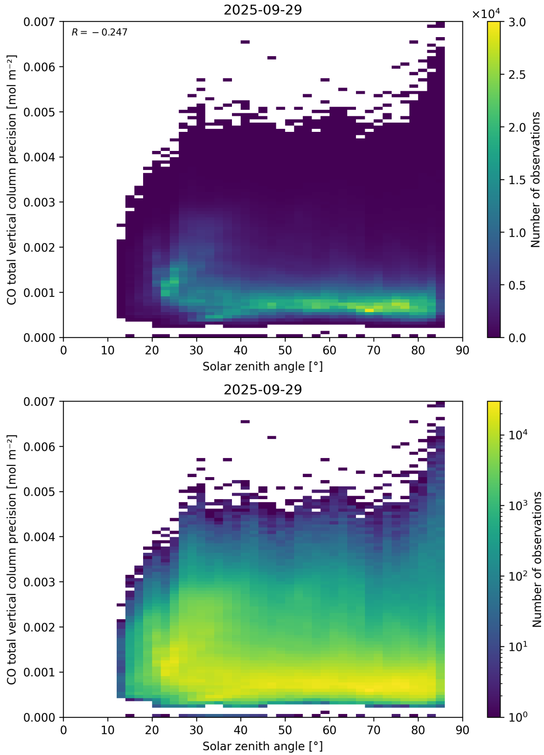
Figure 63: Scatter density plot of “Solar zenith angle” against “CO total vertical column precision” for 2025-09-28 to 2025-09-30.
