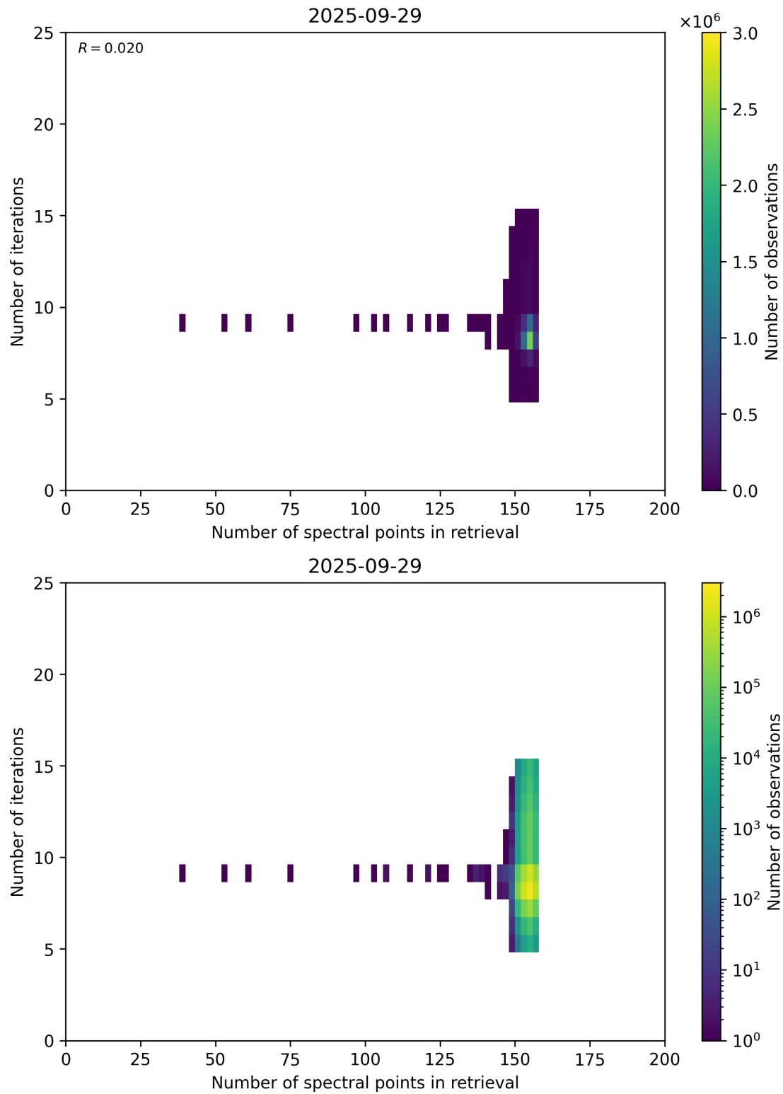
Figure 60: Scatter density plot of “Number of spectral points in retrieval” against “Number of iterations” for 2025-09-28 to 2025-09-30.
