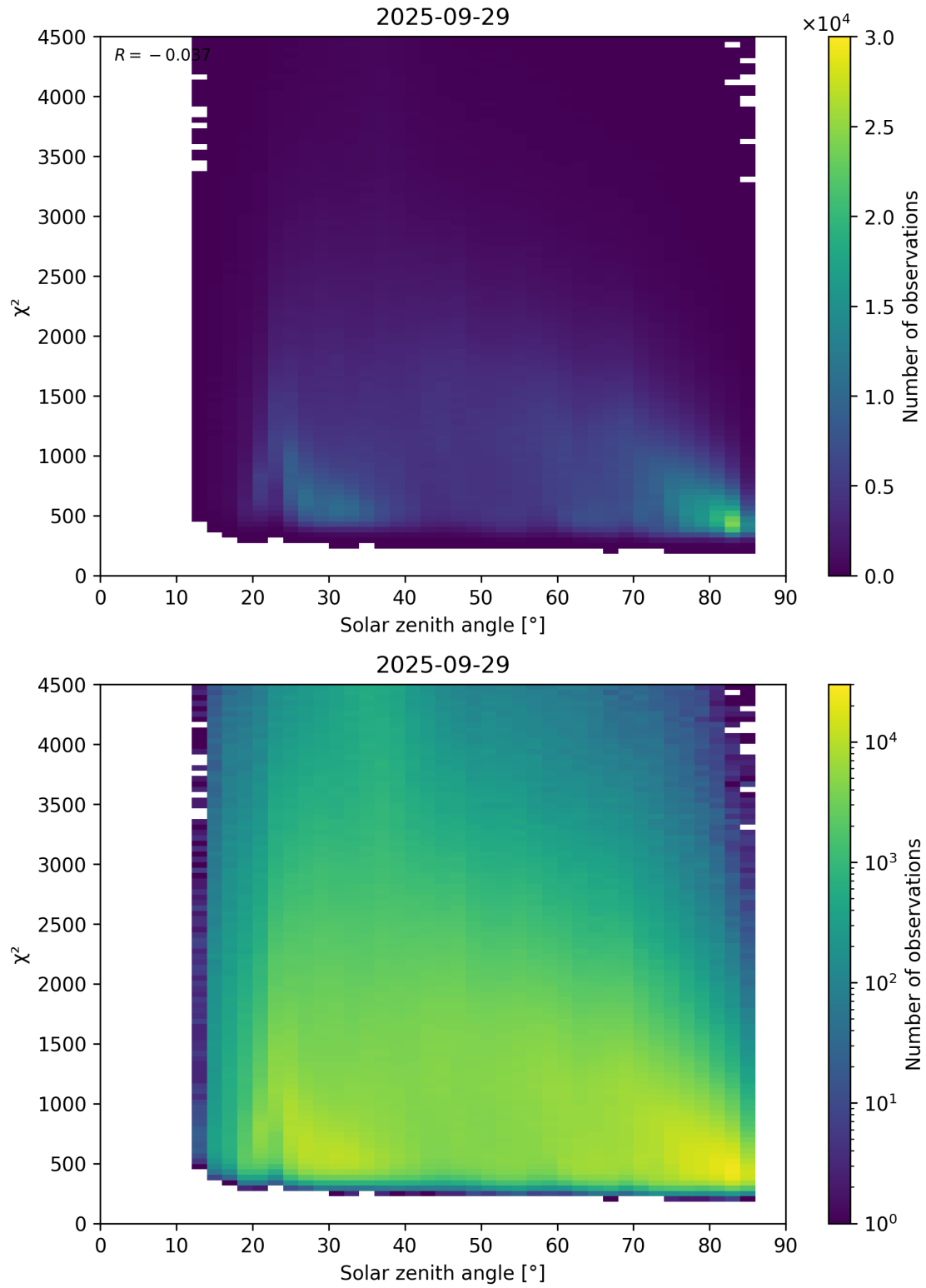
Figure 64: Scatter density plot of “Solar zenith angle” against “ \chi^2 ” for 2025-09-28 to 2025-09-30.
