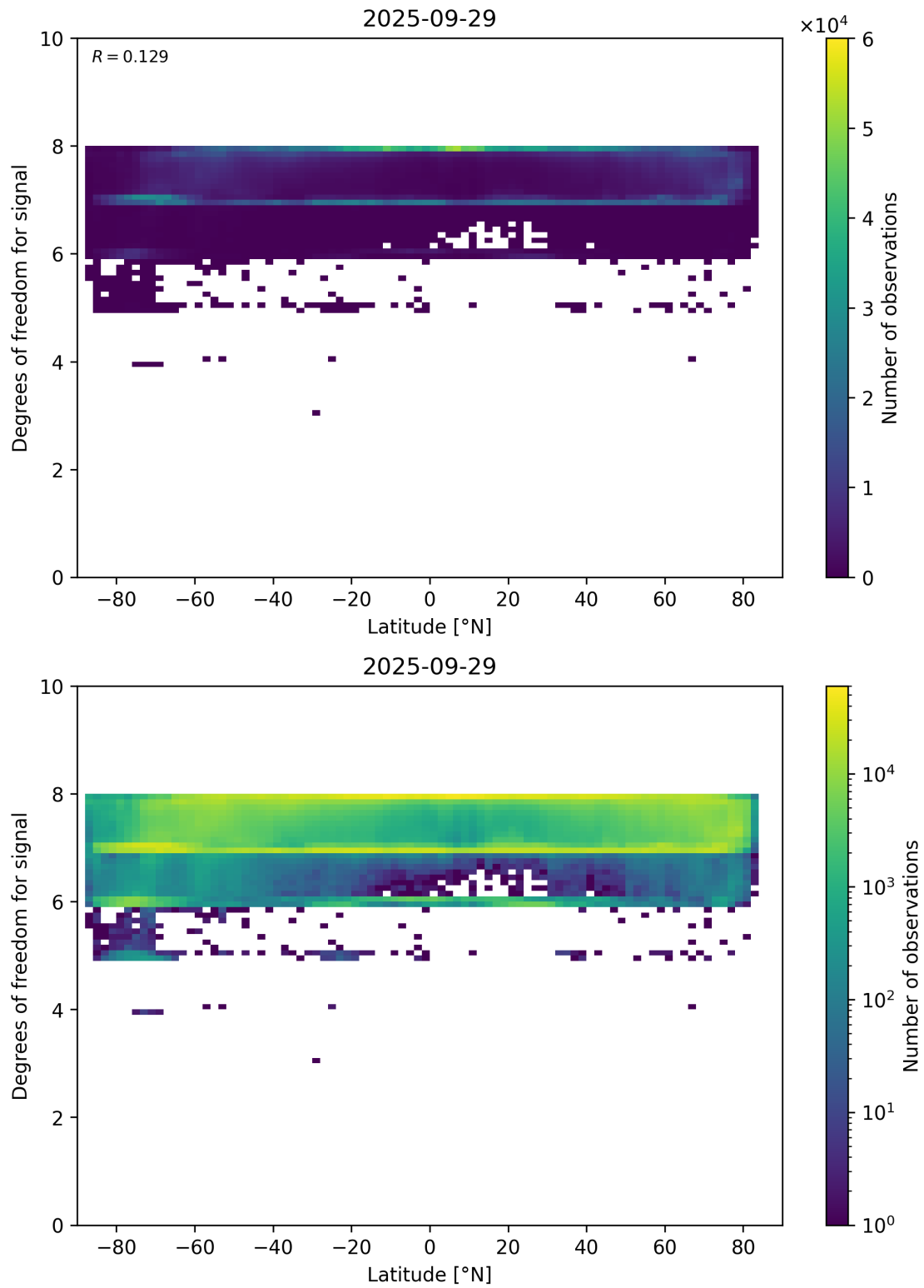
Figure 55: Scatter density plot of “Latitude” against “Degrees of freedom for signal” for 2025-09-28 to 2025-09-30.
