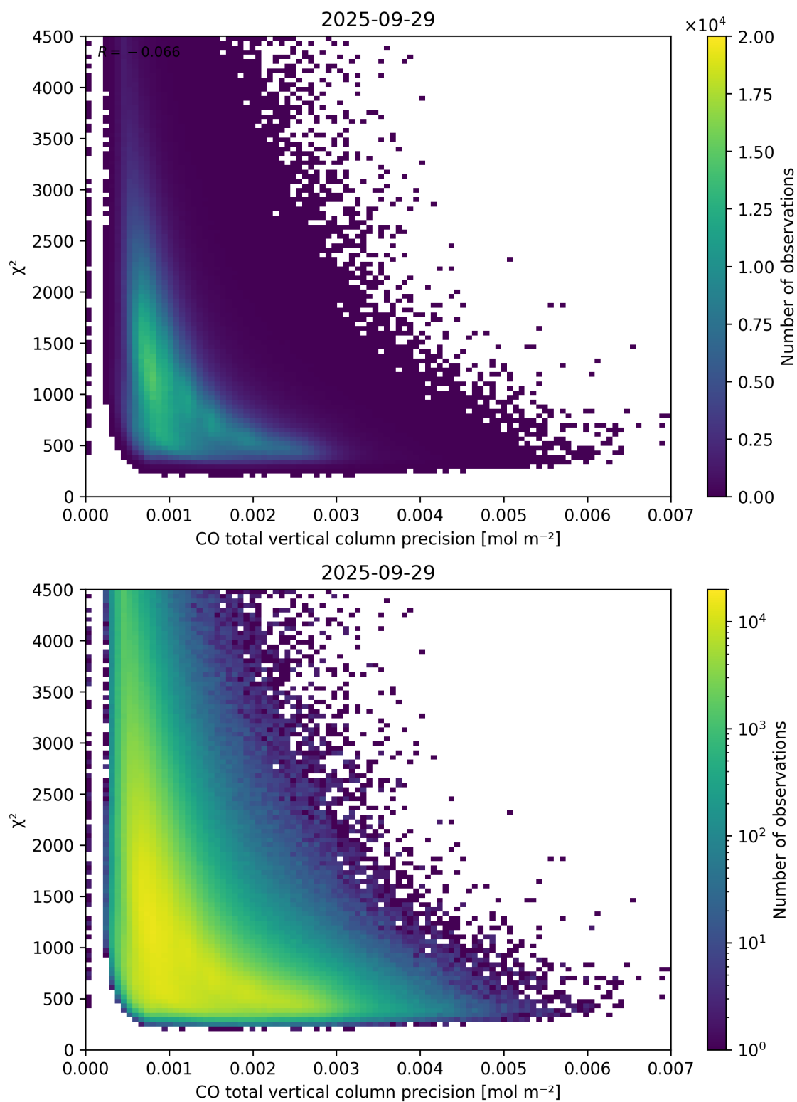
Figure 44: Scatter density plot of “CO total vertical column precision” against “ \chi^2 ” for 2025-09-28 to 2025-09-30.
