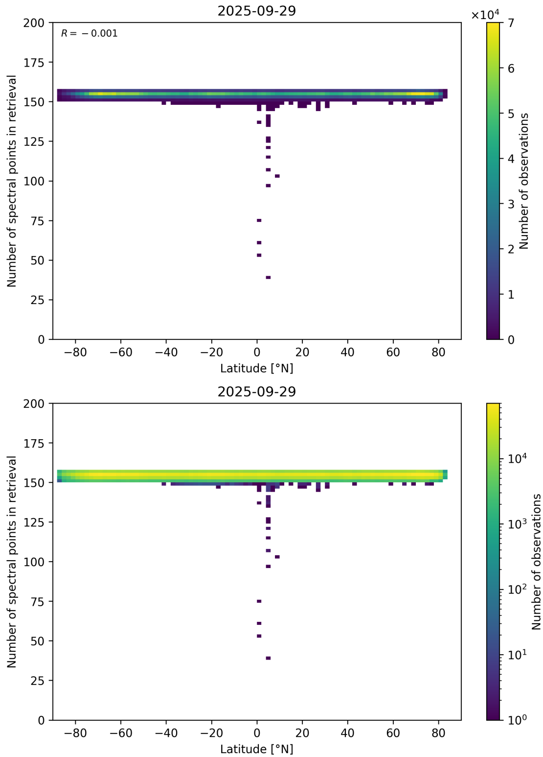
Figure 57: Scatter density plot of “Latitude” against “Number of spectral points in retrieval” for 2025-09-28 to 2025-09-30.
