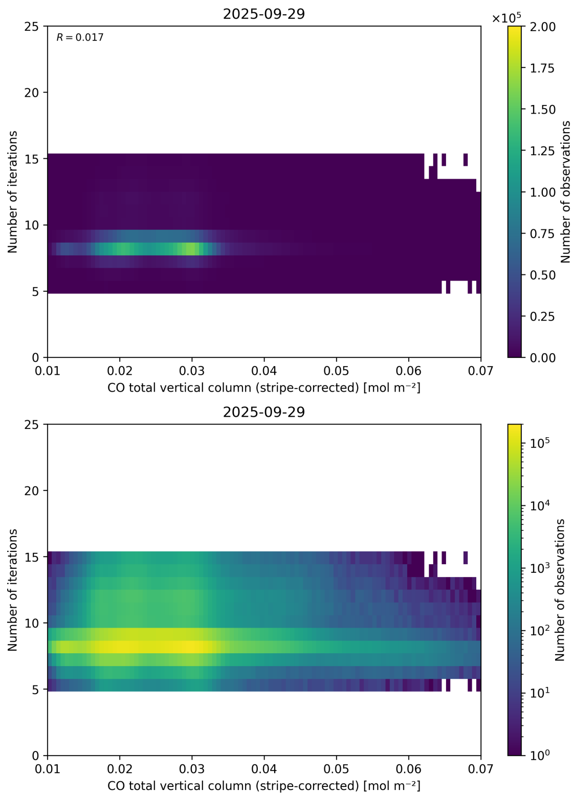
Figure 39: Scatter density plot of “CO total vertical column (stripe-corrected)” against “Number of iterations” for 2025-09-28 to 2025-09-30.
