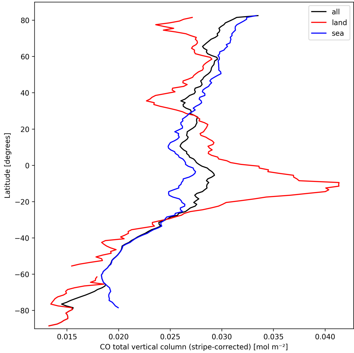
Figure 11: Zonal average of “CO total vertical column (stripe-corrected)” for 2025-09-29 to 2025-10-01.
