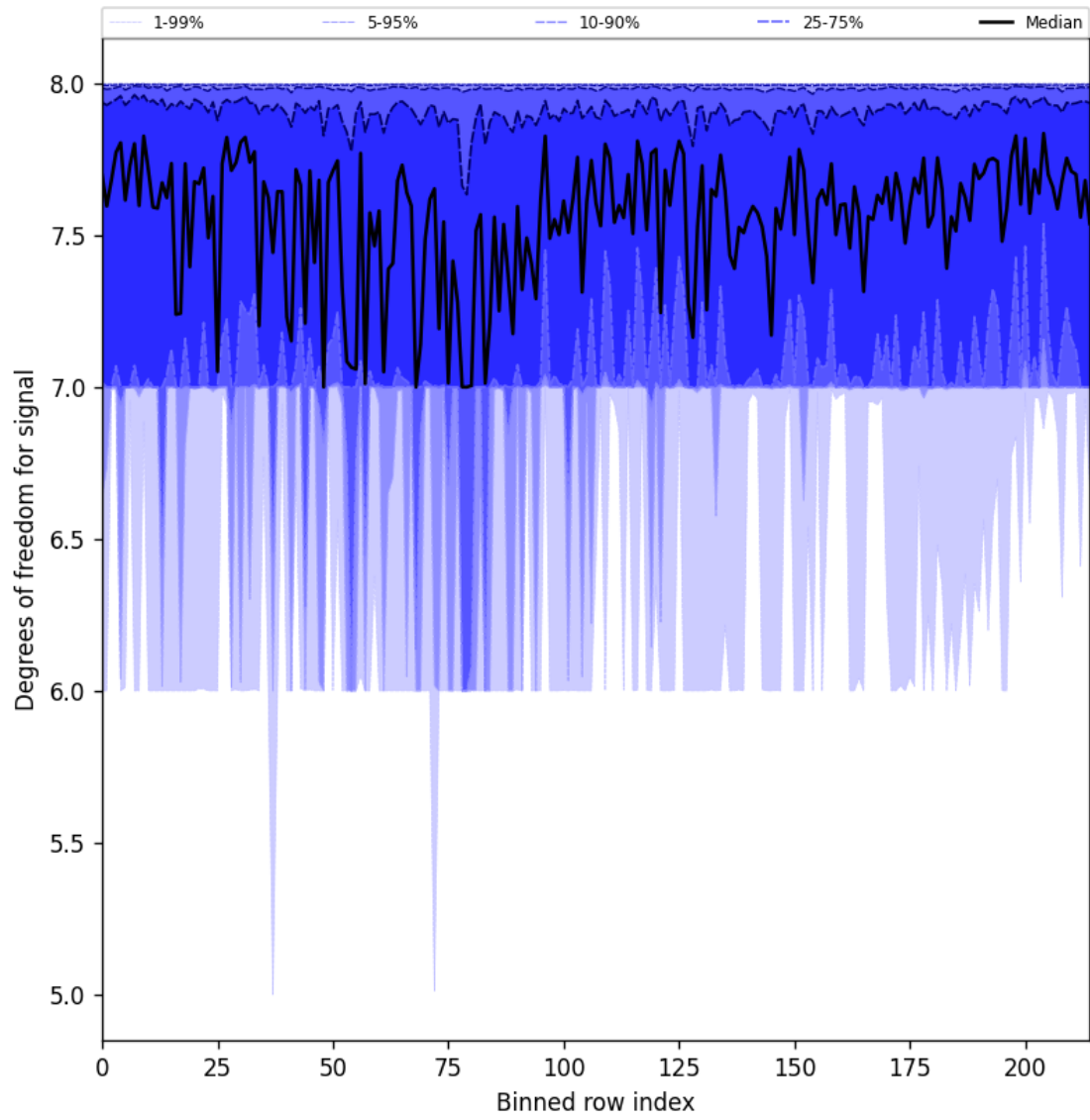
Figure 31: Along track statistics of “Degrees of freedom for signal” for 2025-09-29 to 2025-10-01
