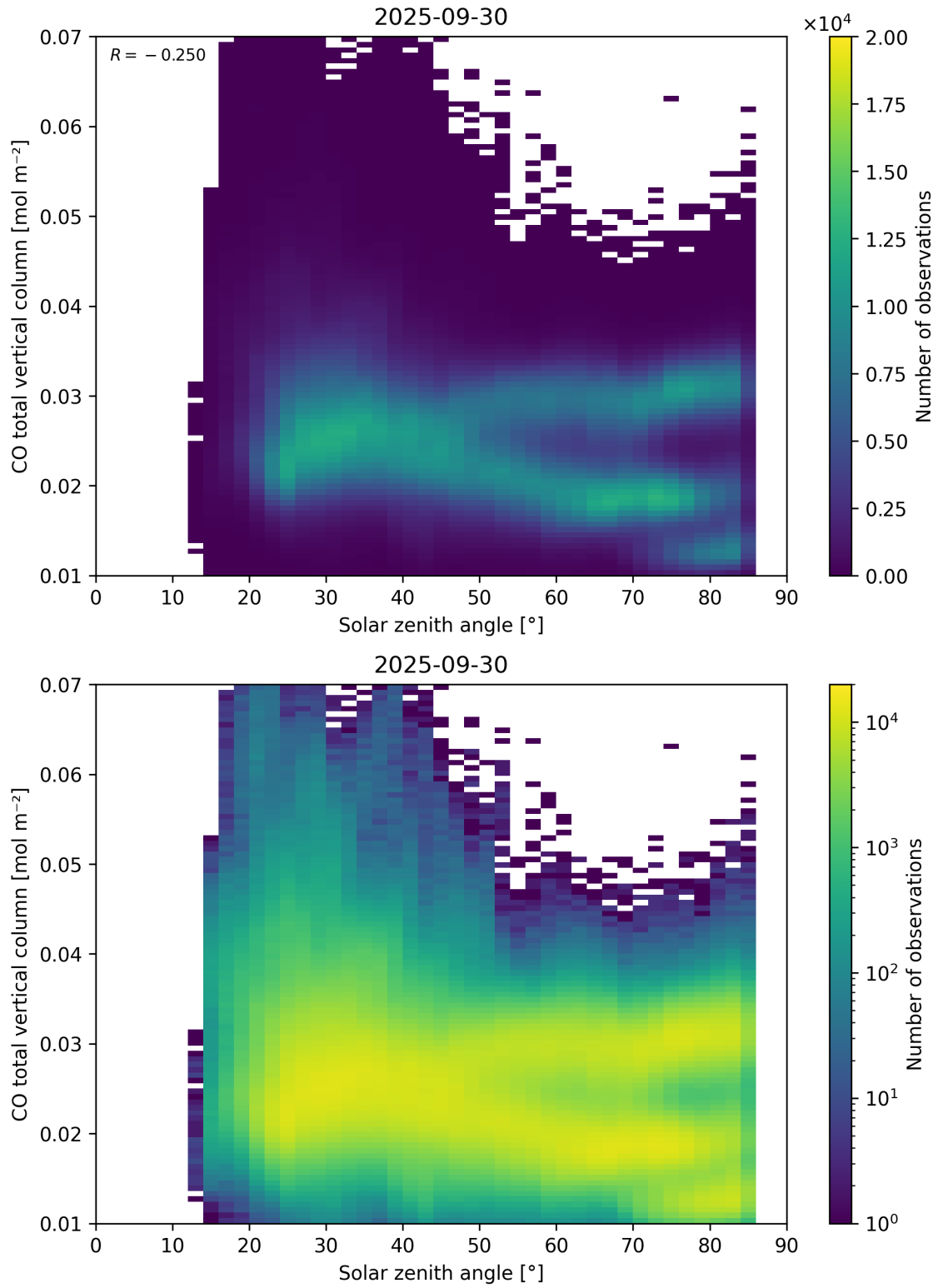
Figure 61: Scatter density plot of “Solar zenith angle” against “CO total vertical column” for 2025-09-29 to 2025-10-01.
