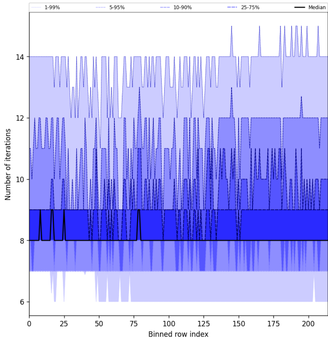
Figure 32: Along track statistics of “Number of iterations” for 2025-09-29 to 2025-10-01
