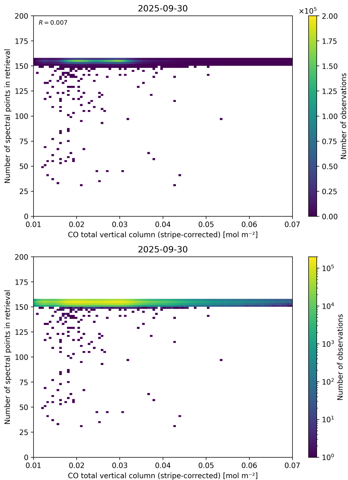
Figure 40: Scatter density plot of “CO total vertical column (stripe-corrected)” against “Number of spectral points in retrieval” for 2025-09-29 to 2025-10-01.
