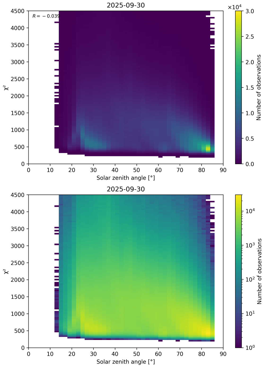
Figure 64: Scatter density plot of “Solar zenith angle” against “ \chi^2 ” for 2025-09-29 to 2025-10-01.
