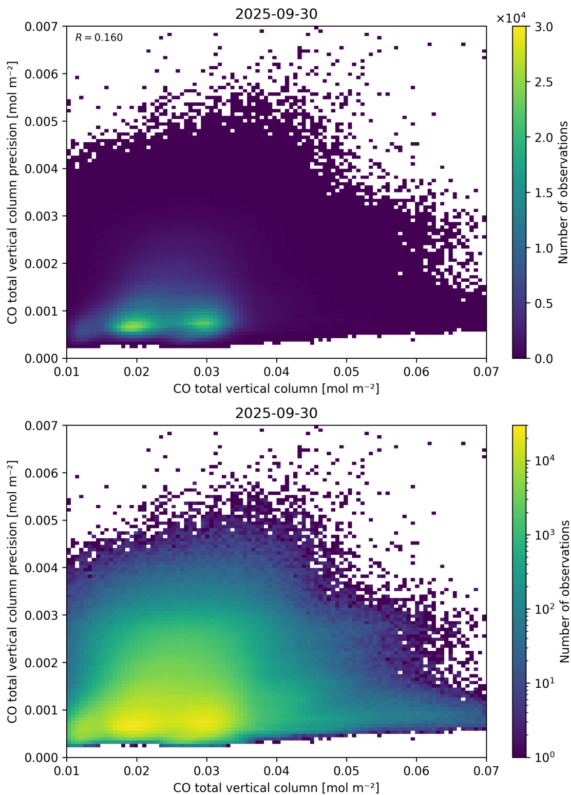
Figure 34: Scatter density plot of “CO total vertical column” against “CO total vertical column precision” for 2025-09-29 to 2025-10-01.
