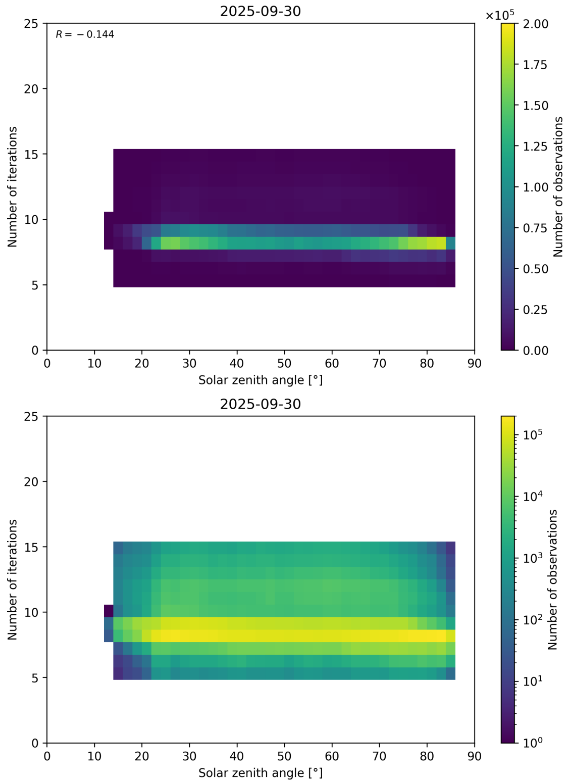
Figure 67: Scatter density plot of “Solar zenith angle” against “Number of iterations” for 2025-09-29 to 2025-10-01.
