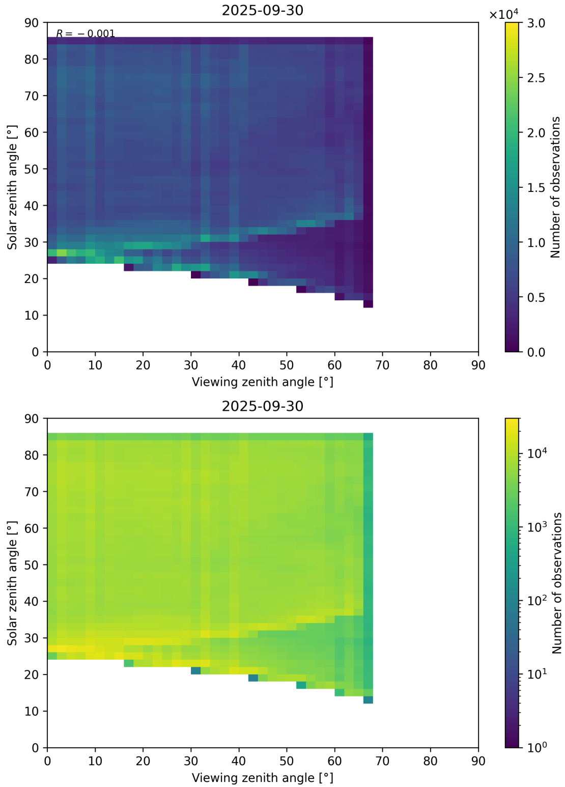
Figure 77: Scatter density plot of “Viewing zenith angle” against “Solar zenith angle” for 2025-09-29 to 2025-10-01.
