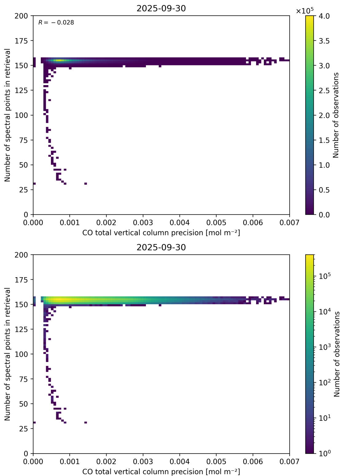
Figure 47: Scatter density plot of “CO total vertical column precision” against “Number of spectral points in retrieval” for 2025-09-29 to 2025-10-01.
