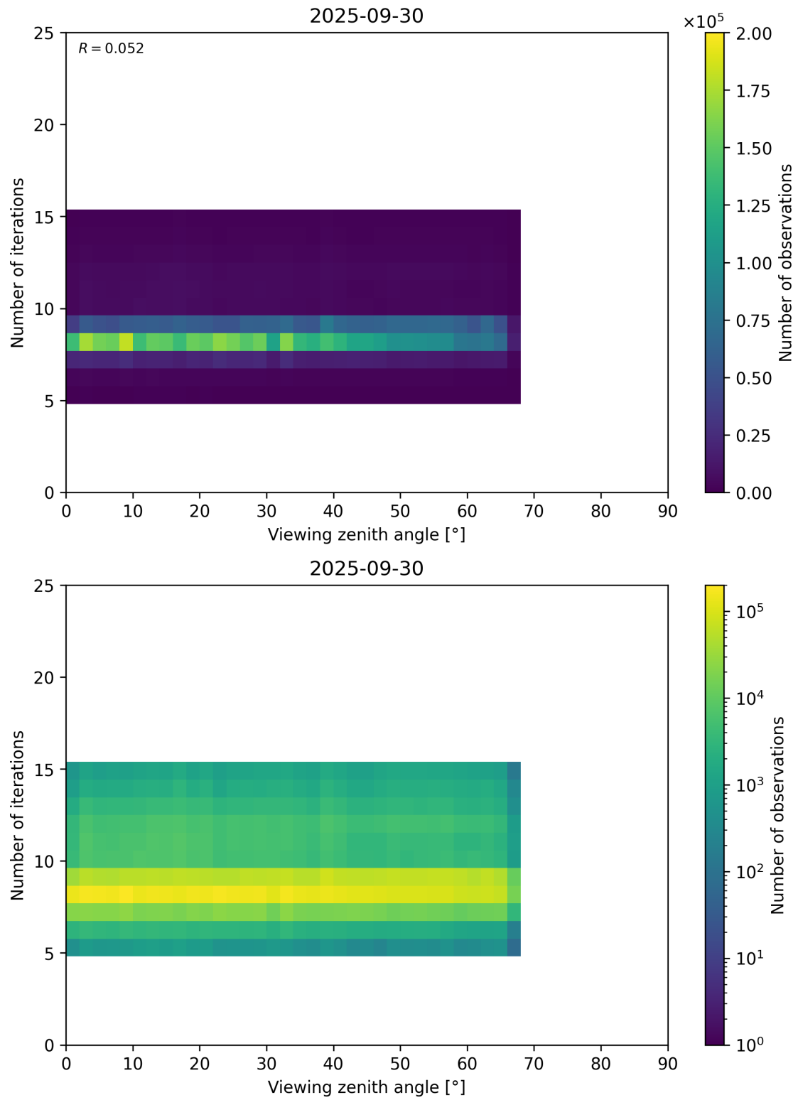
Figure 75: Scatter density plot of “Viewing zenith angle” against “Number of iterations” for 2025-09-29 to 2025-10-01.
