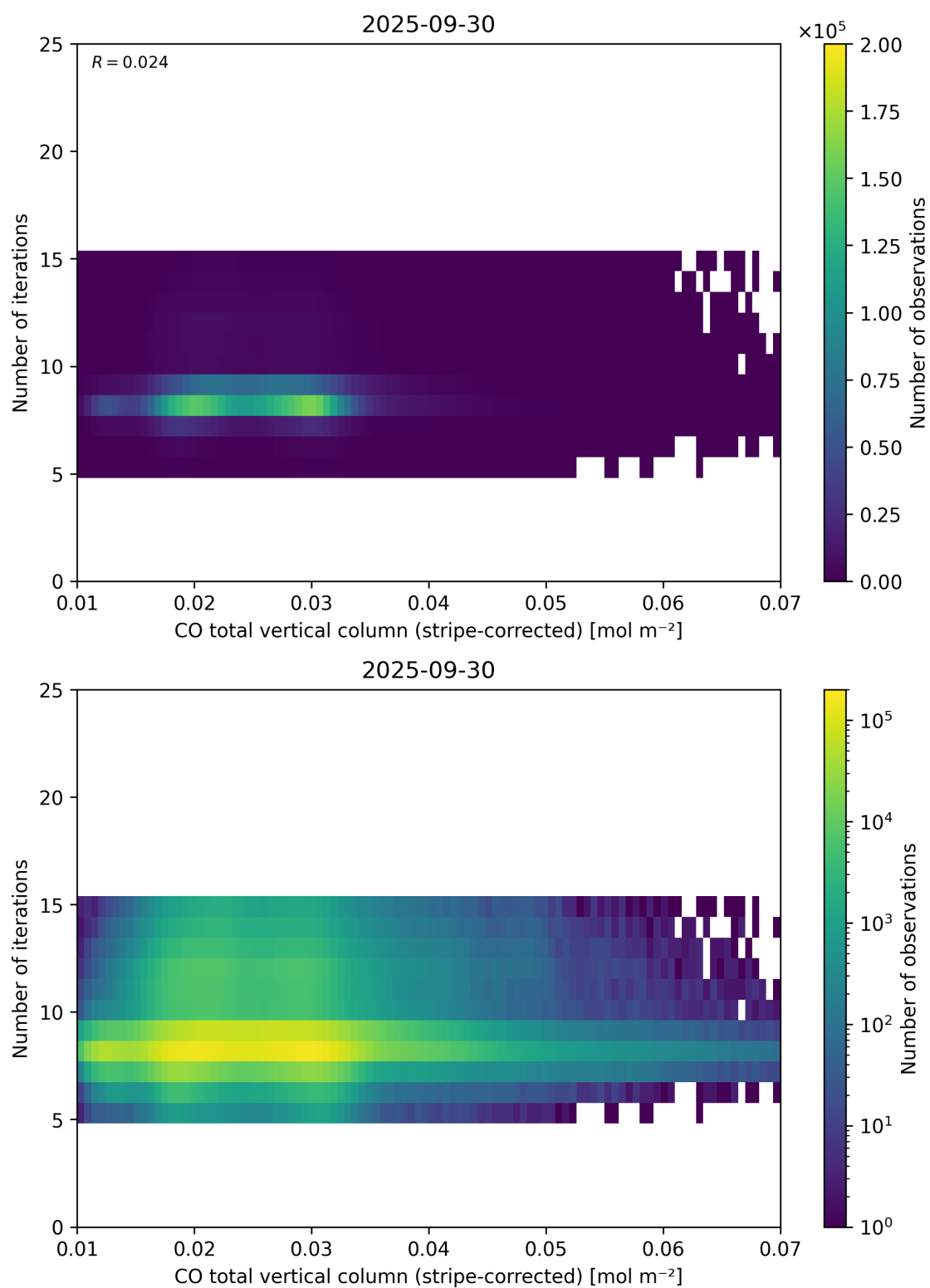
Figure 39: Scatter density plot of “CO total vertical column (stripe-corrected)” against “Number of iterations” for 2025-09-29 to 2025-10-01.
