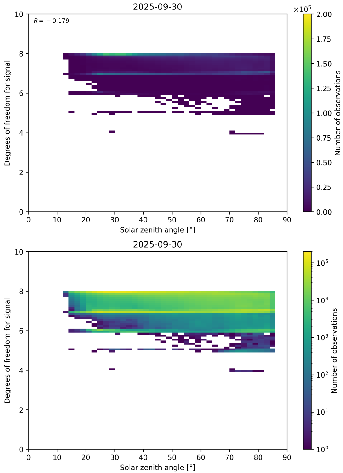
Figure 65: Scatter density plot of “Solar zenith angle” against “Degrees of freedom for signal” for 2025-09-29 to 2025-10-01.
