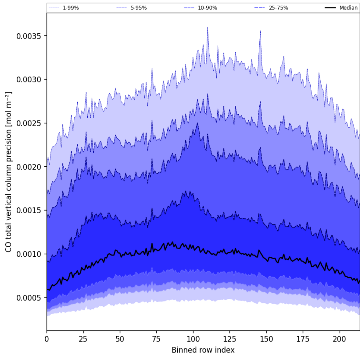
Figure 28: Along track statistics of “CO total vertical column precision” for 2025-09-29 to 2025-10-01
