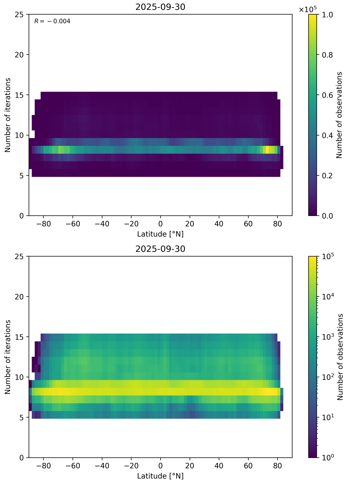
Figure 56: Scatter density plot of “Latitude” against “Number of iterations” for 2025-09-29 to 2025-10-01.
