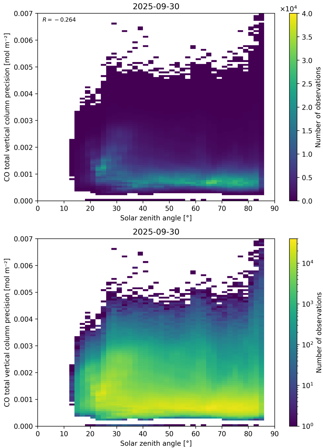
Figure 63: Scatter density plot of “Solar zenith angle” against “CO total vertical column precision” for 2025-09-29 to 2025-10-01.
