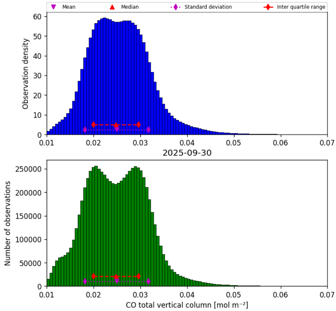
Figure 18: Histogram of “CO total vertical column” for 2025-09-29 to 2025-10-01
