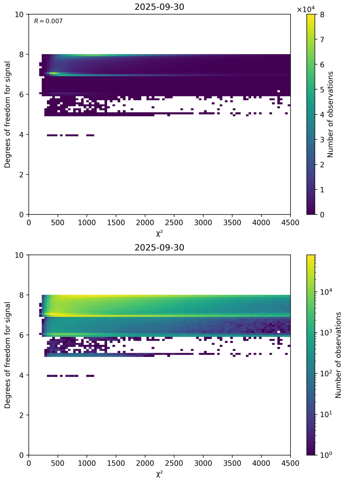
Figure 48: Scatter density plot of " \chi^2 " against "Degrees of freedom for signal" for 2025-09-29 to 2025-10-01.
