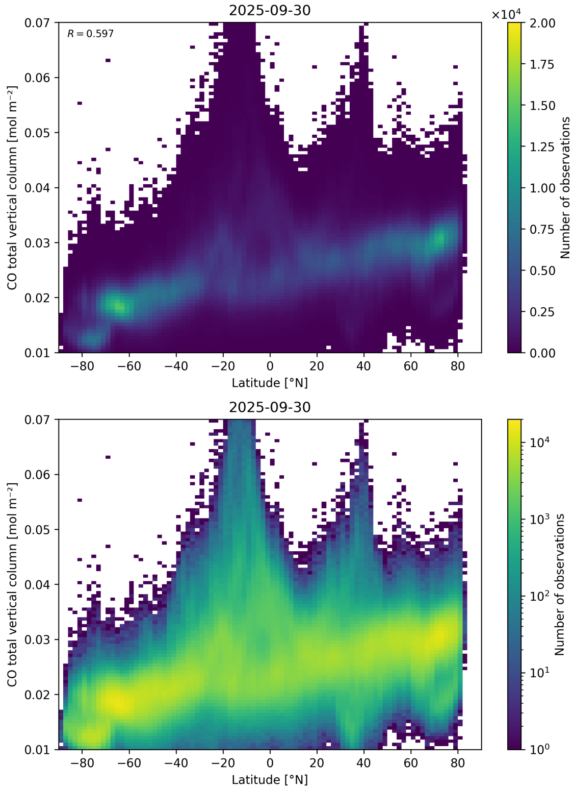
Figure 51: Scatter density plot of “Latitude” against “CO total vertical column” for 2025-09-29 to 2025-10-01.
