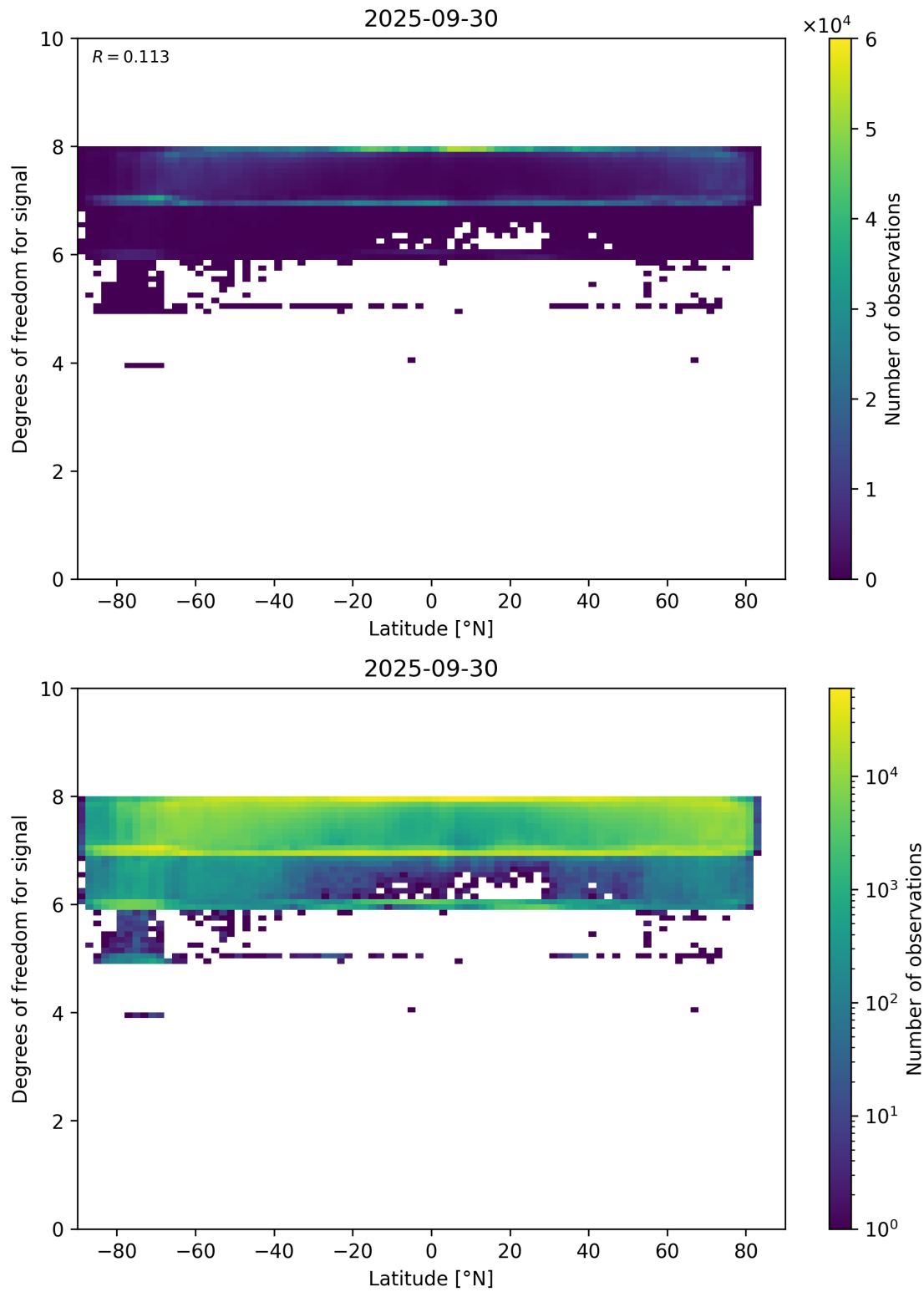
Figure 55: Scatter density plot of “Latitude” against “Degrees of freedom for signal” for 2025-09-29 to 2025-10-01.
