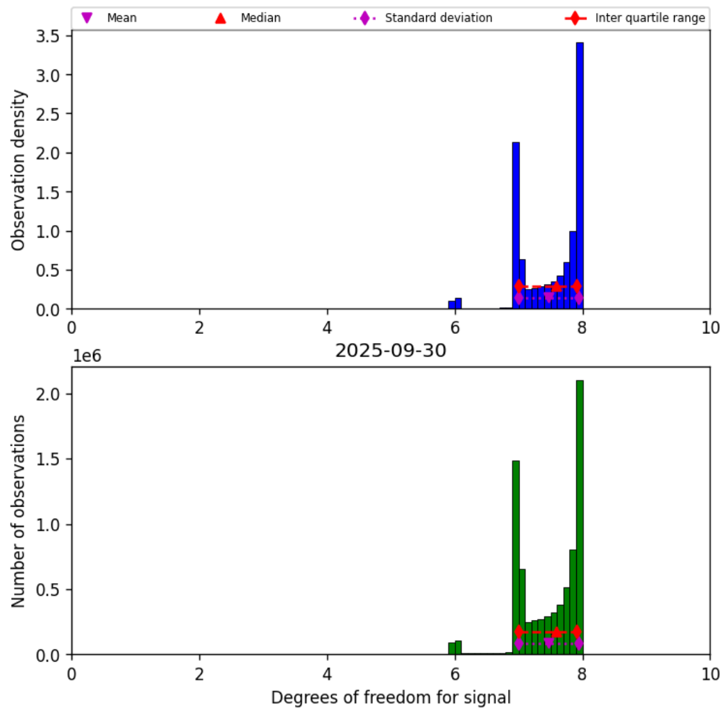
Figure 23: Histogram of “Degrees of freedom for signal” for 2025-09-29 to 2025-10-01
