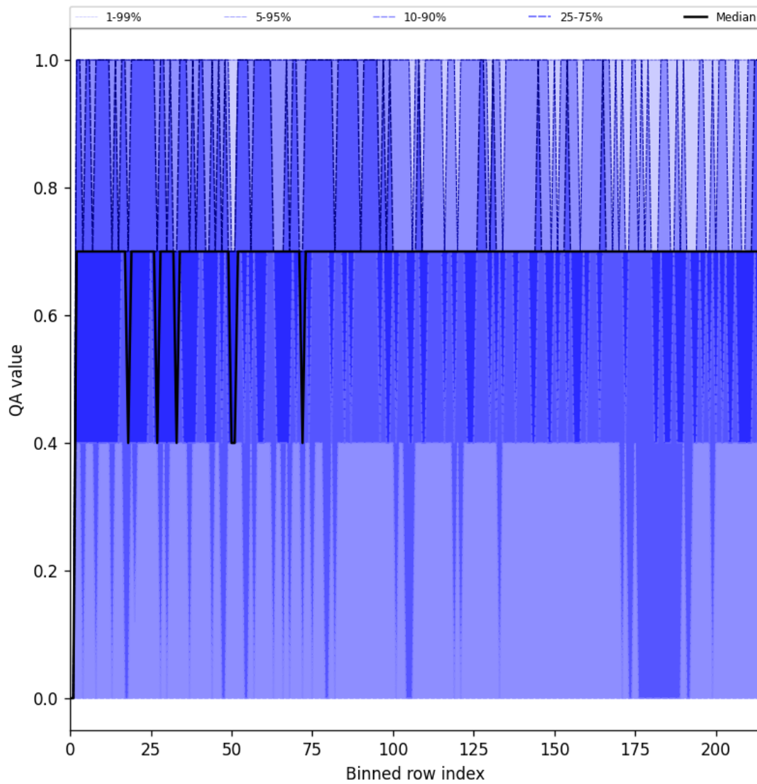
Figure 25: Along track statistics of “QA value” for 2025-09-29 to 2025-10-01
