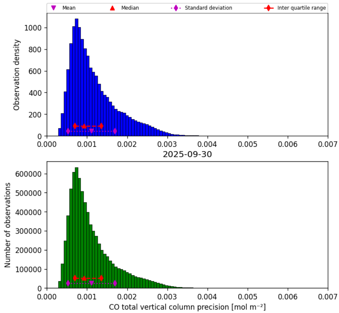
Figure 20: Histogram of “CO total vertical column precision” for 2025-09-29 to 2025-10-01
