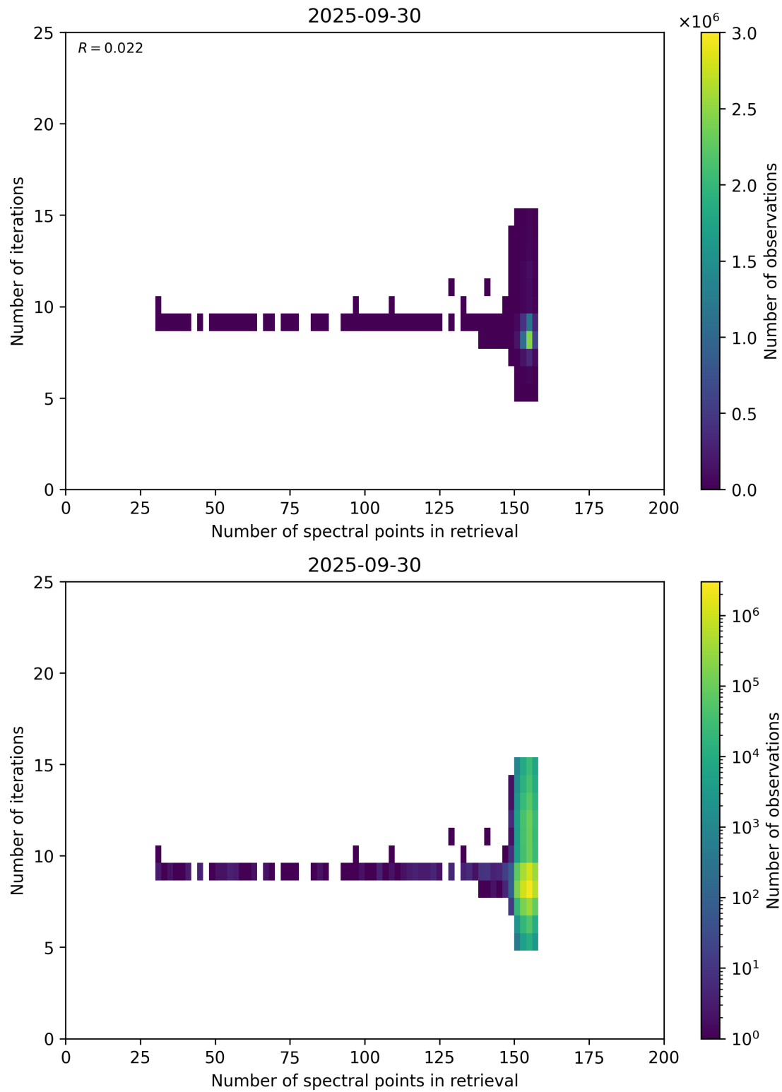
Figure 60: Scatter density plot of “Number of spectral points in retrieval” against “Number of iterations” for 2025-09-29 to 2025-10-01.
