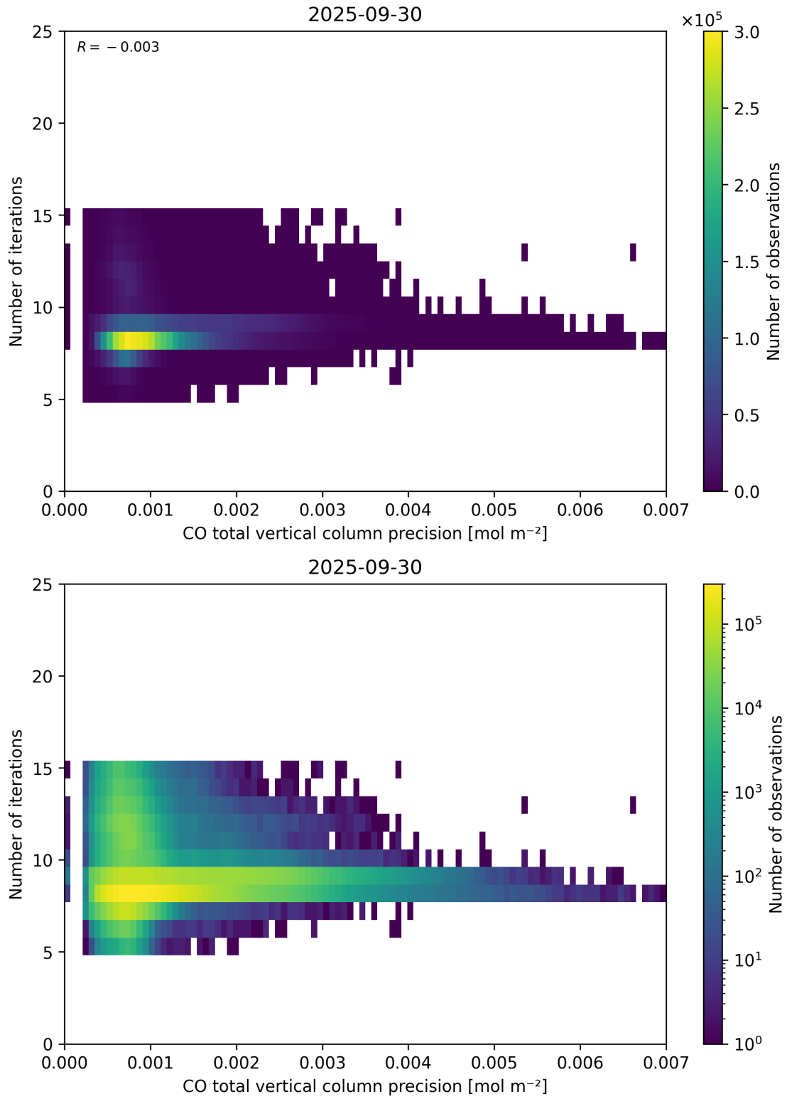
Figure 46: Scatter density plot of “CO total vertical column precision” against “Number of iterations” for 2025-09-29 to 2025-10-01.
