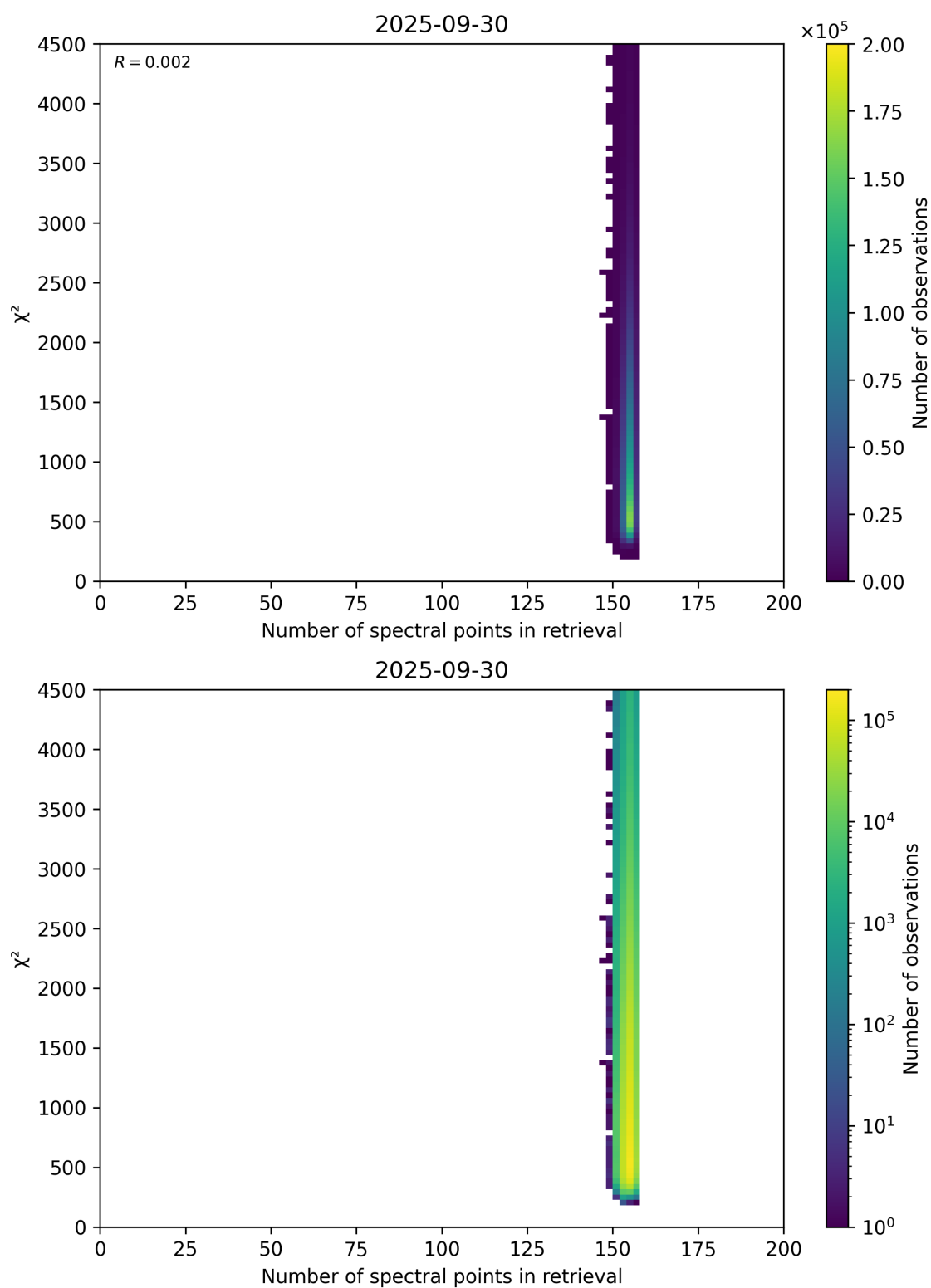
Figure 58: Scatter density plot of “Number of spectral points in retrieval” against “ \chi^2 ” for 2025-09-29 to 2025-10-01.
