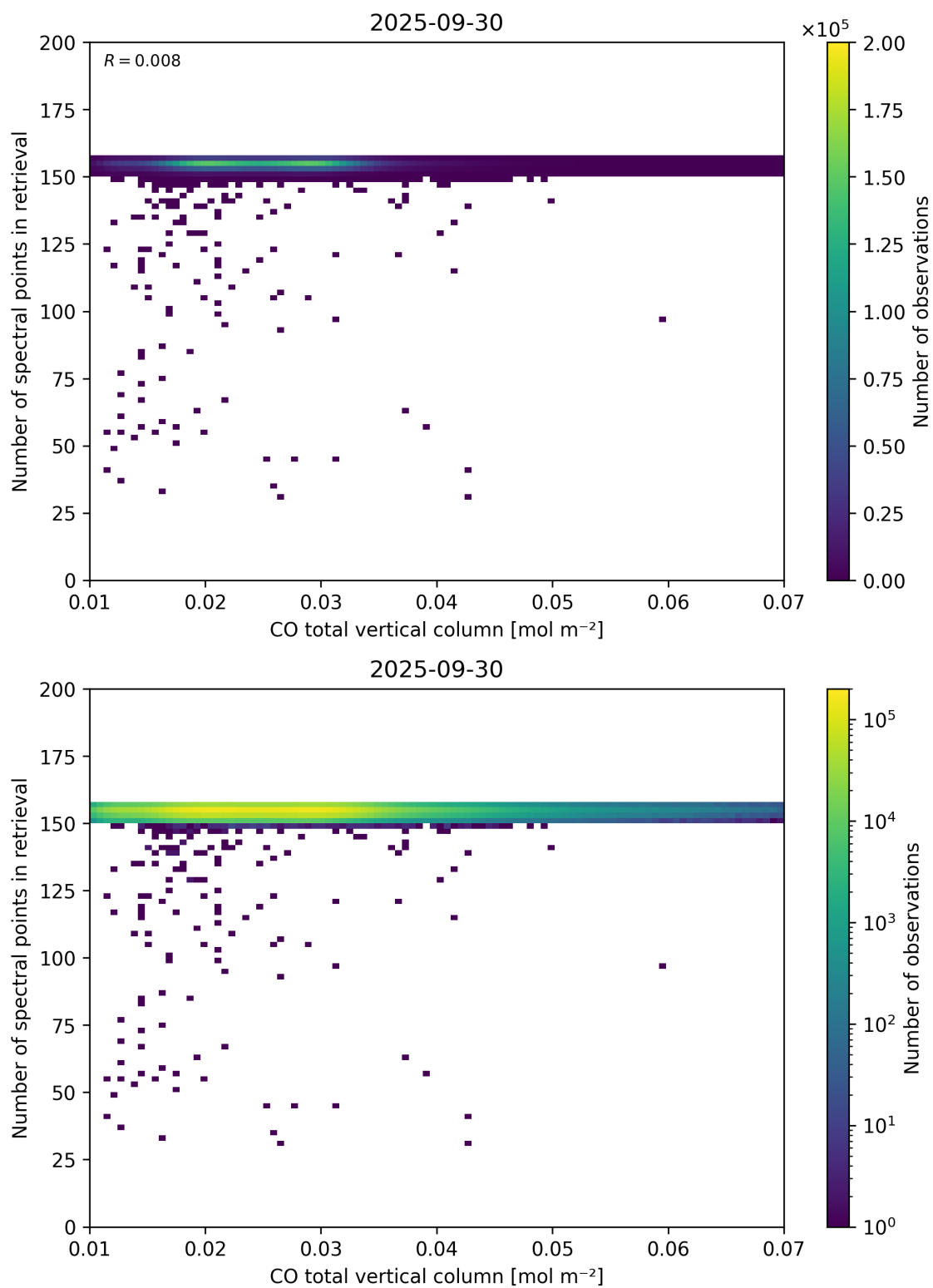
Figure 43: Scatter density plot of “CO total vertical column” against “Number of spectral points in retrieval” for 2025-09-29 to 2025-10-01.
