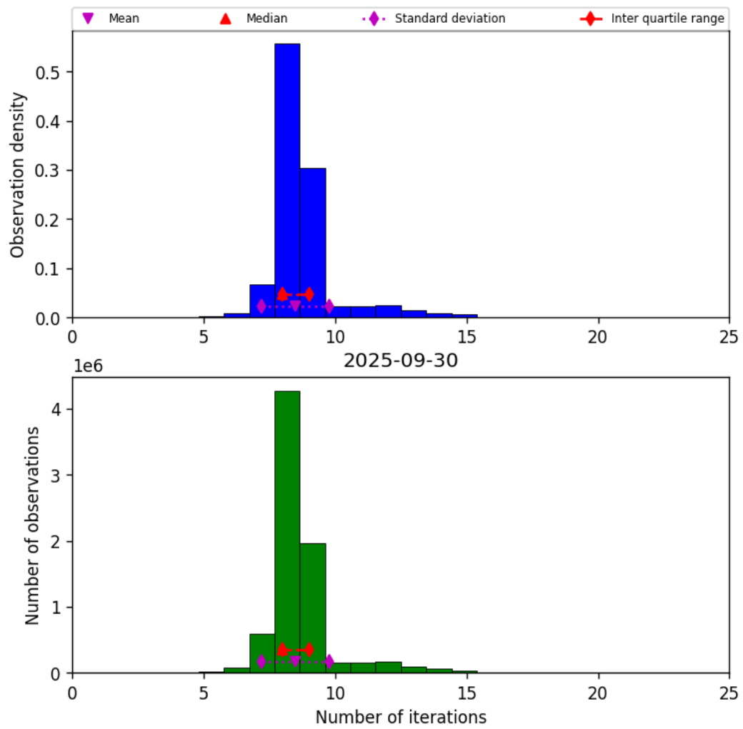
Figure 24: Histogram of “Number of iterations” for 2025-09-29 to 2025-10-01
