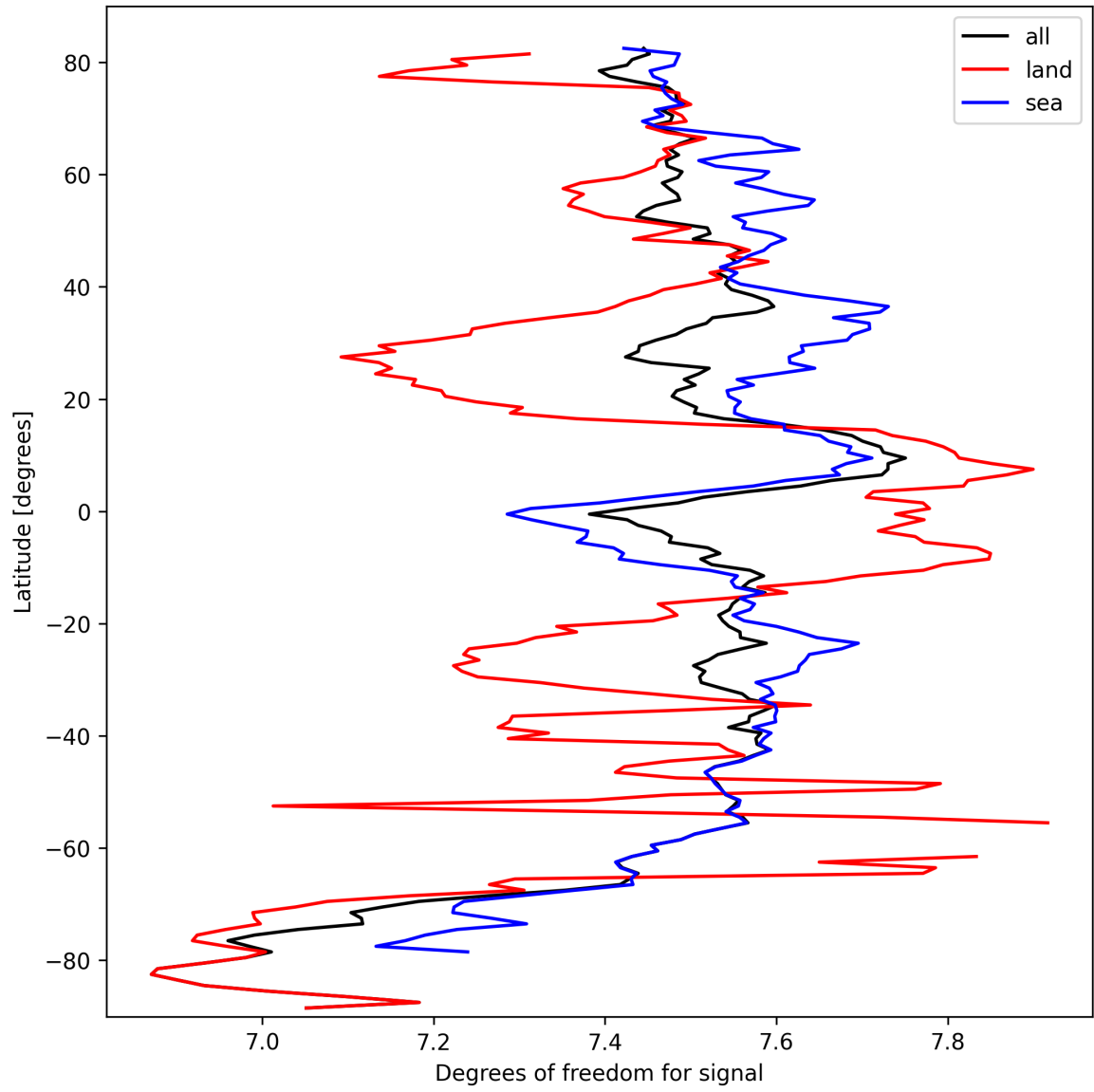
Figure 15: Zonal average of “Degrees of freedom for signal” for 2025-09-29 to 2025-10-01.
