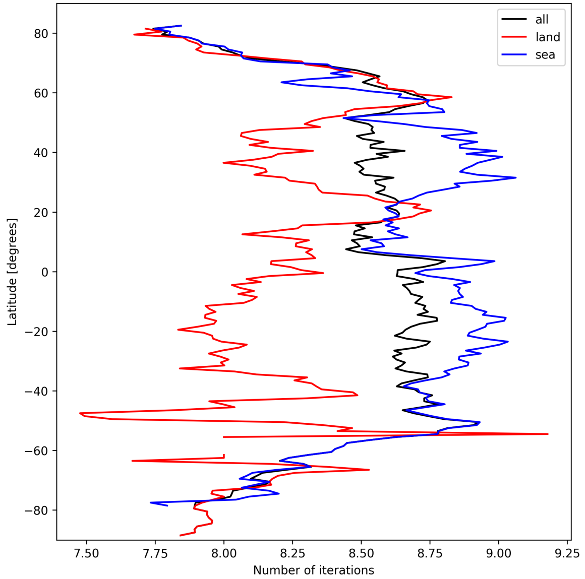
Figure 16: Zonal average of “Number of iterations” for 2025-09-29 to 2025-10-01.
