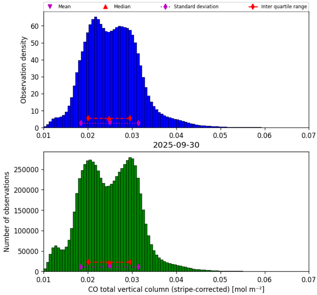
Figure 19: Histogram of “CO total vertical column (stripe-corrected)” for 2025-09-29 to 2025-10-01
