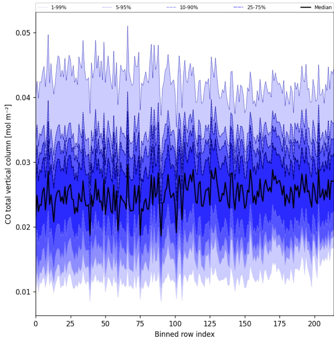
Figure 26: Along track statistics of “CO total vertical column” for 2025-09-29 to 2025-10-01
