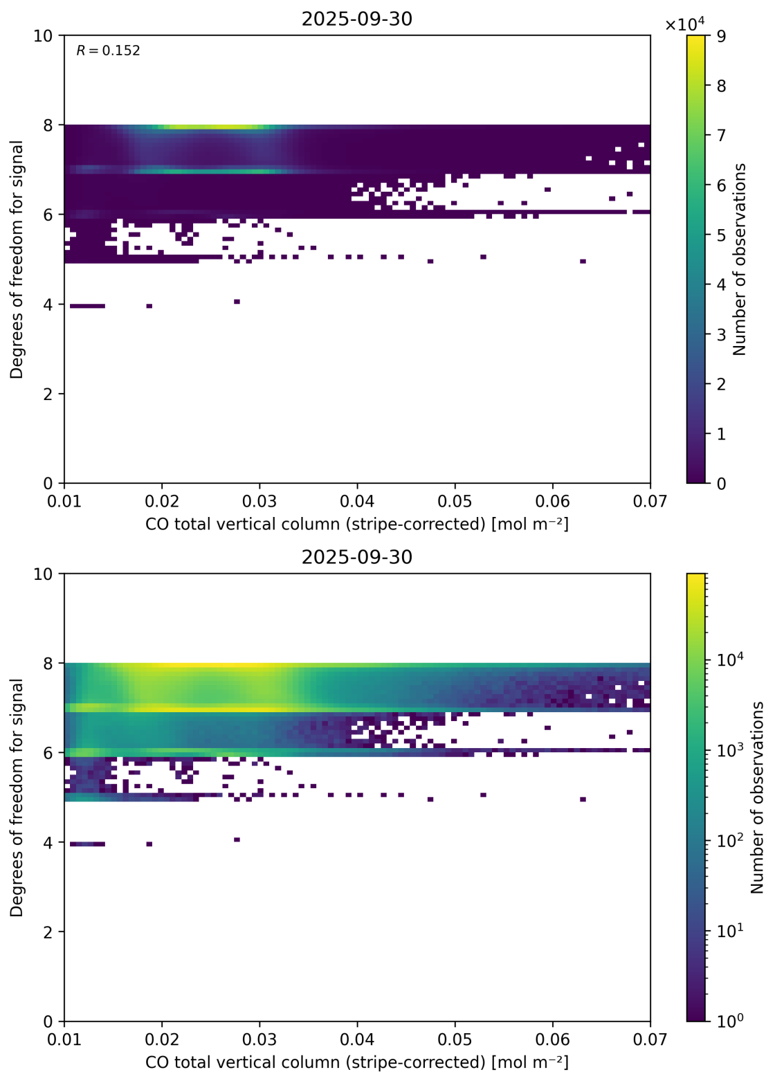
Figure 38: Scatter density plot of “CO total vertical column (stripe-corrected)” against “Degrees of freedom for signal” for 2025-09-29 to 2025-10-01.
