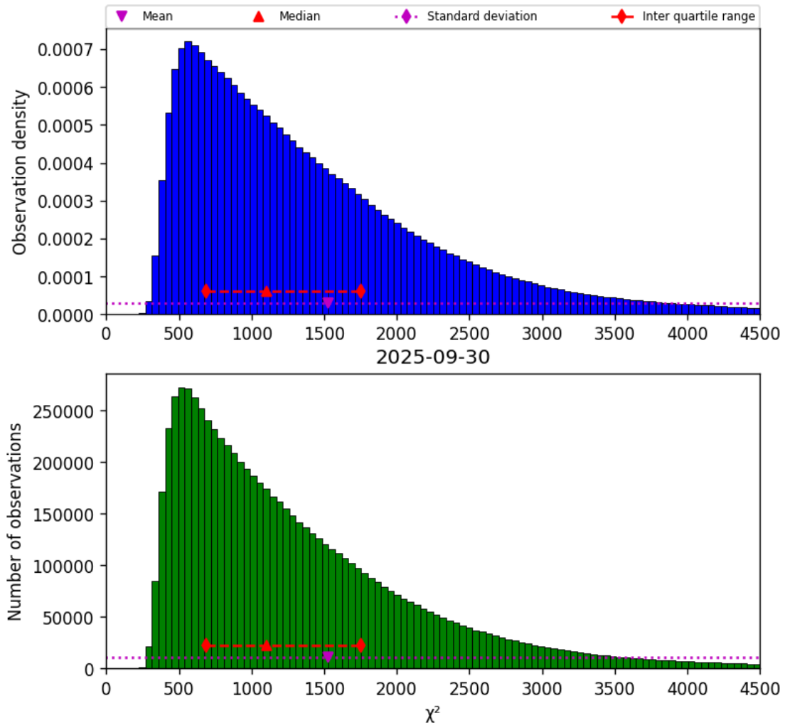
Figure 22: Histogram of “ \chi^2 ” for 2025-09-29 to 2025-10-01
