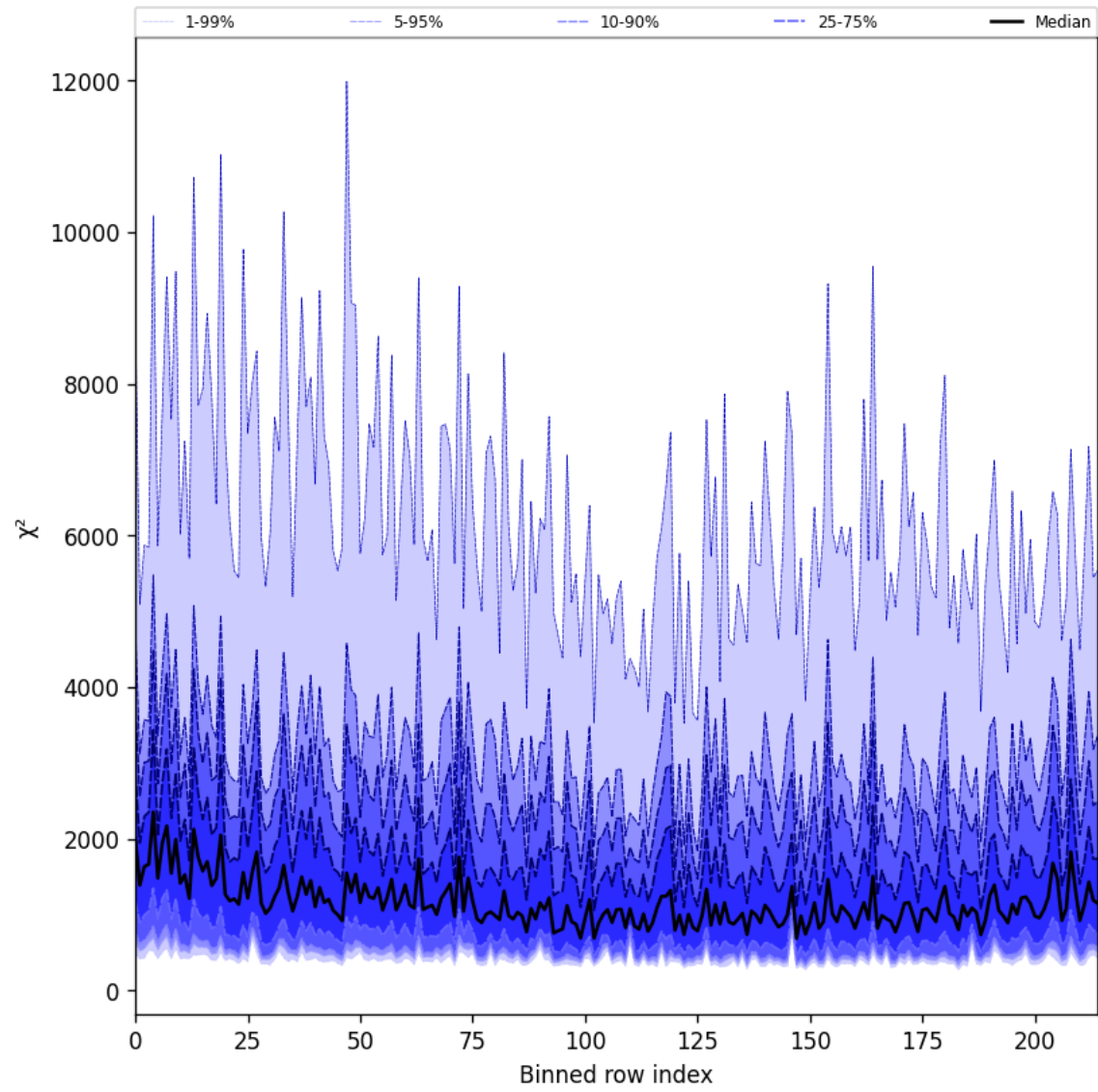
Figure 30: Along track statistics of “ \chi^2 ” for 2025-09-29 to 2025-10-01
