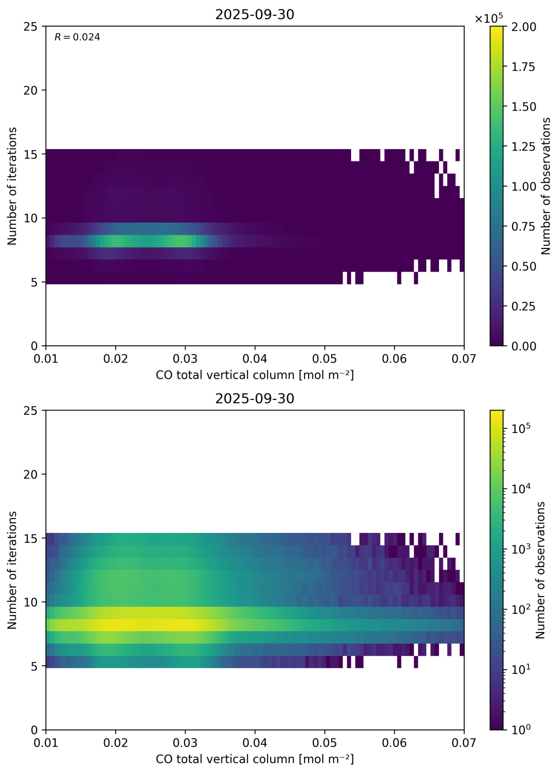
Figure 42: Scatter density plot of “CO total vertical column” against “Number of iterations” for 2025-09-29 to 2025-10-01.
