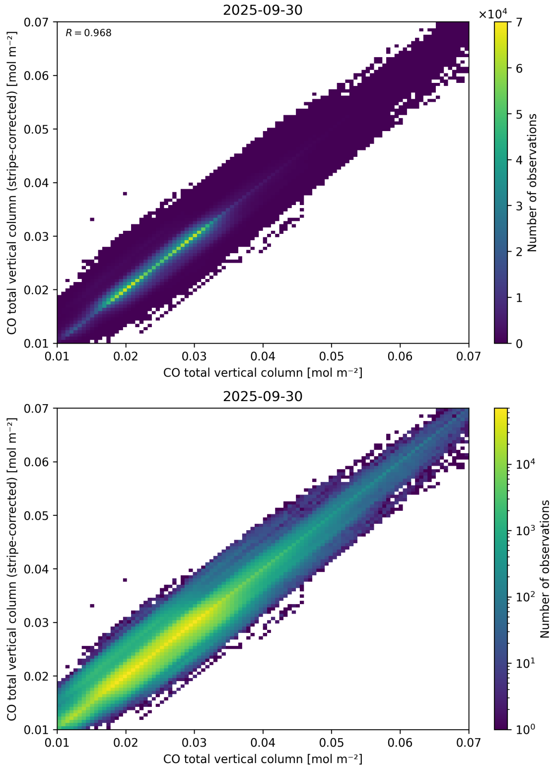
Figure 33: Scatter density plot of “CO total vertical column” against “CO total vertical column (stripe-corrected)” for 2025-09-29 to 2025-10-01.
