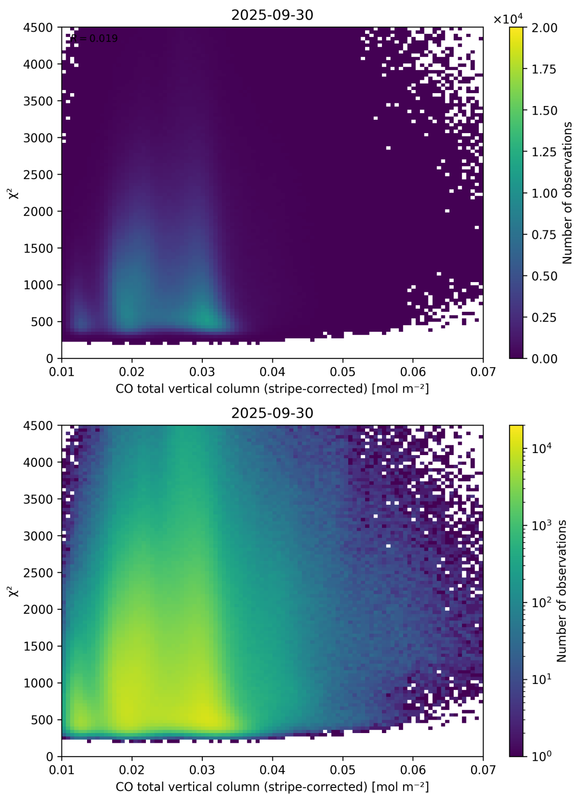
Figure 37: Scatter density plot of “CO total vertical column (stripe-corrected)” against “ \chi^2 ” for 2025-09-29 to 2025-10-01.
