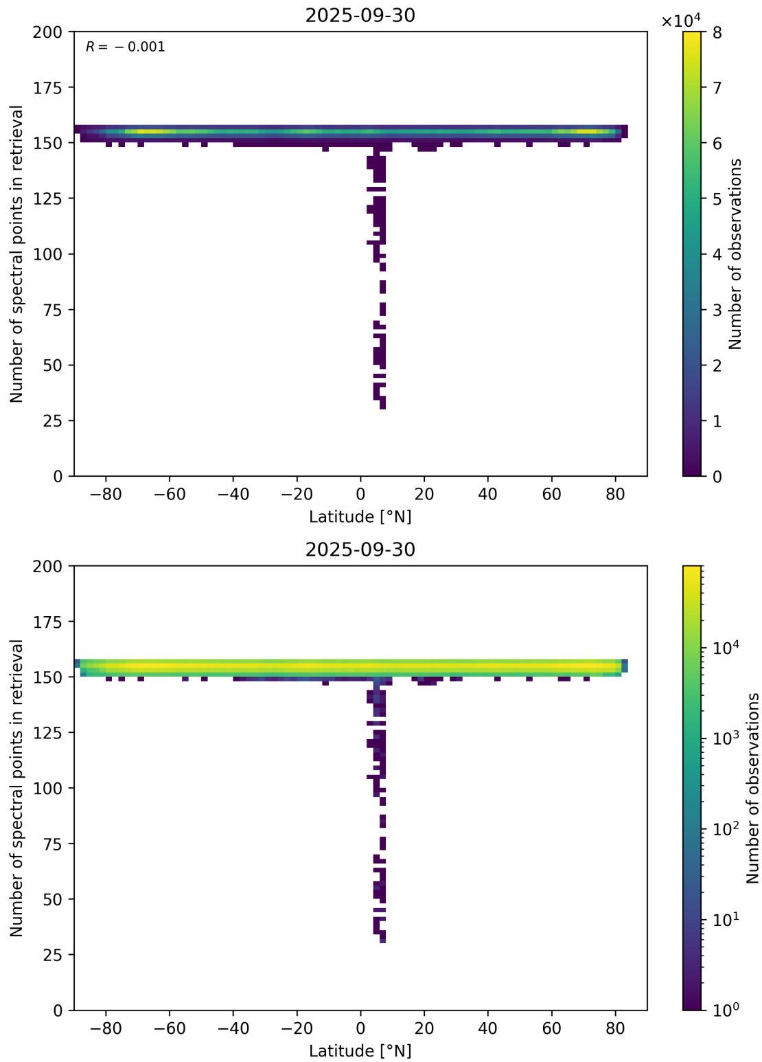
Figure 57: Scatter density plot of “Latitude” against “Number of spectral points in retrieval” for 2025-09-29 to 2025-10-01.
