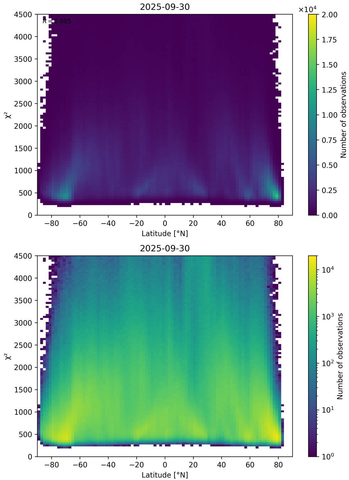
Figure 54: Scatter density plot of “Latitude” against “ \chi^2 ” for 2025-09-29 to 2025-10-01.
