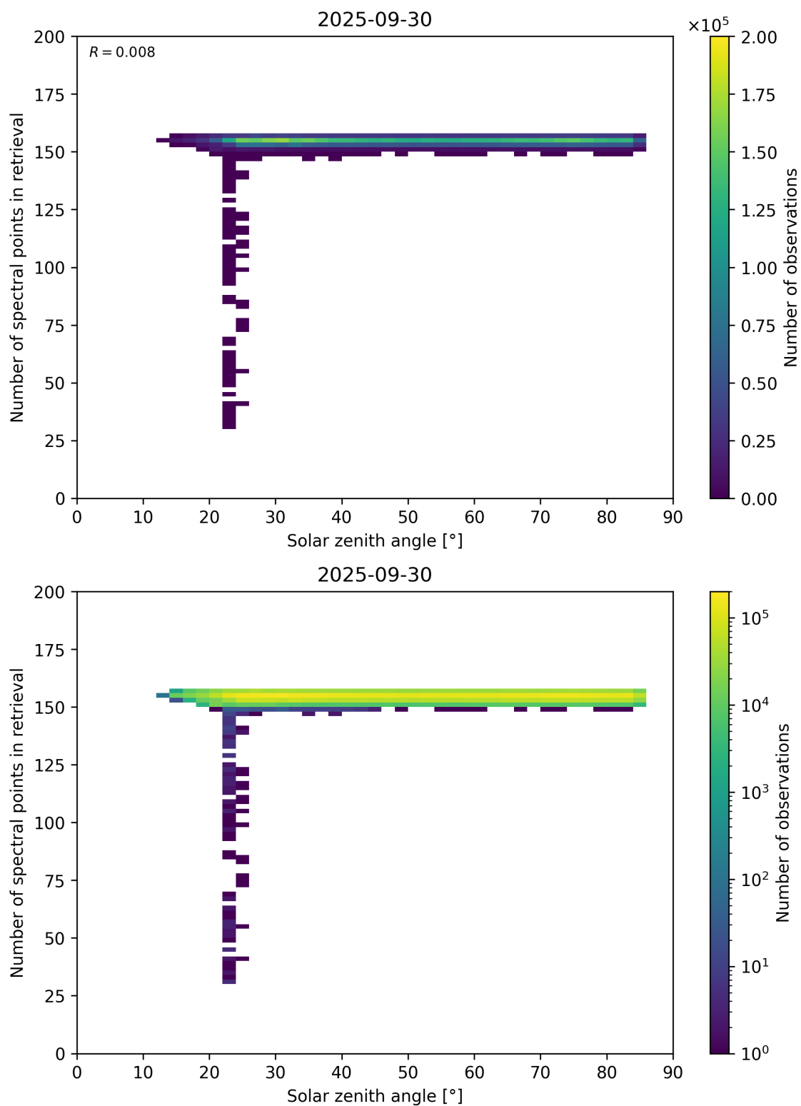
Figure 68: Scatter density plot of “Solar zenith angle” against “Number of spectral points in retrieval” for 2025-09-29 to 2025-10-01.
