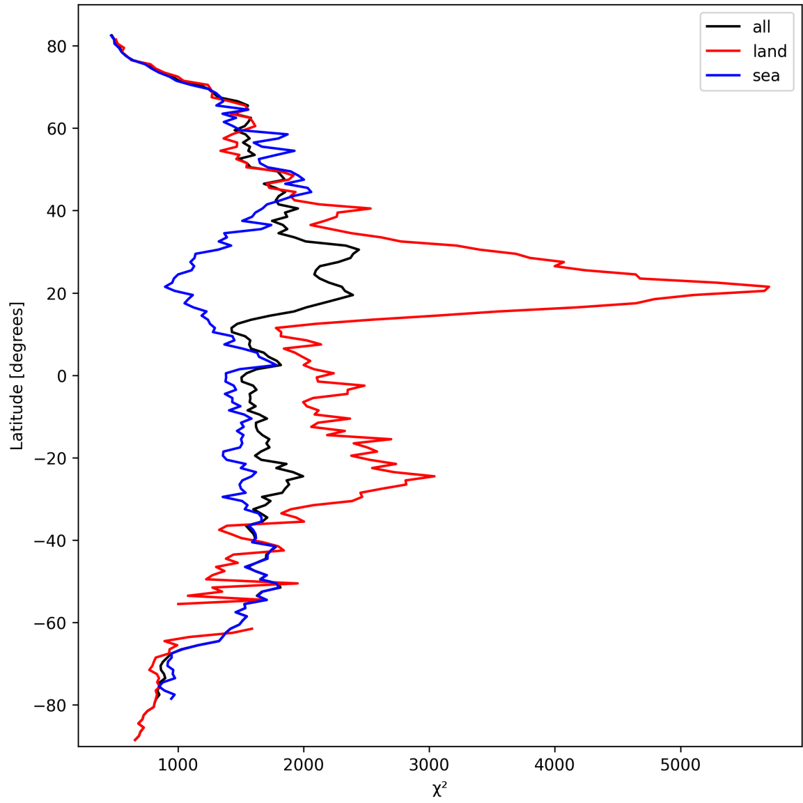
Figure 14: Zonal average of “ \chi^2 ” for 2025-09-29 to 2025-10-01.
