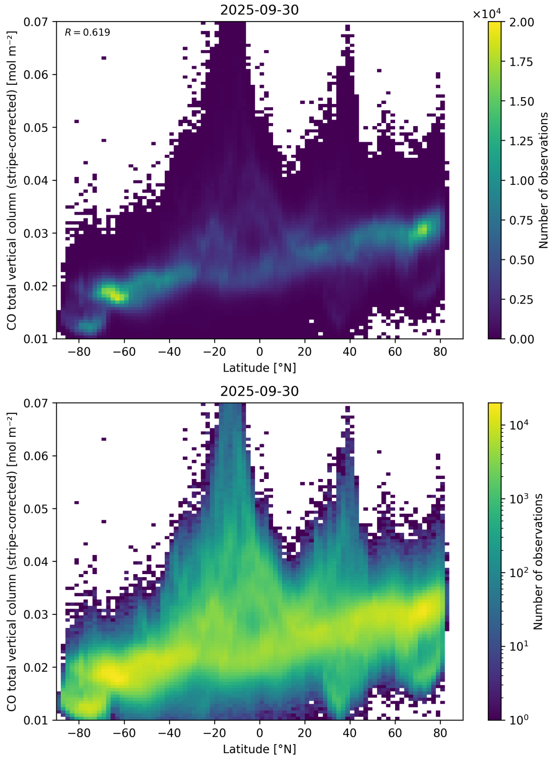
Figure 52: Scatter density plot of “Latitude” against “CO total vertical column (stripe-corrected)” for 2025-09-29 to 2025-10-01.
