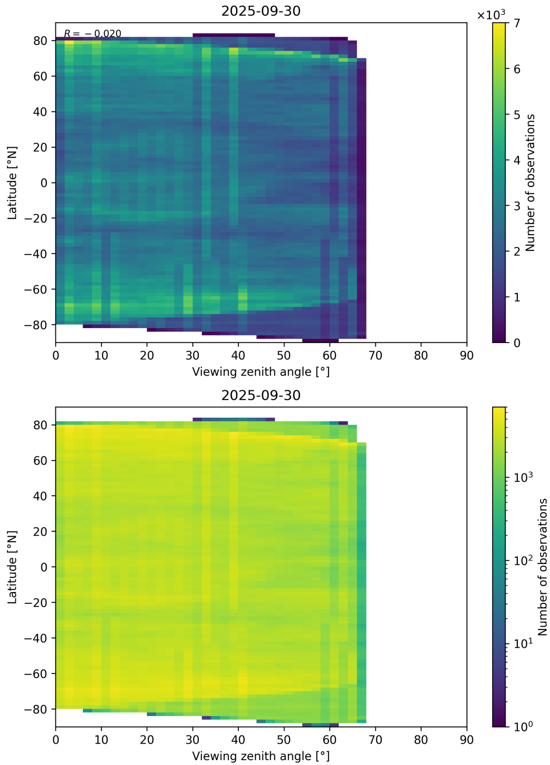
Figure 74: Scatter density plot of “Viewing zenith angle” against “Latitude” for 2025-09-29 to 2025-10-01.
