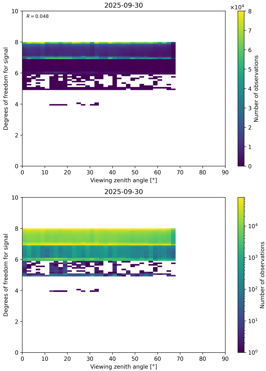
Figure 73: Scatter density plot of “Viewing zenith angle” against “Degrees of freedom for signal” for 2025-09-29 to 2025-10-01.
