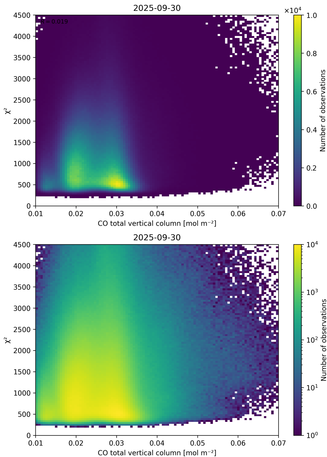
Figure 35: Scatter density plot of “CO total vertical column” against “ \chi^2 ” for 2025-09-29 to 2025-10-01.
