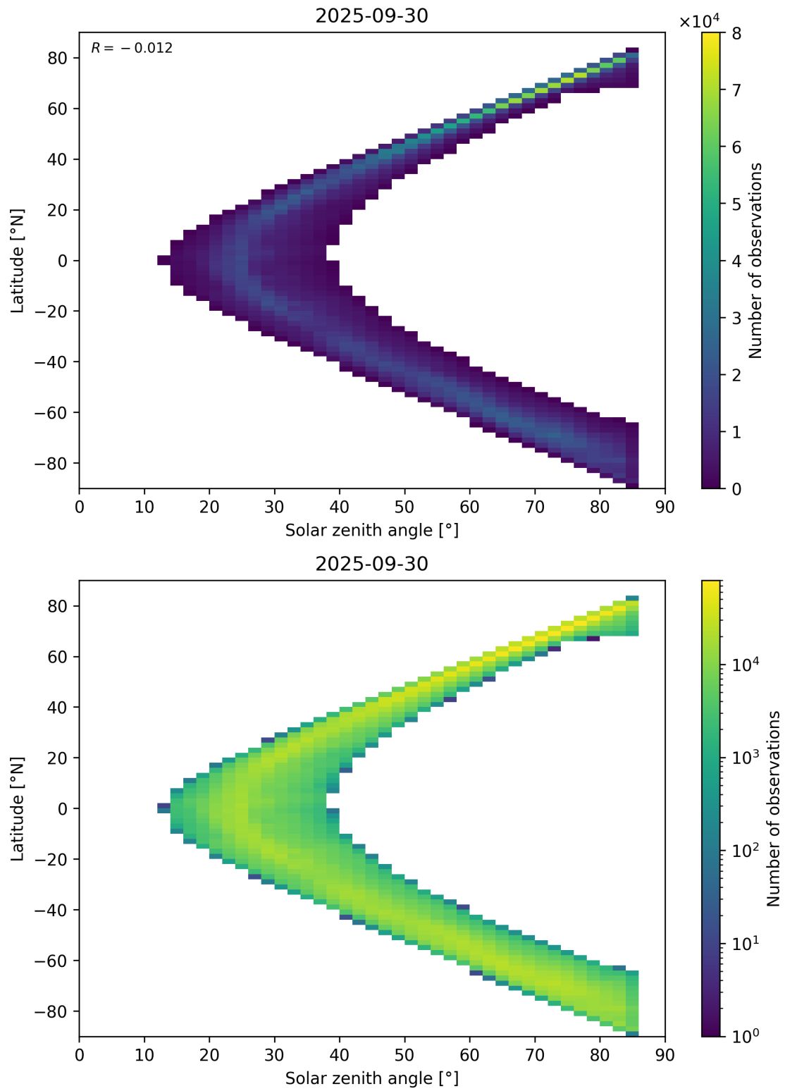
Figure 66: Scatter density plot of “Solar zenith angle” against “Latitude” for 2025-09-29 to 2025-10-01.
