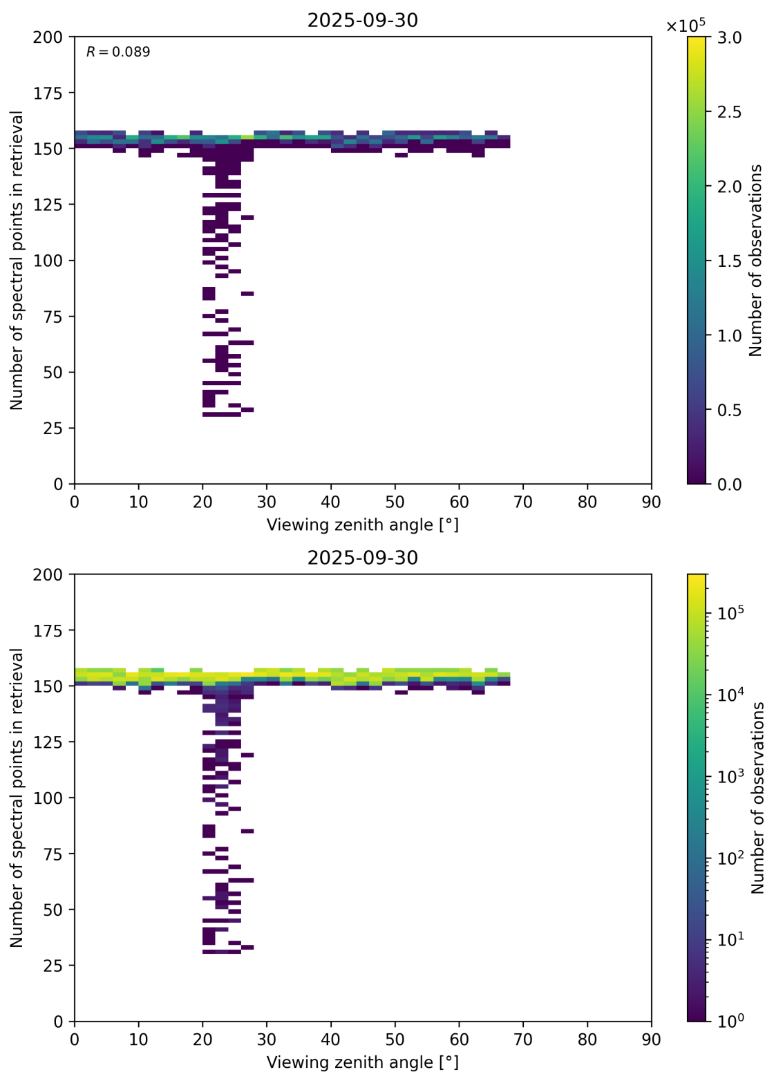
Figure 76: Scatter density plot of “Viewing zenith angle” against “Number of spectral points in retrieval” for 2025-09-29 to 2025-10-01.
