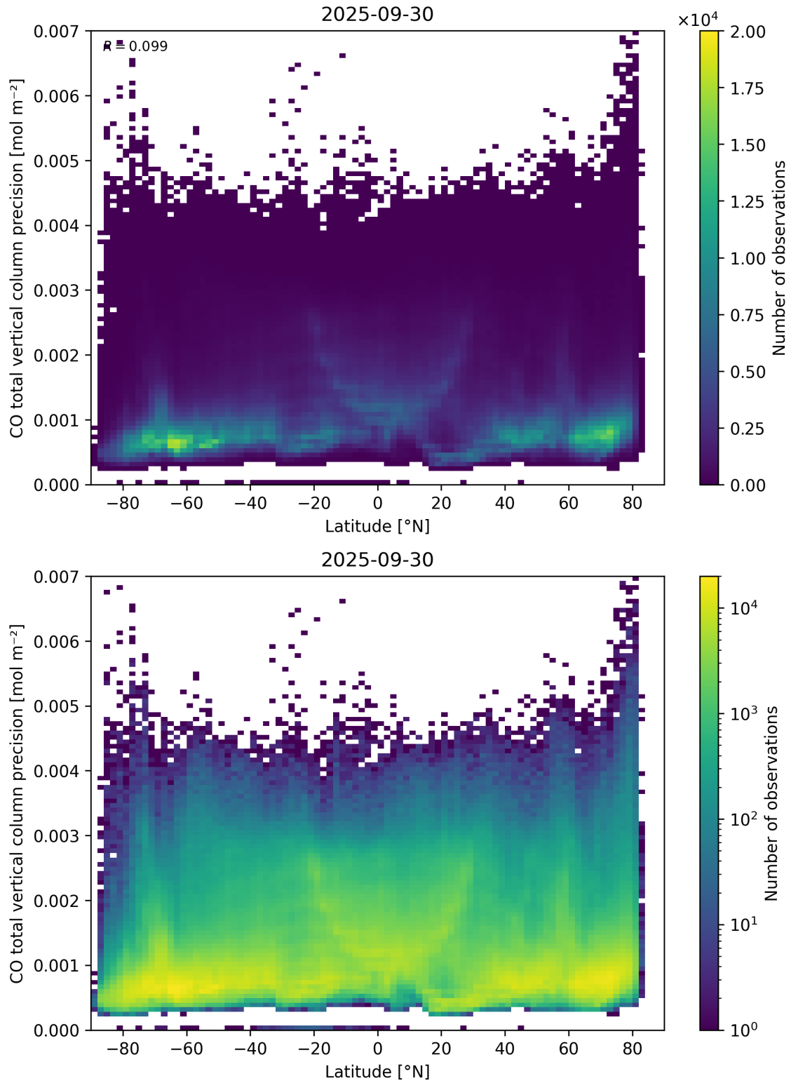
Figure 53: Scatter density plot of “Latitude” against “CO total vertical column precision” for 2025-09-29 to 2025-10-01.
