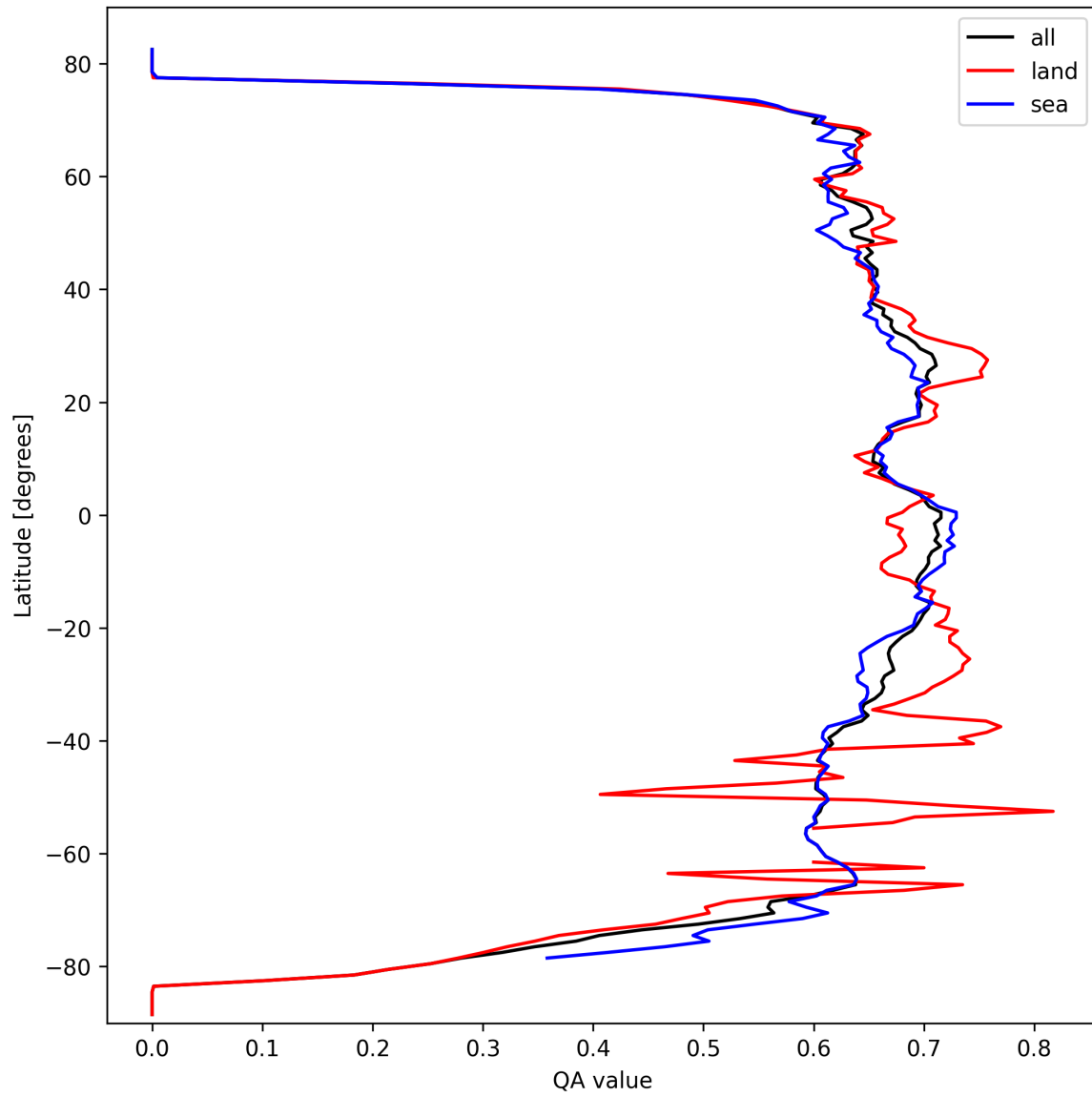
Figure 9: Zonal average of “QA value” for 2025-09-29 to 2025-10-01.
