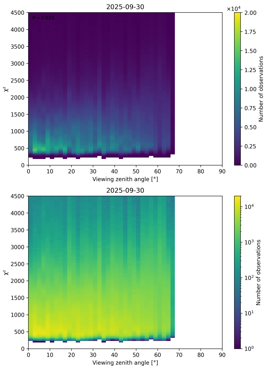
Figure 72: Scatter density plot of “Viewing zenith angle” against “ \chi^2 ” for 2025-09-29 to 2025-10-01.
