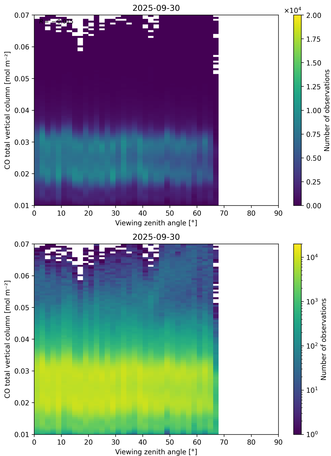
Figure 69: Scatter density plot of “Viewing zenith angle” against “CO total vertical column” for 2025-09-29 to 2025-10-01.
