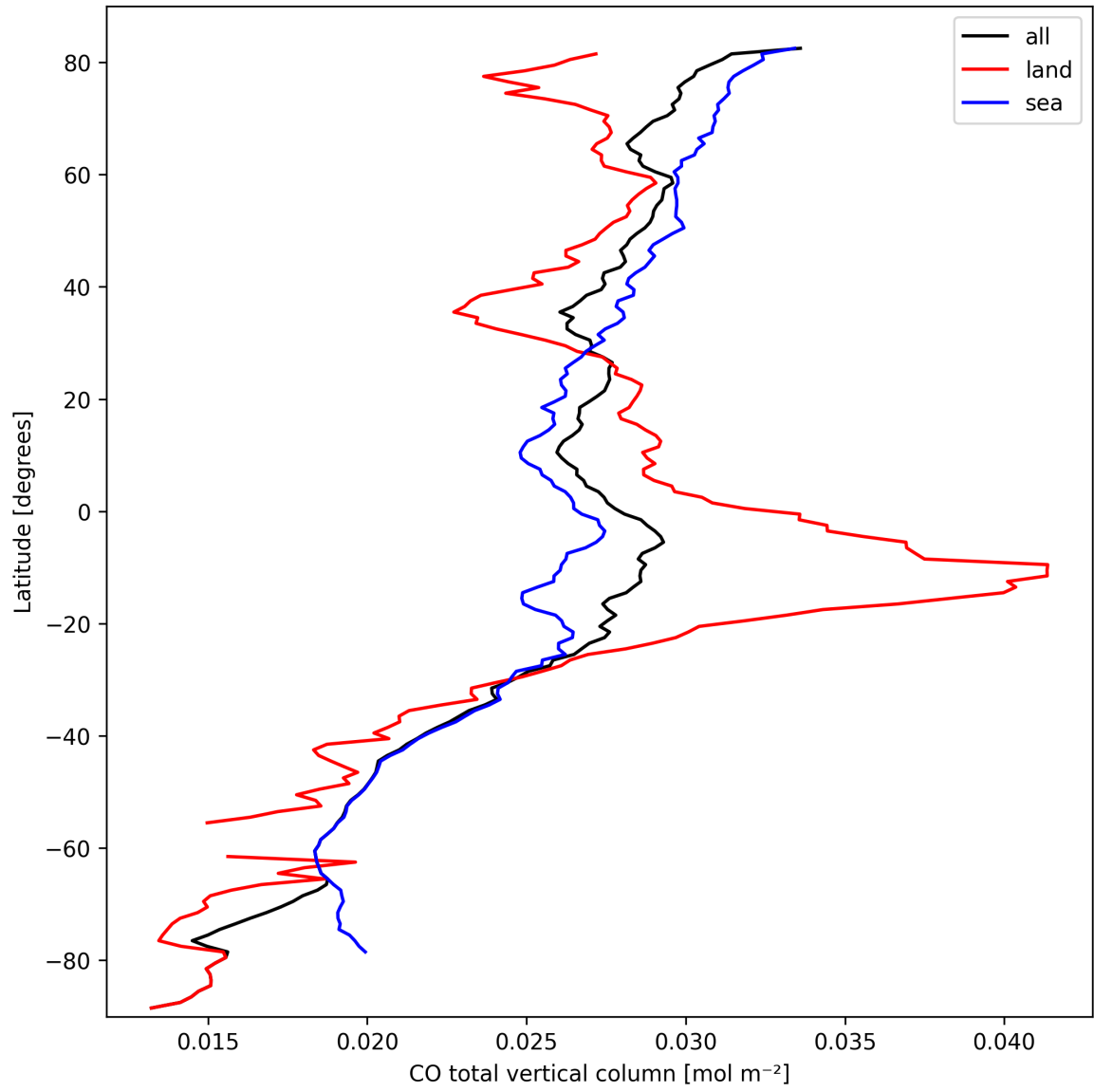
Figure 10: Zonal average of “CO total vertical column” for 2025-09-29 to 2025-10-01.
