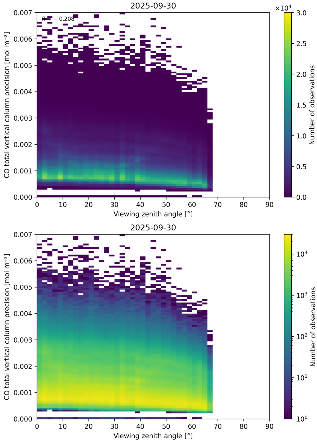
Figure 71: Scatter density plot of “Viewing zenith angle” against “CO total vertical column precision” for 2025-09-29 to 2025-10-01.
