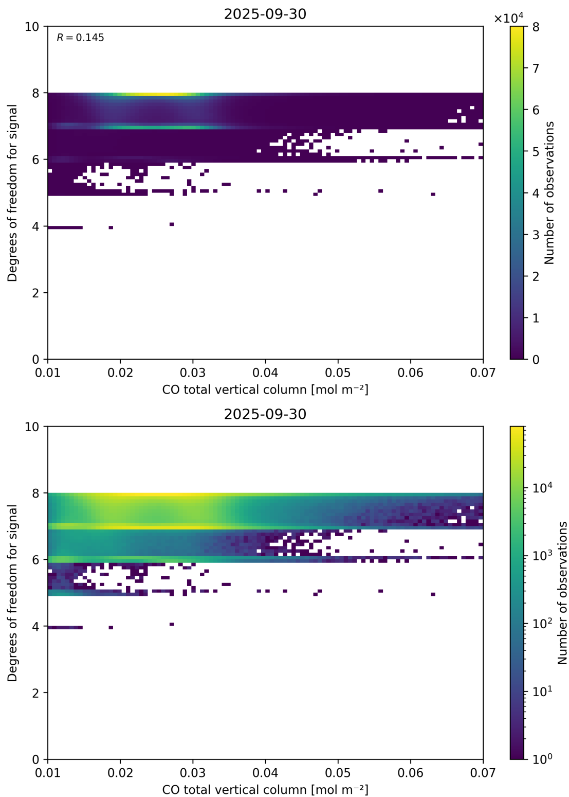
Figure 41: Scatter density plot of “CO total vertical column” against “Degrees of freedom for signal” for 2025-09-29 to 2025-10-01.
