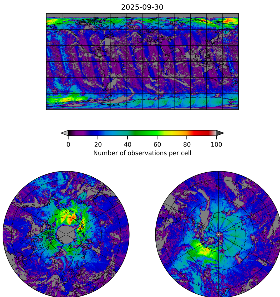
Figure 8: Map of the number of observations for 2025-09-29 to 2025-10-01
