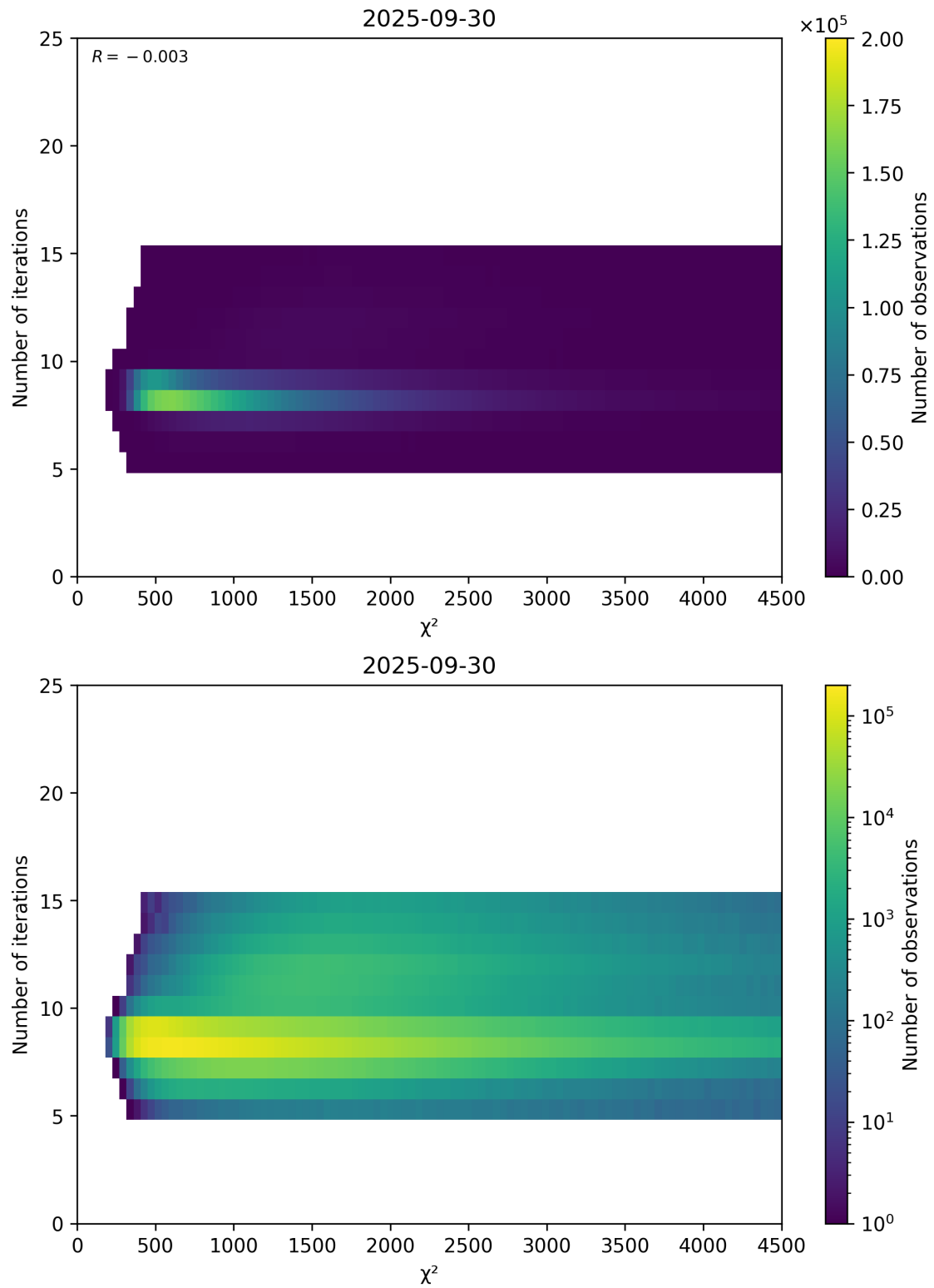
Figure 49: Scatter density plot of “ \chi^2 ” against “Number of iterations” for 2025-09-29 to 2025-10-01.
