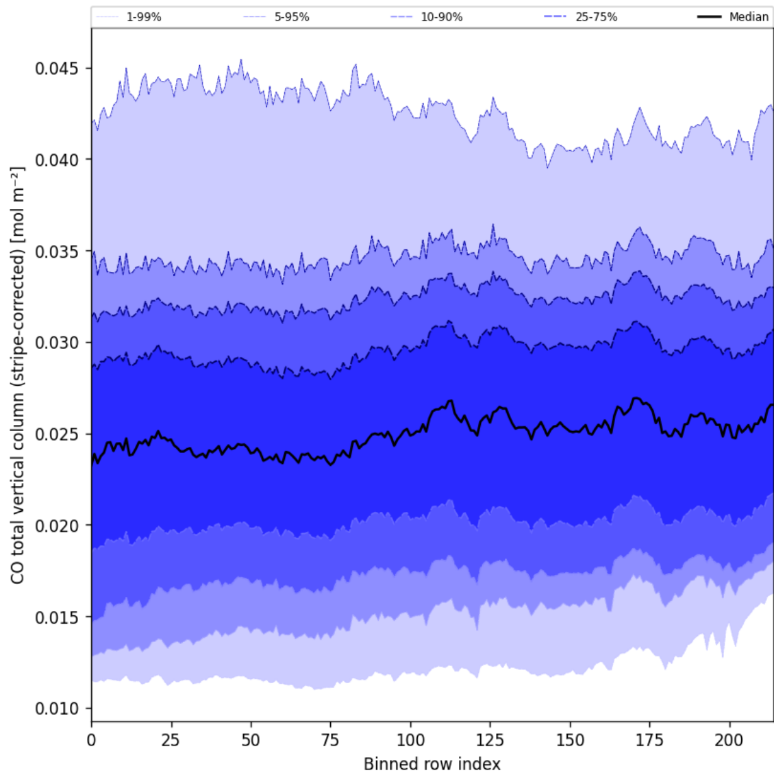
Figure 27: Along track statistics of “CO total vertical column (stripe-corrected)” for 2025-09-29 to 2025-10-01
