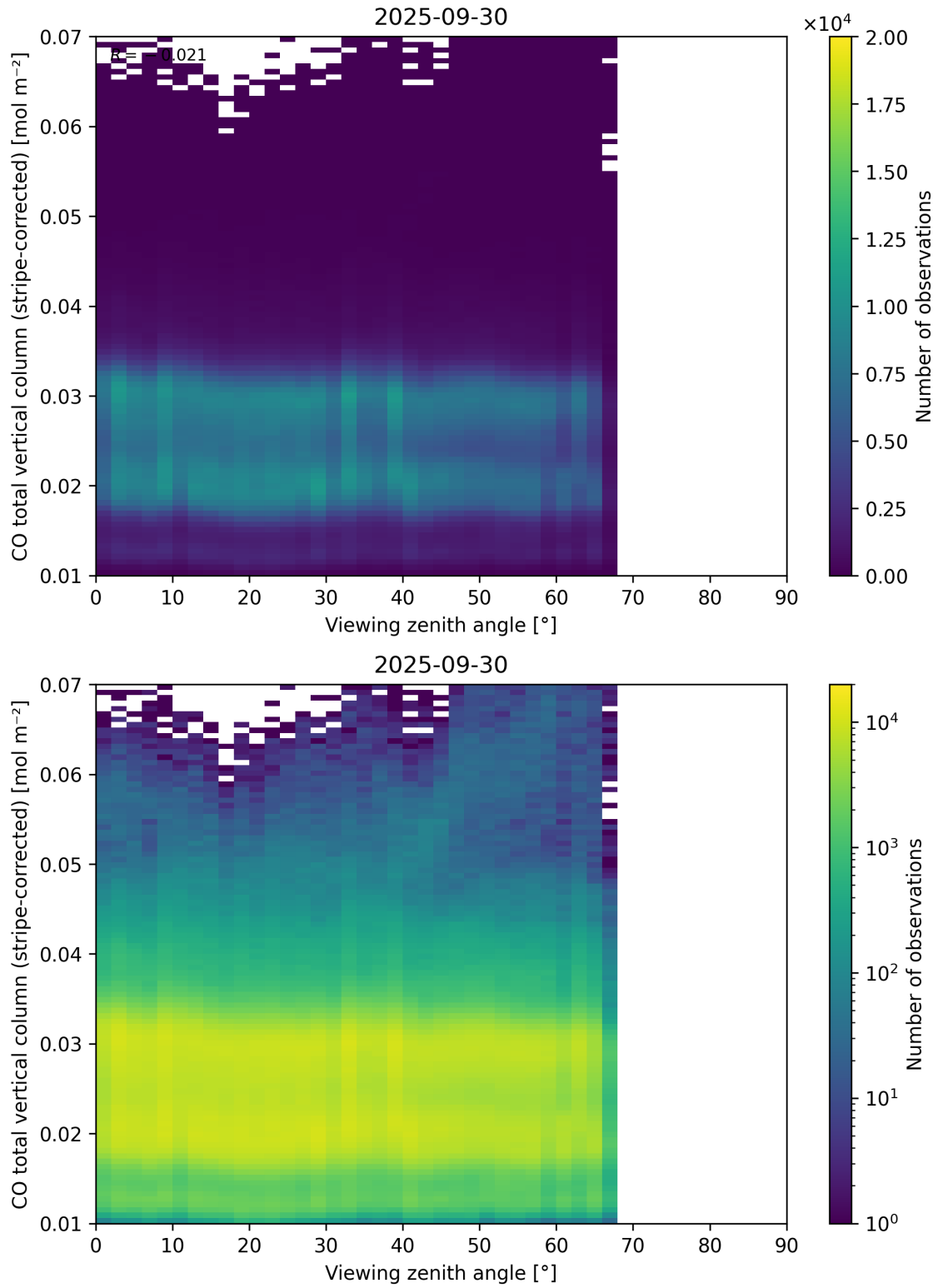
Figure 70: Scatter density plot of “Viewing zenith angle” against “CO total vertical column (stripe-corrected)” for 2025-09-29 to 2025-10-01.
