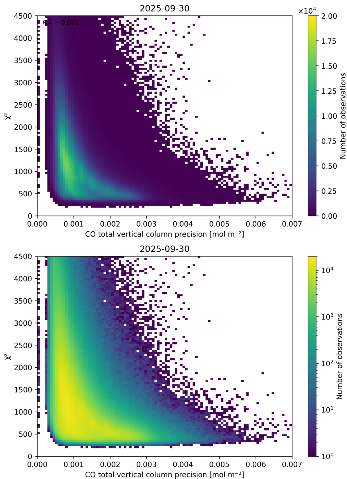
Figure 44: Scatter density plot of “CO total vertical column precision” against “ \chi^2 ” for 2025-09-29 to 2025-10-01.
