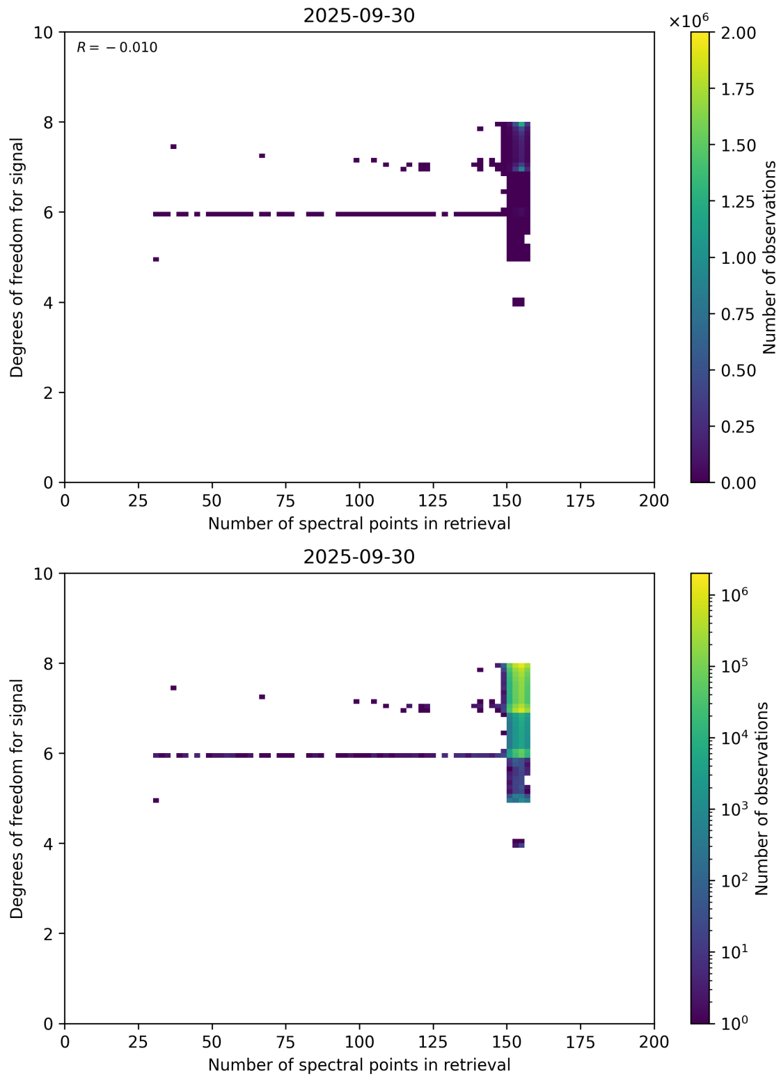
Figure 59: Scatter density plot of “Number of spectral points in retrieval” against “Degrees of freedom for signal” for 2025-09-29 to 2025-10-01.
