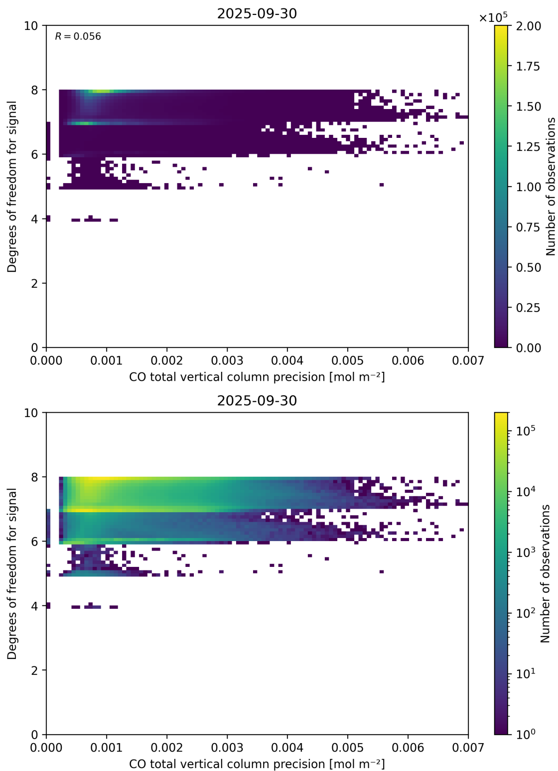
Figure 45: Scatter density plot of “CO total vertical column precision” against “Degrees of freedom for signal” for 2025-09-29 to 2025-10-01.
