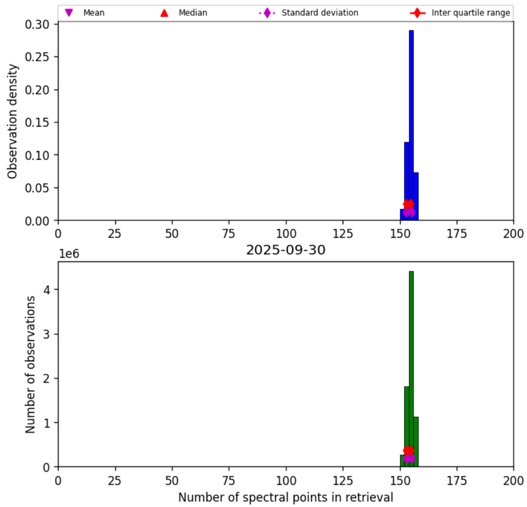
Figure 21: Histogram of “Number of spectral points in retrieval” for 2025-09-29 to 2025-10-01
