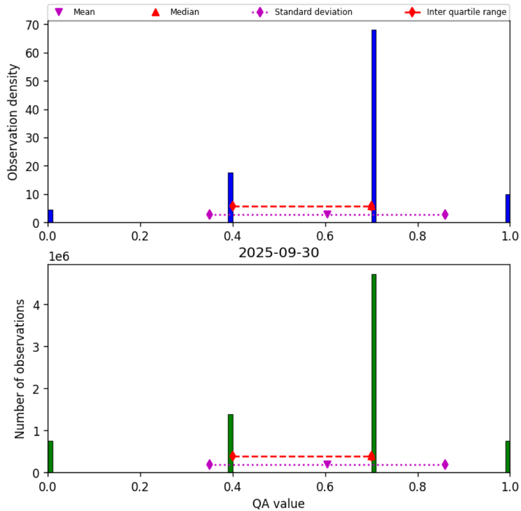
Figure 17: Histogram of “QA value” for 2025-09-29 to 2025-10-01
