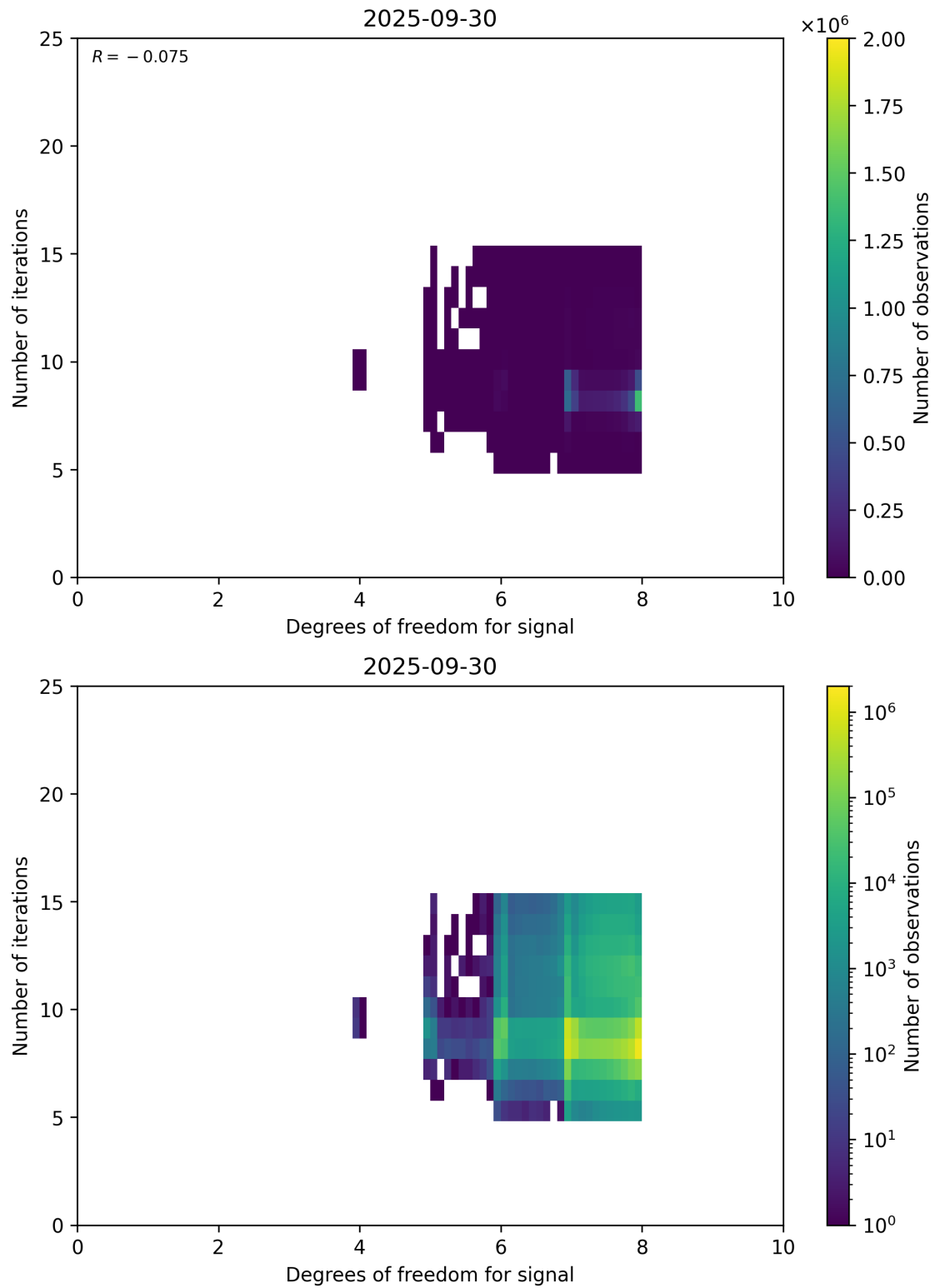
Figure 50: Scatter density plot of “Degrees of freedom for signal” against “Number of iterations” for 2025-09-29 to 2025-10-01.
