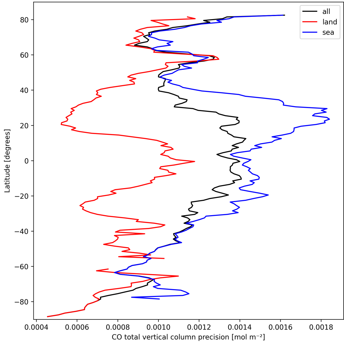
Figure 12: Zonal average of “CO total vertical column precision” for 2025-09-29 to 2025-10-01.
