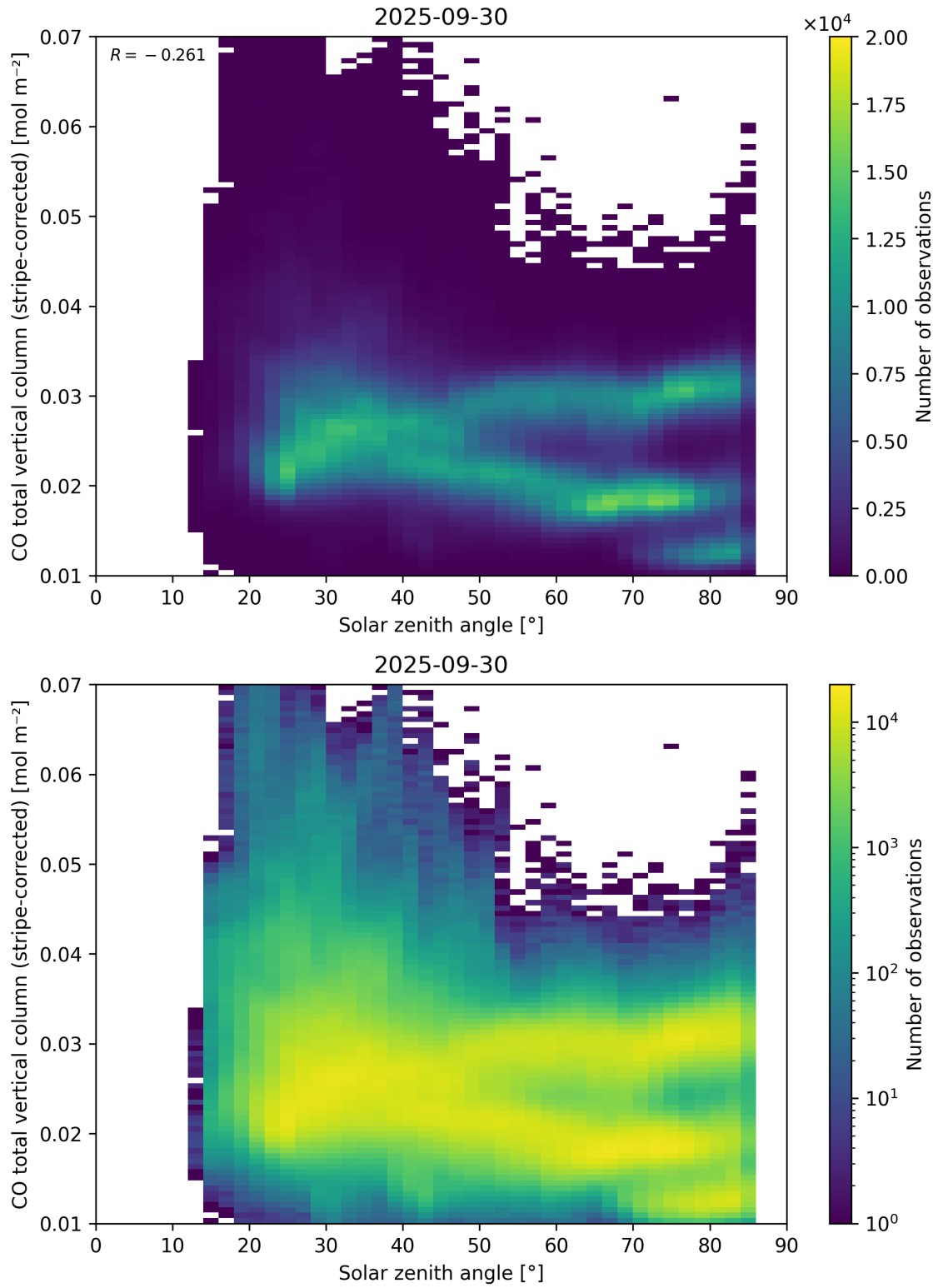
Figure 62: Scatter density plot of “Solar zenith angle” against “CO total vertical column (stripe-corrected)” for 2025-09-29 to 2025-10-01.
