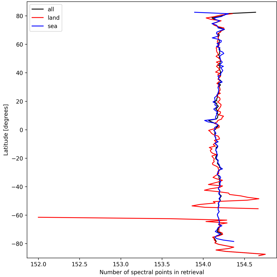
Figure 13: Zonal average of “Number of spectral points in retrieval” for 2025-09-29 to 2025-10-01.
