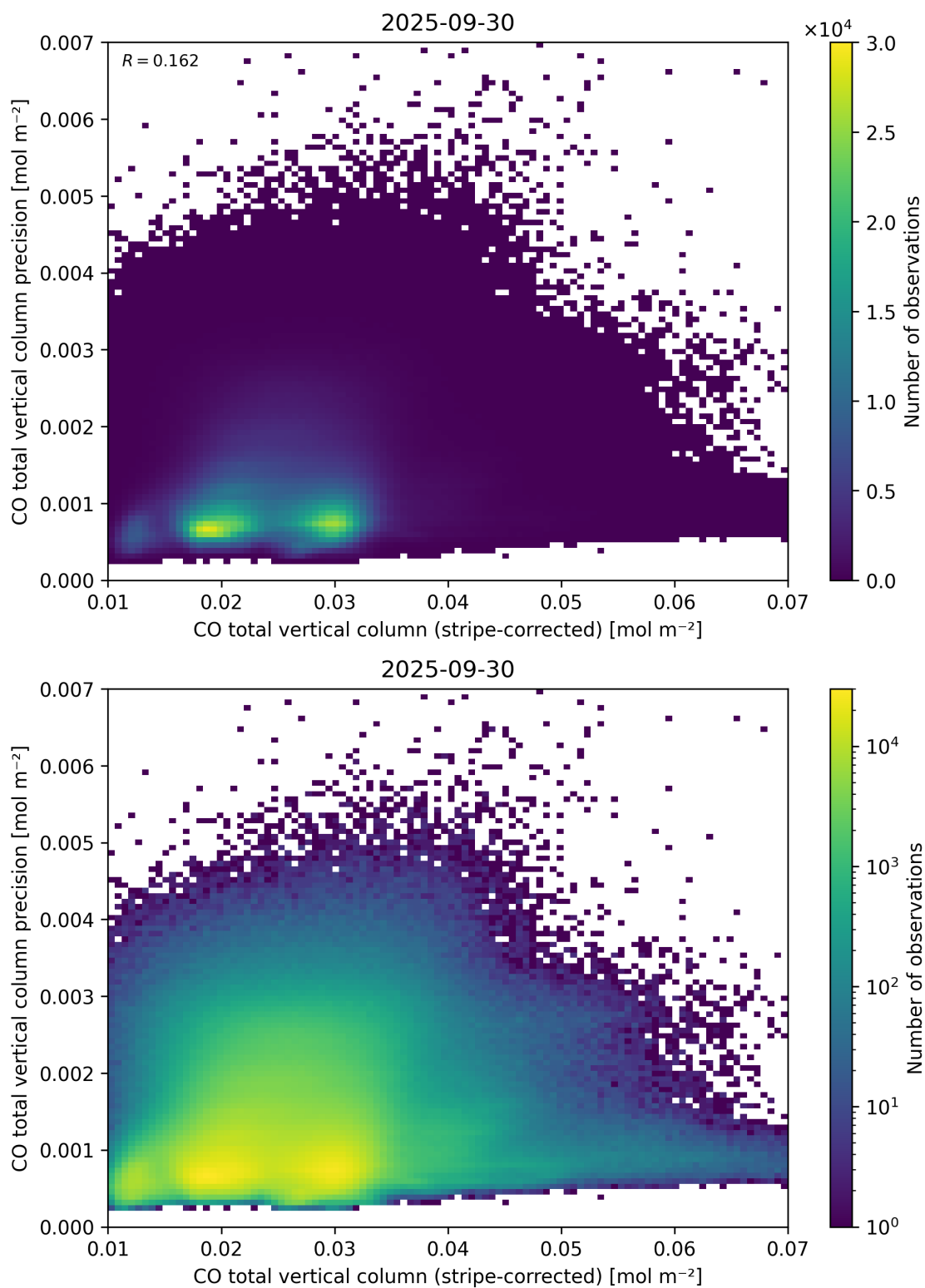
Figure 36: Scatter density plot of “CO total vertical column (stripe-corrected)” against “CO total vertical column precision” for 2025-09-29 to 2025-10-01.
