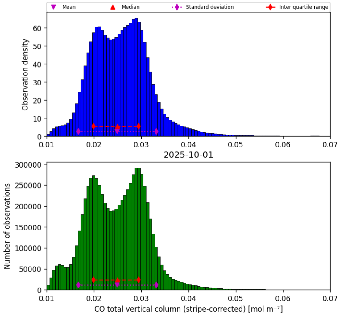
Figure 19: Histogram of “CO total vertical column (stripe-corrected)” for 2025-10-01 to 2025-10-02
