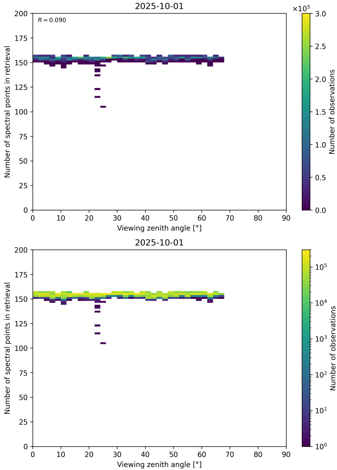
Figure 76: Scatter density plot of “Viewing zenith angle” against “Number of spectral points in retrieval” for 2025-10-01 to 2025-10-02.
