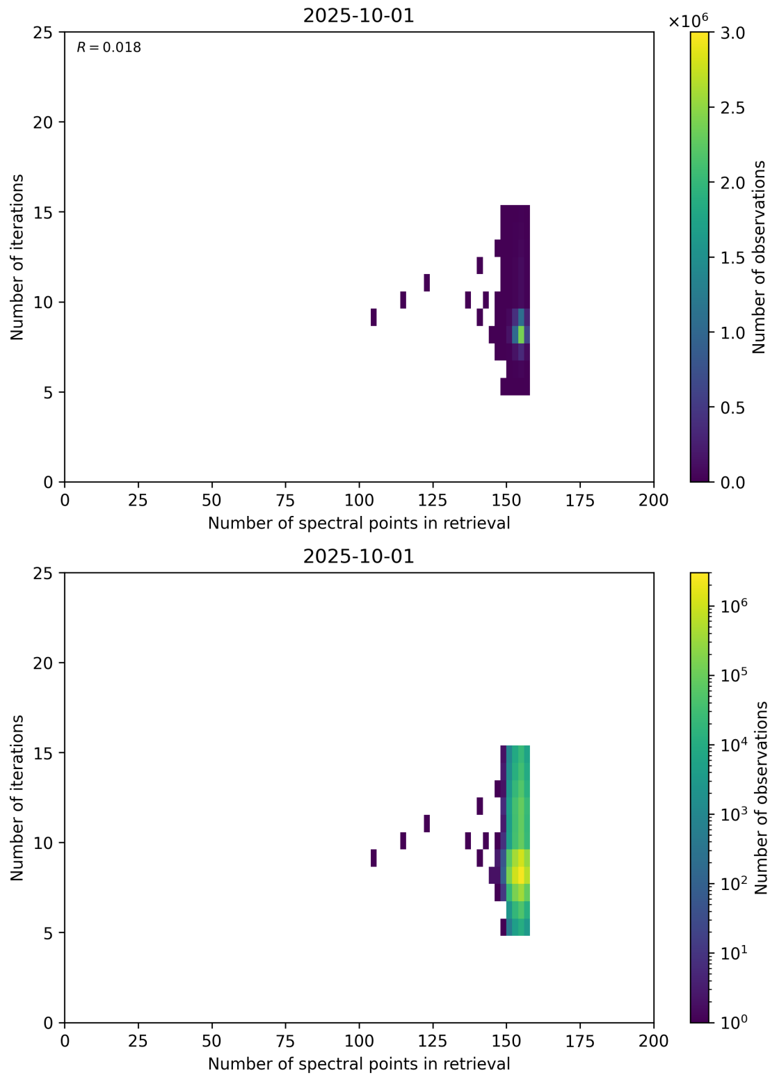
Figure 60: Scatter density plot of “Number of spectral points in retrieval” against “Number of iterations” for 2025-10-01 to 2025-10-02.
