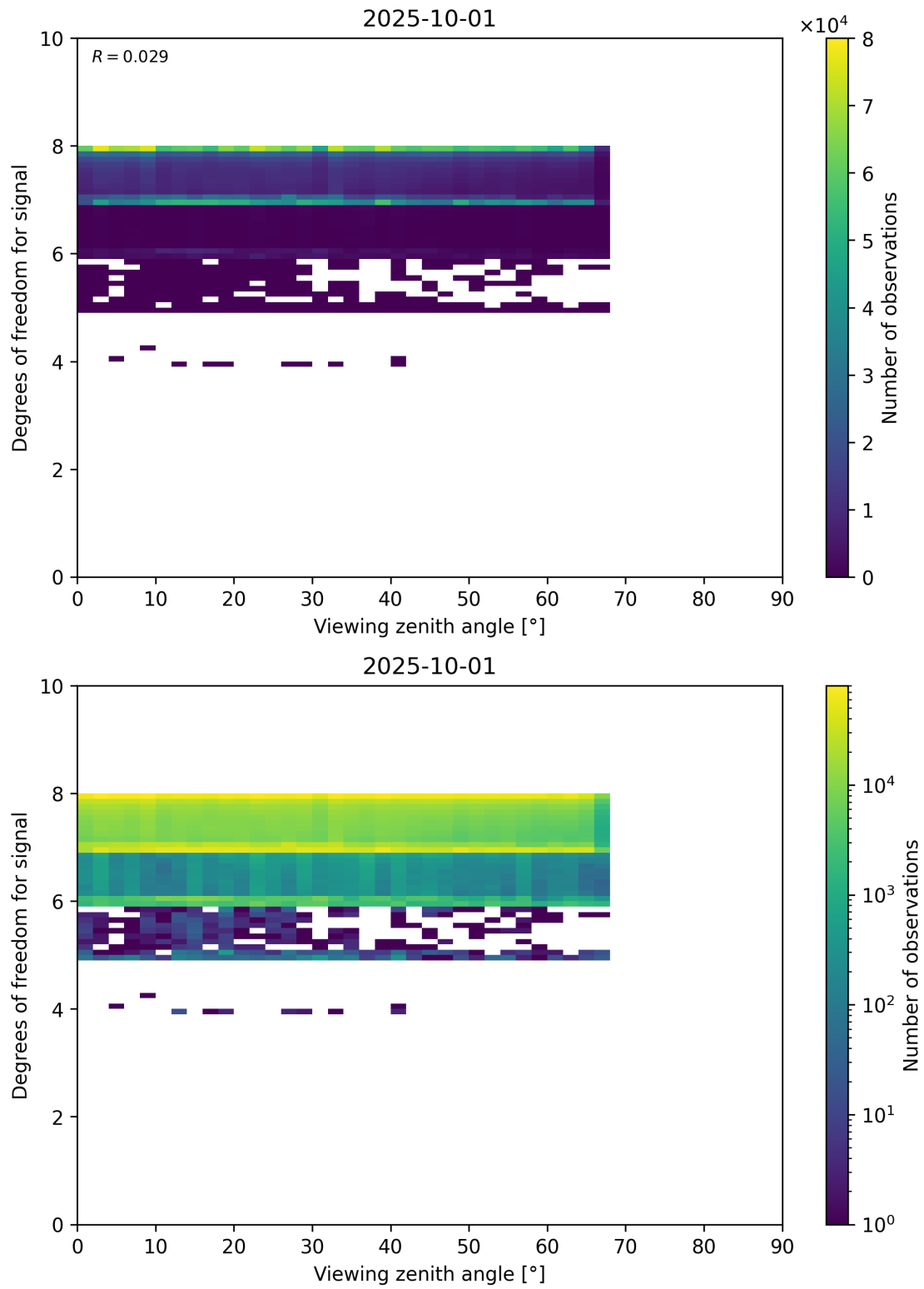
Figure 73: Scatter density plot of “Viewing zenith angle” against “Degrees of freedom for signal” for 2025-10-01 to 2025-10-02.
