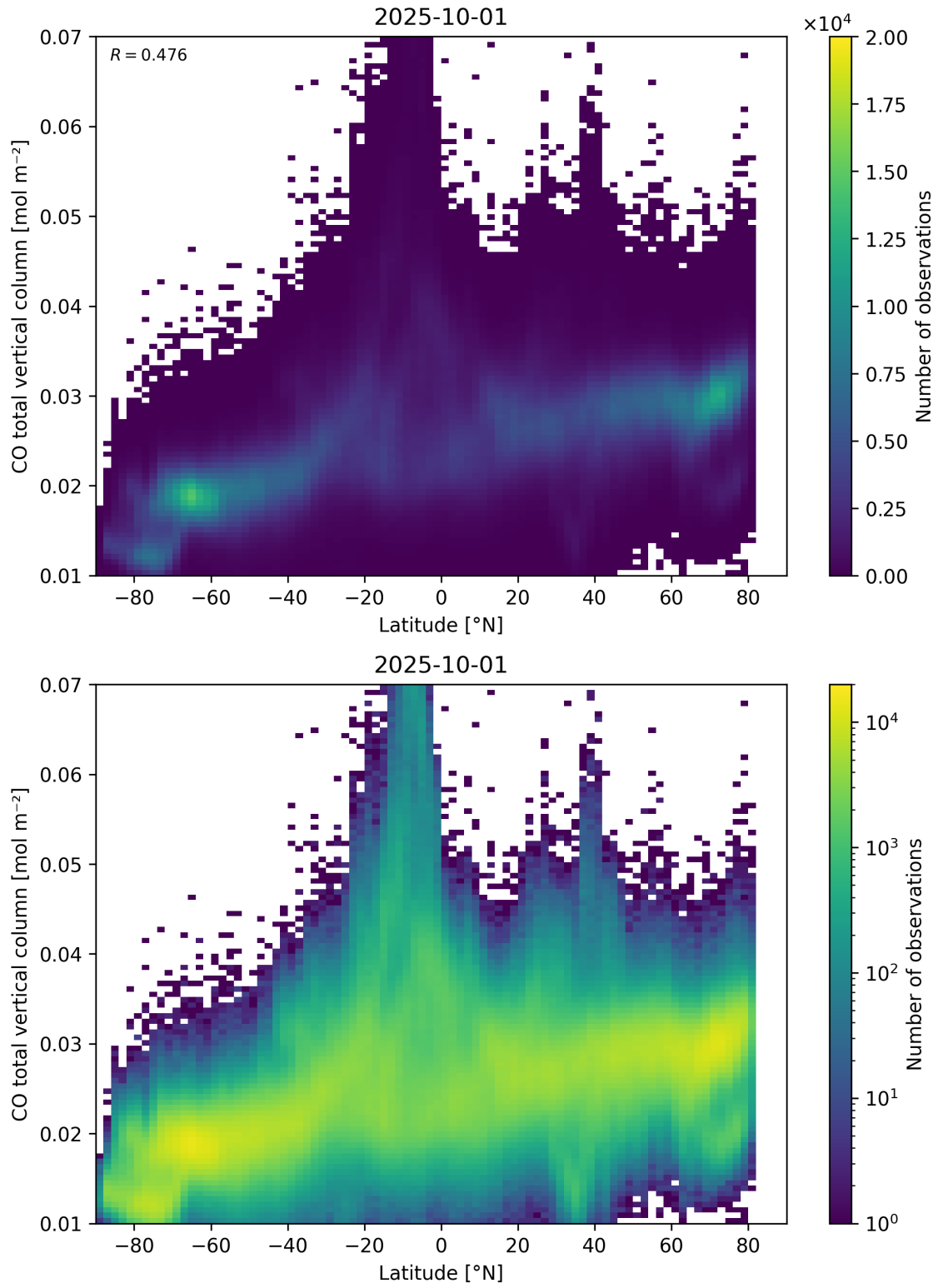
Figure 51: Scatter density plot of “Latitude” against “CO total vertical column” for 2025-10-01 to 2025-10-02.
