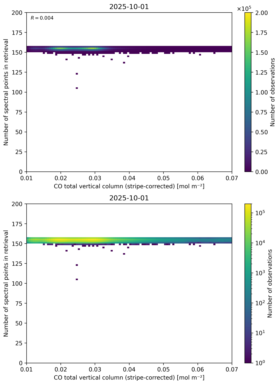
Figure 40: Scatter density plot of “CO total vertical column (stripe-corrected)” against “Number of spectral points in retrieval” for 2025-10-01 to 2025-10-02.
