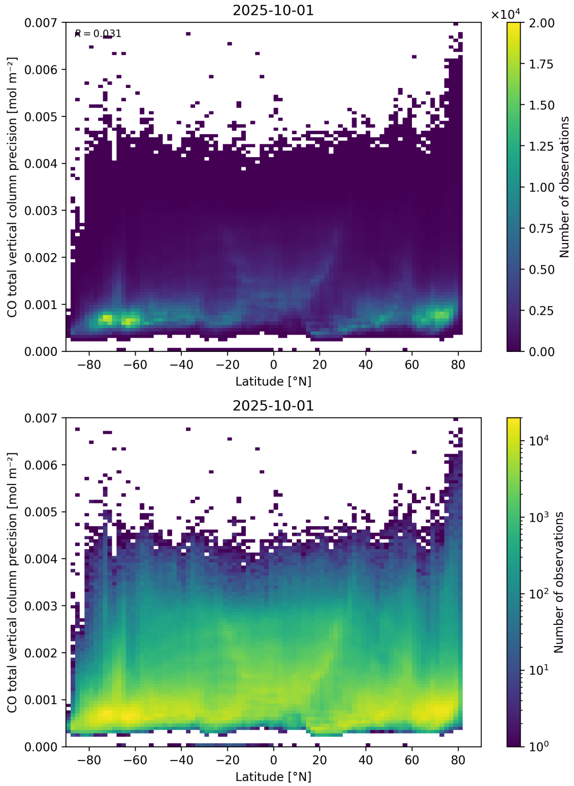
Figure 53: Scatter density plot of “Latitude” against “CO total vertical column precision” for 2025-10-01 to 2025-10-02.
