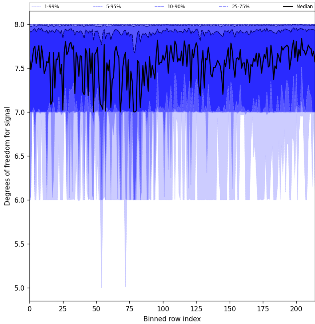
Figure 31: Along track statistics of “Degrees of freedom for signal” for 2025-10-01 to 2025-10-02
