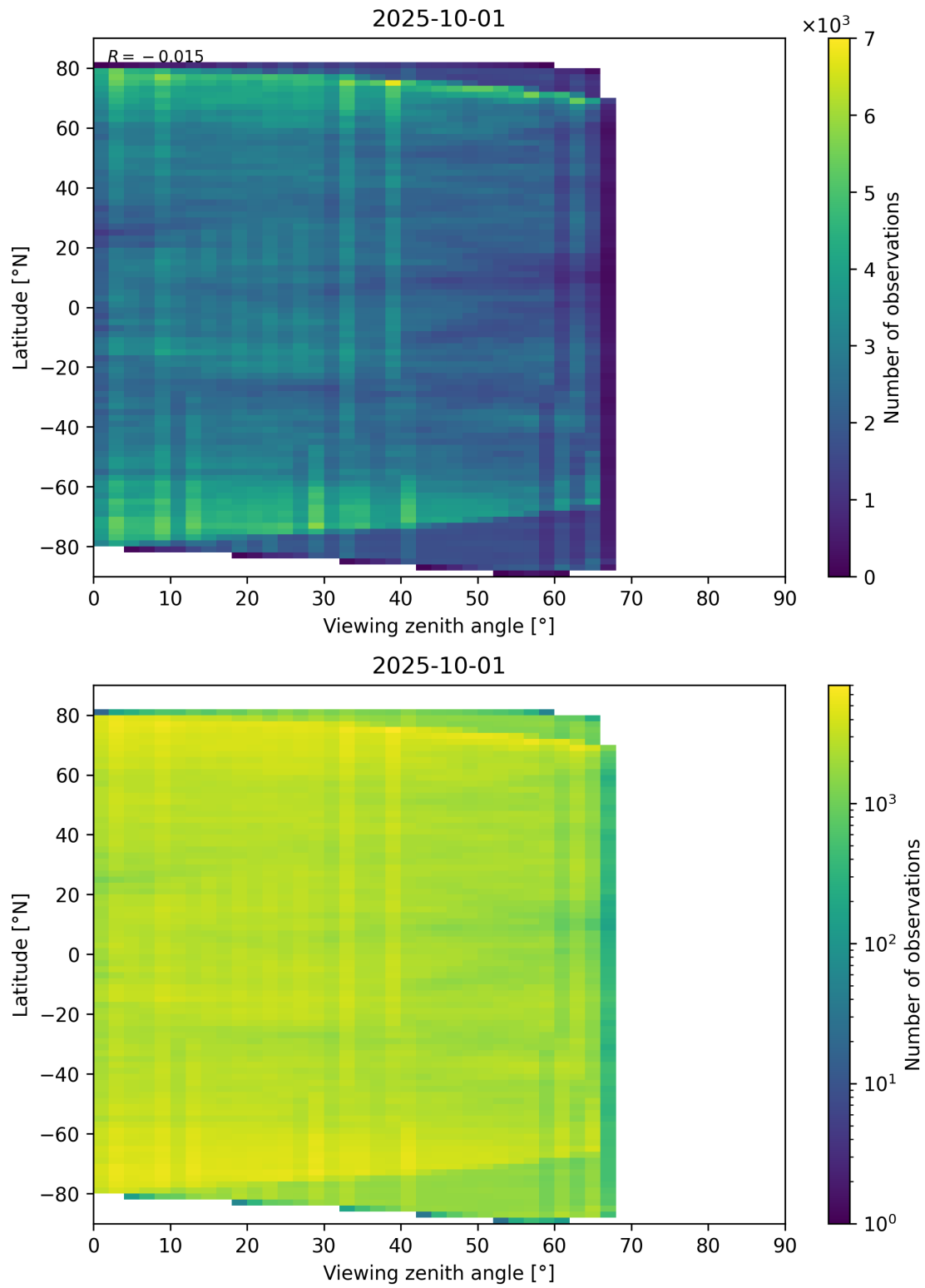
Figure 74: Scatter density plot of “Viewing zenith angle” against “Latitude” for 2025-10-01 to 2025-10-02.
