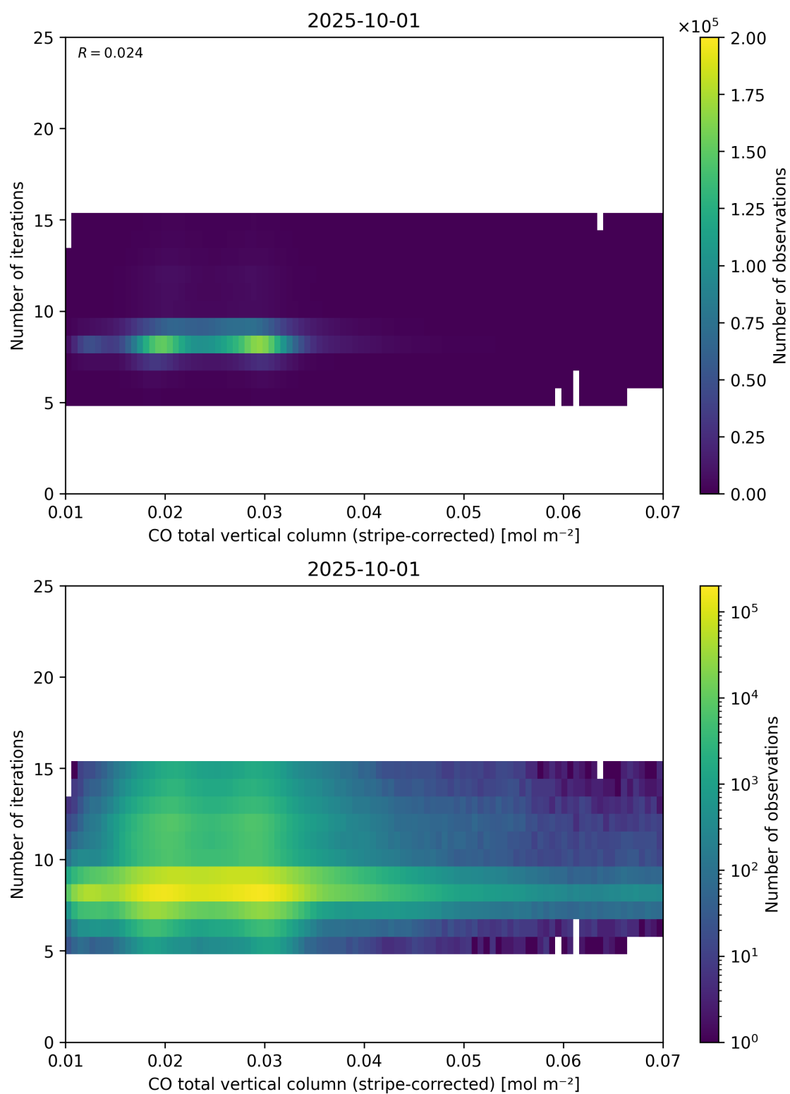
Figure 39: Scatter density plot of “CO total vertical column (stripe-corrected)” against “Number of iterations” for 2025-10-01 to 2025-10-02.
