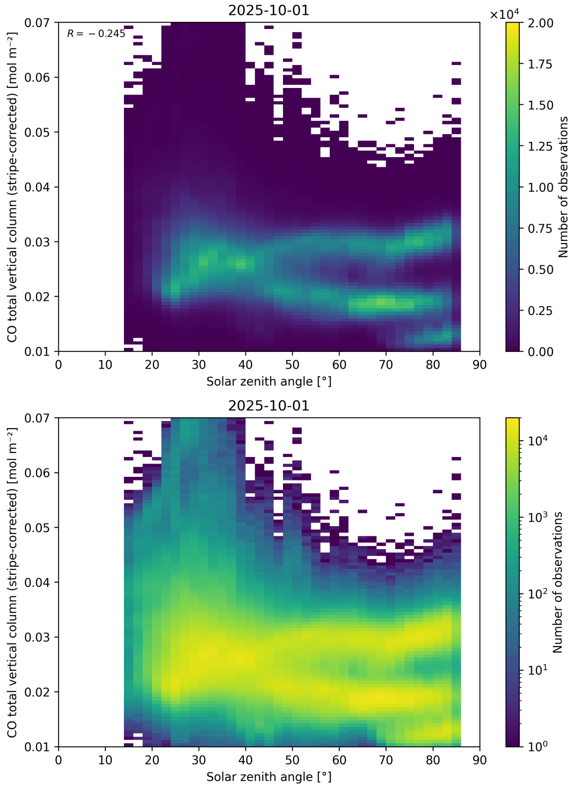
Figure 62: Scatter density plot of “Solar zenith angle” against “CO total vertical column (stripe-corrected)” for 2025-10-01 to 2025-10-02.
