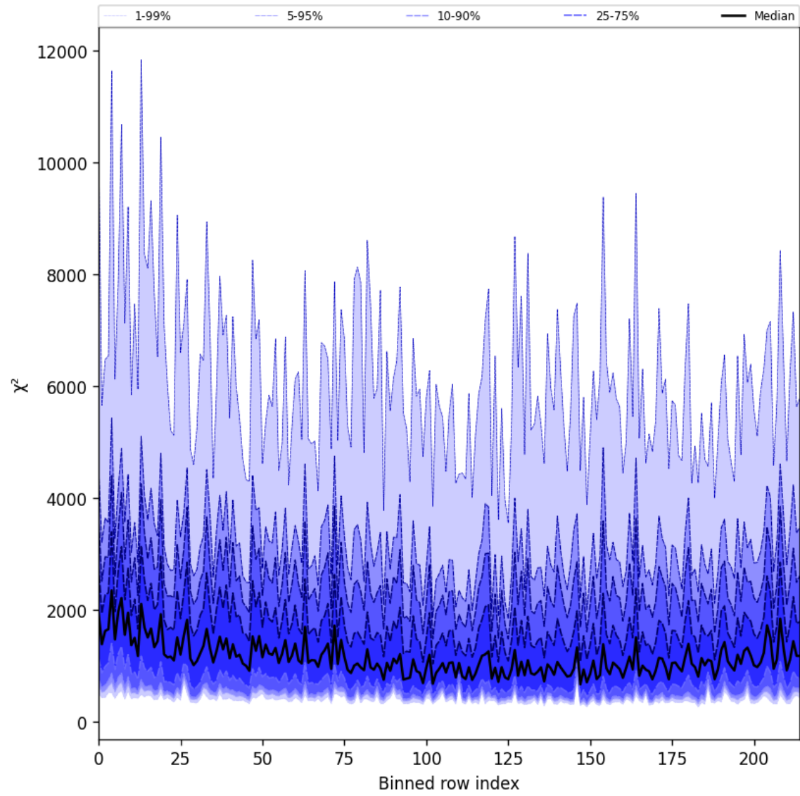
Figure 30: Along track statistics of “ \chi^2 ” for 2025-10-01 to 2025-10-02
