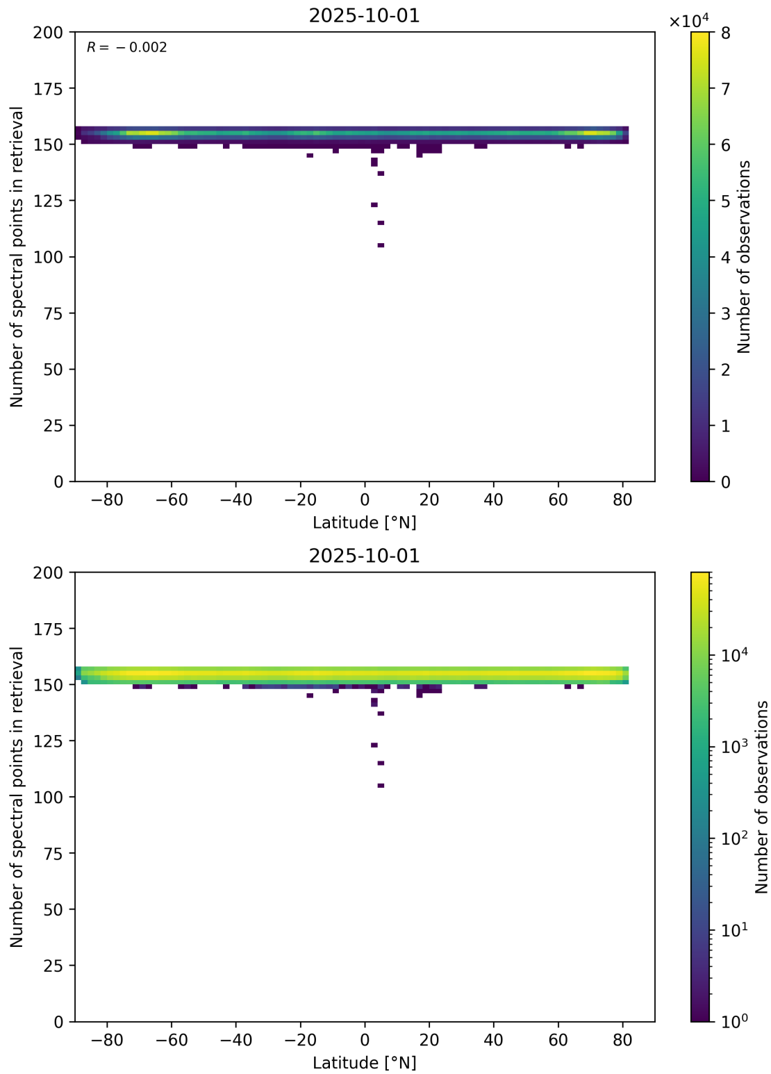
Figure 57: Scatter density plot of “Latitude” against “Number of spectral points in retrieval” for 2025-10-01 to 2025-10-02.
