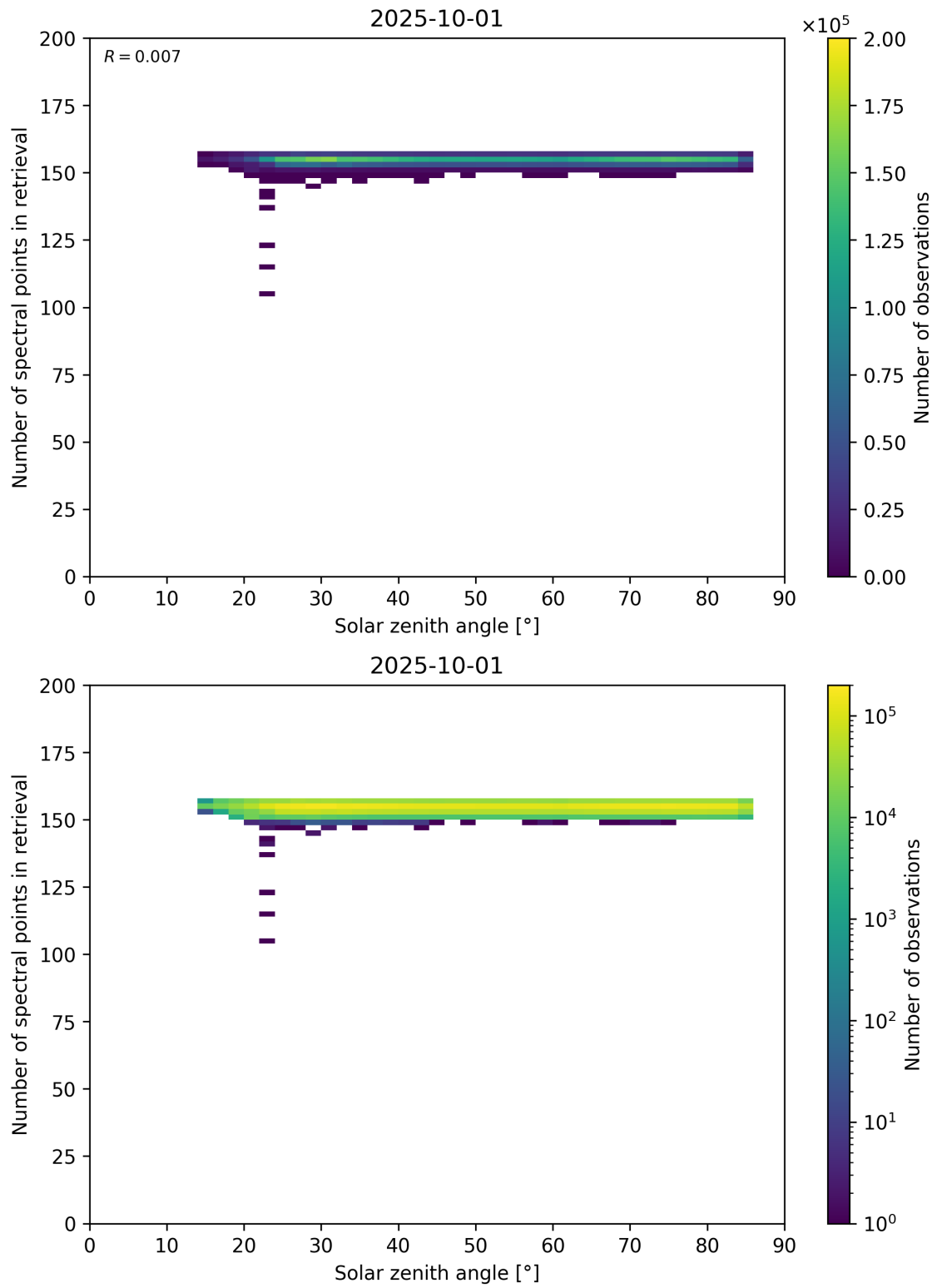
Figure 68: Scatter density plot of “Solar zenith angle” against “Number of spectral points in retrieval” for 2025-10-01 to 2025-10-02.
