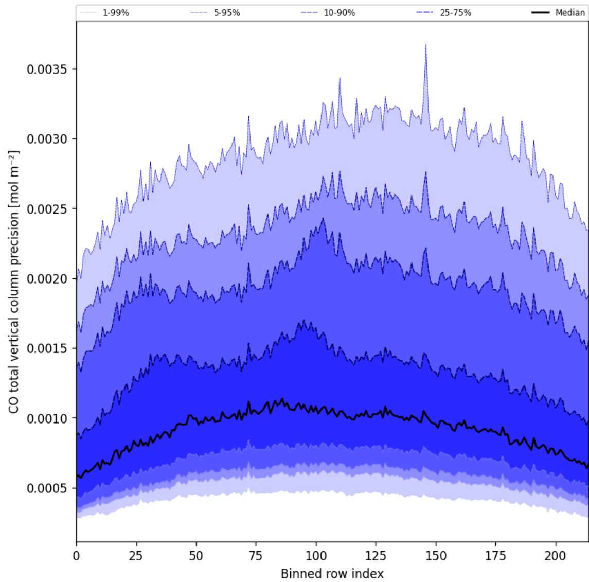
Figure 28: Along track statistics of “CO total vertical column precision” for 2025-10-01 to 2025-10-02
