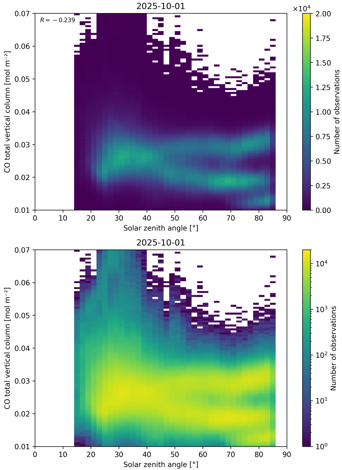
Figure 61: Scatter density plot of “Solar zenith angle” against “CO total vertical column” for 2025-10-01 to 2025-10-02.
