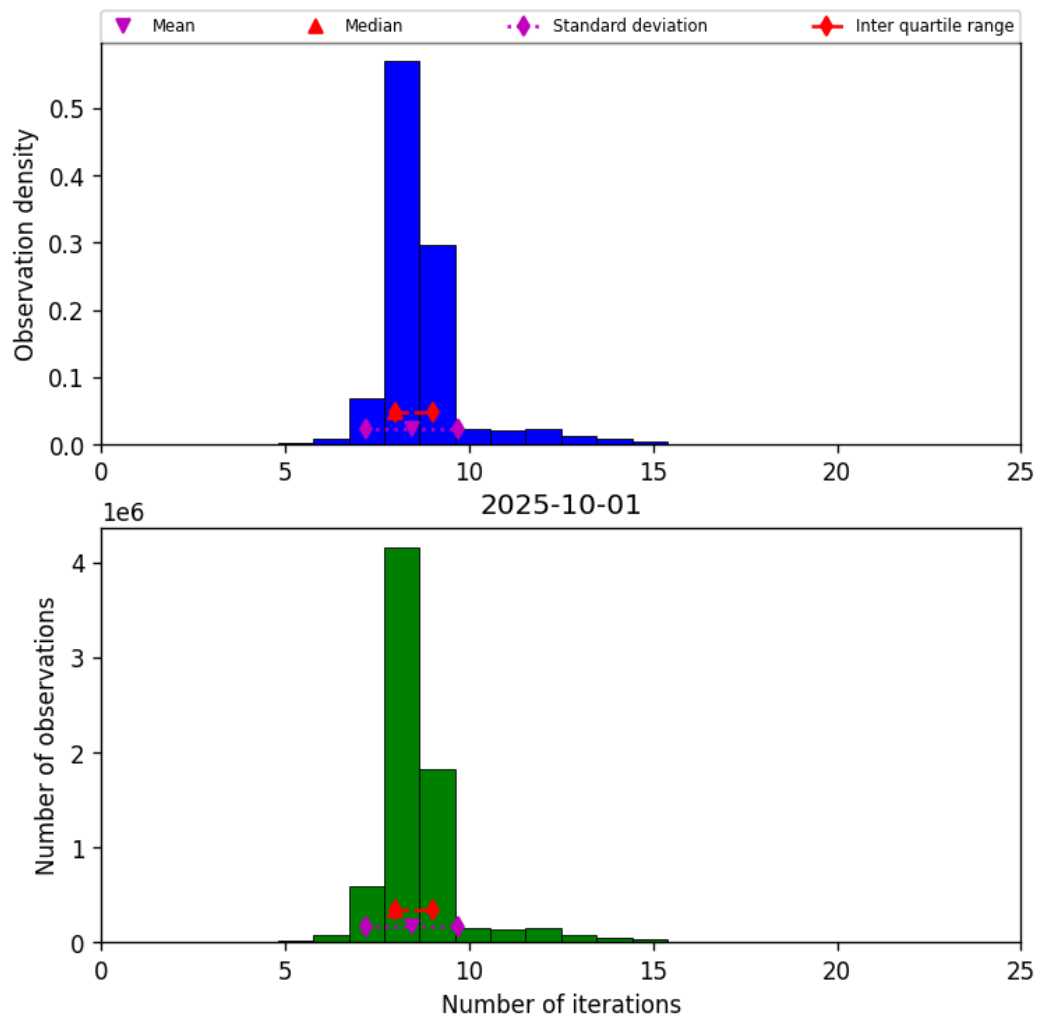
Figure 24: Histogram of “Number of iterations” for 2025-10-01 to 2025-10-02
