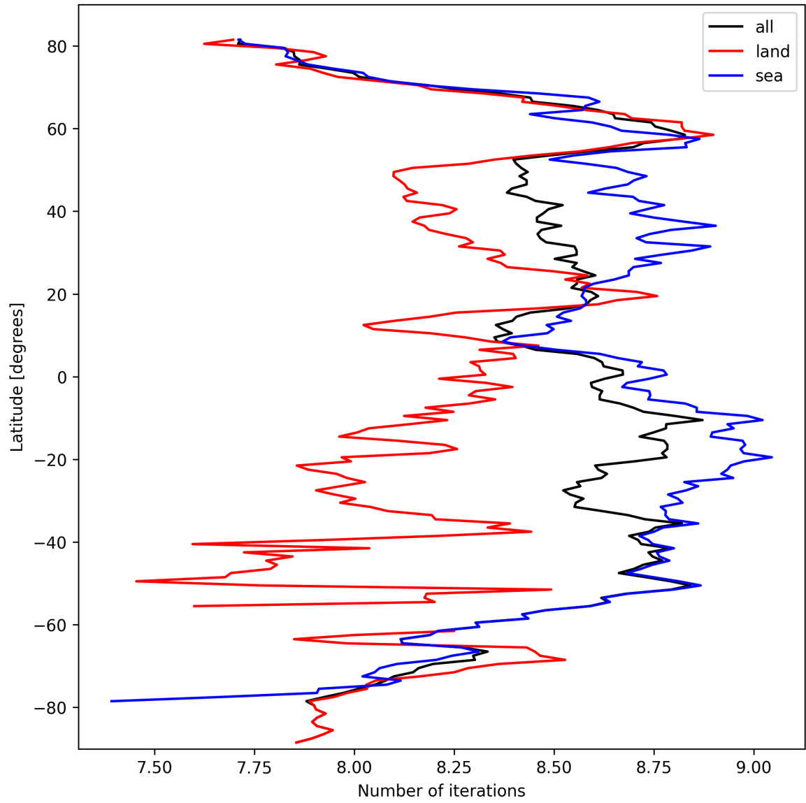
Figure 16: Zonal average of “Number of iterations” for 2025-10-01 to 2025-10-02.
