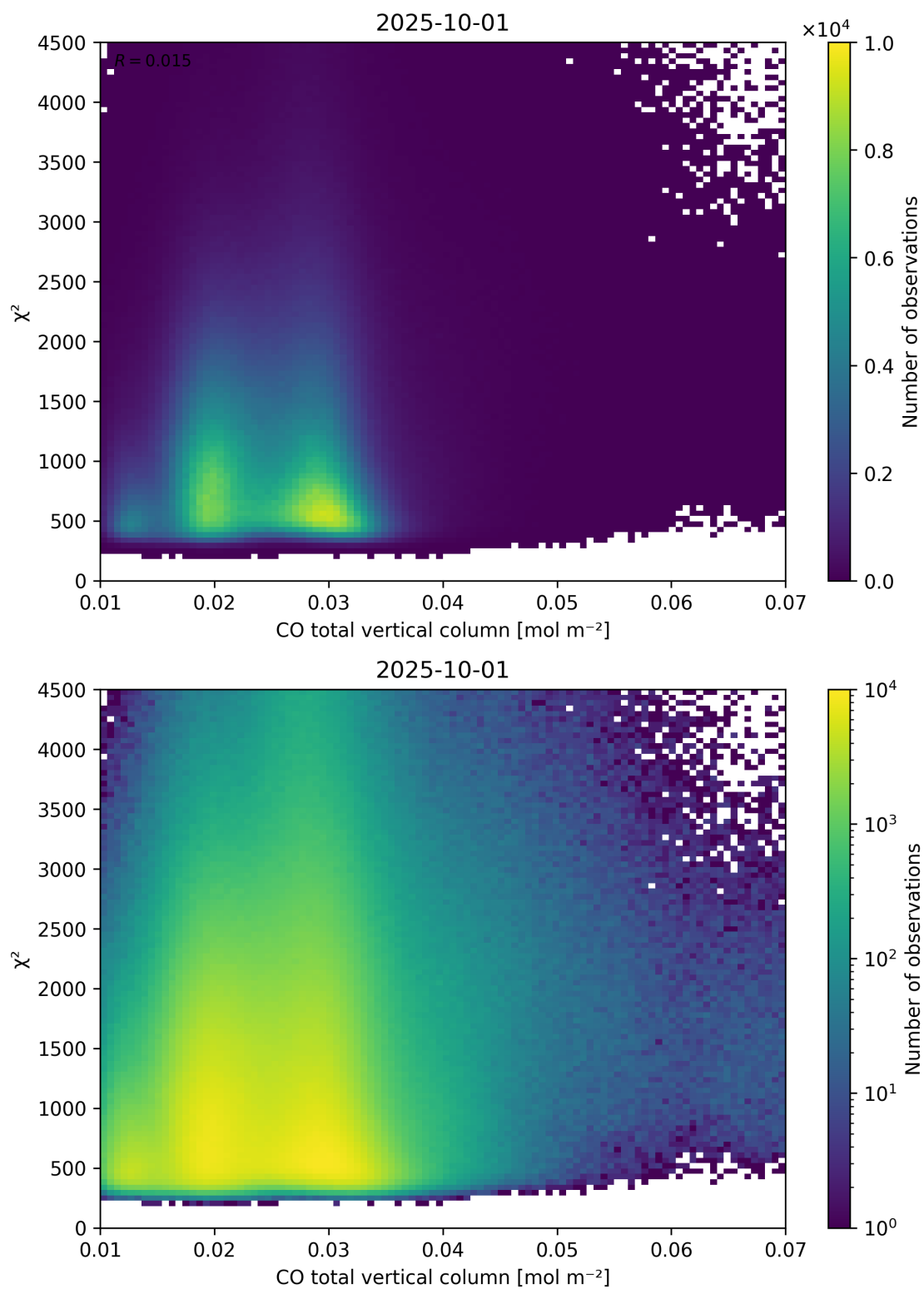
Figure 35: Scatter density plot of “CO total vertical column” against “ \chi^2 ” for 2025-10-01 to 2025-10-02.
