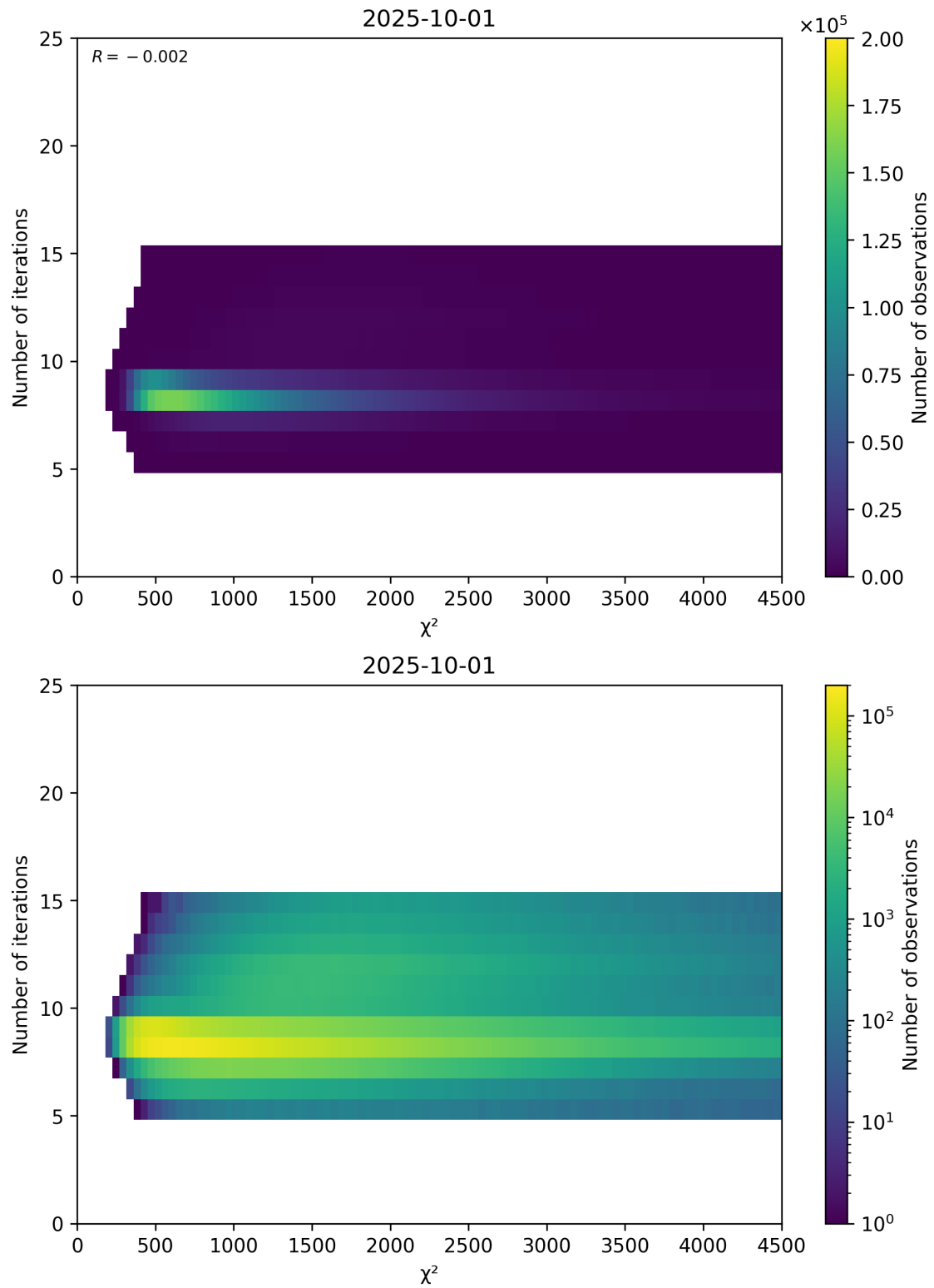
Figure 49: Scatter density plot of “ \chi^2 ” against “Number of iterations” for 2025-10-01 to 2025-10-02.
