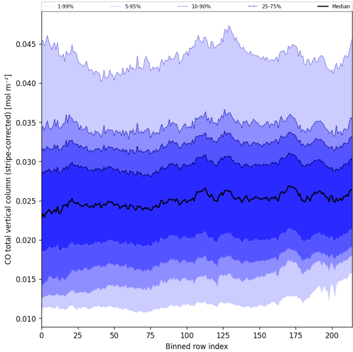
Figure 27: Along track statistics of “CO total vertical column (stripe-corrected)” for 2025-10-01 to 2025-10-02
