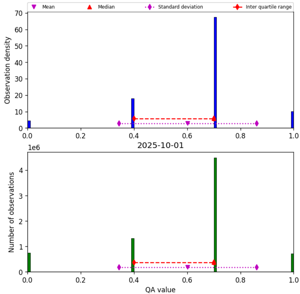
Figure 17: Histogram of “QA value” for 2025-10-01 to 2025-10-02
