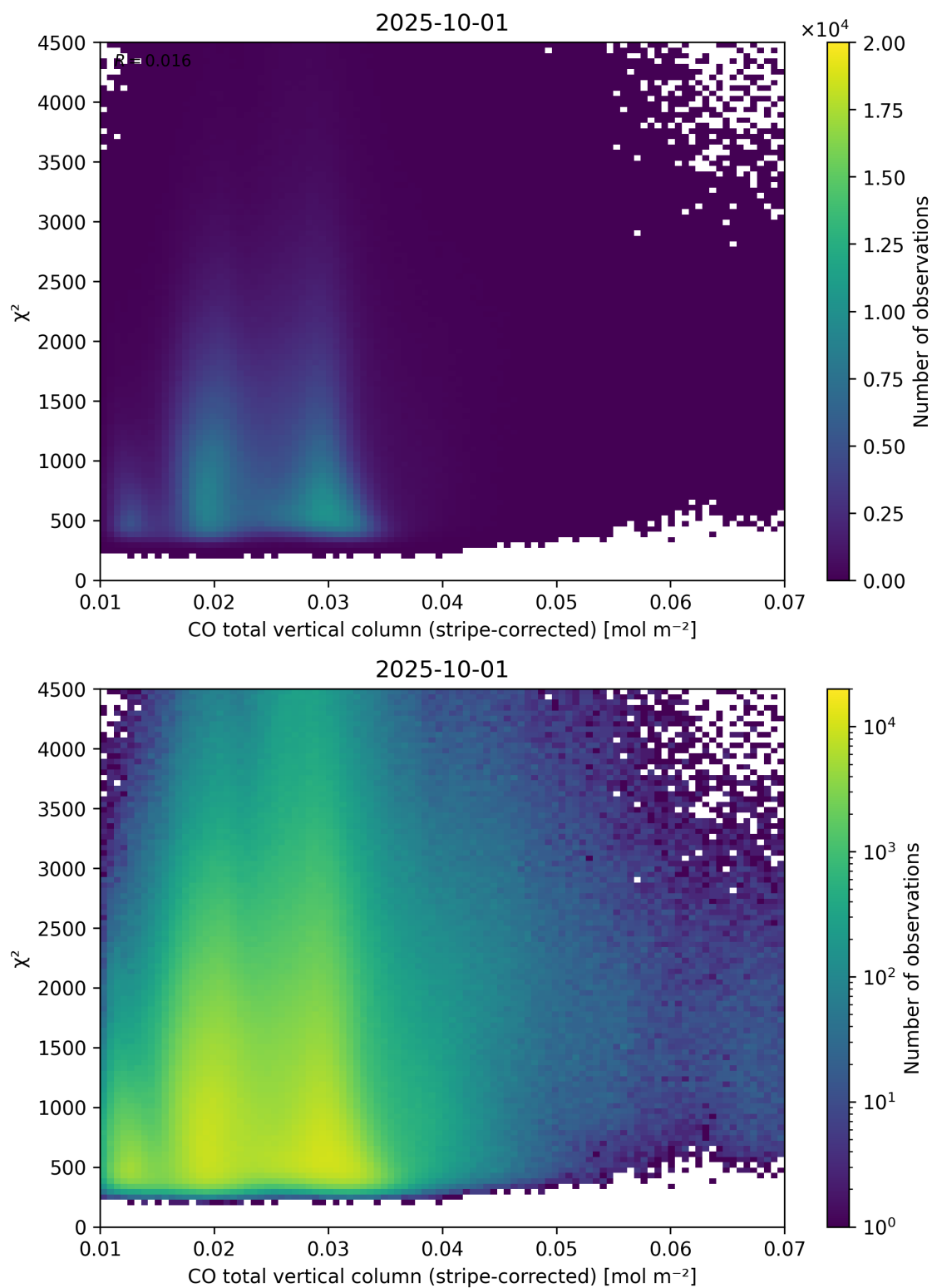
Figure 37: Scatter density plot of “CO total vertical column (stripe-corrected)” against “ \chi^2 ” for 2025-10-01 to 2025-10-02.
