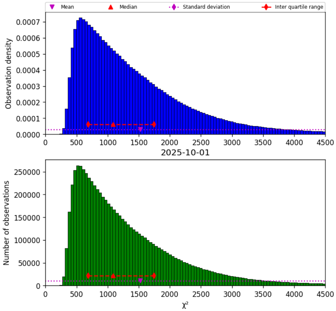
Figure 22: Histogram of " \chi^2 " for 2025-10-01 to 2025-10-02
