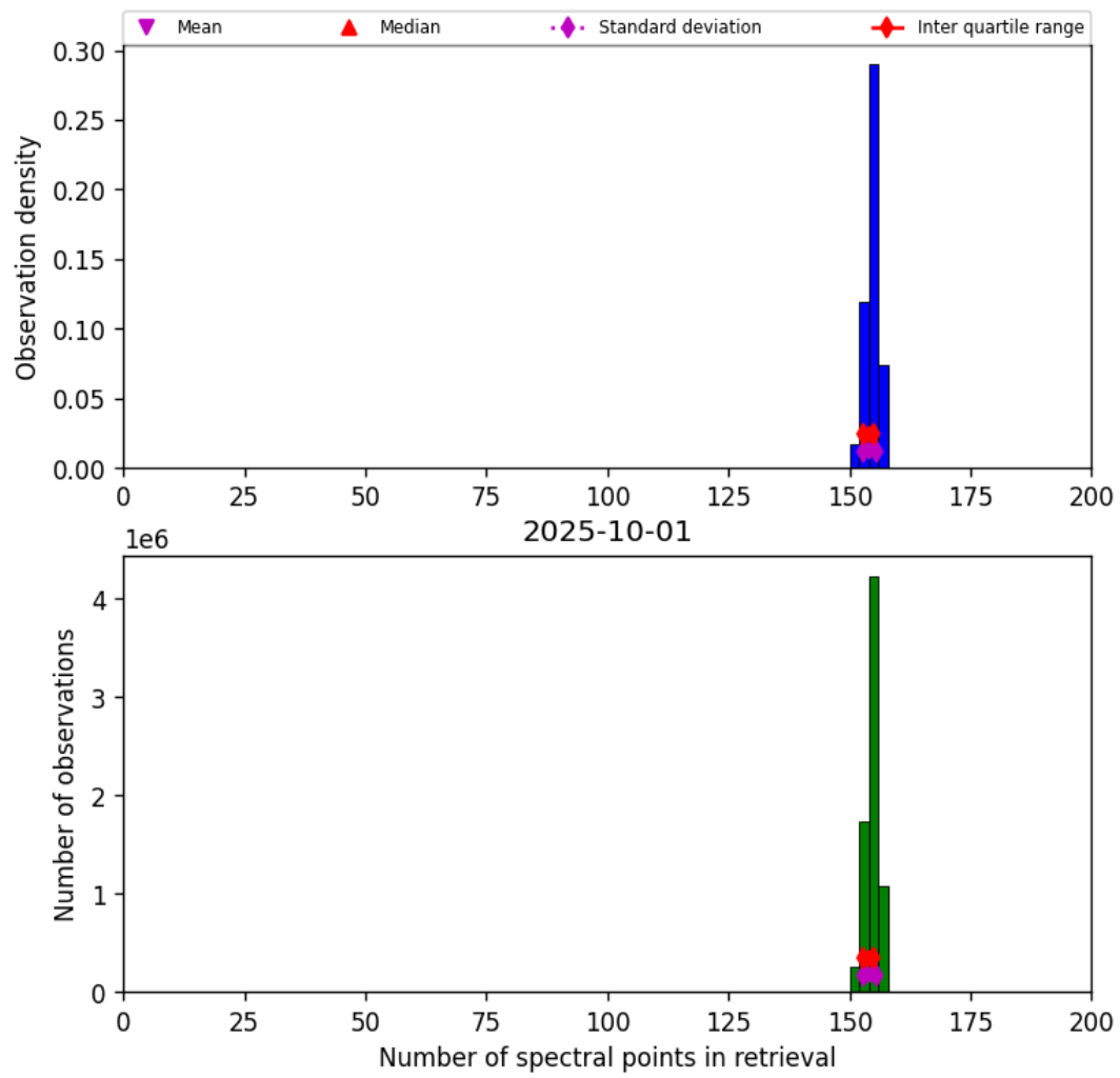
Figure 21: Histogram of “Number of spectral points in retrieval” for 2025-10-01 to 2025-10-02
