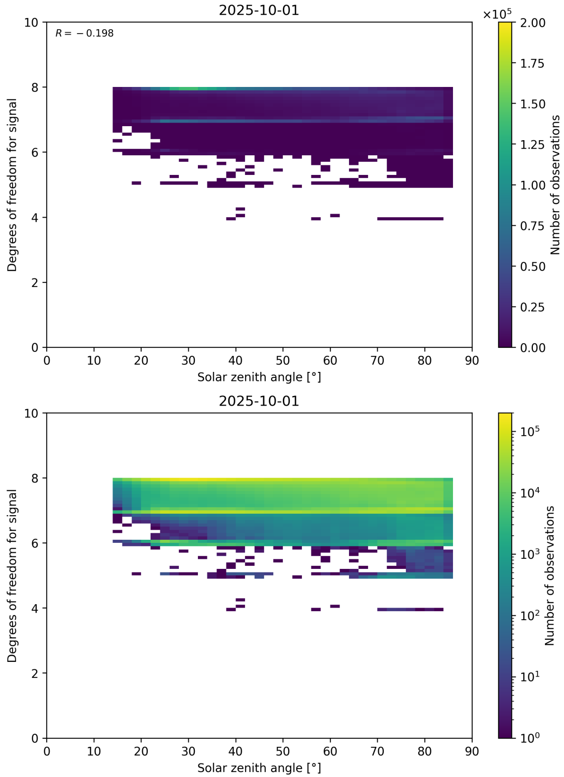
Figure 65: Scatter density plot of “Solar zenith angle” against “Degrees of freedom for signal” for 2025-10-01 to 2025-10-02.
