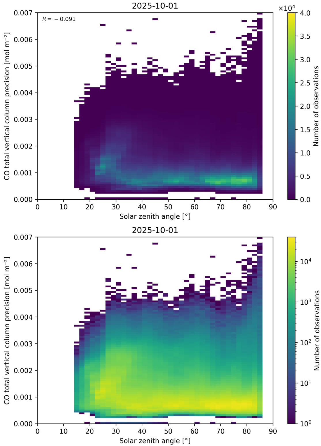
Figure 63: Scatter density plot of “Solar zenith angle” against “CO total vertical column precision” for 2025-10-01 to 2025-10-02.
