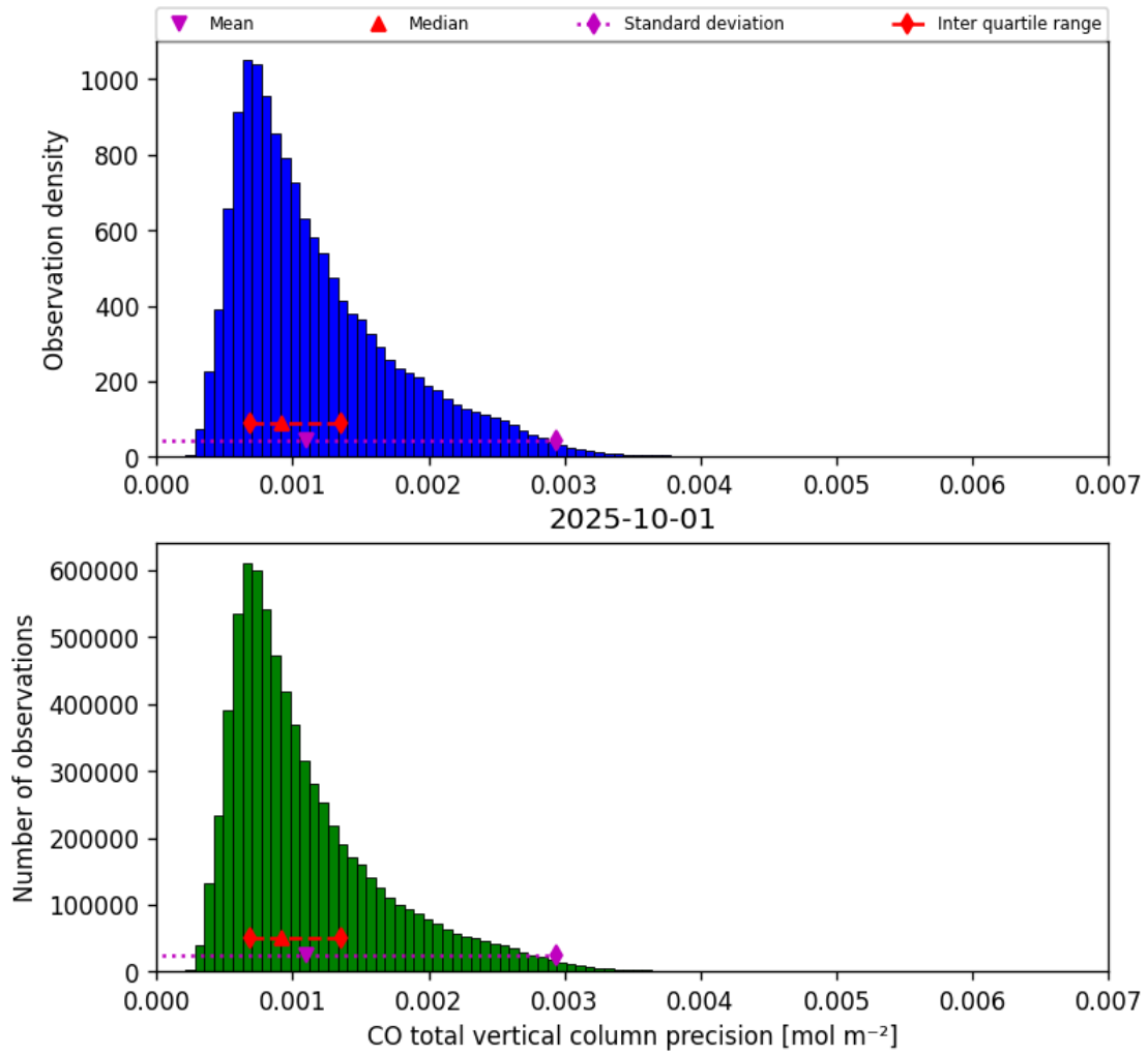
Figure 20: Histogram of “CO total vertical column precision” for 2025-10-01 to 2025-10-02
