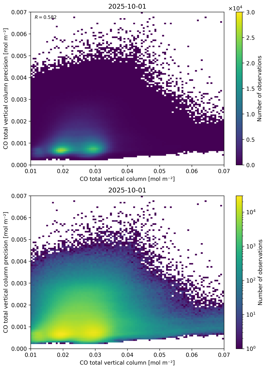
Figure 34: Scatter density plot of “CO total vertical column” against “CO total vertical column precision” for 2025-10-01 to 2025-10-02.
