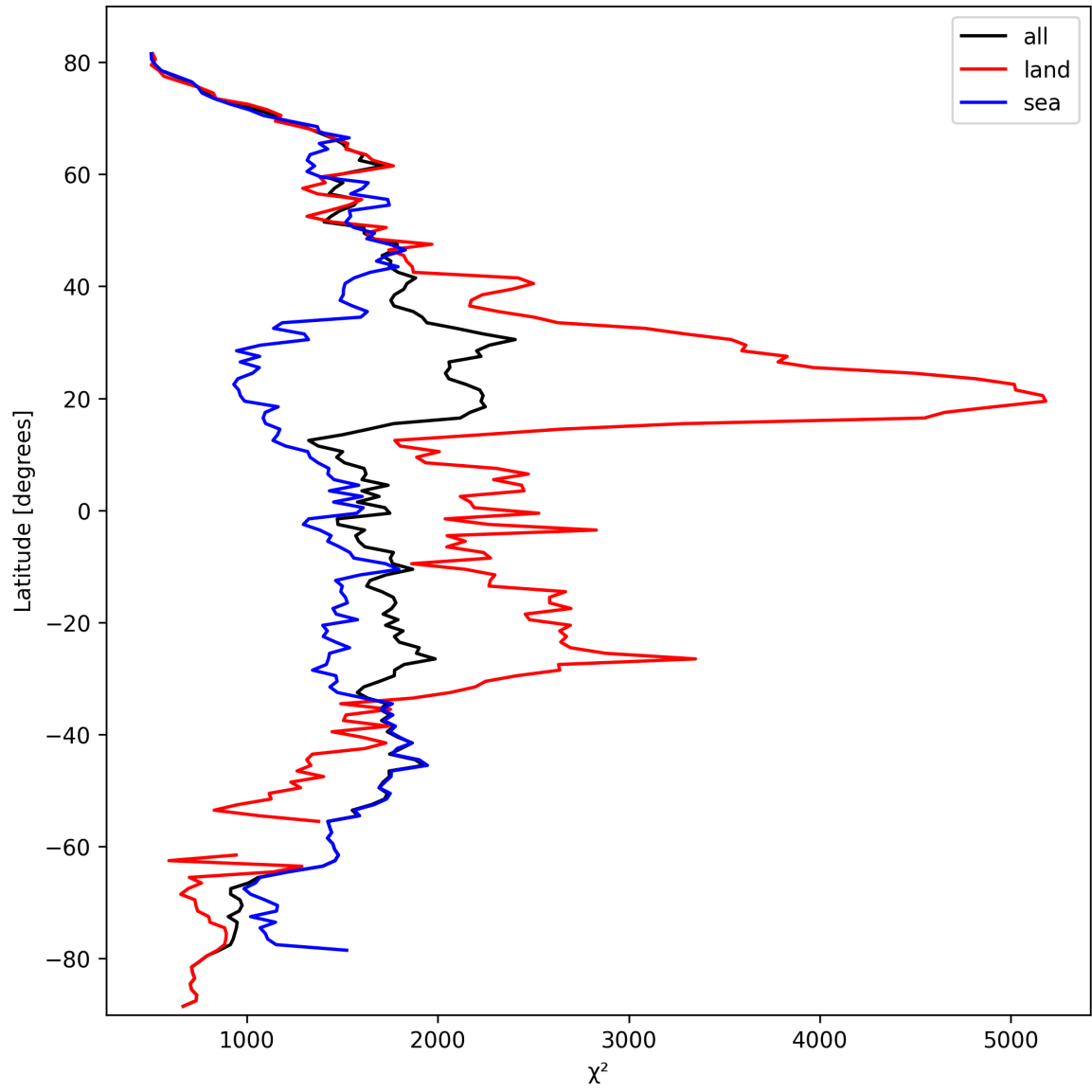
Figure 14: Zonal average of “ \chi^2 ” for 2025-10-01 to 2025-10-02.
