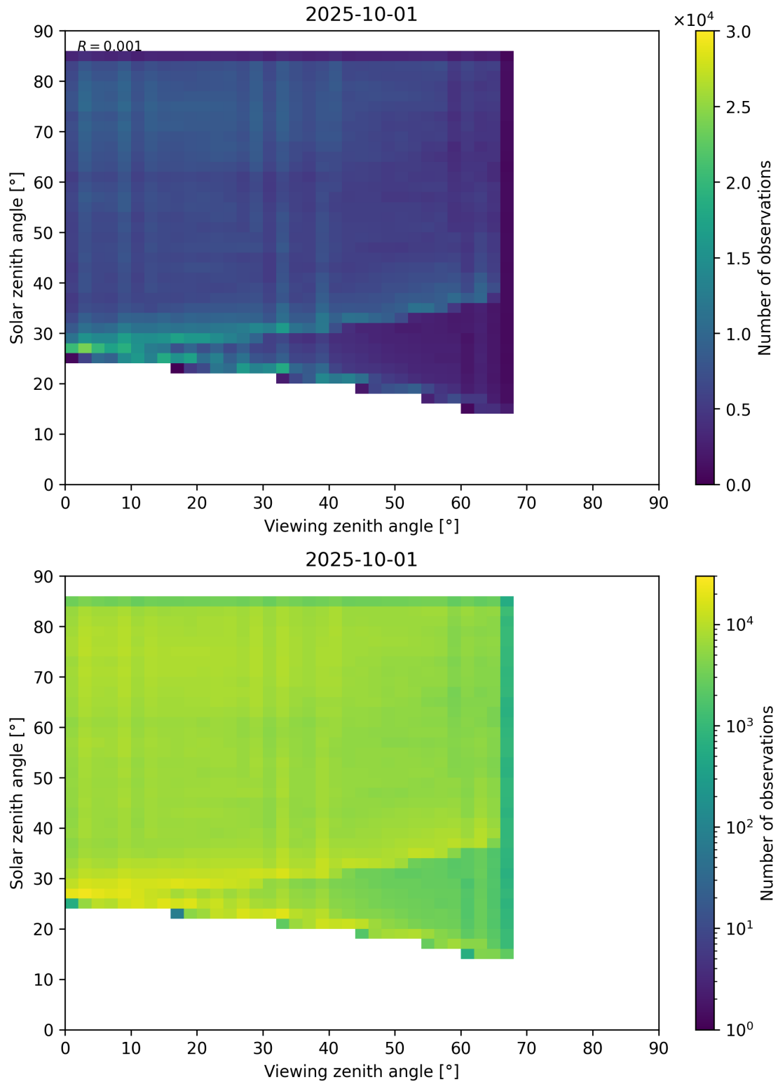
Figure 77: Scatter density plot of “Viewing zenith angle” against “Solar zenith angle” for 2025-10-01 to 2025-10-02.
