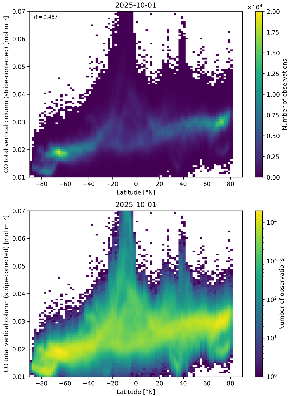
Figure 52: Scatter density plot of “Latitude” against “CO total vertical column (stripe-corrected)” for 2025-10-01 to 2025-10-02.
