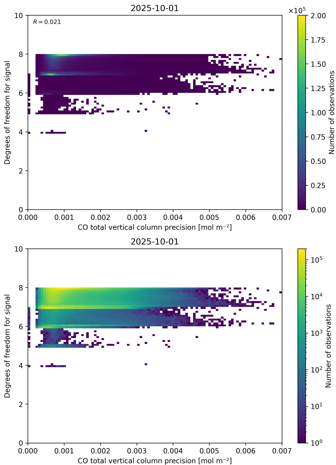
Figure 45: Scatter density plot of “CO total vertical column precision” against “Degrees of freedom for signal” for 2025-10-01 to 2025-10-02.
