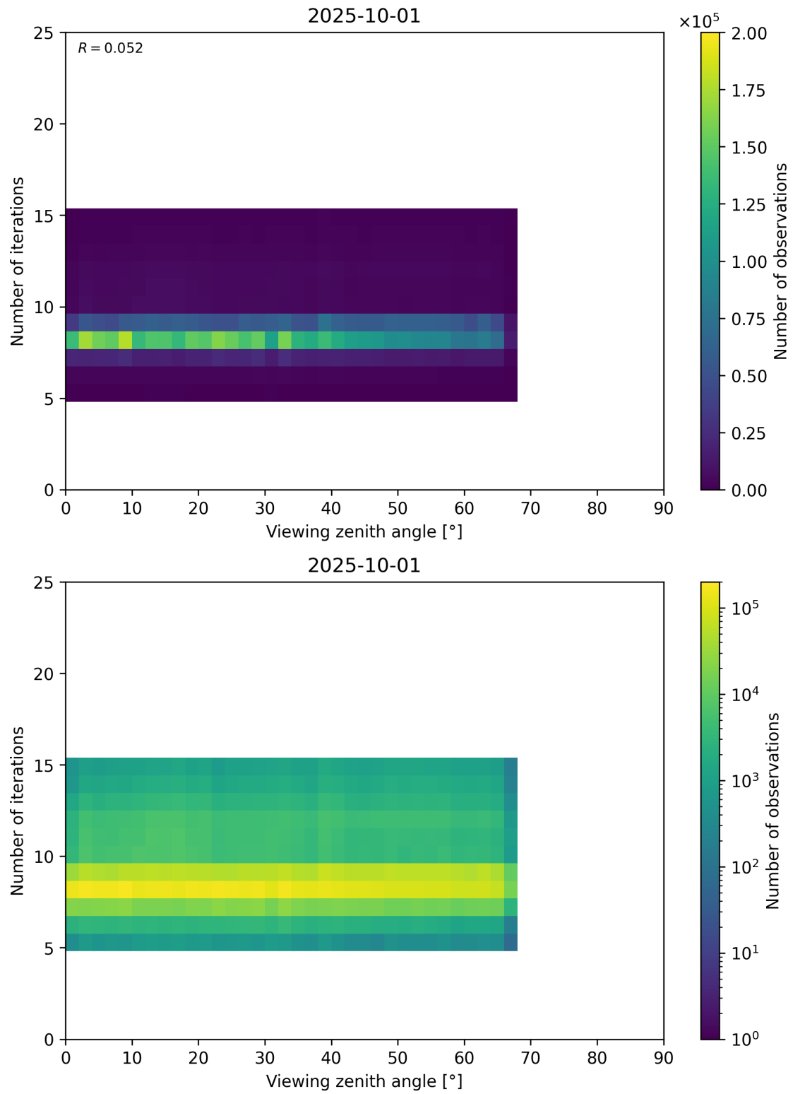
Figure 75: Scatter density plot of “Viewing zenith angle” against “Number of iterations” for 2025-10-01 to 2025-10-02.
