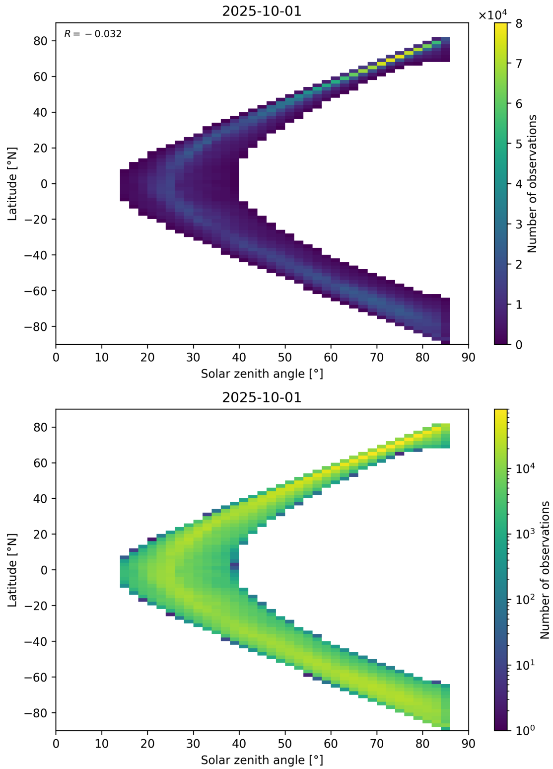
Figure 66: Scatter density plot of “Solar zenith angle” against “Latitude” for 2025-10-01 to 2025-10-02.
