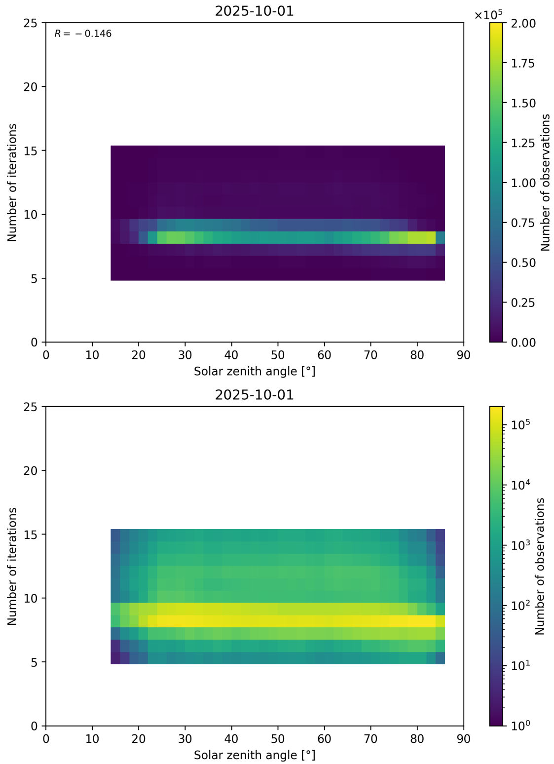
Figure 67: Scatter density plot of “Solar zenith angle” against “Number of iterations” for 2025-10-01 to 2025-10-02.
