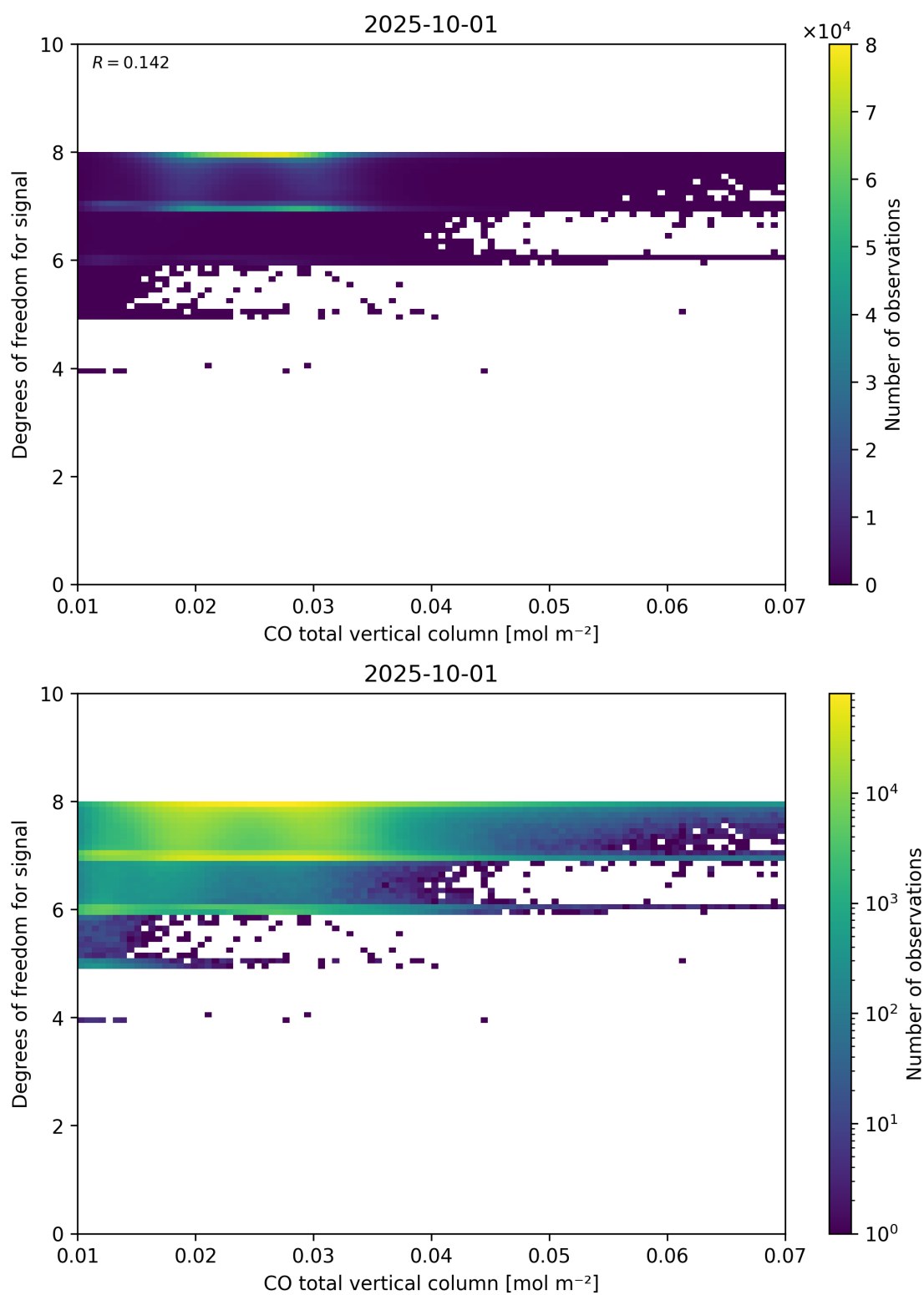
Figure 41: Scatter density plot of “CO total vertical column” against “Degrees of freedom for signal” for 2025-10-01 to 2025-10-02.
