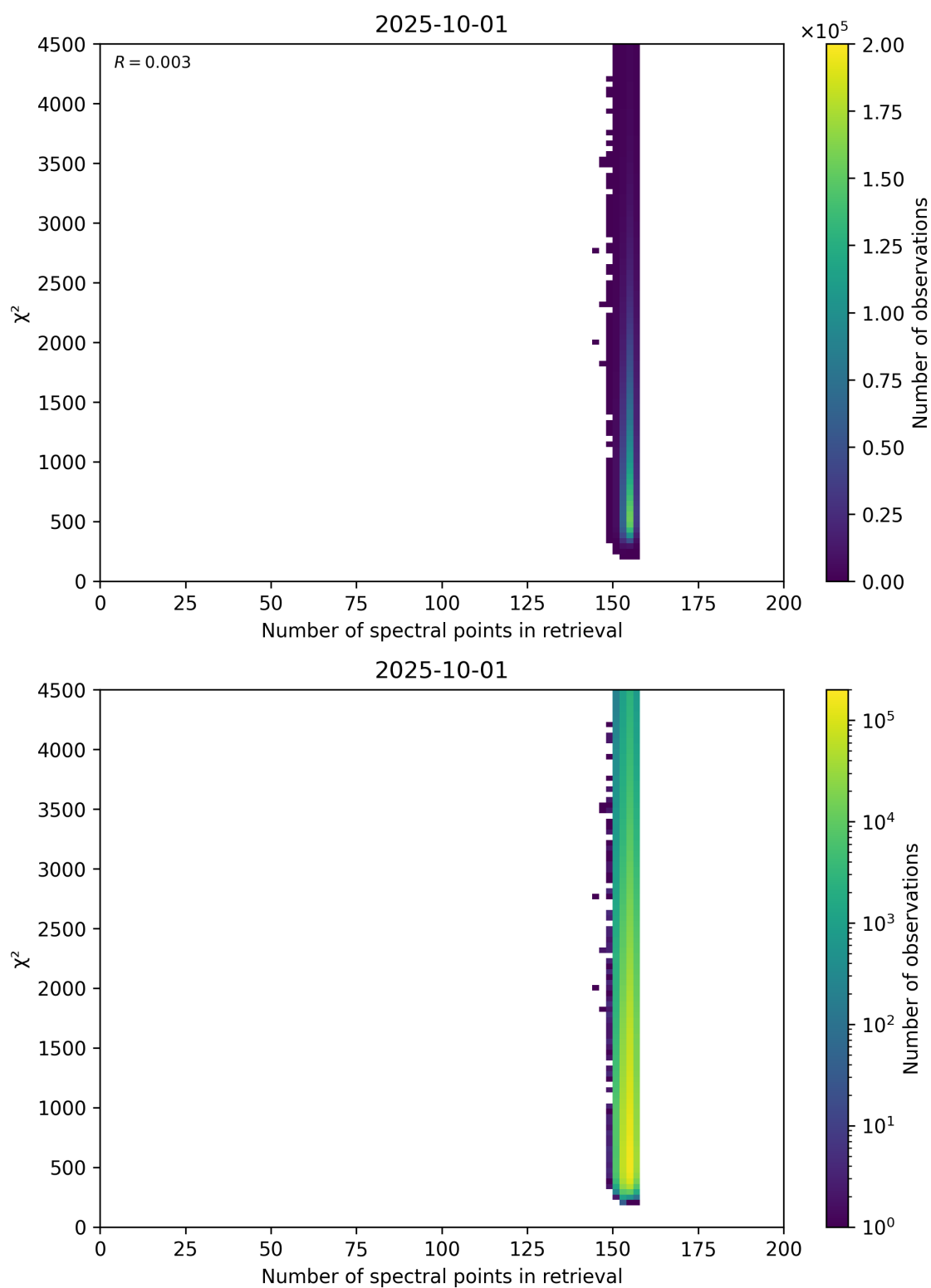
Figure 58: Scatter density plot of “Number of spectral points in retrieval” against “ \chi^2 ” for 2025-10-01 to 2025-10-02.
