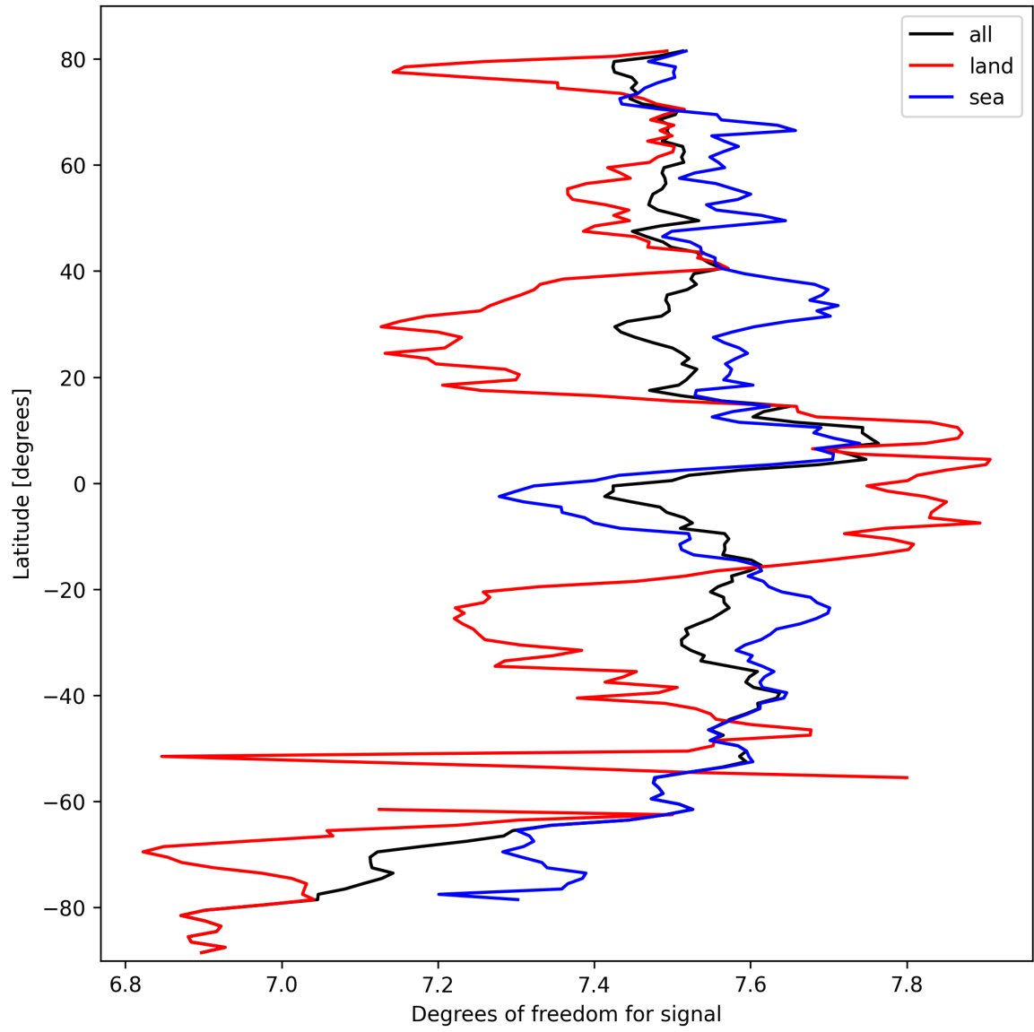
Figure 15: Zonal average of “Degrees of freedom for signal” for 2025-10-01 to 2025-10-02.
