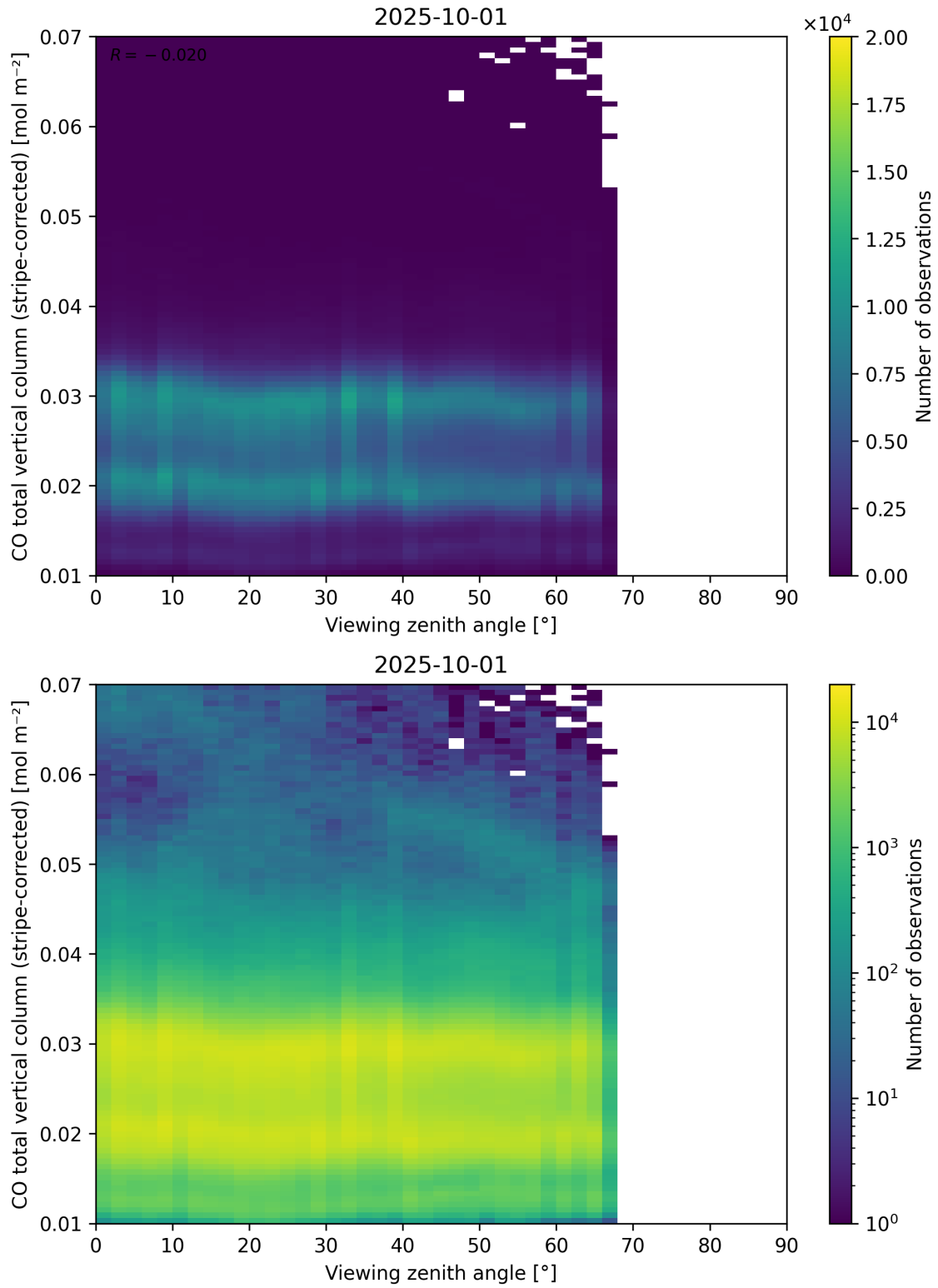
Figure 70: Scatter density plot of “Viewing zenith angle” against “CO total vertical column (stripe-corrected)” for 2025-10-01 to 2025-10-02.
