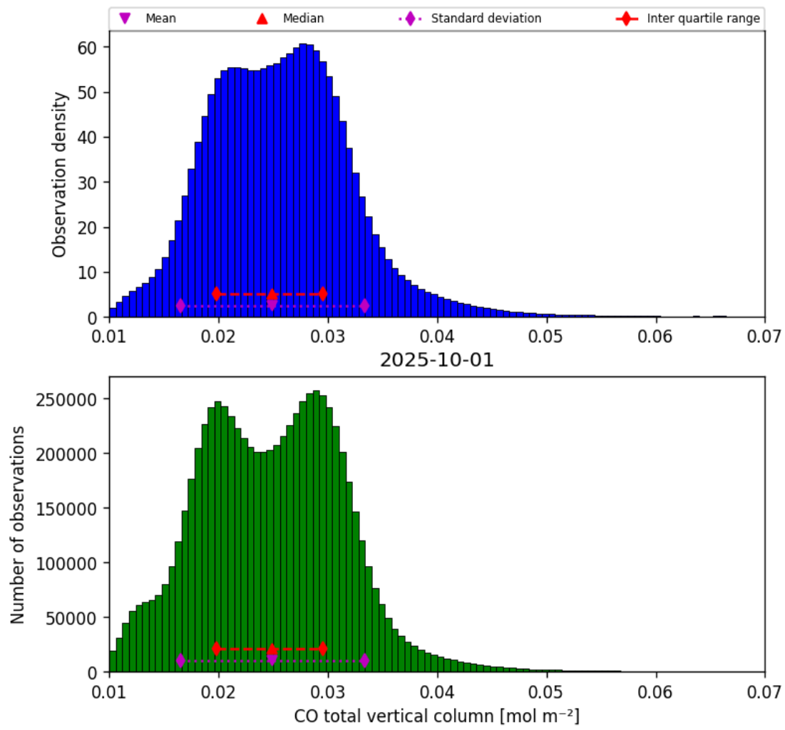
Figure 18: Histogram of “CO total vertical column” for 2025-10-01 to 2025-10-02
