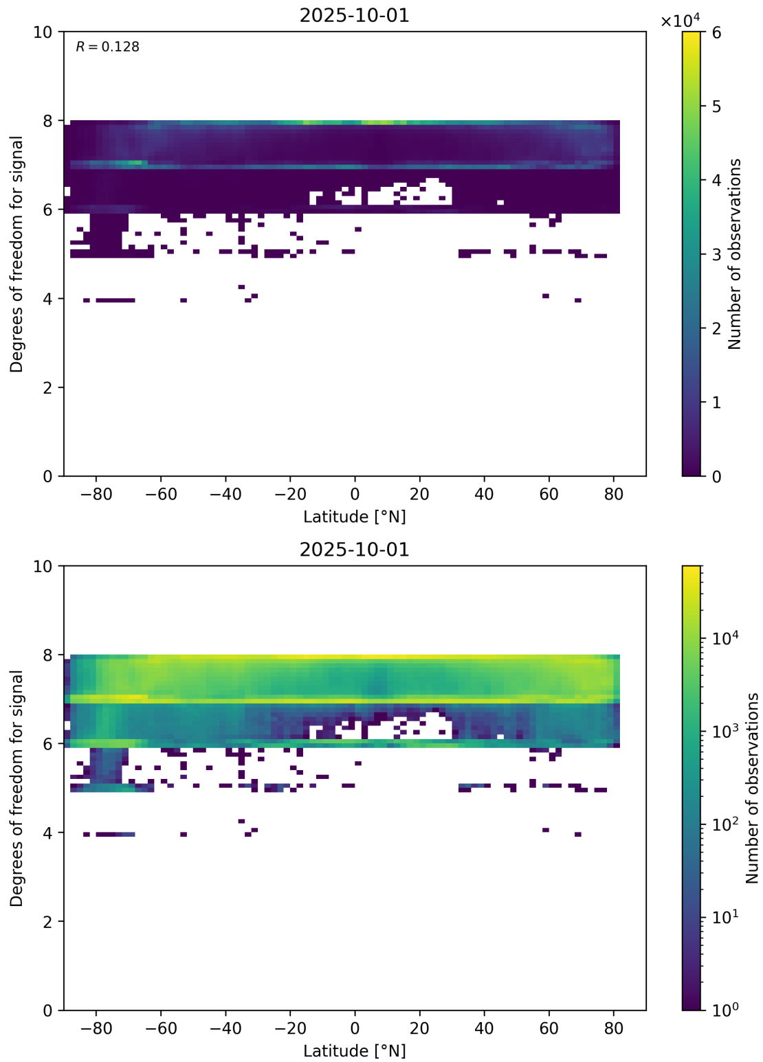
Figure 55: Scatter density plot of “Latitude” against “Degrees of freedom for signal” for 2025-10-01 to 2025-10-02.
