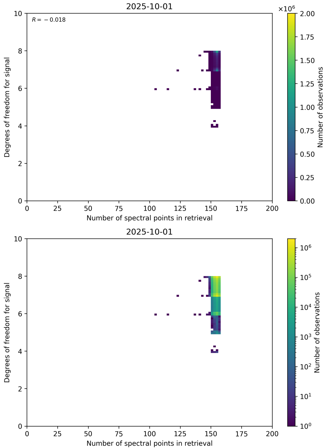
Figure 59: Scatter density plot of “Number of spectral points in retrieval” against “Degrees of freedom for signal” for 2025-10-01 to 2025-10-02.
