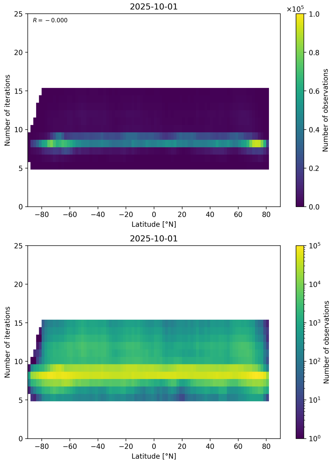
Figure 56: Scatter density plot of “Latitude” against “Number of iterations” for 2025-10-01 to 2025-10-02.
