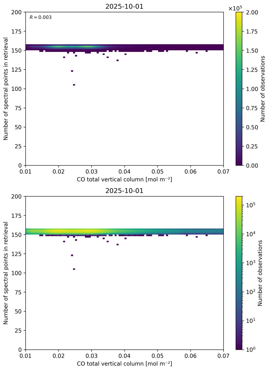
Figure 43: Scatter density plot of “CO total vertical column” against “Number of spectral points in retrieval” for 2025-10-01 to 2025-10-02.
