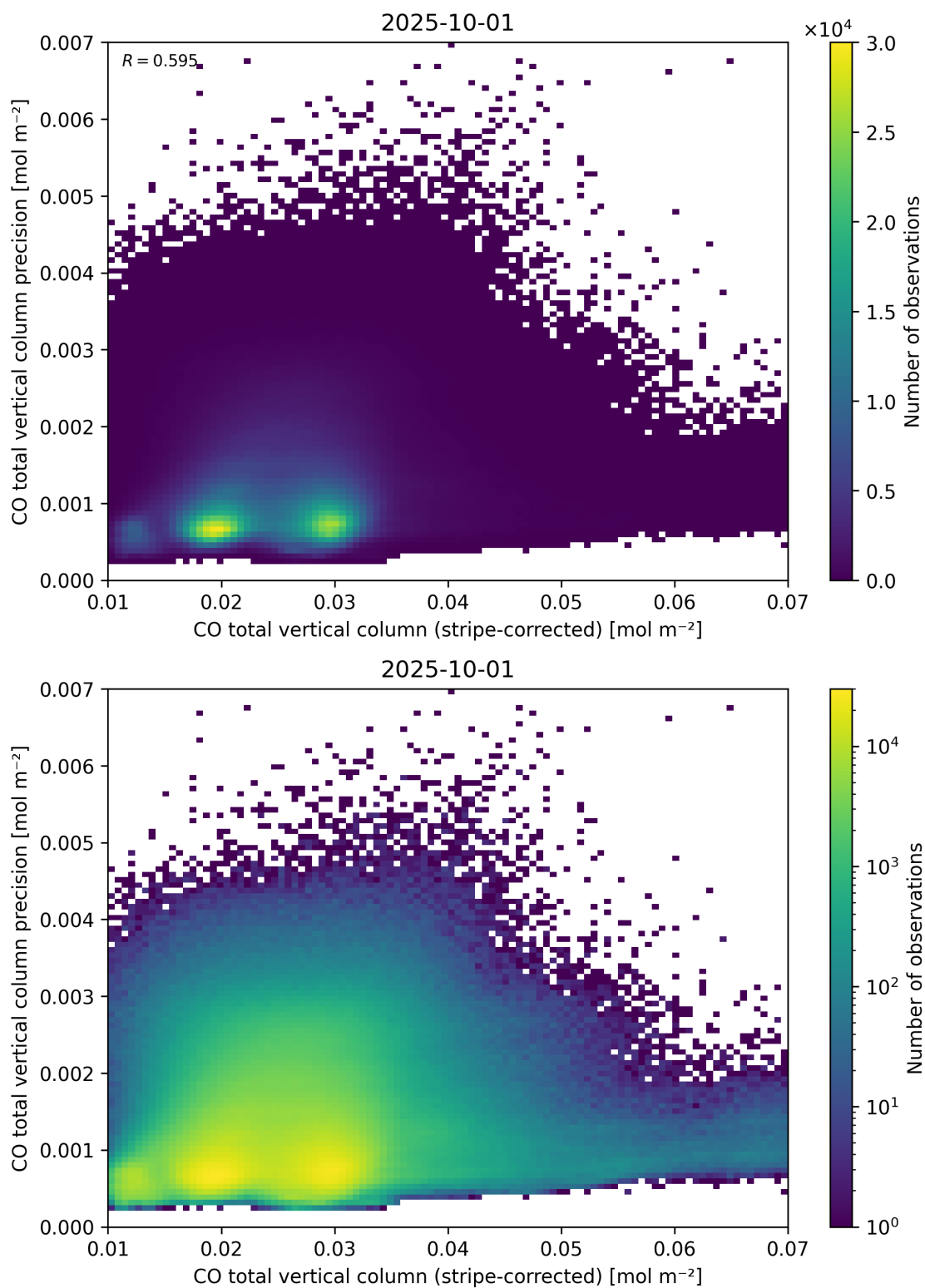
Figure 36: Scatter density plot of “CO total vertical column (stripe-corrected)” against “CO total vertical column precision” for 2025-10-01 to 2025-10-02.
