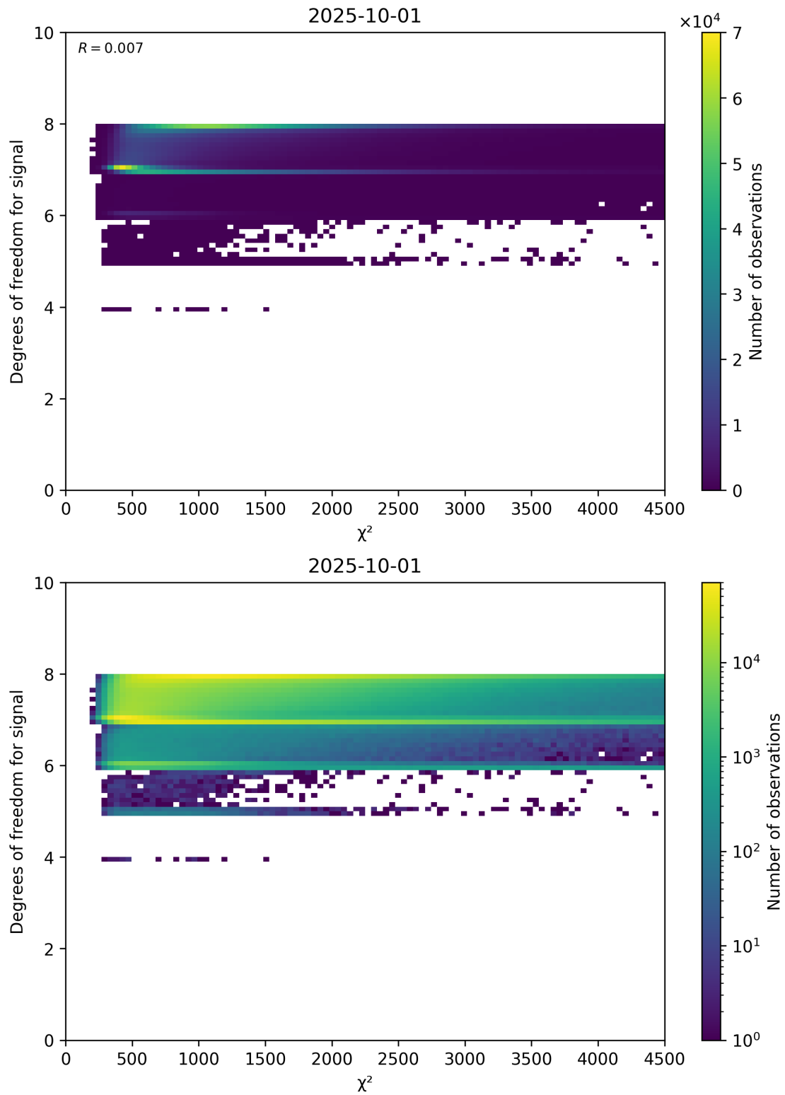
Figure 48: Scatter density plot of “ \chi^2 ” against “Degrees of freedom for signal” for 2025-10-01 to 2025-10-02.
