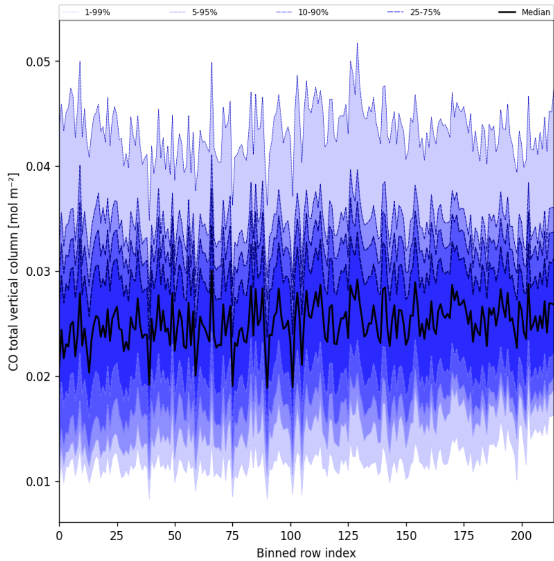
Figure 26: Along track statistics of "CO total vertical column" for 2025-10-01 to 2025-10-02
