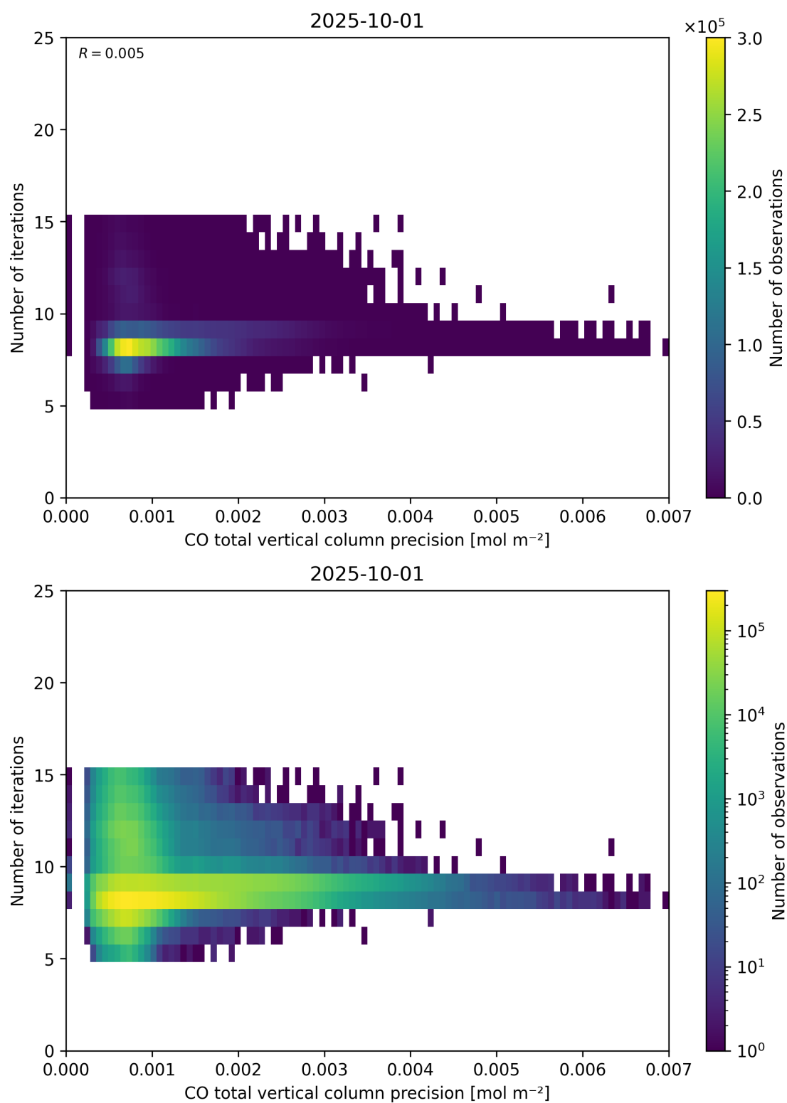
Figure 46: Scatter density plot of “CO total vertical column precision” against “Number of iterations” for 2025-10-01 to 2025-10-02.
