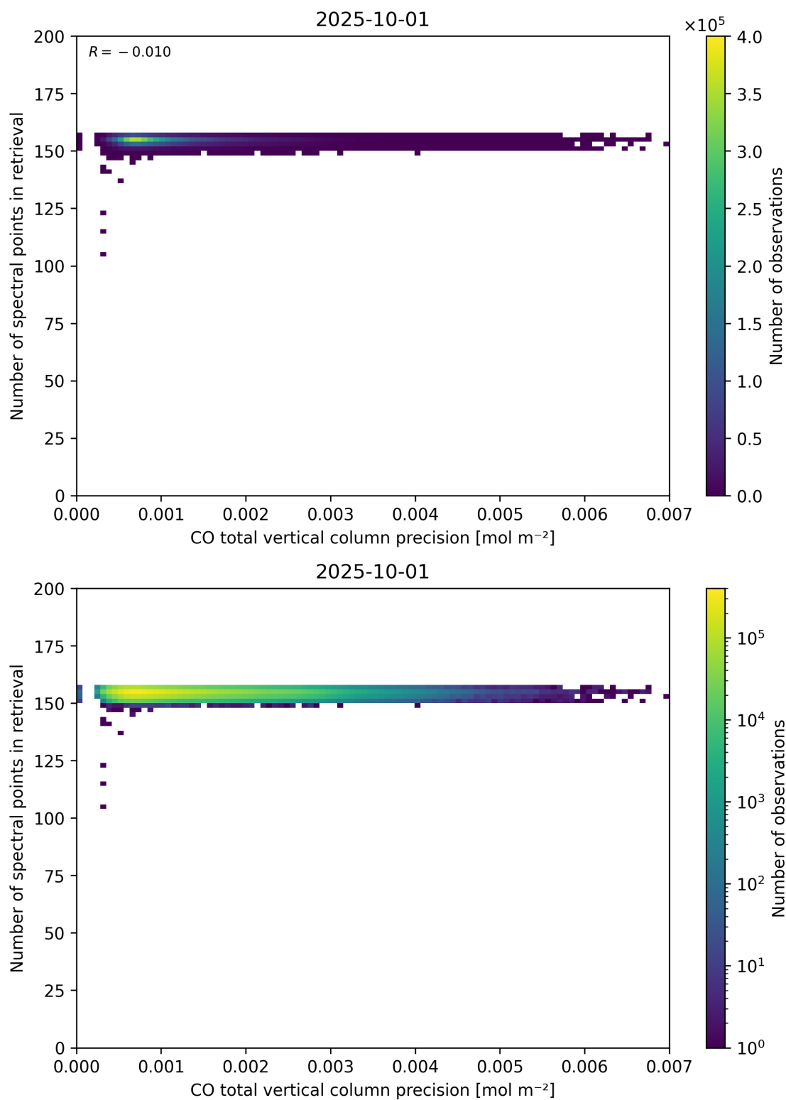
Figure 47: Scatter density plot of “CO total vertical column precision” against “Number of spectral points in retrieval” for 2025-10-01 to 2025-10-02.
