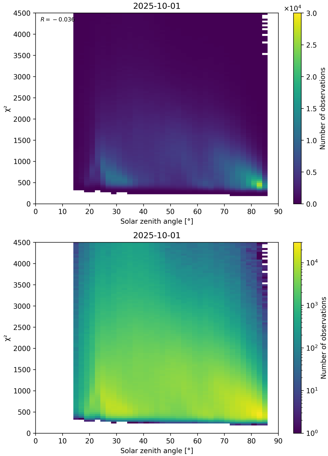
Figure 64: Scatter density plot of “Solar zenith angle” against “ \chi^2 ” for 2025-10-01 to 2025-10-02.
