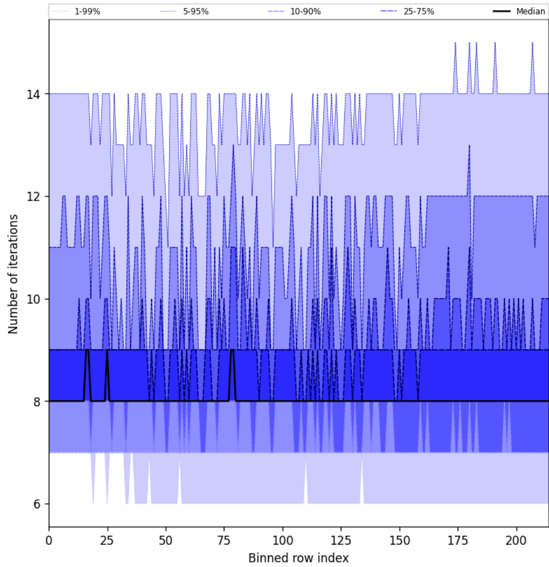
Figure 32: Along track statistics of “Number of iterations” for 2025-10-01 to 2025-10-02
