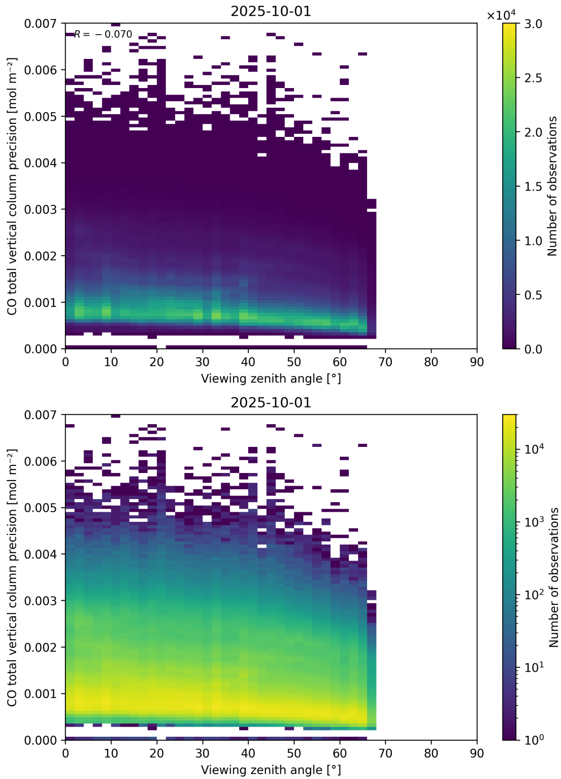
Figure 71: Scatter density plot of “Viewing zenith angle” against “CO total vertical column precision” for 2025-10-01 to 2025-10-02.
