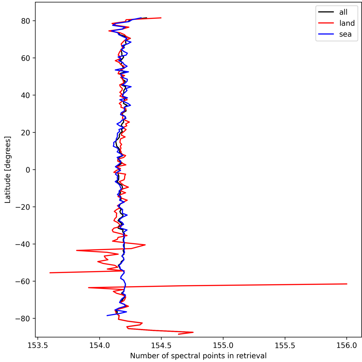
Figure 13: Zonal average of “Number of spectral points in retrieval” for 2025-10-01 to 2025-10-02.
