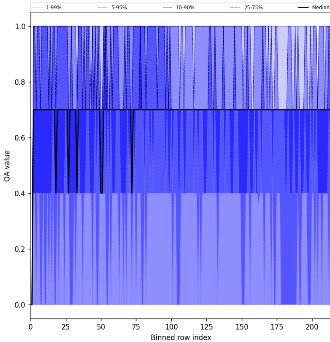
Figure 25: Along track statistics of “QA value” for 2025-10-01 to 2025-10-02
