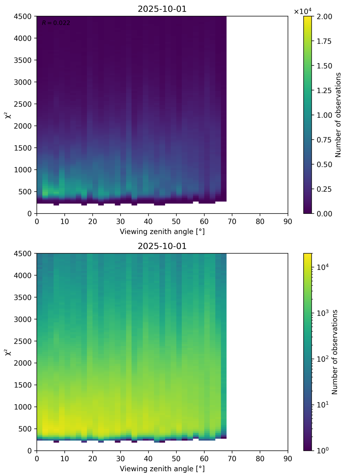
Figure 72: Scatter density plot of “Viewing zenith angle” against “ \chi^2 ” for 2025-10-01 to 2025-10-02.
