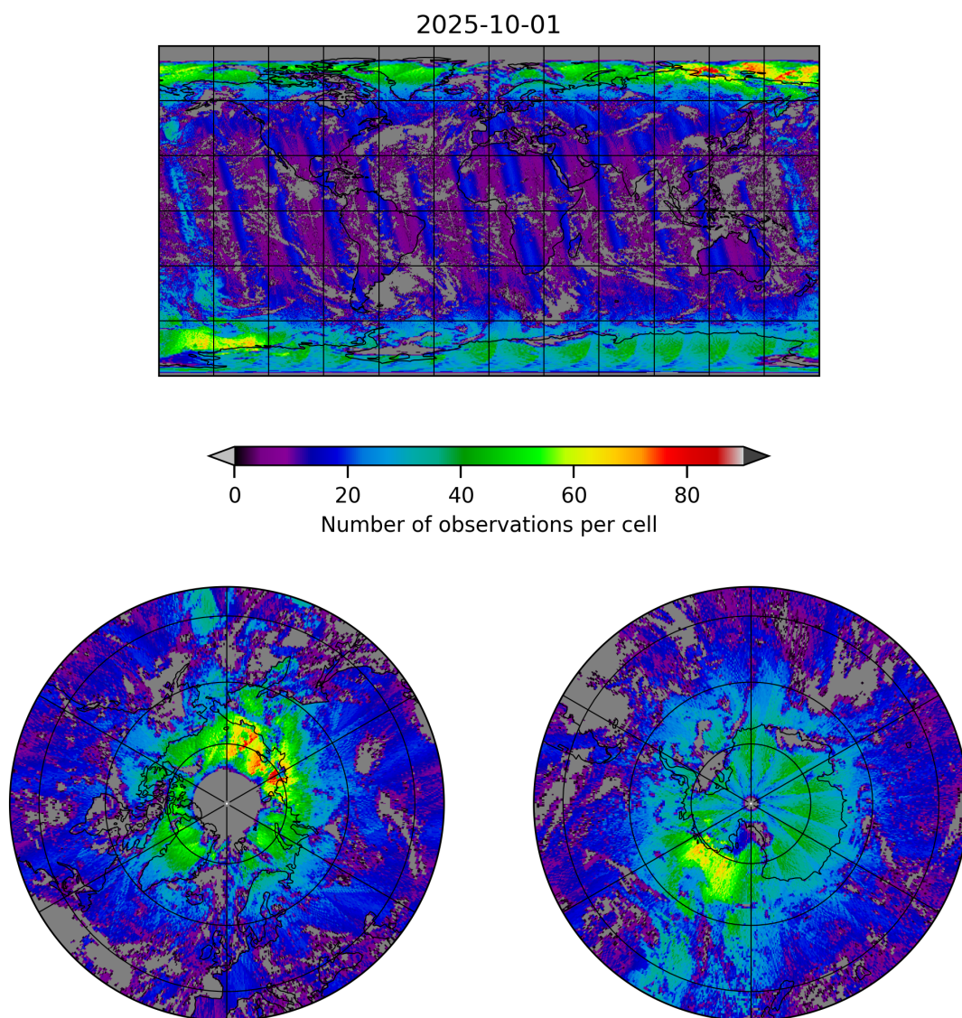
Figure 8: Map of the number of observations for 2025-10-01 to 2025-10-02
