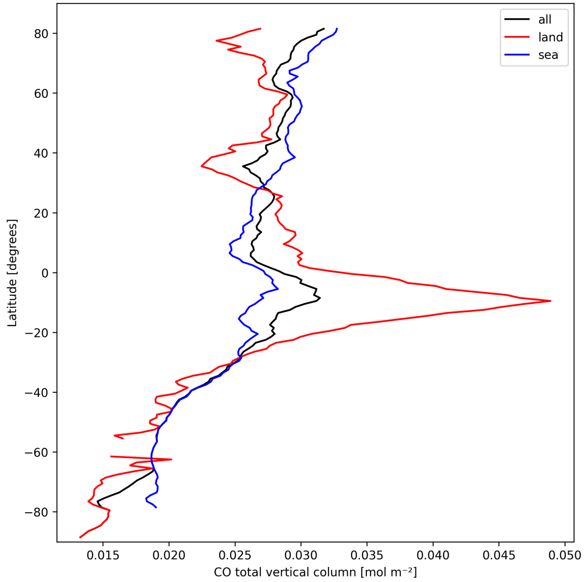
Figure 10: Zonal average of “CO total vertical column” for 2025-10-01 to 2025-10-02.
