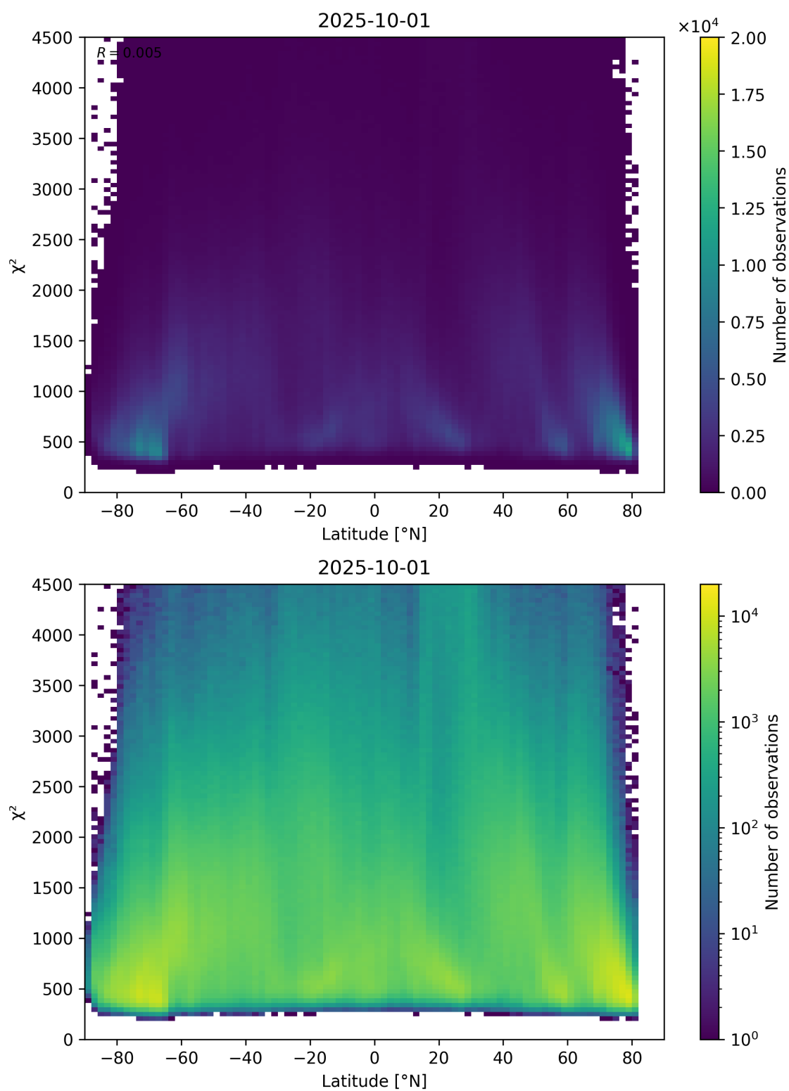
Figure 54: Scatter density plot of “Latitude” against “ \chi^2 ” for 2025-10-01 to 2025-10-02.
