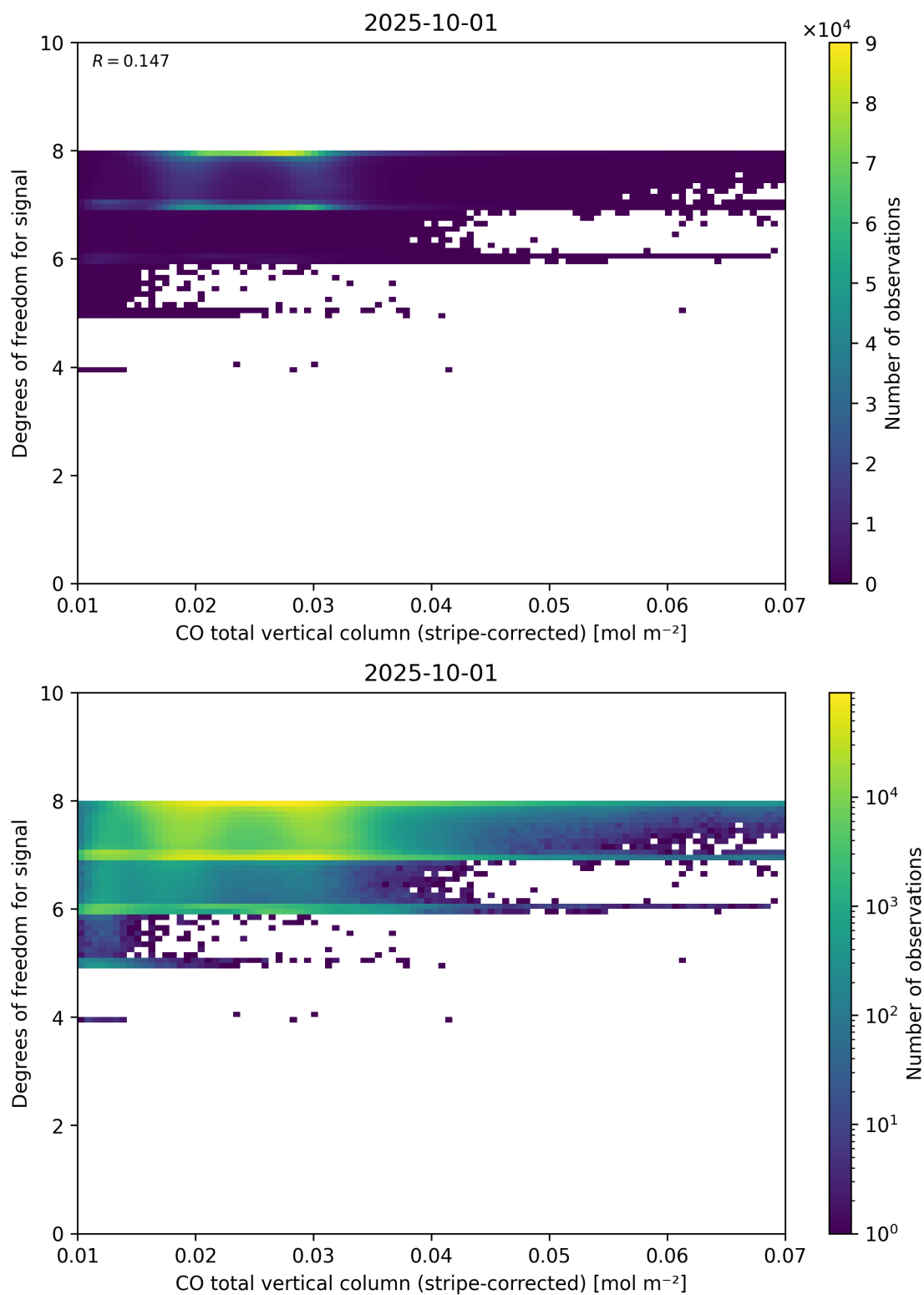
Figure 38: Scatter density plot of “CO total vertical column (stripe-corrected)” against “Degrees of freedom for signal” for 2025-10-01 to 2025-10-02.
