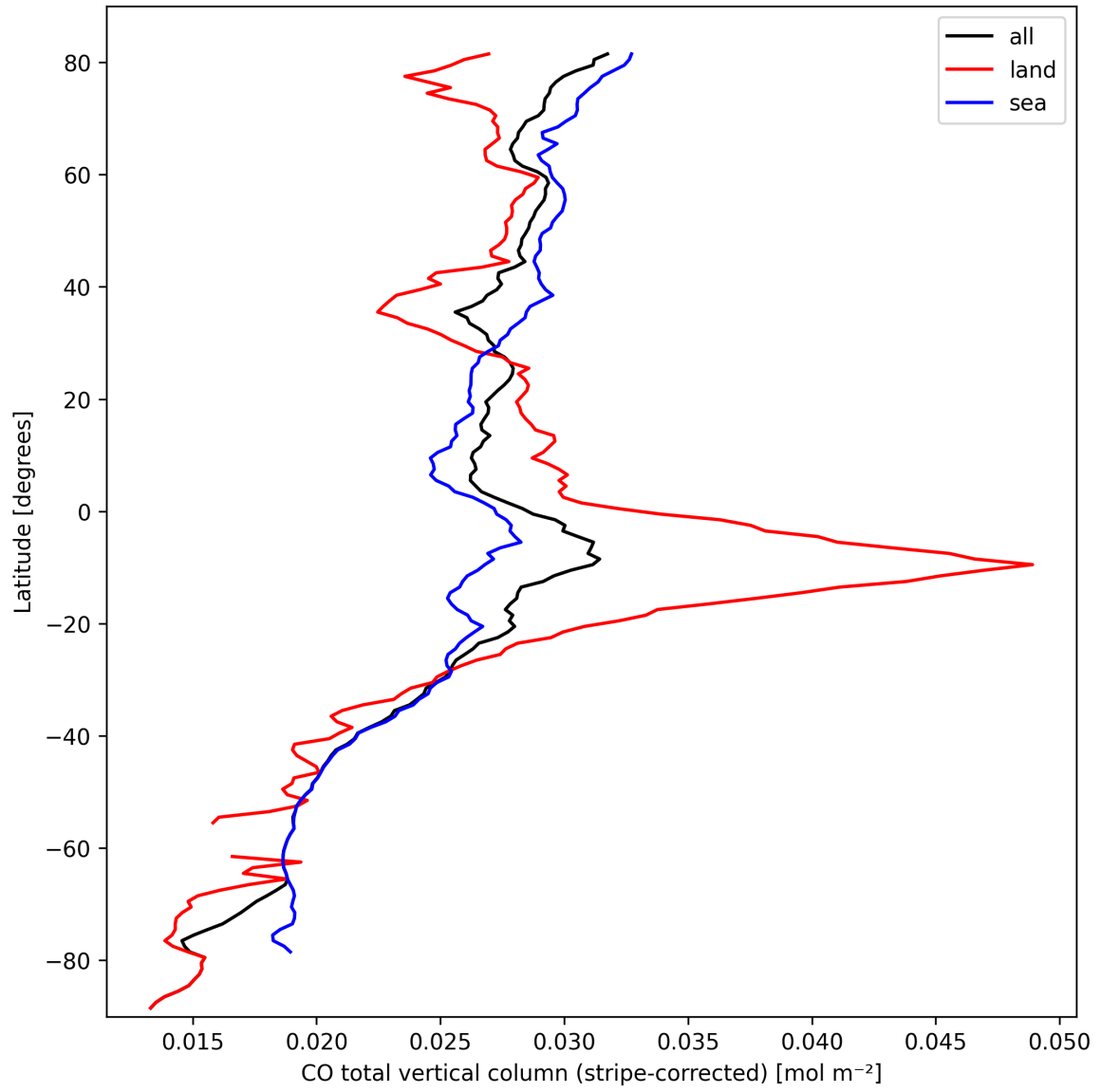
Figure 11: Zonal average of “CO total vertical column (stripe-corrected)” for 2025-10-01 to 2025-10-02.
