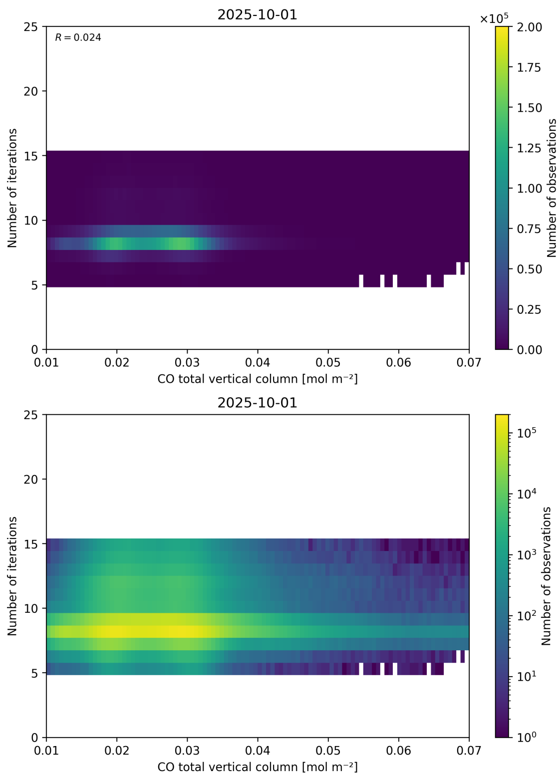
Figure 42: Scatter density plot of “CO total vertical column” against “Number of iterations” for 2025-10-01 to 2025-10-02.
