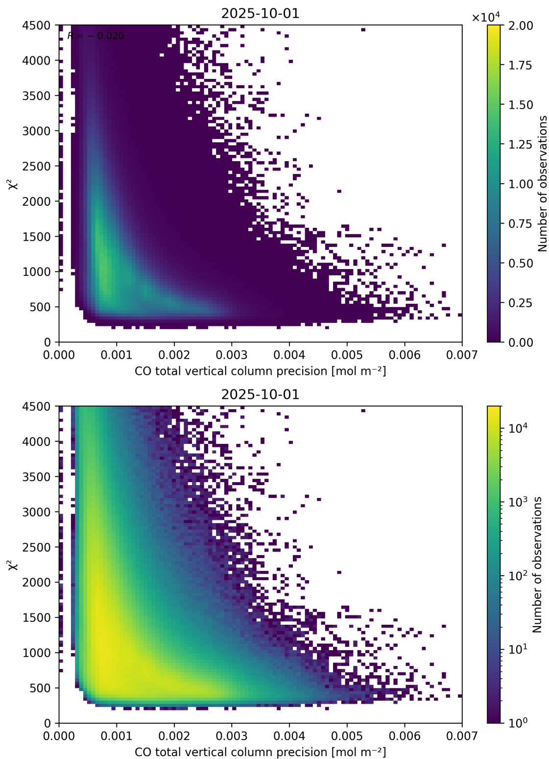
Figure 44: Scatter density plot of “CO total vertical column precision” against “ \chi^2 ” for 2025-10-01 to 2025-10-02.
