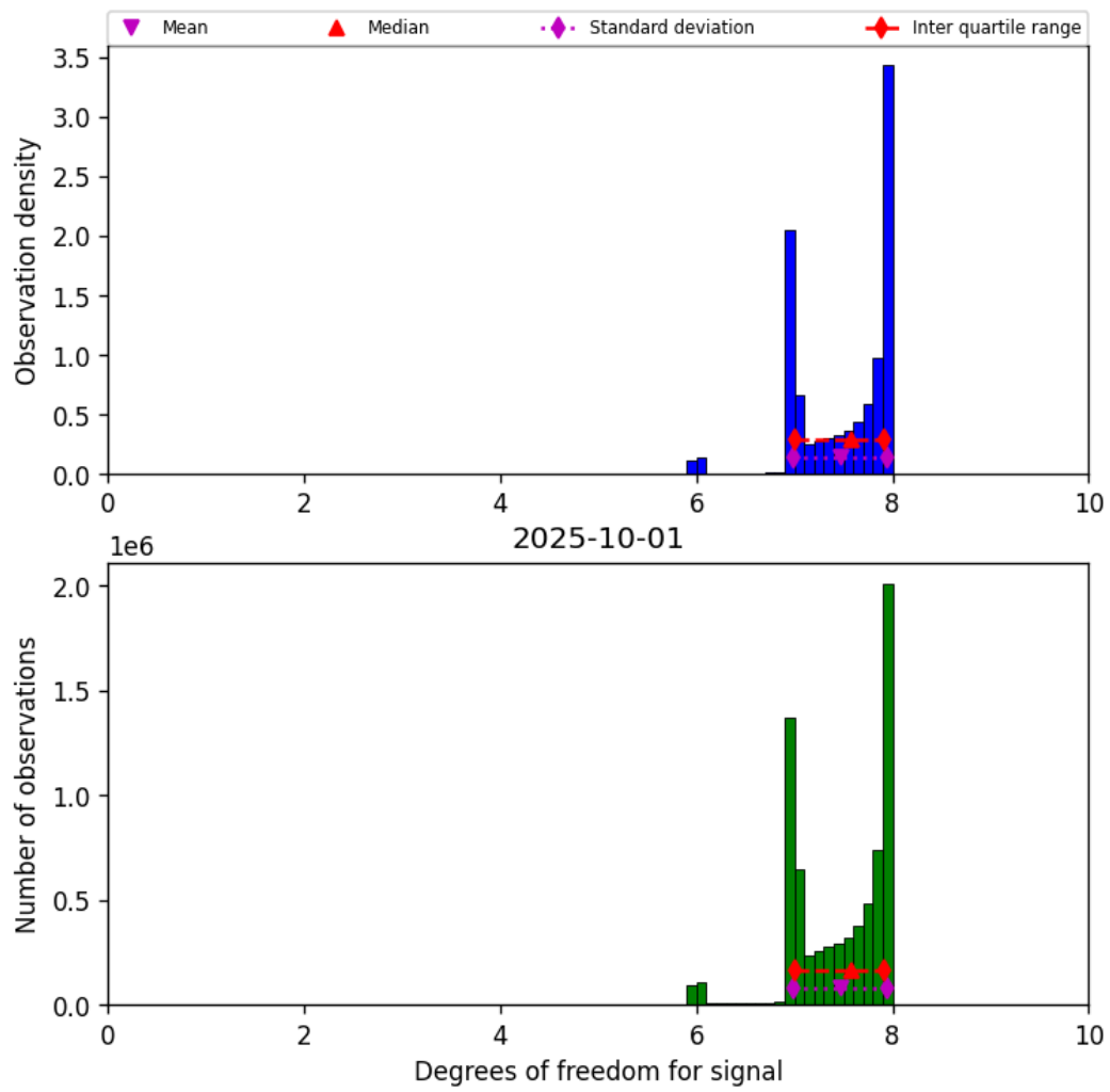
Figure 23: Histogram of “Degrees of freedom for signal” for 2025-10-01 to 2025-10-02
