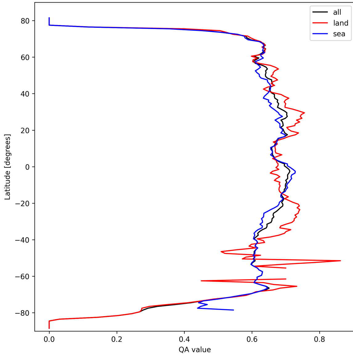
Figure 9: Zonal average of “QA value” for 2025-10-01 to 2025-10-02.
