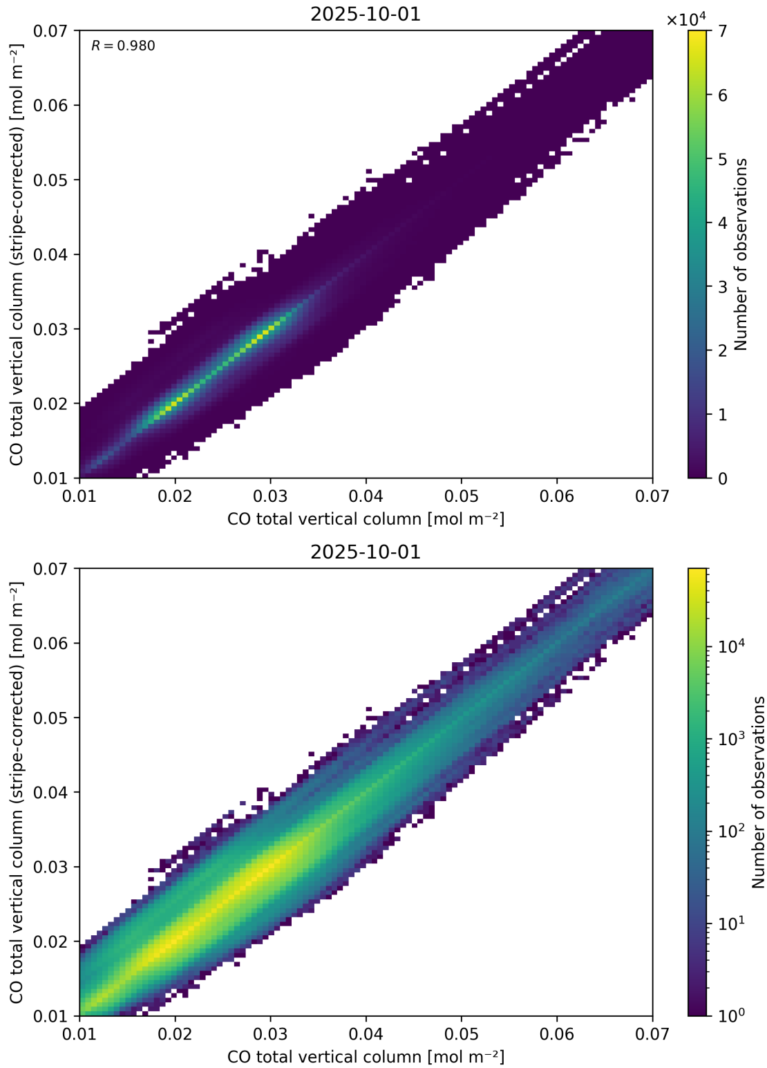
Figure 33: Scatter density plot of “CO total vertical column” against “CO total vertical column (stripe-corrected)” for 2025-10-01 to 2025-10-02.
