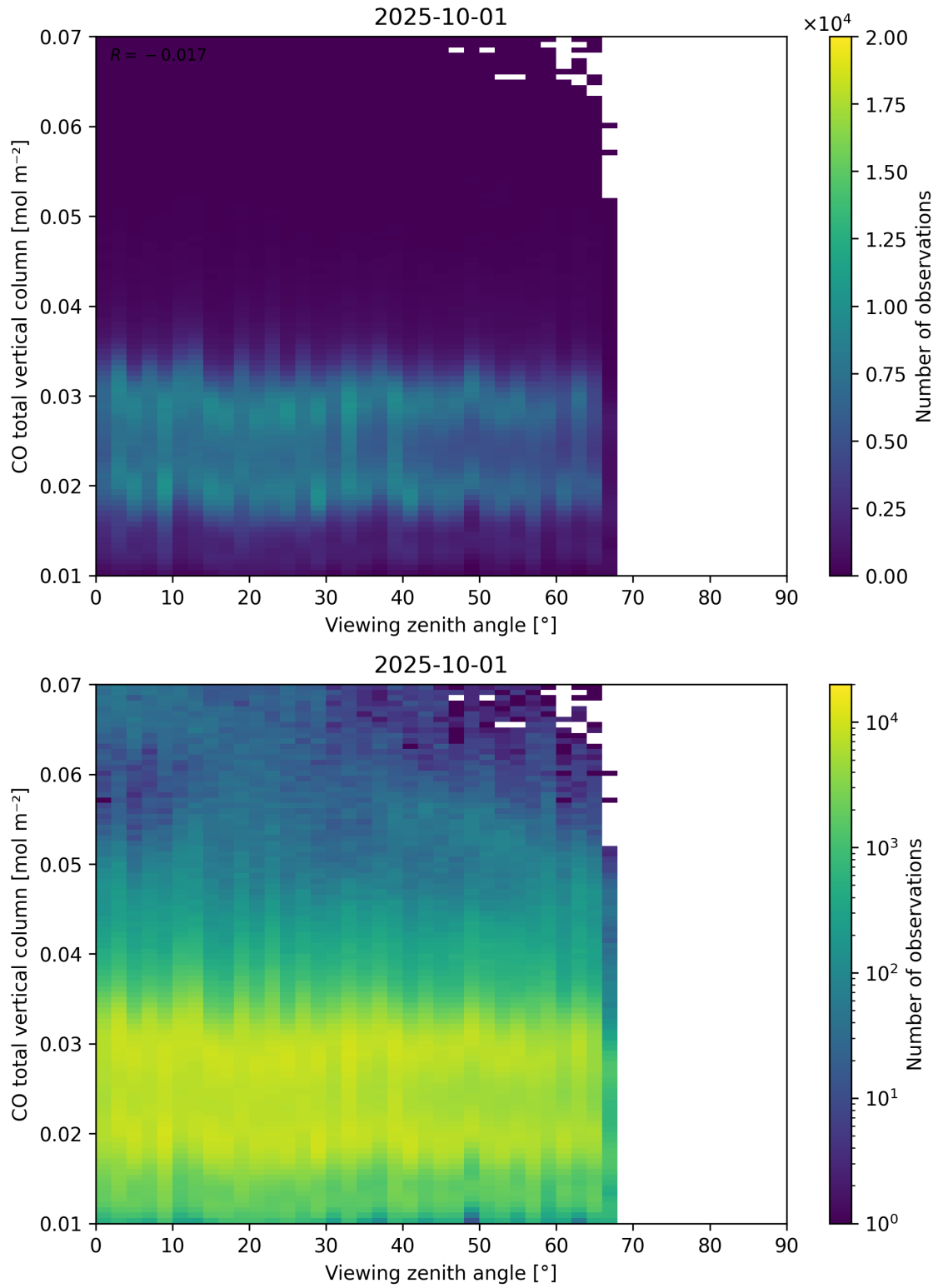
Figure 69: Scatter density plot of “Viewing zenith angle” against “CO total vertical column” for 2025-10-01 to 2025-10-02.
