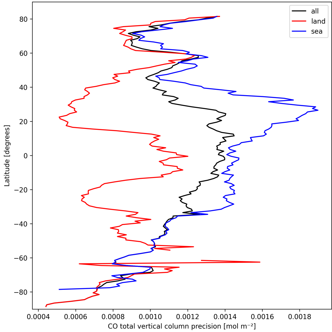
Figure 12: Zonal average of "CO total vertical column precision" for 2025-10-01 to 2025-10-02.
