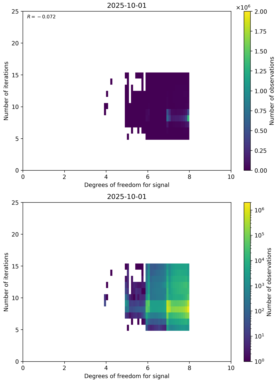
Figure 50: Scatter density plot of “Degrees of freedom for signal” against “Number of iterations” for 2025-10-01 to 2025-10-02.
