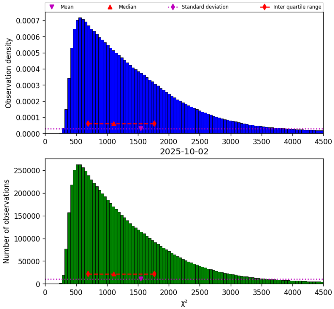
Figure 22: Histogram of “ \chi^2 ” for 2025-10-01 to 2025-10-03
