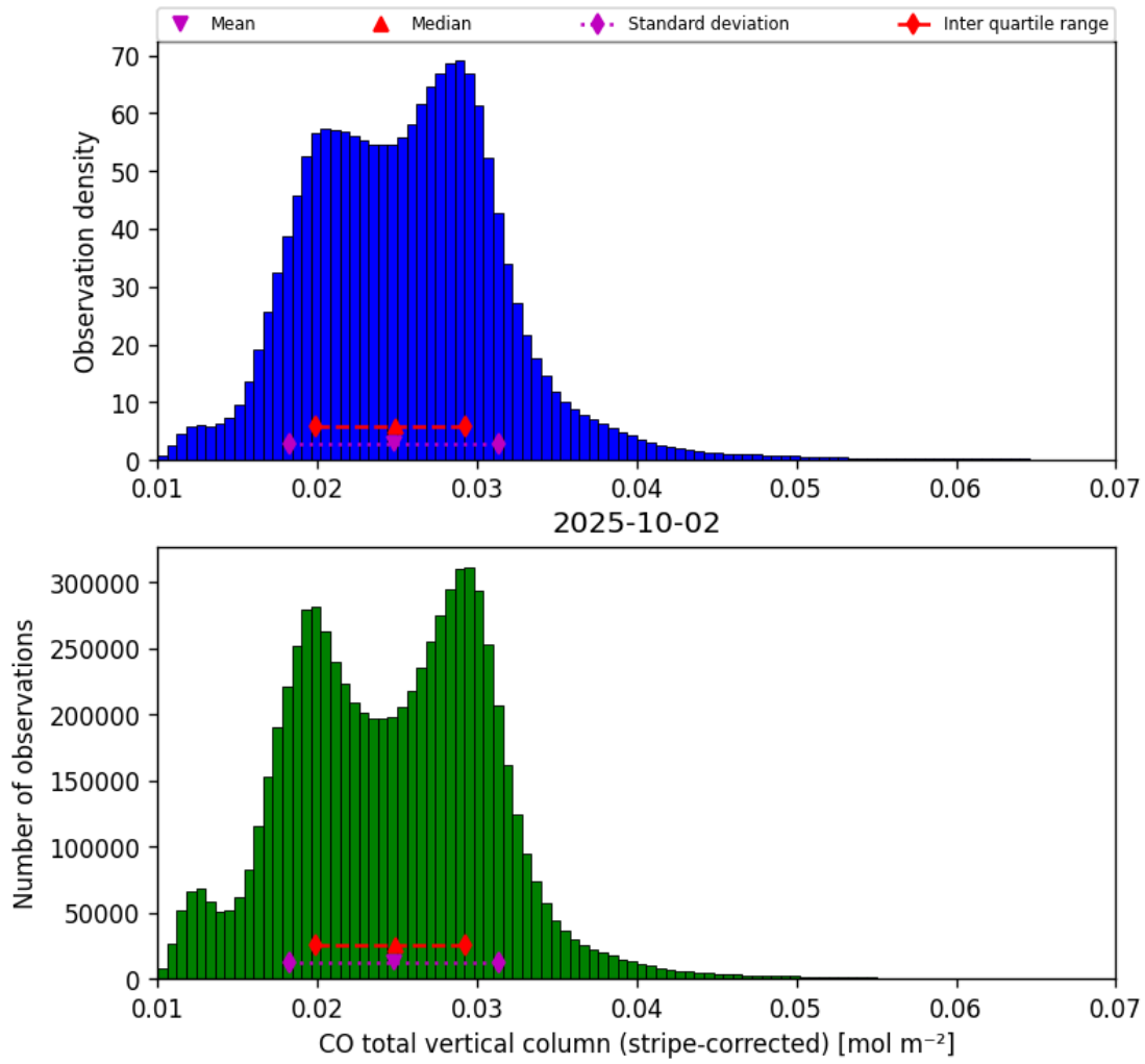
Figure 19: Histogram of “CO total vertical column (stripe-corrected)” for 2025-10-01 to 2025-10-03
