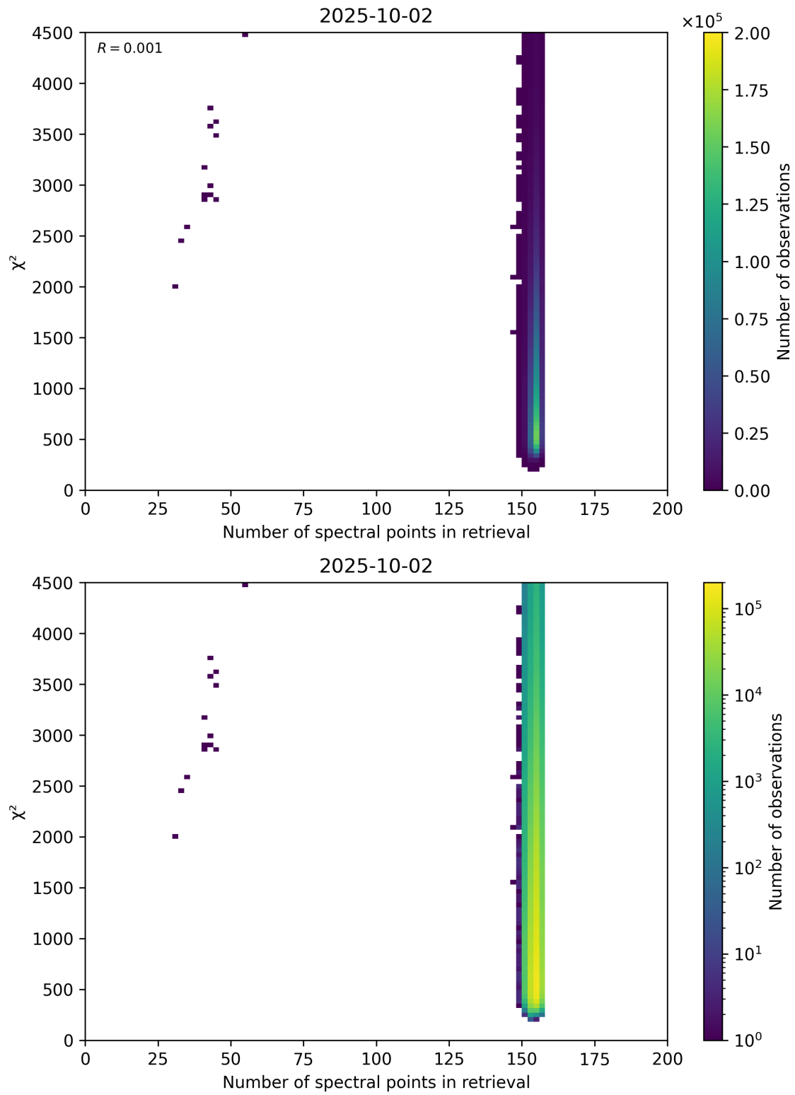
Figure 58: Scatter density plot of “Number of spectral points in retrieval” against “ \chi^2 ” for 2025-10-01 to 2025-10-03.
