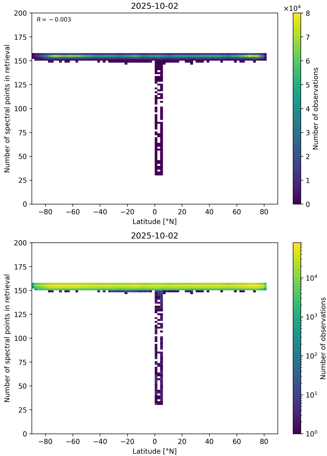
Figure 57: Scatter density plot of “Latitude” against “Number of spectral points in retrieval” for 2025-10-01 to 2025-10-03.
