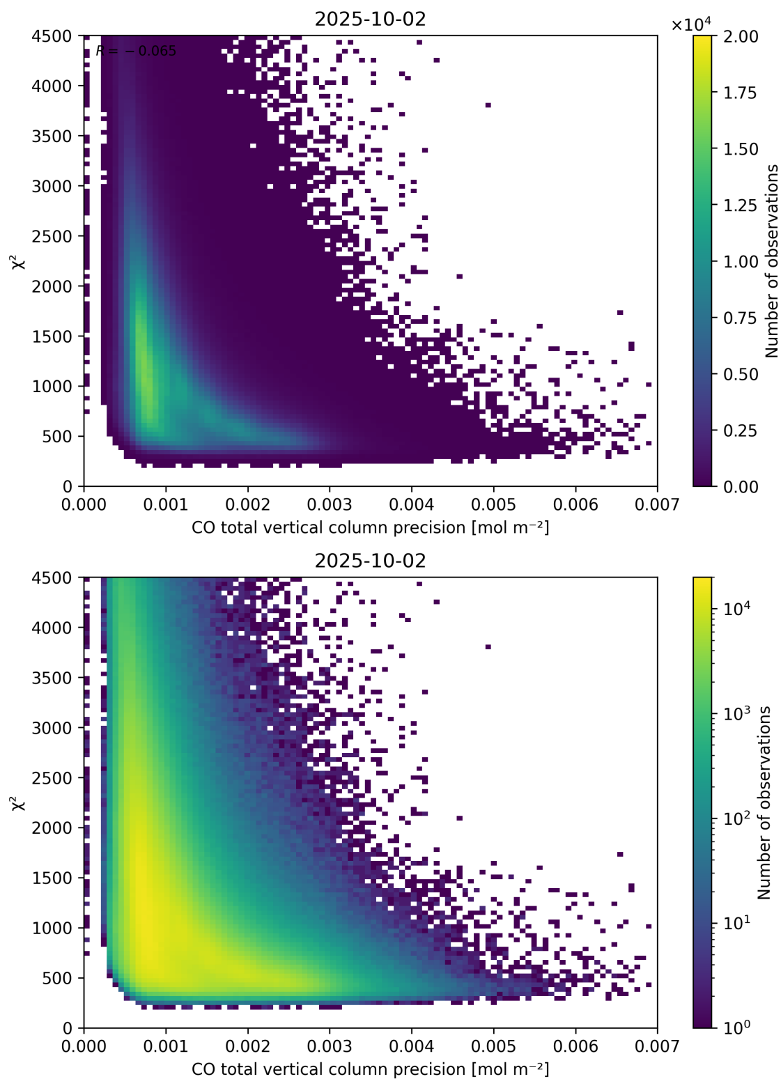
Figure 44: Scatter density plot of “CO total vertical column precision” against “ \chi^2 ” for 2025-10-01 to 2025-10-03.
