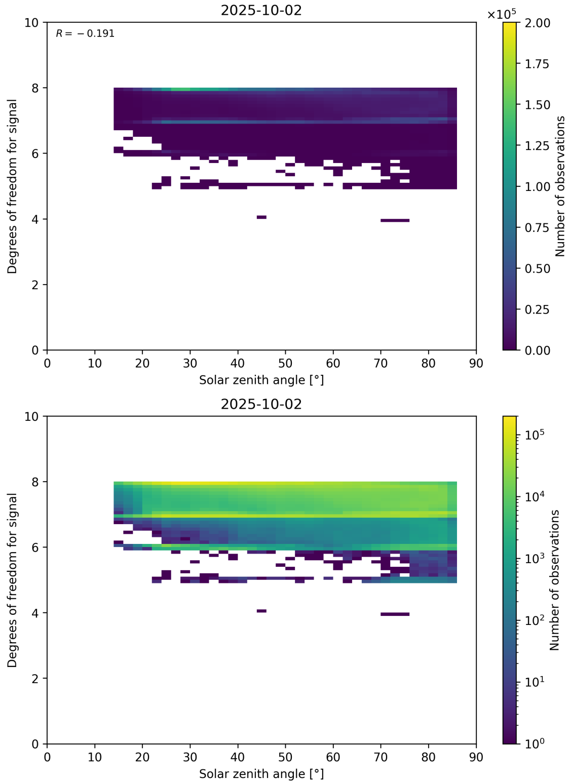
Figure 65: Scatter density plot of “Solar zenith angle” against “Degrees of freedom for signal” for 2025-10-01 to 2025-10-03.
