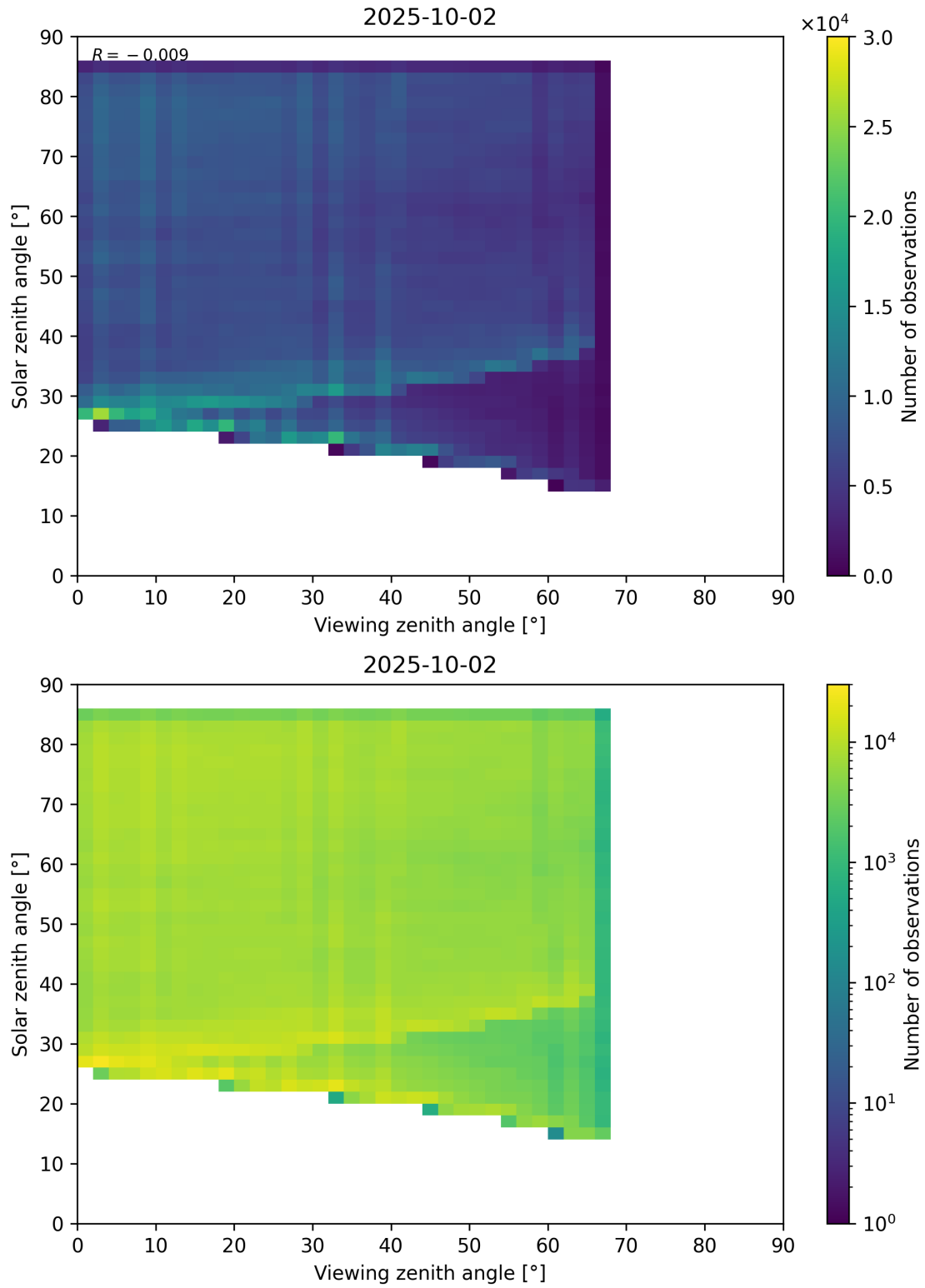
Figure 77: Scatter density plot of “Viewing zenith angle” against “Solar zenith angle” for 2025-10-01 to 2025-10-03.
