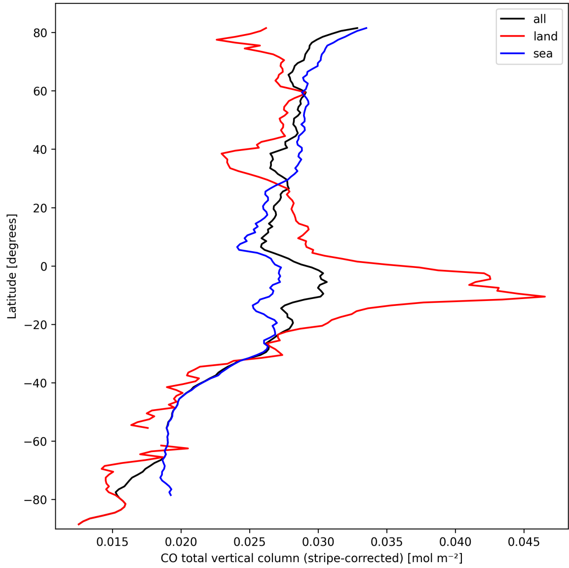
Figure 11: Zonal average of “CO total vertical column (stripe-corrected)” for 2025-10-01 to 2025-10-03.
