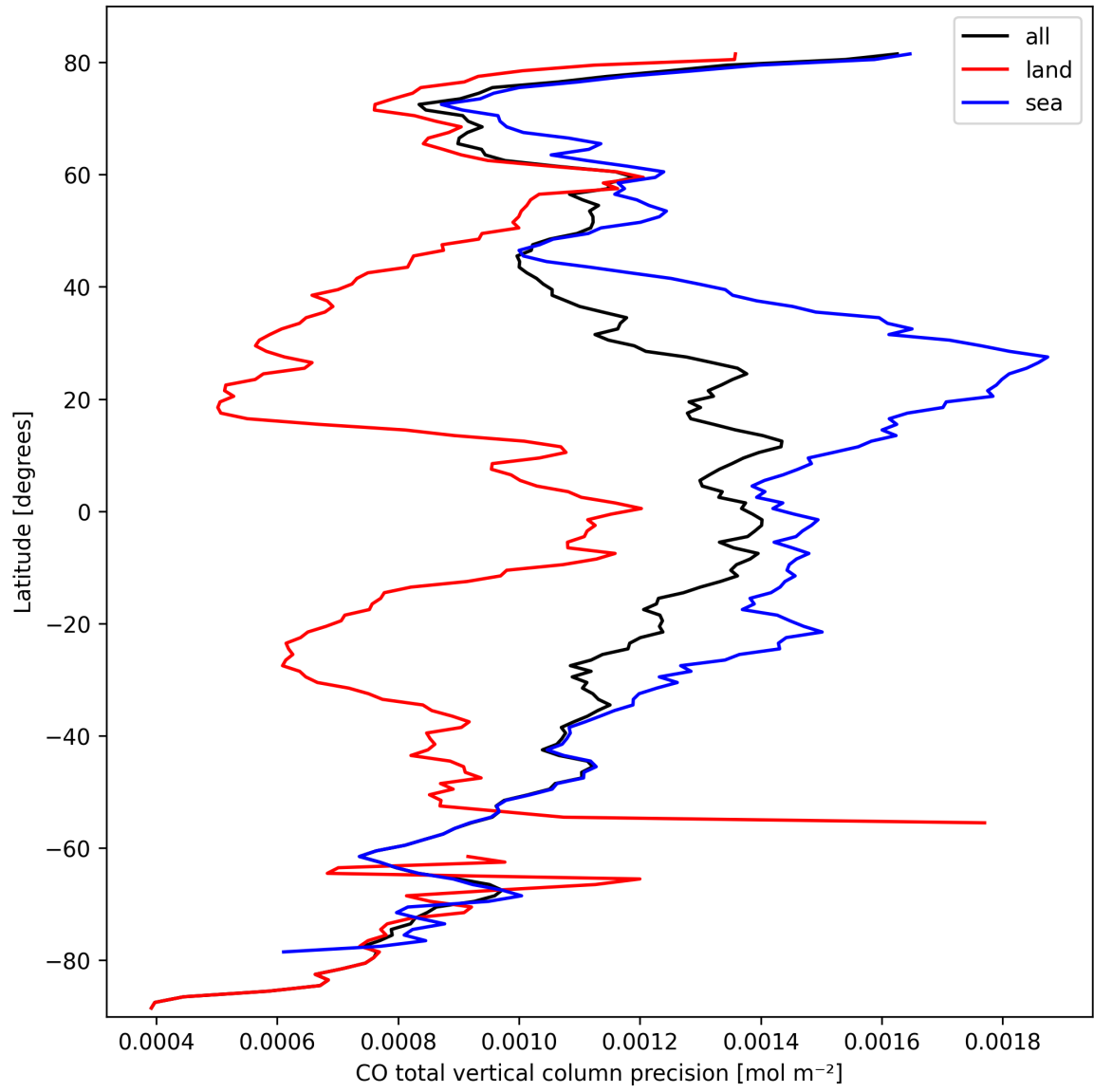
Figure 12: Zonal average of “CO total vertical column precision” for 2025-10-01 to 2025-10-03.
