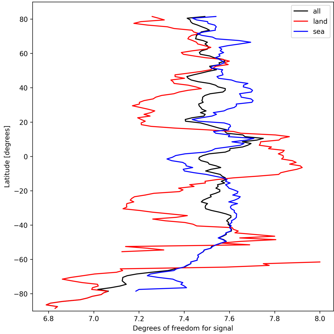
Figure 15: Zonal average of “Degrees of freedom for signal” for 2025-10-01 to 2025-10-03.
