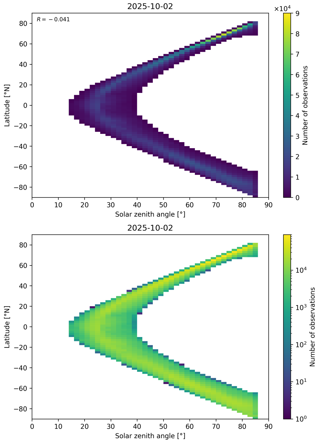
Figure 66: Scatter density plot of “Solar zenith angle” against “Latitude” for 2025-10-01 to 2025-10-03.
