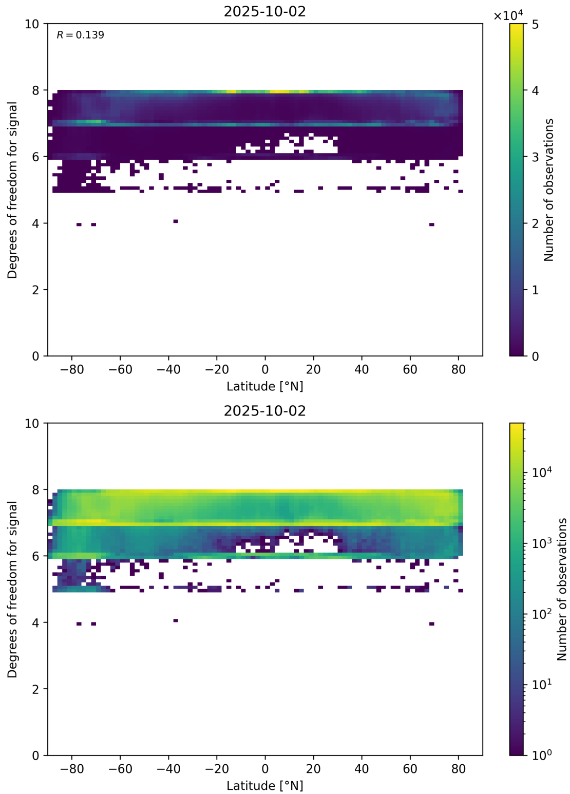
Figure 55: Scatter density plot of “Latitude” against “Degrees of freedom for signal” for 2025-10-01 to 2025-10-03.
