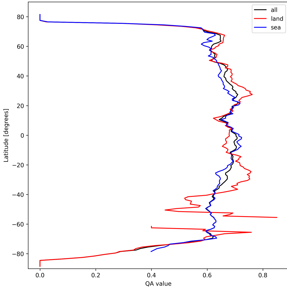
Figure 9: Zonal average of “QA value” for 2025-10-01 to 2025-10-03.
