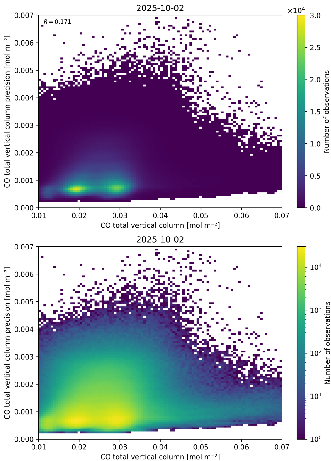
Figure 34: Scatter density plot of “CO total vertical column” against “CO total vertical column precision” for 2025-10-01 to 2025-10-03.
