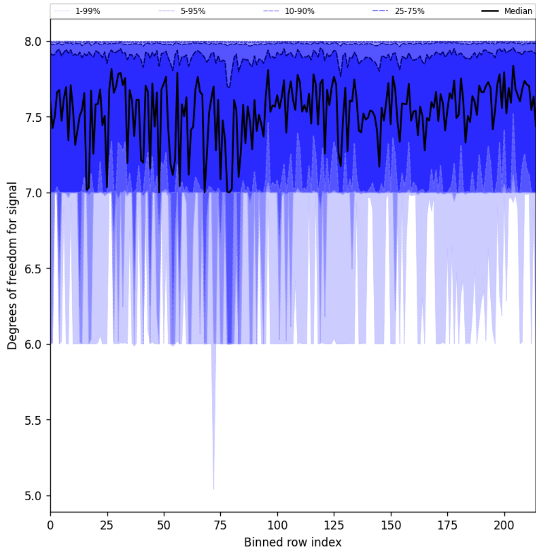
Figure 31: Along track statistics of “Degrees of freedom for signal” for 2025-10-01 to 2025-10-03
