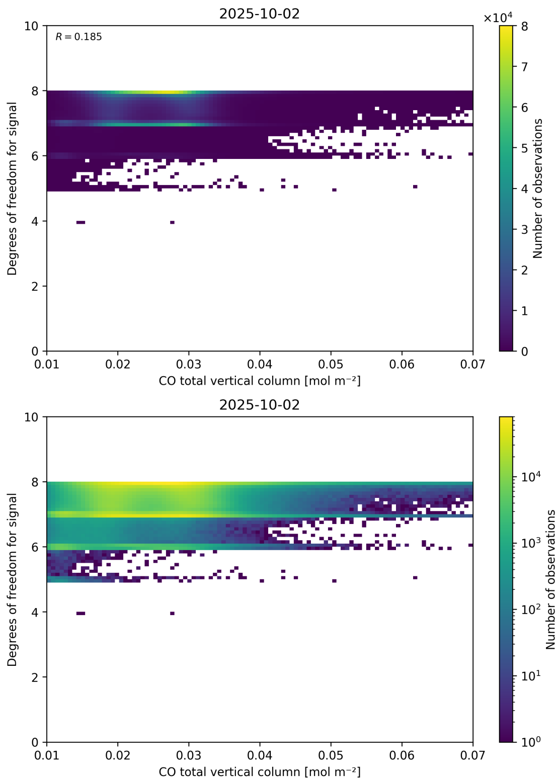
Figure 41: Scatter density plot of “CO total vertical column” against “Degrees of freedom for signal” for 2025-10-01 to 2025-10-03.
