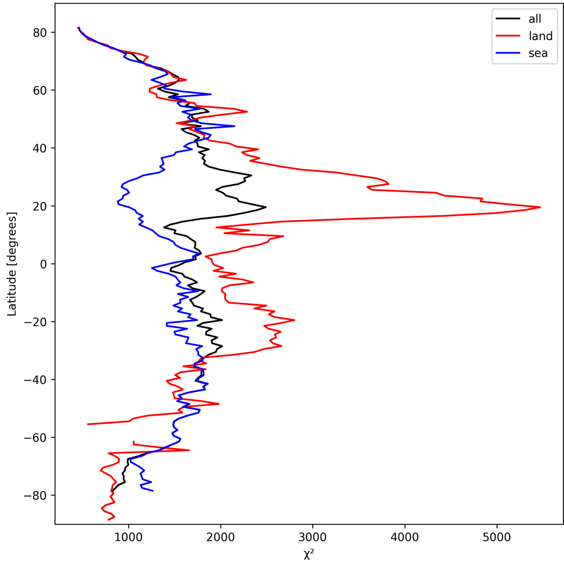
Figure 14: Zonal average of “ \chi^2 ” for 2025-10-01 to 2025-10-03.
