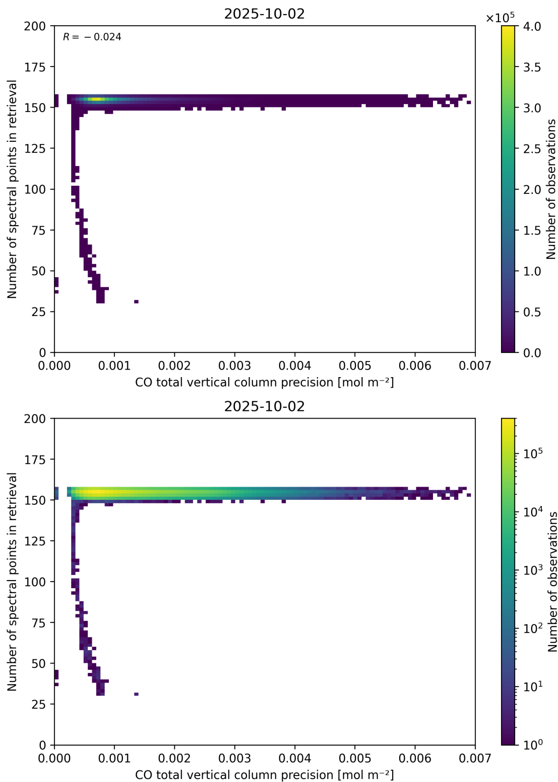
Figure 47: Scatter density plot of “CO total vertical column precision” against “Number of spectral points in retrieval” for 2025-10-01 to 2025-10-03.
