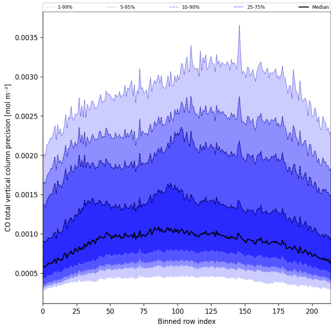
Figure 28: Along track statistics of “CO total vertical column precision” for 2025-10-01 to 2025-10-03
