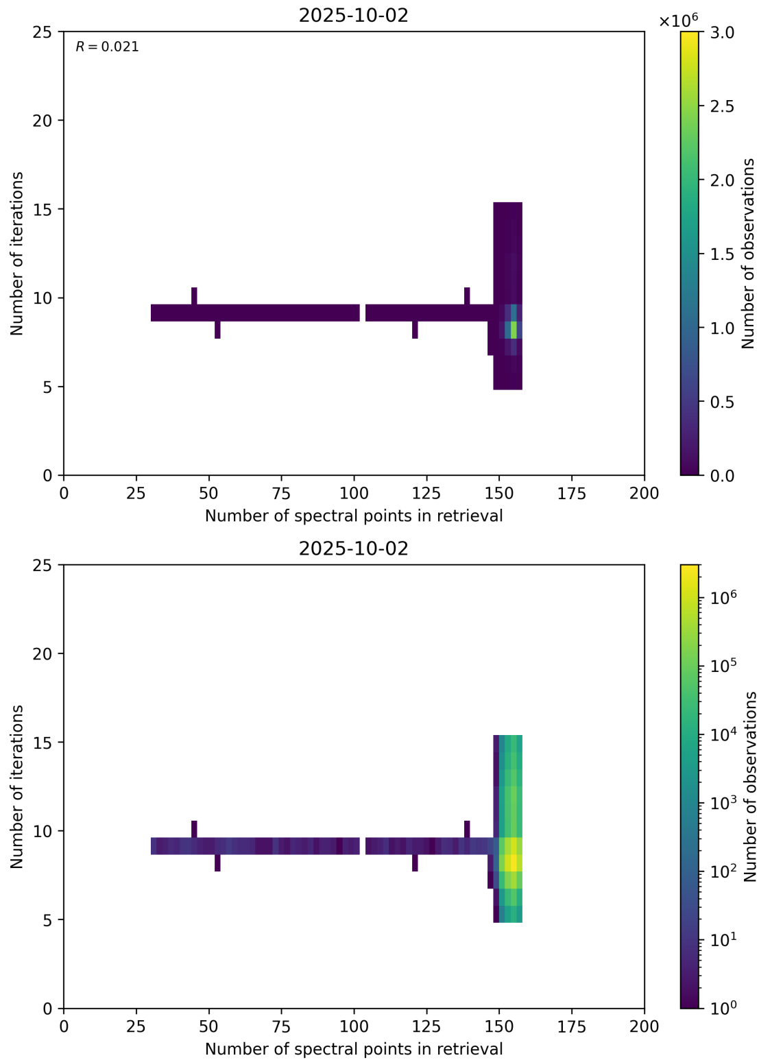
Figure 60: Scatter density plot of “Number of spectral points in retrieval” against “Number of iterations” for 2025-10-01 to 2025-10-03.
