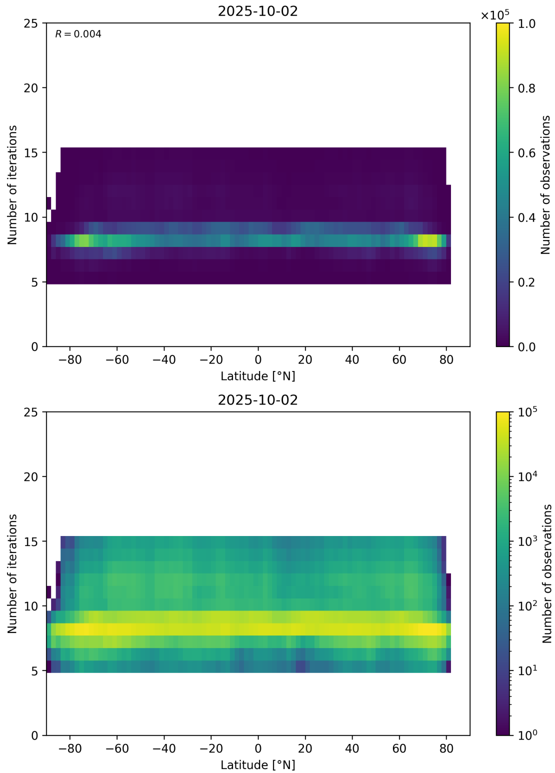
Figure 56: Scatter density plot of “Latitude” against “Number of iterations” for 2025-10-01 to 2025-10-03.
