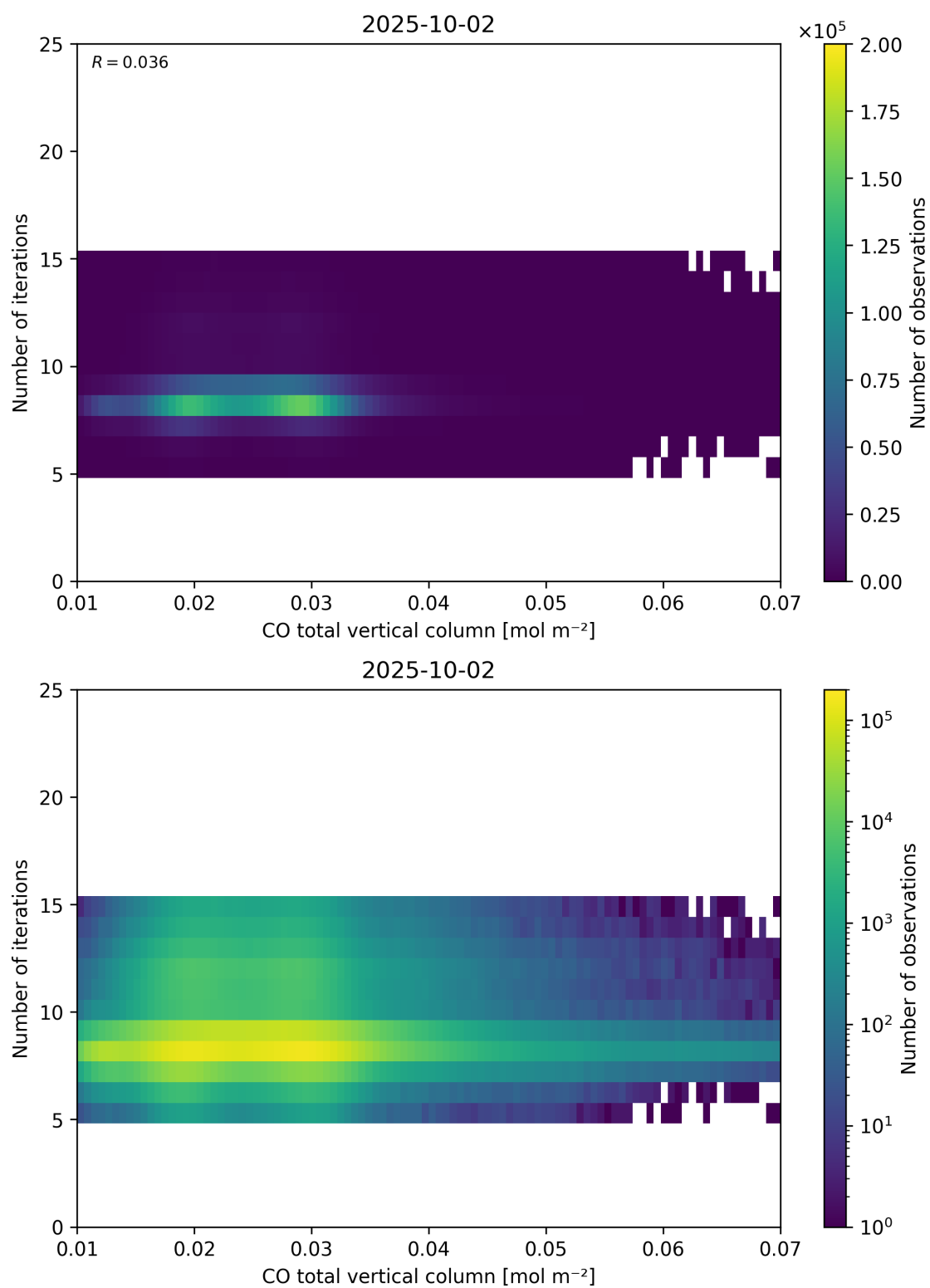
Figure 42: Scatter density plot of “CO total vertical column” against “Number of iterations” for 2025-10-01 to 2025-10-03.
