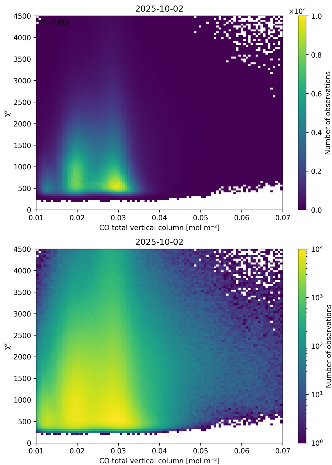
Figure 35: Scatter density plot of “CO total vertical column” against “ \chi^2 ” for 2025-10-01 to 2025-10-03.
