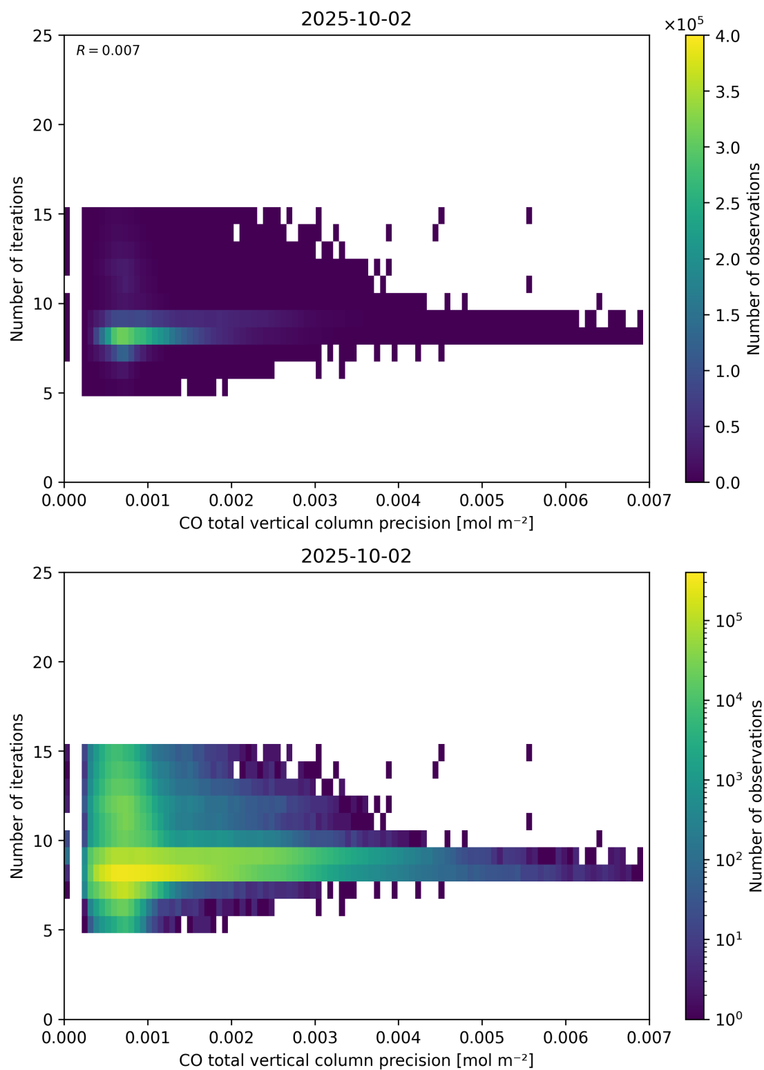
Figure 46: Scatter density plot of “CO total vertical column precision” against “Number of iterations” for 2025-10-01 to 2025-10-03.
