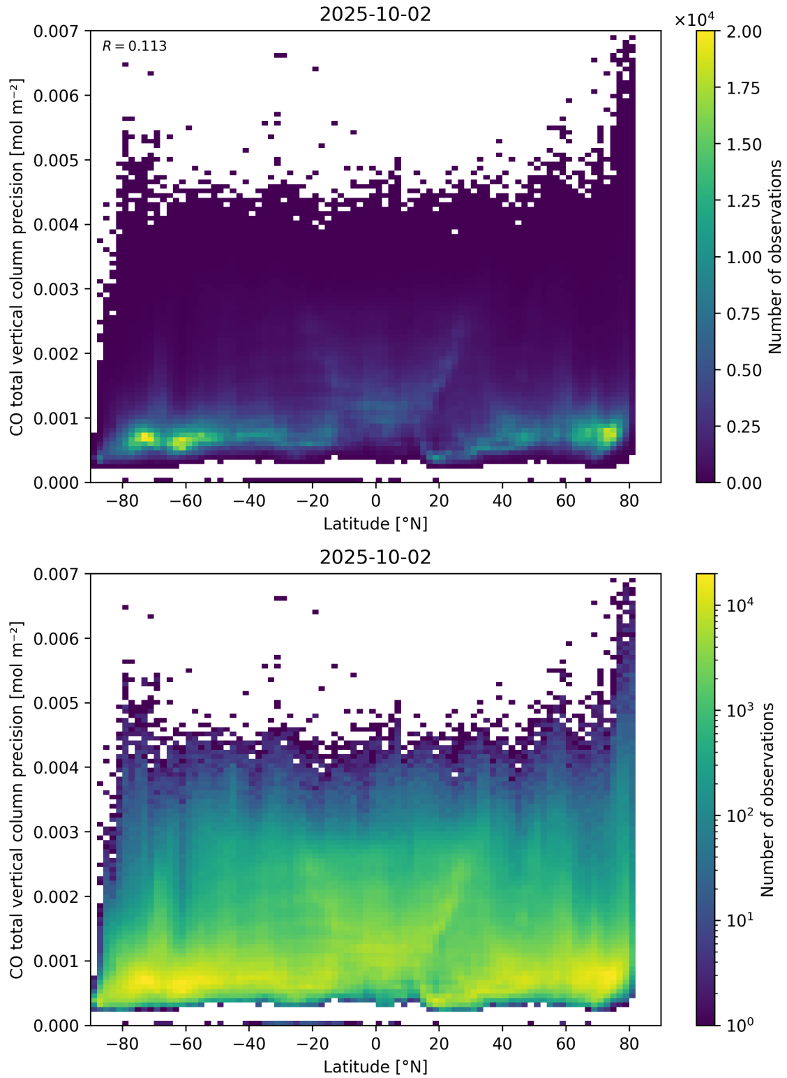
Figure 53: Scatter density plot of “Latitude” against “CO total vertical column precision” for 2025-10-01 to 2025-10-03.
