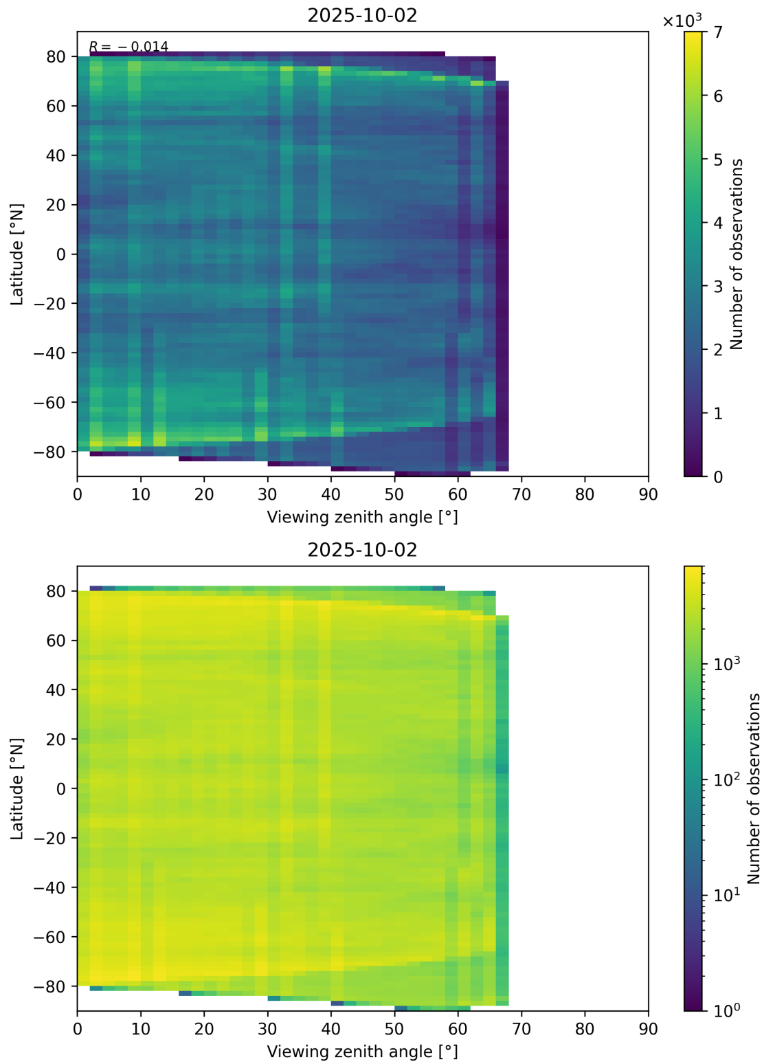
Figure 74: Scatter density plot of “Viewing zenith angle” against “Latitude” for 2025-10-01 to 2025-10-03.
