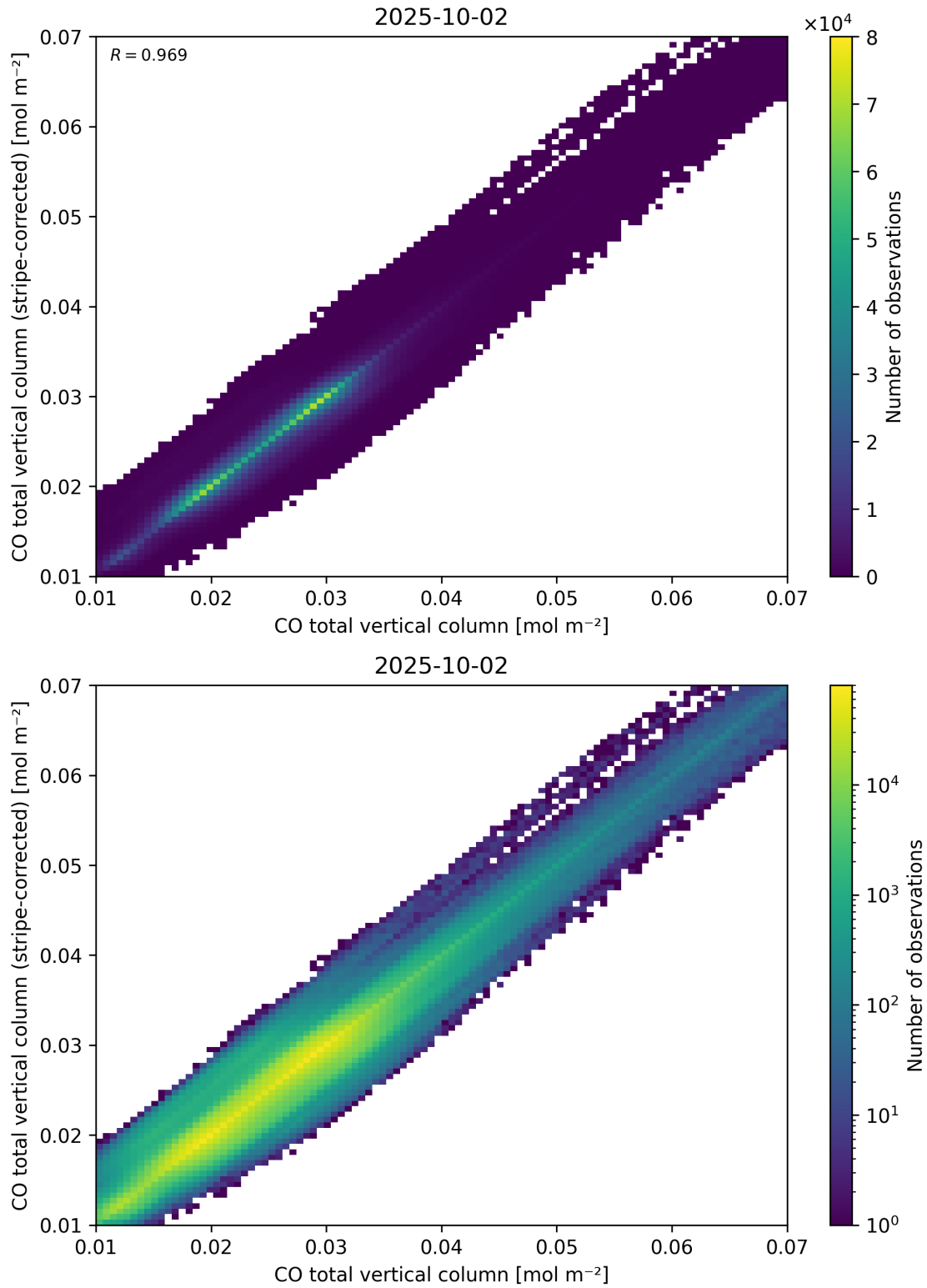
Figure 33: Scatter density plot of “CO total vertical column” against “CO total vertical column (stripe-corrected)” for 2025-10-01 to 2025-10-03.
