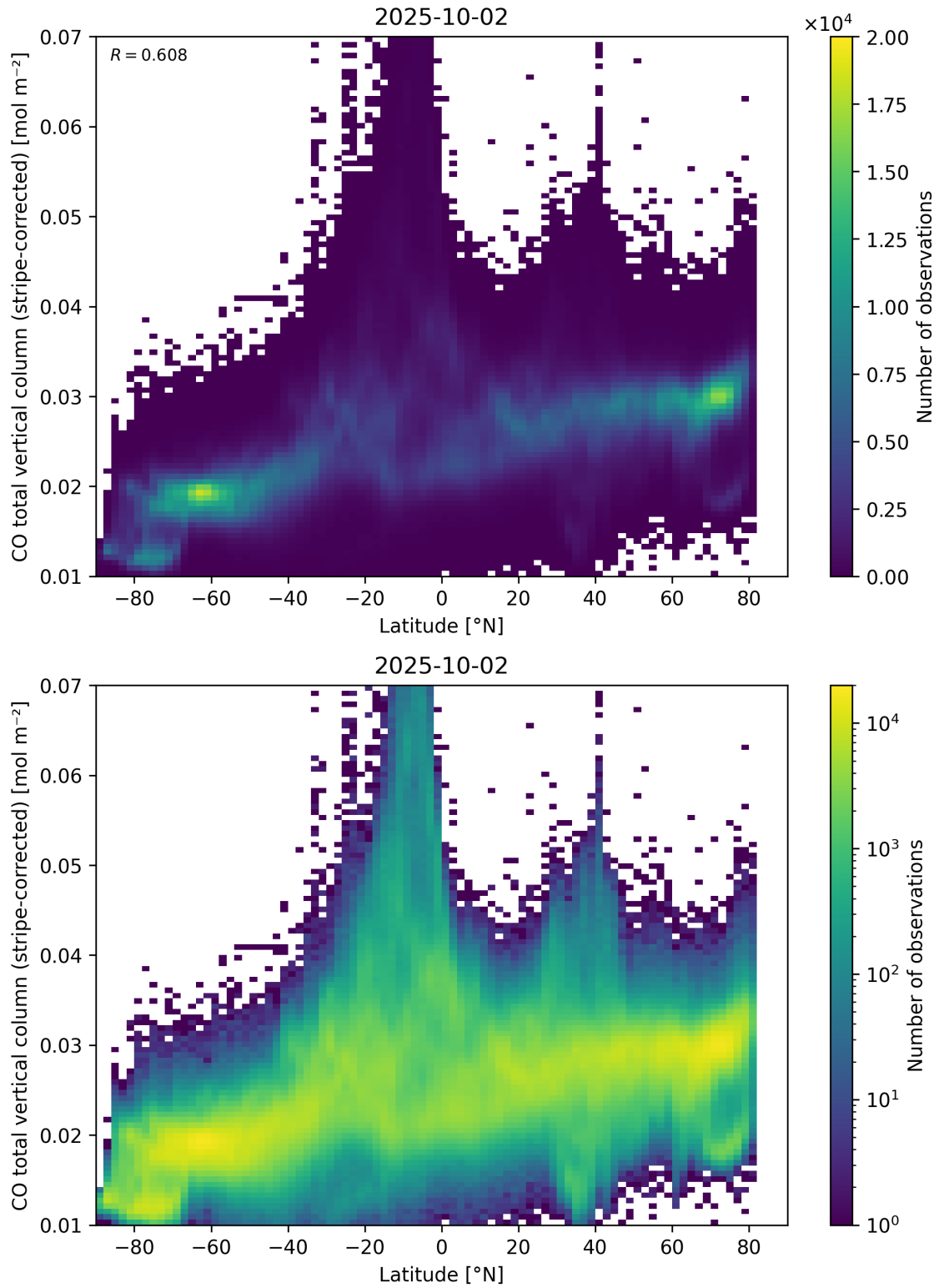
Figure 52: Scatter density plot of “Latitude” against “CO total vertical column (stripe-corrected)” for 2025-10-01 to 2025-10-03.
