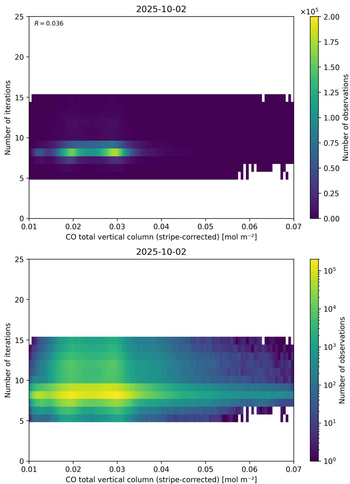
Figure 39: Scatter density plot of “CO total vertical column (stripe-corrected)” against “Number of iterations” for 2025-10-01 to 2025-10-03.
