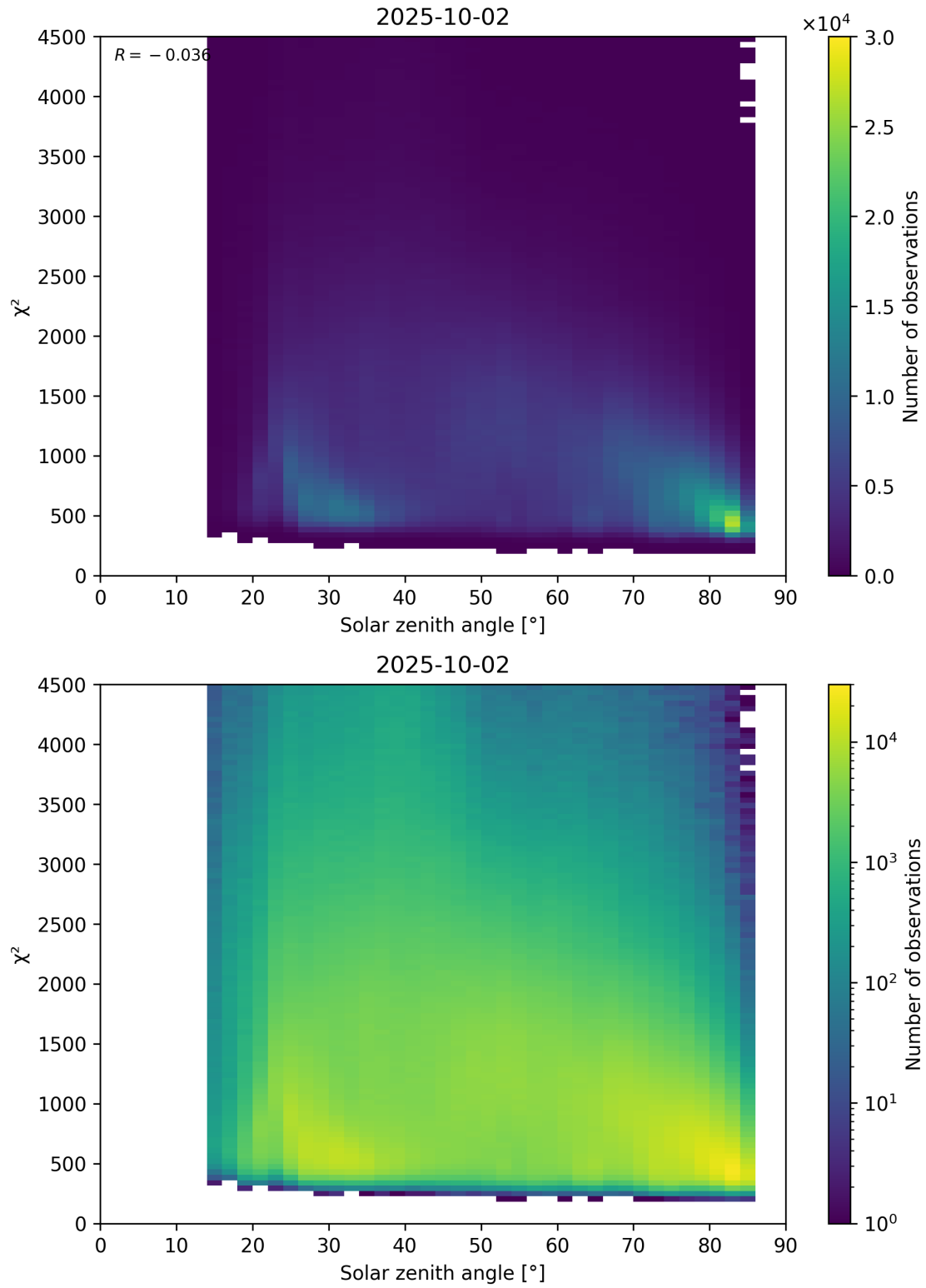
Figure 64: Scatter density plot of “Solar zenith angle” against “ \chi^2 ” for 2025-10-01 to 2025-10-03.
