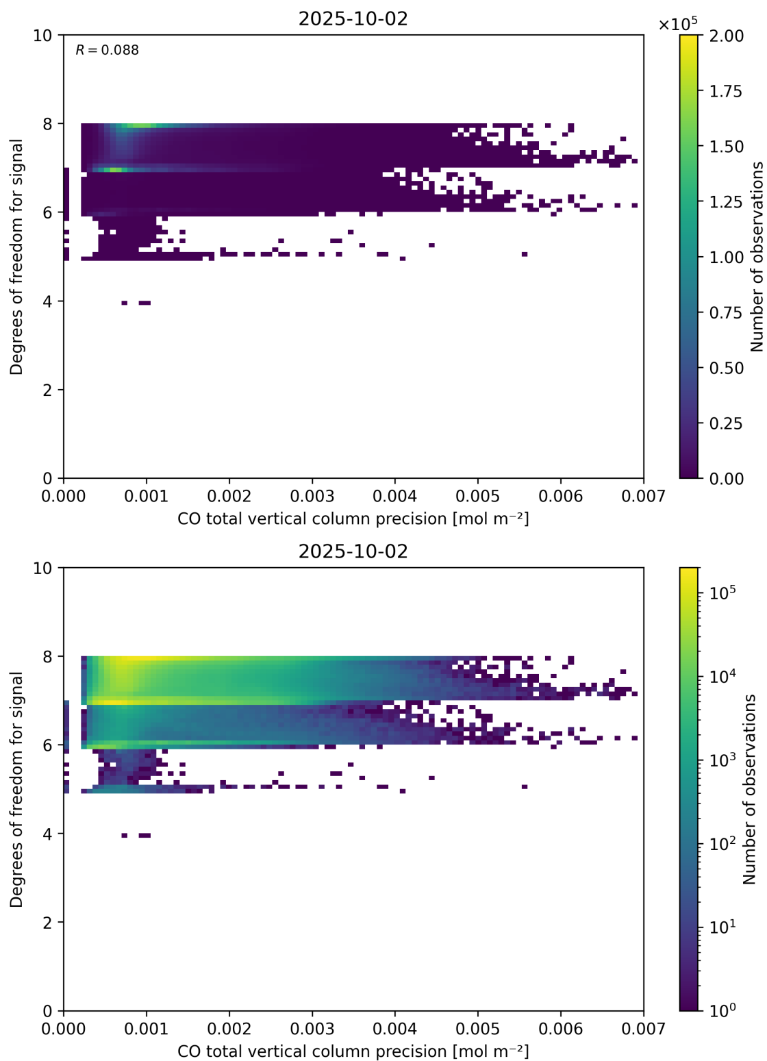
Figure 45: Scatter density plot of “CO total vertical column precision” against “Degrees of freedom for signal” for 2025-10-01 to 2025-10-03.
