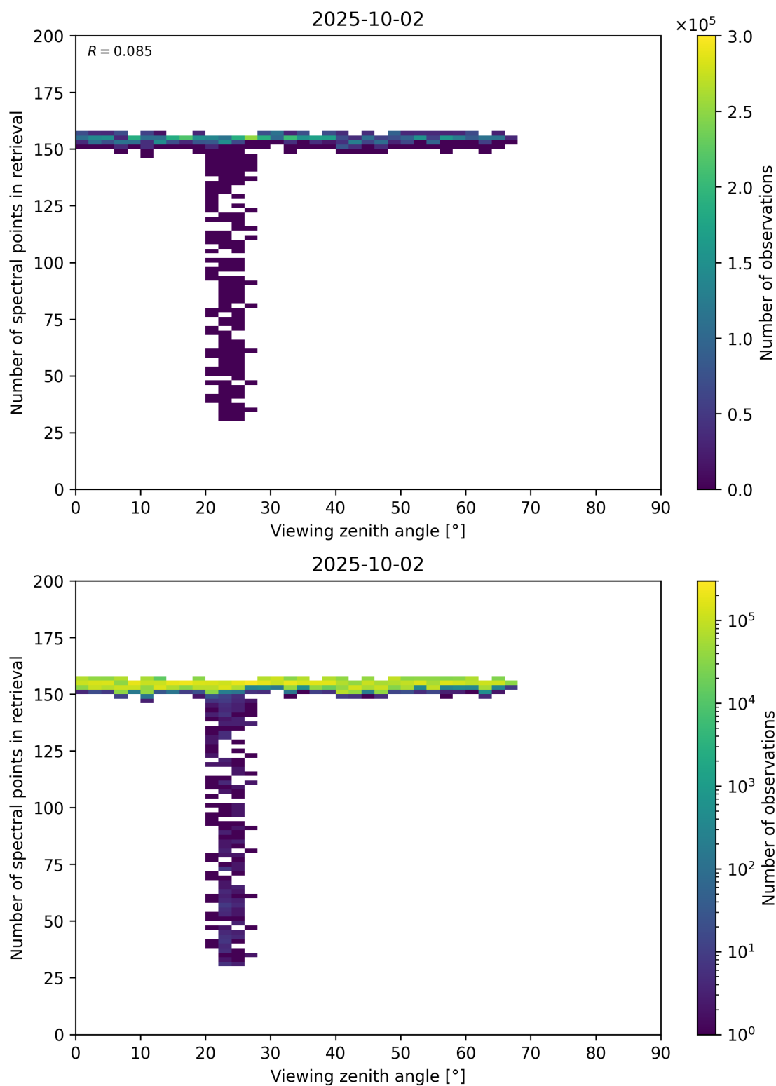
Figure 76: Scatter density plot of “Viewing zenith angle” against “Number of spectral points in retrieval” for 2025-10-01 to 2025-10-03.
