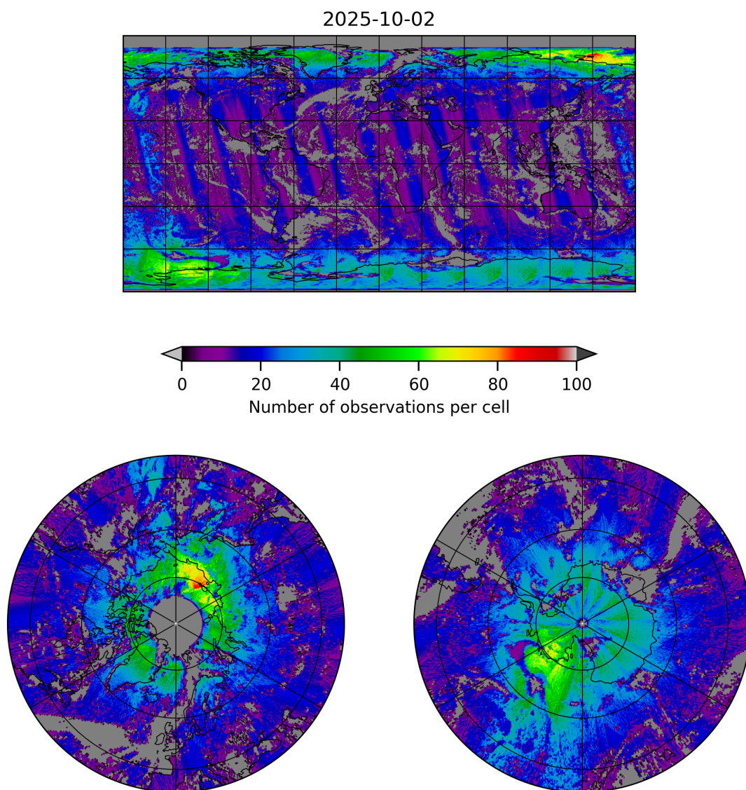
Figure 8: Map of the number of observations for 2025-10-01 to 2025-10-03
