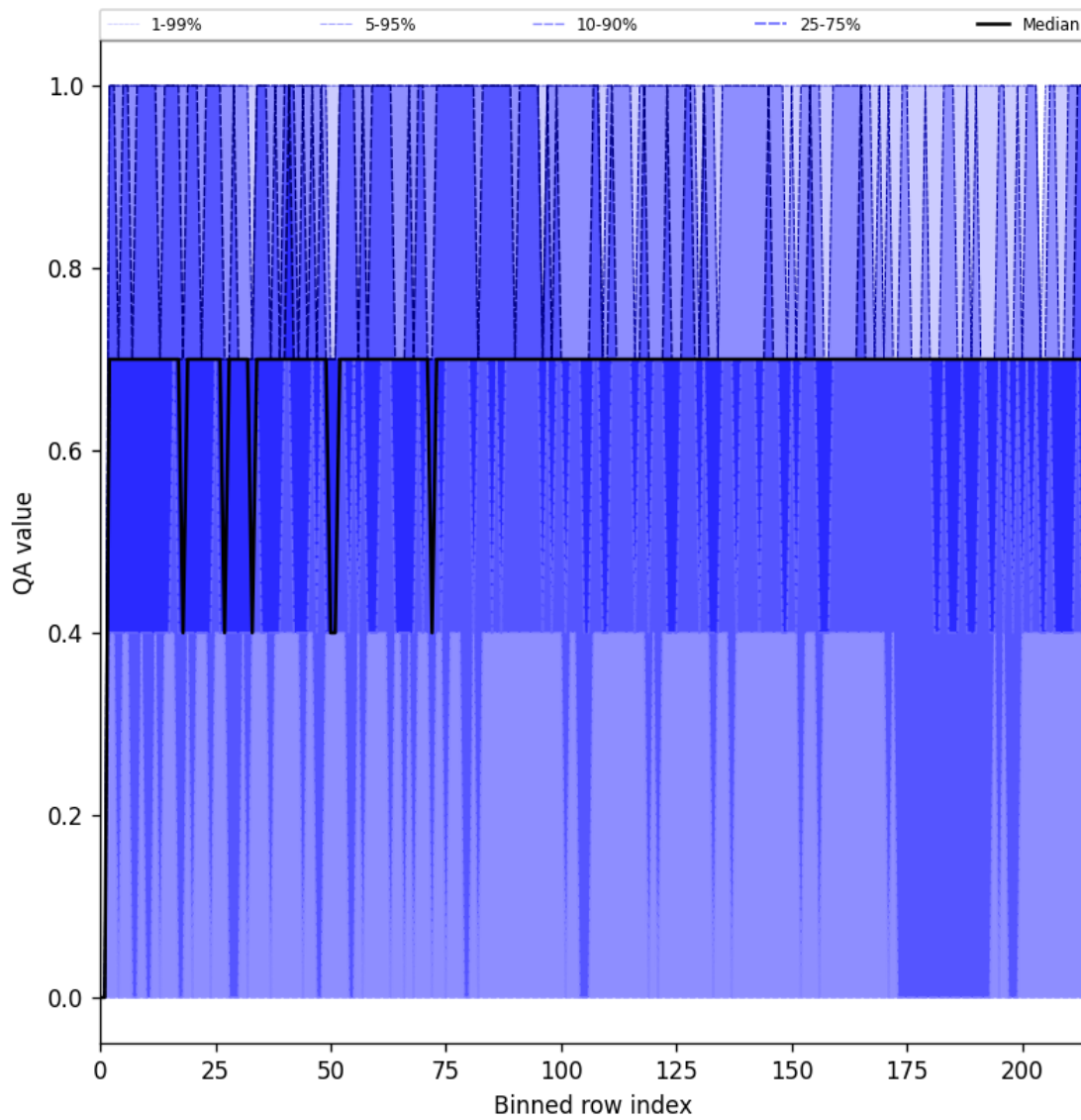
Figure 25: Along track statistics of “QA value” for 2025-10-01 to 2025-10-03
