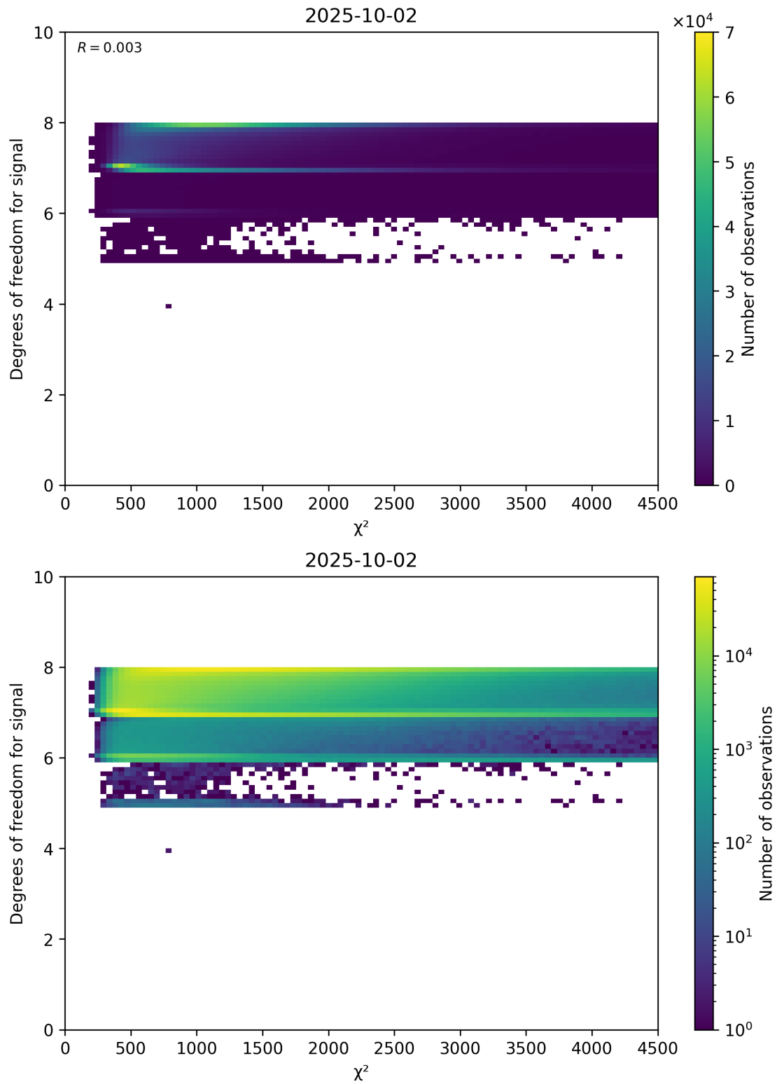
Figure 48: Scatter density plot of “ \chi^2 ” against “Degrees of freedom for signal” for 2025-10-01 to 2025-10-03.
