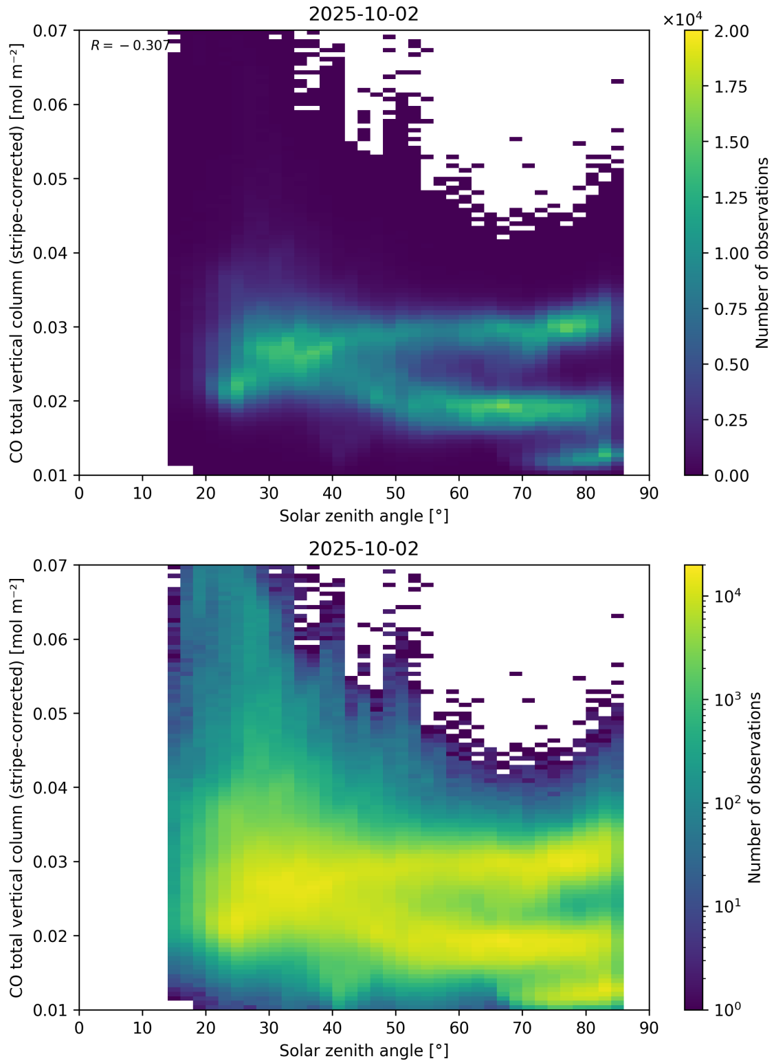
Figure 62: Scatter density plot of “Solar zenith angle” against “CO total vertical column (stripe-corrected)” for 2025-10-01 to 2025-10-03.
