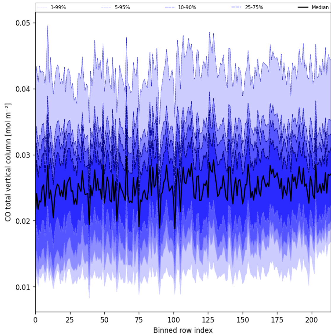
Figure 26: Along track statistics of “CO total vertical column” for 2025-10-01 to 2025-10-03
