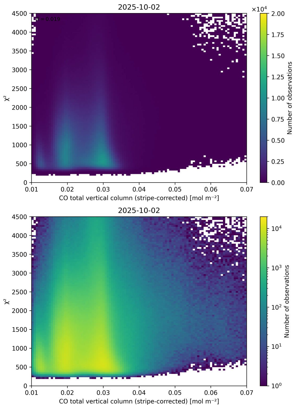
Figure 37: Scatter density plot of “CO total vertical column (stripe-corrected)” against “ \chi^2 ” for 2025-10-01 to 2025-10-03.
