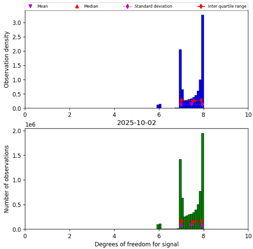
Figure 23: Histogram of “Degrees of freedom for signal” for 2025-10-01 to 2025-10-03
