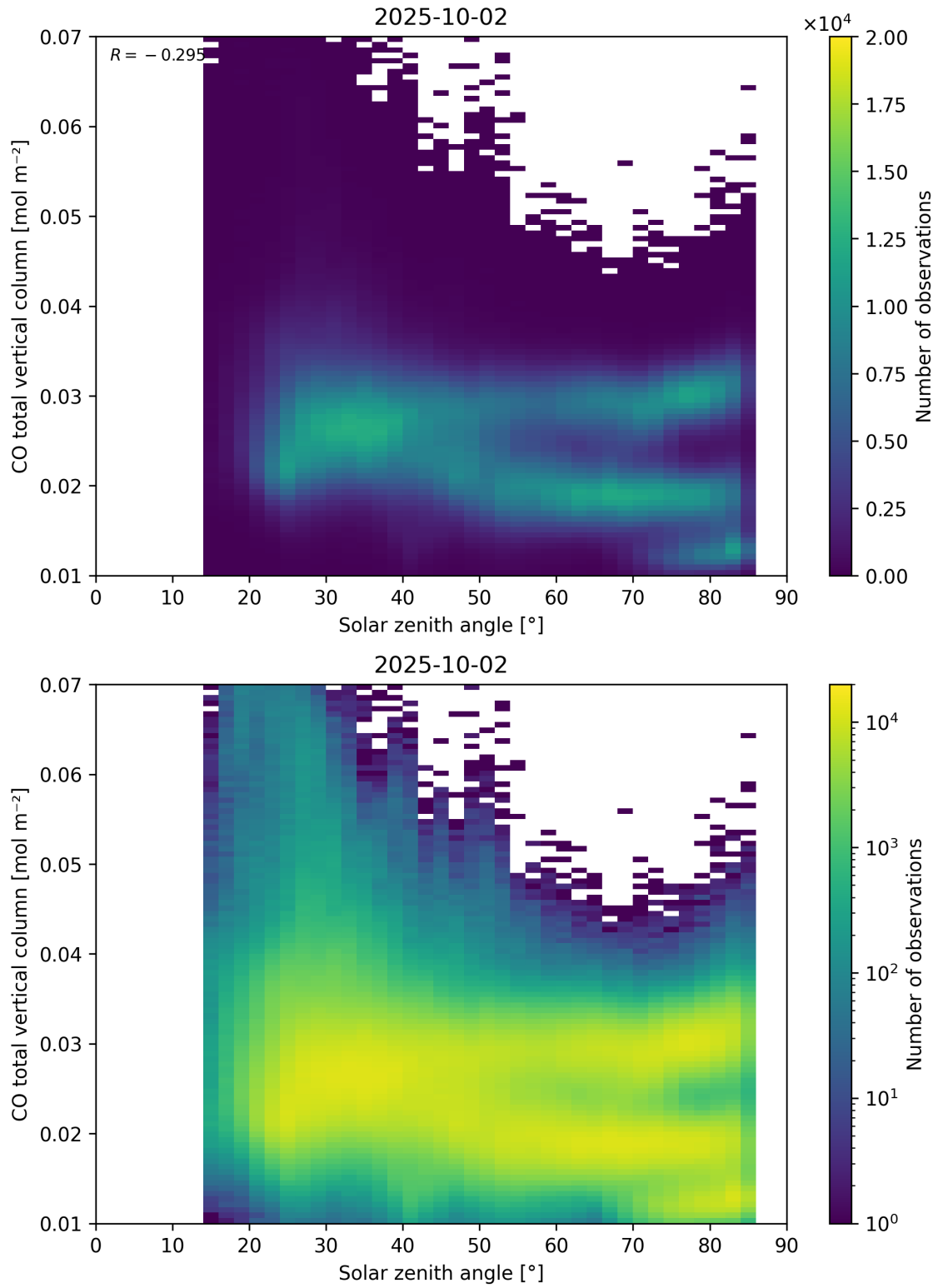
Figure 61: Scatter density plot of “Solar zenith angle” against “CO total vertical column” for 2025-10-01 to 2025-10-03.
