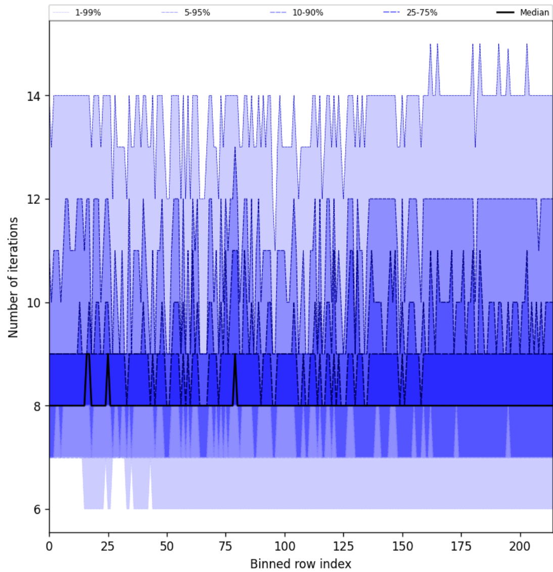
Figure 32: Along track statistics of “Number of iterations” for 2025-10-01 to 2025-10-03
