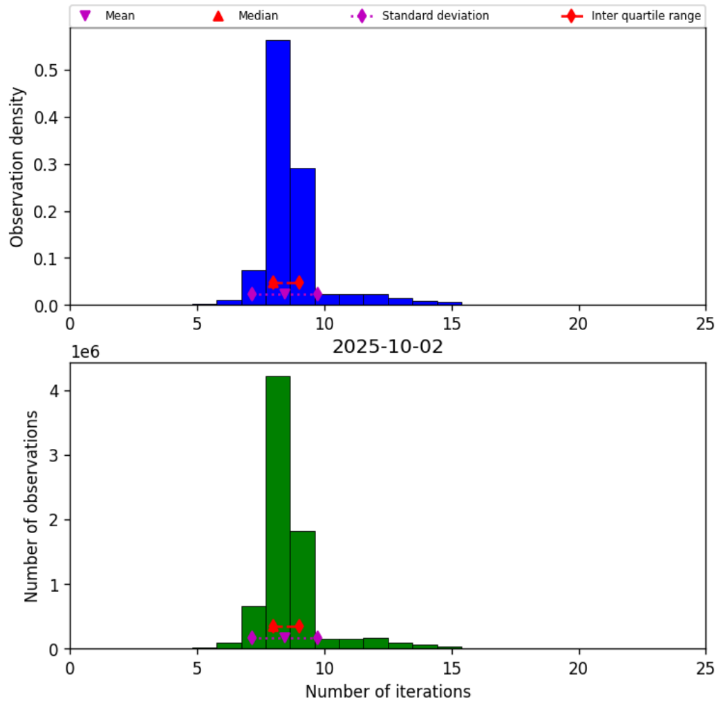
Figure 24: Histogram of “Number of iterations” for 2025-10-01 to 2025-10-03
