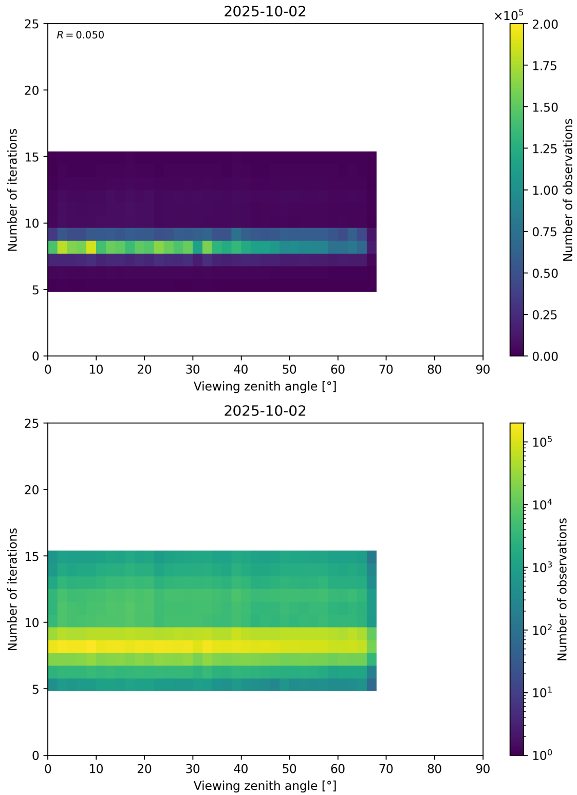
Figure 75: Scatter density plot of “Viewing zenith angle” against “Number of iterations” for 2025-10-01 to 2025-10-03.
