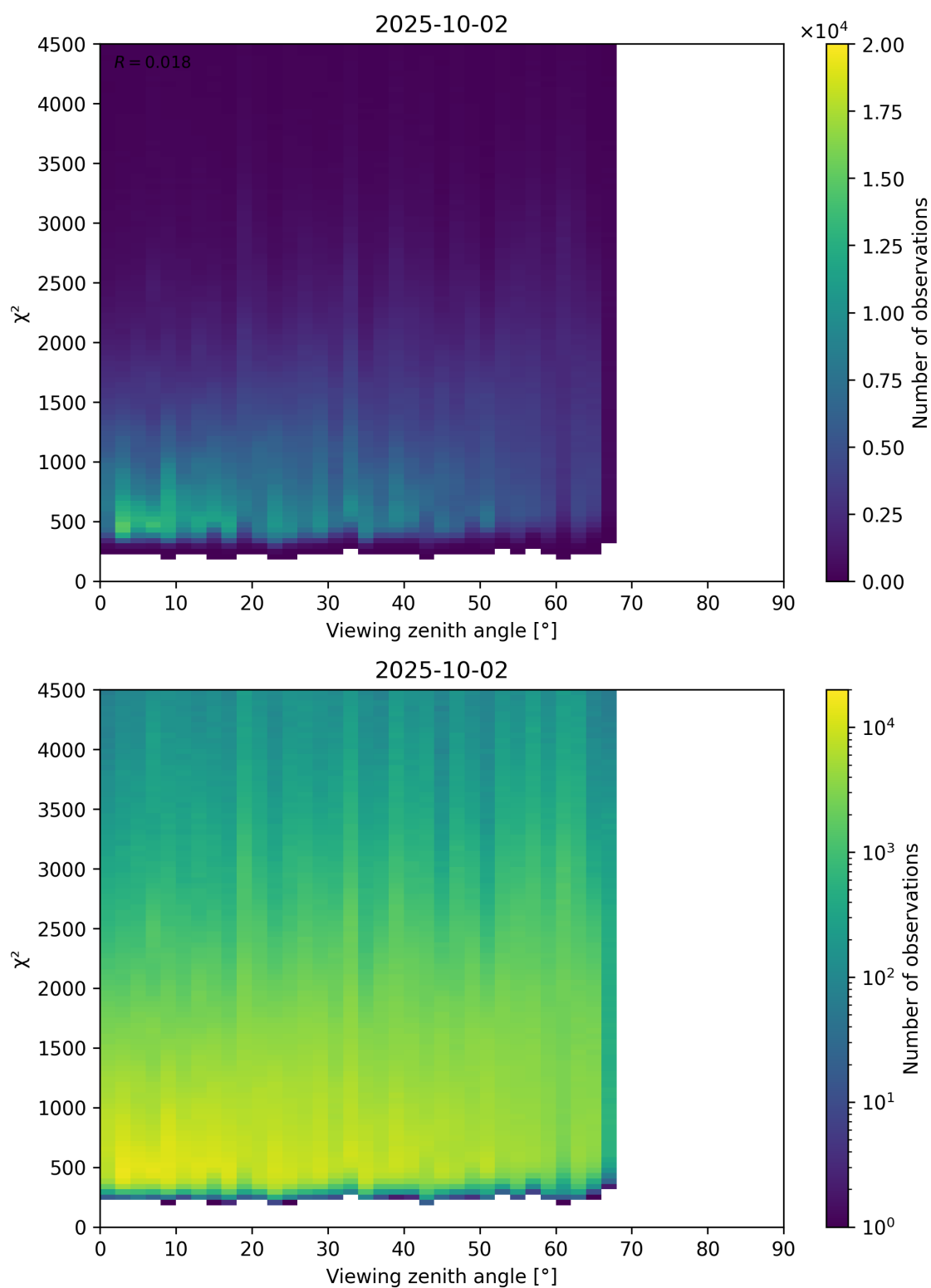
Figure 72: Scatter density plot of “Viewing zenith angle” against “ \chi^2 ” for 2025-10-01 to 2025-10-03.
