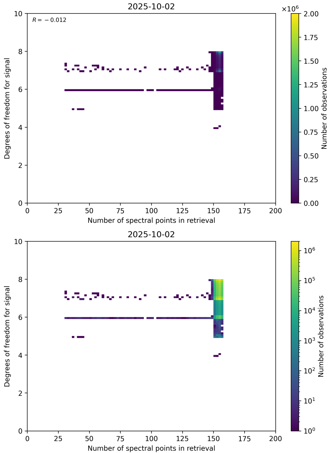
Figure 59: Scatter density plot of “Number of spectral points in retrieval” against “Degrees of freedom for signal” for 2025-10-01 to 2025-10-03.
