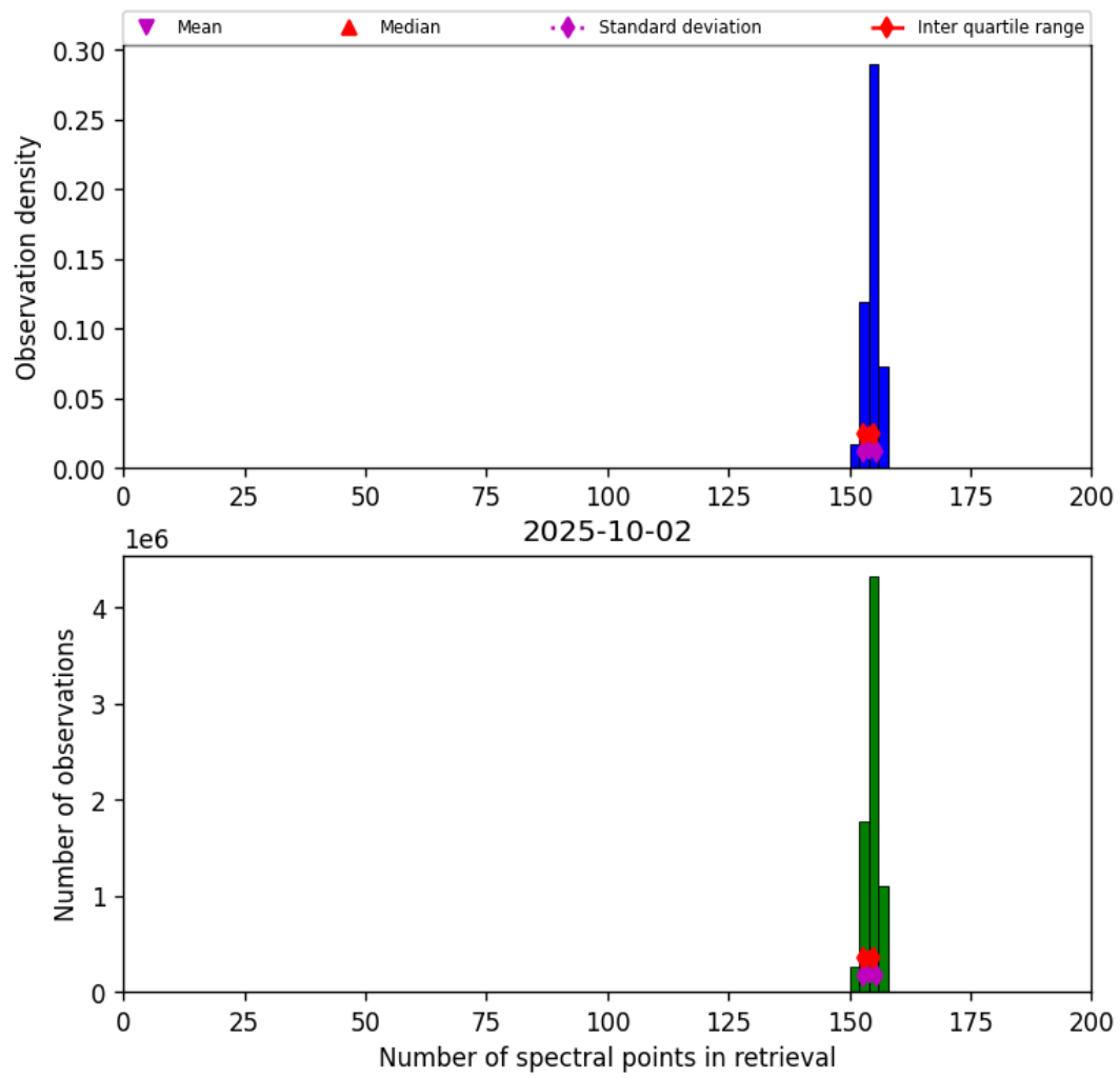
Figure 21: Histogram of “Number of spectral points in retrieval” for 2025-10-01 to 2025-10-03
