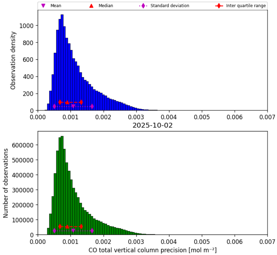
Figure 20: Histogram of “CO total vertical column precision” for 2025-10-01 to 2025-10-03
