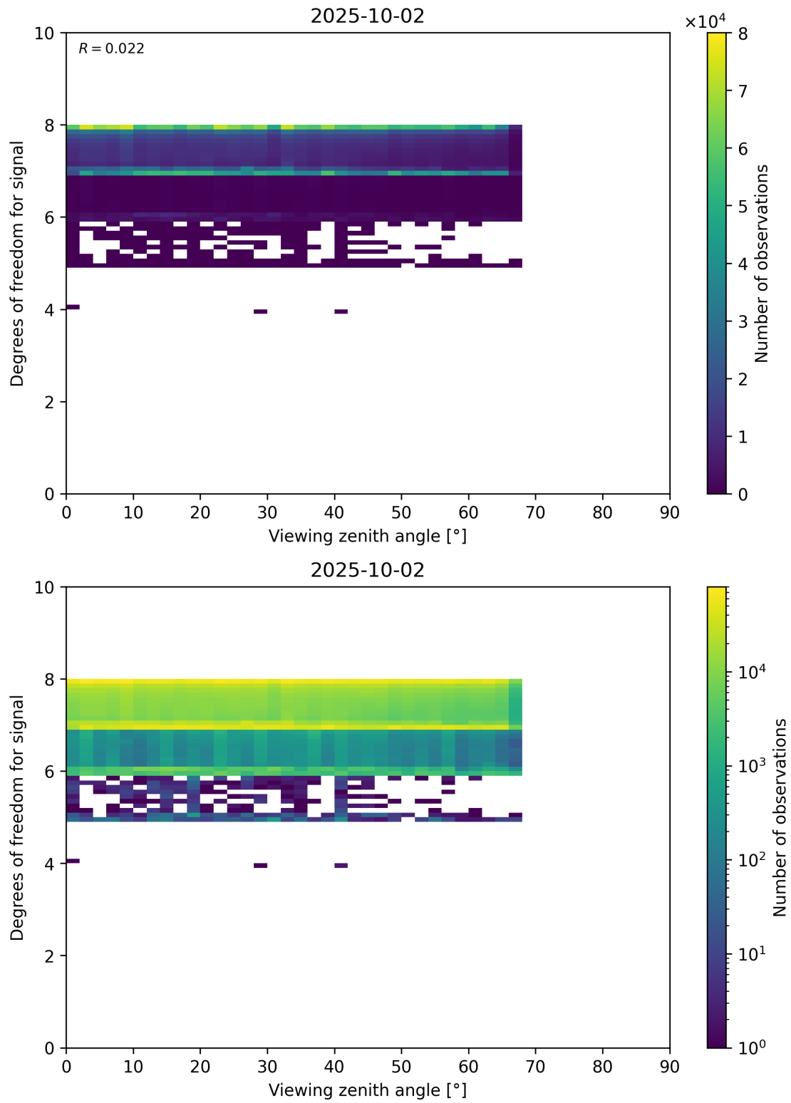
Figure 73: Scatter density plot of “Viewing zenith angle” against “Degrees of freedom for signal” for 2025-10-01 to 2025-10-03.
