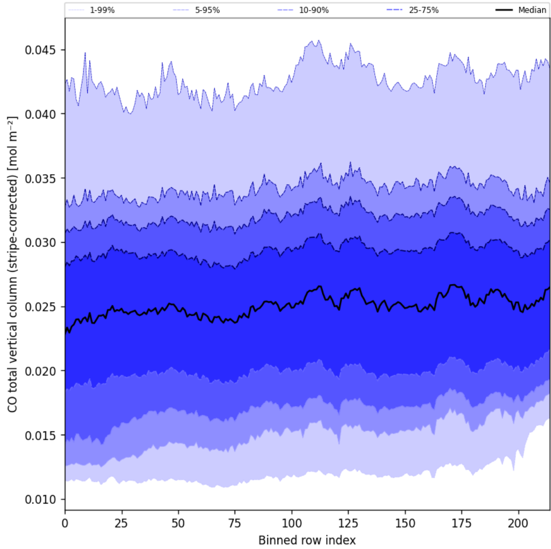
Figure 27: Along track statistics of “CO total vertical column (stripe-corrected)” for 2025-10-01 to 2025-10-03
