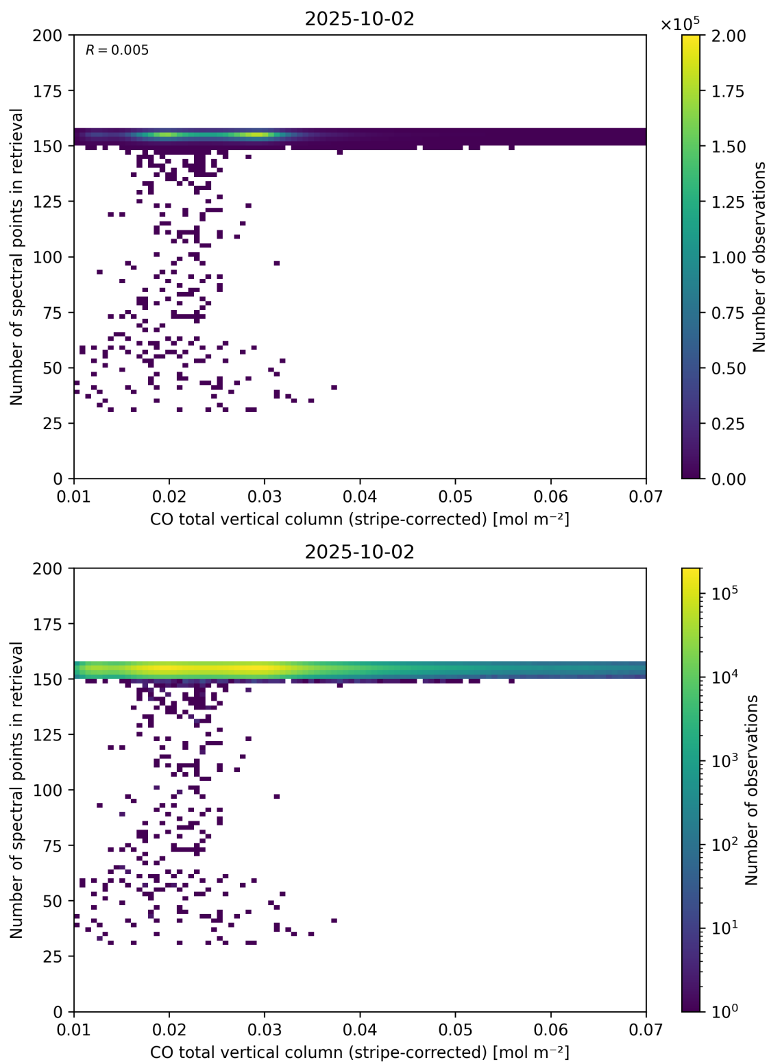
Figure 40: Scatter density plot of “CO total vertical column (stripe-corrected)” against “Number of spectral points in retrieval” for 2025-10-01 to 2025-10-03.
