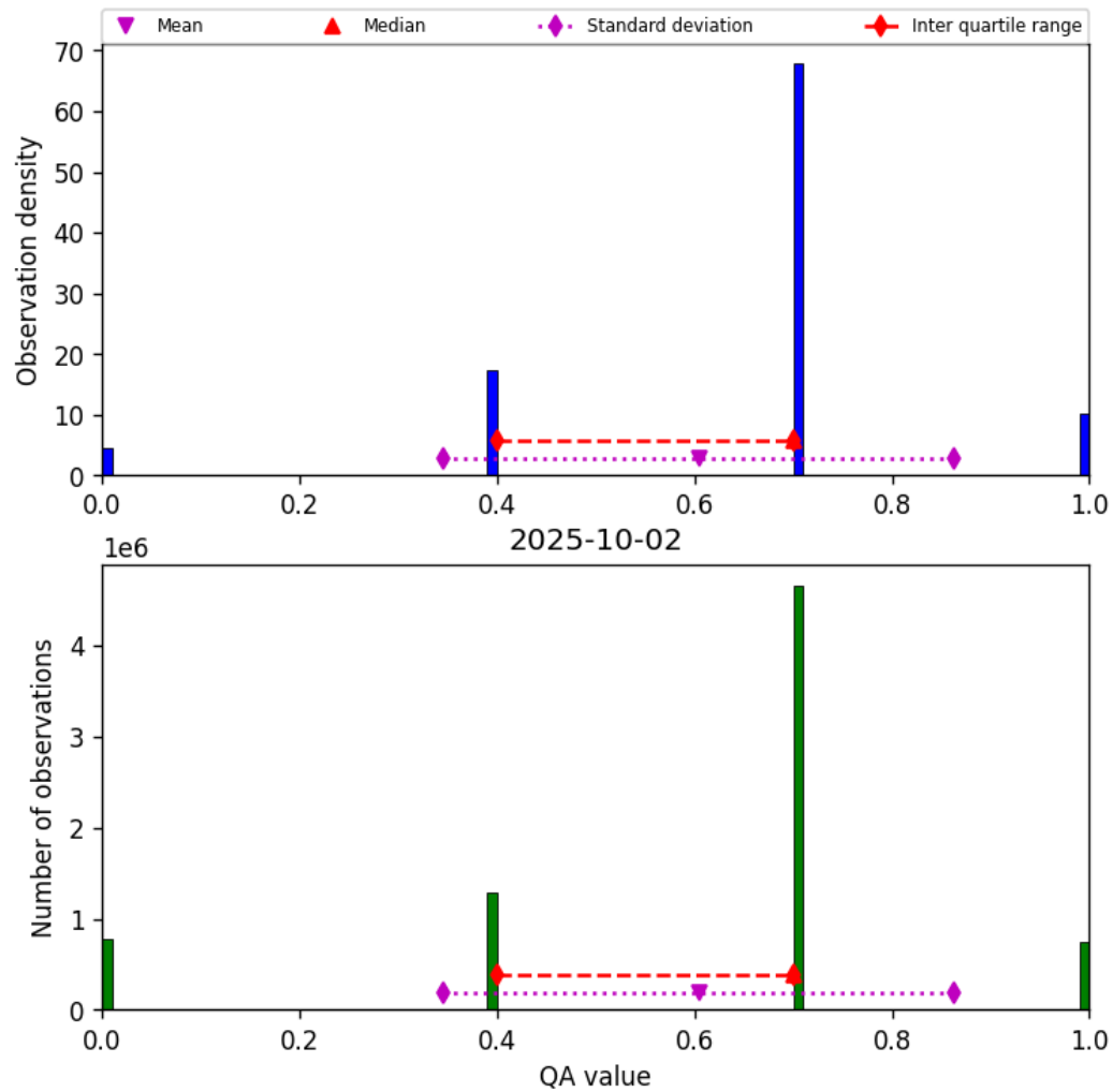
Figure 17: Histogram of “QA value” for 2025-10-01 to 2025-10-03
