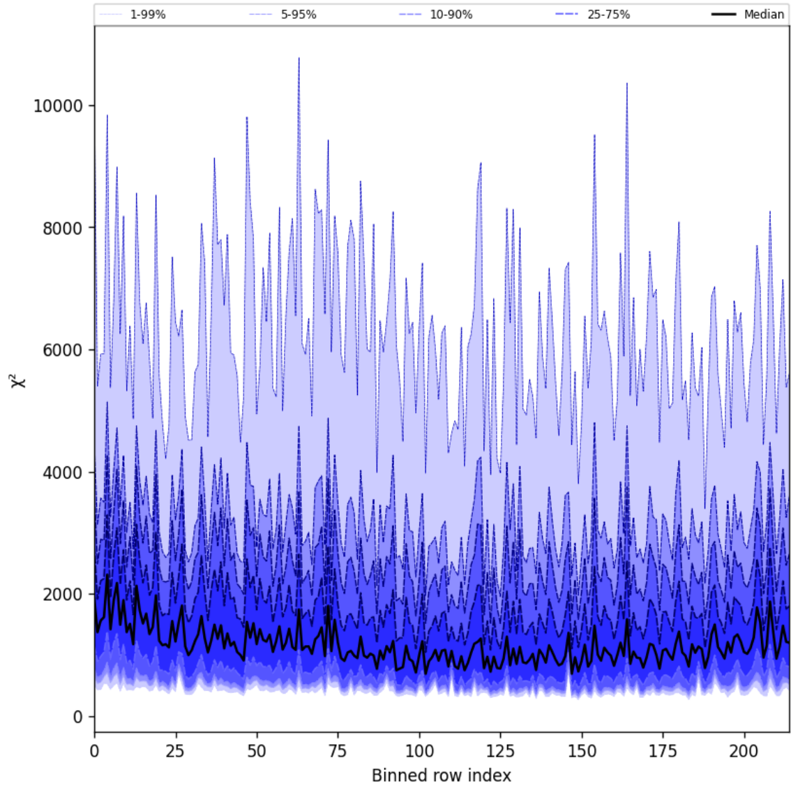
Figure 30: Along track statistics of “ \chi^2 ” for 2025-10-01 to 2025-10-03
