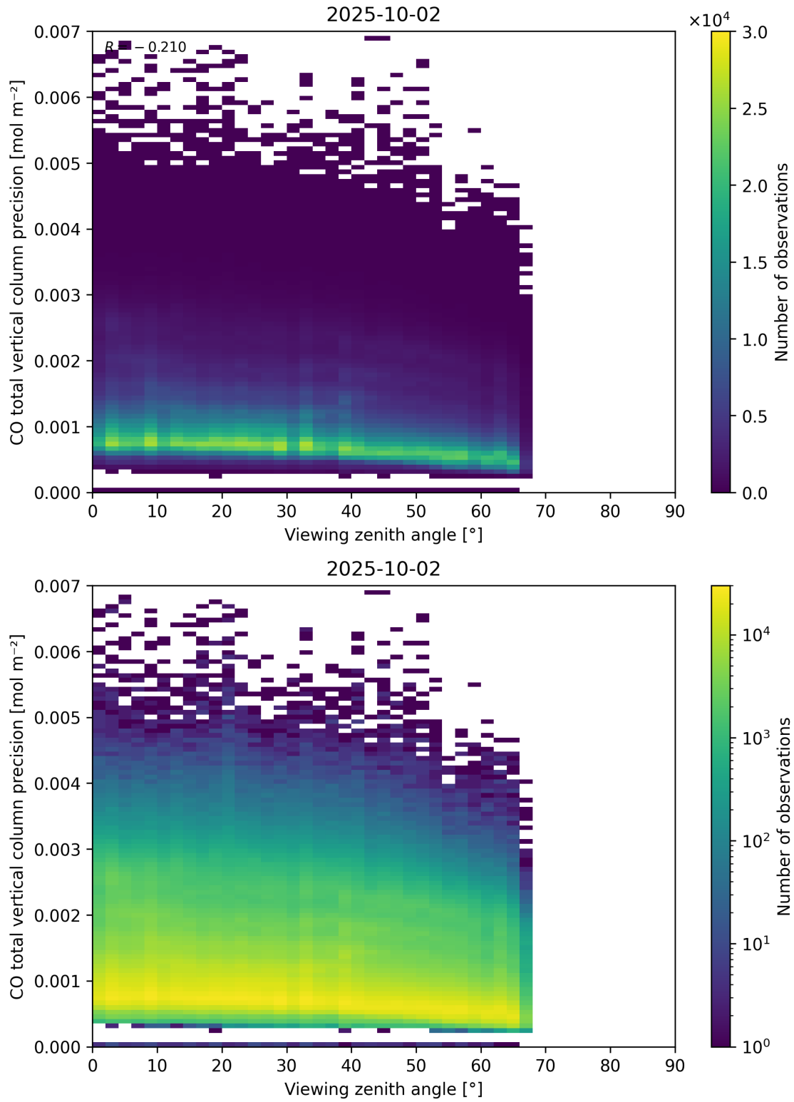
Figure 71: Scatter density plot of “Viewing zenith angle” against “CO total vertical column precision” for 2025-10-01 to 2025-10-03.
