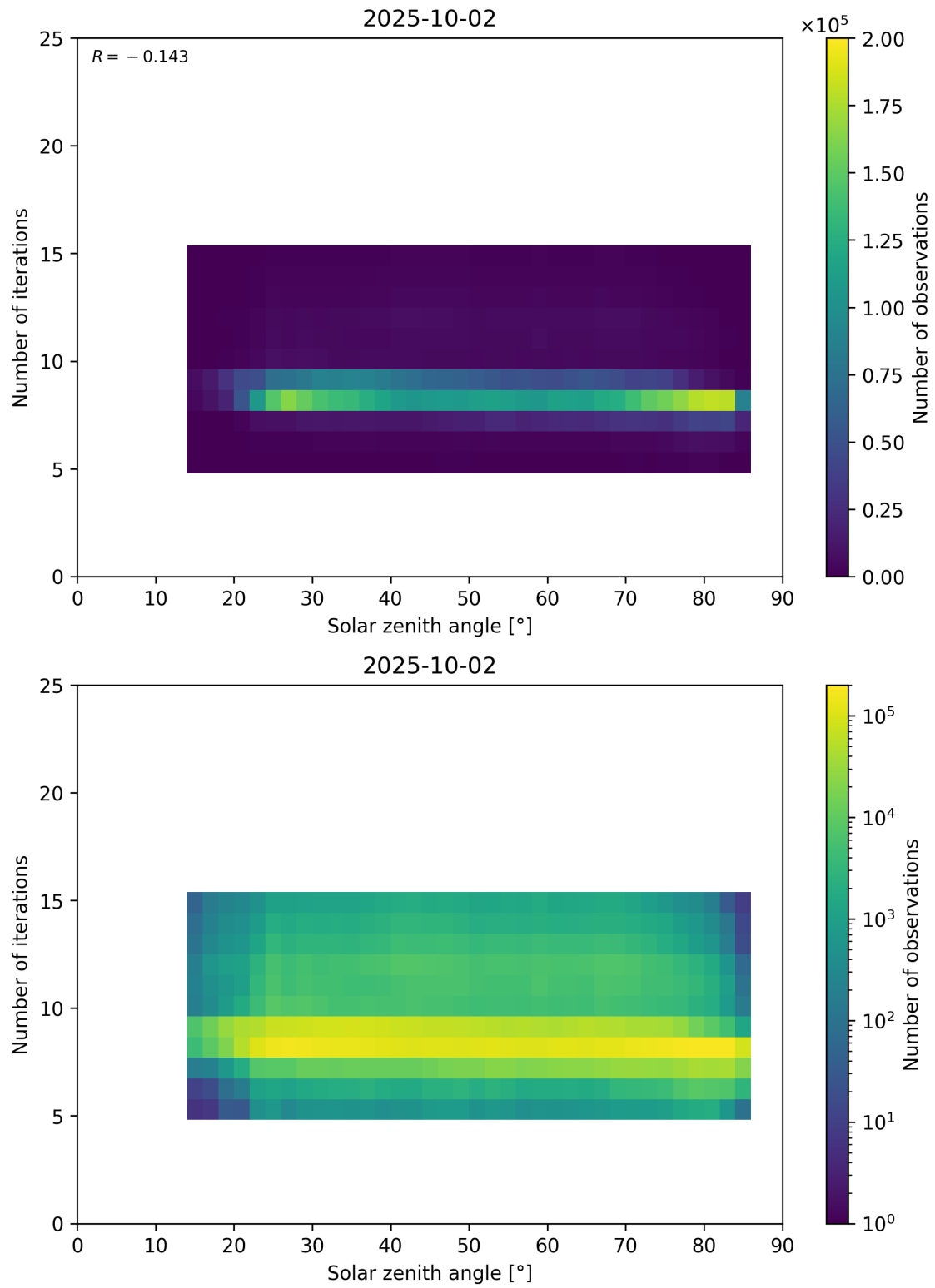
Figure 67: Scatter density plot of “Solar zenith angle” against “Number of iterations” for 2025-10-01 to 2025-10-03.
