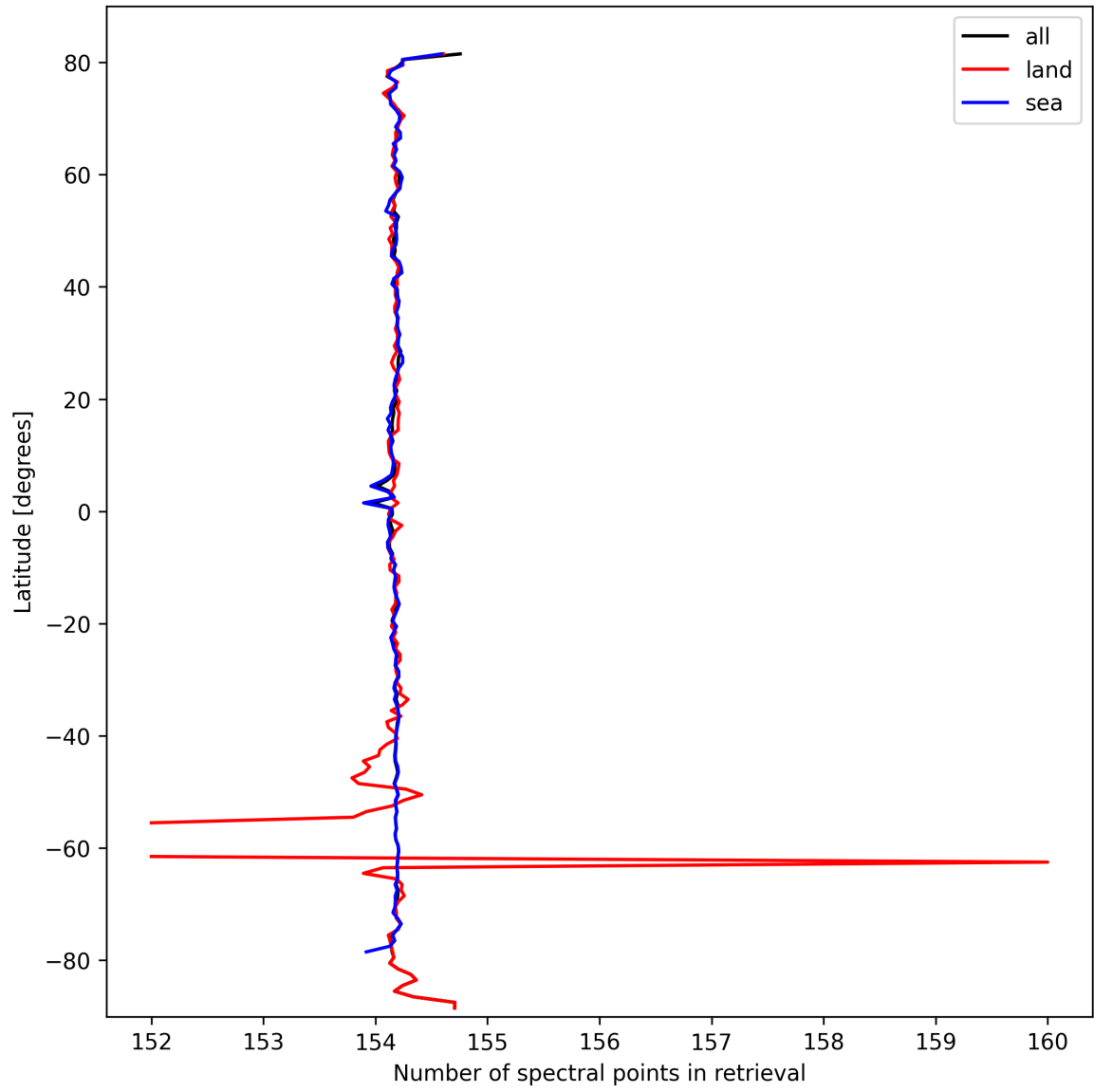
Figure 13: Zonal average of “Number of spectral points in retrieval” for 2025-10-01 to 2025-10-03.
