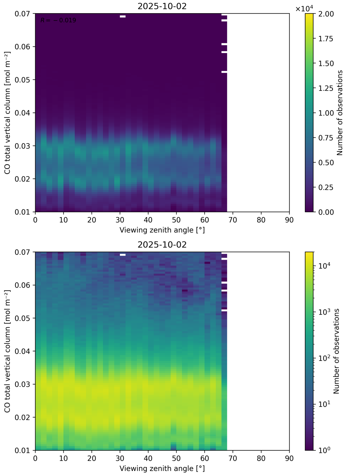
Figure 69: Scatter density plot of “Viewing zenith angle” against “CO total vertical column” for 2025-10-01 to 2025-10-03.
