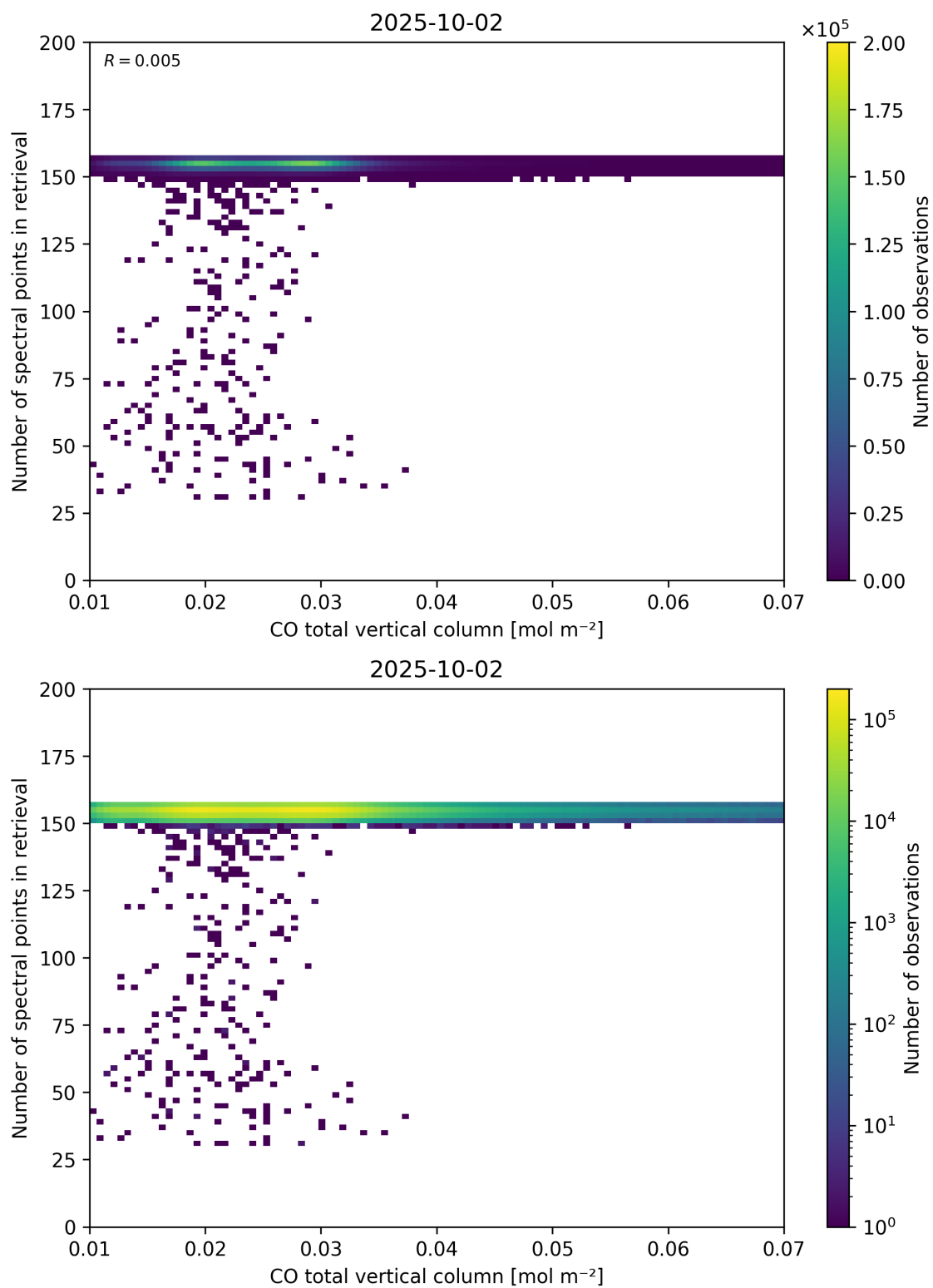
Figure 43: Scatter density plot of “CO total vertical column” against “Number of spectral points in retrieval” for 2025-10-01 to 2025-10-03.
