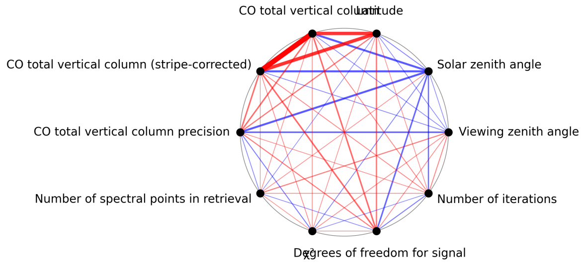
Figure 1: Map of correlation graph for 2025-10-01 to 2025-10-03.
