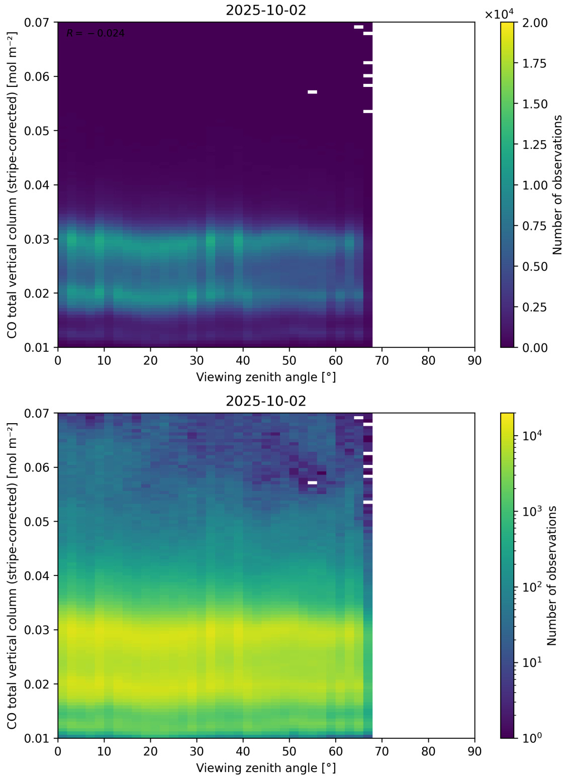
Figure 70: Scatter density plot of “Viewing zenith angle” against “CO total vertical column (stripe-corrected)” for 2025-10-01 to 2025-10-03.
