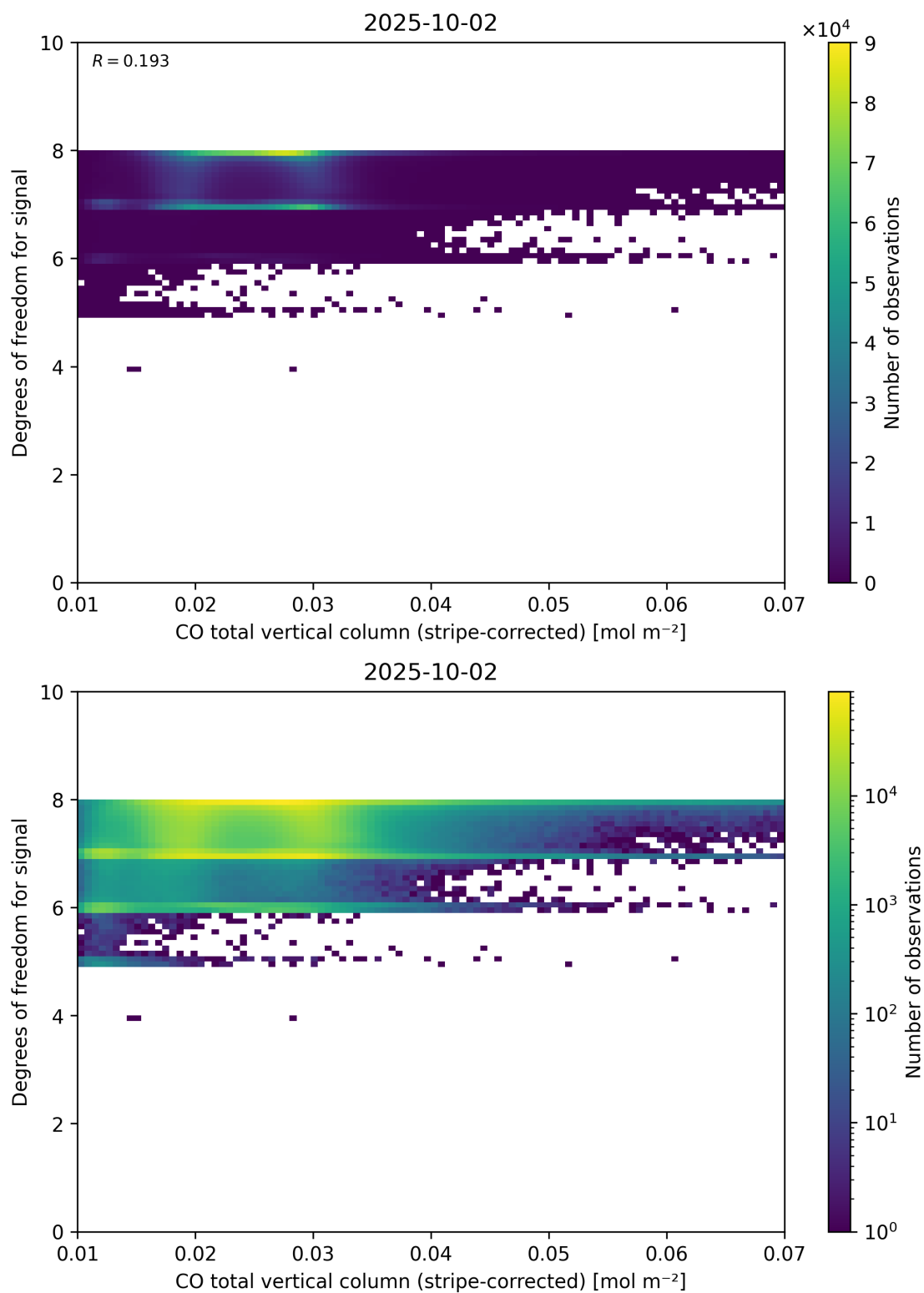
Figure 38: Scatter density plot of “CO total vertical column (stripe-corrected)” against “Degrees of freedom for signal” for 2025-10-01 to 2025-10-03.
