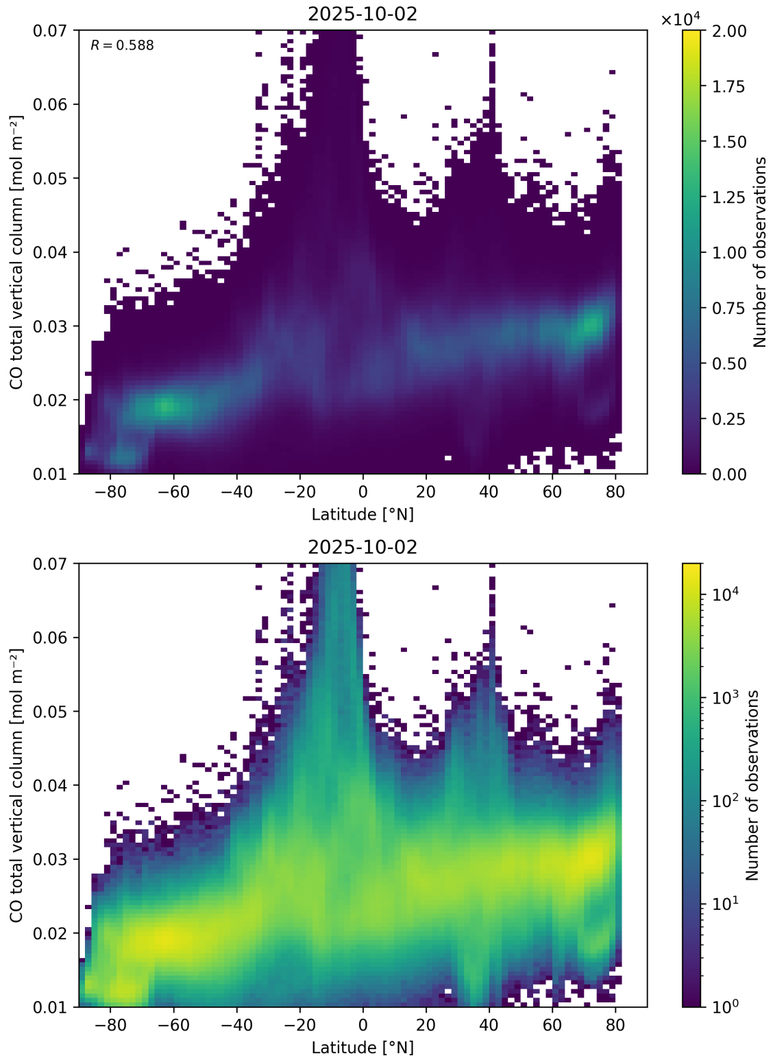
Figure 51: Scatter density plot of “Latitude” against “CO total vertical column” for 2025-10-01 to 2025-10-03.
