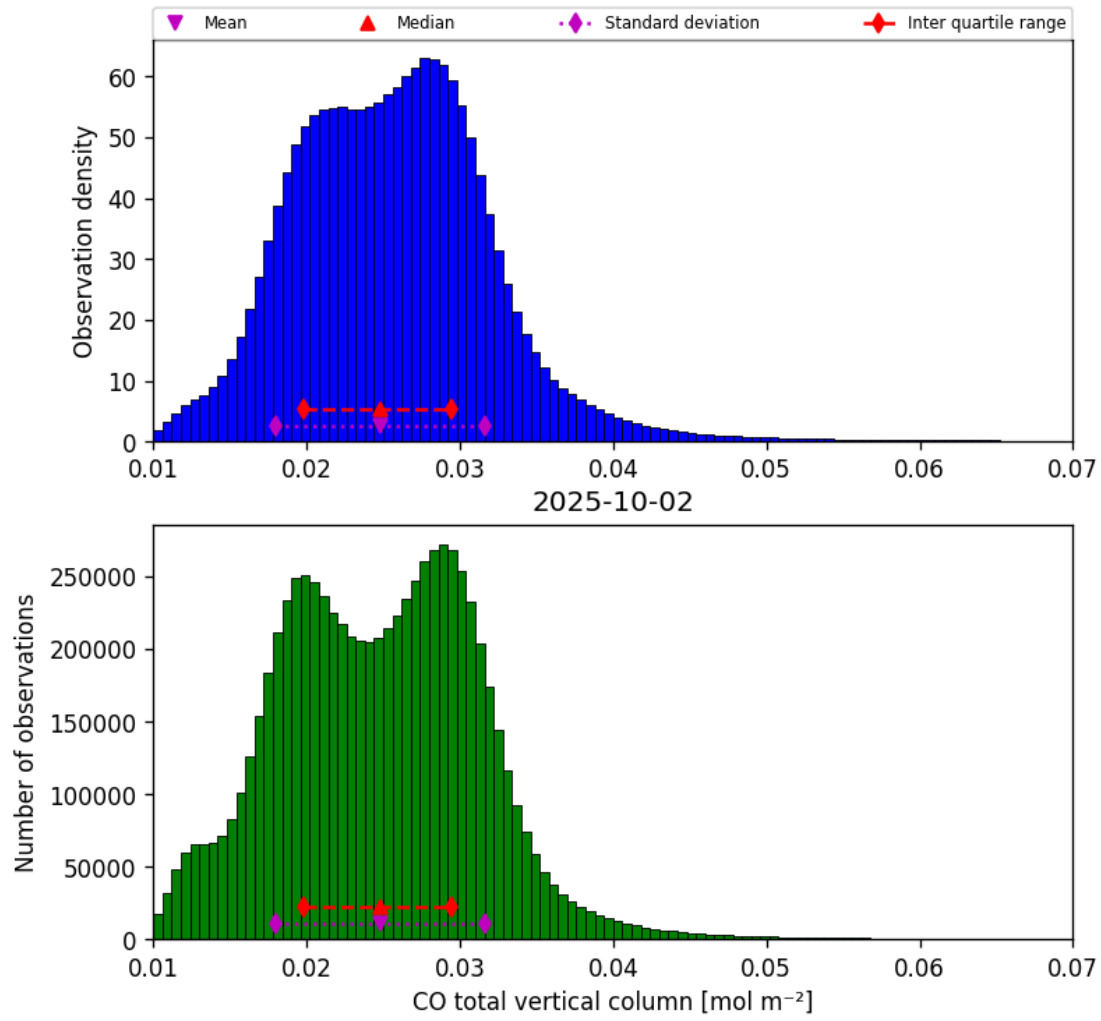
Figure 18: Histogram of “CO total vertical column” for 2025-10-01 to 2025-10-03
