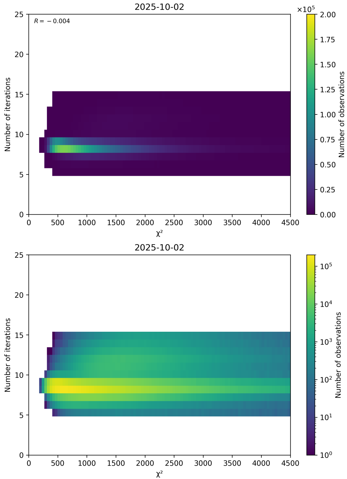
Figure 49: Scatter density plot of “ \chi^2 ” against “Number of iterations” for 2025-10-01 to 2025-10-03.
