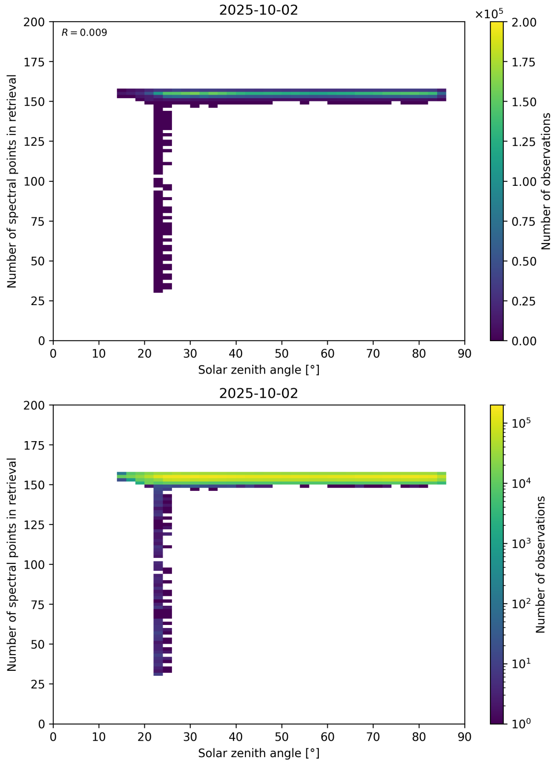
Figure 68: Scatter density plot of “Solar zenith angle” against “Number of spectral points in retrieval” for 2025-10-01 to 2025-10-03.
