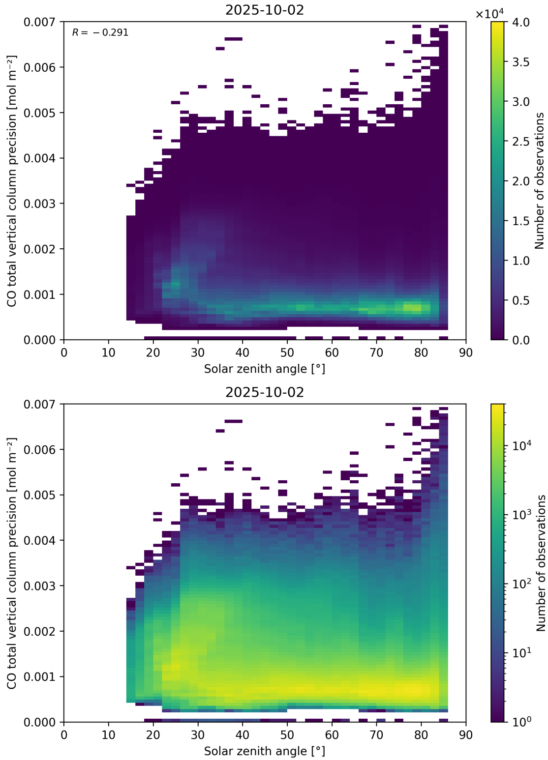
Figure 63: Scatter density plot of “Solar zenith angle” against “CO total vertical column precision” for 2025-10-01 to 2025-10-03.
