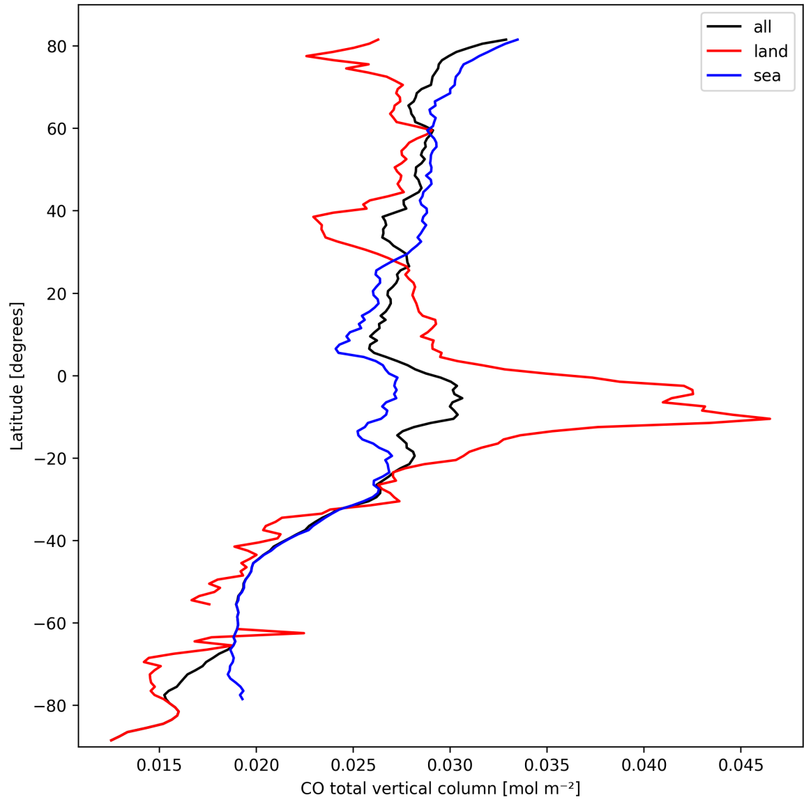
Figure 10: Zonal average of “CO total vertical column” for 2025-10-01 to 2025-10-03.
