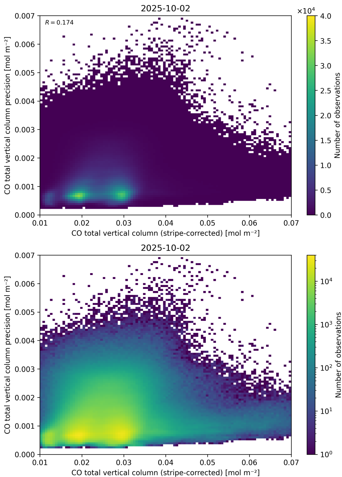
Figure 36: Scatter density plot of “CO total vertical column (stripe-corrected)” against “CO total vertical column precision” for 2025-10-01 to 2025-10-03.
