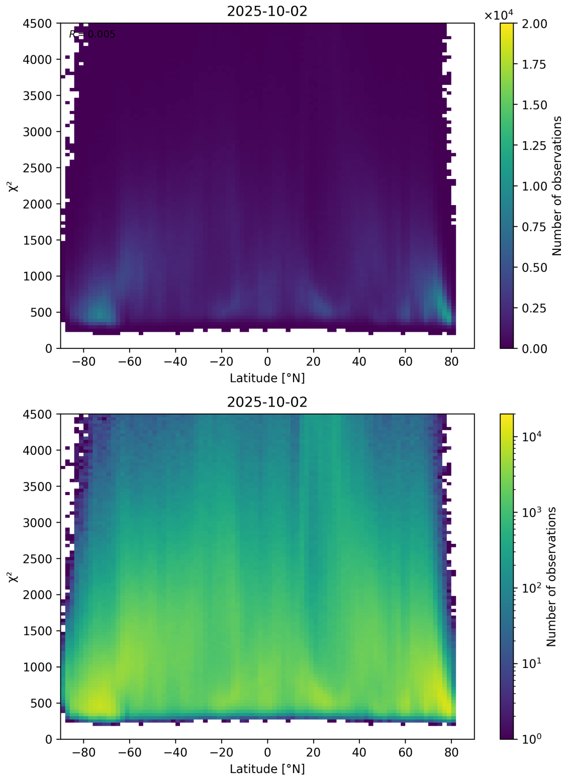
Figure 54: Scatter density plot of “Latitude” against “ \chi^2 ” for 2025-10-01 to 2025-10-03.
