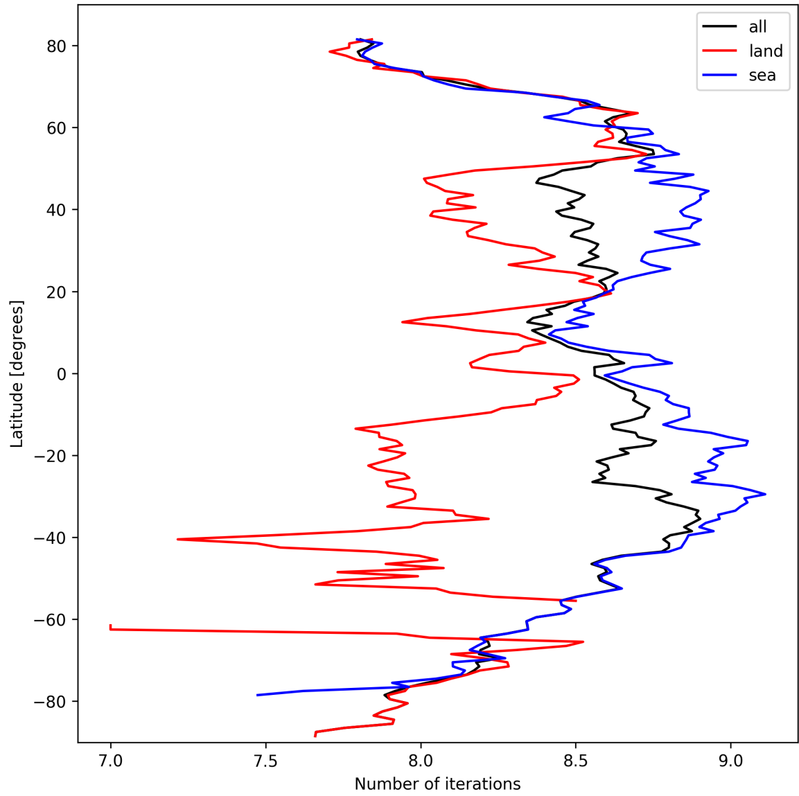
Figure 16: Zonal average of “Number of iterations” for 2025-10-01 to 2025-10-03.
