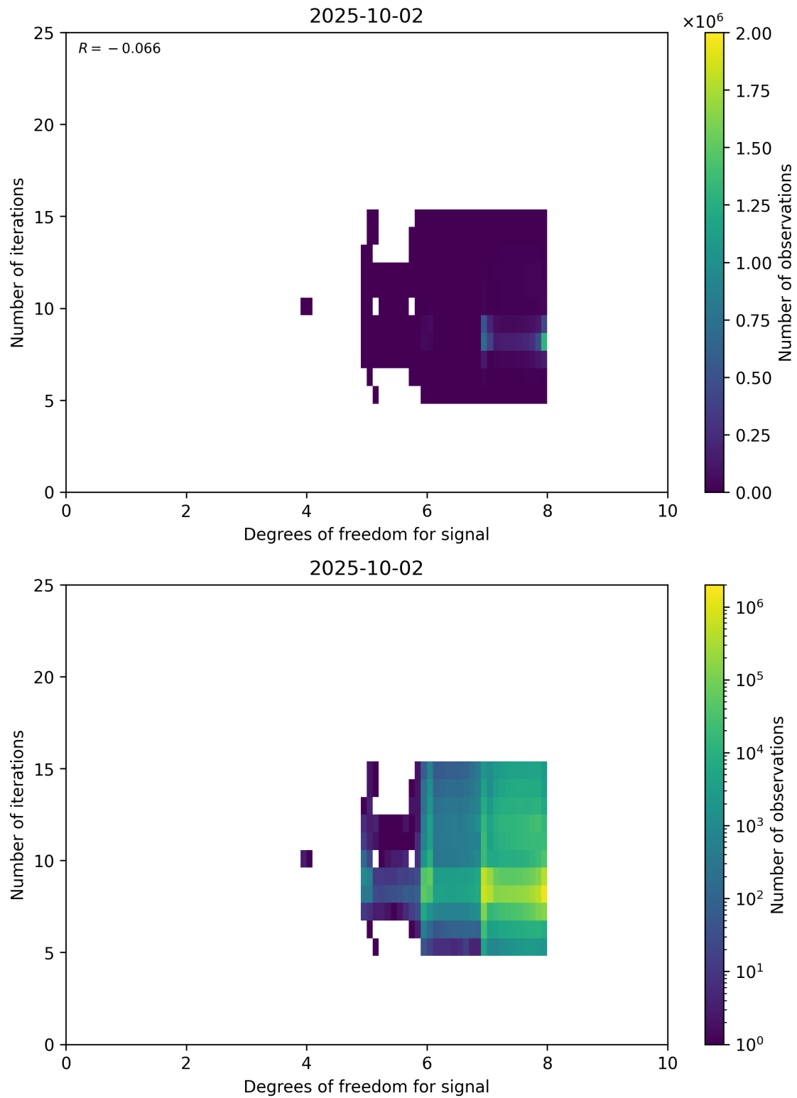
Figure 50: Scatter density plot of “Degrees of freedom for signal” against “Number of iterations” for 2025-10-01 to 2025-10-03.
