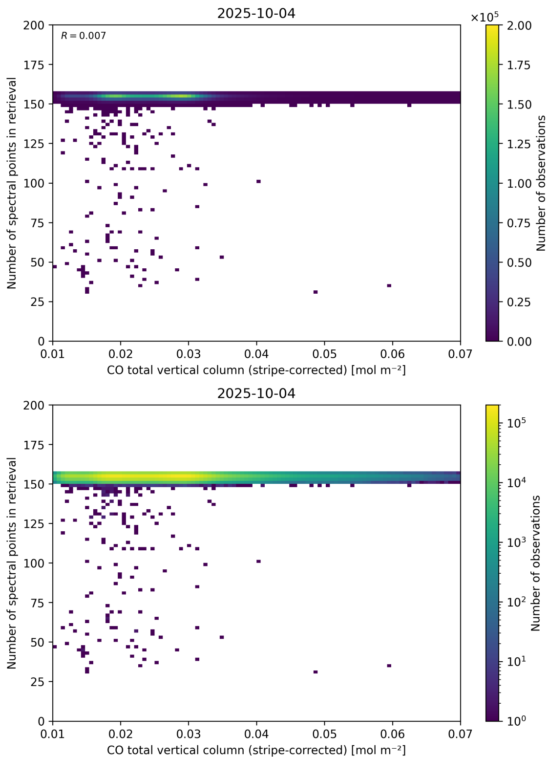
Figure 40: Scatter density plot of “CO total vertical column (stripe-corrected)” against “Number of spectral points in retrieval” for 2025-10-03 to 2025-10-05.
