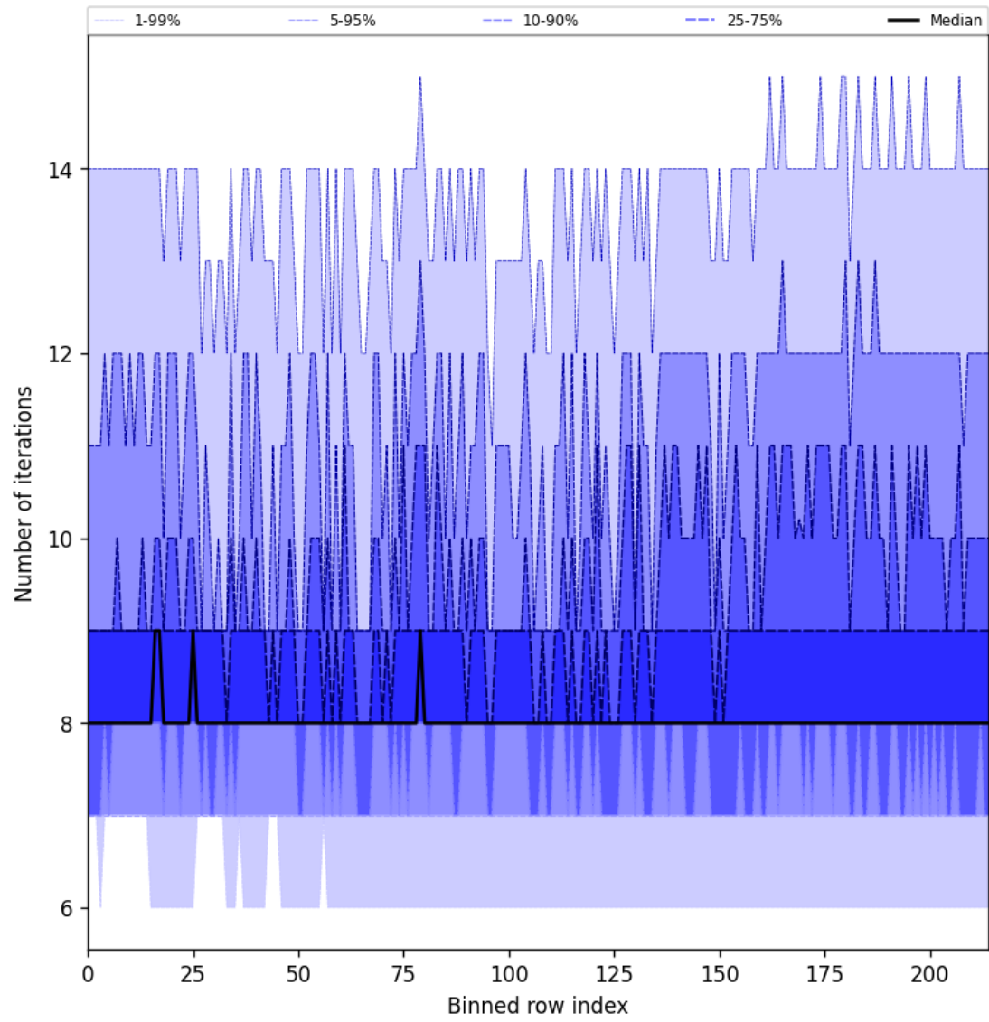
Figure 32: Along track statistics of “Number of iterations” for 2025-10-03 to 2025-10-05
