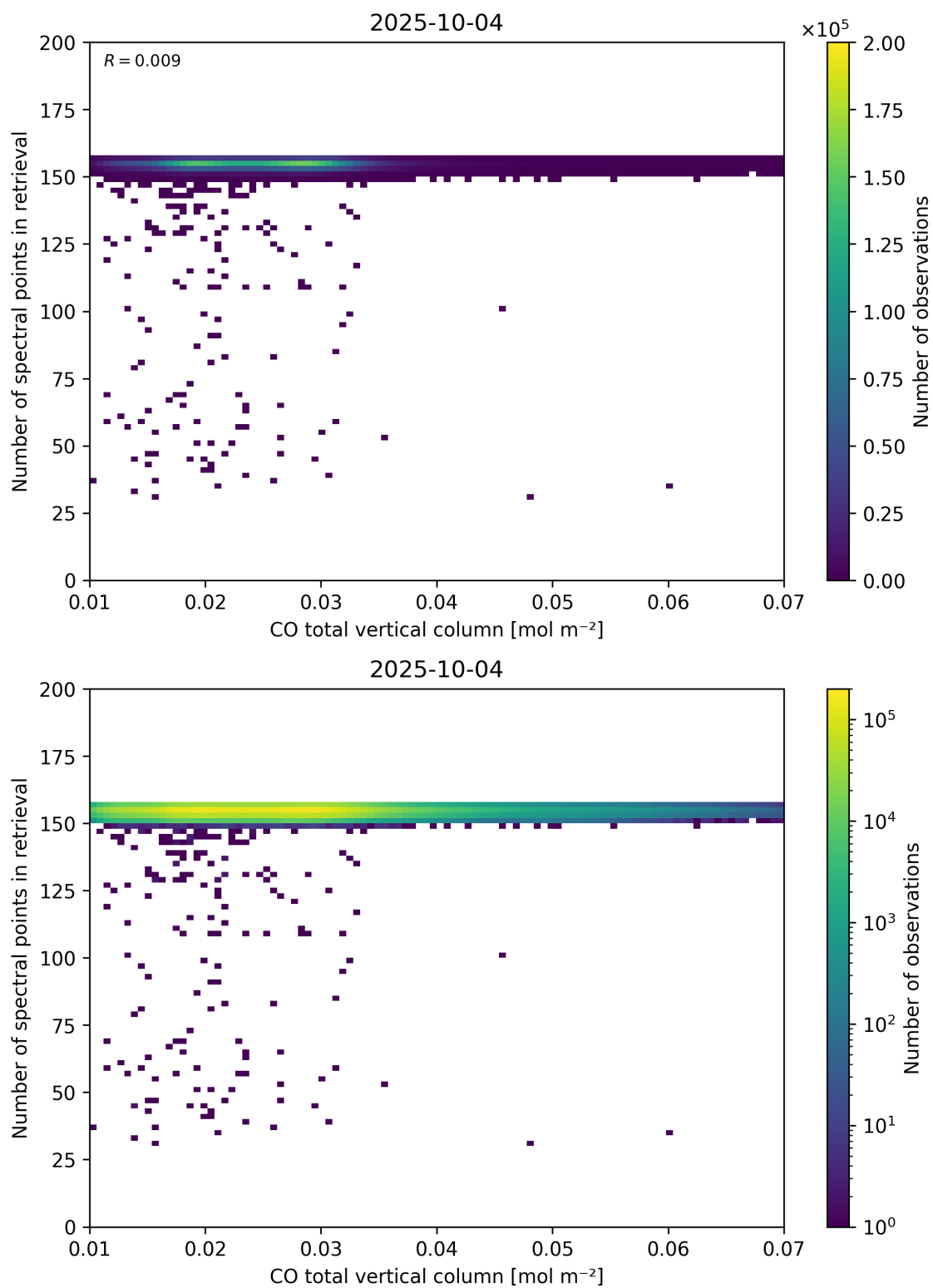
Figure 43: Scatter density plot of “CO total vertical column” against “Number of spectral points in retrieval” for 2025-10-03 to 2025-10-05.
