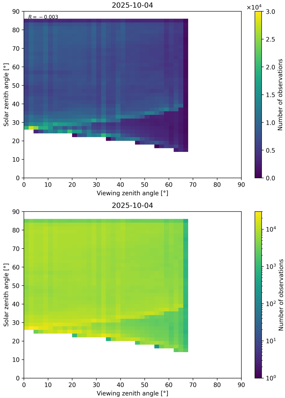
Figure 77: Scatter density plot of “Viewing zenith angle” against “Solar zenith angle” for 2025-10-03 to 2025-10-05.
