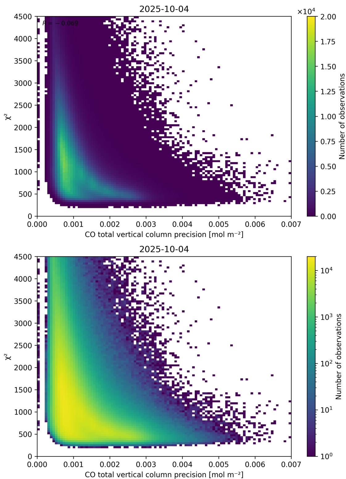
Figure 44: Scatter density plot of “CO total vertical column precision” against “ \chi^2 ” for 2025-10-03 to 2025-10-05.
