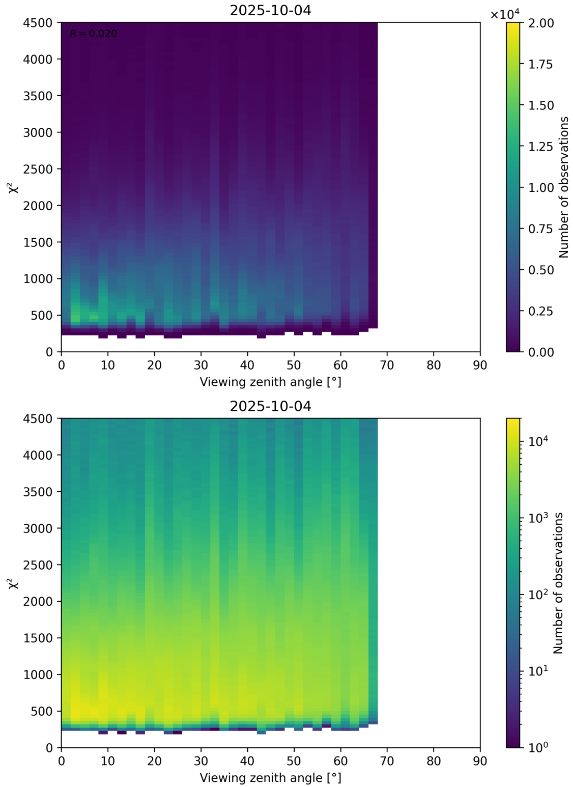
Figure 72: Scatter density plot of “Viewing zenith angle” against “ \chi^2 ” for 2025-10-03 to 2025-10-05.
