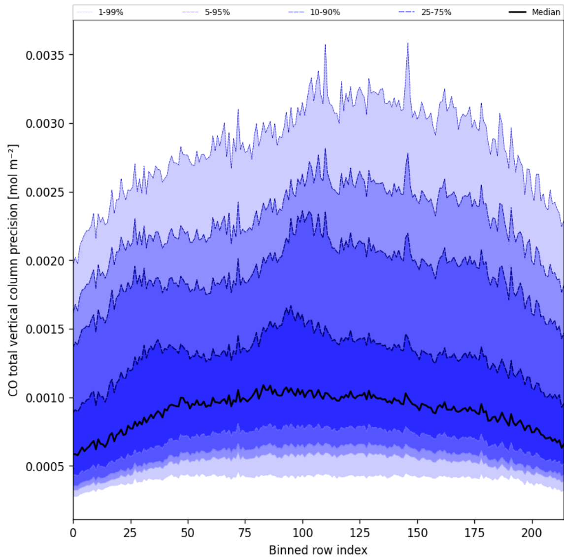
Figure 28: Along track statistics of “CO total vertical column precision” for 2025-10-03 to 2025-10-05
