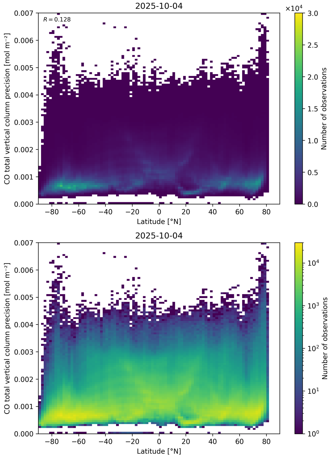
Figure 53: Scatter density plot of “Latitude” against “CO total vertical column precision” for 2025-10-03 to 2025-10-05.
