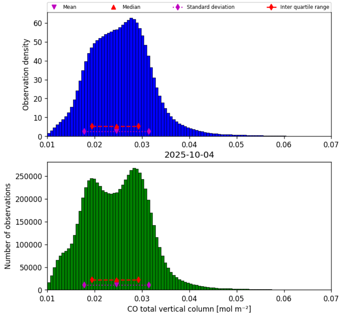
Figure 18: Histogram of “CO total vertical column” for 2025-10-03 to 2025-10-05
