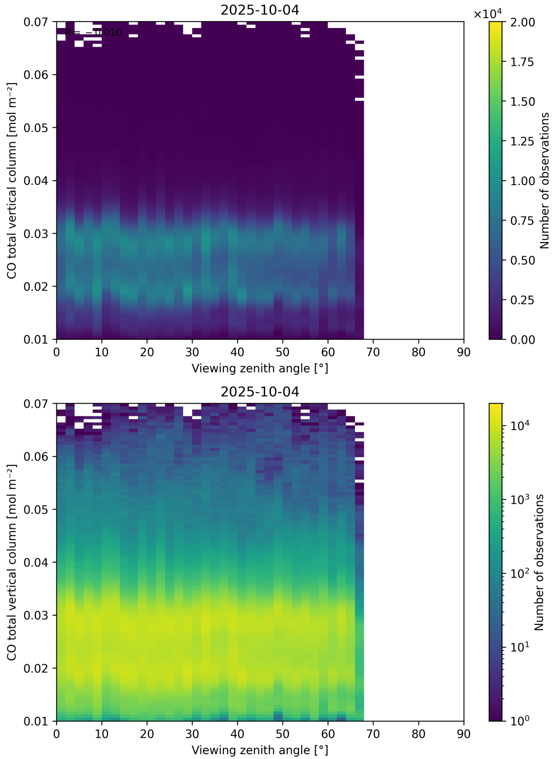
Figure 69: Scatter density plot of “Viewing zenith angle” against “CO total vertical column” for 2025-10-03 to 2025-10-05.
