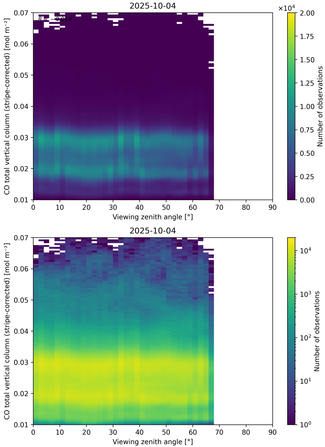
Figure 70: Scatter density plot of “Viewing zenith angle” against “CO total vertical column (stripe-corrected)” for 2025-10-03 to 2025-10-05.
