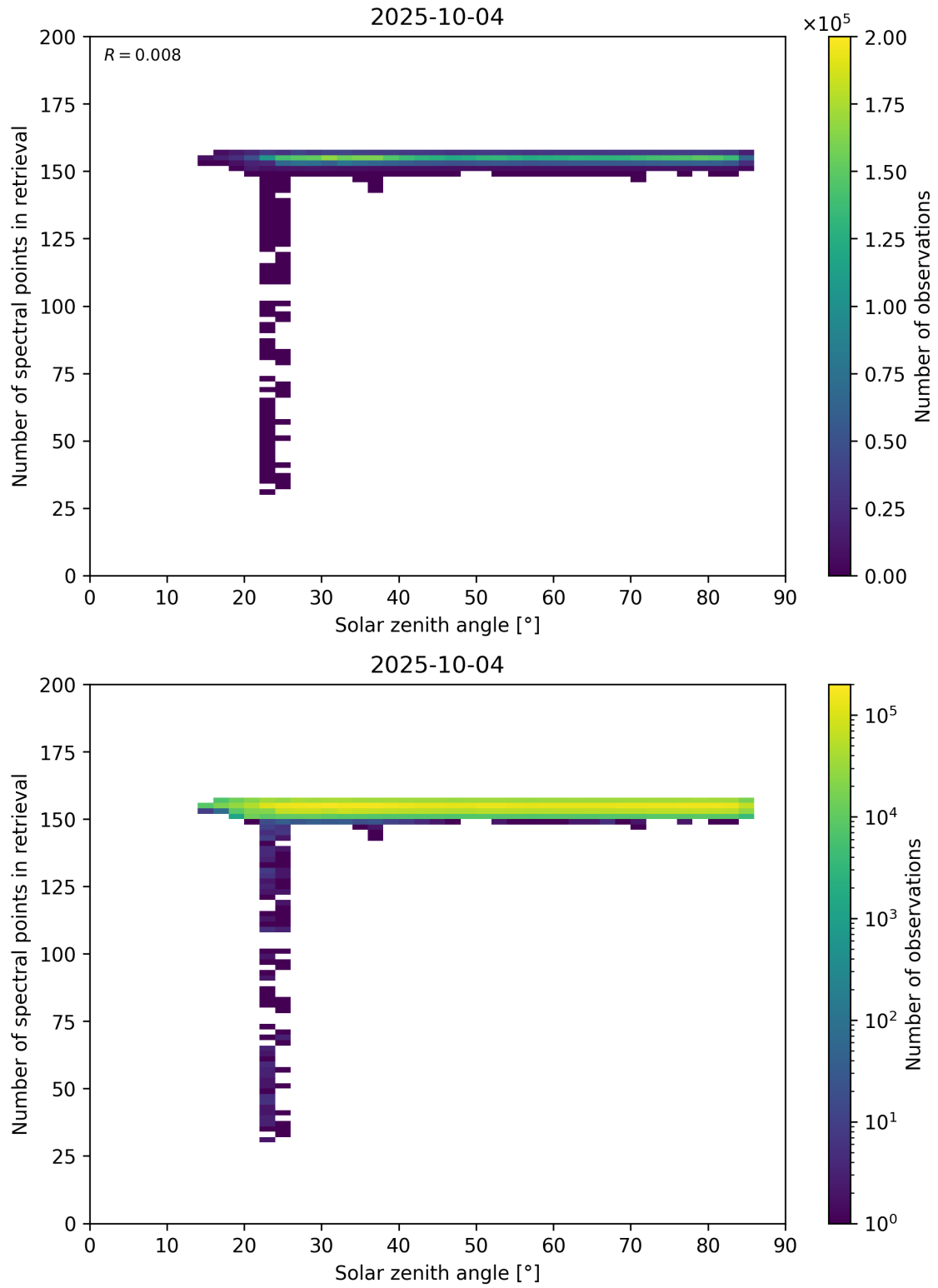
Figure 68: Scatter density plot of “Solar zenith angle” against “Number of spectral points in retrieval” for 2025-10-03 to 2025-10-05.
