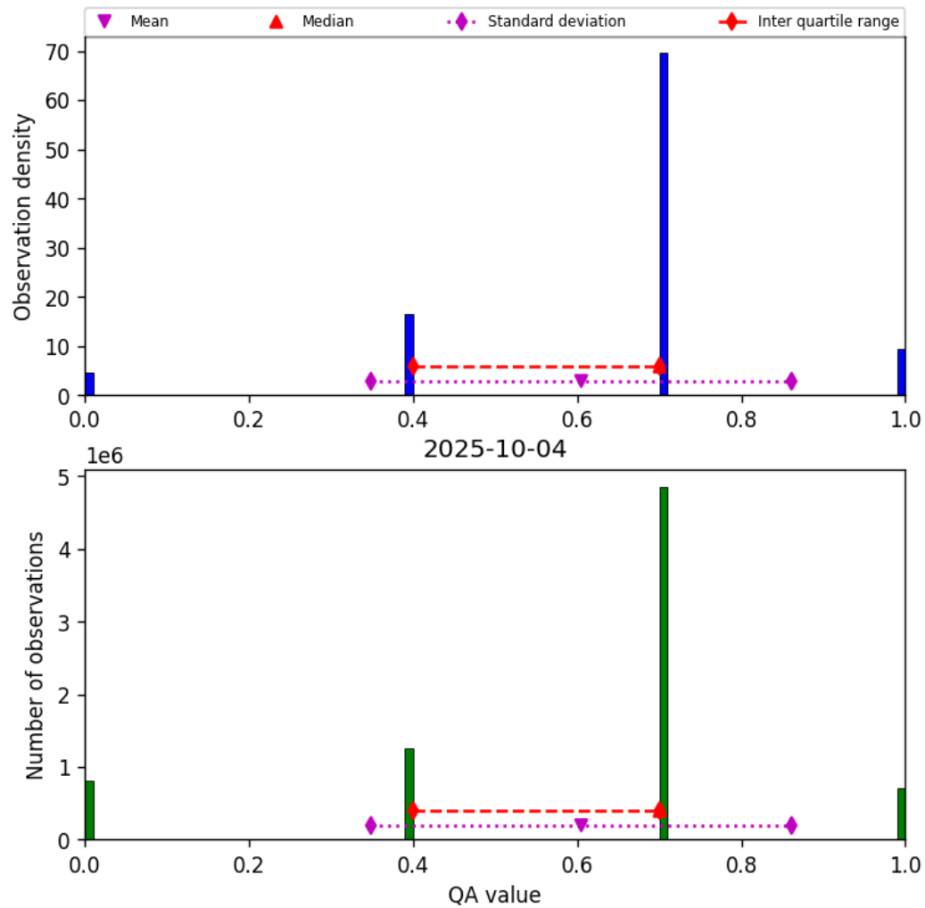
Figure 17: Histogram of “QA value” for 2025-10-03 to 2025-10-05
