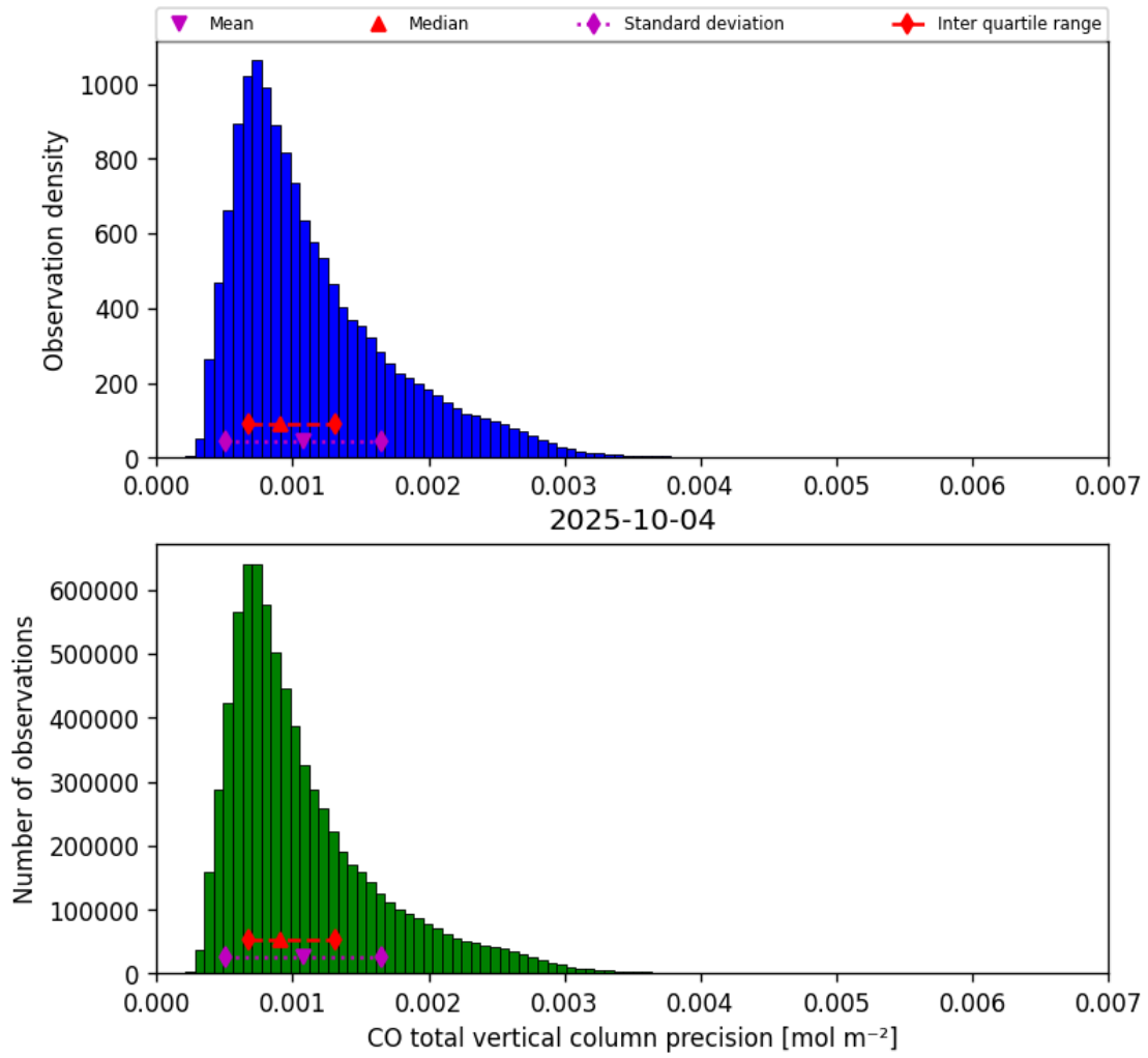
Figure 20: Histogram of “CO total vertical column precision” for 2025-10-03 to 2025-10-05
