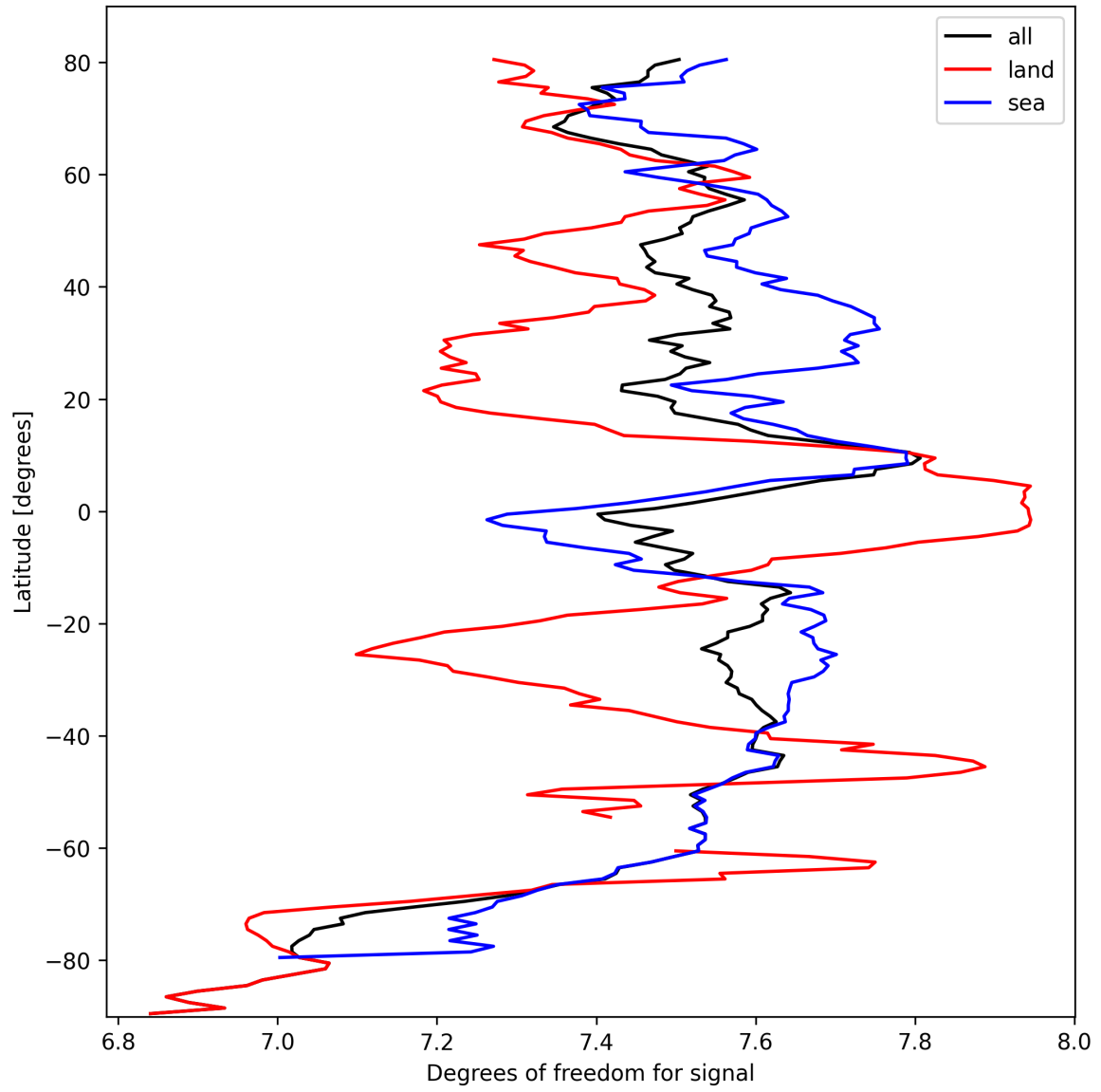
Figure 15: Zonal average of “Degrees of freedom for signal” for 2025-10-03 to 2025-10-05.
