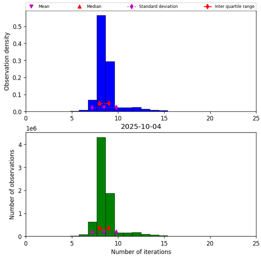
Figure 24: Histogram of “Number of iterations” for 2025-10-03 to 2025-10-05
