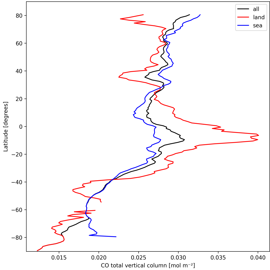
Figure 10: Zonal average of “CO total vertical column” for 2025-10-03 to 2025-10-05.
