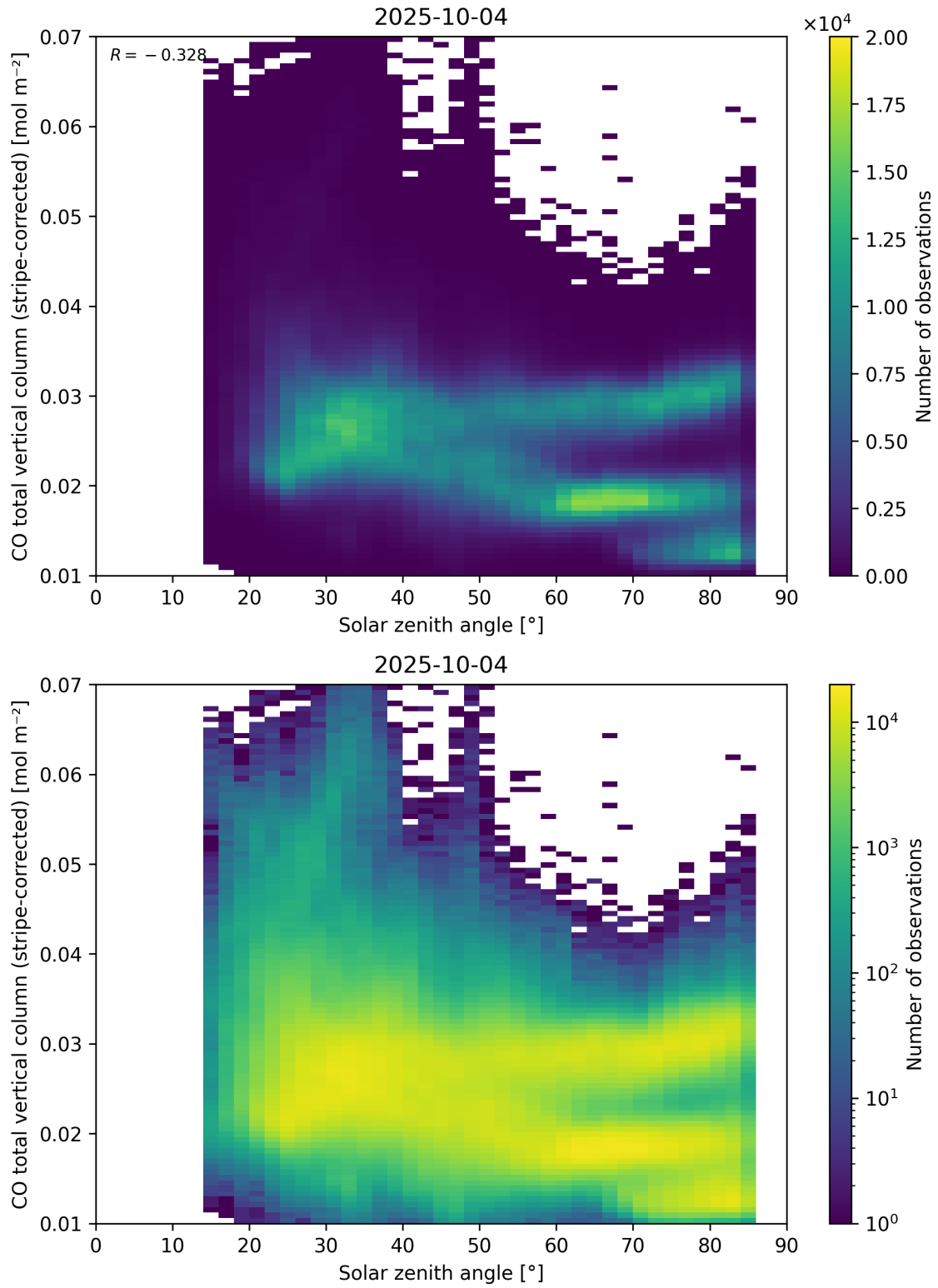
Figure 62: Scatter density plot of “Solar zenith angle” against “CO total vertical column (stripe-corrected)” for 2025-10-03 to 2025-10-05.
