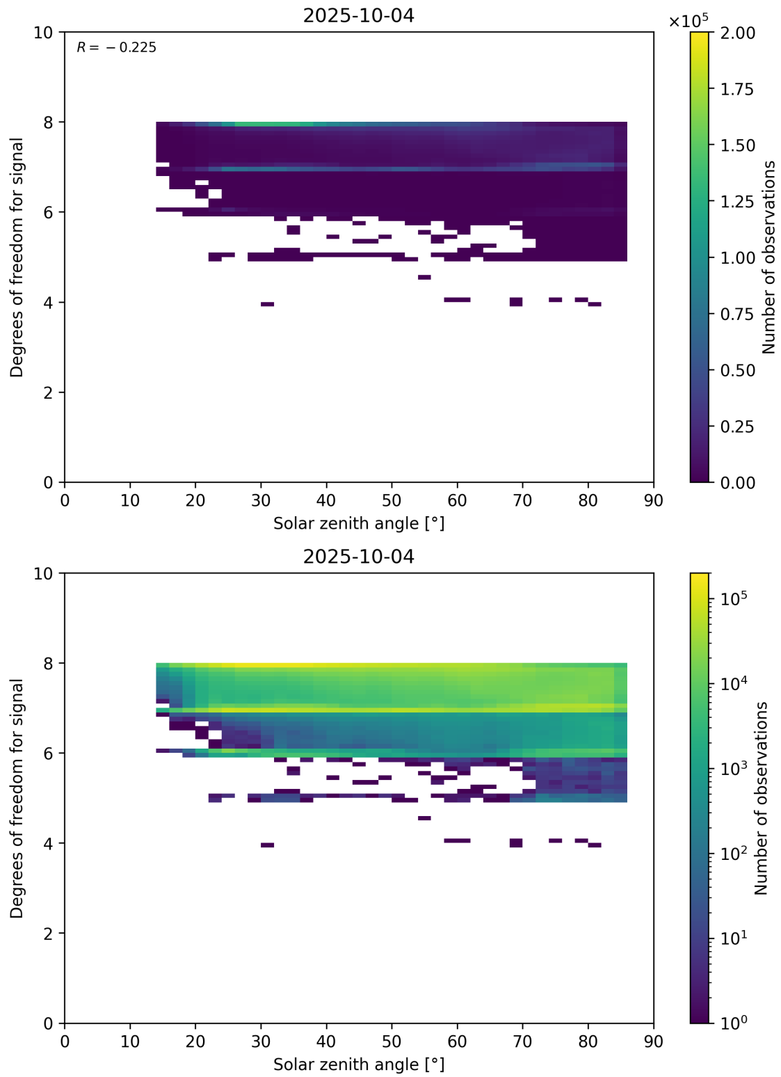
Figure 65: Scatter density plot of “Solar zenith angle” against “Degrees of freedom for signal” for 2025-10-03 to 2025-10-05.
