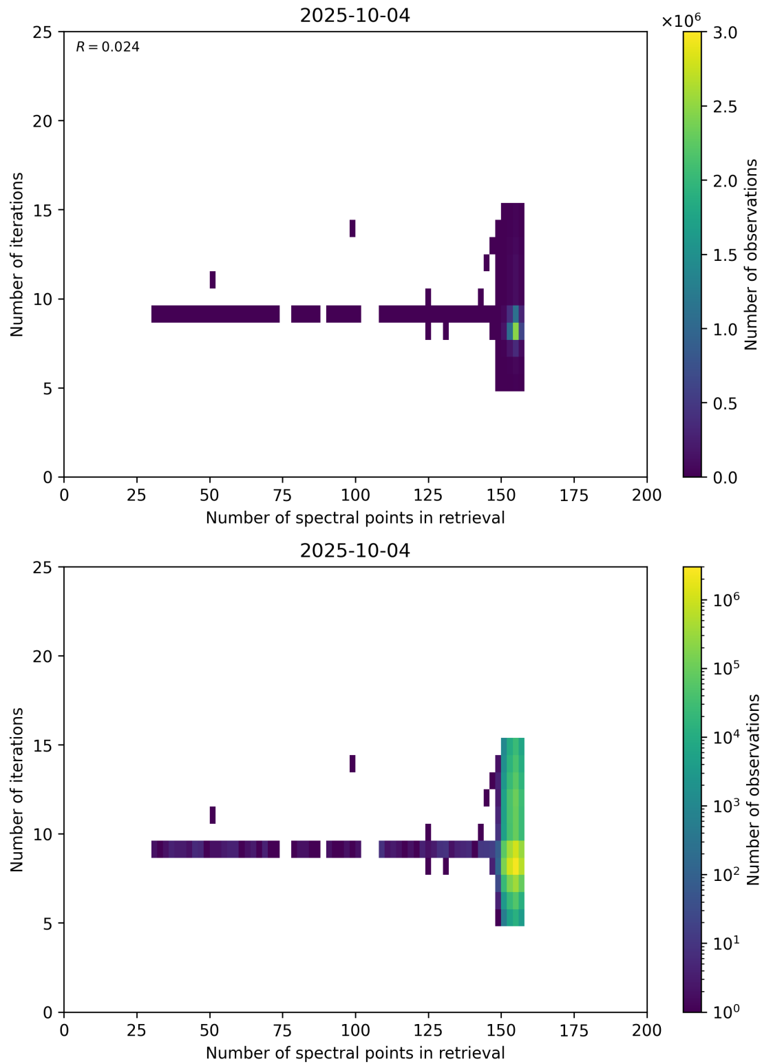
Figure 60: Scatter density plot of “Number of spectral points in retrieval” against “Number of iterations” for 2025-10-03 to 2025-10-05.
