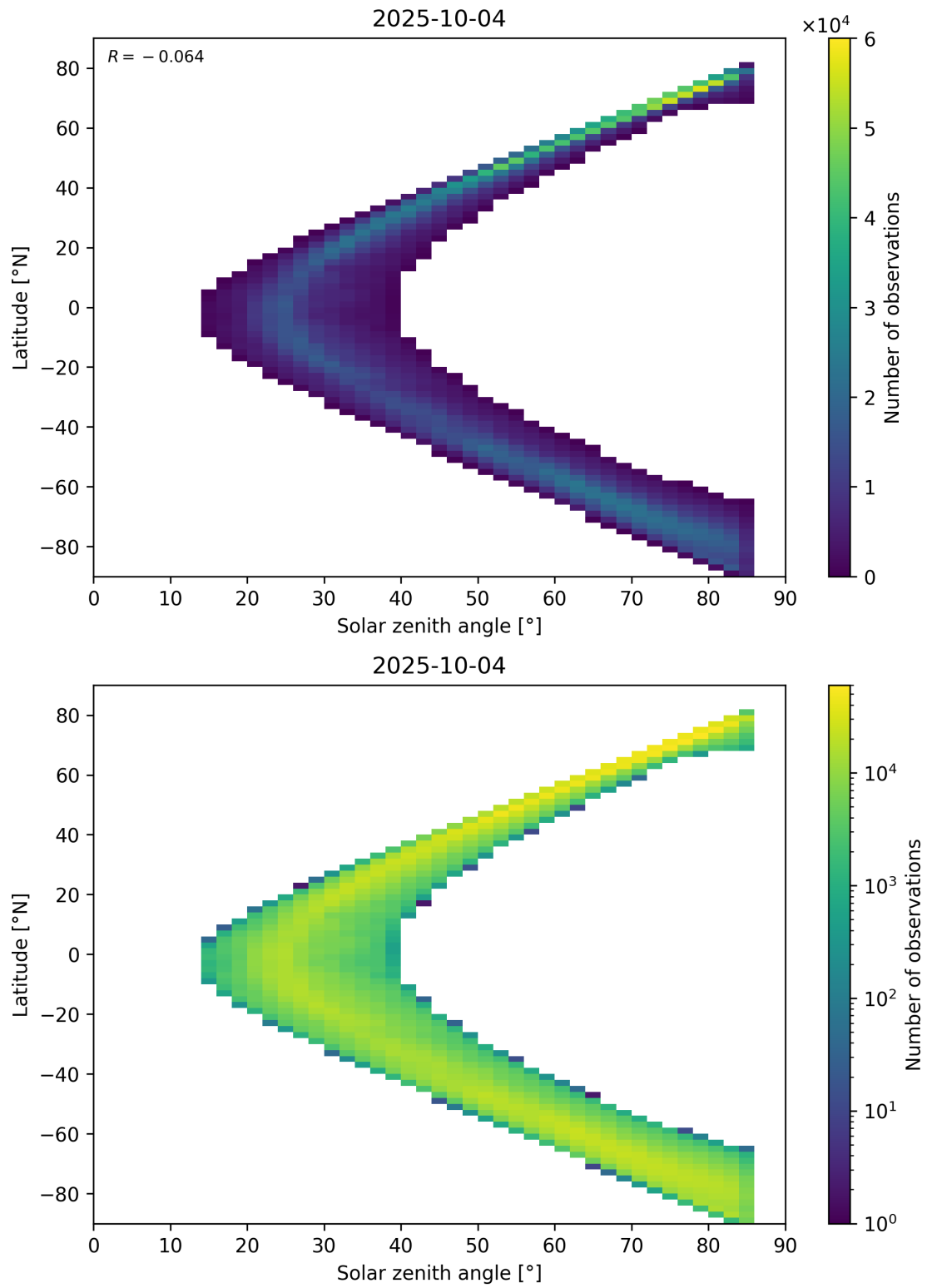
Figure 66: Scatter density plot of “Solar zenith angle” against “Latitude” for 2025-10-03 to 2025-10-05.
