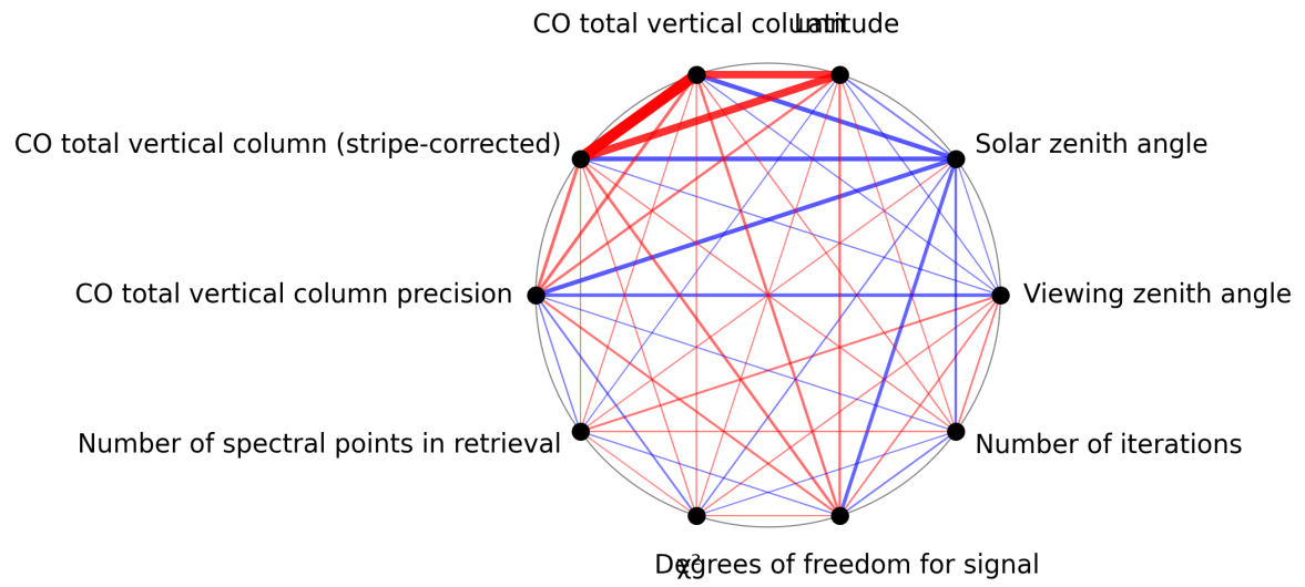
Figure 1: Map of correlation graph for 2025-10-03 to 2025-10-05.
