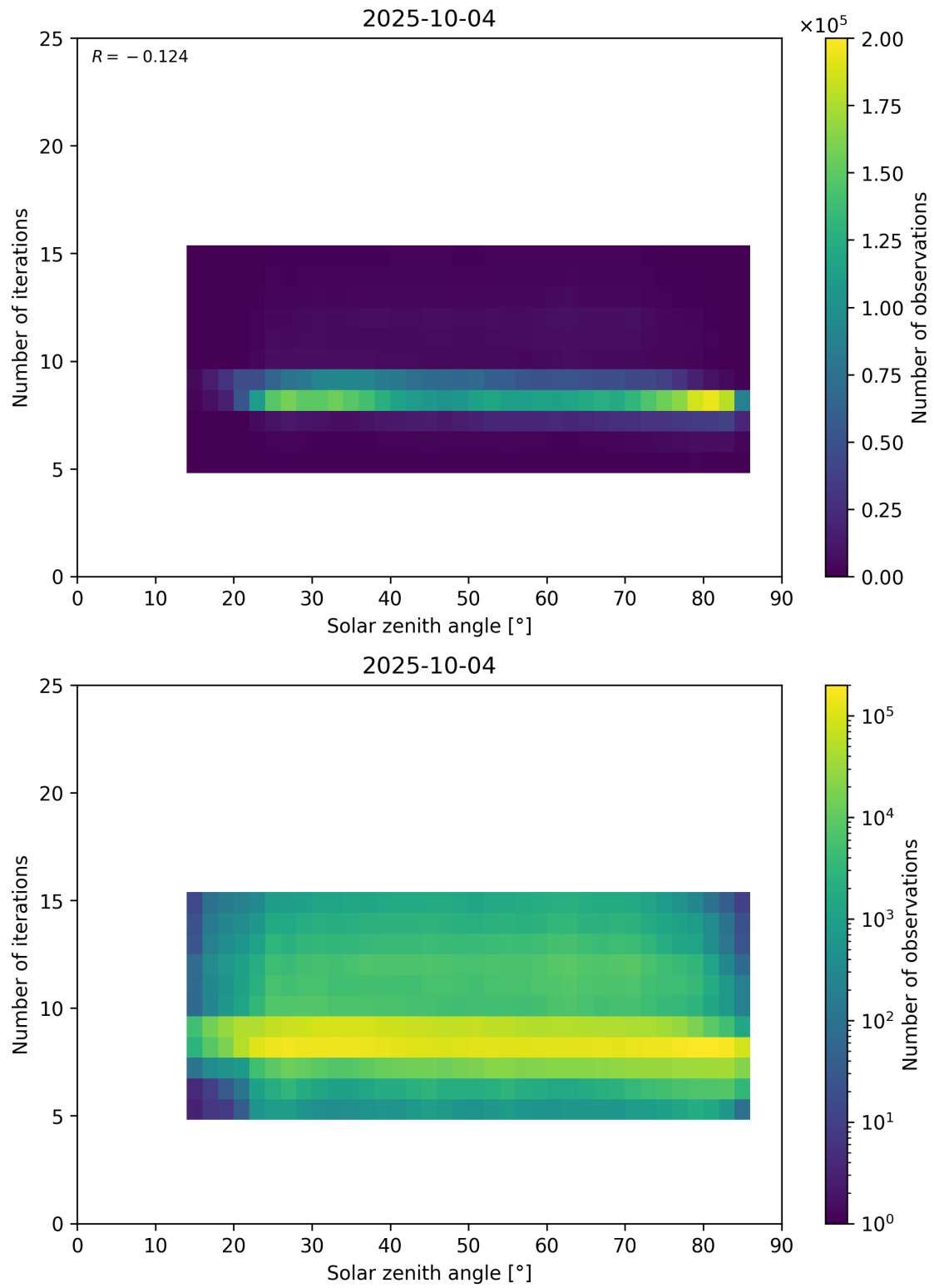
Figure 67: Scatter density plot of “Solar zenith angle” against “Number of iterations” for 2025-10-03 to 2025-10-05.
