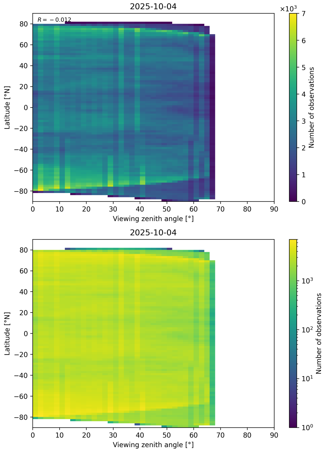
Figure 74: Scatter density plot of “Viewing zenith angle” against “Latitude” for 2025-10-03 to 2025-10-05.
