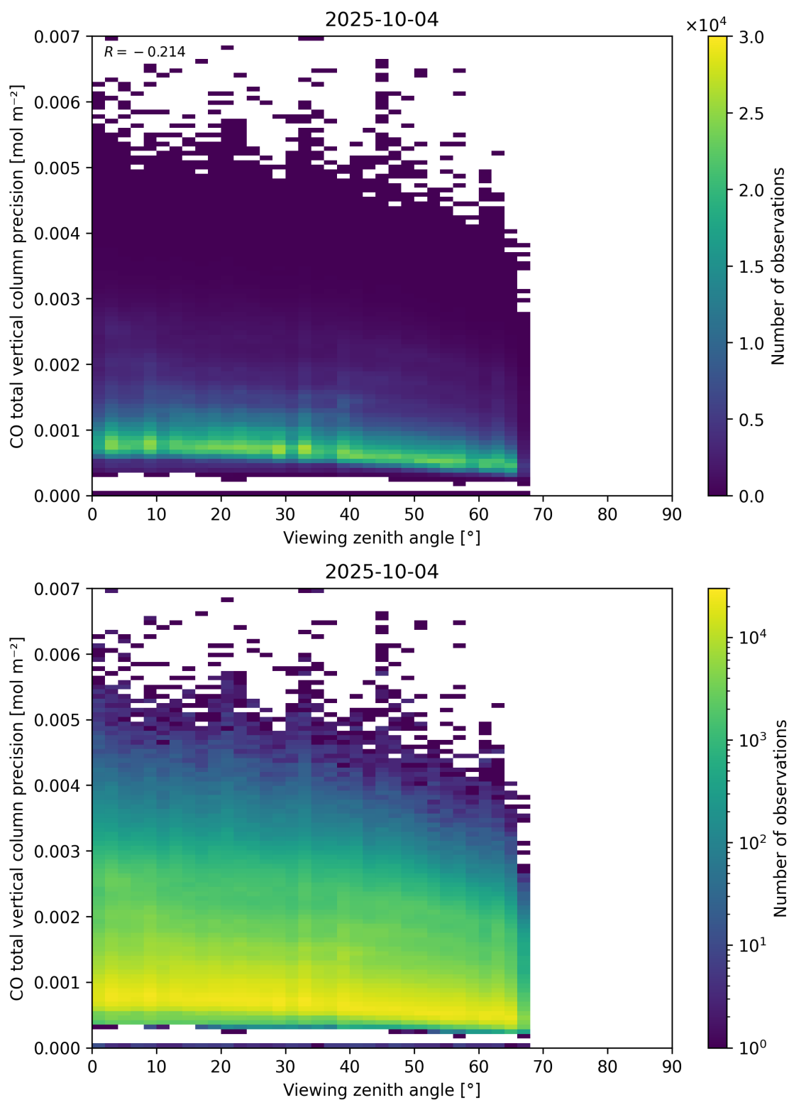
Figure 71: Scatter density plot of “Viewing zenith angle” against “CO total vertical column precision” for 2025-10-03 to 2025-10-05.
