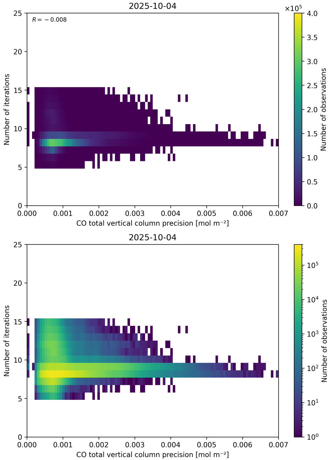
Figure 46: Scatter density plot of “CO total vertical column precision” against “Number of iterations” for 2025-10-03 to 2025-10-05.
