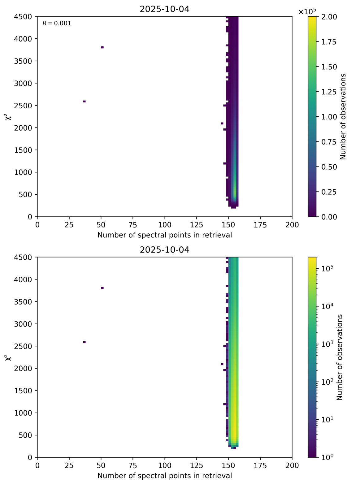
Figure 58: Scatter density plot of “Number of spectral points in retrieval” against “ \chi^2 ” for 2025-10-03 to 2025-10-05.
