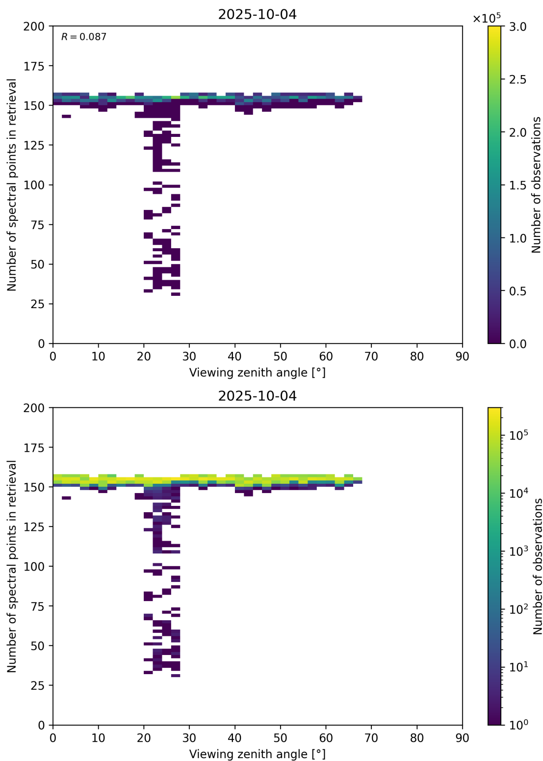
Figure 76: Scatter density plot of “Viewing zenith angle” against “Number of spectral points in retrieval” for 2025-10-03 to 2025-10-05.
