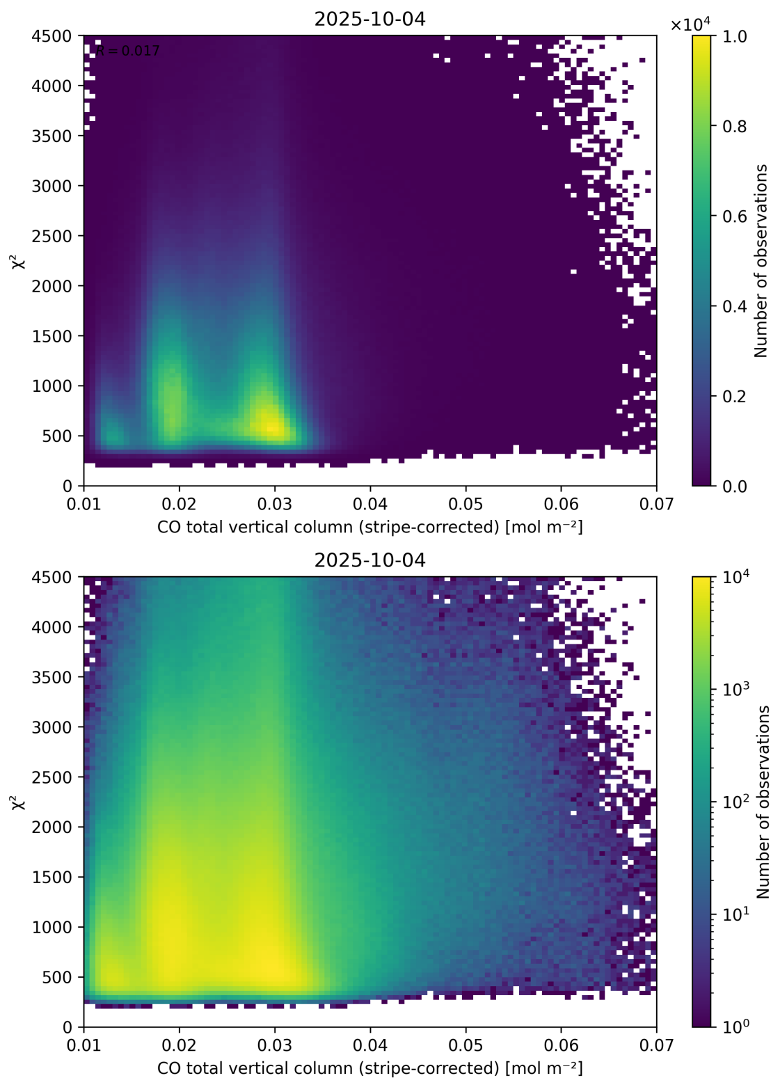
Figure 37: Scatter density plot of “CO total vertical column (stripe-corrected)” against “ \chi^2 ” for 2025-10-03 to 2025-10-05.
