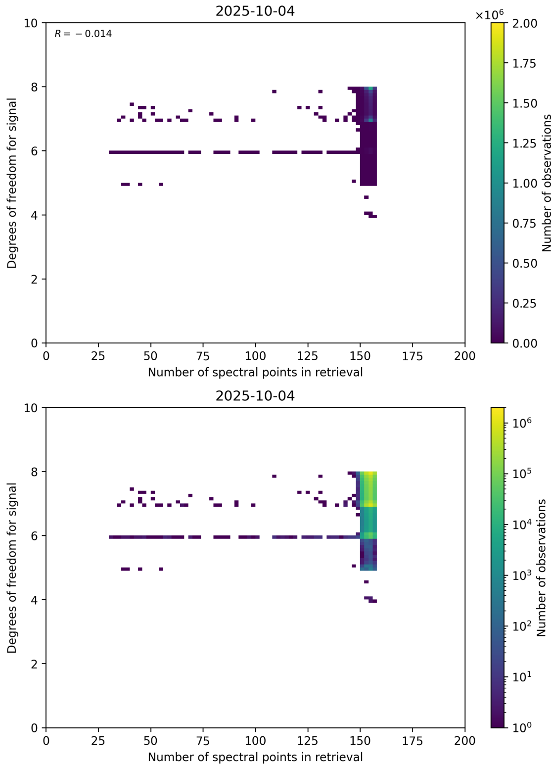
Figure 59: Scatter density plot of “Number of spectral points in retrieval” against “Degrees of freedom for signal” for 2025-10-03 to 2025-10-05.
