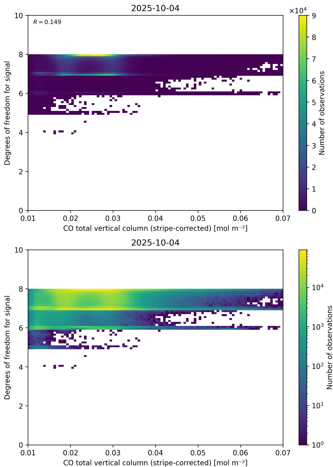
Figure 38: Scatter density plot of “CO total vertical column (stripe-corrected)” against “Degrees of freedom for signal” for 2025-10-03 to 2025-10-05.
