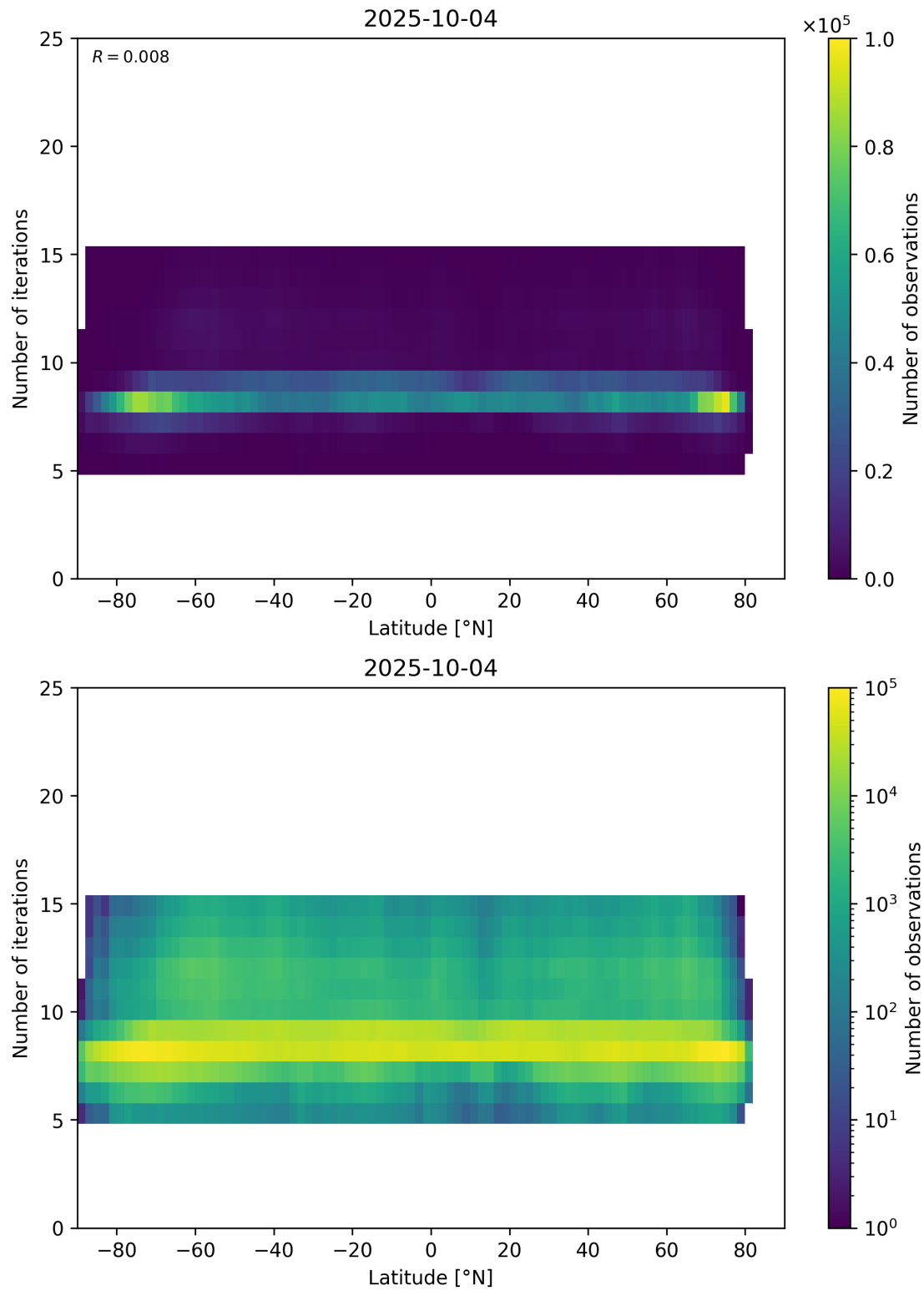
Figure 56: Scatter density plot of “Latitude” against “Number of iterations” for 2025-10-03 to 2025-10-05.
