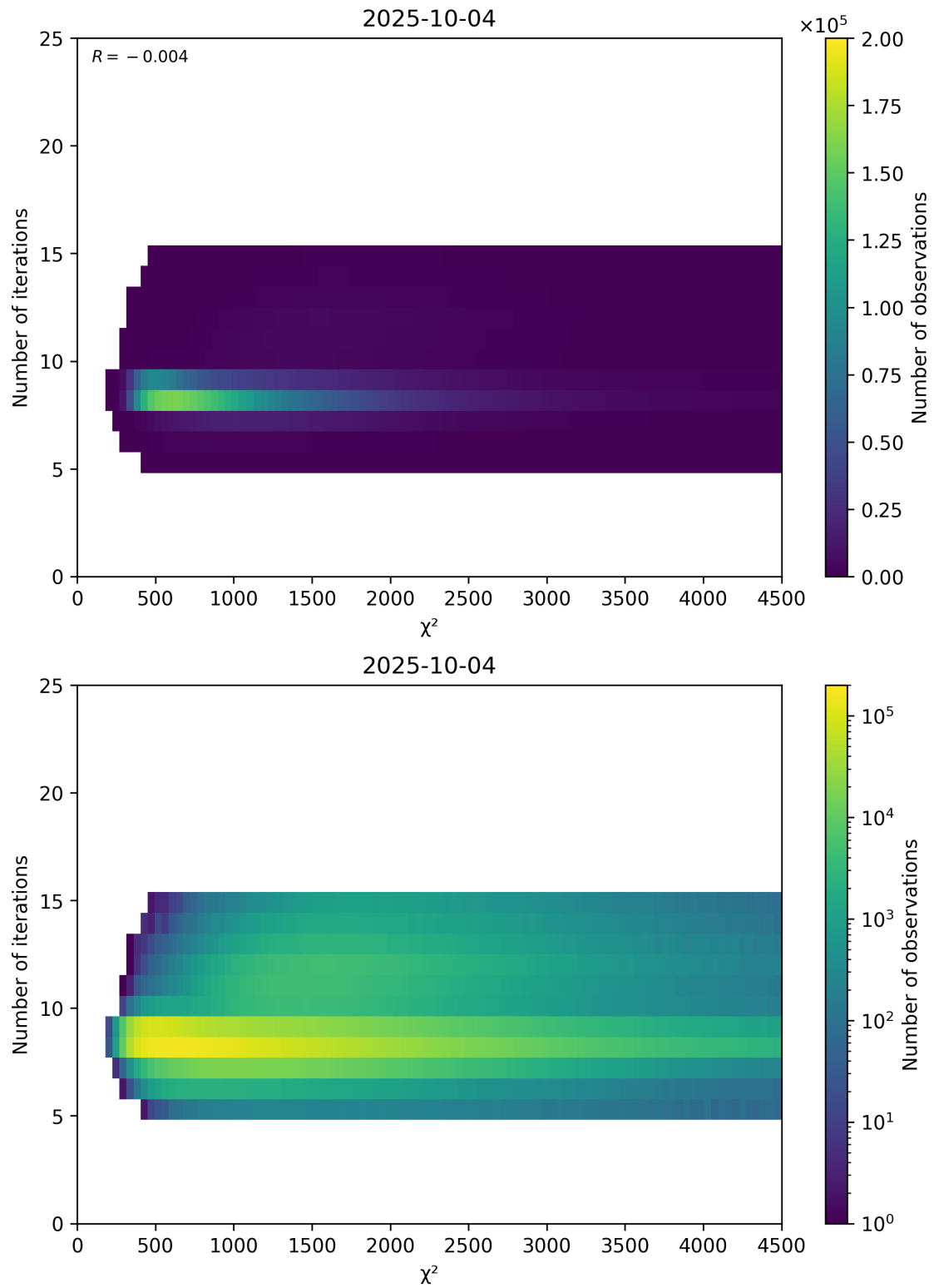
Figure 49: Scatter density plot of “ \chi^2 ” against “Number of iterations” for 2025-10-03 to 2025-10-05.
