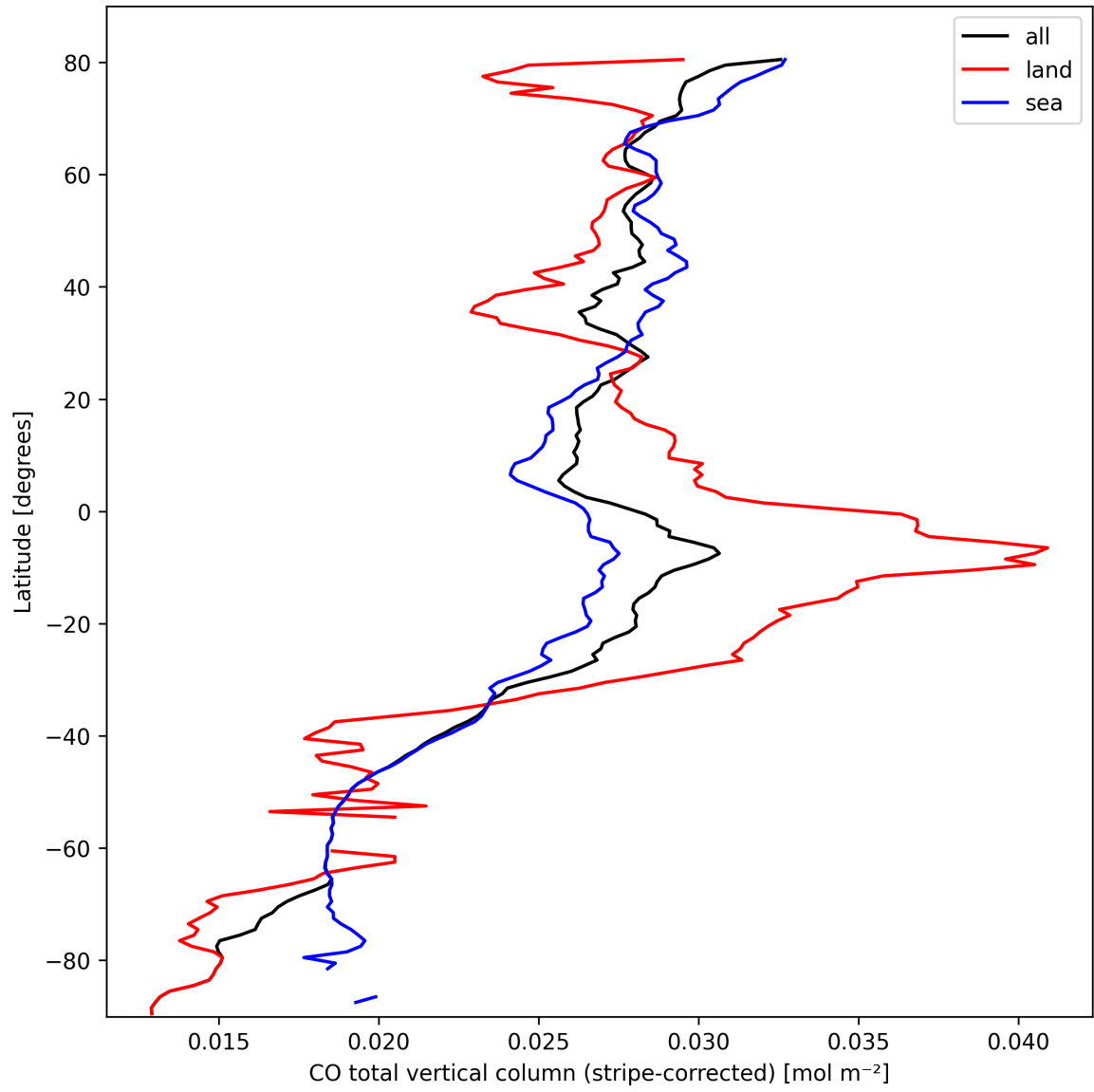
Figure 11: Zonal average of “CO total vertical column (stripe-corrected)” for 2025-10-04 to 2025-10-06.
