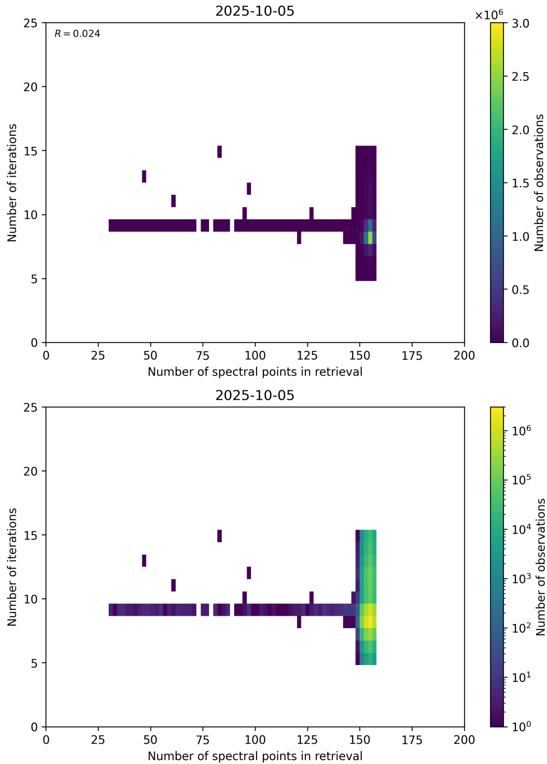
Figure 60: Scatter density plot of “Number of spectral points in retrieval” against “Number of iterations” for 2025-10-04 to 2025-10-06.
