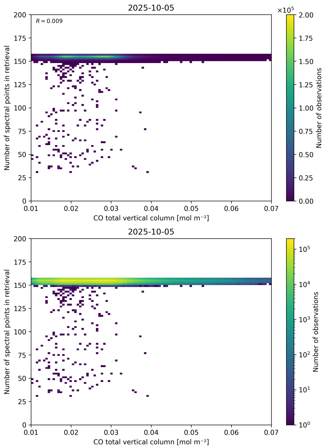
Figure 43: Scatter density plot of “CO total vertical column” against “Number of spectral points in retrieval” for 2025-10-04 to 2025-10-06.
