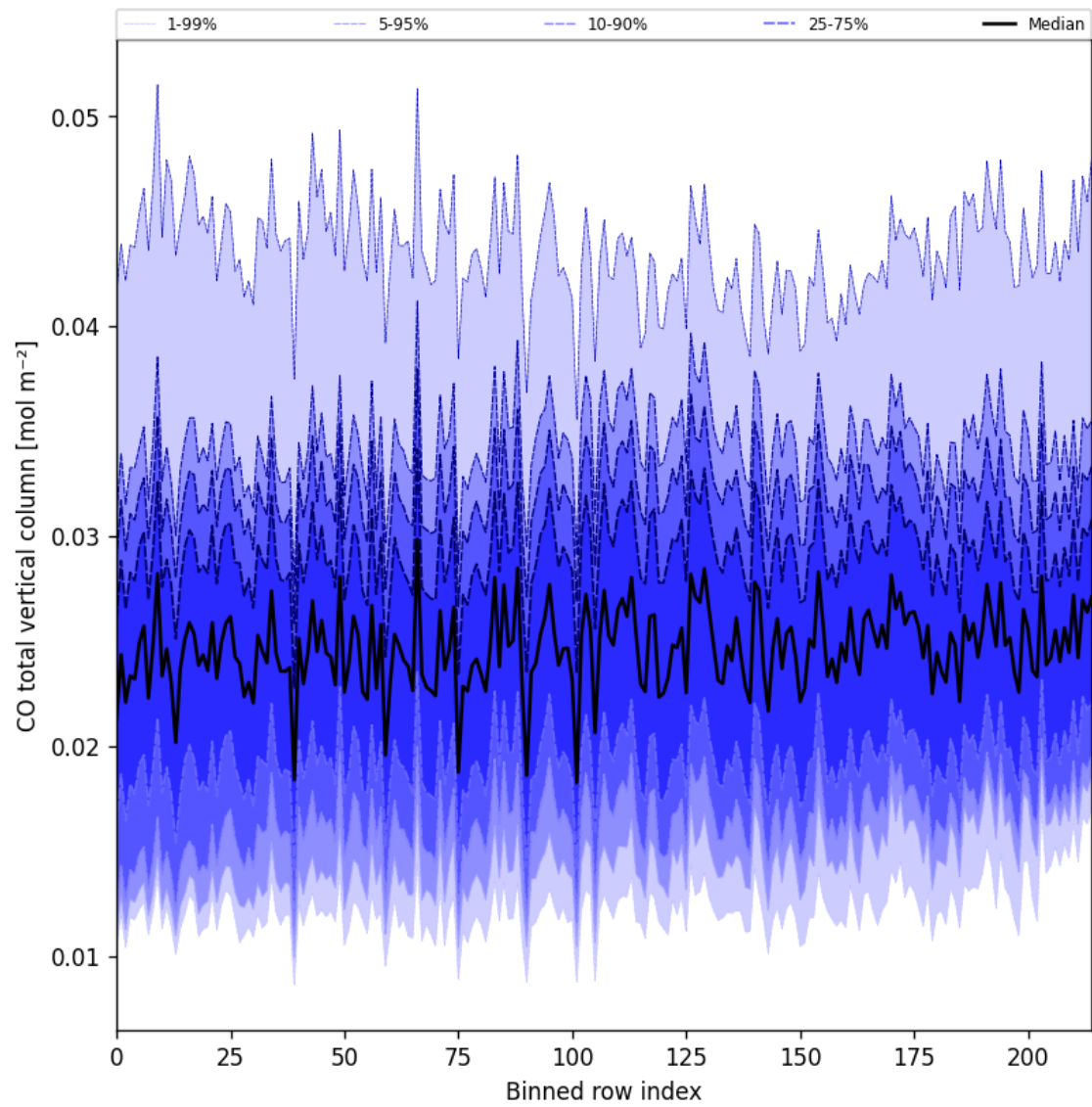
Figure 26: Along track statistics of “CO total vertical column” for 2025-10-04 to 2025-10-06
