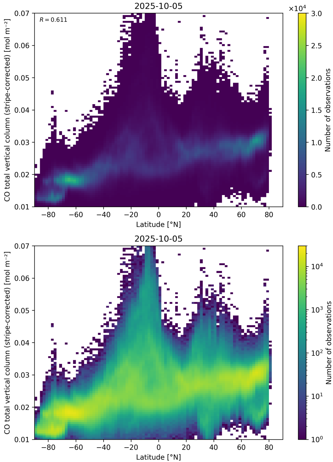
Figure 52: Scatter density plot of “Latitude” against “CO total vertical column (stripe-corrected)” for 2025-10-04 to 2025-10-06.
