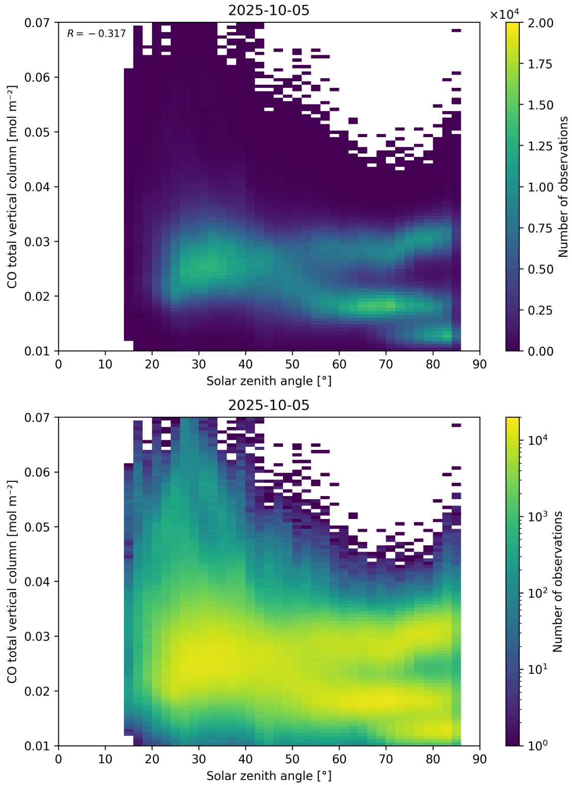
Figure 61: Scatter density plot of “Solar zenith angle” against “CO total vertical column” for 2025-10-04 to 2025-10-06.
