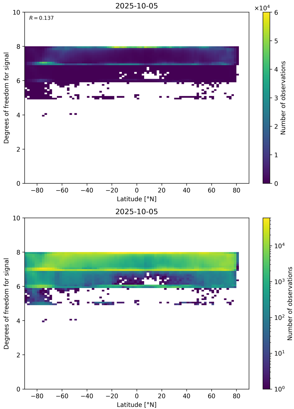
Figure 55: Scatter density plot of “Latitude” against “Degrees of freedom for signal” for 2025-10-04 to 2025-10-06.
