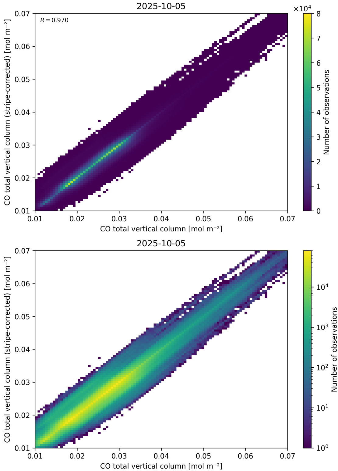
Figure 33: Scatter density plot of “CO total vertical column” against “CO total vertical column (stripe-corrected)” for 2025-10-04 to 2025-10-06.
