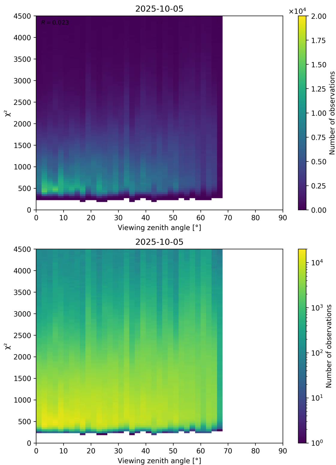
Figure 72: Scatter density plot of “Viewing zenith angle” against “ \chi^2 ” for 2025-10-04 to 2025-10-06.
