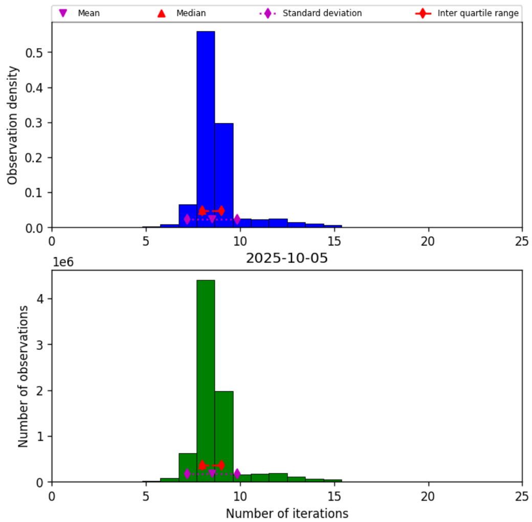
Figure 24: Histogram of “Number of iterations” for 2025-10-04 to 2025-10-06
