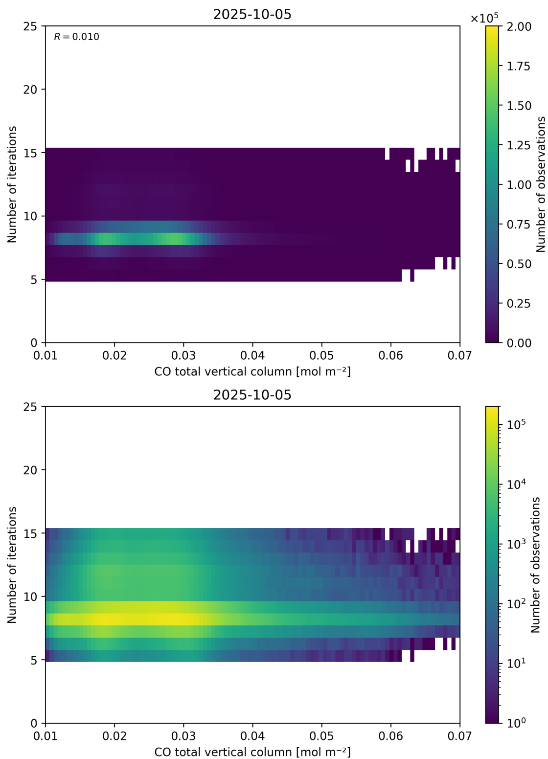
Figure 42: Scatter density plot of “CO total vertical column” against “Number of iterations” for 2025-10-04 to 2025-10-06.
