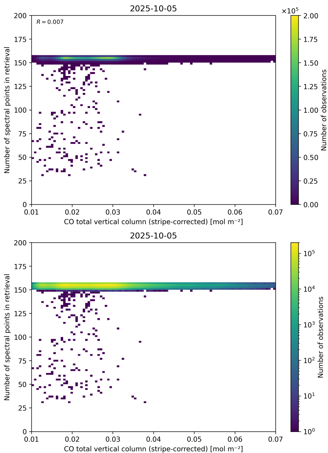
Figure 40: Scatter density plot of “CO total vertical column (stripe-corrected)” against “Number of spectral points in retrieval” for 2025-10-04 to 2025-10-06.
