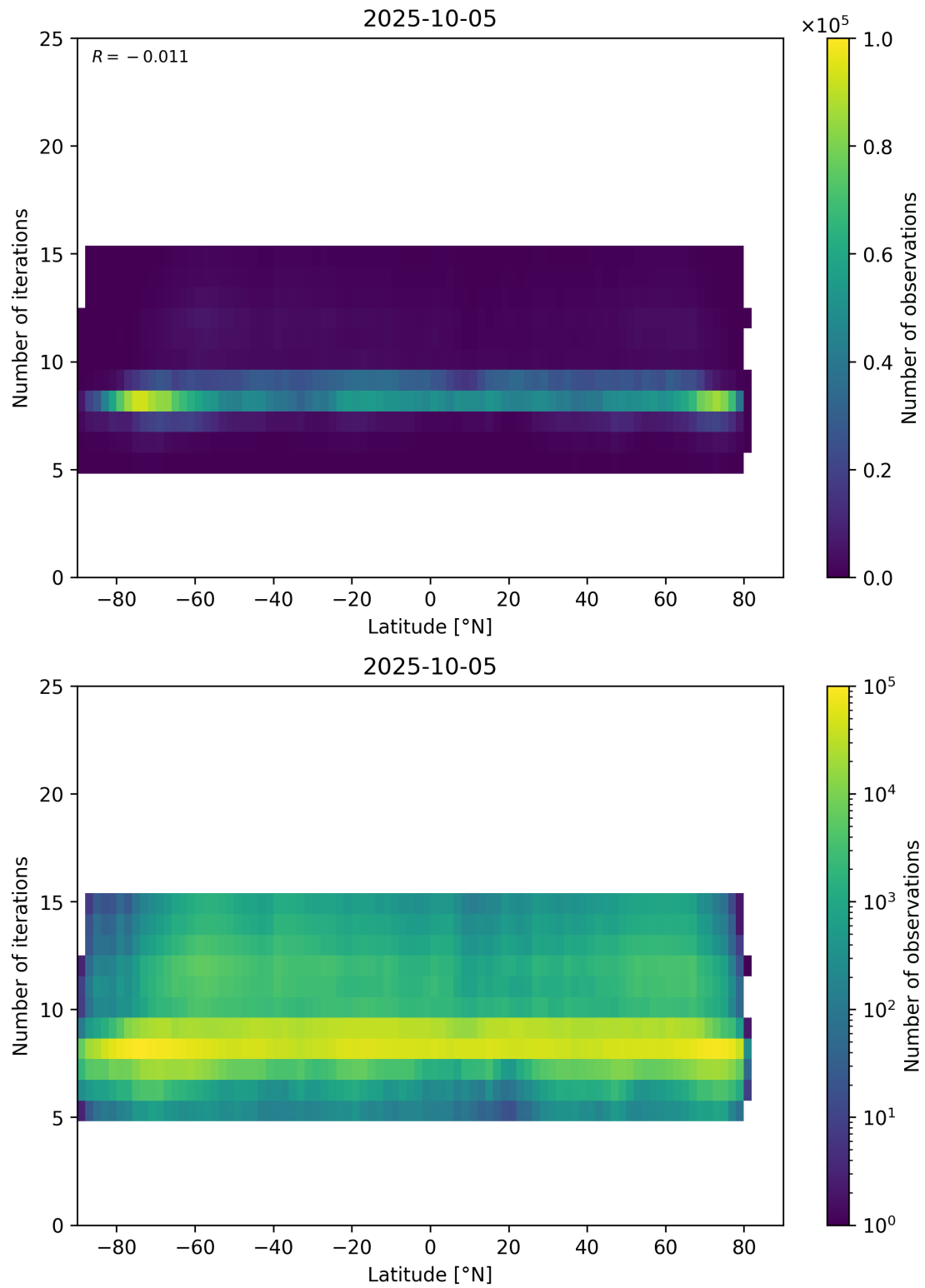
Figure 56: Scatter density plot of “Latitude” against “Number of iterations” for 2025-10-04 to 2025-10-06.
