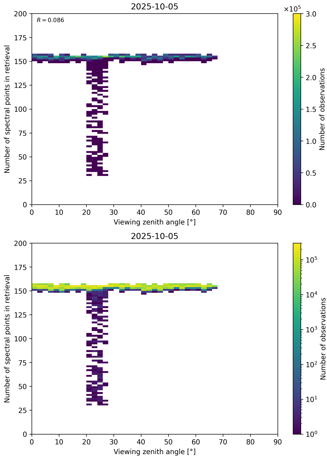
Figure 76: Scatter density plot of “Viewing zenith angle” against “Number of spectral points in retrieval” for 2025-10-04 to 2025-10-06.
