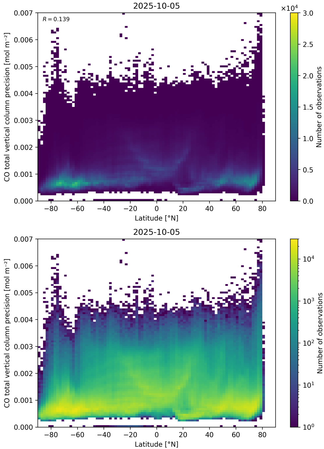
Figure 53: Scatter density plot of “Latitude” against “CO total vertical column precision” for 2025-10-04 to 2025-10-06.
