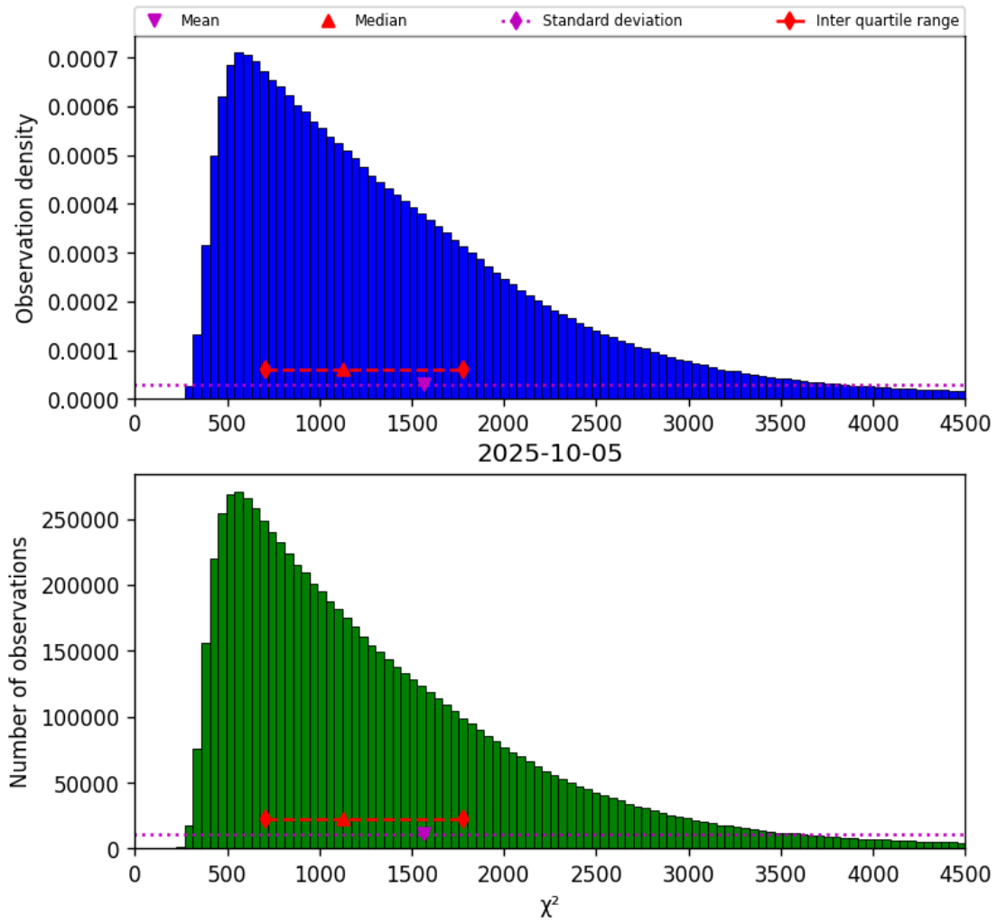
Figure 22: Histogram of “ \chi^2 ” for 2025-10-04 to 2025-10-06
