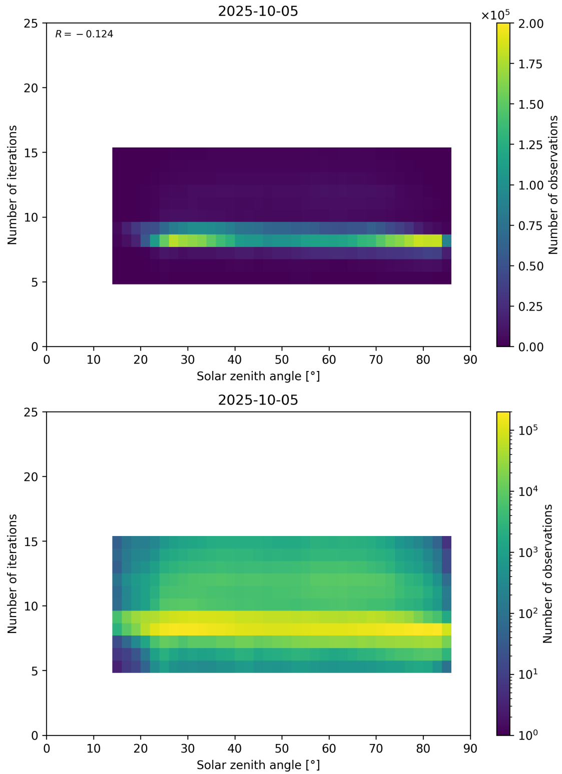
Figure 67: Scatter density plot of “Solar zenith angle” against “Number of iterations” for 2025-10-04 to 2025-10-06.
