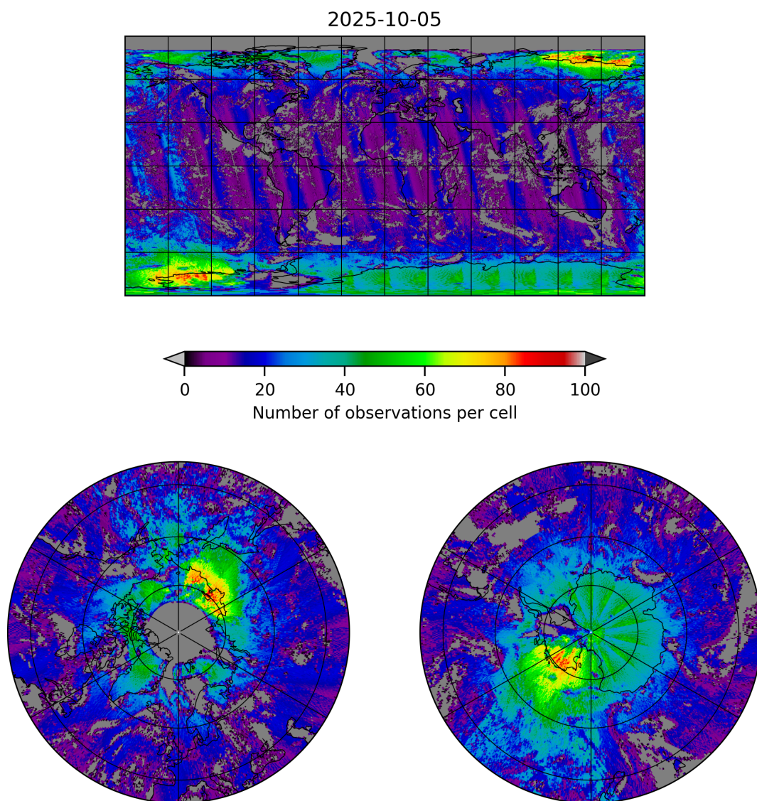
Figure 8: Map of the number of observations for 2025-10-04 to 2025-10-06
