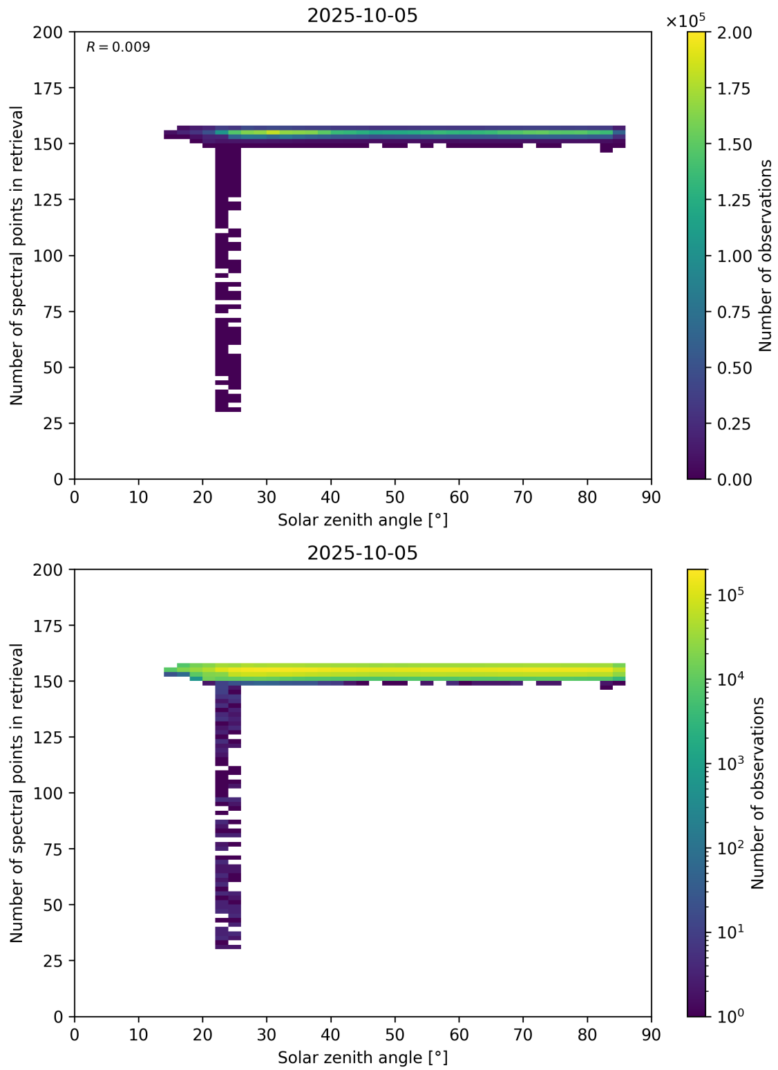
Figure 68: Scatter density plot of “Solar zenith angle” against “Number of spectral points in retrieval” for 2025-10-04 to 2025-10-06.
