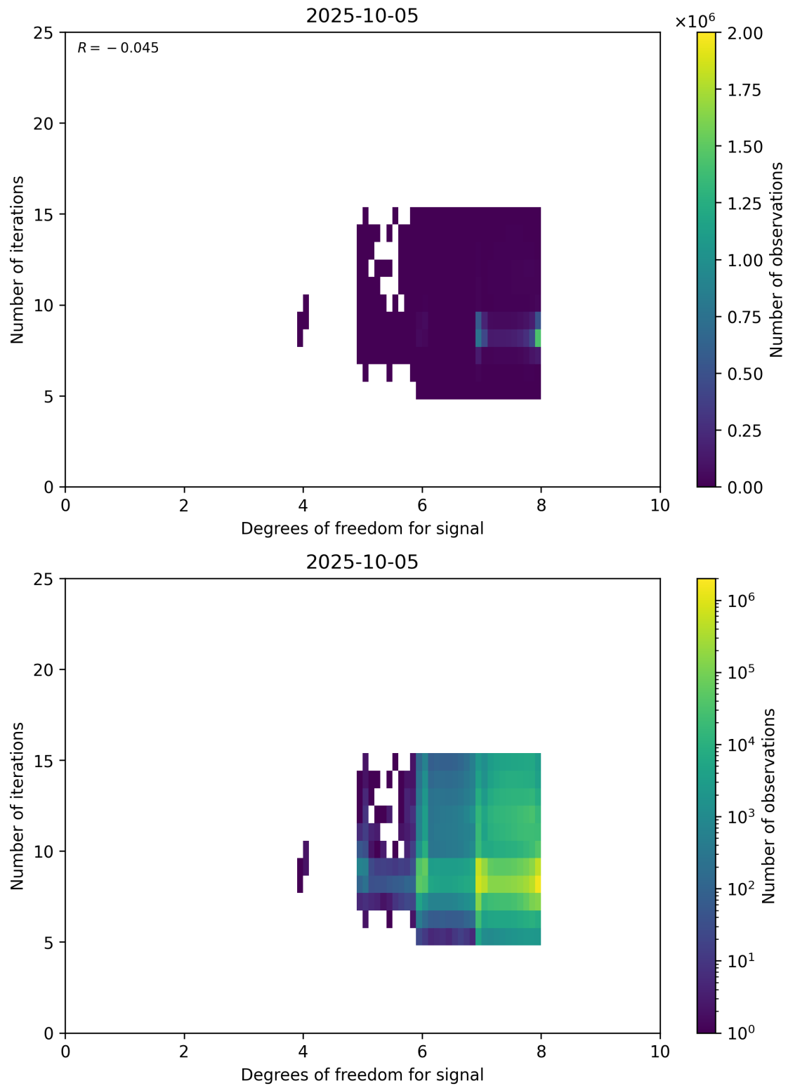
Figure 50: Scatter density plot of “Degrees of freedom for signal” against “Number of iterations” for 2025-10-04 to 2025-10-06.
