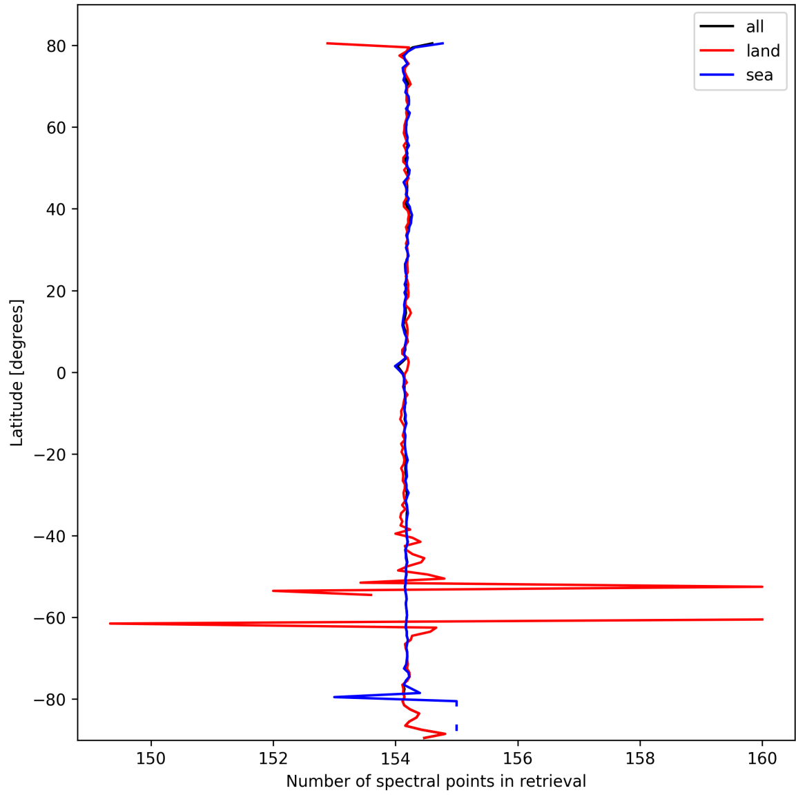
Figure 13: Zonal average of “Number of spectral points in retrieval” for 2025-10-04 to 2025-10-06.
