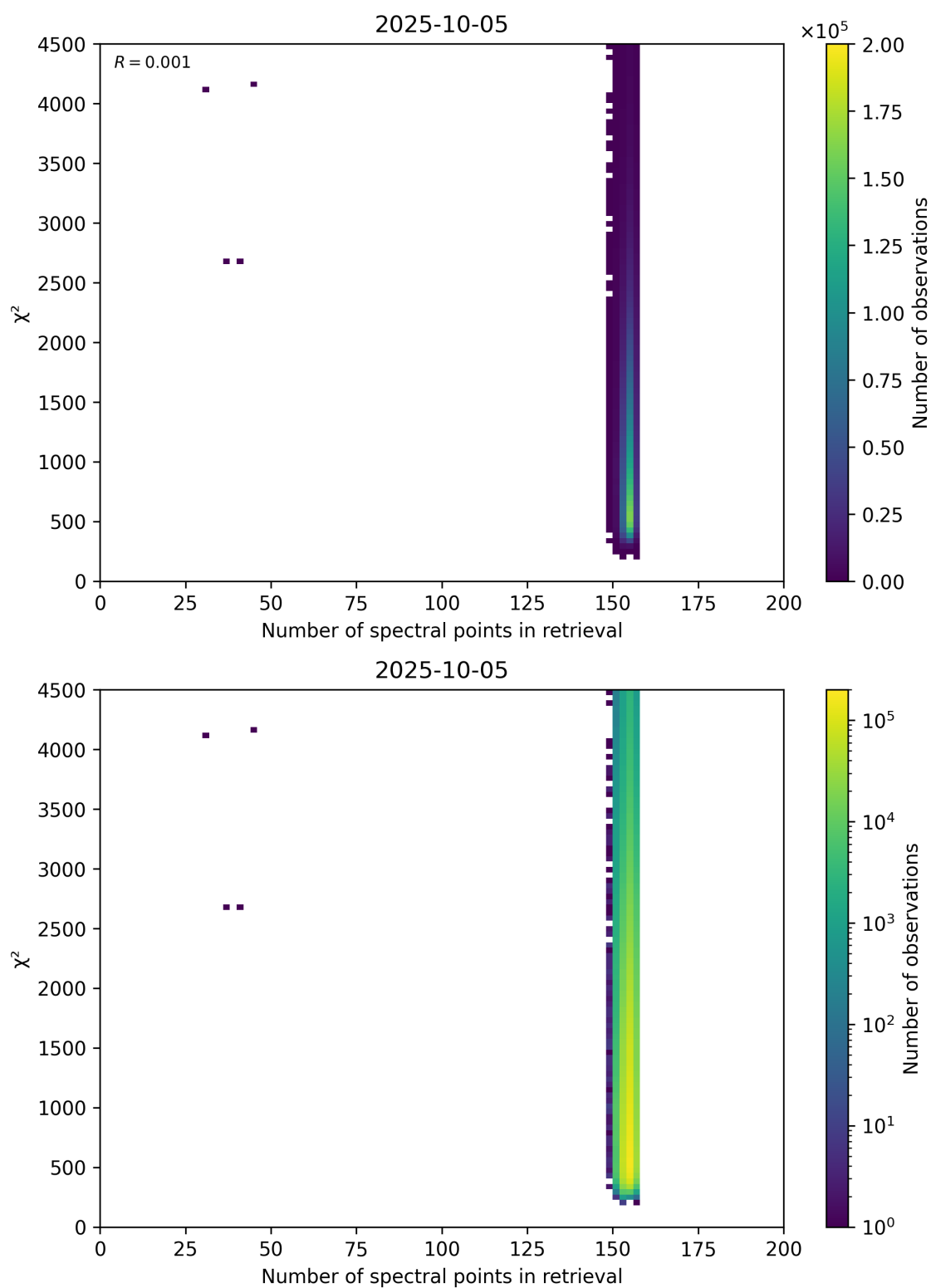
Figure 58: Scatter density plot of “Number of spectral points in retrieval” against “ \chi^2 ” for 2025-10-04 to 2025-10-06.
