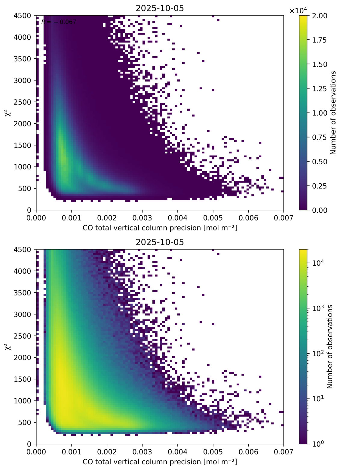
Figure 44: Scatter density plot of “CO total vertical column precision” against “ \chi^2 ” for 2025-10-04 to 2025-10-06.
