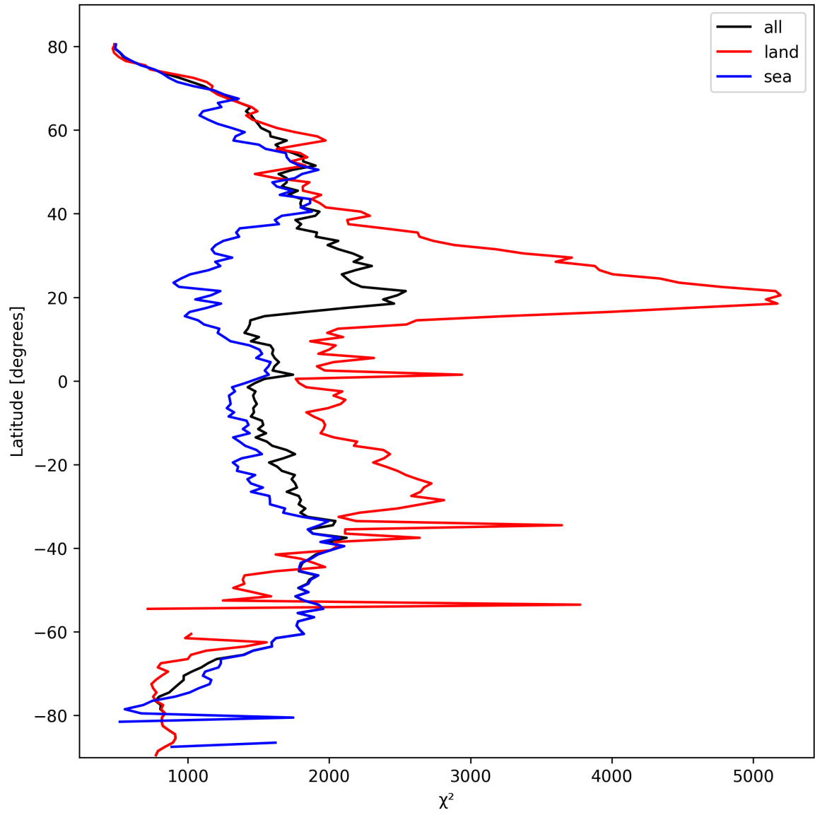
Figure 14: Zonal average of “ \chi^2 ” for 2025-10-04 to 2025-10-06.
