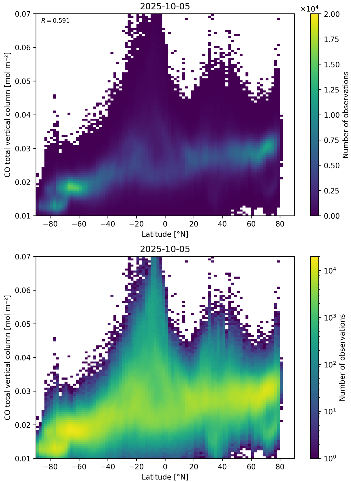
Figure 51: Scatter density plot of “Latitude” against “CO total vertical column” for 2025-10-04 to 2025-10-06.
