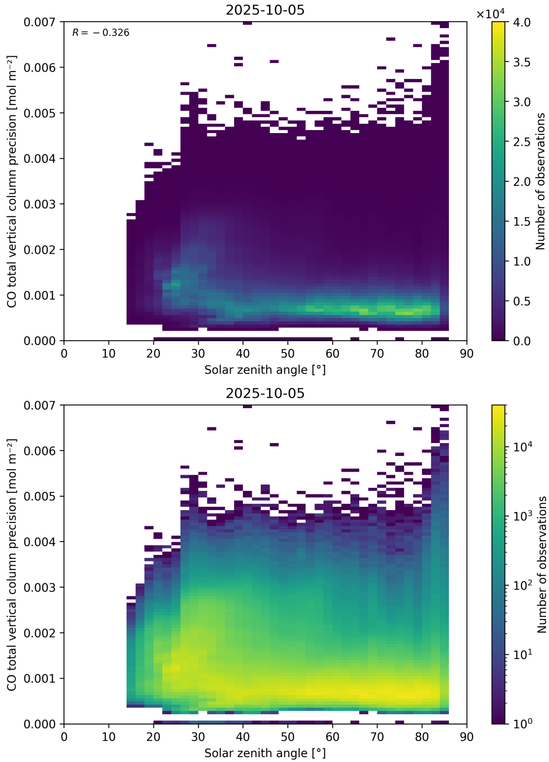
Figure 63: Scatter density plot of “Solar zenith angle” against “CO total vertical column precision” for 2025-10-04 to 2025-10-06.
