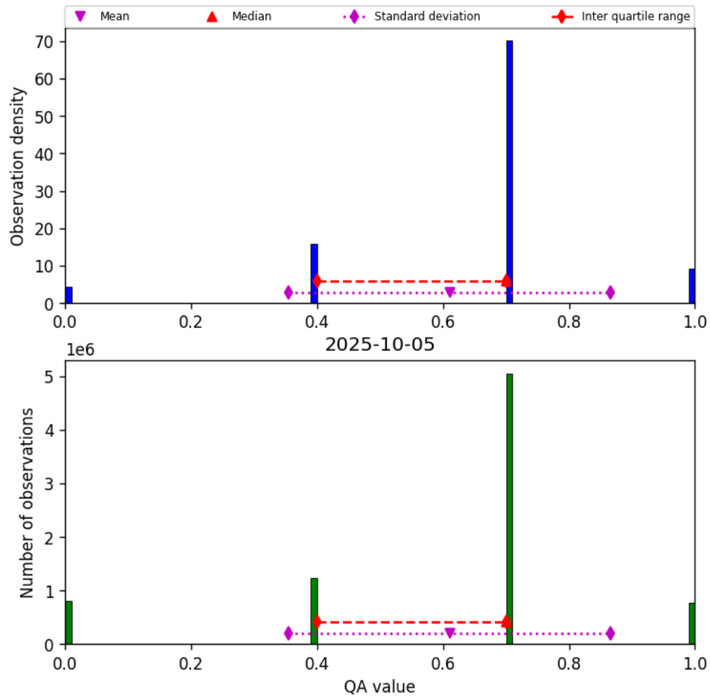
Figure 17: Histogram of “QA value” for 2025-10-04 to 2025-10-06
