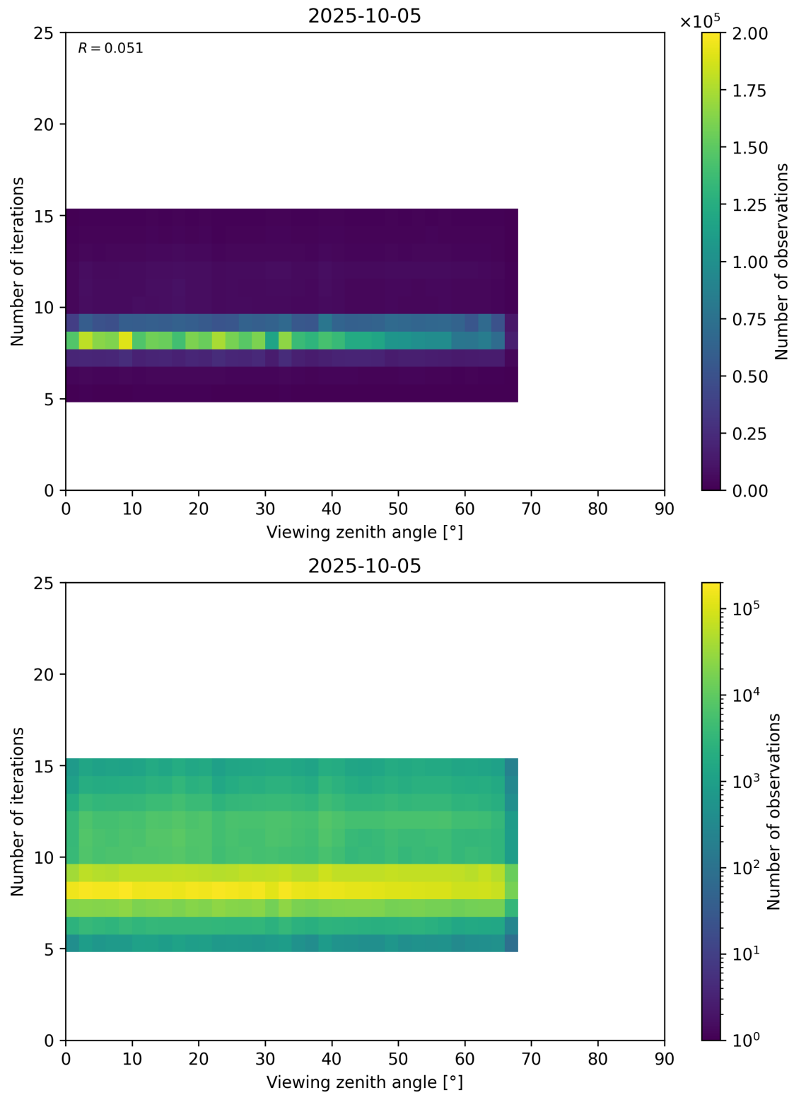
Figure 75: Scatter density plot of “Viewing zenith angle” against “Number of iterations” for 2025-10-04 to 2025-10-06.
