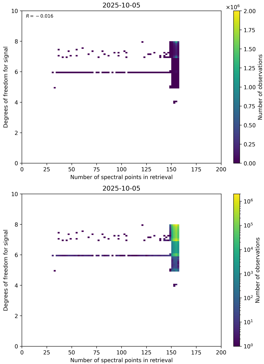
Figure 59: Scatter density plot of “Number of spectral points in retrieval” against “Degrees of freedom for signal” for 2025-10-04 to 2025-10-06.
