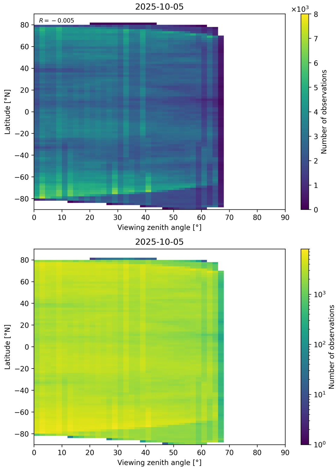
Figure 74: Scatter density plot of “Viewing zenith angle” against “Latitude” for 2025-10-04 to 2025-10-06.
