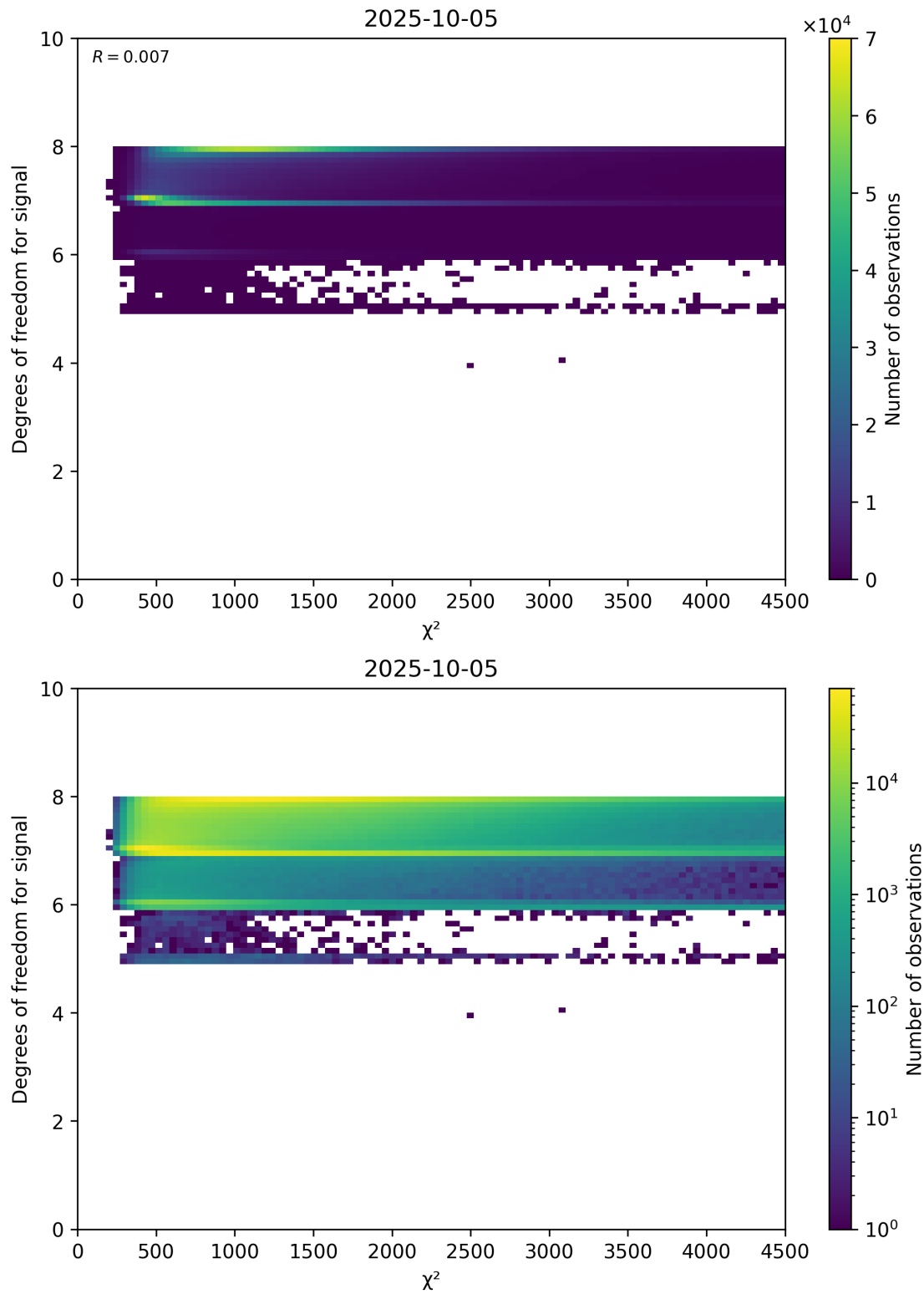
Figure 48: Scatter density plot of “ \chi^2 ” against “Degrees of freedom for signal” for 2025-10-04 to 2025-10-06.
