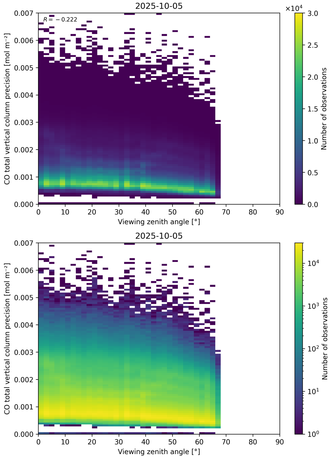
Figure 71: Scatter density plot of “Viewing zenith angle” against “CO total vertical column precision” for 2025-10-04 to 2025-10-06.
