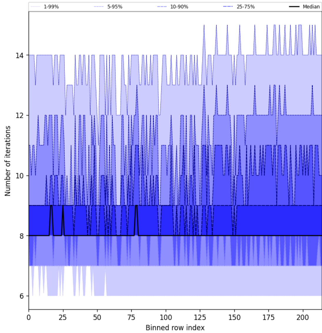
Figure 32: Along track statistics of “Number of iterations” for 2025-10-04 to 2025-10-06
