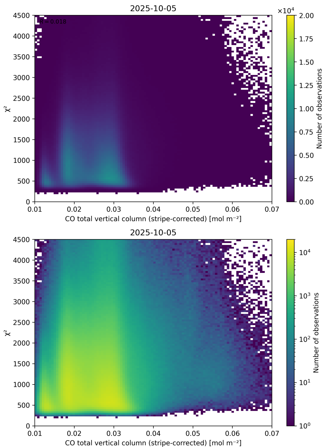
Figure 37: Scatter density plot of “CO total vertical column (stripe-corrected)” against “ \chi^2 ” for 2025-10-04 to 2025-10-06.
