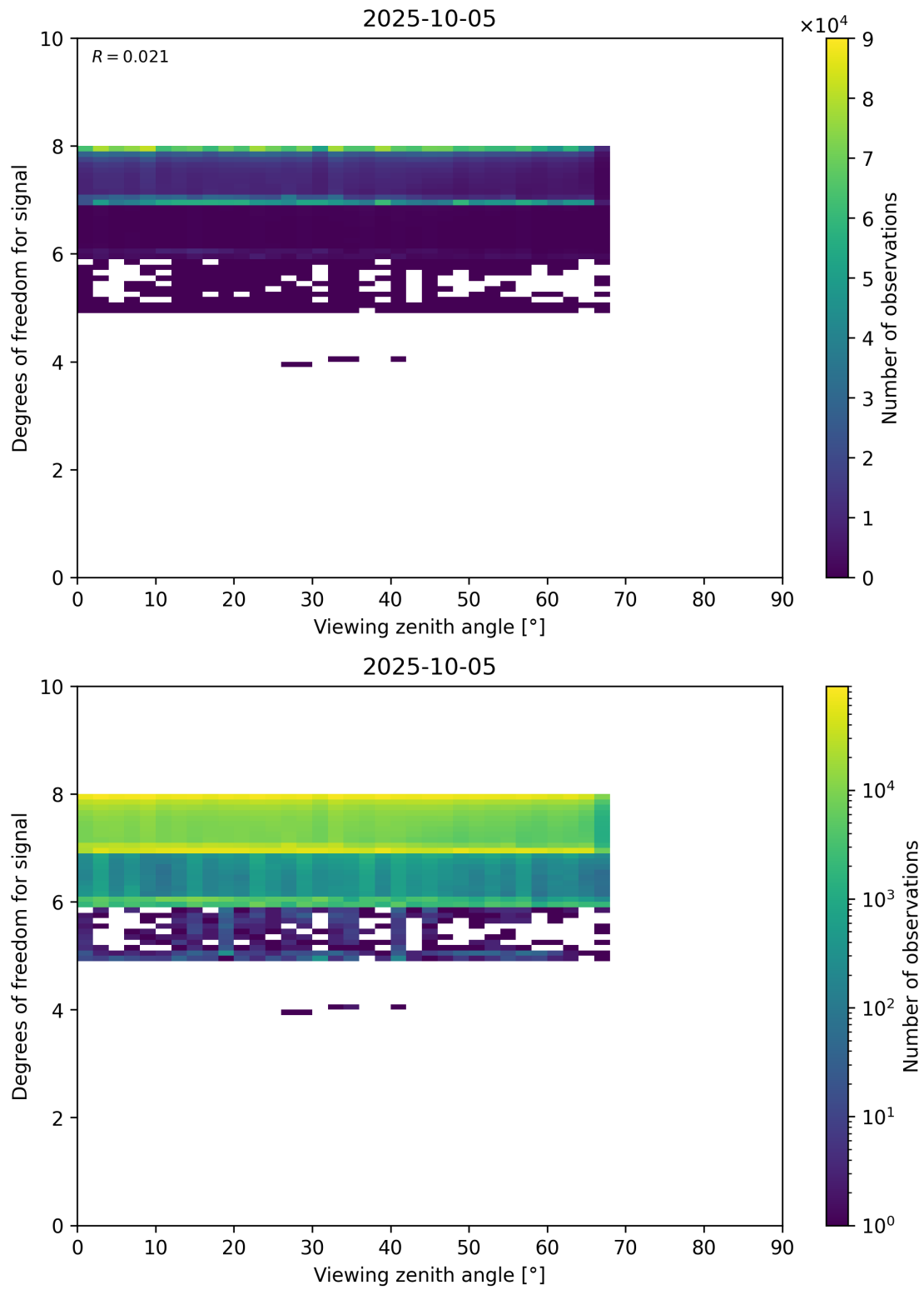
Figure 73: Scatter density plot of “Viewing zenith angle” against “Degrees of freedom for signal” for 2025-10-04 to 2025-10-06.
