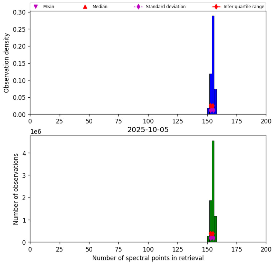
Figure 21: Histogram of “Number of spectral points in retrieval” for 2025-10-04 to 2025-10-06
