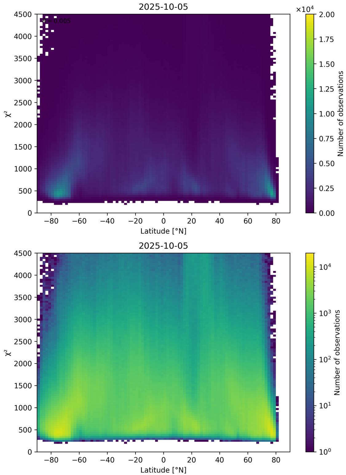
Figure 54: Scatter density plot of “Latitude” against “ \chi^2 ” for 2025-10-04 to 2025-10-06.
