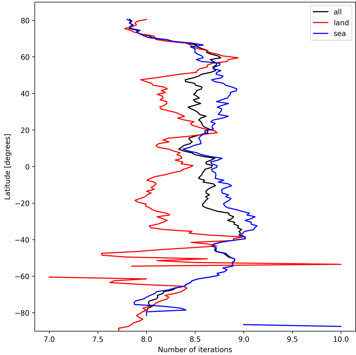
Figure 16: Zonal average of “Number of iterations” for 2025-10-04 to 2025-10-06.
