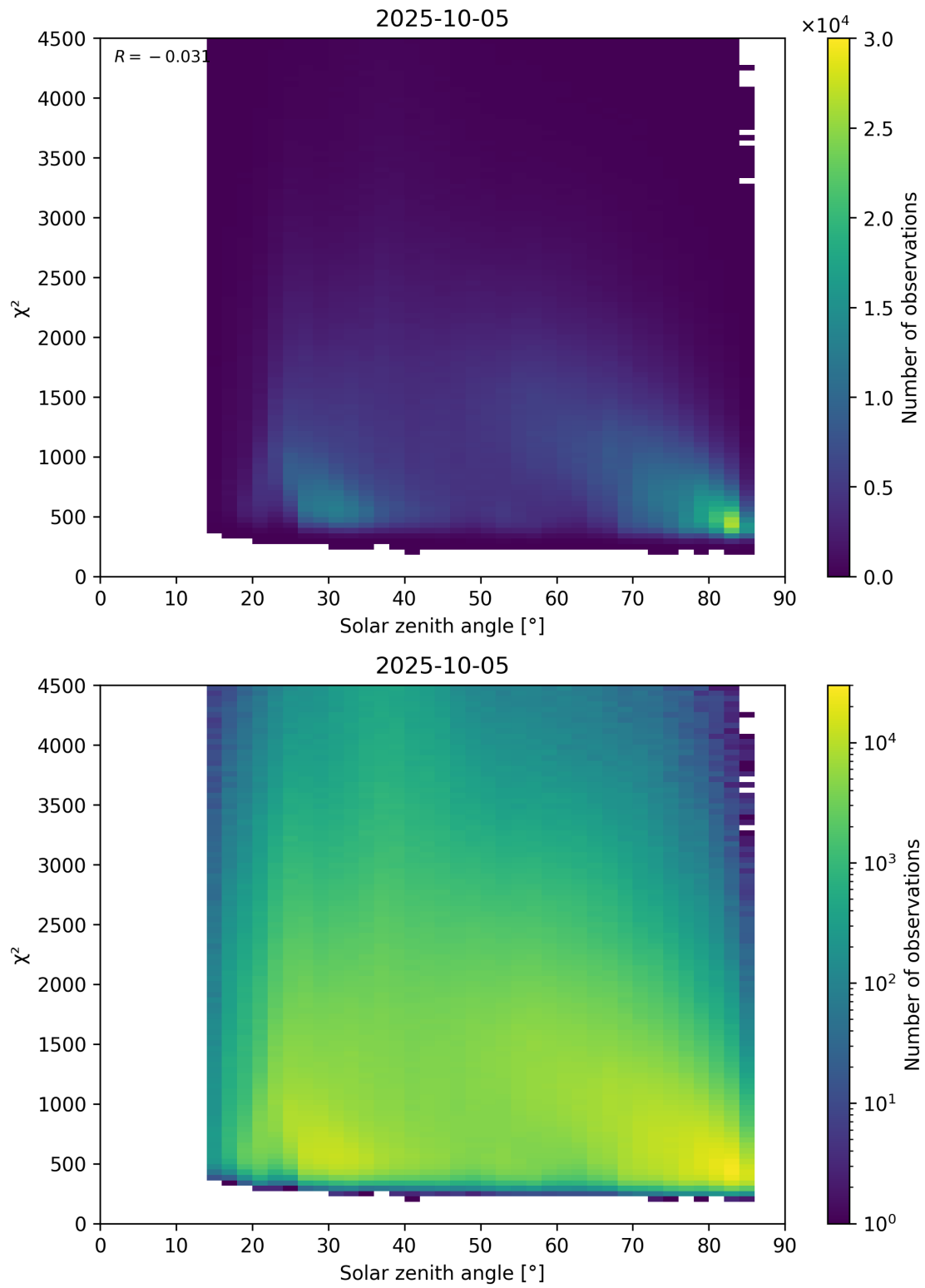
Figure 64: Scatter density plot of “Solar zenith angle” against “ \chi^2 ” for 2025-10-04 to 2025-10-06.
