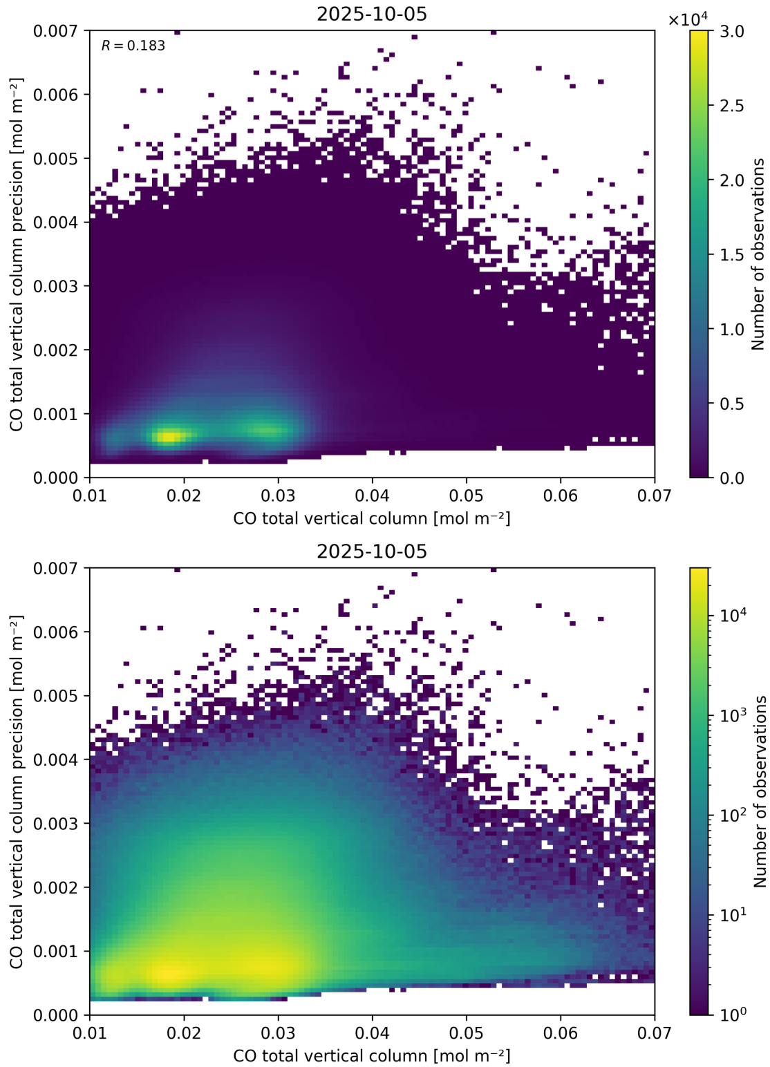
Figure 34: Scatter density plot of “CO total vertical column” against “CO total vertical column precision” for 2025-10-04 to 2025-10-06.
