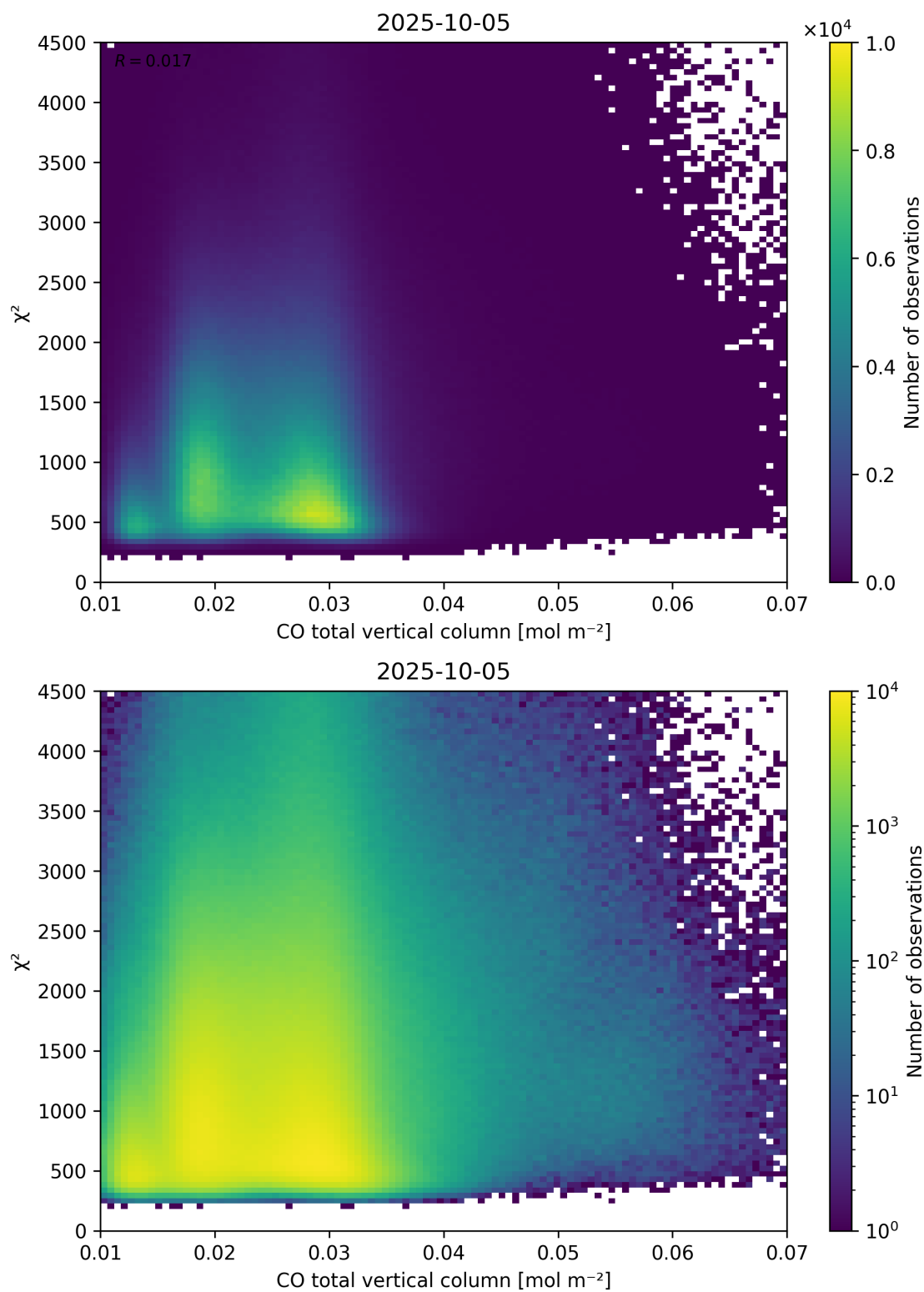
Figure 35: Scatter density plot of “CO total vertical column” against “ \chi^2 ” for 2025-10-04 to 2025-10-06.
