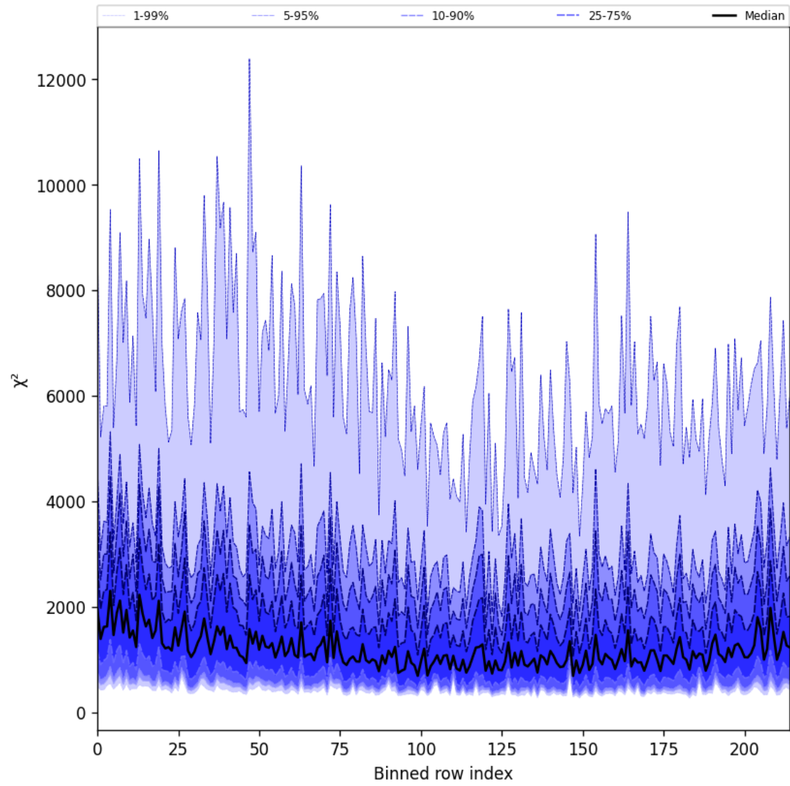
Figure 30: Along track statistics of “ \chi^2 ” for 2025-10-04 to 2025-10-06
