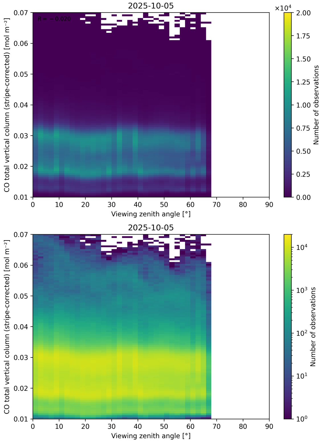
Figure 70: Scatter density plot of “Viewing zenith angle” against “CO total vertical column (stripe-corrected)” for 2025-10-04 to 2025-10-06.
