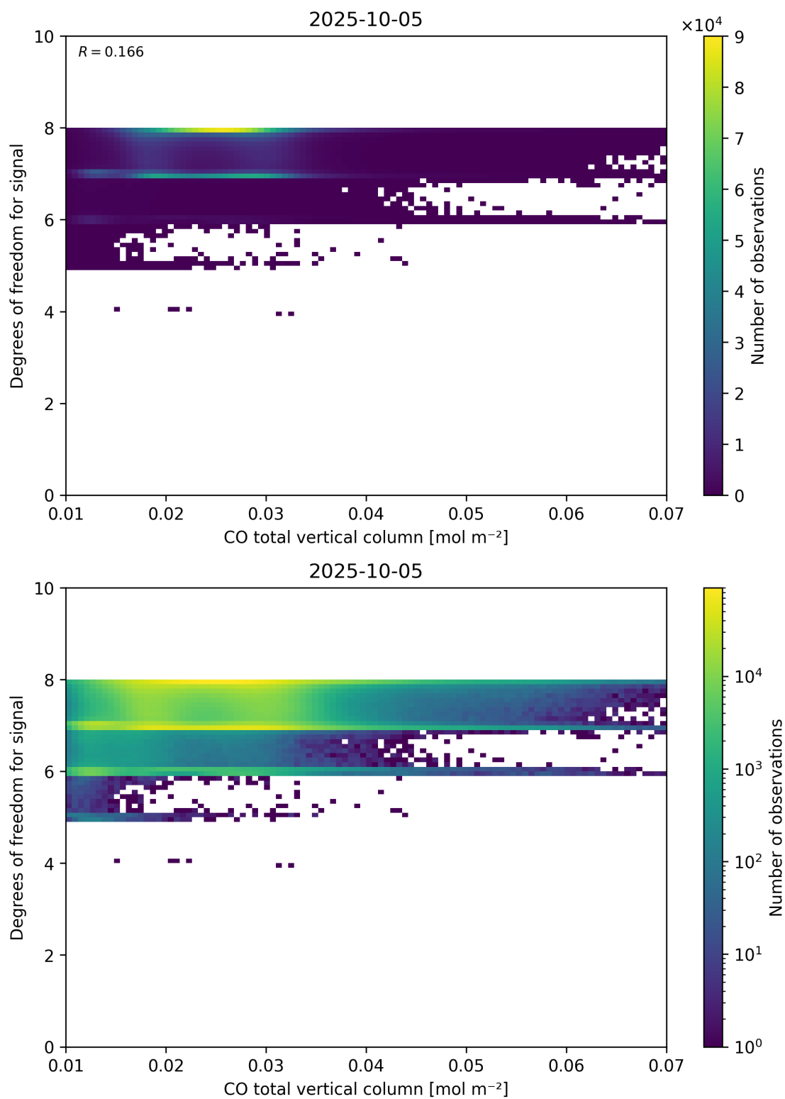
Figure 41: Scatter density plot of “CO total vertical column” against “Degrees of freedom for signal” for 2025-10-04 to 2025-10-06.
