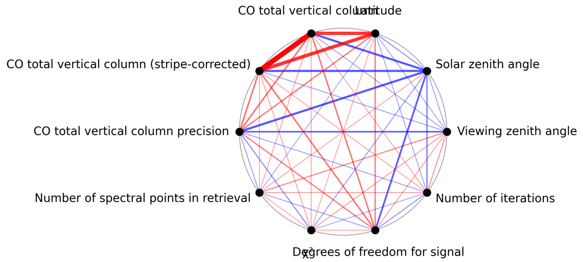
Figure 1: Map of correlation graph for 2025-10-04 to 2025-10-06.
