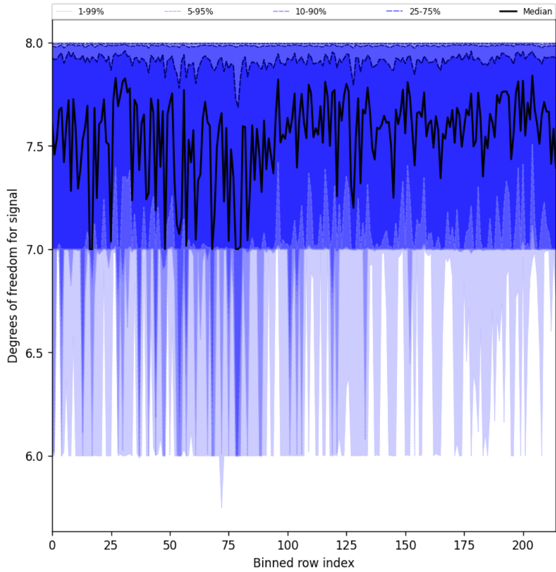
Figure 31: Along track statistics of “Degrees of freedom for signal” for 2025-10-04 to 2025-10-06
