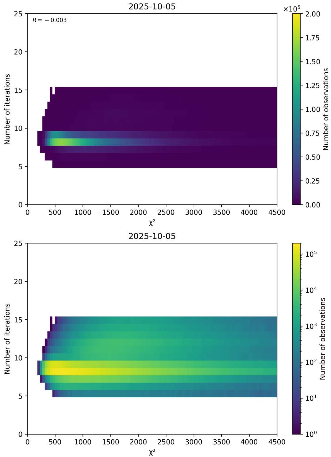
Figure 49: Scatter density plot of “ \chi^2 ” against “Number of iterations” for 2025-10-04 to 2025-10-06.
