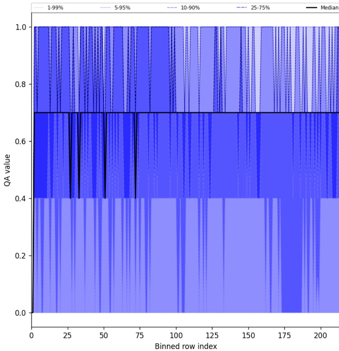
Figure 25: Along track statistics of “QA value” for 2025-10-04 to 2025-10-06
