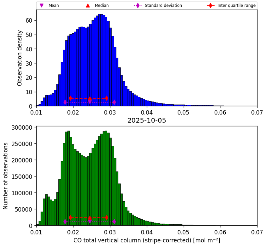
Figure 19: Histogram of “CO total vertical column (stripe-corrected)” for 2025-10-04 to 2025-10-06
