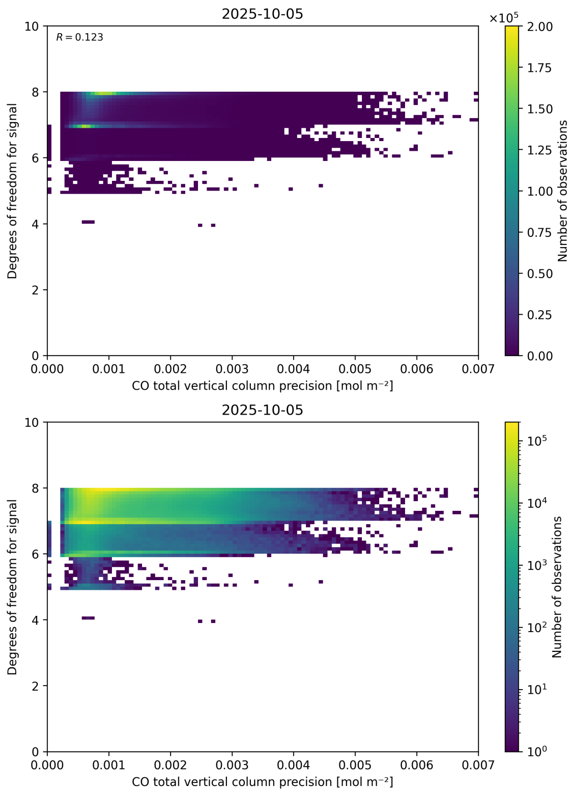
Figure 45: Scatter density plot of “CO total vertical column precision” against “Degrees of freedom for signal” for 2025-10-04 to 2025-10-06.
