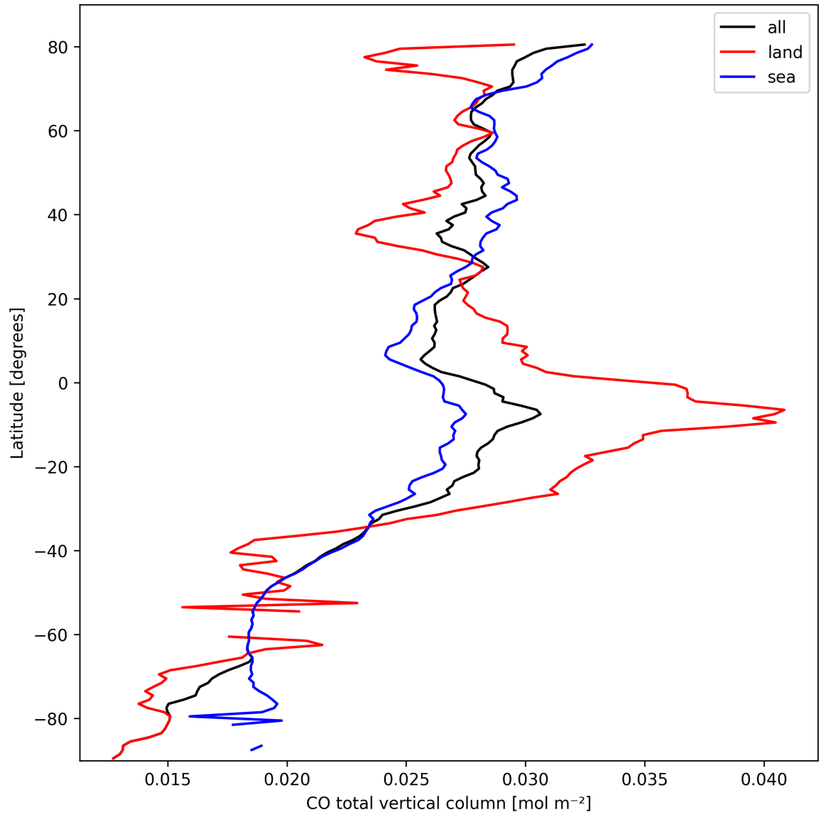
Figure 10: Zonal average of “CO total vertical column” for 2025-10-04 to 2025-10-06.
