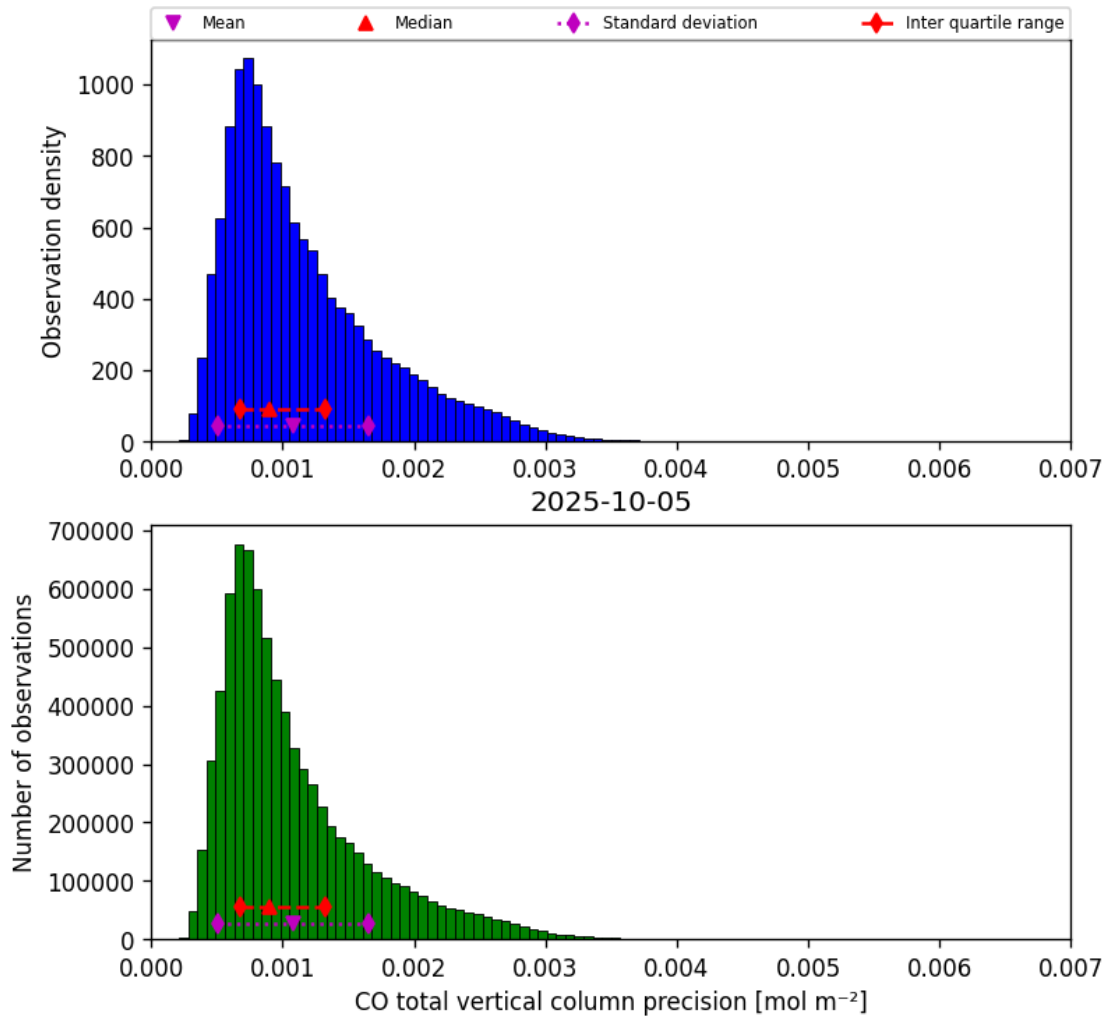
Figure 20: Histogram of “CO total vertical column precision” for 2025-10-04 to 2025-10-06
