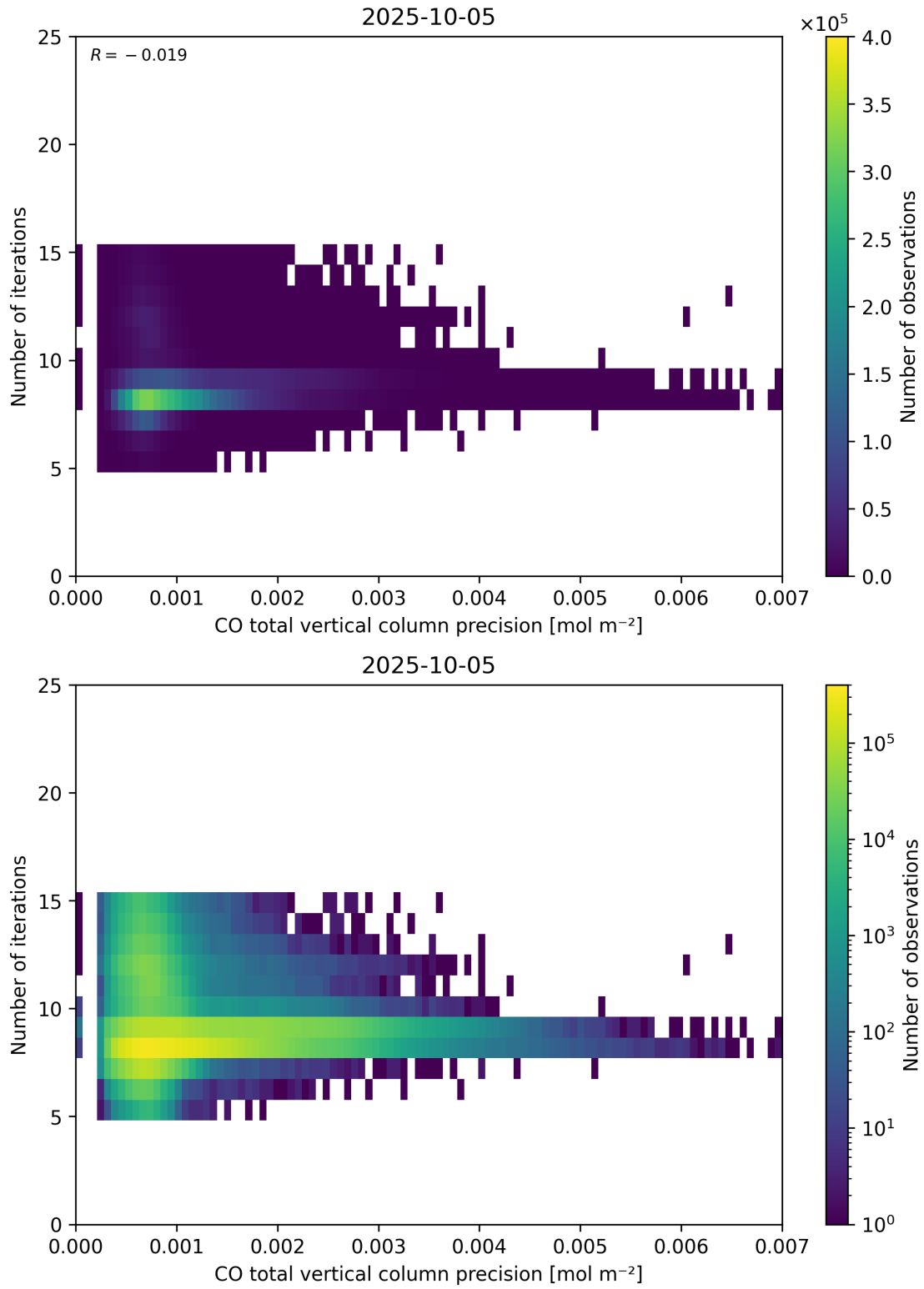
Figure 46: Scatter density plot of “CO total vertical column precision” against “Number of iterations” for 2025-10-04 to 2025-10-06.
