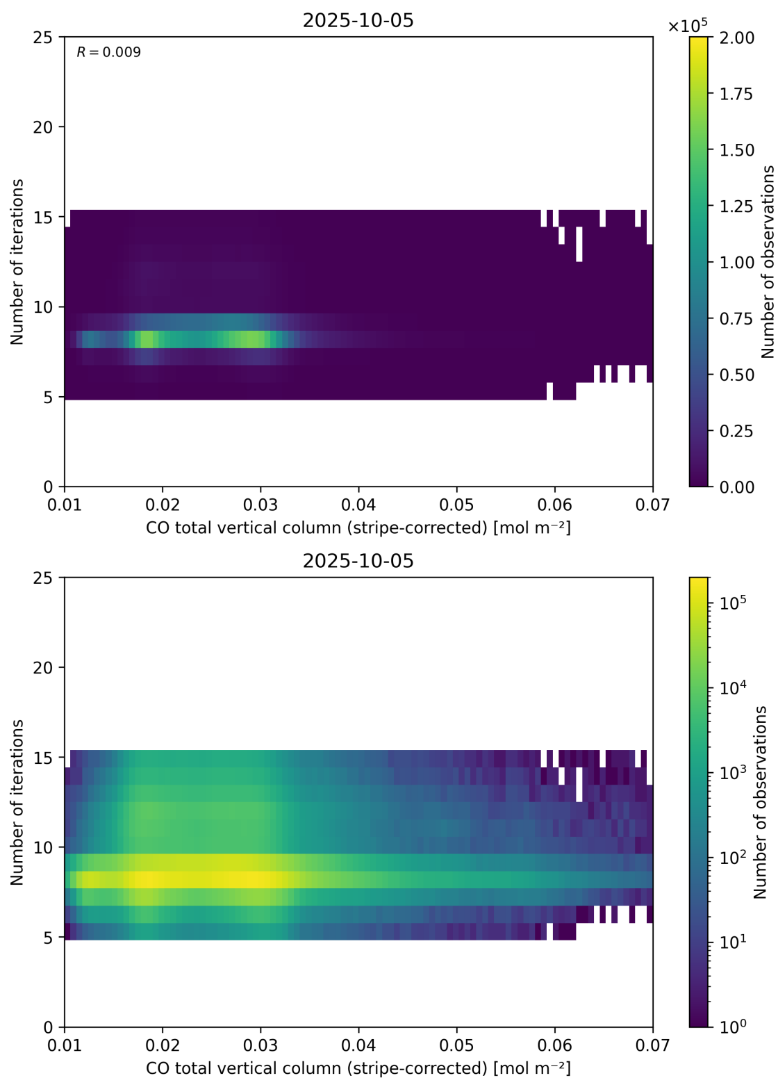
Figure 39: Scatter density plot of “CO total vertical column (stripe-corrected)” against “Number of iterations” for 2025-10-04 to 2025-10-06.
