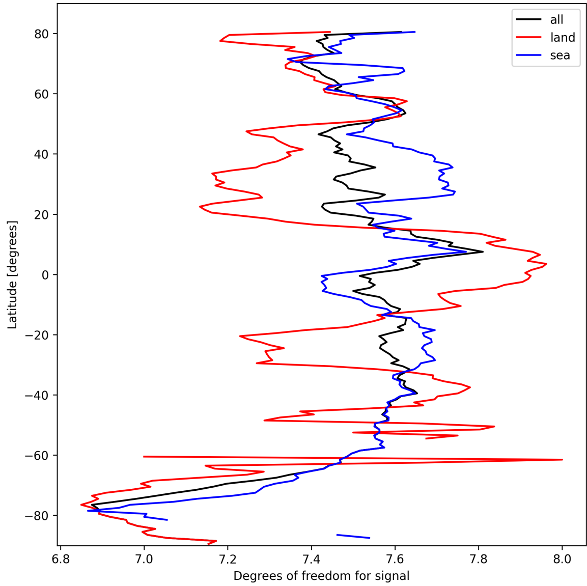
Figure 15: Zonal average of “Degrees of freedom for signal” for 2025-10-04 to 2025-10-06.
