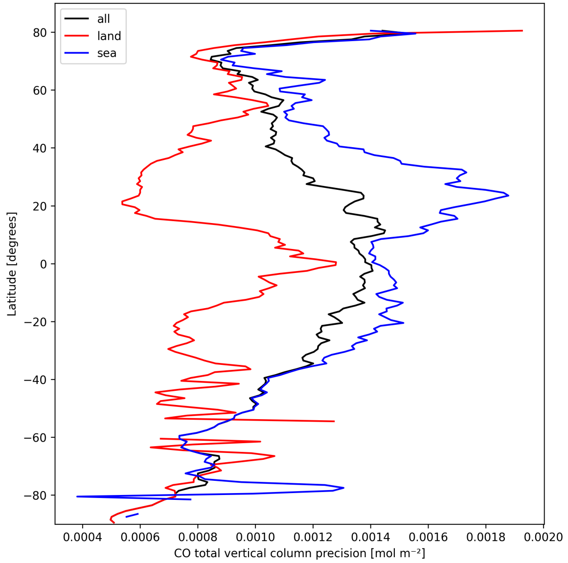
Figure 12: Zonal average of “CO total vertical column precision” for 2025-10-04 to 2025-10-06.
