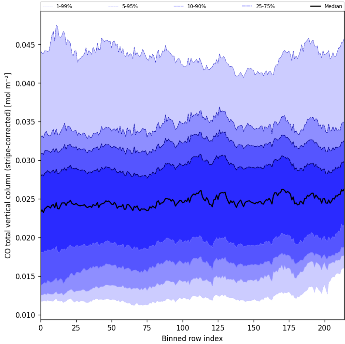
Figure 27: Along track statistics of “CO total vertical column (stripe-corrected)” for 2025-10-04 to 2025-10-06
