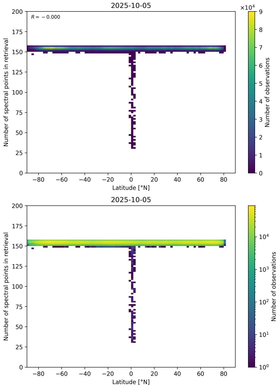
Figure 57: Scatter density plot of “Latitude” against “Number of spectral points in retrieval” for 2025-10-04 to 2025-10-06.
