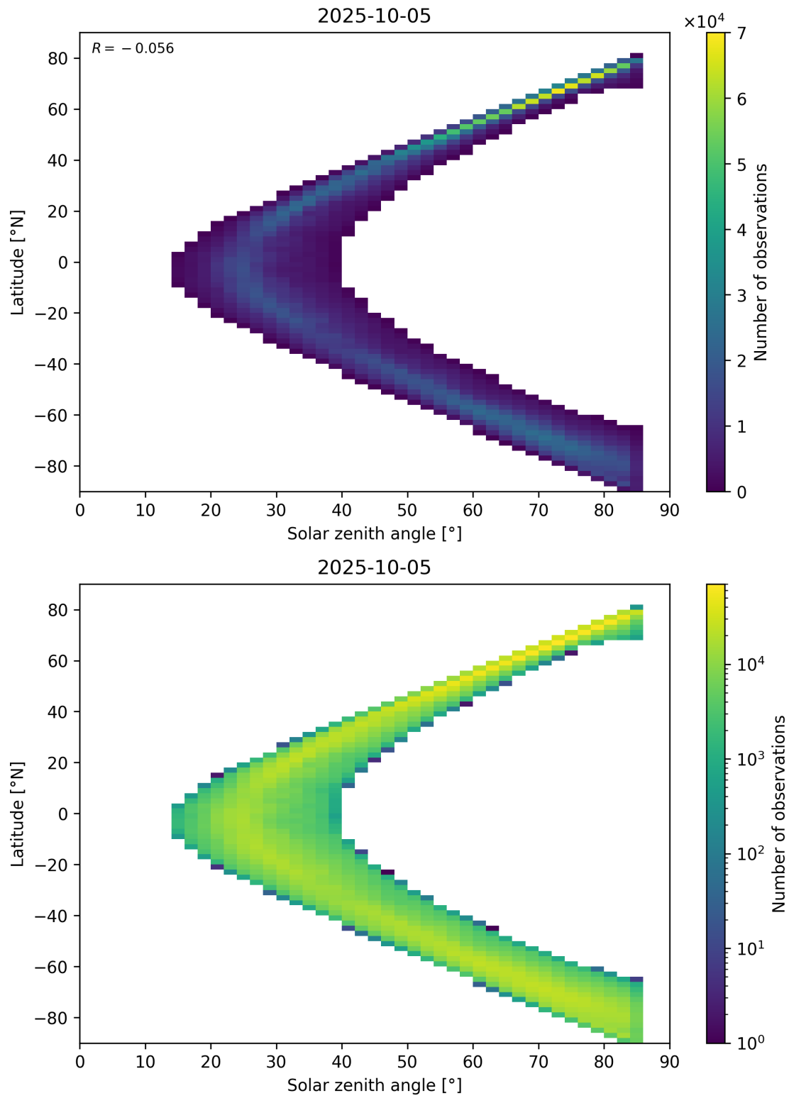
Figure 66: Scatter density plot of “Solar zenith angle” against “Latitude” for 2025-10-04 to 2025-10-06.
