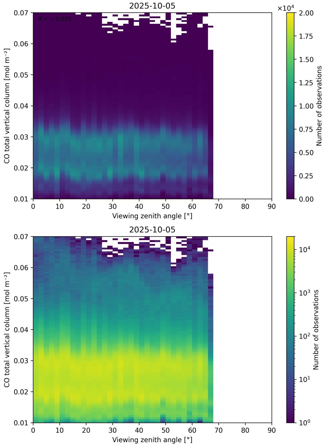
Figure 69: Scatter density plot of “Viewing zenith angle” against “CO total vertical column” for 2025-10-04 to 2025-10-06.
