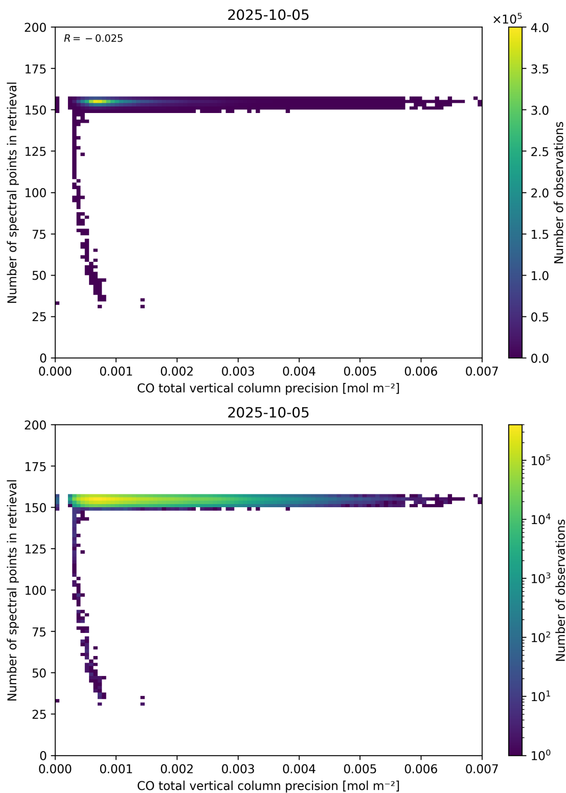
Figure 47: Scatter density plot of “CO total vertical column precision” against “Number of spectral points in retrieval” for 2025-10-04 to 2025-10-06.
