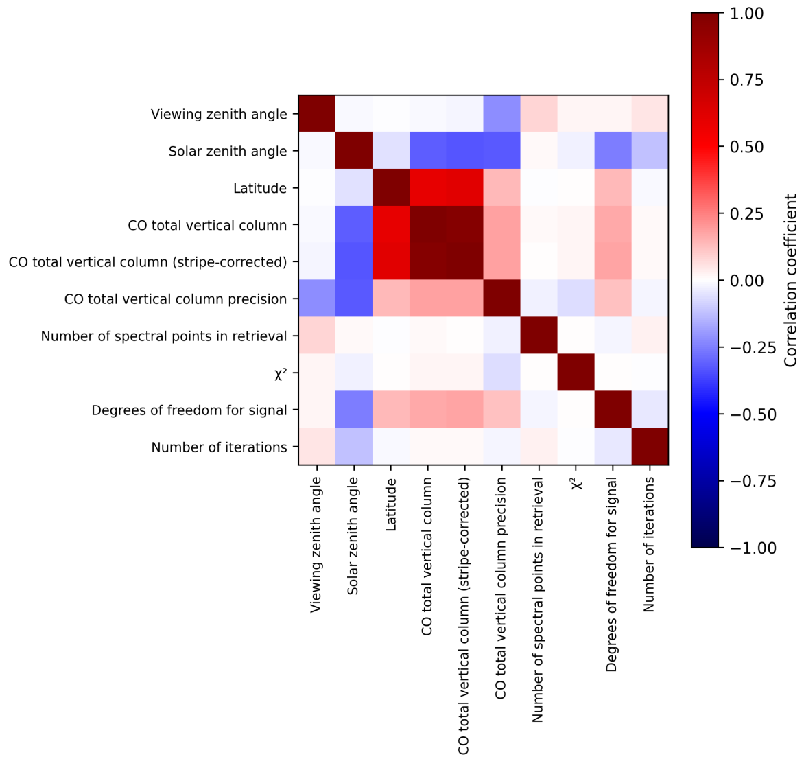
Figure 2: Map of correlation matrix for 2025-10-04 to 2025-10-06.
