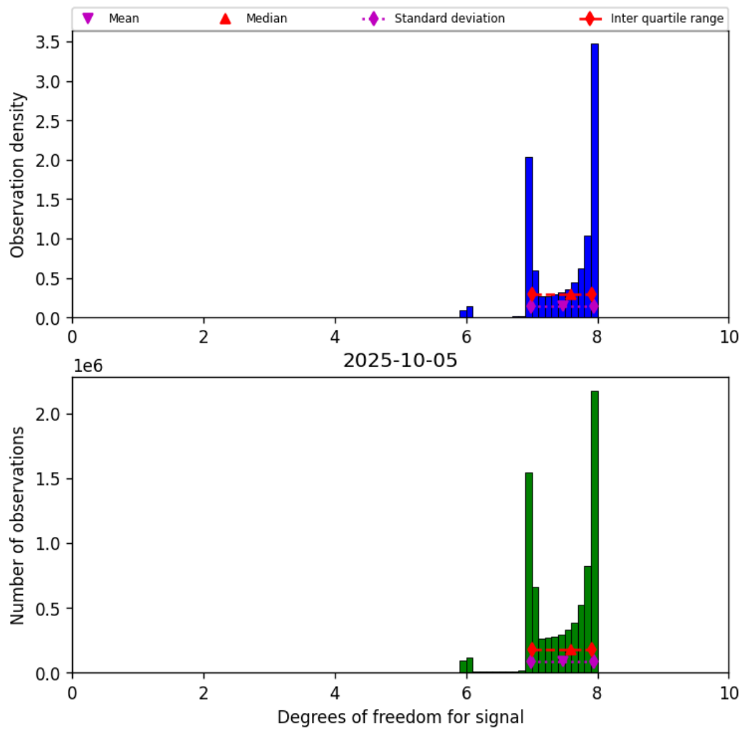
Figure 23: Histogram of “Degrees of freedom for signal” for 2025-10-04 to 2025-10-06
