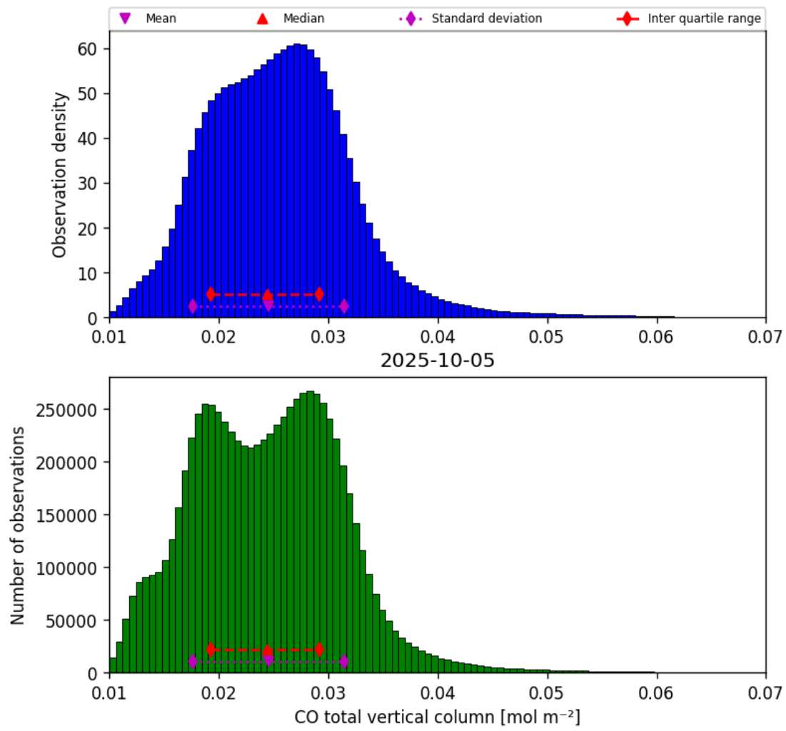
Figure 18: Histogram of “CO total vertical column” for 2025-10-04 to 2025-10-06
