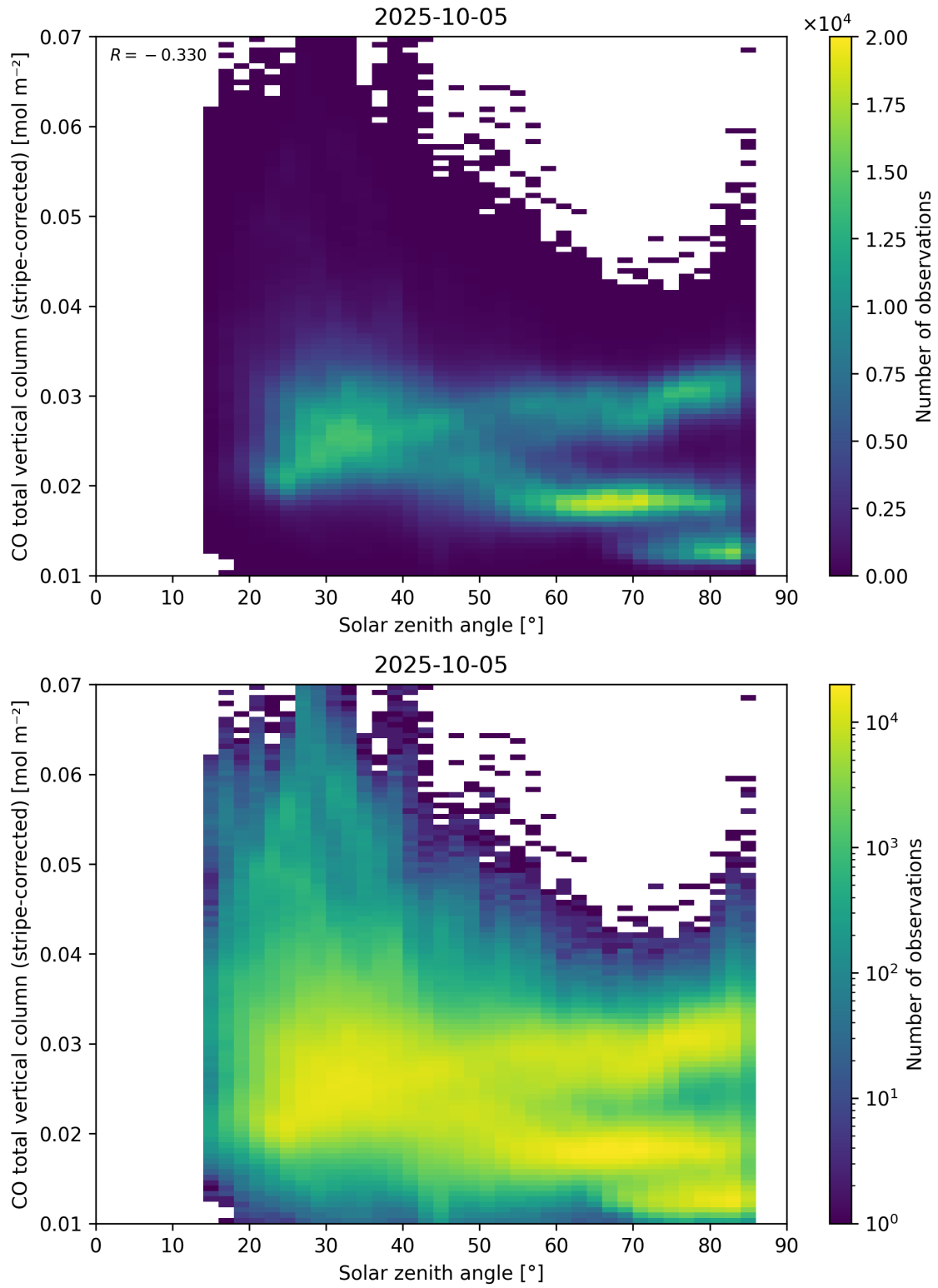
Figure 62: Scatter density plot of “Solar zenith angle” against “CO total vertical column (stripe-corrected)” for 2025-10-04 to 2025-10-06.
