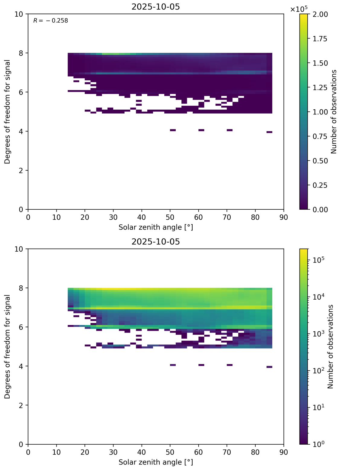
Figure 65: Scatter density plot of “Solar zenith angle” against “Degrees of freedom for signal” for 2025-10-04 to 2025-10-06.
