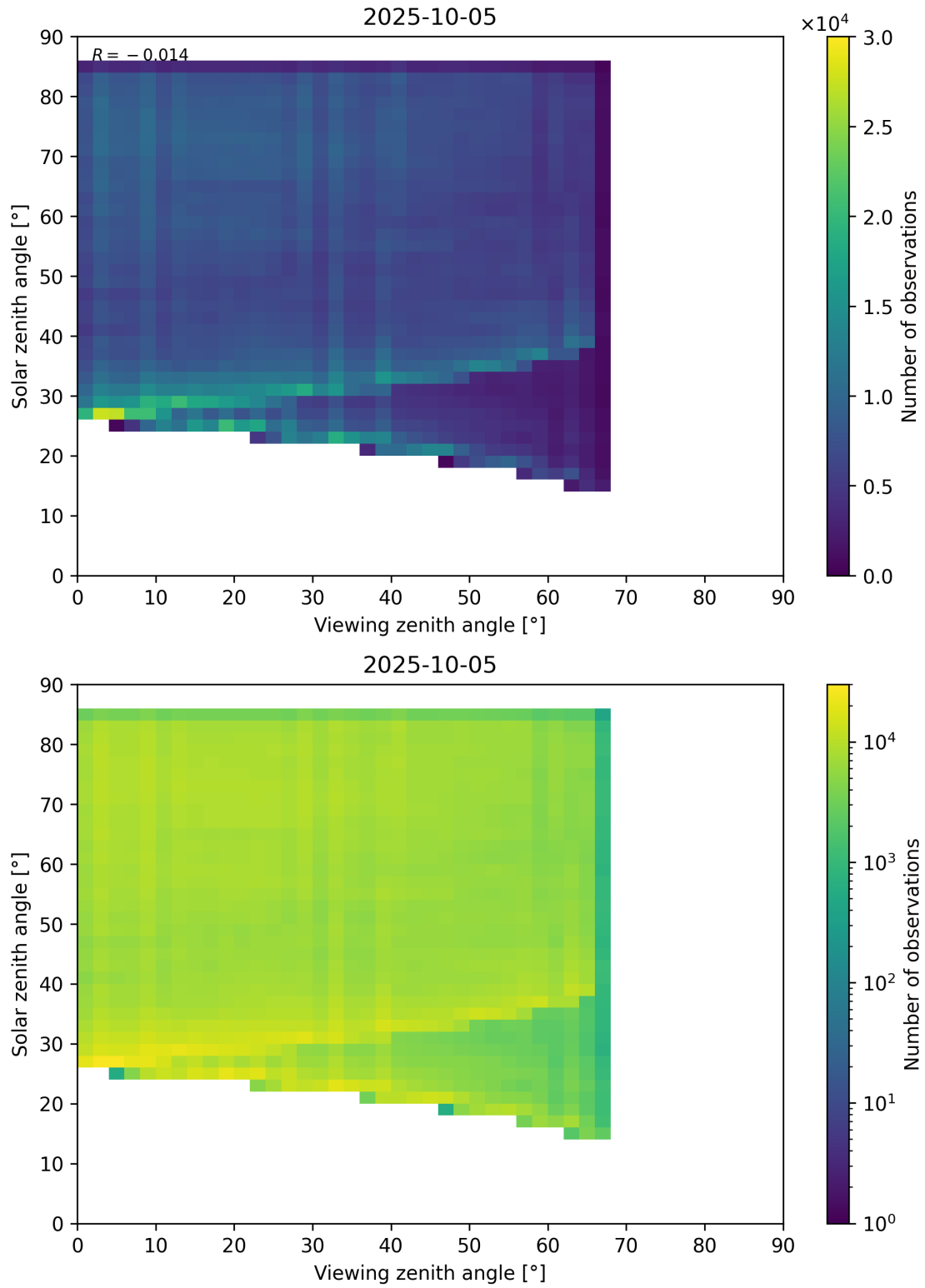
Figure 77: Scatter density plot of “Viewing zenith angle” against “Solar zenith angle” for 2025-10-04 to 2025-10-06.
