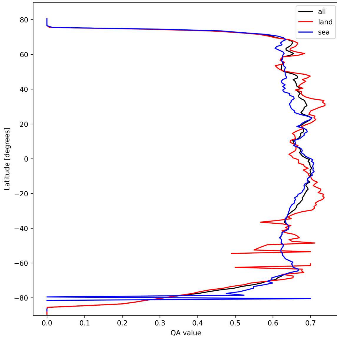
Figure 9: Zonal average of “QA value” for 2025-10-04 to 2025-10-06.
