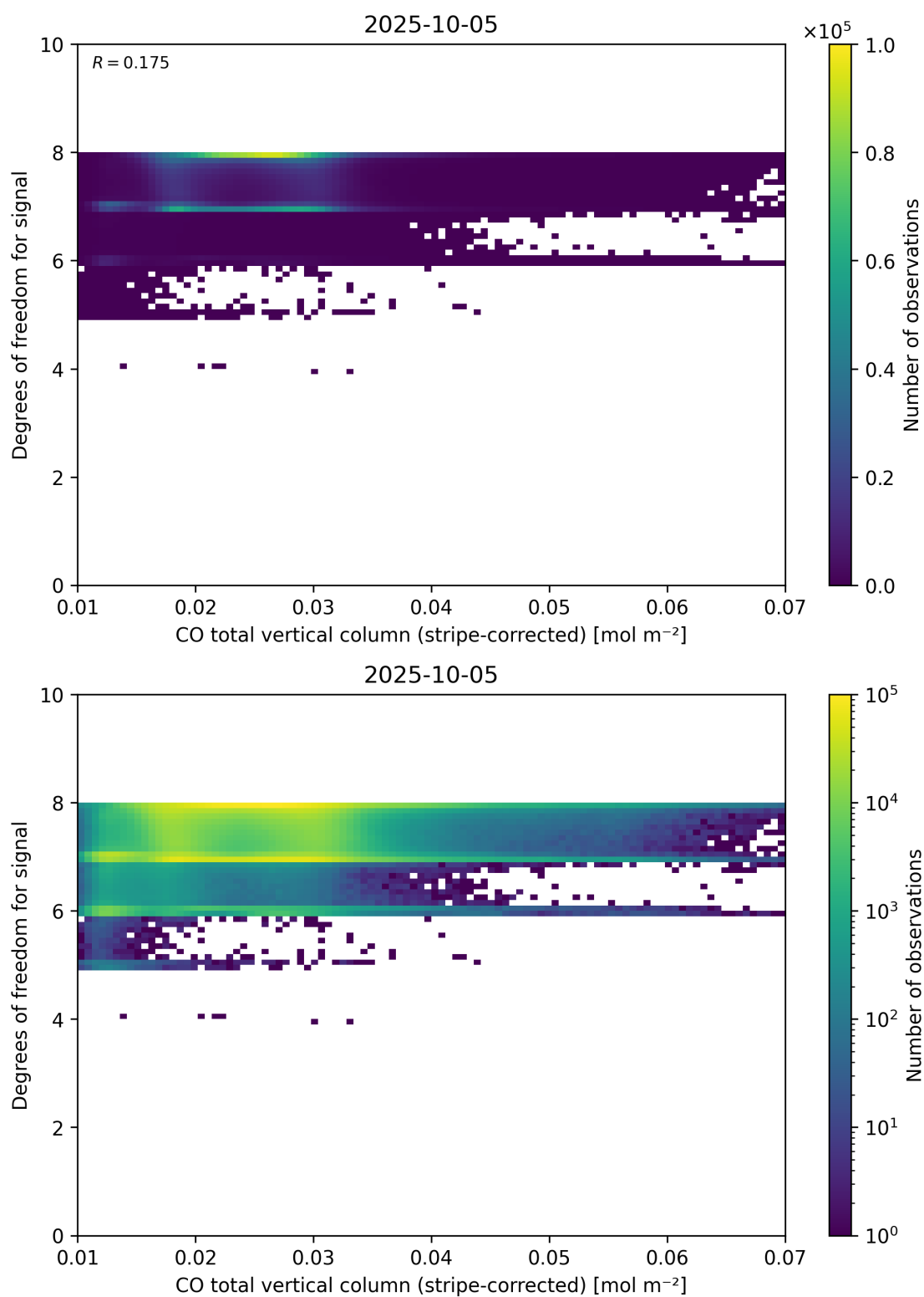
Figure 38: Scatter density plot of “CO total vertical column (stripe-corrected)” against “Degrees of freedom for signal” for 2025-10-04 to 2025-10-06.
