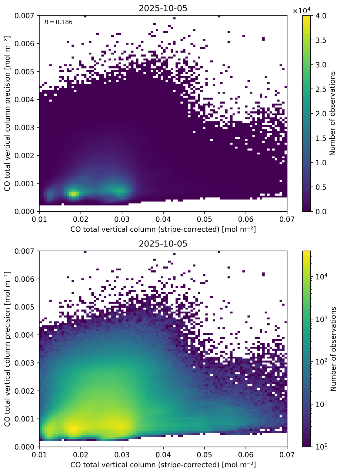
Figure 36: Scatter density plot of “CO total vertical column (stripe-corrected)” against “CO total vertical column precision” for 2025-10-04 to 2025-10-06.
