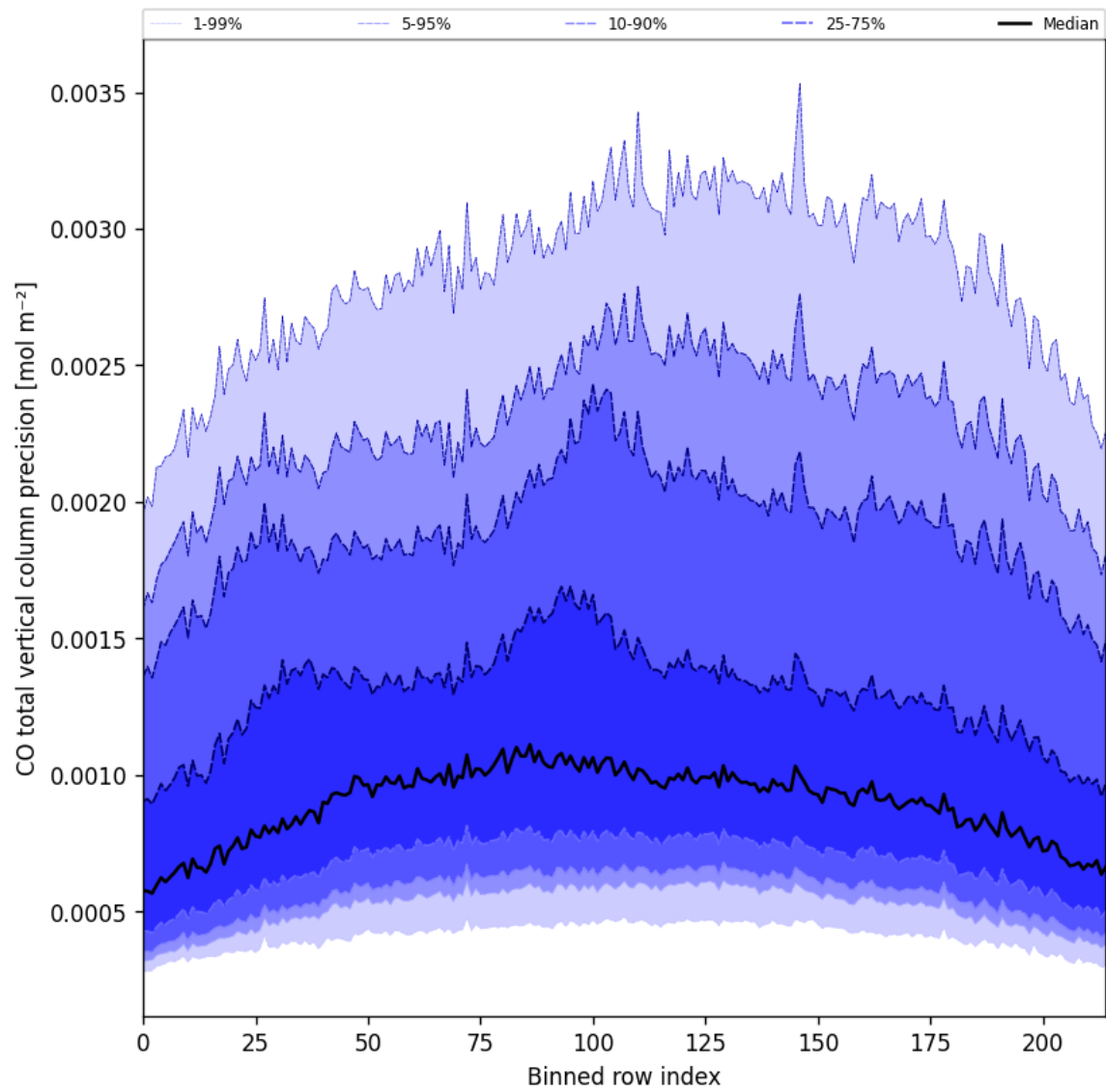
Figure 28: Along track statistics of “CO total vertical column precision” for 2025-10-04 to 2025-10-06
