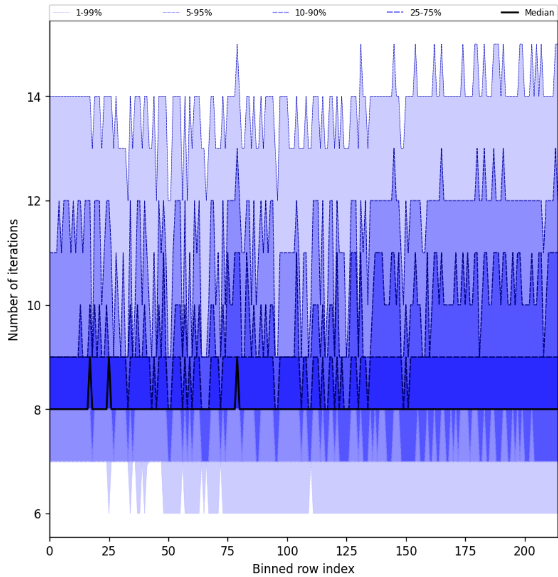
Figure 32: Along track statistics of “Number of iterations” for 2025-10-06 to 2025-10-07
