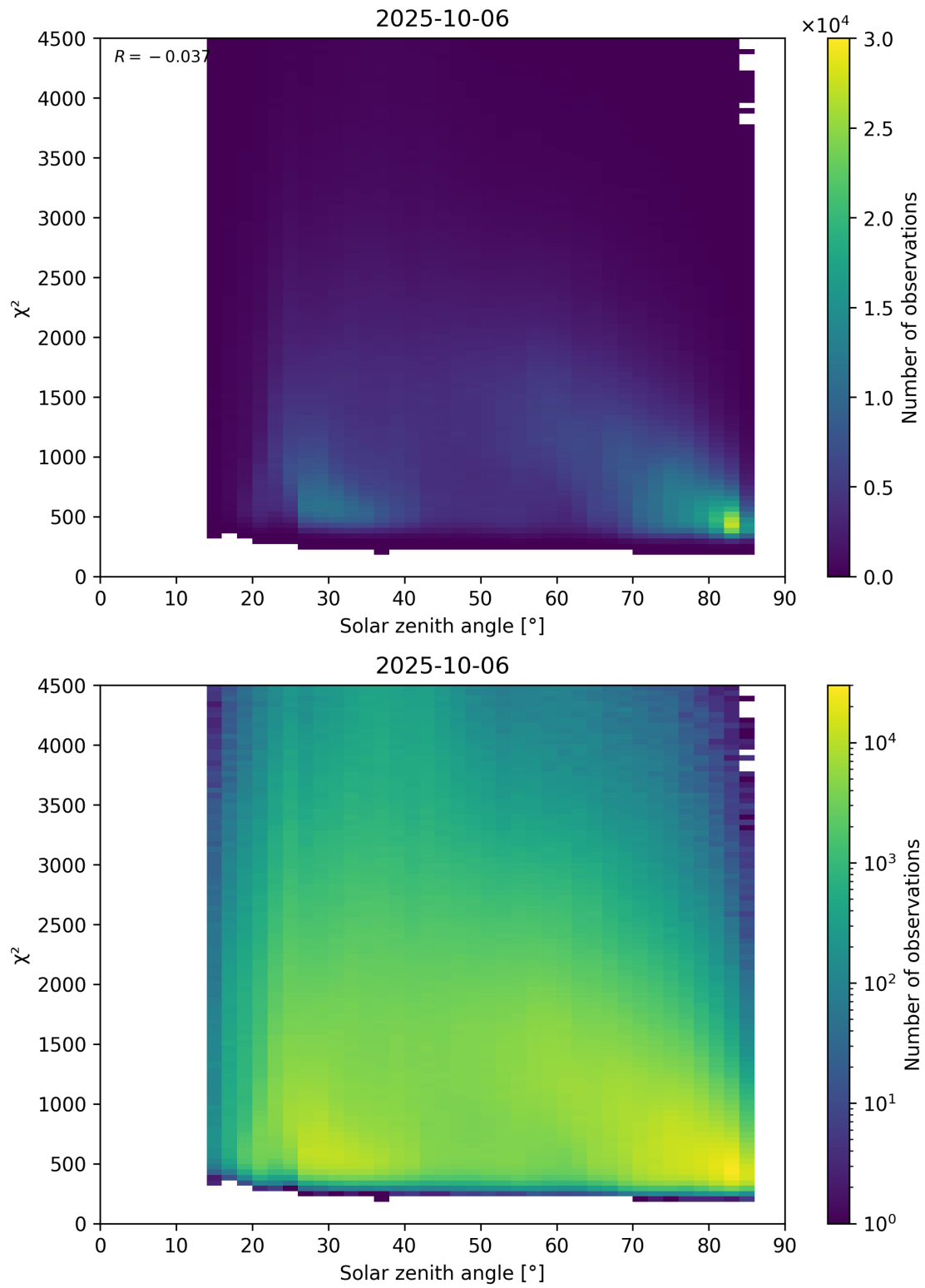
Figure 64: Scatter density plot of “Solar zenith angle” against “ \chi^2 ” for 2025-10-06 to 2025-10-07.
