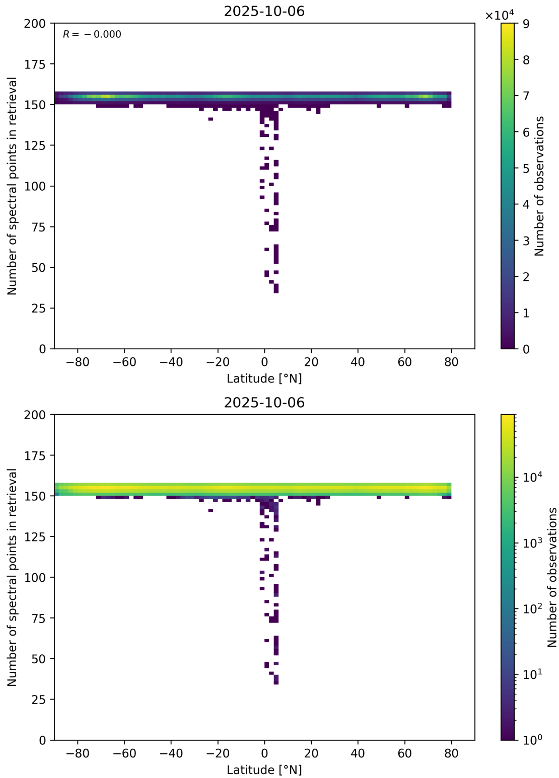
Figure 57: Scatter density plot of “Latitude” against “Number of spectral points in retrieval” for 2025-10-06 to 2025-10-07.
