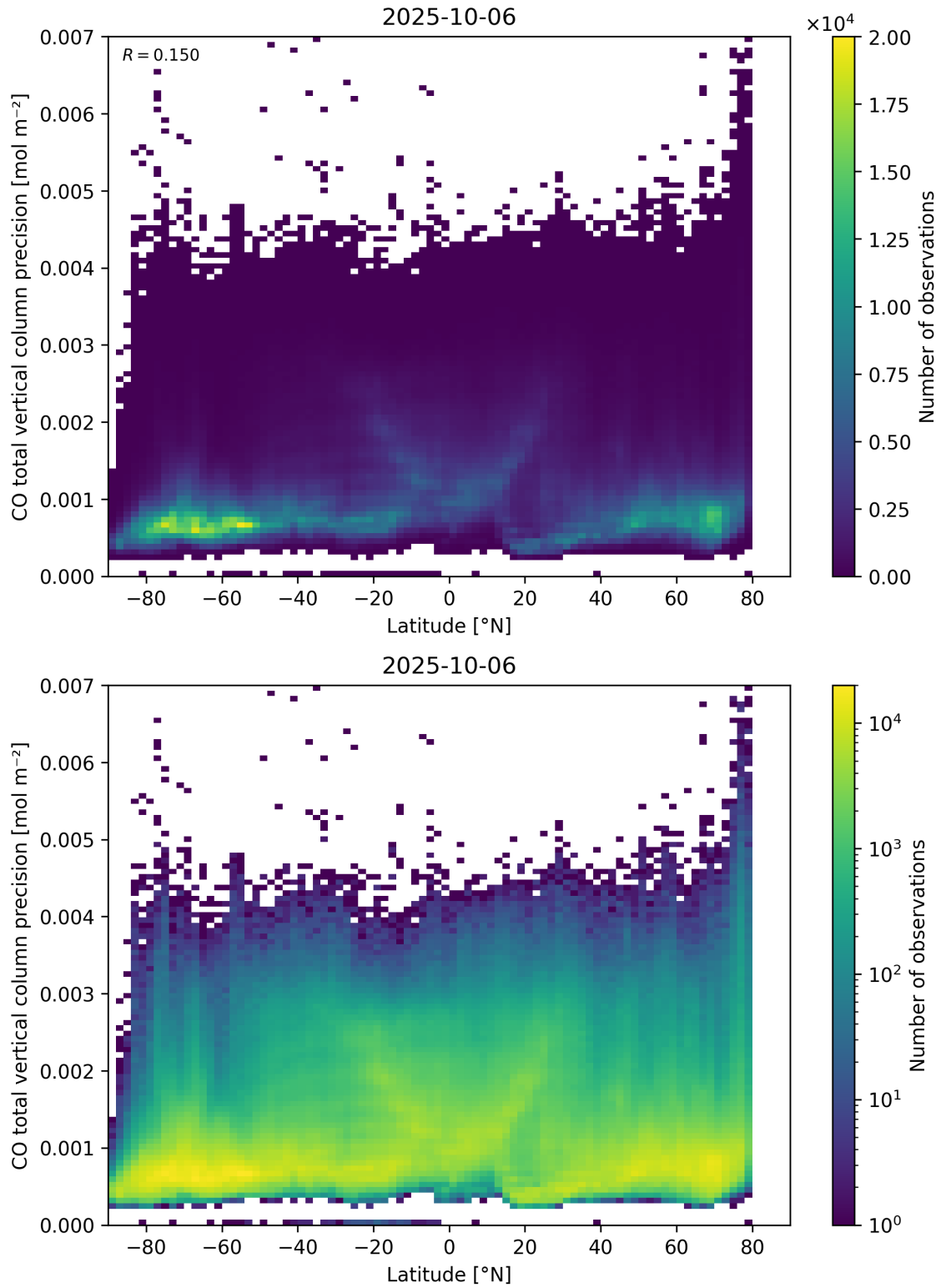
Figure 53: Scatter density plot of “Latitude” against “CO total vertical column precision” for 2025-10-06 to 2025-10-07.
