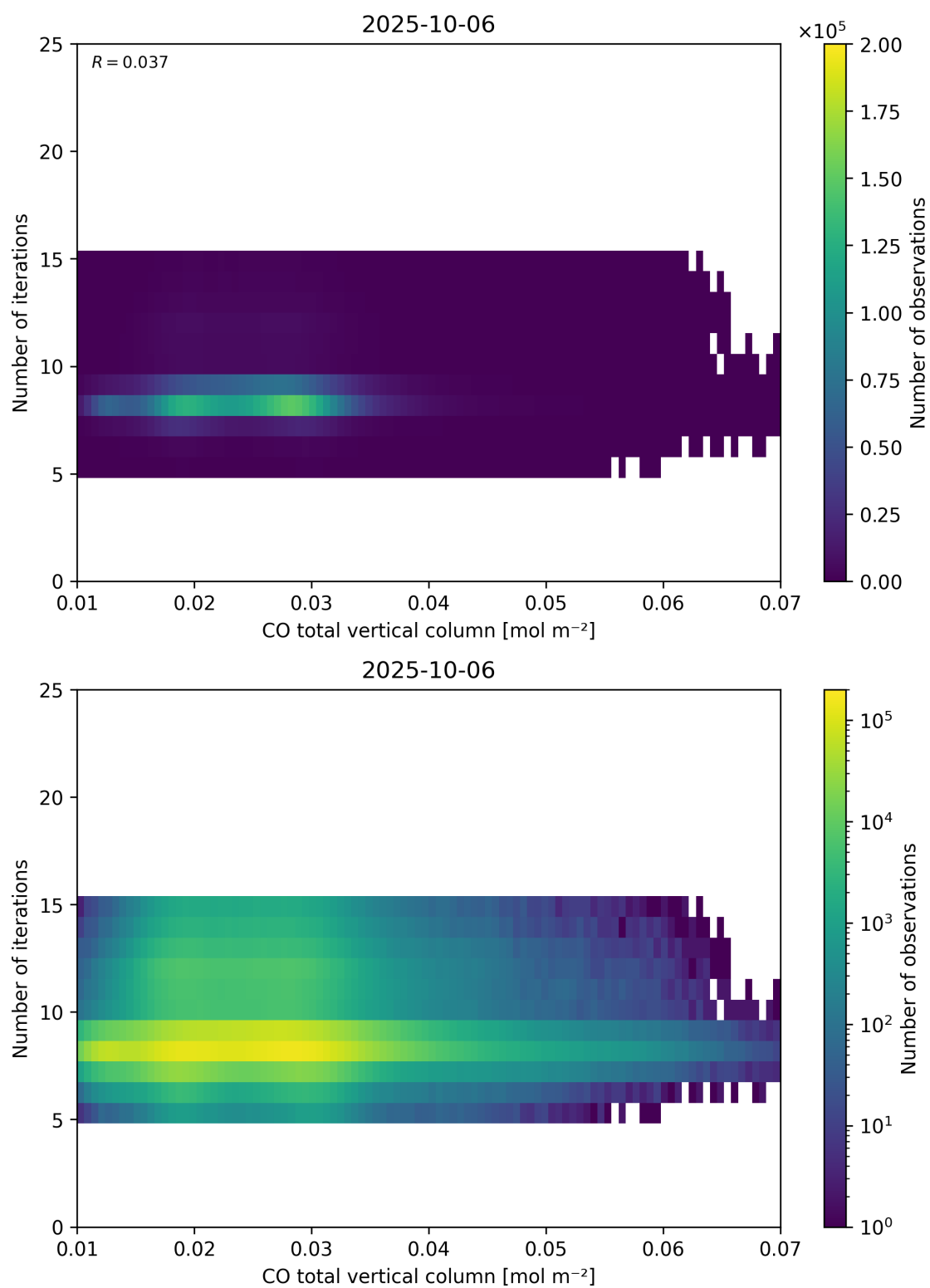
Figure 42: Scatter density plot of “CO total vertical column” against “Number of iterations” for 2025-10-06 to 2025-10-07.
