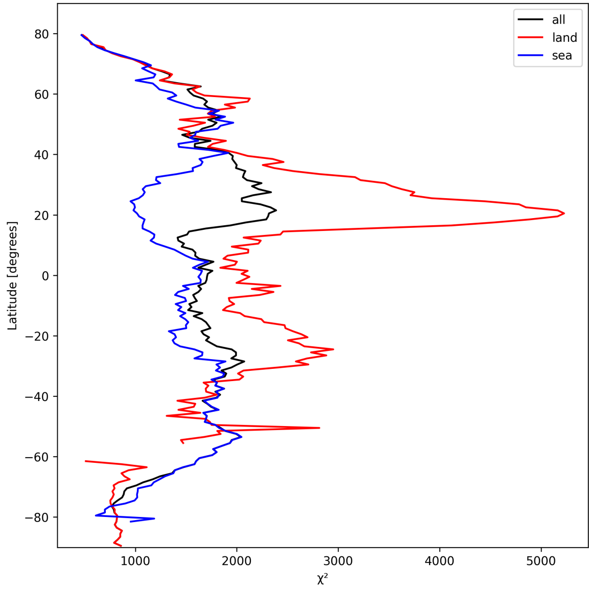
Figure 14: Zonal average of “ \chi^2 ” for 2025-10-06 to 2025-10-07.
