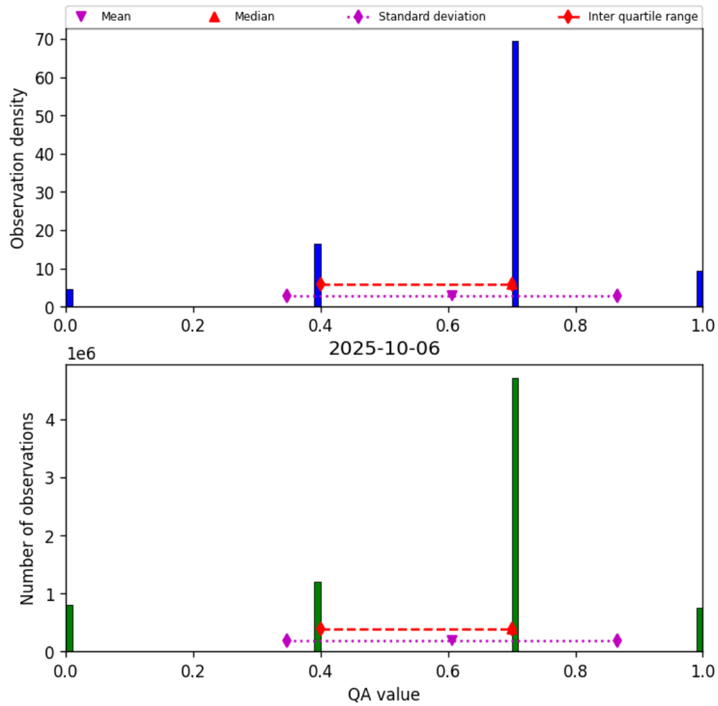
Figure 17: Histogram of “QA value” for 2025-10-06 to 2025-10-07
