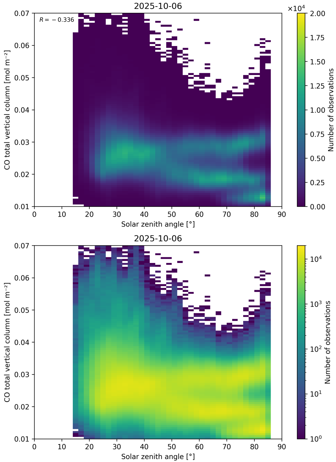
Figure 61: Scatter density plot of “Solar zenith angle” against “CO total vertical column” for 2025-10-06 to 2025-10-07.
