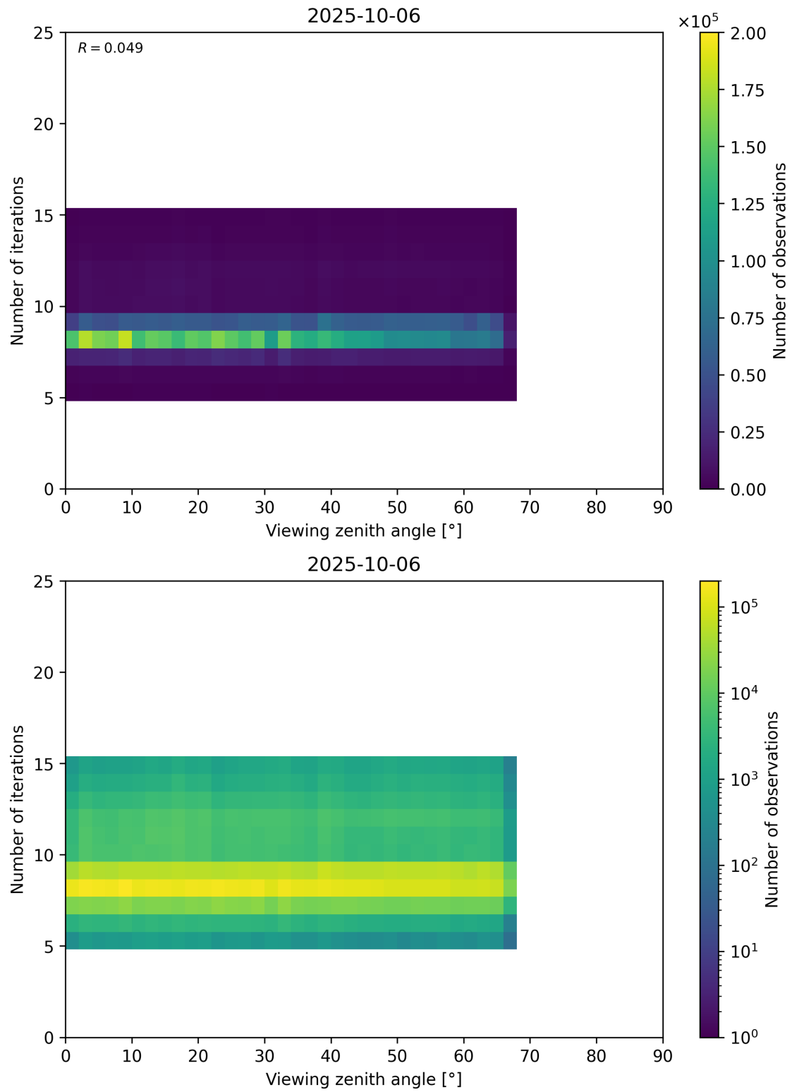
Figure 75: Scatter density plot of “Viewing zenith angle” against “Number of iterations” for 2025-10-06 to 2025-10-07.
