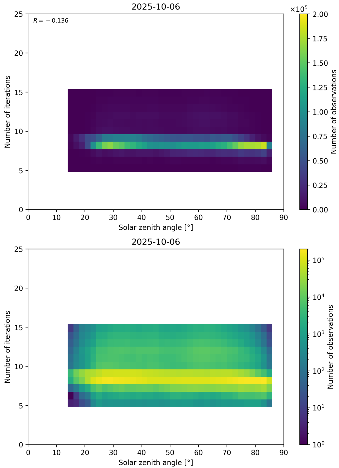
Figure 67: Scatter density plot of “Solar zenith angle” against “Number of iterations” for 2025-10-06 to 2025-10-07.
