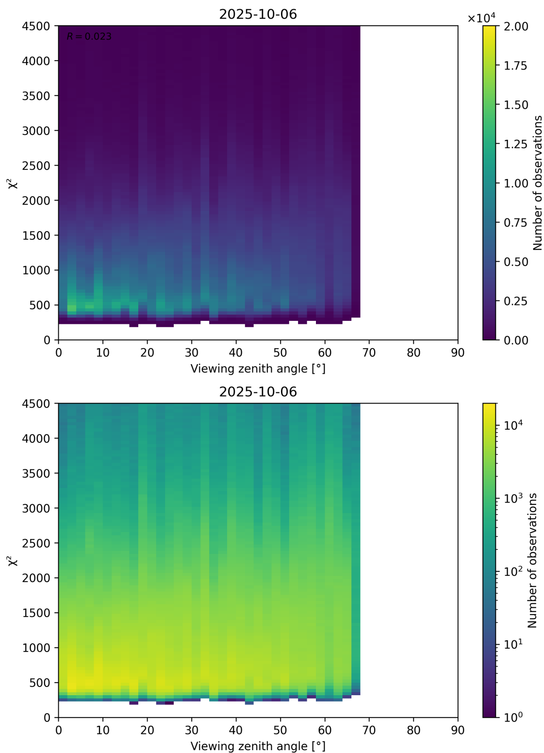
Figure 72: Scatter density plot of “Viewing zenith angle” against “ \chi^2 ” for 2025-10-06 to 2025-10-07.
