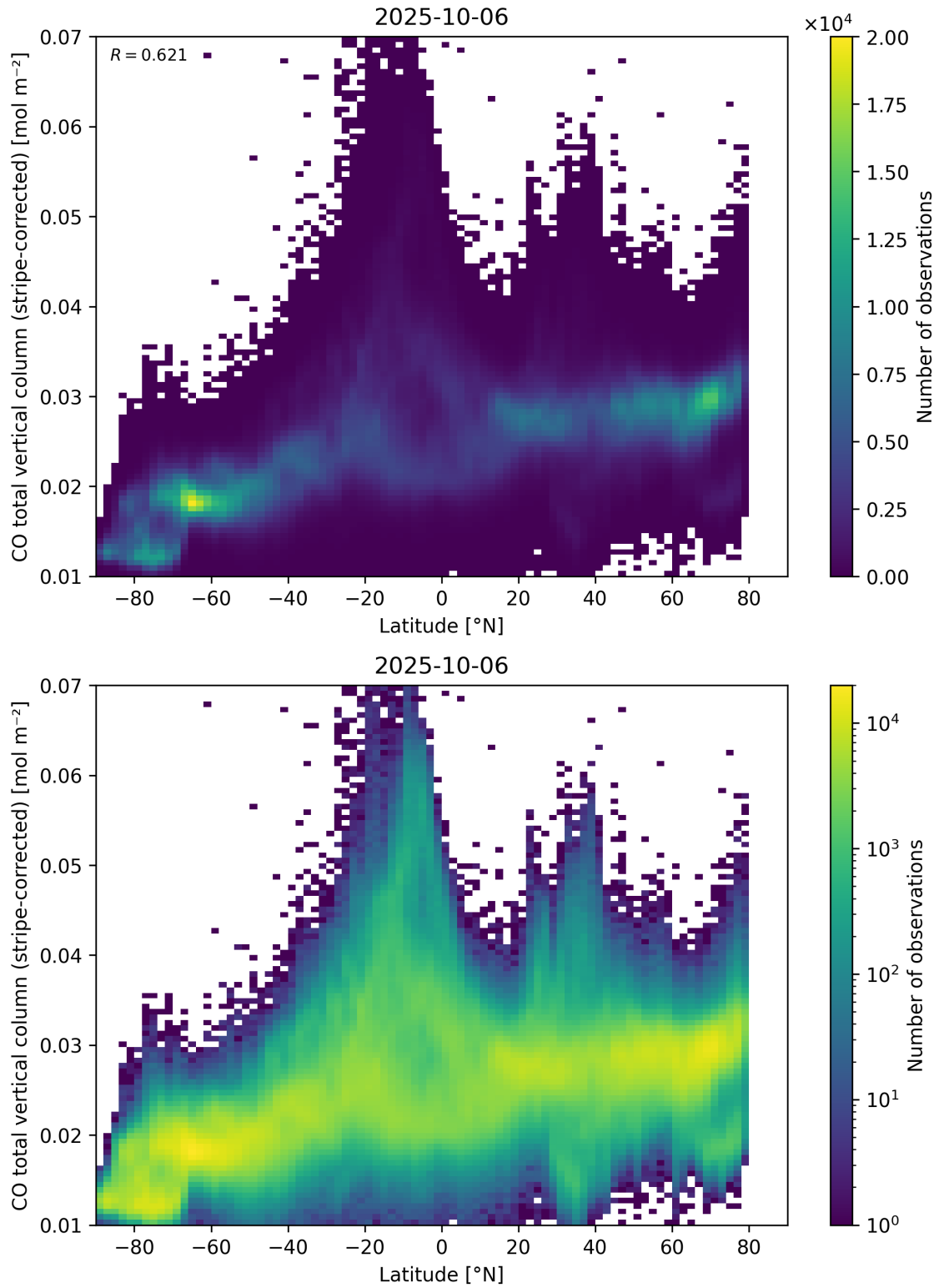
Figure 52: Scatter density plot of “Latitude” against “CO total vertical column (stripe-corrected)” for 2025-10-06 to 2025-10-07.
