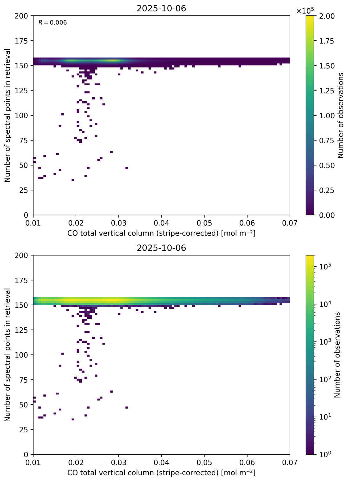
Figure 40: Scatter density plot of “CO total vertical column (stripe-corrected)” against “Number of spectral points in retrieval” for 2025-10-06 to 2025-10-07.
