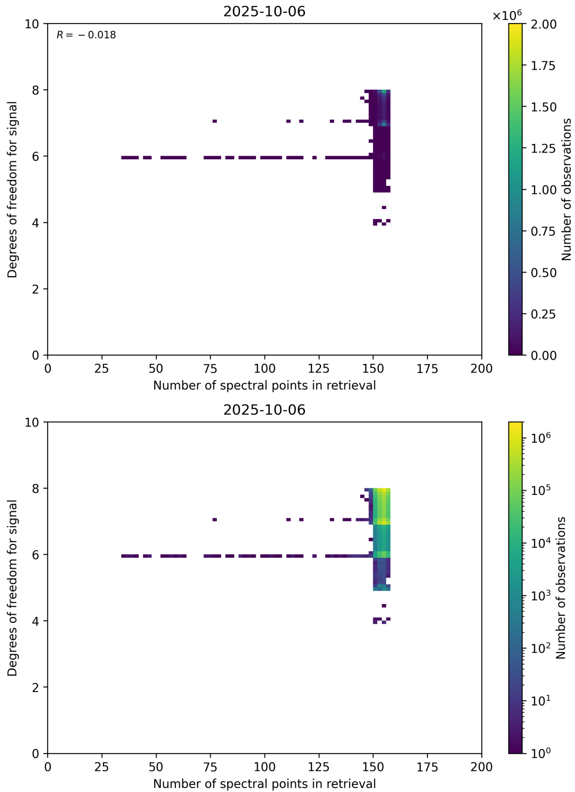
Figure 59: Scatter density plot of “Number of spectral points in retrieval” against “Degrees of freedom for signal” for 2025-10-06 to 2025-10-07.
