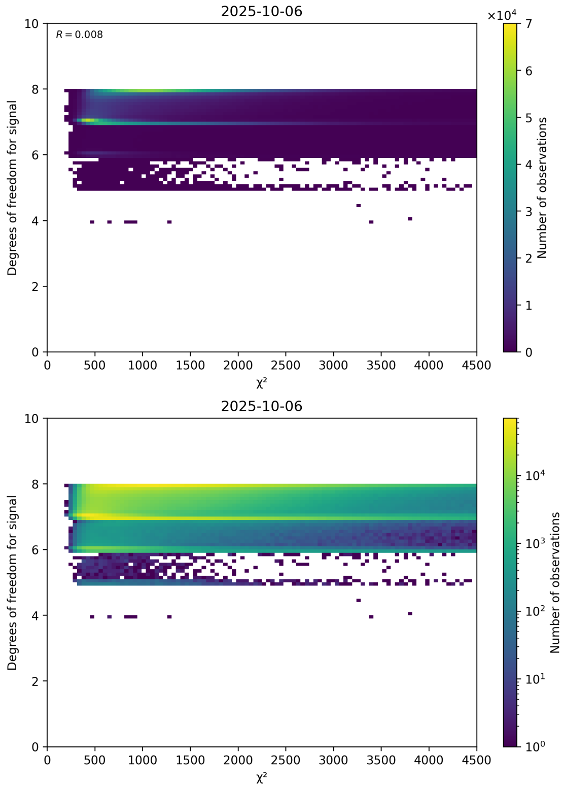
Figure 48: Scatter density plot of “ \chi^2 ” against “Degrees of freedom for signal” for 2025-10-06 to 2025-10-07.
