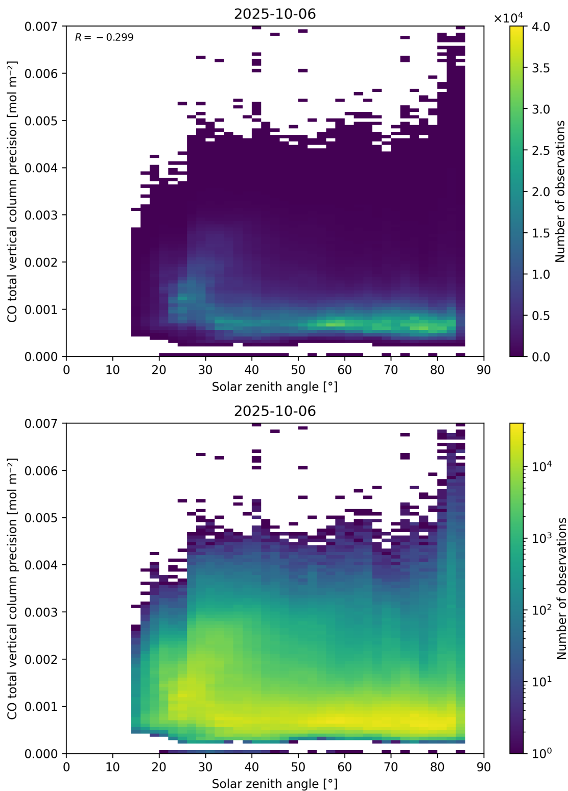
Figure 63: Scatter density plot of “Solar zenith angle” against “CO total vertical column precision” for 2025-10-06 to 2025-10-07.
