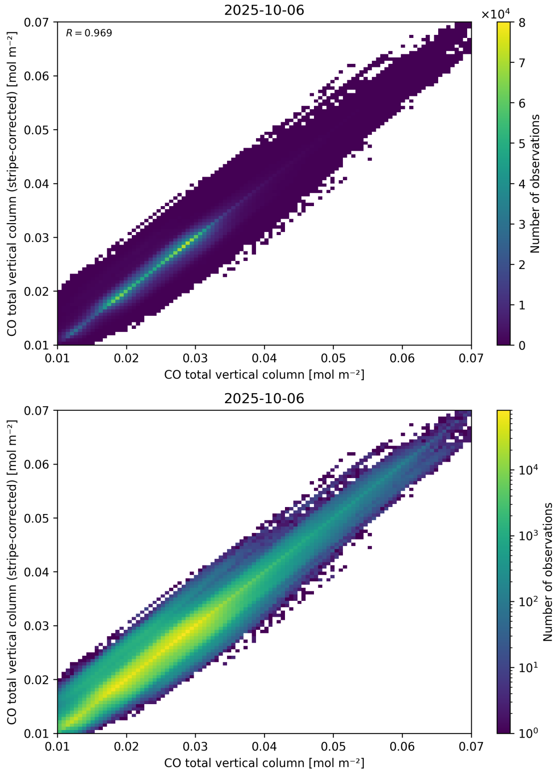
Figure 33: Scatter density plot of “CO total vertical column” against “CO total vertical column (stripe-corrected)” for 2025-10-06 to 2025-10-07.
