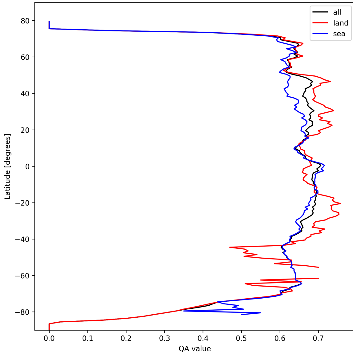
Figure 9: Zonal average of “QA value” for 2025-10-06 to 2025-10-07.
