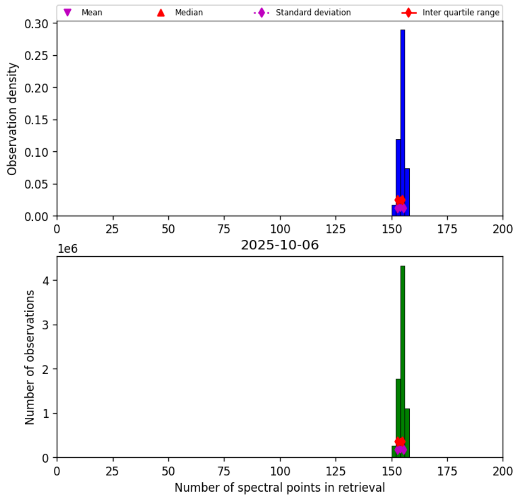
Figure 21: Histogram of “Number of spectral points in retrieval” for 2025-10-06 to 2025-10-07
