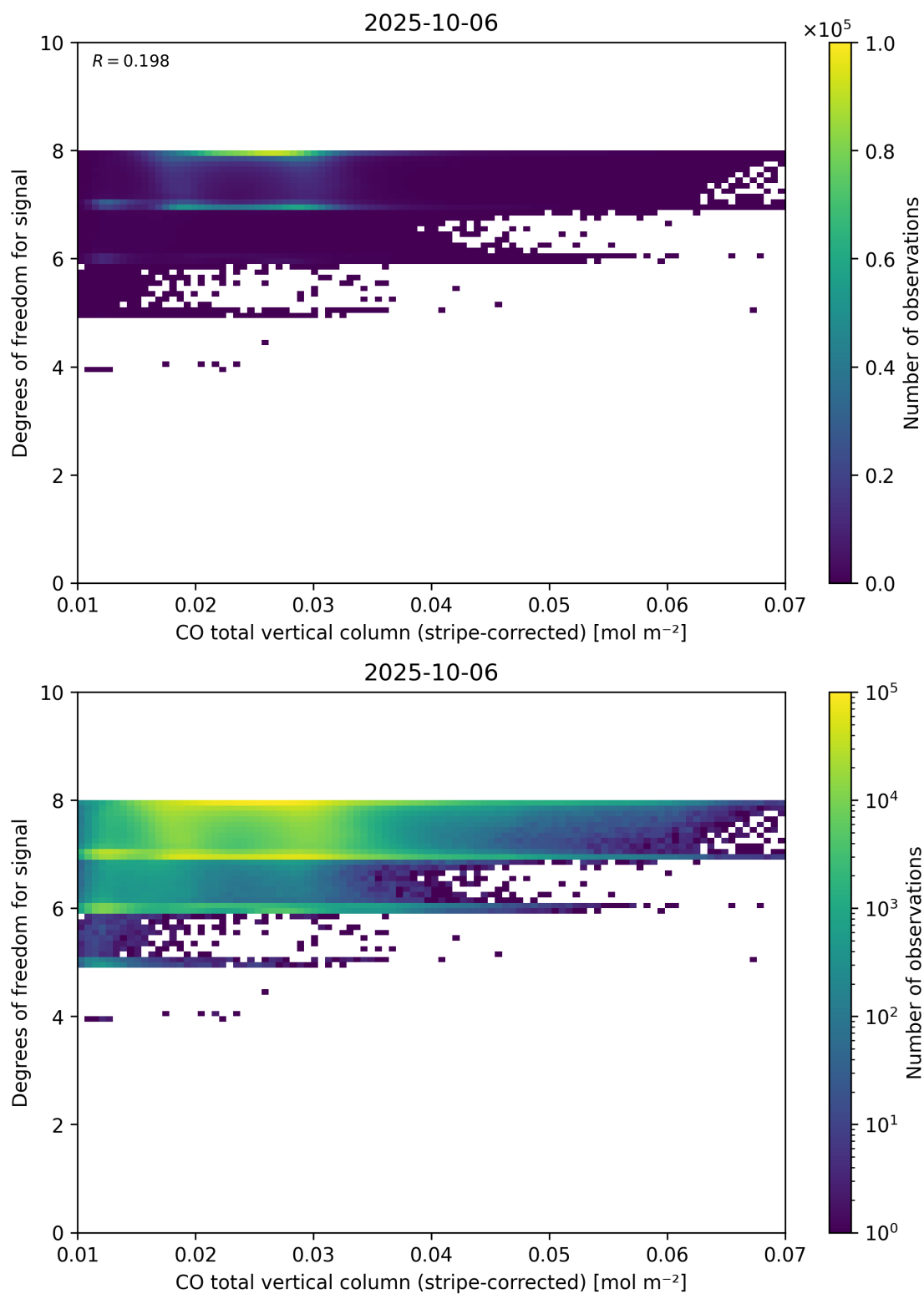
Figure 38: Scatter density plot of “CO total vertical column (stripe-corrected)” against “Degrees of freedom for signal” for 2025-10-06 to 2025-10-07.
