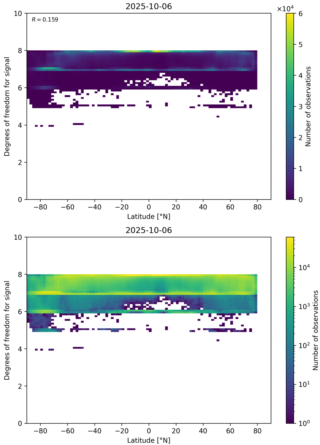
Figure 55: Scatter density plot of “Latitude” against “Degrees of freedom for signal” for 2025-10-06 to 2025-10-07.
