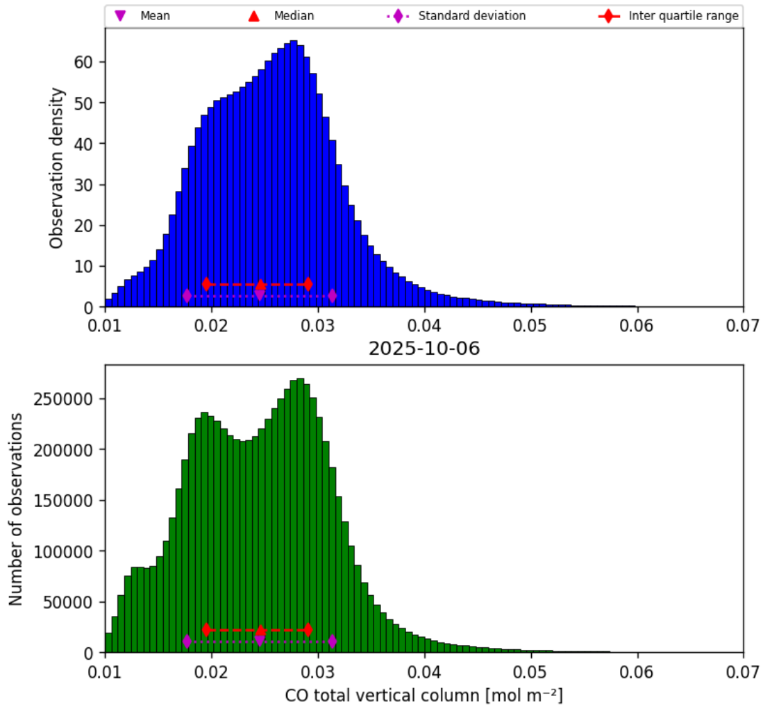
Figure 18: Histogram of “CO total vertical column” for 2025-10-06 to 2025-10-07
