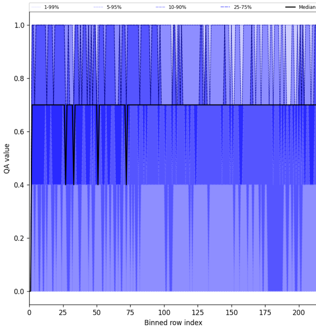
Figure 25: Along track statistics of “QA value” for 2025-10-06 to 2025-10-07
