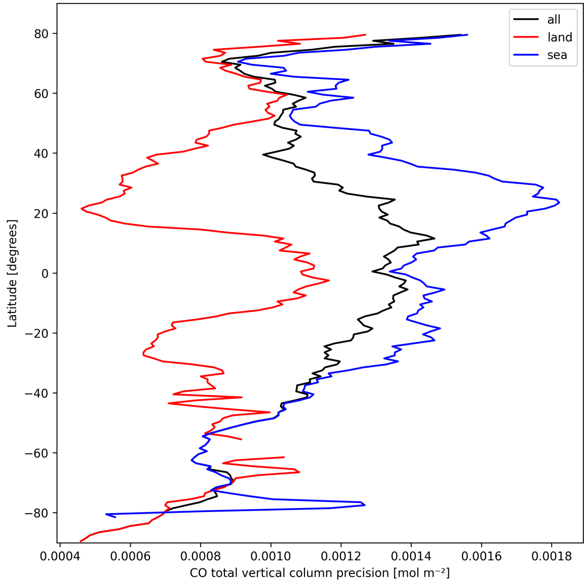
Figure 12: Zonal average of “CO total vertical column precision” for 2025-10-06 to 2025-10-07.
