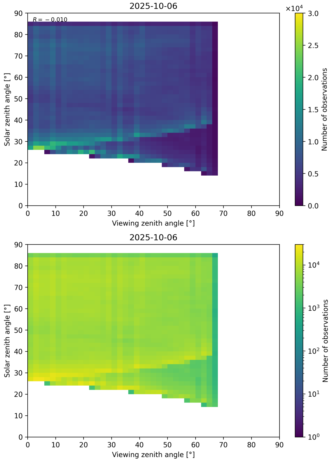
Figure 77: Scatter density plot of “Viewing zenith angle” against “Solar zenith angle” for 2025-10-06 to 2025-10-07.
