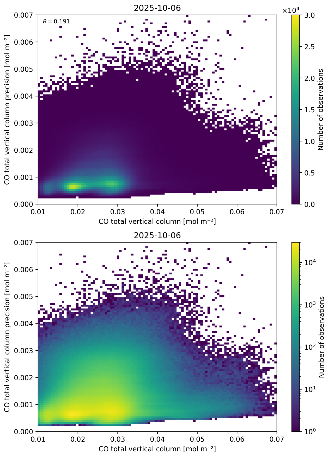
Figure 34: Scatter density plot of “CO total vertical column” against “CO total vertical column precision” for 2025-10-06 to 2025-10-07.
