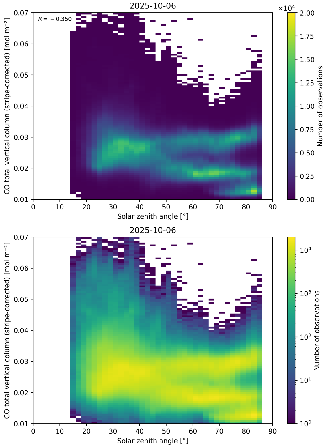
Figure 62: Scatter density plot of “Solar zenith angle” against “CO total vertical column (stripe-corrected)” for 2025-10-06 to 2025-10-07.
