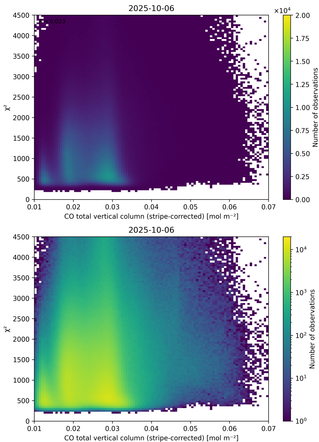
Figure 37: Scatter density plot of “CO total vertical column (stripe-corrected)” against “ \chi^2 ” for 2025-10-06 to 2025-10-07.
