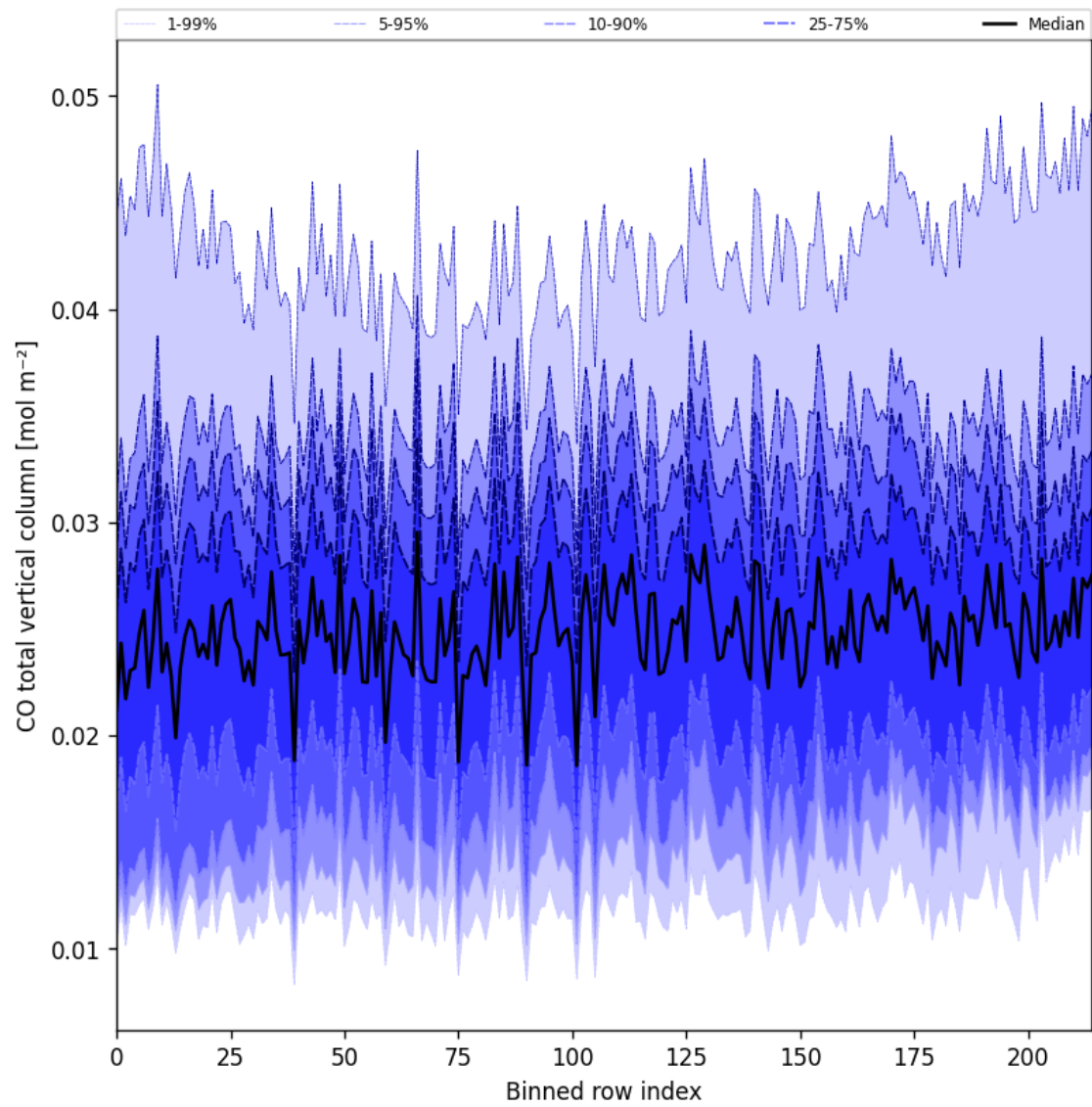
Figure 26: Along track statistics of “CO total vertical column” for 2025-10-06 to 2025-10-07
