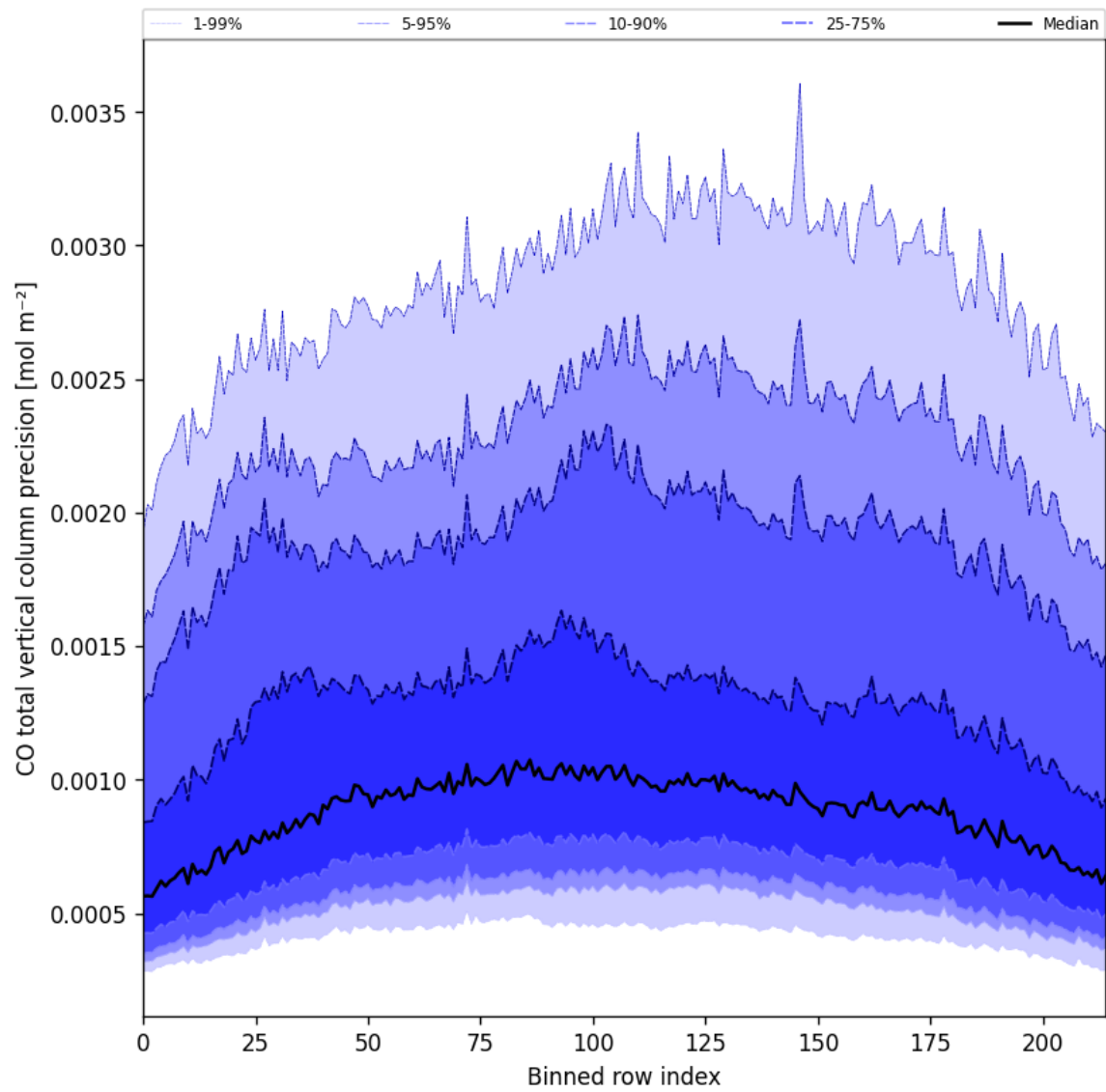
Figure 28: Along track statistics of “CO total vertical column precision” for 2025-10-06 to 2025-10-07
