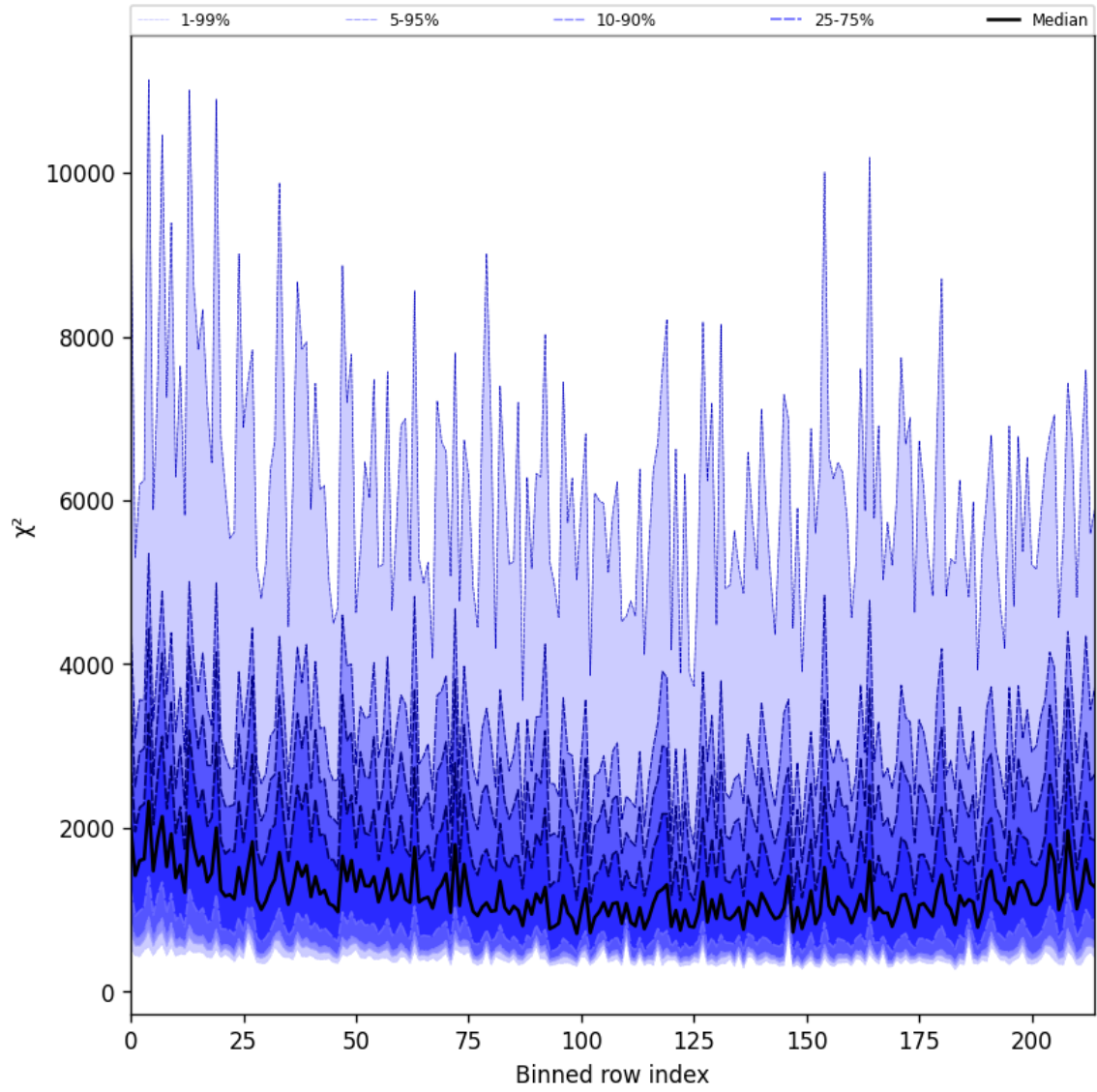
Figure 30: Along track statistics of “ \chi^2 ” for 2025-10-06 to 2025-10-07
