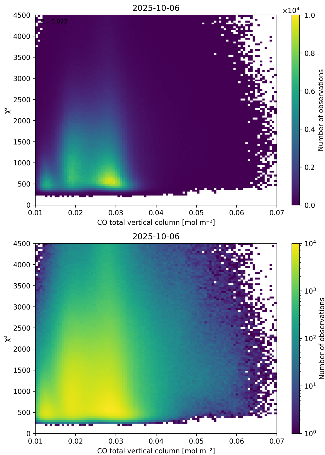
Figure 35: Scatter density plot of “CO total vertical column” against “ \chi^2 ” for 2025-10-06 to 2025-10-07.
