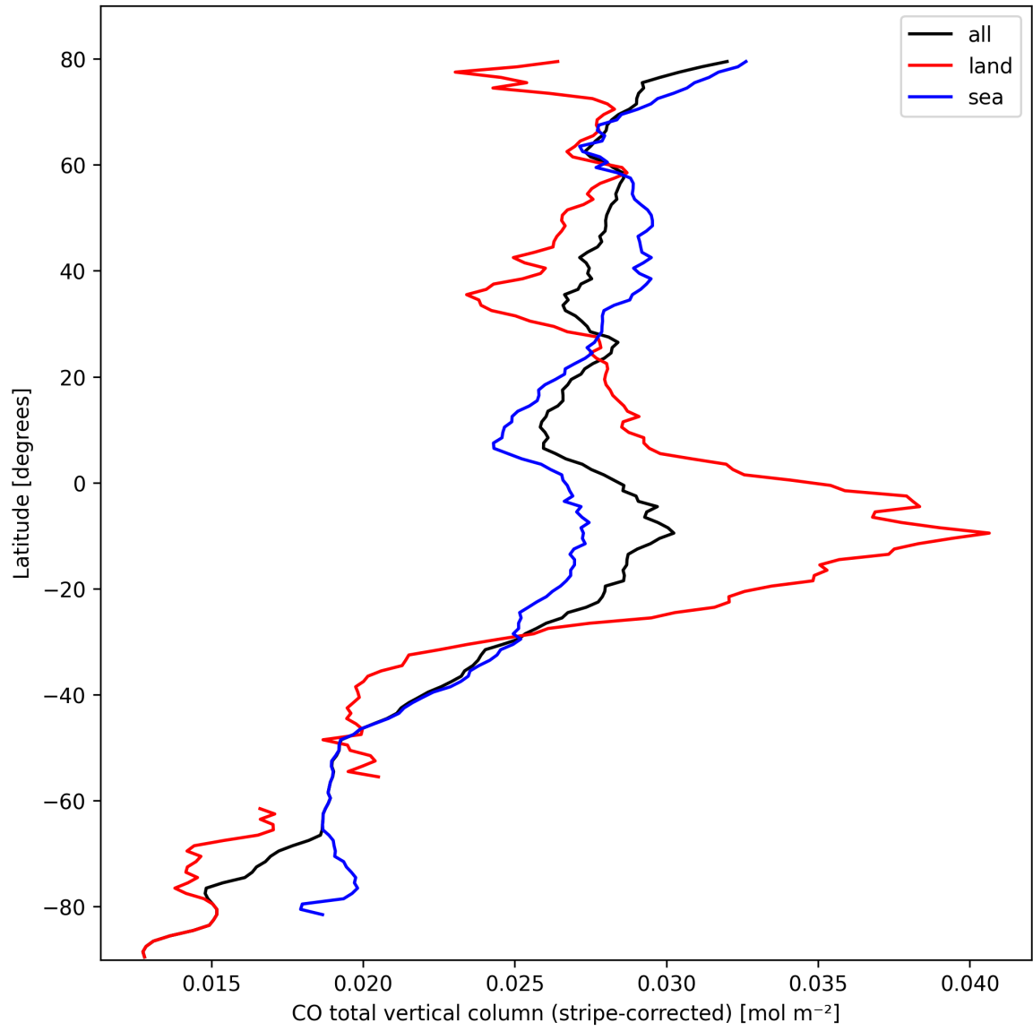
Figure 11: Zonal average of “CO total vertical column (stripe-corrected)” for 2025-10-06 to 2025-10-07.
