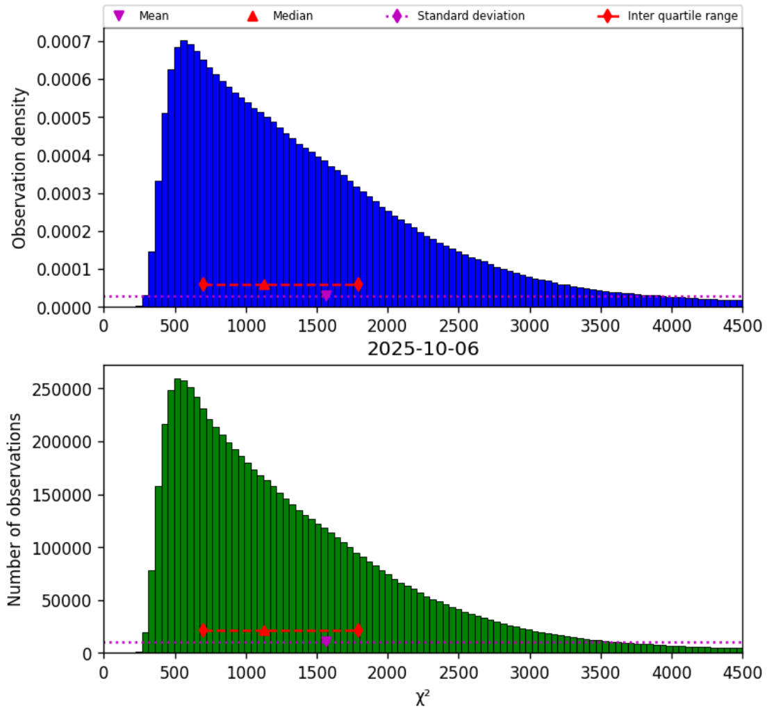
Figure 22: Histogram of " \chi^2 " for 2025-10-06 to 2025-10-07
