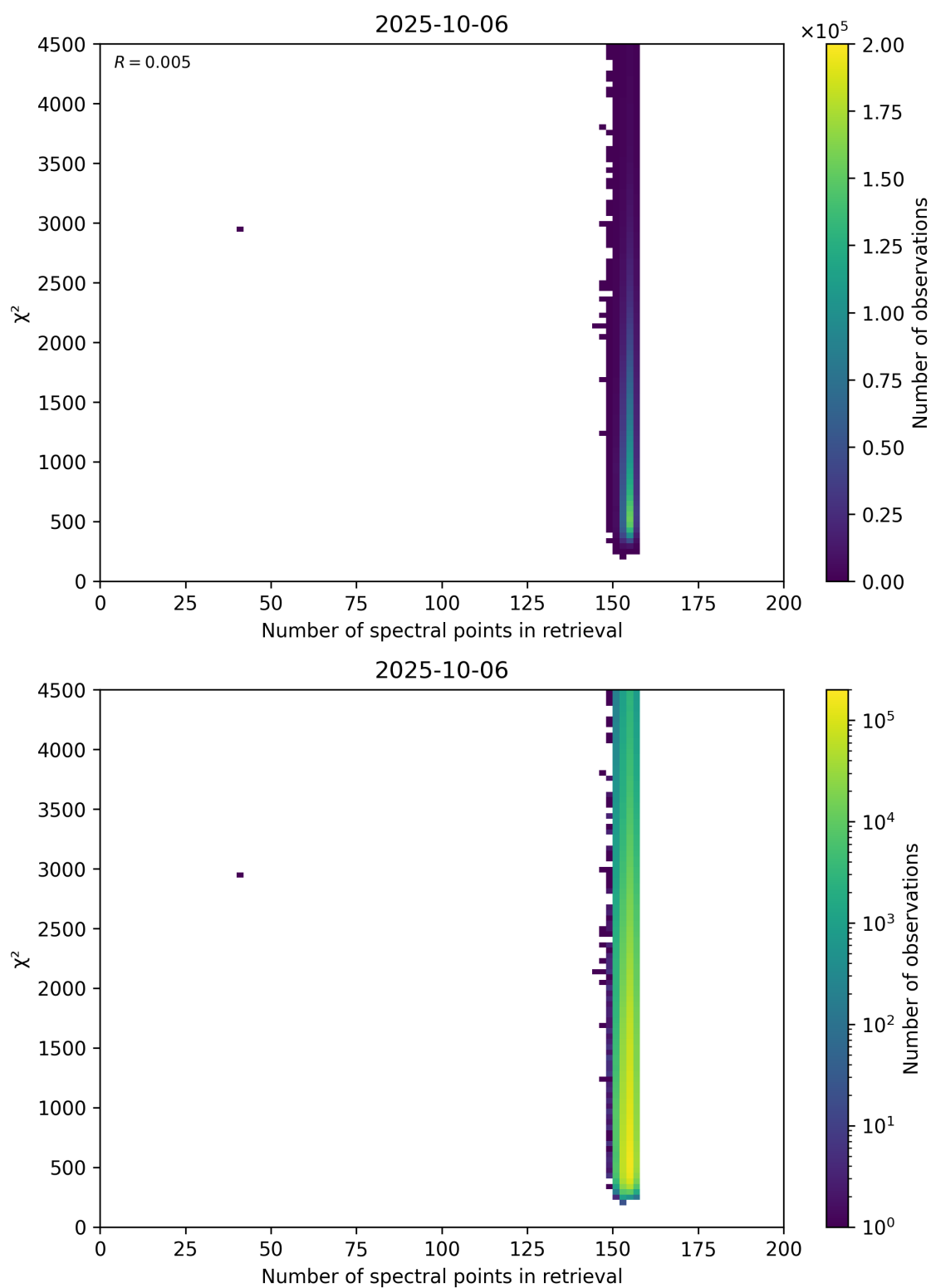
Figure 58: Scatter density plot of “Number of spectral points in retrieval” against “ \chi^2 ” for 2025-10-06 to 2025-10-07.
