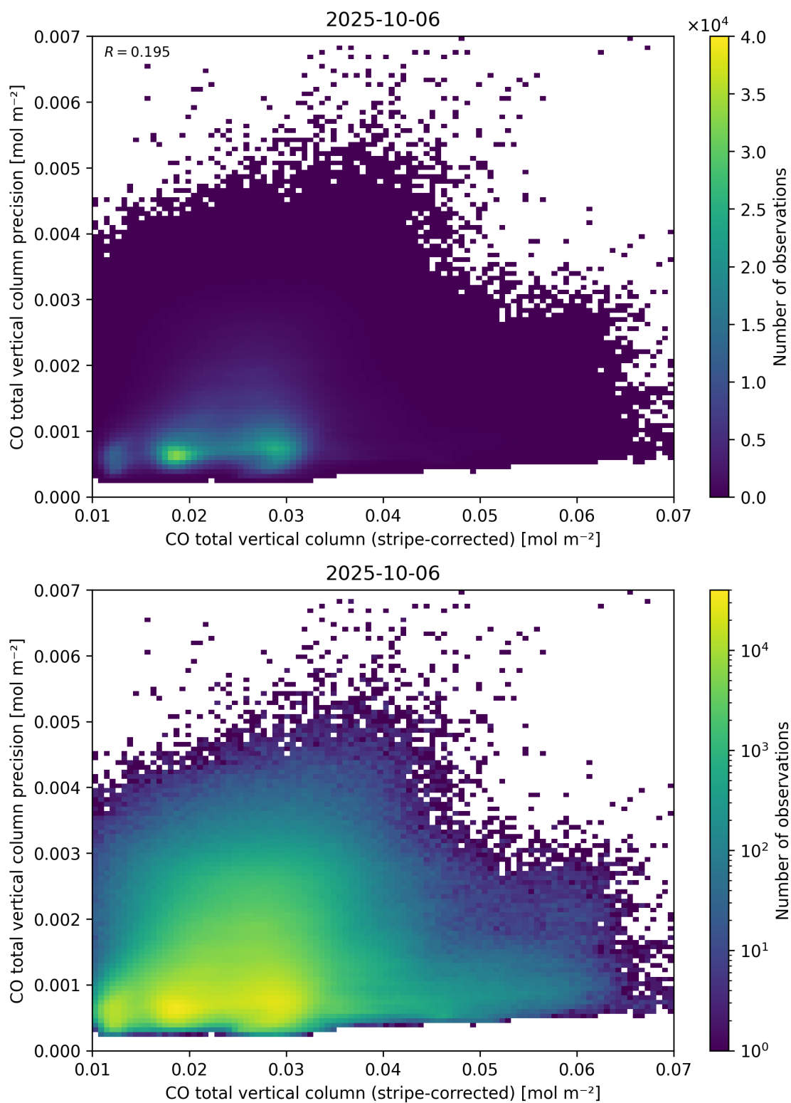
Figure 36: Scatter density plot of “CO total vertical column (stripe-corrected)” against “CO total vertical column precision” for 2025-10-06 to 2025-10-07.
