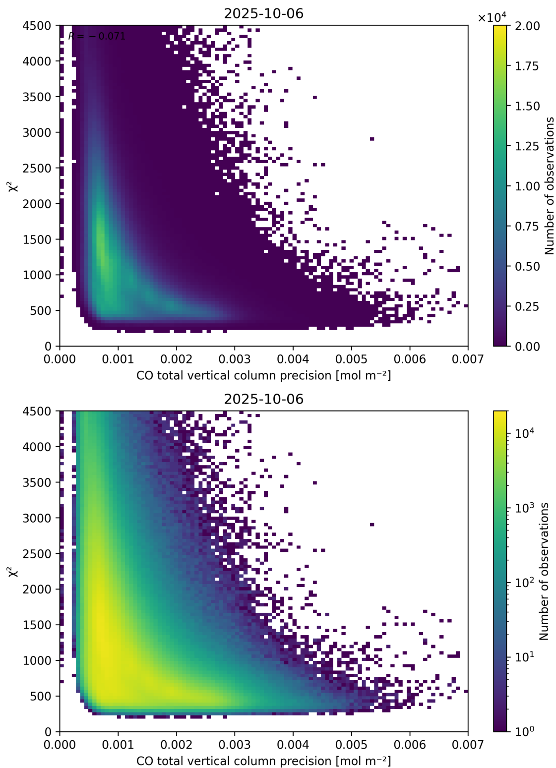
Figure 44: Scatter density plot of “CO total vertical column precision” against “ \chi^2 ” for 2025-10-06 to 2025-10-07.
