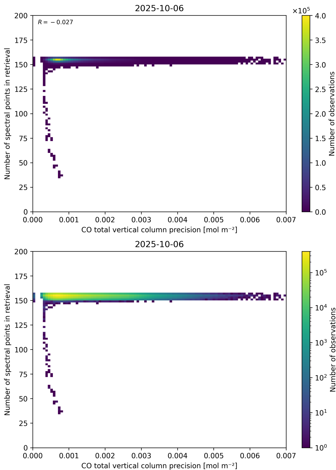
Figure 47: Scatter density plot of “CO total vertical column precision” against “Number of spectral points in retrieval” for 2025-10-06 to 2025-10-07.
