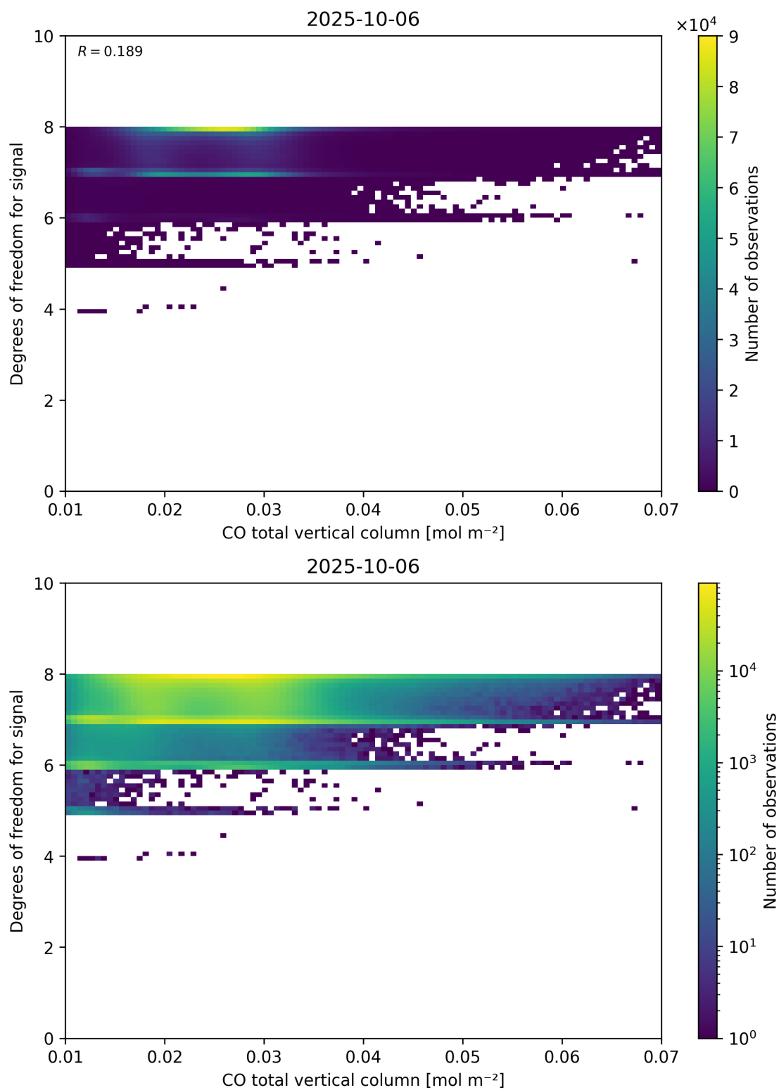
Figure 41: Scatter density plot of “CO total vertical column” against “Degrees of freedom for signal” for 2025-10-06 to 2025-10-07.
