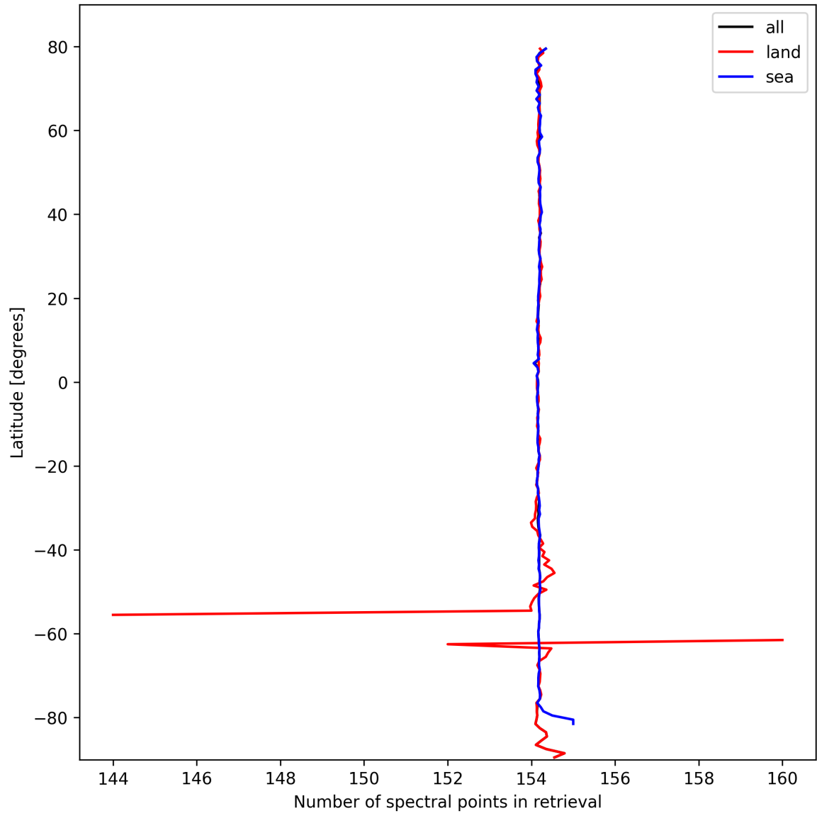
Figure 13: Zonal average of “Number of spectral points in retrieval” for 2025-10-06 to 2025-10-07.
