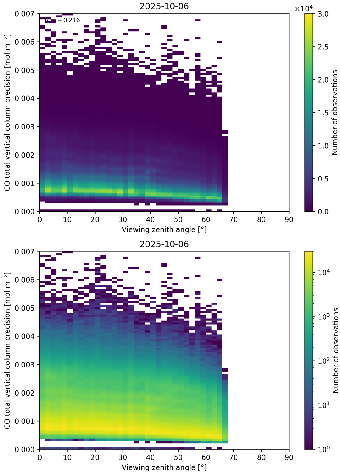
Figure 71: Scatter density plot of “Viewing zenith angle” against “CO total vertical column precision” for 2025-10-06 to 2025-10-07.
