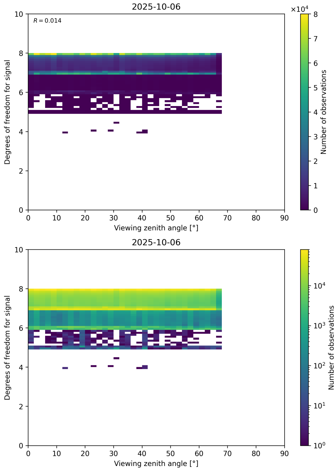
Figure 73: Scatter density plot of “Viewing zenith angle” against “Degrees of freedom for signal” for 2025-10-06 to 2025-10-07.
