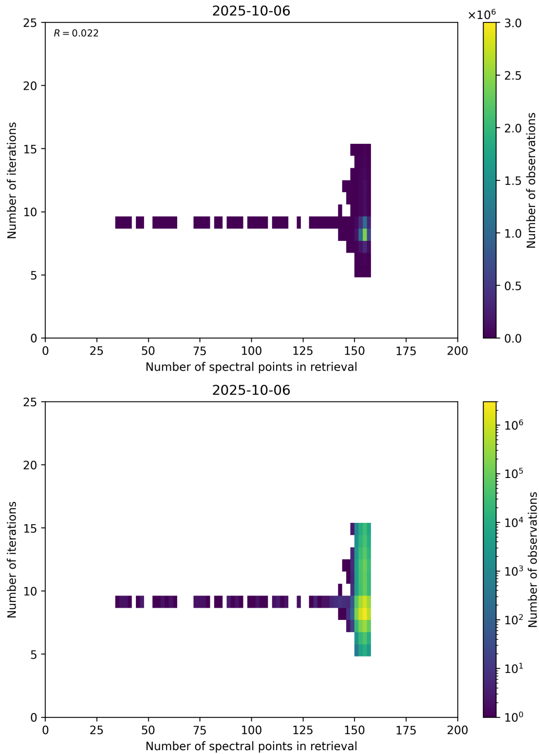
Figure 60: Scatter density plot of “Number of spectral points in retrieval” against “Number of iterations” for 2025-10-06 to 2025-10-07.
