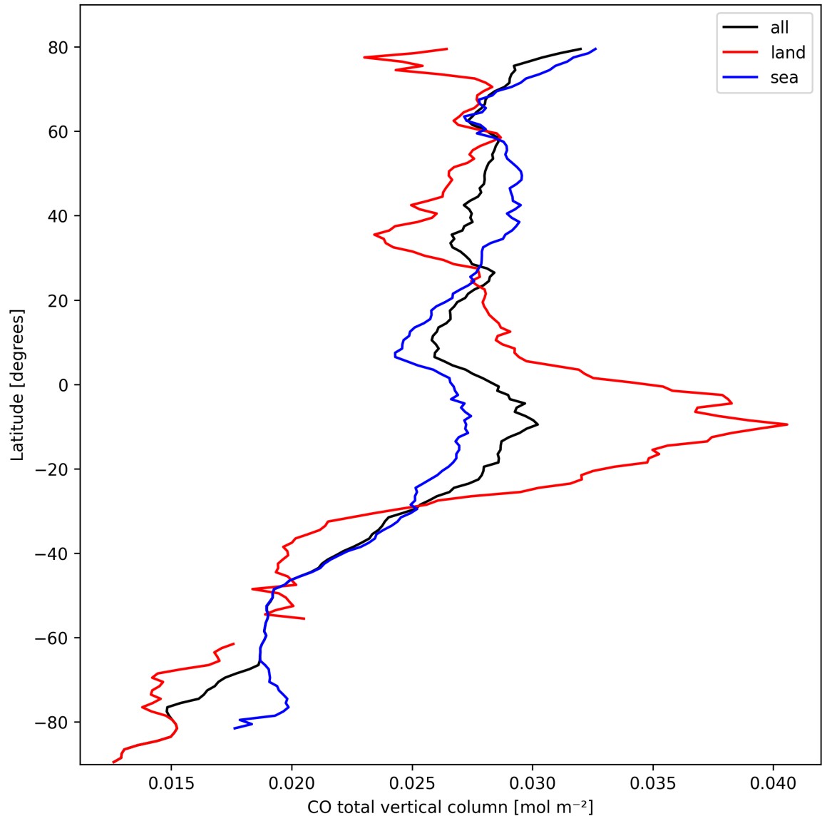
Figure 10: Zonal average of “CO total vertical column” for 2025-10-06 to 2025-10-07.
