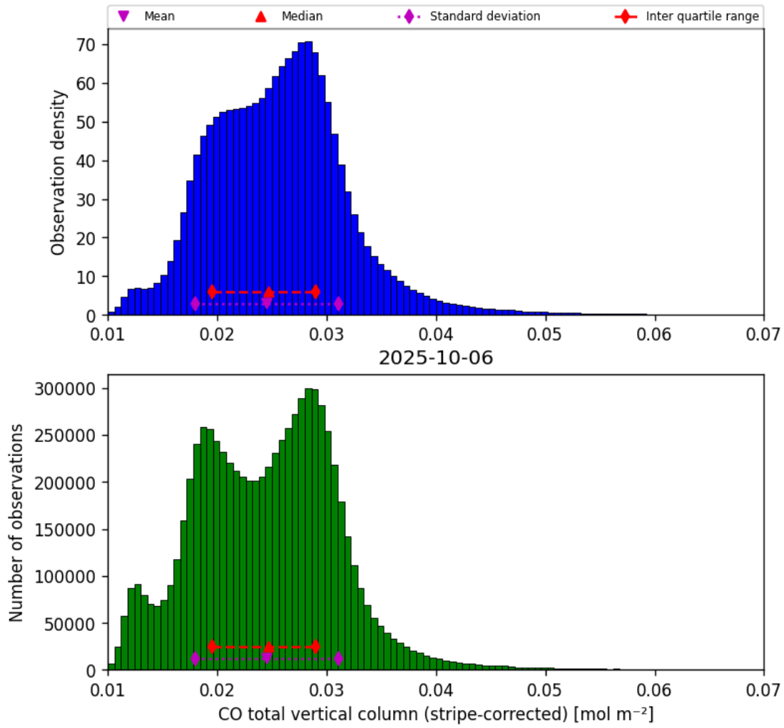
Figure 19: Histogram of “CO total vertical column (stripe-corrected)” for 2025-10-06 to 2025-10-07
