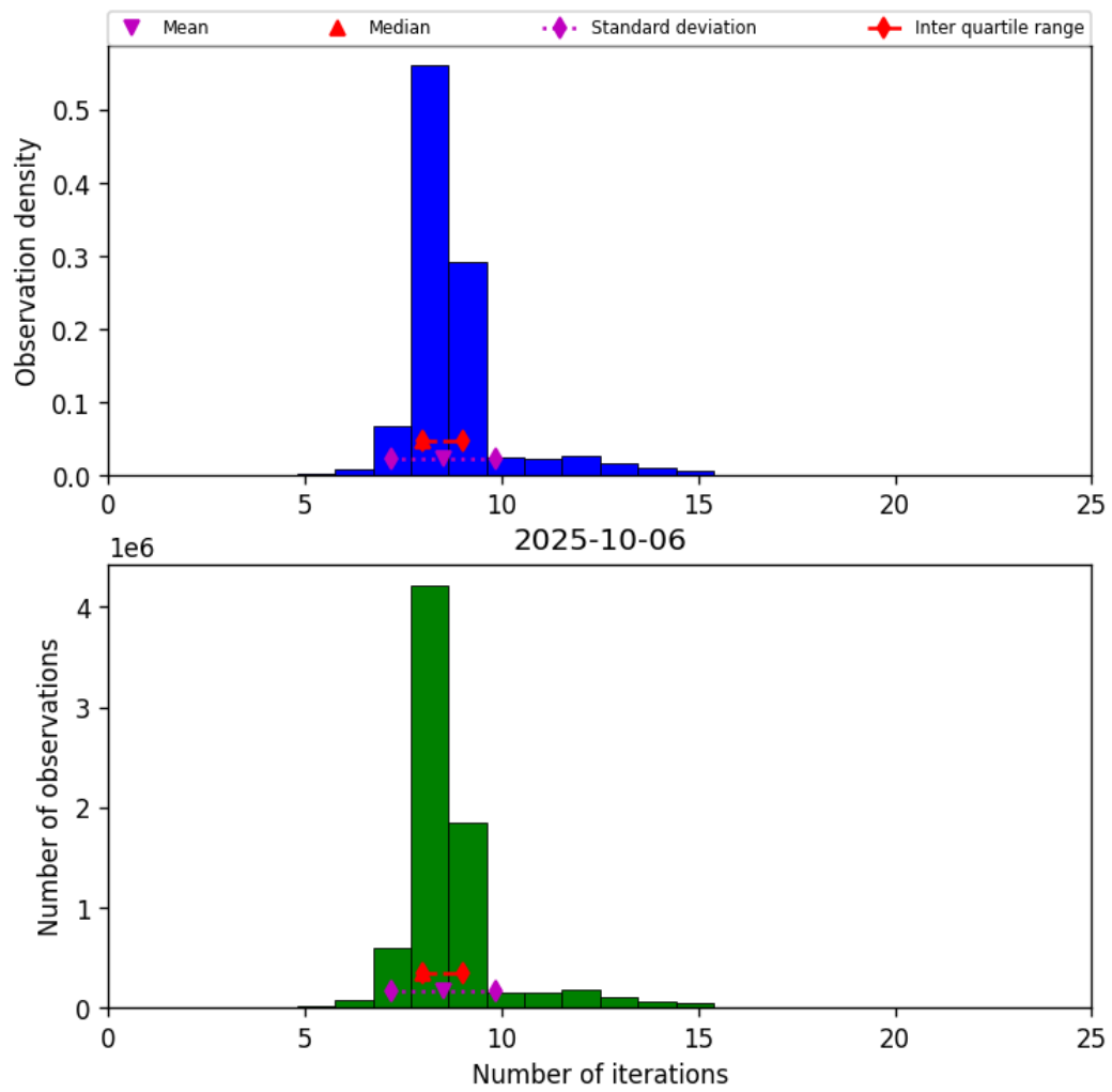
Figure 24: Histogram of “Number of iterations” for 2025-10-06 to 2025-10-07
