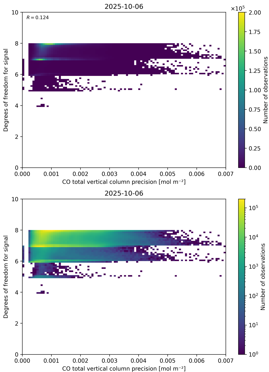
Figure 45: Scatter density plot of “CO total vertical column precision” against “Degrees of freedom for signal” for 2025-10-06 to 2025-10-07.
