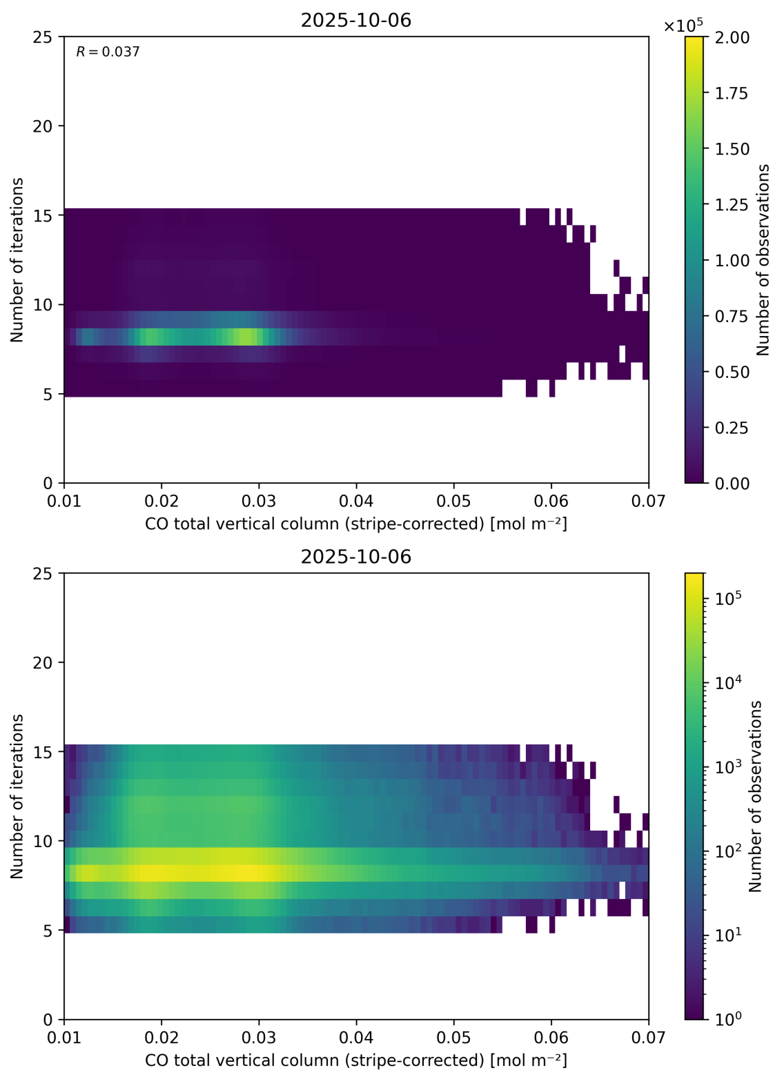
Figure 39: Scatter density plot of “CO total vertical column (stripe-corrected)” against “Number of iterations” for 2025-10-06 to 2025-10-07.
