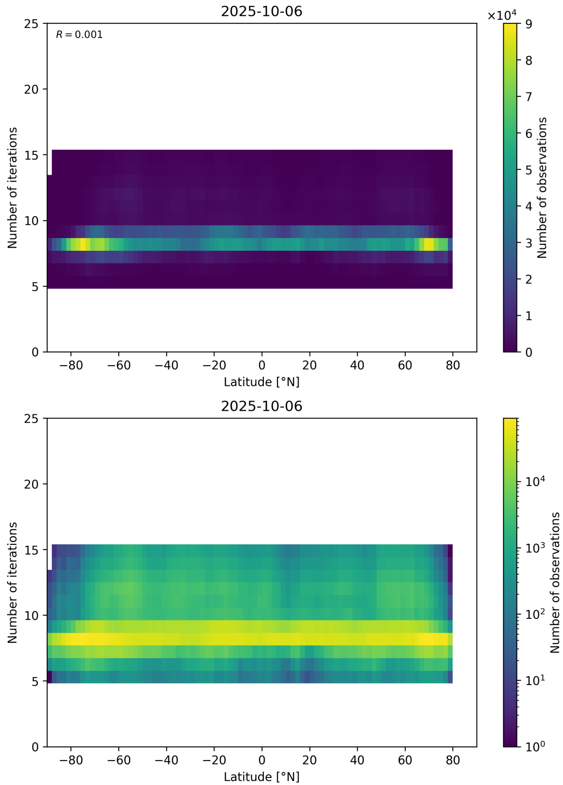
Figure 56: Scatter density plot of “Latitude” against “Number of iterations” for 2025-10-06 to 2025-10-07.
