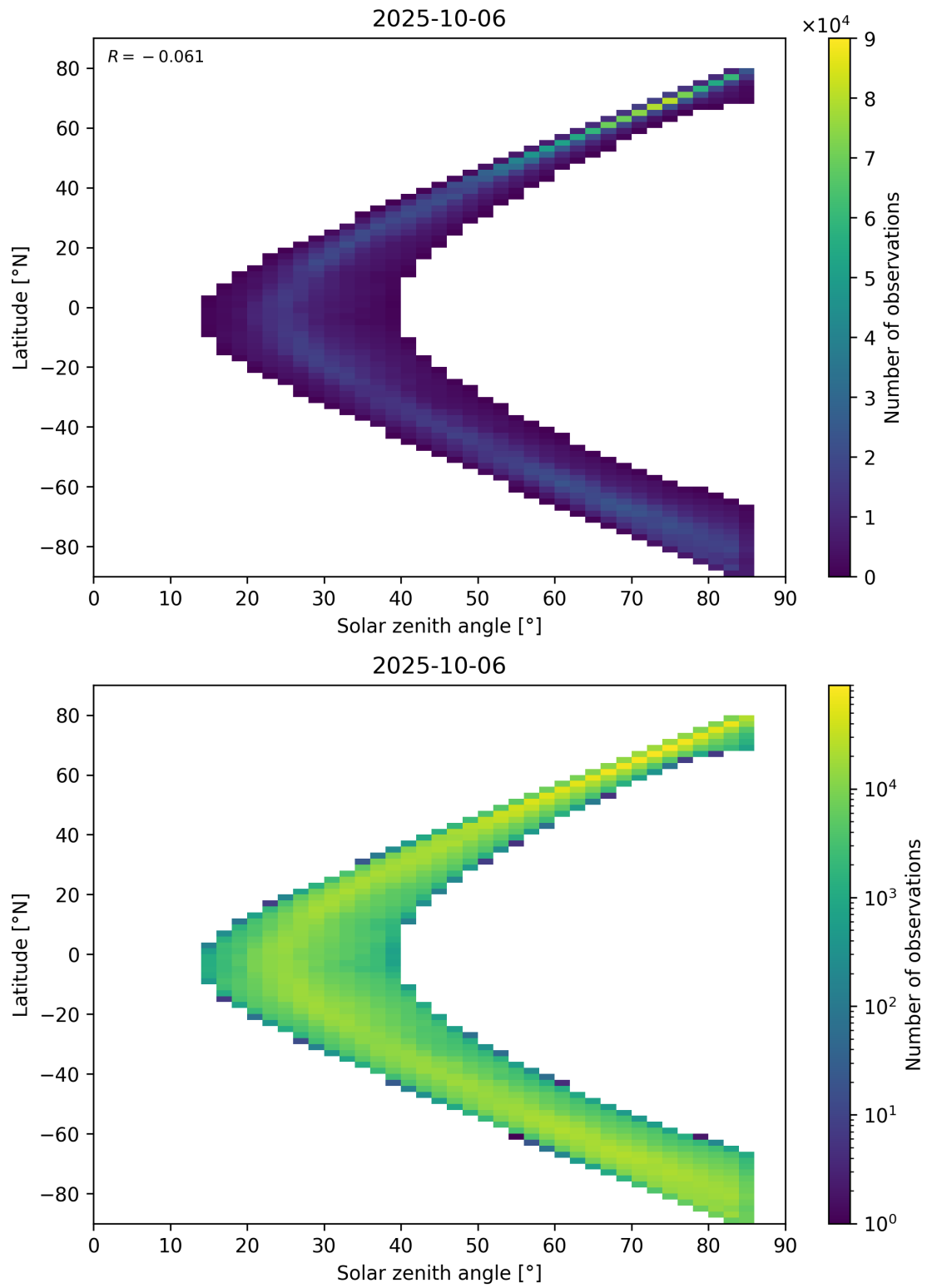
Figure 66: Scatter density plot of “Solar zenith angle” against “Latitude” for 2025-10-06 to 2025-10-07.
