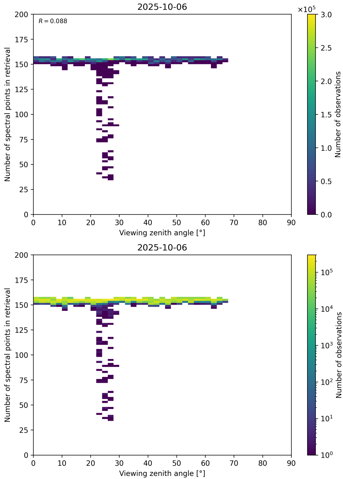
Figure 76: Scatter density plot of “Viewing zenith angle” against “Number of spectral points in retrieval” for 2025-10-06 to 2025-10-07.
