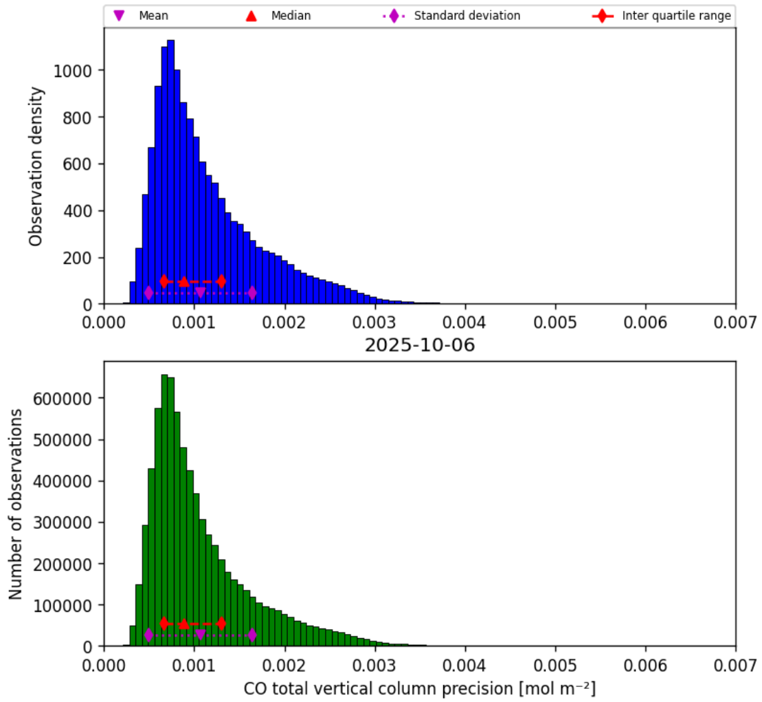
Figure 20: Histogram of “CO total vertical column precision” for 2025-10-06 to 2025-10-07
