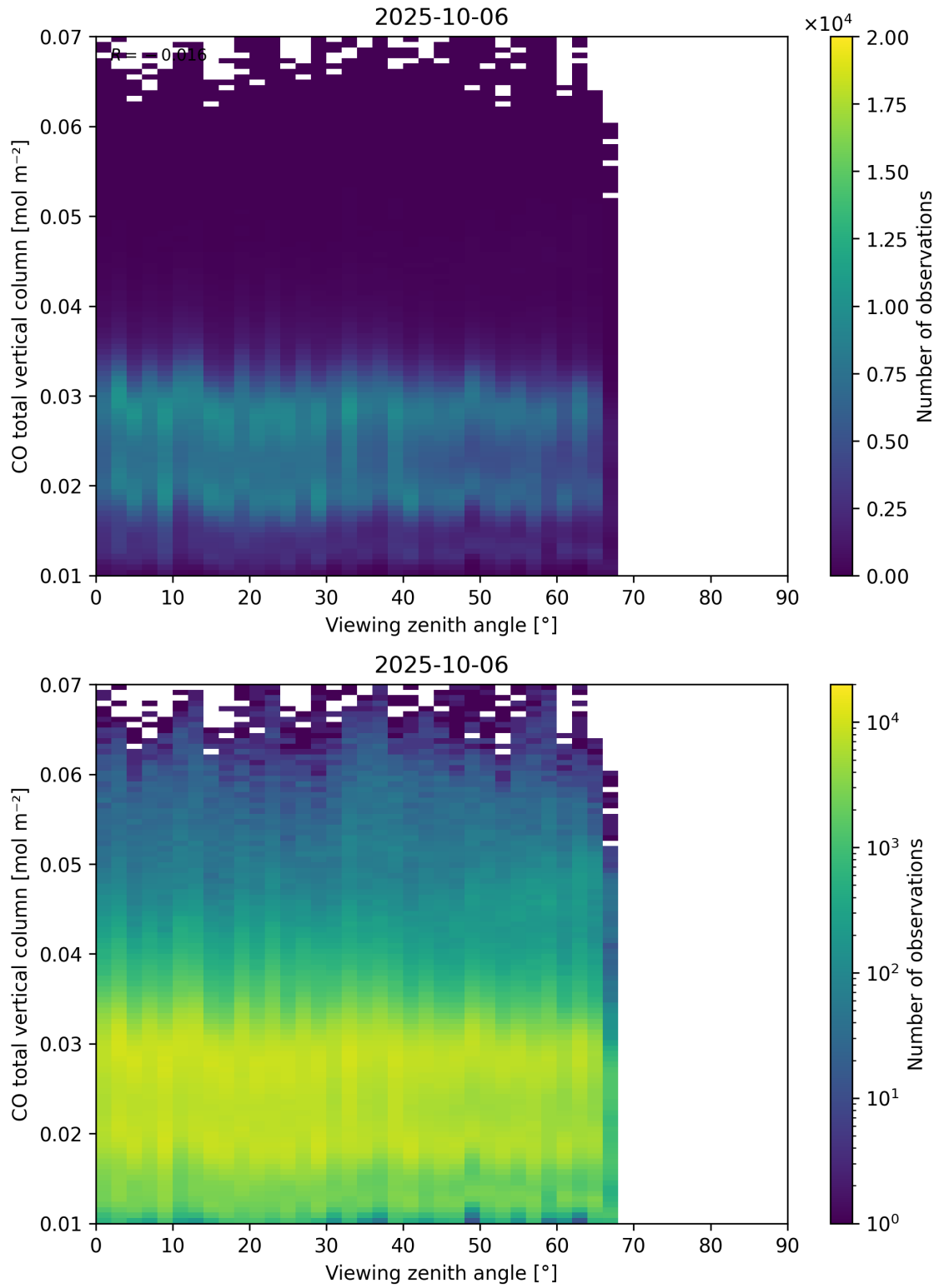
Figure 69: Scatter density plot of “Viewing zenith angle” against “CO total vertical column” for 2025-10-06 to 2025-10-07.
