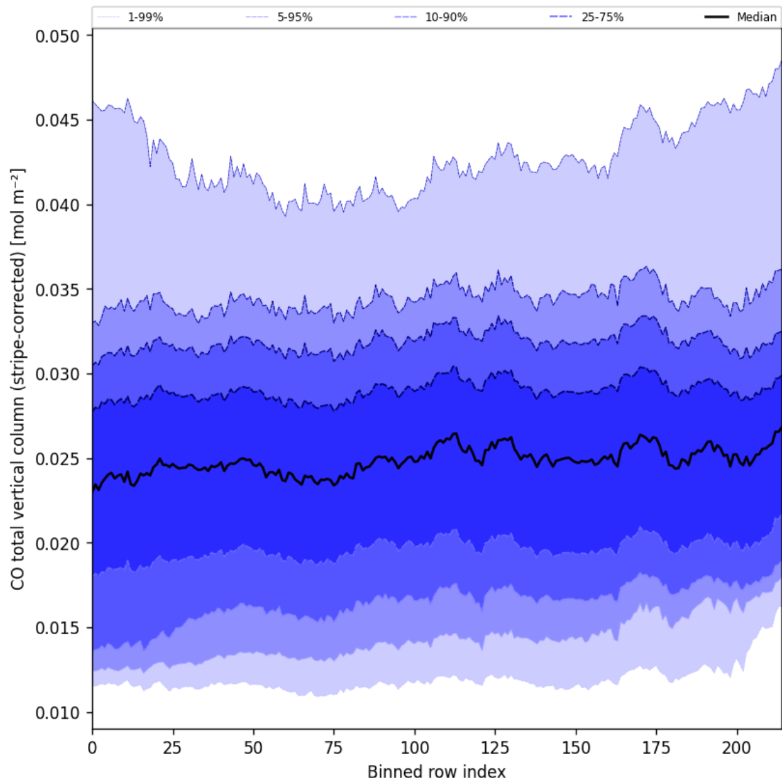
Figure 27: Along track statistics of “CO total vertical column (stripe-corrected)” for 2025-10-06 to 2025-10-07
