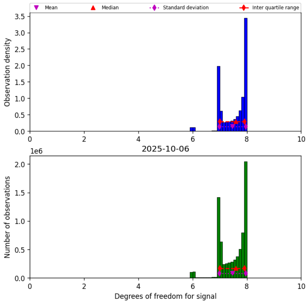
Figure 23: Histogram of “Degrees of freedom for signal” for 2025-10-06 to 2025-10-07
