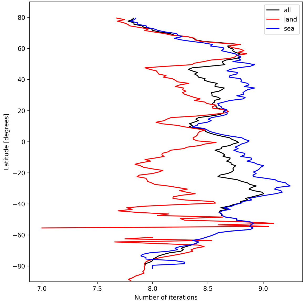
Figure 16: Zonal average of “Number of iterations” for 2025-10-06 to 2025-10-07.
