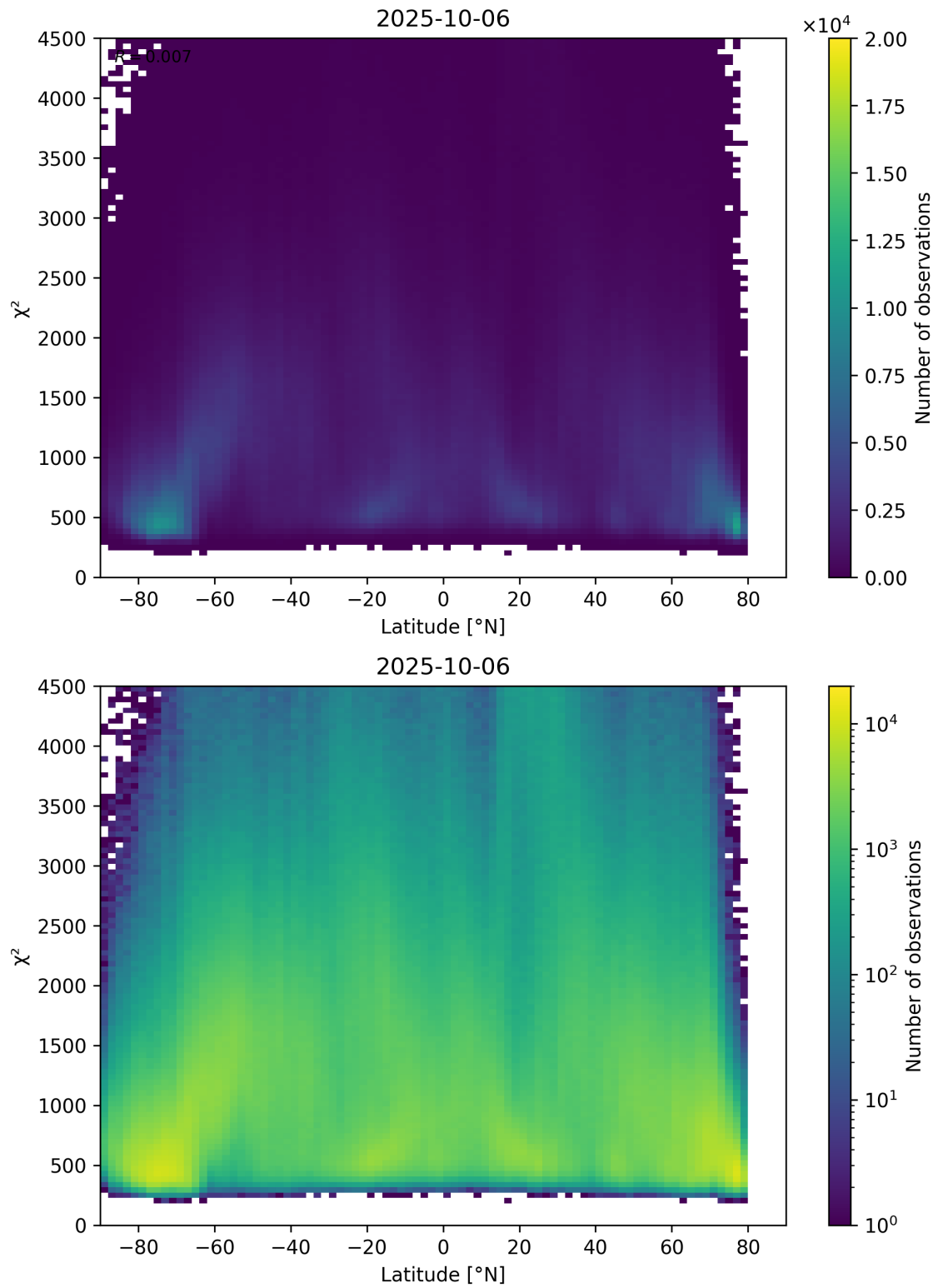
Figure 54: Scatter density plot of “Latitude” against “ \chi^2 ” for 2025-10-06 to 2025-10-07.
