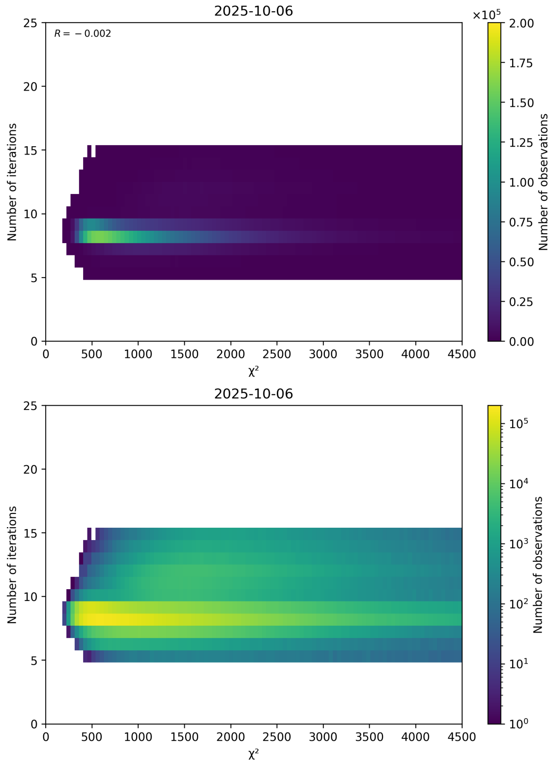
Figure 49: Scatter density plot of “ \chi^2 ” against “Number of iterations” for 2025-10-06 to 2025-10-07.
