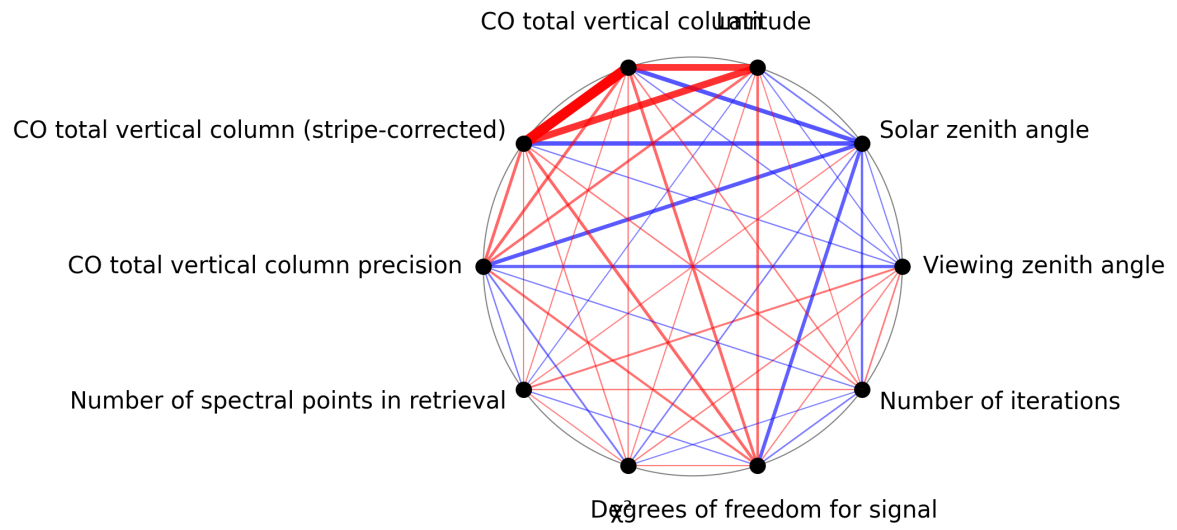
Figure 1: Map of correlation graph for 2025-10-06 to 2025-10-07.
