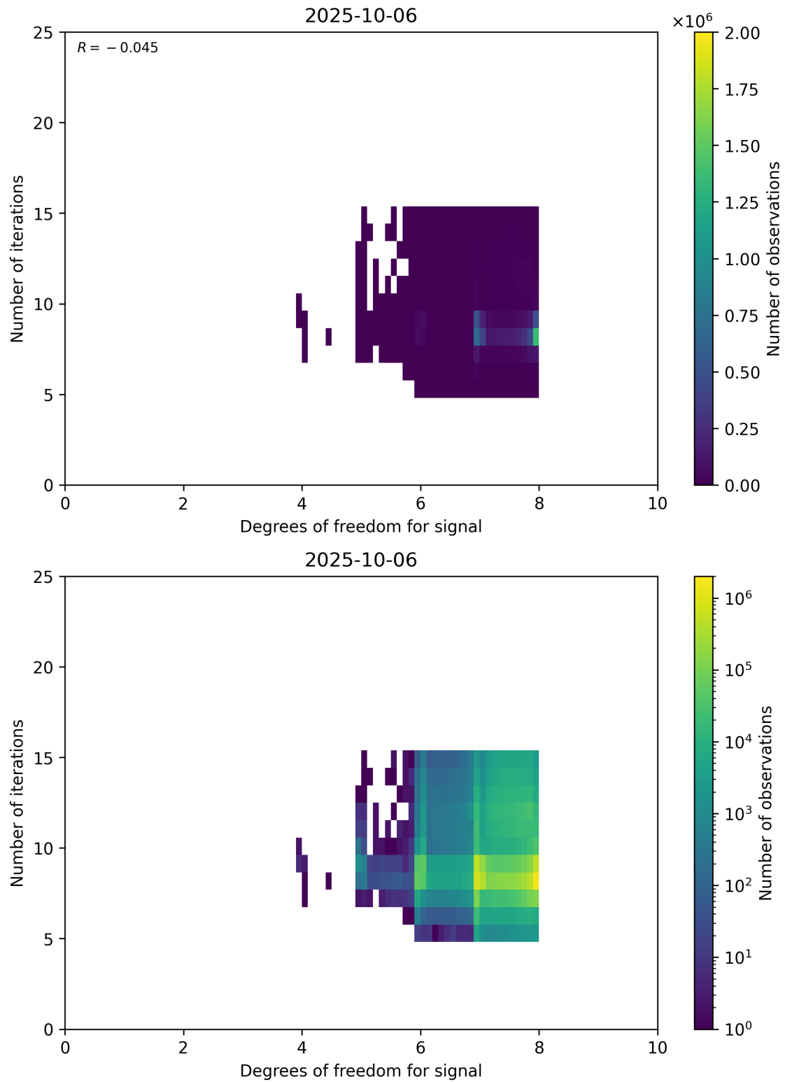
Figure 50: Scatter density plot of “Degrees of freedom for signal” against “Number of iterations” for 2025-10-06 to 2025-10-07.
