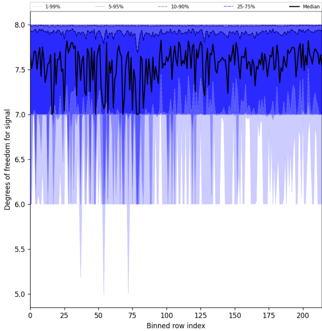
Figure 31: Along track statistics of “Degrees of freedom for signal” for 2025-10-06 to 2025-10-07
