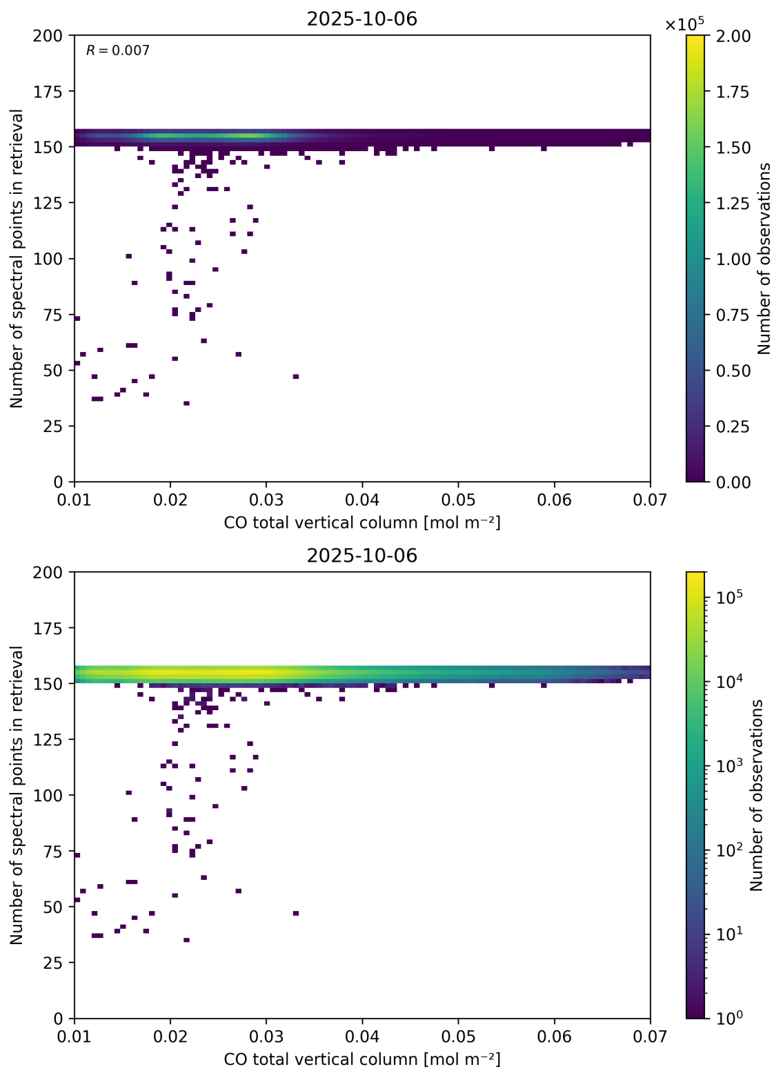
Figure 43: Scatter density plot of “CO total vertical column” against “Number of spectral points in retrieval” for 2025-10-06 to 2025-10-07.
