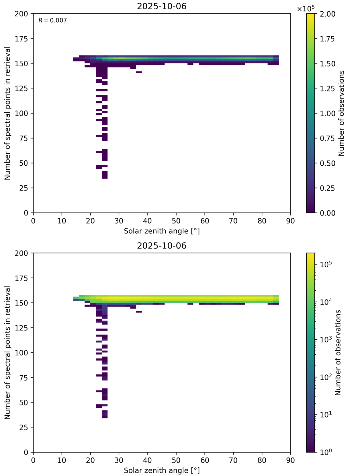
Figure 68: Scatter density plot of “Solar zenith angle” against “Number of spectral points in retrieval” for 2025-10-06 to 2025-10-07.
