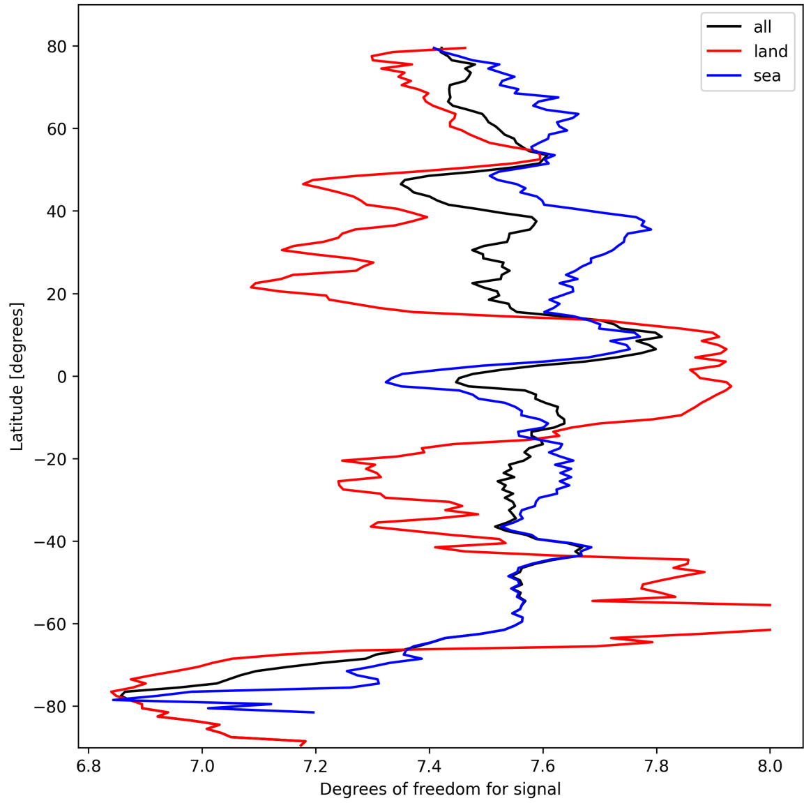
Figure 15: Zonal average of “Degrees of freedom for signal” for 2025-10-06 to 2025-10-07.
