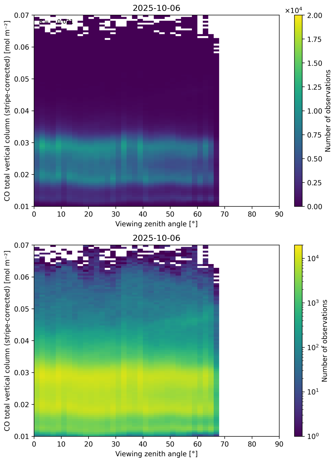
Figure 70: Scatter density plot of “Viewing zenith angle” against “CO total vertical column (stripe-corrected)” for 2025-10-06 to 2025-10-07.
