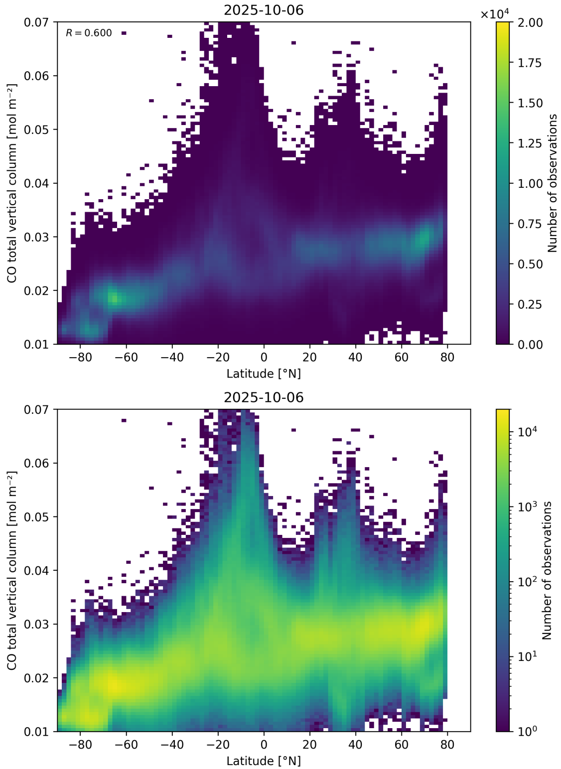
Figure 51: Scatter density plot of “Latitude” against “CO total vertical column” for 2025-10-06 to 2025-10-07.
