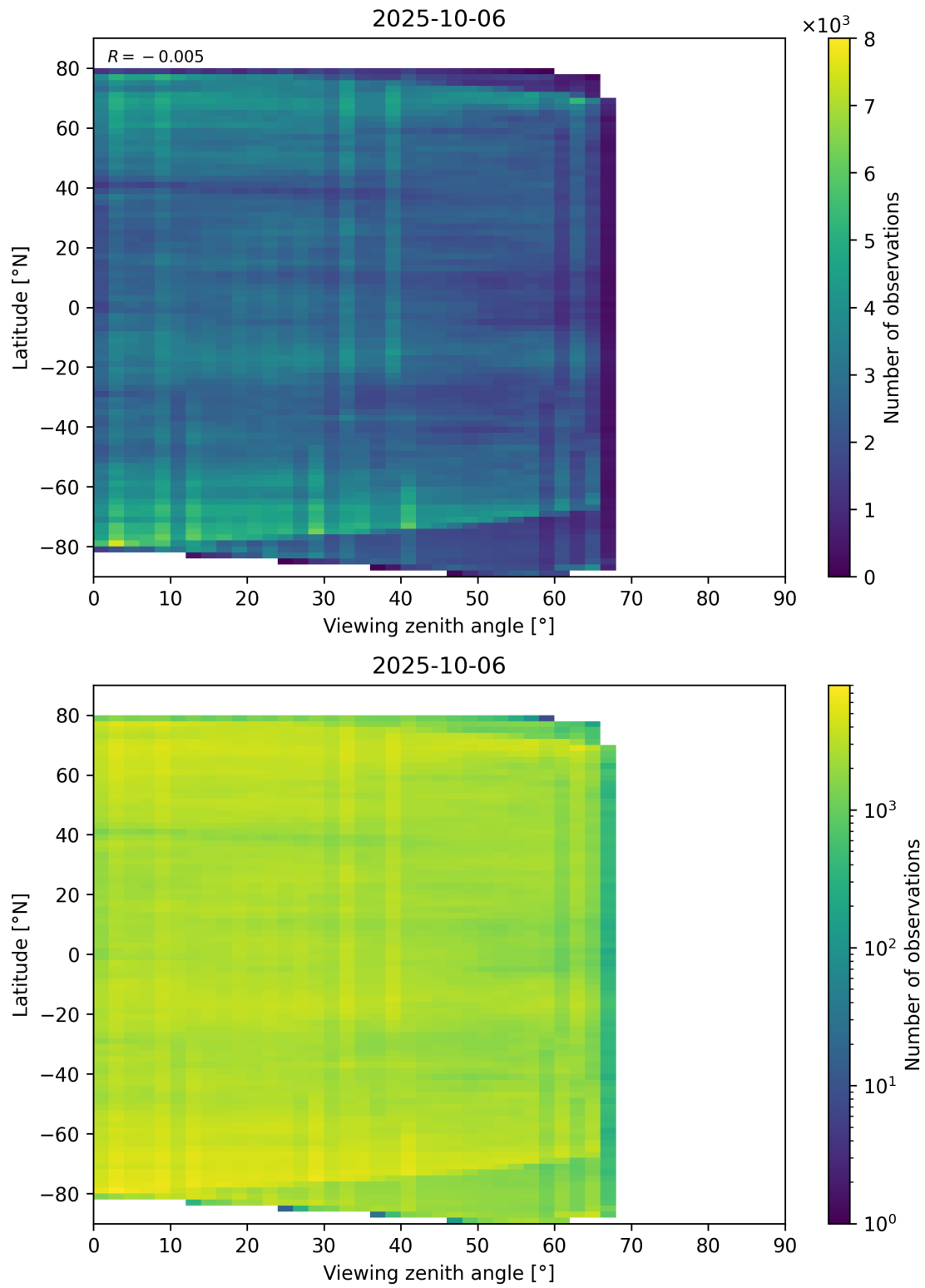
Figure 74: Scatter density plot of “Viewing zenith angle” against “Latitude” for 2025-10-06 to 2025-10-07.
