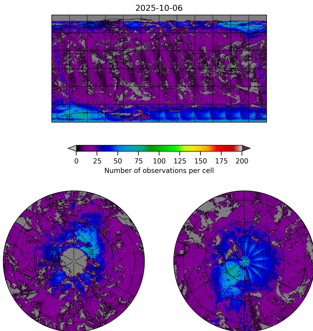
Figure 8: Map of the number of observations for 2025-10-06 to 2025-10-07
