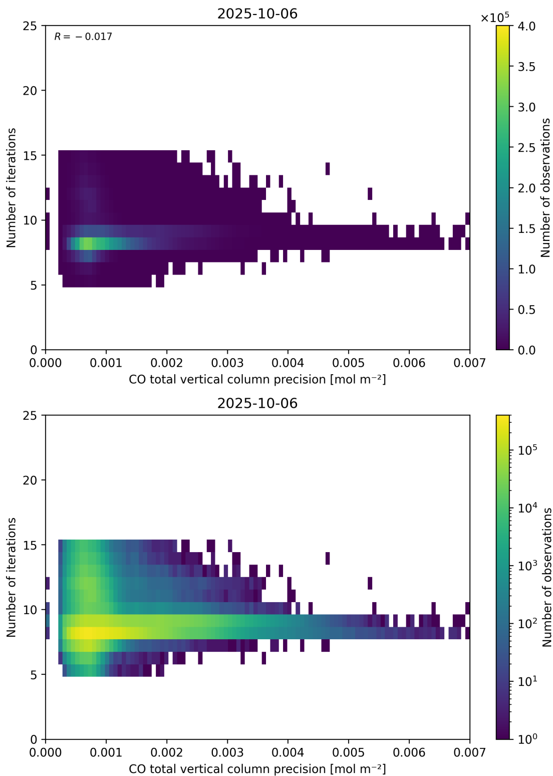
Figure 46: Scatter density plot of “CO total vertical column precision” against “Number of iterations” for 2025-10-06 to 2025-10-07.
