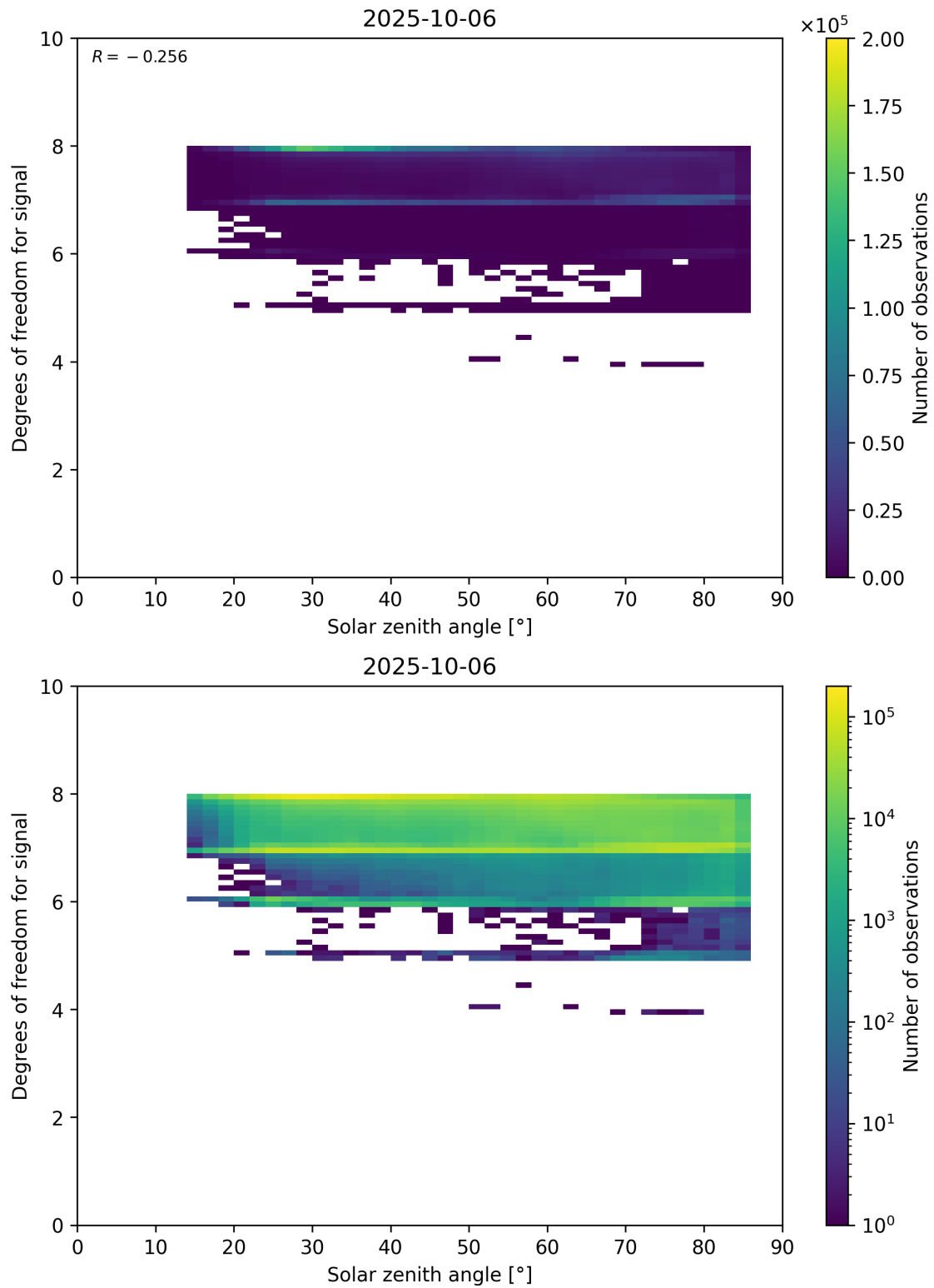
Figure 65: Scatter density plot of “Solar zenith angle” against “Degrees of freedom for signal” for 2025-10-06 to 2025-10-07.
