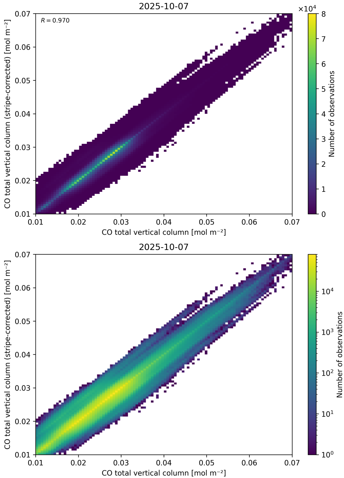
Figure 33: Scatter density plot of “CO total vertical column” against “CO total vertical column (stripe-corrected)” for 2025-10-06 to 2025-10-08.
