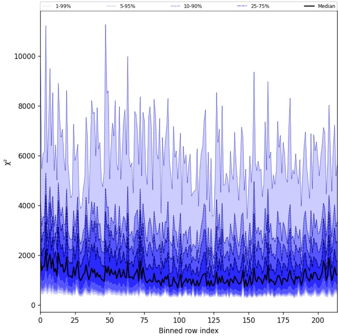
Figure 30: Along track statistics of “ \chi^2 ” for 2025-10-06 to 2025-10-08
