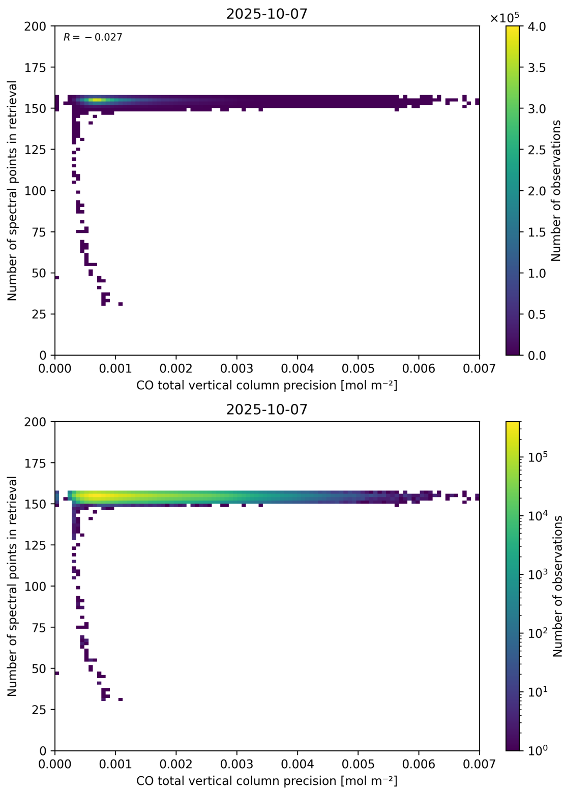
Figure 47: Scatter density plot of “CO total vertical column precision” against “Number of spectral points in retrieval” for 2025-10-06 to 2025-10-08.
