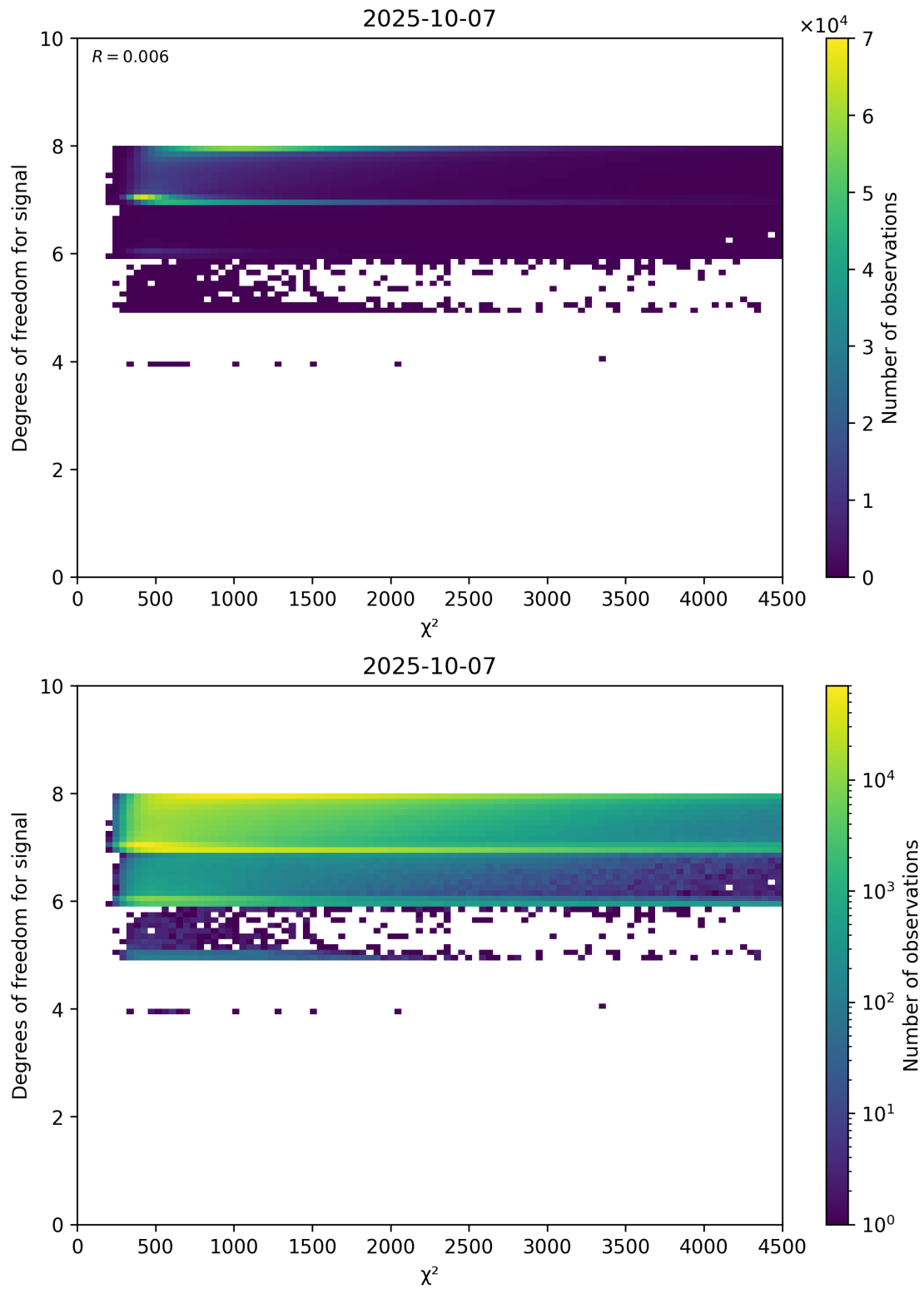
Figure 48: Scatter density plot of “ \chi^2 ” against “Degrees of freedom for signal” for 2025-10-06 to 2025-10-08.
