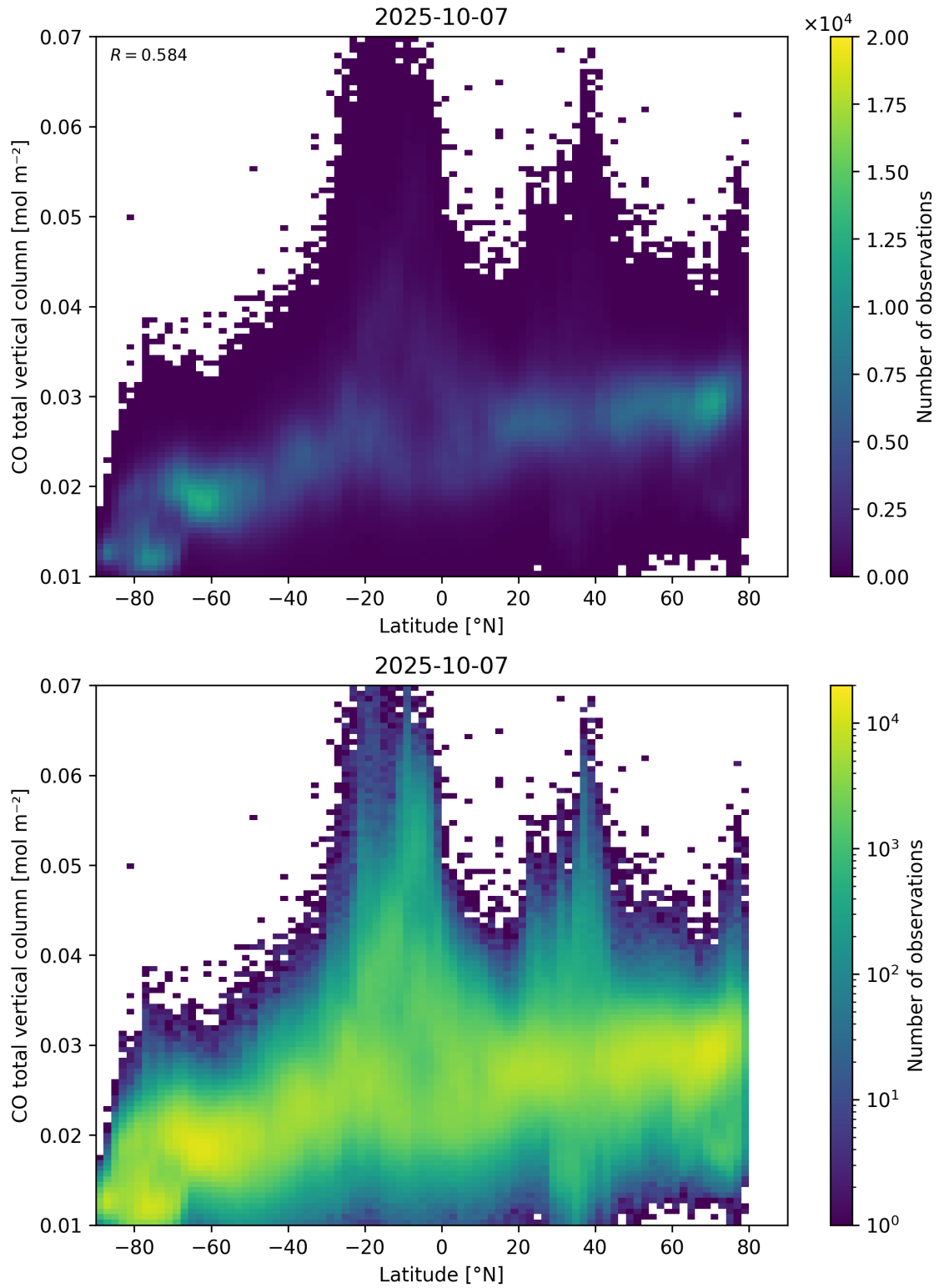
Figure 51: Scatter density plot of “Latitude” against “CO total vertical column” for 2025-10-06 to 2025-10-08.
