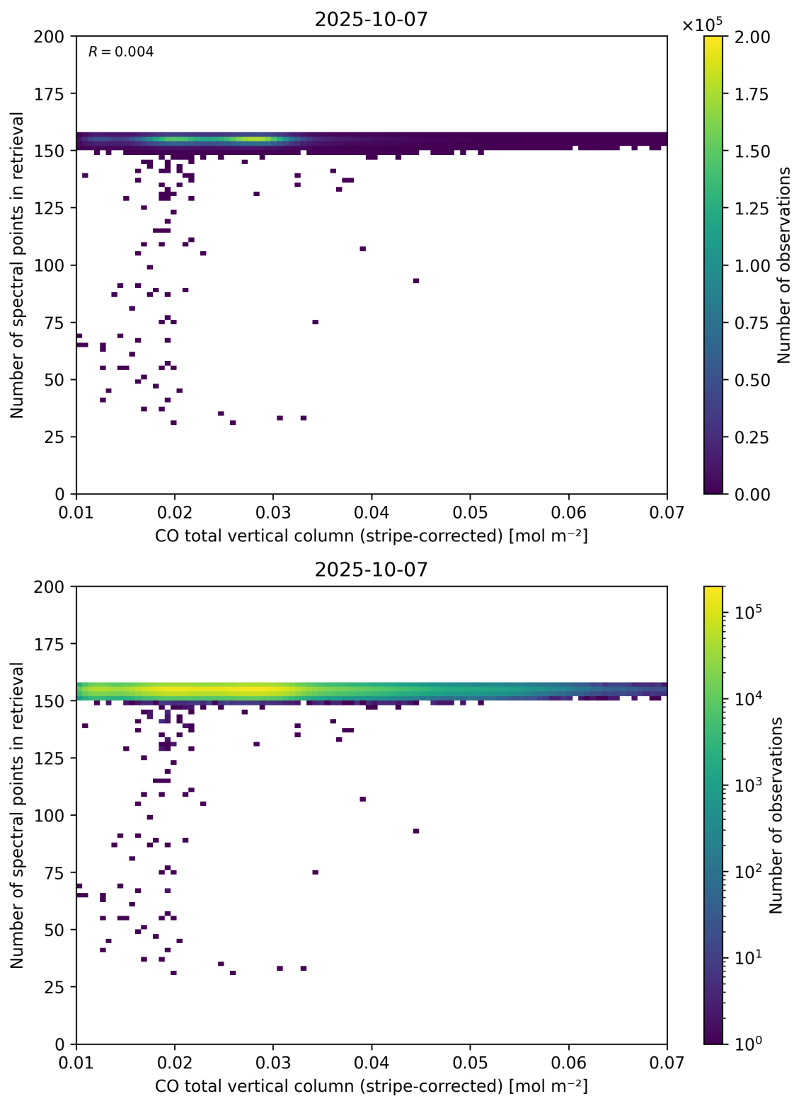
Figure 40: Scatter density plot of “CO total vertical column (stripe-corrected)” against “Number of spectral points in retrieval” for 2025-10-06 to 2025-10-08.
