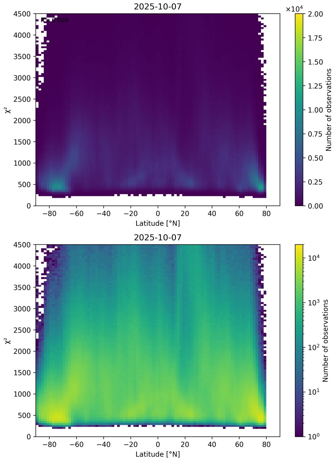
Figure 54: Scatter density plot of “Latitude” against “ \chi^2 ” for 2025-10-06 to 2025-10-08.
