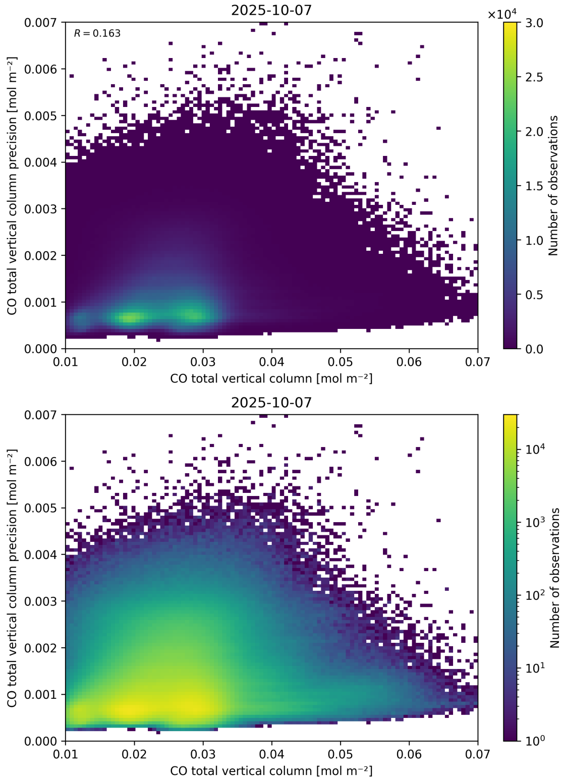
Figure 34: Scatter density plot of “CO total vertical column” against “CO total vertical column precision” for 2025-10-06 to 2025-10-08.
