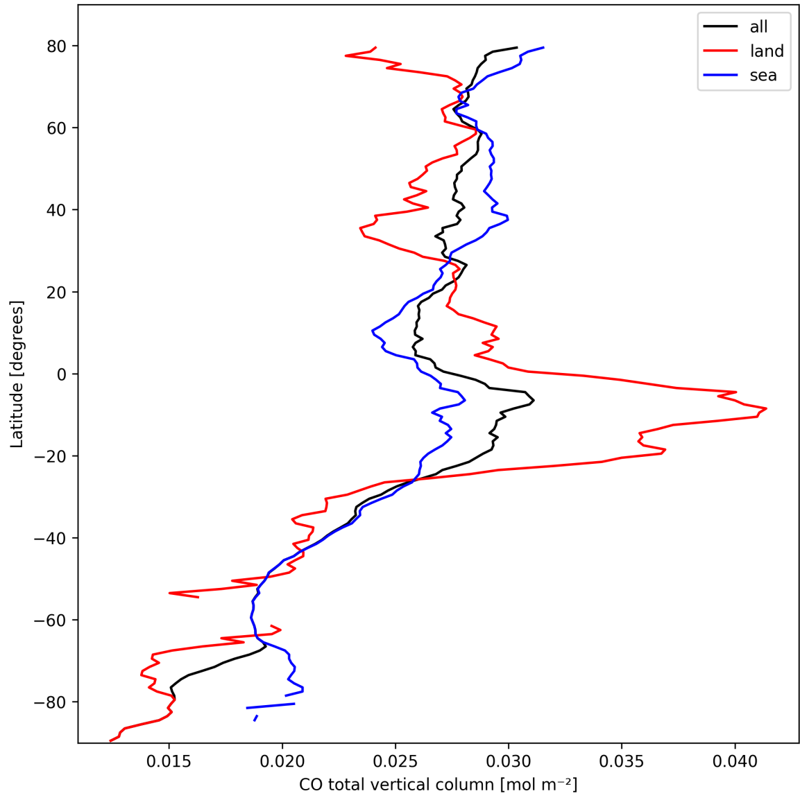
Figure 10: Zonal average of “CO total vertical column” for 2025-10-06 to 2025-10-08.
