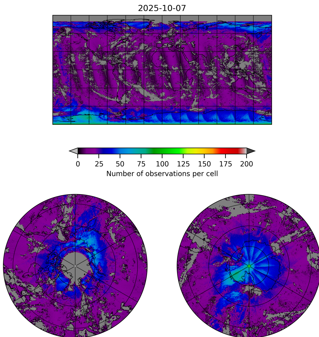
Figure 8: Map of the number of observations for 2025-10-06 to 2025-10-08
