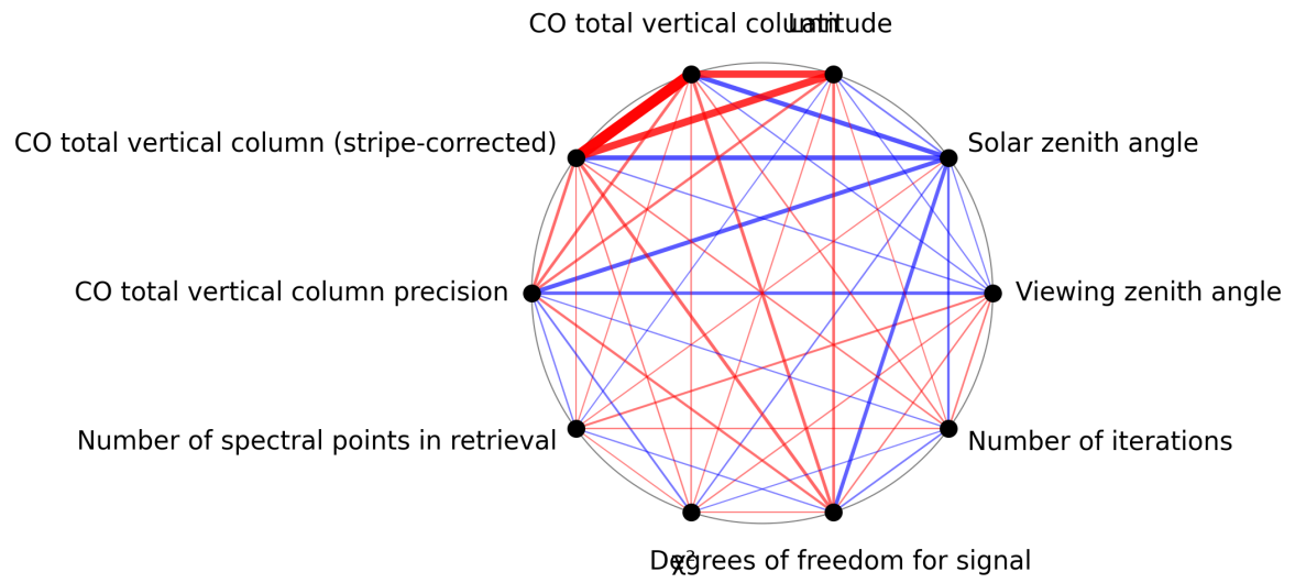
Figure 1: Map of correlation graph for 2025-10-06 to 2025-10-08.
