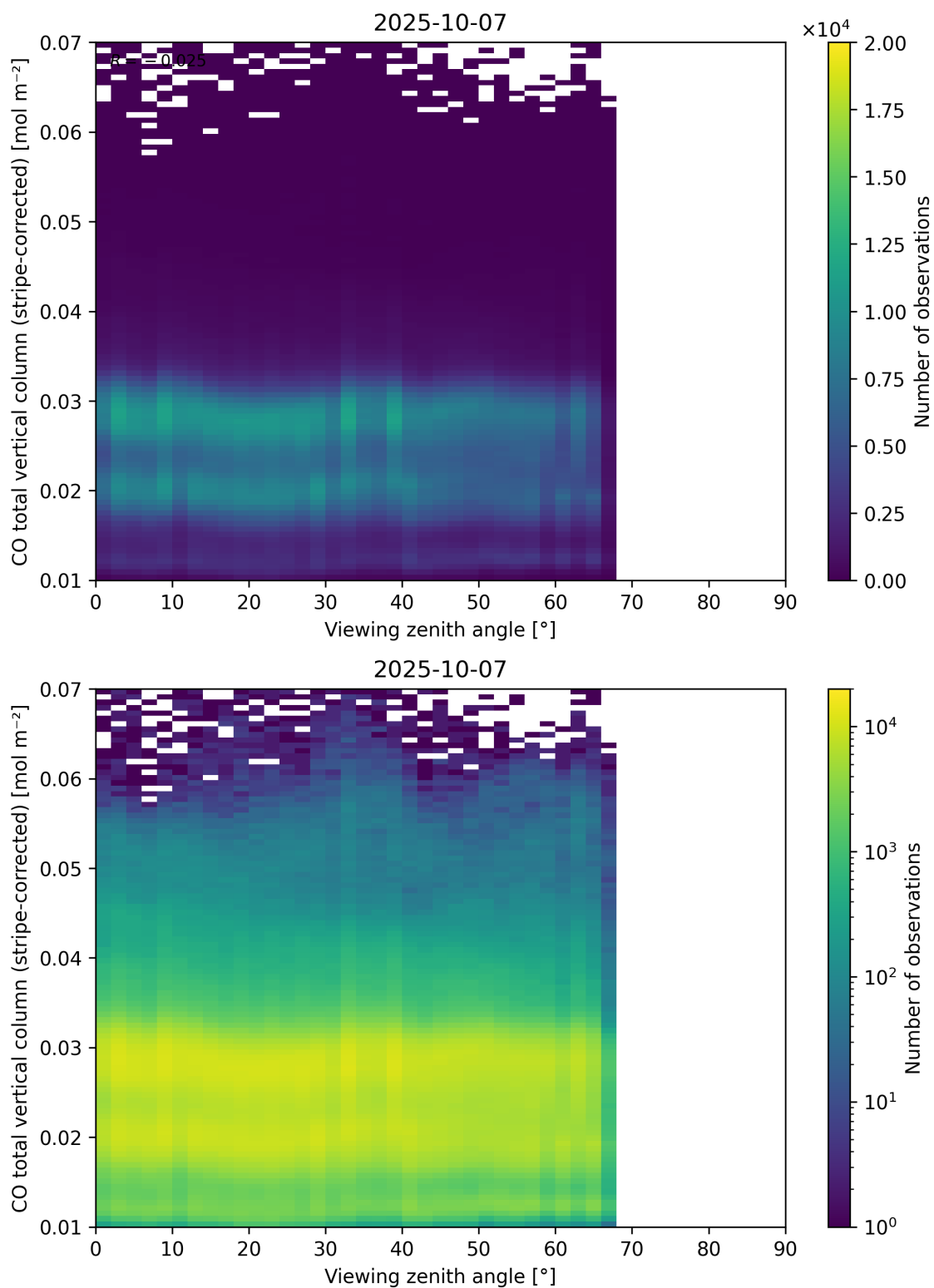
Figure 70: Scatter density plot of “Viewing zenith angle” against “CO total vertical column (stripe-corrected)” for 2025-10-06 to 2025-10-08.
