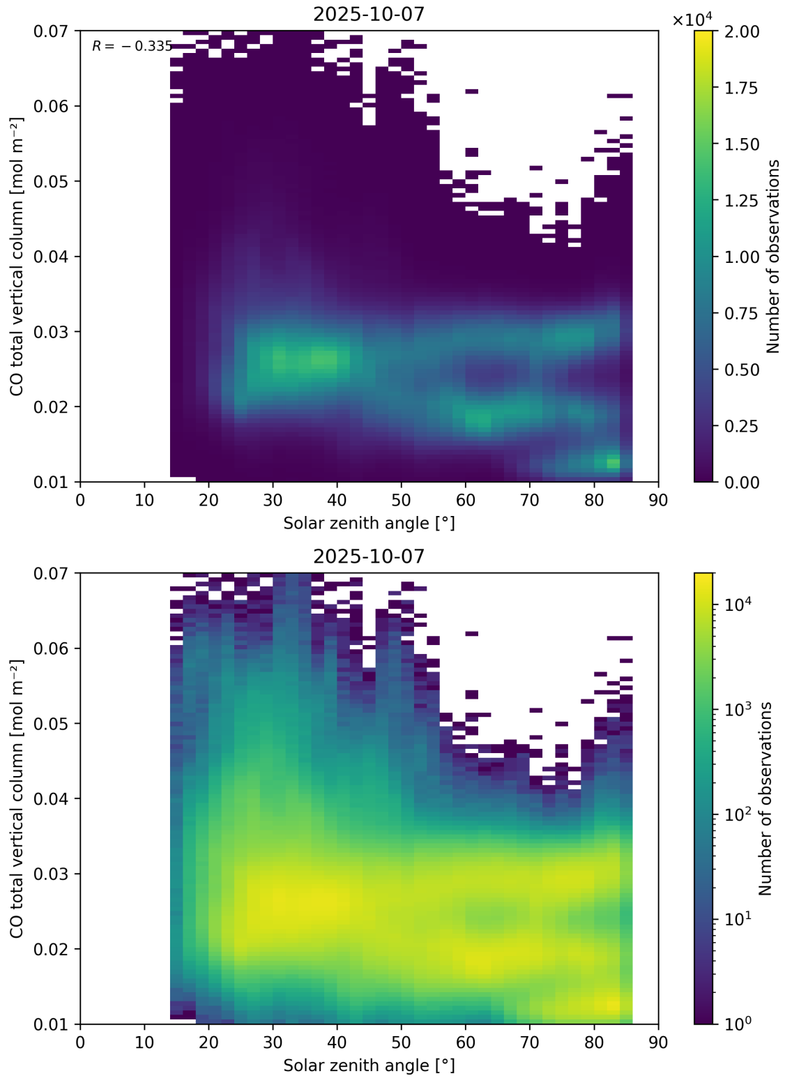
Figure 61: Scatter density plot of “Solar zenith angle” against “CO total vertical column” for 2025-10-06 to 2025-10-08.
