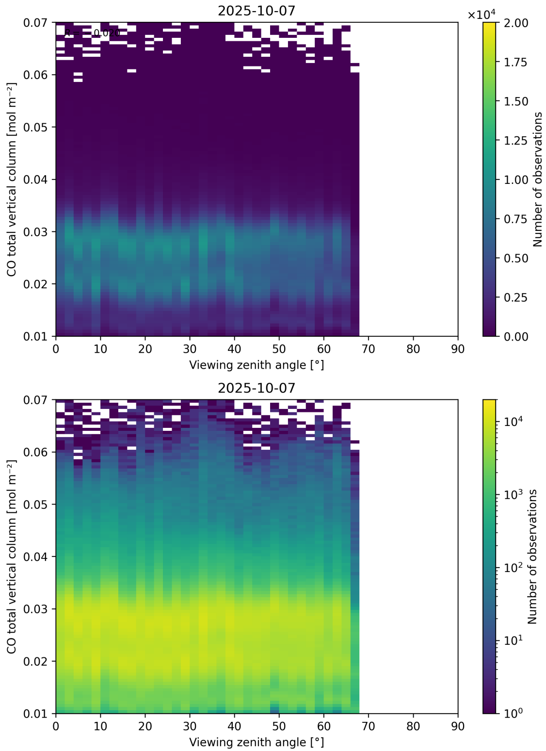
Figure 69: Scatter density plot of “Viewing zenith angle” against “CO total vertical column” for 2025-10-06 to 2025-10-08.
