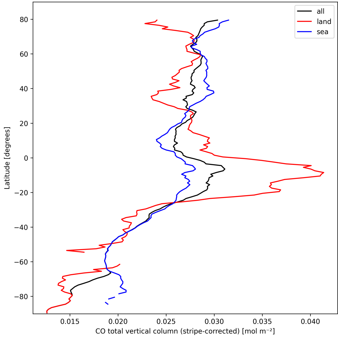
Figure 11: Zonal average of “CO total vertical column (stripe-corrected)” for 2025-10-06 to 2025-10-08.
