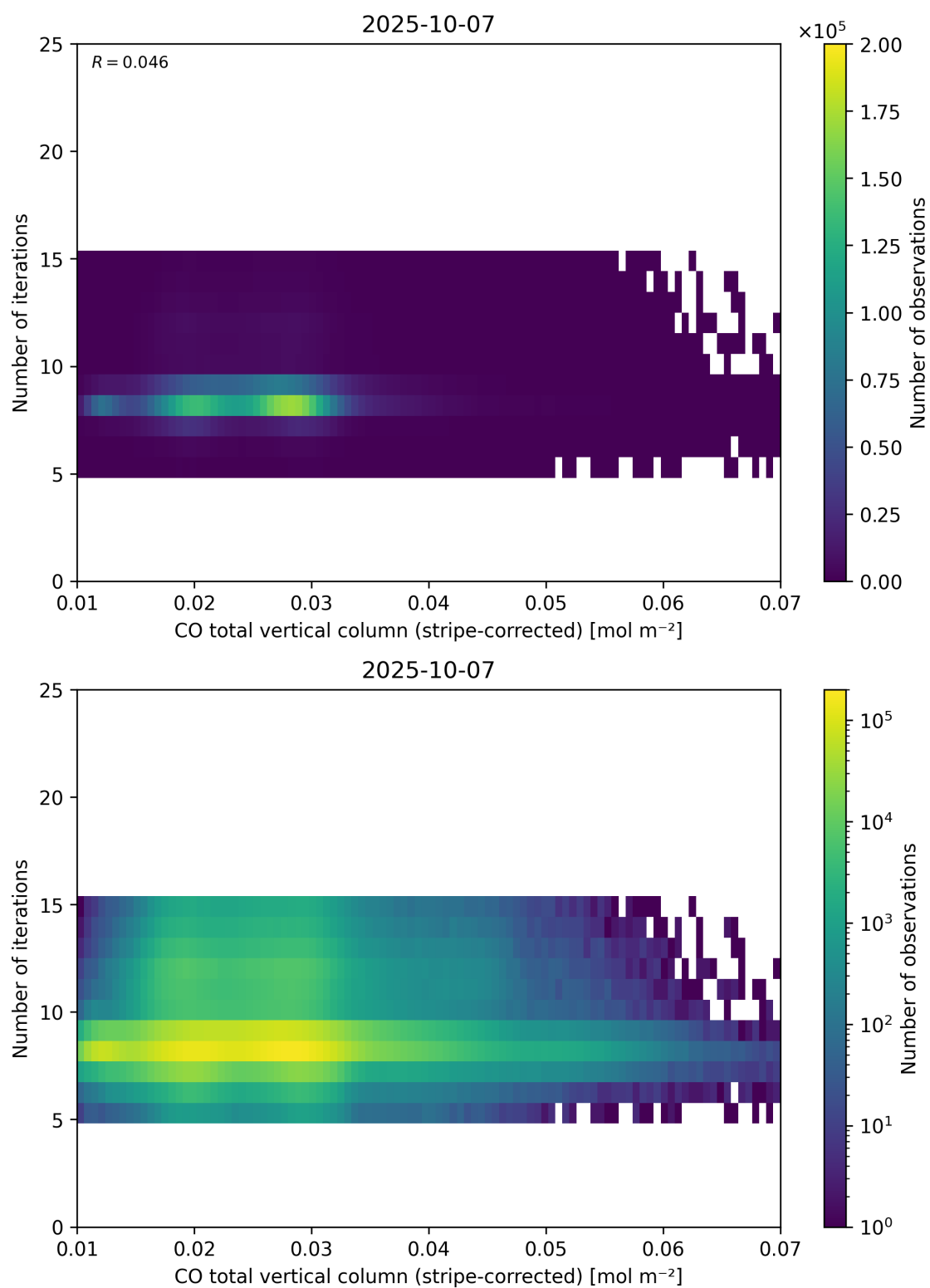
Figure 39: Scatter density plot of “CO total vertical column (stripe-corrected)” against “Number of iterations” for 2025-10-06 to 2025-10-08.
