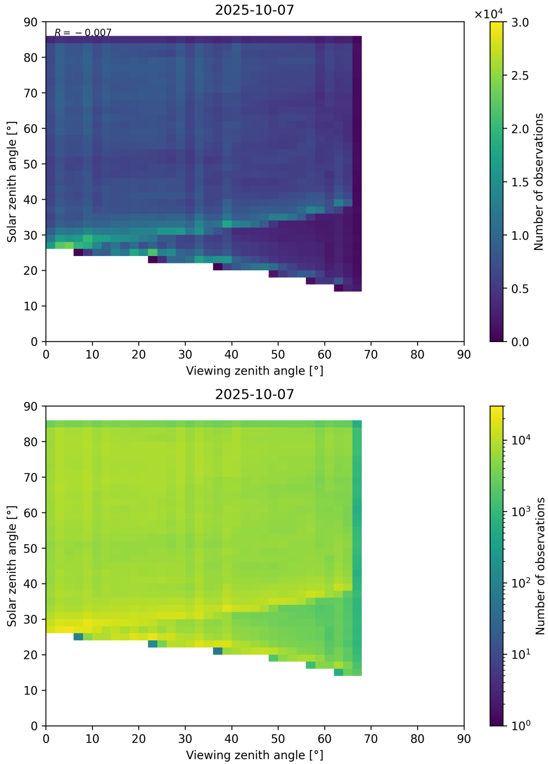
Figure 77: Scatter density plot of “Viewing zenith angle” against “Solar zenith angle” for 2025-10-06 to 2025-10-08.
