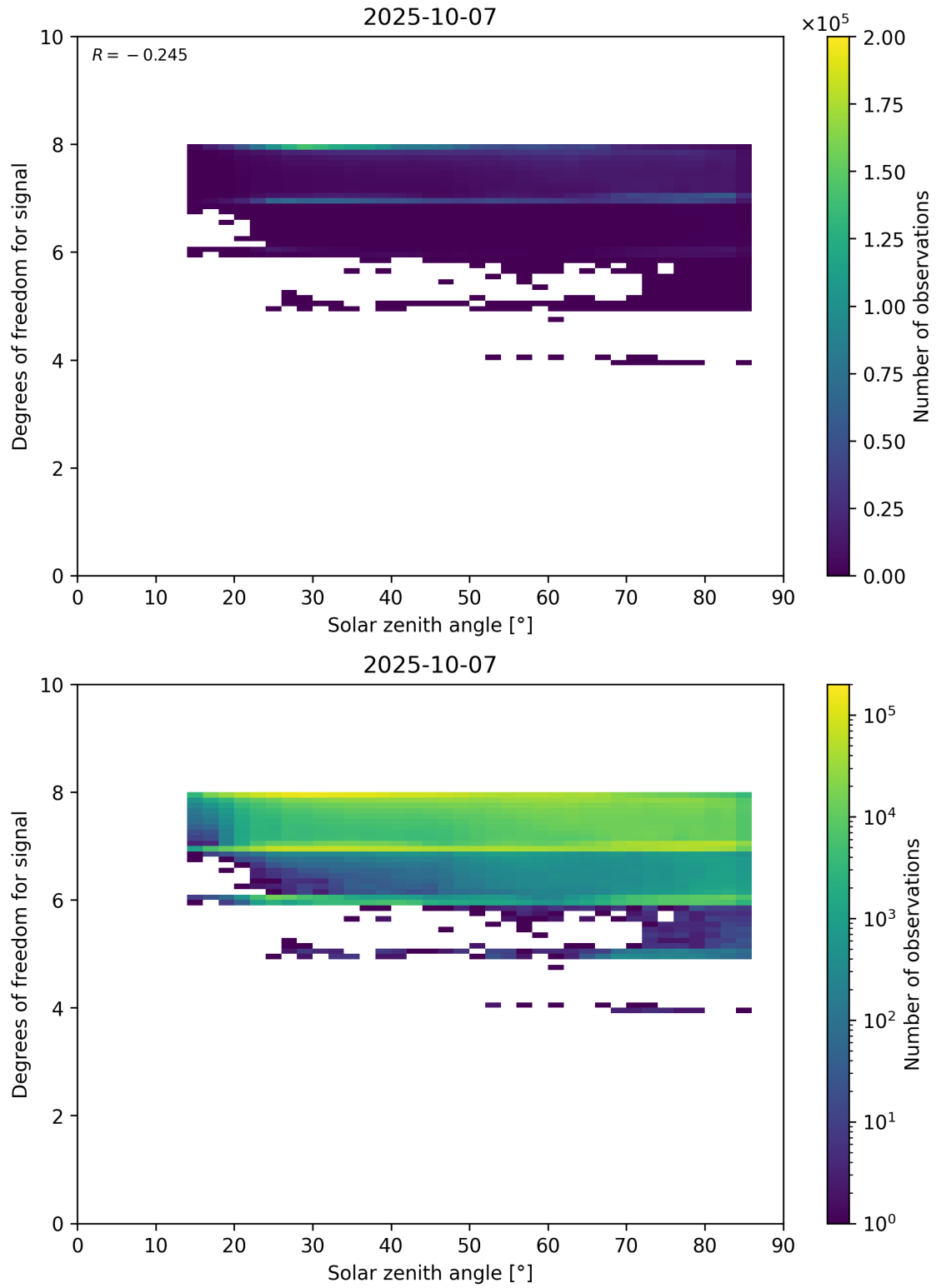
Figure 65: Scatter density plot of “Solar zenith angle” against “Degrees of freedom for signal” for 2025-10-06 to 2025-10-08.
