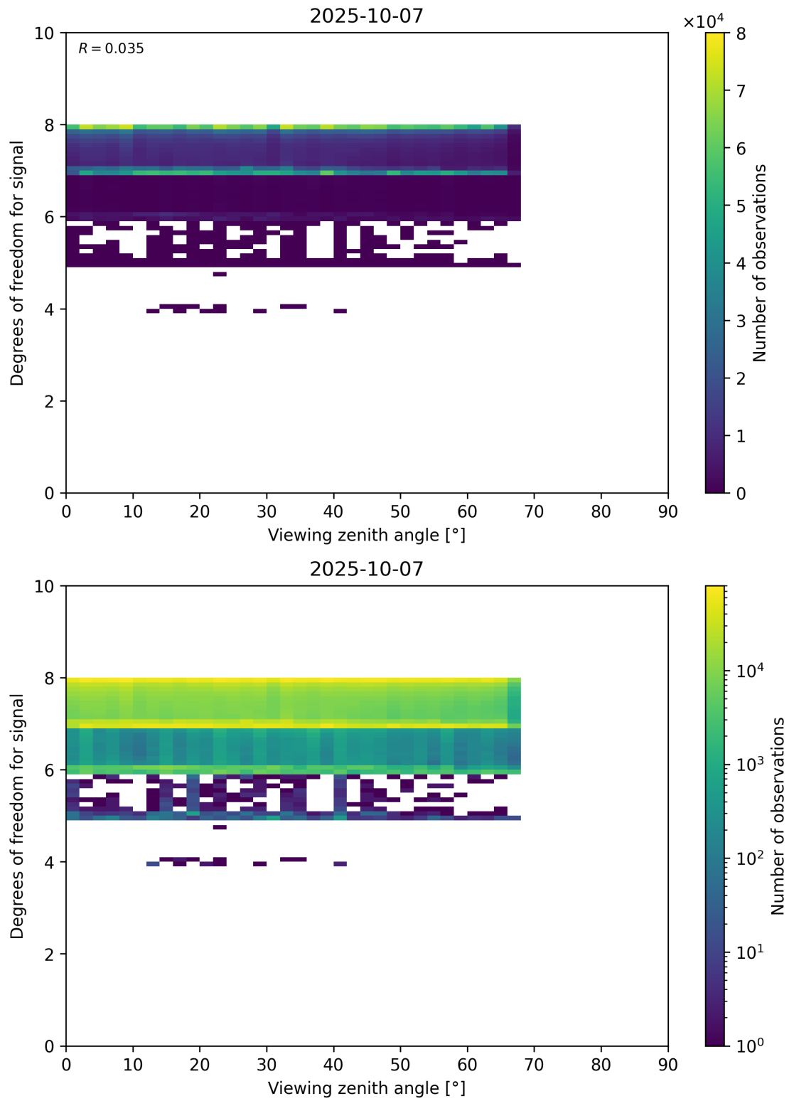
Figure 73: Scatter density plot of “Viewing zenith angle” against “Degrees of freedom for signal” for 2025-10-06 to 2025-10-08.
