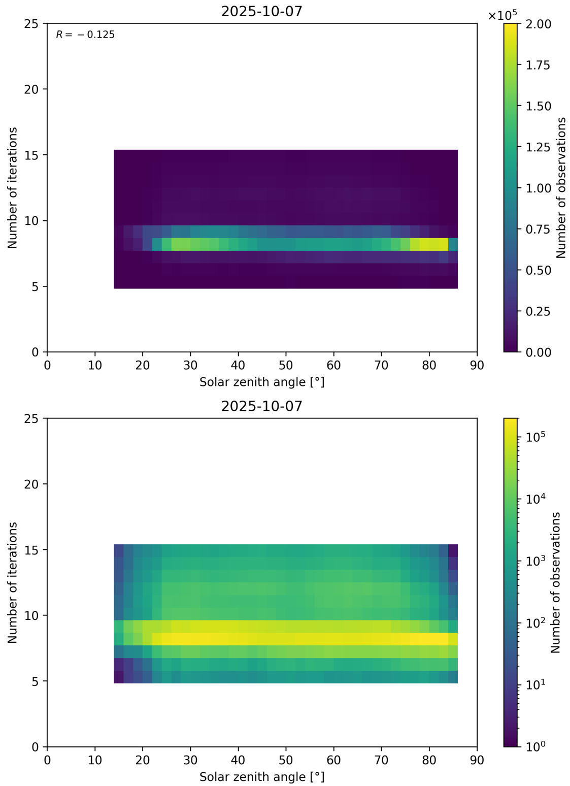
Figure 67: Scatter density plot of “Solar zenith angle” against “Number of iterations” for 2025-10-06 to 2025-10-08.
