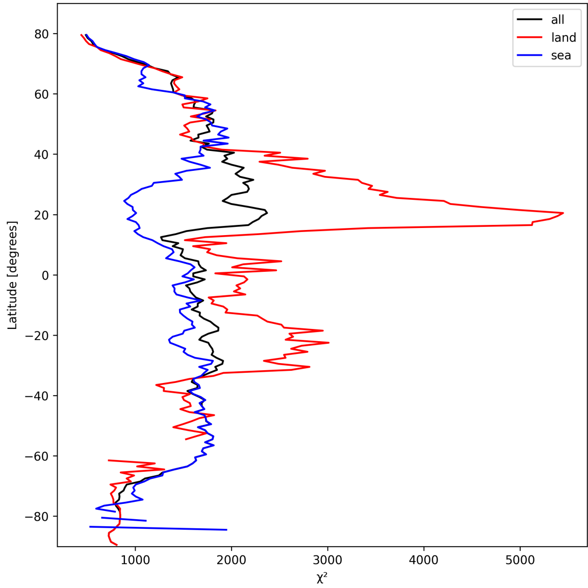
Figure 14: Zonal average of “ \chi^2 ” for 2025-10-06 to 2025-10-08.
