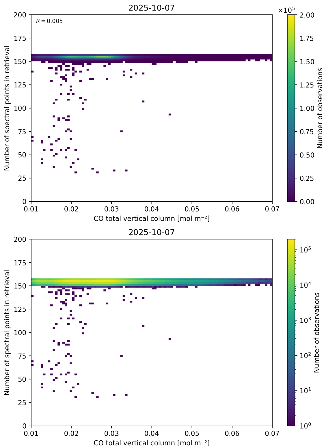
Figure 43: Scatter density plot of “CO total vertical column” against “Number of spectral points in retrieval” for 2025-10-06 to 2025-10-08.
