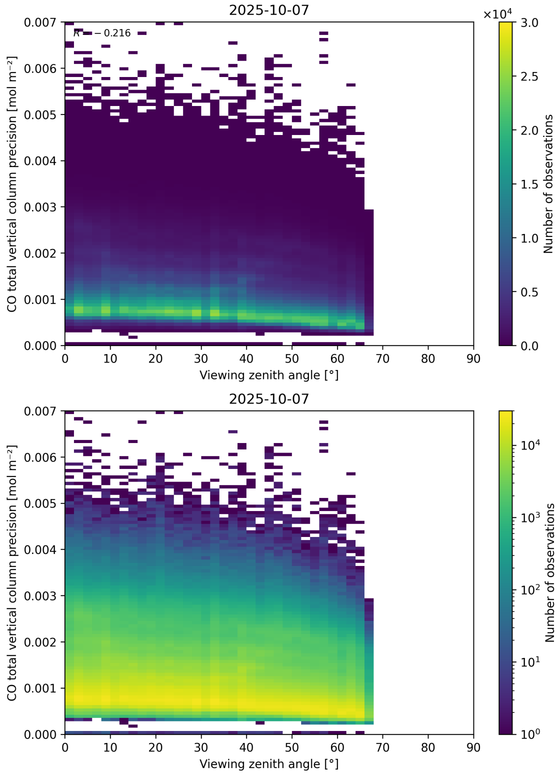
Figure 71: Scatter density plot of “Viewing zenith angle” against “CO total vertical column precision” for 2025-10-06 to 2025-10-08.
