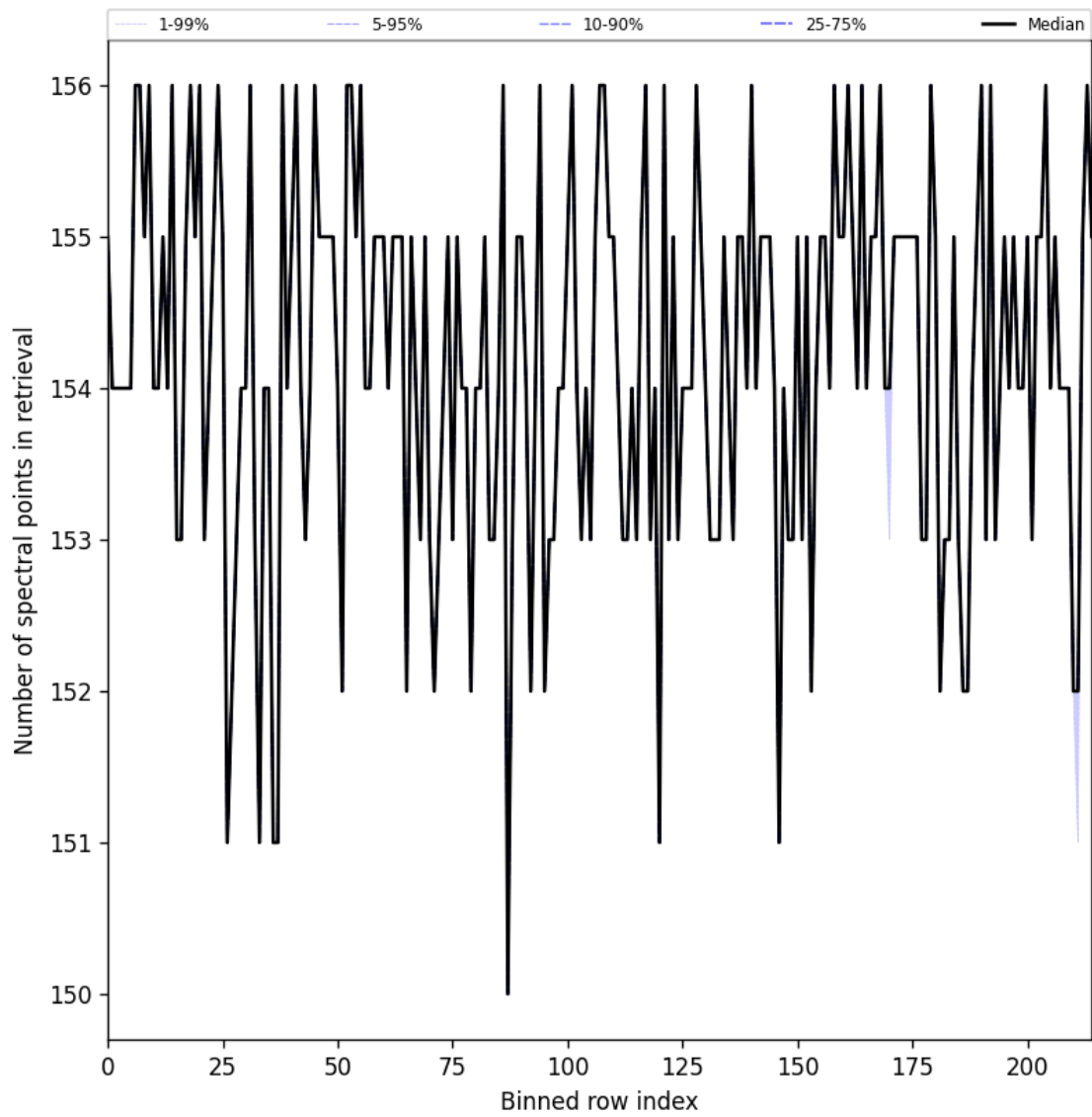
Figure 29: Along track statistics of “Number of spectral points in retrieval” for 2025-10-06 to 2025-10-08
