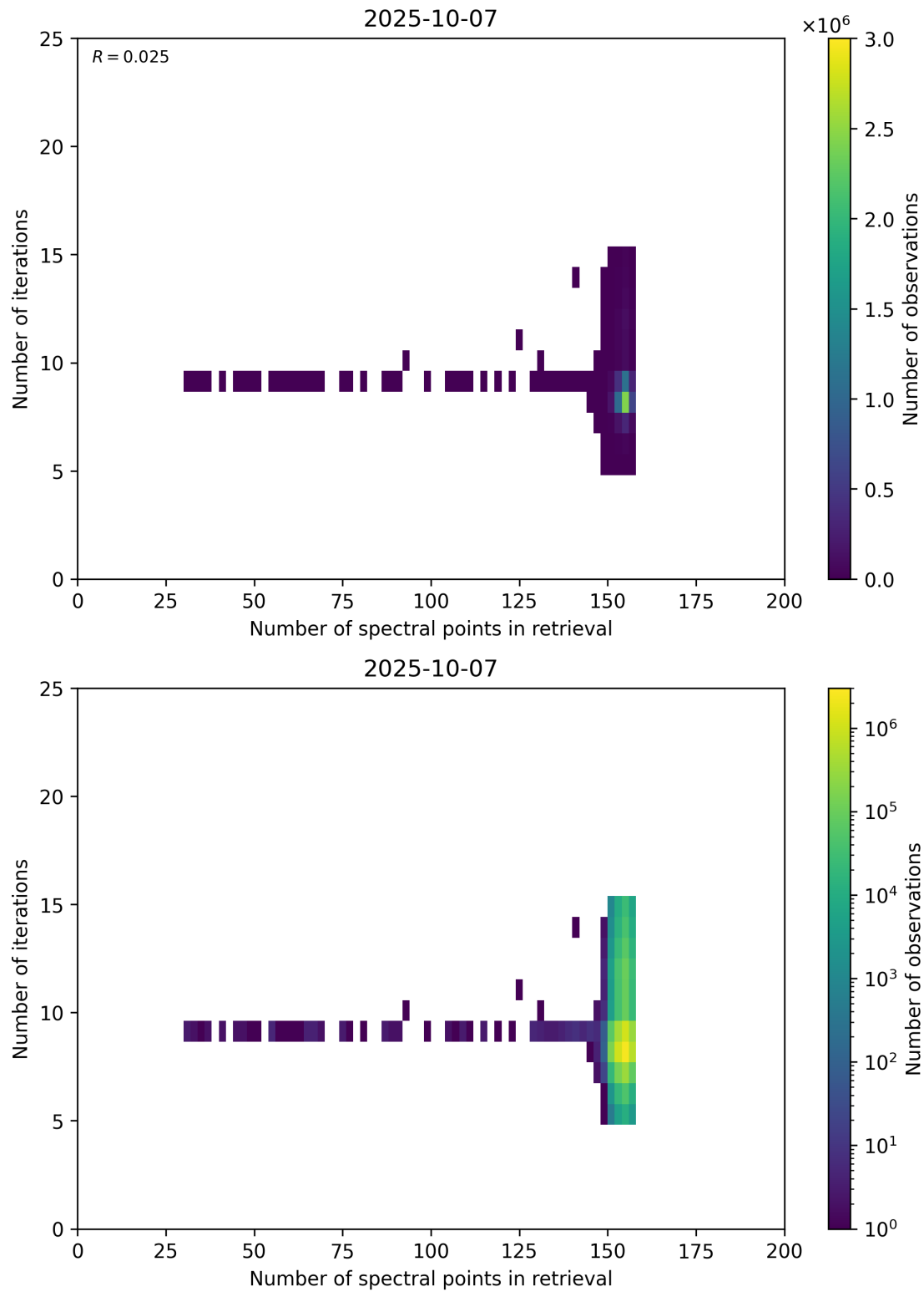
Figure 60: Scatter density plot of “Number of spectral points in retrieval” against “Number of iterations” for 2025-10-06 to 2025-10-08.
