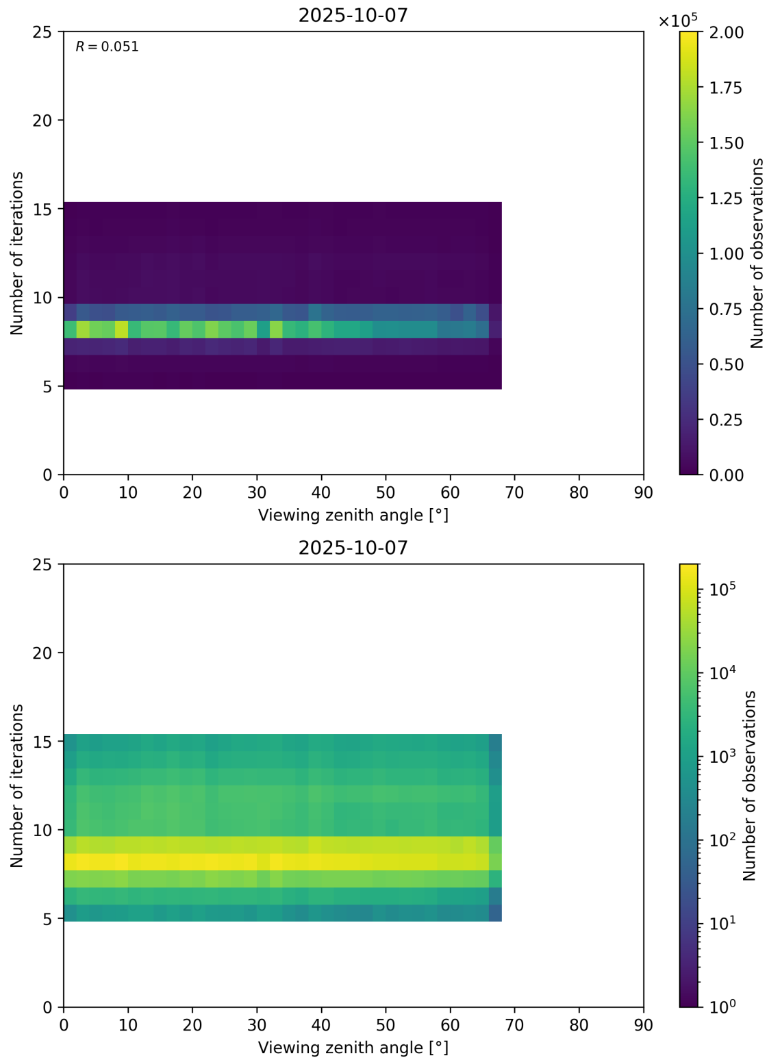
Figure 75: Scatter density plot of “Viewing zenith angle” against “Number of iterations” for 2025-10-06 to 2025-10-08.
