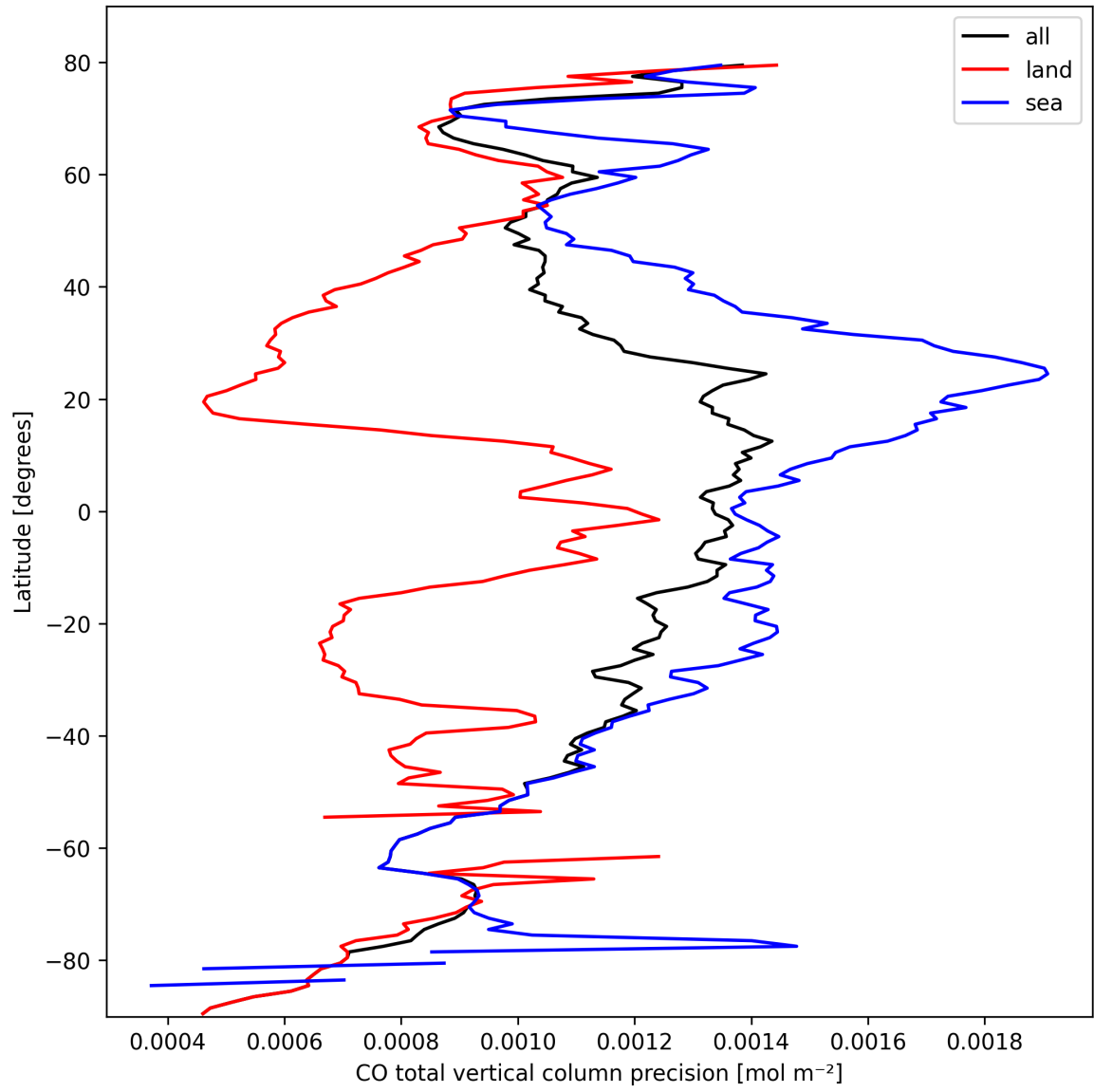
Figure 12: Zonal average of “CO total vertical column precision” for 2025-10-06 to 2025-10-08.
