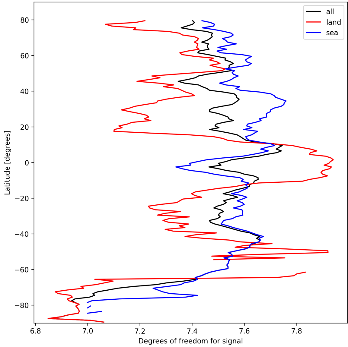
Figure 15: Zonal average of “Degrees of freedom for signal” for 2025-10-06 to 2025-10-08.
