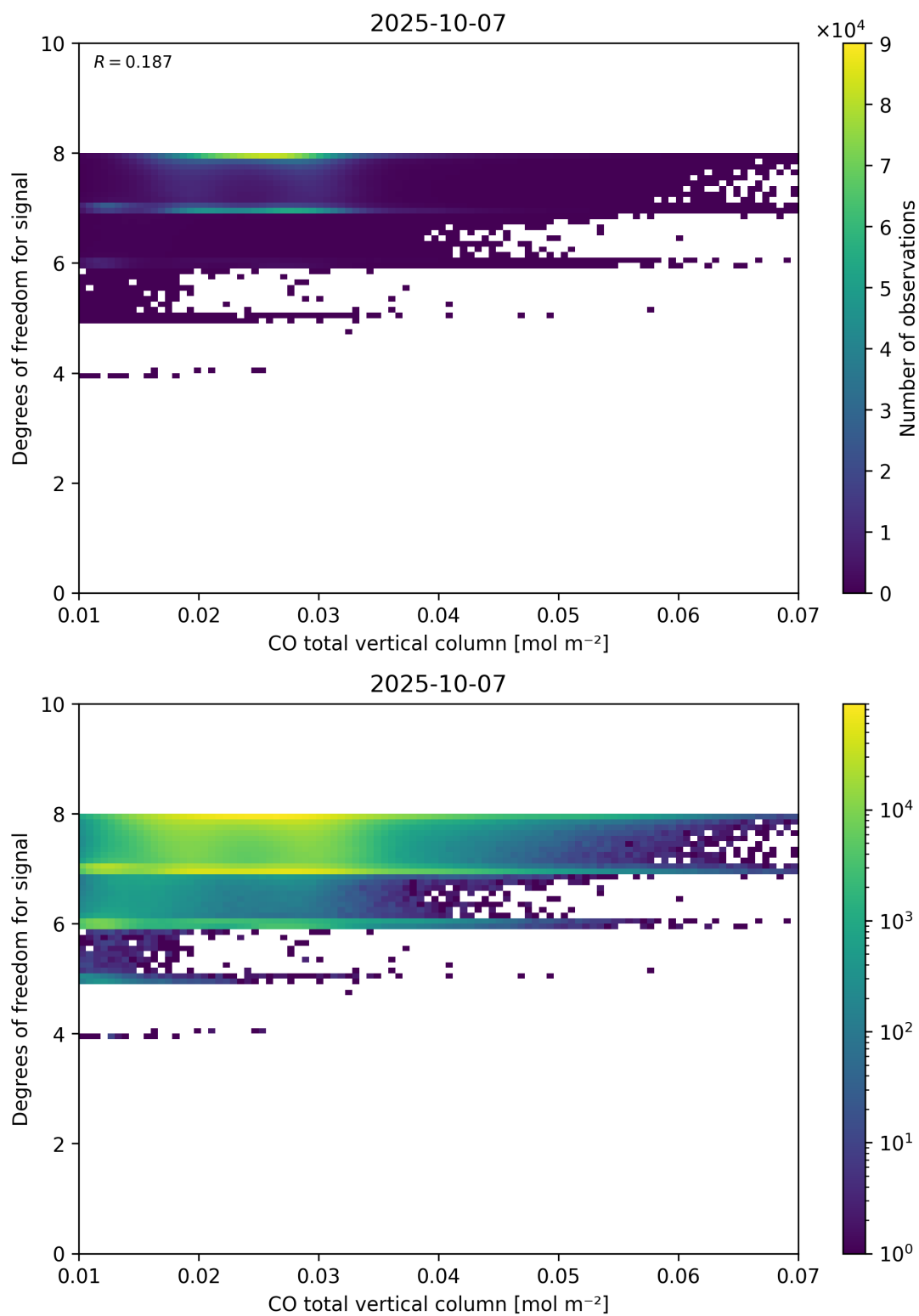
Figure 41: Scatter density plot of “CO total vertical column” against “Degrees of freedom for signal” for 2025-10-06 to 2025-10-08.
