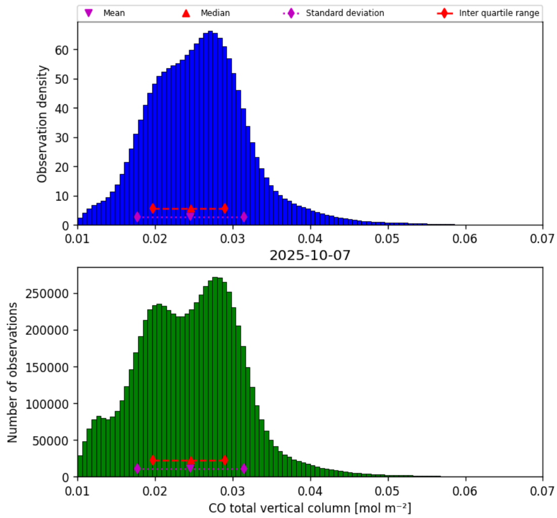
Figure 18: Histogram of “CO total vertical column” for 2025-10-06 to 2025-10-08
