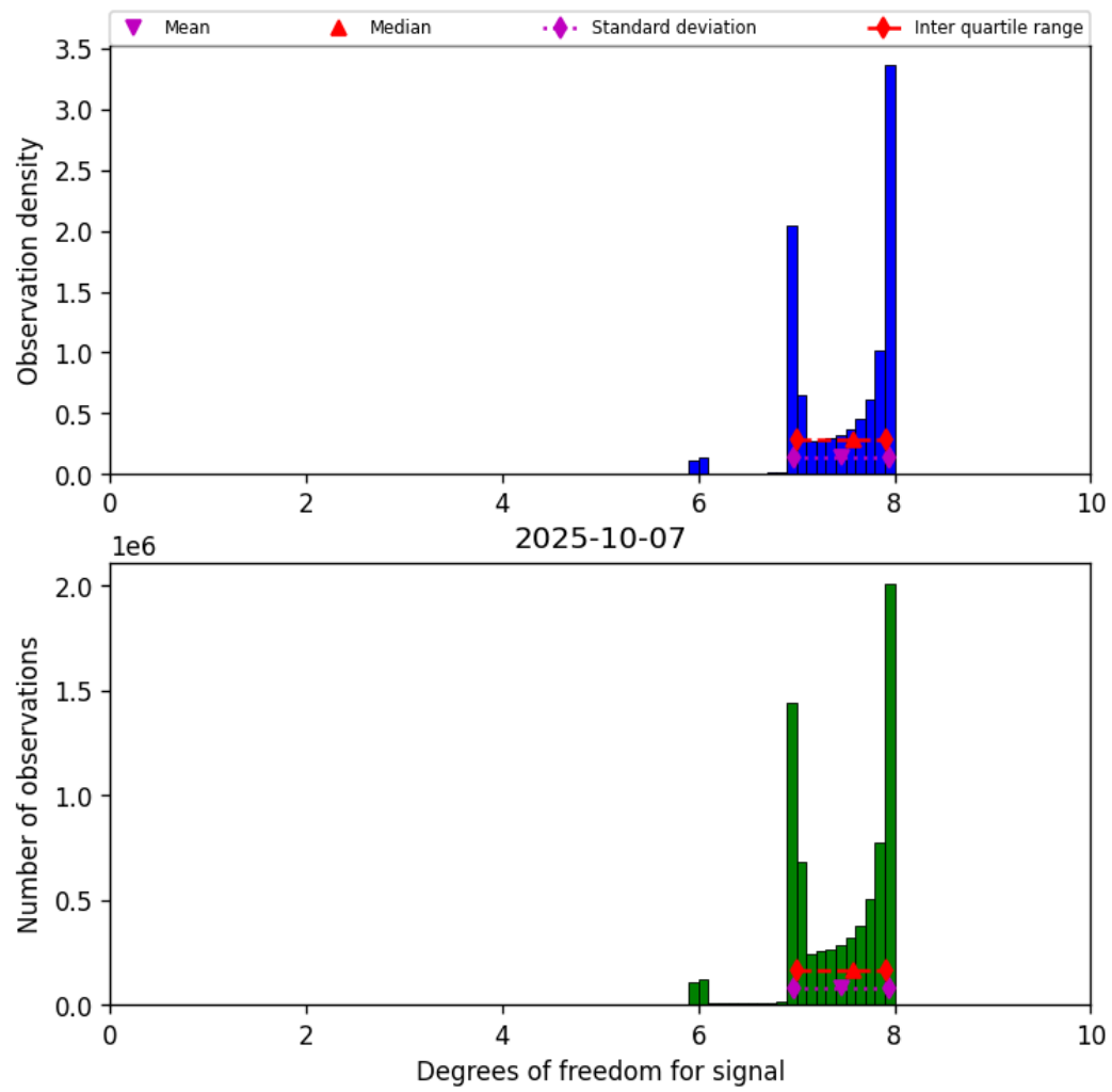
Figure 23: Histogram of “Degrees of freedom for signal” for 2025-10-06 to 2025-10-08
