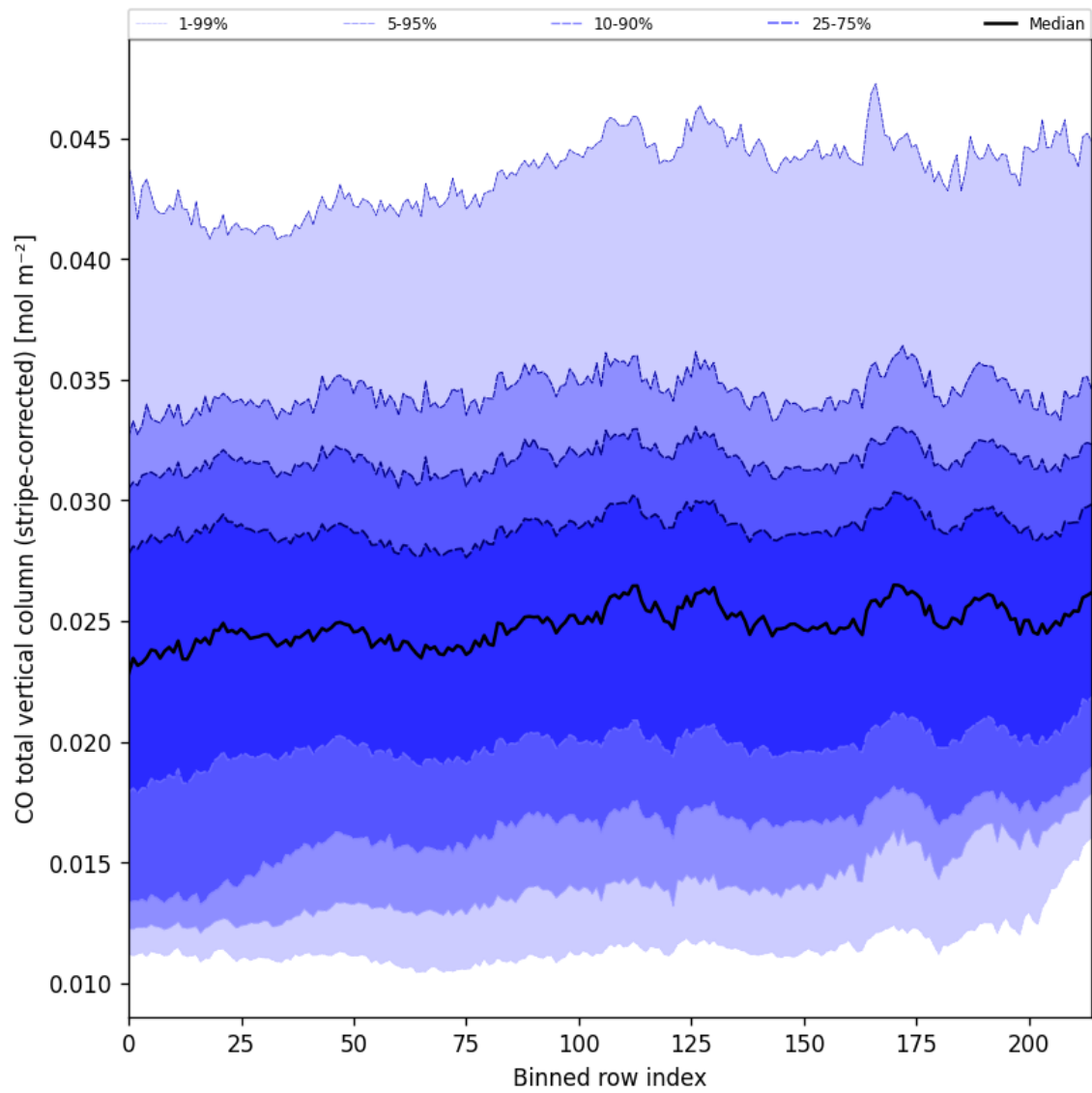
Figure 27: Along track statistics of “CO total vertical column (stripe-corrected)” for 2025-10-06 to 2025-10-08
