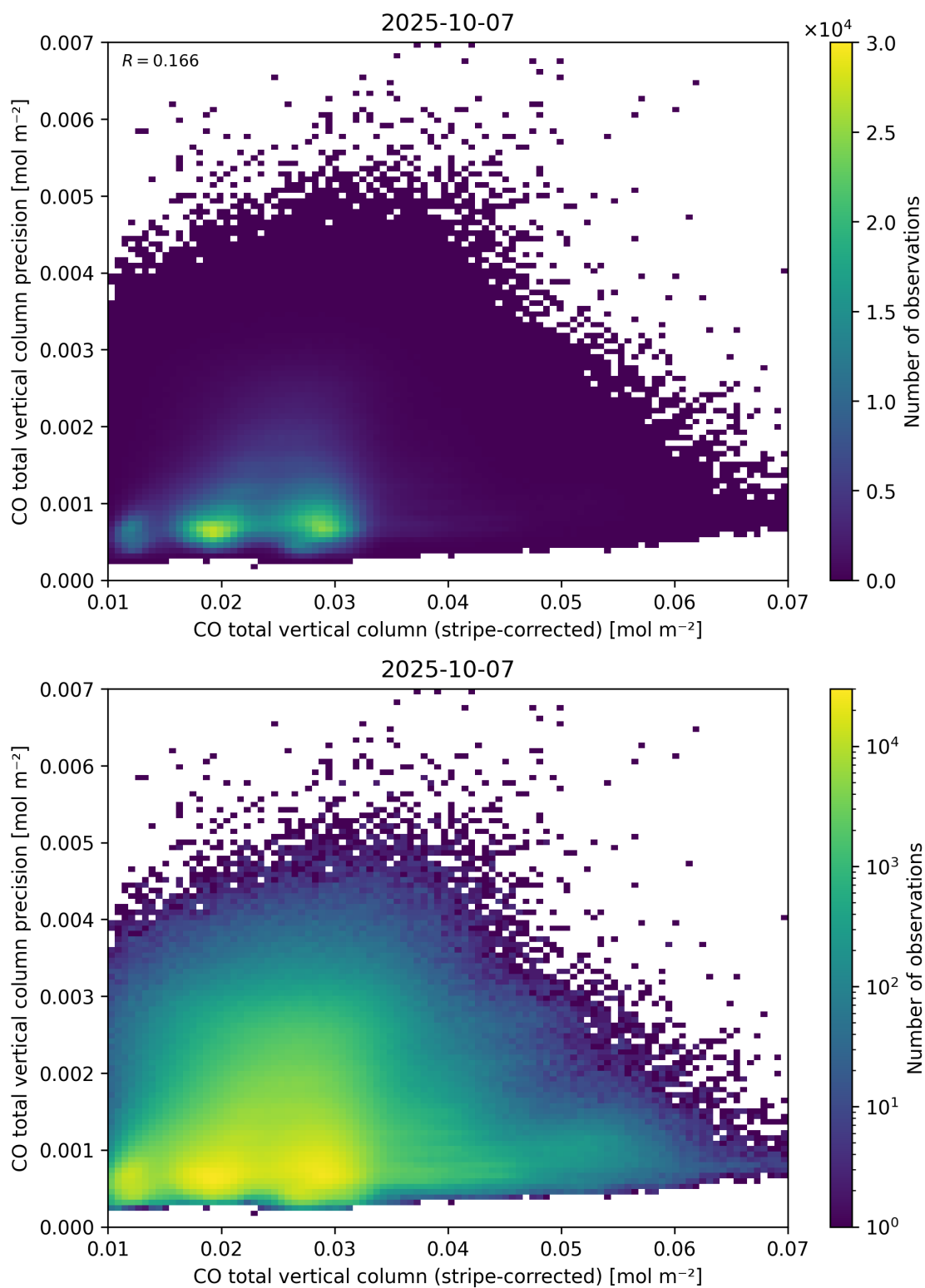
Figure 36: Scatter density plot of “CO total vertical column (stripe-corrected)” against “CO total vertical column precision” for 2025-10-06 to 2025-10-08.
