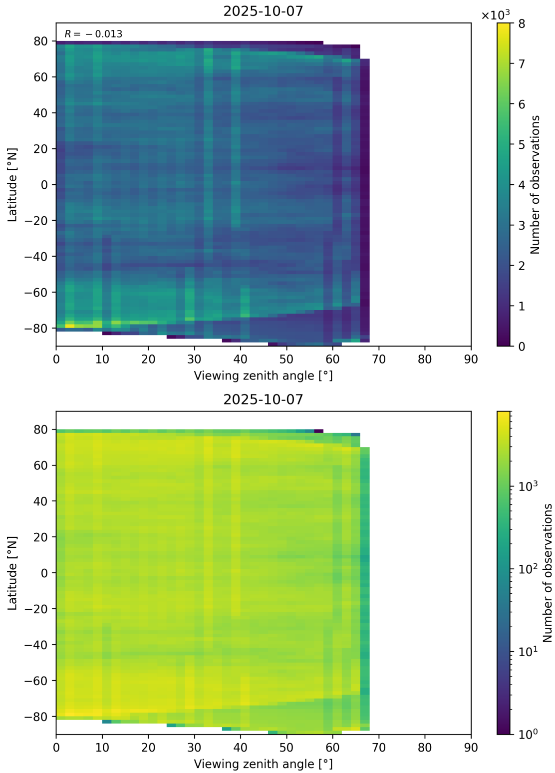
Figure 74: Scatter density plot of “Viewing zenith angle” against “Latitude” for 2025-10-06 to 2025-10-08.
