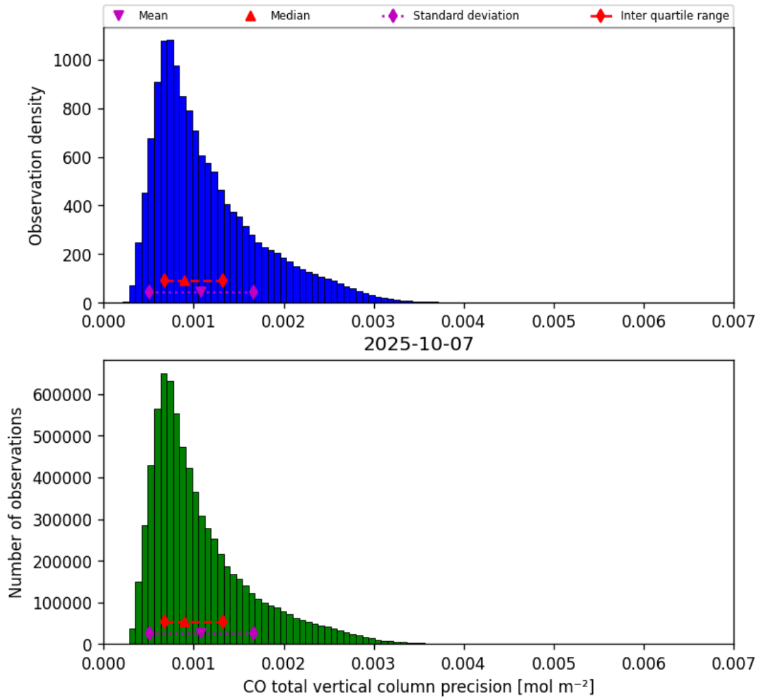
Figure 20: Histogram of “CO total vertical column precision” for 2025-10-06 to 2025-10-08
