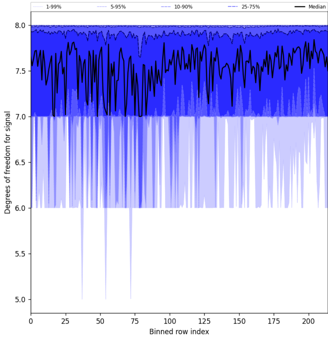
Figure 31: Along track statistics of “Degrees of freedom for signal” for 2025-10-06 to 2025-10-08
