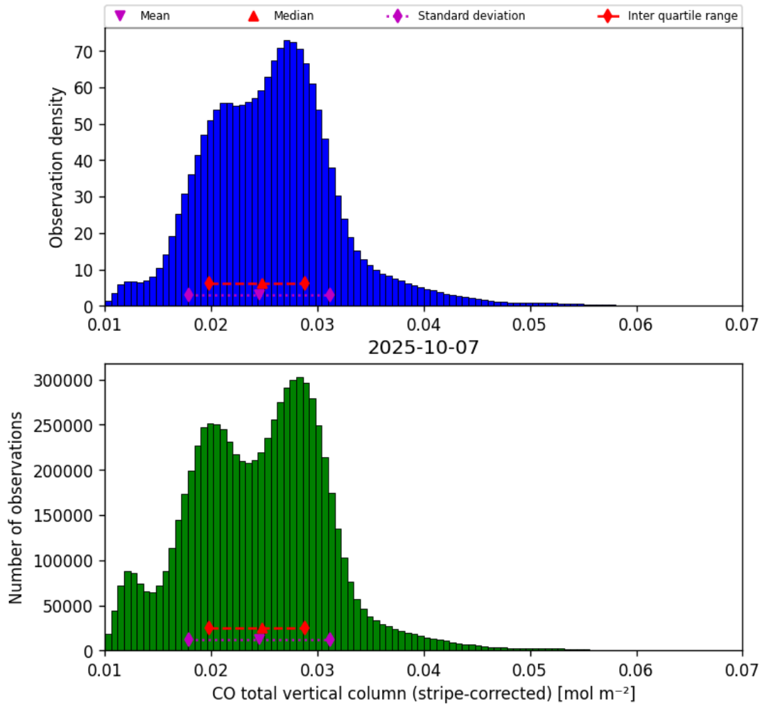
Figure 19: Histogram of “CO total vertical column (stripe-corrected)” for 2025-10-06 to 2025-10-08
