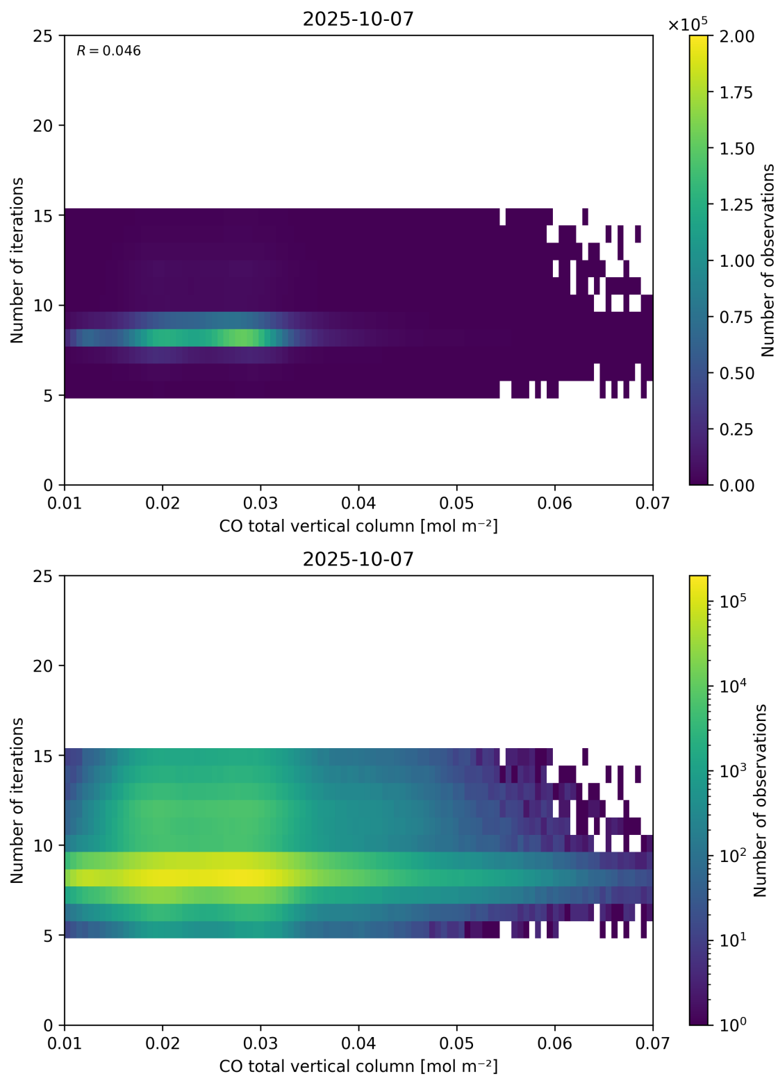
Figure 42: Scatter density plot of “CO total vertical column” against “Number of iterations” for 2025-10-06 to 2025-10-08.
