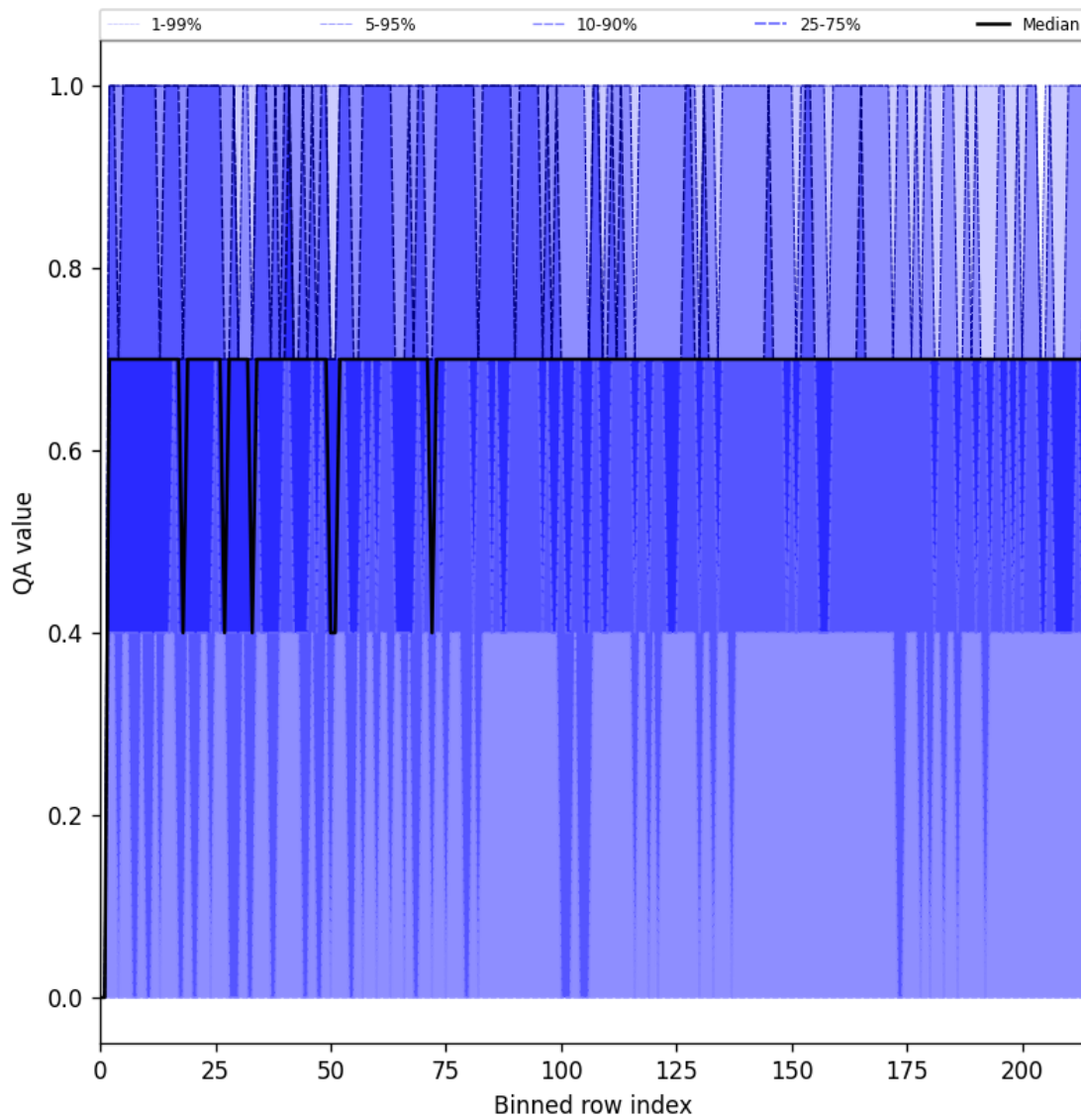
Figure 25: Along track statistics of “QA value” for 2025-10-06 to 2025-10-08
