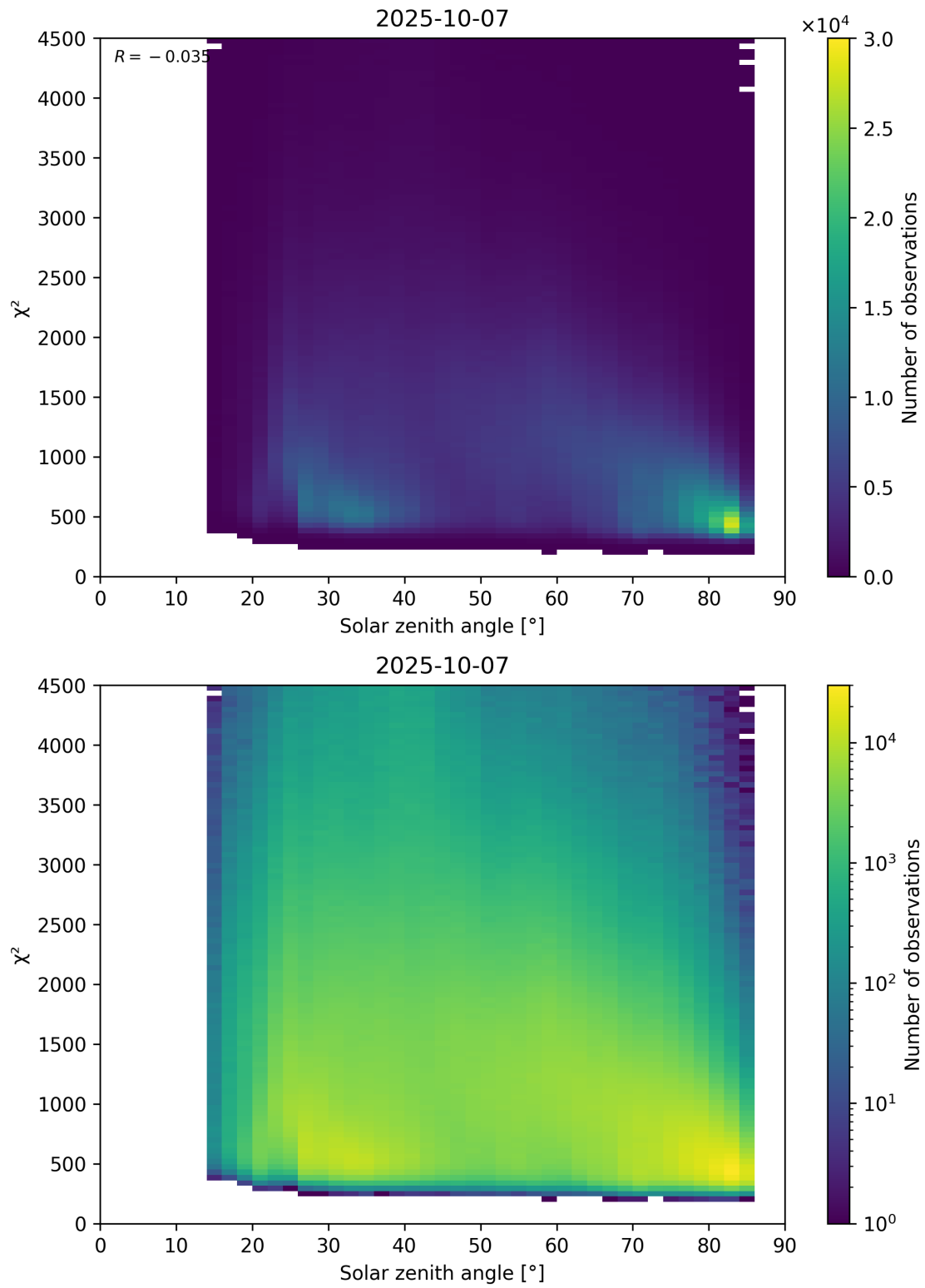
Figure 64: Scatter density plot of “Solar zenith angle” against “ \chi^2 ” for 2025-10-06 to 2025-10-08.
