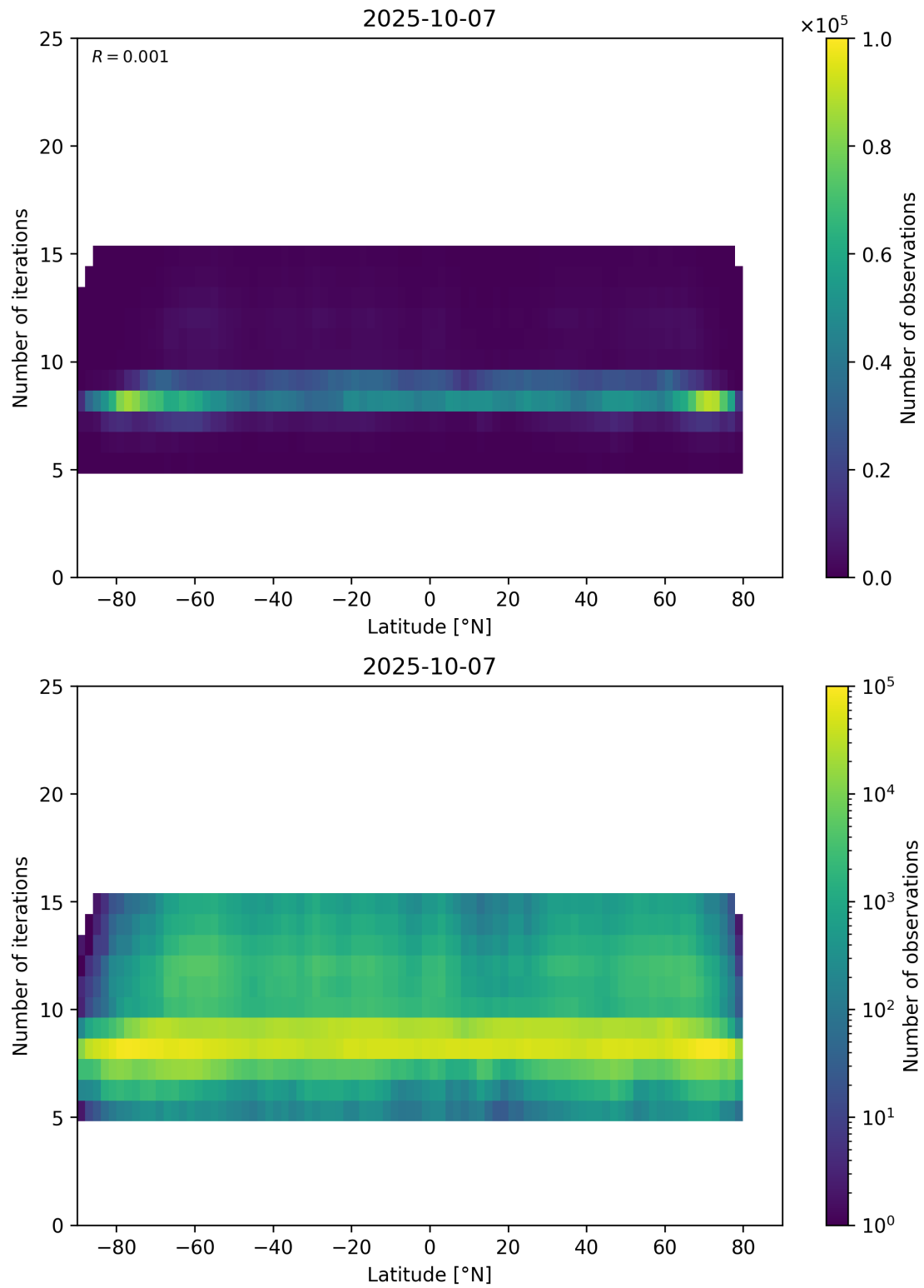
Figure 56: Scatter density plot of “Latitude” against “Number of iterations” for 2025-10-06 to 2025-10-08.
