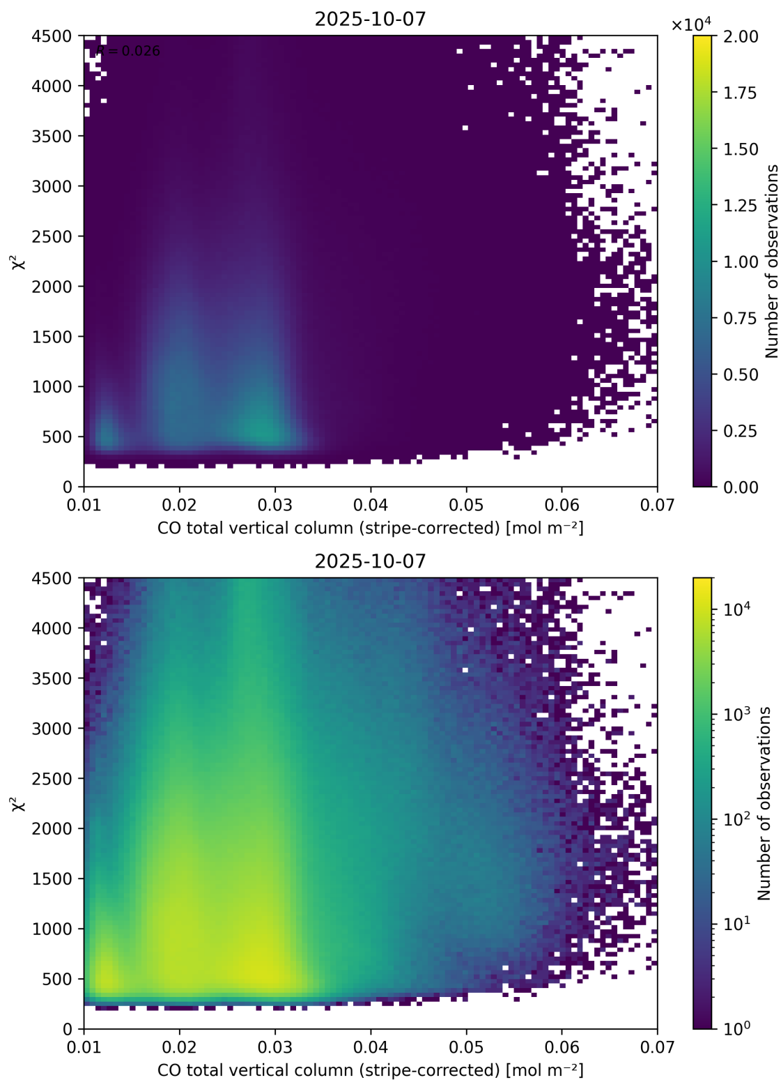
Figure 37: Scatter density plot of “CO total vertical column (stripe-corrected)” against “ \chi^2 ” for 2025-10-06 to 2025-10-08.
