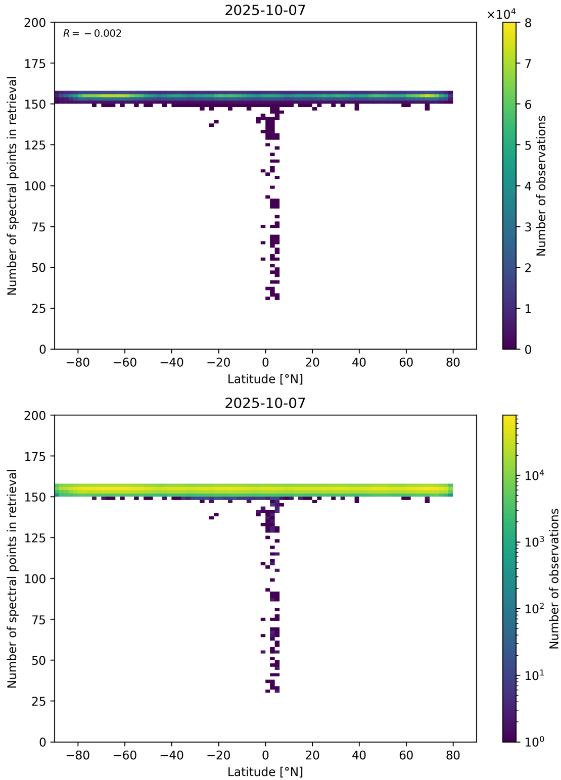
Figure 57: Scatter density plot of “Latitude” against “Number of spectral points in retrieval” for 2025-10-06 to 2025-10-08.
