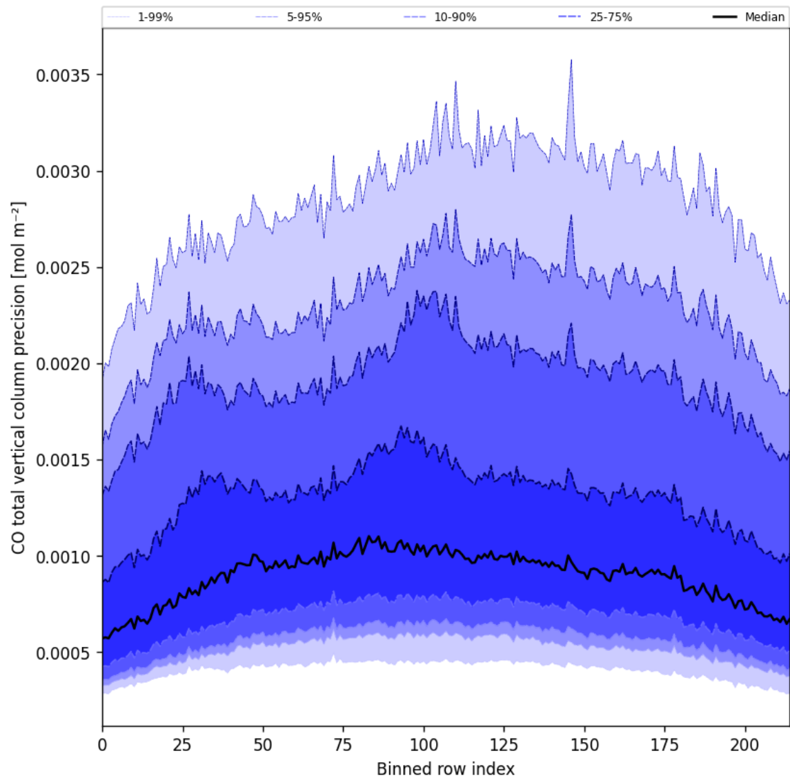
Figure 28: Along track statistics of “CO total vertical column precision” for 2025-10-06 to 2025-10-08
