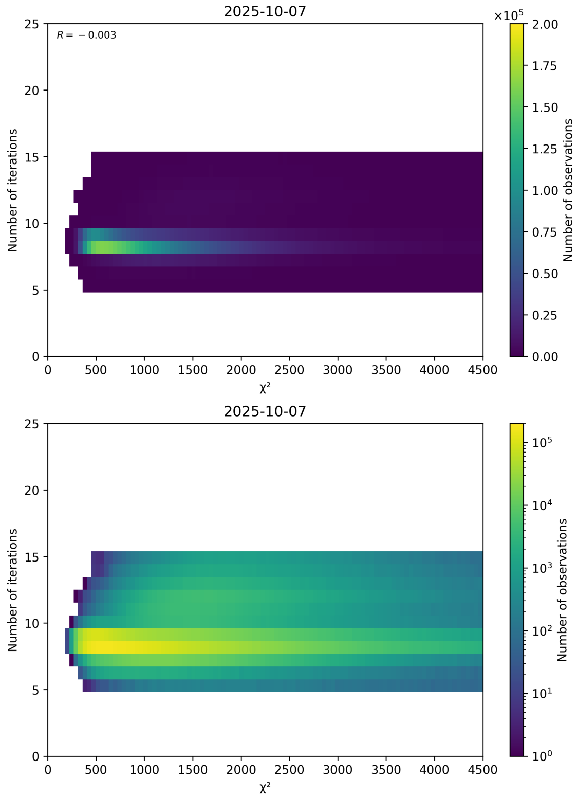
Figure 49: Scatter density plot of “ \chi^2 ” against “Number of iterations” for 2025-10-06 to 2025-10-08.
