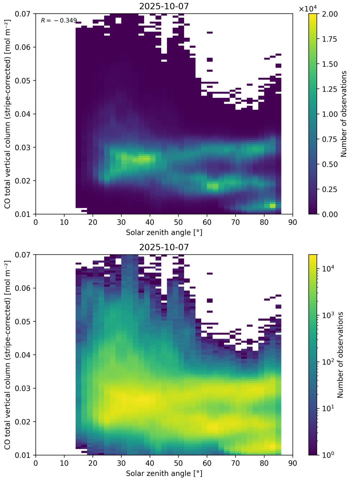
Figure 62: Scatter density plot of “Solar zenith angle” against “CO total vertical column (stripe-corrected)” for 2025-10-06 to 2025-10-08.
