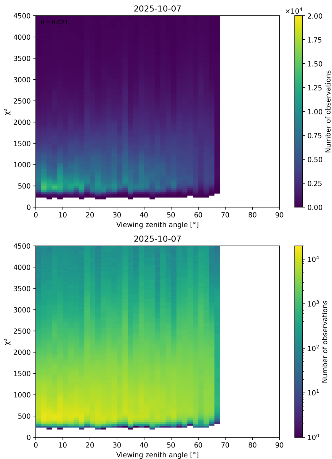
Figure 72: Scatter density plot of “Viewing zenith angle” against “ \chi^2 ” for 2025-10-06 to 2025-10-08.
