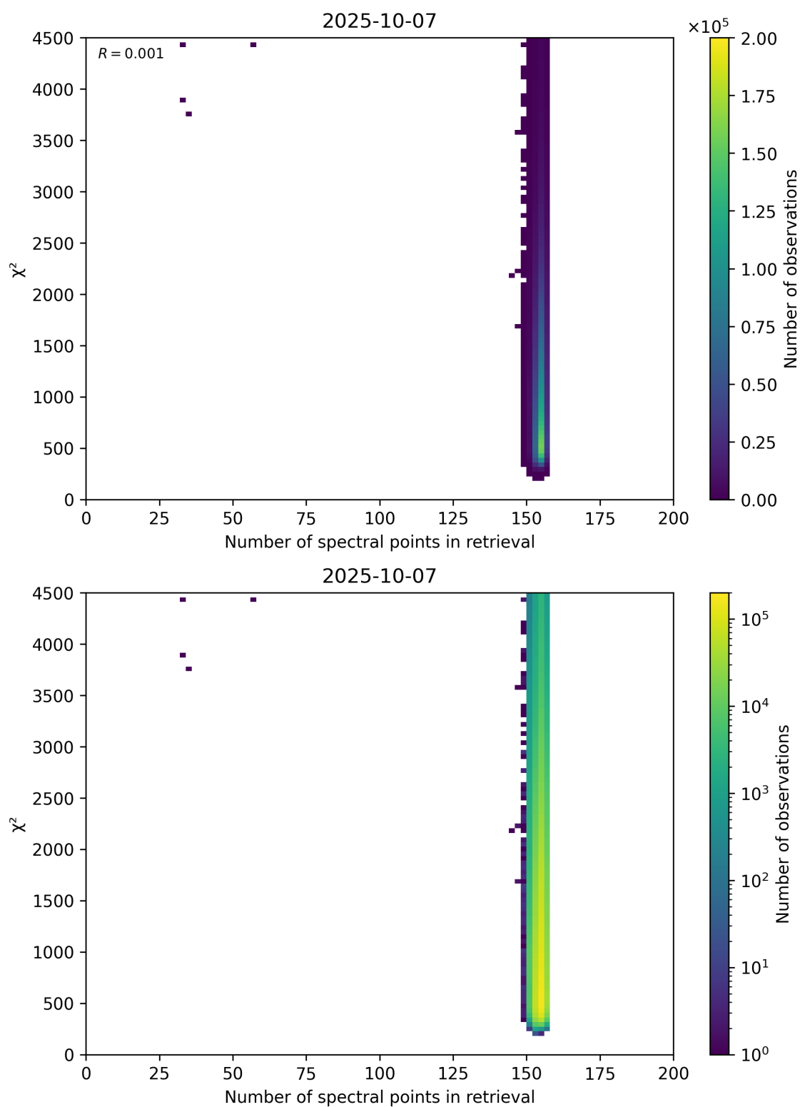
Figure 58: Scatter density plot of “Number of spectral points in retrieval” against “ \chi^2 ” for 2025-10-06 to 2025-10-08.
