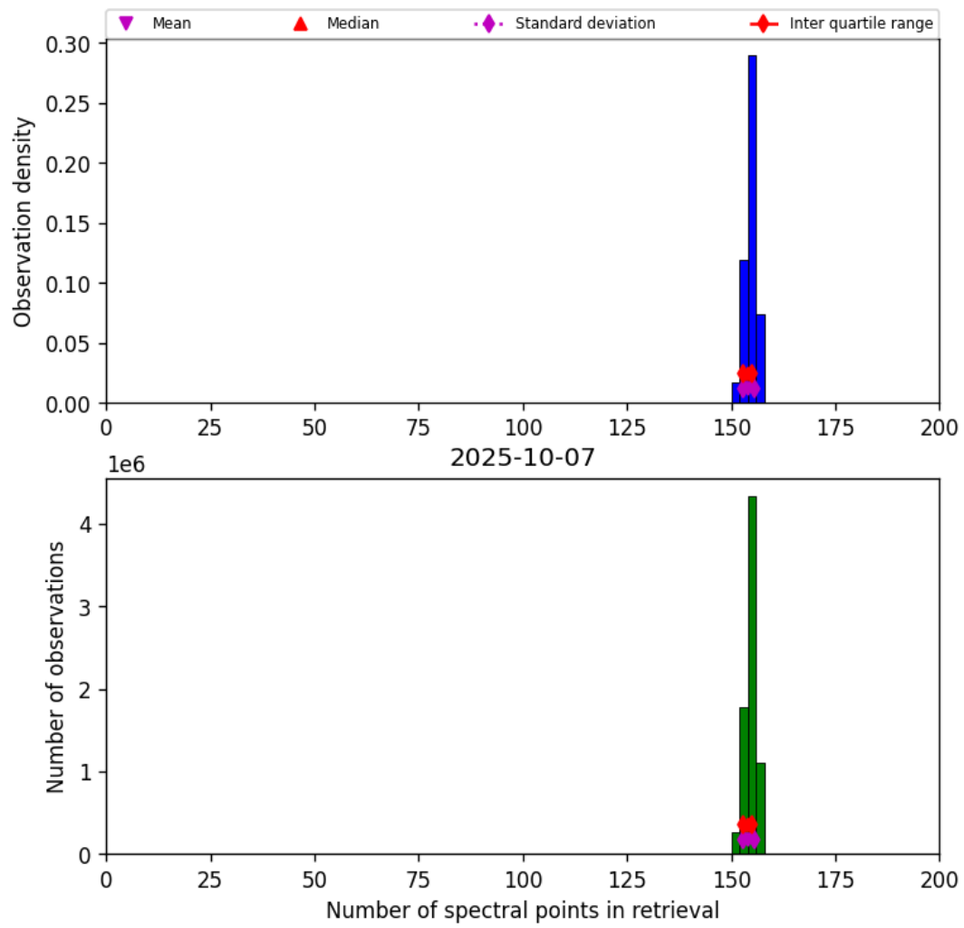
Figure 21: Histogram of “Number of spectral points in retrieval” for 2025-10-06 to 2025-10-08
