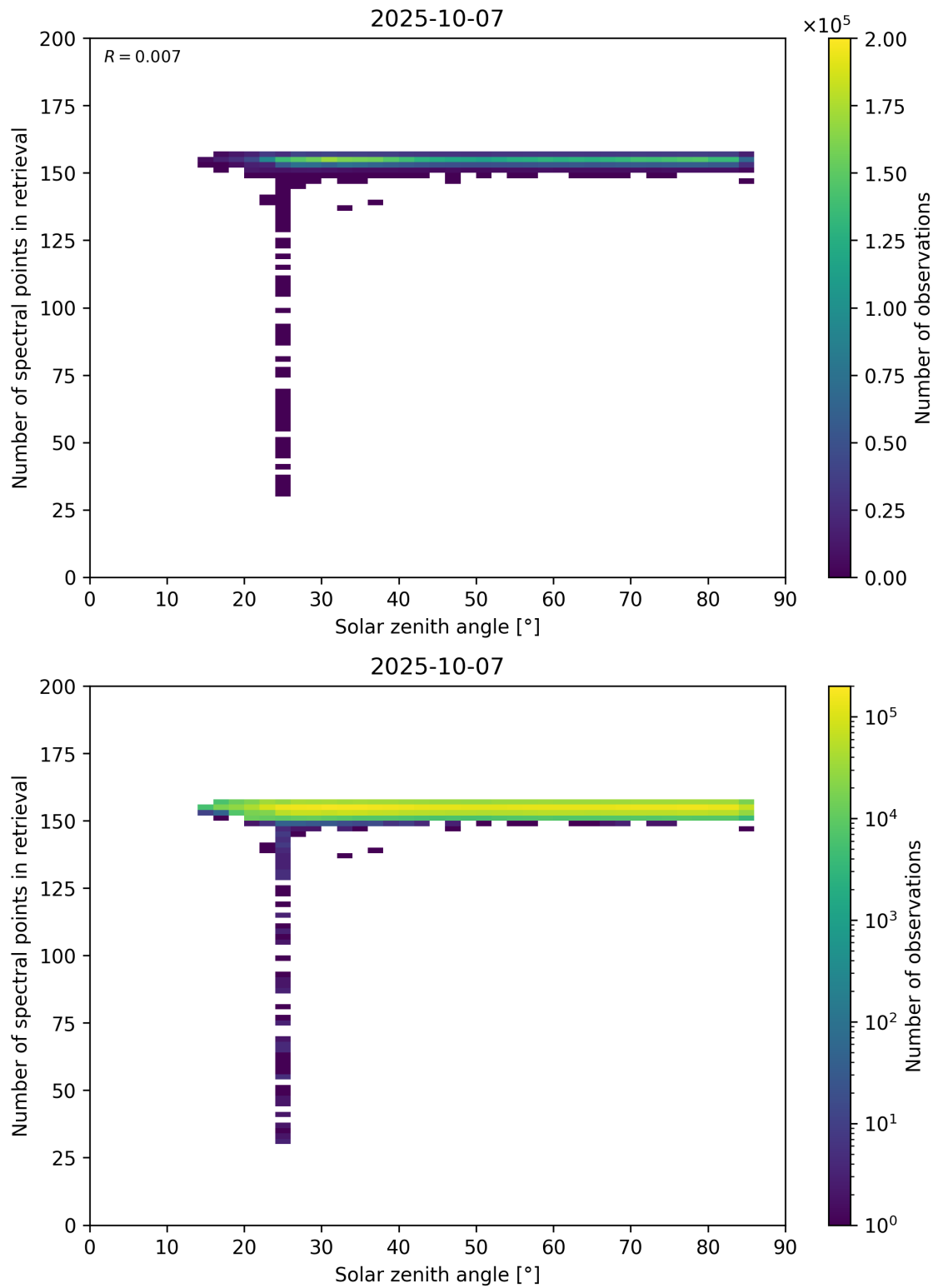
Figure 68: Scatter density plot of “Solar zenith angle” against “Number of spectral points in retrieval” for 2025-10-06 to 2025-10-08.
