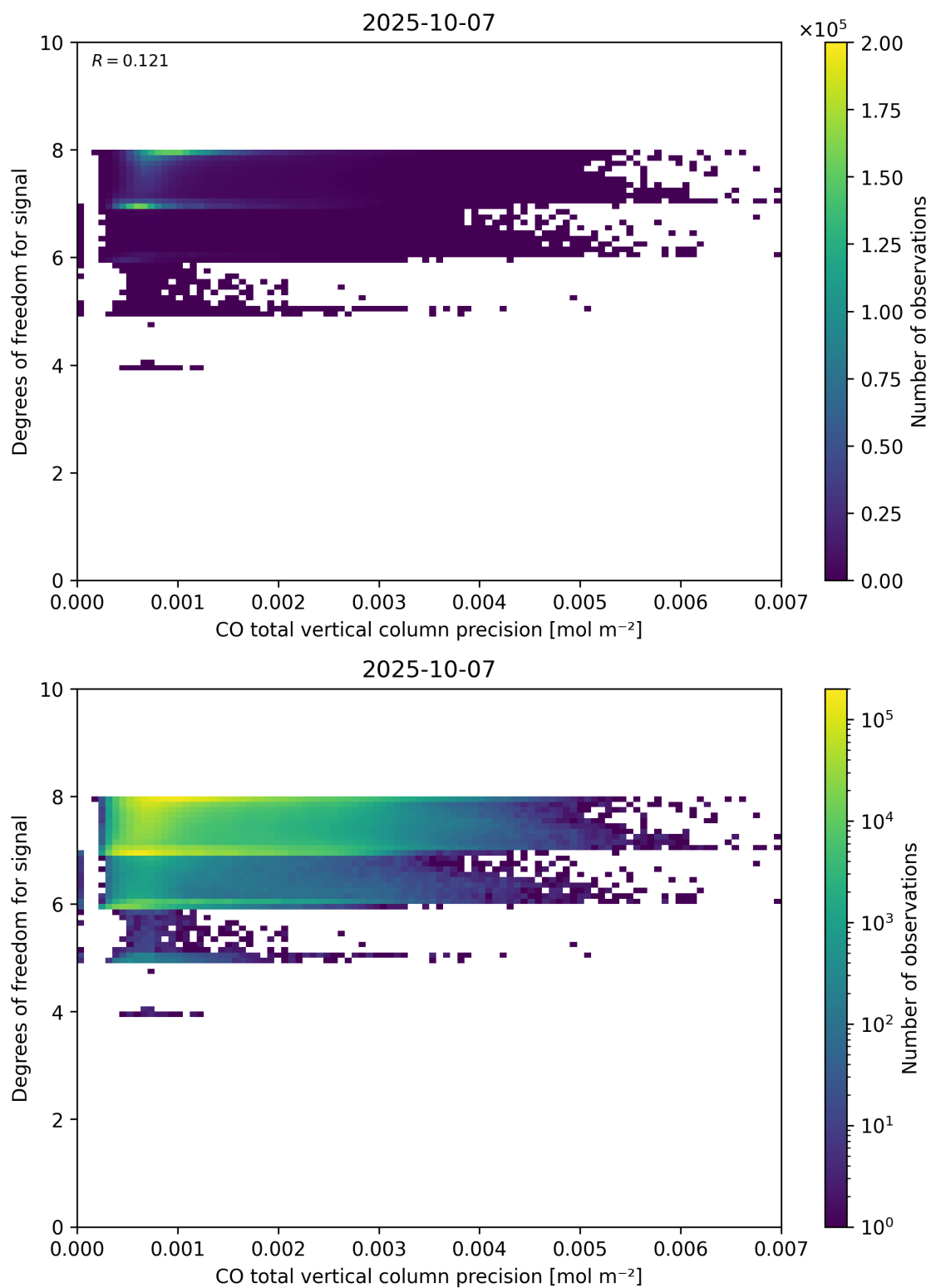
Figure 45: Scatter density plot of “CO total vertical column precision” against “Degrees of freedom for signal” for 2025-10-06 to 2025-10-08.
