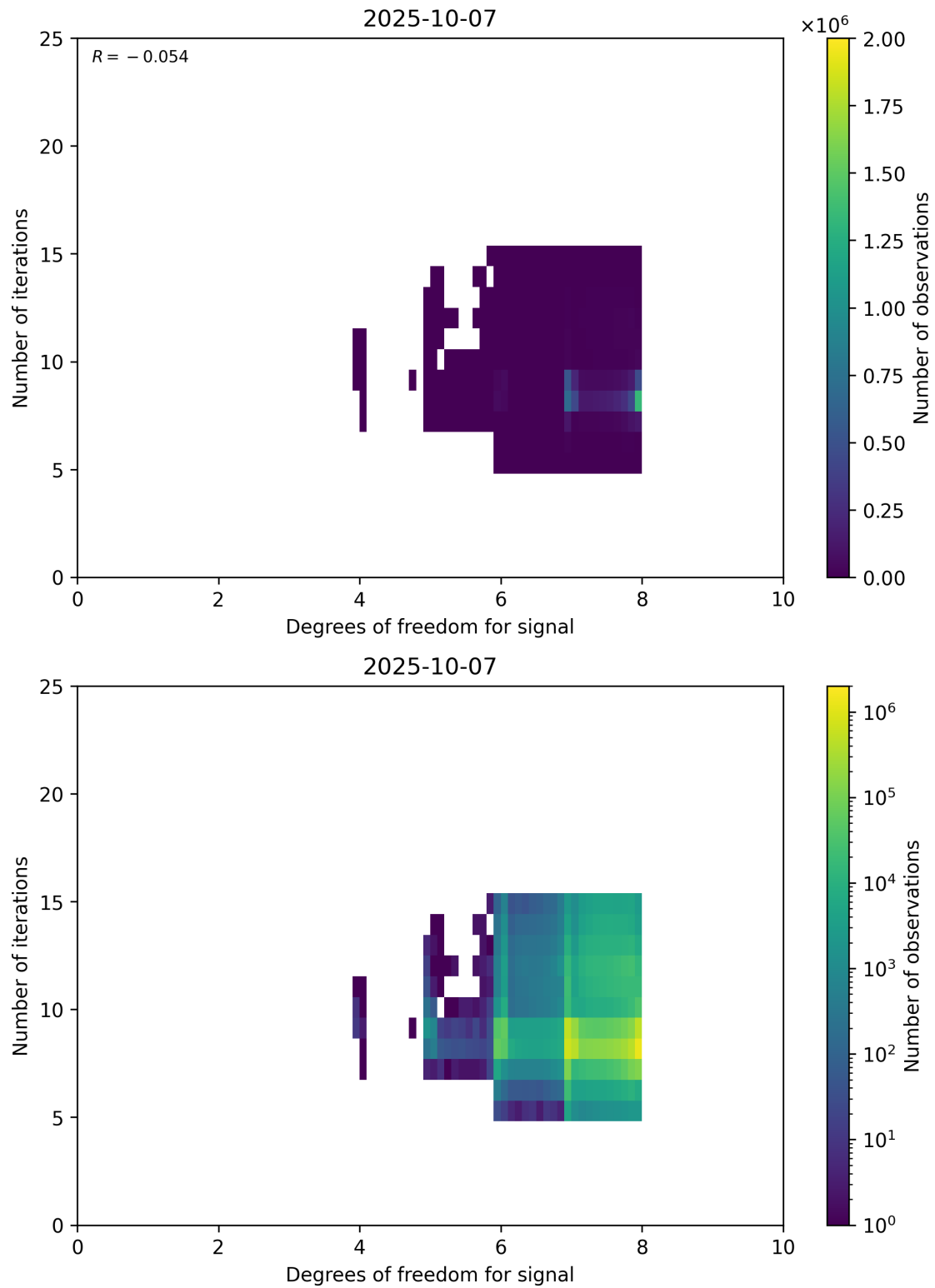
Figure 50: Scatter density plot of “Degrees of freedom for signal” against “Number of iterations” for 2025-10-06 to 2025-10-08.
