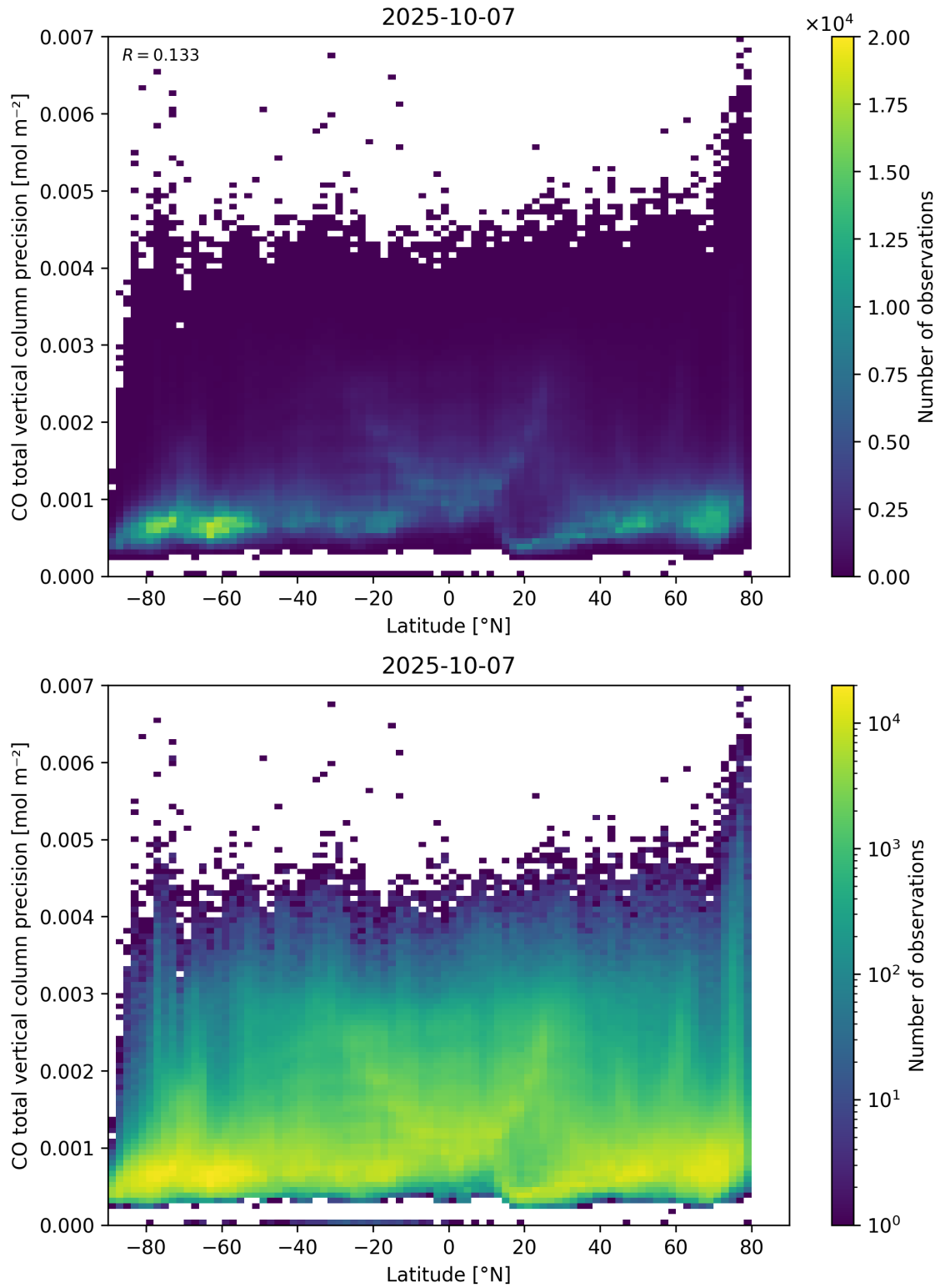
Figure 53: Scatter density plot of “Latitude” against “CO total vertical column precision” for 2025-10-06 to 2025-10-08.
