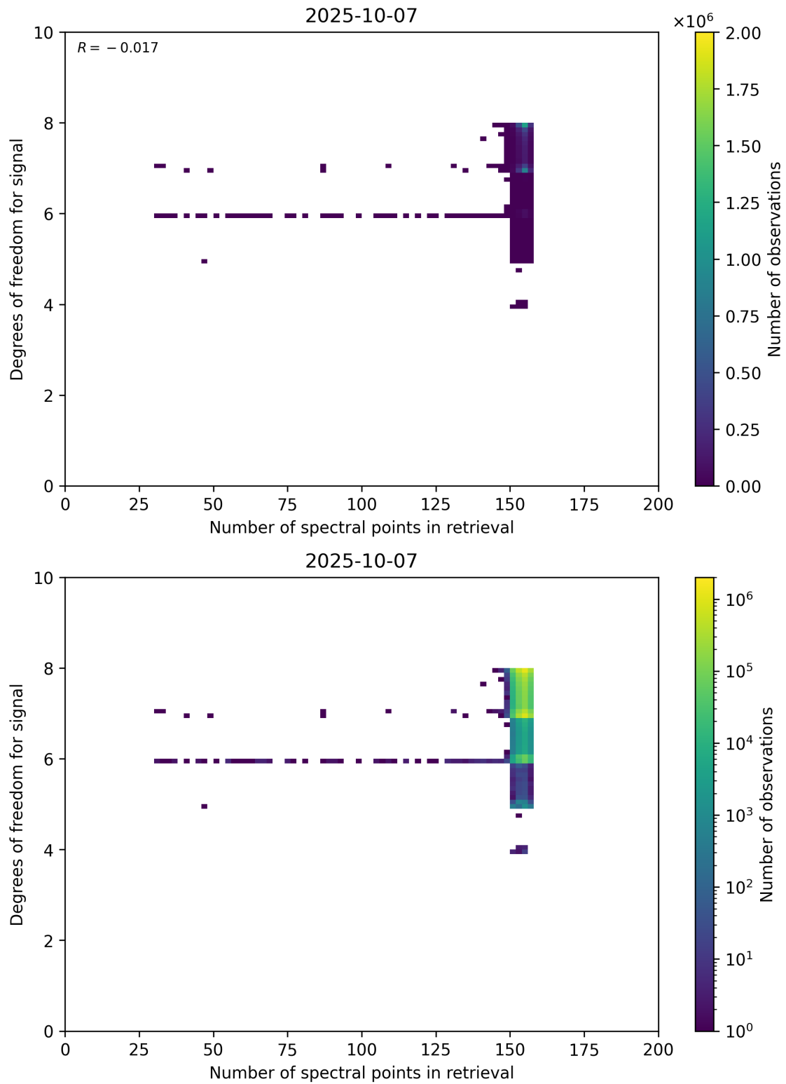
Figure 59: Scatter density plot of “Number of spectral points in retrieval” against “Degrees of freedom for signal” for 2025-10-06 to 2025-10-08.
