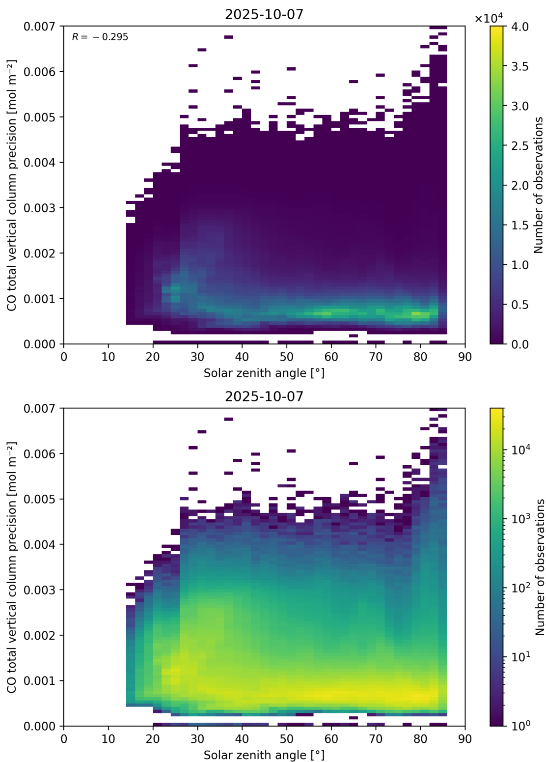
Figure 63: Scatter density plot of “Solar zenith angle” against “CO total vertical column precision” for 2025-10-06 to 2025-10-08.
