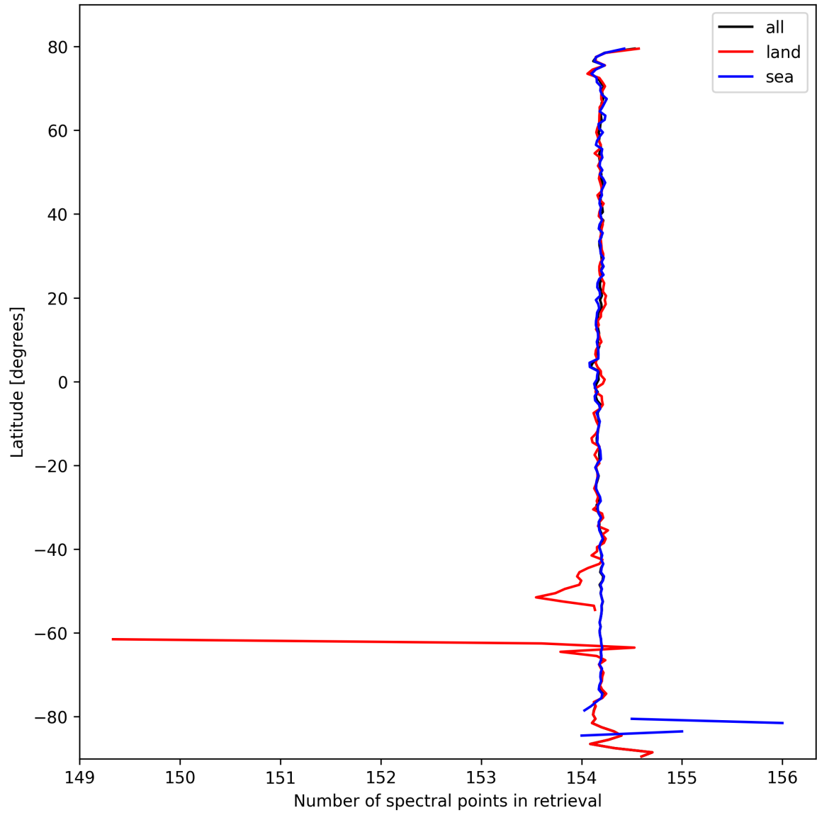
Figure 13: Zonal average of “Number of spectral points in retrieval” for 2025-10-06 to 2025-10-08.
