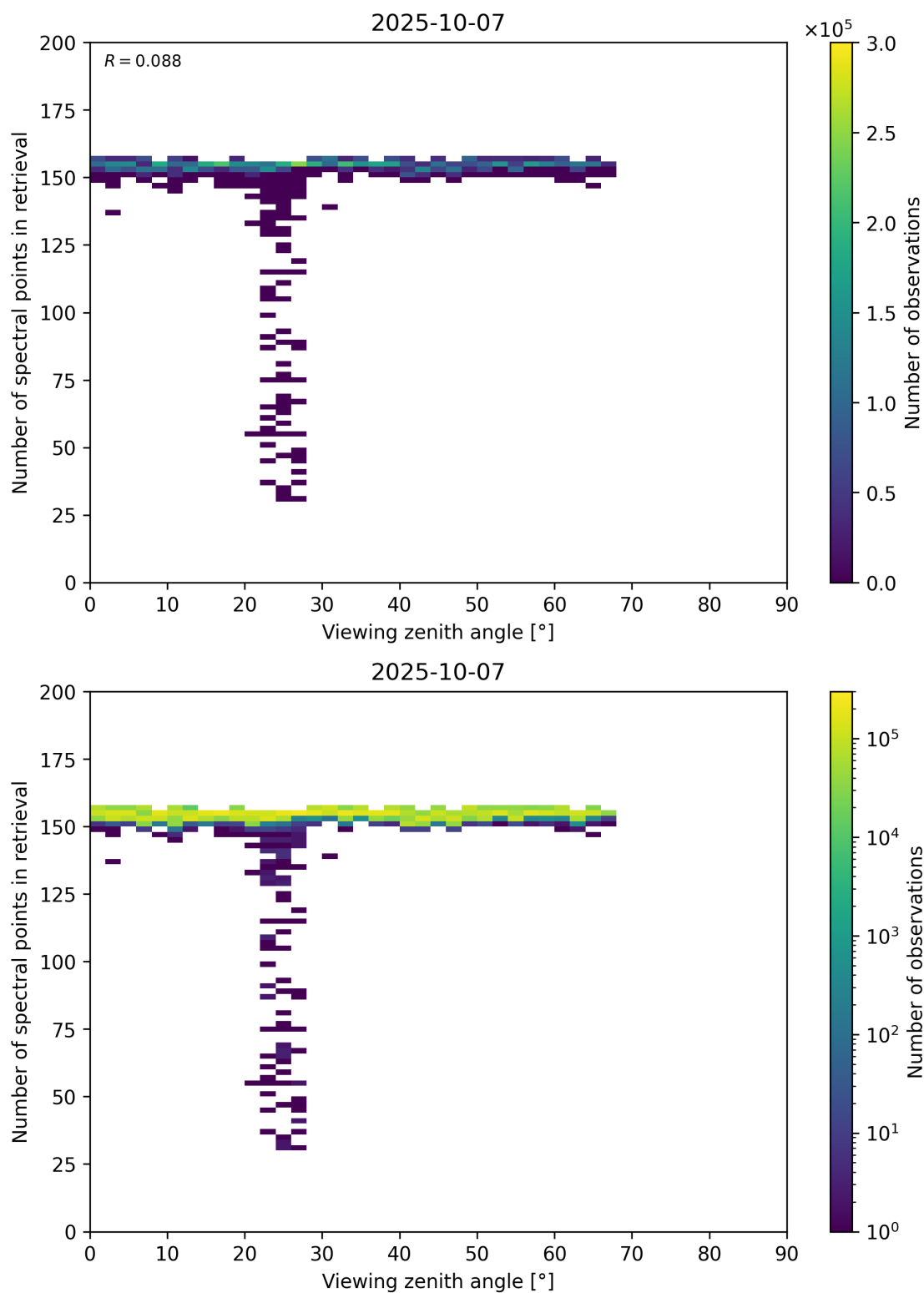
Figure 76: Scatter density plot of “Viewing zenith angle” against “Number of spectral points in retrieval” for 2025-10-06 to 2025-10-08.
