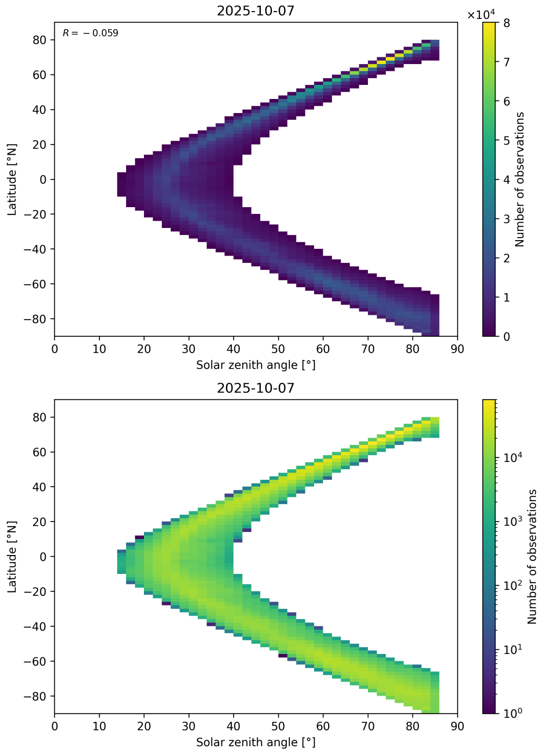
Figure 66: Scatter density plot of “Solar zenith angle” against “Latitude” for 2025-10-06 to 2025-10-08.
