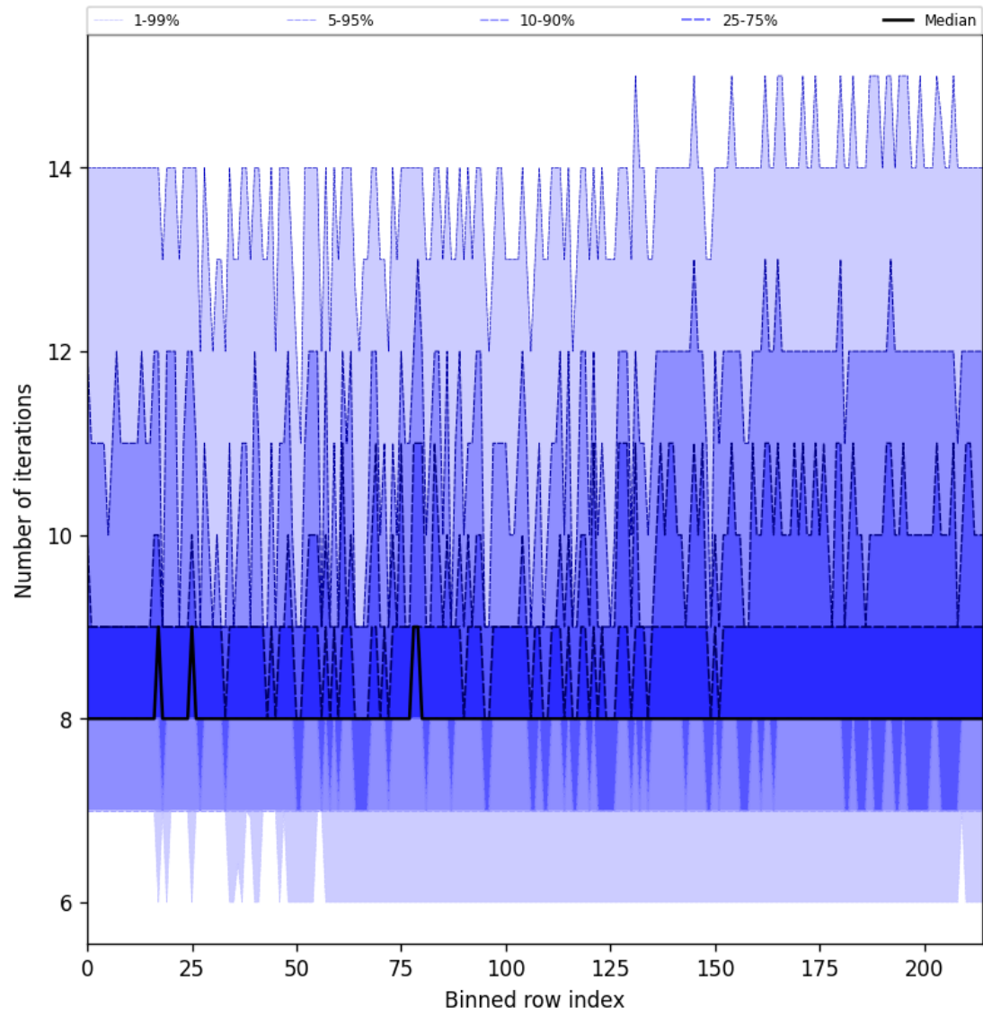
Figure 32: Along track statistics of “Number of iterations” for 2025-10-06 to 2025-10-08
