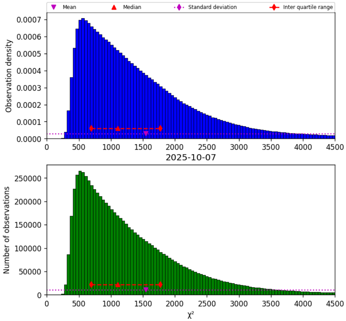
Figure 22: Histogram of “ \chi^2 ” for 2025-10-06 to 2025-10-08
