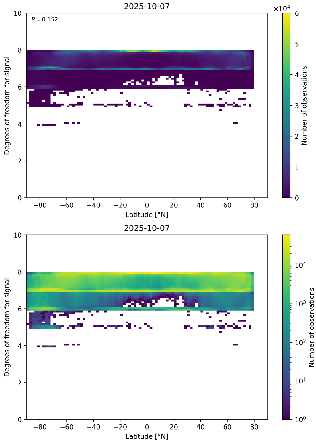
Figure 55: Scatter density plot of “Latitude” against “Degrees of freedom for signal” for 2025-10-06 to 2025-10-08.
