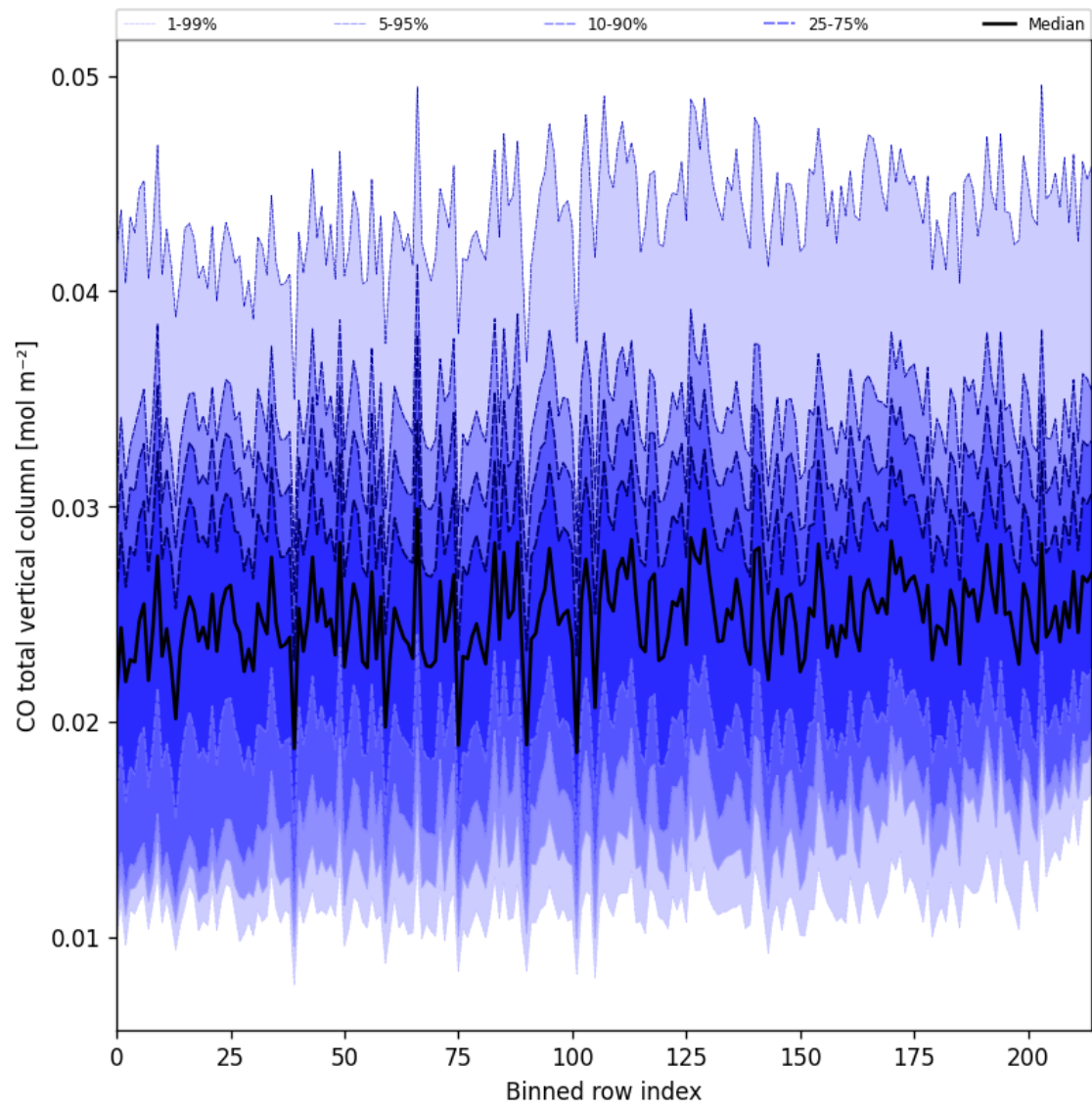
Figure 26: Along track statistics of “CO total vertical column” for 2025-10-06 to 2025-10-08
