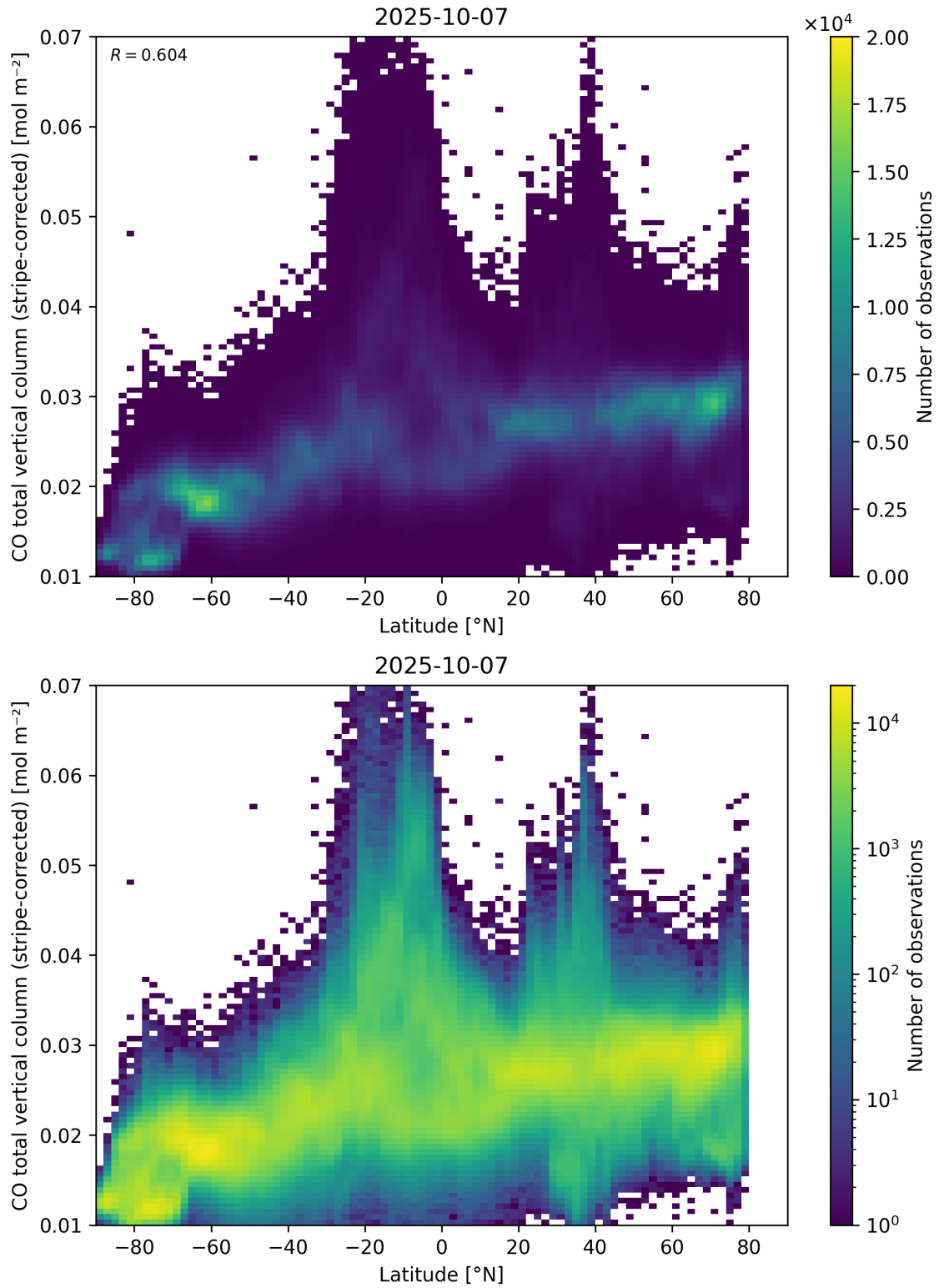
Figure 52: Scatter density plot of “Latitude” against “CO total vertical column (stripe-corrected)” for 2025-10-06 to 2025-10-08.
