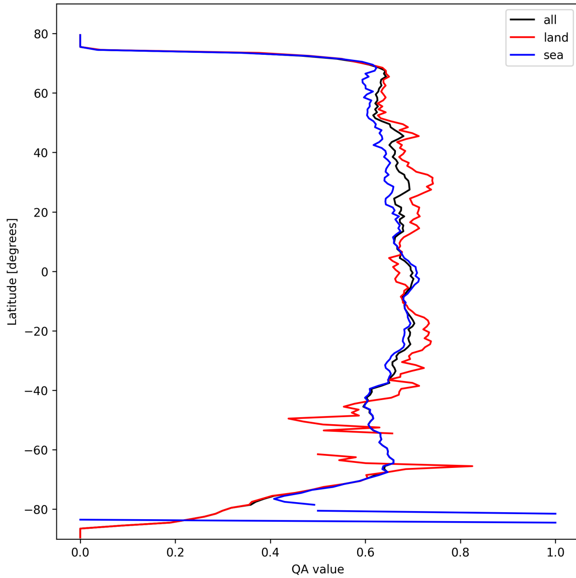
Figure 9: Zonal average of “QA value” for 2025-10-06 to 2025-10-08.
