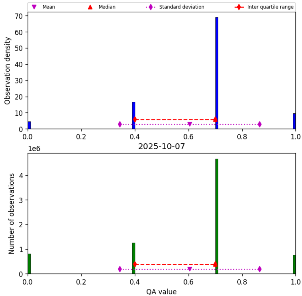
Figure 17: Histogram of “QA value” for 2025-10-06 to 2025-10-08
