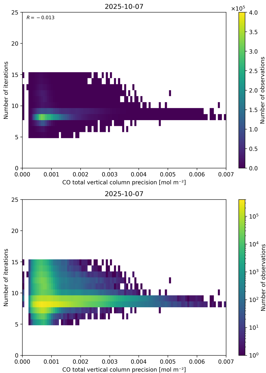
Figure 46: Scatter density plot of “CO total vertical column precision” against “Number of iterations” for 2025-10-06 to 2025-10-08.
