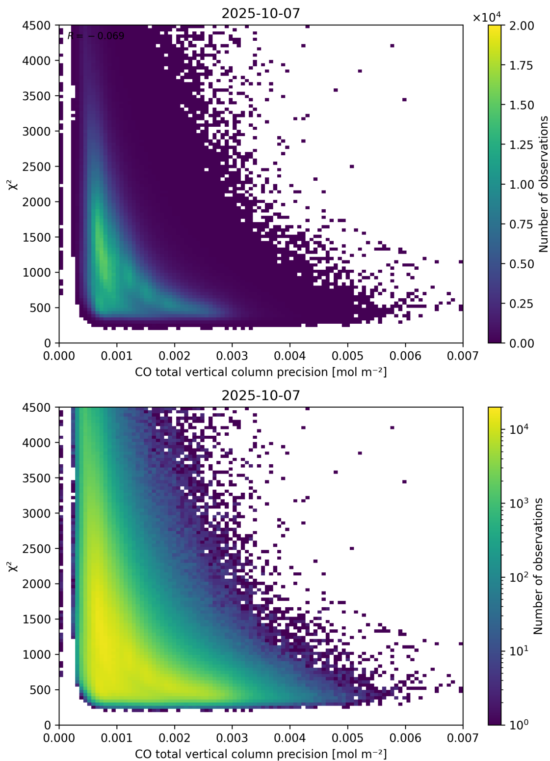
Figure 44: Scatter density plot of “CO total vertical column precision” against “ \chi^2 ” for 2025-10-06 to 2025-10-08.
