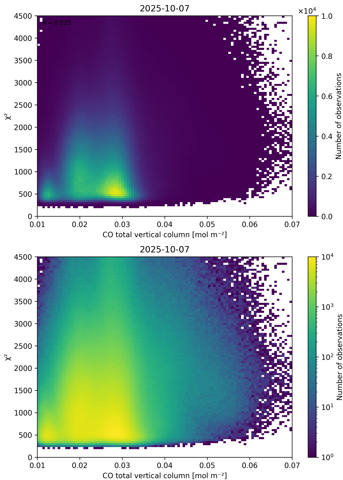
Figure 35: Scatter density plot of “CO total vertical column” against “ \chi^2 ” for 2025-10-06 to 2025-10-08.
