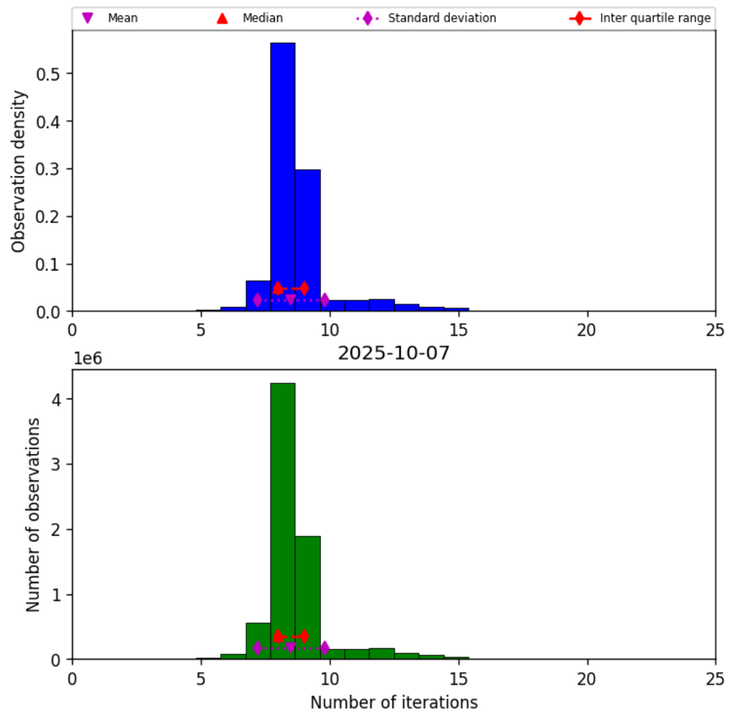
Figure 24: Histogram of “Number of iterations” for 2025-10-06 to 2025-10-08
