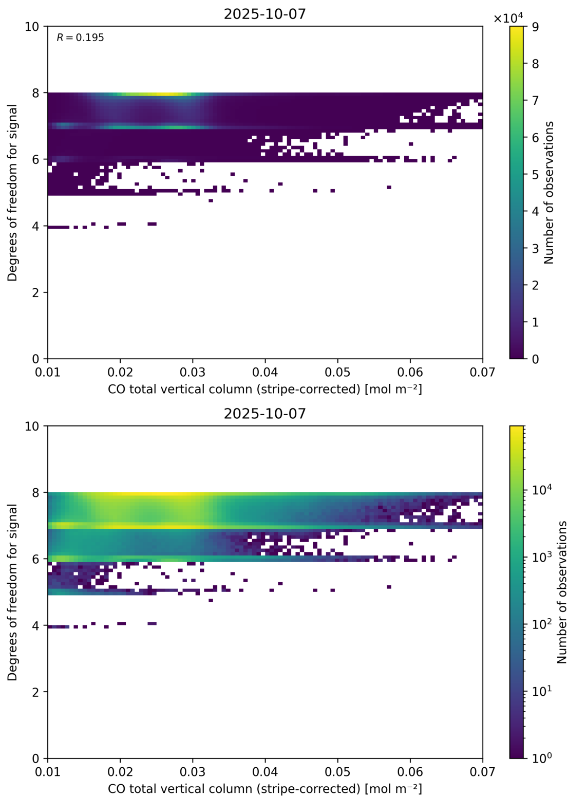
Figure 38: Scatter density plot of “CO total vertical column (stripe-corrected)” against “Degrees of freedom for signal” for 2025-10-06 to 2025-10-08.
