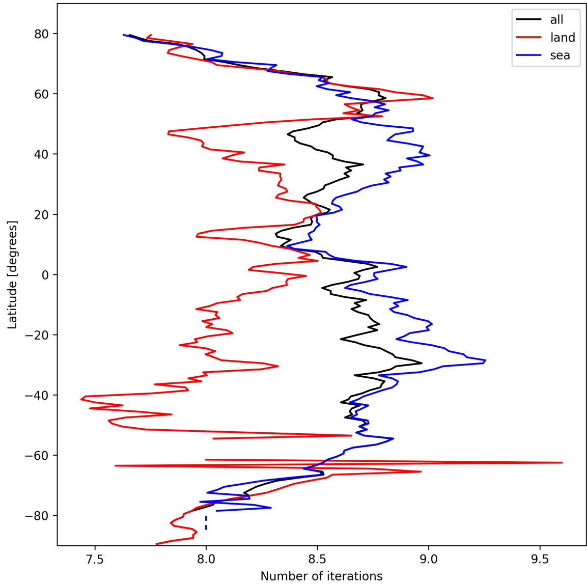
Figure 16: Zonal average of “Number of iterations” for 2025-10-06 to 2025-10-08.
