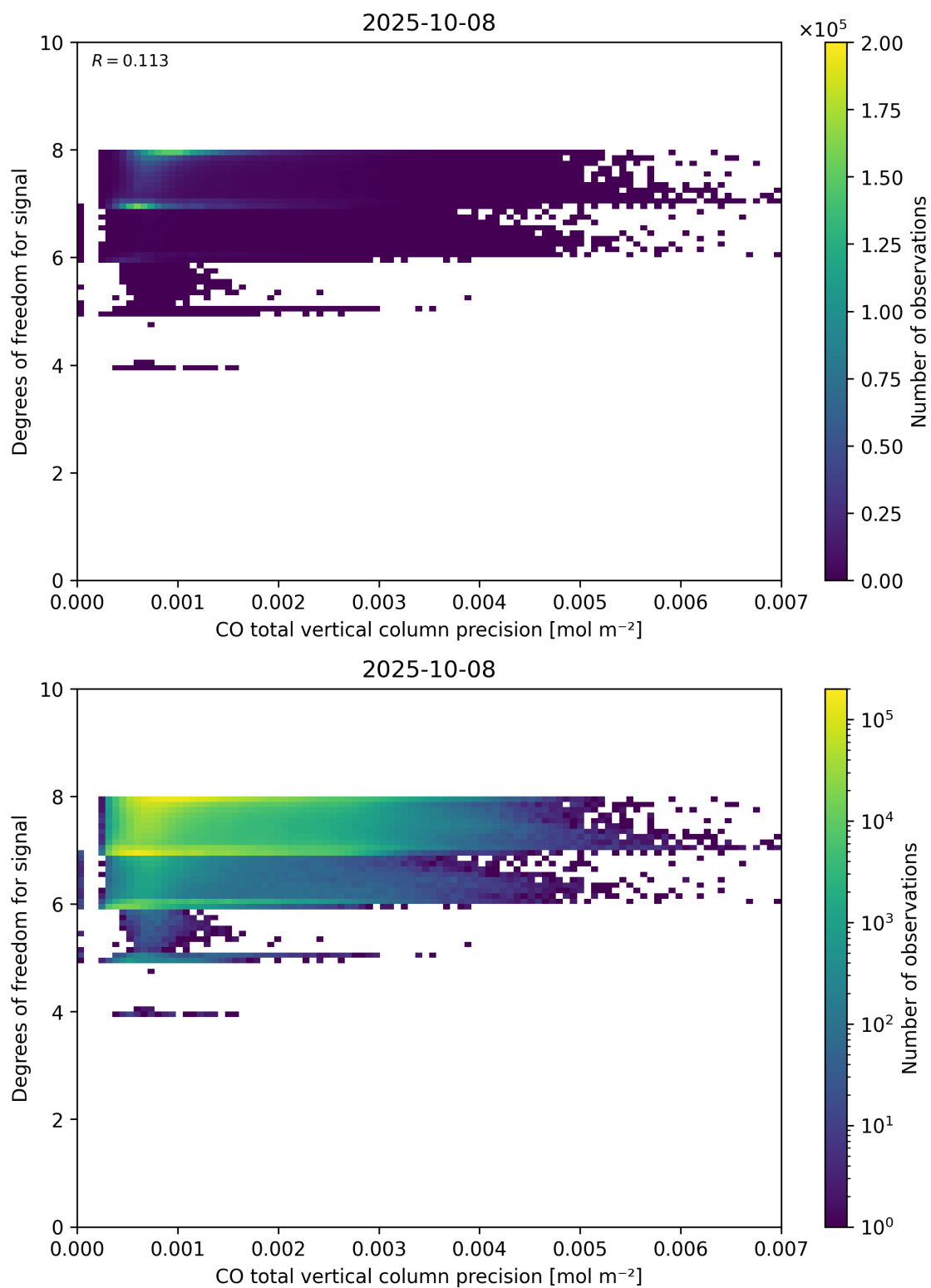
Figure 45: Scatter density plot of “CO total vertical column precision” against “Degrees of freedom for signal” for 2025-10-07 to 2025-10-09.
