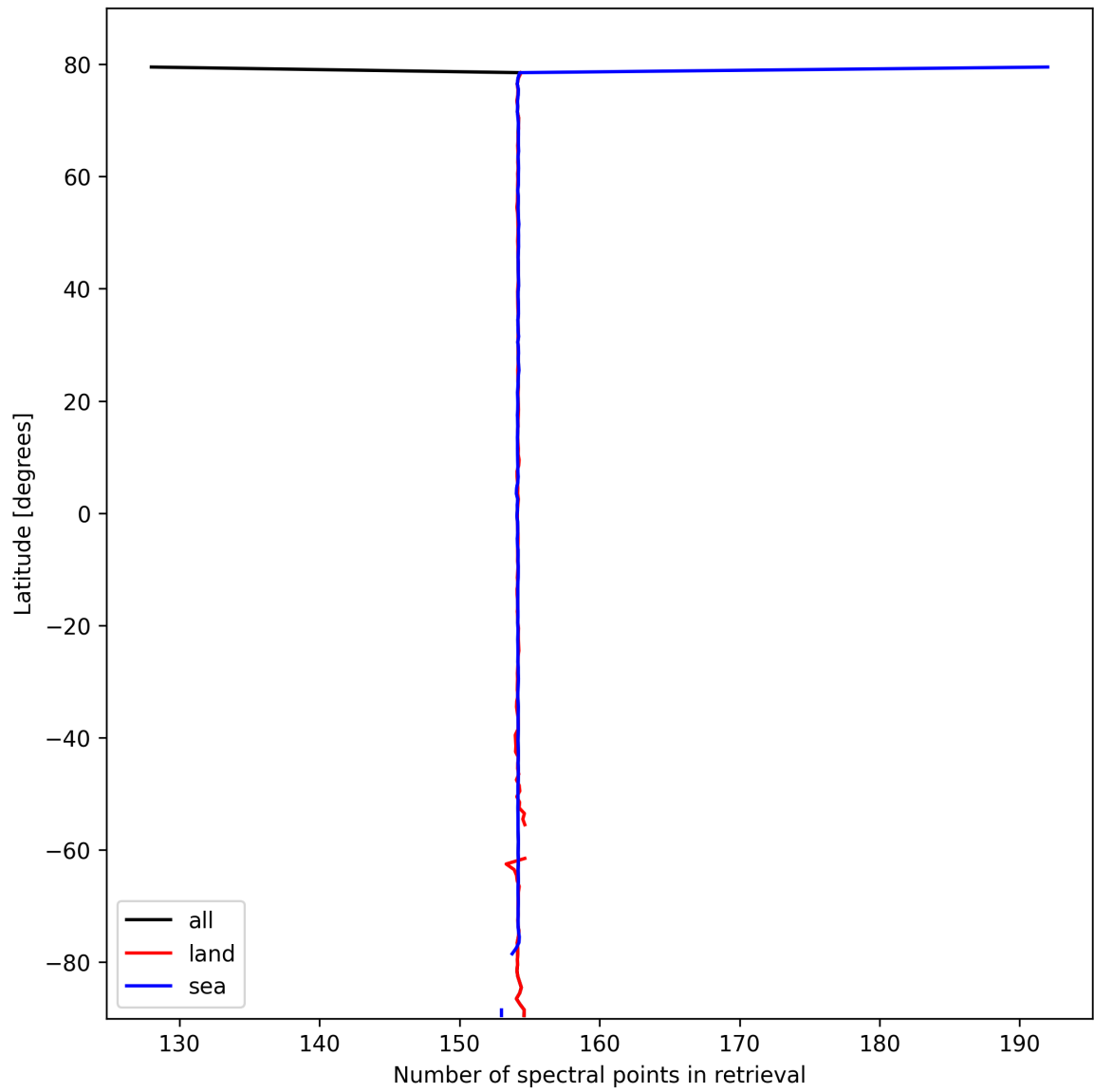
Figure 13: Zonal average of “Number of spectral points in retrieval” for 2025-10-07 to 2025-10-09.
