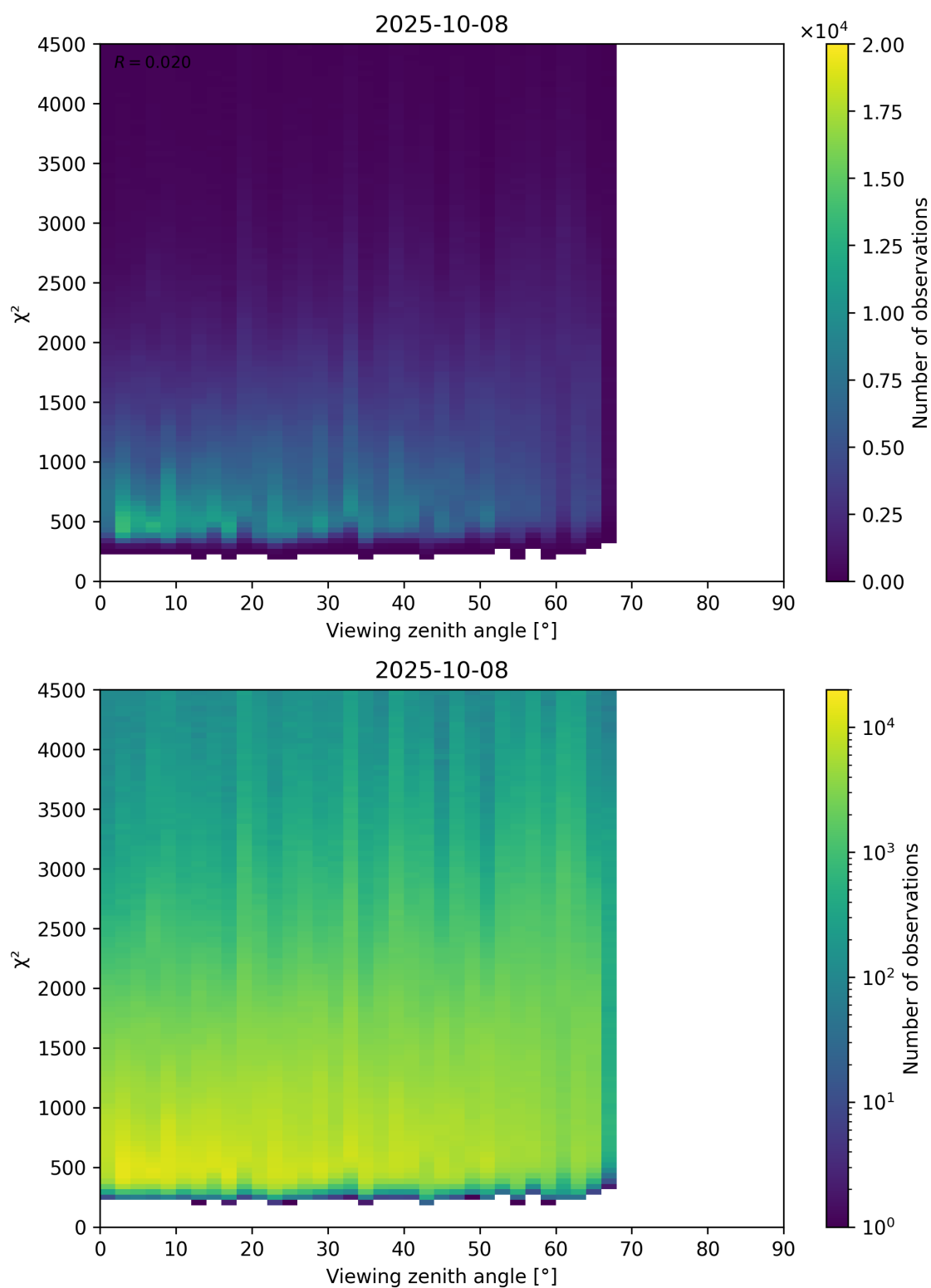
Figure 72: Scatter density plot of “Viewing zenith angle” against “ \chi^2 ” for 2025-10-07 to 2025-10-09.
