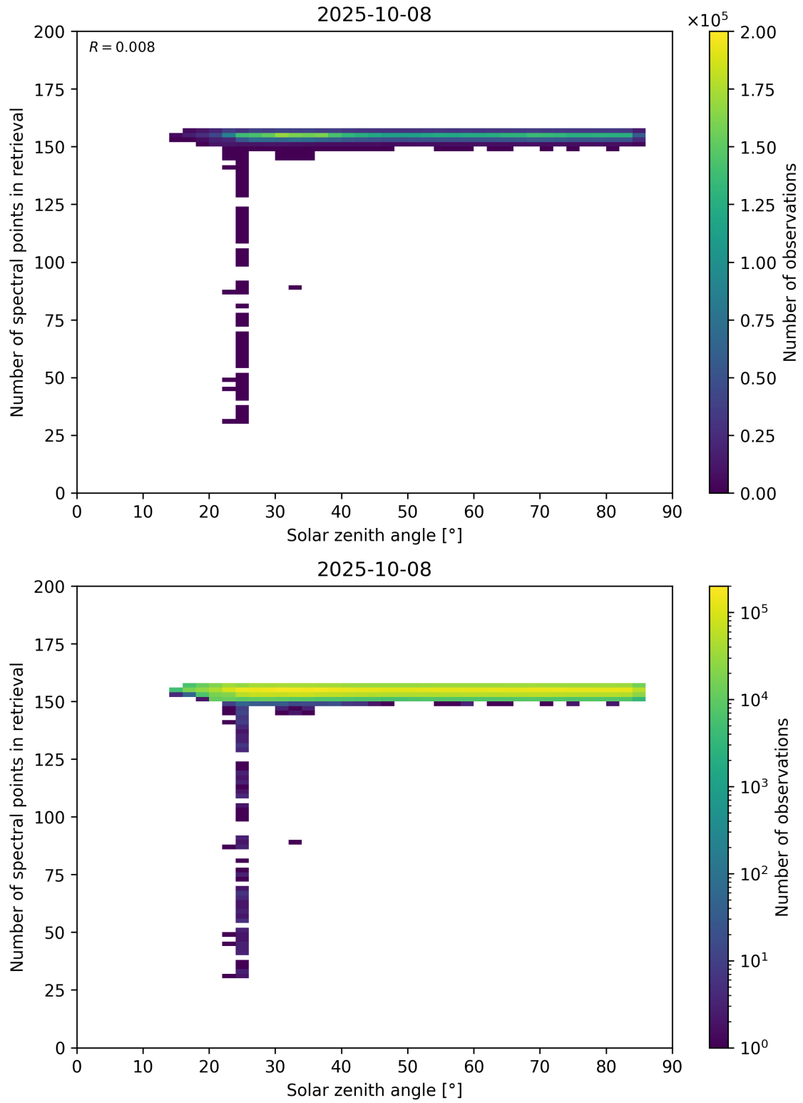
Figure 68: Scatter density plot of “Solar zenith angle” against “Number of spectral points in retrieval” for 2025-10-07 to 2025-10-09.
