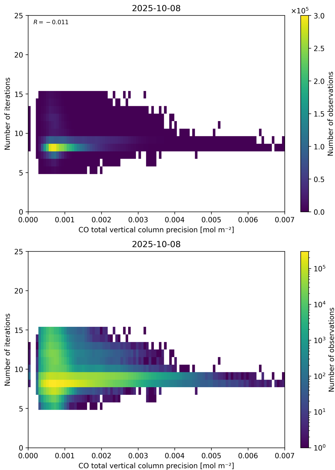
Figure 46: Scatter density plot of “CO total vertical column precision” against “Number of iterations” for 2025-10-07 to 2025-10-09.
