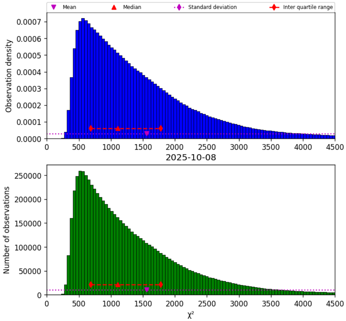
Figure 22: Histogram of " \chi^2 " for 2025-10-07 to 2025-10-09
