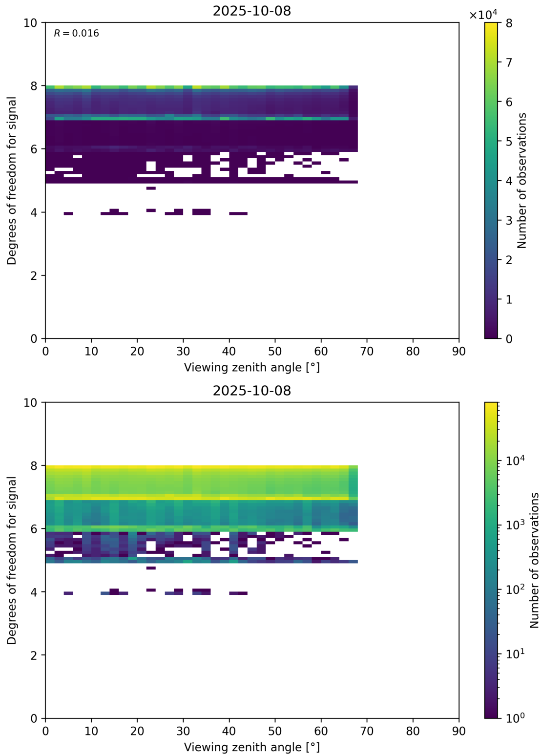
Figure 73: Scatter density plot of “Viewing zenith angle” against “Degrees of freedom for signal” for 2025-10-07 to 2025-10-09.
