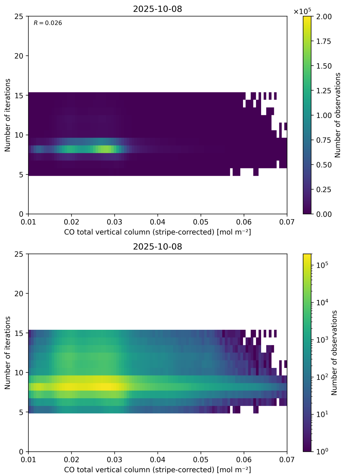
Figure 39: Scatter density plot of “CO total vertical column (stripe-corrected)” against “Number of iterations” for 2025-10-07 to 2025-10-09.
