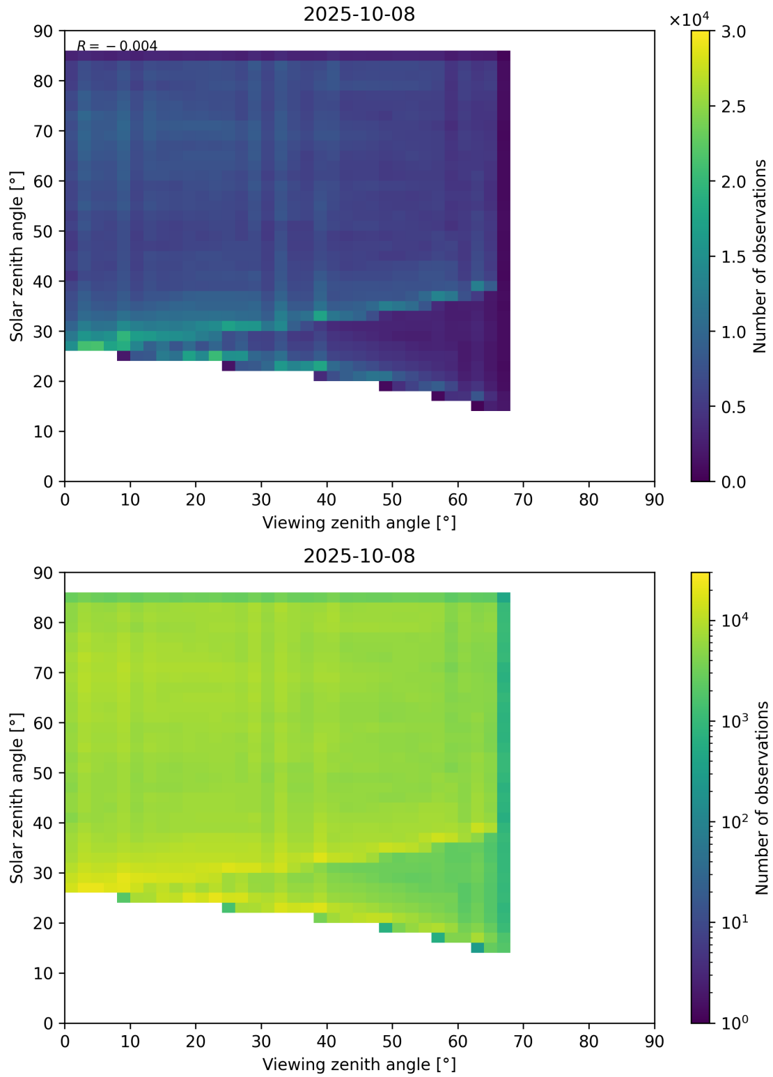
Figure 77: Scatter density plot of “Viewing zenith angle” against “Solar zenith angle” for 2025-10-07 to 2025-10-09.
