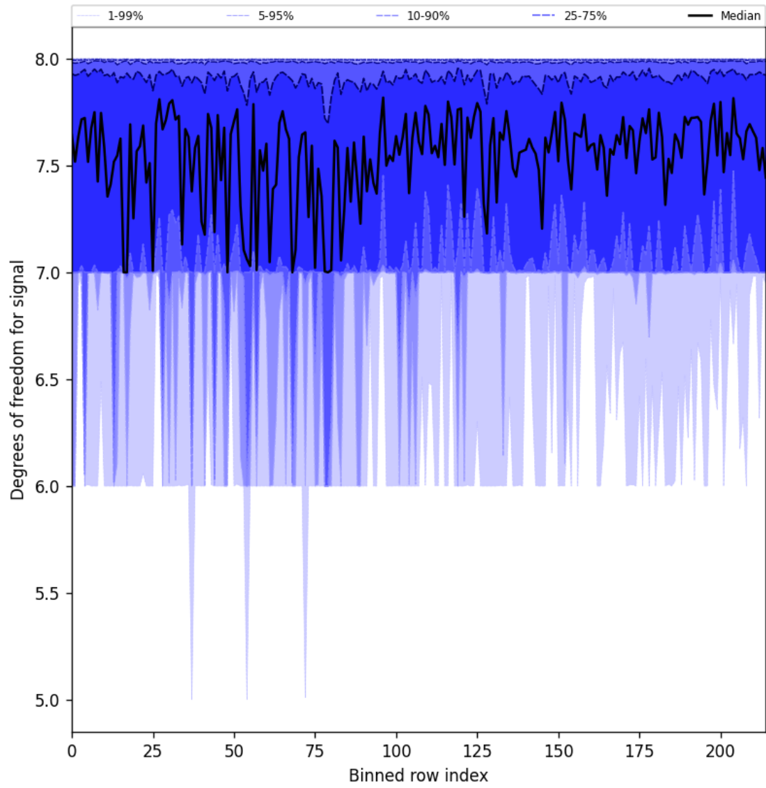
Figure 31: Along track statistics of “Degrees of freedom for signal” for 2025-10-07 to 2025-10-09
