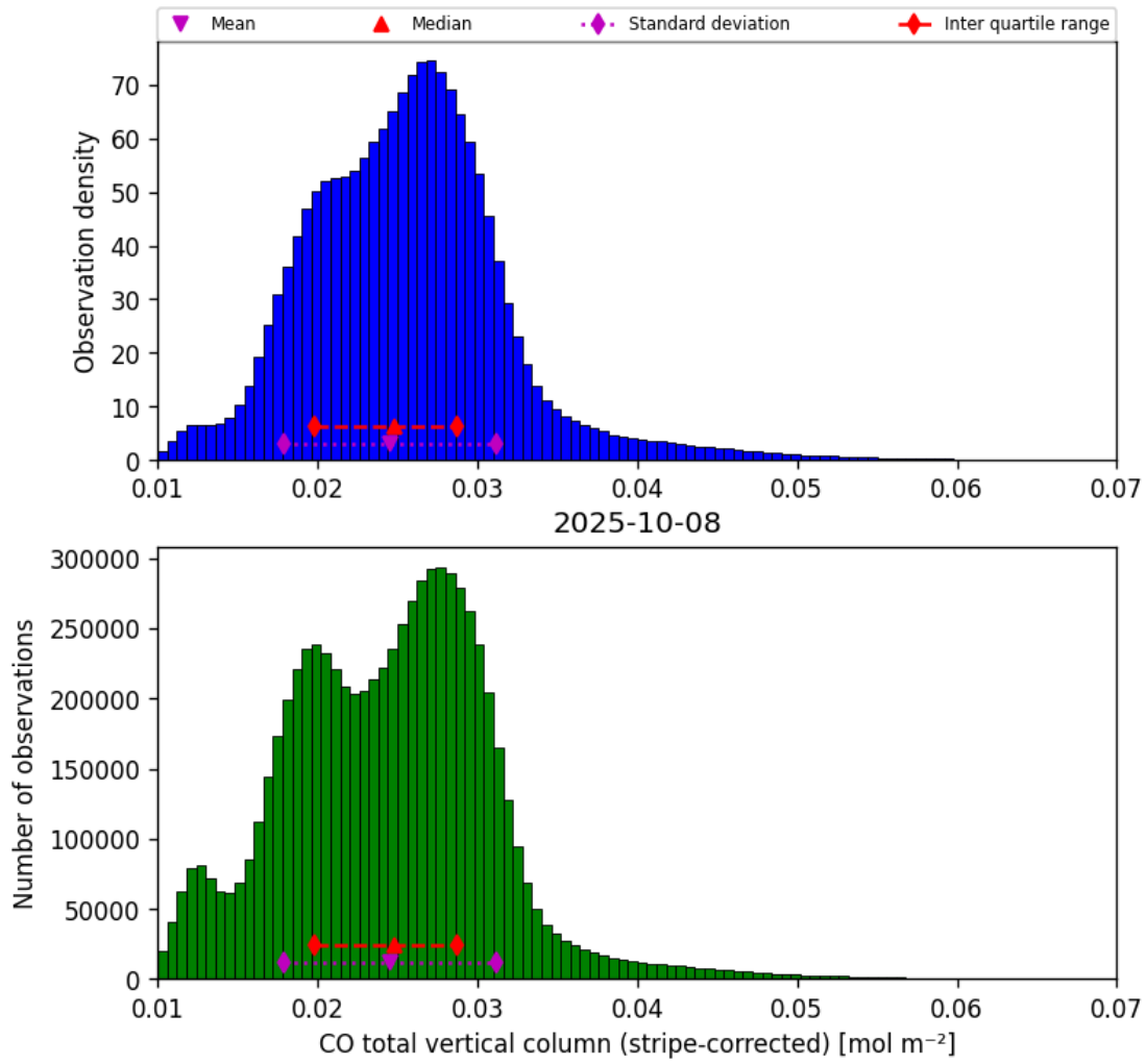
Figure 19: Histogram of “CO total vertical column (stripe-corrected)” for 2025-10-07 to 2025-10-09
