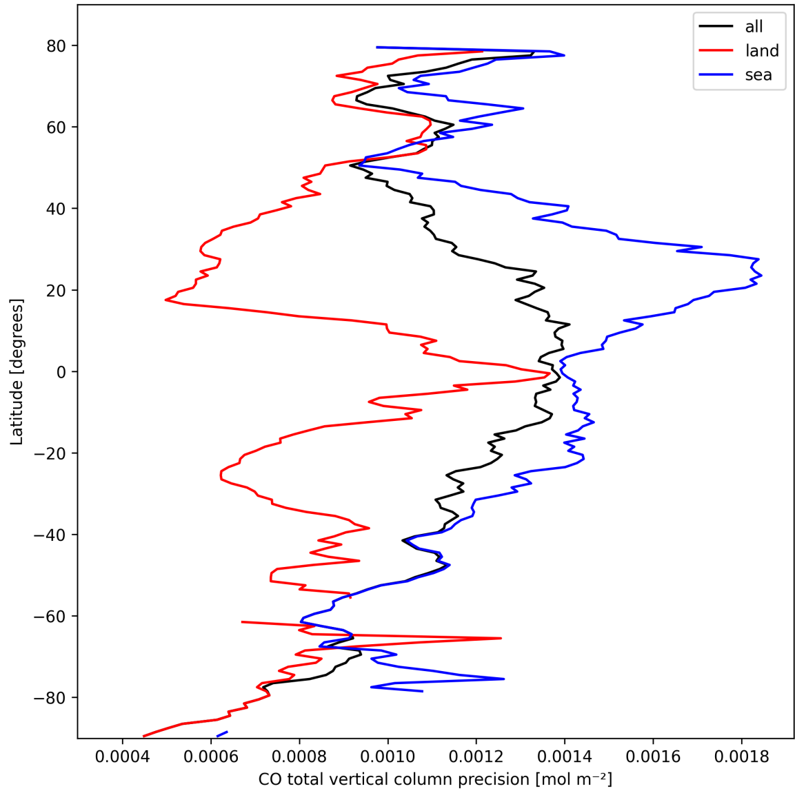
Figure 12: Zonal average of “CO total vertical column precision” for 2025-10-07 to 2025-10-09.
