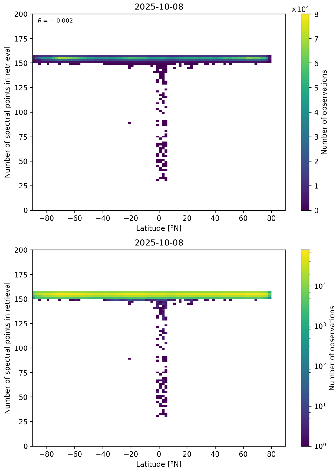
Figure 57: Scatter density plot of “Latitude” against “Number of spectral points in retrieval” for 2025-10-07 to 2025-10-09.
