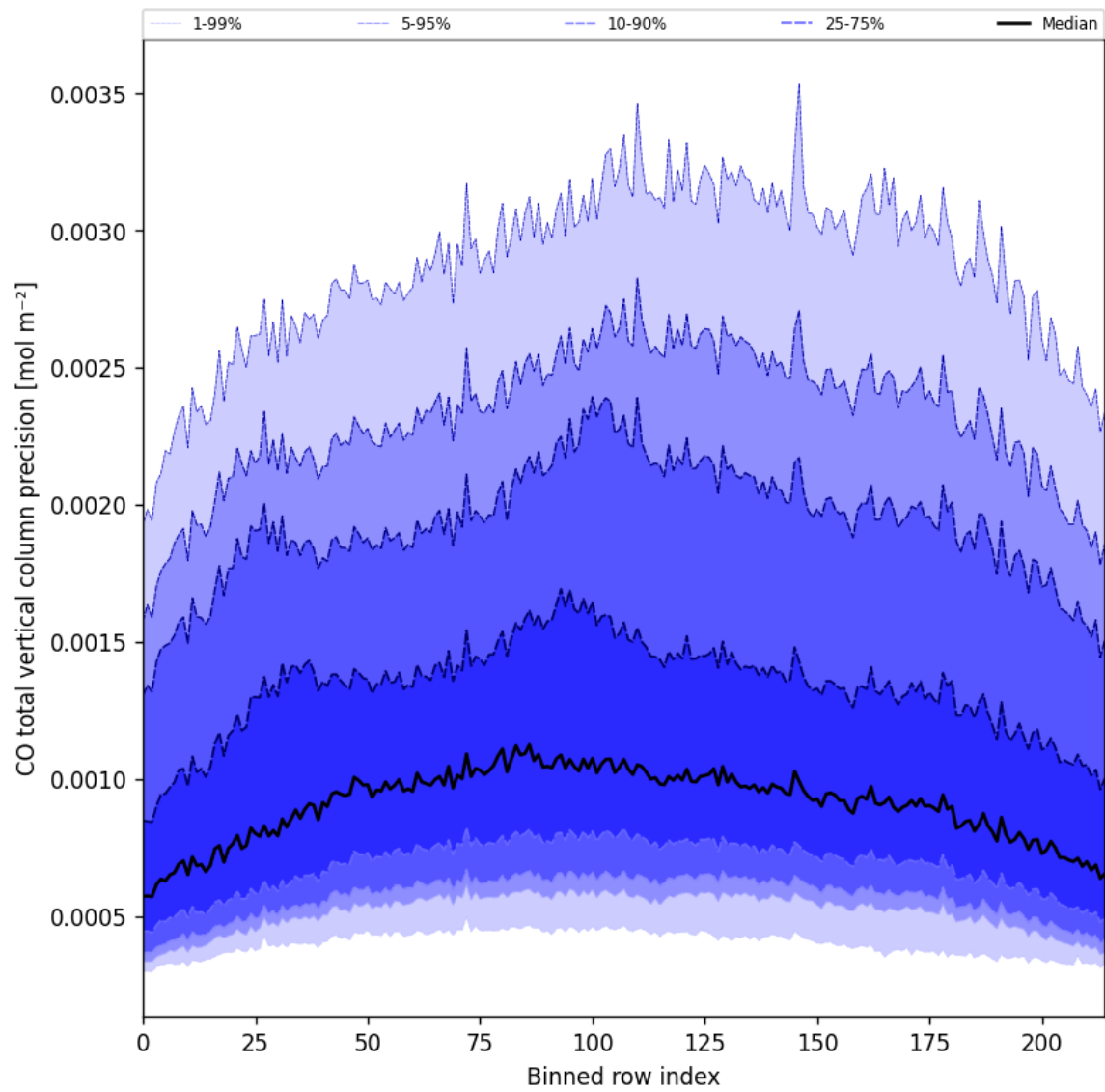
Figure 28: Along track statistics of “CO total vertical column precision” for 2025-10-07 to 2025-10-09
