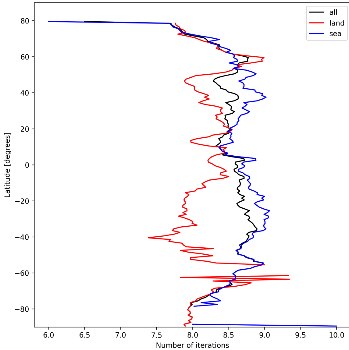
Figure 16: Zonal average of “Number of iterations” for 2025-10-07 to 2025-10-09.
