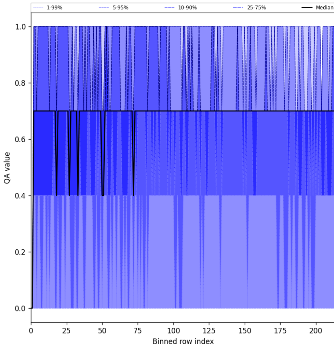
Figure 25: Along track statistics of “QA value” for 2025-10-07 to 2025-10-09
