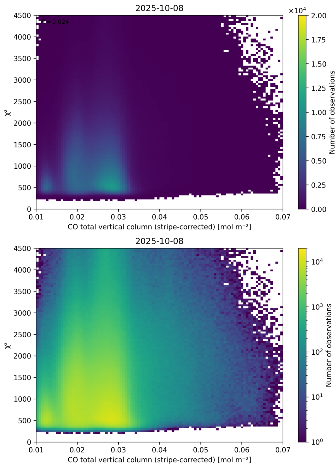
Figure 37: Scatter density plot of “CO total vertical column (stripe-corrected)” against “ \chi^2 ” for 2025-10-07 to 2025-10-09.
