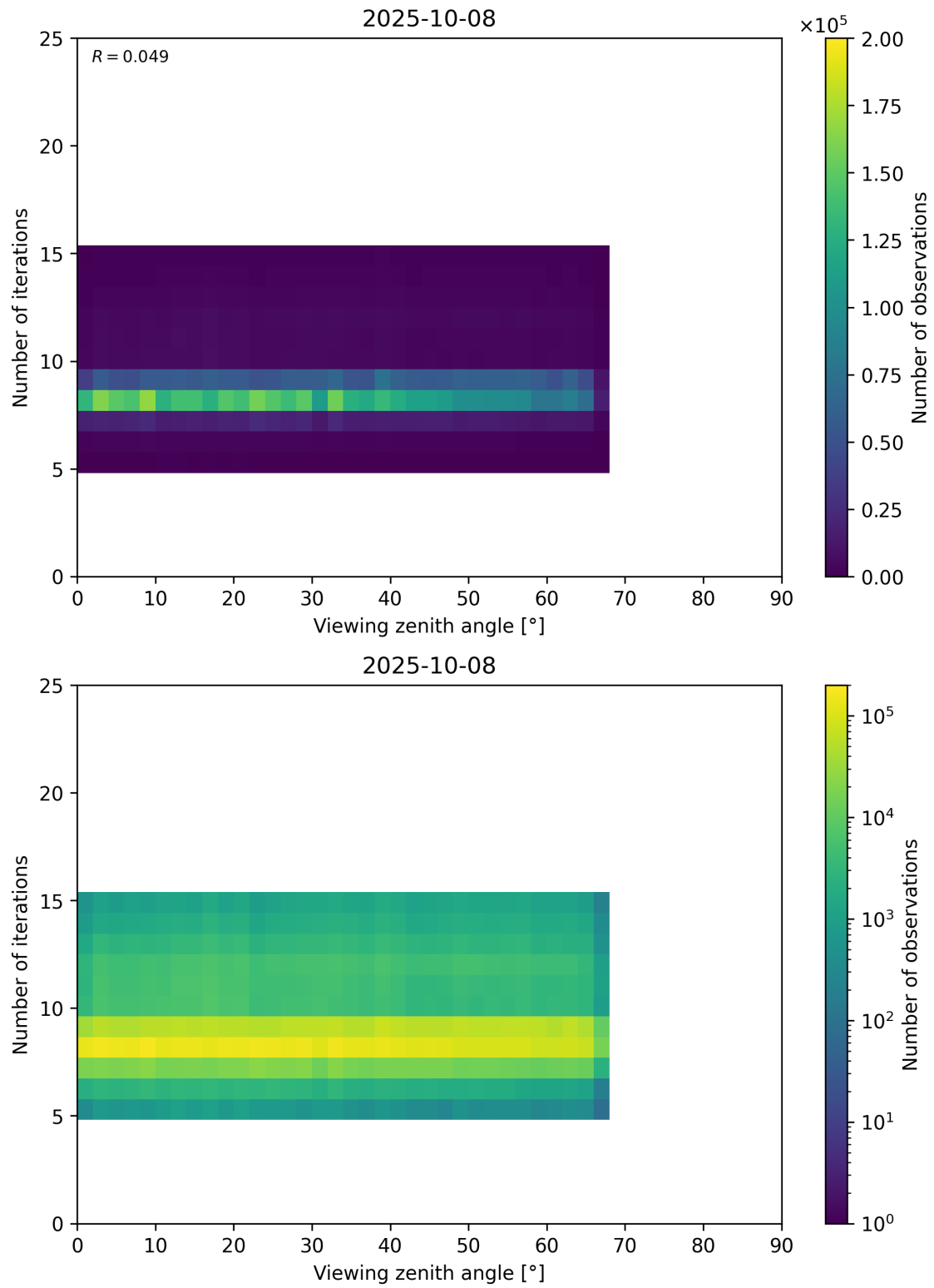
Figure 75: Scatter density plot of “Viewing zenith angle” against “Number of iterations” for 2025-10-07 to 2025-10-09.
