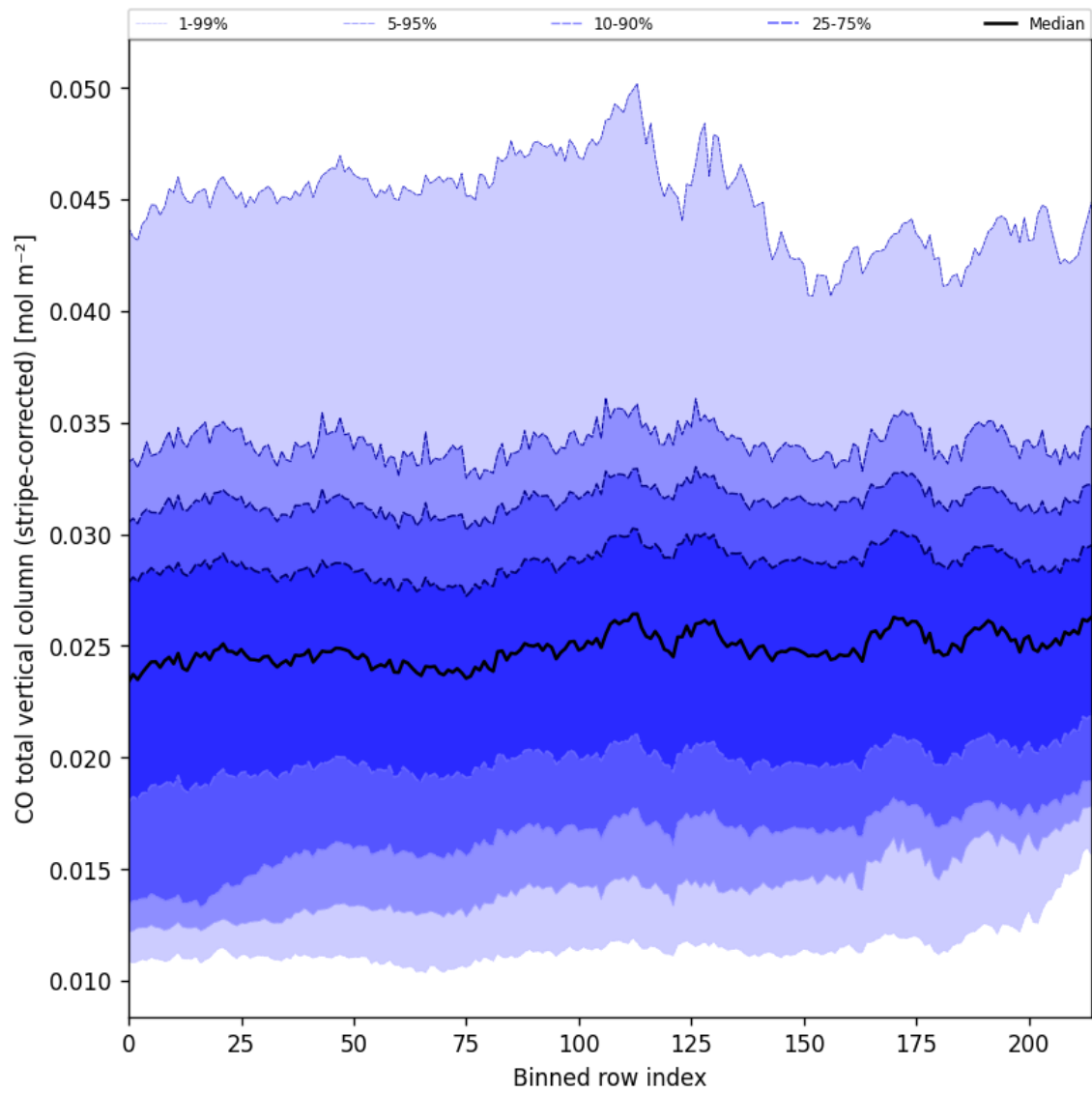
Figure 27: Along track statistics of “CO total vertical column (stripe-corrected)” for 2025-10-07 to 2025-10-09
