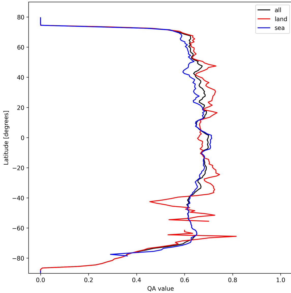
Figure 9: Zonal average of “QA value” for 2025-10-07 to 2025-10-09.
