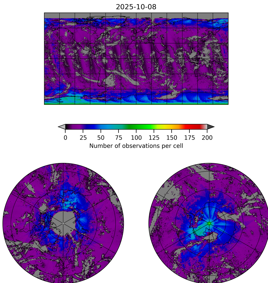
Figure 8: Map of the number of observations for 2025-10-07 to 2025-10-09
