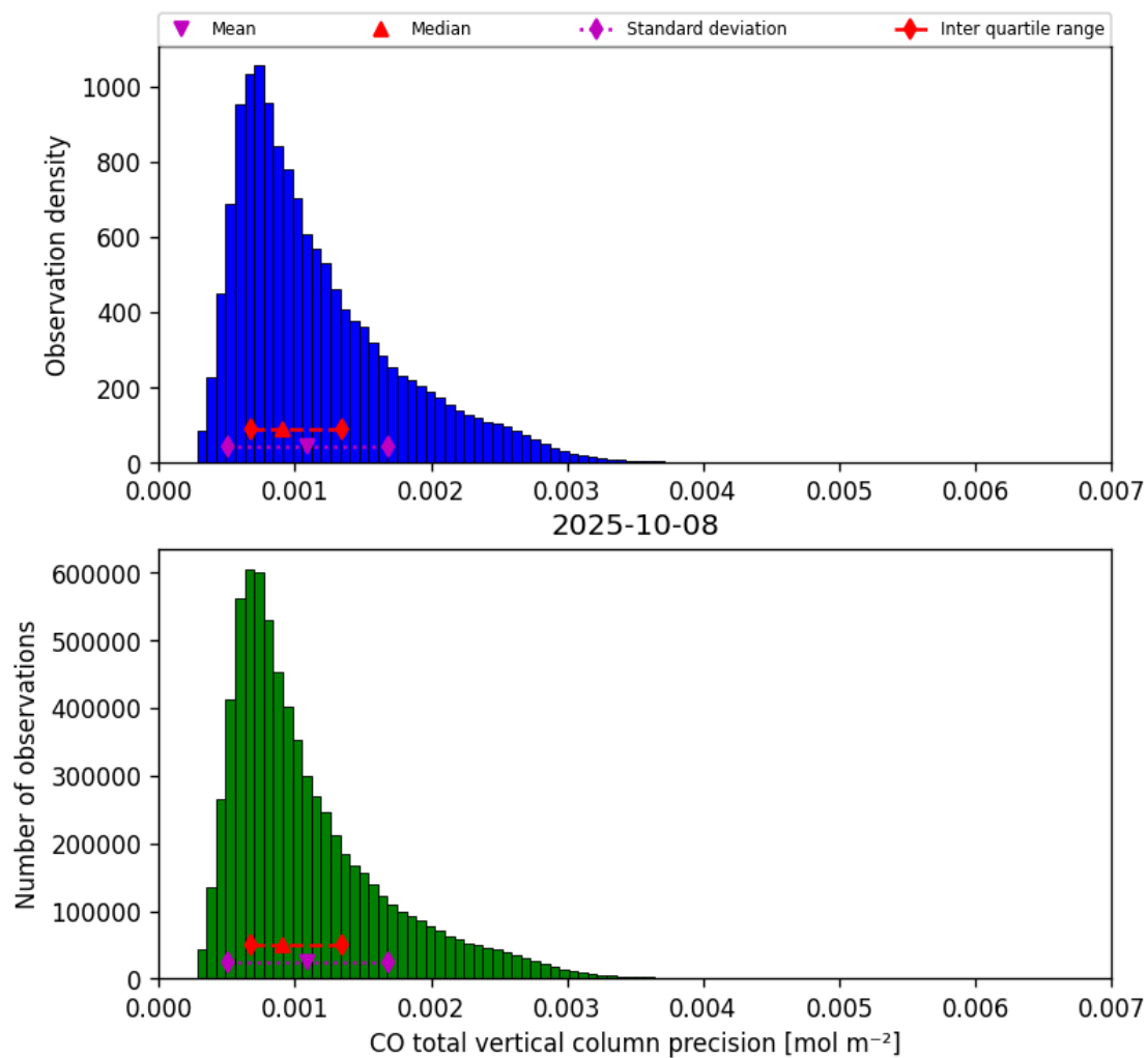
Figure 20: Histogram of “CO total vertical column precision” for 2025-10-07 to 2025-10-09
