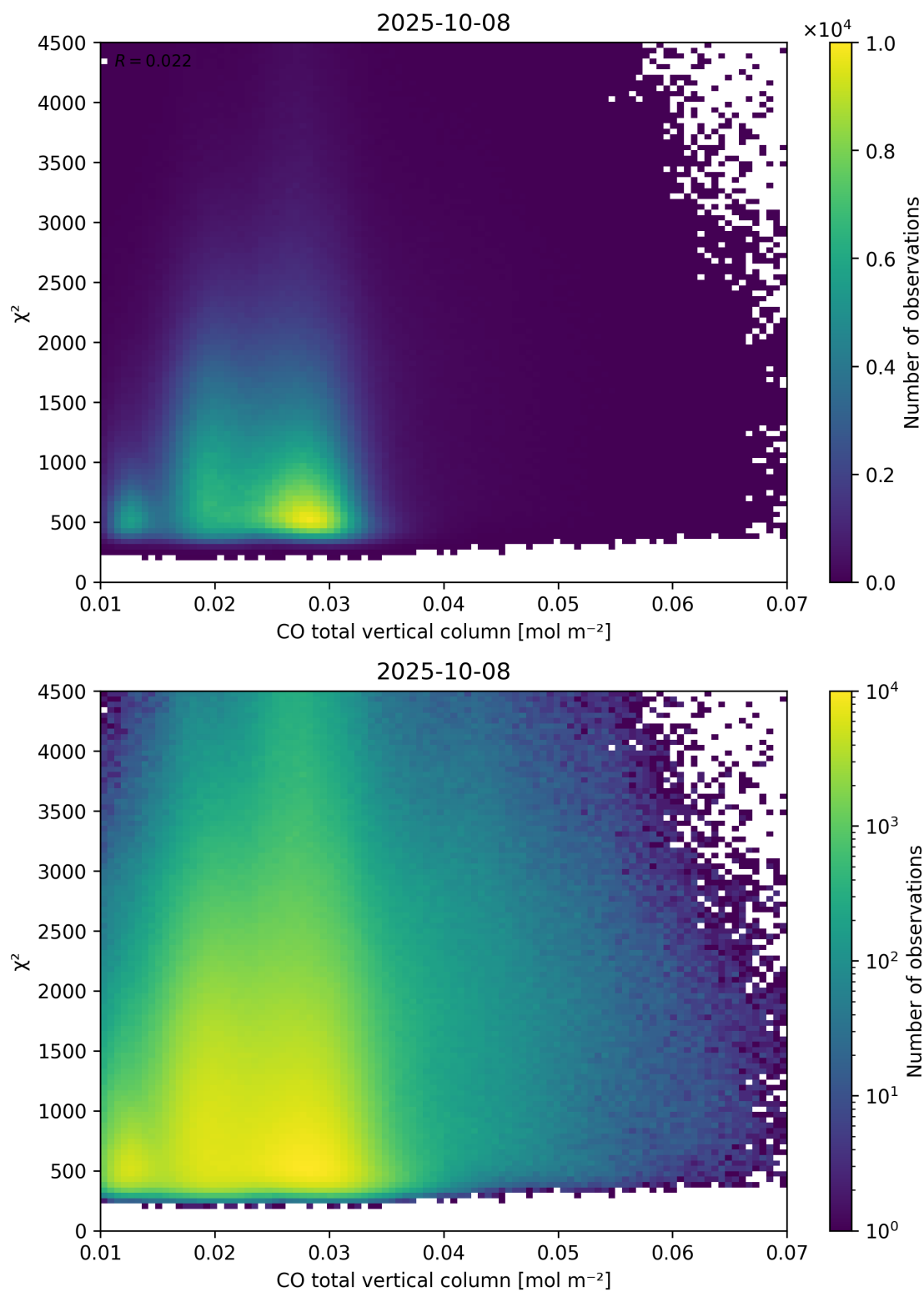
Figure 35: Scatter density plot of “CO total vertical column” against “ \chi^2 ” for 2025-10-07 to 2025-10-09.
