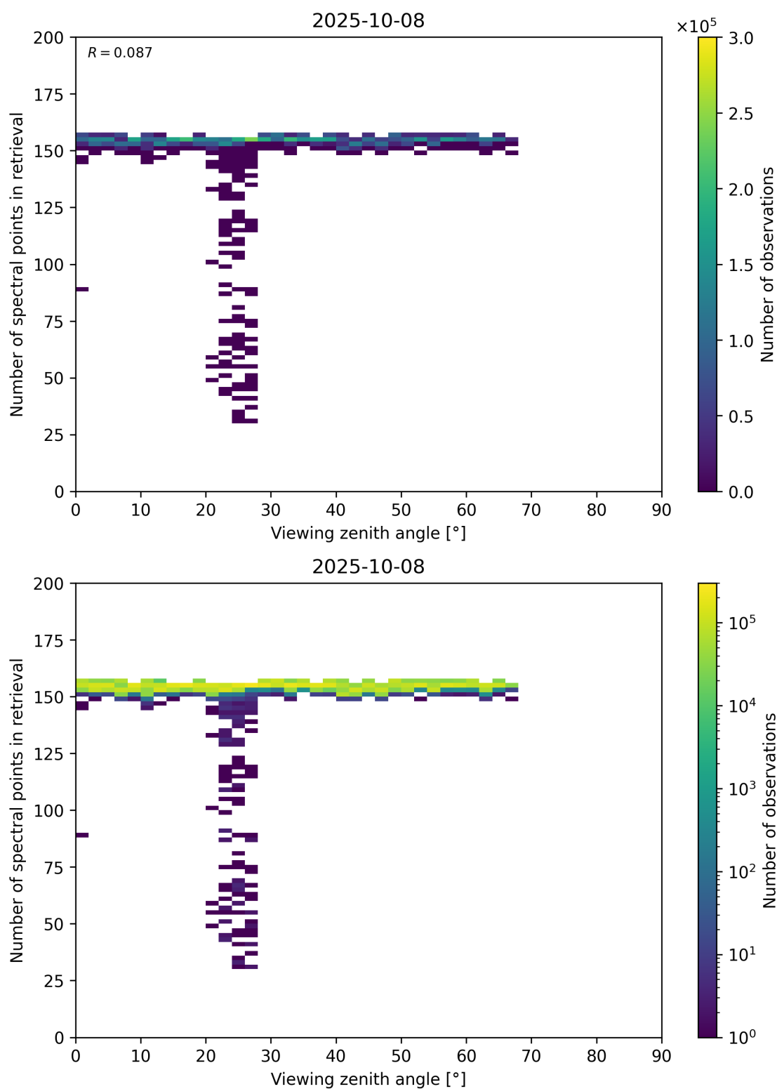
Figure 76: Scatter density plot of “Viewing zenith angle” against “Number of spectral points in retrieval” for 2025-10-07 to 2025-10-09.
