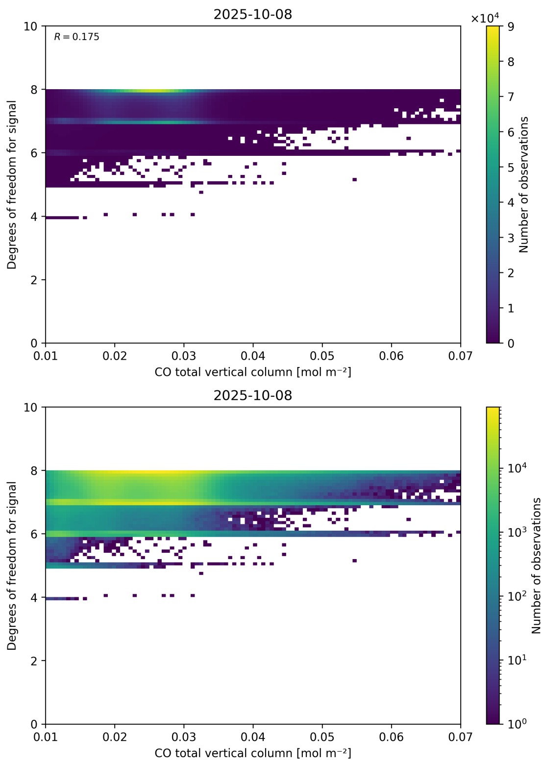
Figure 41: Scatter density plot of “CO total vertical column” against “Degrees of freedom for signal” for 2025-10-07 to 2025-10-09.
