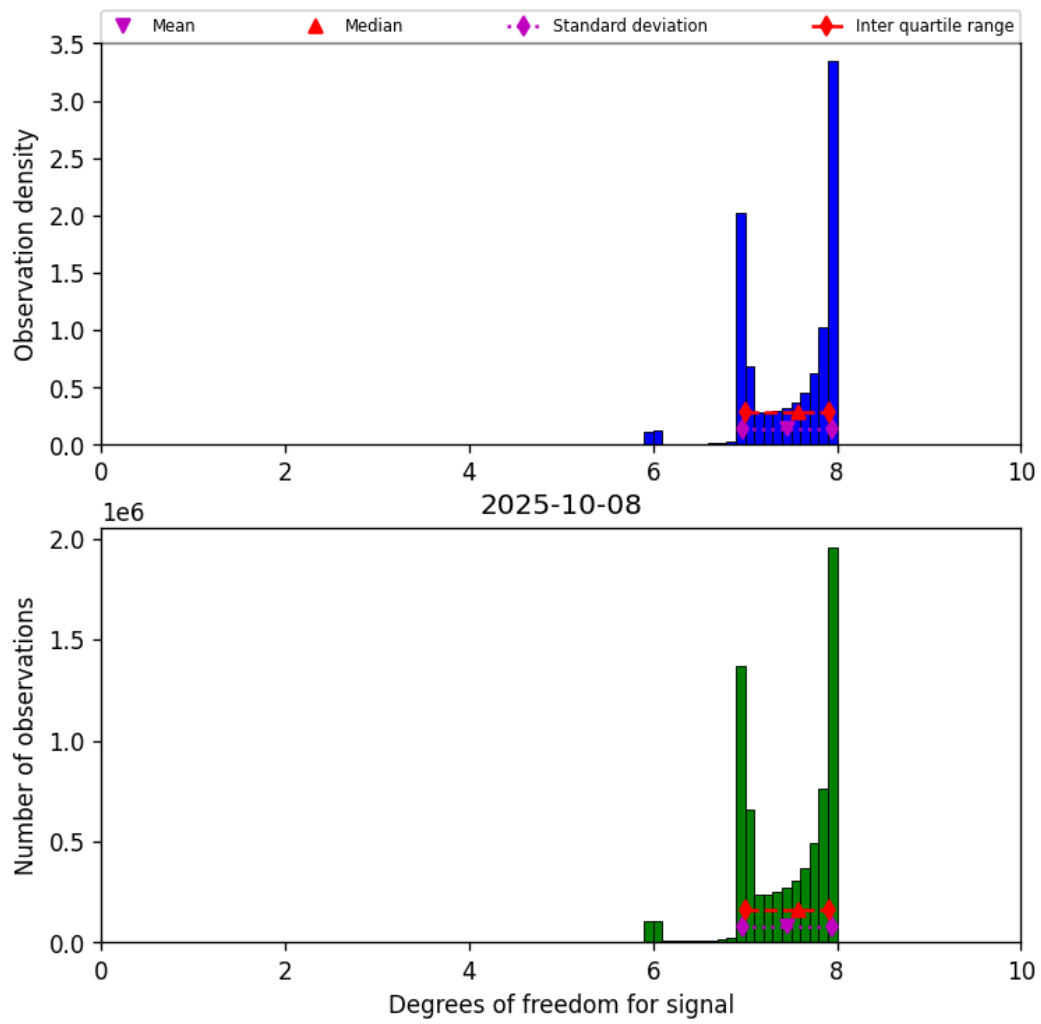
Figure 23: Histogram of “Degrees of freedom for signal” for 2025-10-07 to 2025-10-09
