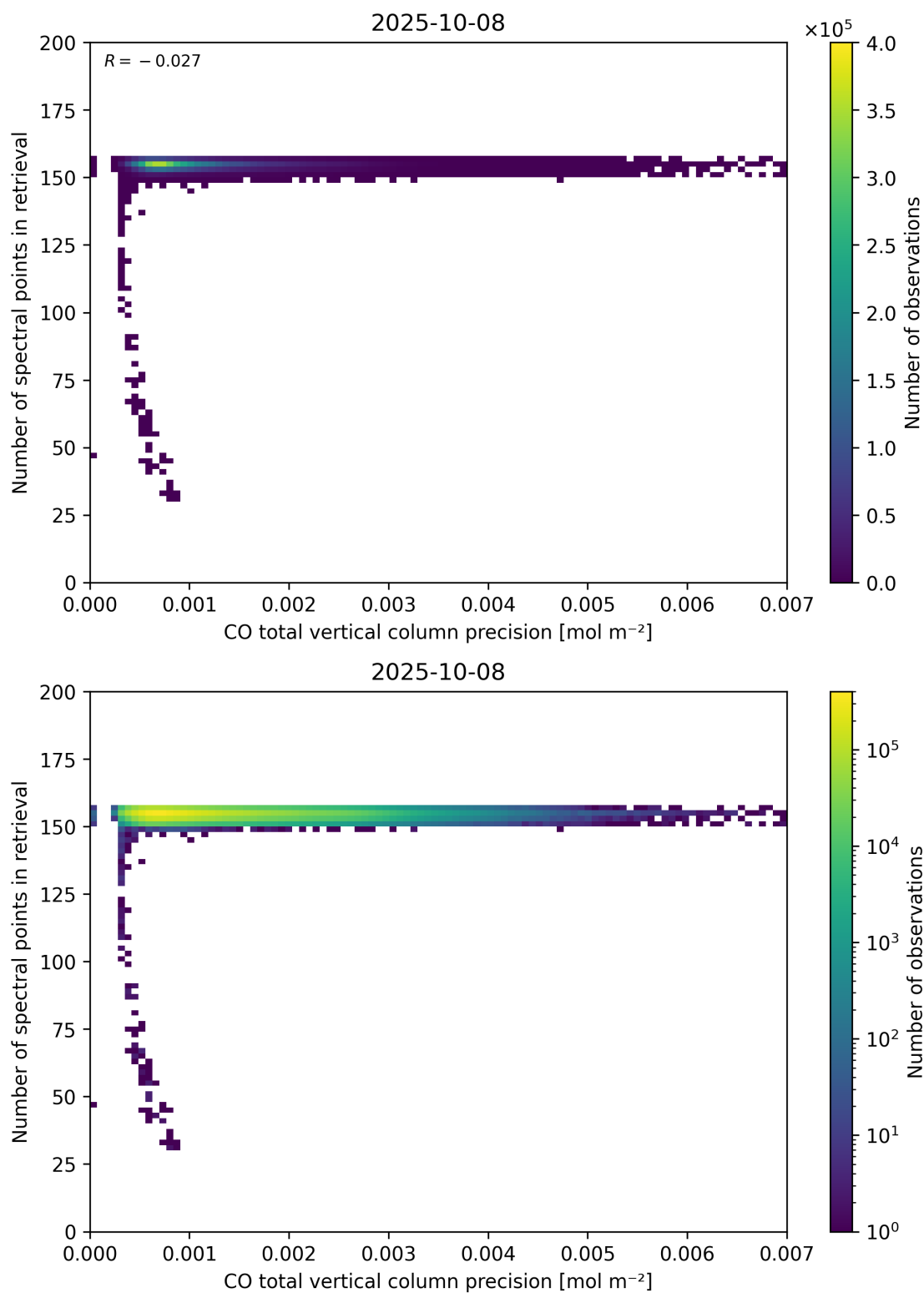
Figure 47: Scatter density plot of “CO total vertical column precision” against “Number of spectral points in retrieval” for 2025-10-07 to 2025-10-09.
