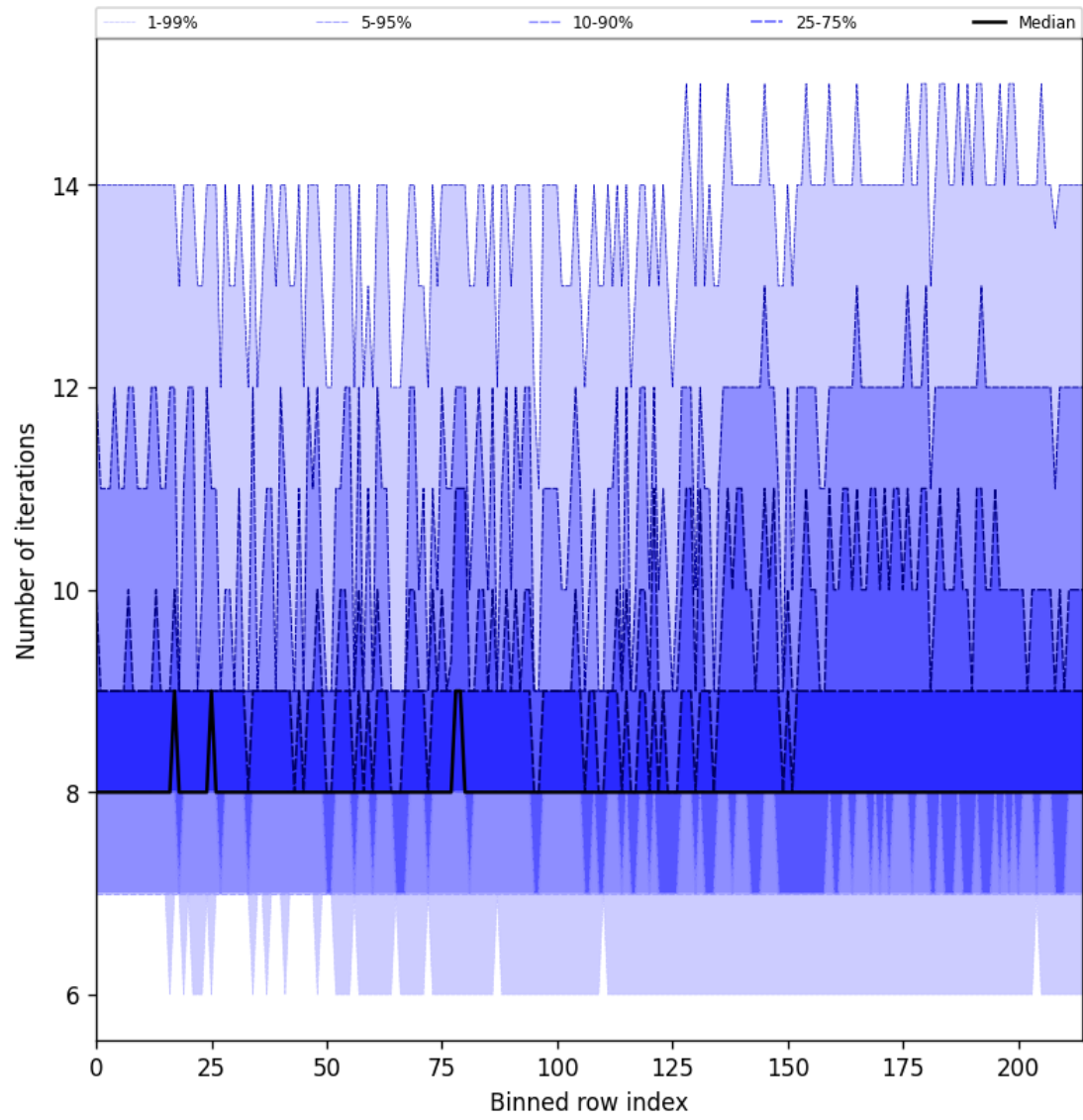
Figure 32: Along track statistics of “Number of iterations” for 2025-10-07 to 2025-10-09
