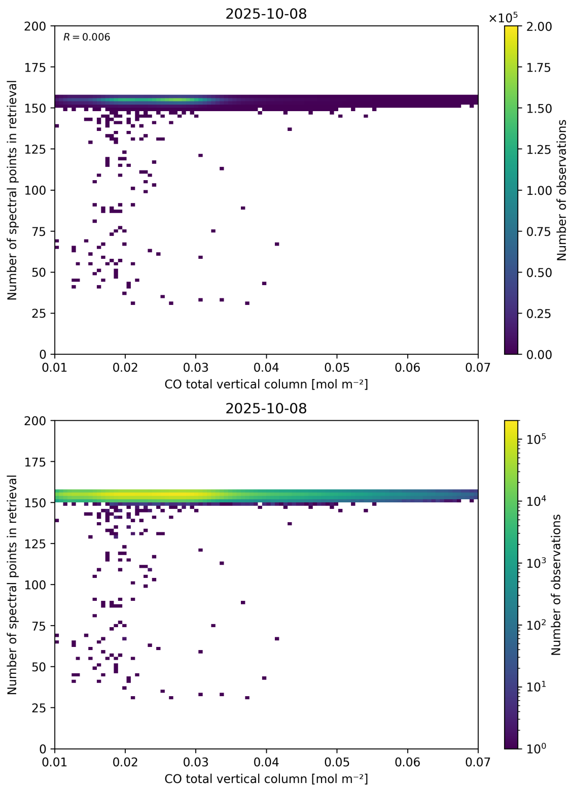
Figure 43: Scatter density plot of “CO total vertical column” against “Number of spectral points in retrieval” for 2025-10-07 to 2025-10-09.
