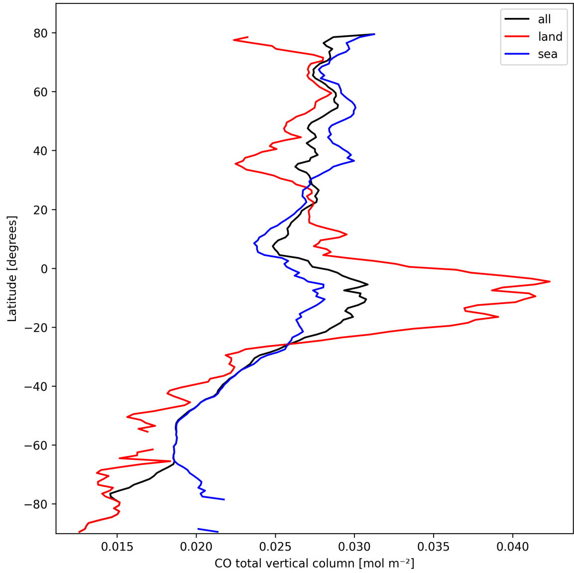
Figure 10: Zonal average of “CO total vertical column” for 2025-10-07 to 2025-10-09.
