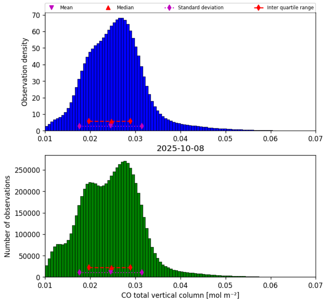
Figure 18: Histogram of “CO total vertical column” for 2025-10-07 to 2025-10-09
