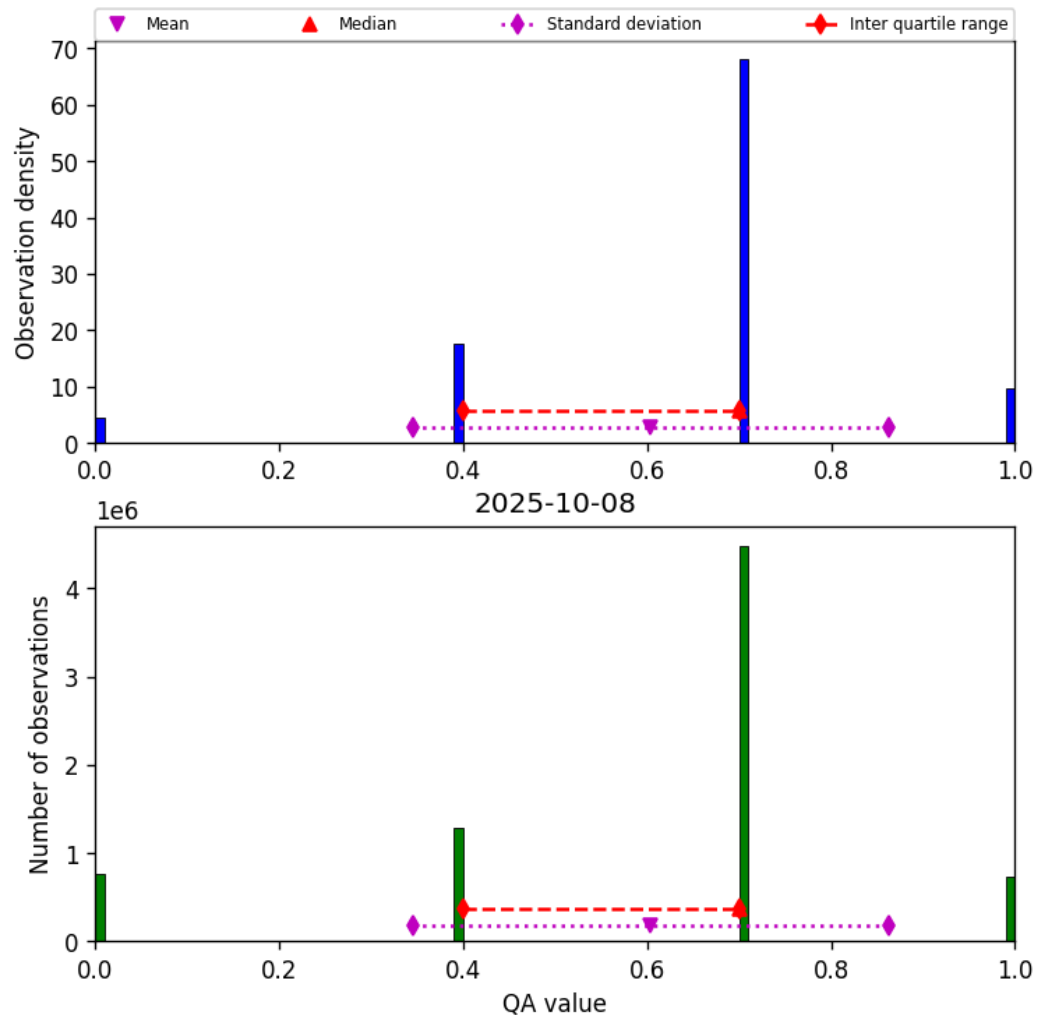
Figure 17: Histogram of “QA value” for 2025-10-07 to 2025-10-09
