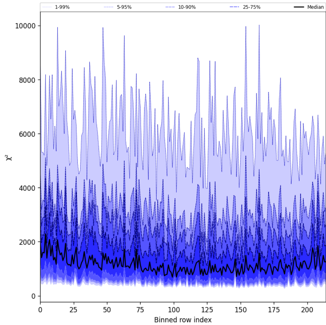
Figure 30: Along track statistics of “ \chi^2 ” for 2025-10-07 to 2025-10-09
