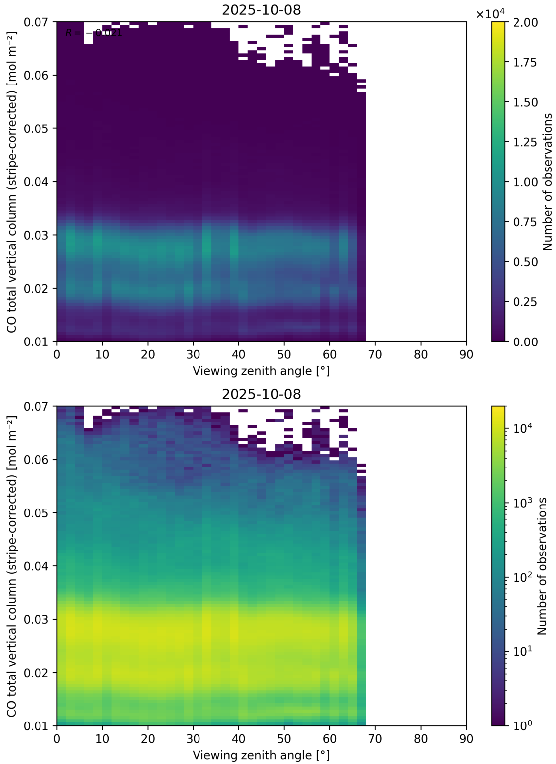
Figure 70: Scatter density plot of “Viewing zenith angle” against “CO total vertical column (stripe-corrected)” for 2025-10-07 to 2025-10-09.
