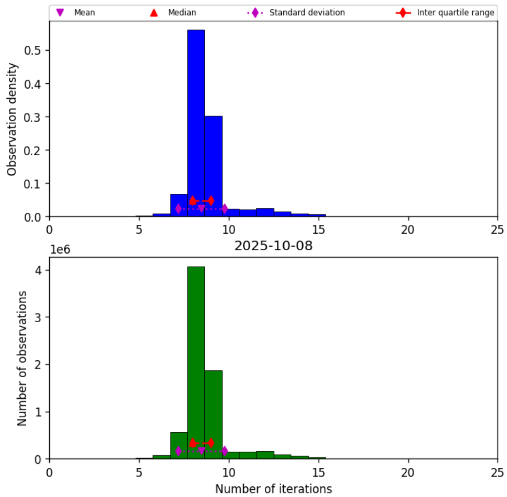
Figure 24: Histogram of “Number of iterations” for 2025-10-07 to 2025-10-09
