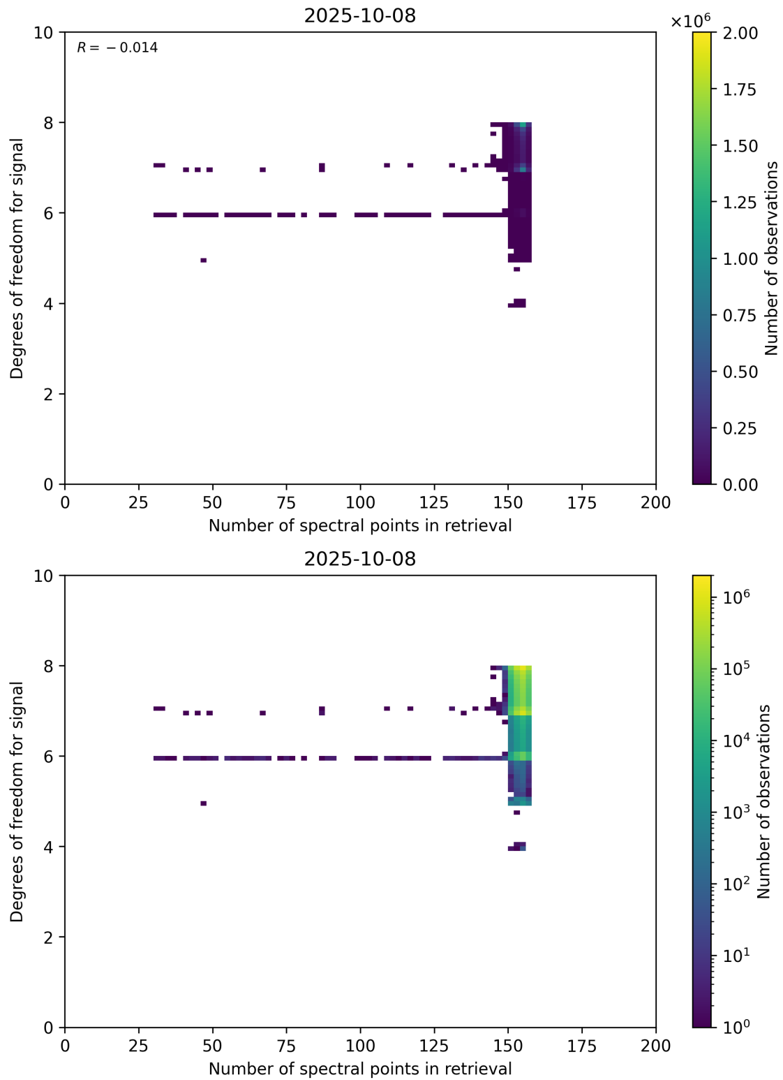
Figure 59: Scatter density plot of “Number of spectral points in retrieval” against “Degrees of freedom for signal” for 2025-10-07 to 2025-10-09.
