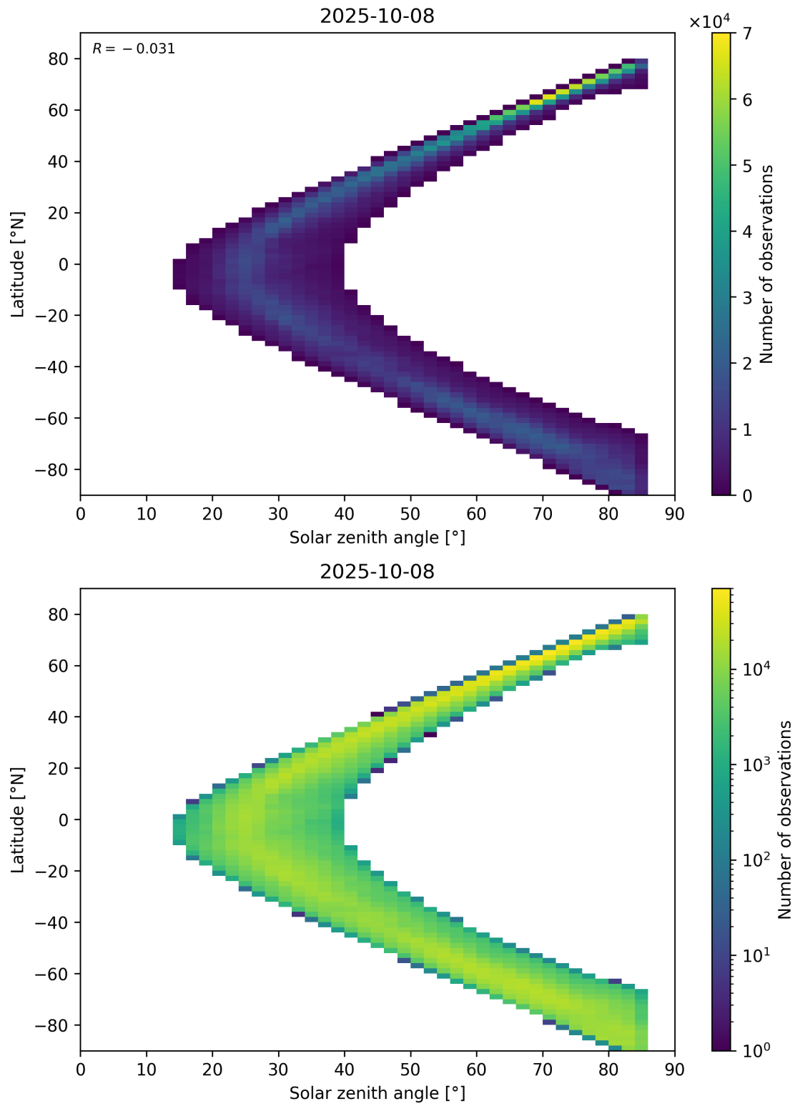
Figure 66: Scatter density plot of “Solar zenith angle” against “Latitude” for 2025-10-07 to 2025-10-09.
