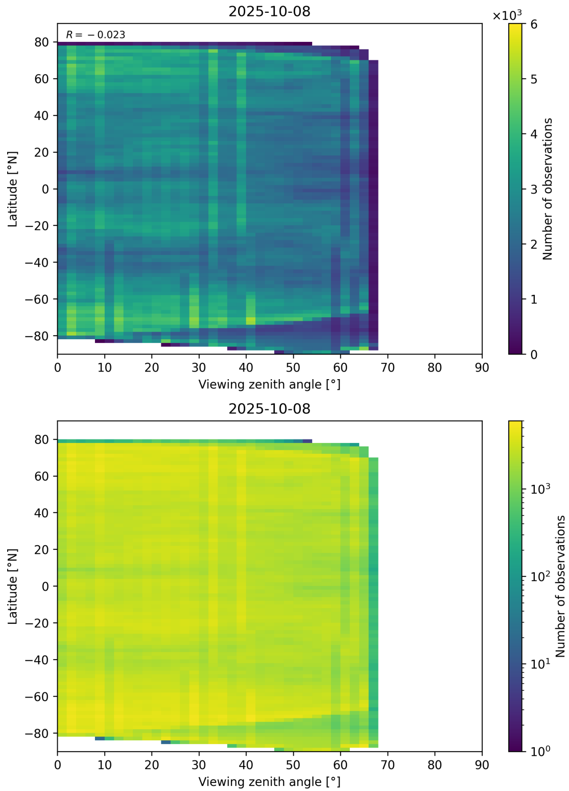
Figure 74: Scatter density plot of “Viewing zenith angle” against “Latitude” for 2025-10-07 to 2025-10-09.
