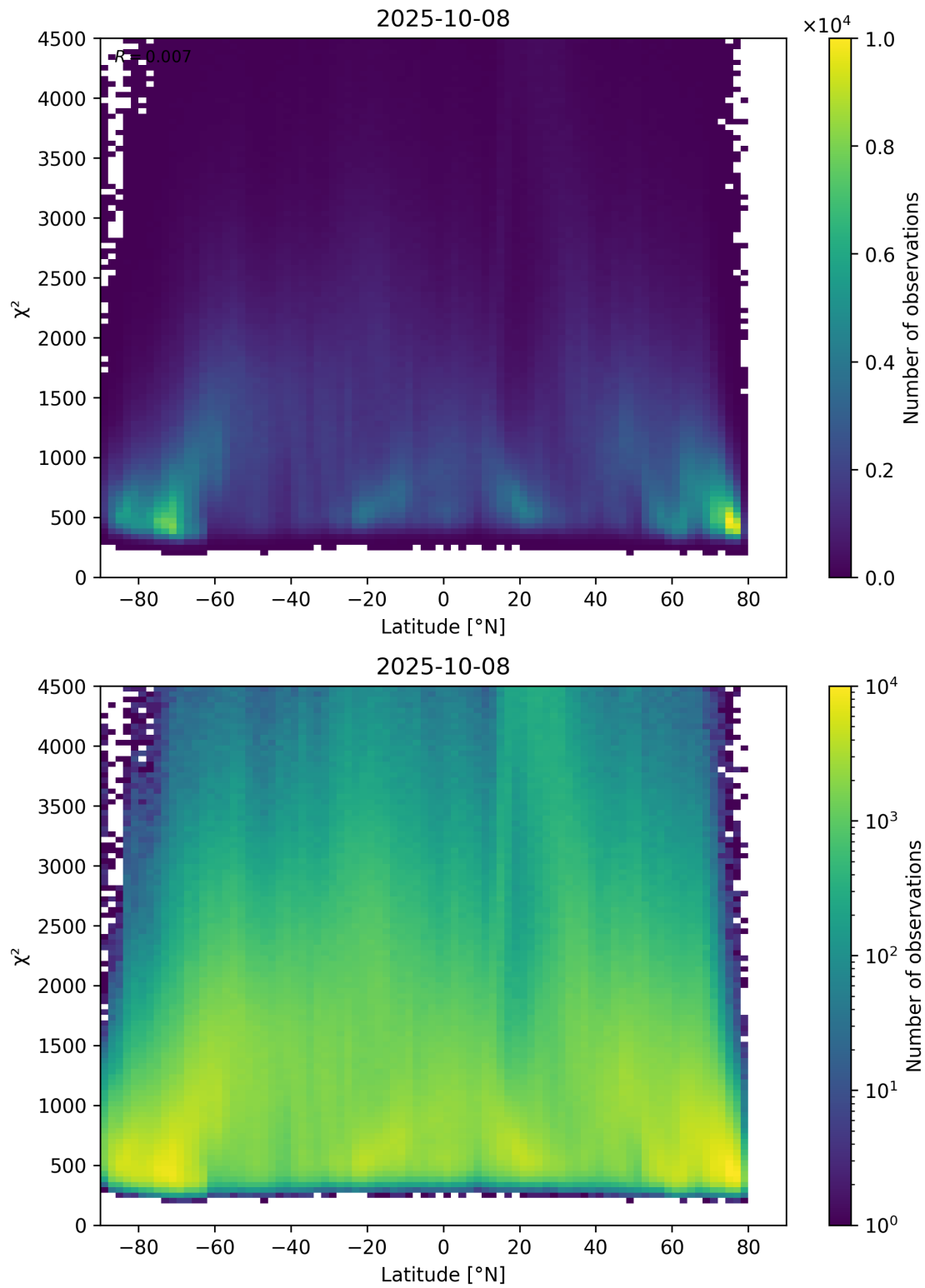
Figure 54: Scatter density plot of “Latitude” against “ \chi^2 ” for 2025-10-07 to 2025-10-09.
