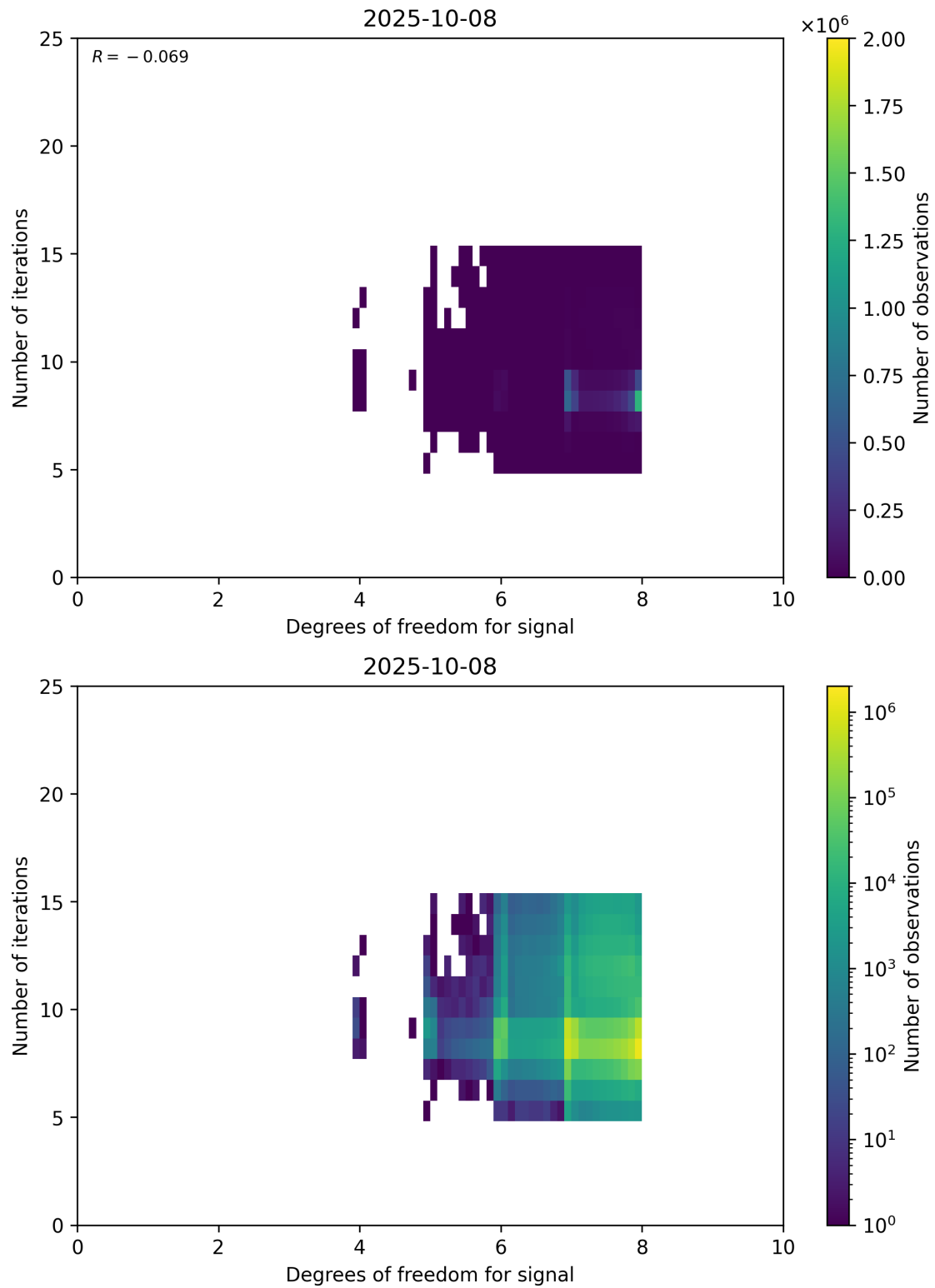
Figure 50: Scatter density plot of “Degrees of freedom for signal” against “Number of iterations” for 2025-10-07 to 2025-10-09.
