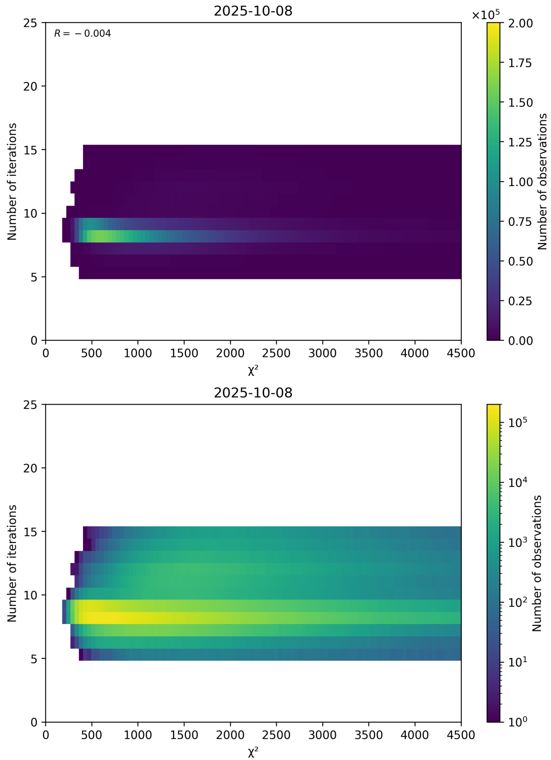
Figure 49: Scatter density plot of “ \chi^2 ” against “Number of iterations” for 2025-10-07 to 2025-10-09.
