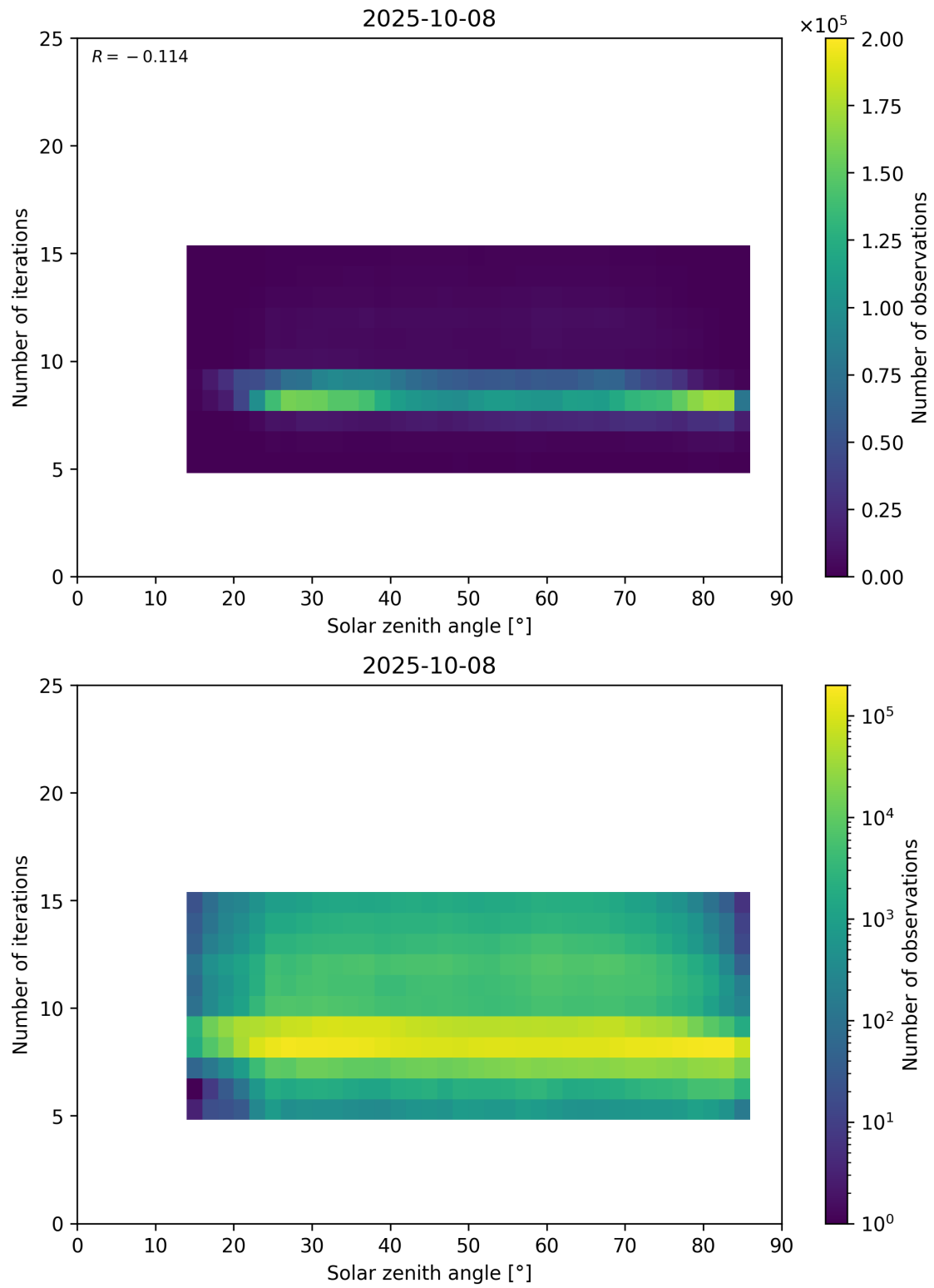
Figure 67: Scatter density plot of “Solar zenith angle” against “Number of iterations” for 2025-10-07 to 2025-10-09.
