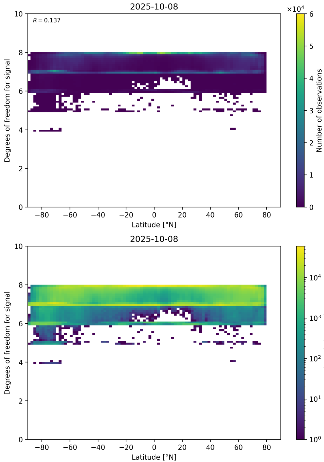
Figure 55: Scatter density plot of “Latitude” against “Degrees of freedom for signal” for 2025-10-07 to 2025-10-09.
