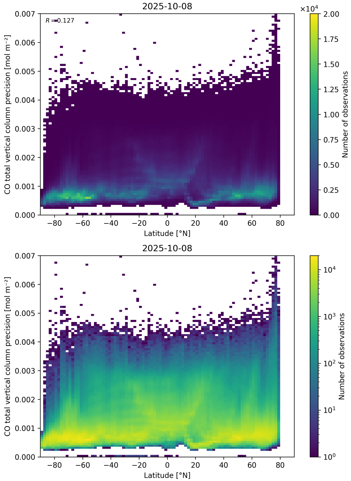
Figure 53: Scatter density plot of “Latitude” against “CO total vertical column precision” for 2025-10-07 to 2025-10-09.
