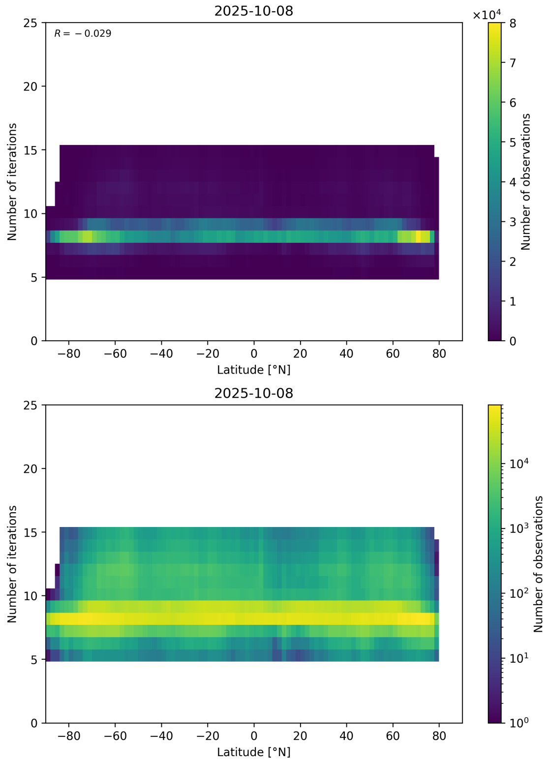
Figure 56: Scatter density plot of “Latitude” against “Number of iterations” for 2025-10-07 to 2025-10-09.
