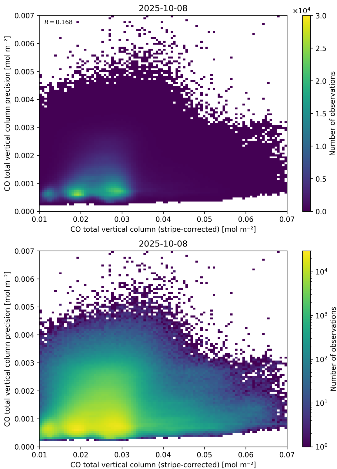
Figure 36: Scatter density plot of “CO total vertical column (stripe-corrected)” against “CO total vertical column precision” for 2025-10-07 to 2025-10-09.
