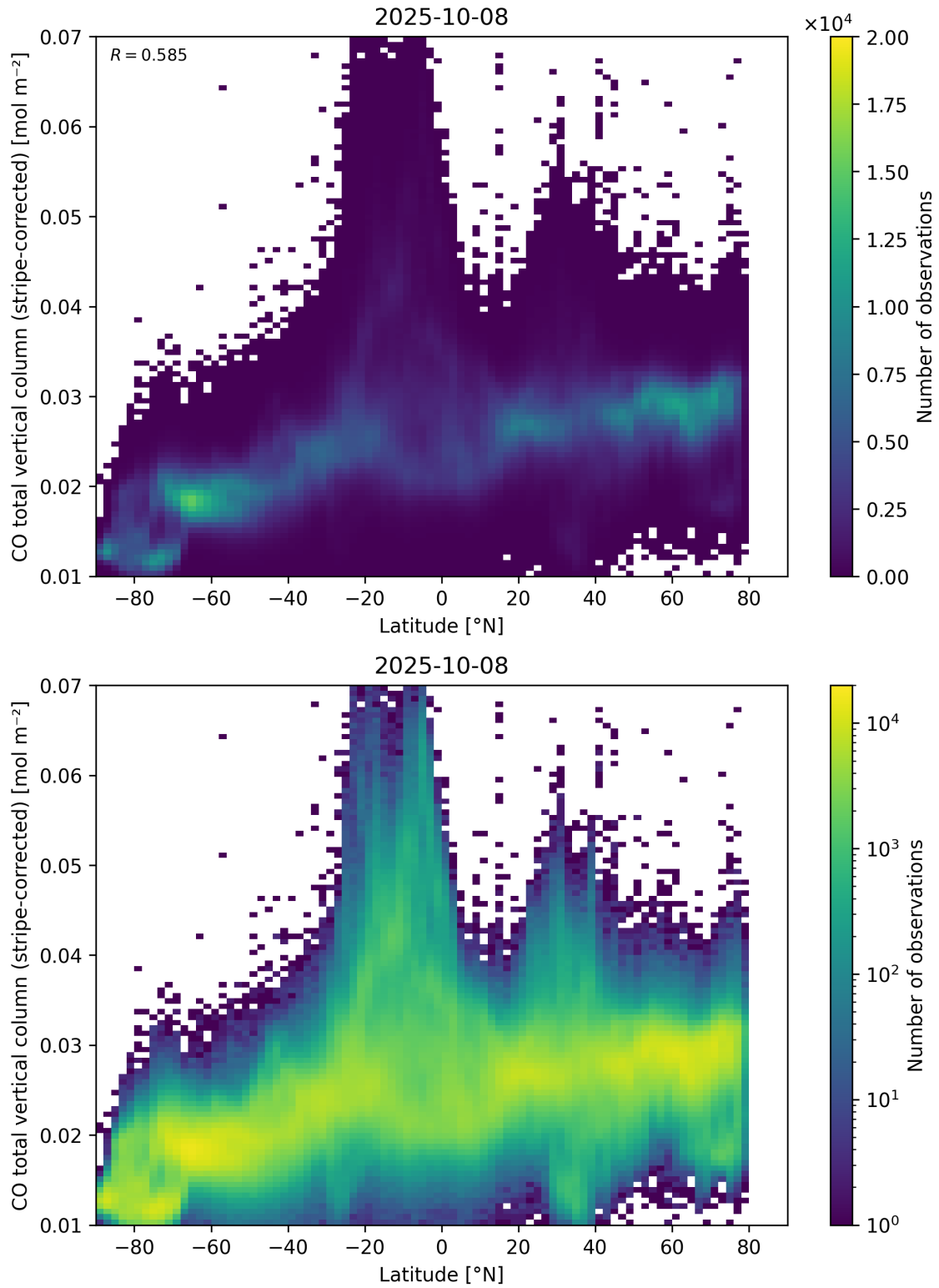
Figure 52: Scatter density plot of “Latitude” against “CO total vertical column (stripe-corrected)” for 2025-10-07 to 2025-10-09.
