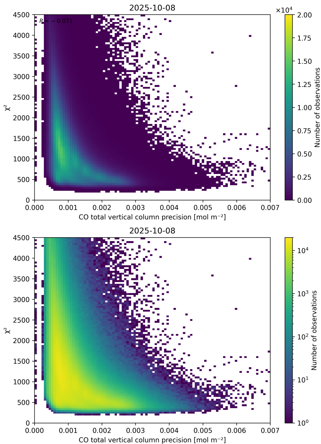
Figure 44: Scatter density plot of “CO total vertical column precision” against “ \chi^2 ” for 2025-10-07 to 2025-10-09.
