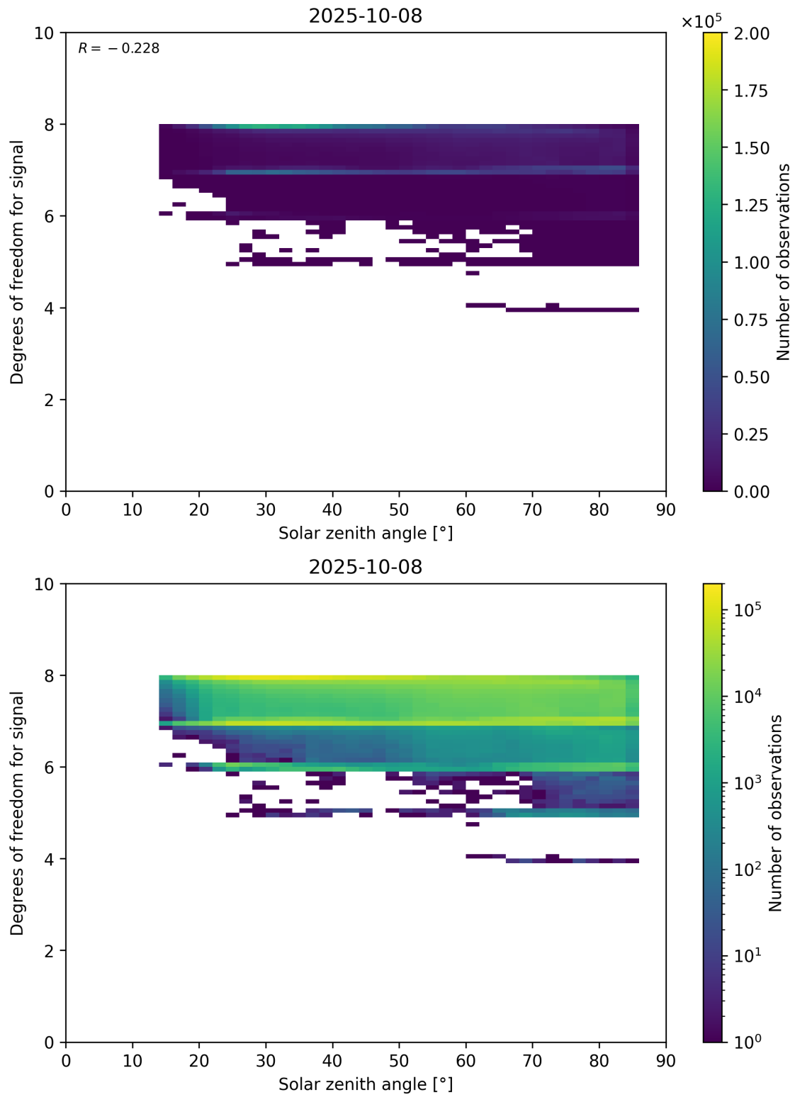
Figure 65: Scatter density plot of “Solar zenith angle” against “Degrees of freedom for signal” for 2025-10-07 to 2025-10-09.
