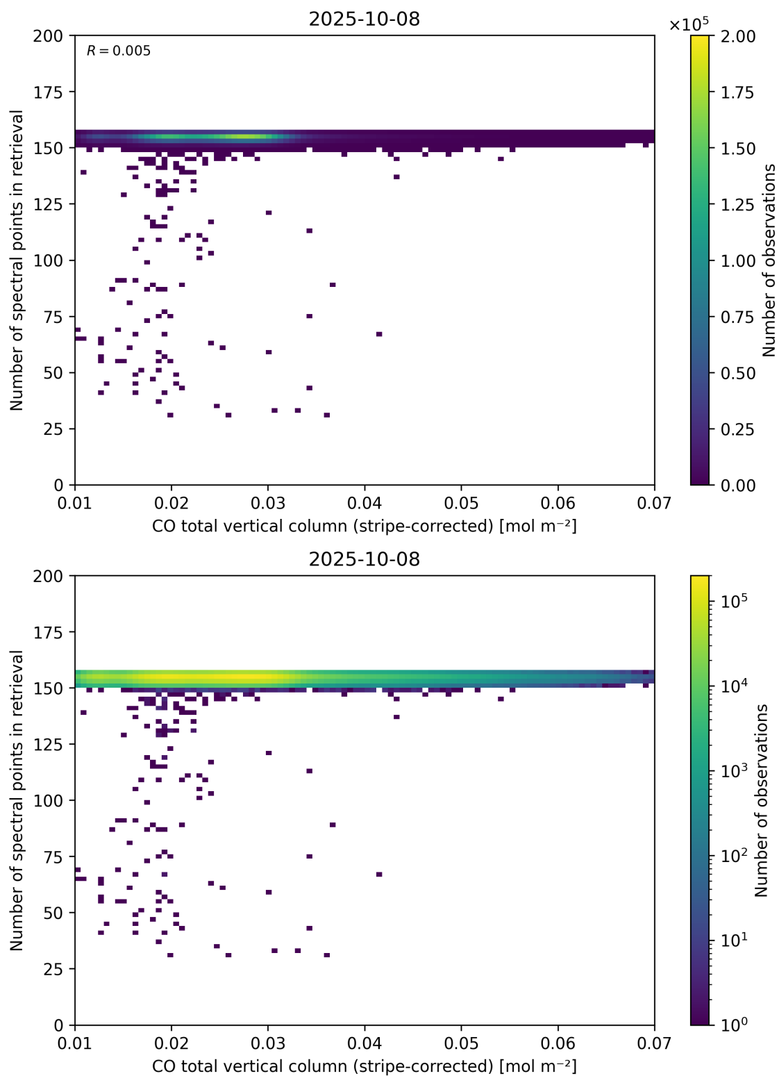
Figure 40: Scatter density plot of “CO total vertical column (stripe-corrected)” against “Number of spectral points in retrieval” for 2025-10-07 to 2025-10-09.
