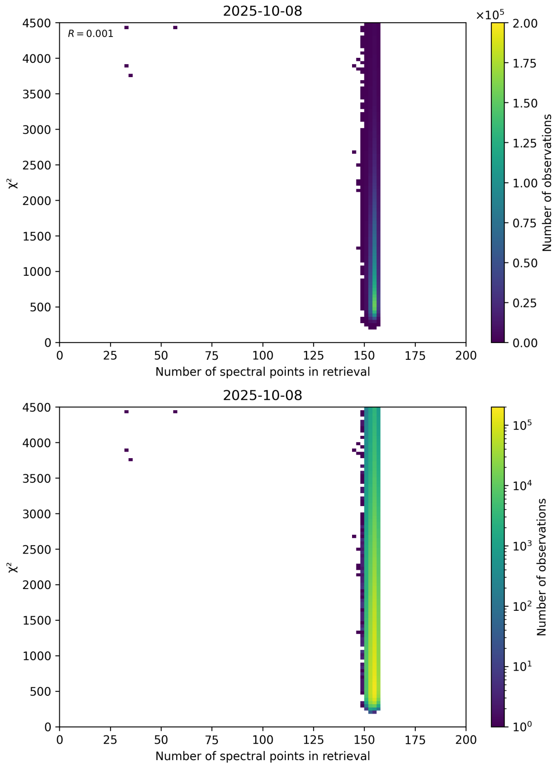
Figure 58: Scatter density plot of “Number of spectral points in retrieval” against “ \chi^2 ” for 2025-10-07 to 2025-10-09.
