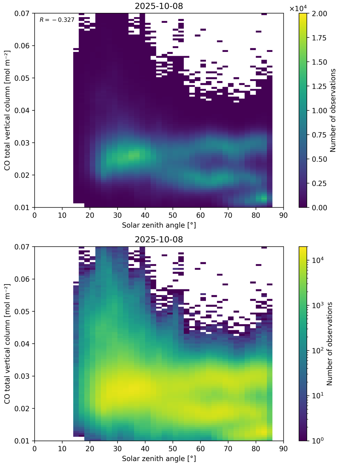
Figure 61: Scatter density plot of “Solar zenith angle” against “CO total vertical column” for 2025-10-07 to 2025-10-09.
