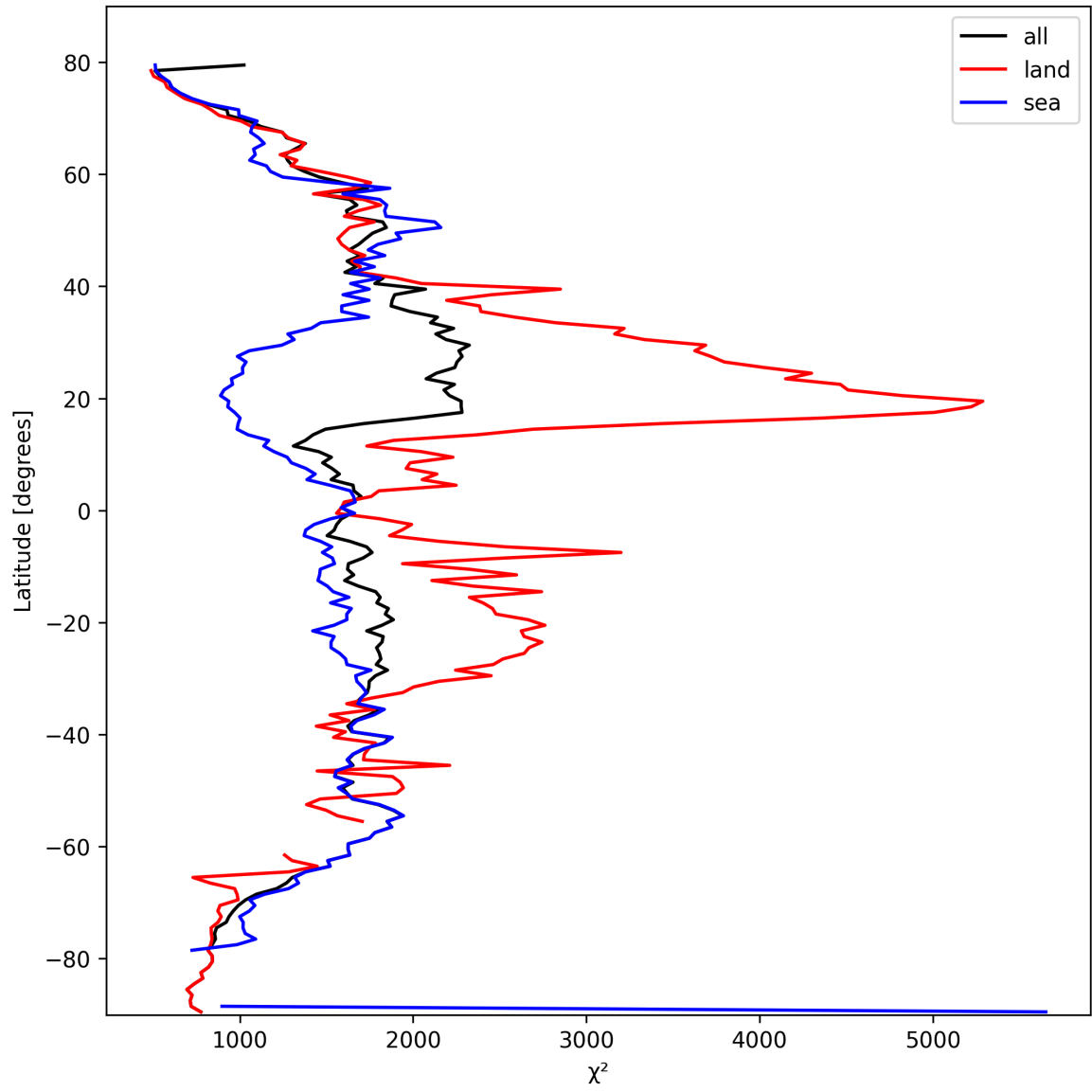
Figure 14: Zonal average of “ \chi^2 ” for 2025-10-07 to 2025-10-09.
