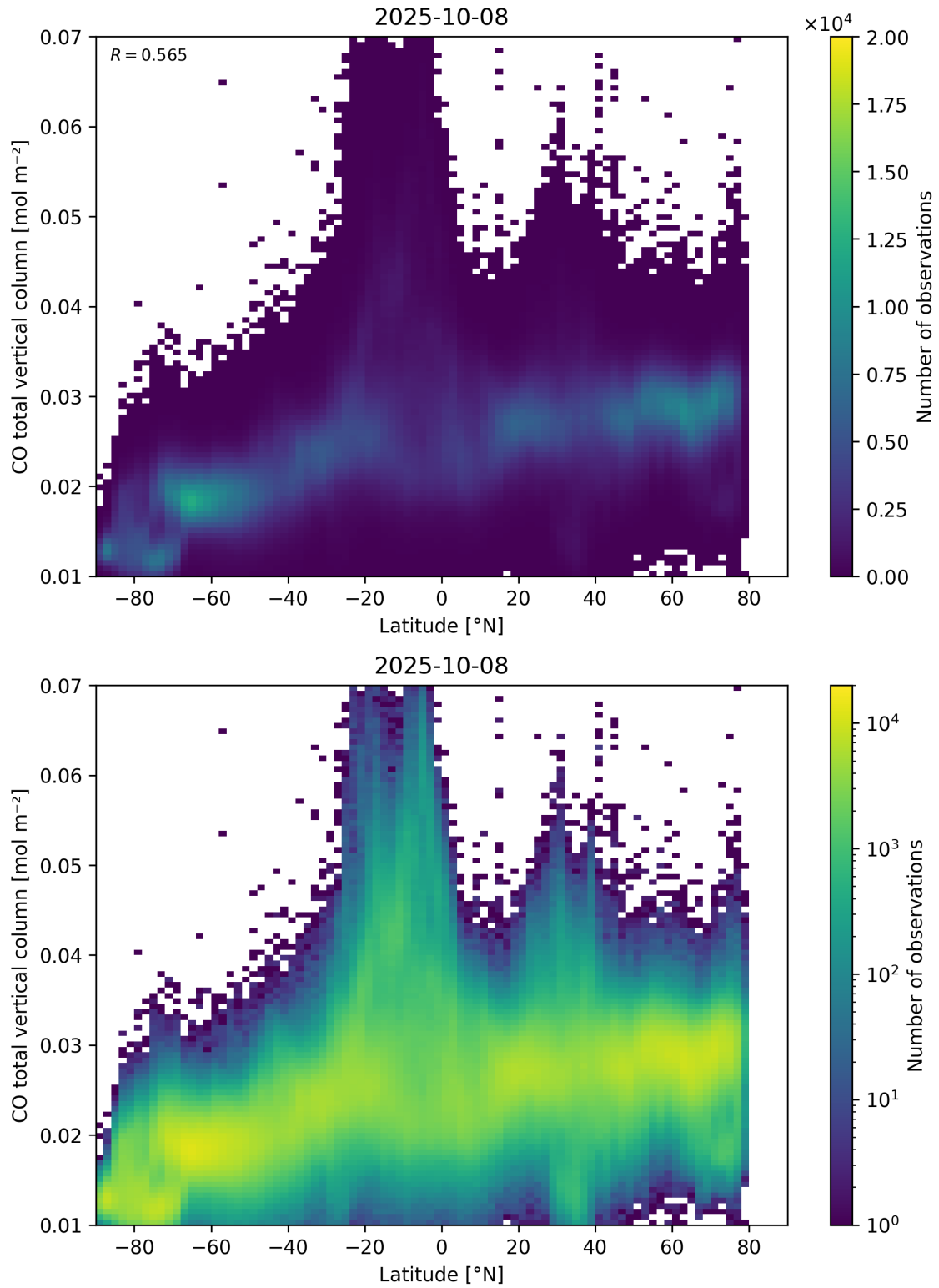
Figure 51: Scatter density plot of “Latitude” against “CO total vertical column” for 2025-10-07 to 2025-10-09.
