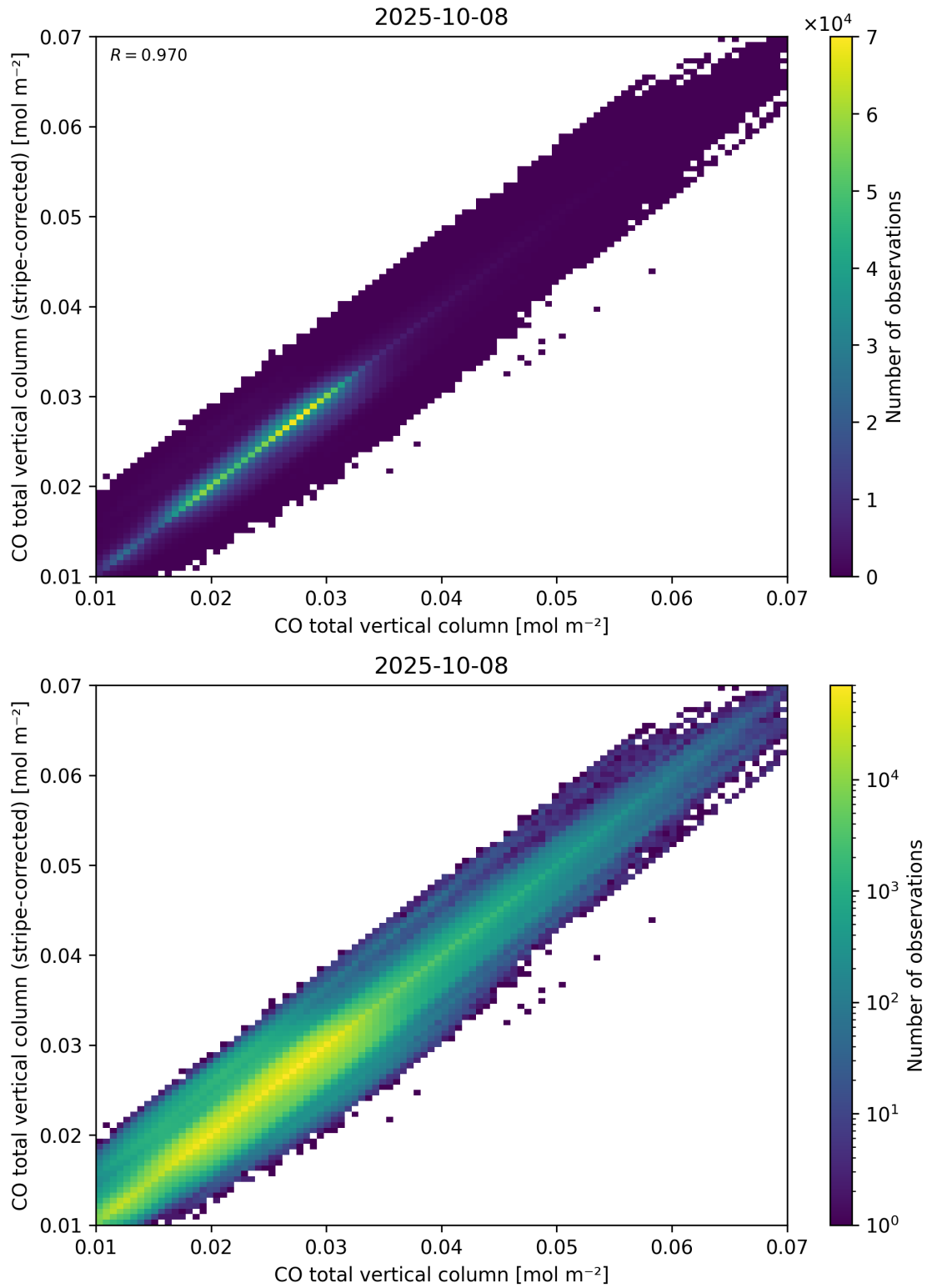
Figure 33: Scatter density plot of “CO total vertical column” against “CO total vertical column (stripe-corrected)” for 2025-10-07 to 2025-10-09.
