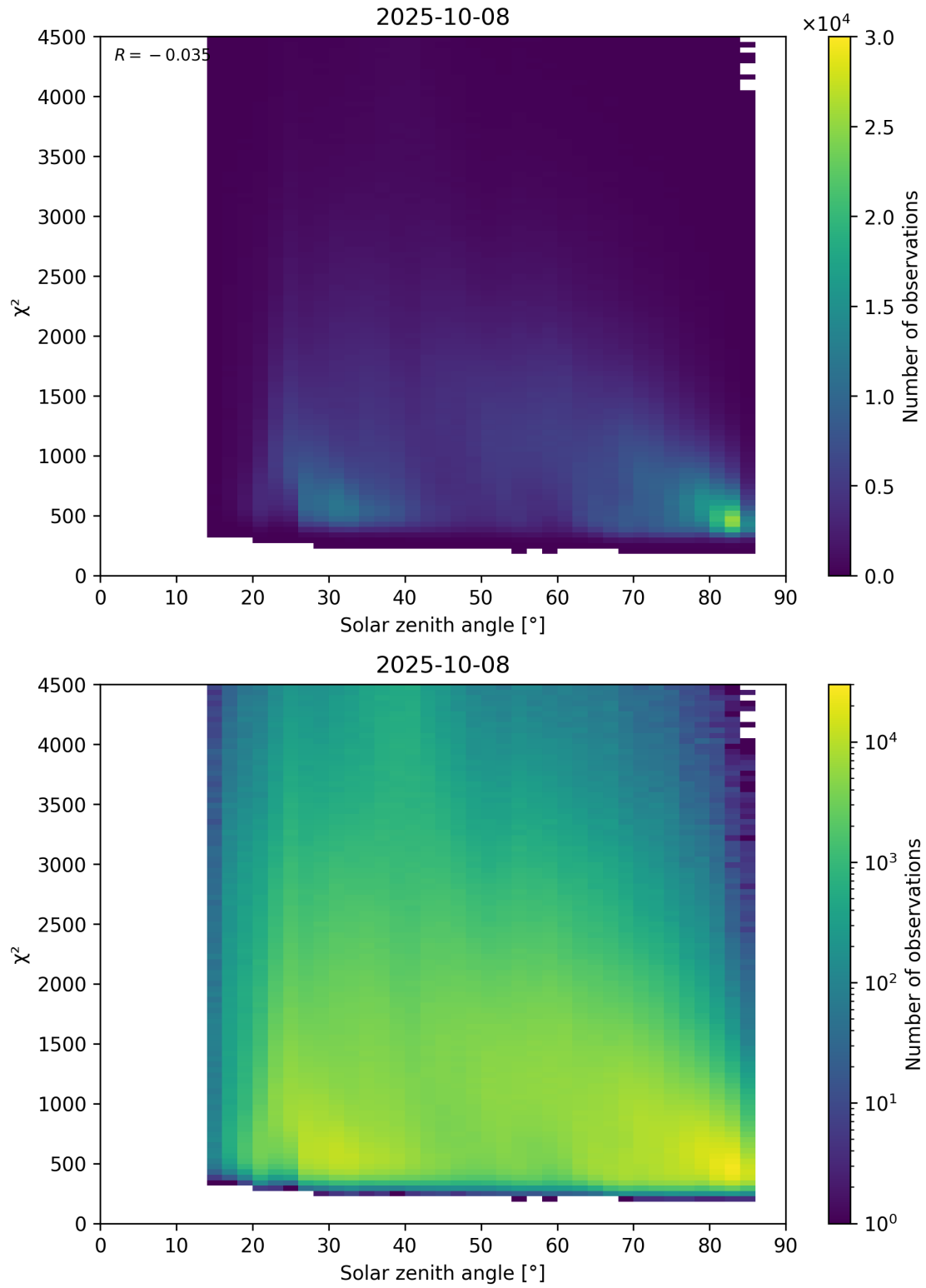
Figure 64: Scatter density plot of “Solar zenith angle” against “ \chi^2 ” for 2025-10-07 to 2025-10-09.
