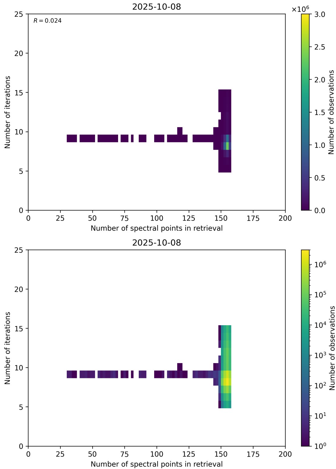
Figure 60: Scatter density plot of “Number of spectral points in retrieval” against “Number of iterations” for 2025-10-07 to 2025-10-09.
