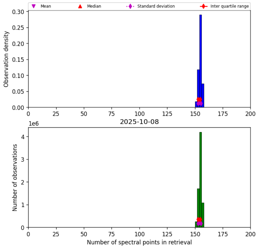
Figure 21: Histogram of “Number of spectral points in retrieval” for 2025-10-07 to 2025-10-09
