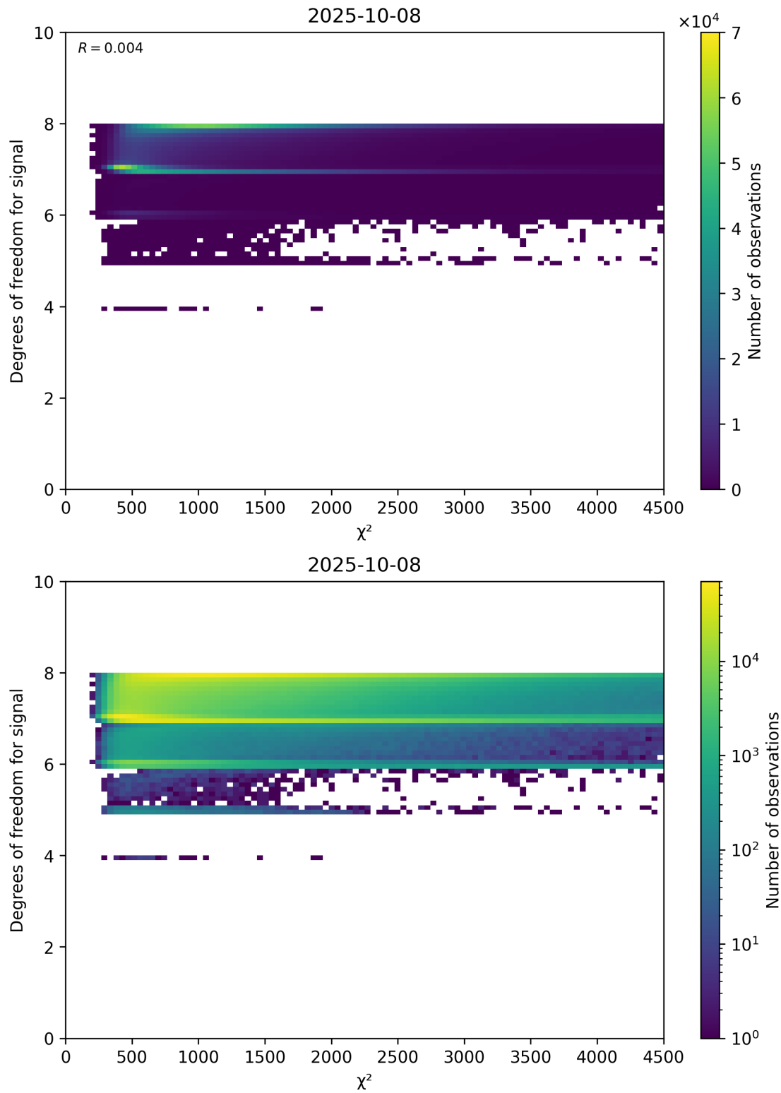
Figure 48: Scatter density plot of “ \chi^2 ” against “Degrees of freedom for signal” for 2025-10-07 to 2025-10-09.
