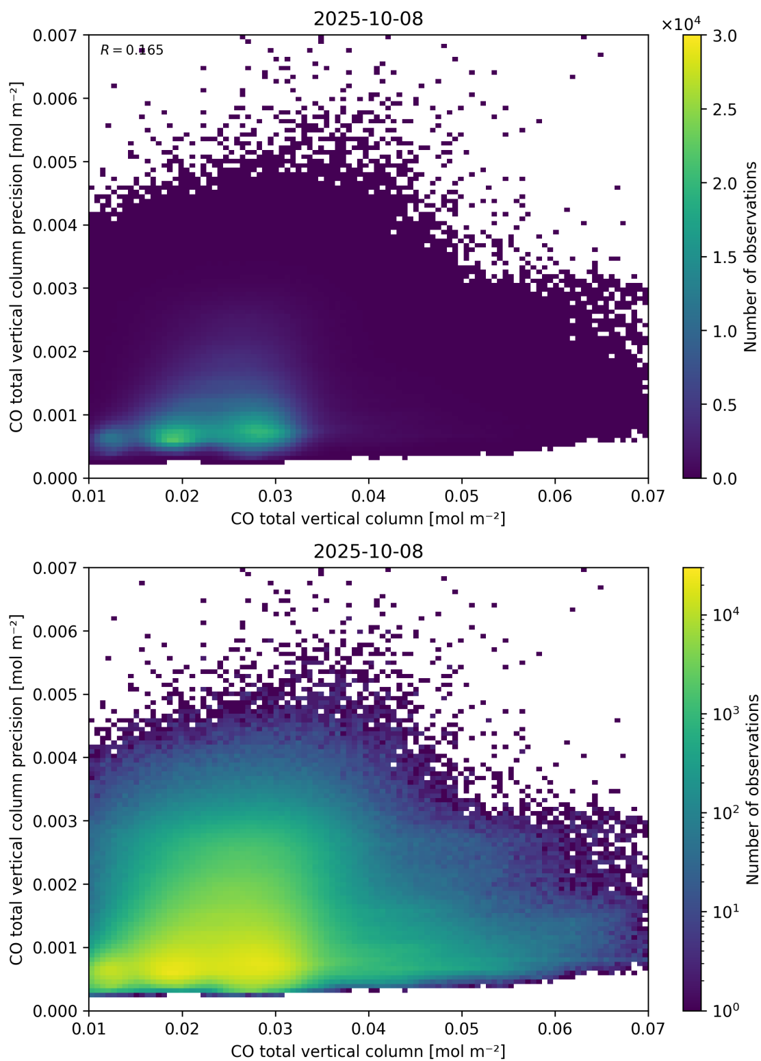
Figure 34: Scatter density plot of “CO total vertical column” against “CO total vertical column precision” for 2025-10-07 to 2025-10-09.
