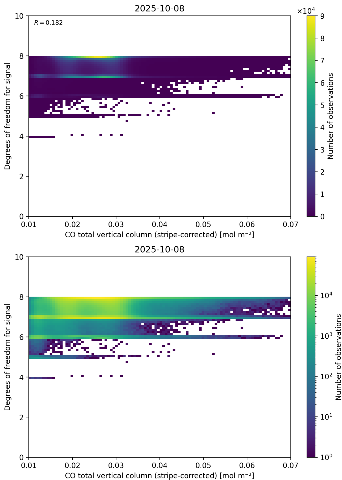
Figure 38: Scatter density plot of “CO total vertical column (stripe-corrected)” against “Degrees of freedom for signal” for 2025-10-07 to 2025-10-09.
