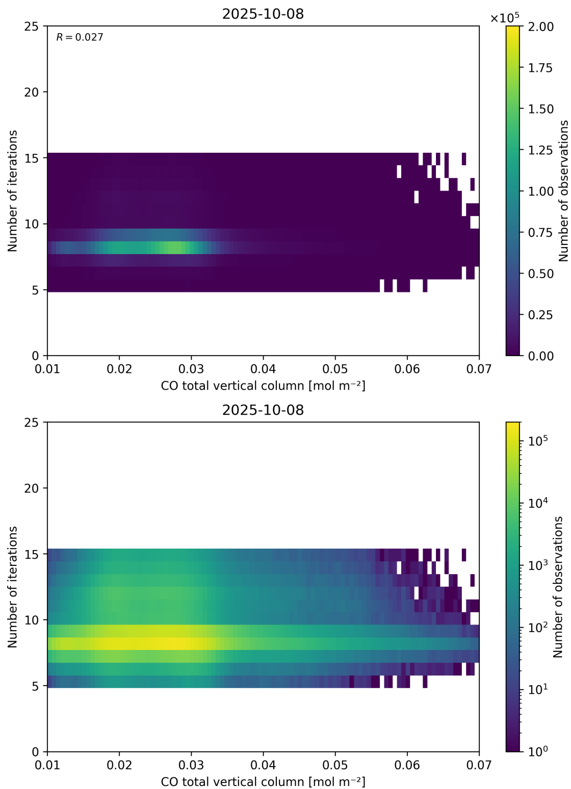
Figure 42: Scatter density plot of “CO total vertical column” against “Number of iterations” for 2025-10-07 to 2025-10-09.
