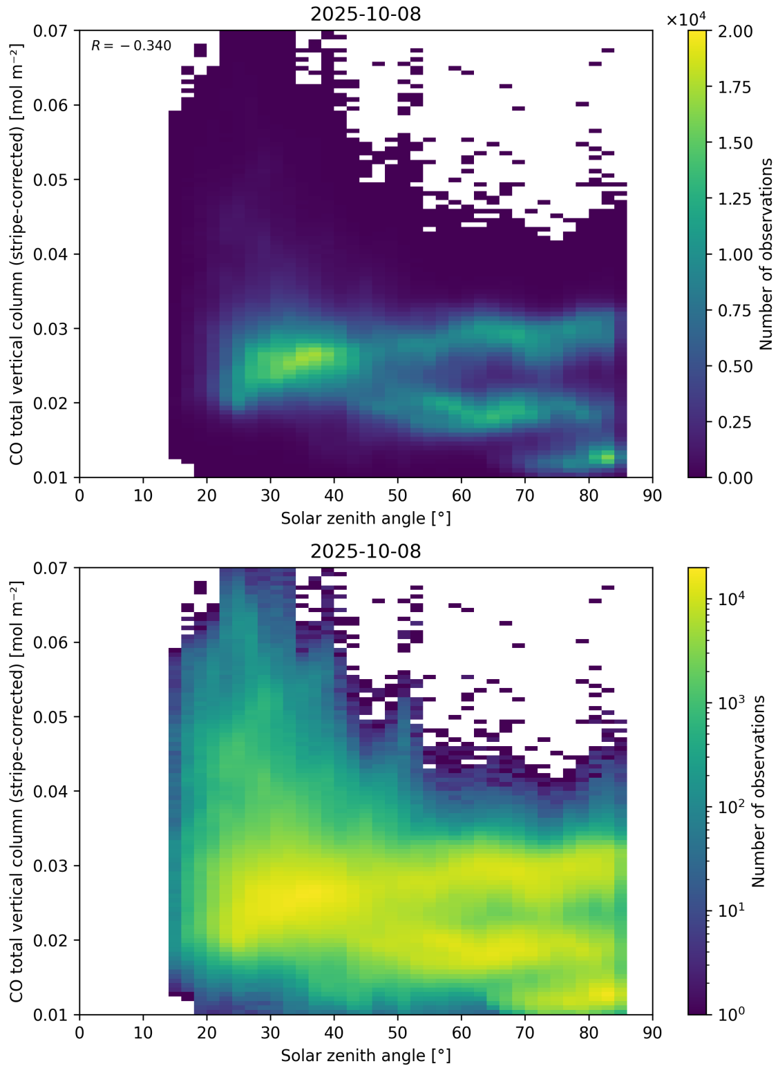
Figure 62: Scatter density plot of “Solar zenith angle” against “CO total vertical column (stripe-corrected)” for 2025-10-07 to 2025-10-09.
