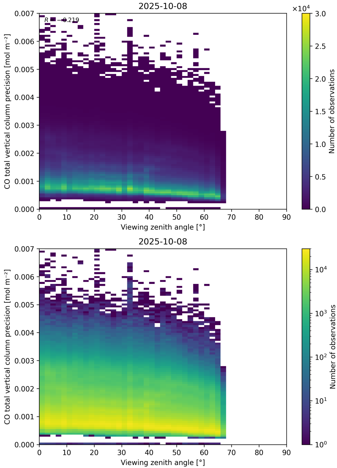
Figure 71: Scatter density plot of “Viewing zenith angle” against “CO total vertical column precision” for 2025-10-07 to 2025-10-09.
