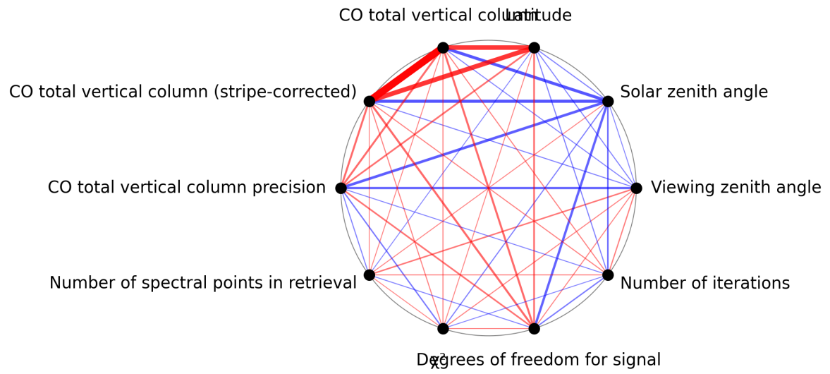
Figure 1: Map of correlation graph for 2025-10-07 to 2025-10-09.
