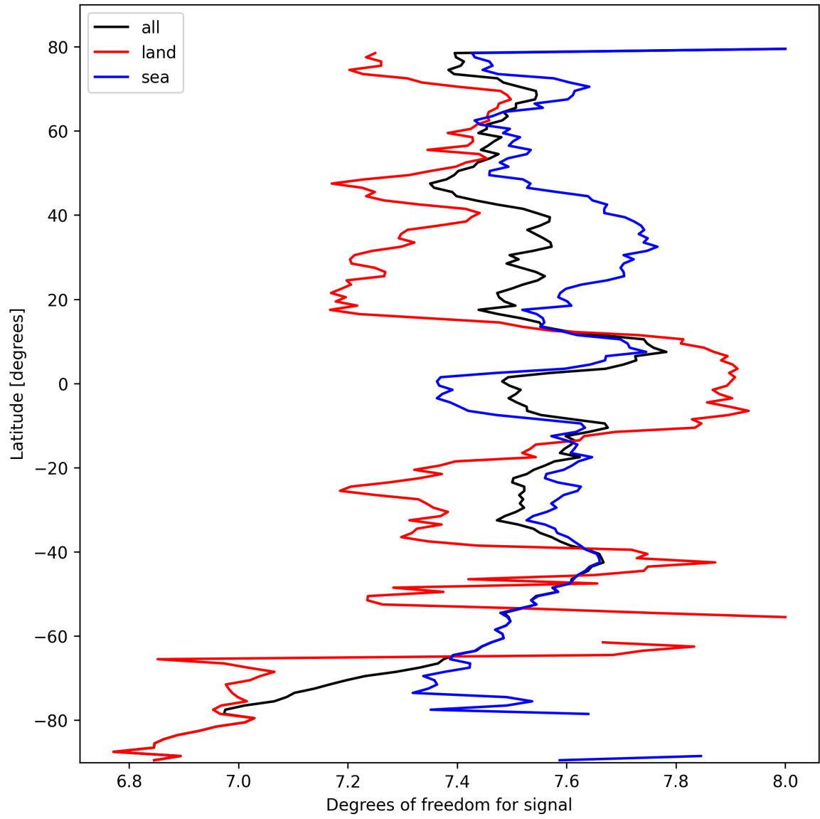
Figure 15: Zonal average of “Degrees of freedom for signal” for 2025-10-07 to 2025-10-09.
