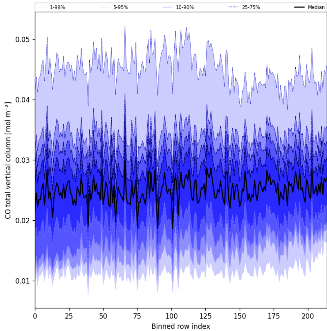
Figure 26: Along track statistics of “CO total vertical column” for 2025-10-07 to 2025-10-09
