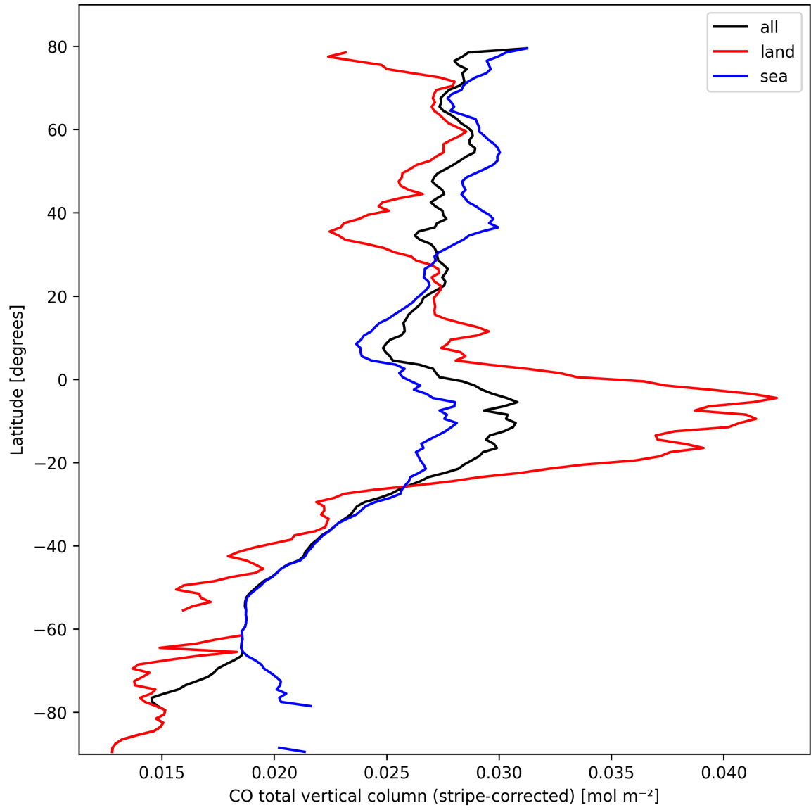
Figure 11: Zonal average of “CO total vertical column (stripe-corrected)” for 2025-10-07 to 2025-10-09.
