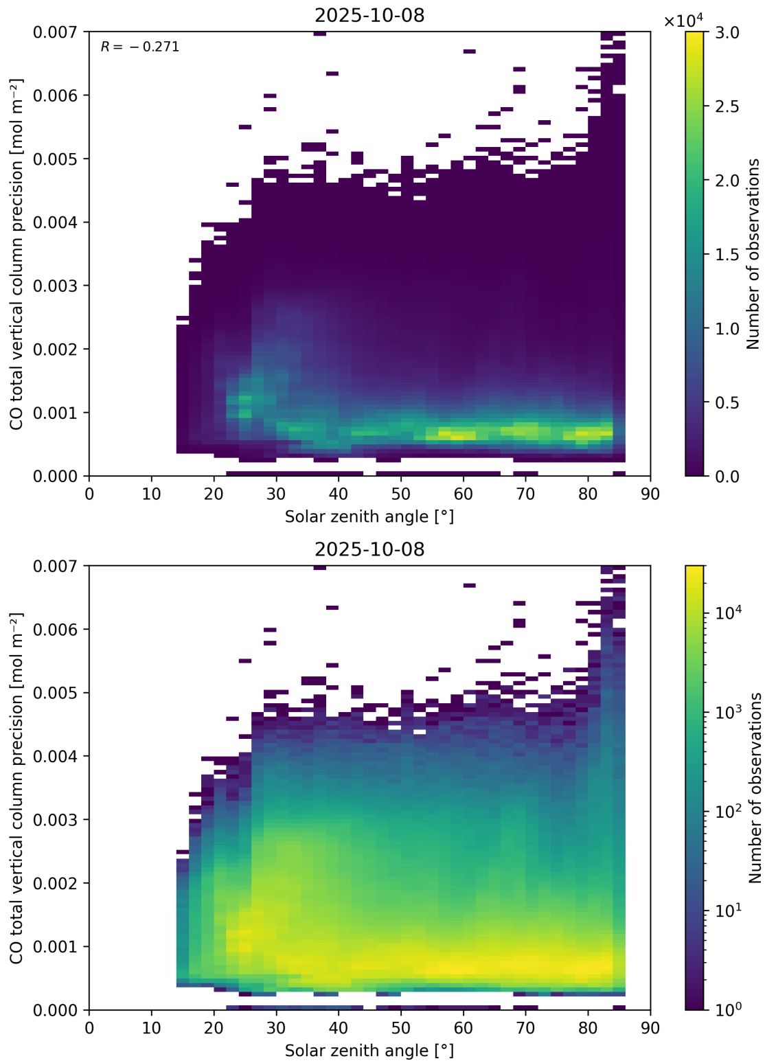
Figure 63: Scatter density plot of “Solar zenith angle” against “CO total vertical column precision” for 2025-10-07 to 2025-10-09.
