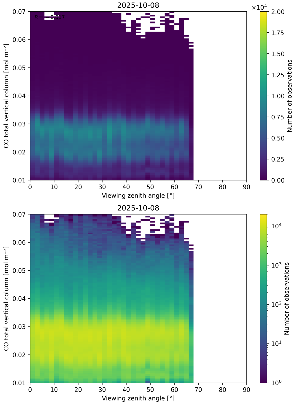
Figure 69: Scatter density plot of “Viewing zenith angle” against “CO total vertical column” for 2025-10-07 to 2025-10-09.
