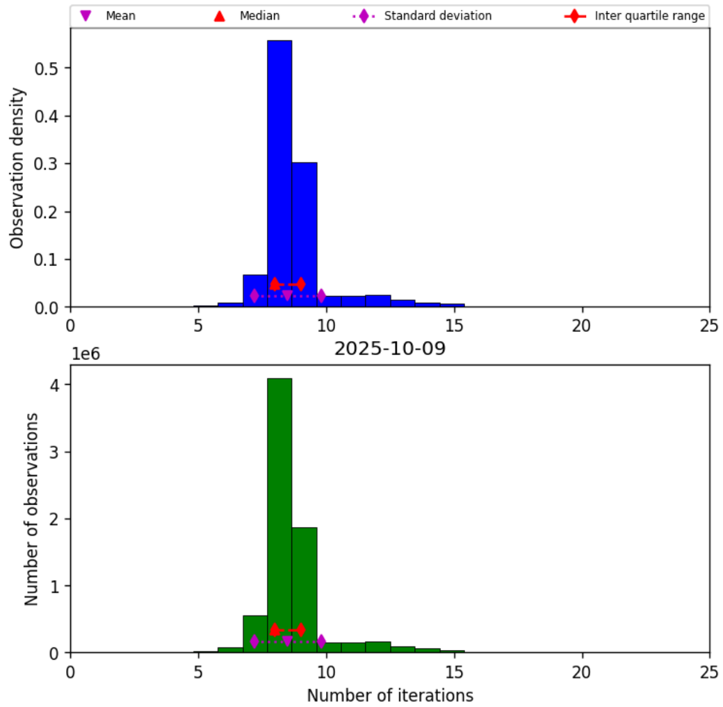
Figure 24: Histogram of “Number of iterations” for 2025-10-08 to 2025-10-10
