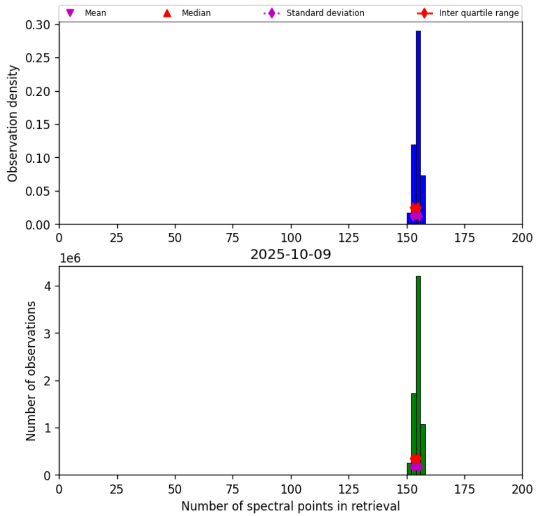
Figure 21: Histogram of “Number of spectral points in retrieval” for 2025-10-08 to 2025-10-10
