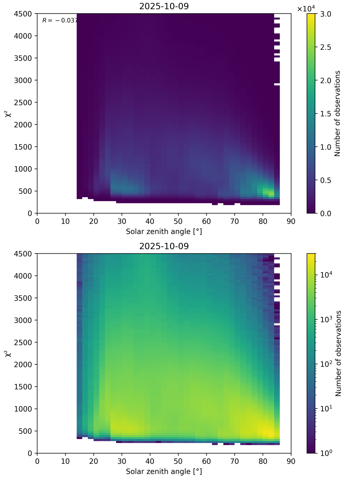
Figure 64: Scatter density plot of “Solar zenith angle” against “ \chi^2 ” for 2025-10-08 to 2025-10-10.
