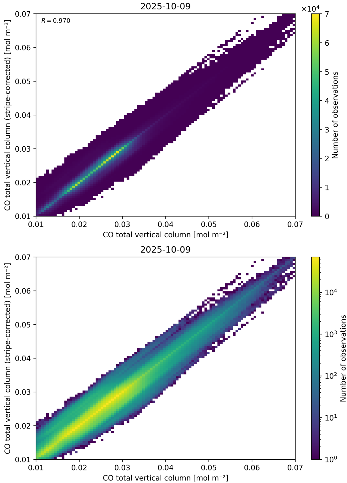
Figure 33: Scatter density plot of “CO total vertical column” against “CO total vertical column (stripe-corrected)” for 2025-10-08 to 2025-10-10.
