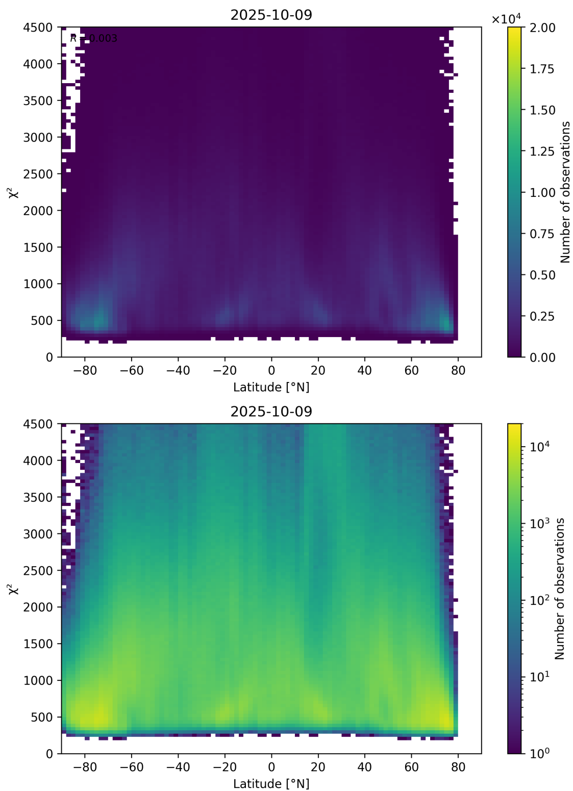
Figure 54: Scatter density plot of “Latitude” against “ \chi^2 ” for 2025-10-08 to 2025-10-10.
