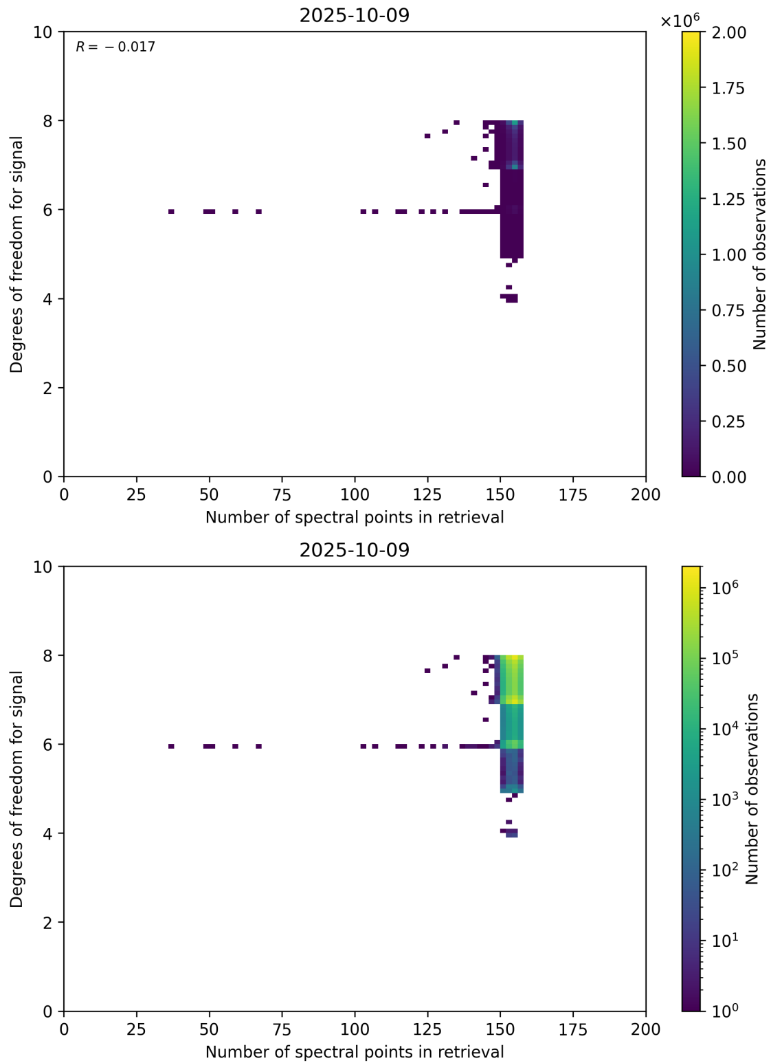
Figure 59: Scatter density plot of “Number of spectral points in retrieval” against “Degrees of freedom for signal” for 2025-10-08 to 2025-10-10.
