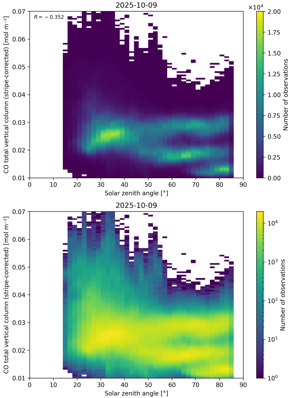
Figure 62: Scatter density plot of “Solar zenith angle” against “CO total vertical column (stripe-corrected)” for 2025-10-08 to 2025-10-10.
