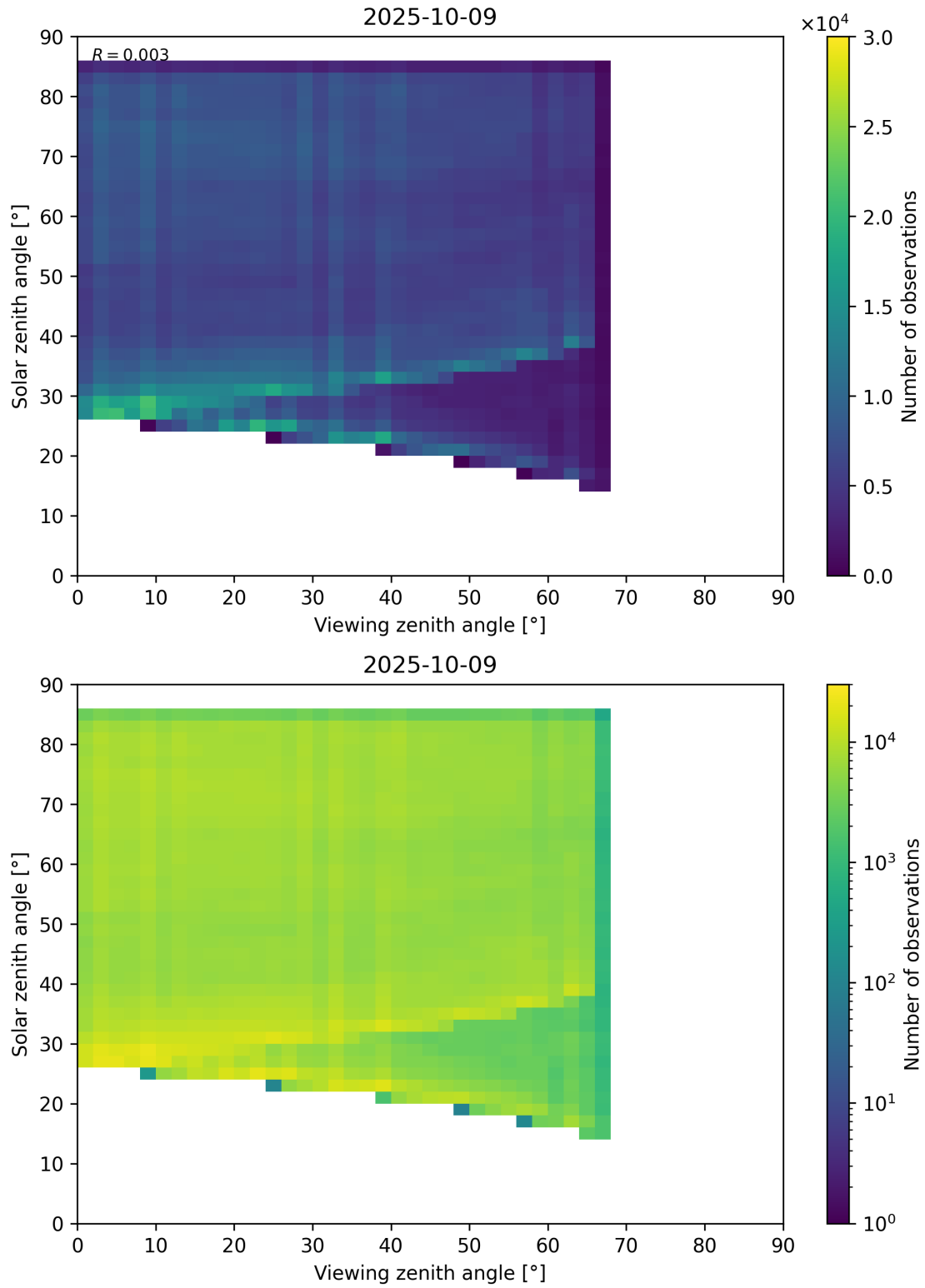
Figure 77: Scatter density plot of “Viewing zenith angle” against “Solar zenith angle” for 2025-10-08 to 2025-10-10.
