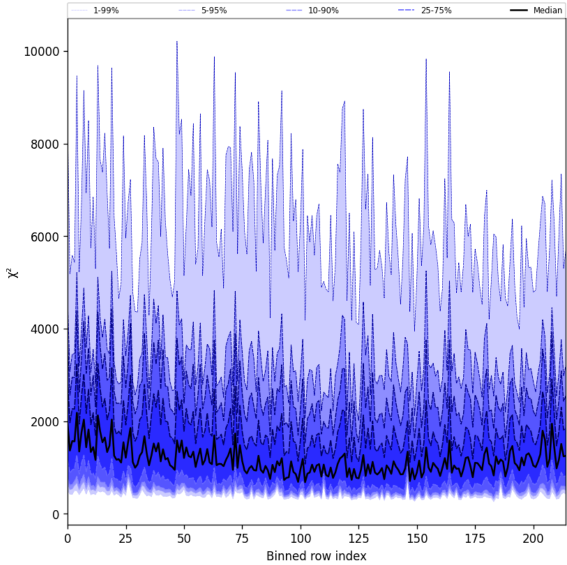
Figure 30: Along track statistics of “ \chi^2 ” for 2025-10-08 to 2025-10-10
