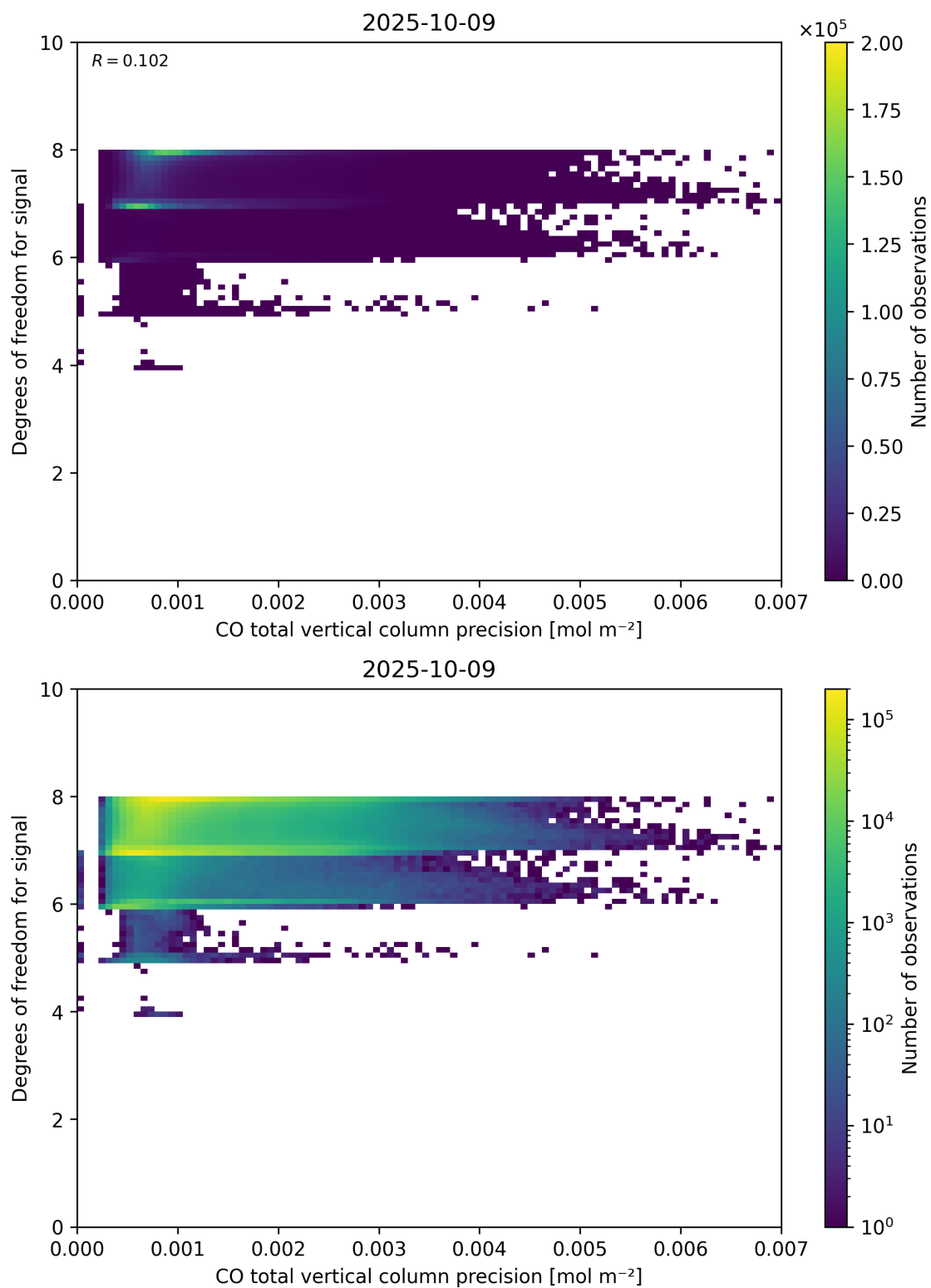
Figure 45: Scatter density plot of “CO total vertical column precision” against “Degrees of freedom for signal” for 2025-10-08 to 2025-10-10.
