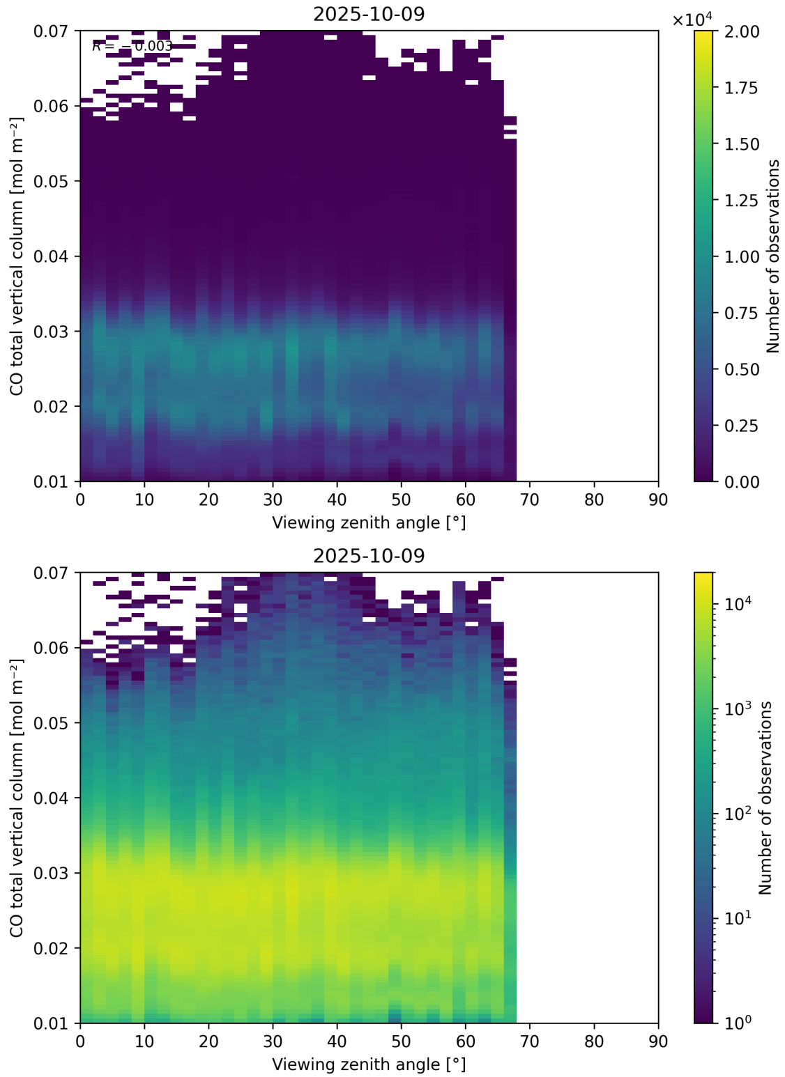
Figure 69: Scatter density plot of “Viewing zenith angle” against “CO total vertical column” for 2025-10-08 to 2025-10-10.
