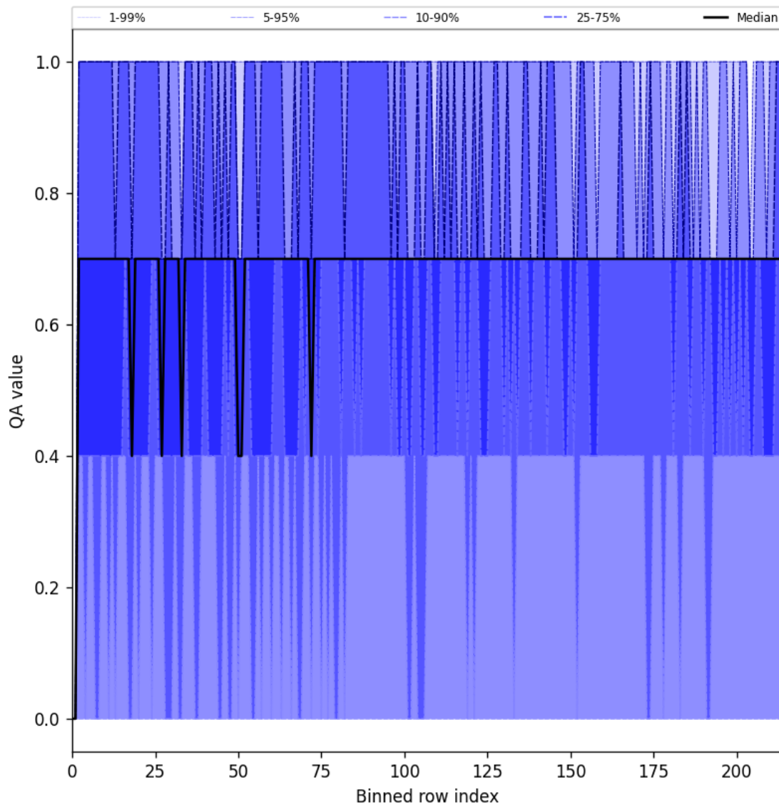
Figure 25: Along track statistics of “QA value” for 2025-10-08 to 2025-10-10
