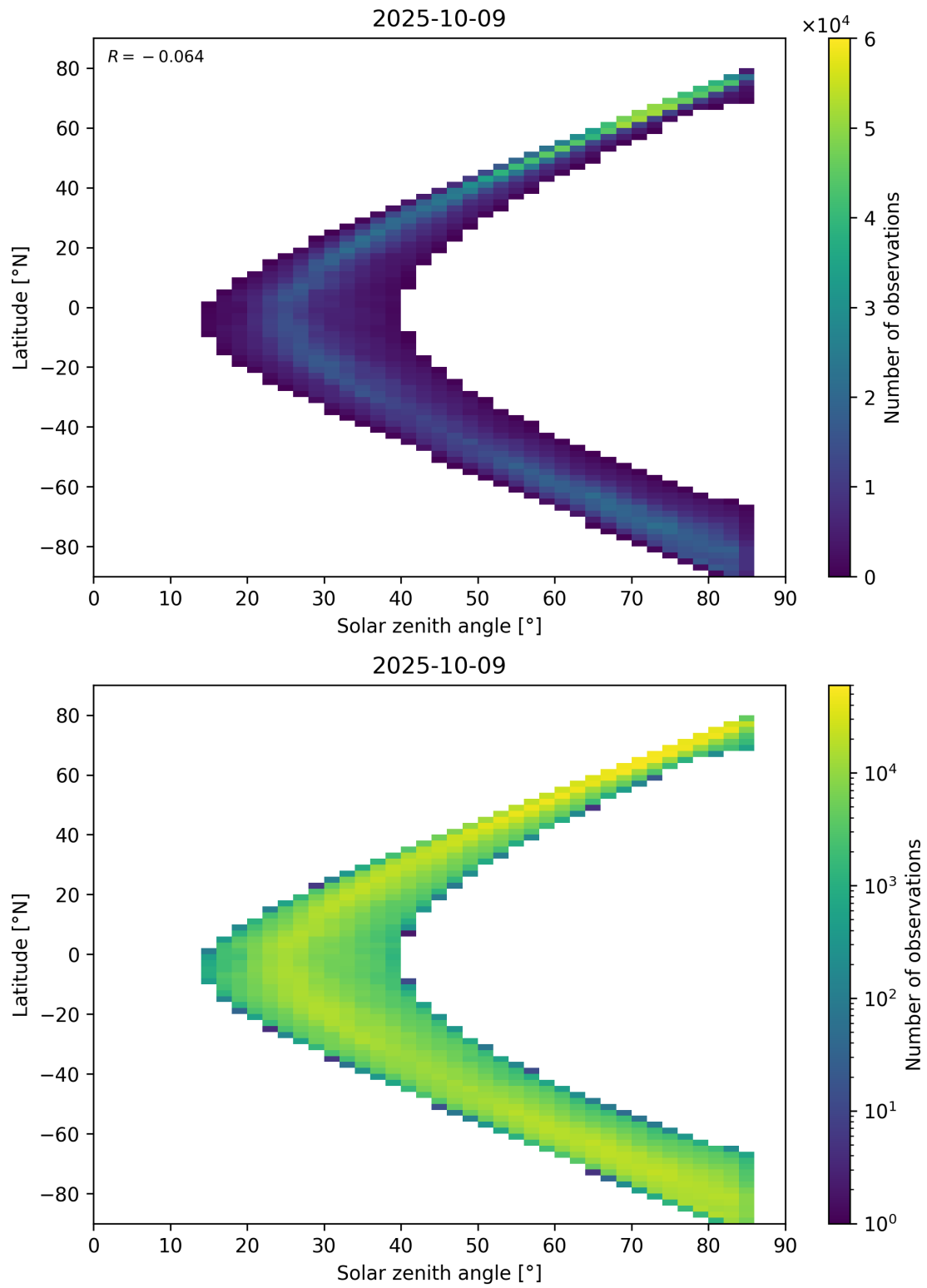
Figure 66: Scatter density plot of “Solar zenith angle” against “Latitude” for 2025-10-08 to 2025-10-10.
