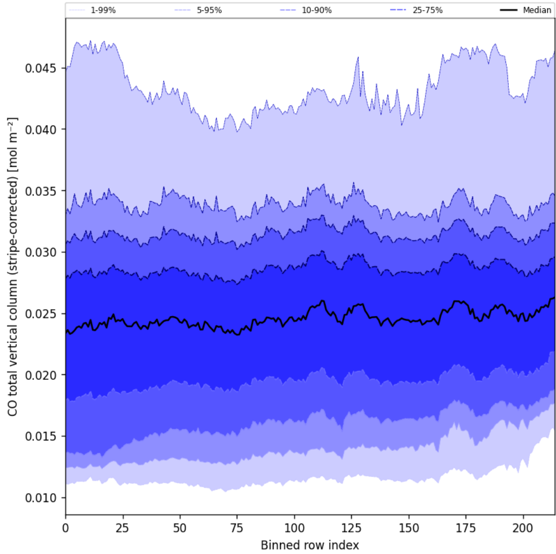
Figure 27: Along track statistics of “CO total vertical column (stripe-corrected)” for 2025-10-08 to 2025-10-10
