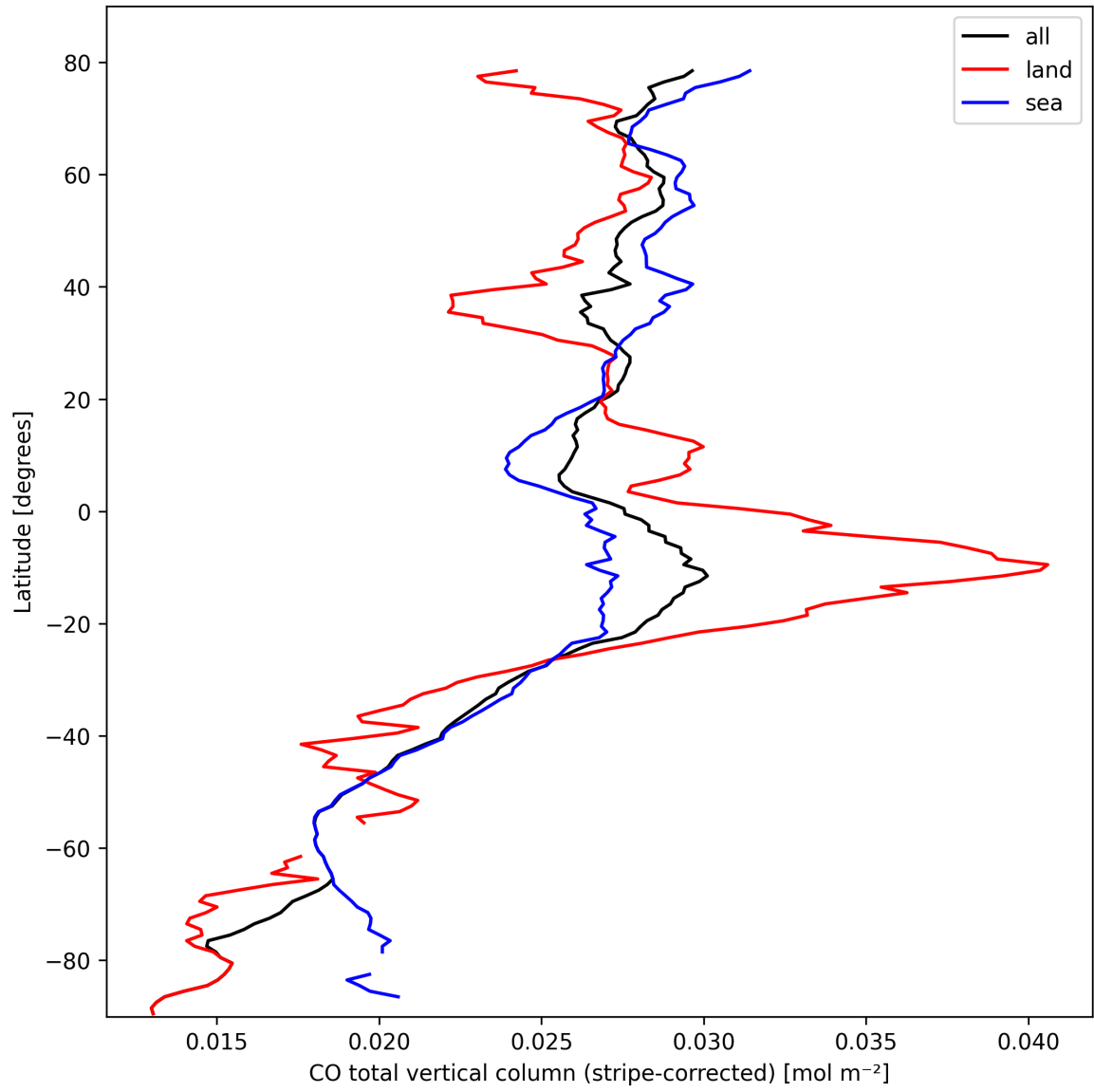
Figure 11: Zonal average of “CO total vertical column (stripe-corrected)” for 2025-10-08 to 2025-10-10.
