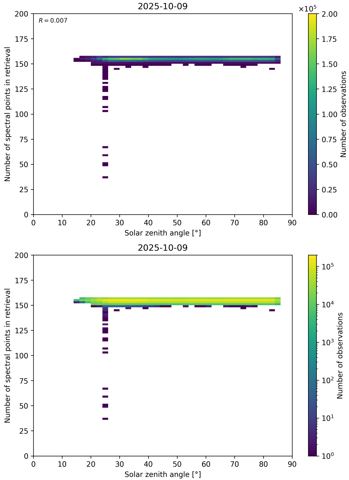
Figure 68: Scatter density plot of “Solar zenith angle” against “Number of spectral points in retrieval” for 2025-10-08 to 2025-10-10.
