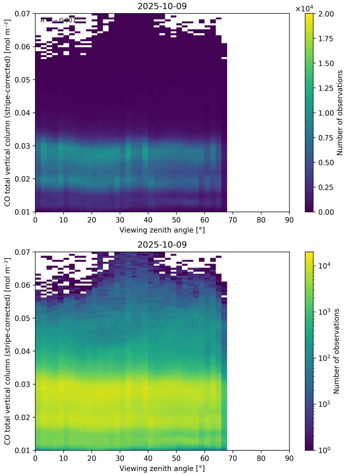
Figure 70: Scatter density plot of “Viewing zenith angle” against “CO total vertical column (stripe-corrected)” for 2025-10-08 to 2025-10-10.
