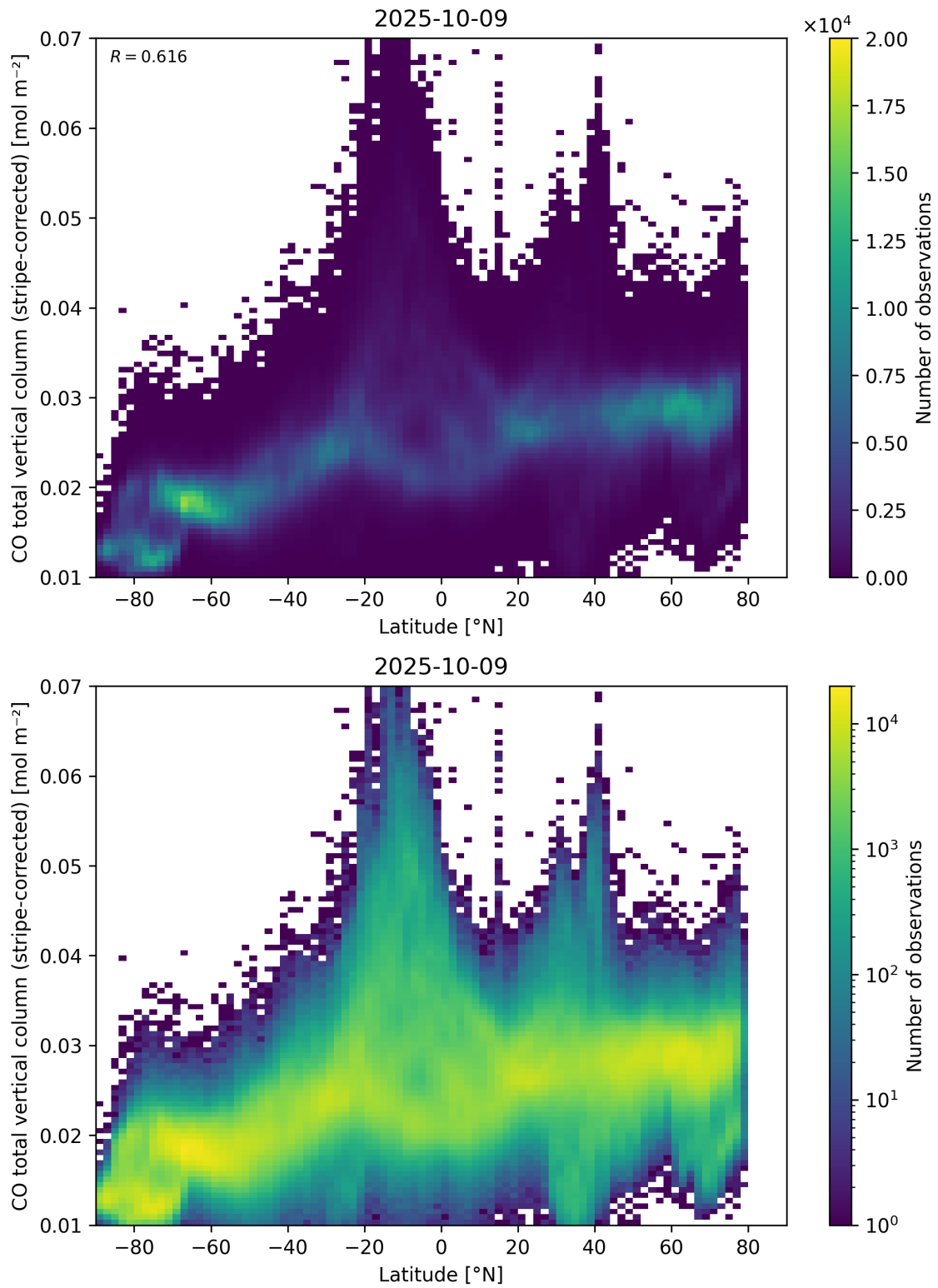
Figure 52: Scatter density plot of “Latitude” against “CO total vertical column (stripe-corrected)” for 2025-10-08 to 2025-10-10.
