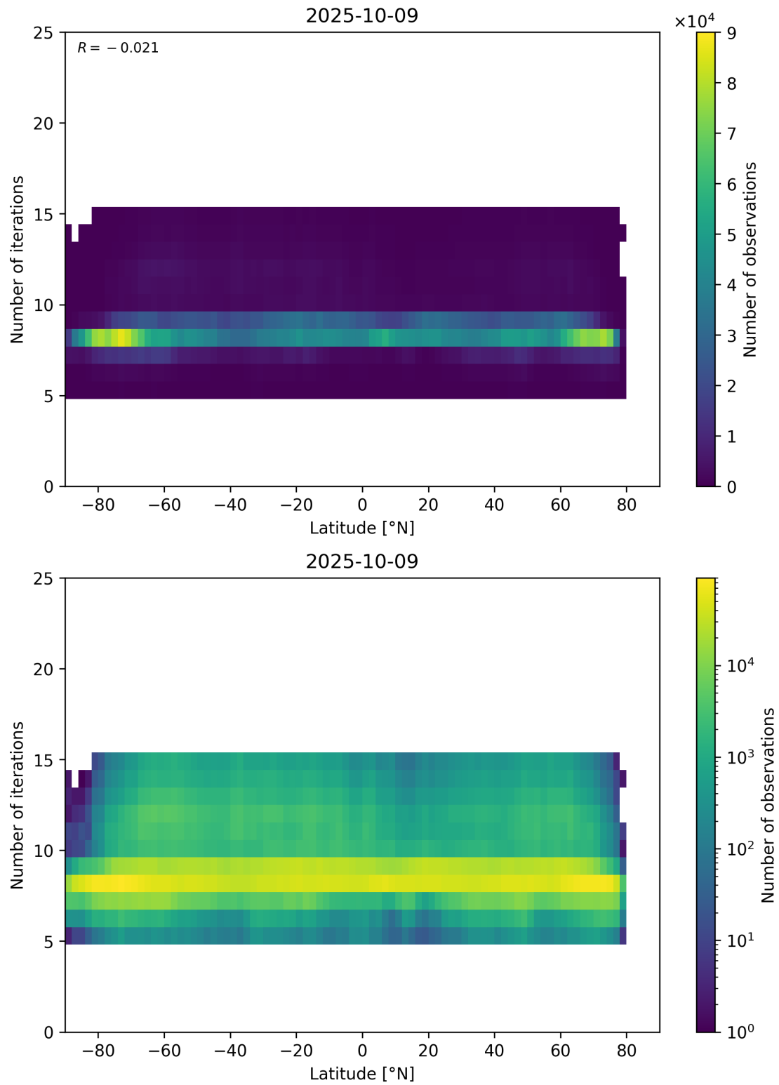
Figure 56: Scatter density plot of “Latitude” against “Number of iterations” for 2025-10-08 to 2025-10-10.
