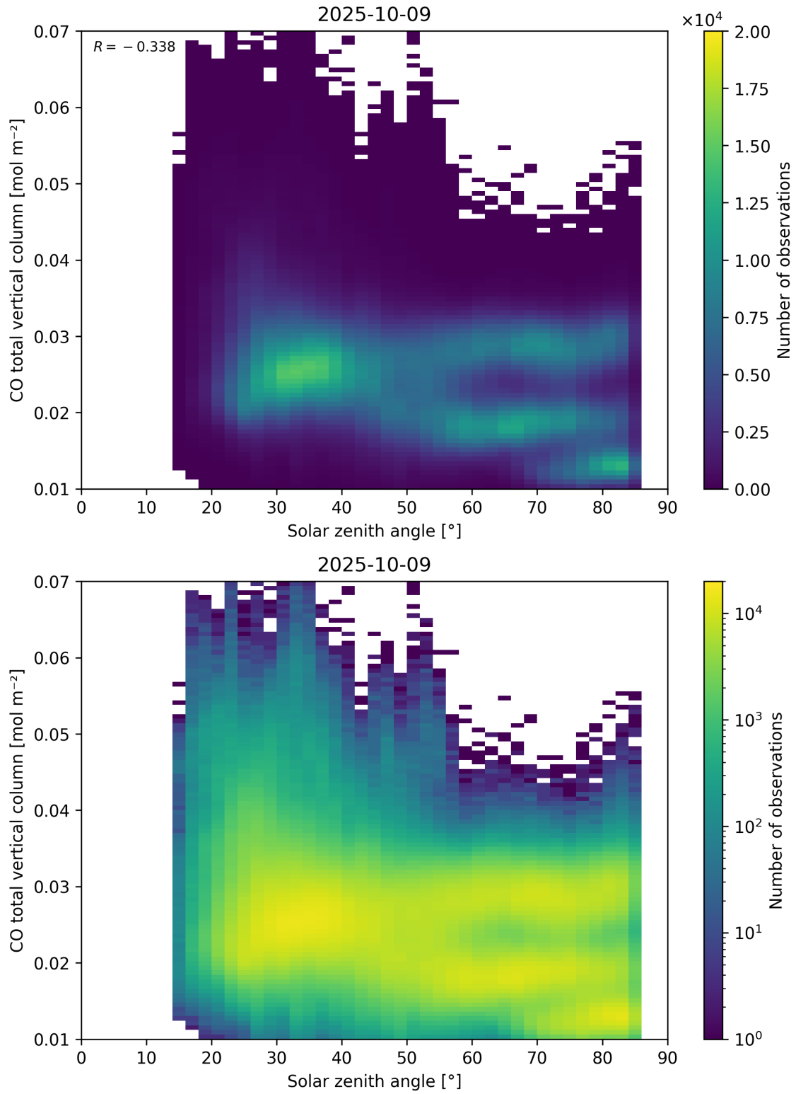
Figure 61: Scatter density plot of “Solar zenith angle” against “CO total vertical column” for 2025-10-08 to 2025-10-10.
