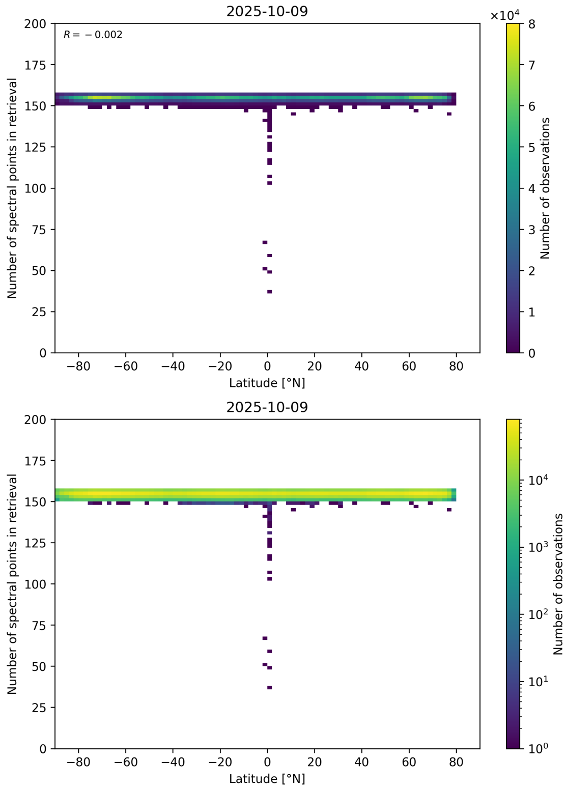
Figure 57: Scatter density plot of “Latitude” against “Number of spectral points in retrieval” for 2025-10-08 to 2025-10-10.
