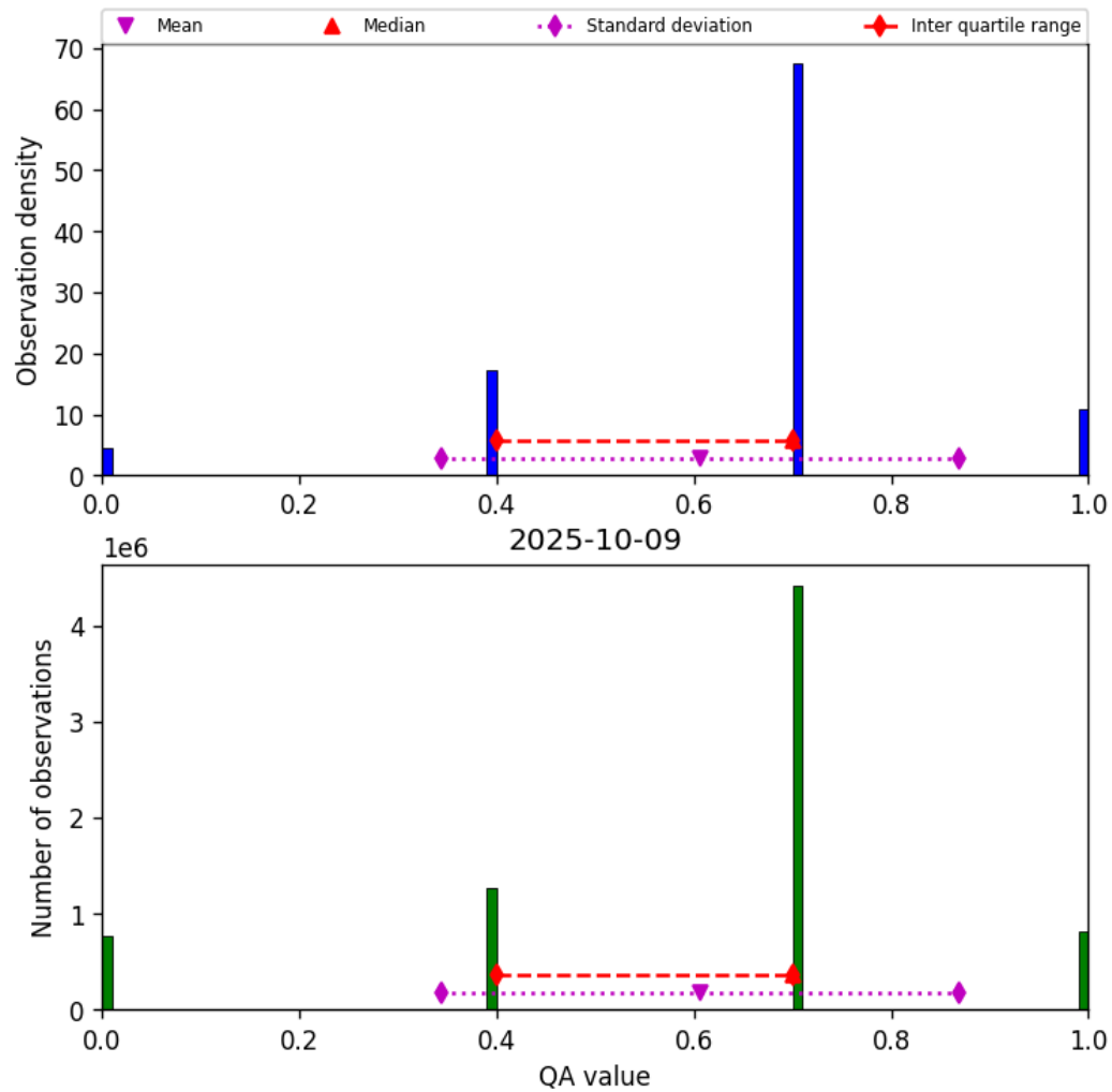
Figure 17: Histogram of “QA value” for 2025-10-08 to 2025-10-10
