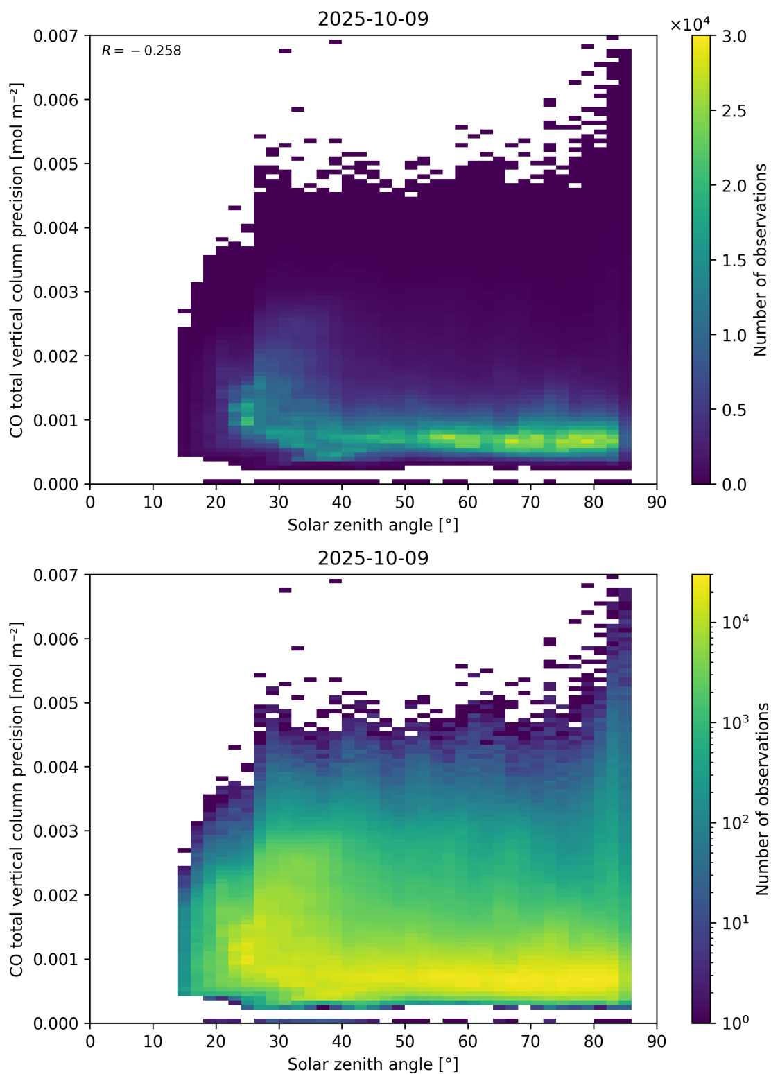
Figure 63: Scatter density plot of “Solar zenith angle” against “CO total vertical column precision” for 2025-10-08 to 2025-10-10.
