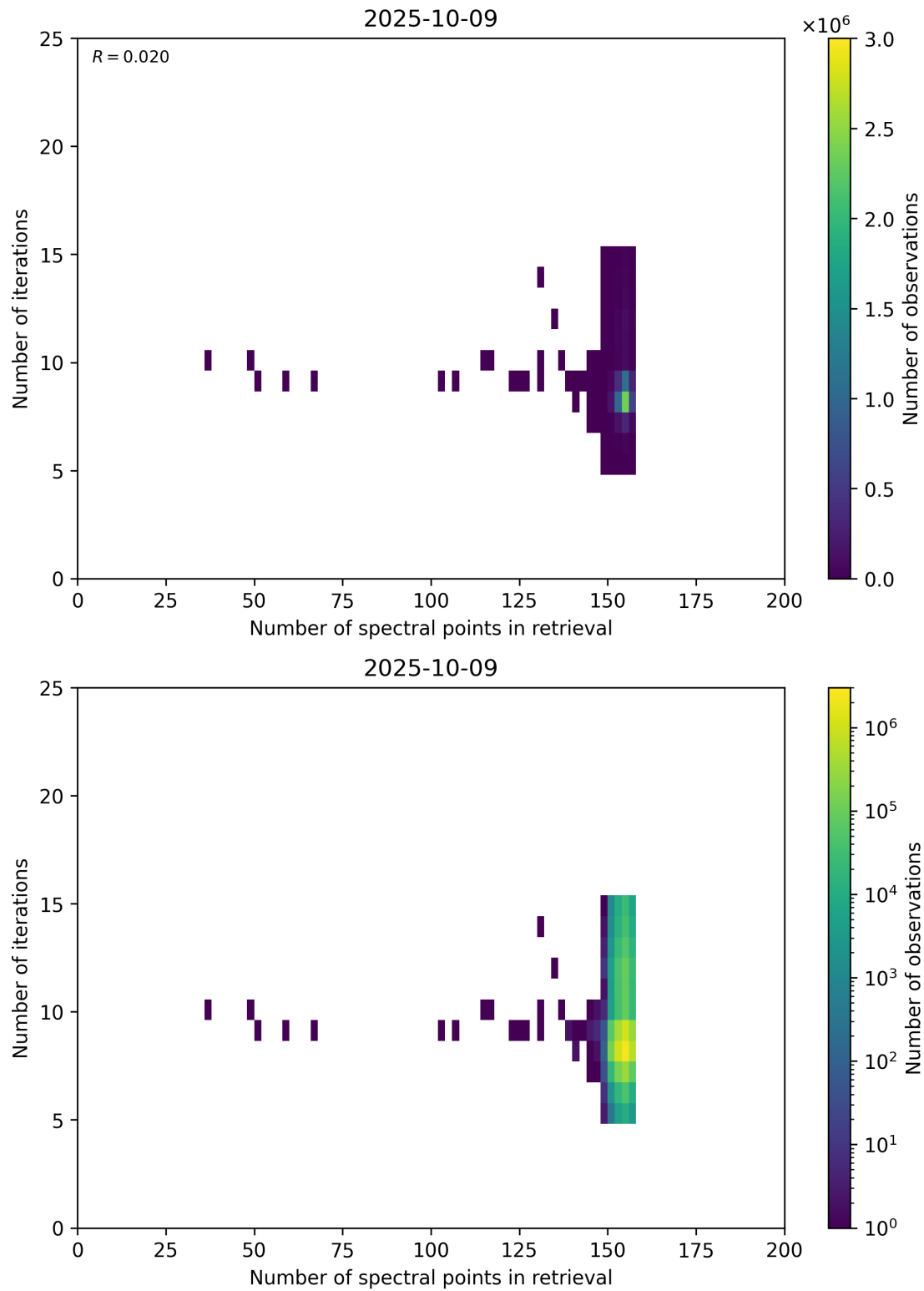
Figure 60: Scatter density plot of “Number of spectral points in retrieval” against “Number of iterations” for 2025-10-08 to 2025-10-10.
