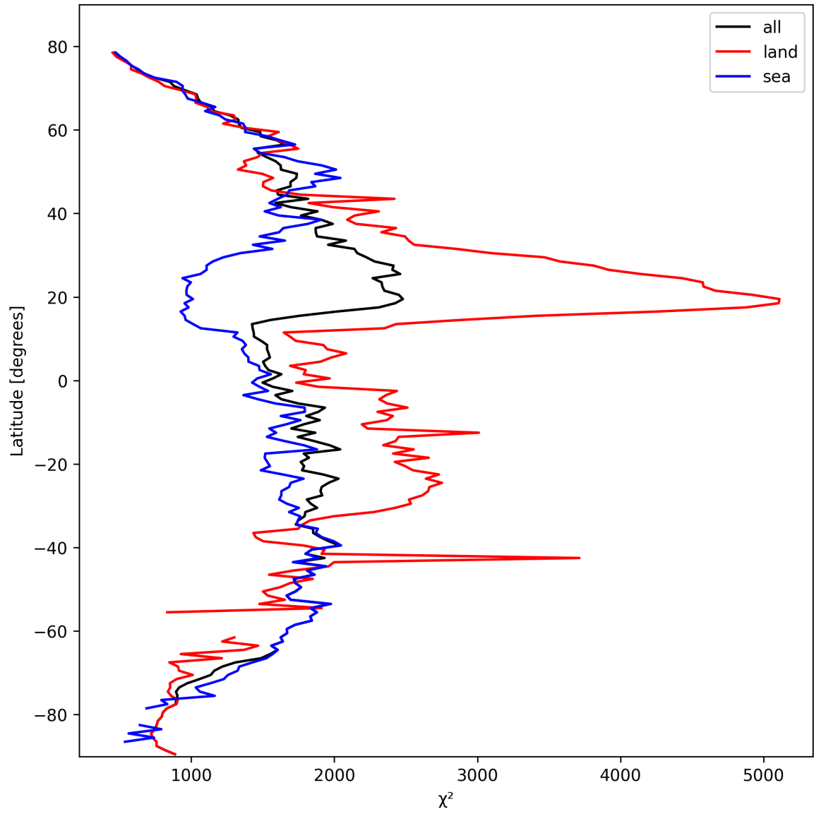
Figure 14: Zonal average of “ \chi^2 ” for 2025-10-08 to 2025-10-10.
