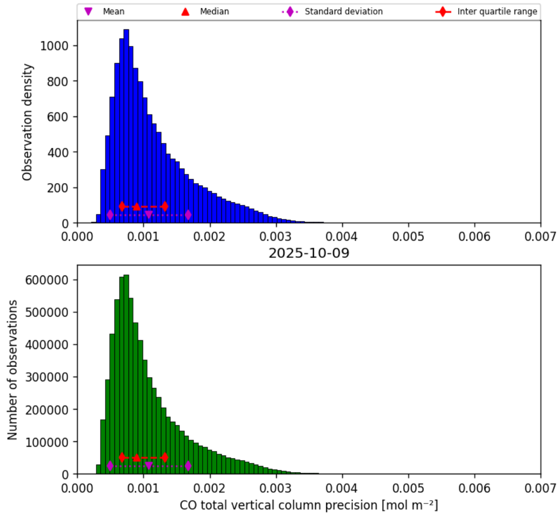
Figure 20: Histogram of “CO total vertical column precision” for 2025-10-08 to 2025-10-10
