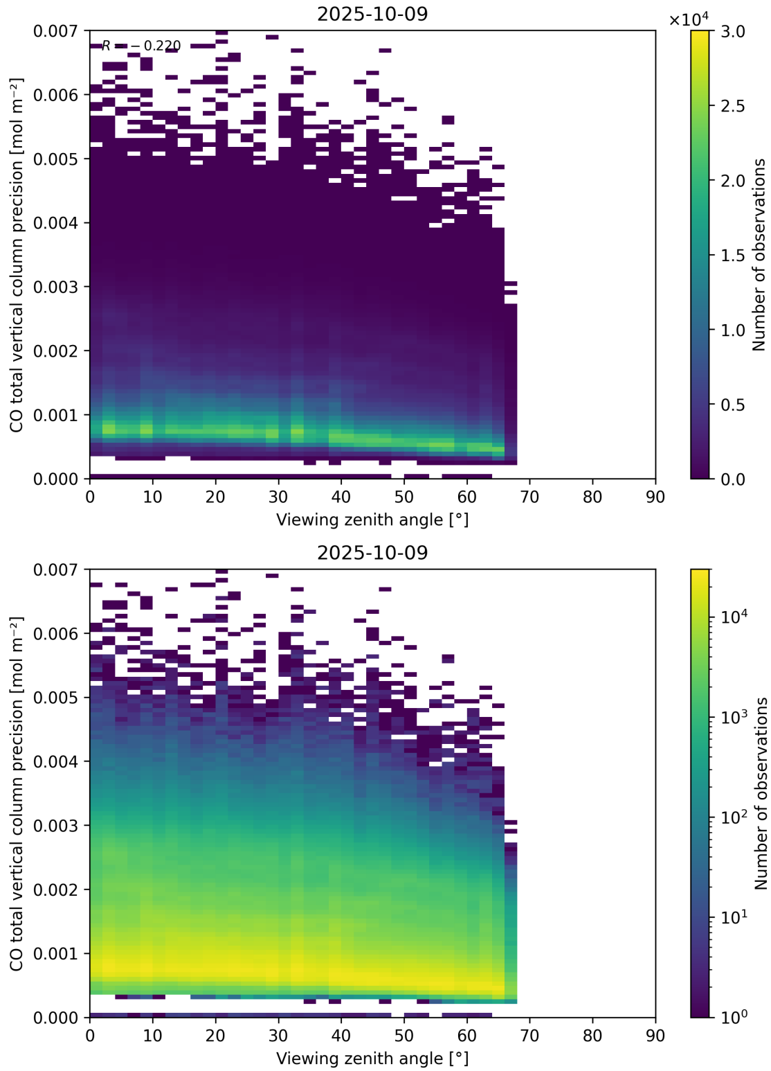
Figure 71: Scatter density plot of “Viewing zenith angle” against “CO total vertical column precision” for 2025-10-08 to 2025-10-10.
