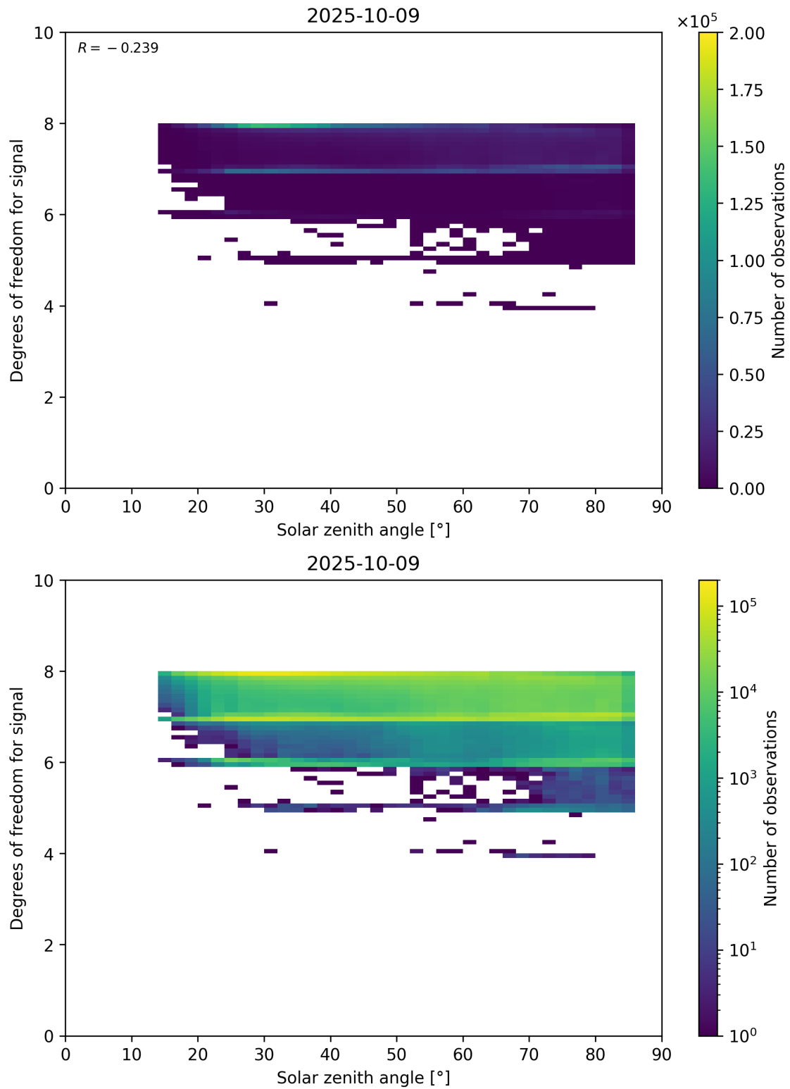
Figure 65: Scatter density plot of “Solar zenith angle” against “Degrees of freedom for signal” for 2025-10-08 to 2025-10-10.
