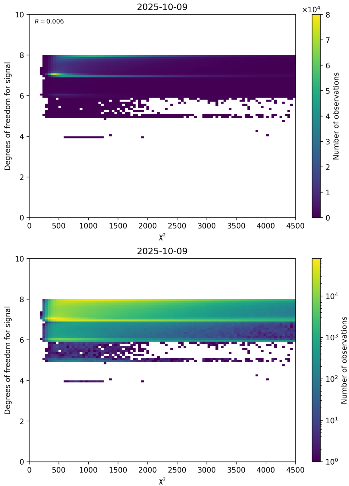
Figure 48: Scatter density plot of “ \chi^2 ” against “Degrees of freedom for signal” for 2025-10-08 to 2025-10-10.
