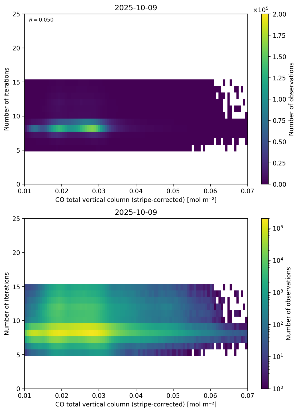
Figure 39: Scatter density plot of “CO total vertical column (stripe-corrected)” against “Number of iterations” for 2025-10-08 to 2025-10-10.
