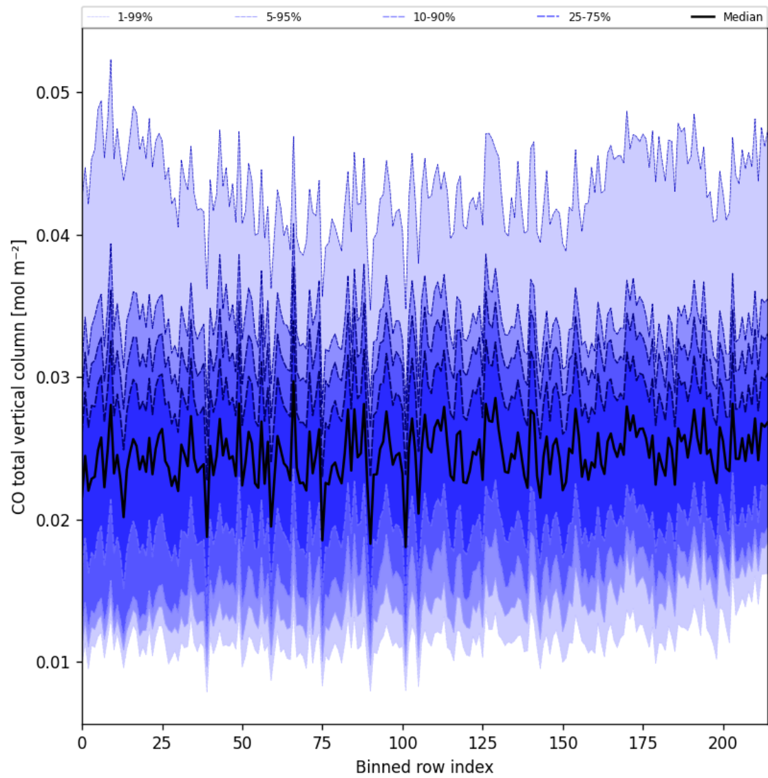
Figure 26: Along track statistics of “CO total vertical column” for 2025-10-08 to 2025-10-10
