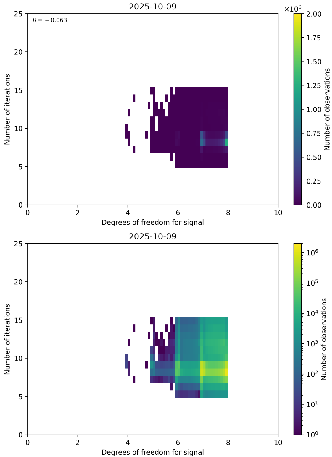
Figure 50: Scatter density plot of “Degrees of freedom for signal” against “Number of iterations” for 2025-10-08 to 2025-10-10.
