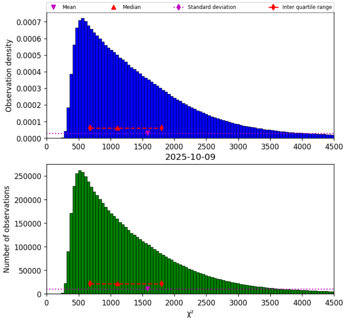
Figure 22: Histogram of “ \chi^2 ” for 2025-10-08 to 2025-10-10
