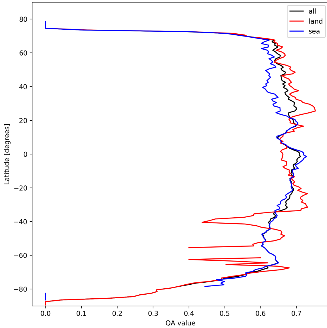
Figure 9: Zonal average of “QA value” for 2025-10-08 to 2025-10-10.
