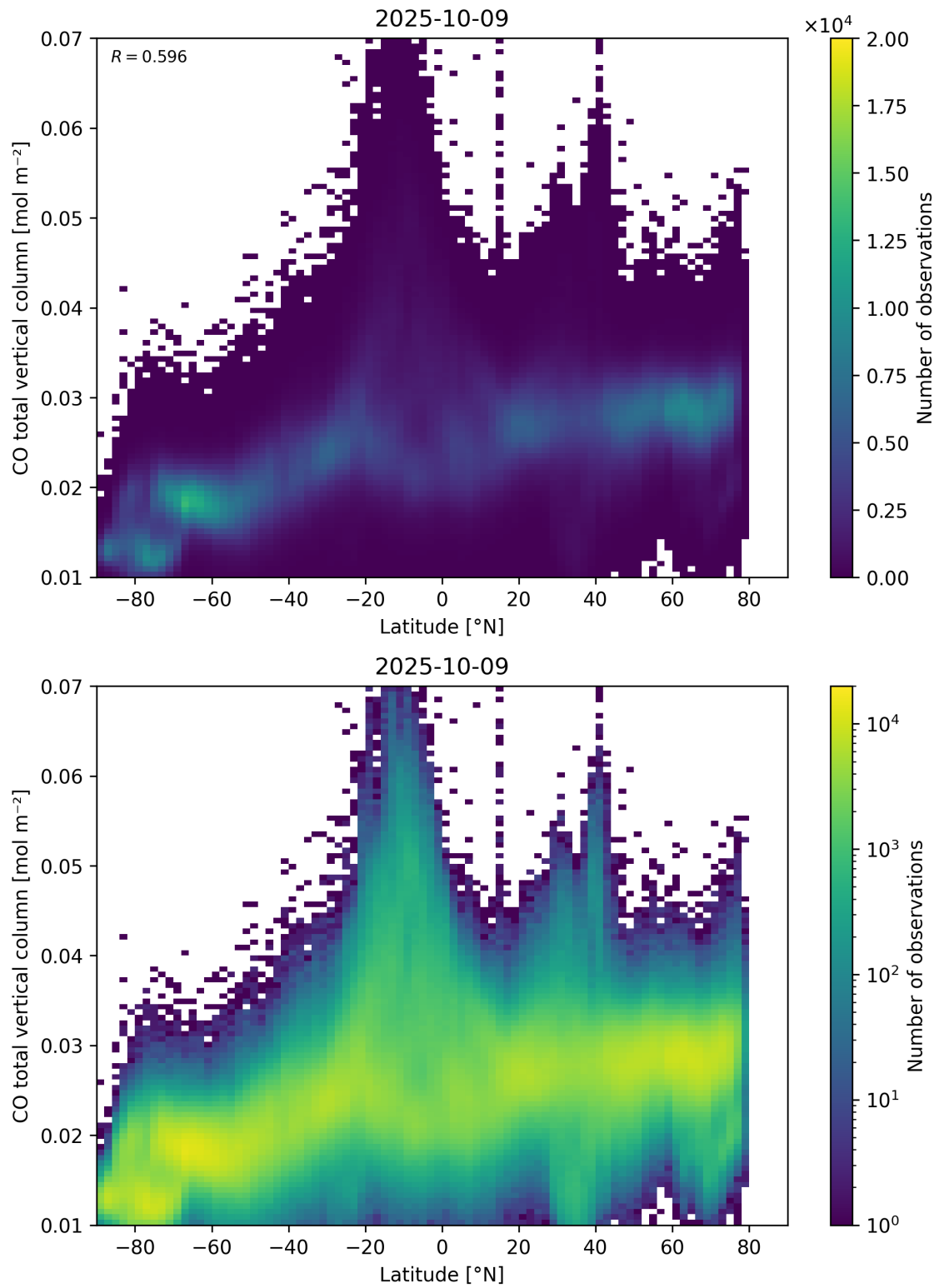
Figure 51: Scatter density plot of “Latitude” against “CO total vertical column” for 2025-10-08 to 2025-10-10.
