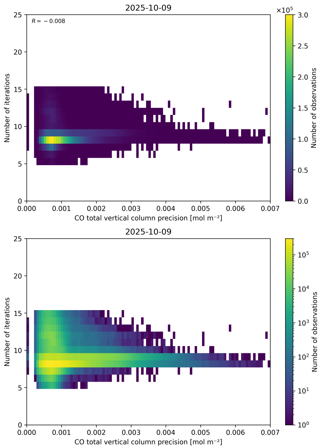
Figure 46: Scatter density plot of “CO total vertical column precision” against “Number of iterations” for 2025-10-08 to 2025-10-10.
