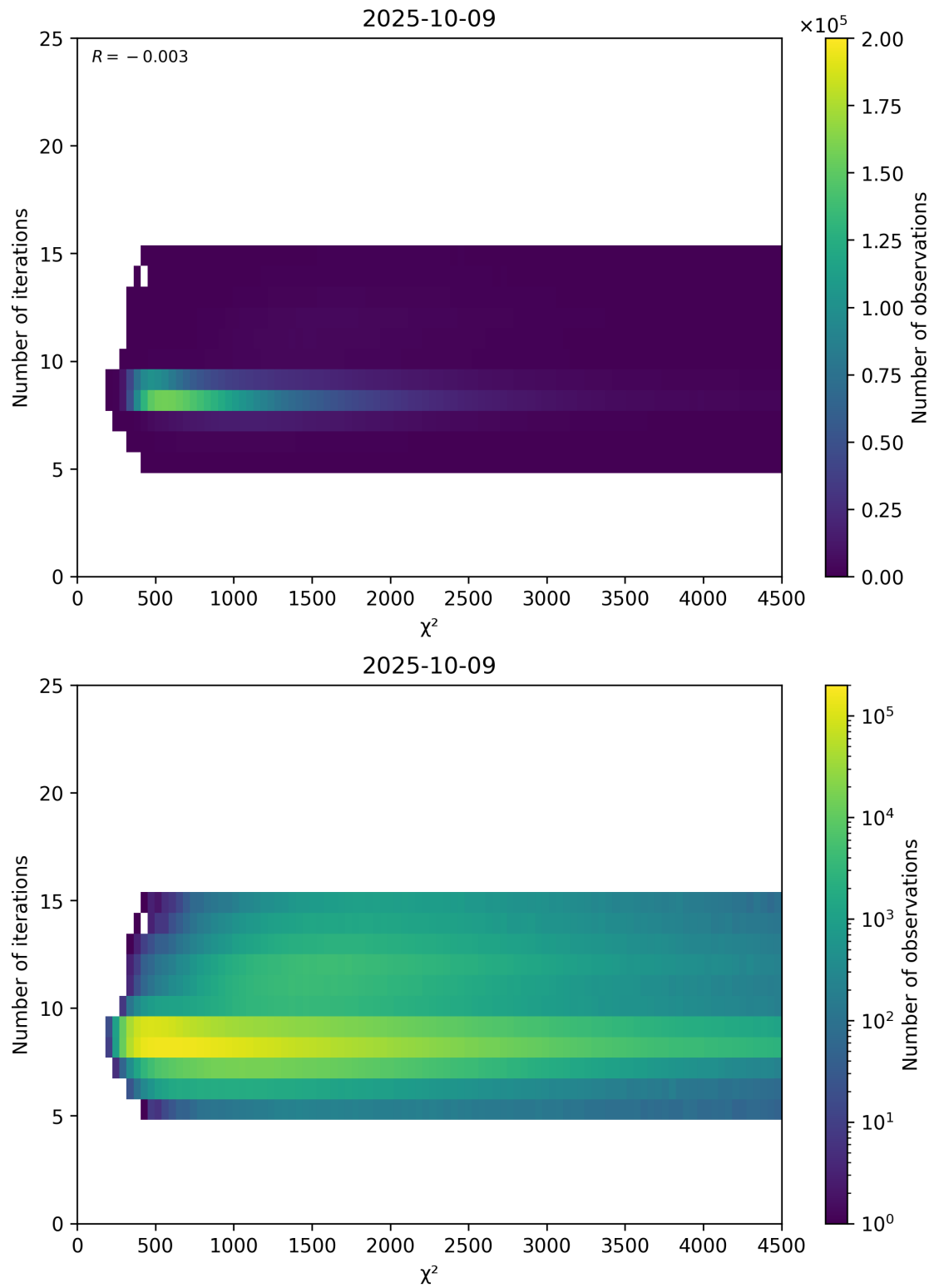
Figure 49: Scatter density plot of “ \chi^2 ” against “Number of iterations” for 2025-10-08 to 2025-10-10.
