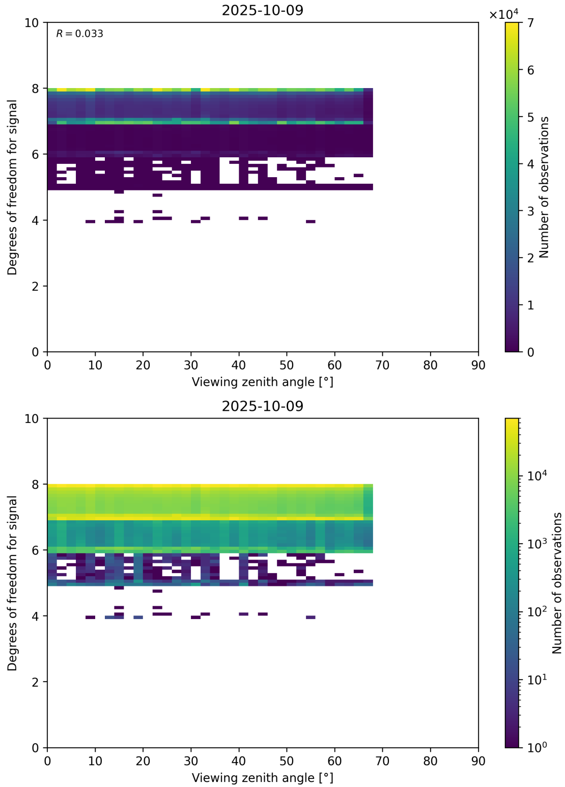
Figure 73: Scatter density plot of “Viewing zenith angle” against “Degrees of freedom for signal” for 2025-10-08 to 2025-10-10.
