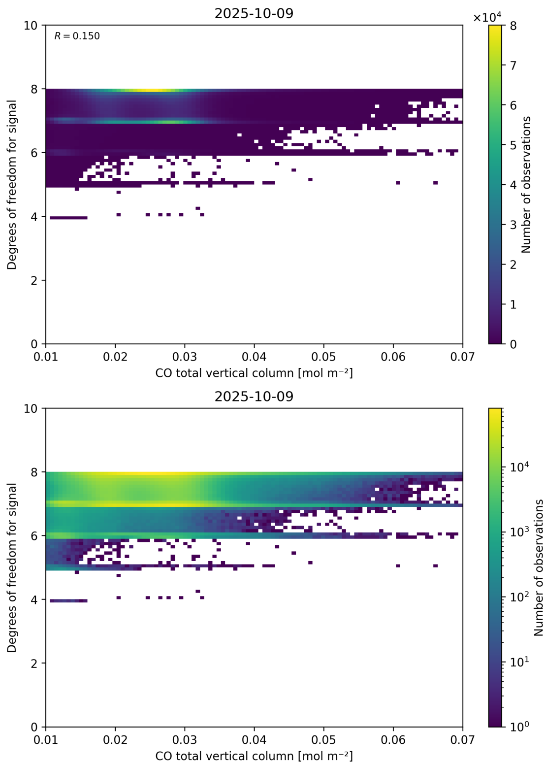
Figure 41: Scatter density plot of “CO total vertical column” against “Degrees of freedom for signal” for 2025-10-08 to 2025-10-10.
