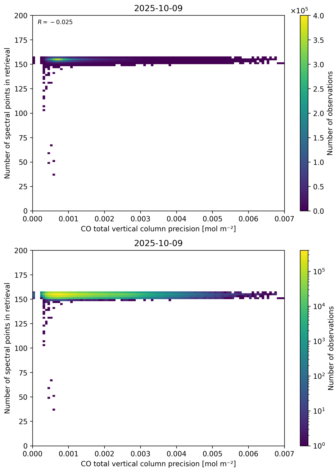
Figure 47: Scatter density plot of “CO total vertical column precision” against “Number of spectral points in retrieval” for 2025-10-08 to 2025-10-10.
