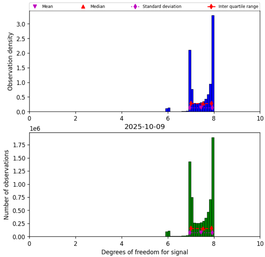
Figure 23: Histogram of “Degrees of freedom for signal” for 2025-10-08 to 2025-10-10
