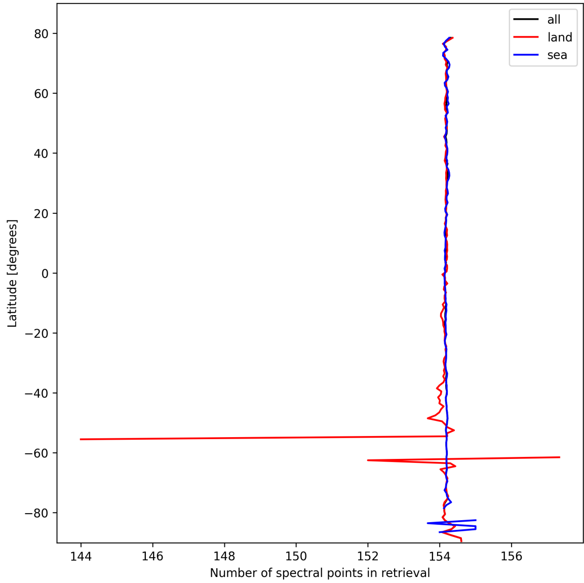
Figure 13: Zonal average of “Number of spectral points in retrieval” for 2025-10-08 to 2025-10-10.
