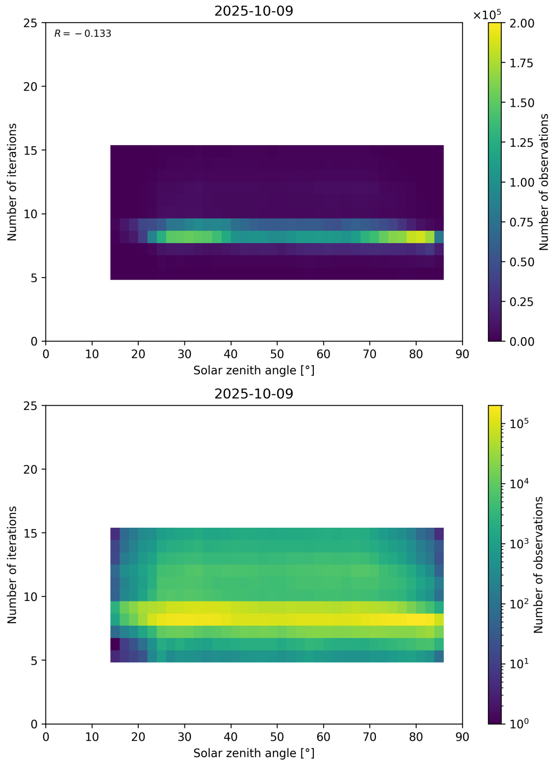
Figure 67: Scatter density plot of “Solar zenith angle” against “Number of iterations” for 2025-10-08 to 2025-10-10.
