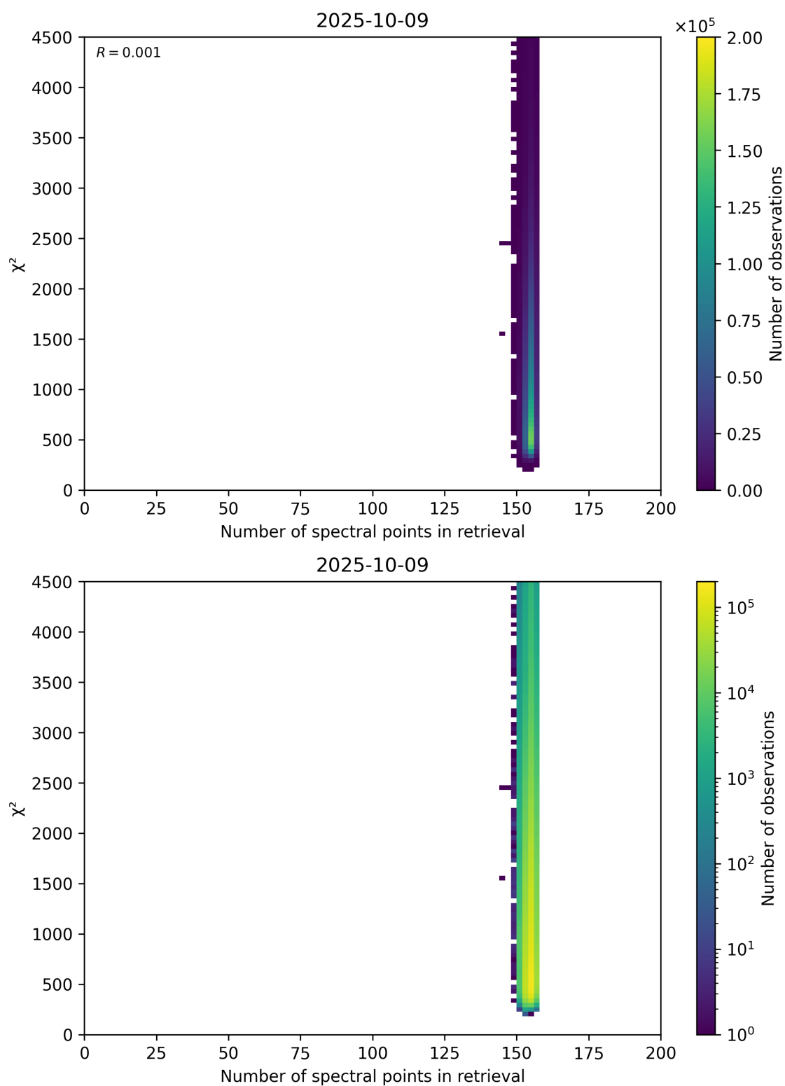
Figure 58: Scatter density plot of “Number of spectral points in retrieval” against “ \chi^2 ” for 2025-10-08 to 2025-10-10.
