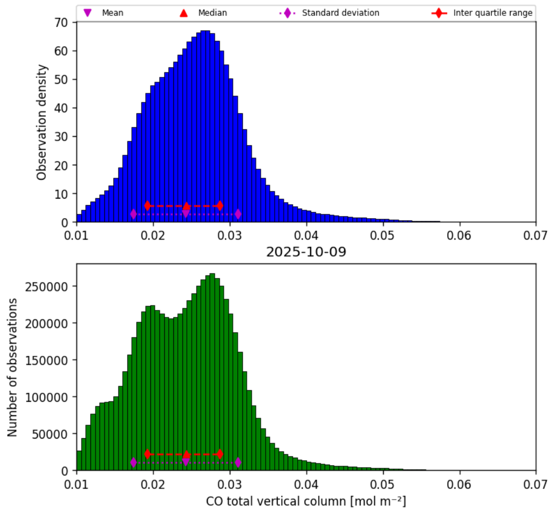
Figure 18: Histogram of “CO total vertical column” for 2025-10-08 to 2025-10-10
