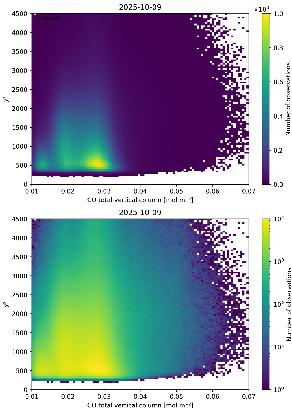
Figure 35: Scatter density plot of “CO total vertical column” against “ \chi^2 ” for 2025-10-08 to 2025-10-10.
