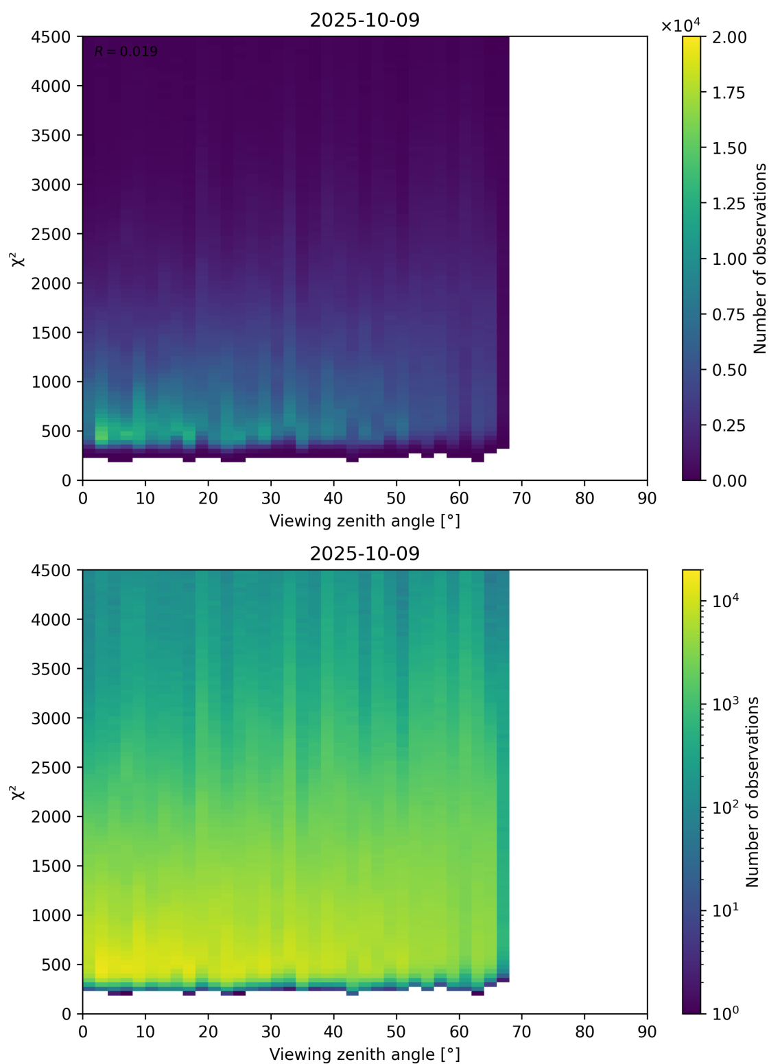
Figure 72: Scatter density plot of “Viewing zenith angle” against “ \chi^2 ” for 2025-10-08 to 2025-10-10.
