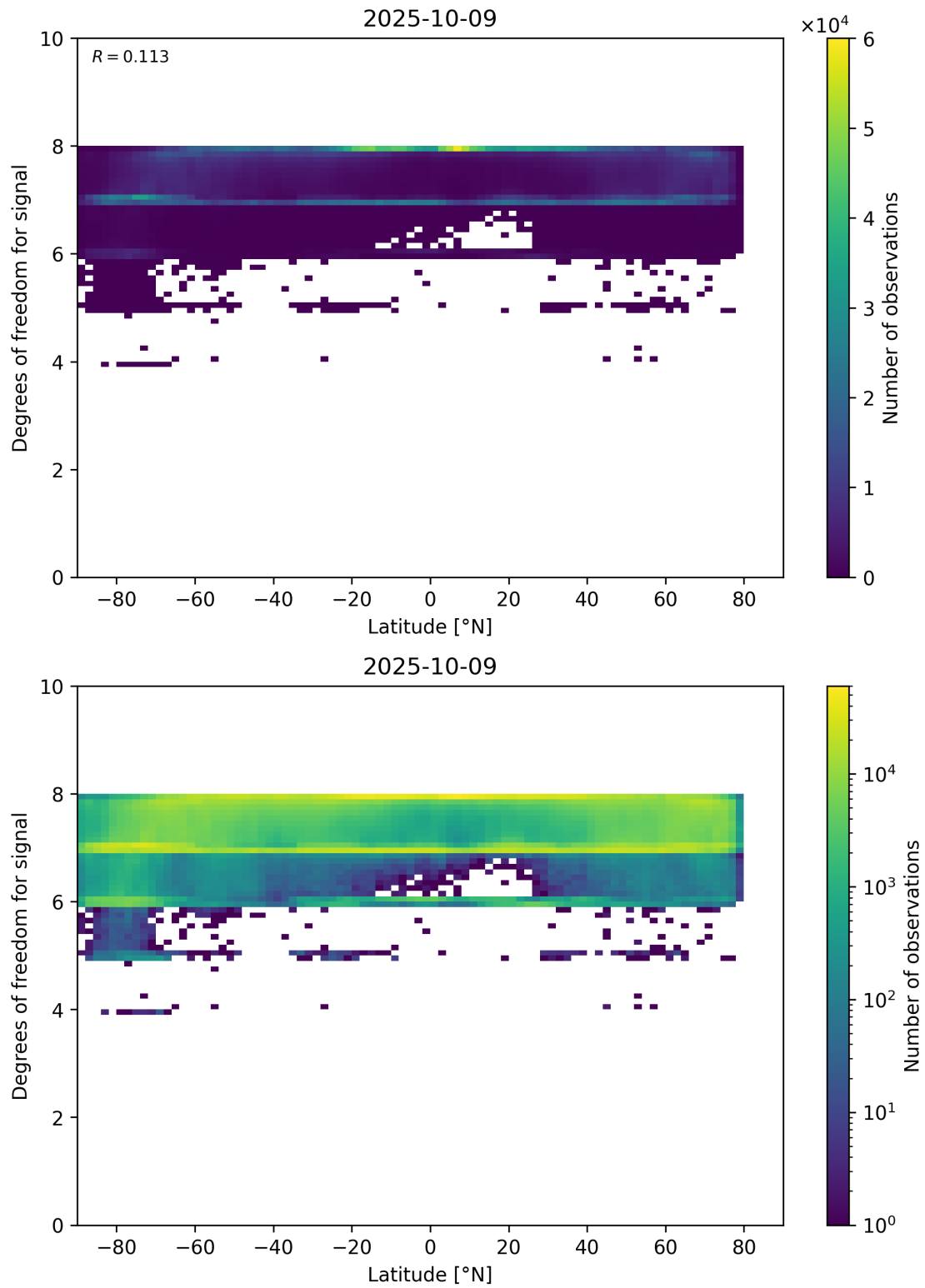
Figure 55: Scatter density plot of “Latitude” against “Degrees of freedom for signal” for 2025-10-08 to 2025-10-10.
