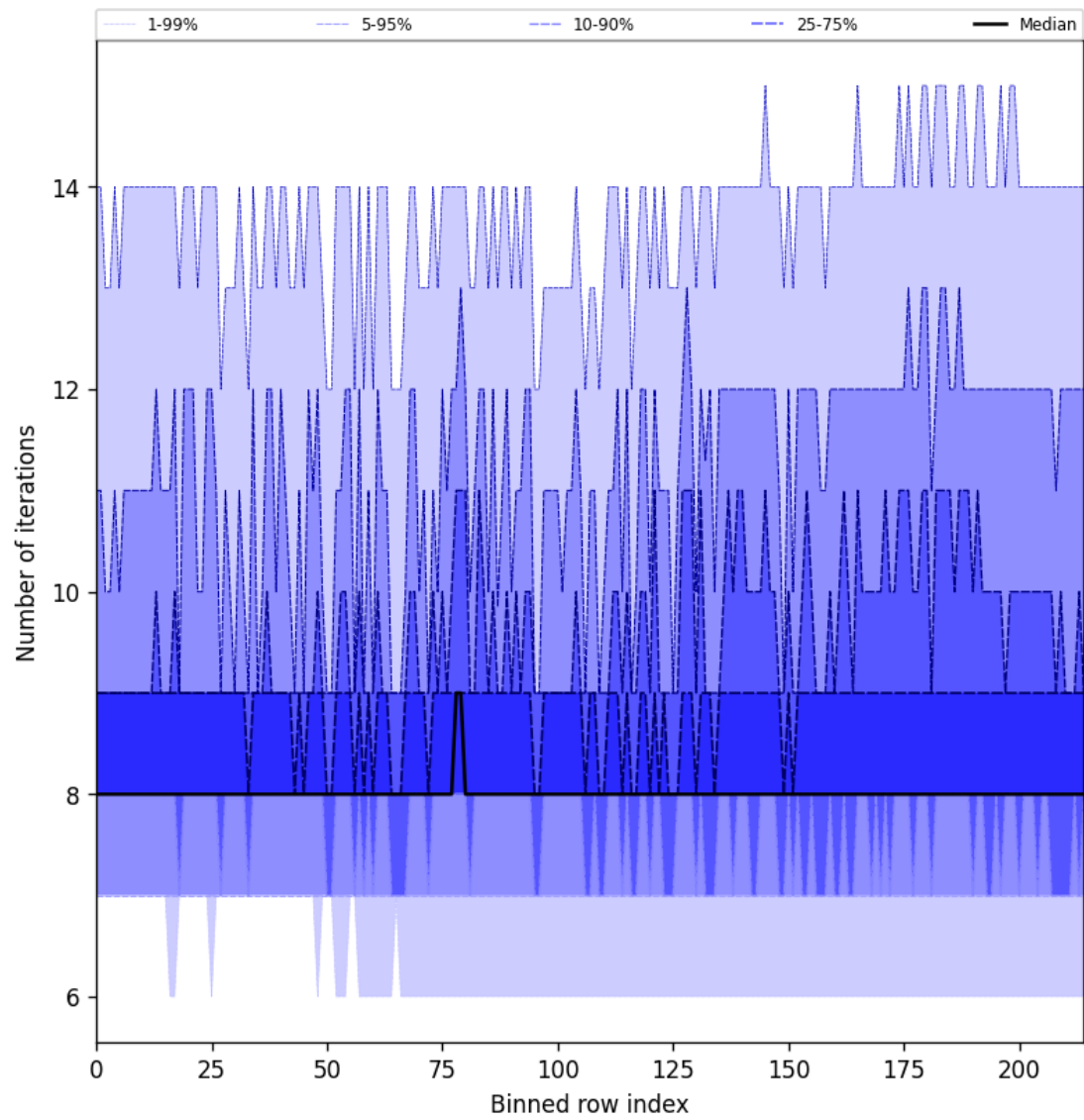
Figure 32: Along track statistics of “Number of iterations” for 2025-10-08 to 2025-10-10
