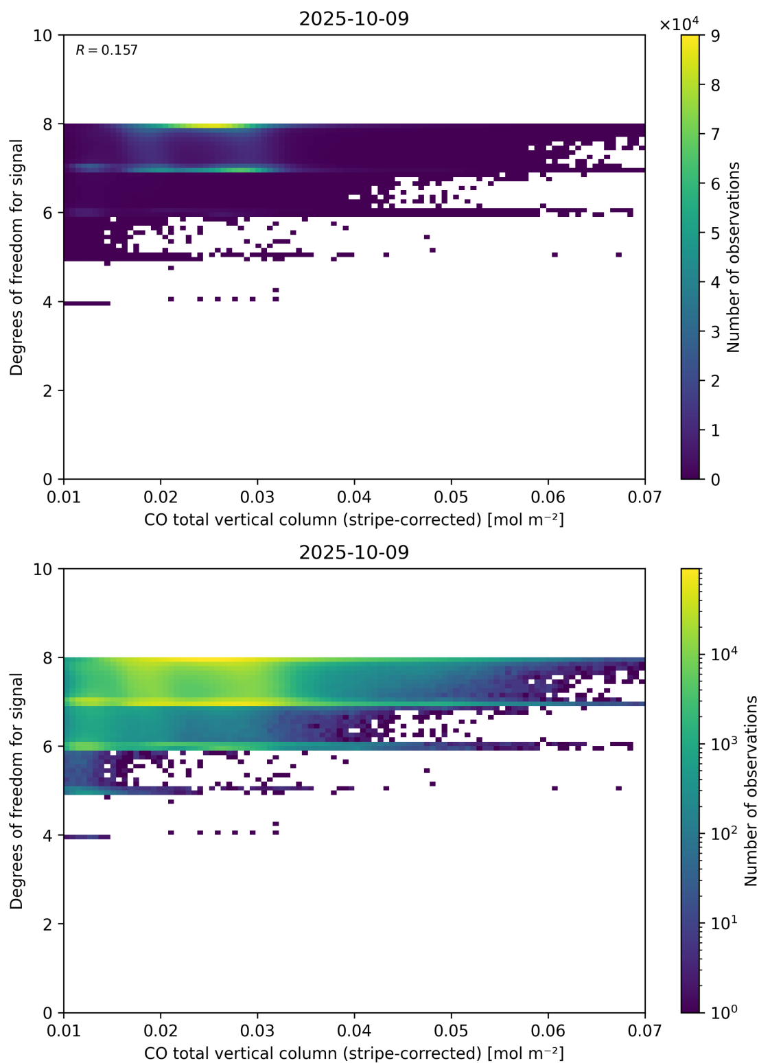
Figure 38: Scatter density plot of “CO total vertical column (stripe-corrected)” against “Degrees of freedom for signal” for 2025-10-08 to 2025-10-10.
