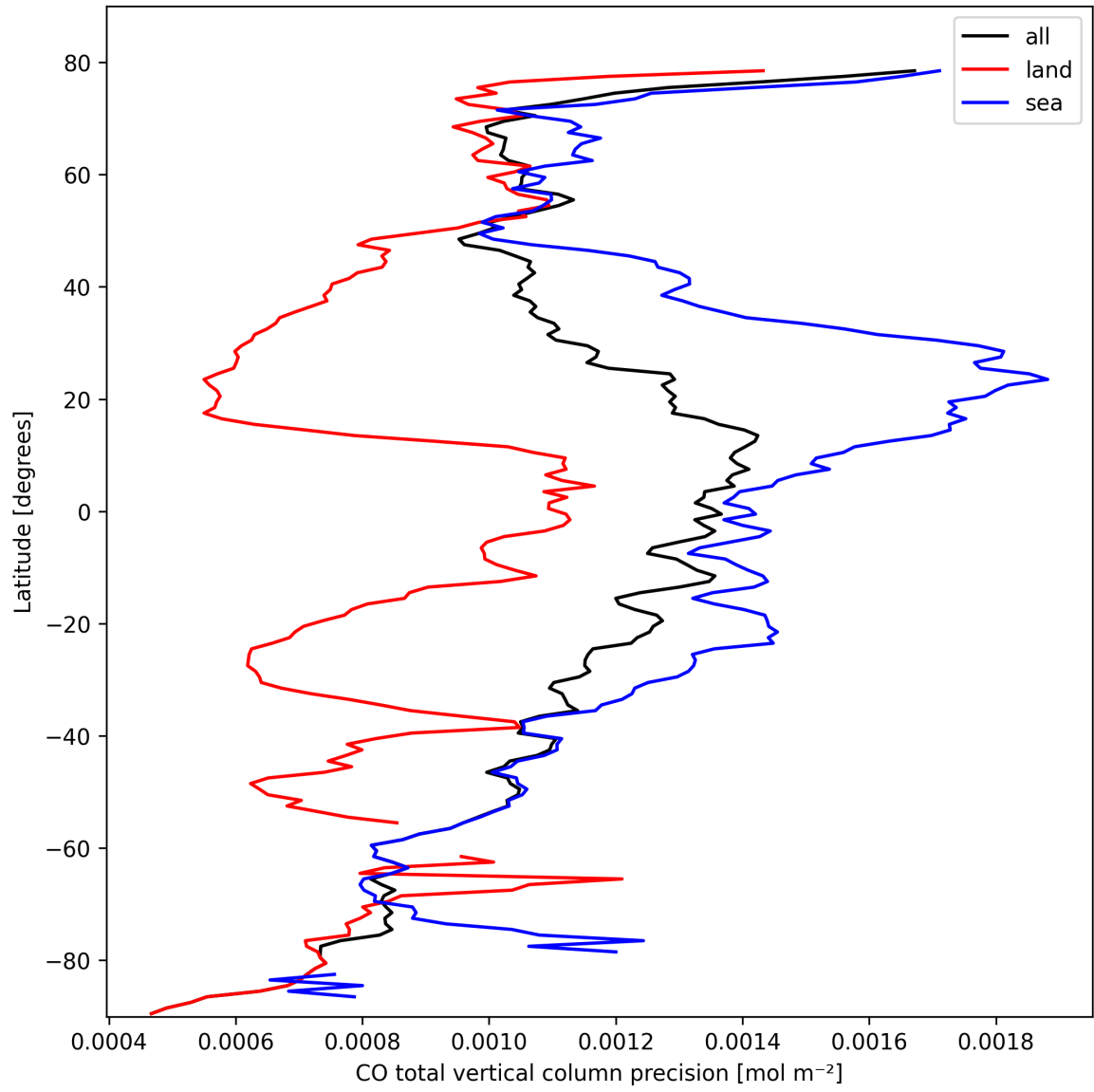
Figure 12: Zonal average of “CO total vertical column precision” for 2025-10-08 to 2025-10-10.
