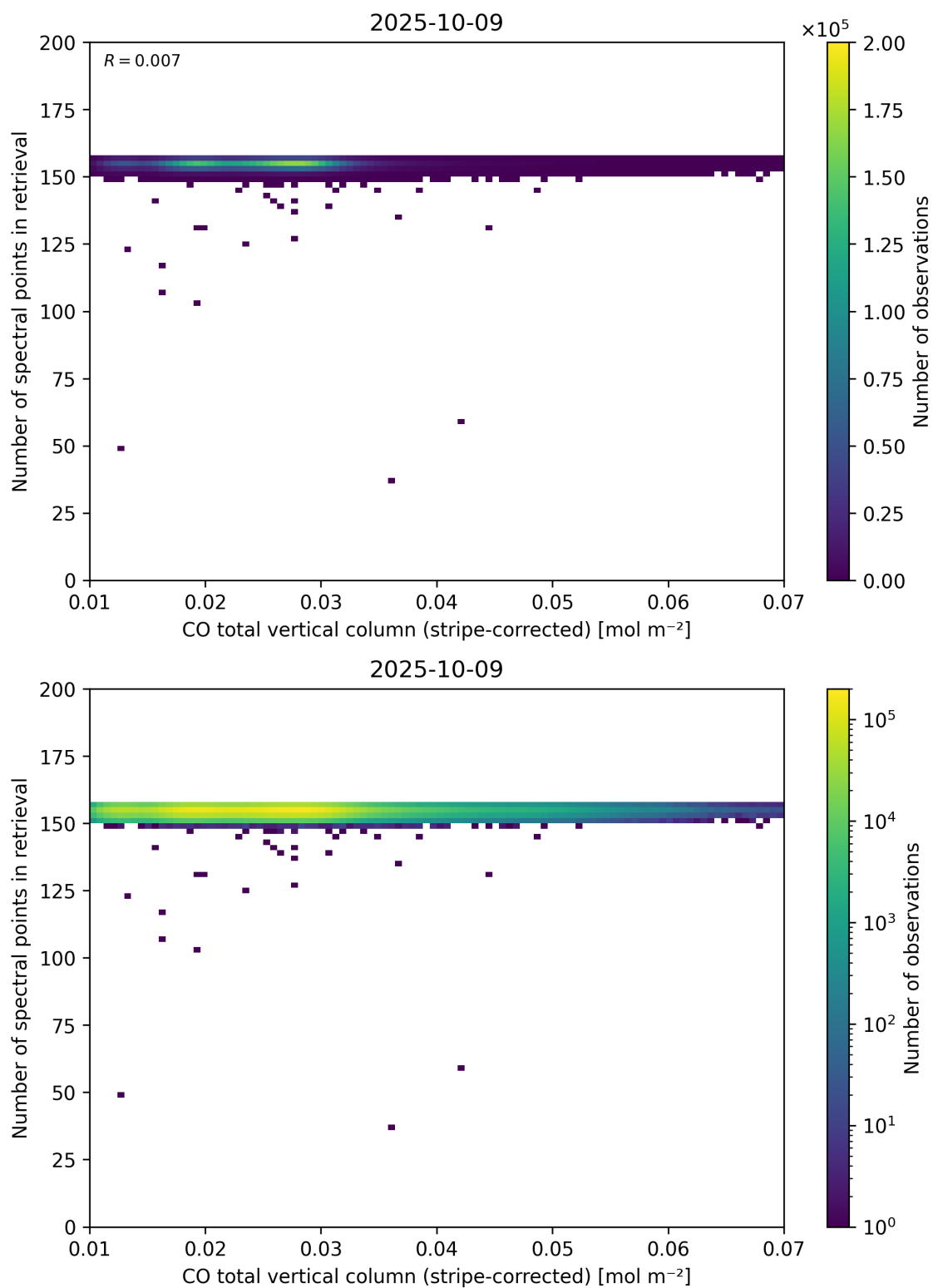
Figure 40: Scatter density plot of “CO total vertical column (stripe-corrected)” against “Number of spectral points in retrieval” for 2025-10-08 to 2025-10-10.
