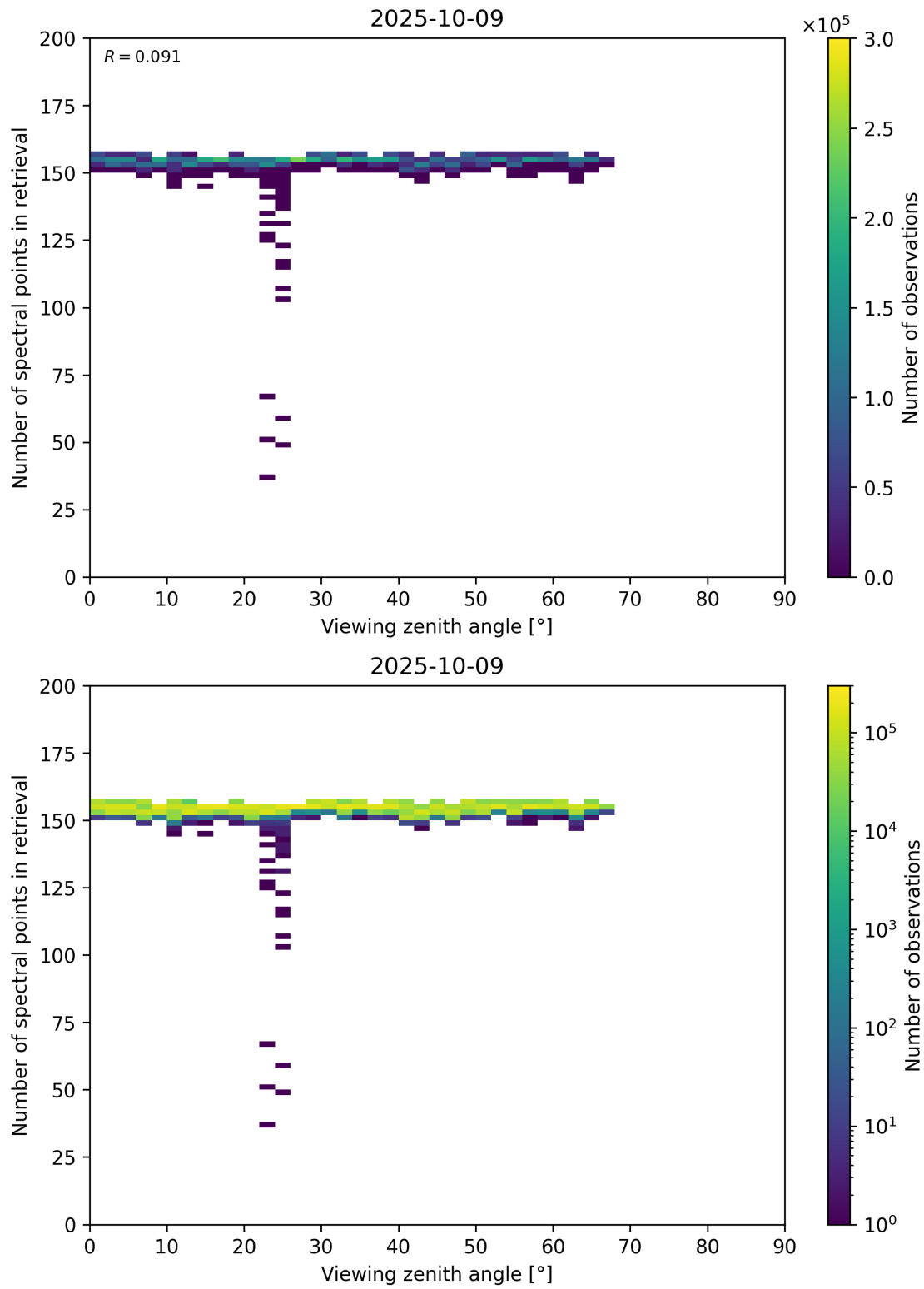
Figure 76: Scatter density plot of “Viewing zenith angle” against “Number of spectral points in retrieval” for 2025-10-08 to 2025-10-10.
