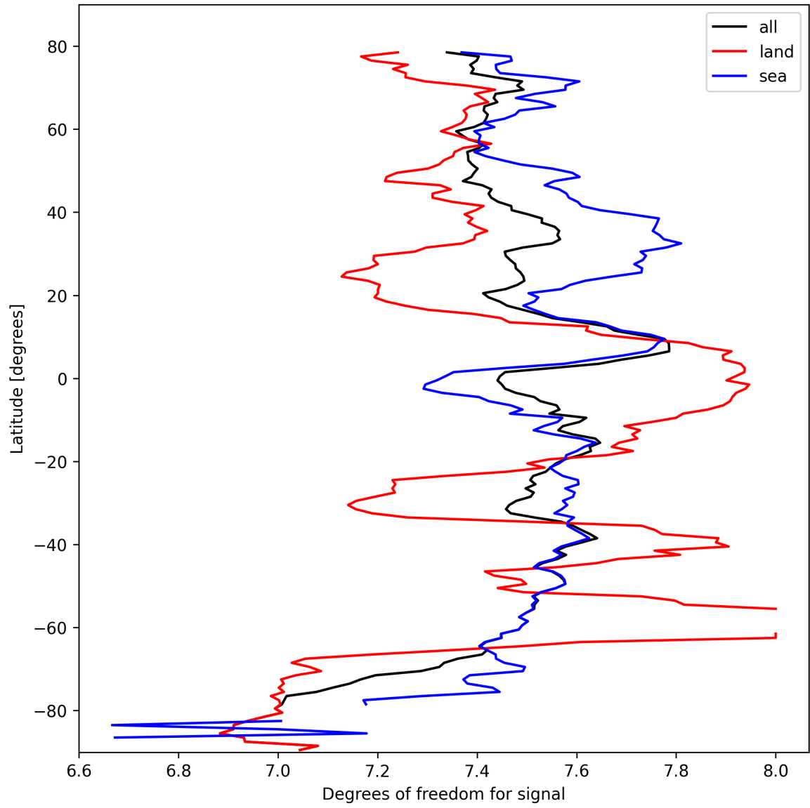
Figure 15: Zonal average of “Degrees of freedom for signal” for 2025-10-08 to 2025-10-10.
