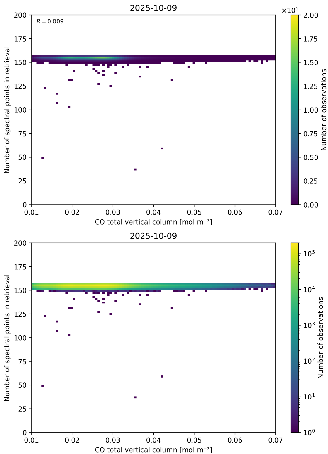
Figure 43: Scatter density plot of “CO total vertical column” against “Number of spectral points in retrieval” for 2025-10-08 to 2025-10-10.
