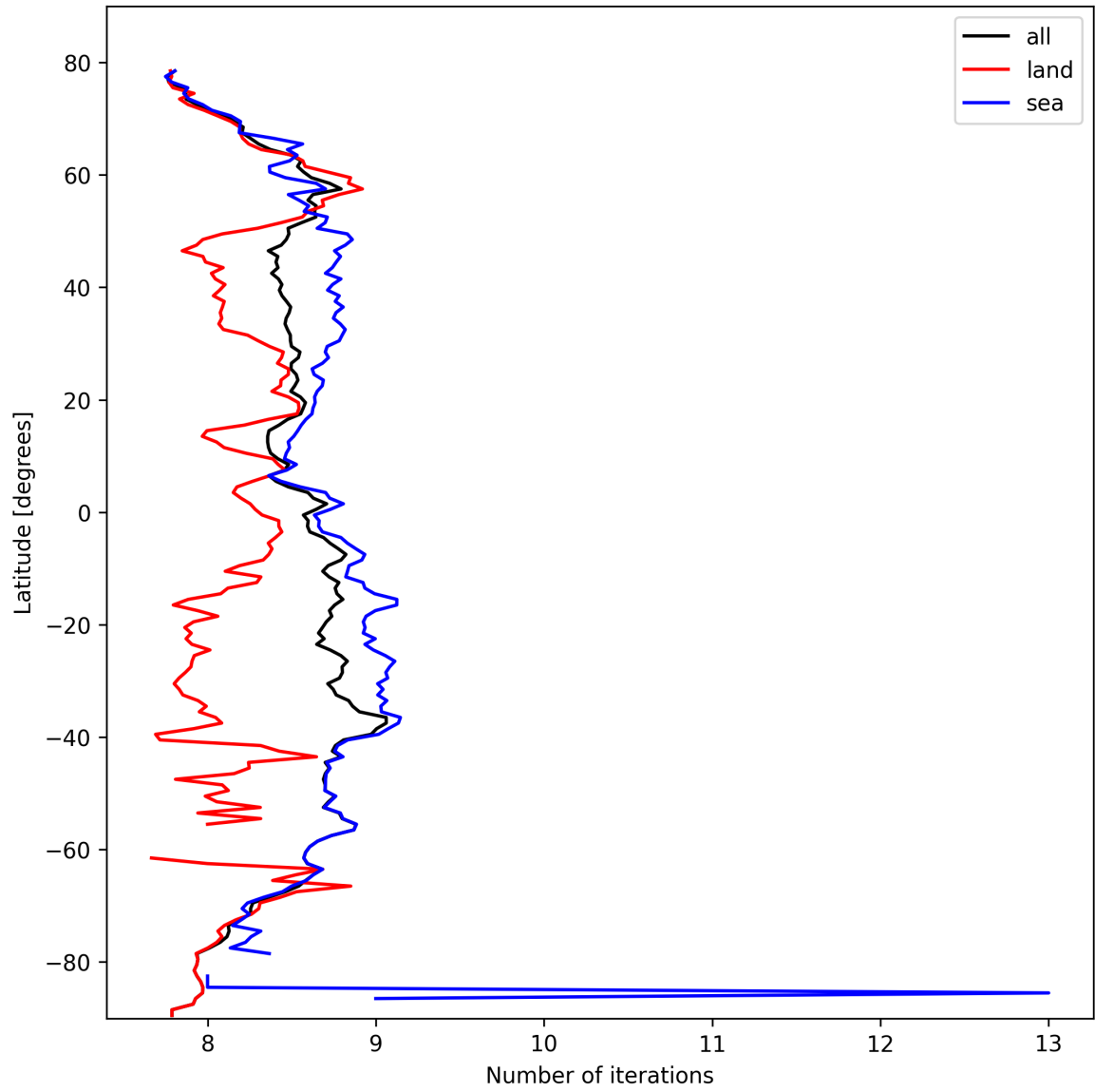
Figure 16: Zonal average of “Number of iterations” for 2025-10-08 to 2025-10-10.
