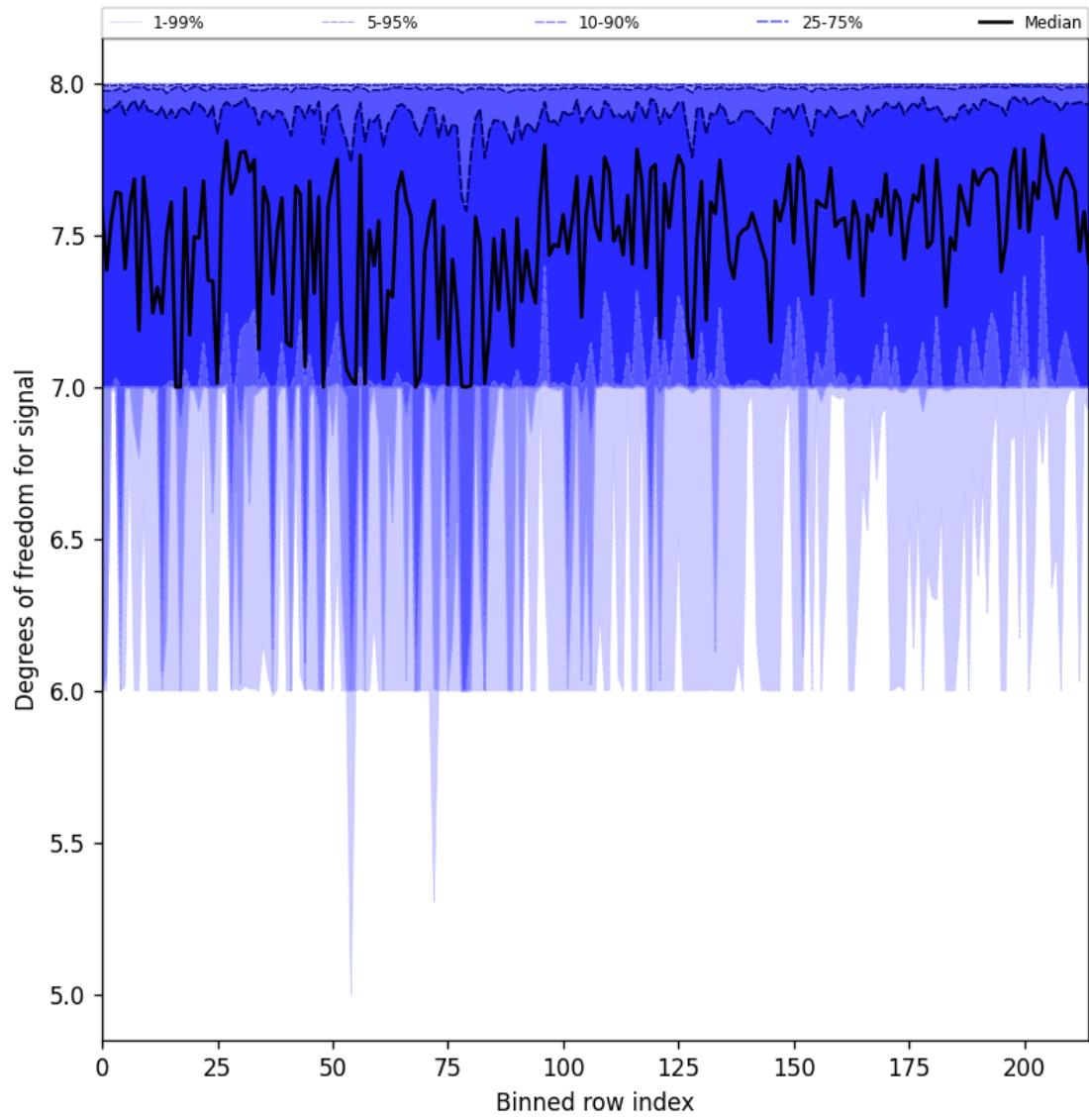
Figure 31: Along track statistics of “Degrees of freedom for signal” for 2025-10-08 to 2025-10-10
