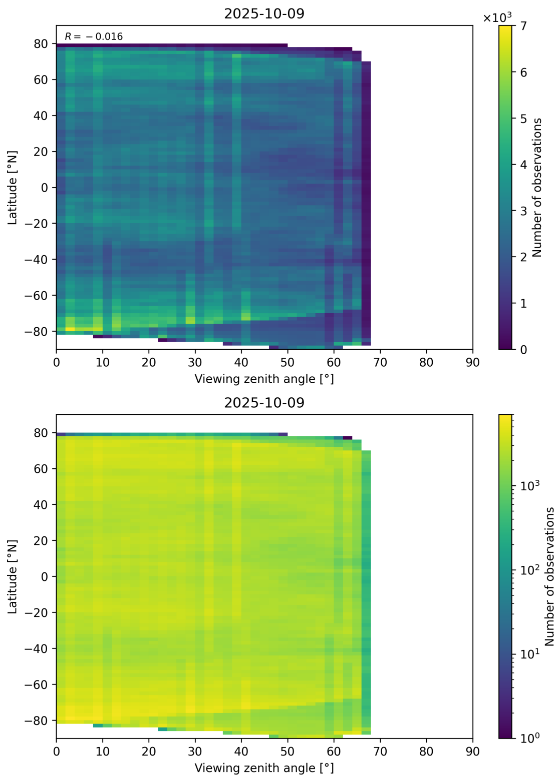
Figure 74: Scatter density plot of “Viewing zenith angle” against “Latitude” for 2025-10-08 to 2025-10-10.
