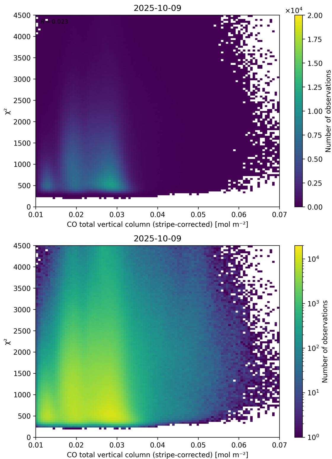
Figure 37: Scatter density plot of “CO total vertical column (stripe-corrected)” against “ \chi^2 ” for 2025-10-08 to 2025-10-10.
