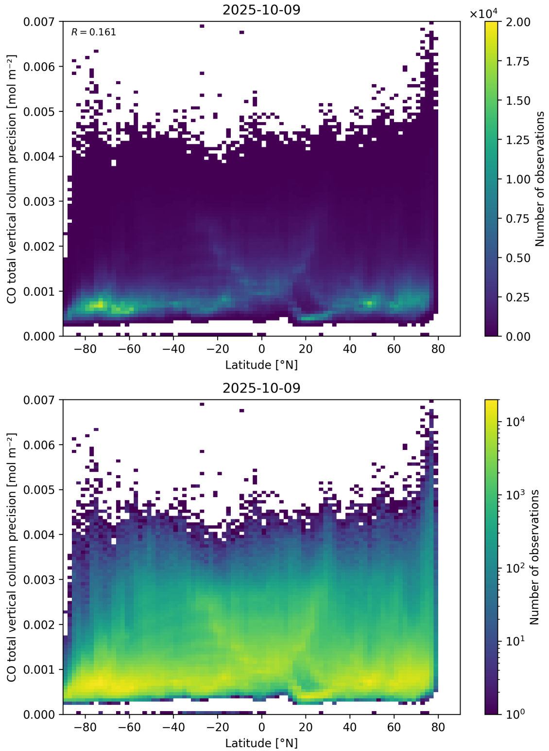
Figure 53: Scatter density plot of “Latitude” against “CO total vertical column precision” for 2025-10-08 to 2025-10-10.
