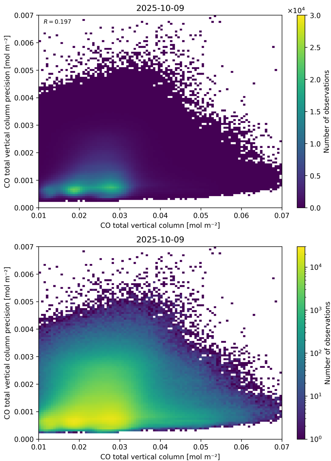
Figure 34: Scatter density plot of “CO total vertical column” against “CO total vertical column precision” for 2025-10-08 to 2025-10-10.
