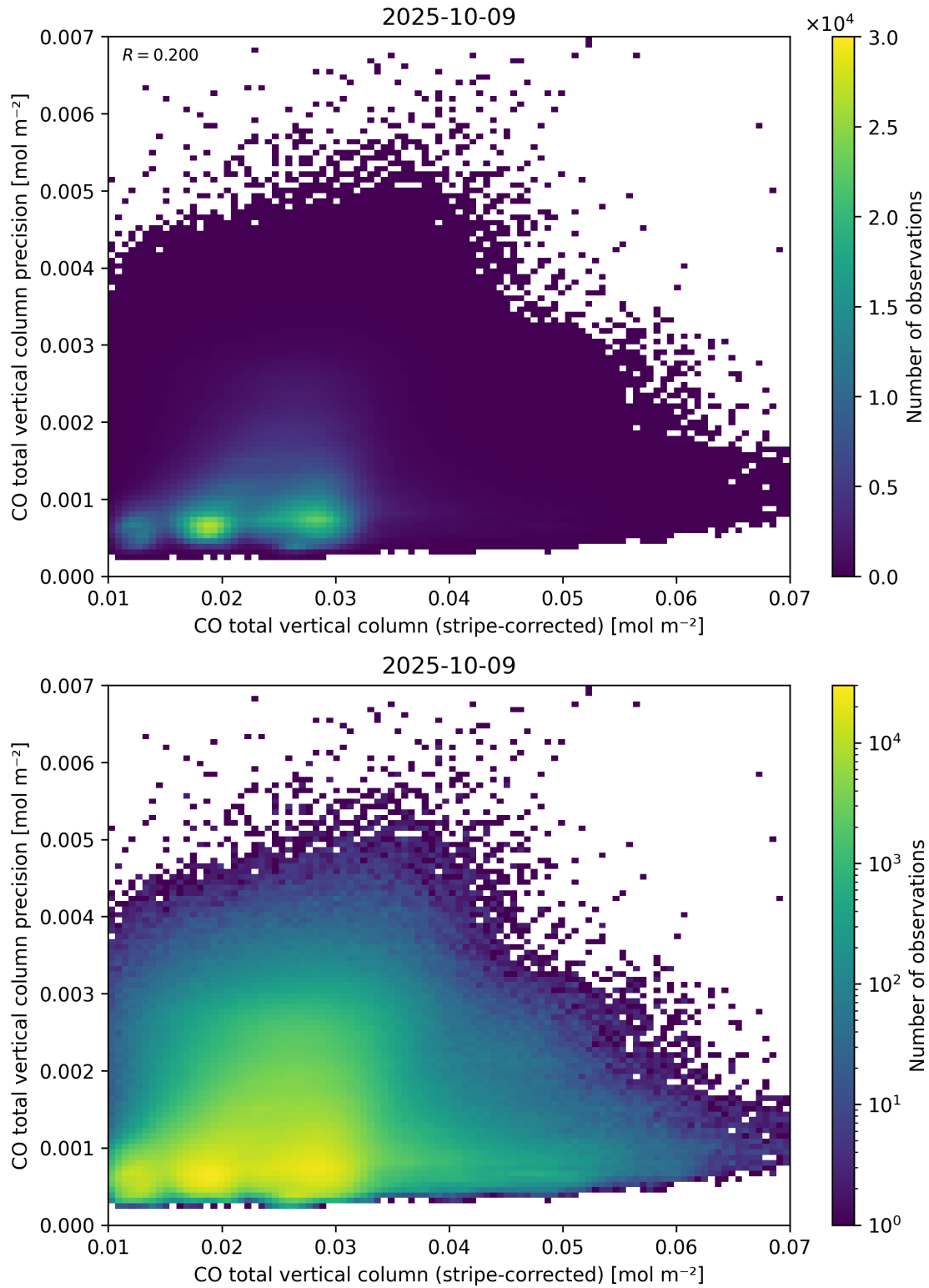
Figure 36: Scatter density plot of “CO total vertical column (stripe-corrected)” against “CO total vertical column precision” for 2025-10-08 to 2025-10-10.
