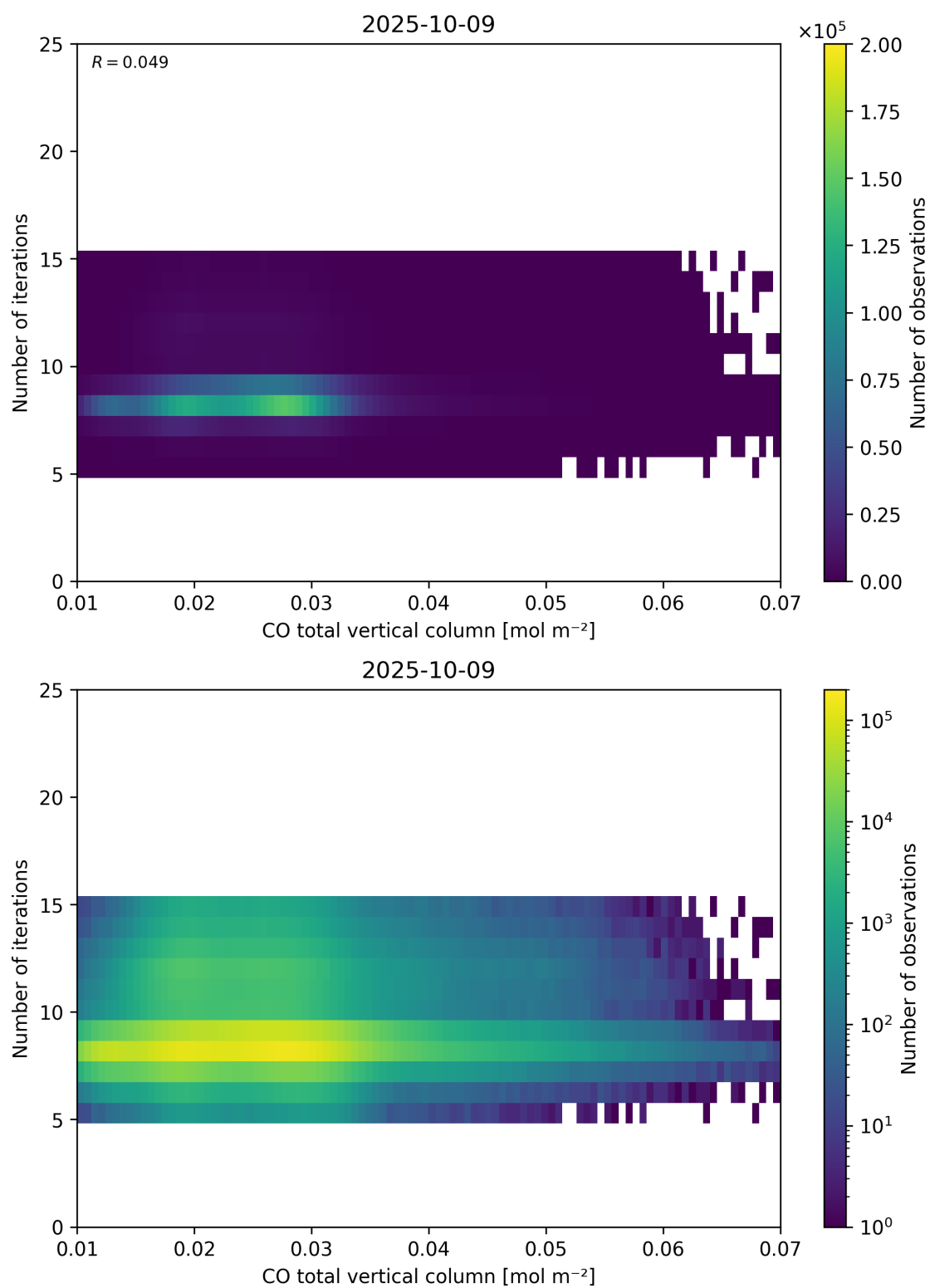
Figure 42: Scatter density plot of “CO total vertical column” against “Number of iterations” for 2025-10-08 to 2025-10-10.
