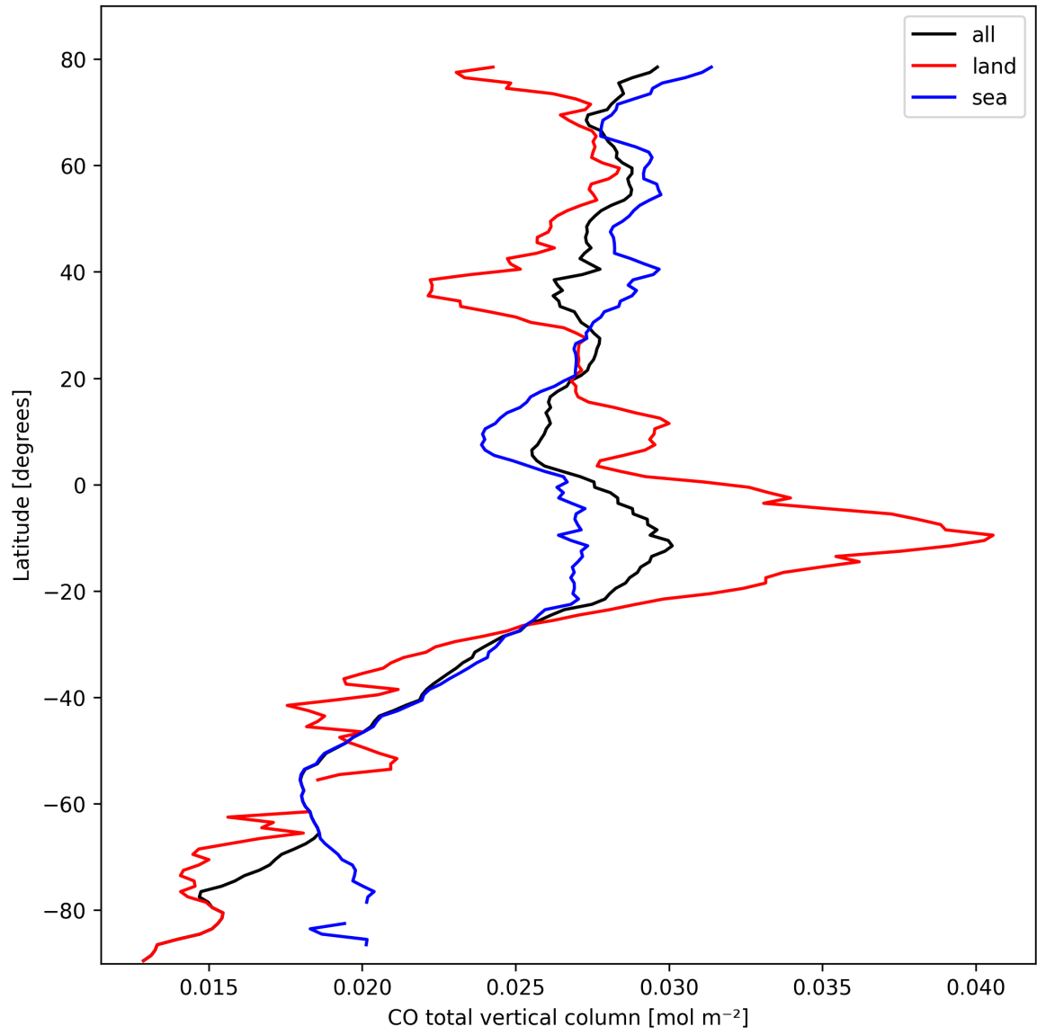
Figure 10: Zonal average of “CO total vertical column” for 2025-10-08 to 2025-10-10.
