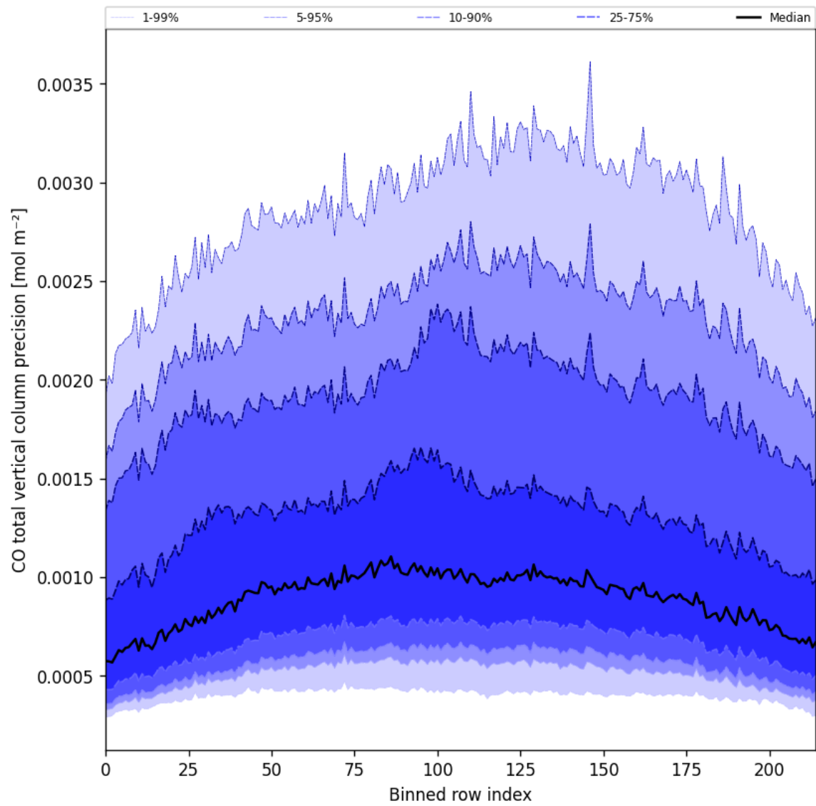
Figure 28: Along track statistics of “CO total vertical column precision” for 2025-10-08 to 2025-10-10
