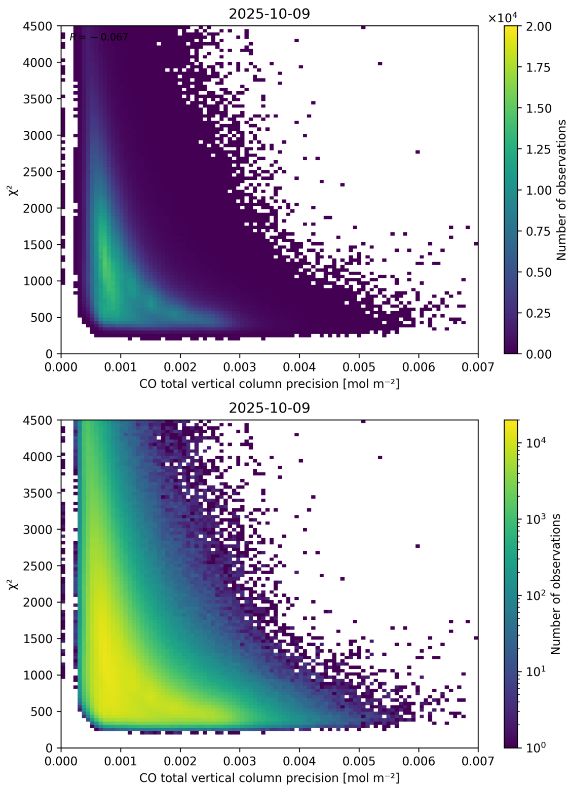
Figure 44: Scatter density plot of “CO total vertical column precision” against “ \chi^2 ” for 2025-10-08 to 2025-10-10.
