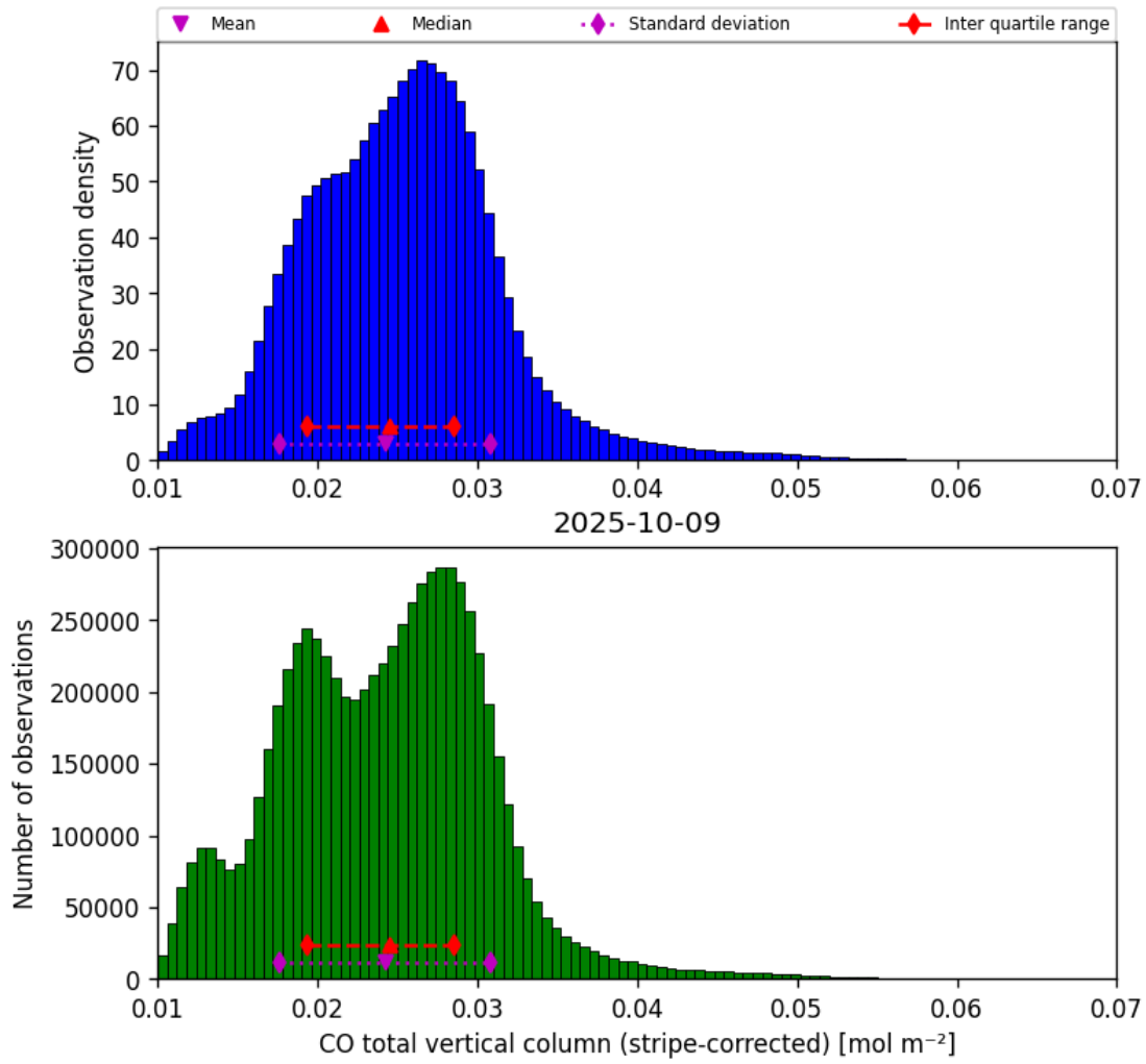
Figure 19: Histogram of “CO total vertical column (stripe-corrected)” for 2025-10-08 to 2025-10-10
