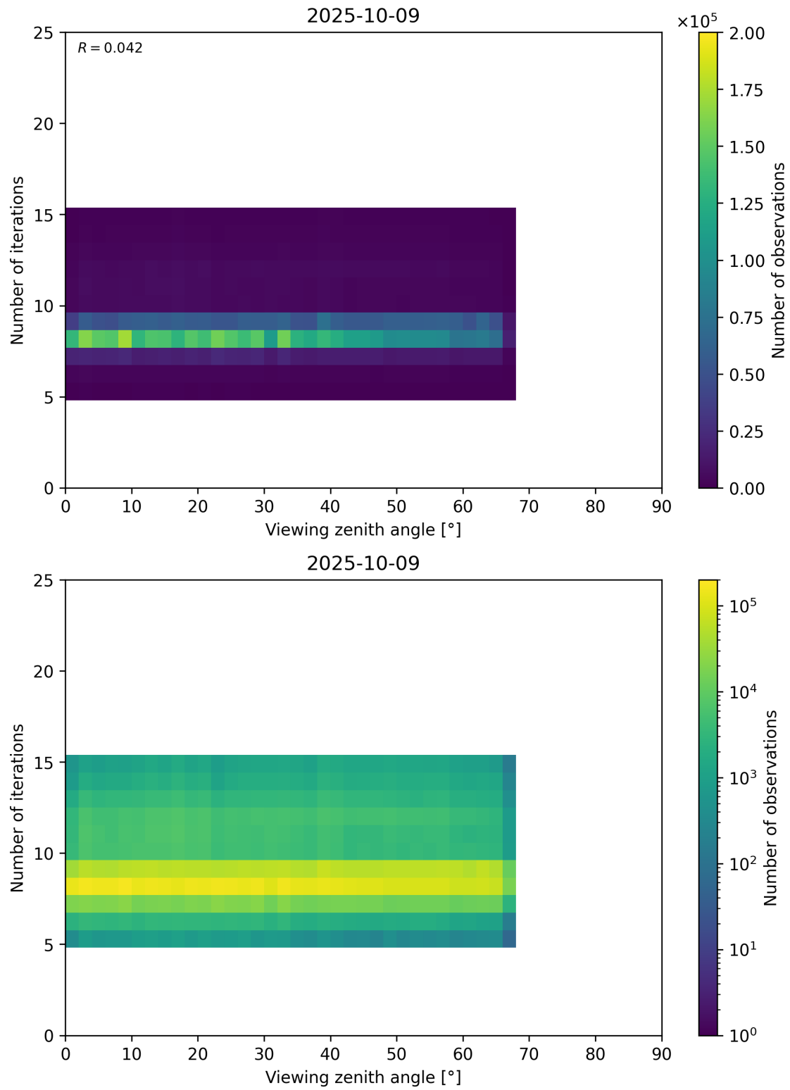
Figure 75: Scatter density plot of “Viewing zenith angle” against “Number of iterations” for 2025-10-08 to 2025-10-10.
