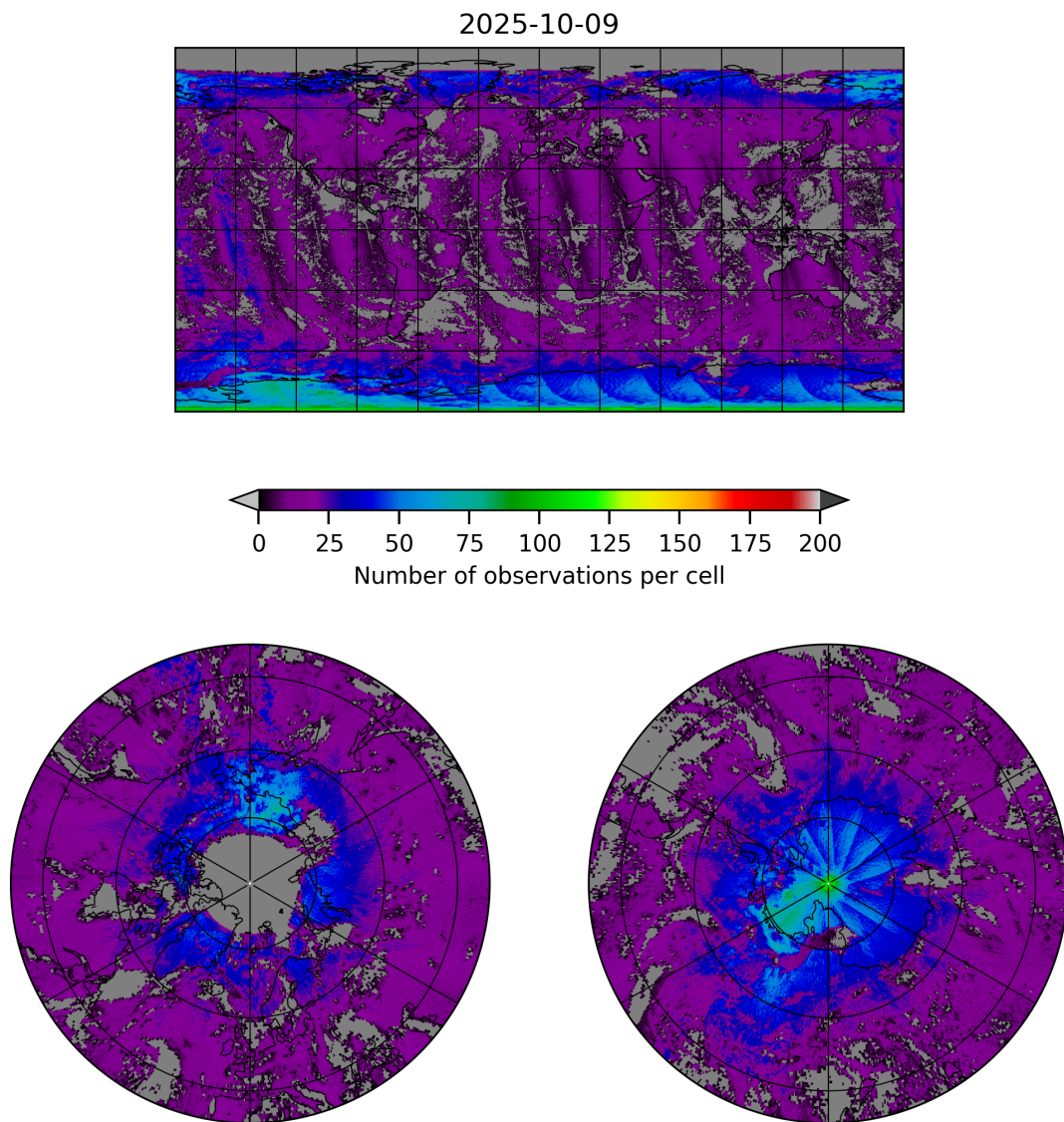
Figure 8: Map of the number of observations for 2025-10-08 to 2025-10-10
