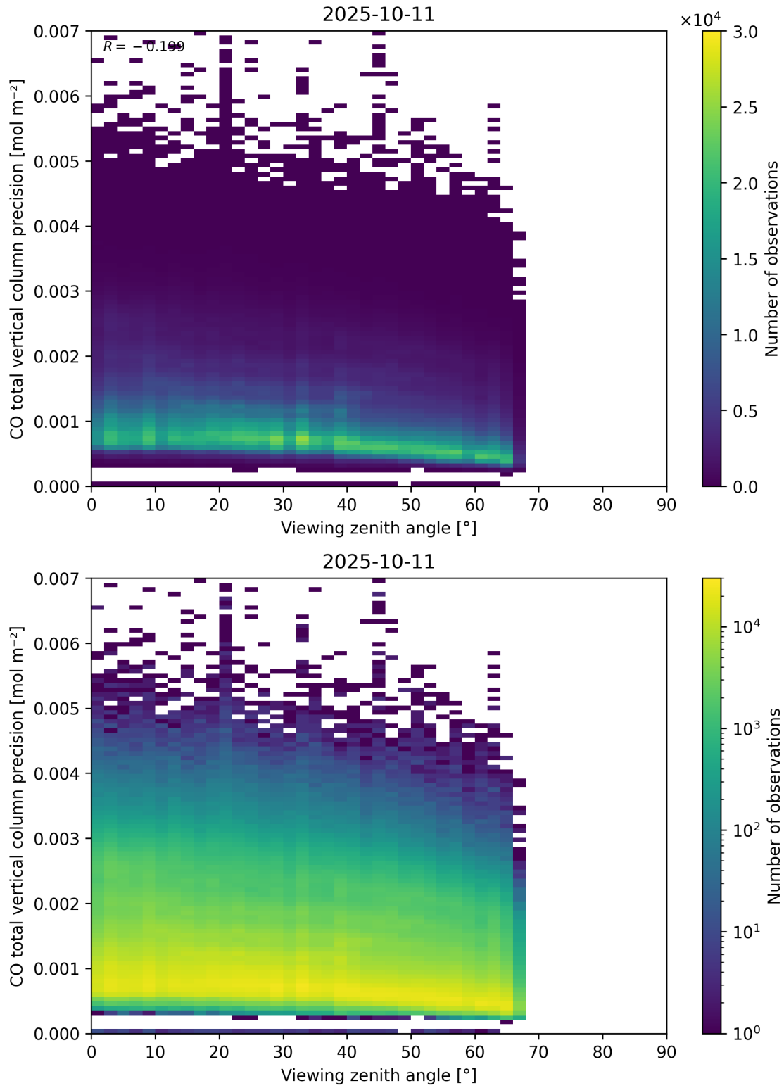
Figure 71: Scatter density plot of “Viewing zenith angle” against “CO total vertical column precision” for 2025-10-11 to 2025-10-12.
