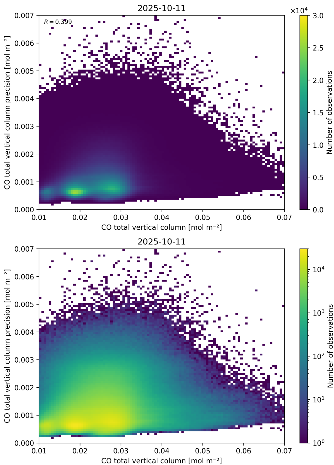
Figure 34: Scatter density plot of “CO total vertical column” against “CO total vertical column precision” for 2025-10-11 to 2025-10-12.
