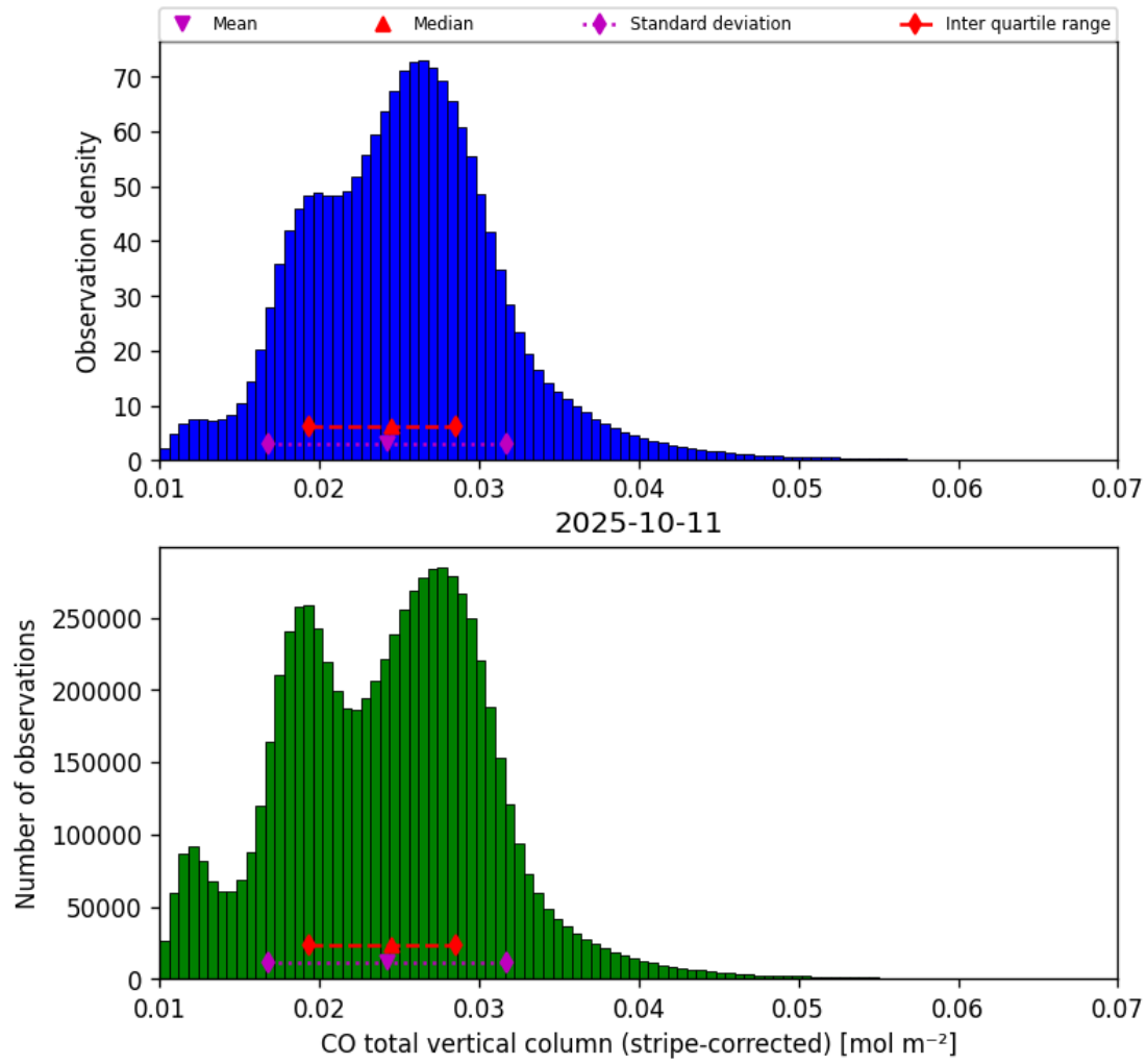
Figure 19: Histogram of “CO total vertical column (stripe-corrected)” for 2025-10-11 to 2025-10-12
