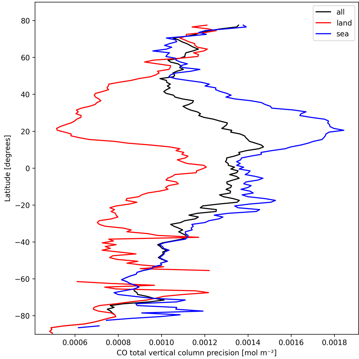
Figure 12: Zonal average of “CO total vertical column precision” for 2025-10-11 to 2025-10-12.
