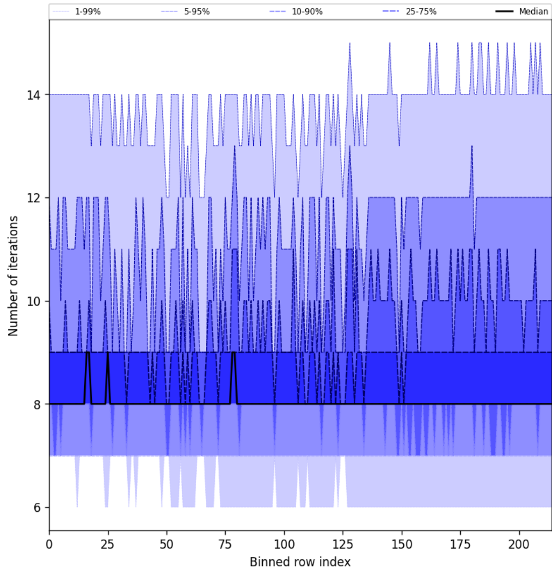
Figure 32: Along track statistics of “Number of iterations” for 2025-10-11 to 2025-10-12
