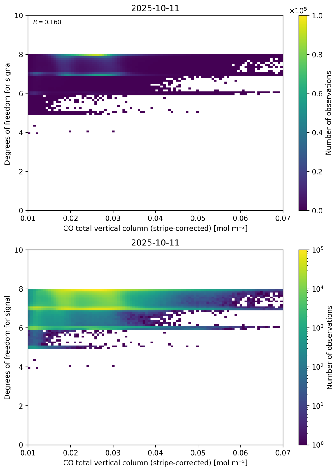
Figure 38: Scatter density plot of “CO total vertical column (stripe-corrected)” against “Degrees of freedom for signal” for 2025-10-11 to 2025-10-12.
