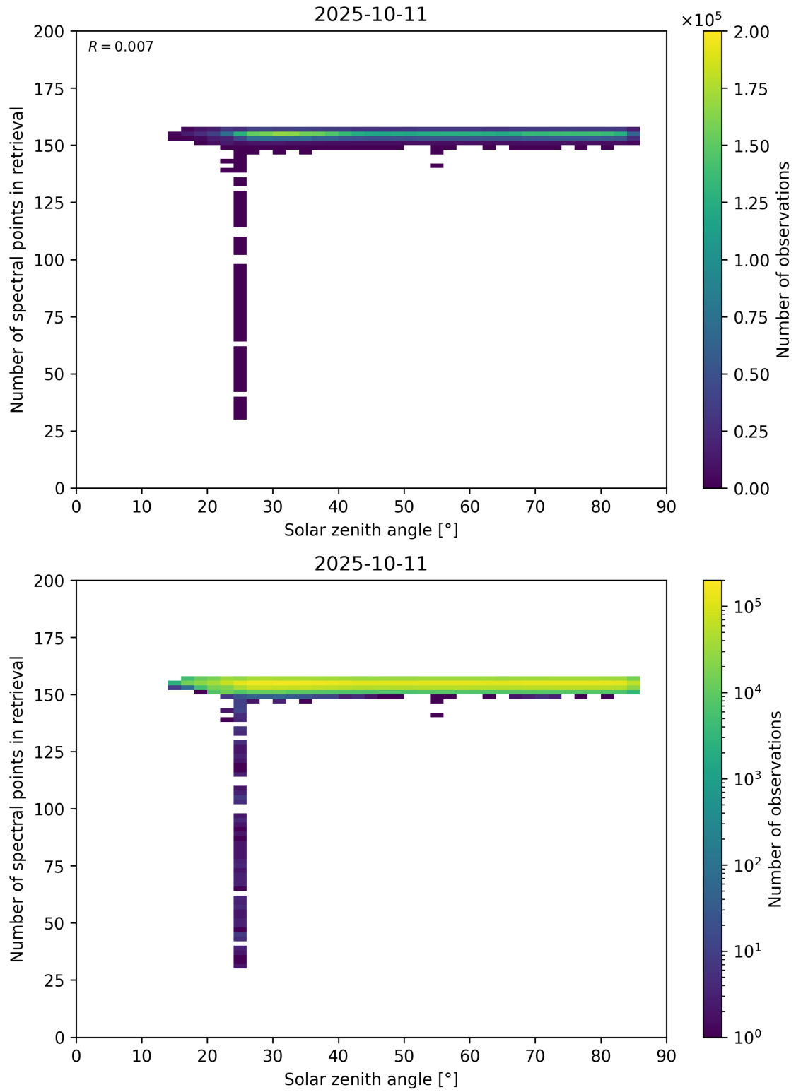
Figure 68: Scatter density plot of “Solar zenith angle” against “Number of spectral points in retrieval” for 2025-10-11 to 2025-10-12.
