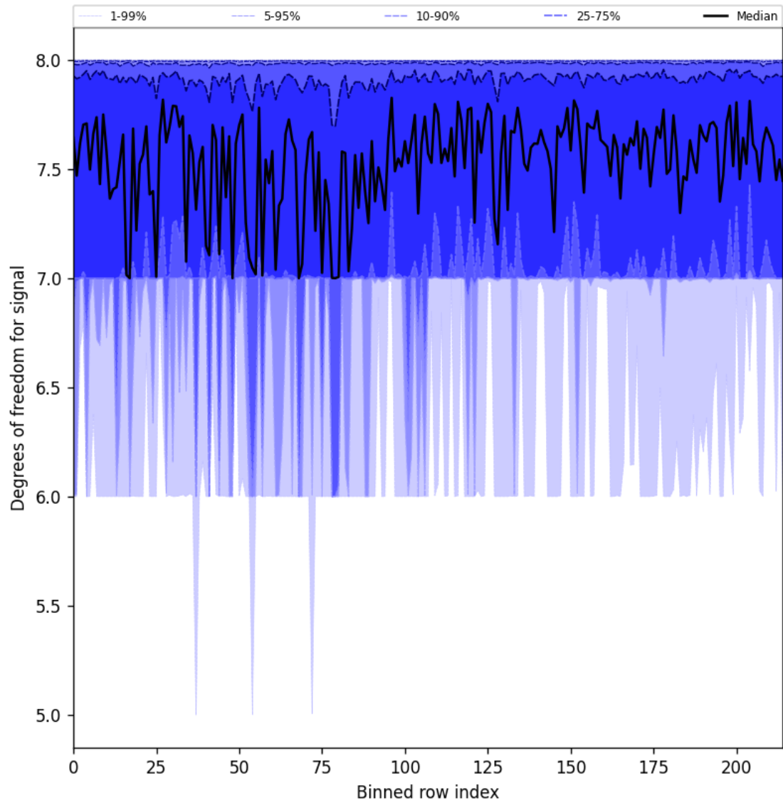
Figure 31: Along track statistics of “Degrees of freedom for signal” for 2025-10-11 to 2025-10-12
