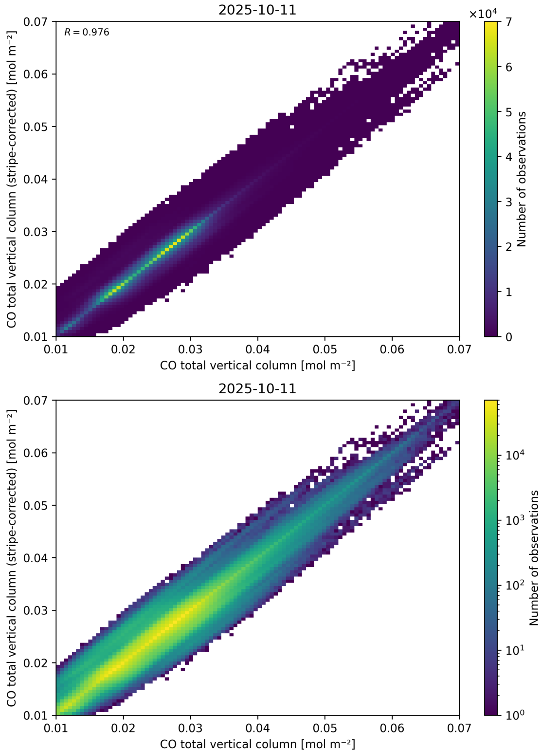
Figure 33: Scatter density plot of “CO total vertical column” against “CO total vertical column (stripe-corrected)” for 2025-10-11 to 2025-10-12.
