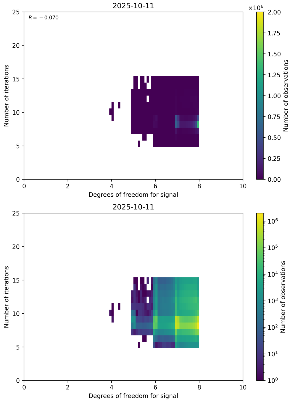
Figure 50: Scatter density plot of “Degrees of freedom for signal” against “Number of iterations” for 2025-10-11 to 2025-10-12.
