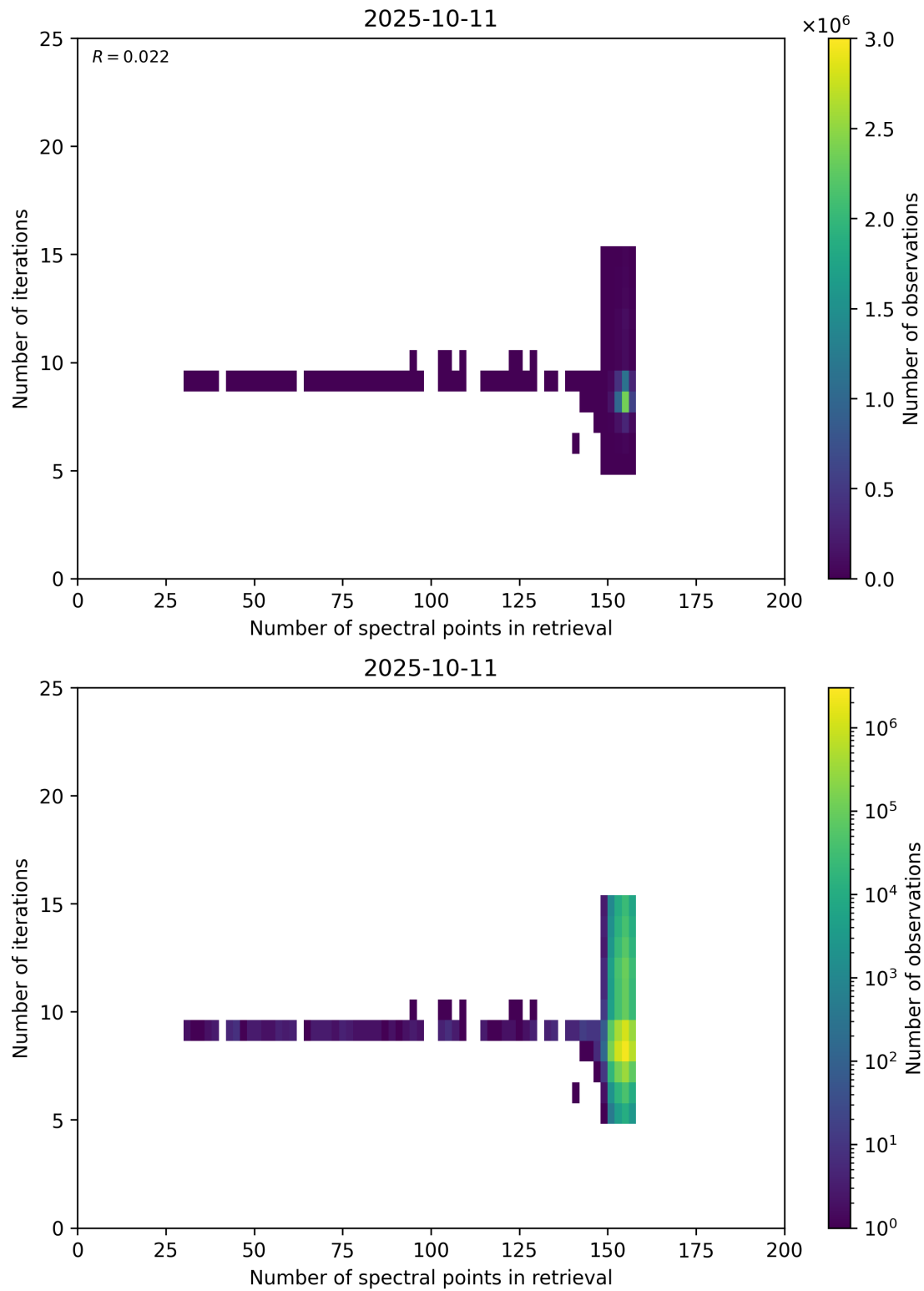
Figure 60: Scatter density plot of “Number of spectral points in retrieval” against “Number of iterations” for 2025-10-11 to 2025-10-12.
