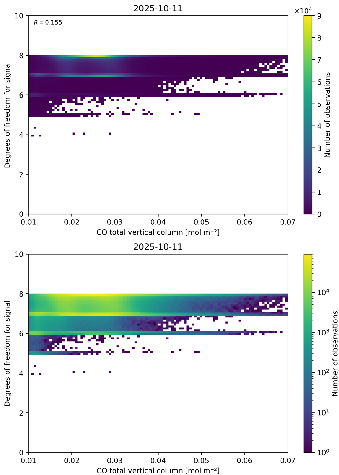
Figure 41: Scatter density plot of “CO total vertical column” against “Degrees of freedom for signal” for 2025-10-11 to 2025-10-12.
