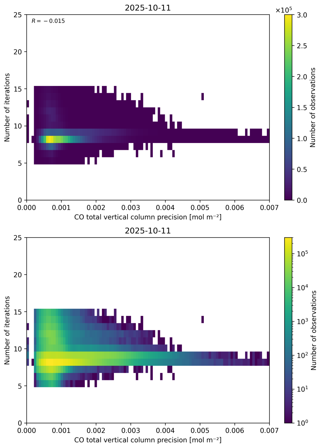
Figure 46: Scatter density plot of “CO total vertical column precision” against “Number of iterations” for 2025-10-11 to 2025-10-12.
