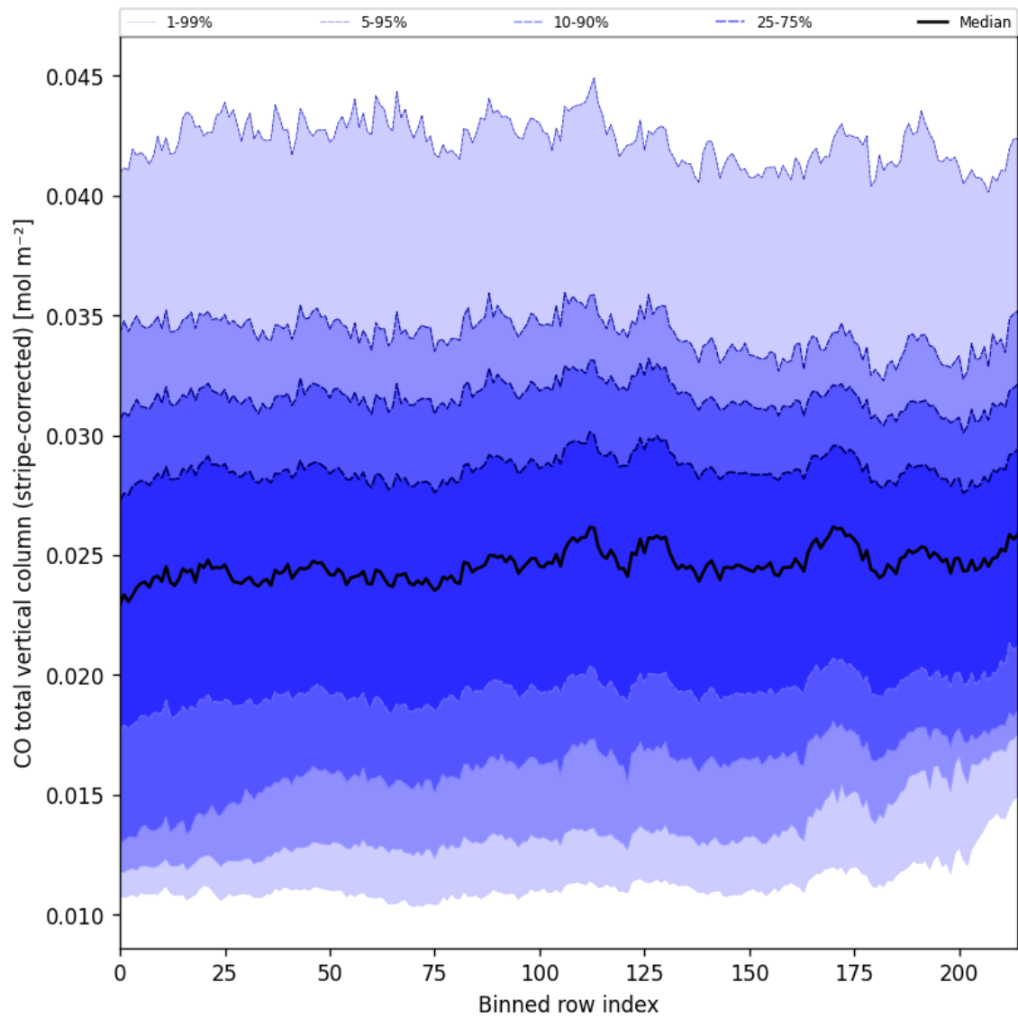
Figure 27: Along track statistics of “CO total vertical column (stripe-corrected)” for 2025-10-11 to 2025-10-12
