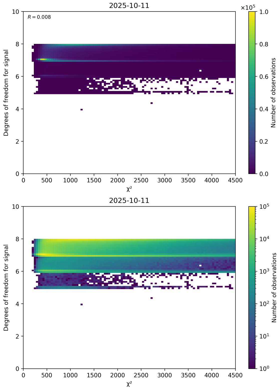
Figure 48: Scatter density plot of “ \chi^2 ” against “Degrees of freedom for signal” for 2025-10-11 to 2025-10-12.
