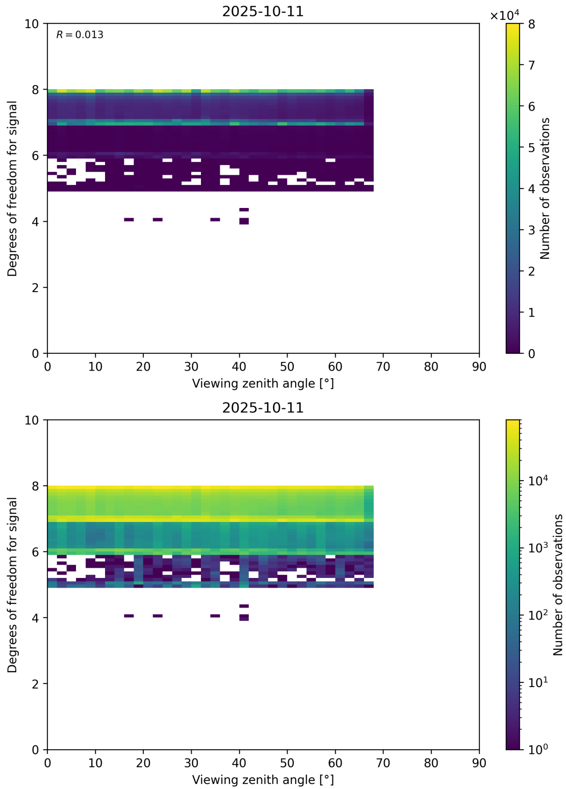
Figure 73: Scatter density plot of “Viewing zenith angle” against “Degrees of freedom for signal” for 2025-10-11 to 2025-10-12.
