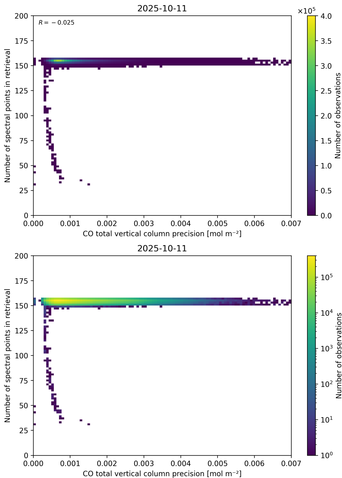
Figure 47: Scatter density plot of “CO total vertical column precision” against “Number of spectral points in retrieval” for 2025-10-11 to 2025-10-12.
