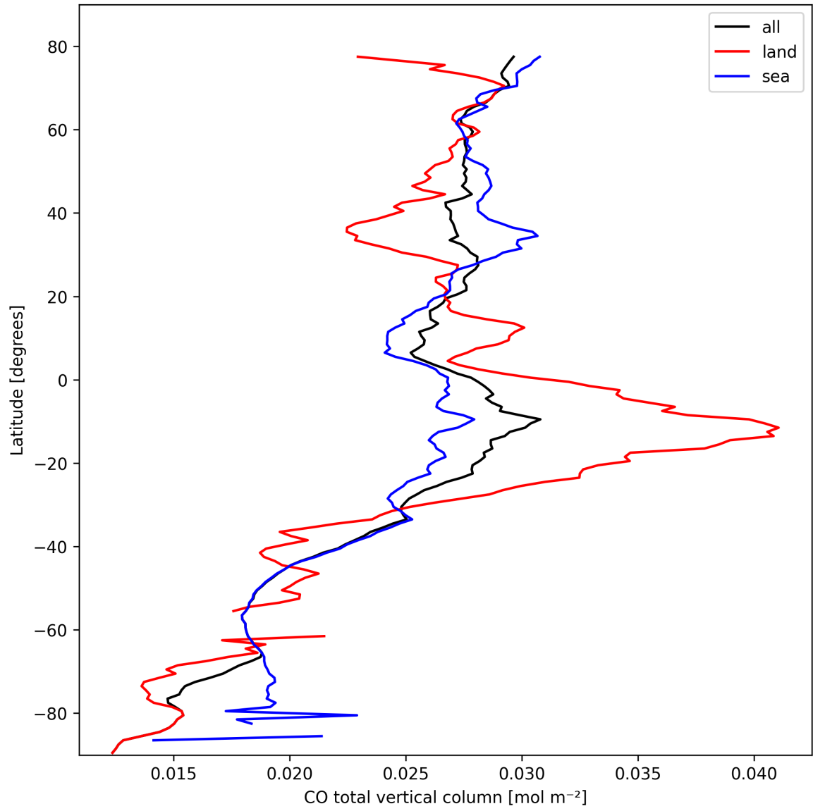
Figure 10: Zonal average of “CO total vertical column” for 2025-10-11 to 2025-10-12.
