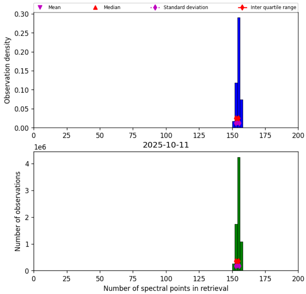
Figure 21: Histogram of “Number of spectral points in retrieval” for 2025-10-11 to 2025-10-12
