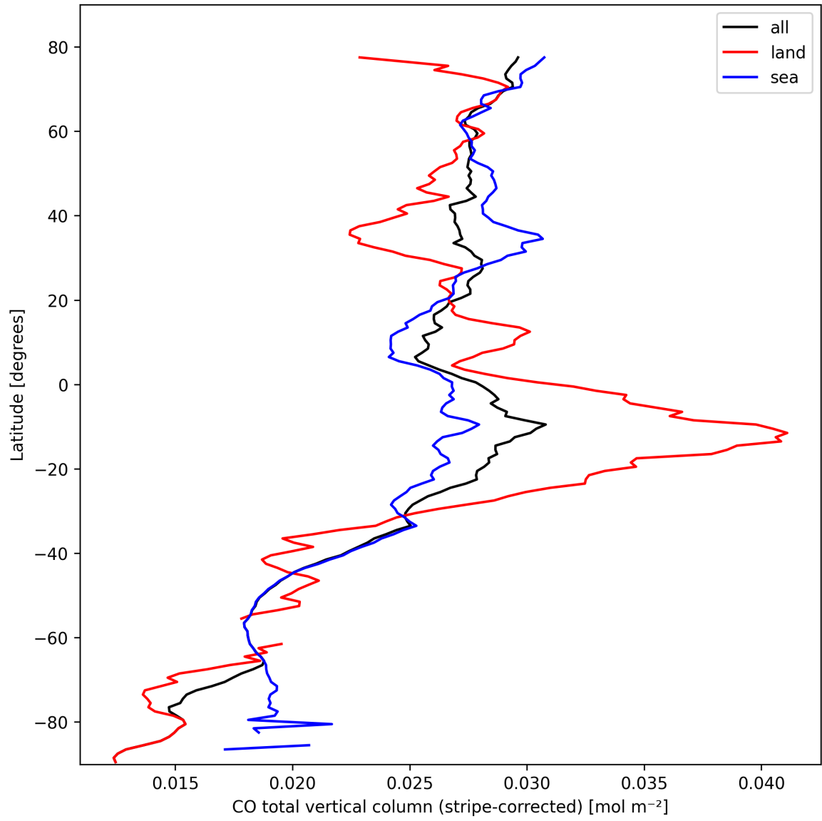
Figure 11: Zonal average of “CO total vertical column (stripe-corrected)” for 2025-10-11 to 2025-10-12.
