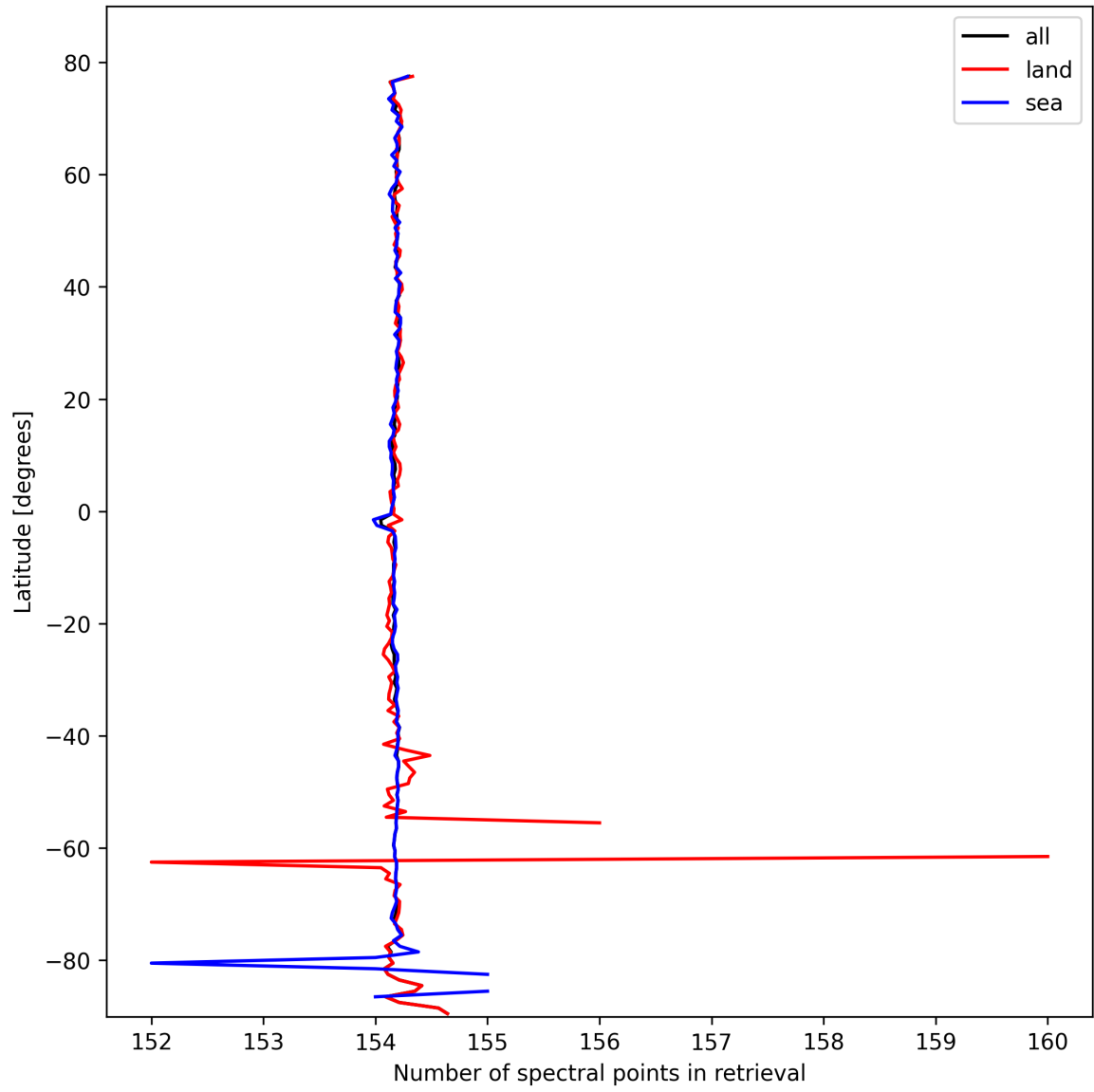
Figure 13: Zonal average of “Number of spectral points in retrieval” for 2025-10-11 to 2025-10-12.
