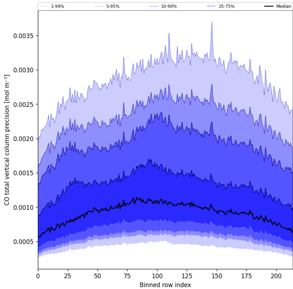
Figure 28: Along track statistics of “CO total vertical column precision” for 2025-10-11 to 2025-10-12
