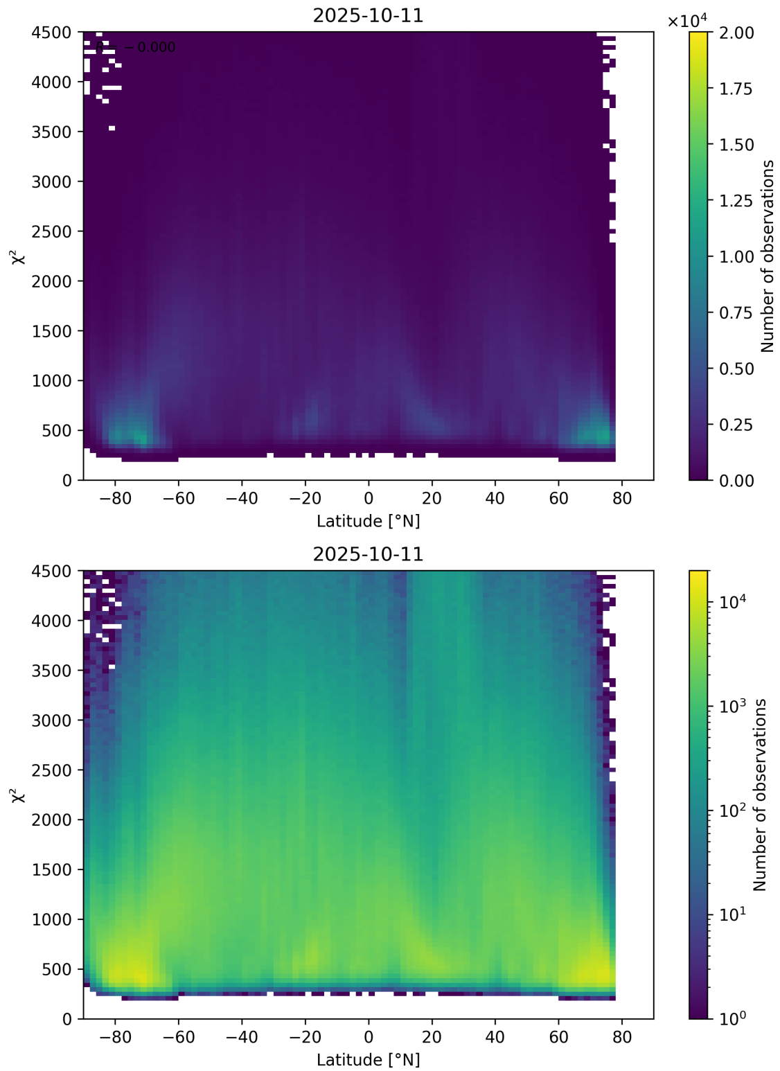
Figure 54: Scatter density plot of “Latitude” against “ \chi^2 ” for 2025-10-11 to 2025-10-12.
