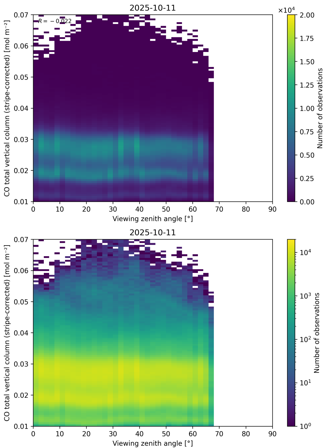
Figure 70: Scatter density plot of “Viewing zenith angle” against “CO total vertical column (stripe-corrected)” for 2025-10-11 to 2025-10-12.
