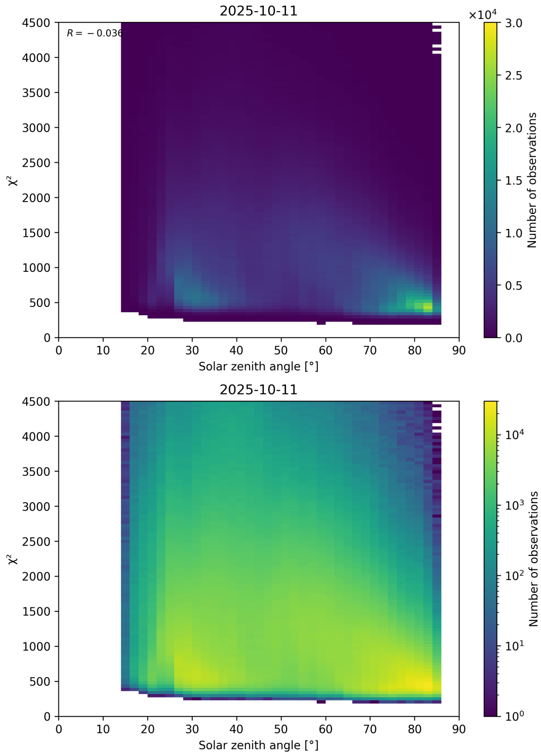
Figure 64: Scatter density plot of “Solar zenith angle” against “ \chi^2 ” for 2025-10-11 to 2025-10-12.
