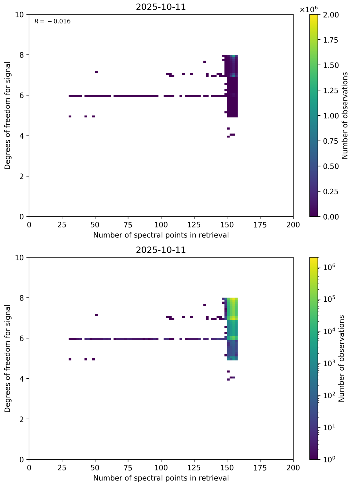
Figure 59: Scatter density plot of “Number of spectral points in retrieval” against “Degrees of freedom for signal” for 2025-10-11 to 2025-10-12.
