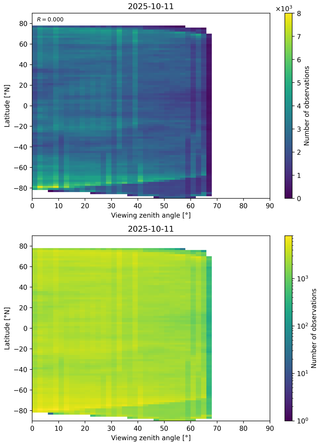
Figure 74: Scatter density plot of “Viewing zenith angle” against “Latitude” for 2025-10-11 to 2025-10-12.
