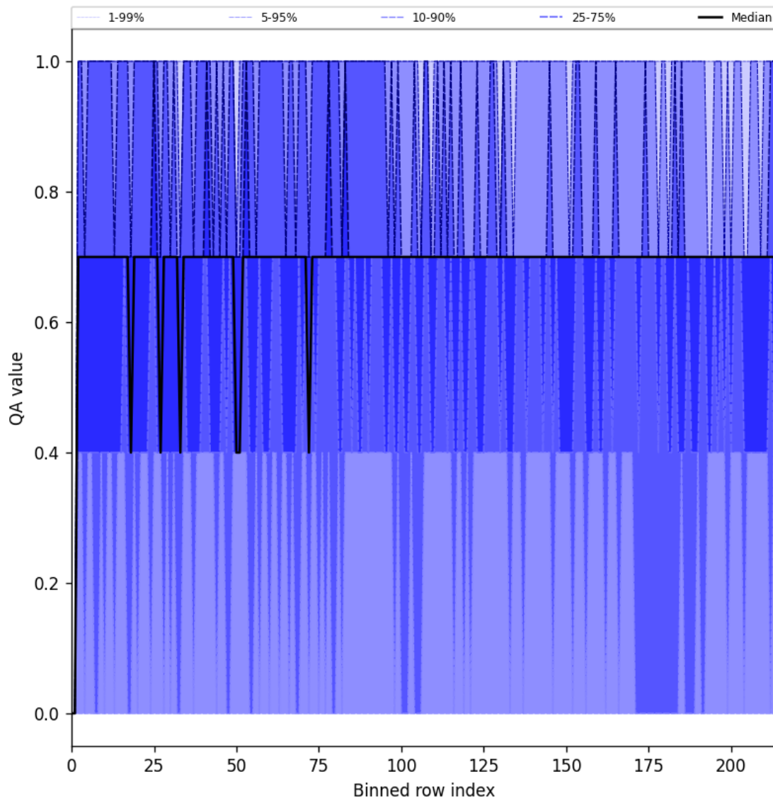
Figure 25: Along track statistics of “QA value” for 2025-10-11 to 2025-10-12
