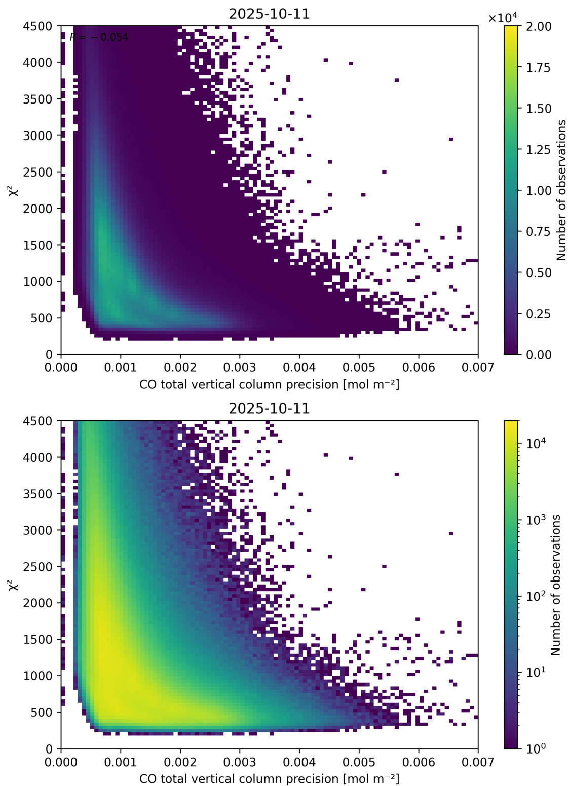
Figure 44: Scatter density plot of “CO total vertical column precision” against “ \chi^2 ” for 2025-10-11 to 2025-10-12.
