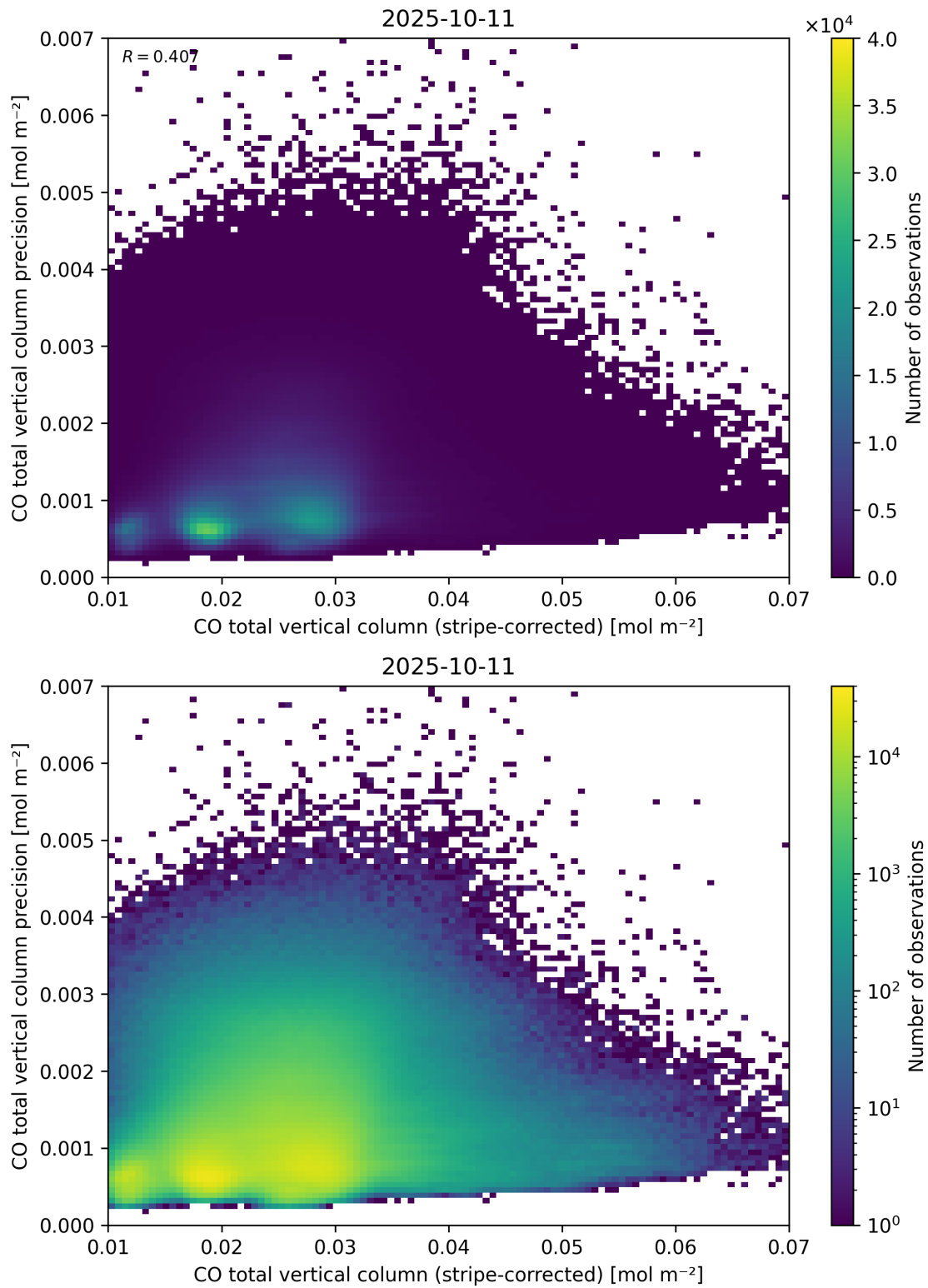
Figure 36: Scatter density plot of “CO total vertical column (stripe-corrected)” against “CO total vertical column precision” for 2025-10-11 to 2025-10-12.
