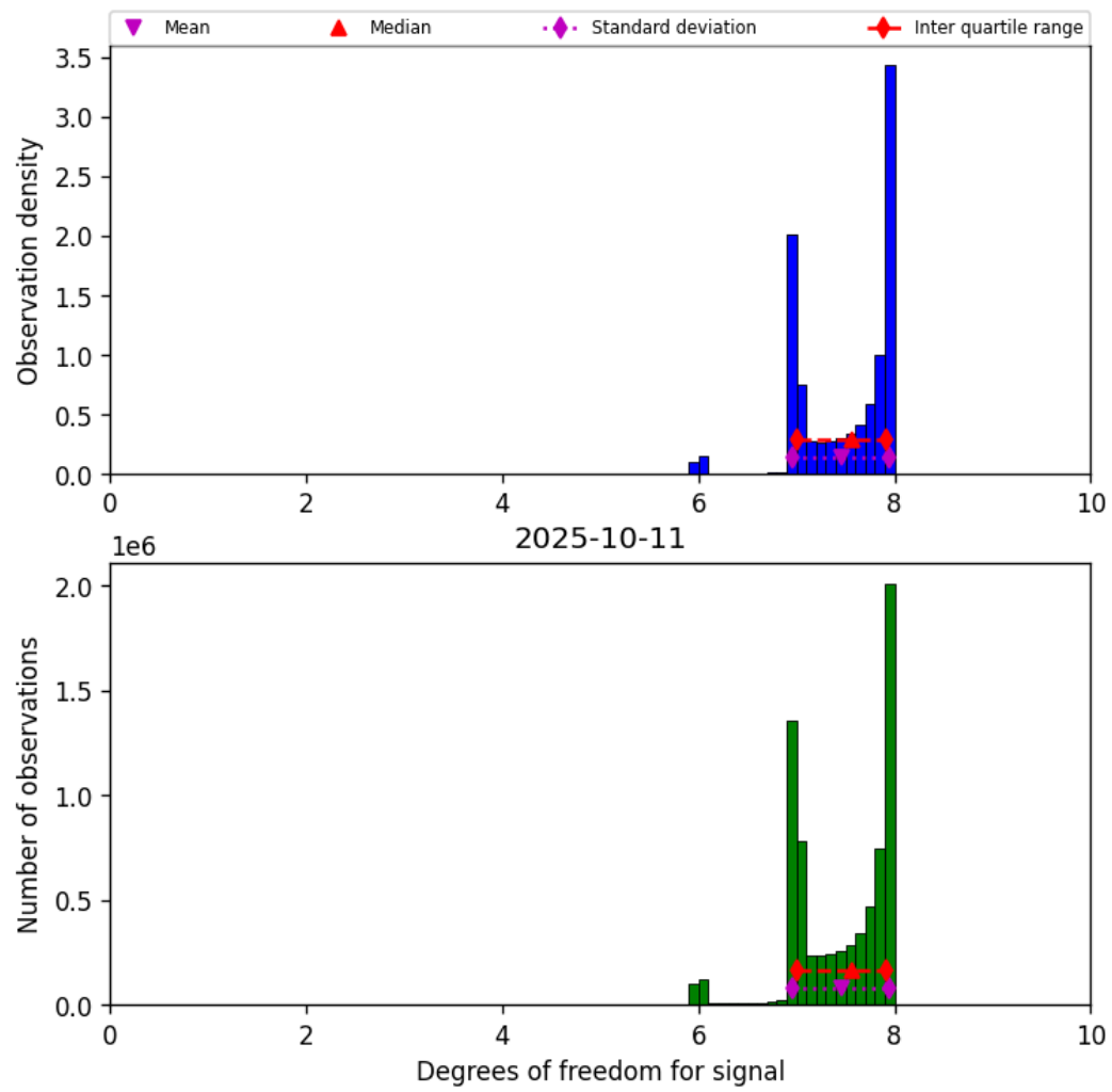
Figure 23: Histogram of “Degrees of freedom for signal” for 2025-10-11 to 2025-10-12
