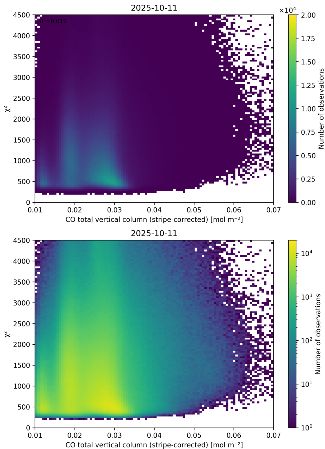
Figure 37: Scatter density plot of “CO total vertical column (stripe-corrected)” against “ \chi^2 ” for 2025-10-11 to 2025-10-12.
