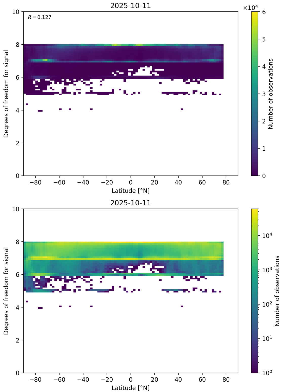
Figure 55: Scatter density plot of “Latitude” against “Degrees of freedom for signal” for 2025-10-11 to 2025-10-12.
