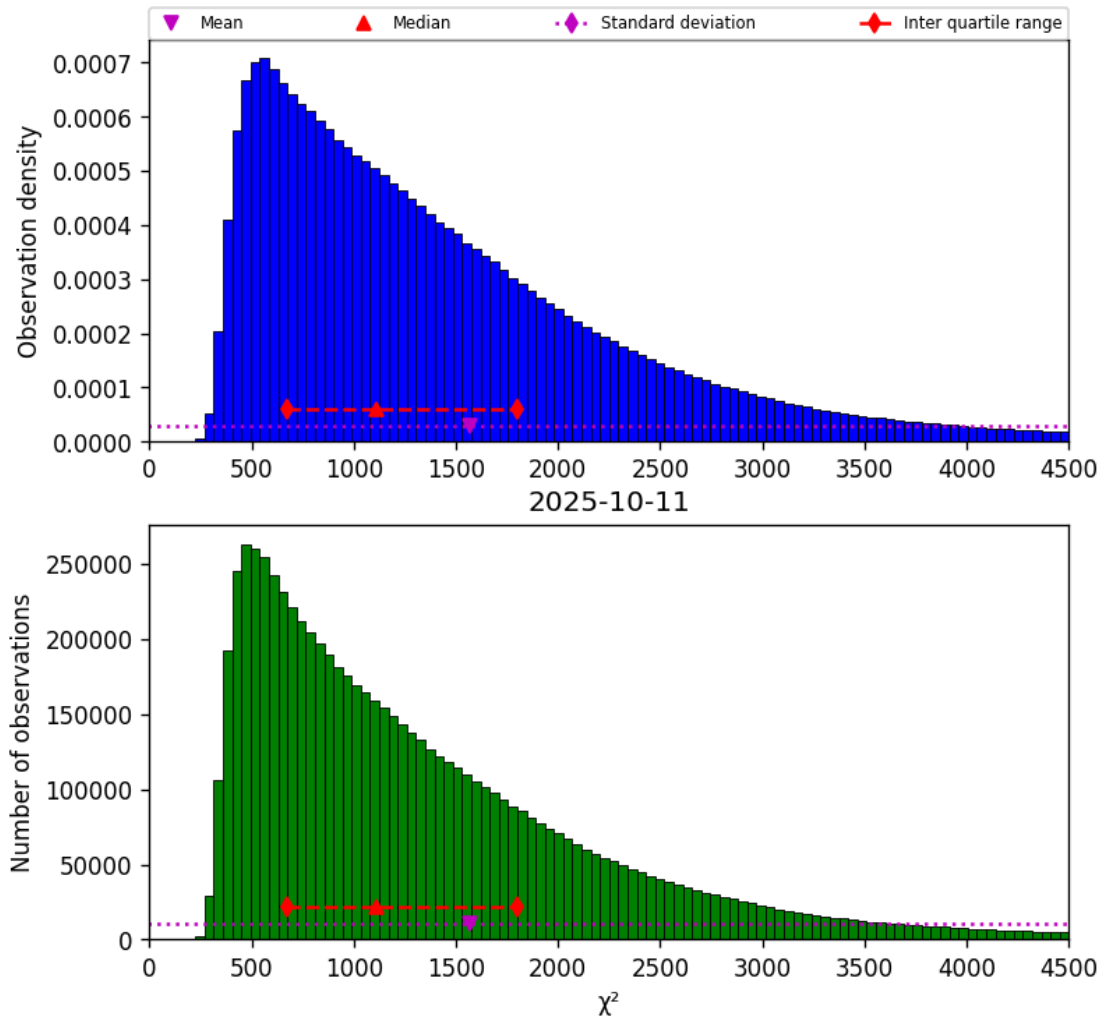
Figure 22: Histogram of “ \chi^2 ” for 2025-10-11 to 2025-10-12
