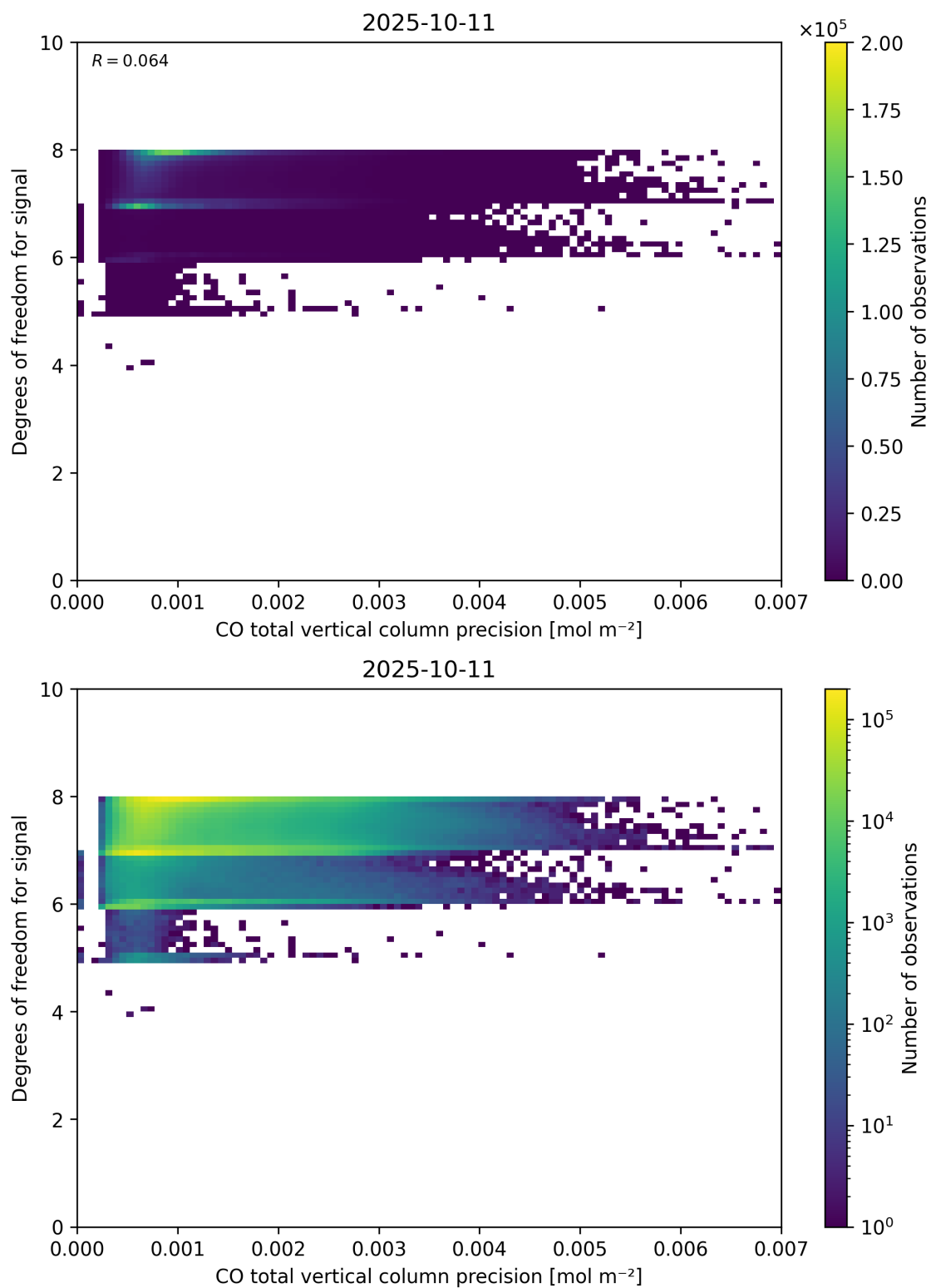
Figure 45: Scatter density plot of “CO total vertical column precision” against “Degrees of freedom for signal” for 2025-10-11 to 2025-10-12.
