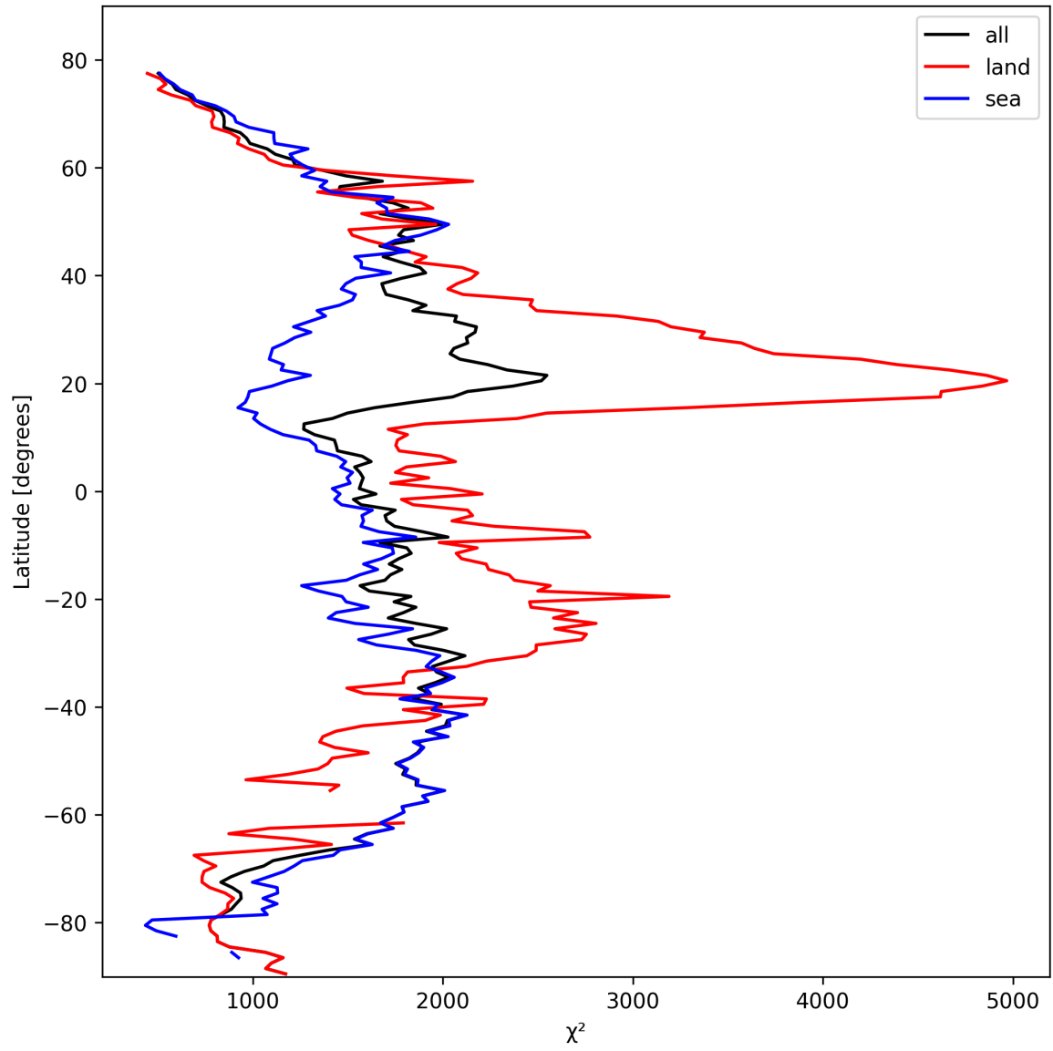
Figure 14: Zonal average of “ \chi^2 ” for 2025-10-11 to 2025-10-12.
