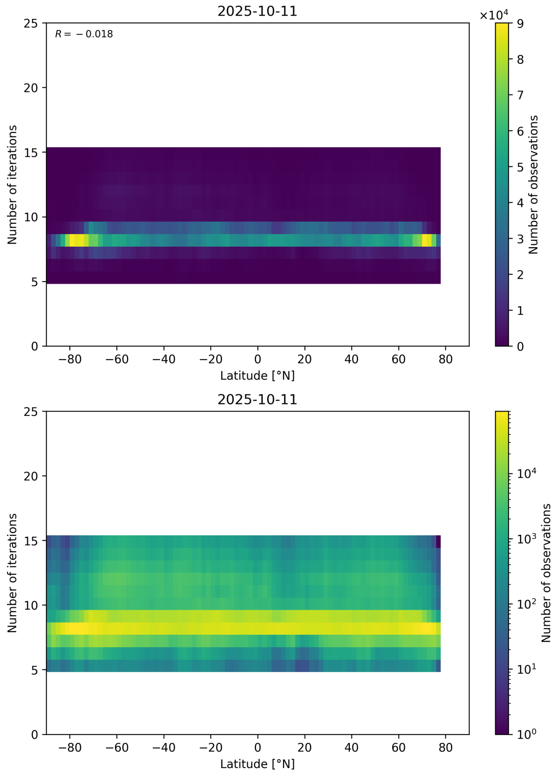
Figure 56: Scatter density plot of “Latitude” against “Number of iterations” for 2025-10-11 to 2025-10-12.
