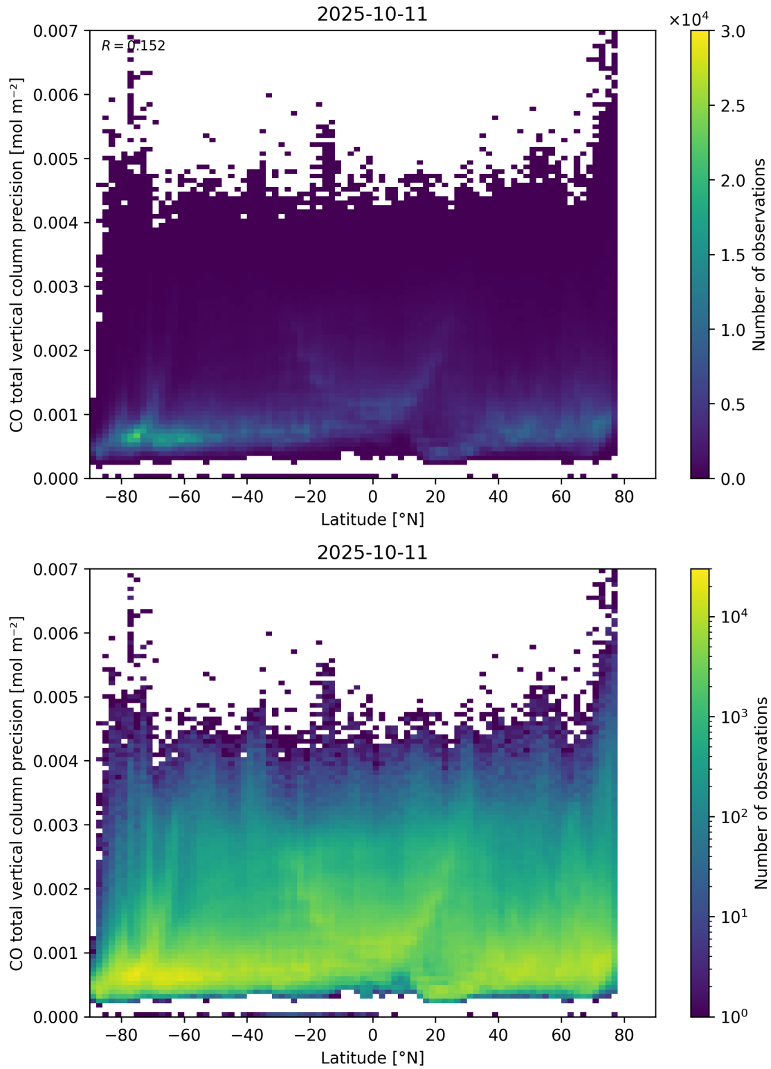
Figure 53: Scatter density plot of “Latitude” against “CO total vertical column precision” for 2025-10-11 to 2025-10-12.
