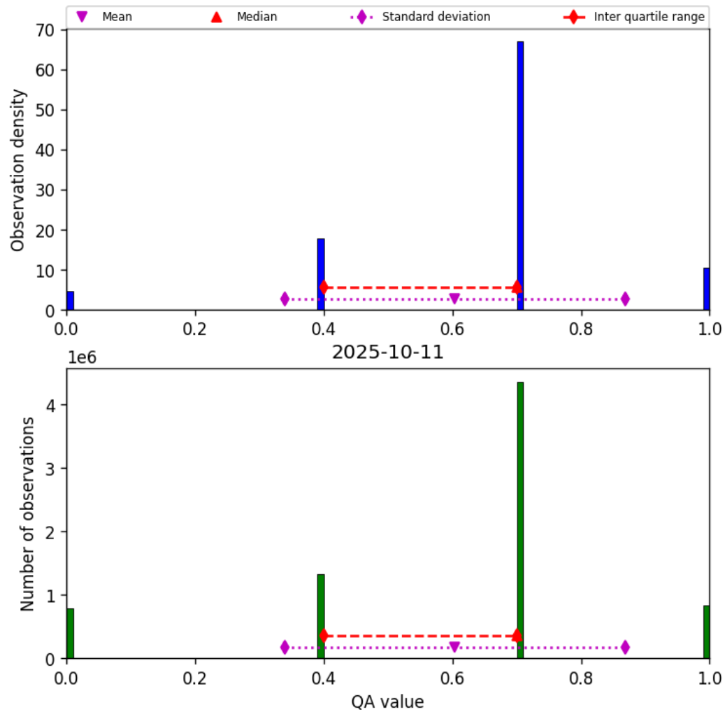
Figure 17: Histogram of “QA value” for 2025-10-11 to 2025-10-12
