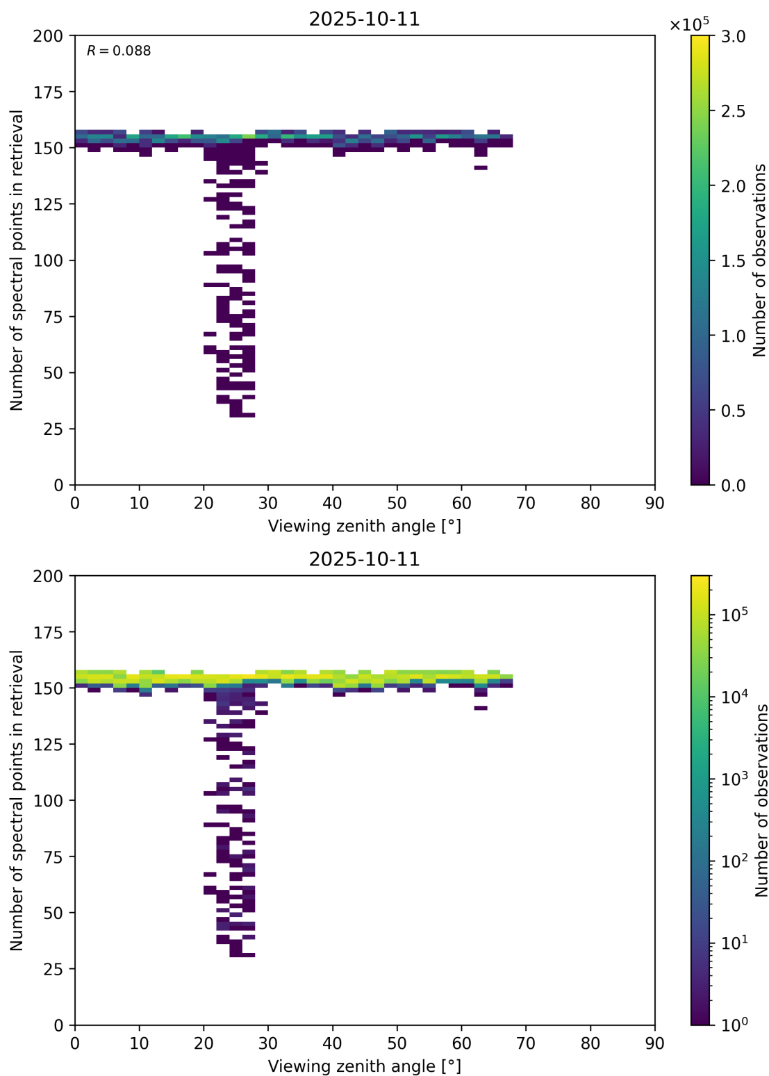
Figure 76: Scatter density plot of “Viewing zenith angle” against “Number of spectral points in retrieval” for 2025-10-11 to 2025-10-12.
