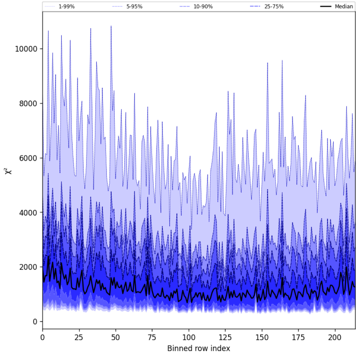
Figure 30: Along track statistics of “ \chi^2 ” for 2025-10-11 to 2025-10-12
