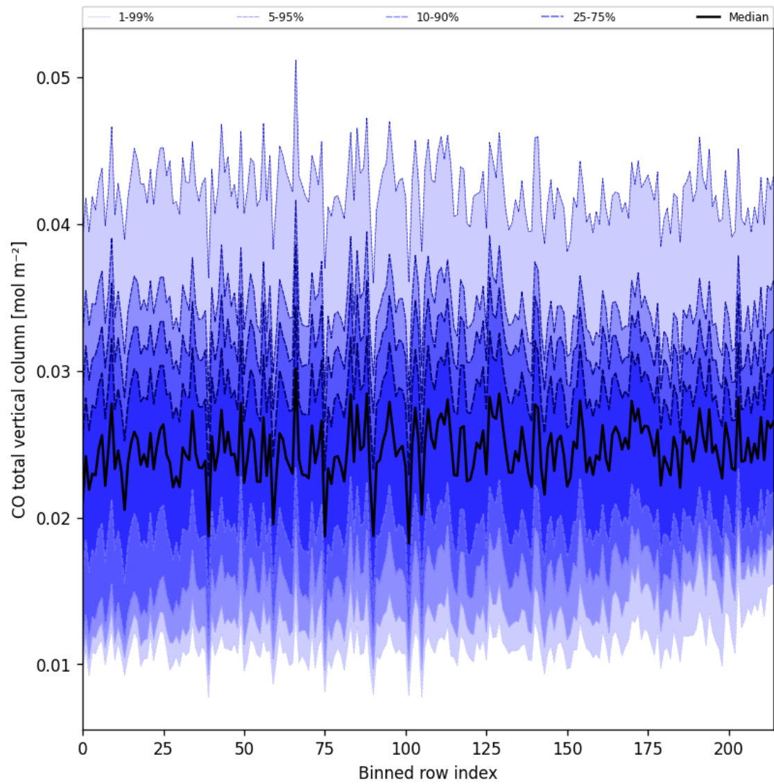
Figure 26: Along track statistics of “CO total vertical column” for 2025-10-11 to 2025-10-12
