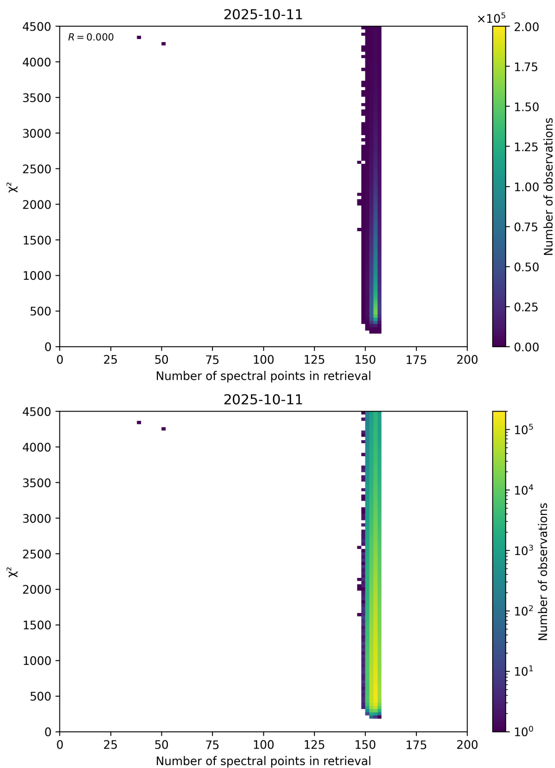
Figure 58: Scatter density plot of “Number of spectral points in retrieval” against “ \chi^2 ” for 2025-10-11 to 2025-10-12.
