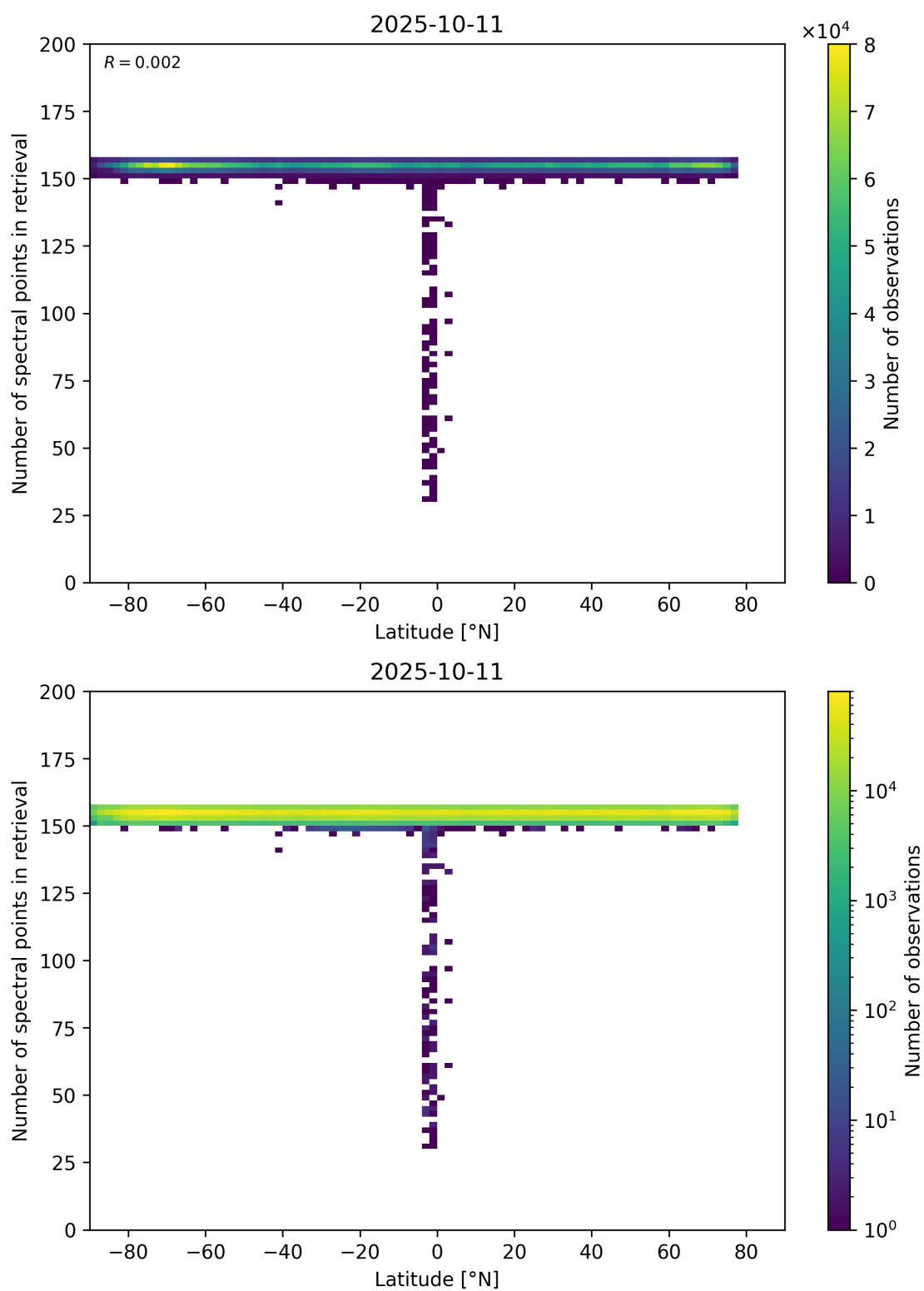
Figure 57: Scatter density plot of “Latitude” against “Number of spectral points in retrieval” for 2025-10-11 to 2025-10-12.
