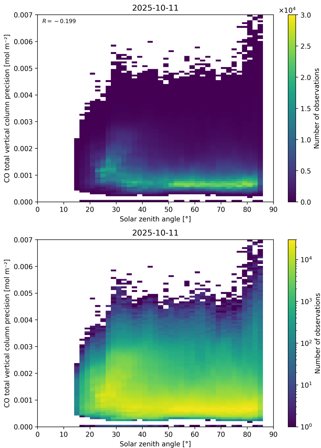
Figure 63: Scatter density plot of “Solar zenith angle” against “CO total vertical column precision” for 2025-10-11 to 2025-10-12.
