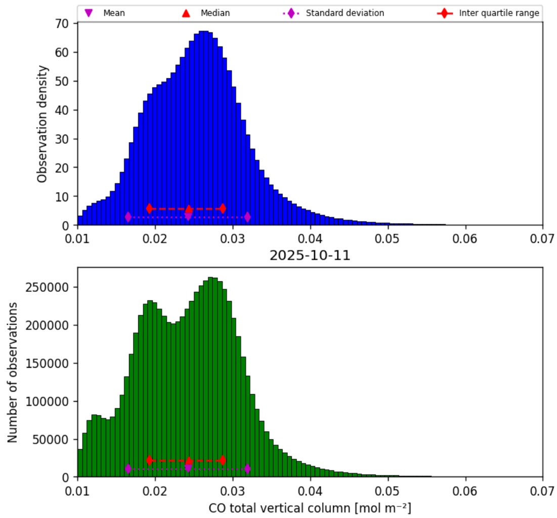
Figure 18: Histogram of “CO total vertical column” for 2025-10-11 to 2025-10-12
