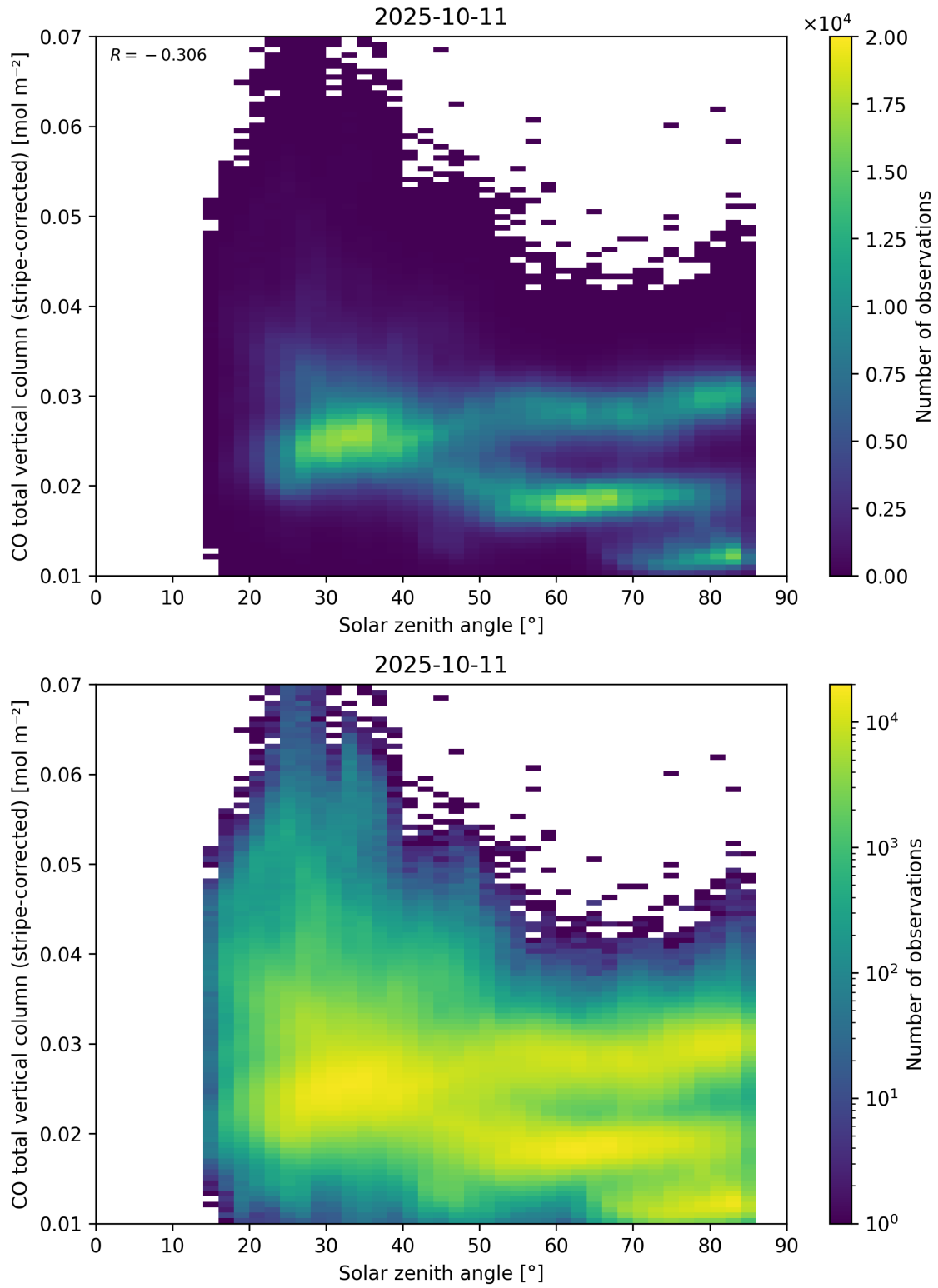
Figure 62: Scatter density plot of “Solar zenith angle” against “CO total vertical column (stripe-corrected)” for 2025-10-11 to 2025-10-12.
