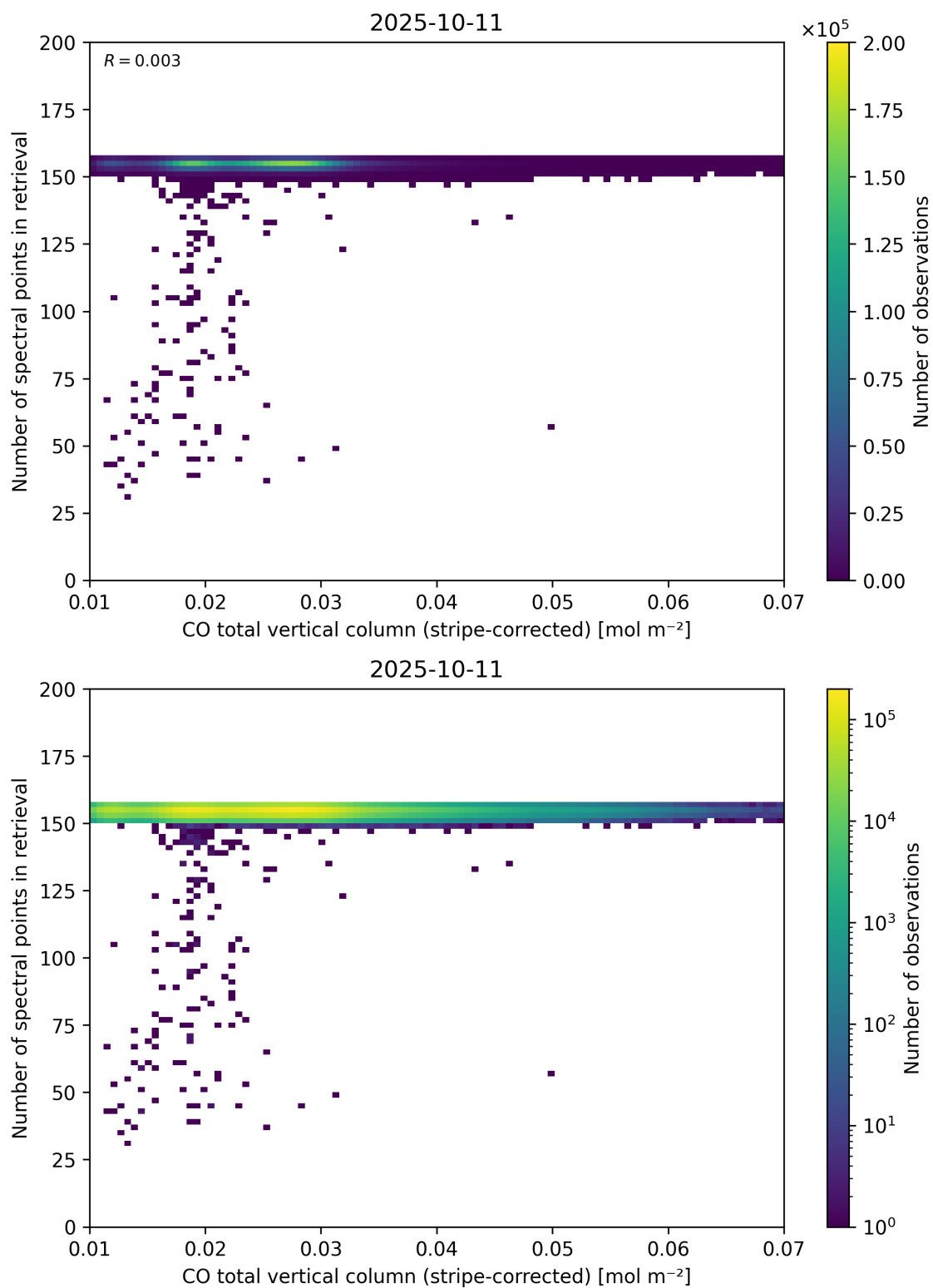
Figure 40: Scatter density plot of “CO total vertical column (stripe-corrected)” against “Number of spectral points in retrieval” for 2025-10-11 to 2025-10-12.
