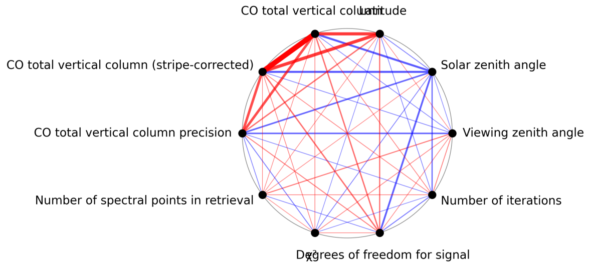
Figure 1: Map of correlation graph for 2025-10-11 to 2025-10-12.
