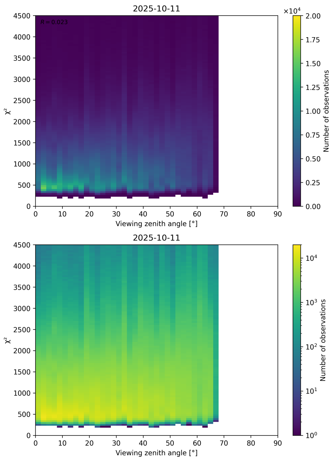
Figure 72: Scatter density plot of “Viewing zenith angle” against “ \chi^2 ” for 2025-10-11 to 2025-10-12.
