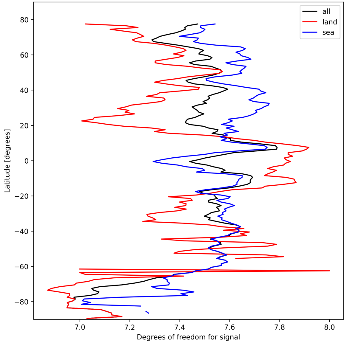
Figure 15: Zonal average of “Degrees of freedom for signal” for 2025-10-11 to 2025-10-12.
