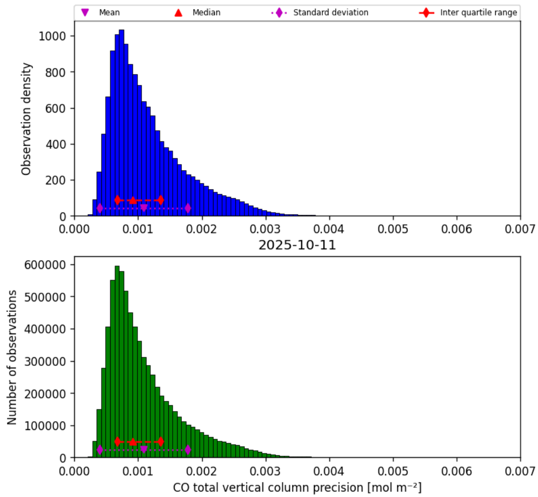
Figure 20: Histogram of “CO total vertical column precision” for 2025-10-11 to 2025-10-12
