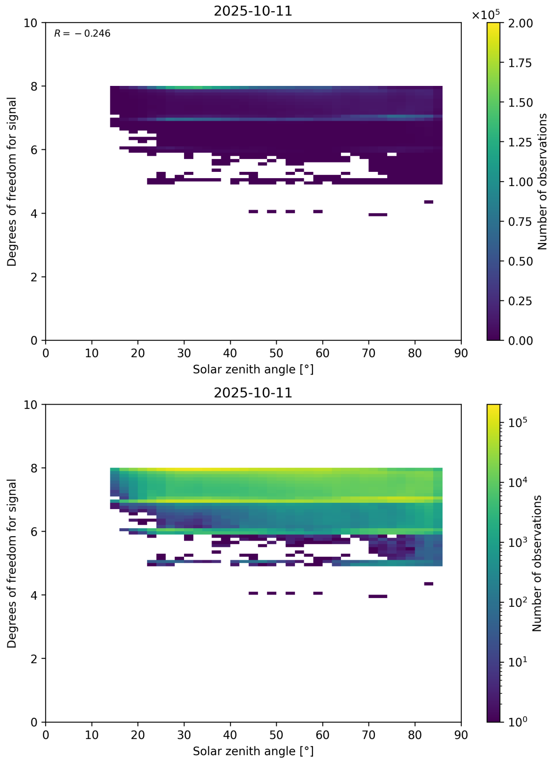
Figure 65: Scatter density plot of “Solar zenith angle” against “Degrees of freedom for signal” for 2025-10-11 to 2025-10-12.
