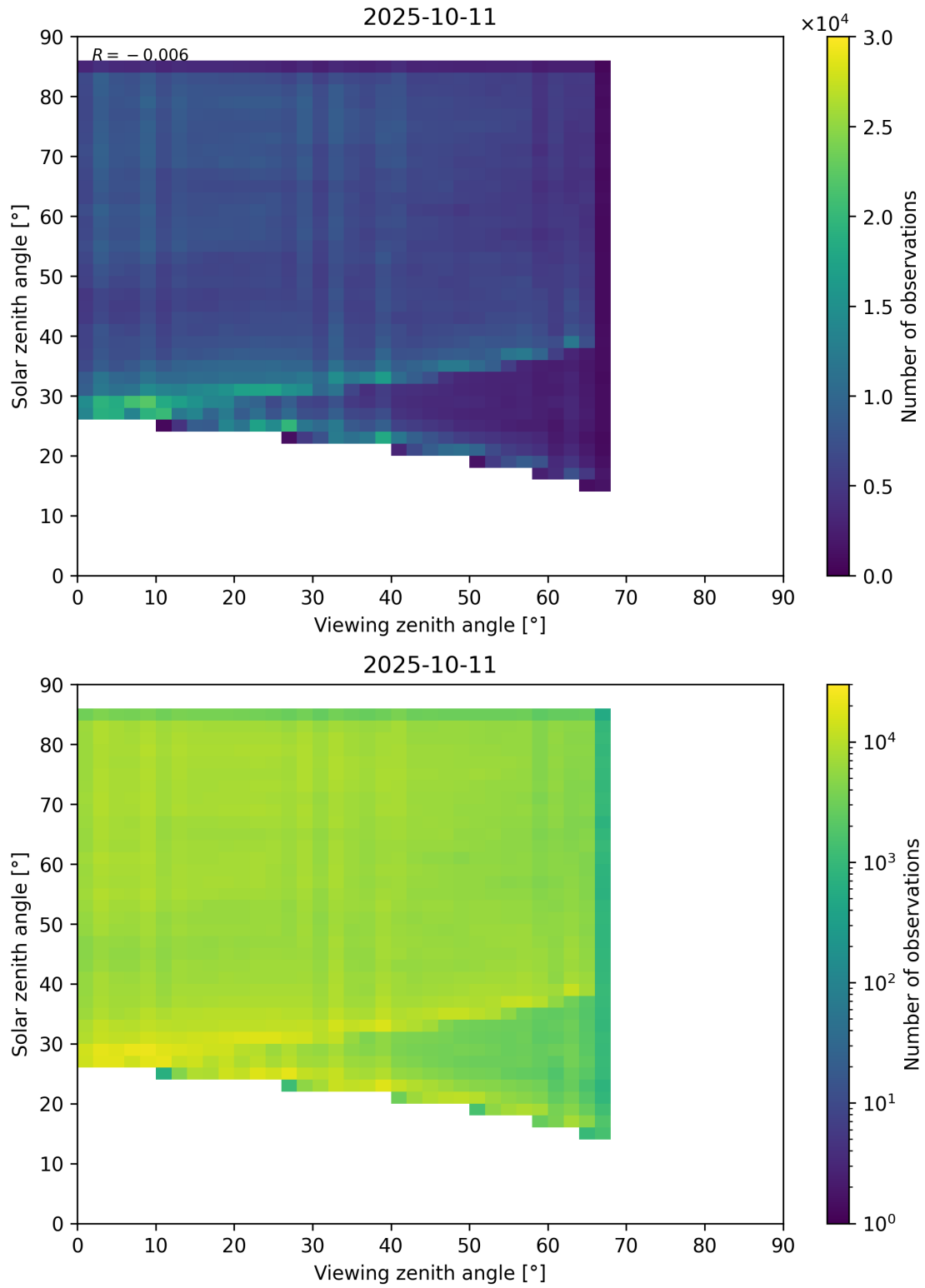
Figure 77: Scatter density plot of “Viewing zenith angle” against “Solar zenith angle” for 2025-10-11 to 2025-10-12.
