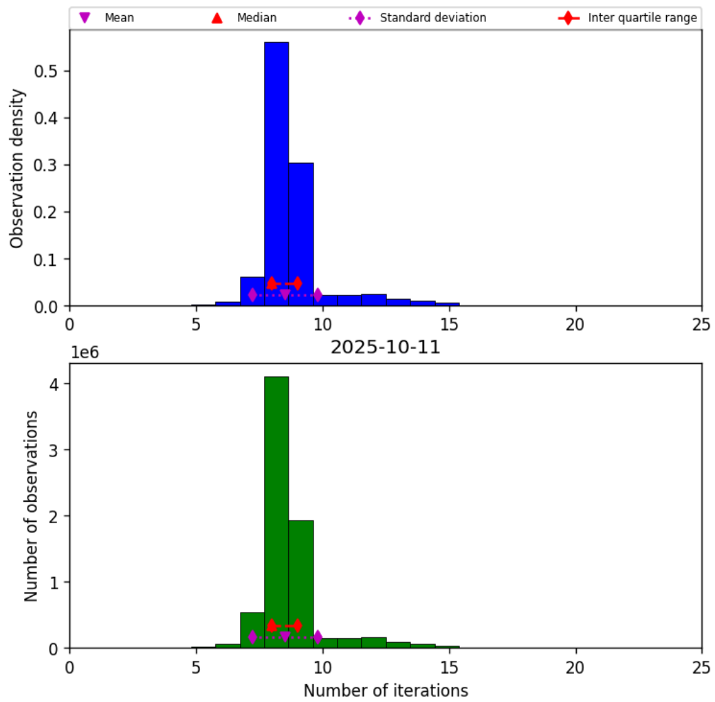
Figure 24: Histogram of “Number of iterations” for 2025-10-11 to 2025-10-12
