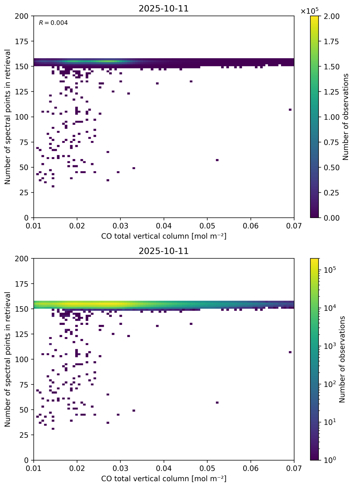
Figure 43: Scatter density plot of “CO total vertical column” against “Number of spectral points in retrieval” for 2025-10-11 to 2025-10-12.
