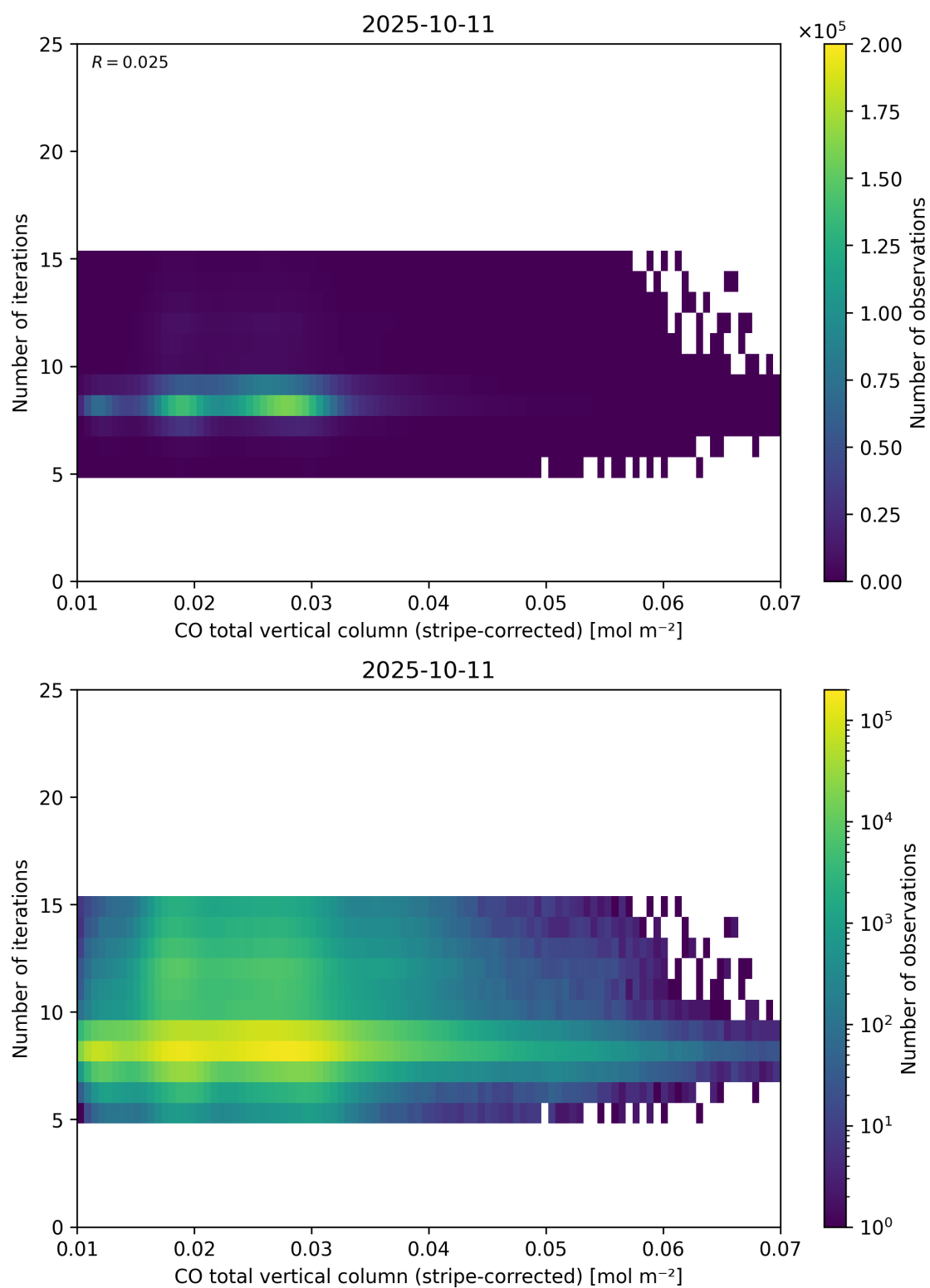
Figure 39: Scatter density plot of “CO total vertical column (stripe-corrected)” against “Number of iterations” for 2025-10-11 to 2025-10-12.
