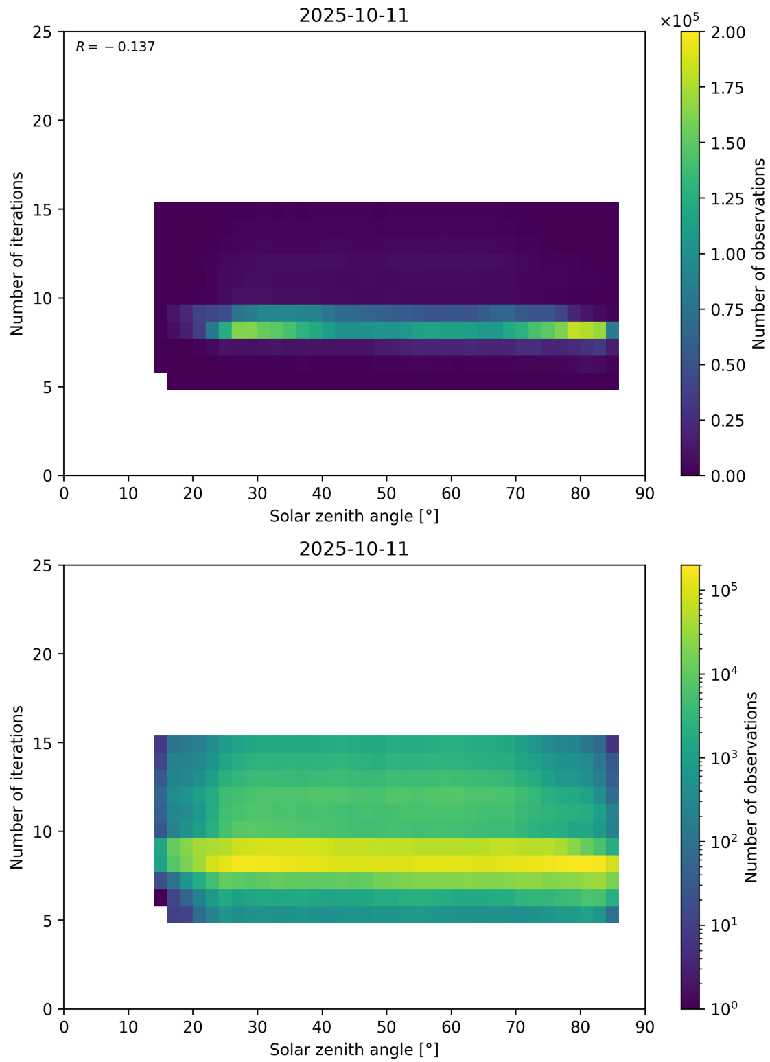
Figure 67: Scatter density plot of “Solar zenith angle” against “Number of iterations” for 2025-10-11 to 2025-10-12.
