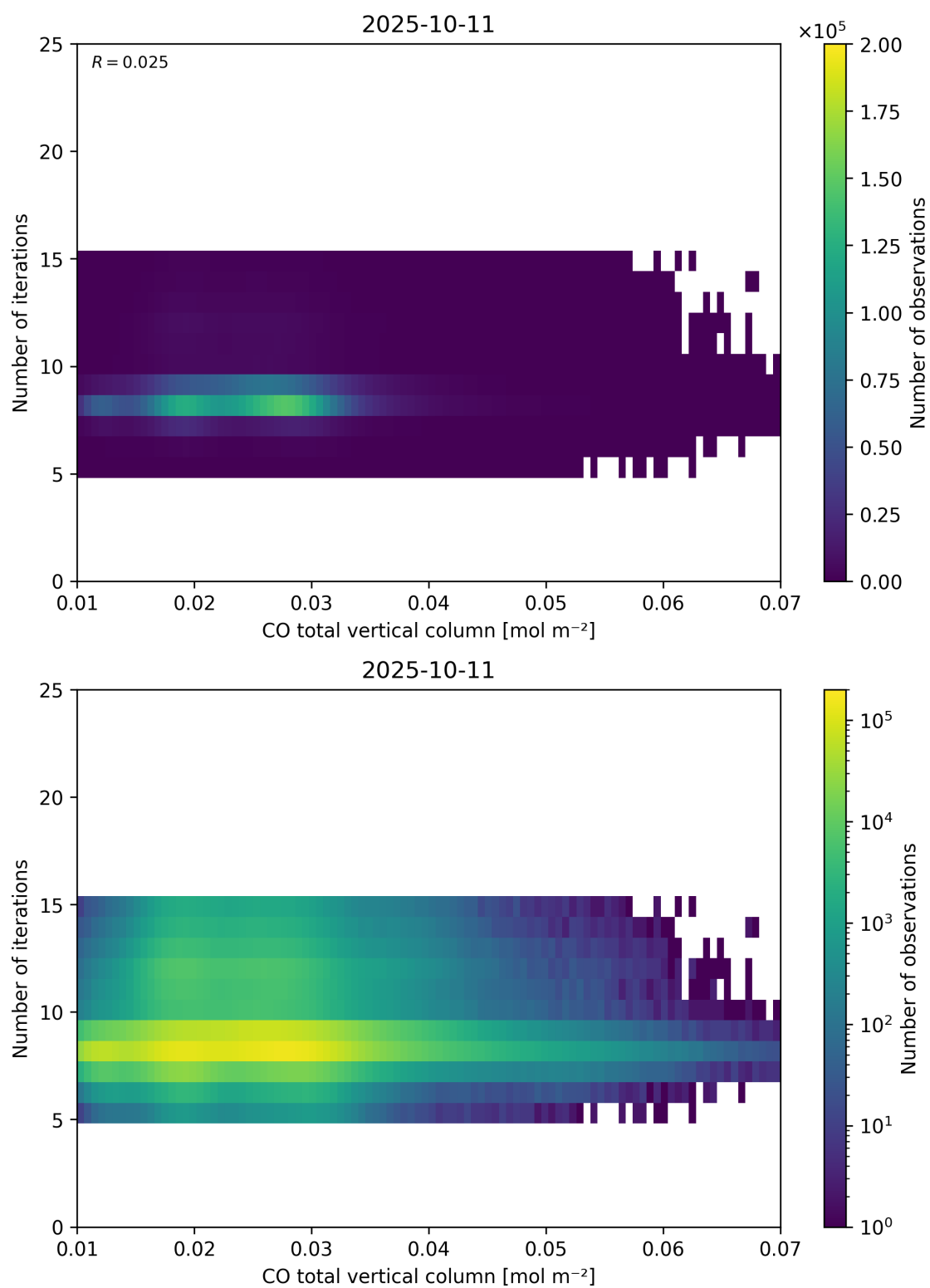
Figure 42: Scatter density plot of “CO total vertical column” against “Number of iterations” for 2025-10-11 to 2025-10-12.
