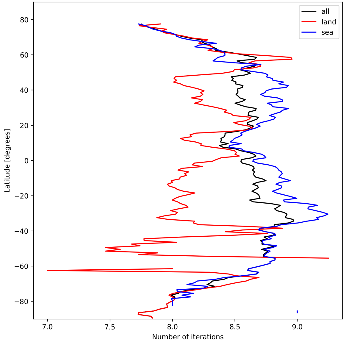
Figure 16: Zonal average of “Number of iterations” for 2025-10-11 to 2025-10-12.
