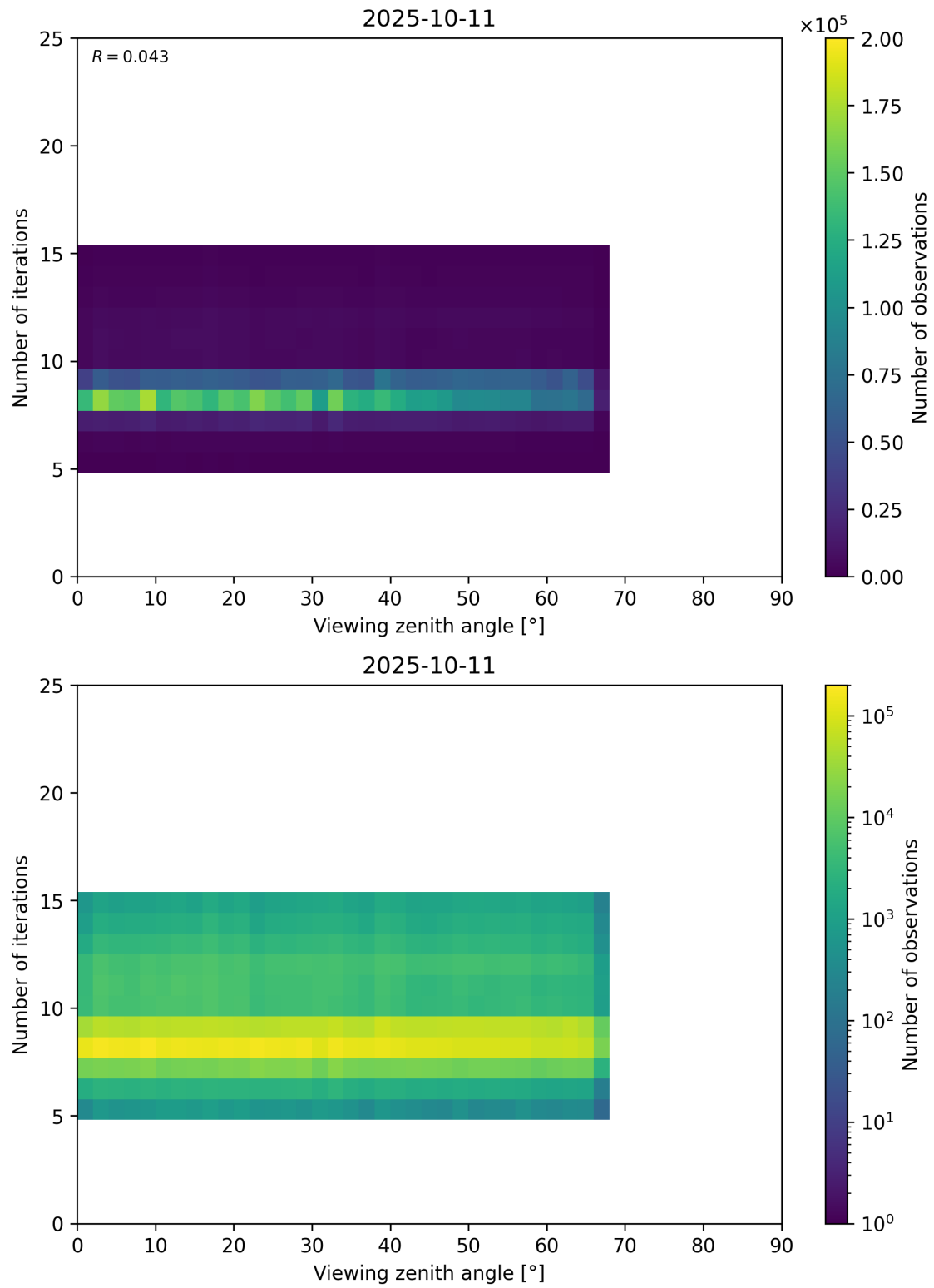
Figure 75: Scatter density plot of “Viewing zenith angle” against “Number of iterations” for 2025-10-11 to 2025-10-12.
