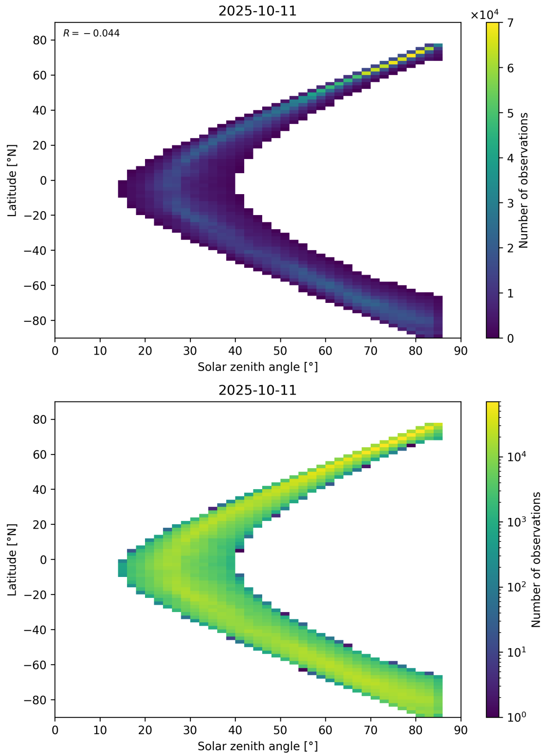
Figure 66: Scatter density plot of “Solar zenith angle” against “Latitude” for 2025-10-11 to 2025-10-12.
