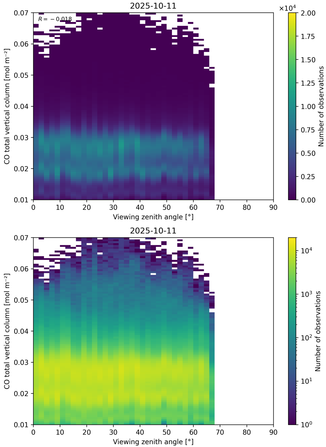
Figure 69: Scatter density plot of “Viewing zenith angle” against “CO total vertical column” for 2025-10-11 to 2025-10-12.
