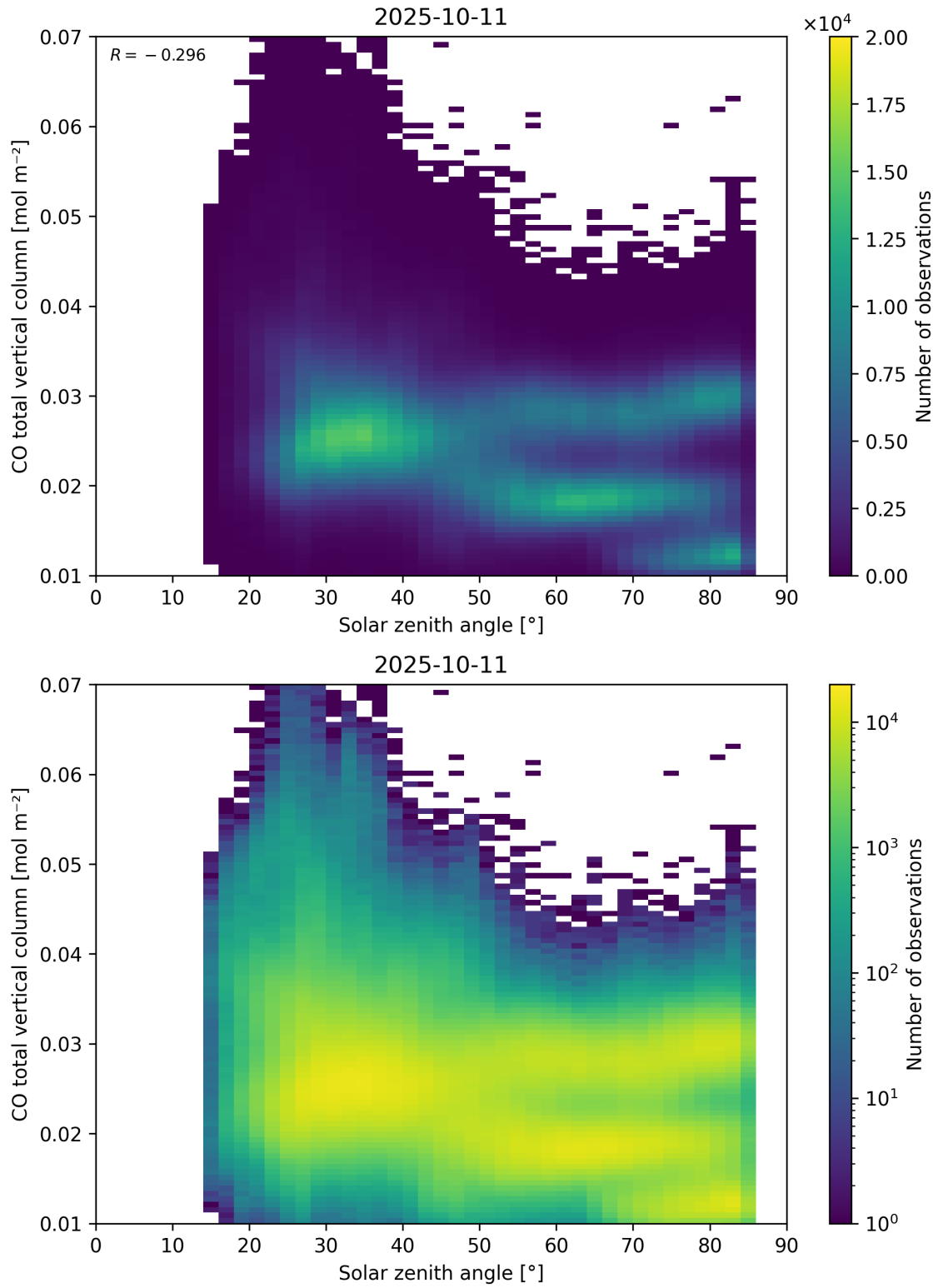
Figure 61: Scatter density plot of “Solar zenith angle” against “CO total vertical column” for 2025-10-11 to 2025-10-12.
