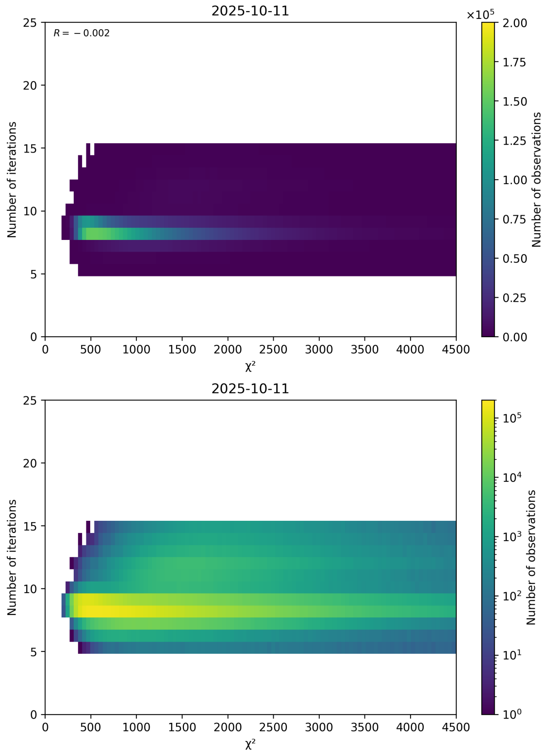
Figure 49: Scatter density plot of “ \chi^2 ” against “Number of iterations” for 2025-10-11 to 2025-10-12.
