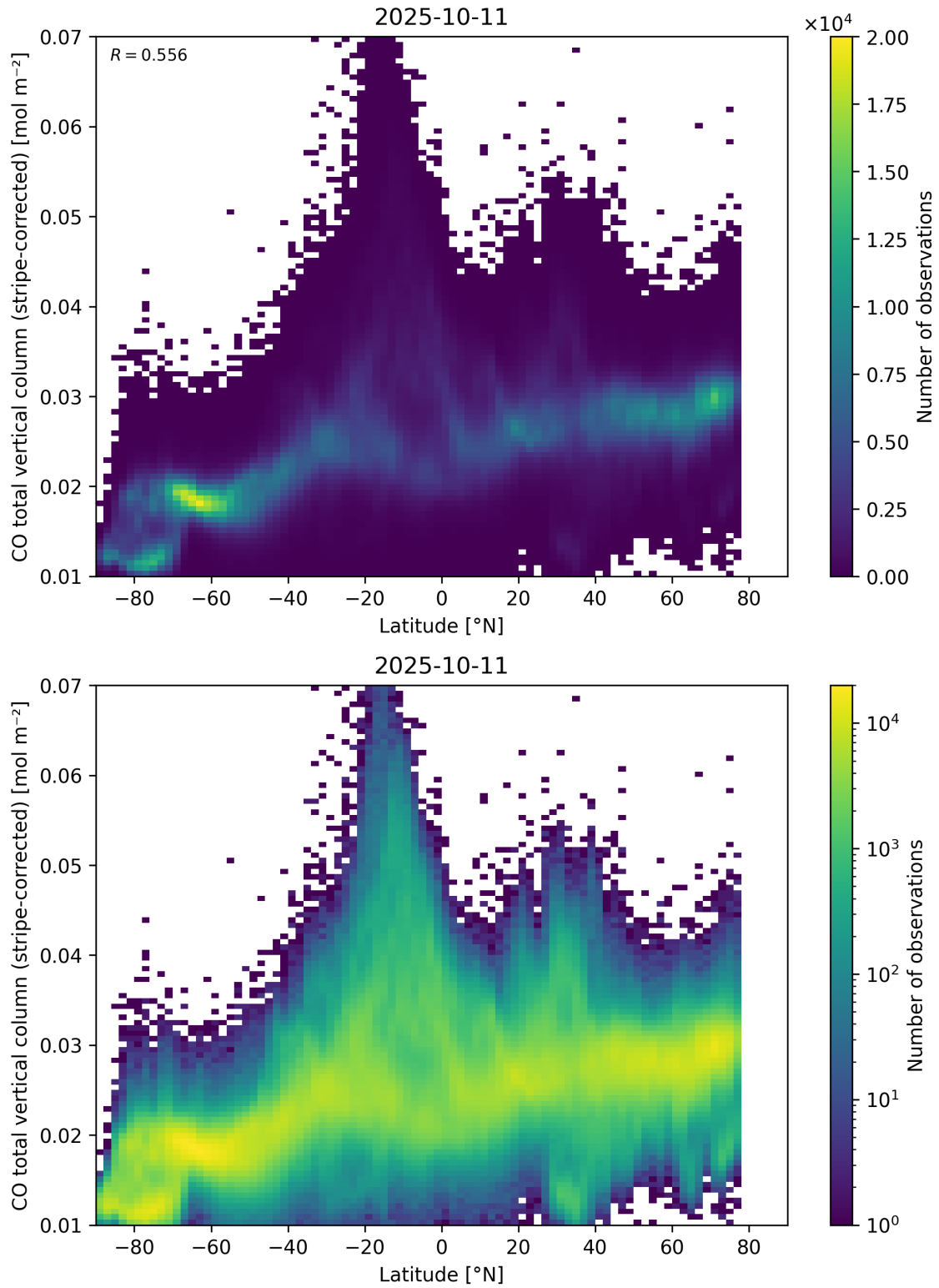
Figure 52: Scatter density plot of “Latitude” against “CO total vertical column (stripe-corrected)” for 2025-10-11 to 2025-10-12.
