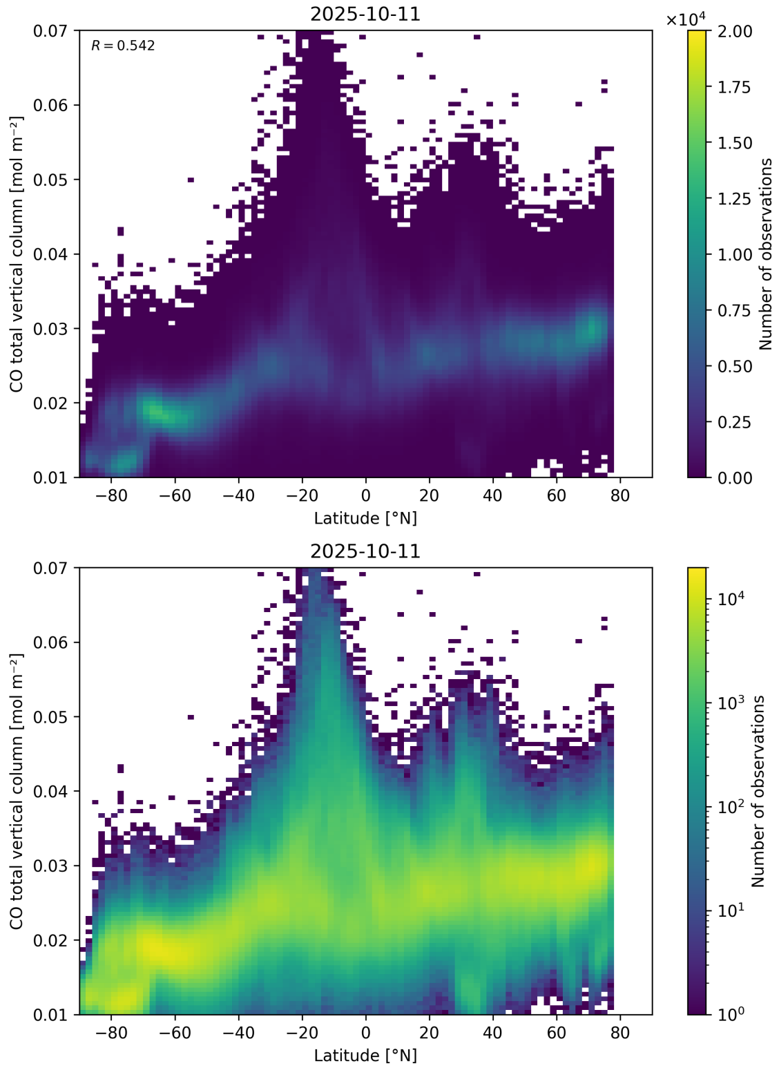
Figure 51: Scatter density plot of “Latitude” against “CO total vertical column” for 2025-10-11 to 2025-10-12.
