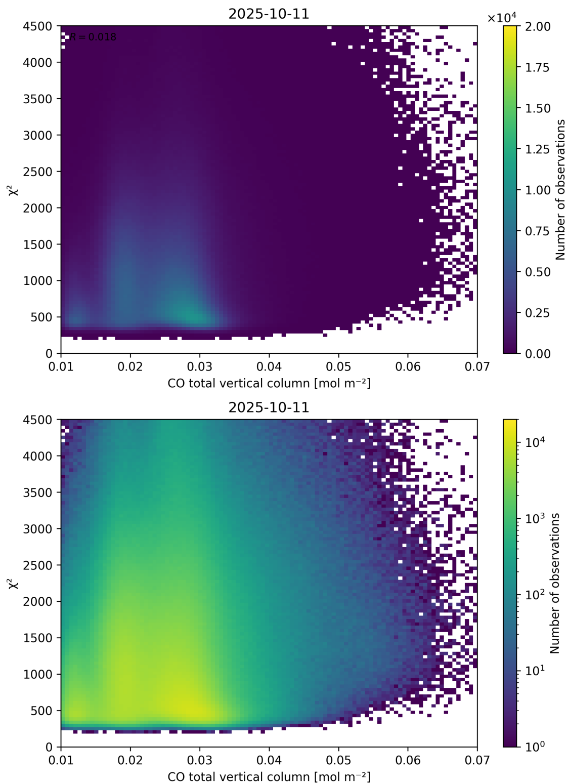
Figure 35: Scatter density plot of “CO total vertical column” against “ \chi^2 ” for 2025-10-11 to 2025-10-12.
