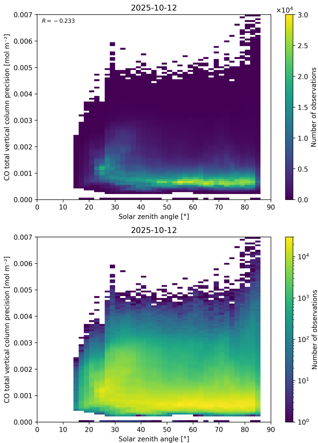
Figure 63: Scatter density plot of “Solar zenith angle” against “CO total vertical column precision” for 2025-10-11 to 2025-10-13.
