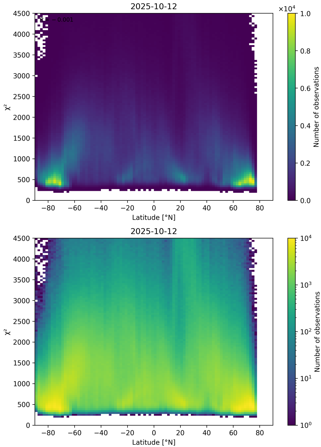
Figure 54: Scatter density plot of “Latitude” against “ \chi^2 ” for 2025-10-11 to 2025-10-13.
