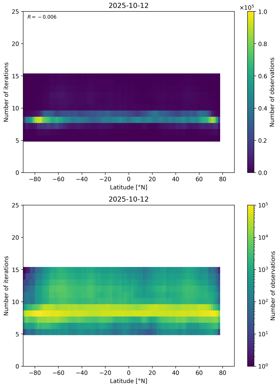
Figure 56: Scatter density plot of “Latitude” against “Number of iterations” for 2025-10-11 to 2025-10-13.
