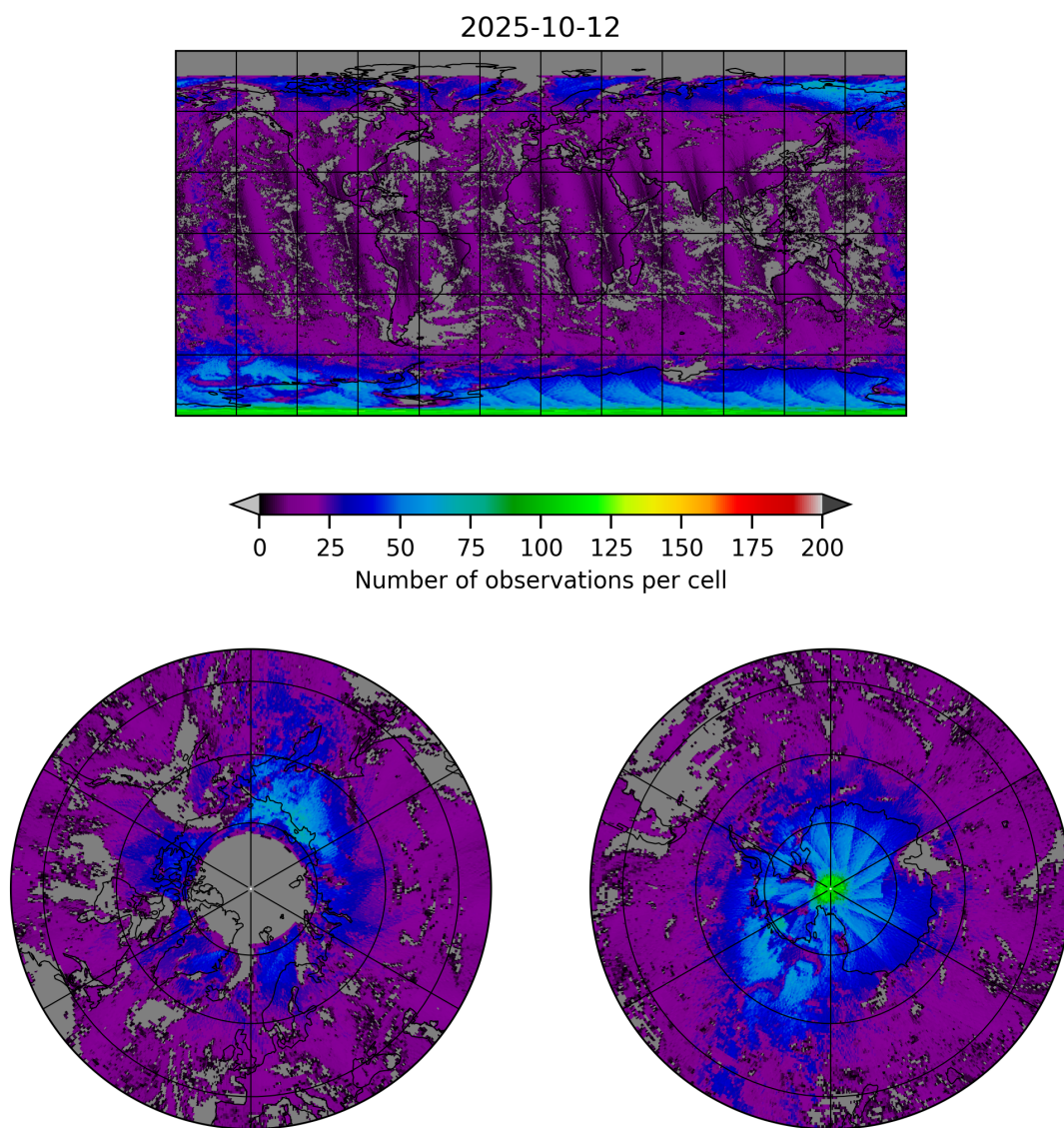
Figure 8: Map of the number of observations for 2025-10-11 to 2025-10-13
