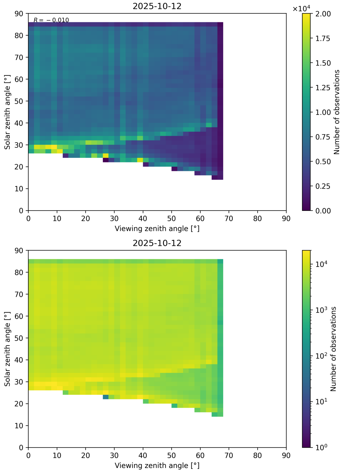
Figure 77: Scatter density plot of “Viewing zenith angle” against “Solar zenith angle” for 2025-10-11 to 2025-10-13.
