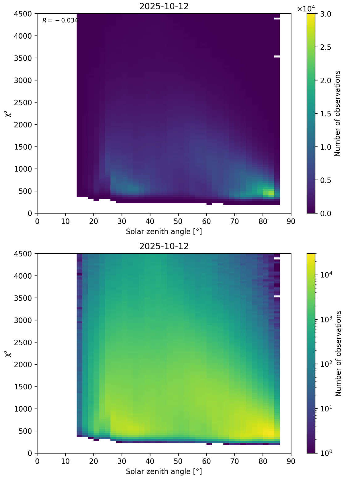
Figure 64: Scatter density plot of “Solar zenith angle” against “ \chi^2 ” for 2025-10-11 to 2025-10-13.
