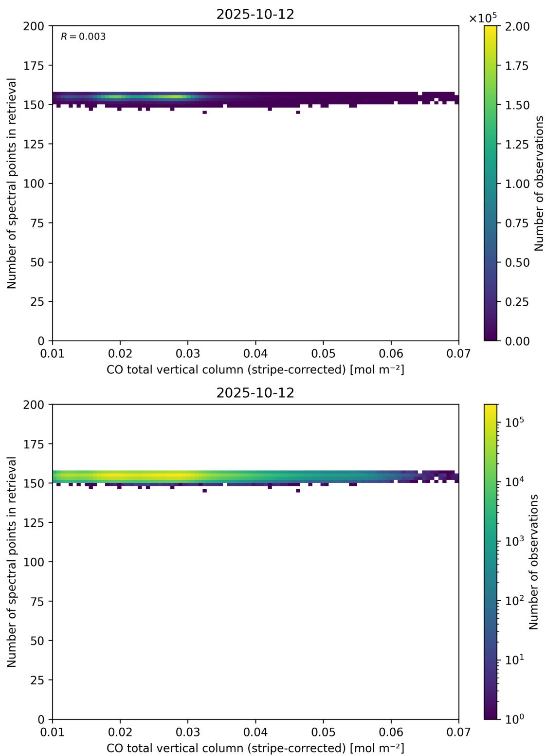
Figure 40: Scatter density plot of “CO total vertical column (stripe-corrected)” against “Number of spectral points in retrieval” for 2025-10-11 to 2025-10-13.
