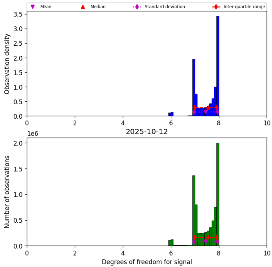
Figure 23: Histogram of “Degrees of freedom for signal” for 2025-10-11 to 2025-10-13
