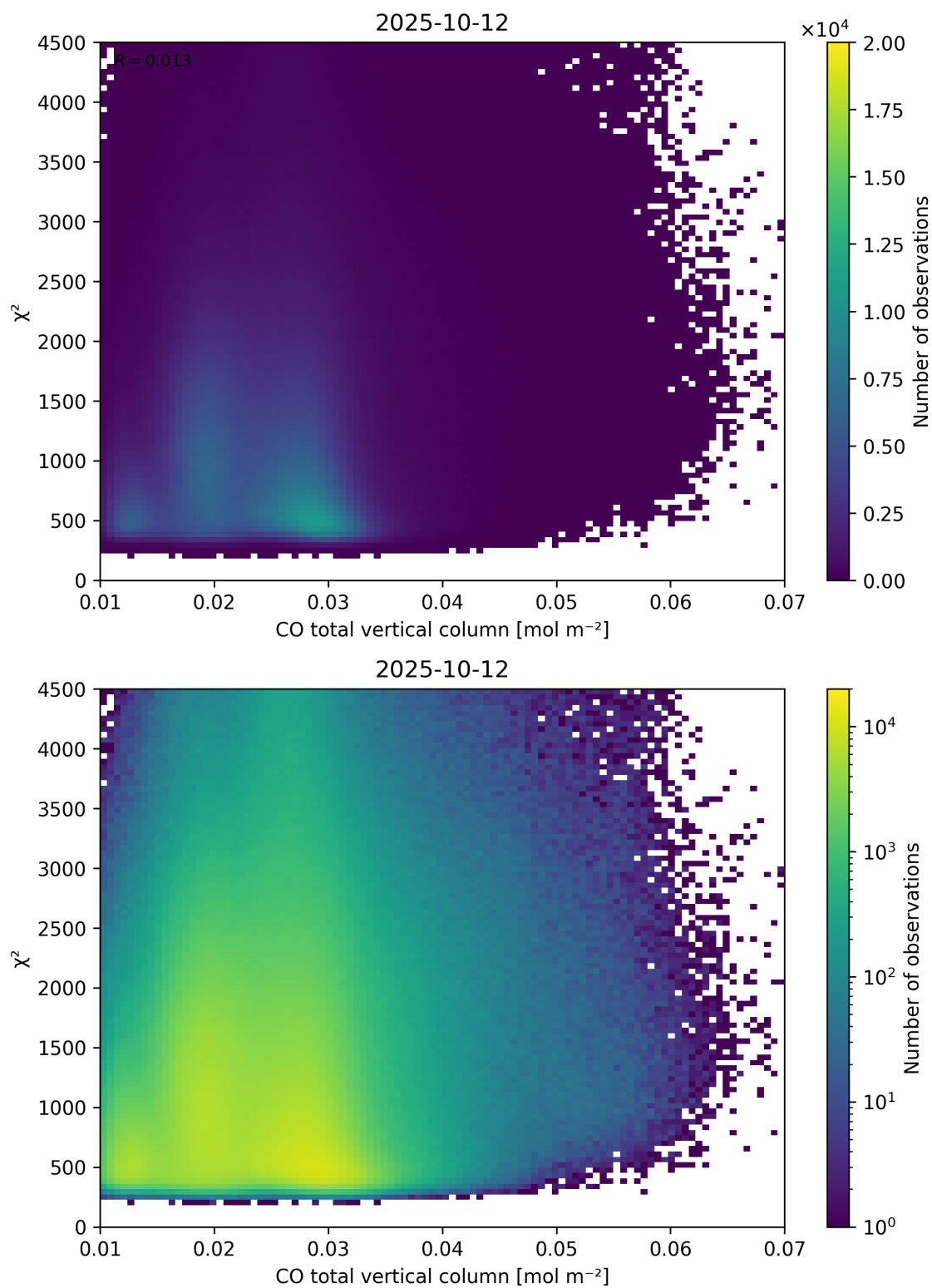
Figure 35: Scatter density plot of “CO total vertical column” against “ \chi^2 ” for 2025-10-11 to 2025-10-13.
