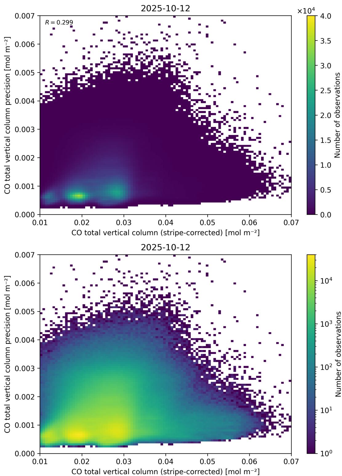
Figure 36: Scatter density plot of “CO total vertical column (stripe-corrected)” against “CO total vertical column precision” for 2025-10-11 to 2025-10-13.
