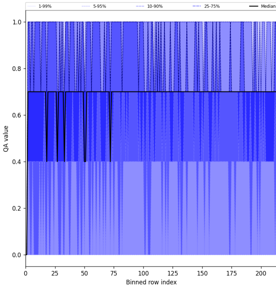
Figure 25: Along track statistics of “QA value” for 2025-10-11 to 2025-10-13
