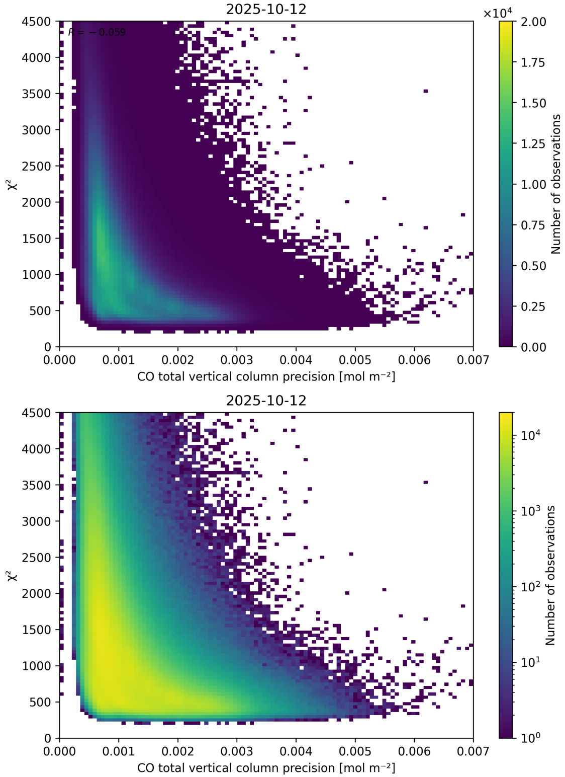
Figure 44: Scatter density plot of “CO total vertical column precision” against “ \chi^2 ” for 2025-10-11 to 2025-10-13.
