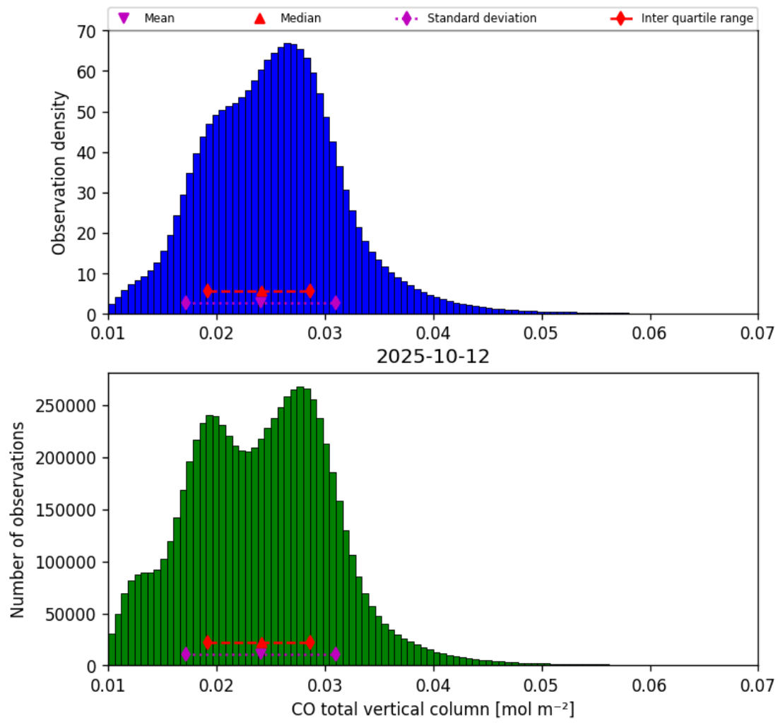
Figure 18: Histogram of “CO total vertical column” for 2025-10-11 to 2025-10-13
