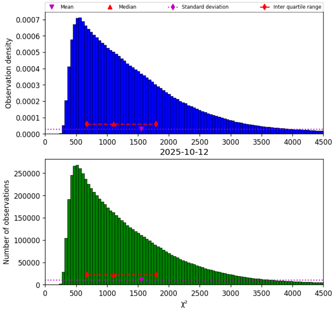
Figure 22: Histogram of “ \chi^2 ” for 2025-10-11 to 2025-10-13
