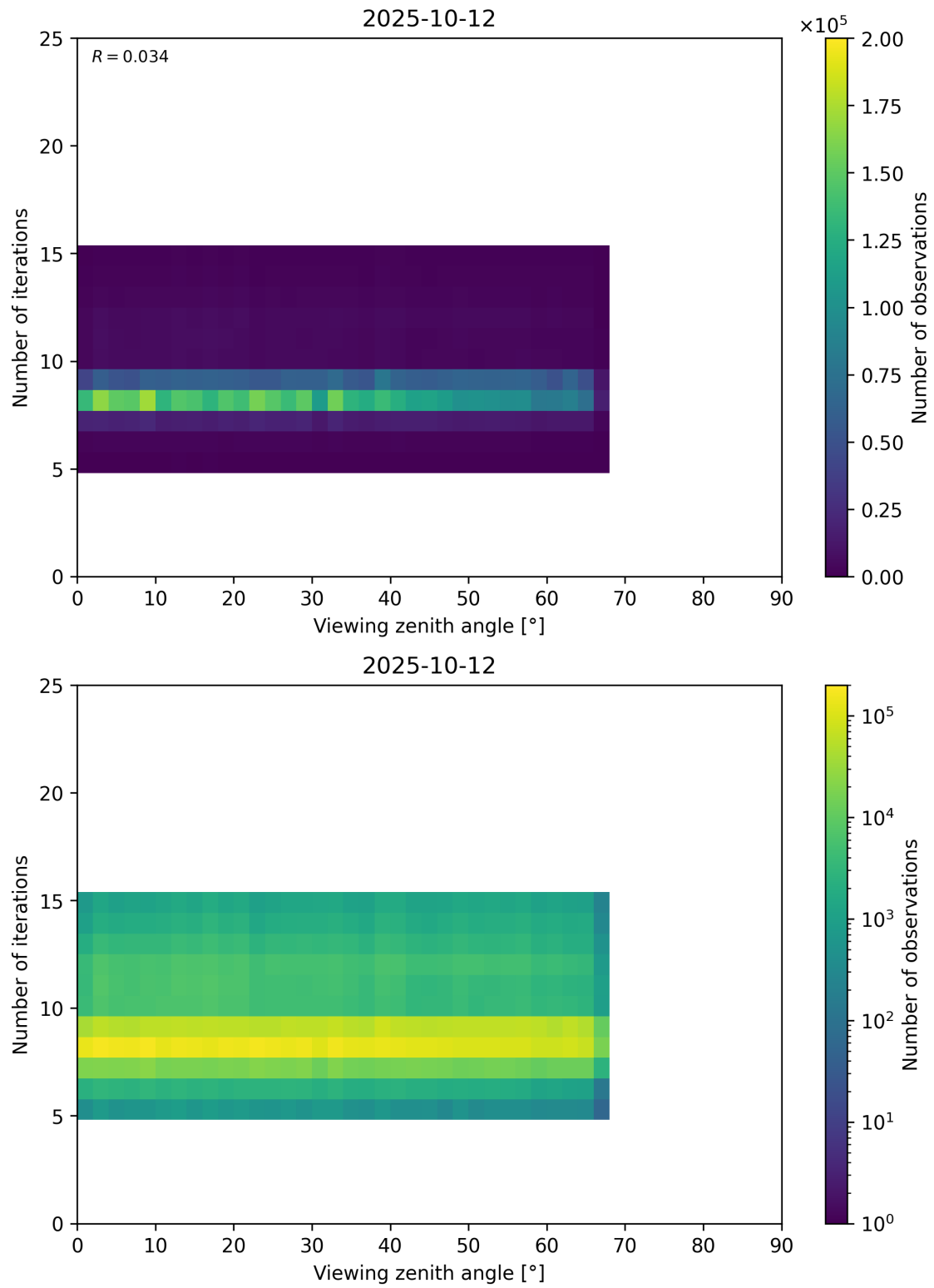
Figure 75: Scatter density plot of “Viewing zenith angle” against “Number of iterations” for 2025-10-11 to 2025-10-13.
