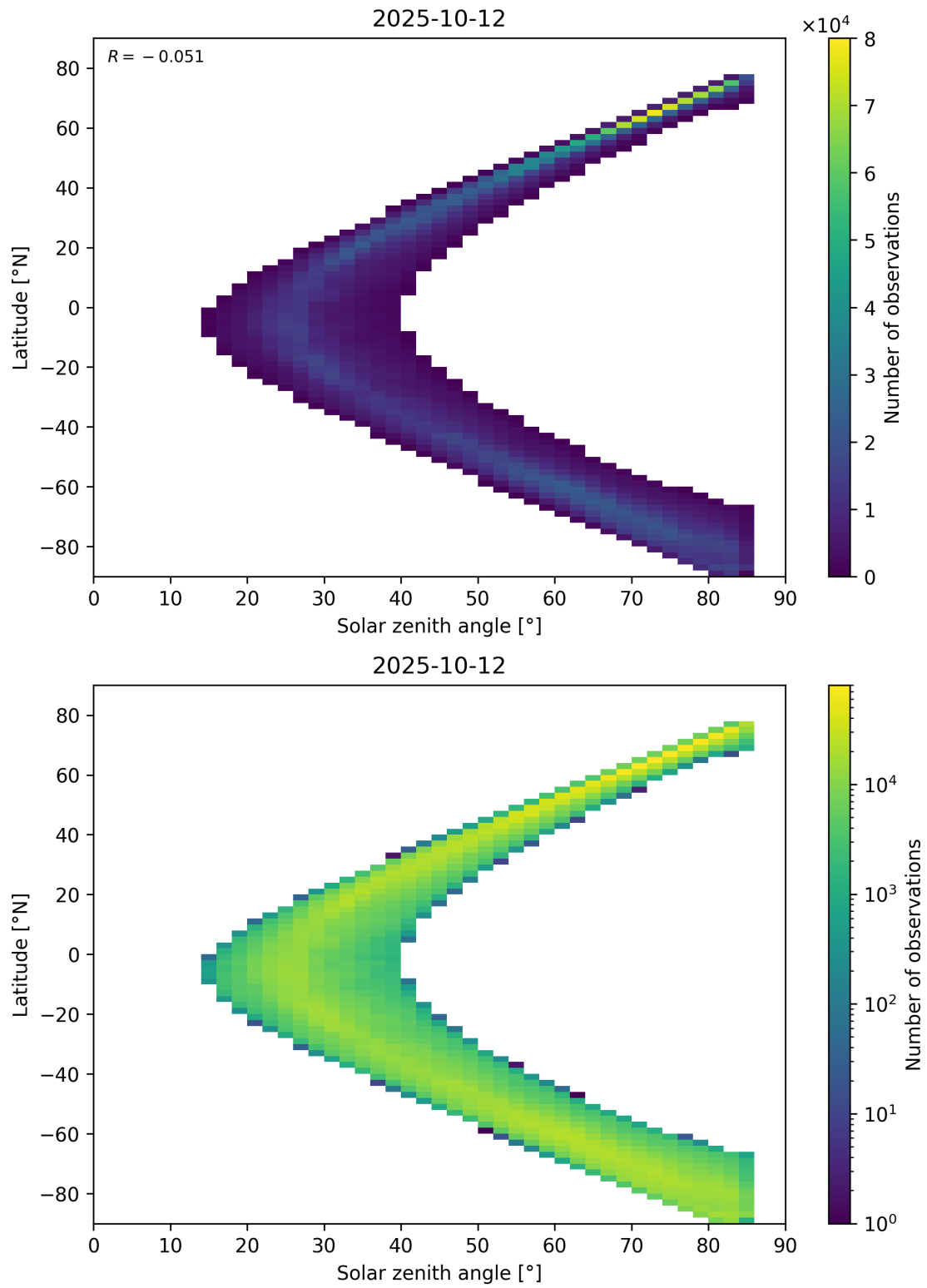
Figure 66: Scatter density plot of “Solar zenith angle” against “Latitude” for 2025-10-11 to 2025-10-13.
