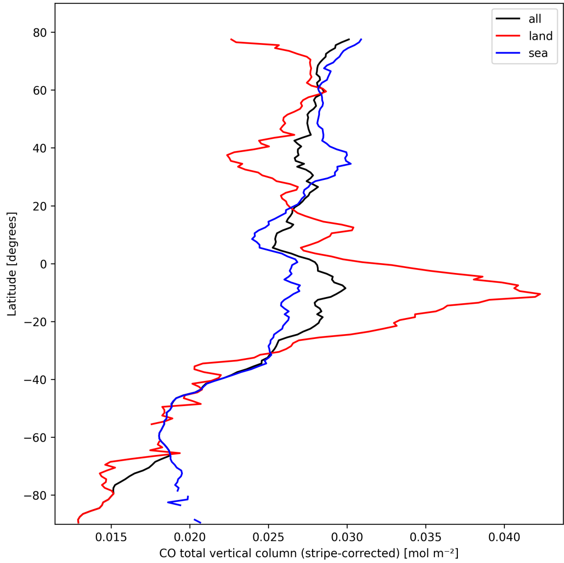
Figure 11: Zonal average of “CO total vertical column (stripe-corrected)” for 2025-10-11 to 2025-10-13.
