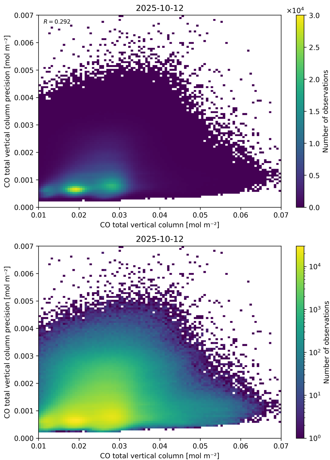
Figure 34: Scatter density plot of “CO total vertical column” against “CO total vertical column precision” for 2025-10-11 to 2025-10-13.
