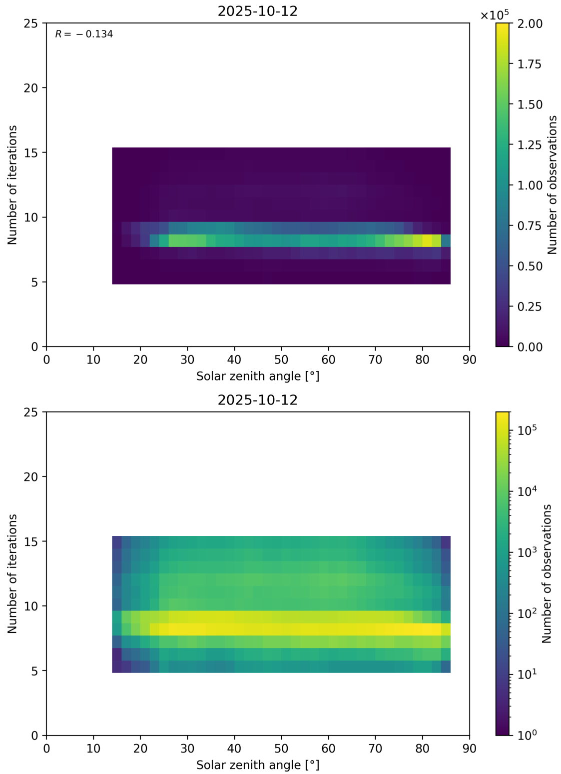
Figure 67: Scatter density plot of “Solar zenith angle” against “Number of iterations” for 2025-10-11 to 2025-10-13.
