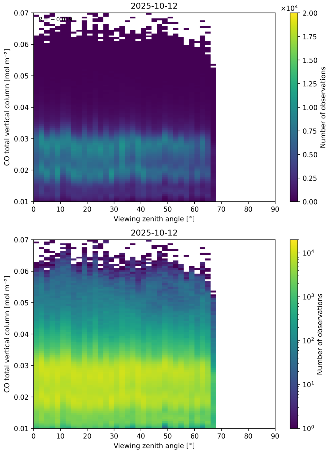
Figure 69: Scatter density plot of “Viewing zenith angle” against “CO total vertical column” for 2025-10-11 to 2025-10-13.
