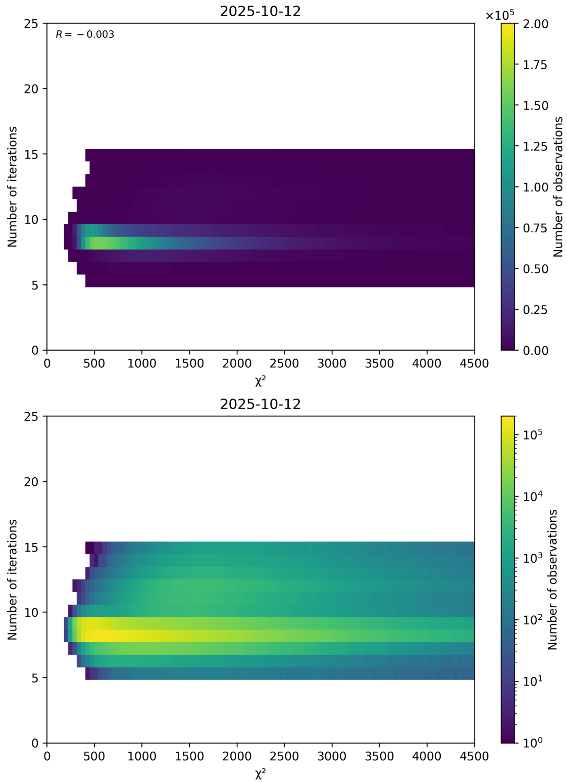
Figure 49: Scatter density plot of “ \chi^2 ” against “Number of iterations” for 2025-10-11 to 2025-10-13.
