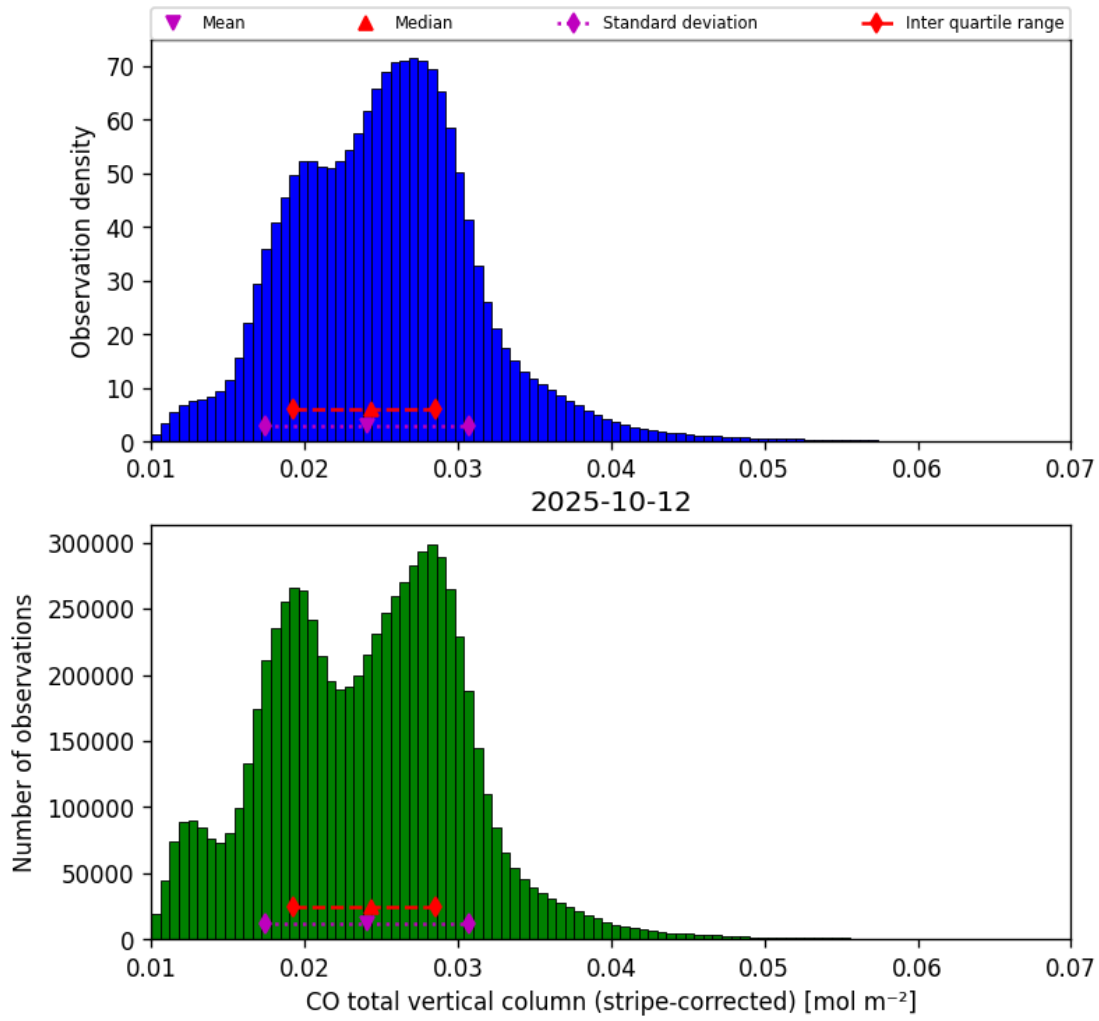
Figure 19: Histogram of “CO total vertical column (stripe-corrected)” for 2025-10-11 to 2025-10-13
