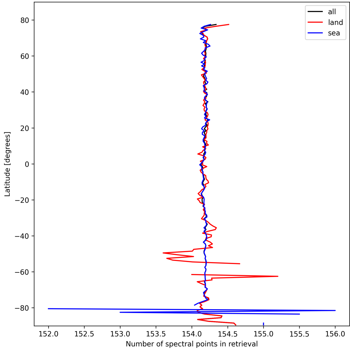
Figure 13: Zonal average of “Number of spectral points in retrieval” for 2025-10-11 to 2025-10-13.
