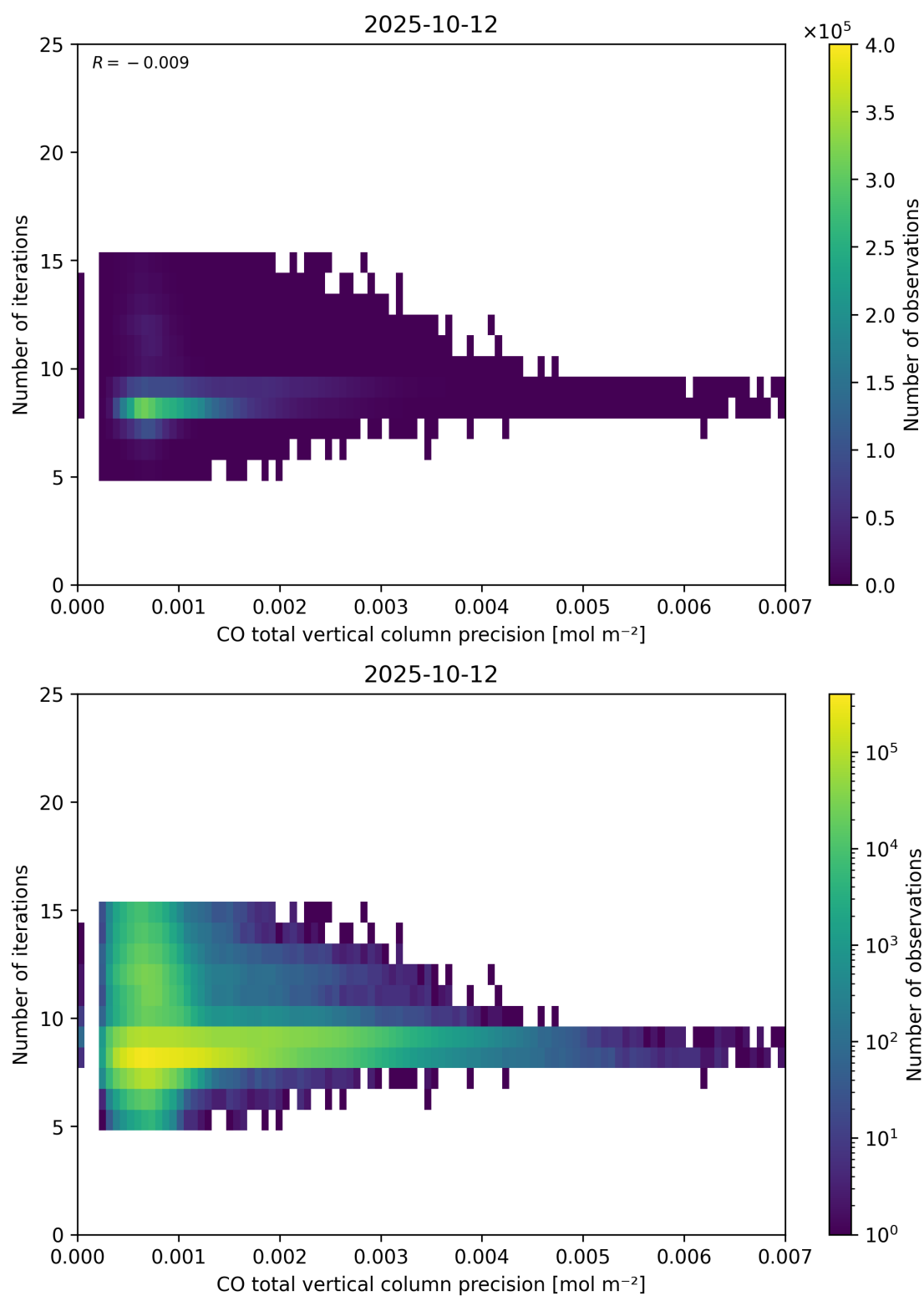
Figure 46: Scatter density plot of “CO total vertical column precision” against “Number of iterations” for 2025-10-11 to 2025-10-13.
