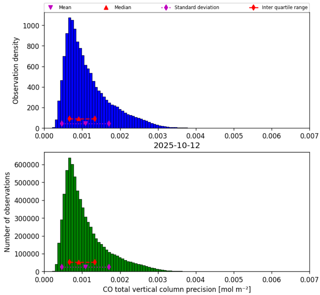
Figure 20: Histogram of “CO total vertical column precision” for 2025-10-11 to 2025-10-13
