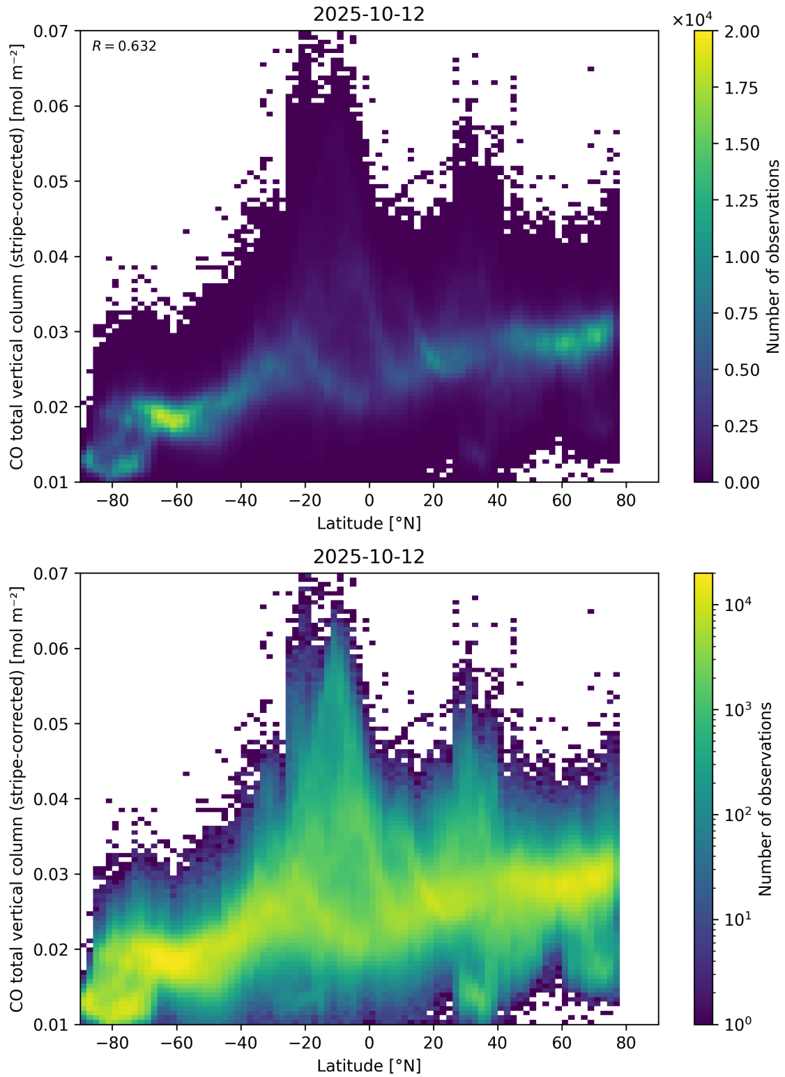
Figure 52: Scatter density plot of “Latitude” against “CO total vertical column (stripe-corrected)” for 2025-10-11 to 2025-10-13.
