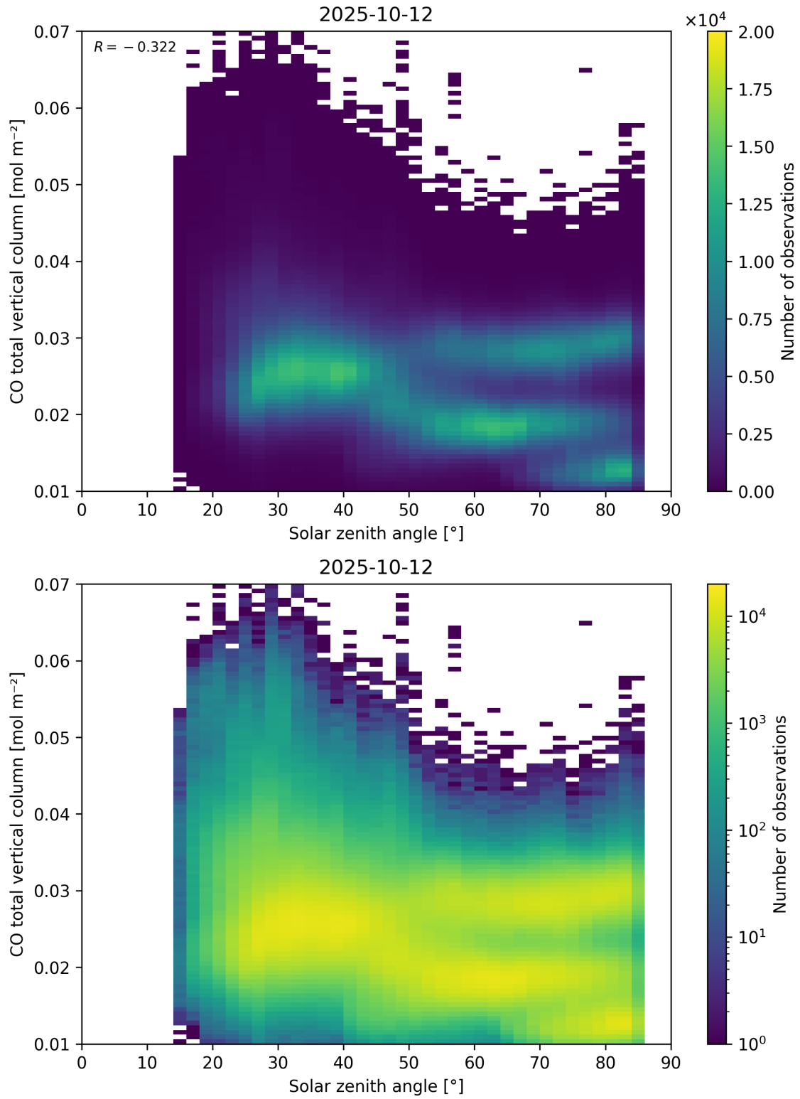
Figure 61: Scatter density plot of “Solar zenith angle” against “CO total vertical column” for 2025-10-11 to 2025-10-13.
