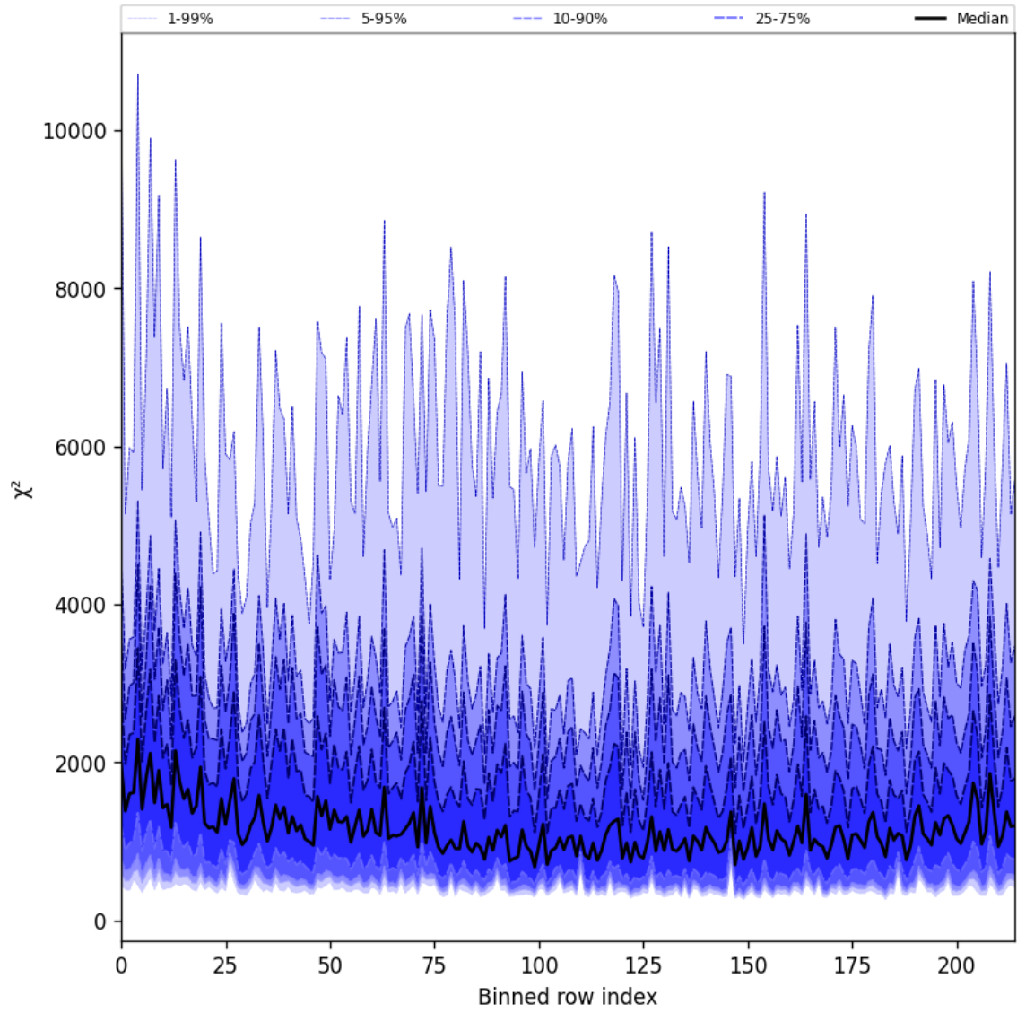
Figure 30: Along track statistics of “ \chi^2 ” for 2025-10-11 to 2025-10-13
