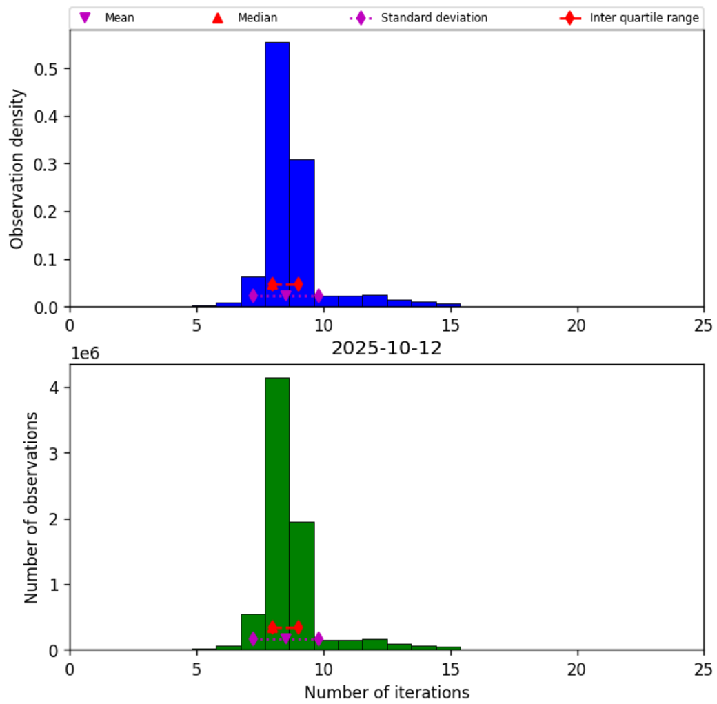
Figure 24: Histogram of “Number of iterations” for 2025-10-11 to 2025-10-13
