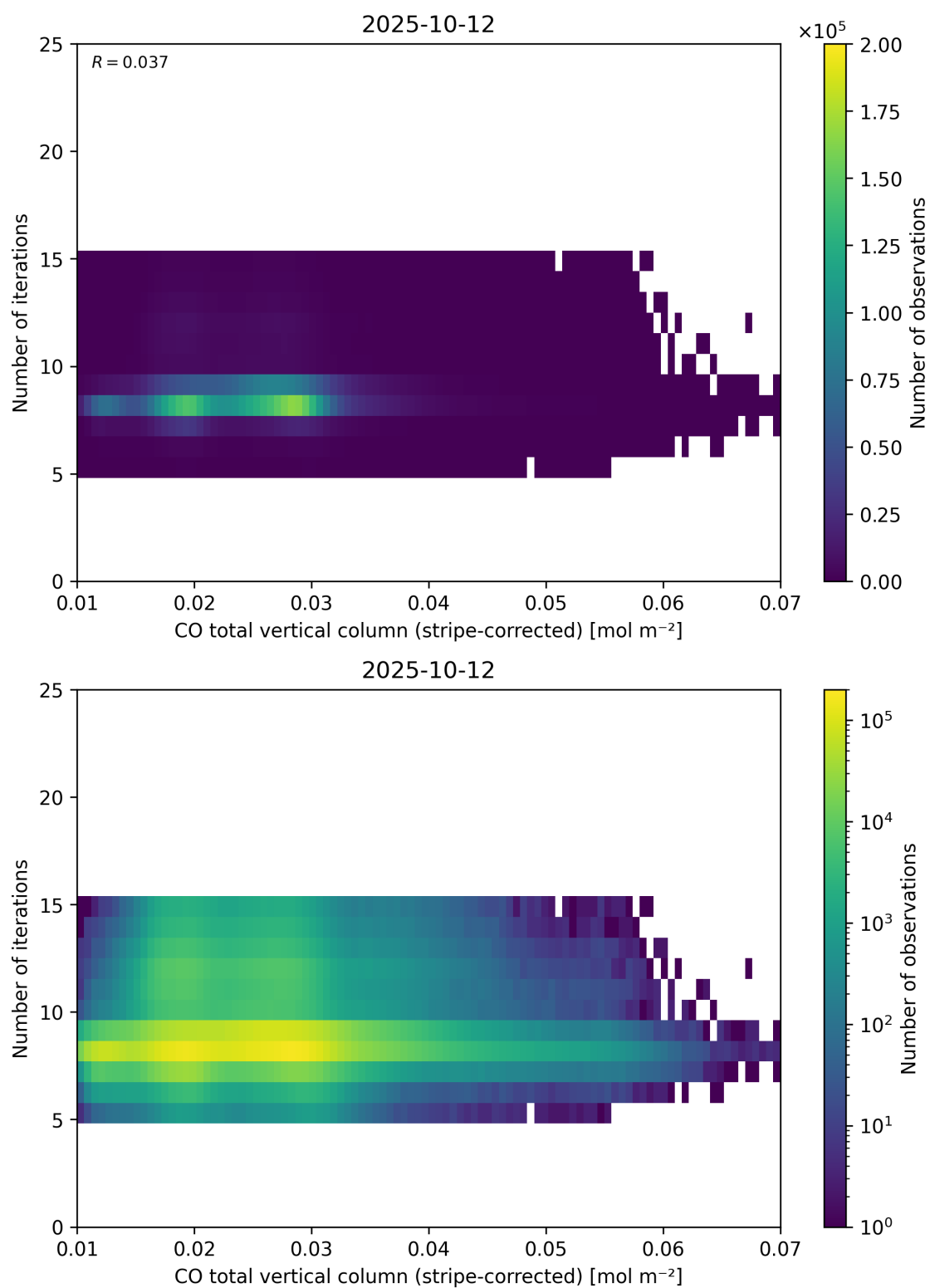
Figure 39: Scatter density plot of “CO total vertical column (stripe-corrected)” against “Number of iterations” for 2025-10-11 to 2025-10-13.
