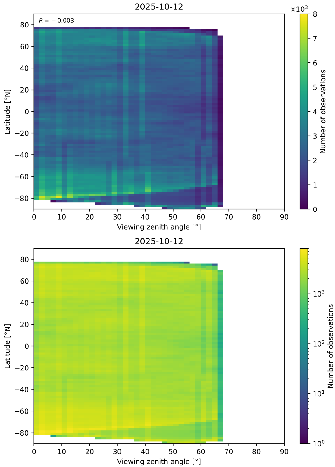
Figure 74: Scatter density plot of “Viewing zenith angle” against “Latitude” for 2025-10-11 to 2025-10-13.
