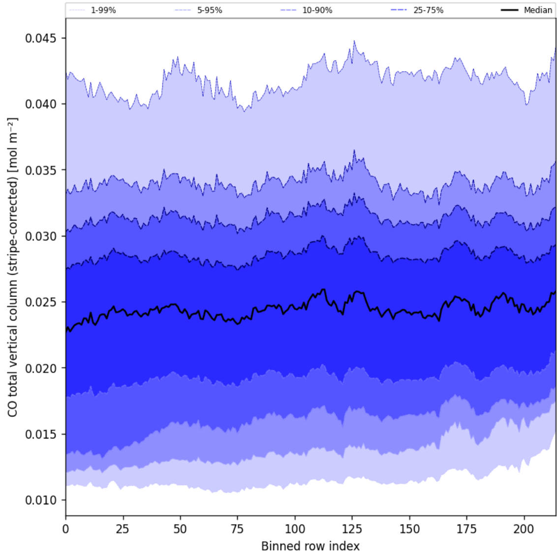
Figure 27: Along track statistics of “CO total vertical column (stripe-corrected)” for 2025-10-11 to 2025-10-13
