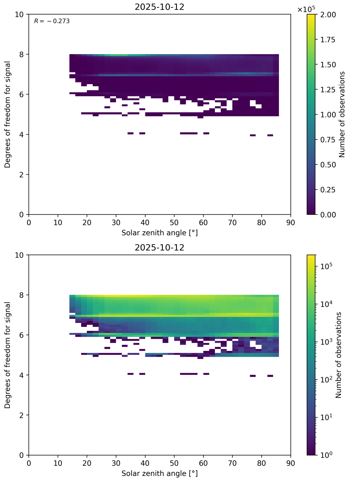
Figure 65: Scatter density plot of “Solar zenith angle” against “Degrees of freedom for signal” for 2025-10-11 to 2025-10-13.
