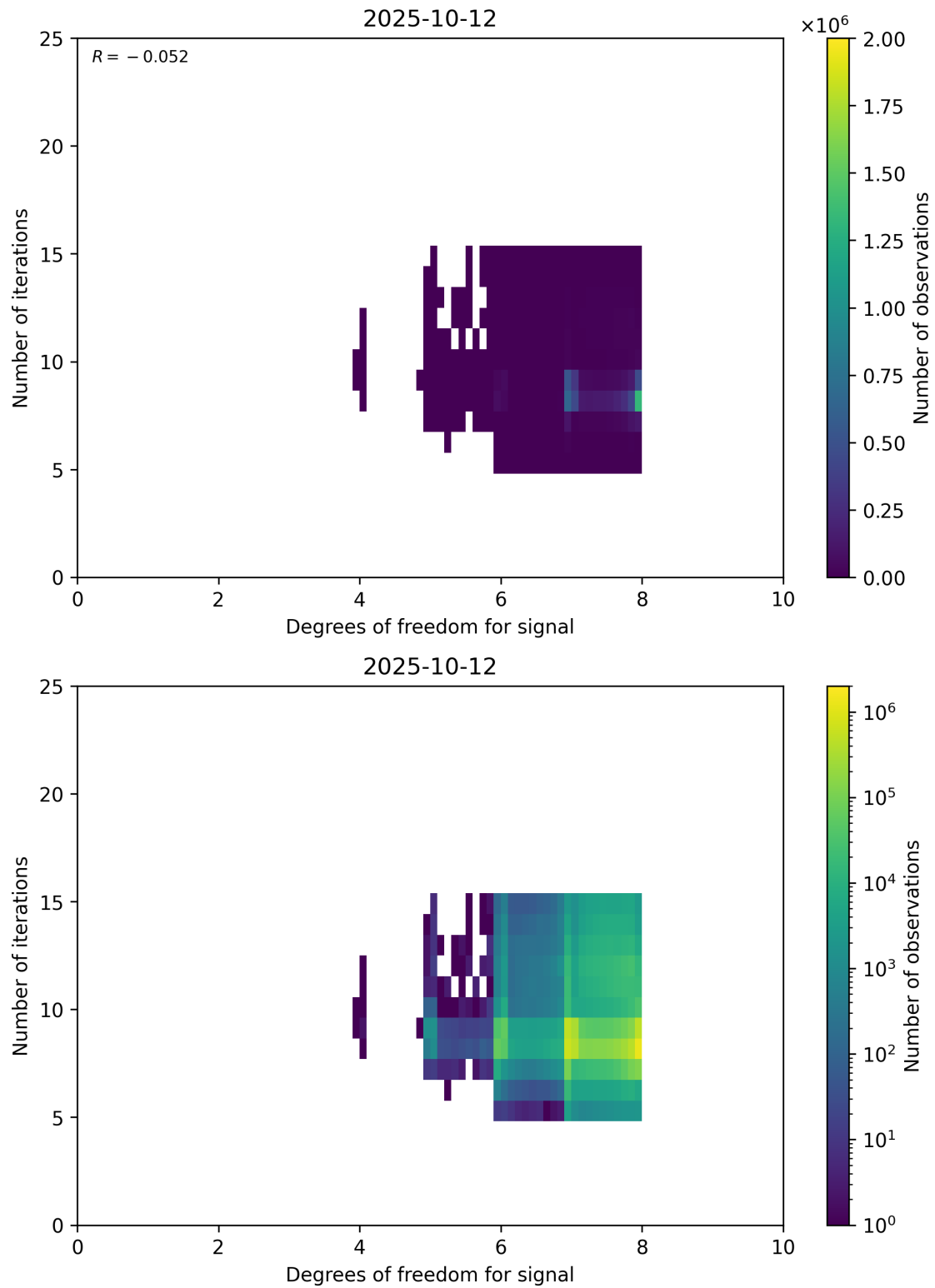
Figure 50: Scatter density plot of “Degrees of freedom for signal” against “Number of iterations” for 2025-10-11 to 2025-10-13.
