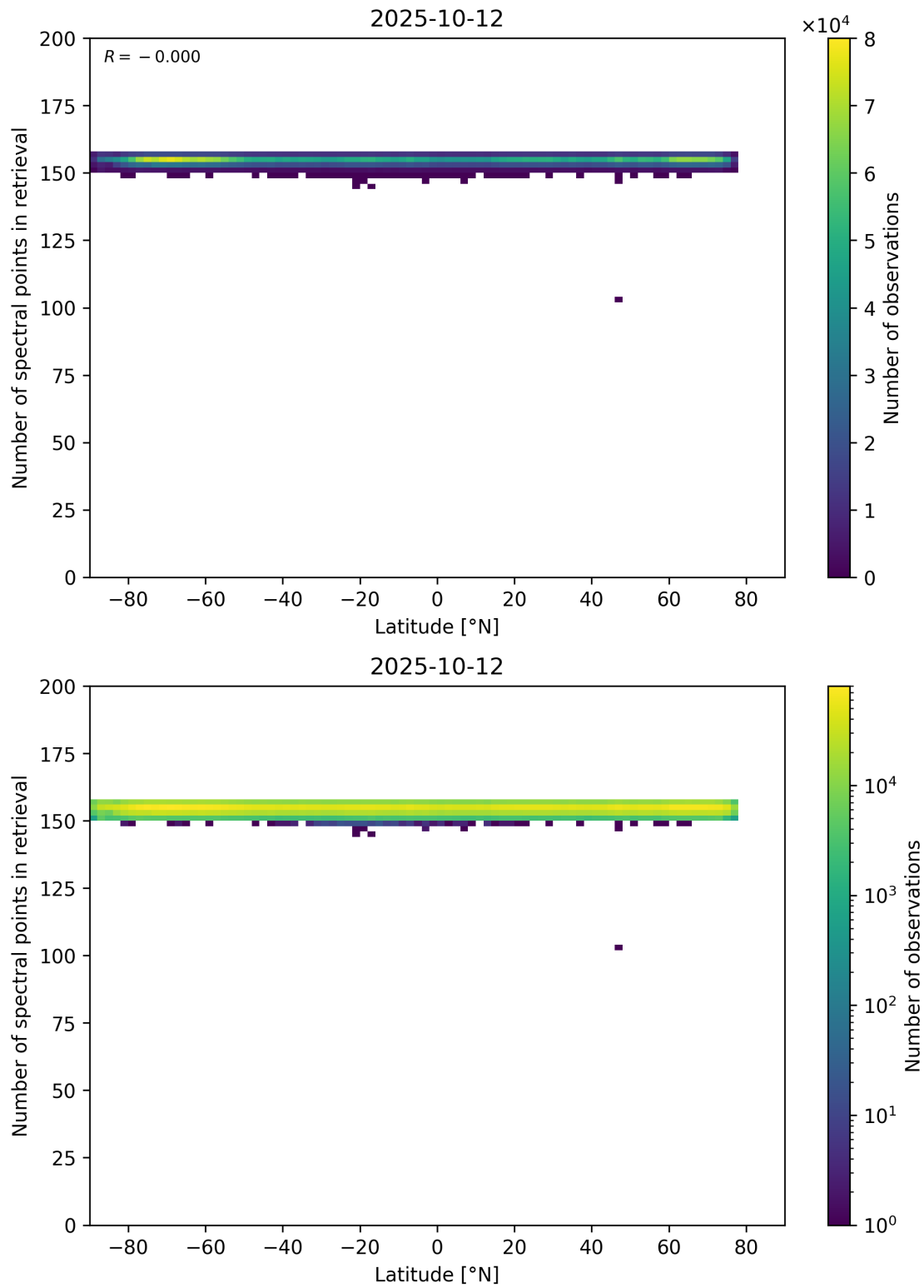
Figure 57: Scatter density plot of “Latitude” against “Number of spectral points in retrieval” for 2025-10-11 to 2025-10-13.
