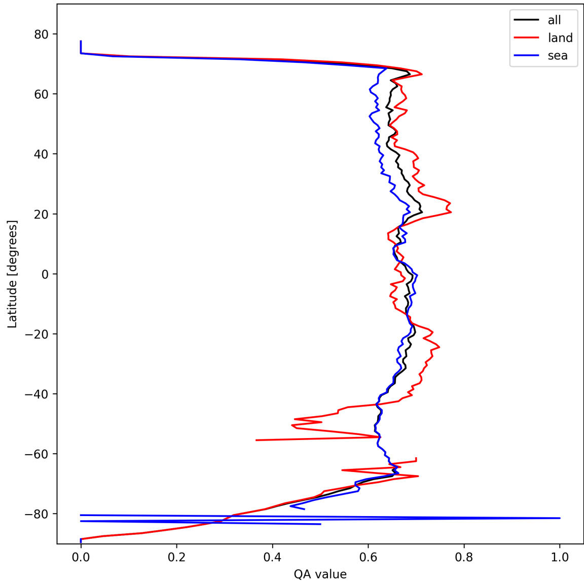
Figure 9: Zonal average of “QA value” for 2025-10-11 to 2025-10-13.
