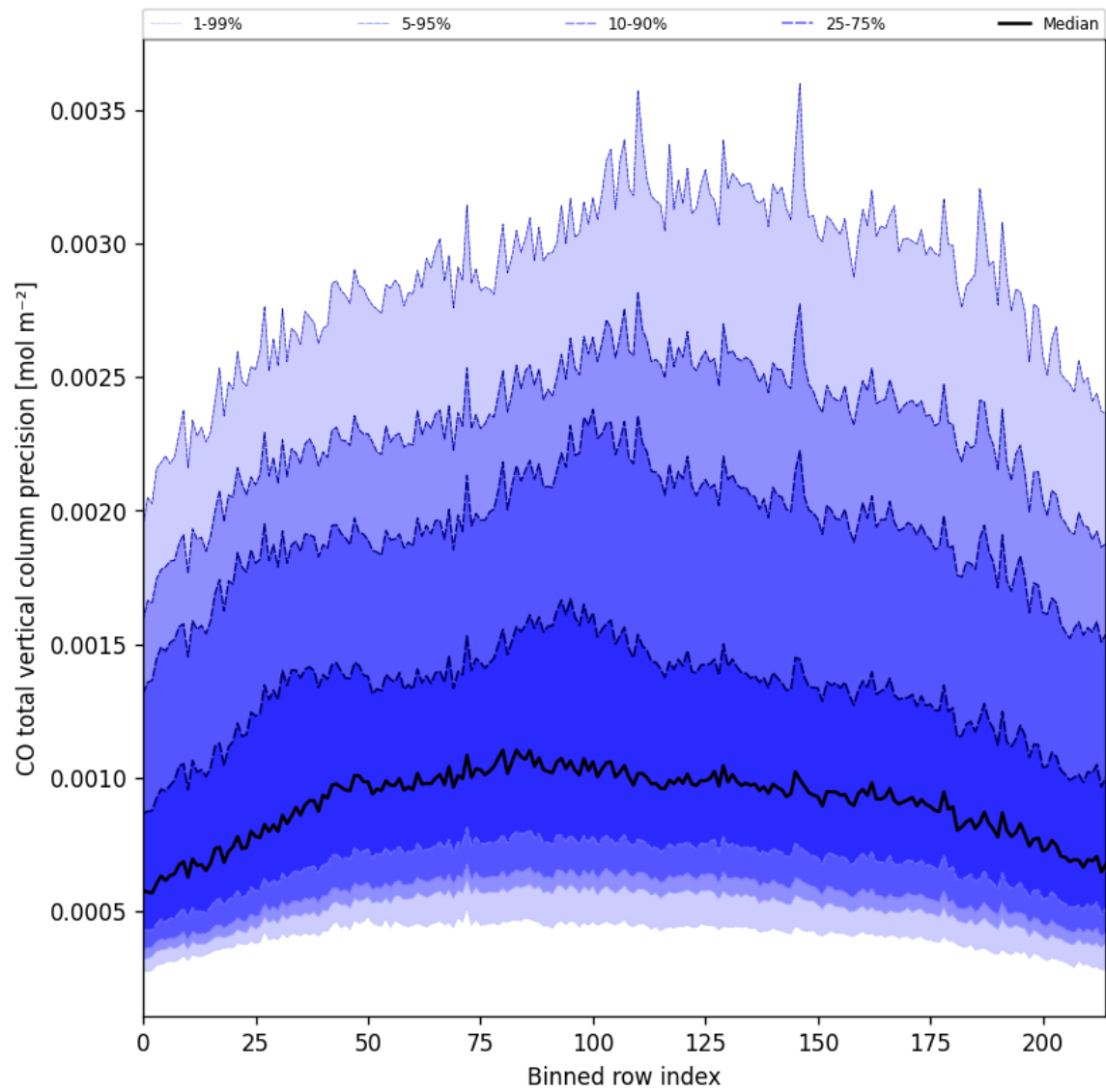
Figure 28: Along track statistics of “CO total vertical column precision” for 2025-10-11 to 2025-10-13
