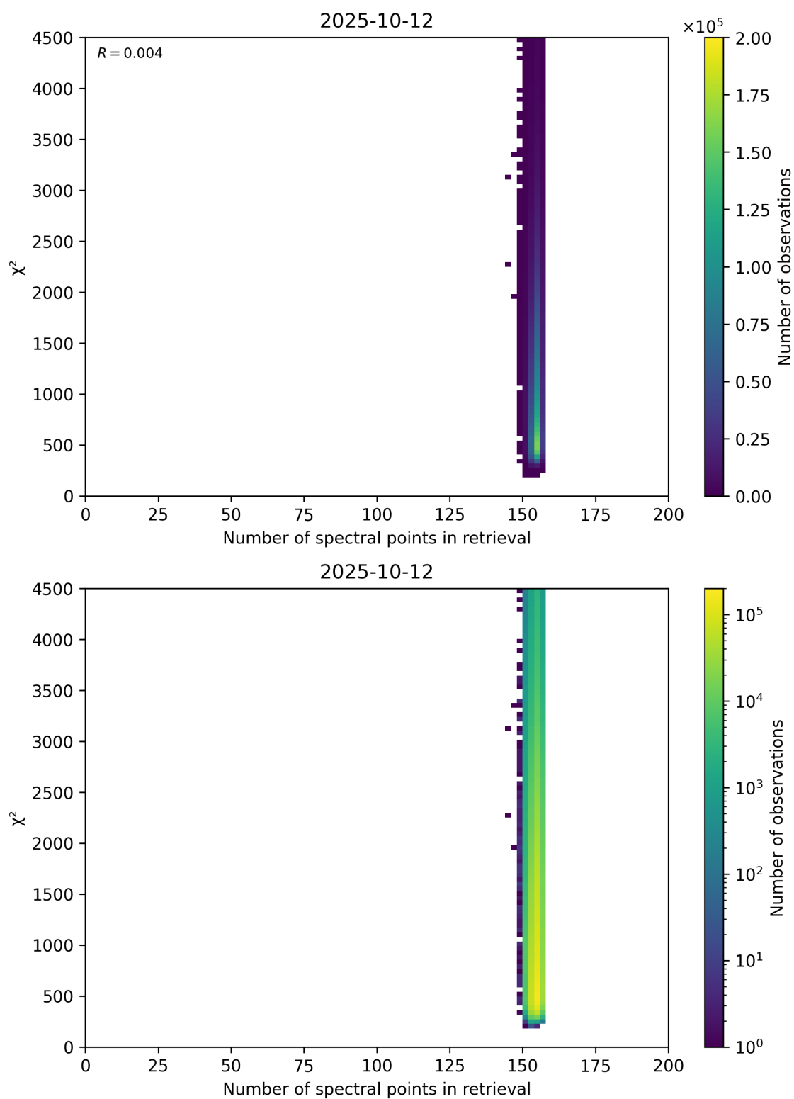
Figure 58: Scatter density plot of “Number of spectral points in retrieval” against “ \chi^2 ” for 2025-10-11 to 2025-10-13.
