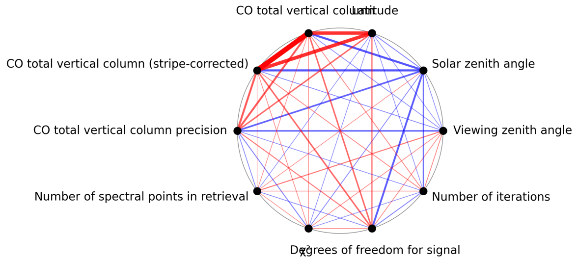
Figure 1: Map of correlation graph for 2025-10-11 to 2025-10-13.
