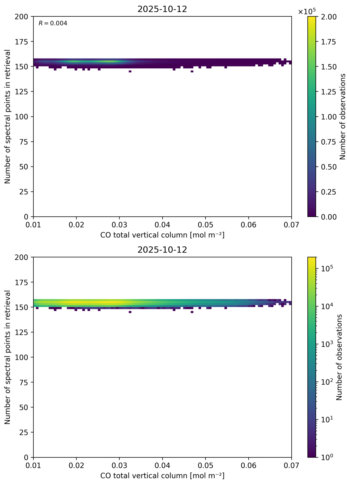
Figure 43: Scatter density plot of “CO total vertical column” against “Number of spectral points in retrieval” for 2025-10-11 to 2025-10-13.
