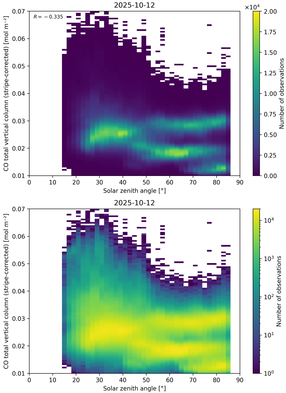
Figure 62: Scatter density plot of “Solar zenith angle” against “CO total vertical column (stripe-corrected)” for 2025-10-11 to 2025-10-13.
