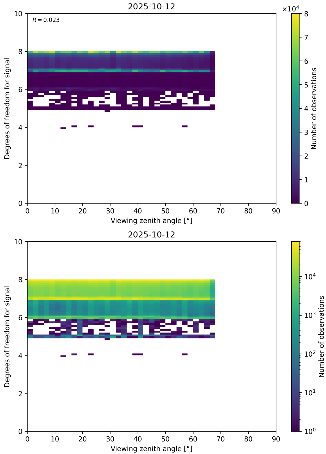
Figure 73: Scatter density plot of “Viewing zenith angle” against “Degrees of freedom for signal” for 2025-10-11 to 2025-10-13.
