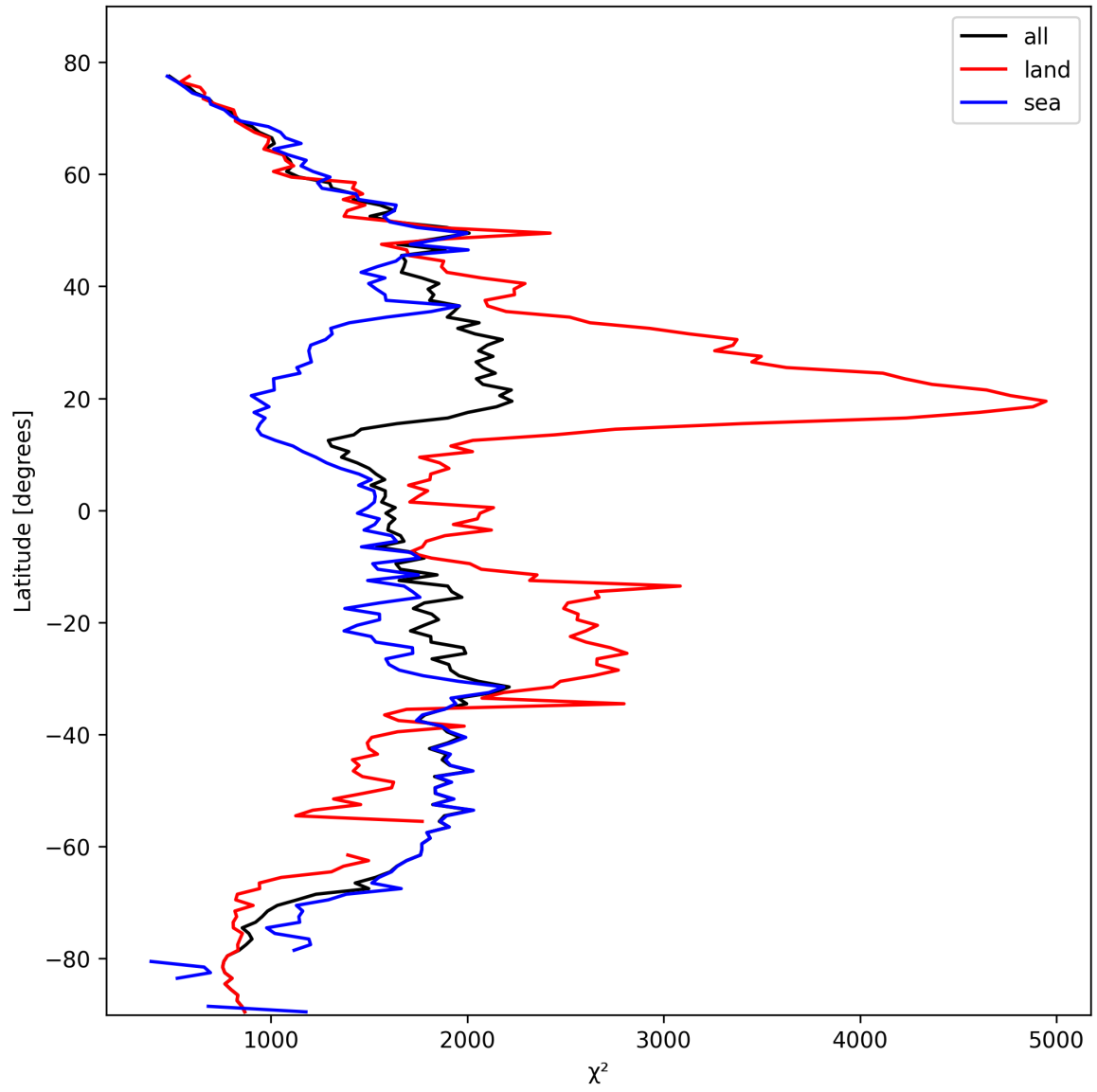
Figure 14: Zonal average of “ \chi^2 ” for 2025-10-11 to 2025-10-13.
