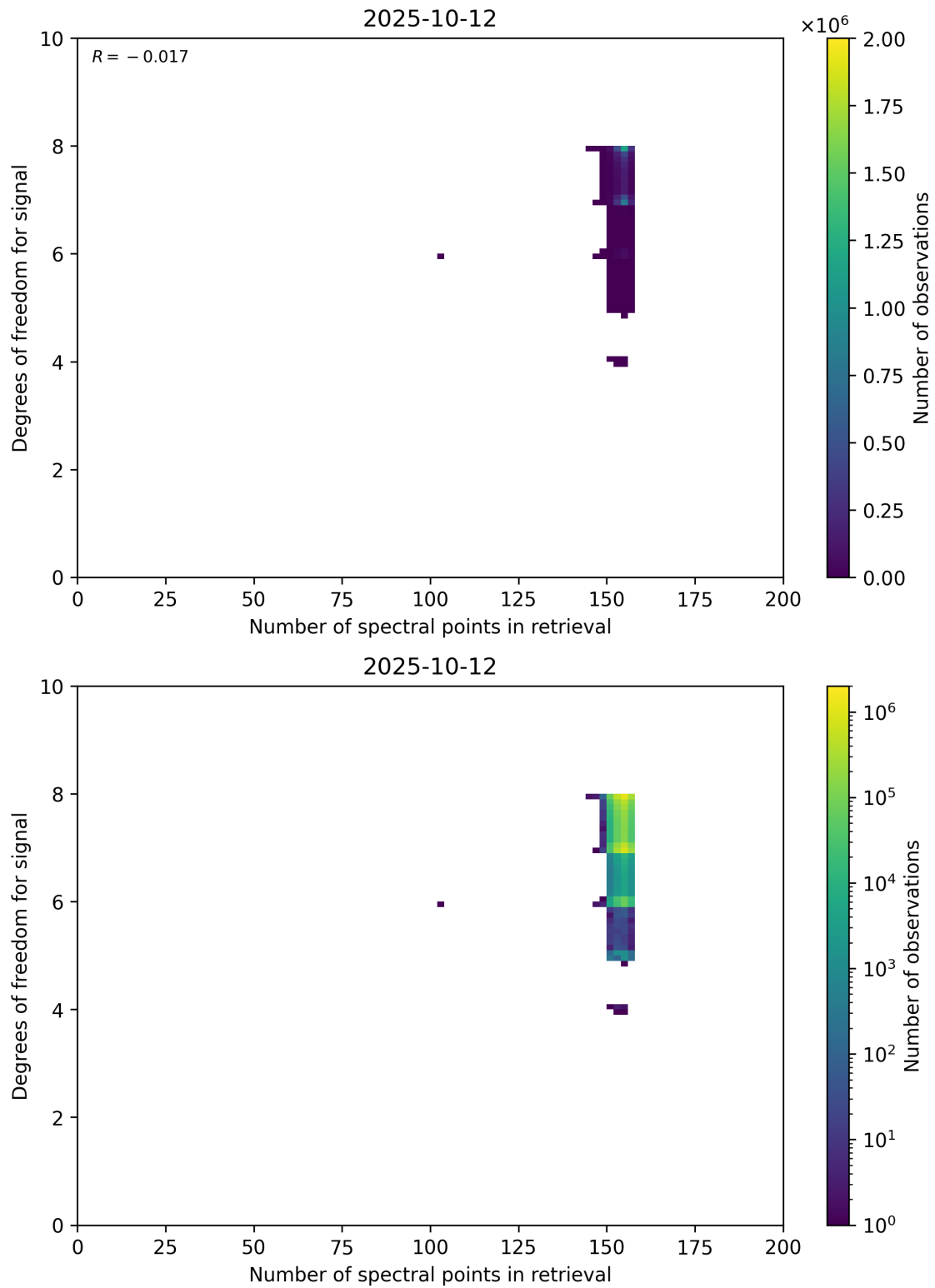
Figure 59: Scatter density plot of “Number of spectral points in retrieval” against “Degrees of freedom for signal” for 2025-10-11 to 2025-10-13.
