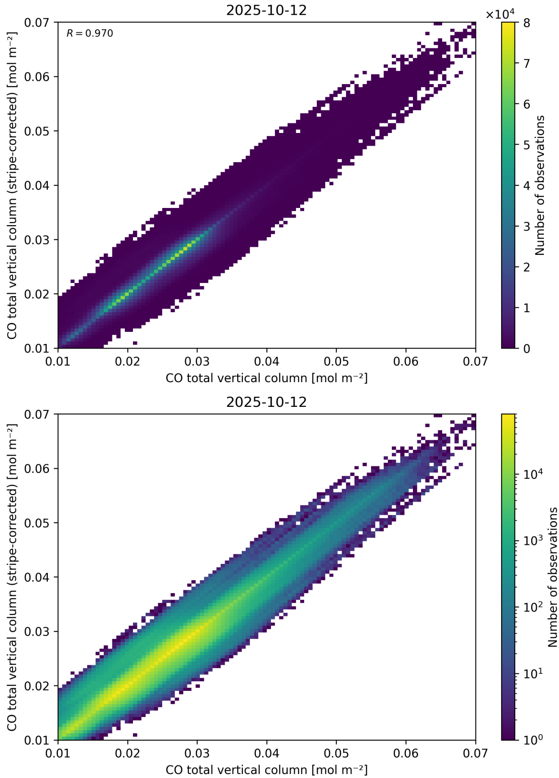
Figure 33: Scatter density plot of “CO total vertical column” against “CO total vertical column (stripe-corrected)” for 2025-10-11 to 2025-10-13.
