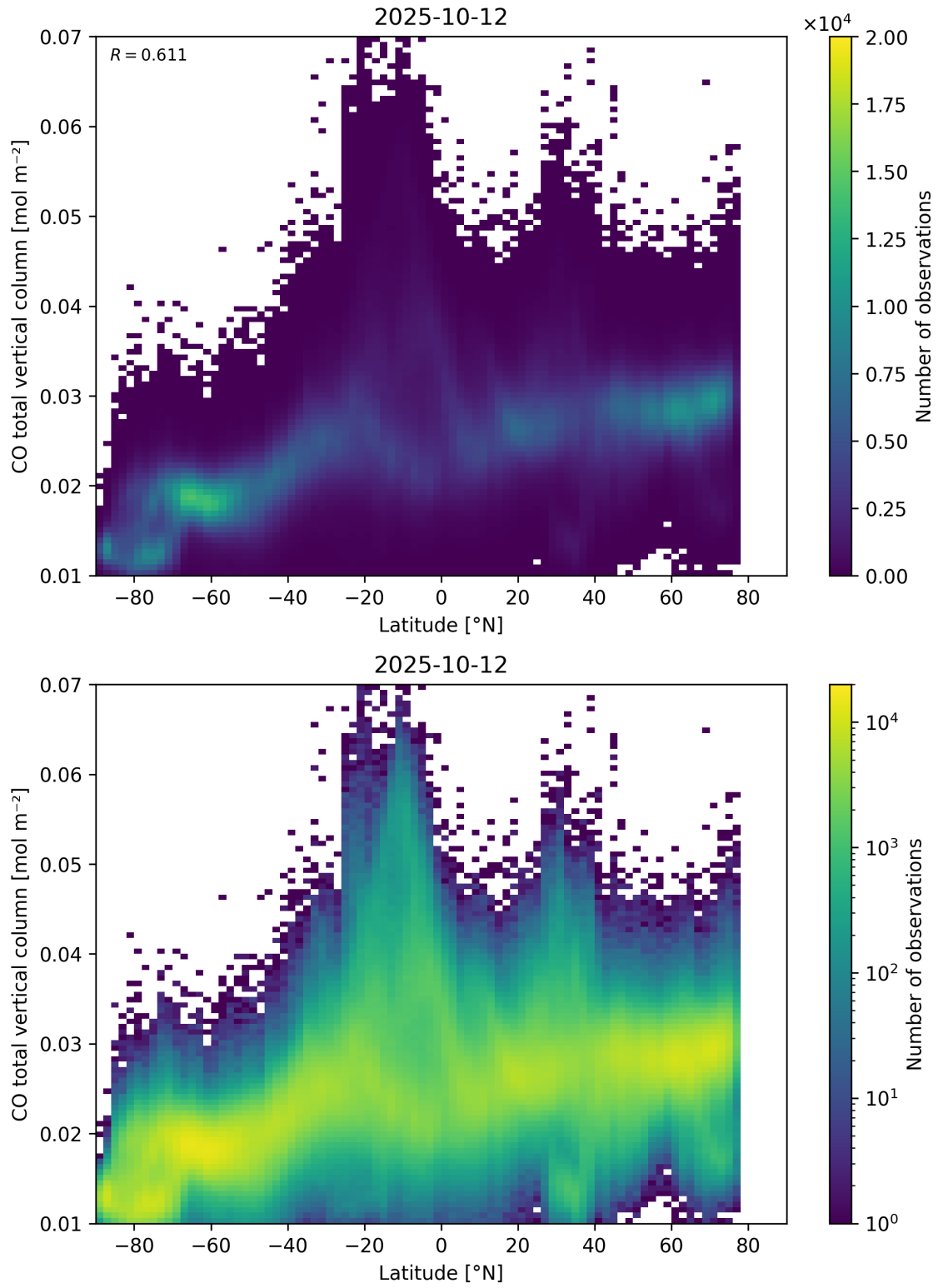
Figure 51: Scatter density plot of “Latitude” against “CO total vertical column” for 2025-10-11 to 2025-10-13.
