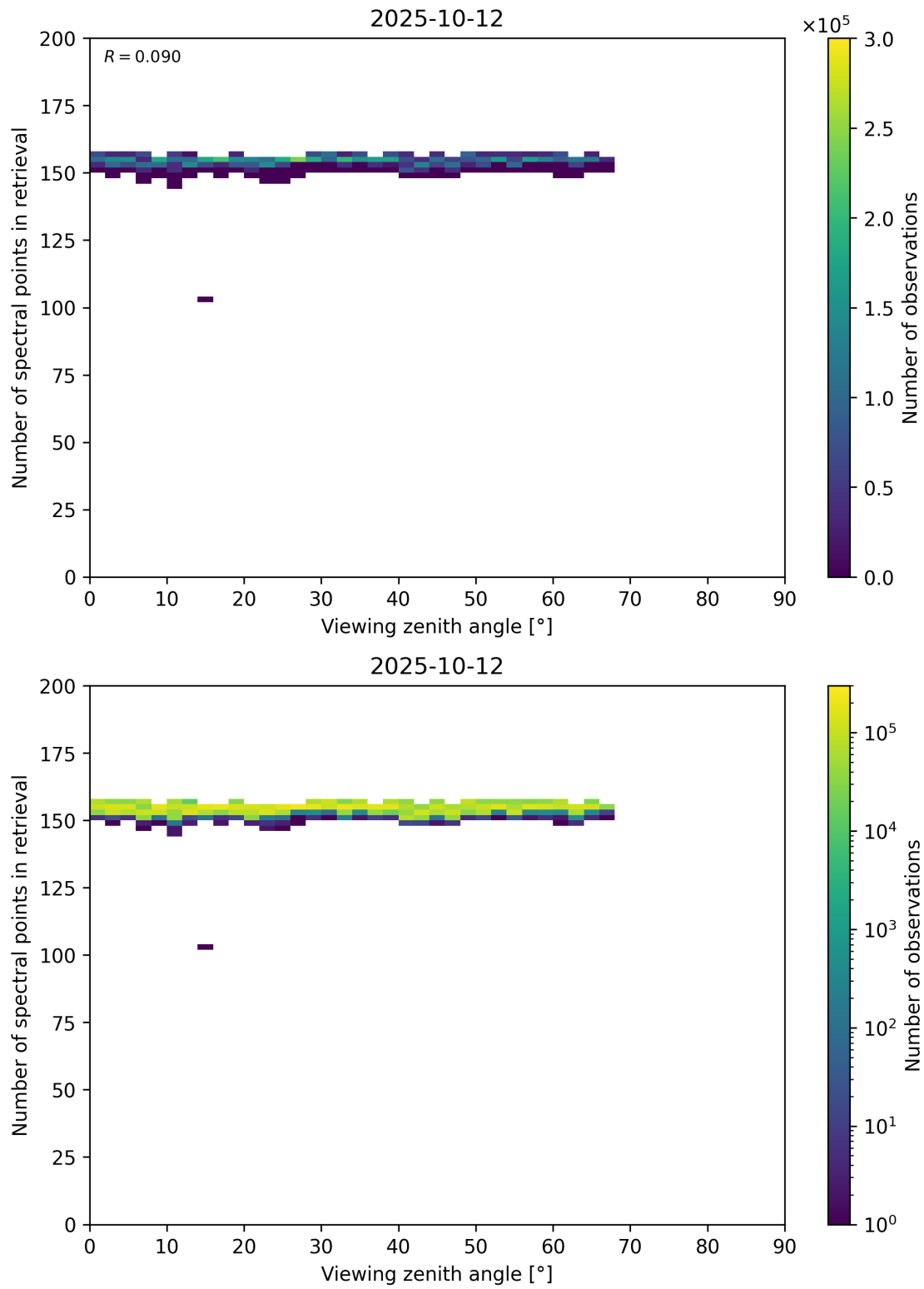
Figure 76: Scatter density plot of “Viewing zenith angle” against “Number of spectral points in retrieval” for 2025-10-11 to 2025-10-13.
