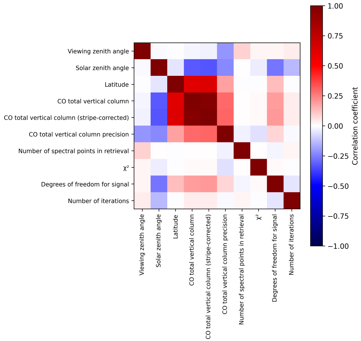
Figure 2: Map of correlation matrix for 2025-10-11 to 2025-10-13.
