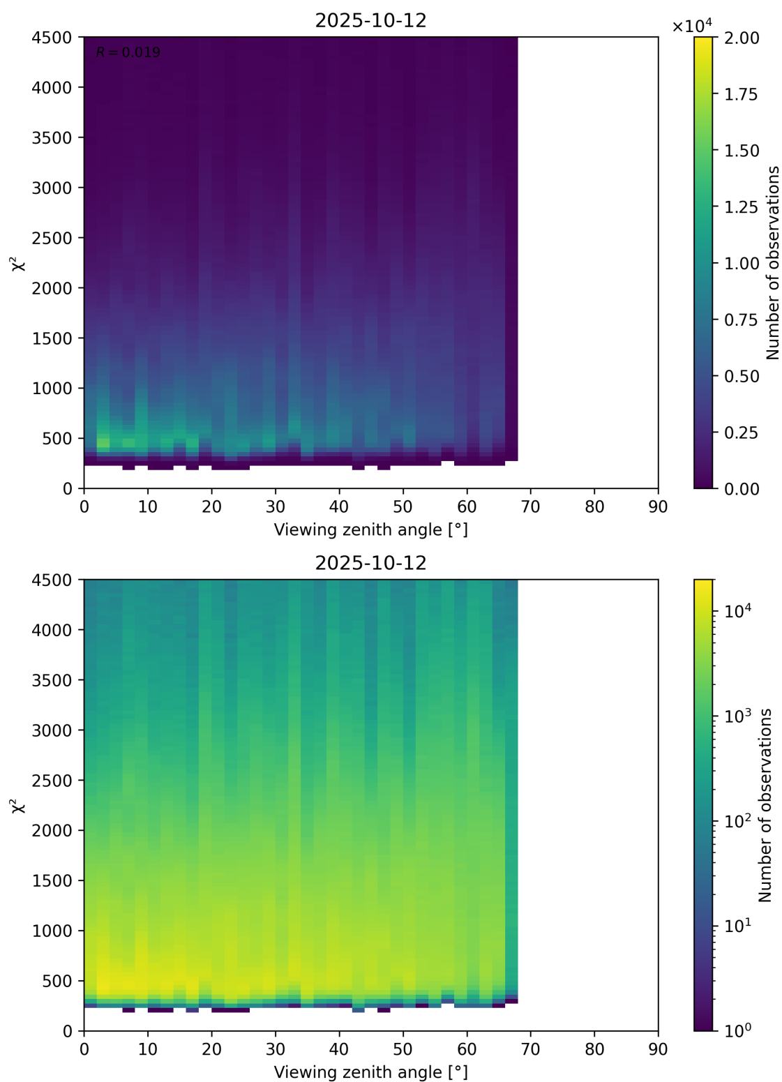
Figure 72: Scatter density plot of “Viewing zenith angle” against “ \chi^2 ” for 2025-10-11 to 2025-10-13.
