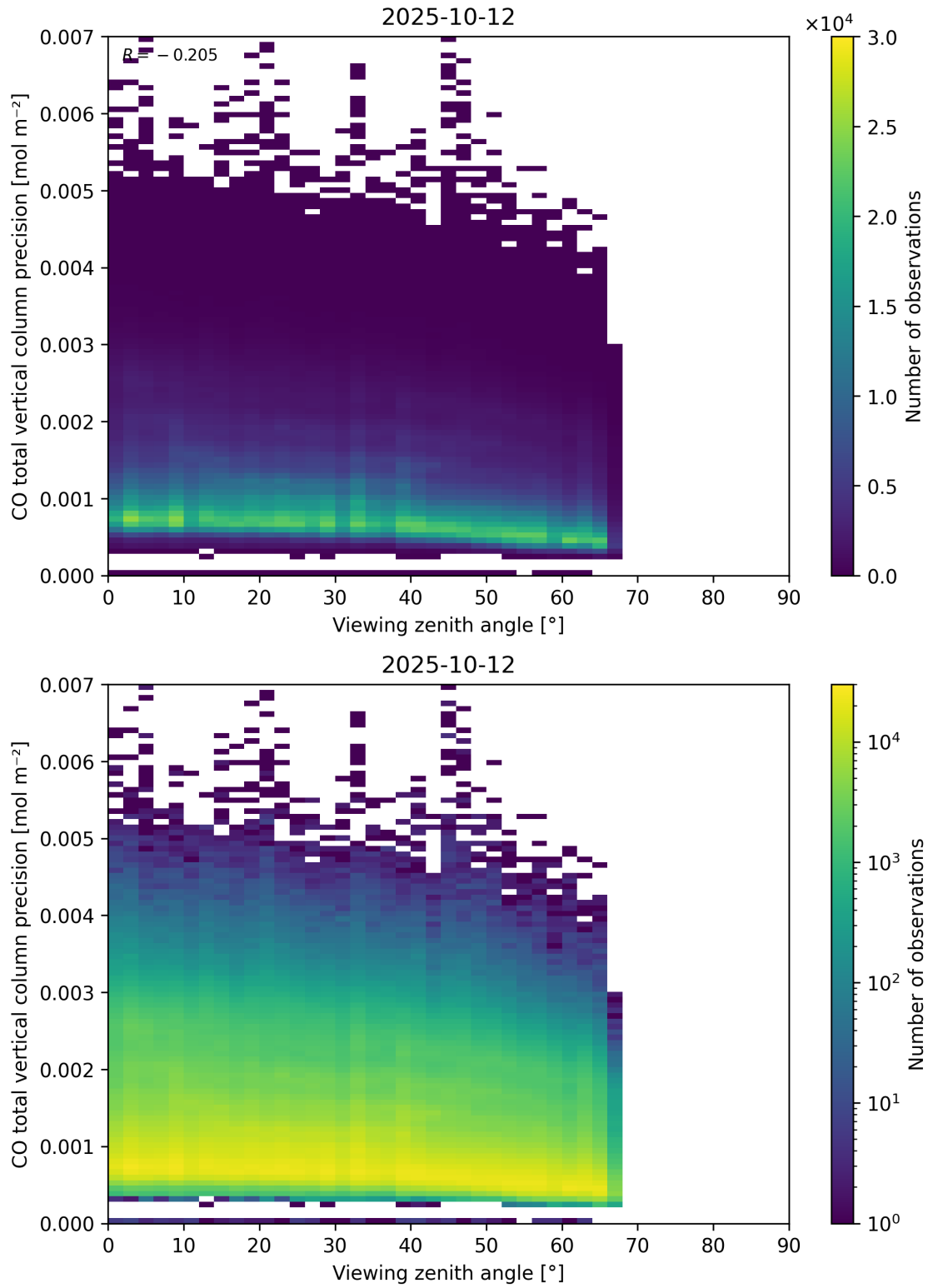
Figure 71: Scatter density plot of “Viewing zenith angle” against “CO total vertical column precision” for 2025-10-11 to 2025-10-13.
