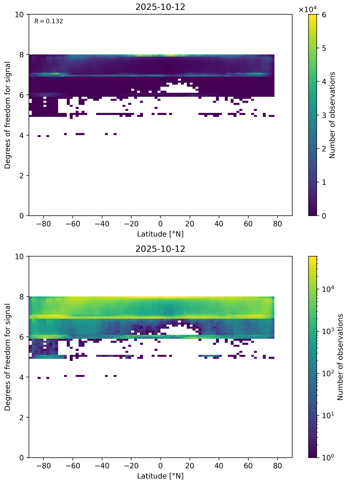
Figure 55: Scatter density plot of “Latitude” against “Degrees of freedom for signal” for 2025-10-11 to 2025-10-13.
