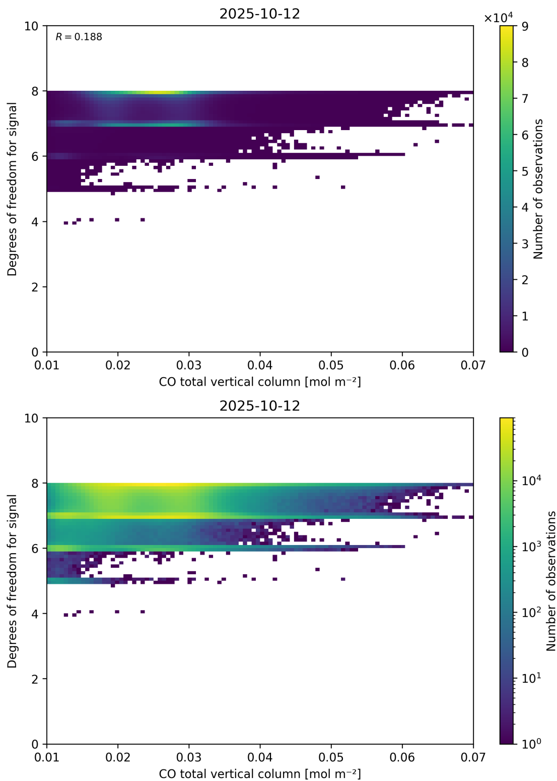
Figure 41: Scatter density plot of “CO total vertical column” against “Degrees of freedom for signal” for 2025-10-11 to 2025-10-13.
