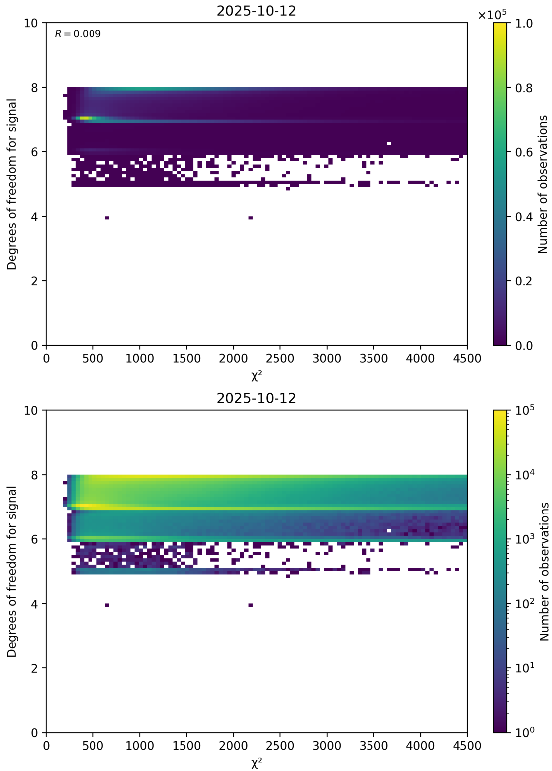
Figure 48: Scatter density plot of “ \chi^2 ” against “Degrees of freedom for signal” for 2025-10-11 to 2025-10-13.
