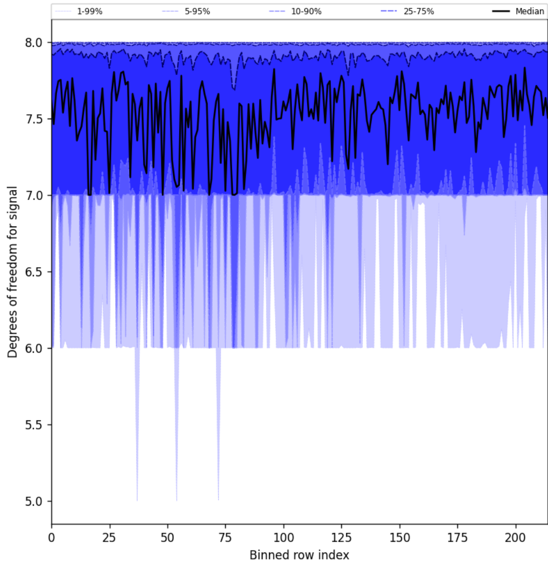
Figure 31: Along track statistics of “Degrees of freedom for signal” for 2025-10-11 to 2025-10-13
