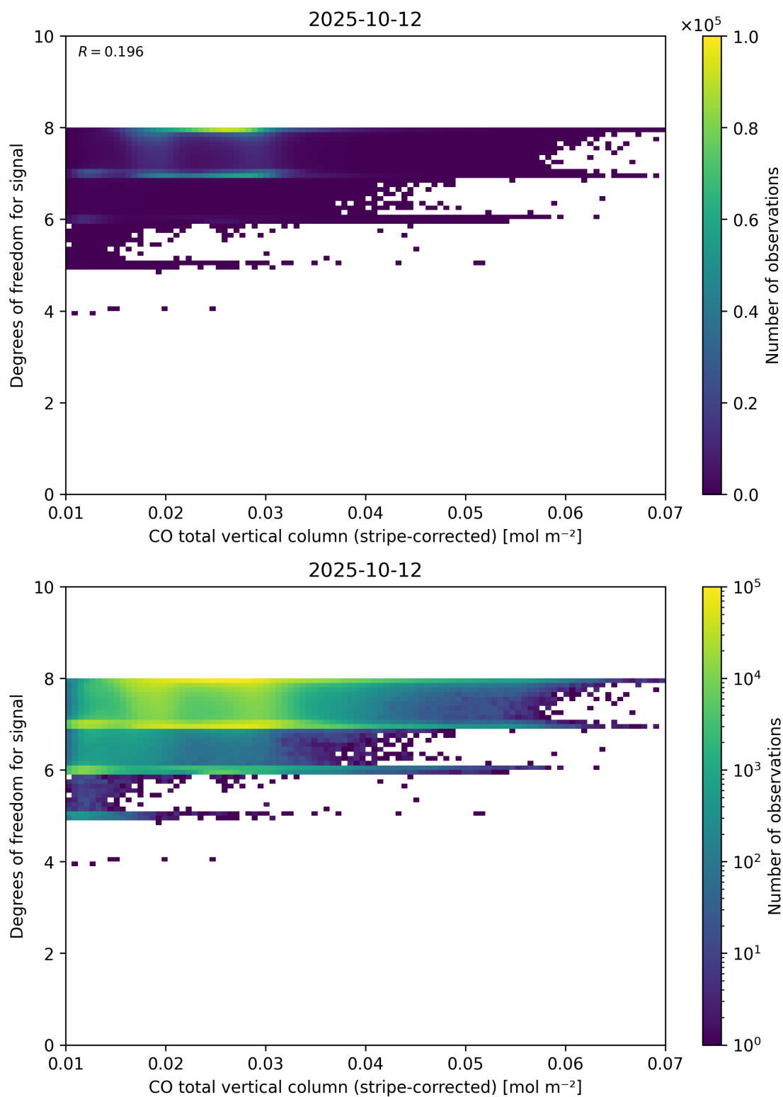
Figure 38: Scatter density plot of “CO total vertical column (stripe-corrected)” against “Degrees of freedom for signal” for 2025-10-11 to 2025-10-13.
