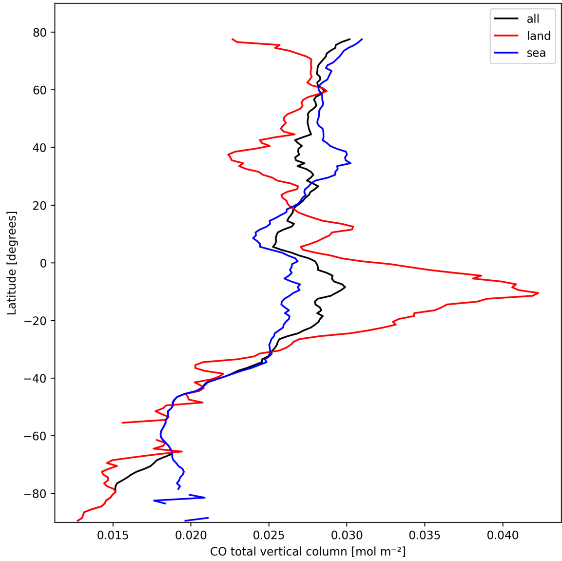
Figure 10: Zonal average of “CO total vertical column” for 2025-10-11 to 2025-10-13.
