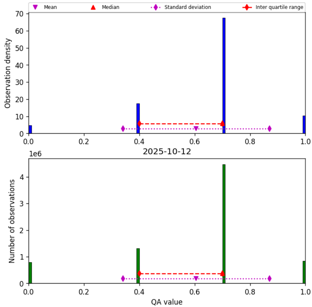
Figure 17: Histogram of “QA value” for 2025-10-11 to 2025-10-13
