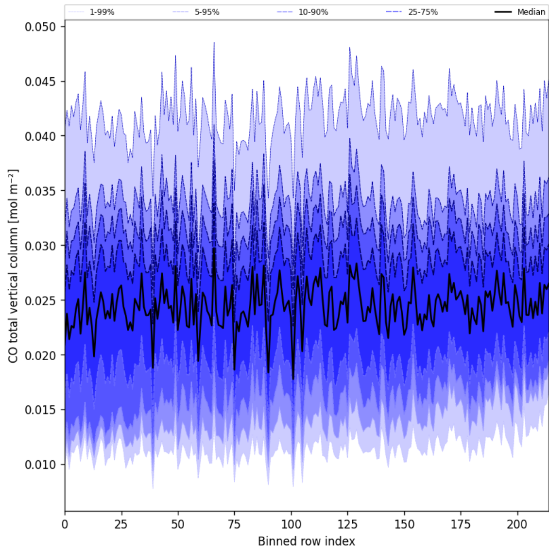
Figure 26: Along track statistics of “CO total vertical column” for 2025-10-11 to 2025-10-13
