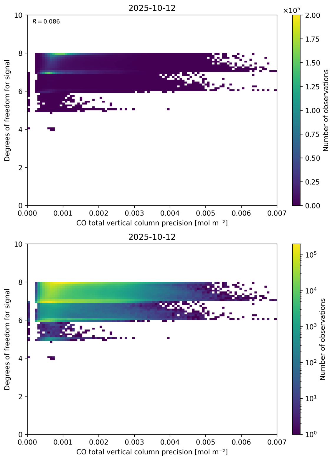
Figure 45: Scatter density plot of “CO total vertical column precision” against “Degrees of freedom for signal” for 2025-10-11 to 2025-10-13.
