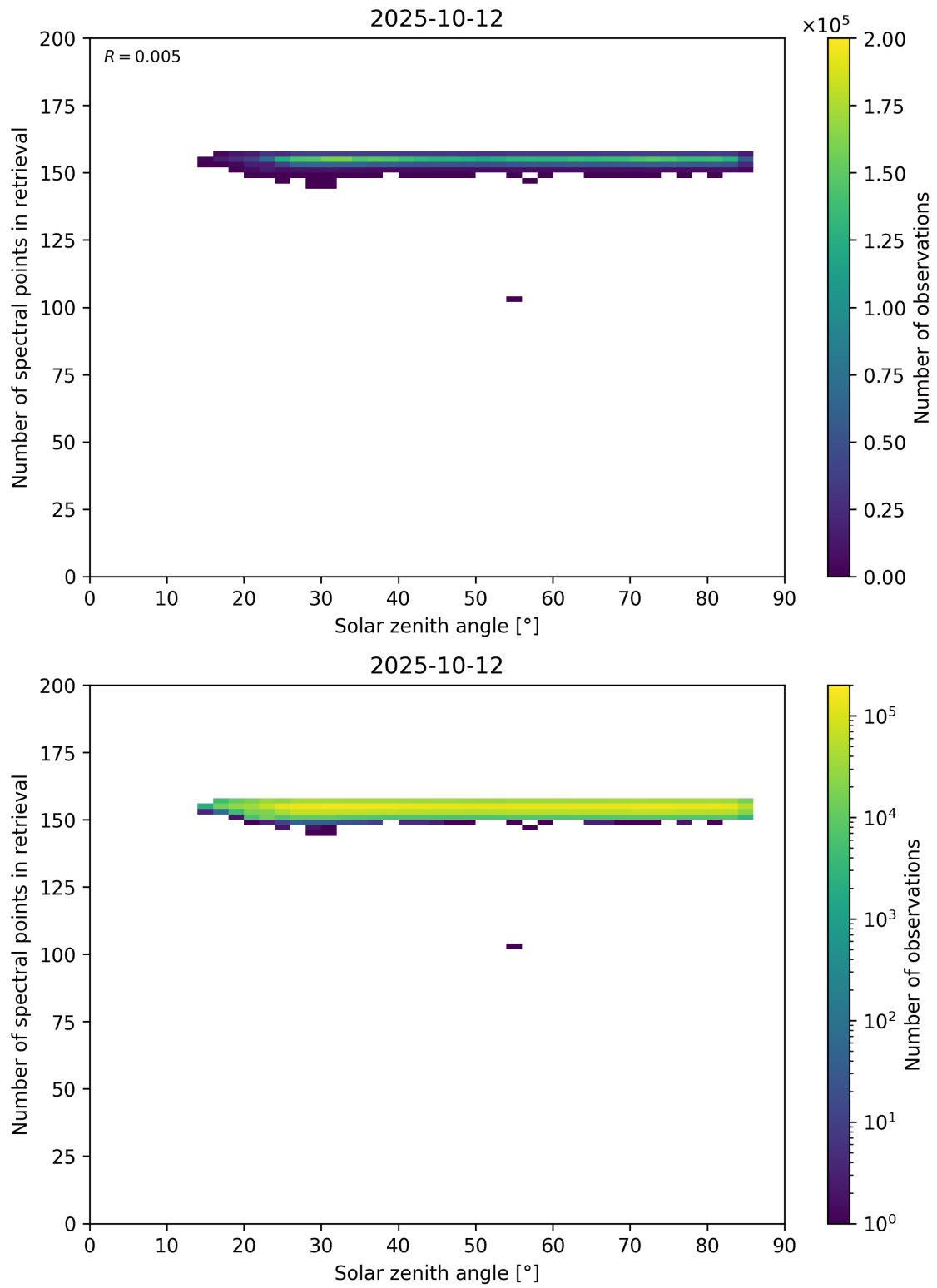
Figure 68: Scatter density plot of “Solar zenith angle” against “Number of spectral points in retrieval” for 2025-10-11 to 2025-10-13.
