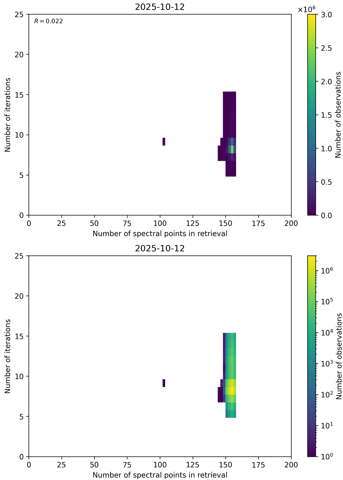
Figure 60: Scatter density plot of “Number of spectral points in retrieval” against “Number of iterations” for 2025-10-11 to 2025-10-13.
