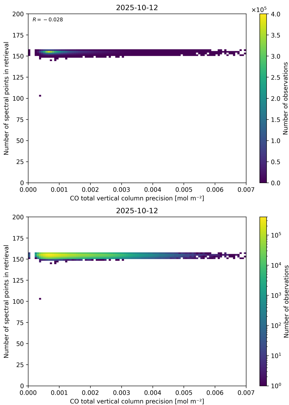
Figure 47: Scatter density plot of “CO total vertical column precision” against “Number of spectral points in retrieval” for 2025-10-11 to 2025-10-13.
