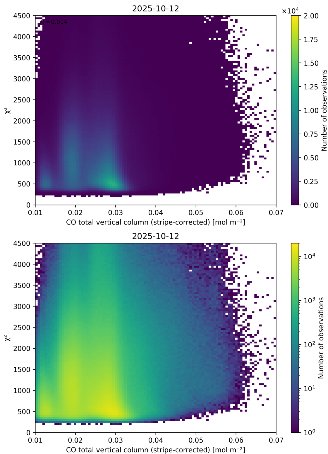
Figure 37: Scatter density plot of “CO total vertical column (stripe-corrected)” against “ \chi^2 ” for 2025-10-11 to 2025-10-13.
