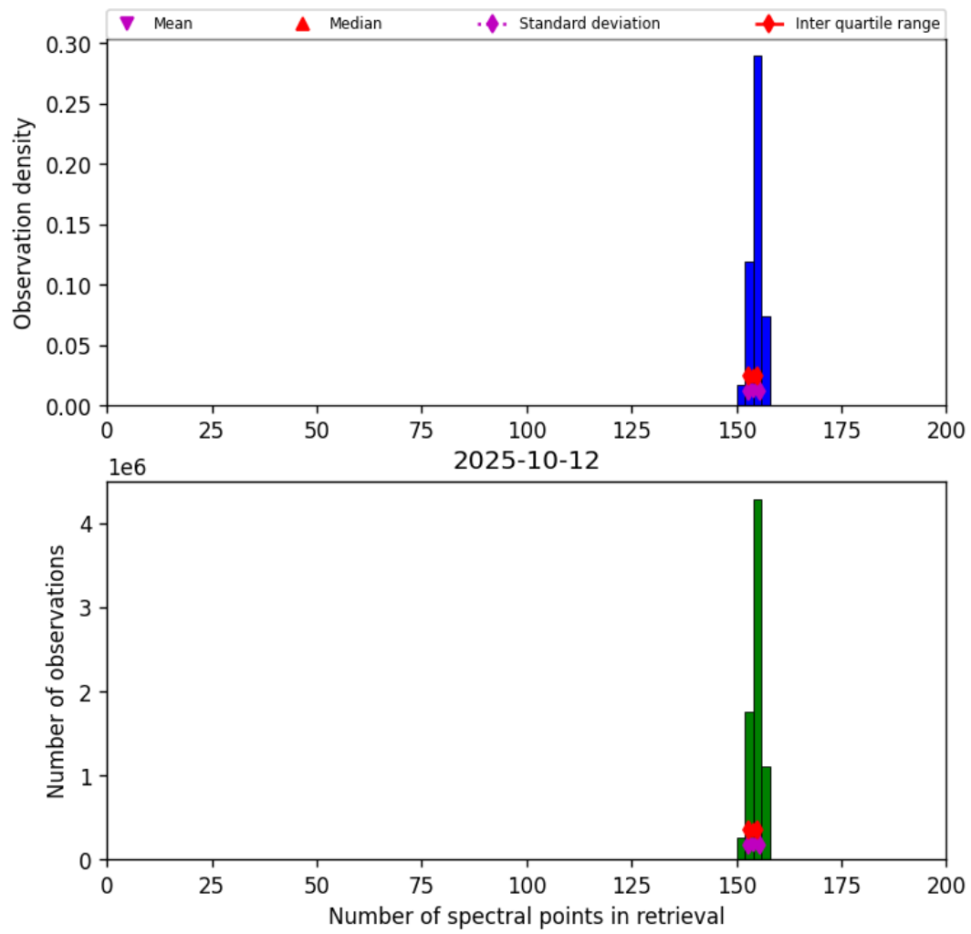
Figure 21: Histogram of “Number of spectral points in retrieval” for 2025-10-11 to 2025-10-13
