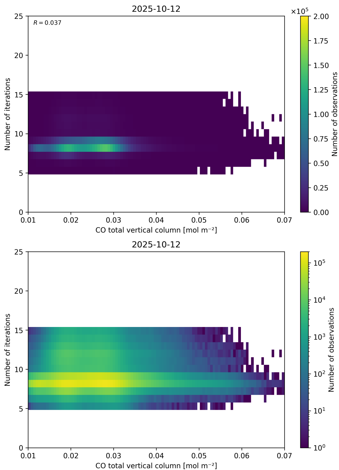
Figure 42: Scatter density plot of “CO total vertical column” against “Number of iterations” for 2025-10-11 to 2025-10-13.
