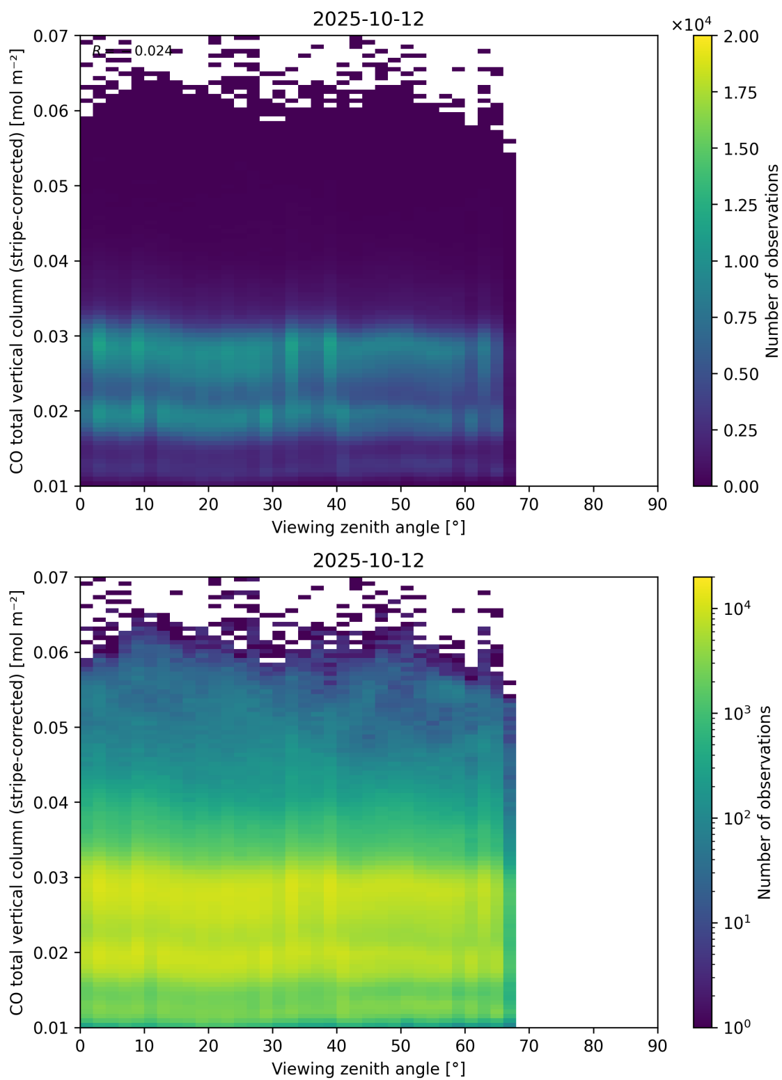
Figure 70: Scatter density plot of “Viewing zenith angle” against “CO total vertical column (stripe-corrected)” for 2025-10-11 to 2025-10-13.
