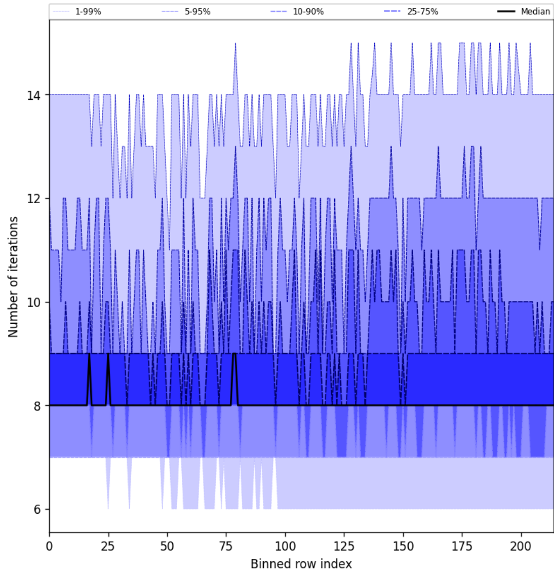
Figure 32: Along track statistics of “Number of iterations” for 2025-10-11 to 2025-10-13
