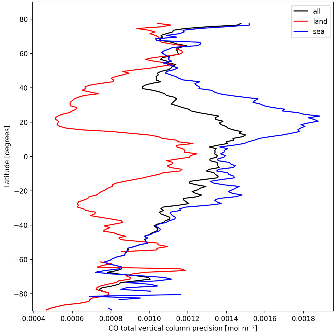
Figure 12: Zonal average of “CO total vertical column precision” for 2025-10-11 to 2025-10-13.
