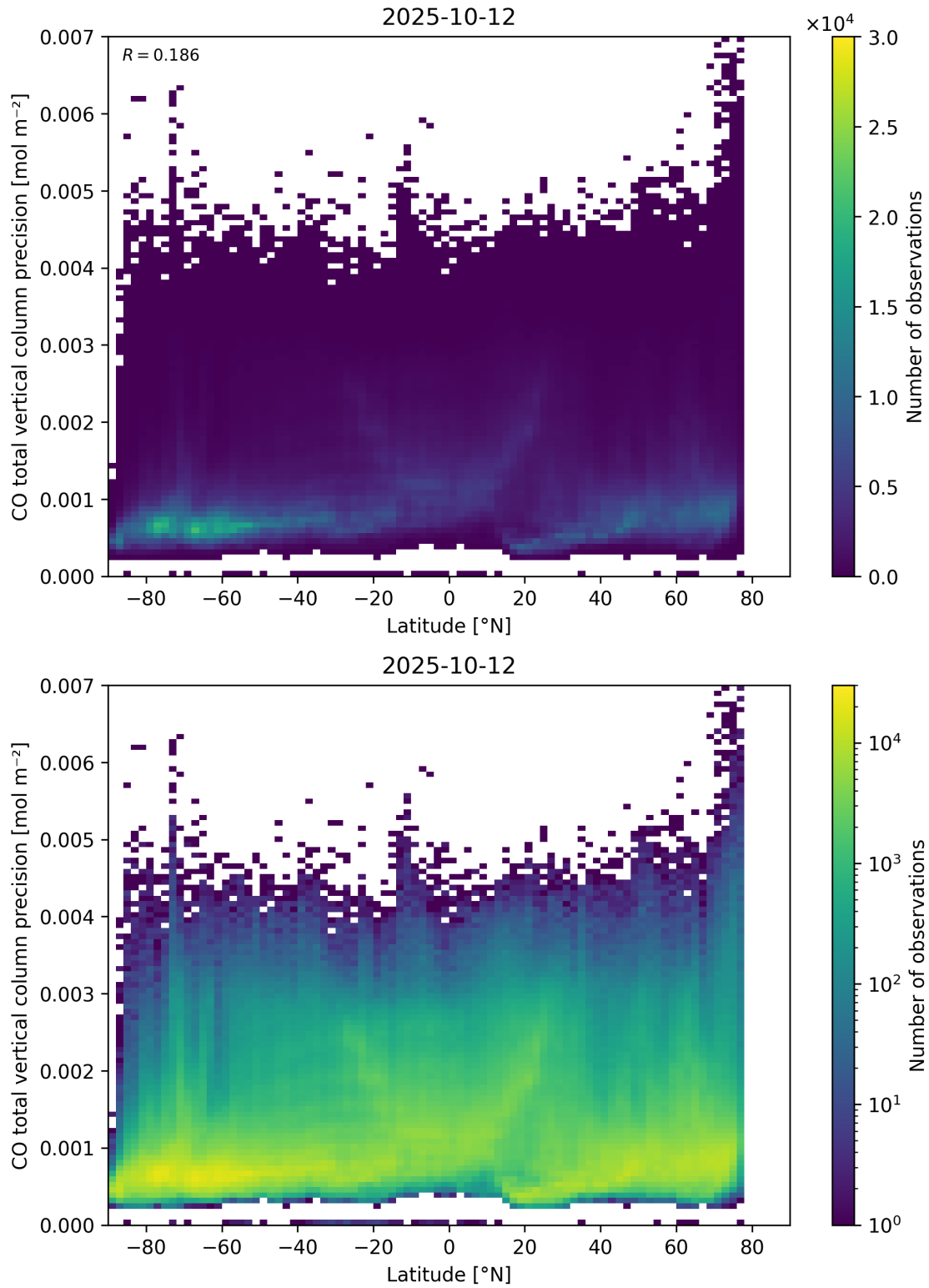
Figure 53: Scatter density plot of “Latitude” against “CO total vertical column precision” for 2025-10-11 to 2025-10-13.
