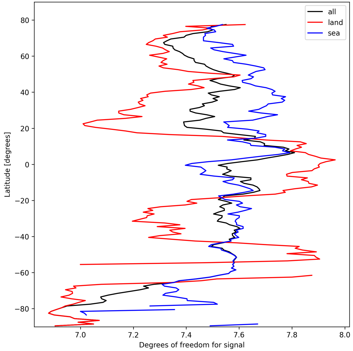
Figure 15: Zonal average of “Degrees of freedom for signal” for 2025-10-11 to 2025-10-13.
