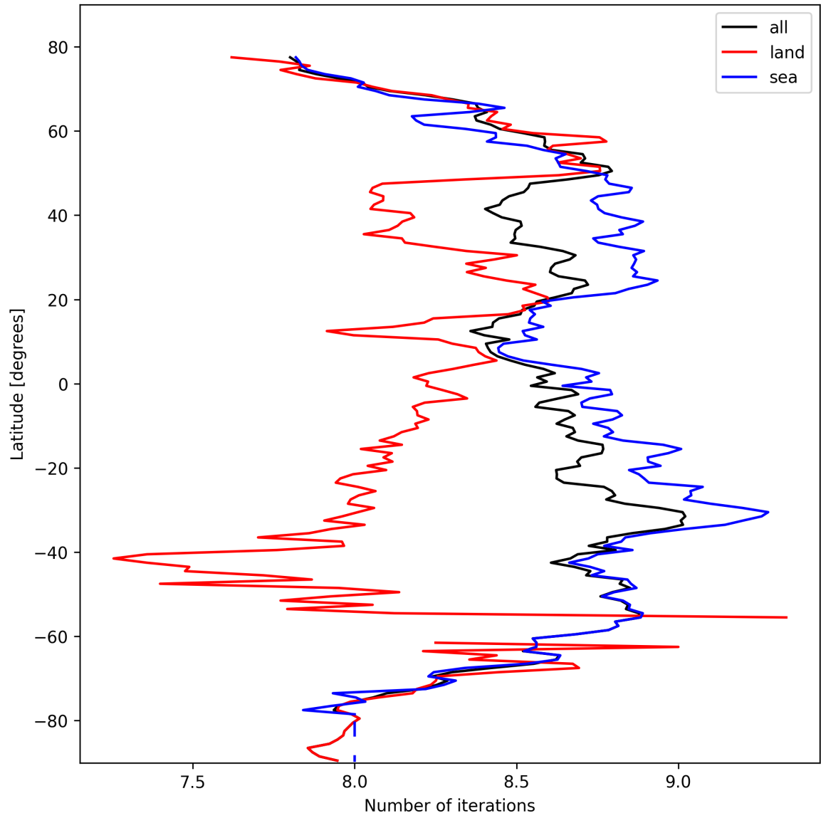
Figure 16: Zonal average of “Number of iterations” for 2025-10-11 to 2025-10-13.
