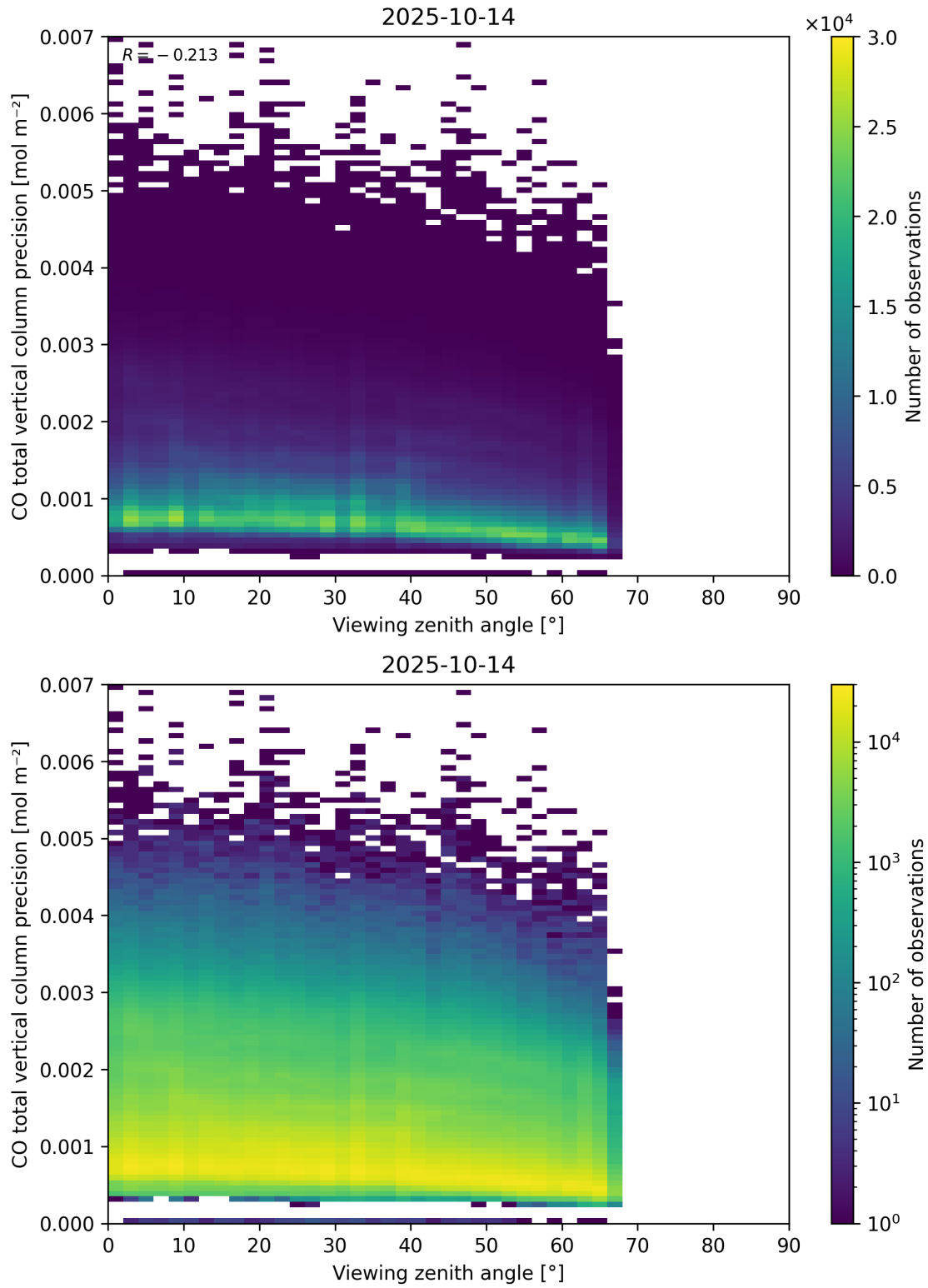
Figure 71: Scatter density plot of “Viewing zenith angle” against “CO total vertical column precision” for 2025-10-13 to 2025-10-15.
