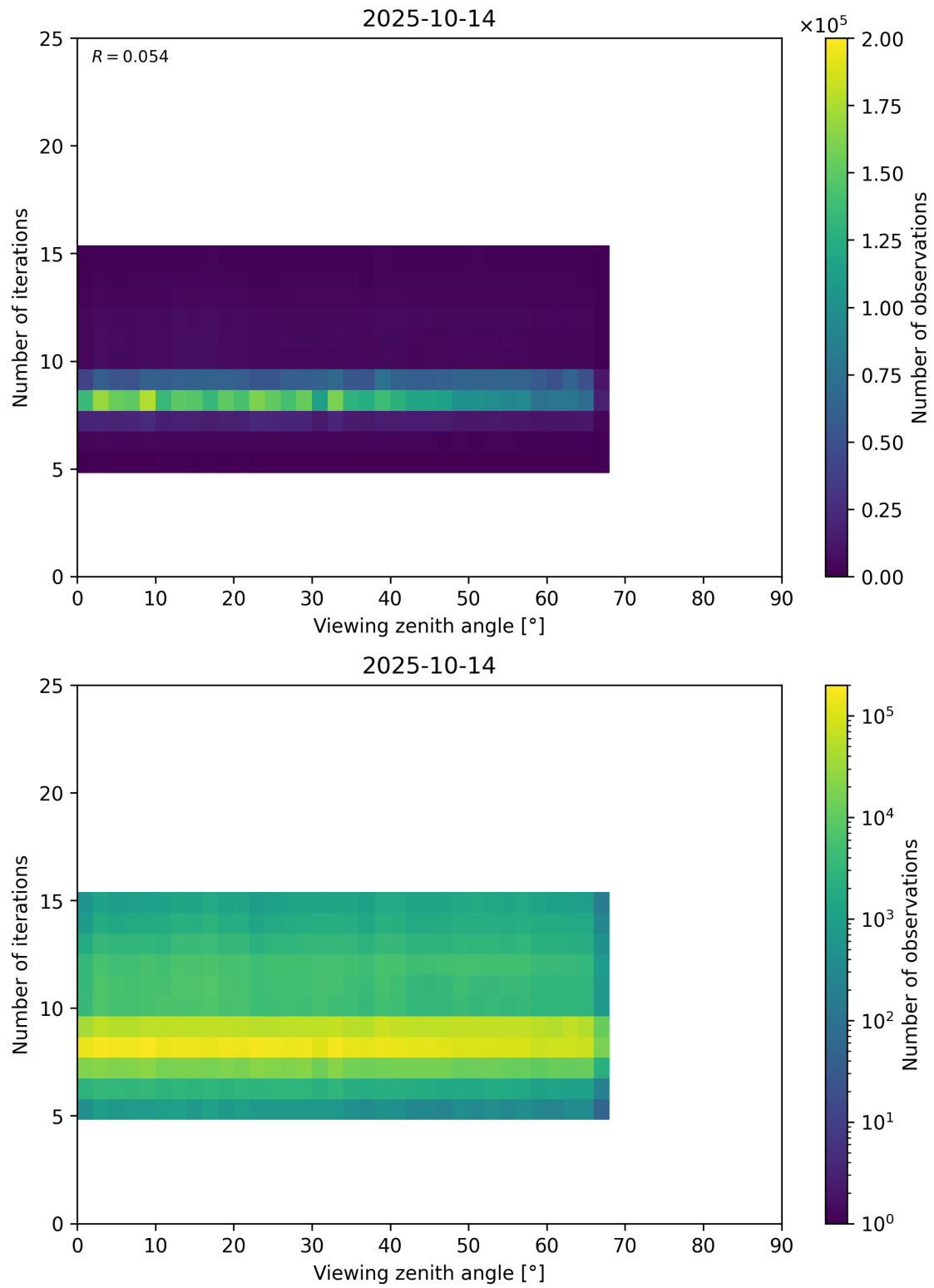
Figure 75: Scatter density plot of “Viewing zenith angle” against “Number of iterations” for 2025-10-13 to 2025-10-15.
