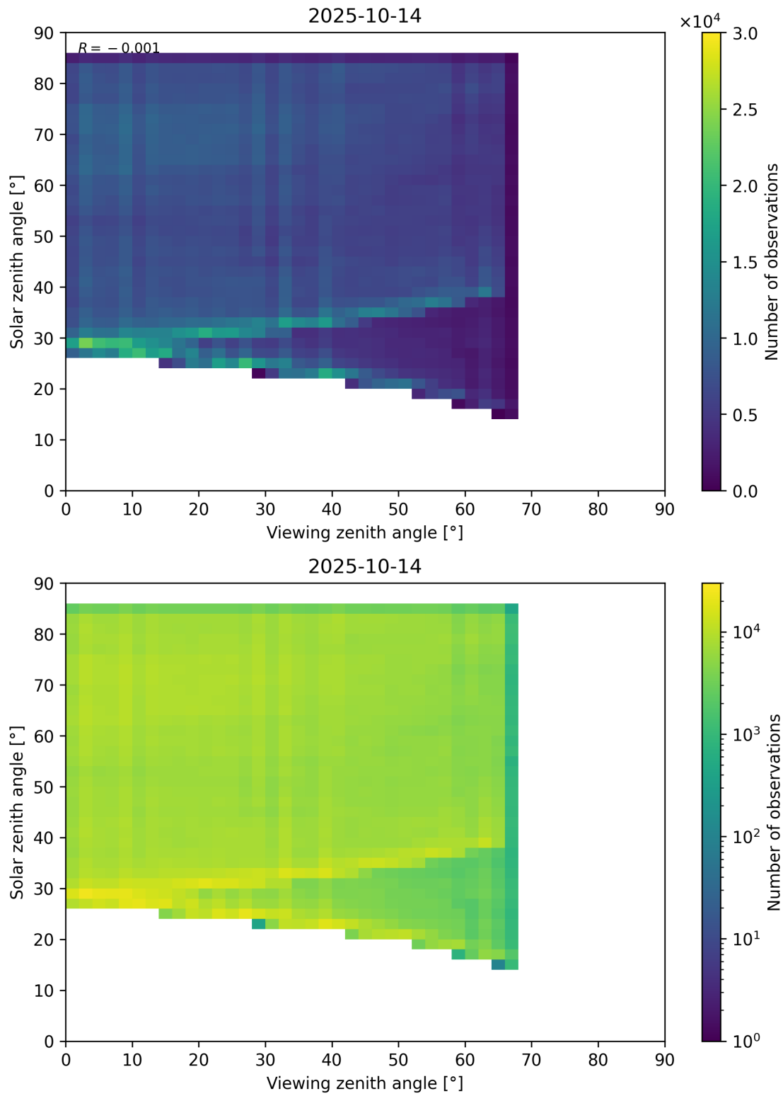
Figure 77: Scatter density plot of “Viewing zenith angle” against “Solar zenith angle” for 2025-10-13 to 2025-10-15.
