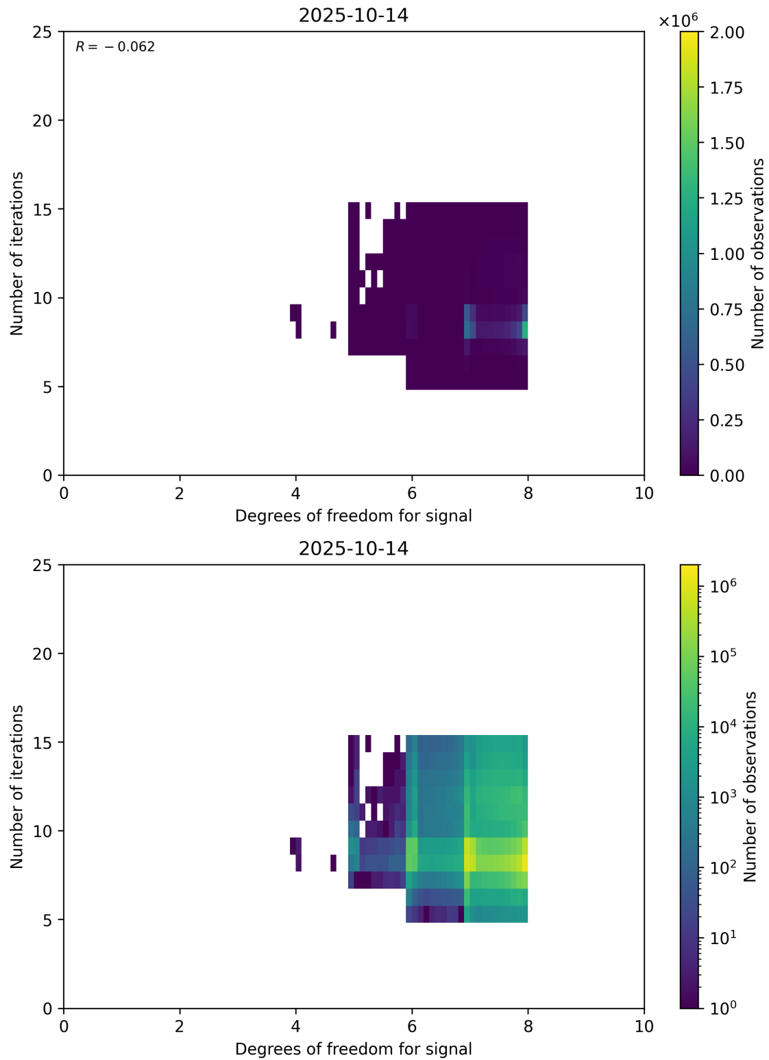
Figure 50: Scatter density plot of “Degrees of freedom for signal” against “Number of iterations” for 2025-10-13 to 2025-10-15.
