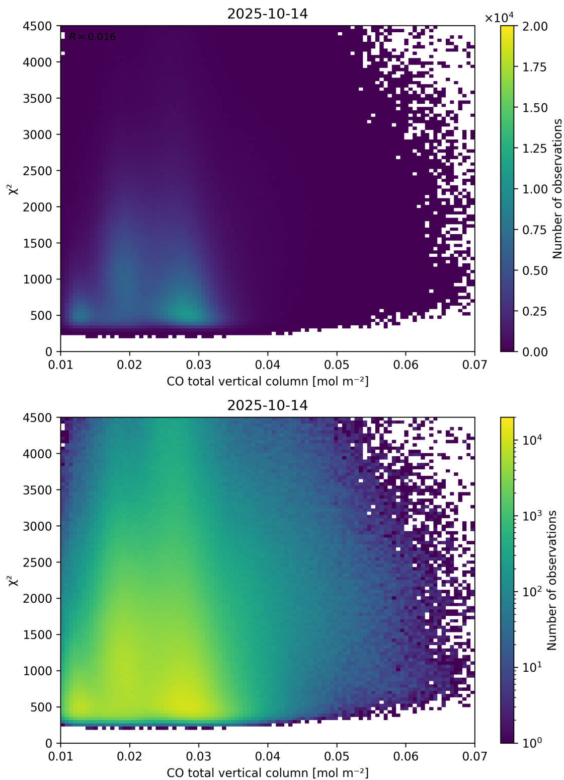
Figure 35: Scatter density plot of “CO total vertical column” against “ \chi^2 ” for 2025-10-13 to 2025-10-15.
