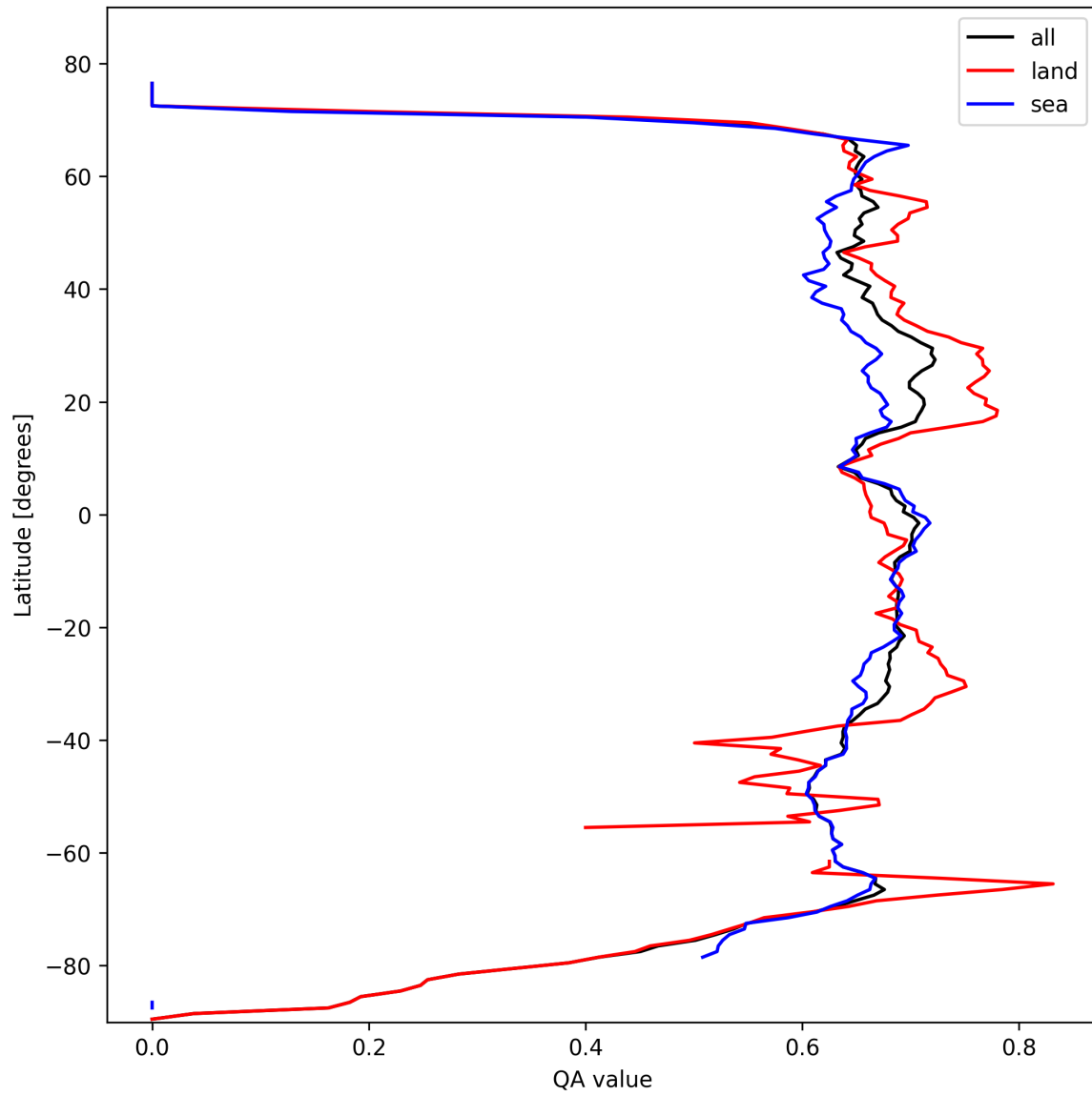
Figure 9: Zonal average of “QA value” for 2025-10-13 to 2025-10-15.
