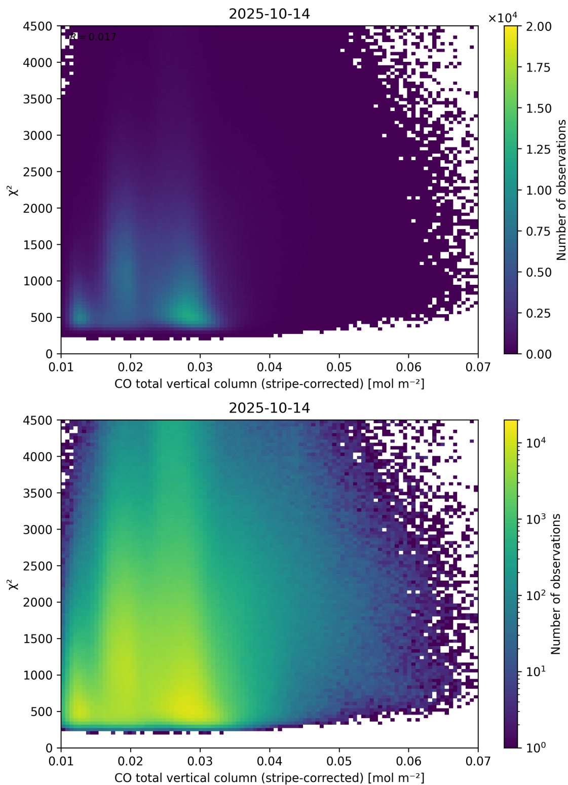
Figure 37: Scatter density plot of “CO total vertical column (stripe-corrected)” against “ \chi^2 ” for 2025-10-13 to 2025-10-15.
