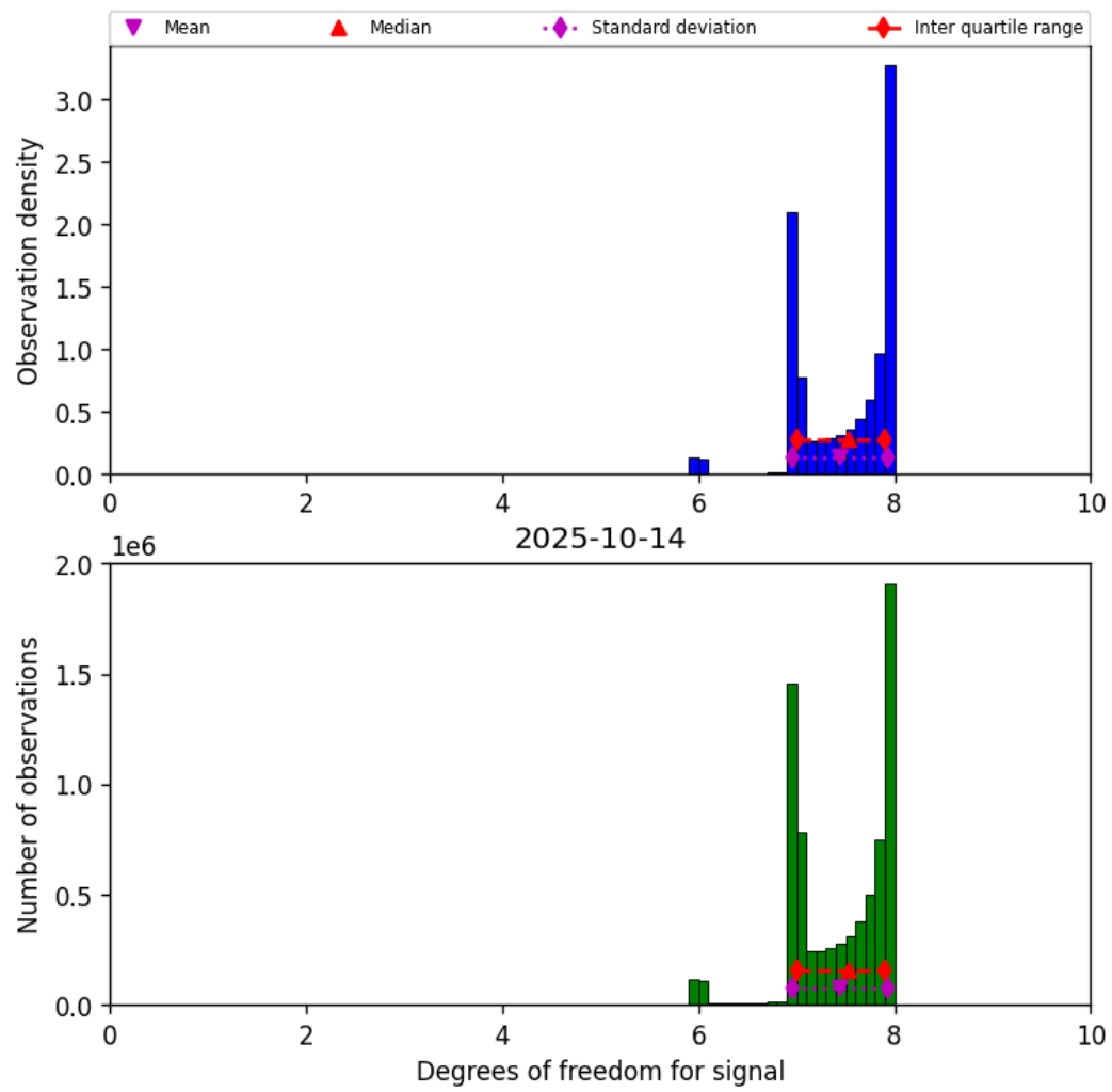
Figure 23: Histogram of “Degrees of freedom for signal” for 2025-10-13 to 2025-10-15
