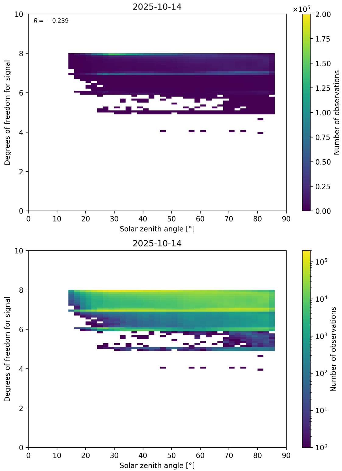
Figure 65: Scatter density plot of “Solar zenith angle” against “Degrees of freedom for signal” for 2025-10-13 to 2025-10-15.
