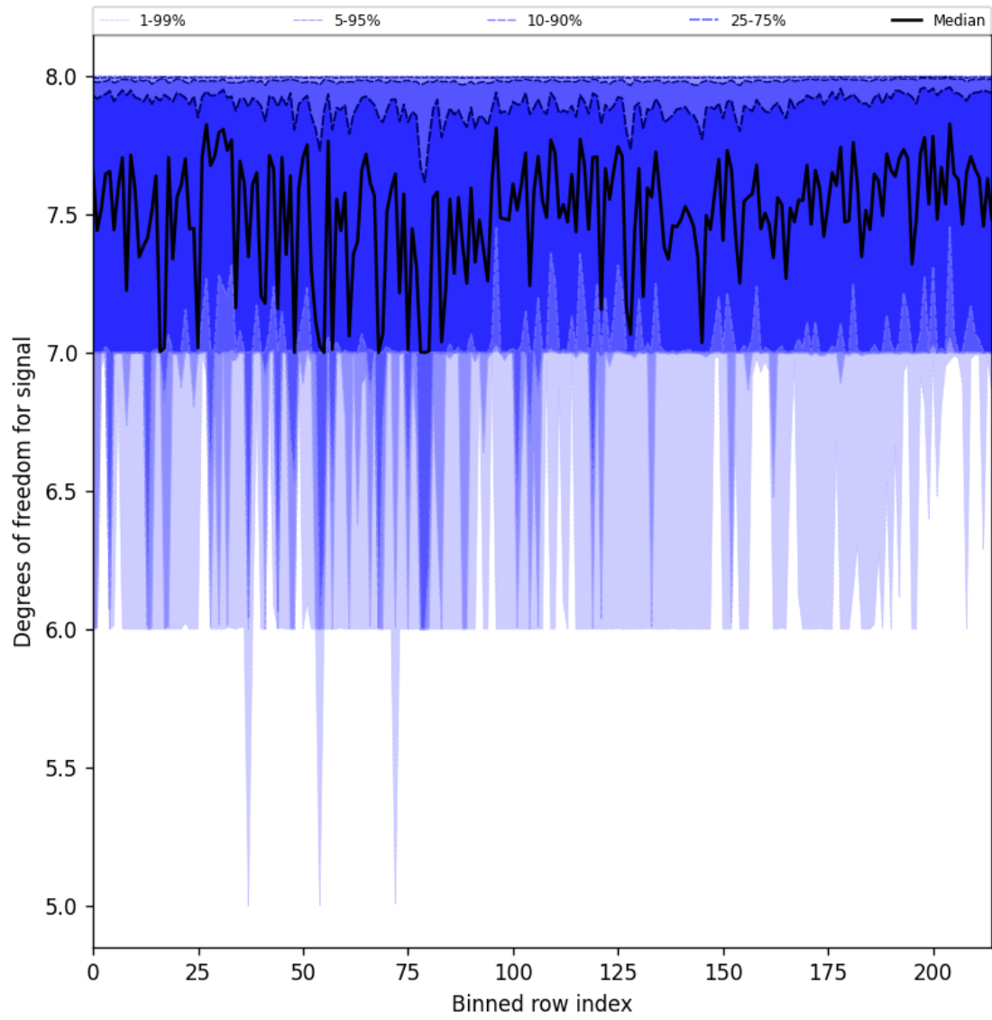
Figure 31: Along track statistics of “Degrees of freedom for signal” for 2025-10-13 to 2025-10-15
