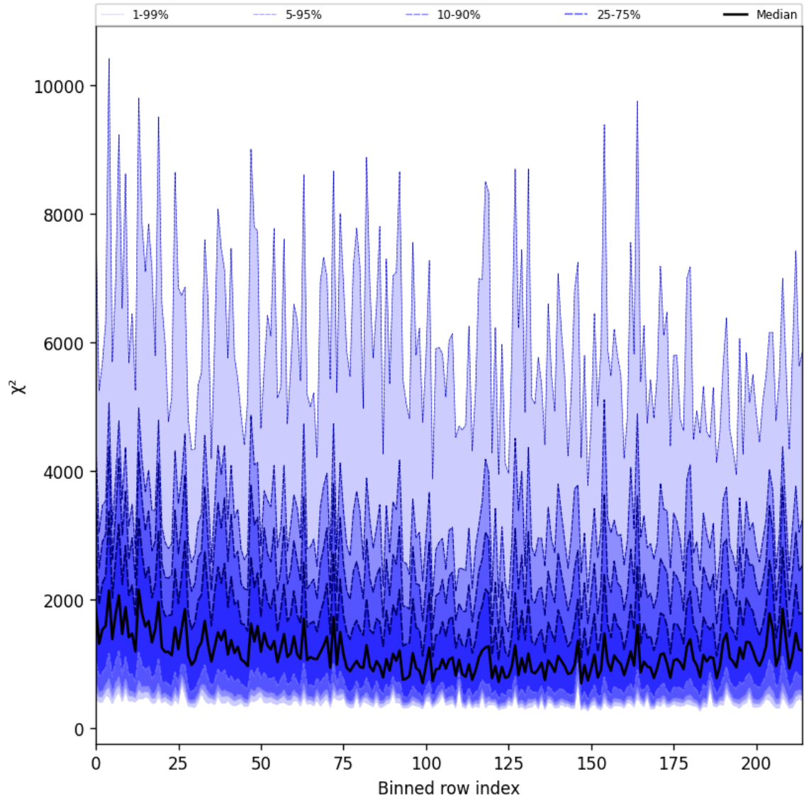
Figure 30: Along track statistics of “ \chi^2 ” for 2025-10-13 to 2025-10-15
