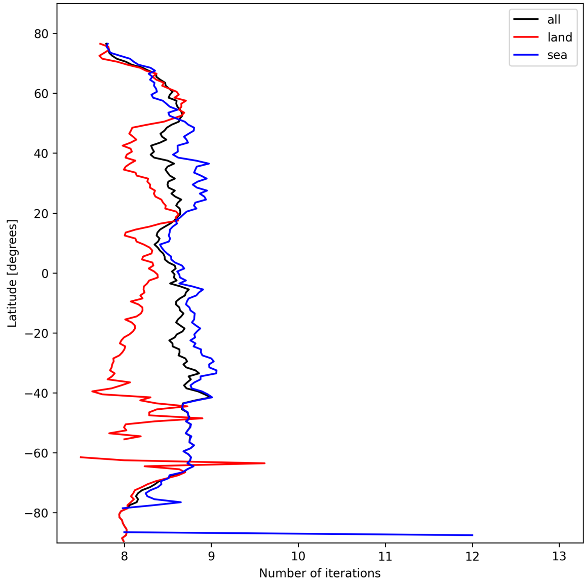
Figure 16: Zonal average of “Number of iterations” for 2025-10-13 to 2025-10-15.
