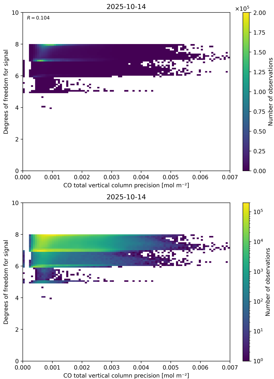
Figure 45: Scatter density plot of “CO total vertical column precision” against “Degrees of freedom for signal” for 2025-10-13 to 2025-10-15.
