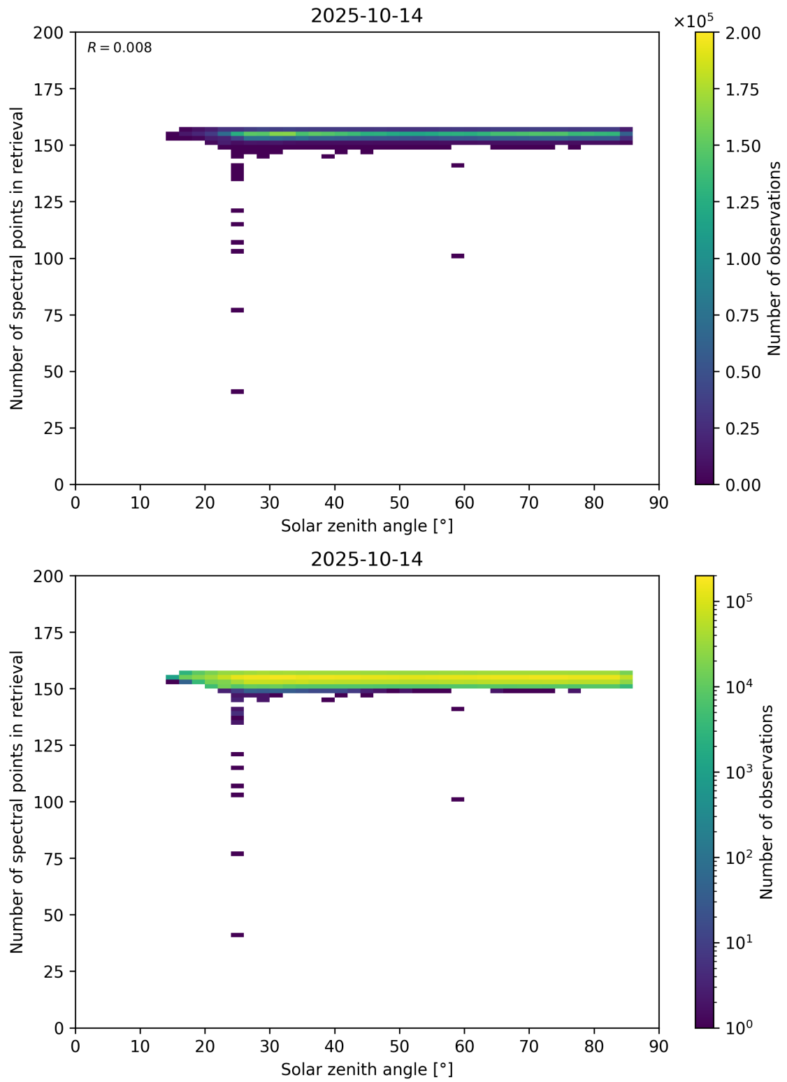
Figure 68: Scatter density plot of “Solar zenith angle” against “Number of spectral points in retrieval” for 2025-10-13 to 2025-10-15.
