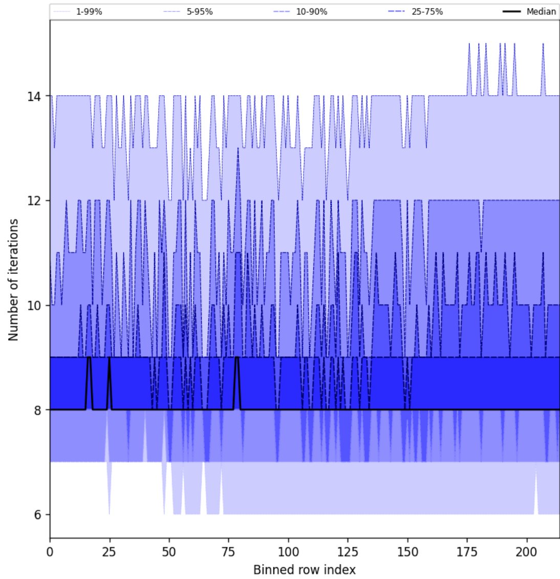
Figure 32: Along track statistics of “Number of iterations” for 2025-10-13 to 2025-10-15
