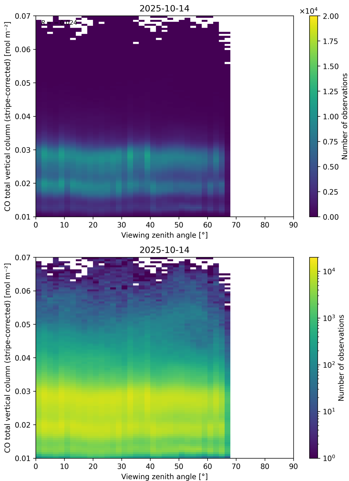
Figure 70: Scatter density plot of “Viewing zenith angle” against “CO total vertical column (stripe-corrected)” for 2025-10-13 to 2025-10-15.
