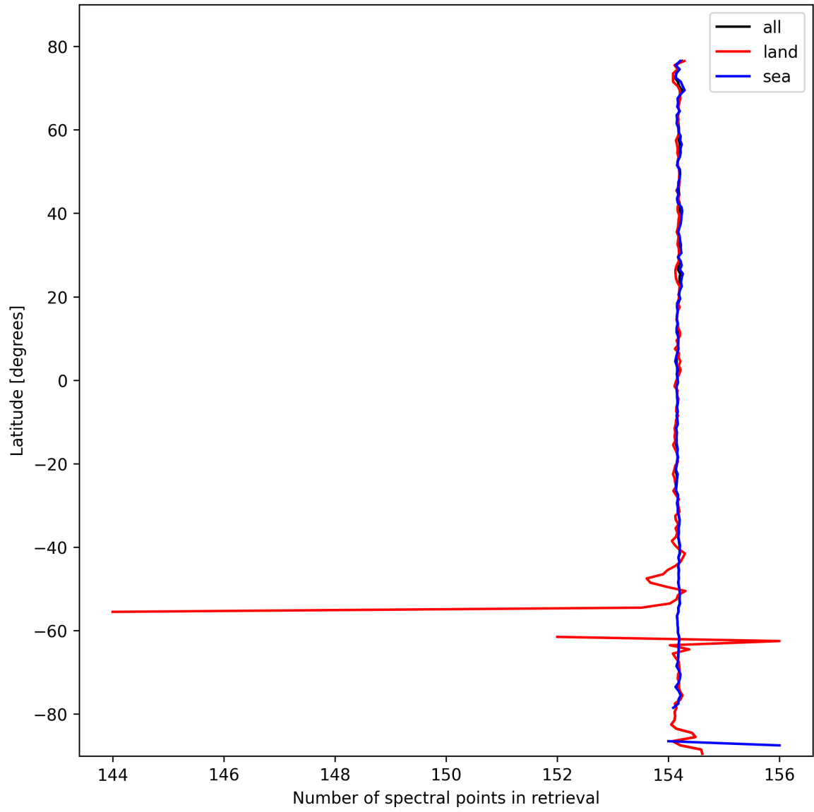
Figure 13: Zonal average of “Number of spectral points in retrieval” for 2025-10-13 to 2025-10-15.
