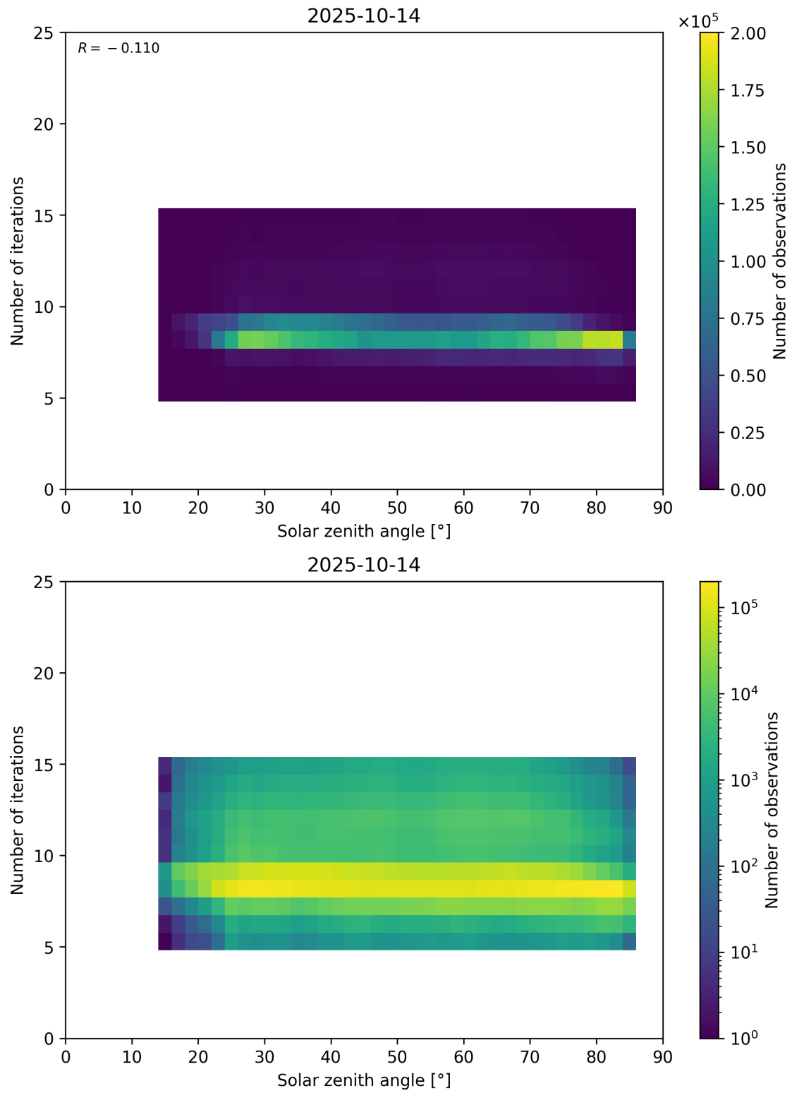
Figure 67: Scatter density plot of “Solar zenith angle” against “Number of iterations” for 2025-10-13 to 2025-10-15.
