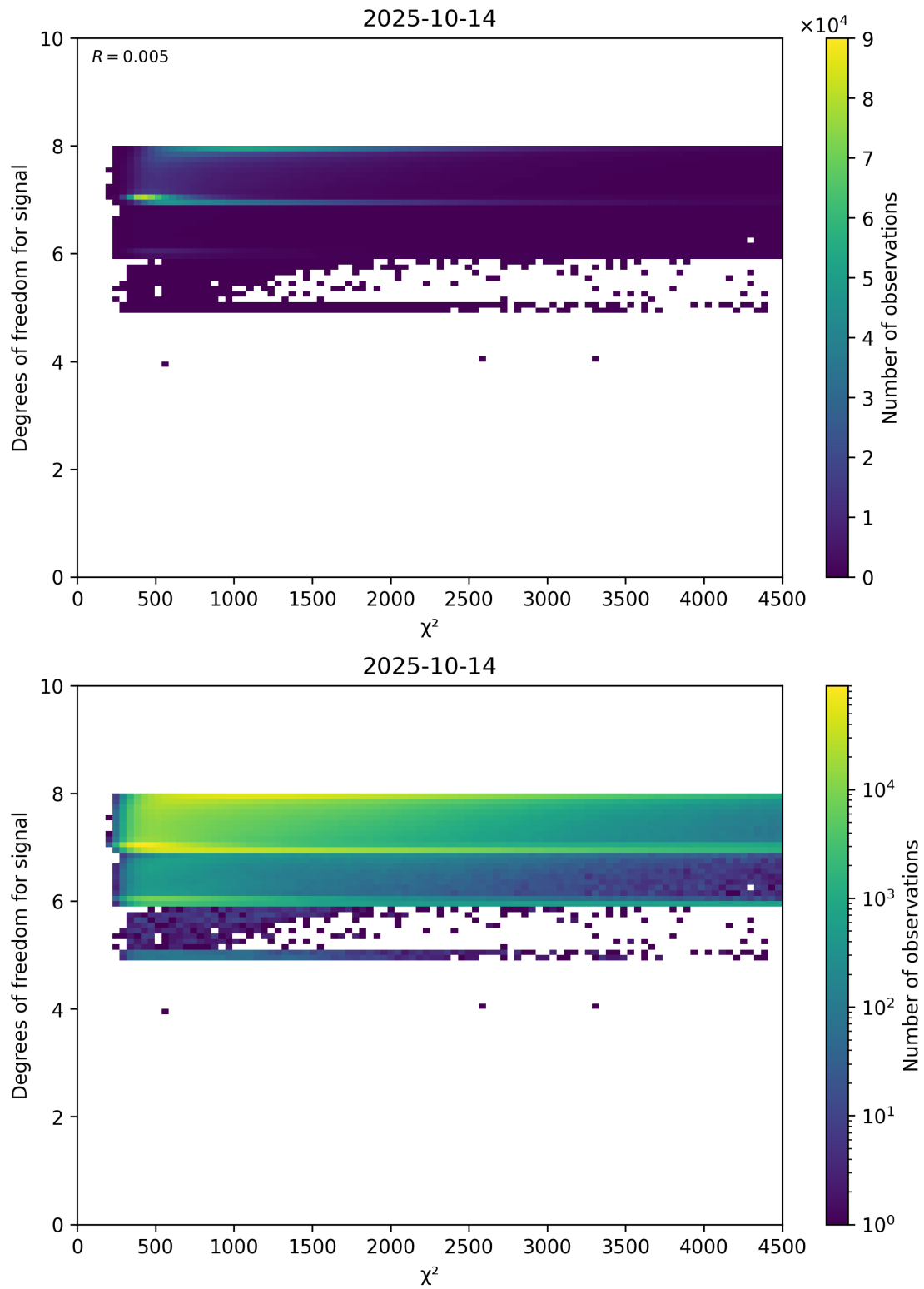
Figure 48: Scatter density plot of “ \chi^2 ” against “Degrees of freedom for signal” for 2025-10-13 to 2025-10-15.
