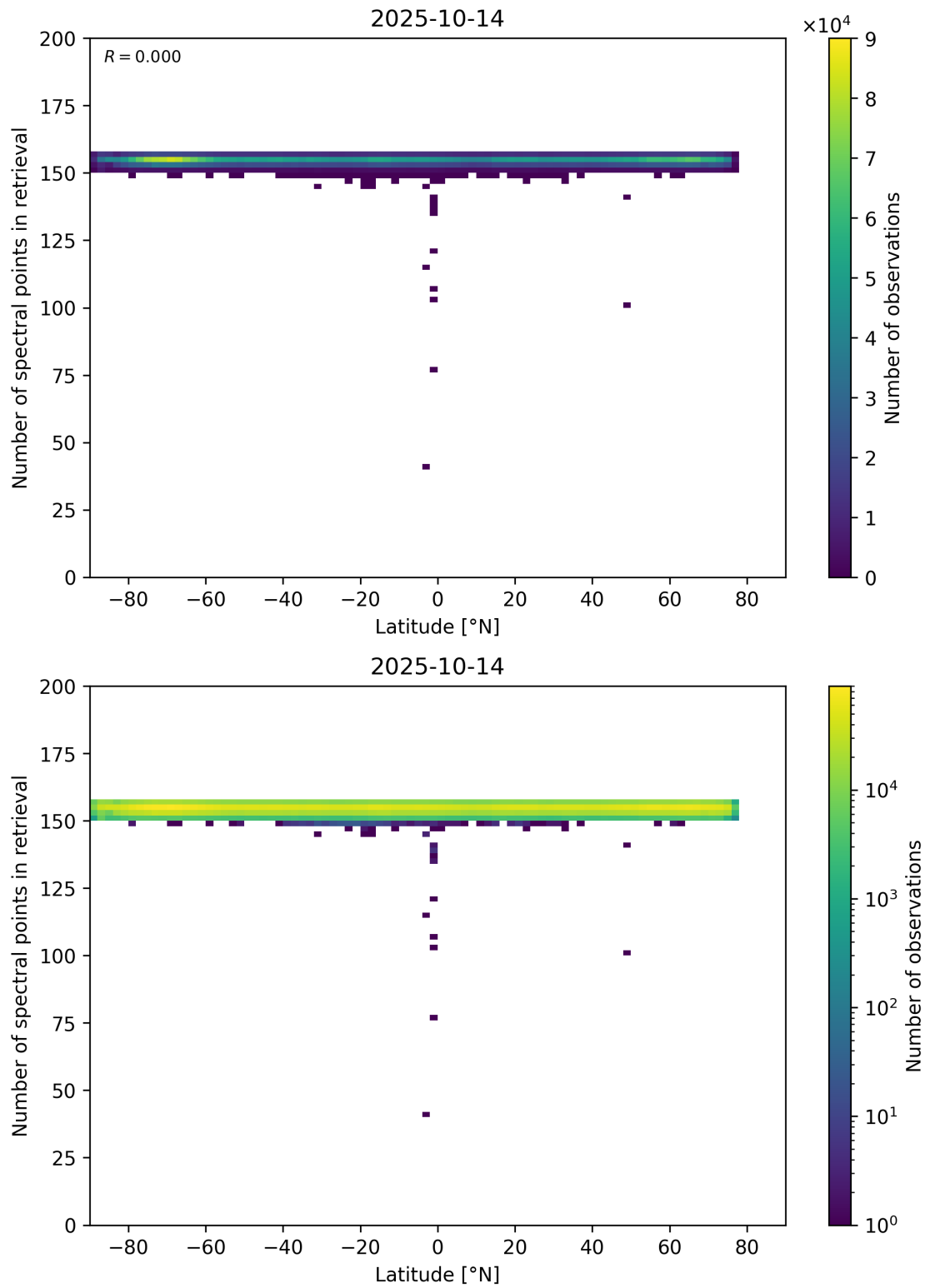
Figure 57: Scatter density plot of “Latitude” against “Number of spectral points in retrieval” for 2025-10-13 to 2025-10-15.
