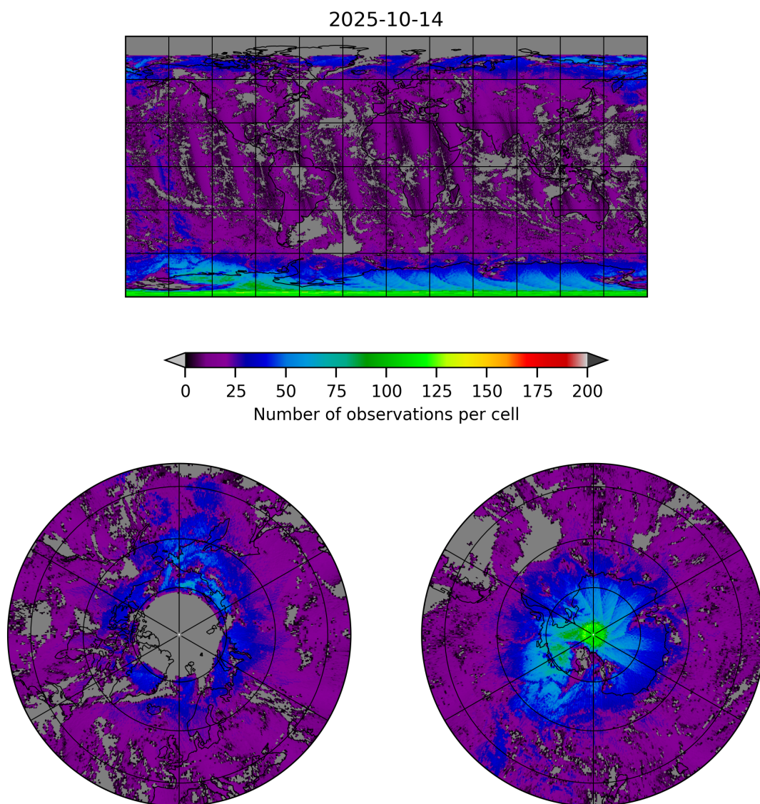
Figure 8: Map of the number of observations for 2025-10-13 to 2025-10-15
