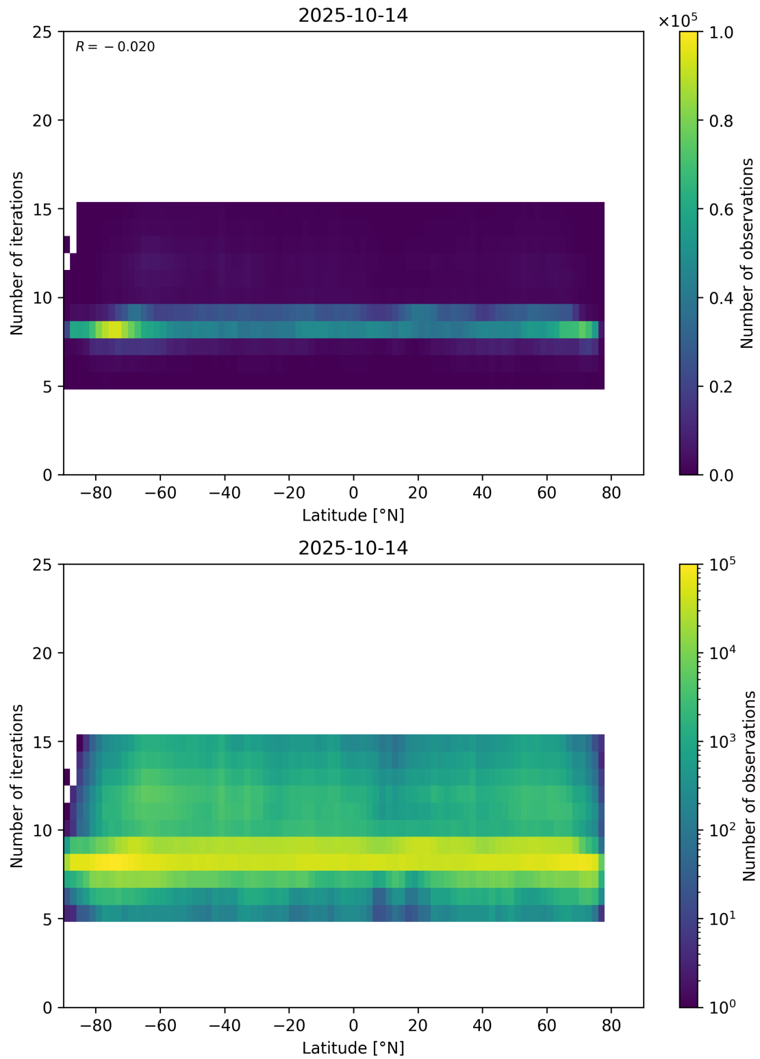
Figure 56: Scatter density plot of “Latitude” against “Number of iterations” for 2025-10-13 to 2025-10-15.
