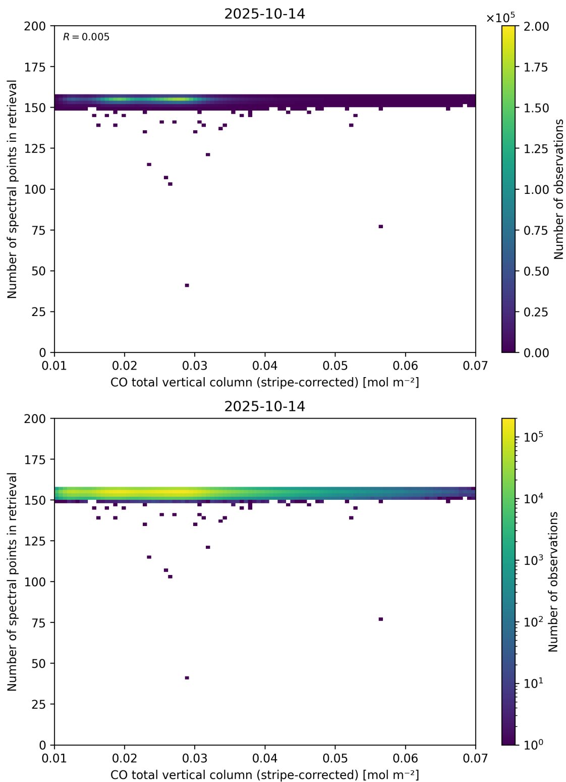
Figure 40: Scatter density plot of “CO total vertical column (stripe-corrected)” against “Number of spectral points in retrieval” for 2025-10-13 to 2025-10-15.
