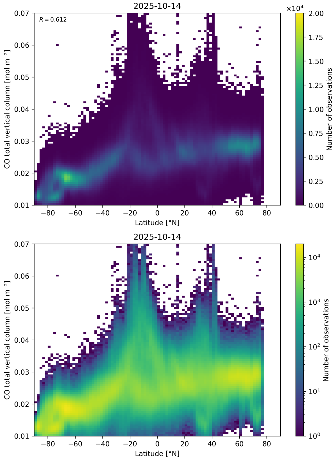
Figure 51: Scatter density plot of “Latitude” against “CO total vertical column” for 2025-10-13 to 2025-10-15.
