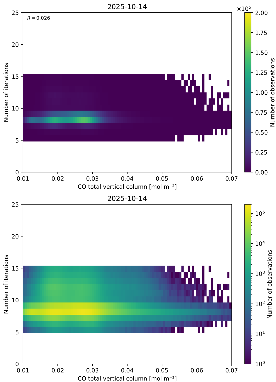
Figure 42: Scatter density plot of “CO total vertical column” against “Number of iterations” for 2025-10-13 to 2025-10-15.
