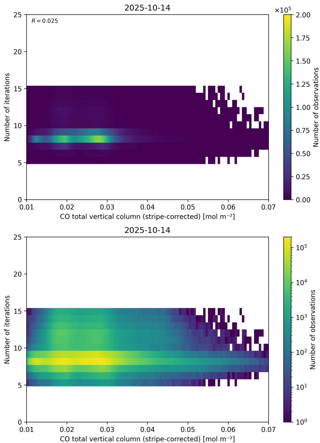
Figure 39: Scatter density plot of “CO total vertical column (stripe-corrected)” against “Number of iterations” for 2025-10-13 to 2025-10-15.
