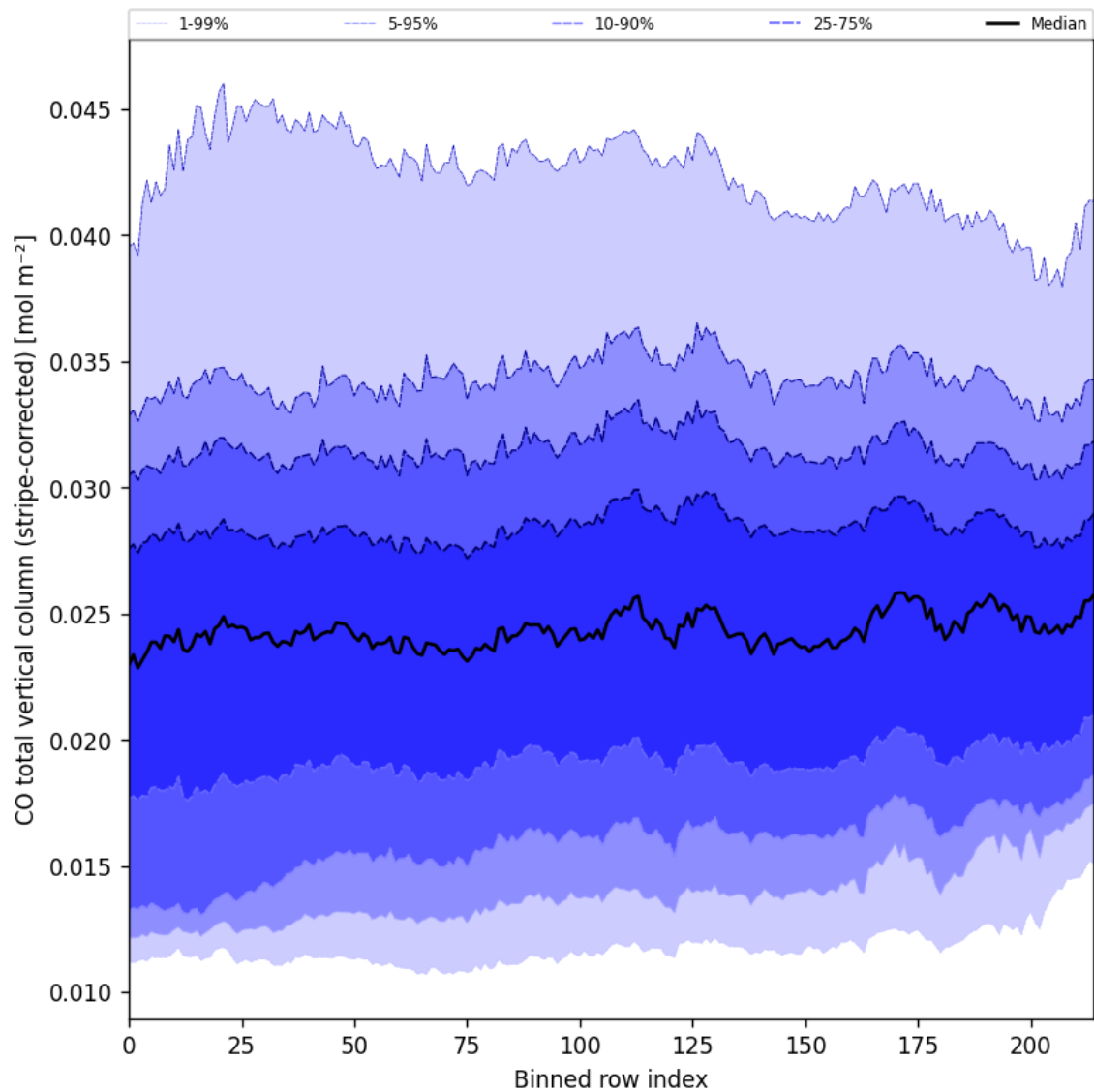
Figure 27: Along track statistics of "CO total vertical column (stripe-corrected)" for 2025-10-13 to 2025-10-15
