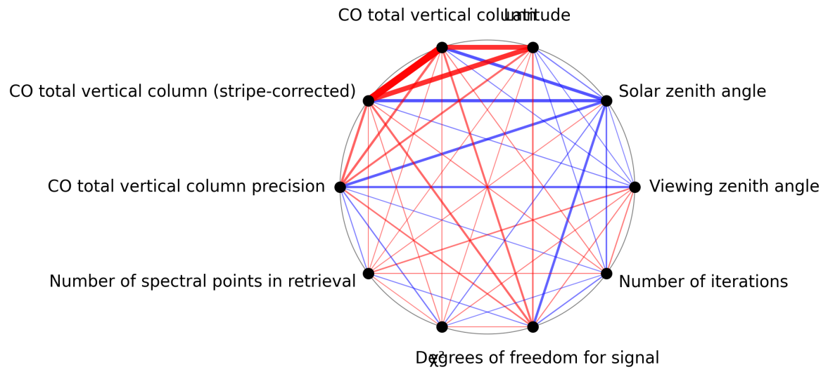
Figure 1: Map of correlation graph for 2025-10-13 to 2025-10-15.
