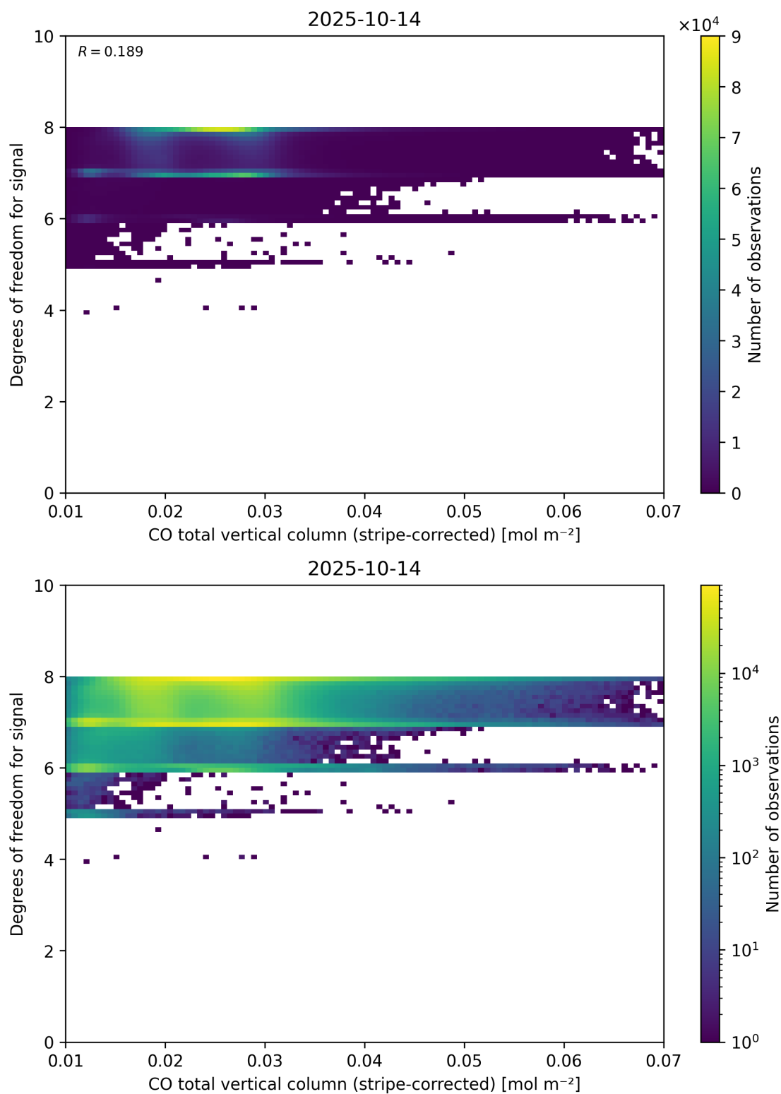
Figure 38: Scatter density plot of “CO total vertical column (stripe-corrected)” against “Degrees of freedom for signal” for 2025-10-13 to 2025-10-15.
