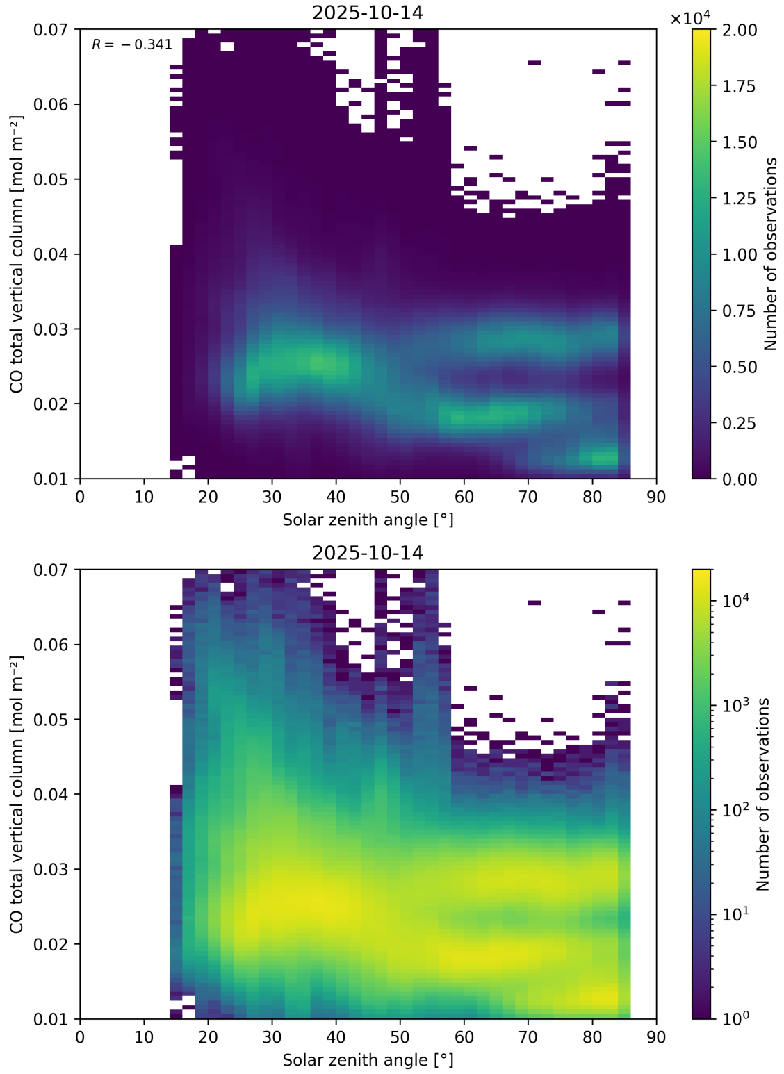
Figure 61: Scatter density plot of “Solar zenith angle” against “CO total vertical column” for 2025-10-13 to 2025-10-15.
