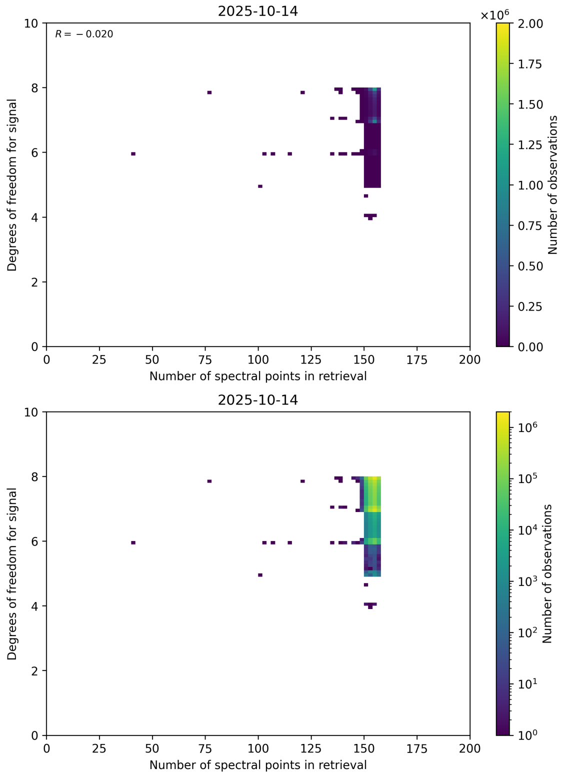
Figure 59: Scatter density plot of “Number of spectral points in retrieval” against “Degrees of freedom for signal” for 2025-10-13 to 2025-10-15.
