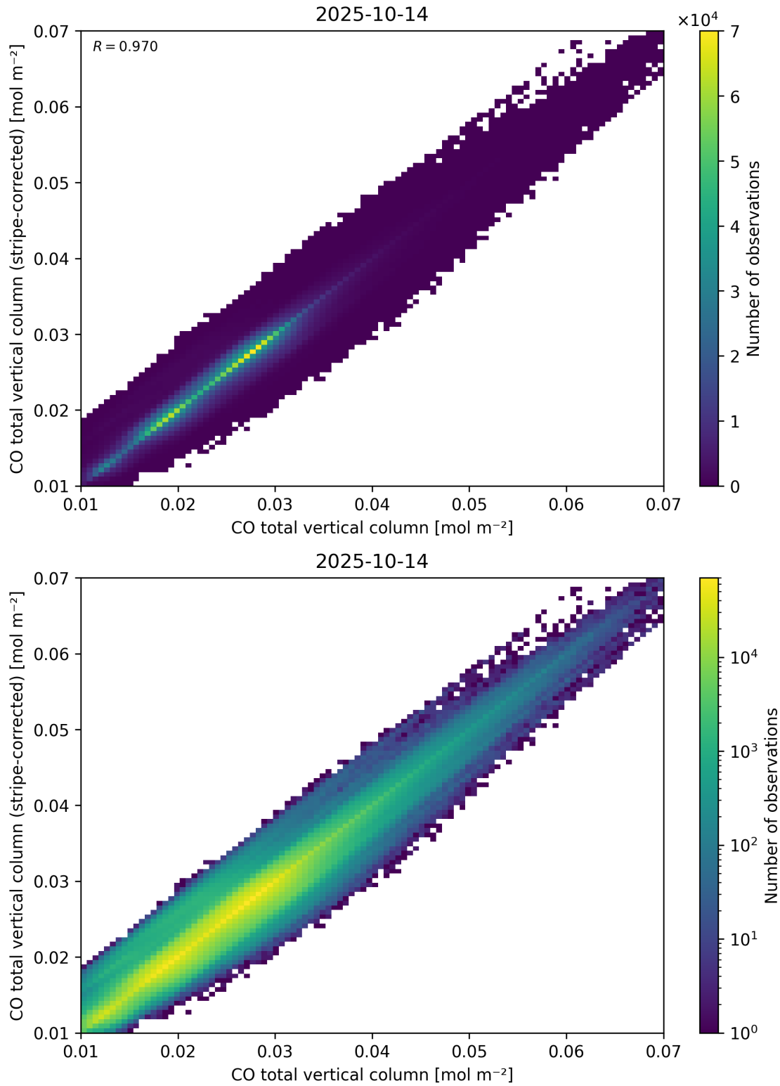
Figure 33: Scatter density plot of “CO total vertical column” against “CO total vertical column (stripe-corrected)” for 2025-10-13 to 2025-10-15.
