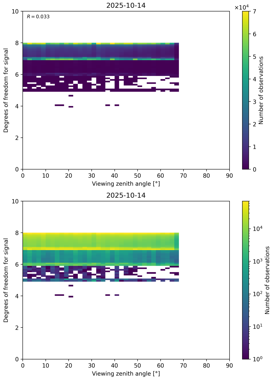
Figure 73: Scatter density plot of “Viewing zenith angle” against “Degrees of freedom for signal” for 2025-10-13 to 2025-10-15.
