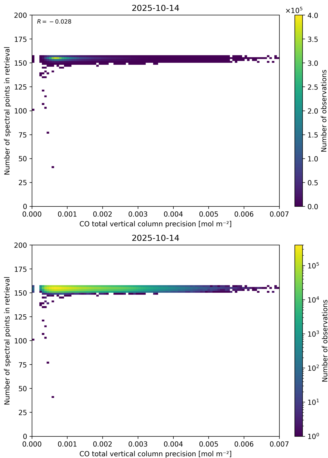
Figure 47: Scatter density plot of “CO total vertical column precision” against “Number of spectral points in retrieval” for 2025-10-13 to 2025-10-15.
