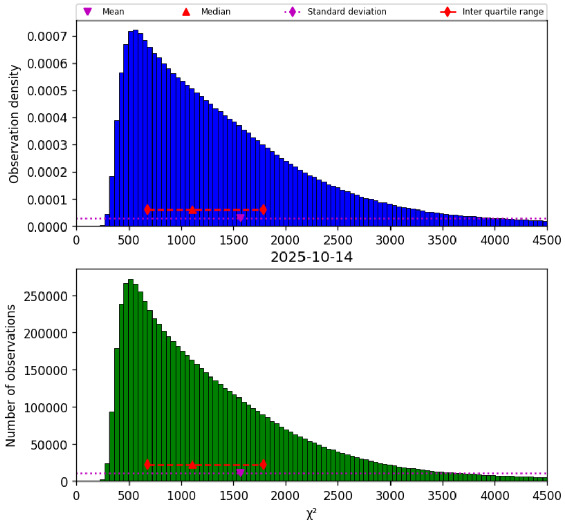
Figure 22: Histogram of “ \chi^2 ” for 2025-10-13 to 2025-10-15
