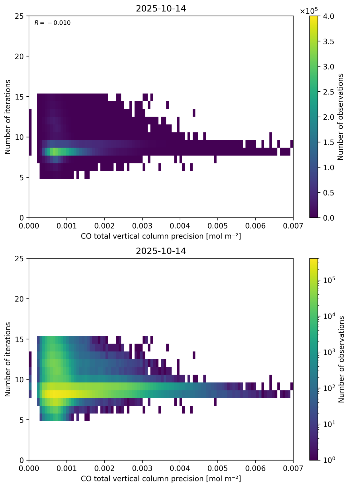
Figure 46: Scatter density plot of “CO total vertical column precision” against “Number of iterations” for 2025-10-13 to 2025-10-15.
