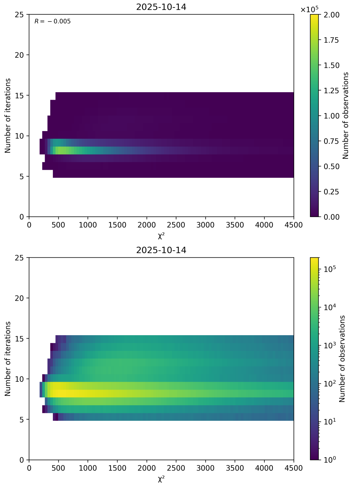
Figure 49: Scatter density plot of “ \chi^2 ” against “Number of iterations” for 2025-10-13 to 2025-10-15.
