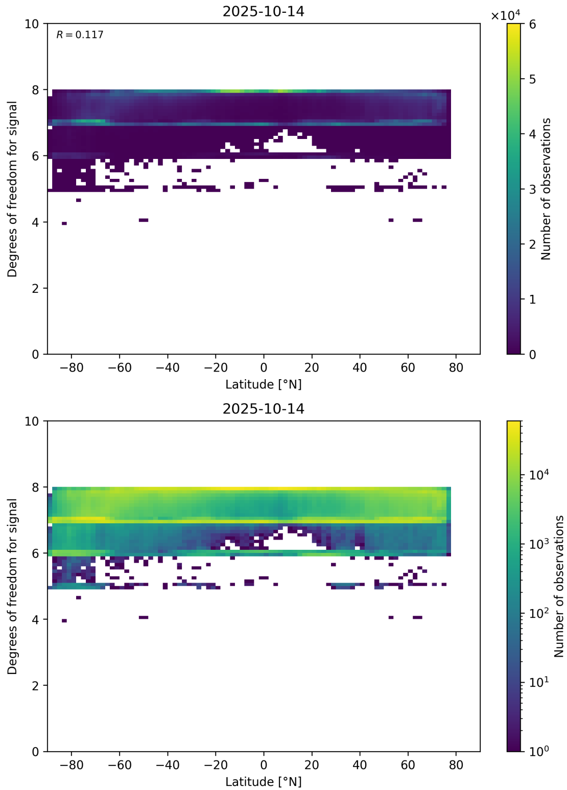
Figure 55: Scatter density plot of “Latitude” against “Degrees of freedom for signal” for 2025-10-13 to 2025-10-15.
