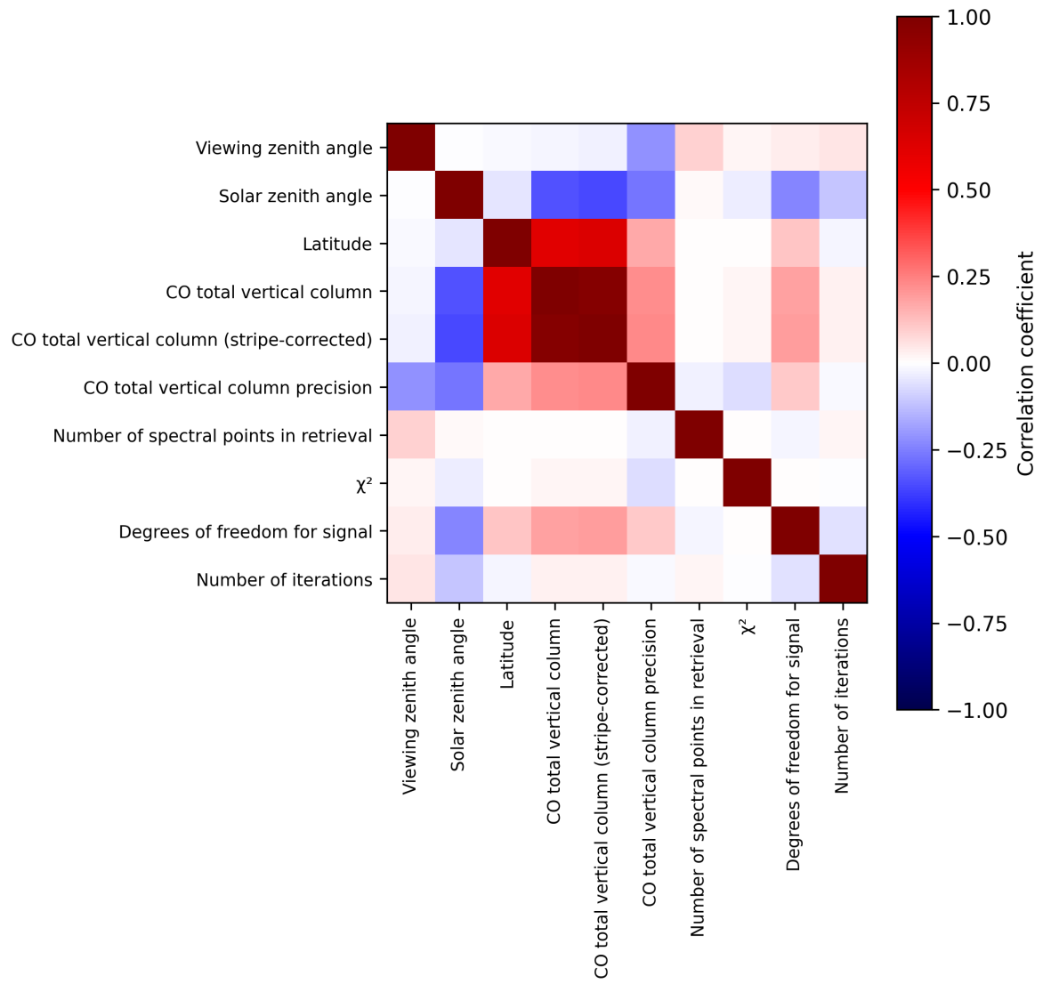
Figure 2: Map of correlation matrix for 2025-10-13 to 2025-10-15.
