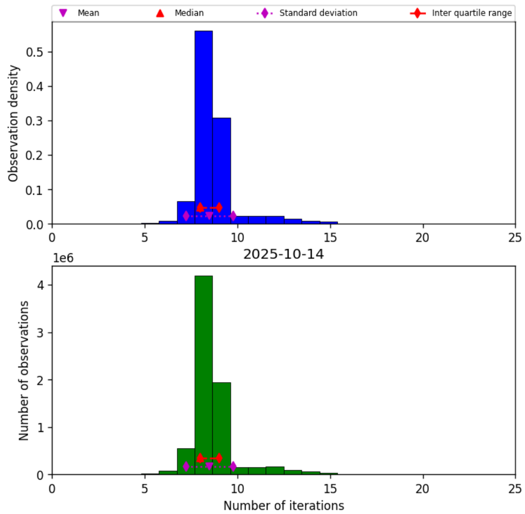
Figure 24: Histogram of “Number of iterations” for 2025-10-13 to 2025-10-15
