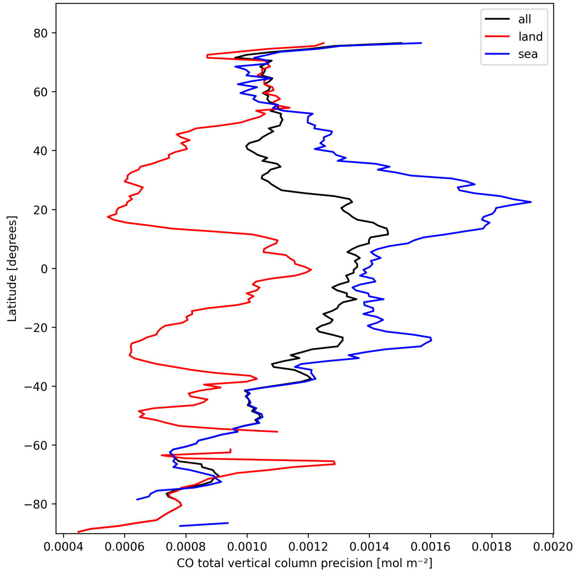
Figure 12: Zonal average of “CO total vertical column precision” for 2025-10-13 to 2025-10-15.
