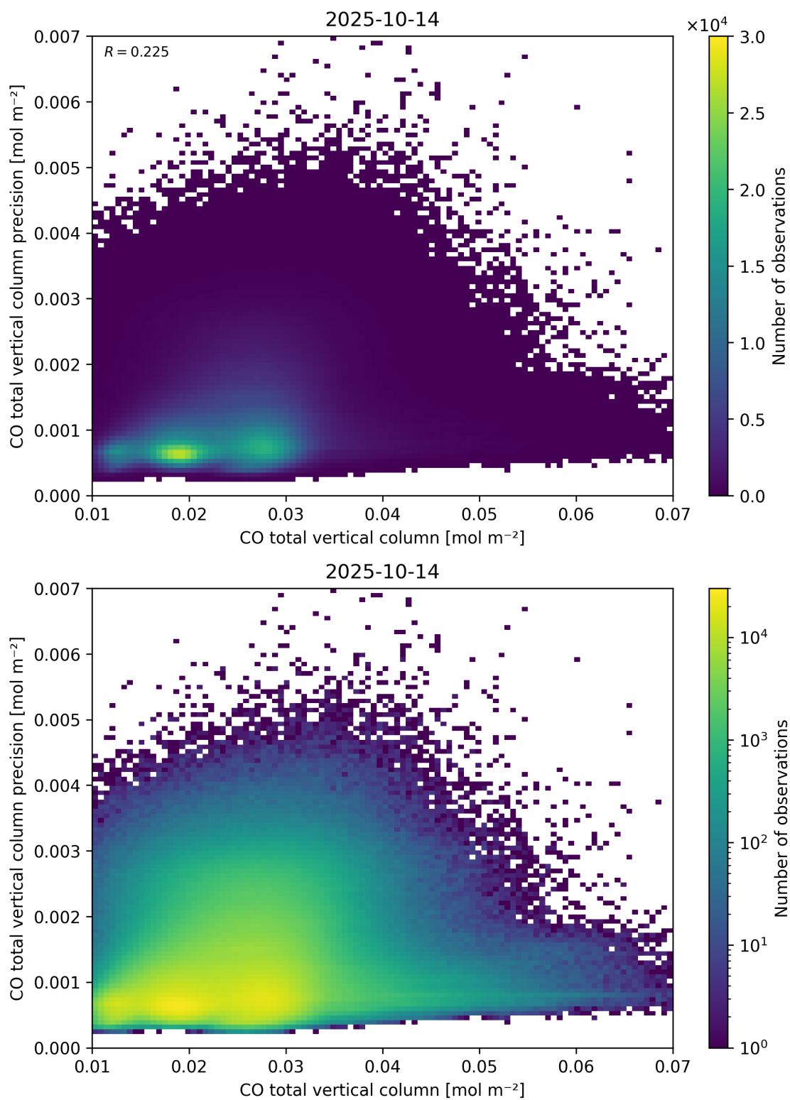
Figure 34: Scatter density plot of “CO total vertical column” against “CO total vertical column precision” for 2025-10-13 to 2025-10-15.
