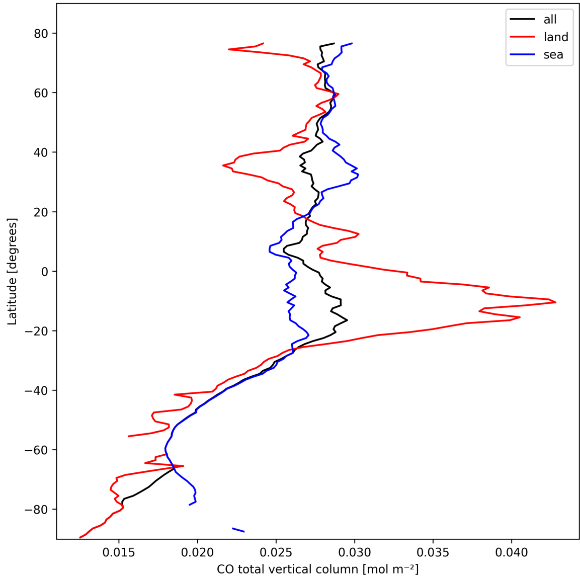
Figure 10: Zonal average of “CO total vertical column” for 2025-10-13 to 2025-10-15.
