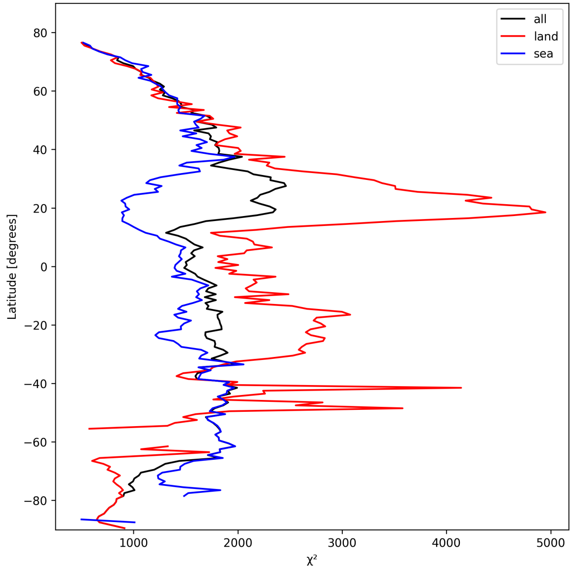
Figure 14: Zonal average of “ \chi^2 ” for 2025-10-13 to 2025-10-15.
