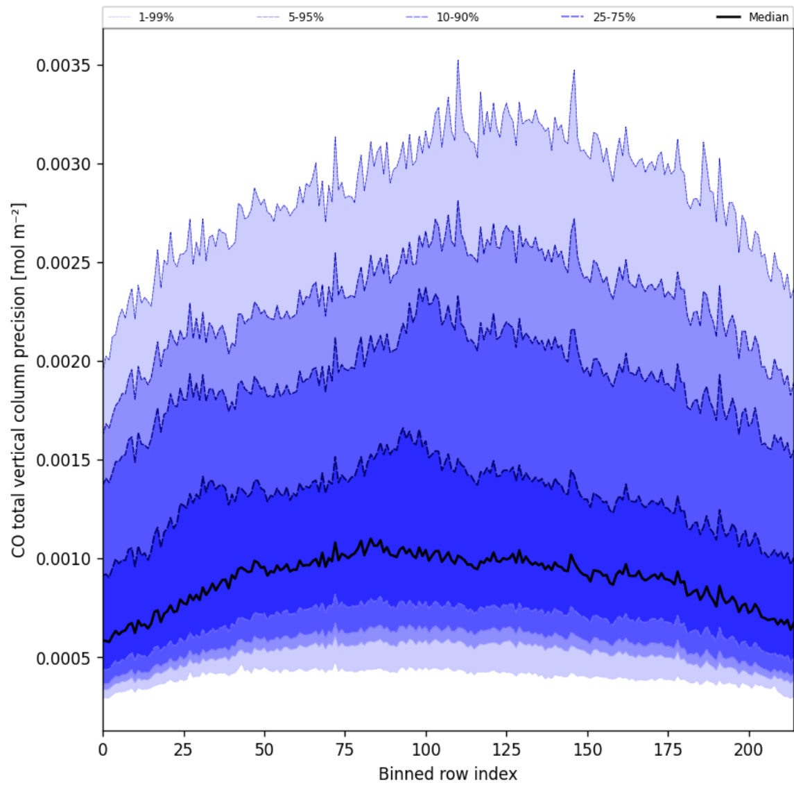
Figure 28: Along track statistics of “CO total vertical column precision” for 2025-10-13 to 2025-10-15
