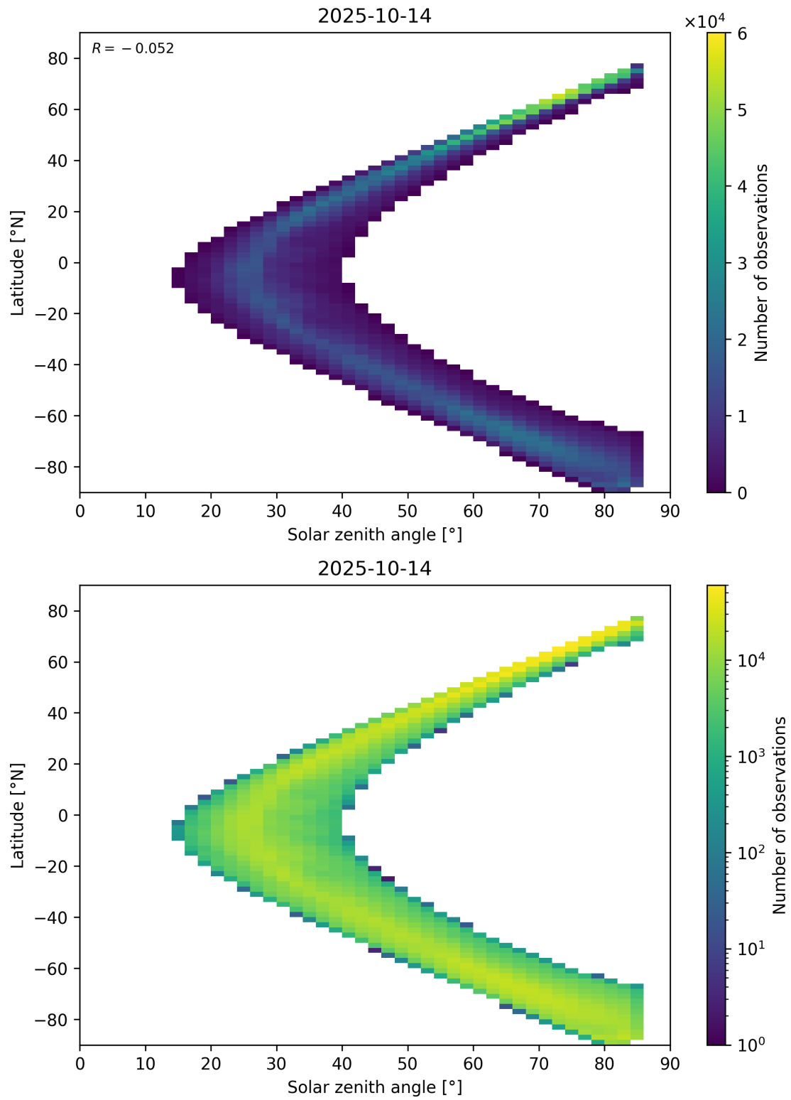
Figure 66: Scatter density plot of “Solar zenith angle” against “Latitude” for 2025-10-13 to 2025-10-15.
