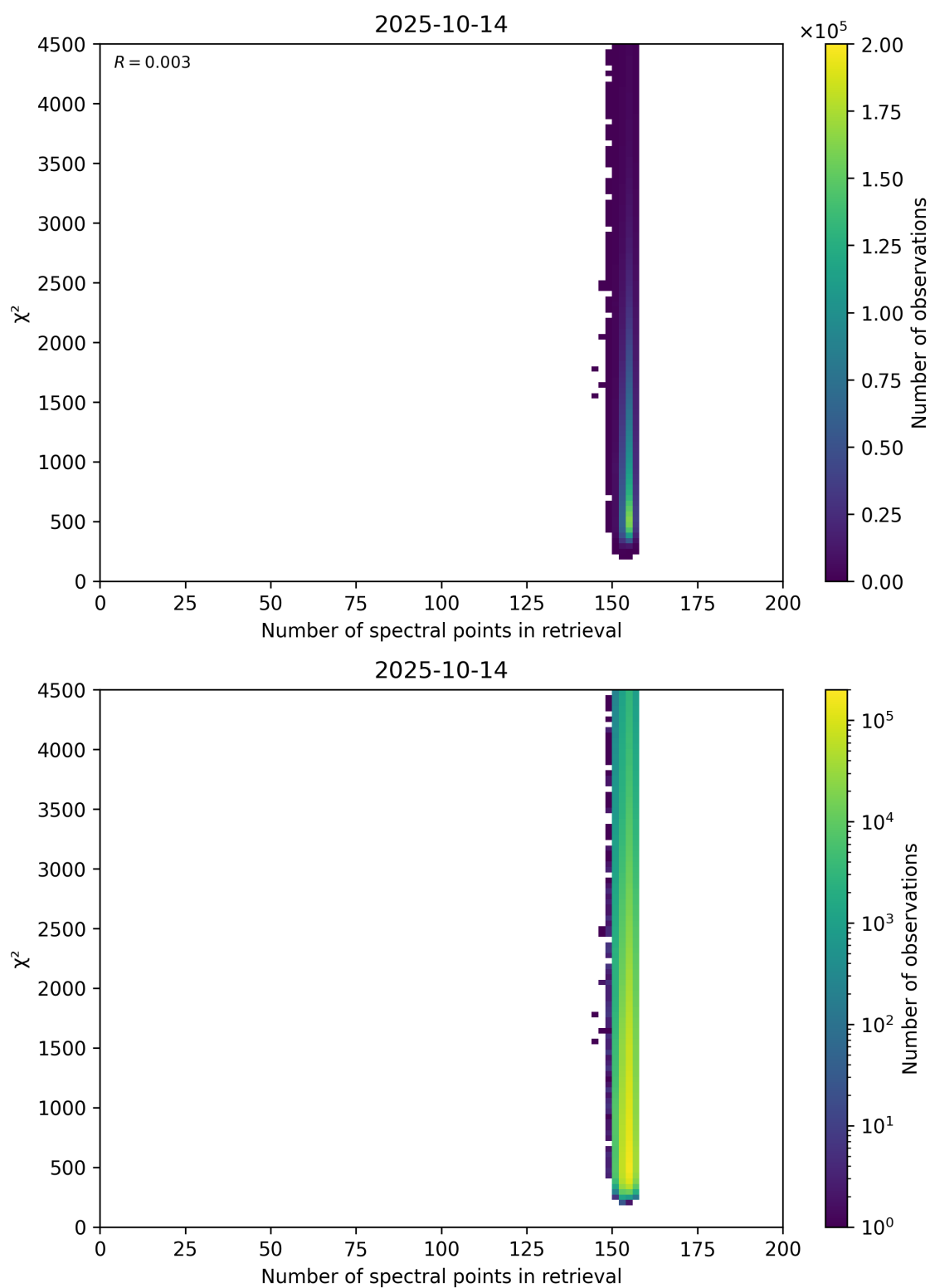
Figure 58: Scatter density plot of “Number of spectral points in retrieval” against “ \chi^2 ” for 2025-10-13 to 2025-10-15.
