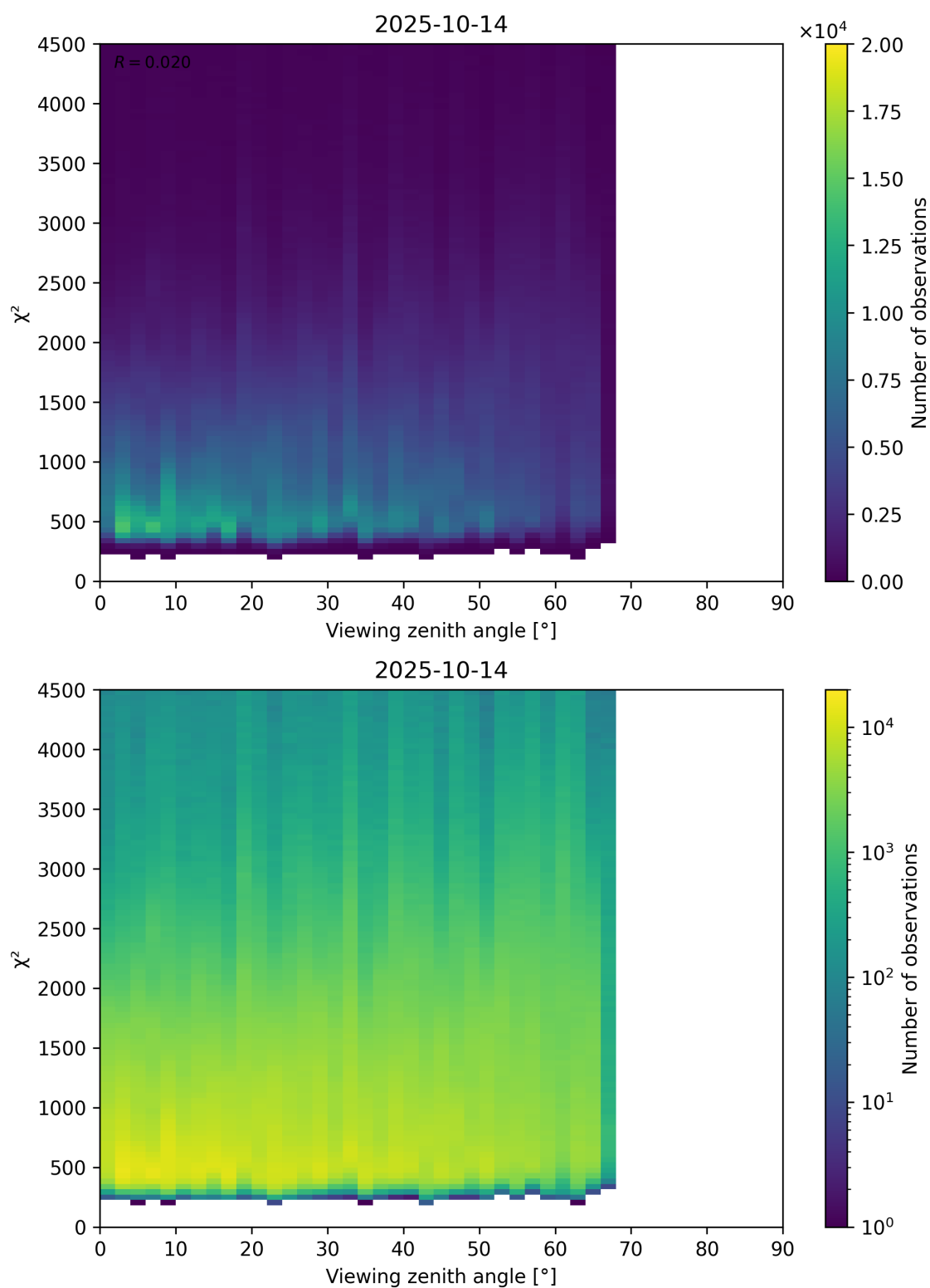
Figure 72: Scatter density plot of “Viewing zenith angle” against “ \chi^2 ” for 2025-10-13 to 2025-10-15.
