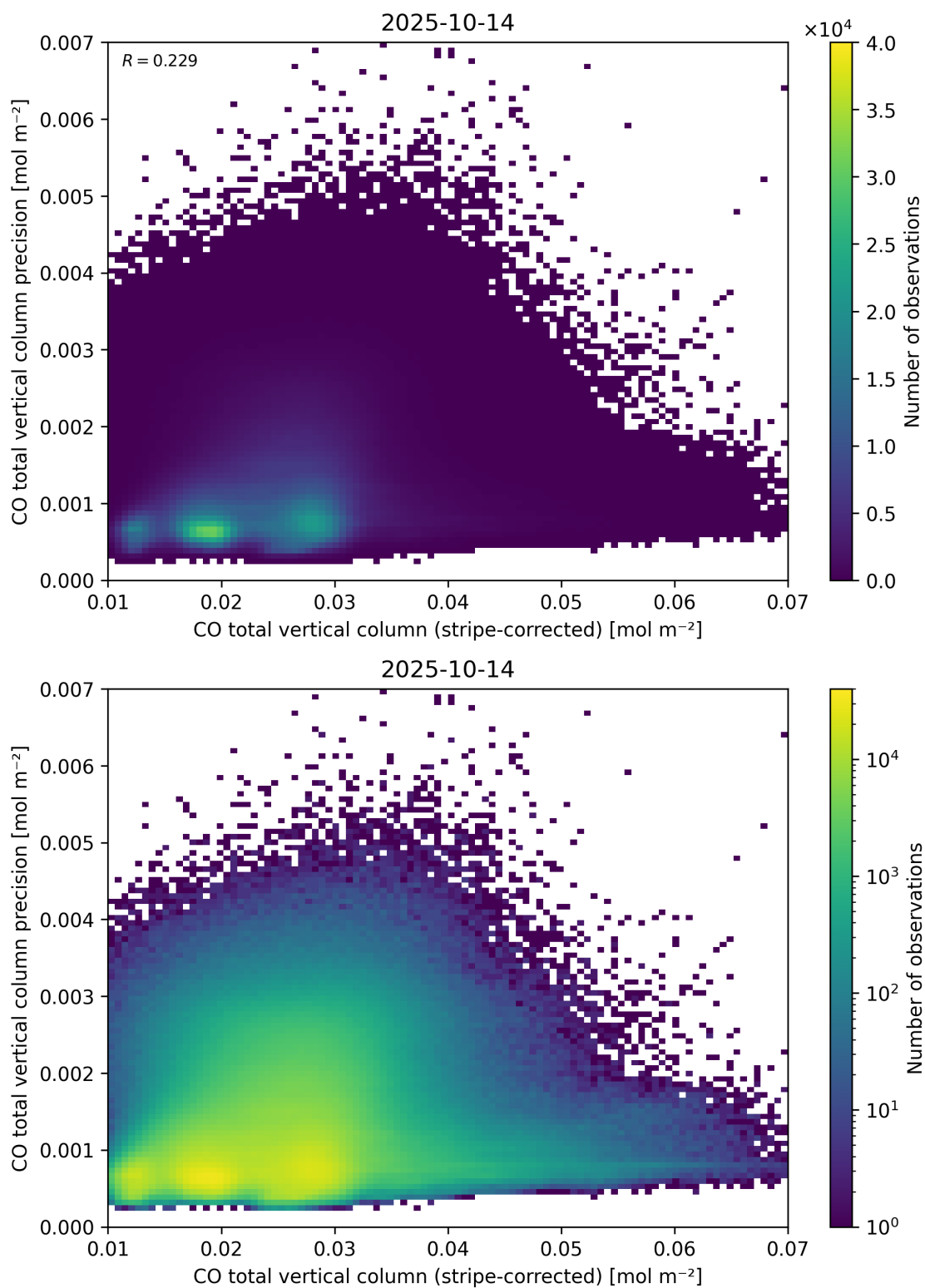
Figure 36: Scatter density plot of “CO total vertical column (stripe-corrected)” against “CO total vertical column precision” for 2025-10-13 to 2025-10-15.
