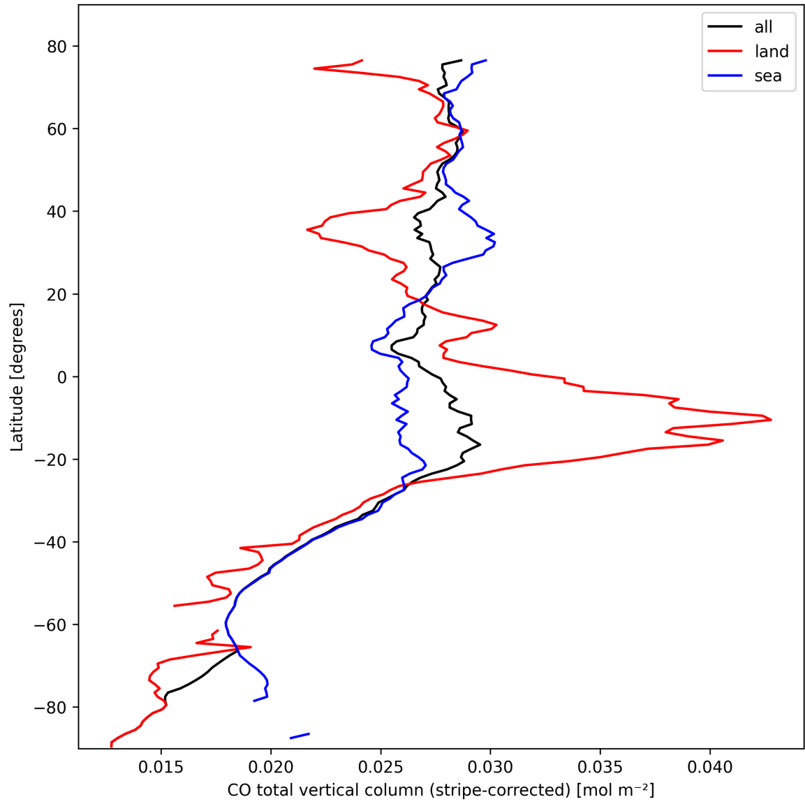
Figure 11: Zonal average of “CO total vertical column (stripe-corrected)” for 2025-10-13 to 2025-10-15.
