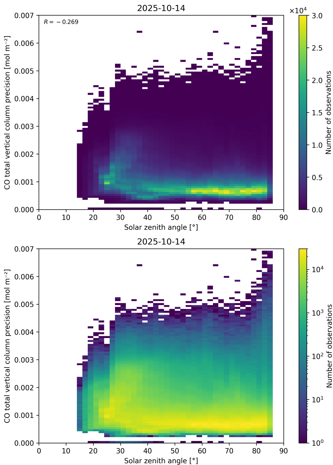
Figure 63: Scatter density plot of “Solar zenith angle” against “CO total vertical column precision” for 2025-10-13 to 2025-10-15.
