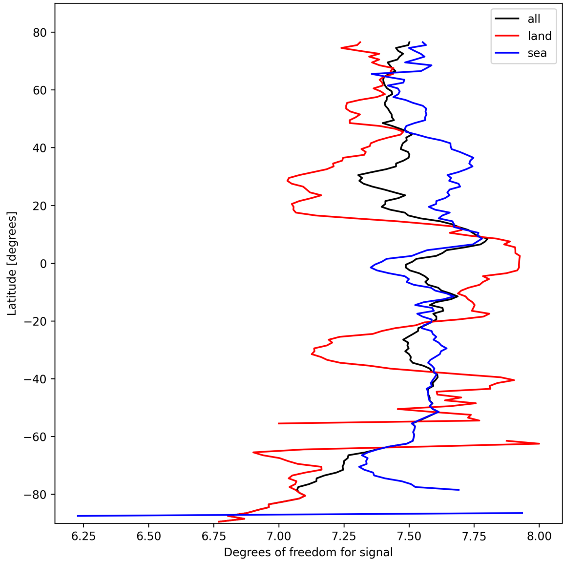
Figure 15: Zonal average of “Degrees of freedom for signal” for 2025-10-13 to 2025-10-15.
