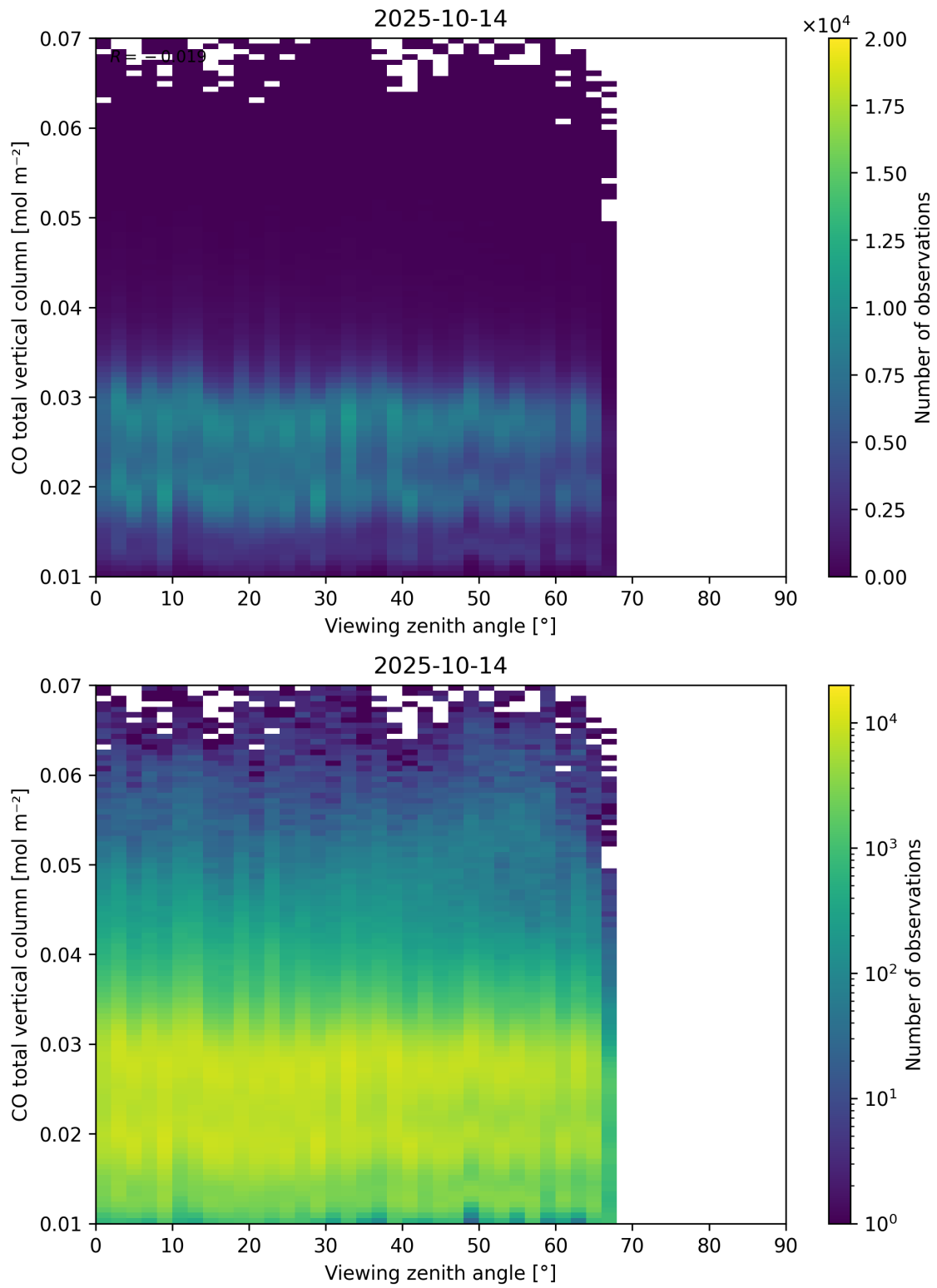
Figure 69: Scatter density plot of “Viewing zenith angle” against “CO total vertical column” for 2025-10-13 to 2025-10-15.
