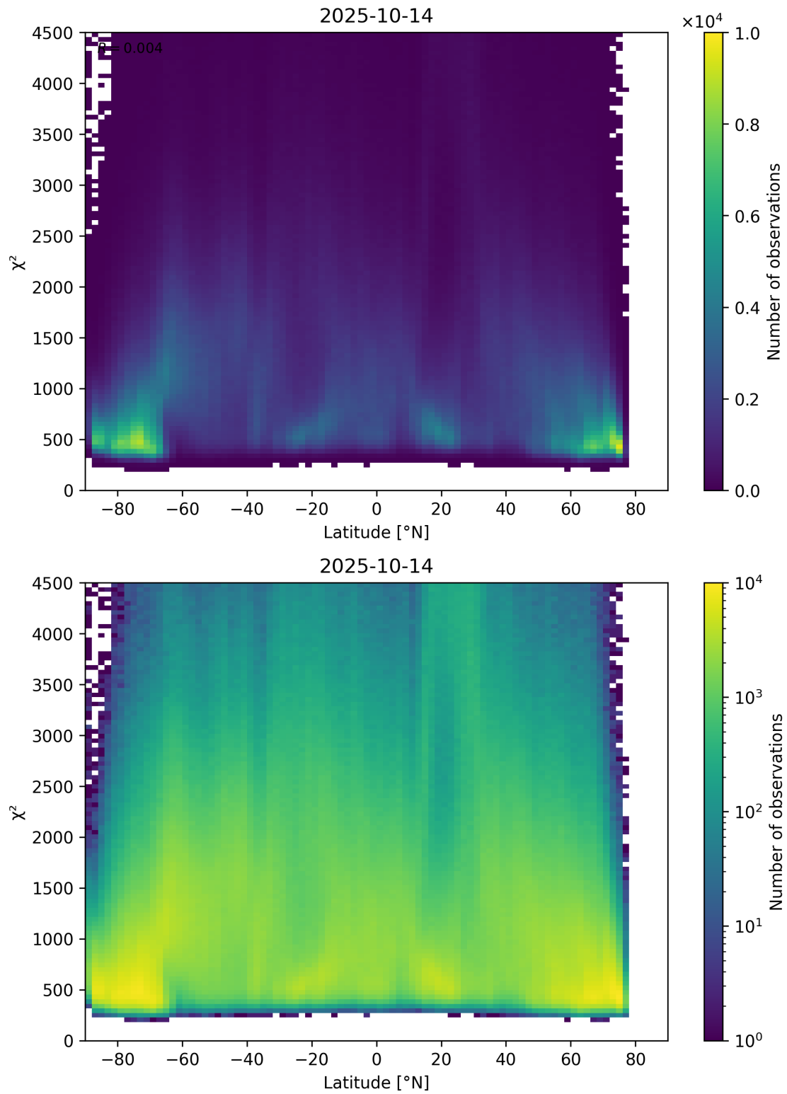
Figure 54: Scatter density plot of “Latitude” against “ \chi^2 ” for 2025-10-13 to 2025-10-15.
