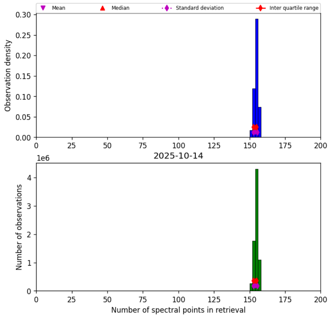
Figure 21: Histogram of “Number of spectral points in retrieval” for 2025-10-13 to 2025-10-15
