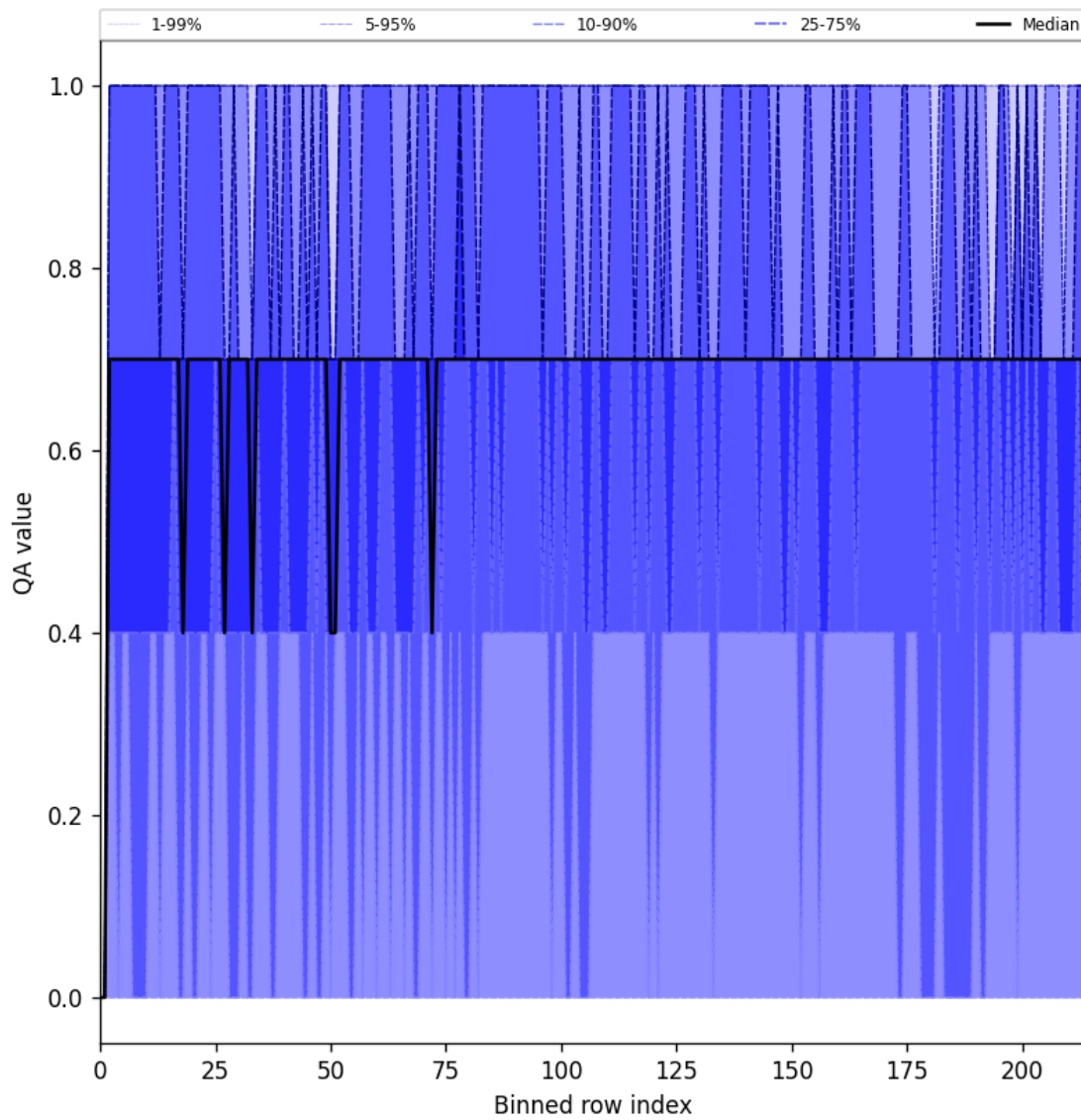
Figure 25: Along track statistics of “QA value” for 2025-10-13 to 2025-10-15
