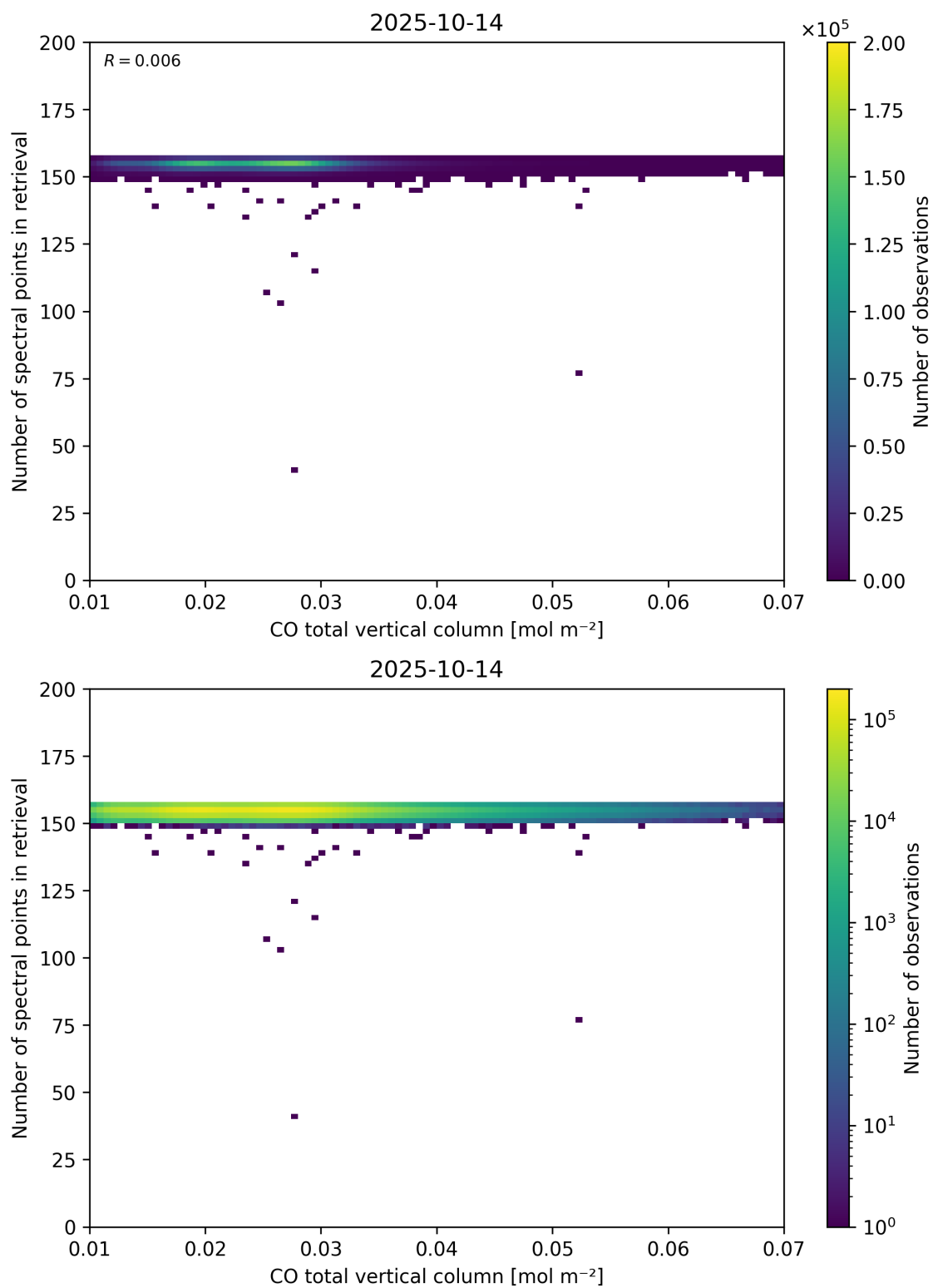
Figure 43: Scatter density plot of “CO total vertical column” against “Number of spectral points in retrieval” for 2025-10-13 to 2025-10-15.
