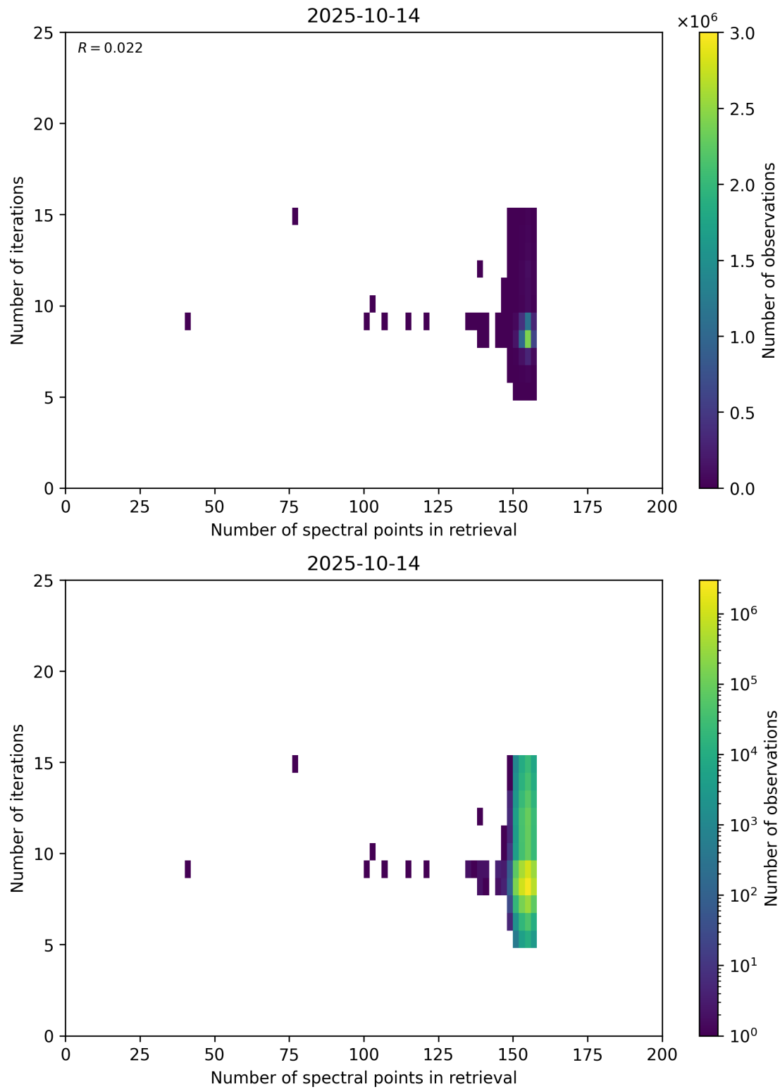
Figure 60: Scatter density plot of “Number of spectral points in retrieval” against “Number of iterations” for 2025-10-13 to 2025-10-15.
