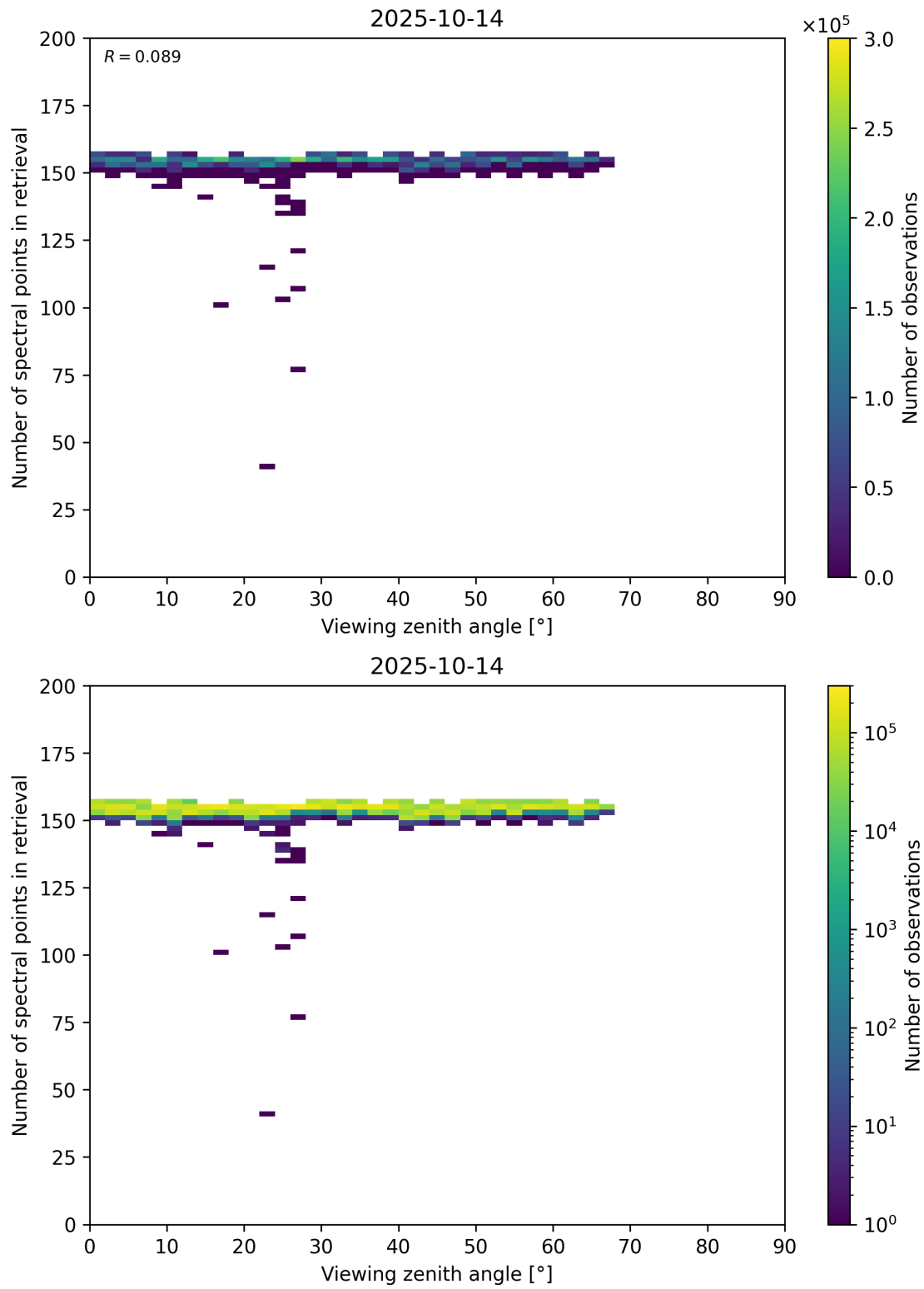
Figure 76: Scatter density plot of “Viewing zenith angle” against “Number of spectral points in retrieval” for 2025-10-13 to 2025-10-15.
