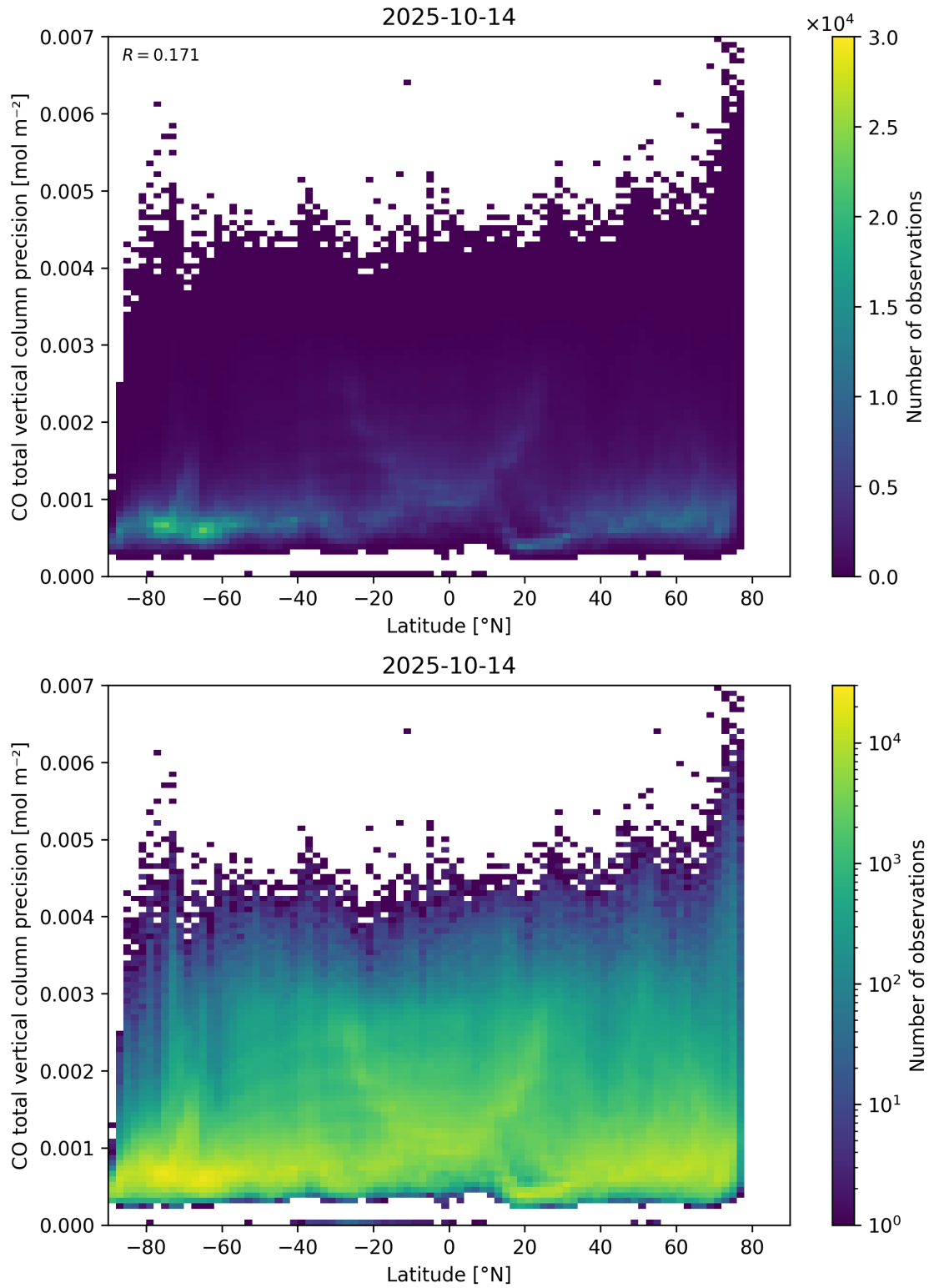
Figure 53: Scatter density plot of “Latitude” against “CO total vertical column precision” for 2025-10-13 to 2025-10-15.
