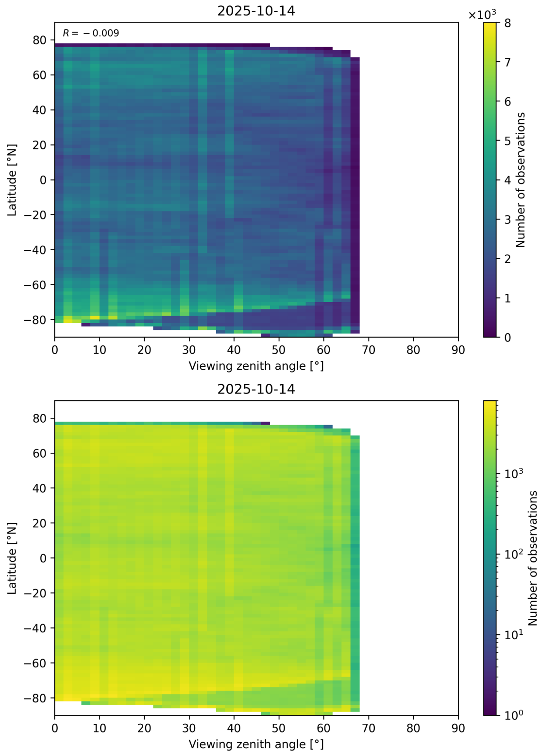
Figure 74: Scatter density plot of “Viewing zenith angle” against “Latitude” for 2025-10-13 to 2025-10-15.
