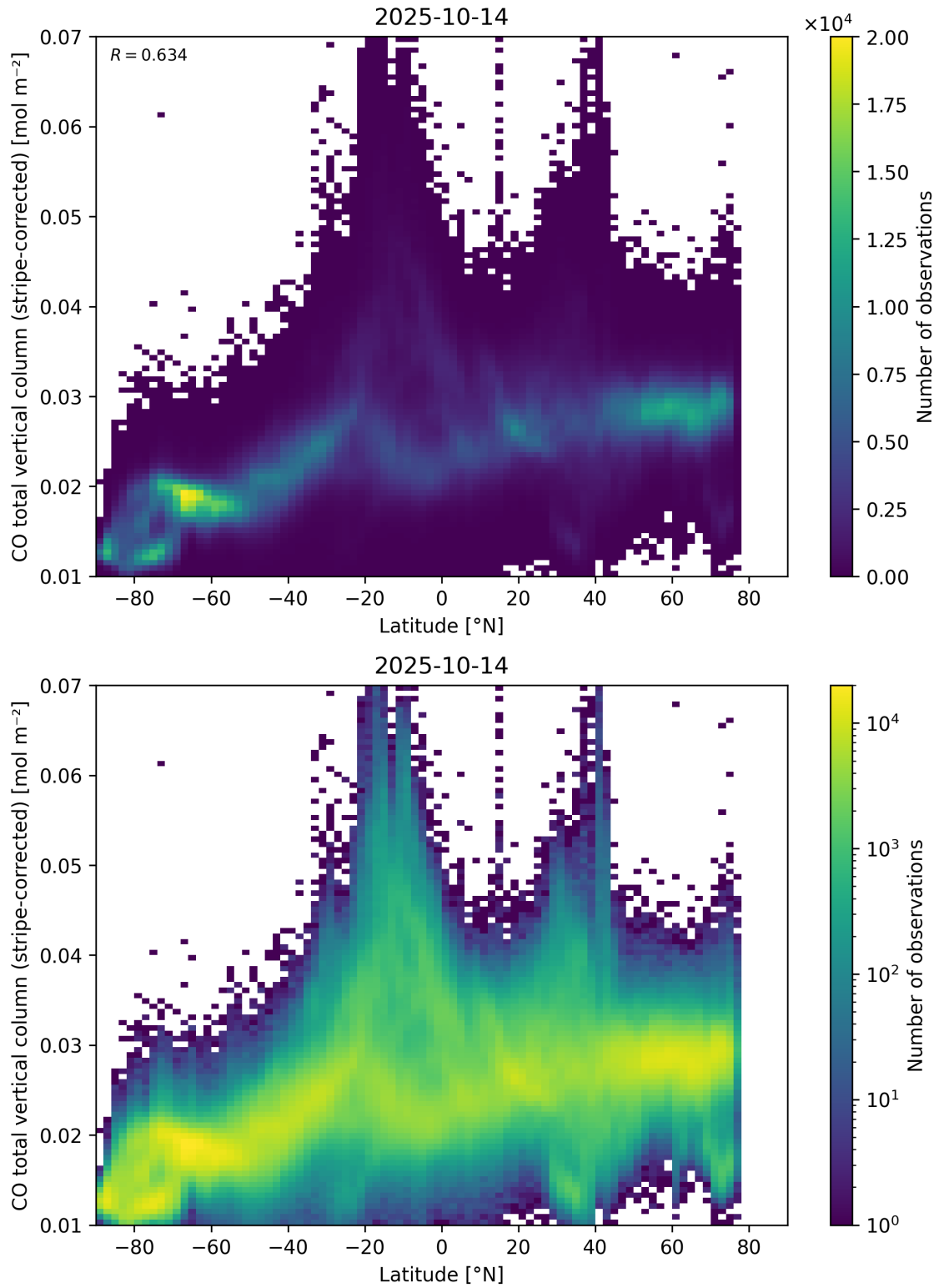
Figure 52: Scatter density plot of “Latitude” against “CO total vertical column (stripe-corrected)” for 2025-10-13 to 2025-10-15.
