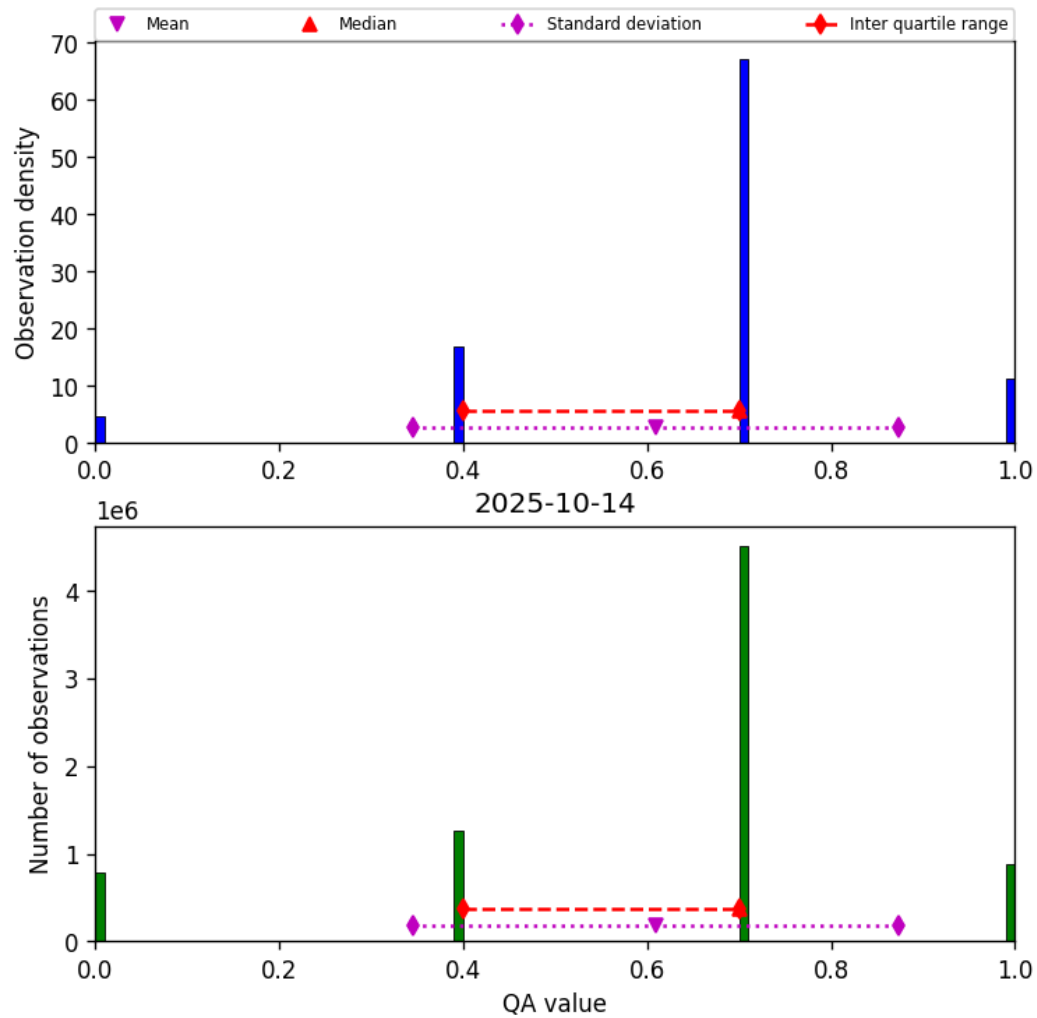
Figure 17: Histogram of “QA value” for 2025-10-13 to 2025-10-15
