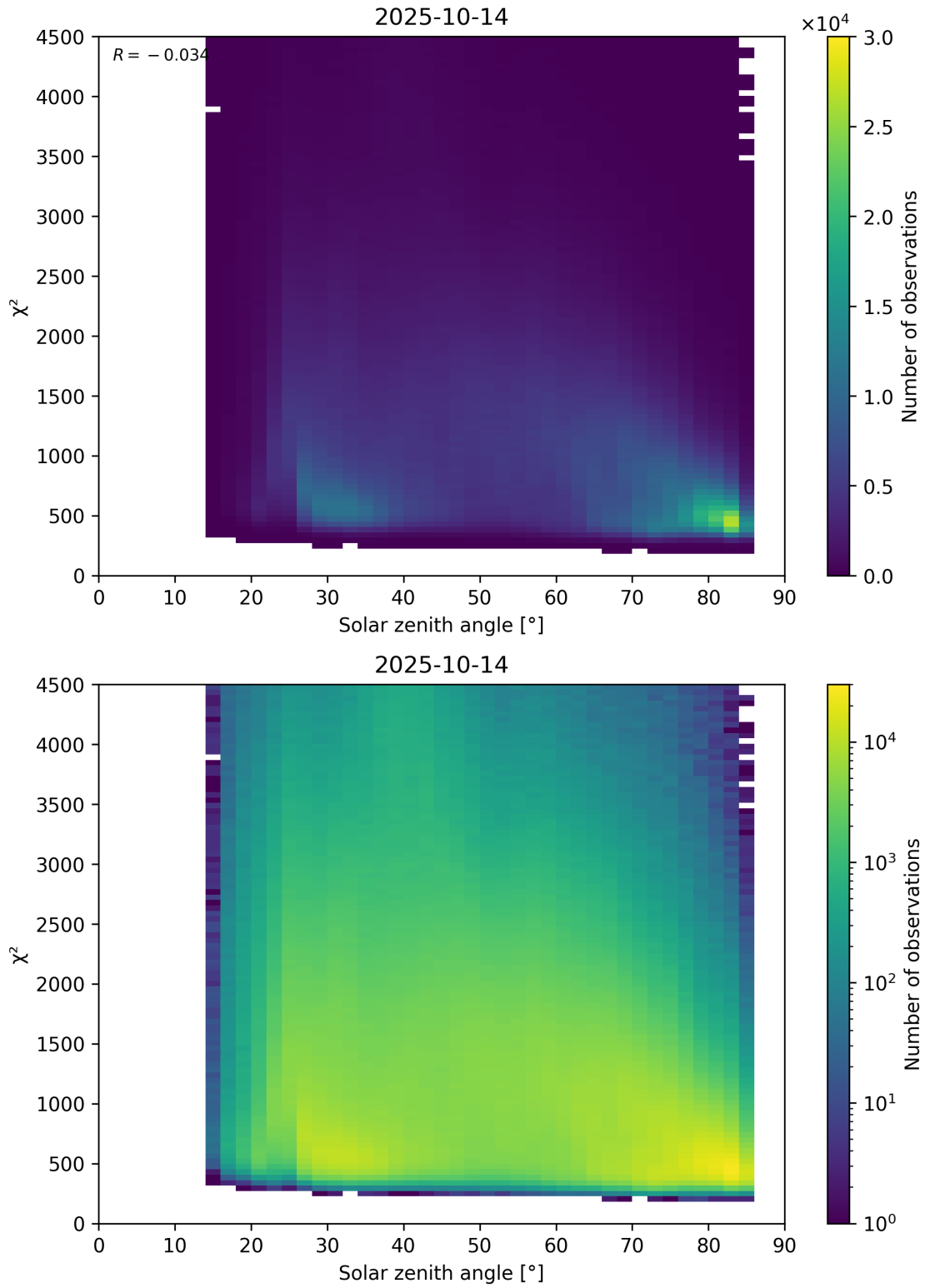
Figure 64: Scatter density plot of “Solar zenith angle” against “ \chi^2 ” for 2025-10-13 to 2025-10-15.
