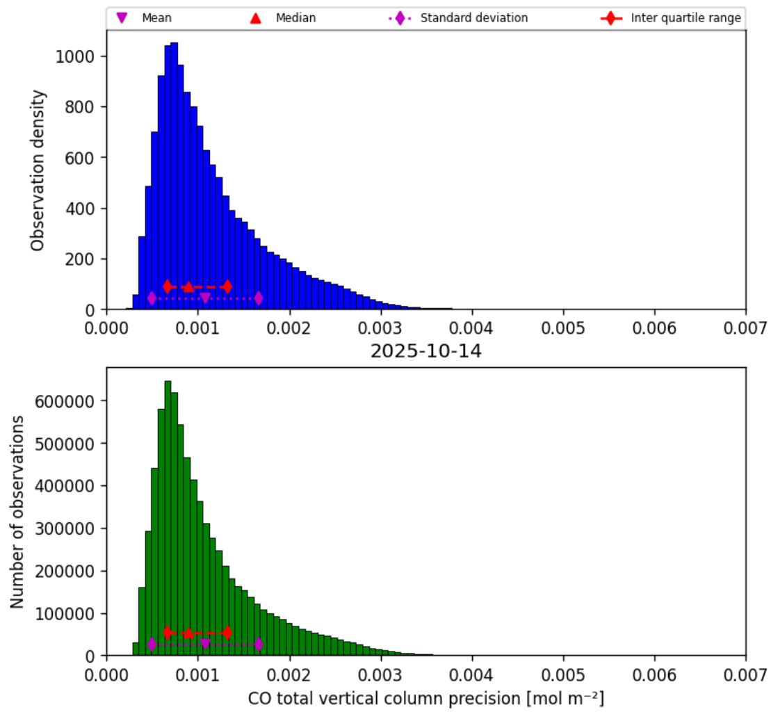
Figure 20: Histogram of “CO total vertical column precision” for 2025-10-13 to 2025-10-15
