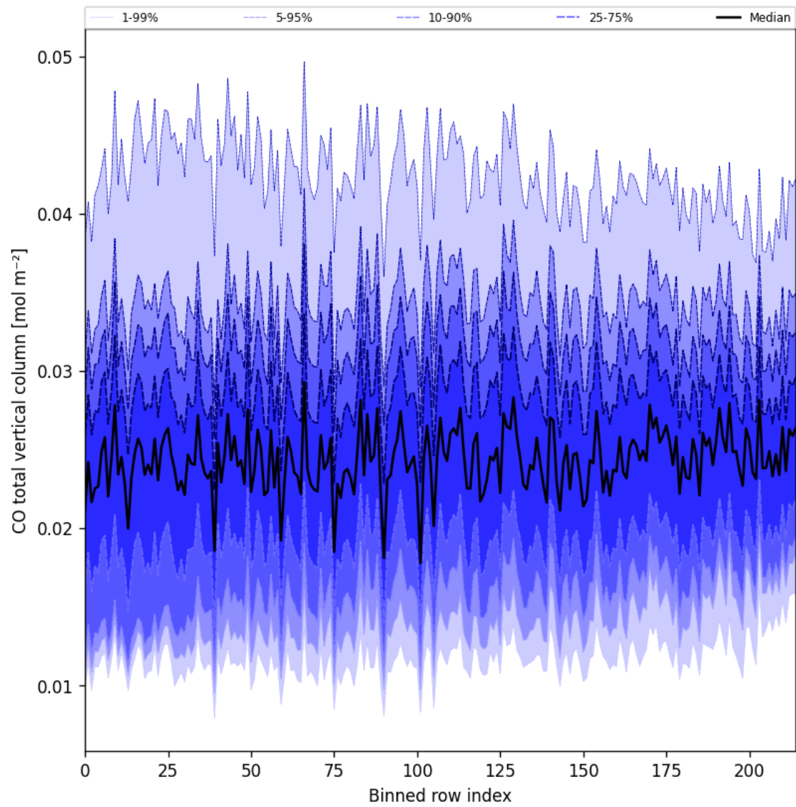
Figure 26: Along track statistics of “CO total vertical column” for 2025-10-13 to 2025-10-15
