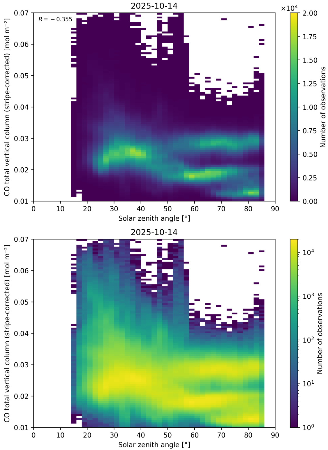
Figure 62: Scatter density plot of “Solar zenith angle” against “CO total vertical column (stripe-corrected)” for 2025-10-13 to 2025-10-15.
