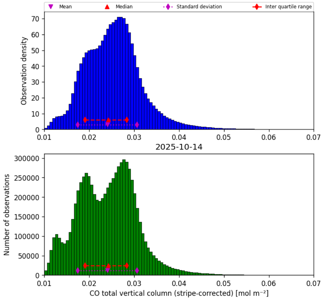
Figure 19: Histogram of “CO total vertical column (stripe-corrected)” for 2025-10-13 to 2025-10-15
