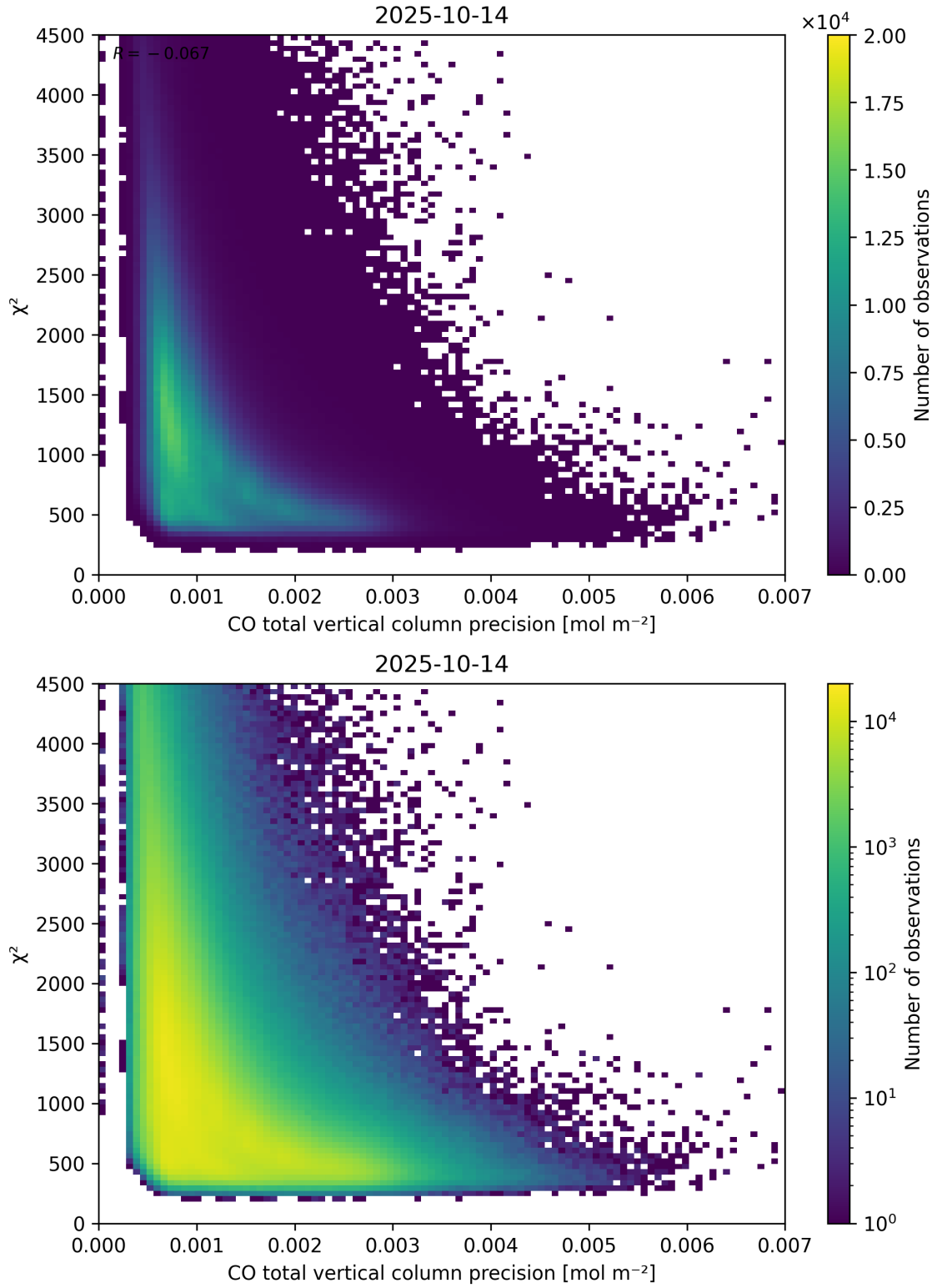
Figure 44: Scatter density plot of “CO total vertical column precision” against “ \chi^2 ” for 2025-10-13 to 2025-10-15.
