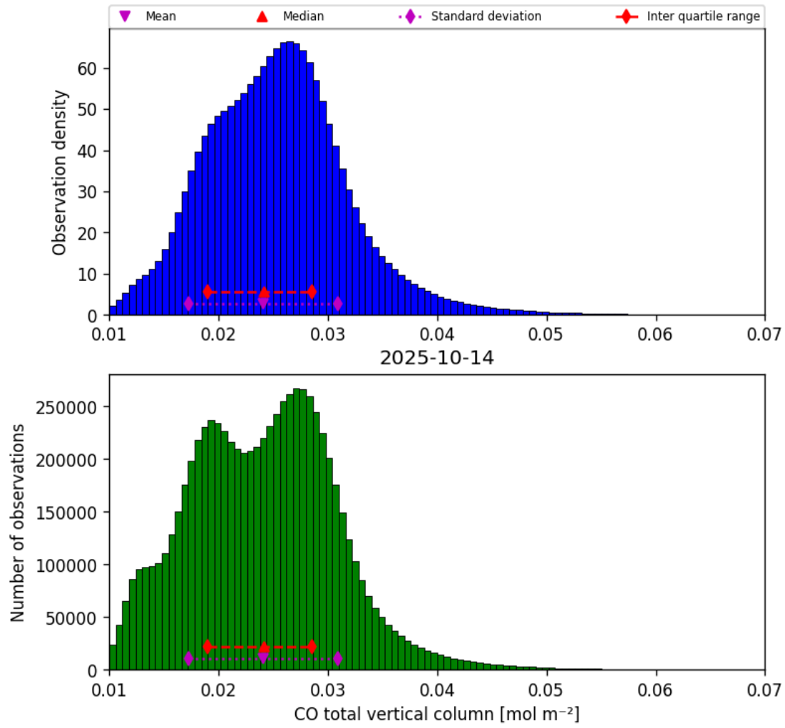
Figure 18: Histogram of “CO total vertical column” for 2025-10-13 to 2025-10-15
