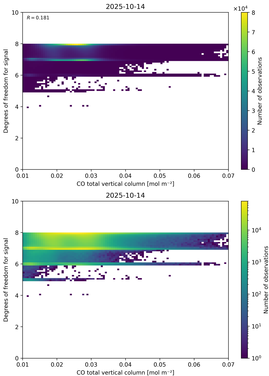
Figure 41: Scatter density plot of “CO total vertical column” against “Degrees of freedom for signal” for 2025-10-13 to 2025-10-15.
