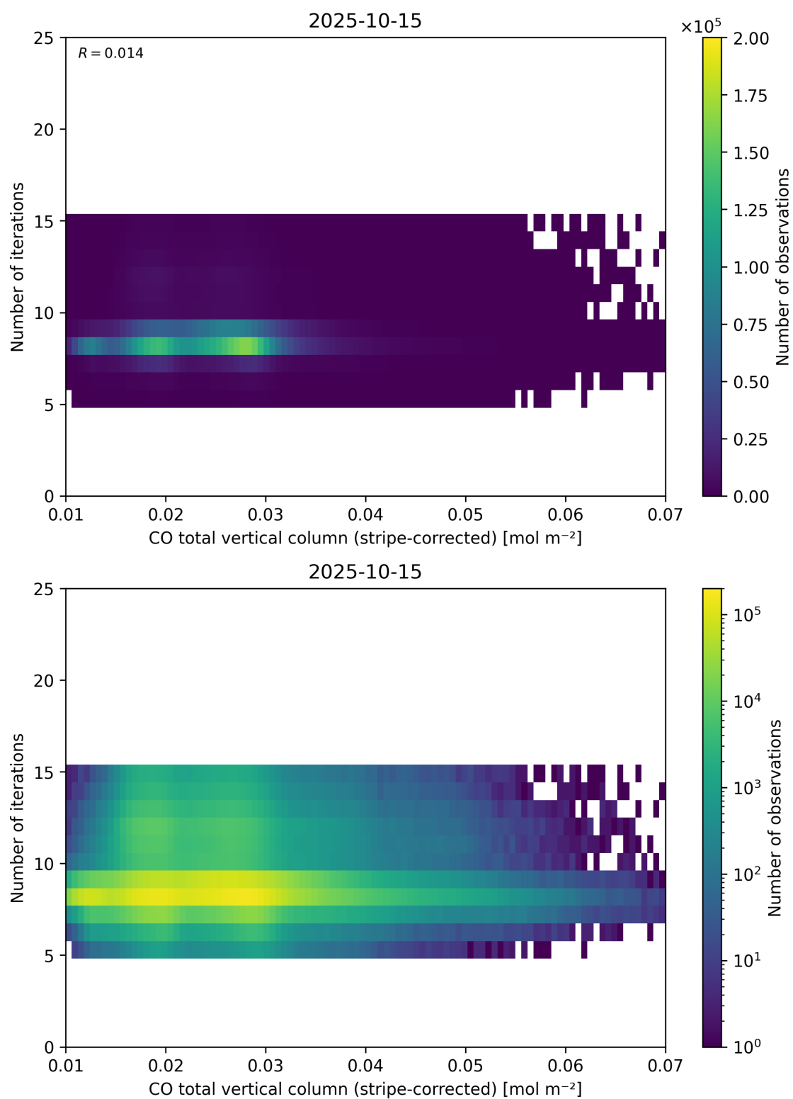
Figure 39: Scatter density plot of “CO total vertical column (stripe-corrected)” against “Number of iterations” for 2025-10-14 to 2025-10-16.
