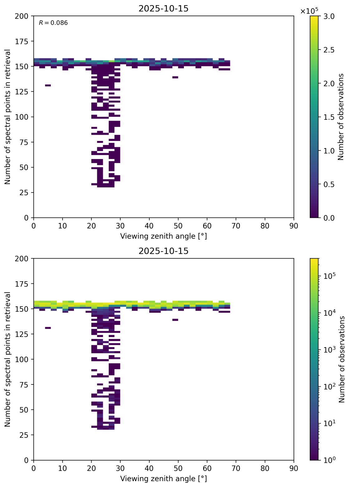
Figure 76: Scatter density plot of “Viewing zenith angle” against “Number of spectral points in retrieval” for 2025-10-14 to 2025-10-16.
