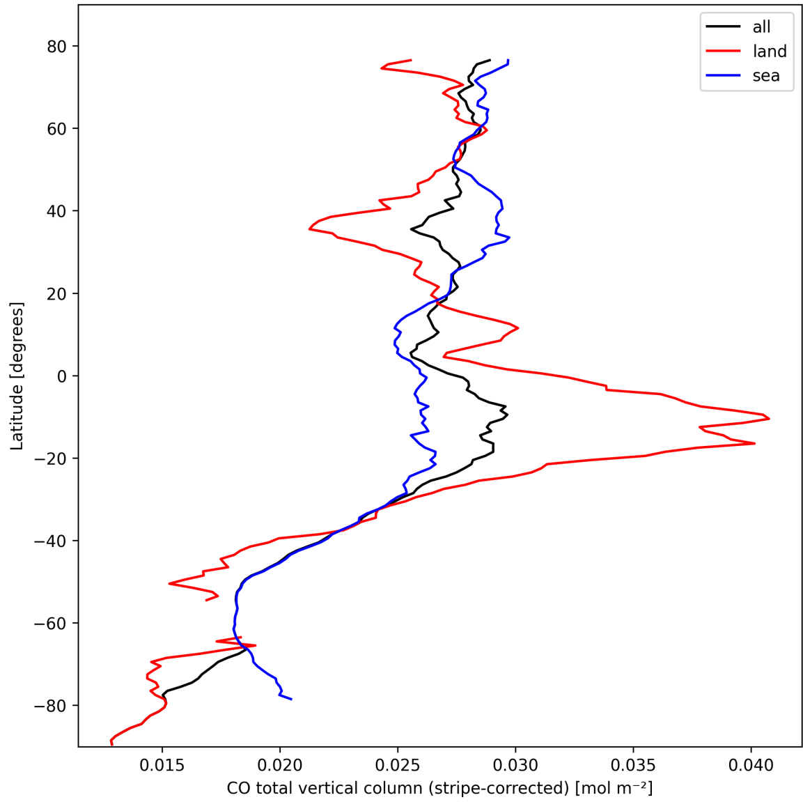
Figure 11: Zonal average of “CO total vertical column (stripe-corrected)” for 2025-10-14 to 2025-10-16.
