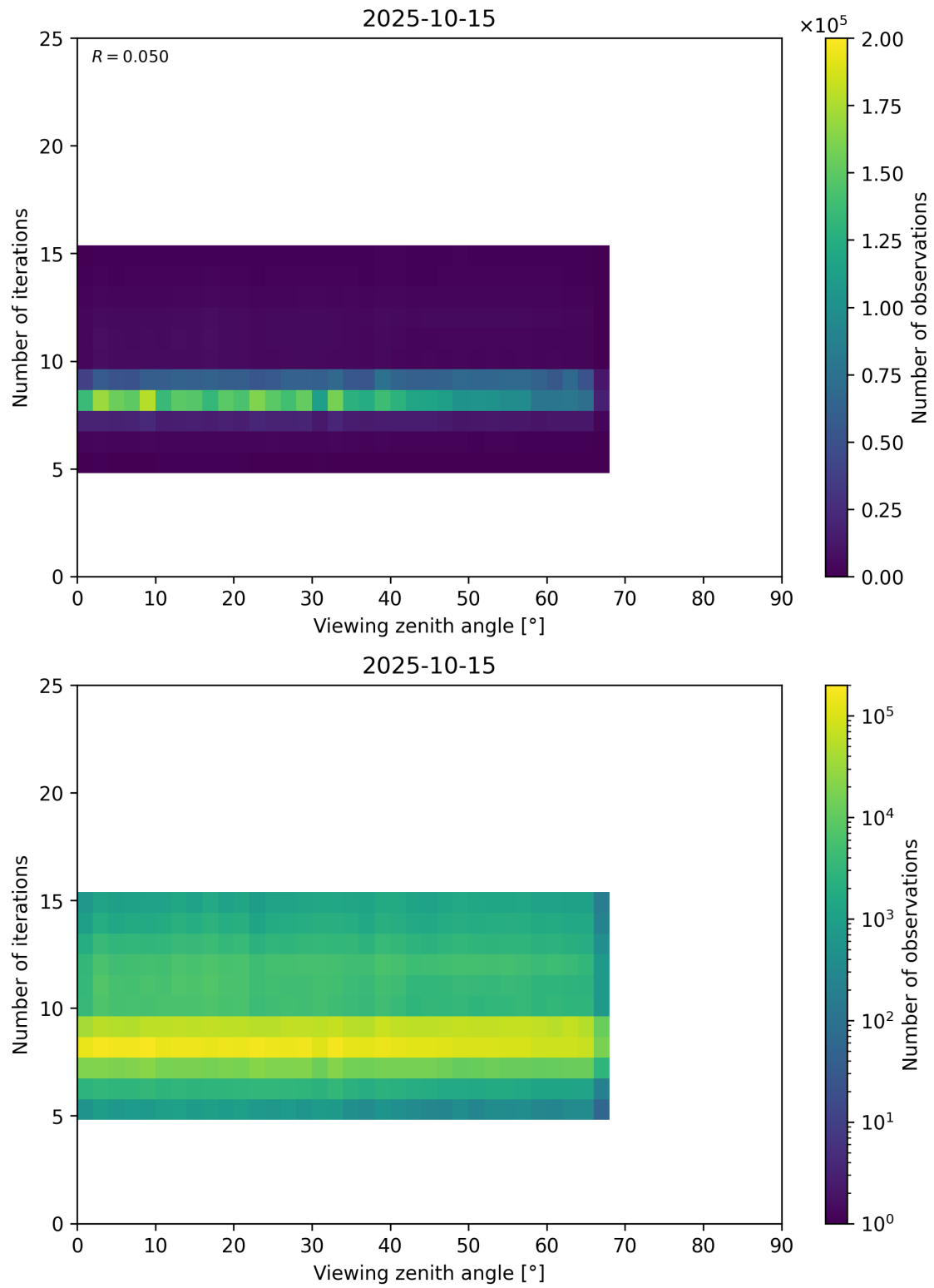
Figure 75: Scatter density plot of “Viewing zenith angle” against “Number of iterations” for 2025-10-14 to 2025-10-16.
