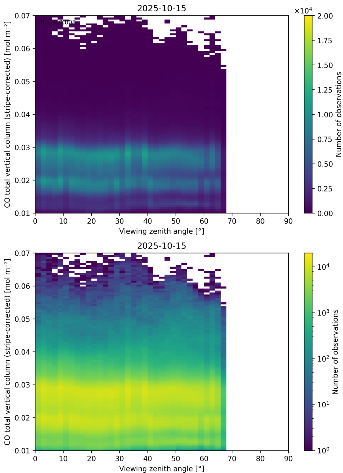
Figure 70: Scatter density plot of “Viewing zenith angle” against “CO total vertical column (stripe-corrected)” for 2025-10-14 to 2025-10-16.
