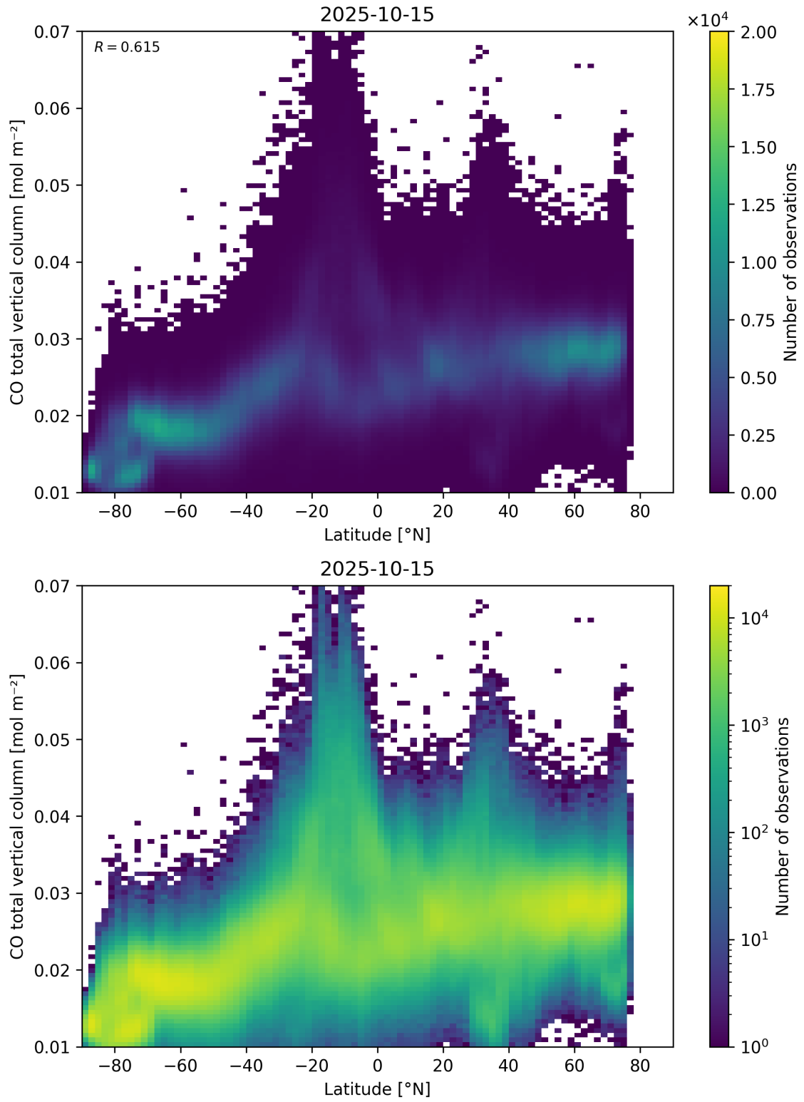
Figure 51: Scatter density plot of “Latitude” against “CO total vertical column” for 2025-10-14 to 2025-10-16.
