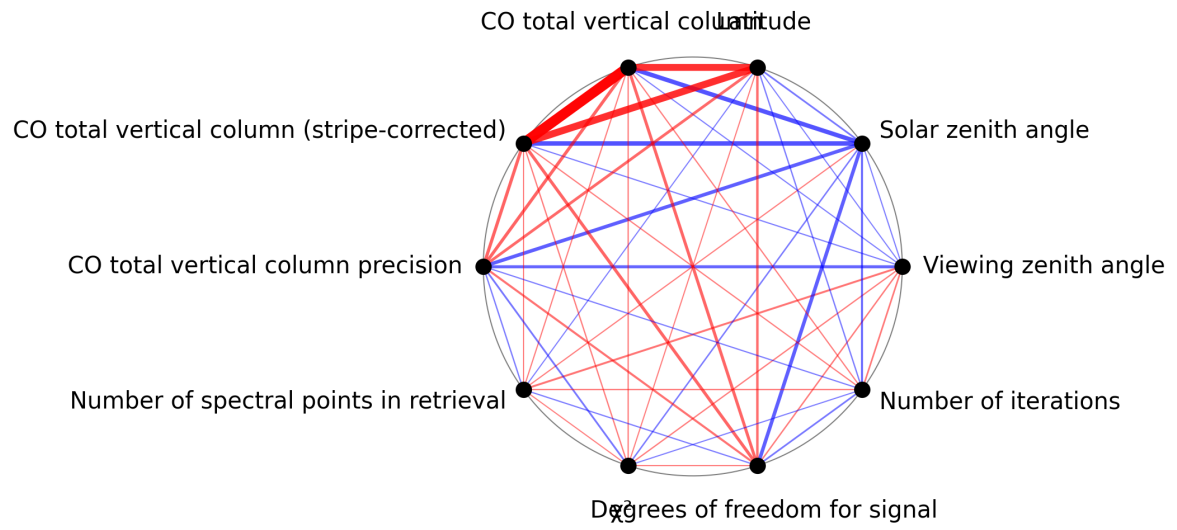
Figure 1: Map of correlation graph for 2025-10-14 to 2025-10-16.
