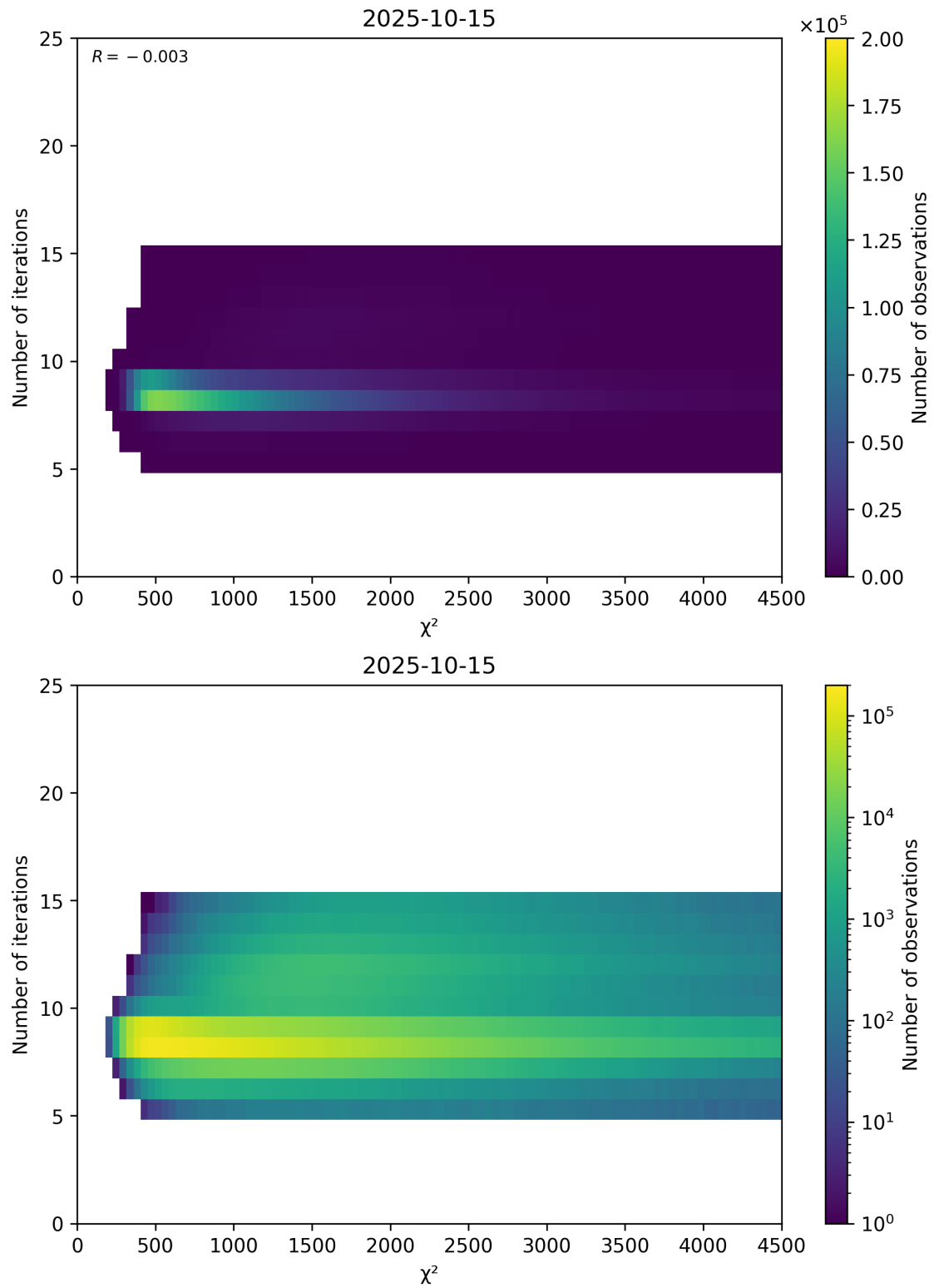
Figure 49: Scatter density plot of “ \chi^2 ” against “Number of iterations” for 2025-10-14 to 2025-10-16.
