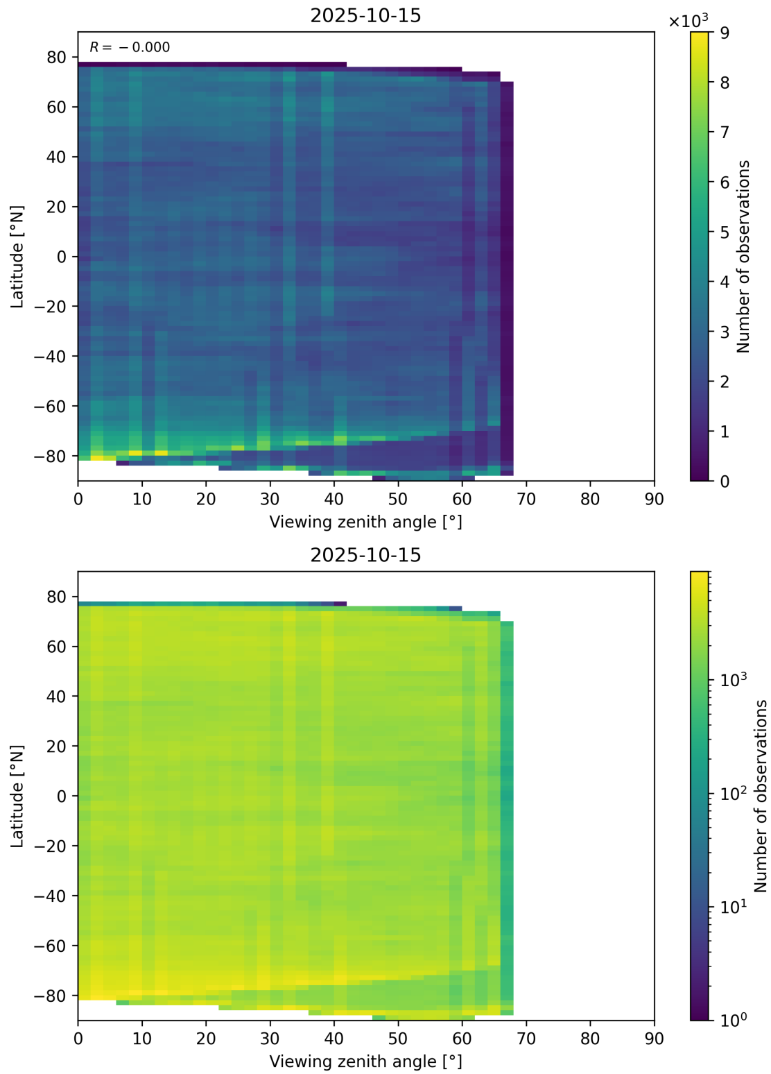
Figure 74: Scatter density plot of “Viewing zenith angle” against “Latitude” for 2025-10-14 to 2025-10-16.
