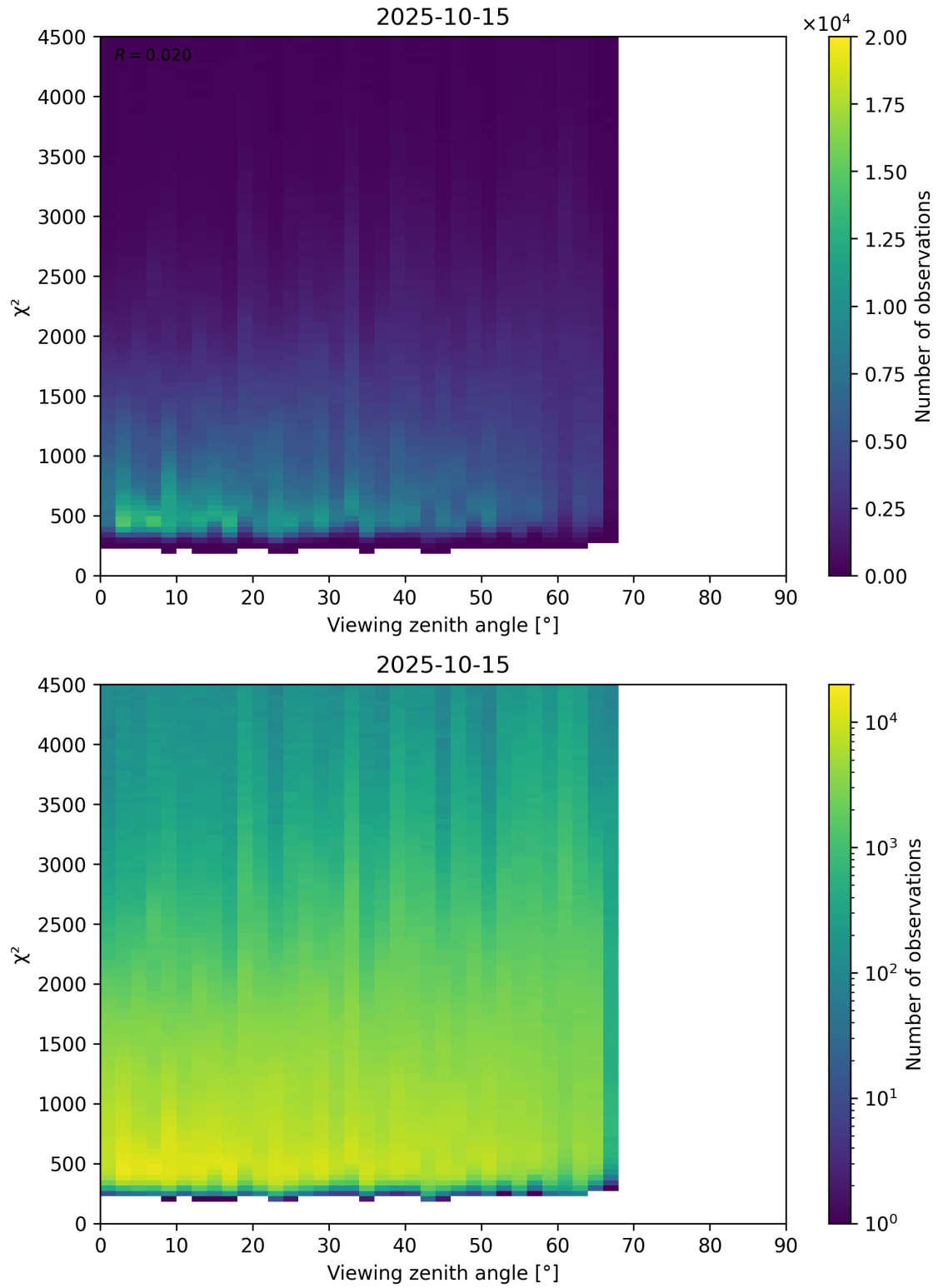
Figure 72: Scatter density plot of “Viewing zenith angle” against “ \chi^2 ” for 2025-10-14 to 2025-10-16.
