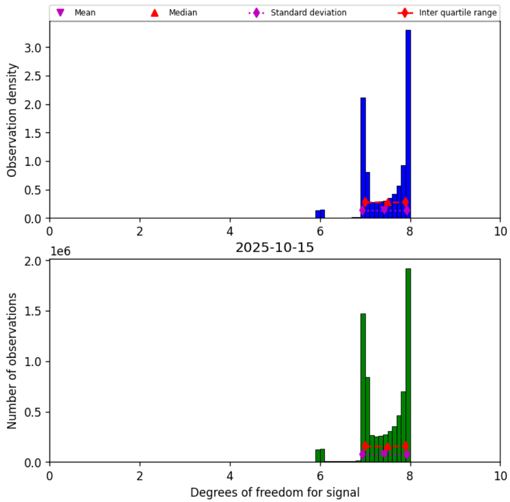
Figure 23: Histogram of “Degrees of freedom for signal” for 2025-10-14 to 2025-10-16
