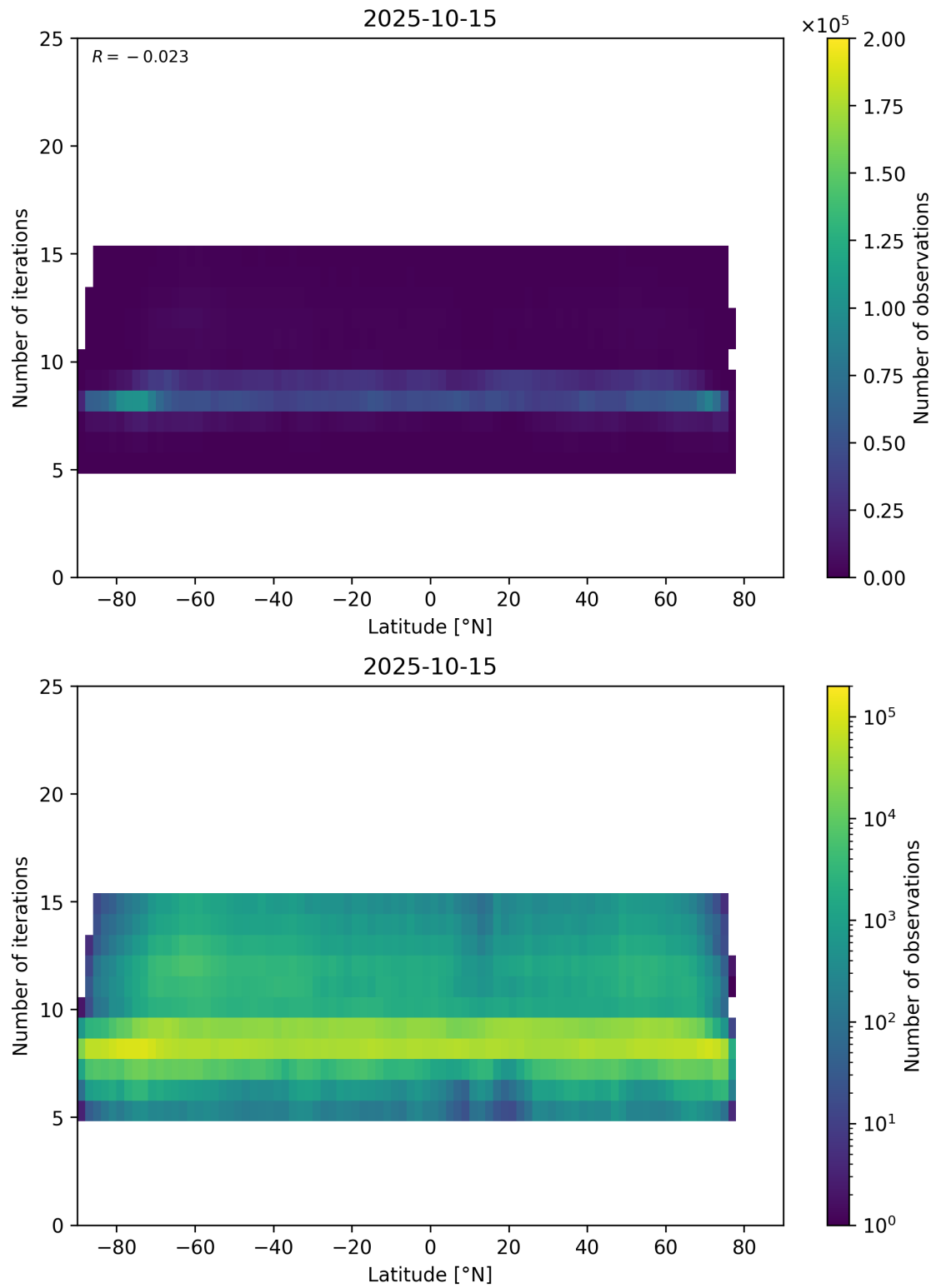
Figure 56: Scatter density plot of “Latitude” against “Number of iterations” for 2025-10-14 to 2025-10-16.
