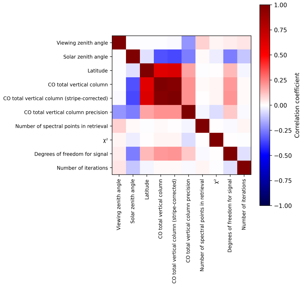
Figure 2: Map of correlation matrix for 2025-10-14 to 2025-10-16.
