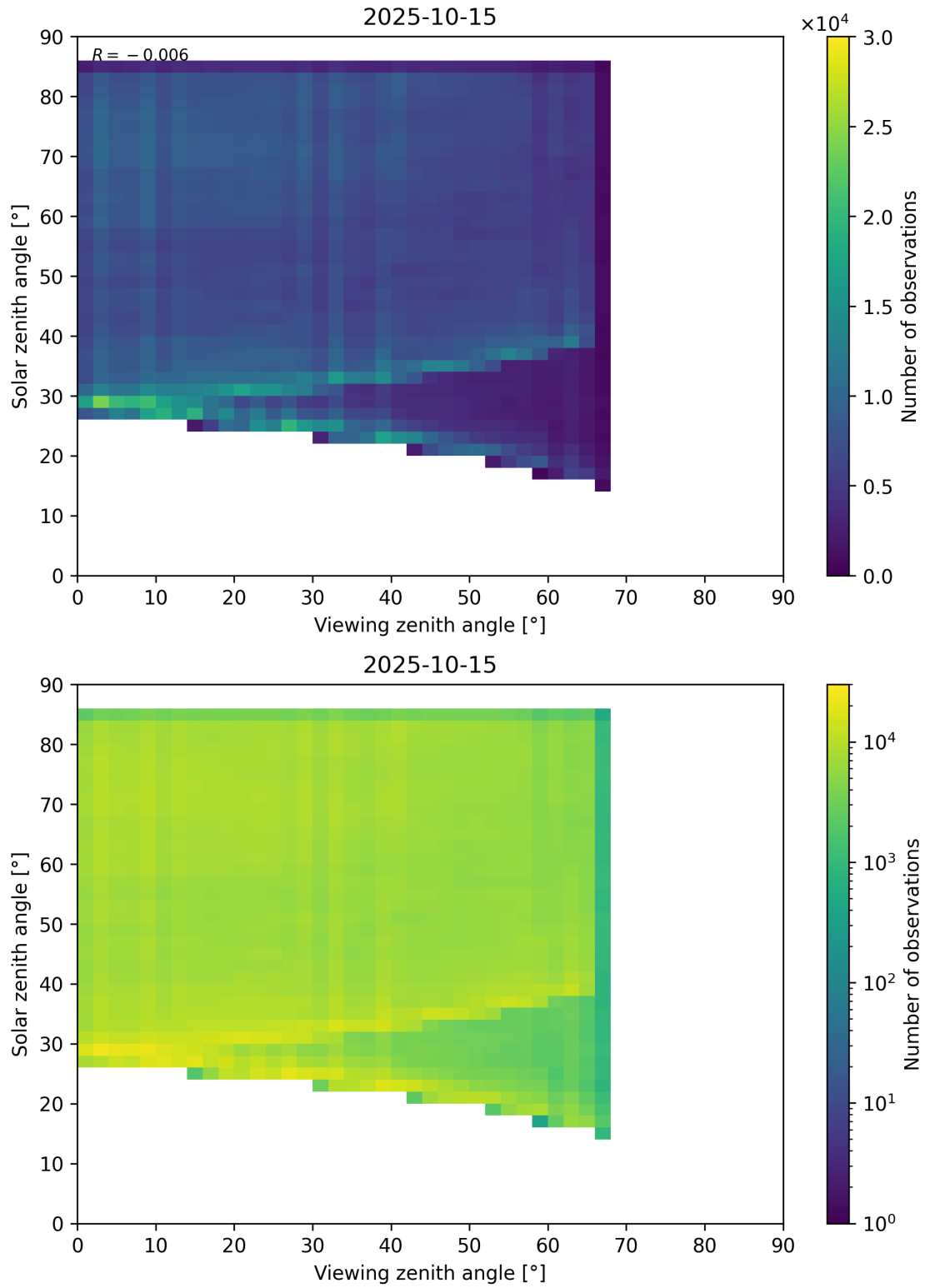
Figure 77: Scatter density plot of “Viewing zenith angle” against “Solar zenith angle” for 2025-10-14 to 2025-10-16.
