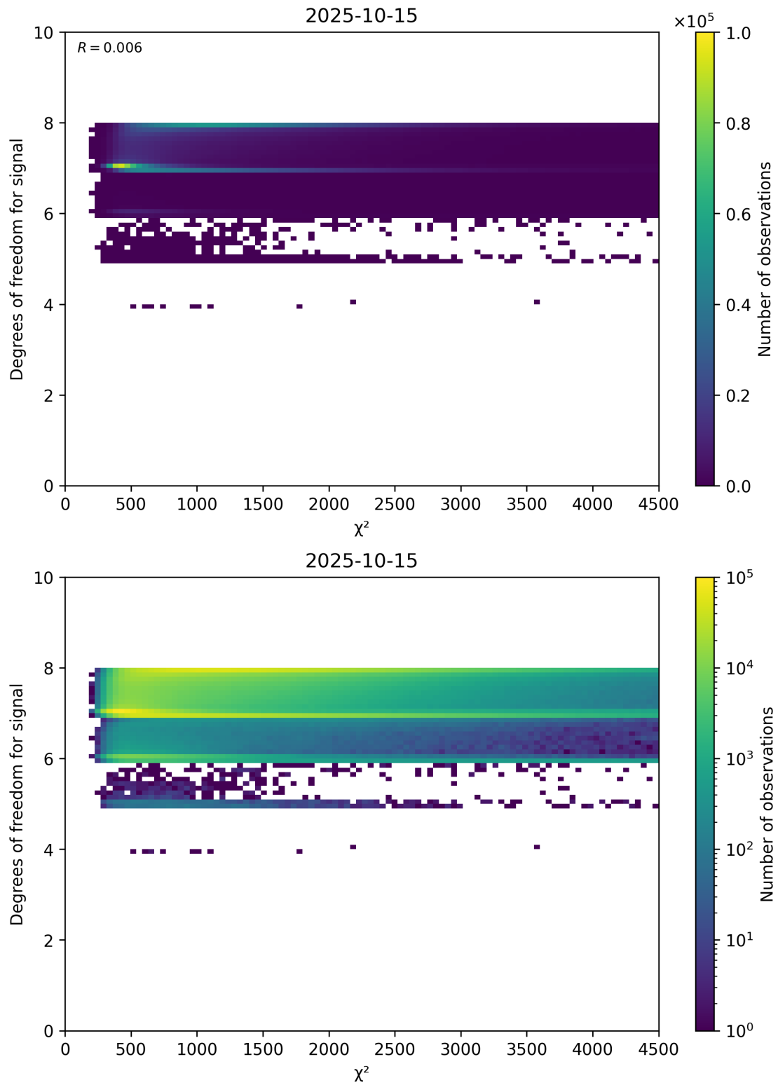
Figure 48: Scatter density plot of “ \chi^2 ” against “Degrees of freedom for signal” for 2025-10-14 to 2025-10-16.
