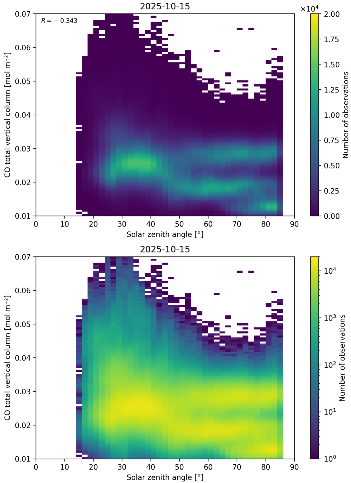
Figure 61: Scatter density plot of “Solar zenith angle” against “CO total vertical column” for 2025-10-14 to 2025-10-16.
