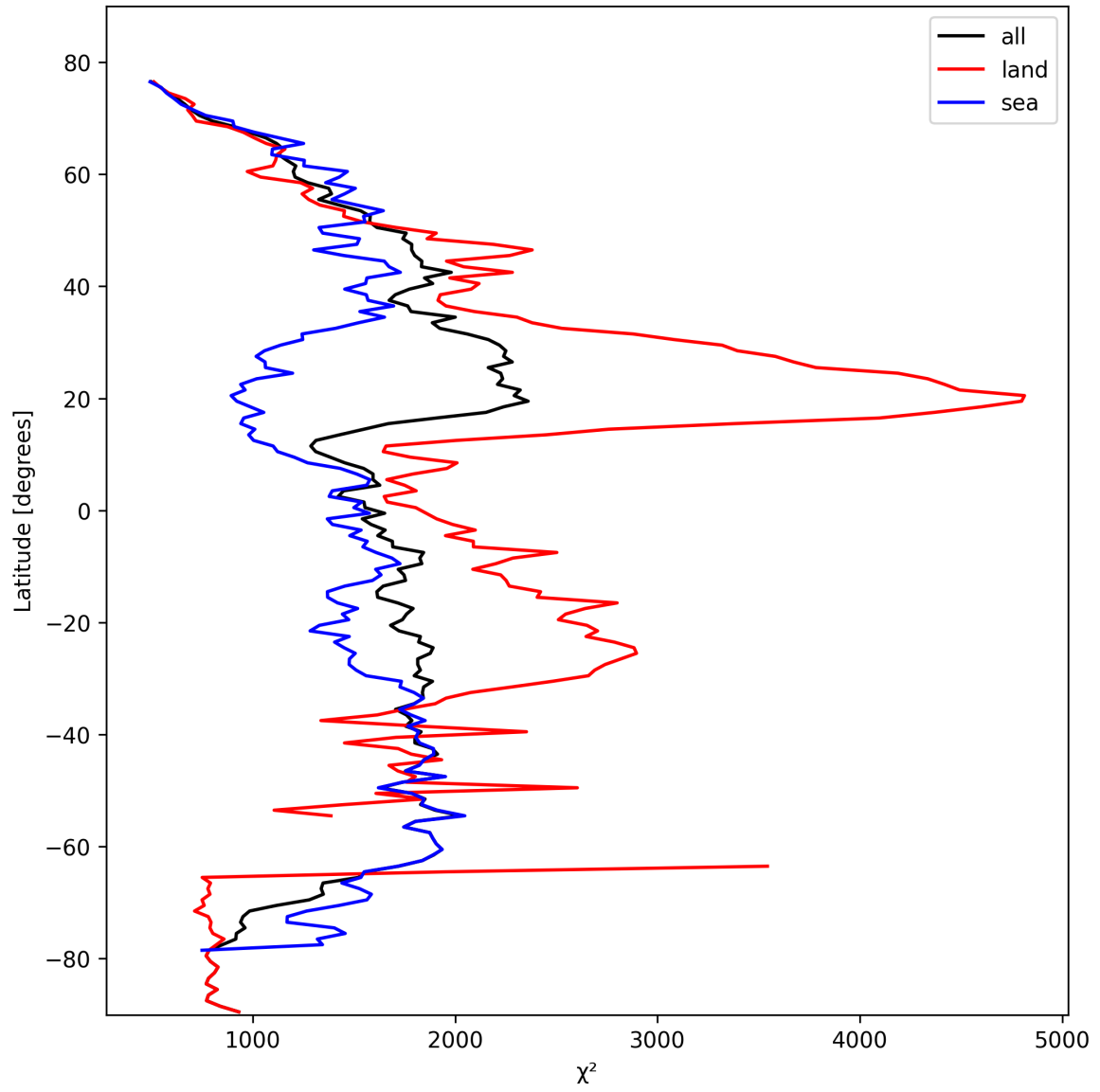
Figure 14: Zonal average of “ \chi^2 ” for 2025-10-14 to 2025-10-16.
