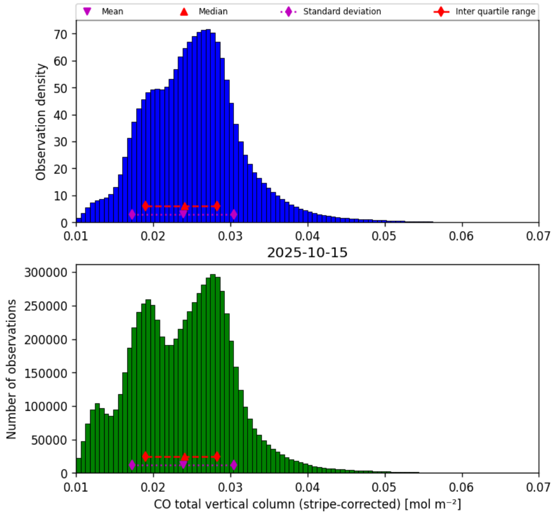
Figure 19: Histogram of “CO total vertical column (stripe-corrected)” for 2025-10-14 to 2025-10-16
