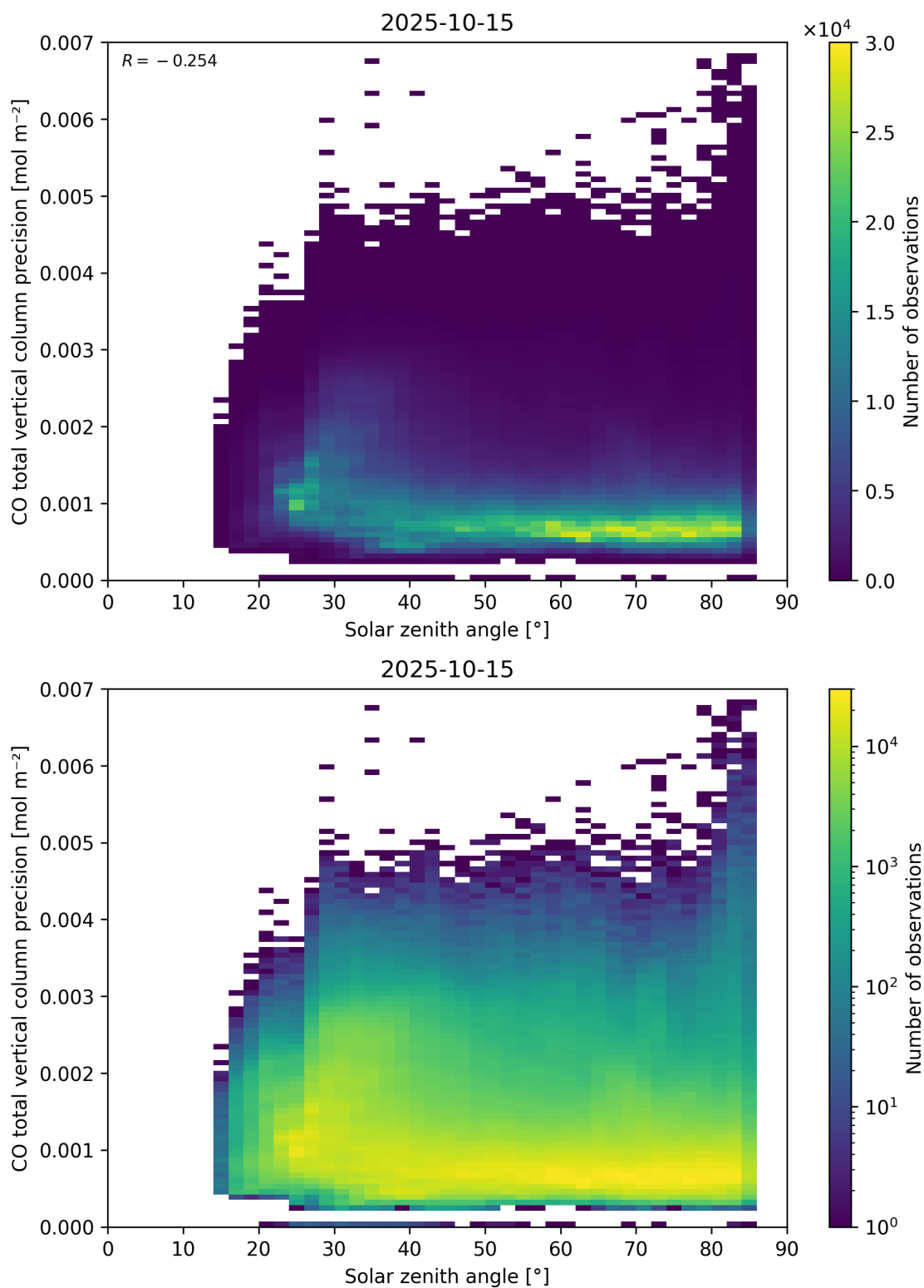
Figure 63: Scatter density plot of “Solar zenith angle” against “CO total vertical column precision” for 2025-10-14 to 2025-10-16.
