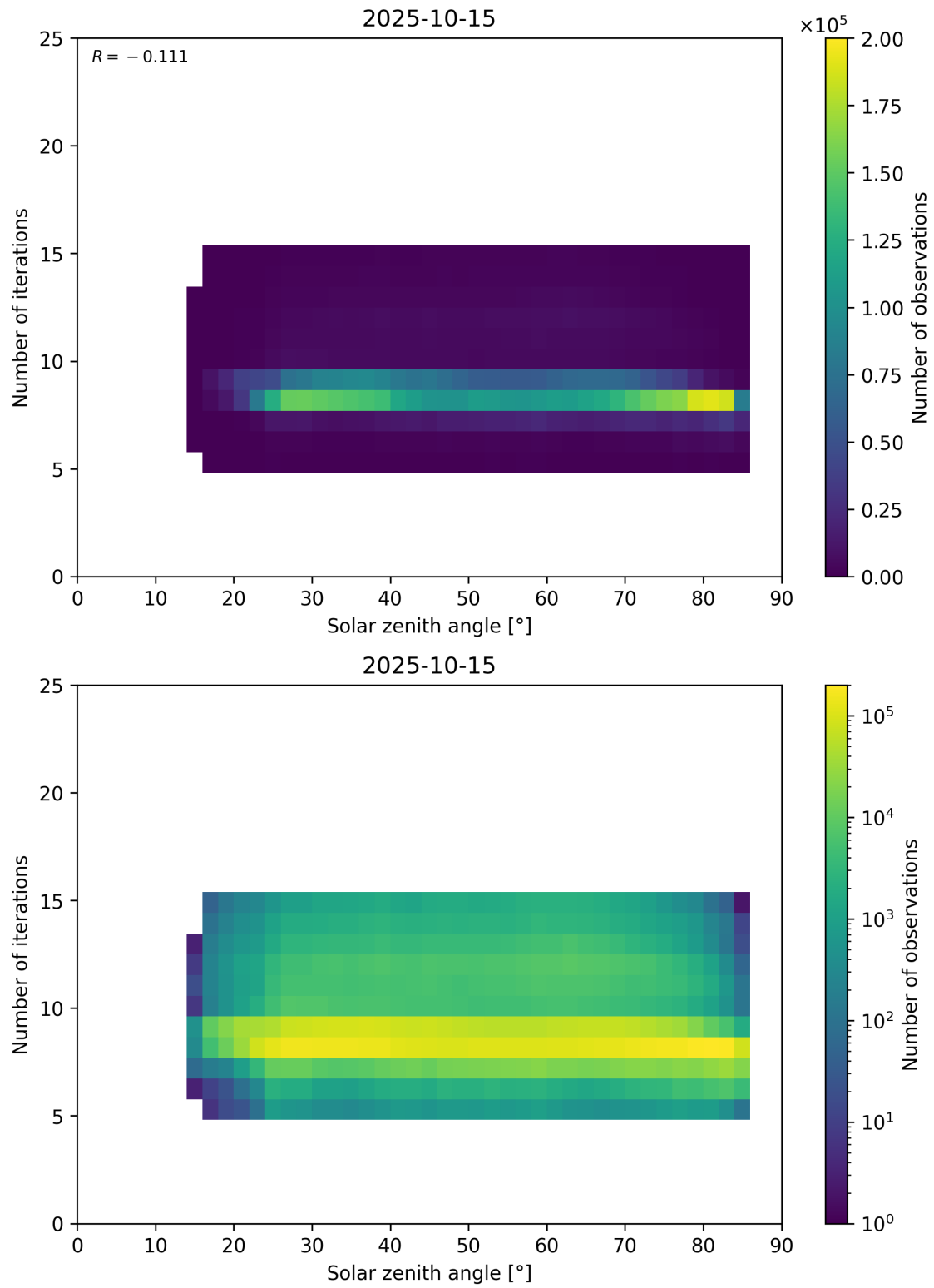
Figure 67: Scatter density plot of “Solar zenith angle” against “Number of iterations” for 2025-10-14 to 2025-10-16.
