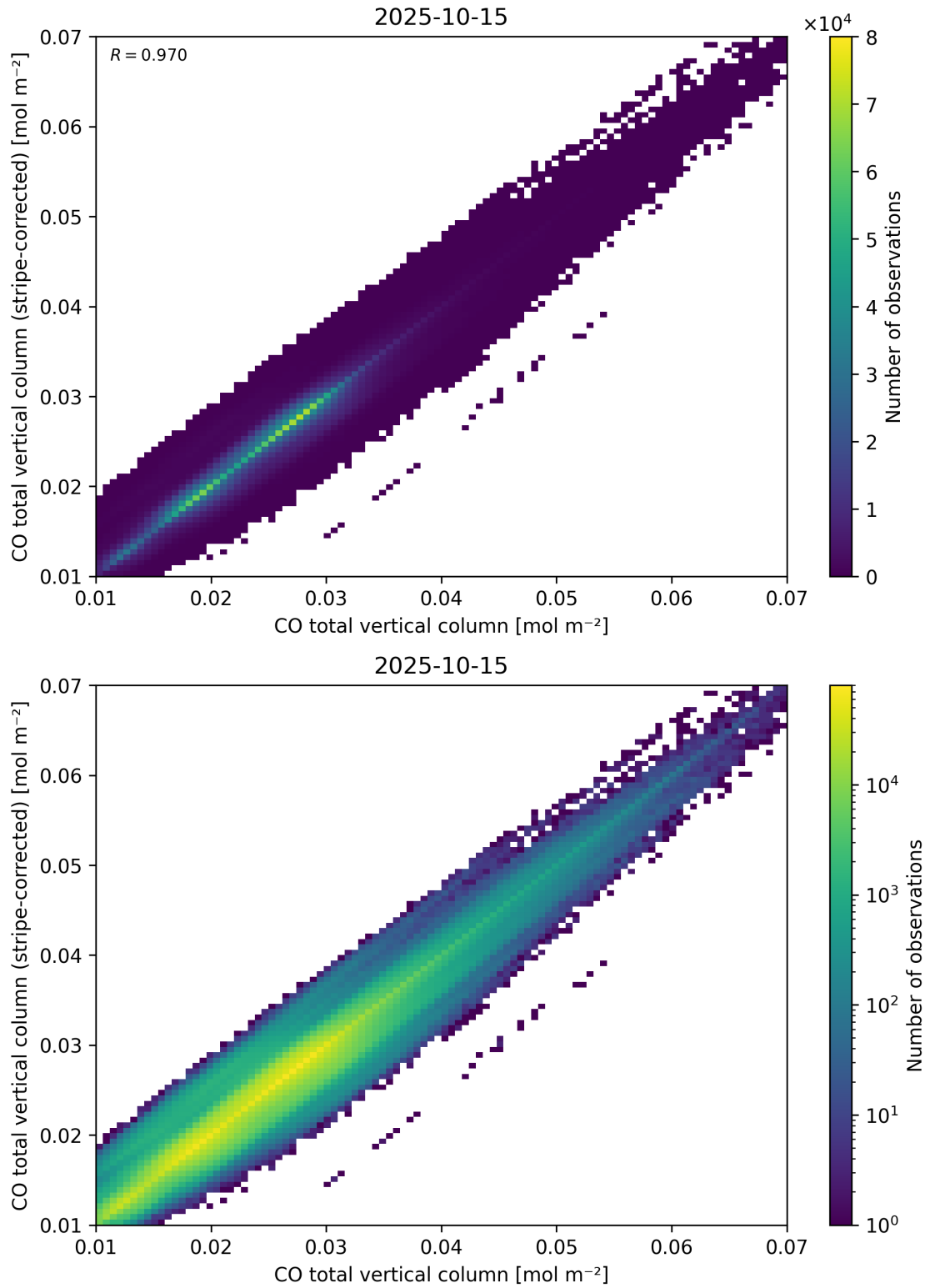
Figure 33: Scatter density plot of “CO total vertical column” against “CO total vertical column (stripe-corrected)” for 2025-10-14 to 2025-10-16.
