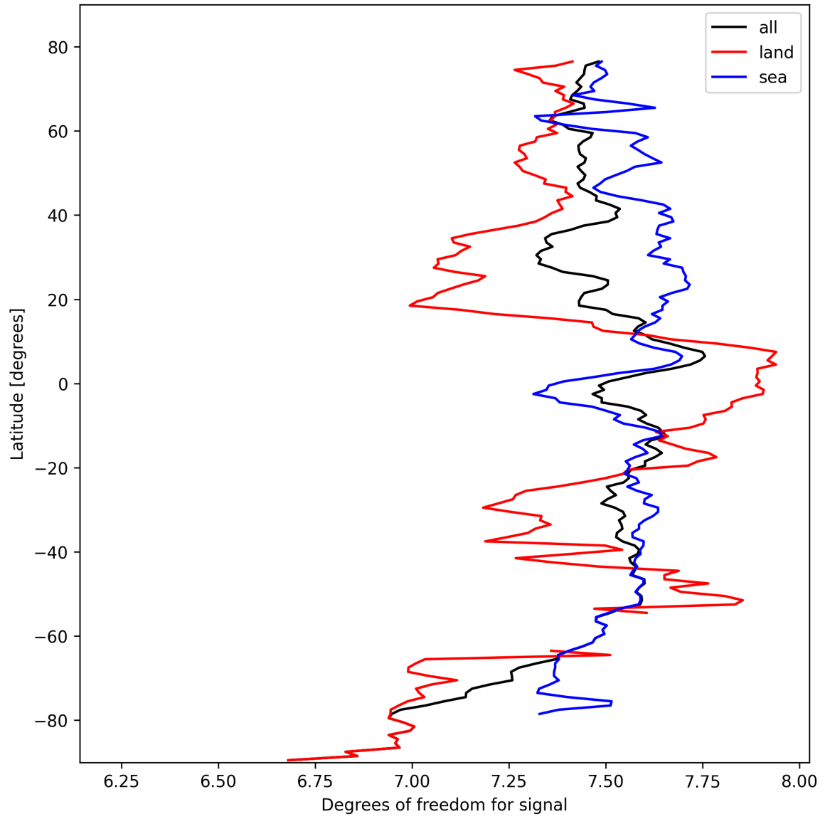
Figure 15: Zonal average of “Degrees of freedom for signal” for 2025-10-14 to 2025-10-16.
