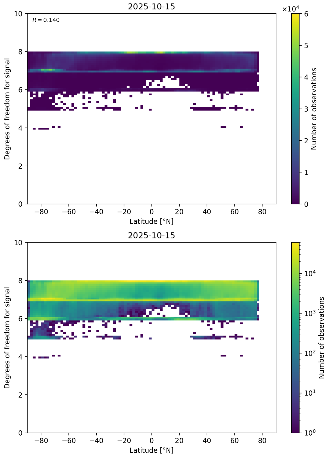
Figure 55: Scatter density plot of “Latitude” against “Degrees of freedom for signal” for 2025-10-14 to 2025-10-16.
