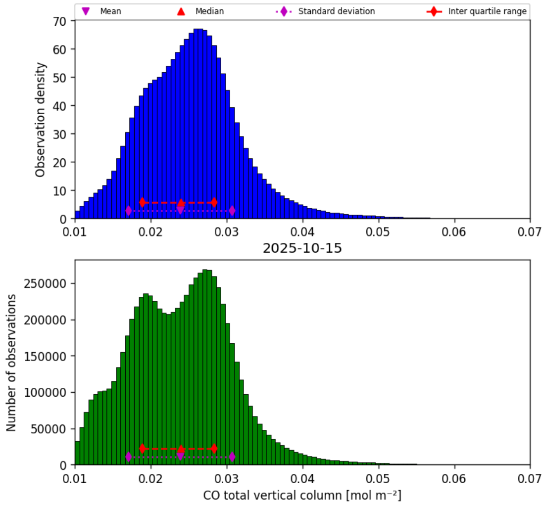
Figure 18: Histogram of “CO total vertical column” for 2025-10-14 to 2025-10-16
