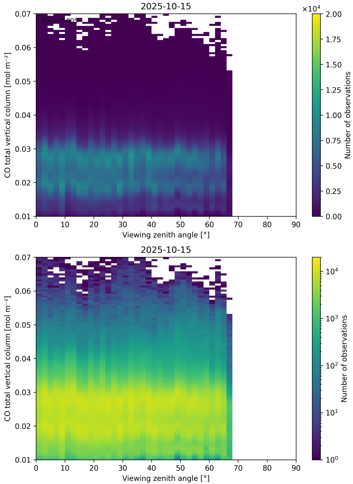
Figure 69: Scatter density plot of “Viewing zenith angle” against “CO total vertical column” for 2025-10-14 to 2025-10-16.
