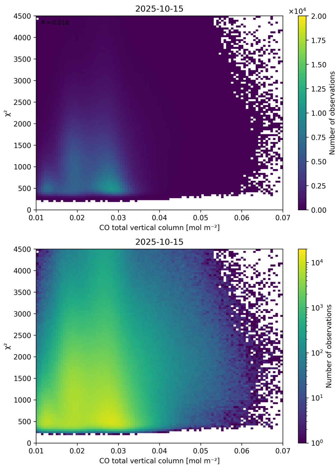
Figure 35: Scatter density plot of “CO total vertical column” against “ \chi^2 ” for 2025-10-14 to 2025-10-16.
