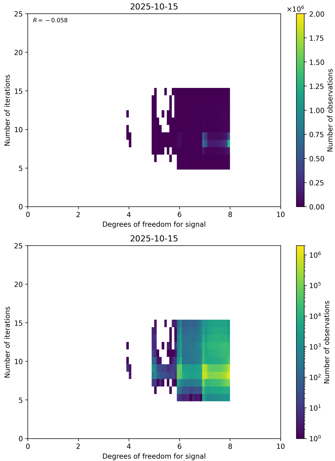
Figure 50: Scatter density plot of “Degrees of freedom for signal” against “Number of iterations” for 2025-10-14 to 2025-10-16.
