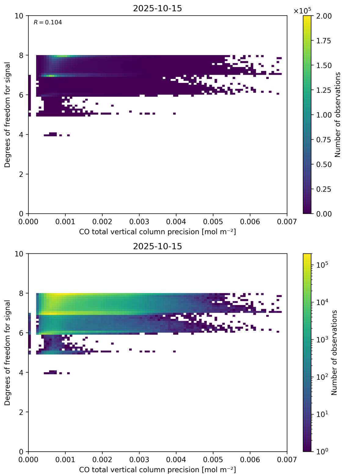
Figure 45: Scatter density plot of “CO total vertical column precision” against “Degrees of freedom for signal” for 2025-10-14 to 2025-10-16.
