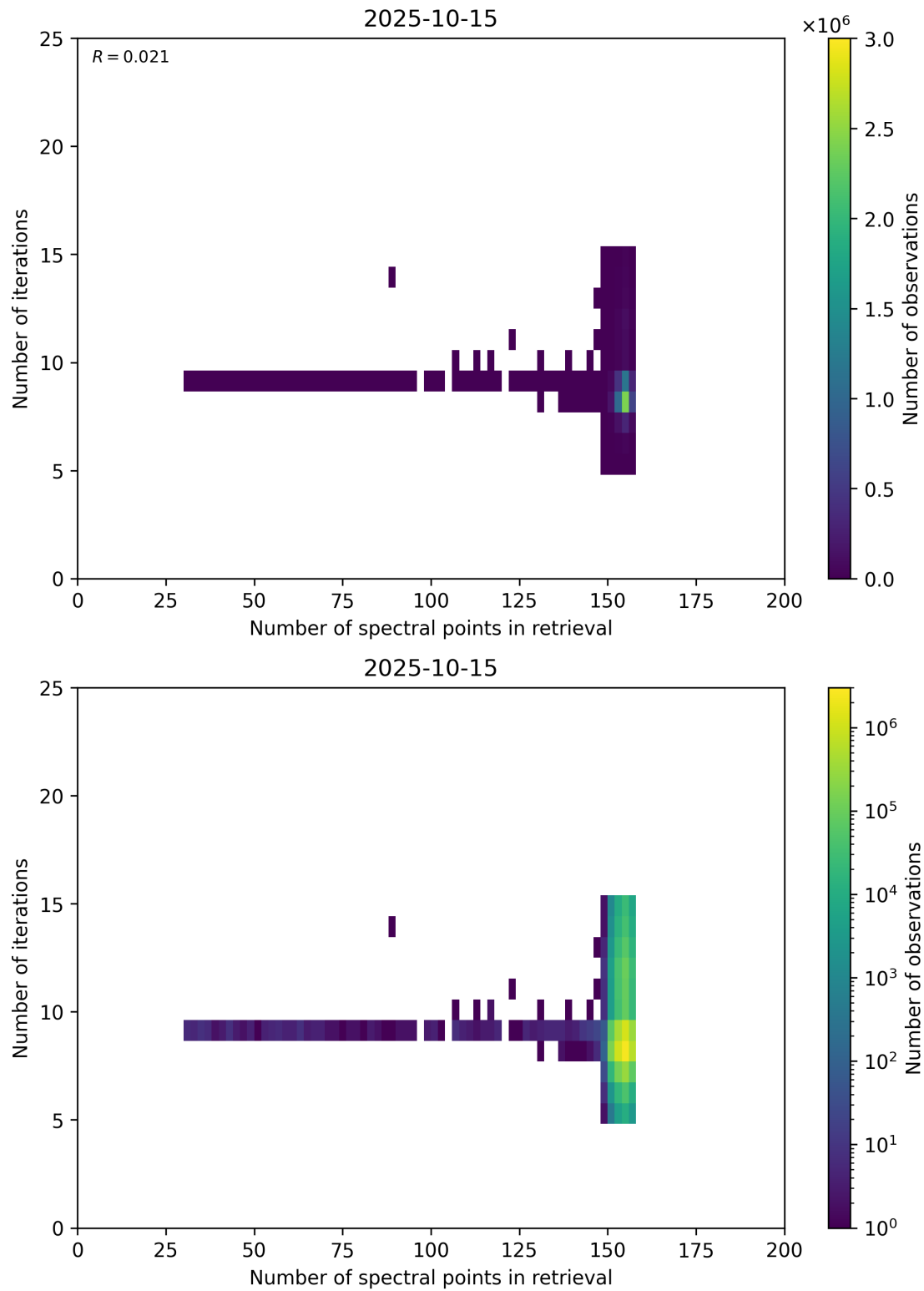
Figure 60: Scatter density plot of “Number of spectral points in retrieval” against “Number of iterations” for 2025-10-14 to 2025-10-16.
