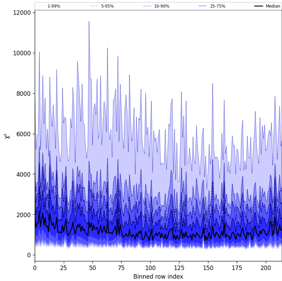
Figure 30: Along track statistics of “ \chi^2 ” for 2025-10-14 to 2025-10-16
