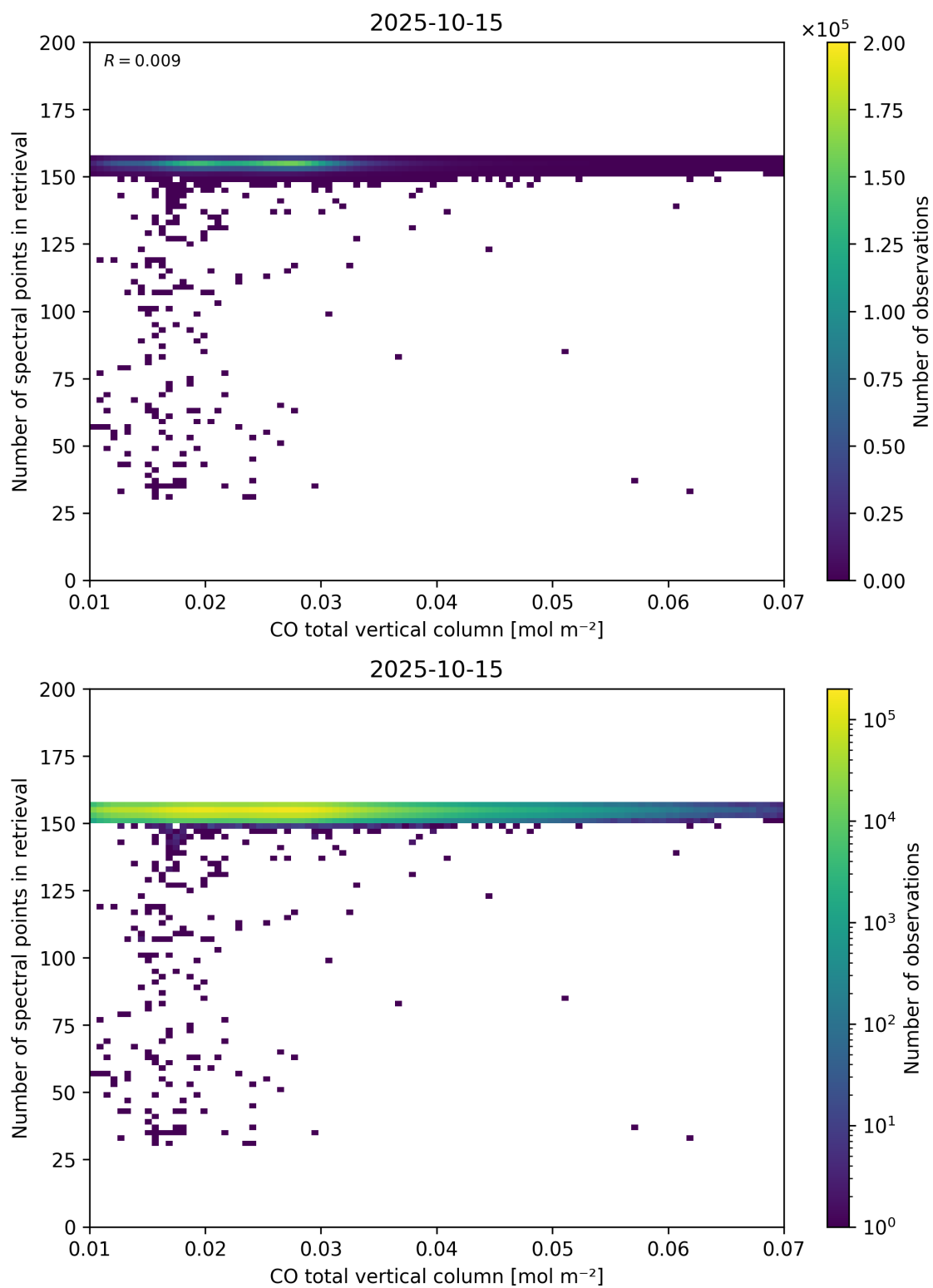
Figure 43: Scatter density plot of “CO total vertical column” against “Number of spectral points in retrieval” for 2025-10-14 to 2025-10-16.
