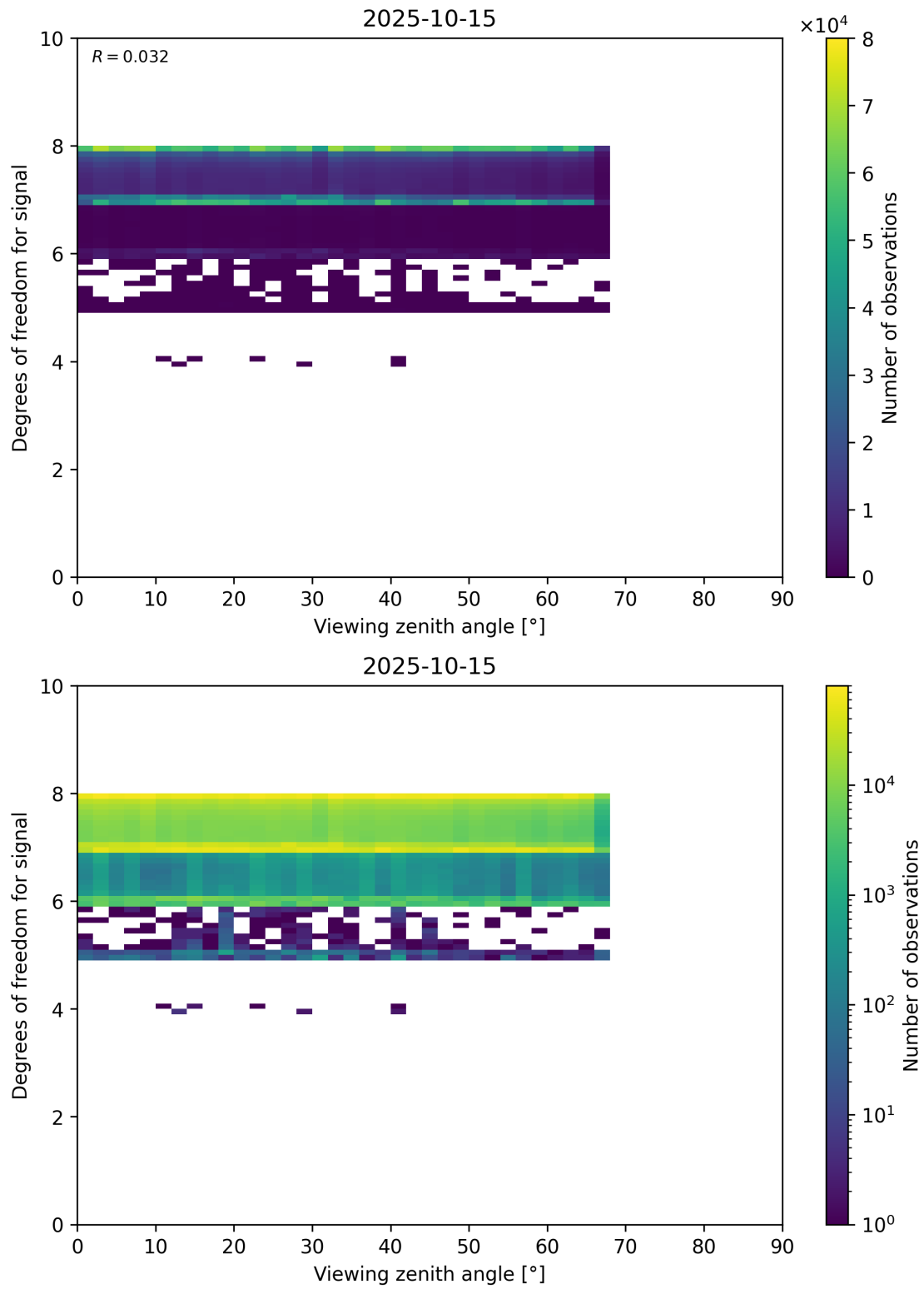
Figure 73: Scatter density plot of “Viewing zenith angle” against “Degrees of freedom for signal” for 2025-10-14 to 2025-10-16.
