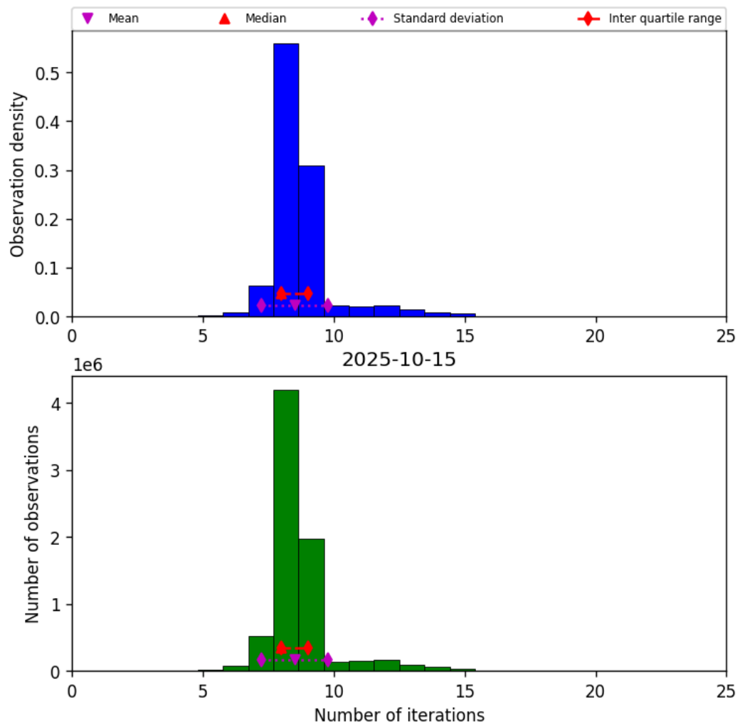
Figure 24: Histogram of “Number of iterations” for 2025-10-14 to 2025-10-16
