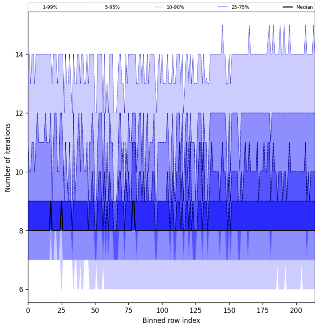
Figure 32: Along track statistics of “Number of iterations” for 2025-10-14 to 2025-10-16
