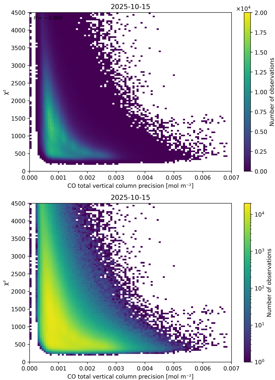
Figure 44: Scatter density plot of “CO total vertical column precision” against “ \chi^2 ” for 2025-10-14 to 2025-10-16.
