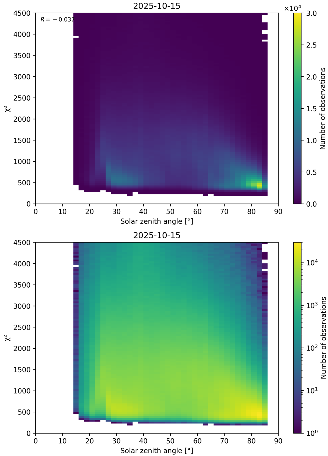
Figure 64: Scatter density plot of “Solar zenith angle” against “ \chi^2 ” for 2025-10-14 to 2025-10-16.
