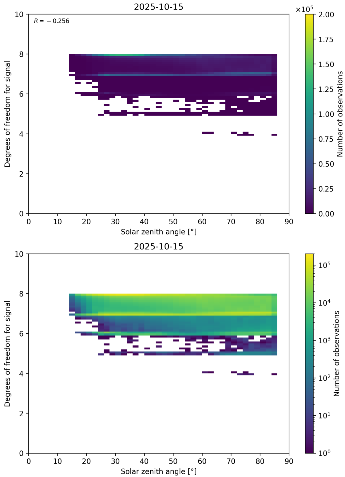
Figure 65: Scatter density plot of “Solar zenith angle” against “Degrees of freedom for signal” for 2025-10-14 to 2025-10-16.
