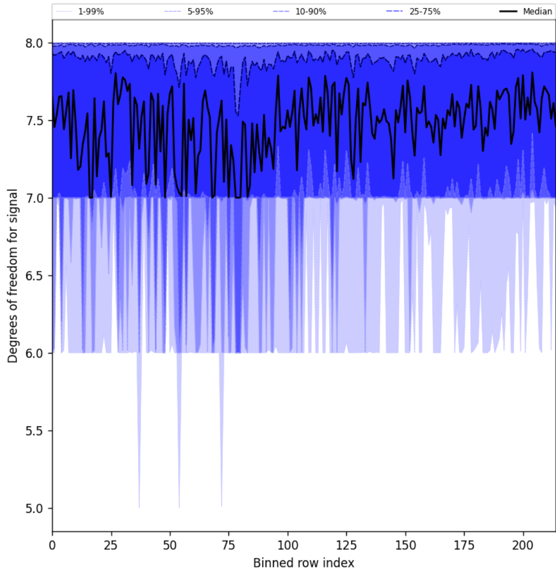
Figure 31: Along track statistics of “Degrees of freedom for signal” for 2025-10-14 to 2025-10-16
