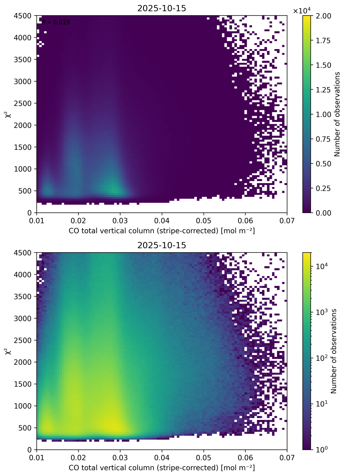
Figure 37: Scatter density plot of “CO total vertical column (stripe-corrected)” against “ \chi^2 ” for 2025-10-14 to 2025-10-16.
