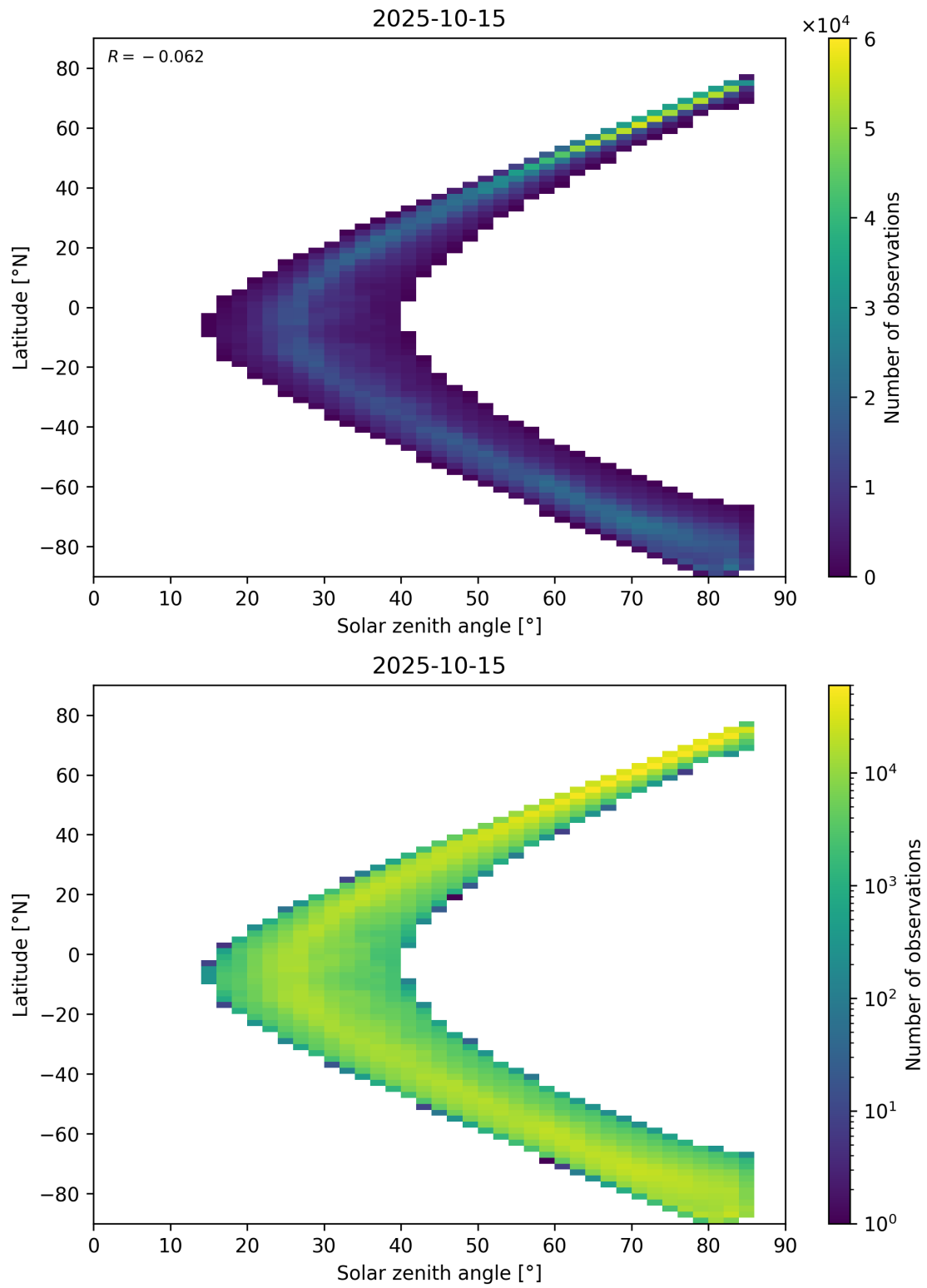
Figure 66: Scatter density plot of “Solar zenith angle” against “Latitude” for 2025-10-14 to 2025-10-16.
