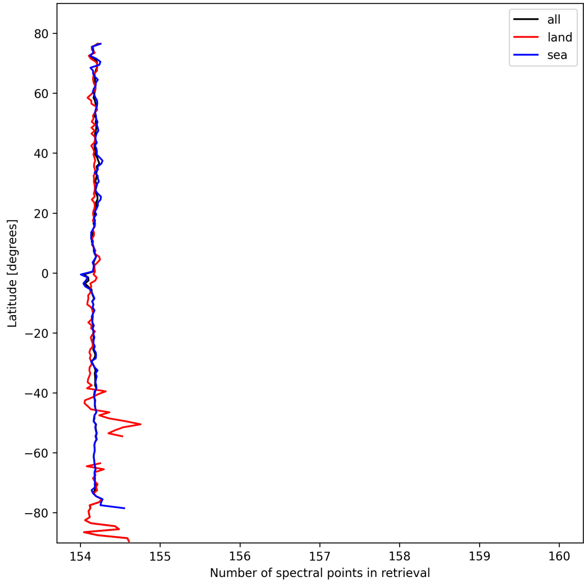
Figure 13: Zonal average of “Number of spectral points in retrieval” for 2025-10-14 to 2025-10-16.
