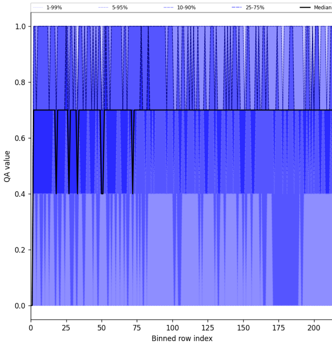
Figure 25: Along track statistics of “QA value” for 2025-10-14 to 2025-10-16
