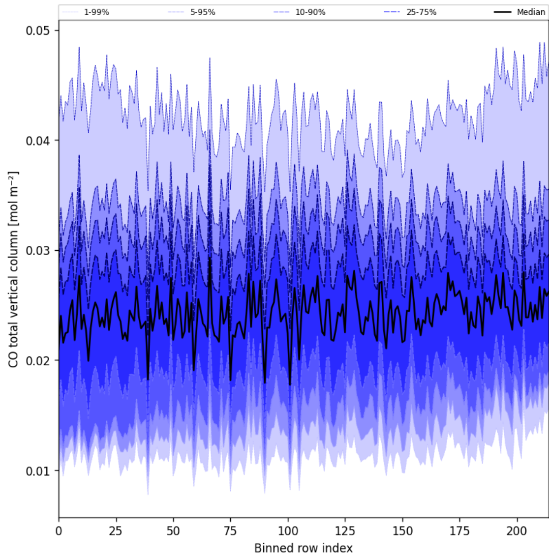
Figure 26: Along track statistics of “CO total vertical column” for 2025-10-14 to 2025-10-16
