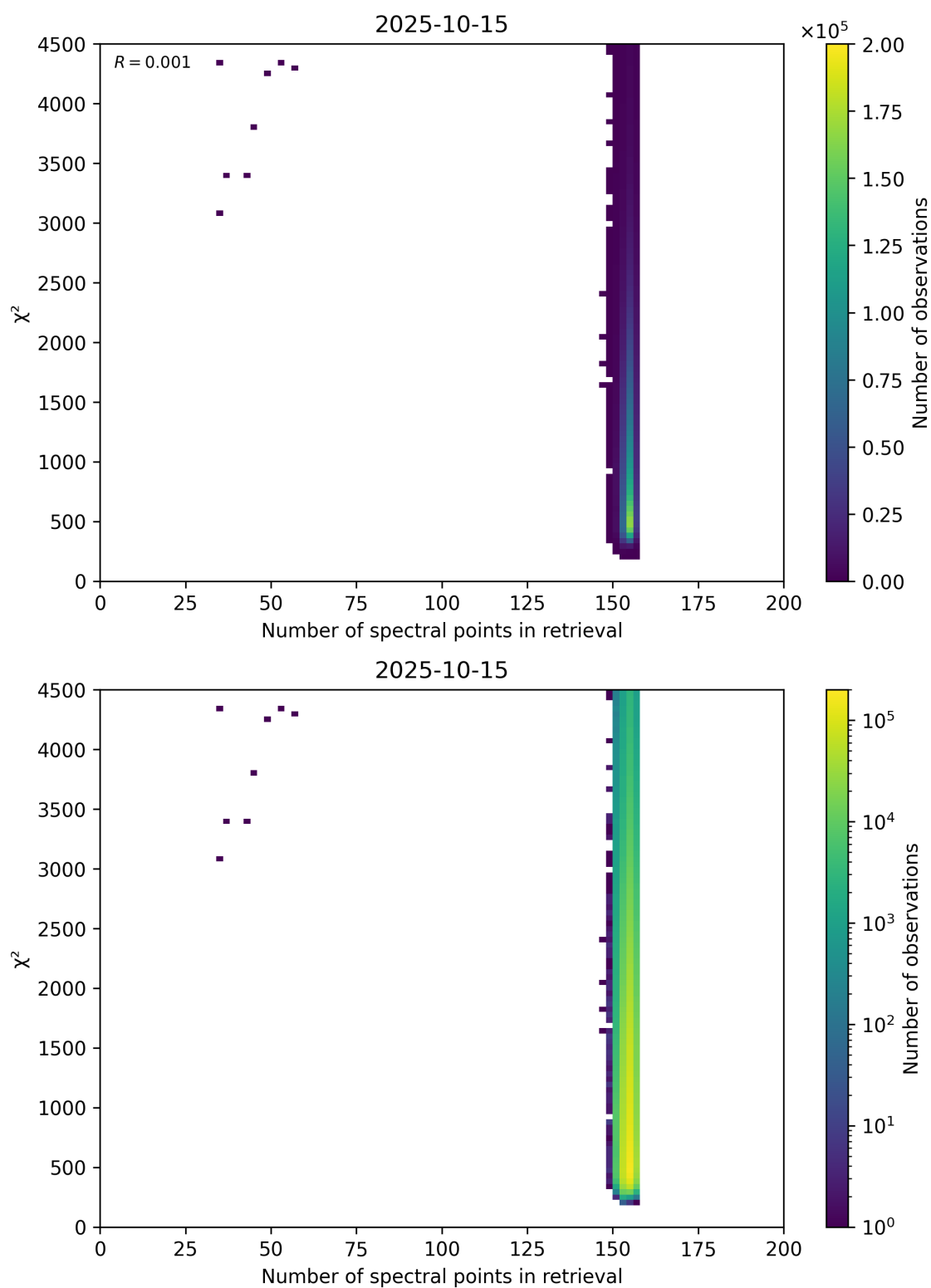
Figure 58: Scatter density plot of “Number of spectral points in retrieval” against “ \chi^2 ” for 2025-10-14 to 2025-10-16.
