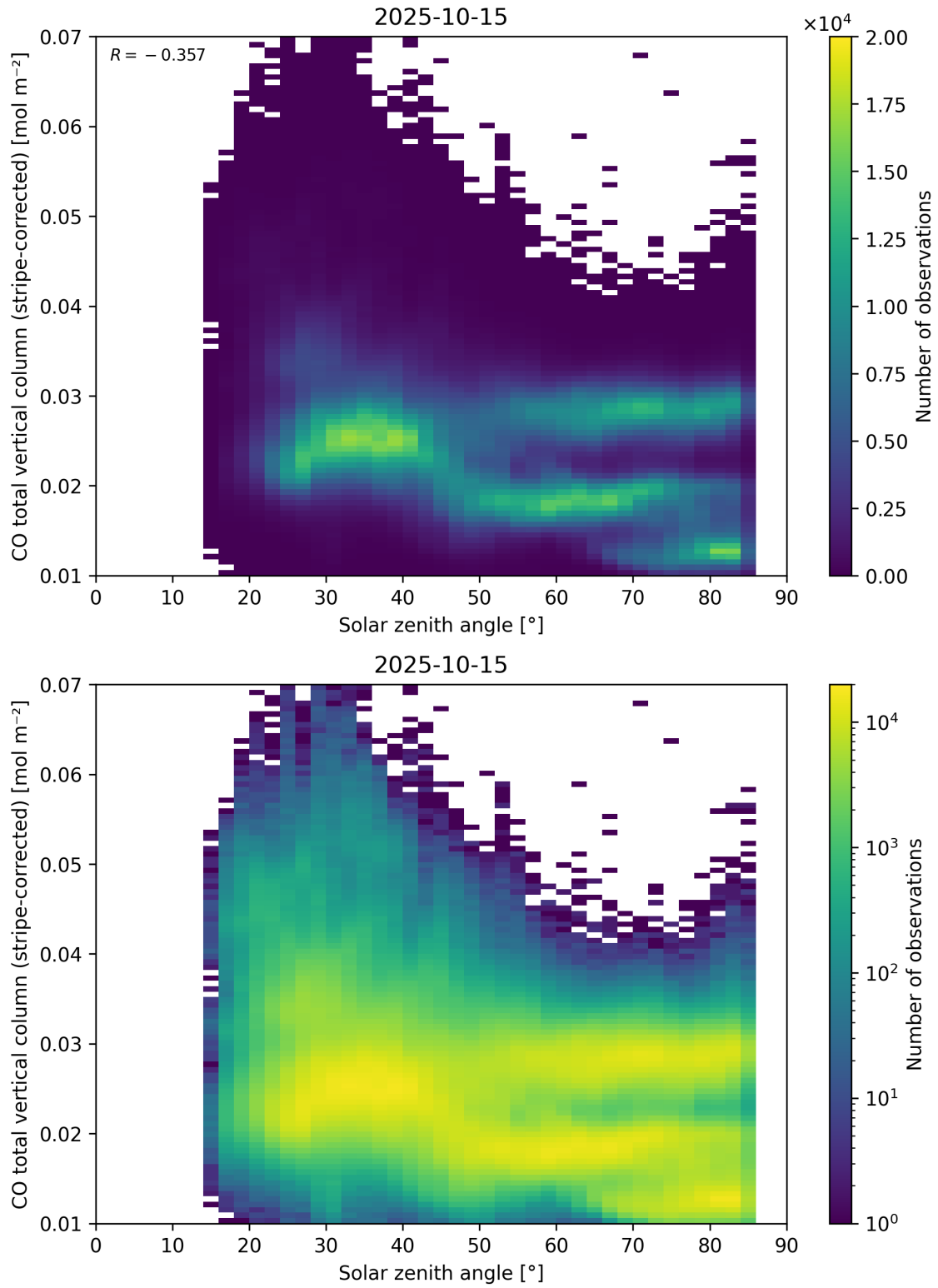
Figure 62: Scatter density plot of “Solar zenith angle” against “CO total vertical column (stripe-corrected)” for 2025-10-14 to 2025-10-16.
