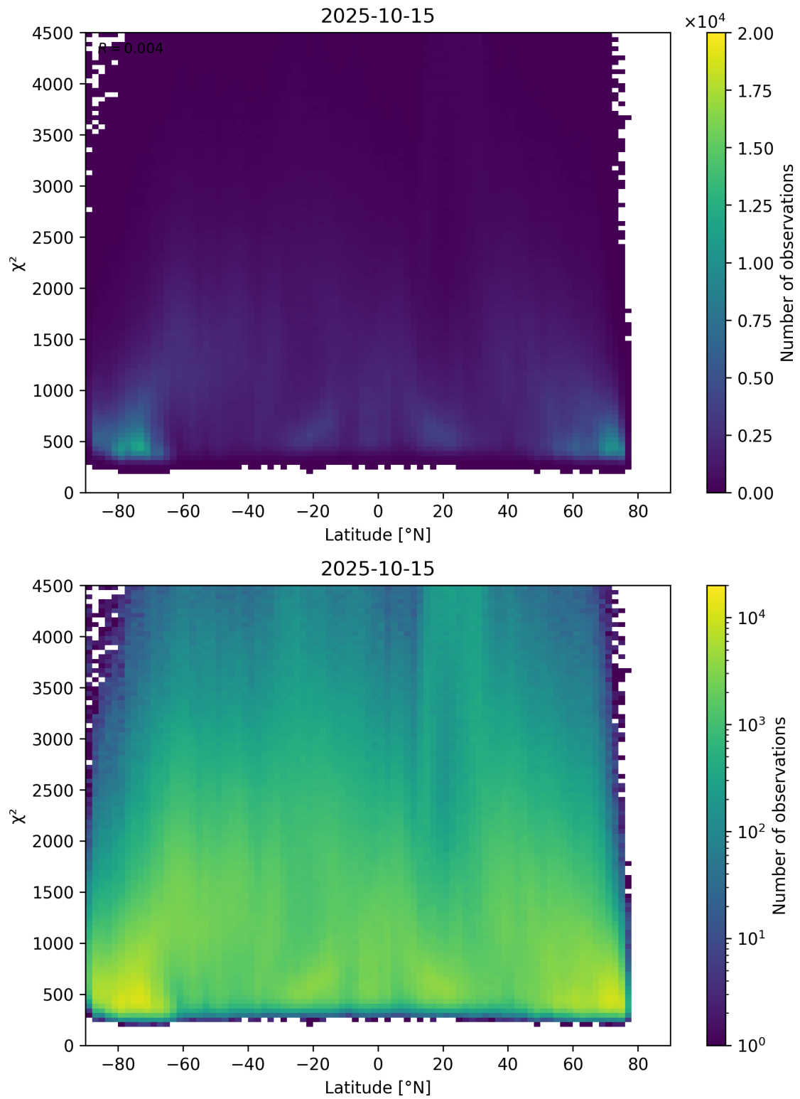
Figure 54: Scatter density plot of “Latitude” against “ \chi^2 ” for 2025-10-14 to 2025-10-16.
