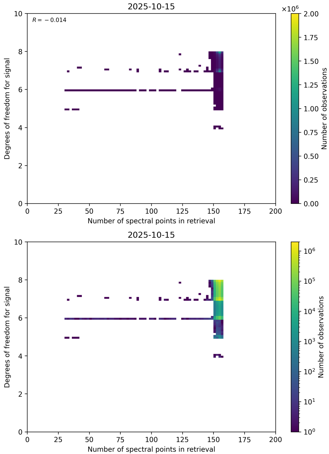
Figure 59: Scatter density plot of “Number of spectral points in retrieval” against “Degrees of freedom for signal” for 2025-10-14 to 2025-10-16.
