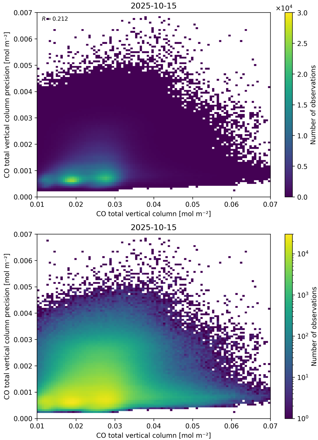
Figure 34: Scatter density plot of “CO total vertical column” against “CO total vertical column precision” for 2025-10-14 to 2025-10-16.
