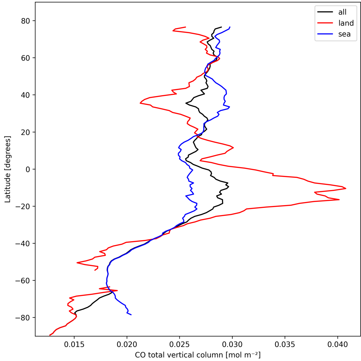
Figure 10: Zonal average of “CO total vertical column” for 2025-10-14 to 2025-10-16.
