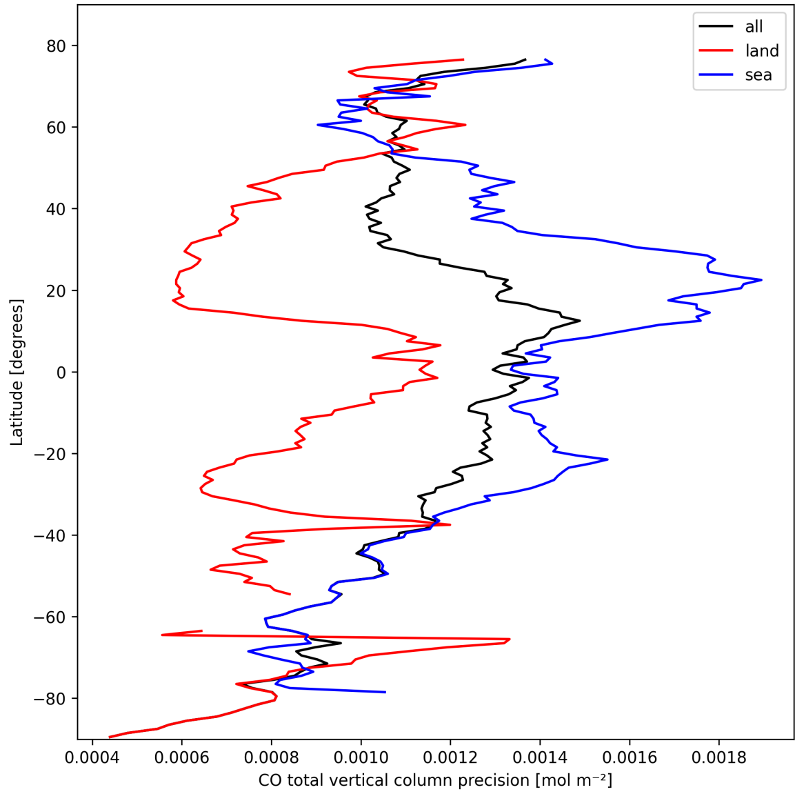
Figure 12: Zonal average of “CO total vertical column precision” for 2025-10-14 to 2025-10-16.
