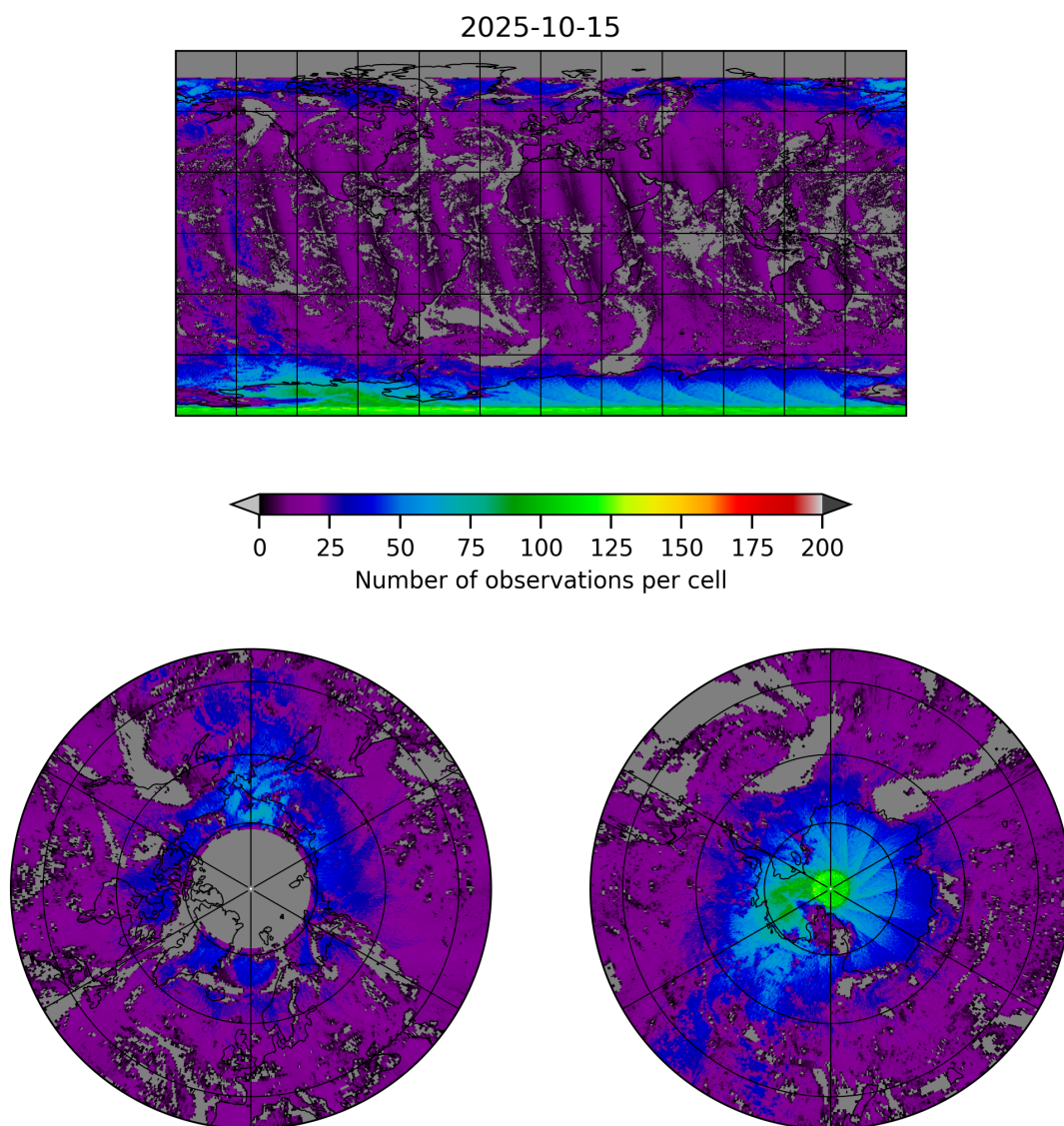
Figure 8: Map of the number of observations for 2025-10-14 to 2025-10-16
