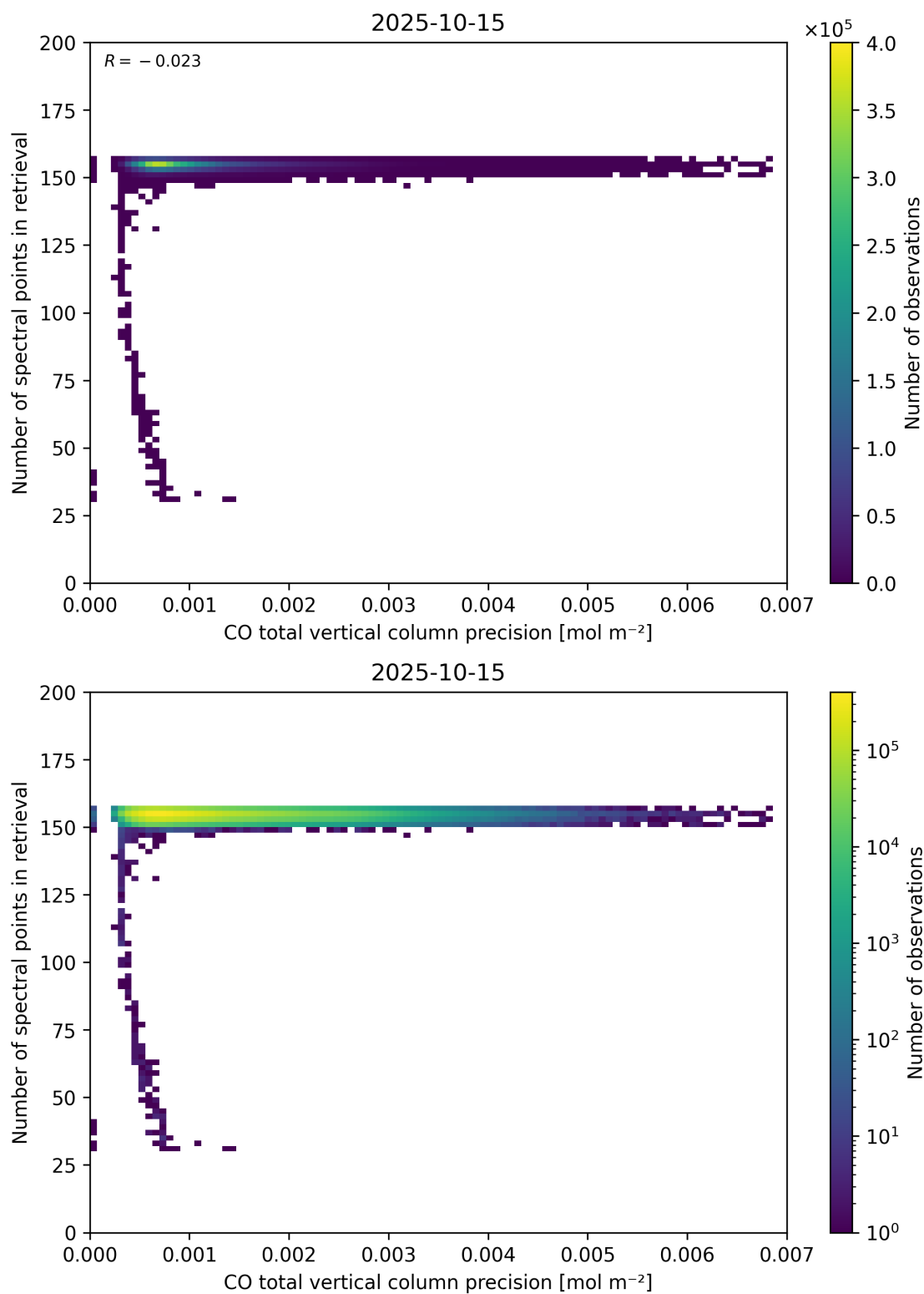
Figure 47: Scatter density plot of “CO total vertical column precision” against “Number of spectral points in retrieval” for 2025-10-14 to 2025-10-16.
