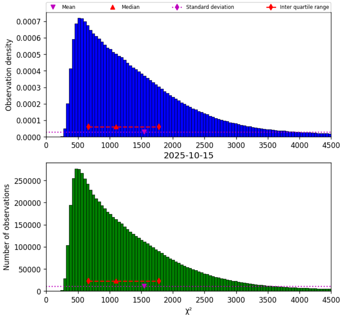
Figure 22: Histogram of “ \chi^2 ” for 2025-10-14 to 2025-10-16
