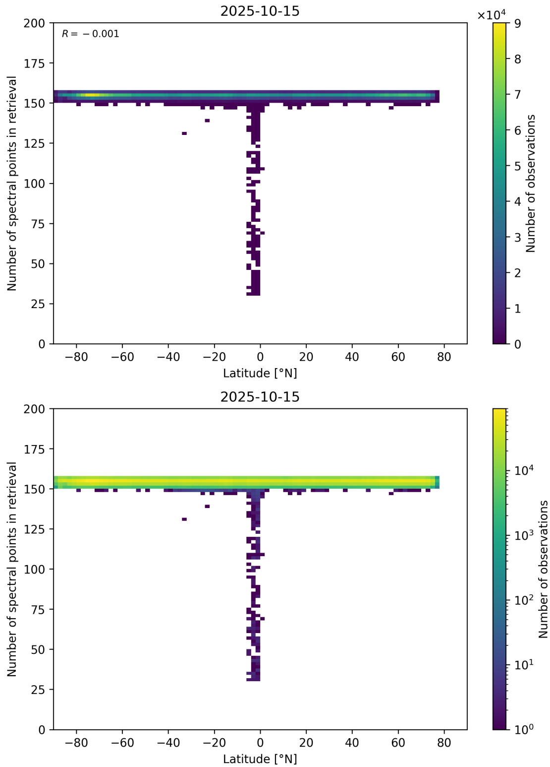
Figure 57: Scatter density plot of “Latitude” against “Number of spectral points in retrieval” for 2025-10-14 to 2025-10-16.
