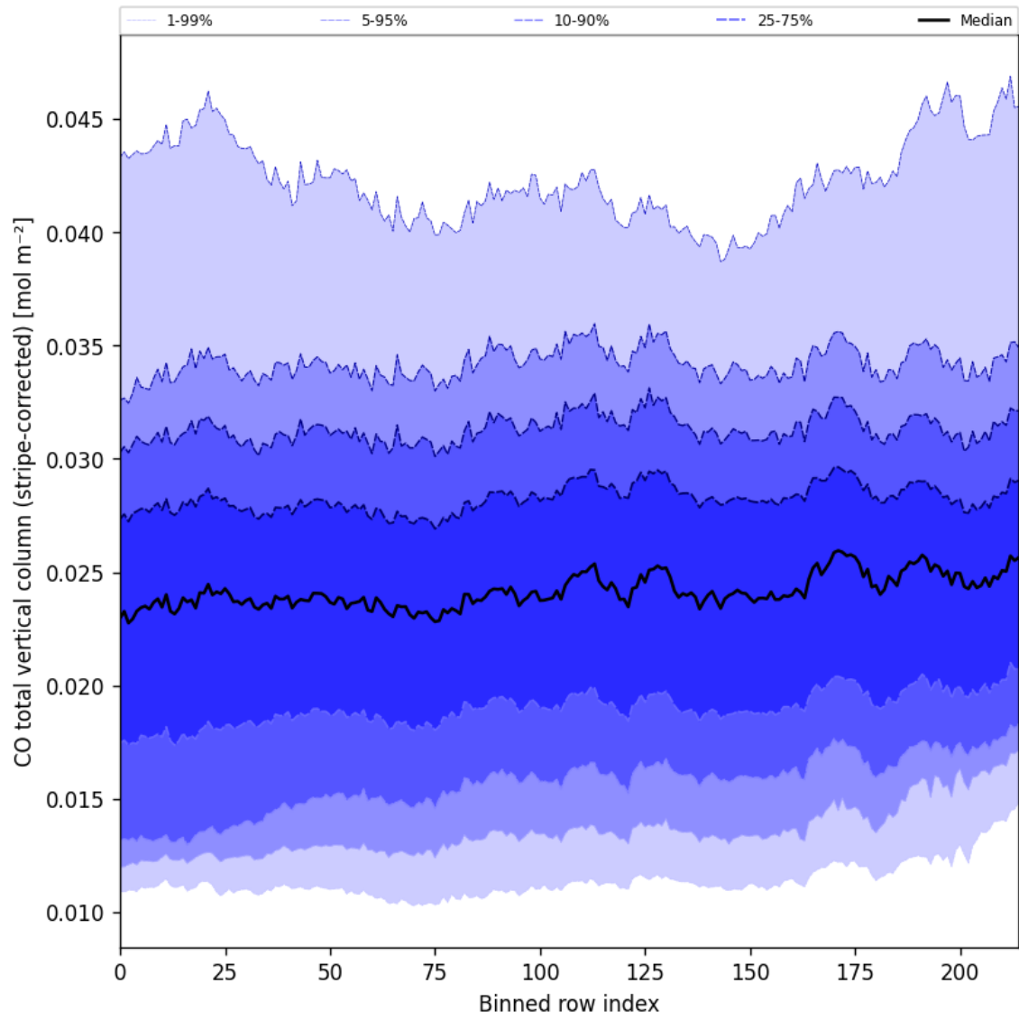
Figure 27: Along track statistics of “CO total vertical column (stripe-corrected)” for 2025-10-14 to 2025-10-16
