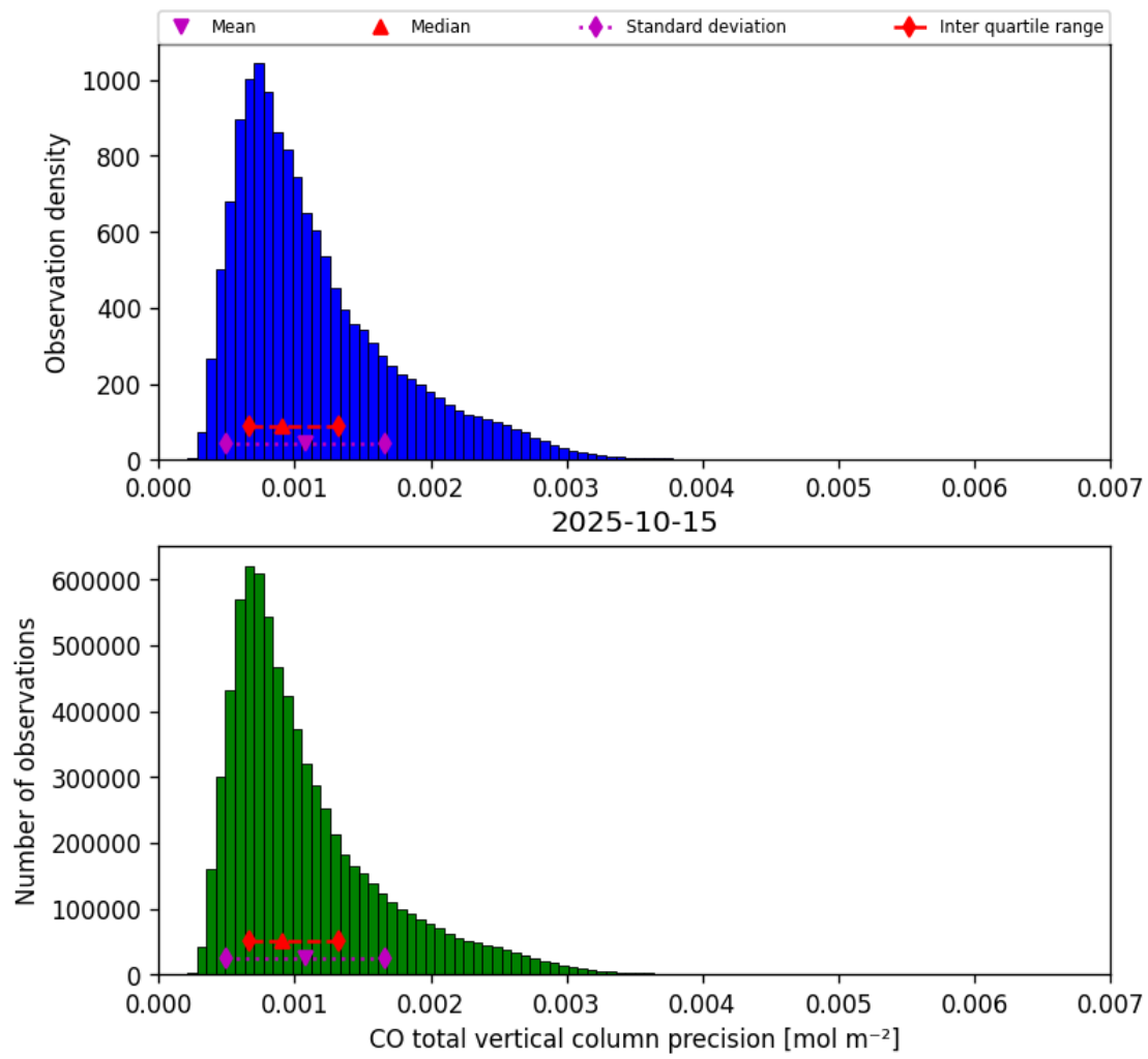
Figure 20: Histogram of “CO total vertical column precision” for 2025-10-14 to 2025-10-16
