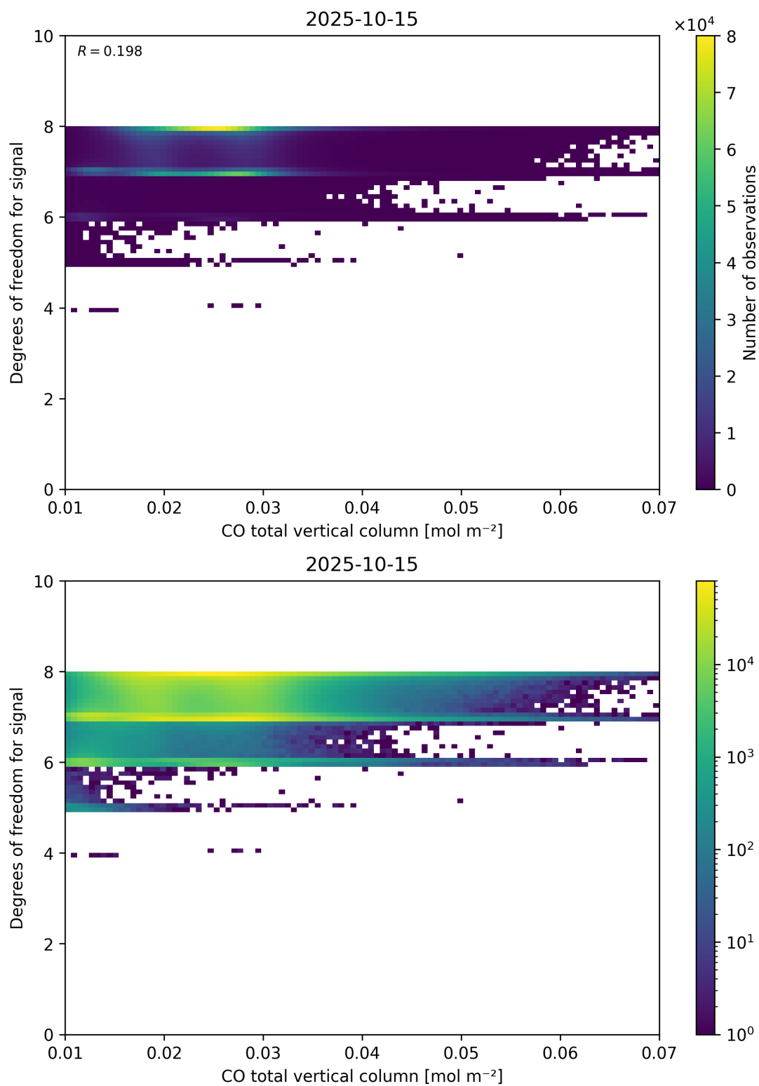
Figure 41: Scatter density plot of “CO total vertical column” against “Degrees of freedom for signal” for 2025-10-14 to 2025-10-16.
