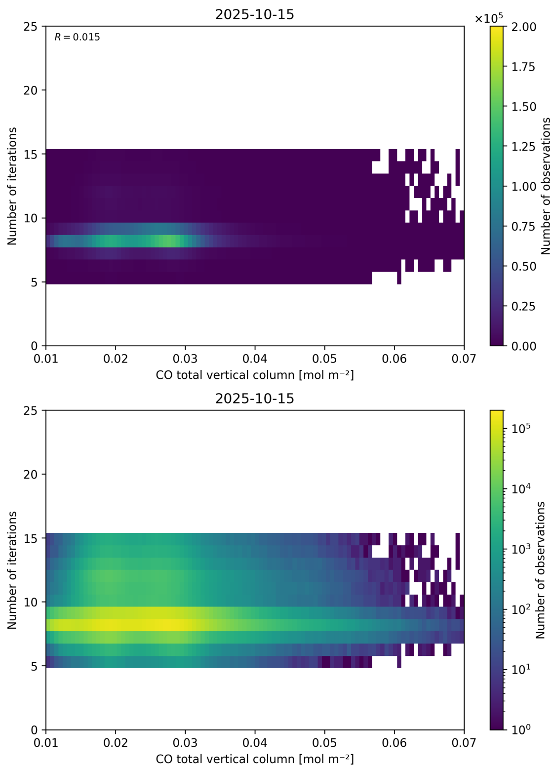
Figure 42: Scatter density plot of “CO total vertical column” against “Number of iterations” for 2025-10-14 to 2025-10-16.
