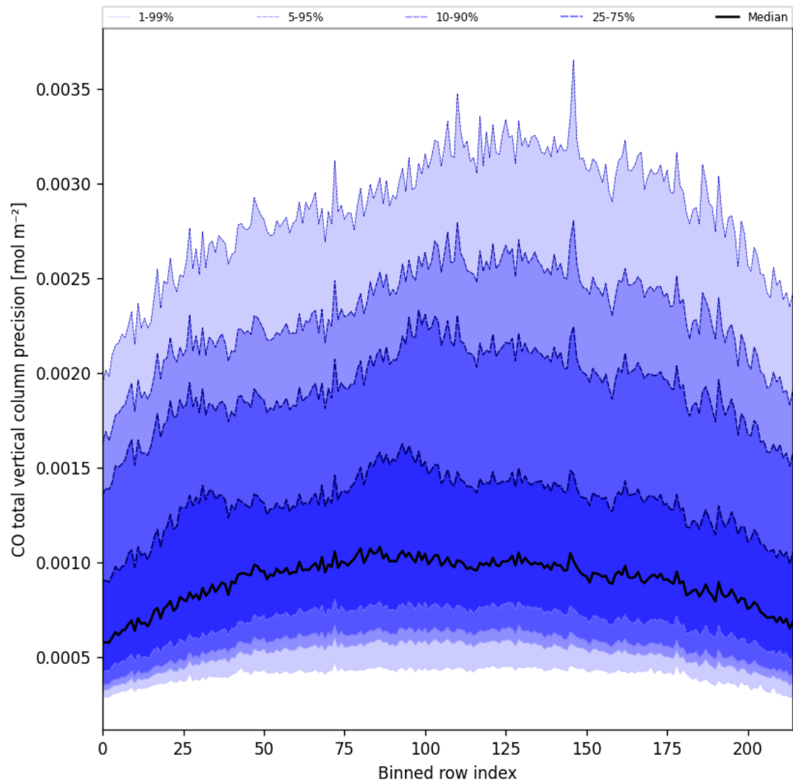
Figure 28: Along track statistics of “CO total vertical column precision” for 2025-10-14 to 2025-10-16
