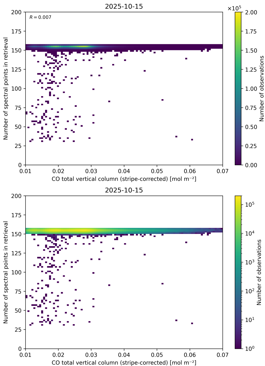
Figure 40: Scatter density plot of “CO total vertical column (stripe-corrected)” against “Number of spectral points in retrieval” for 2025-10-14 to 2025-10-16.
