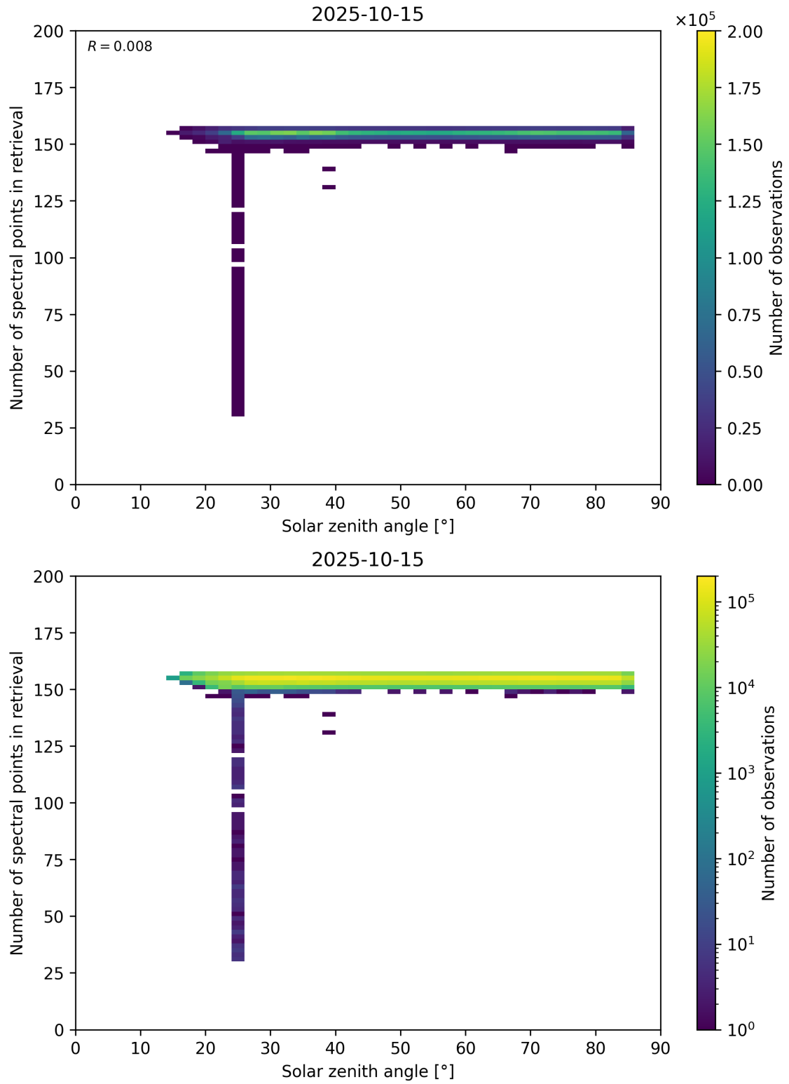
Figure 68: Scatter density plot of “Solar zenith angle” against “Number of spectral points in retrieval” for 2025-10-14 to 2025-10-16.
