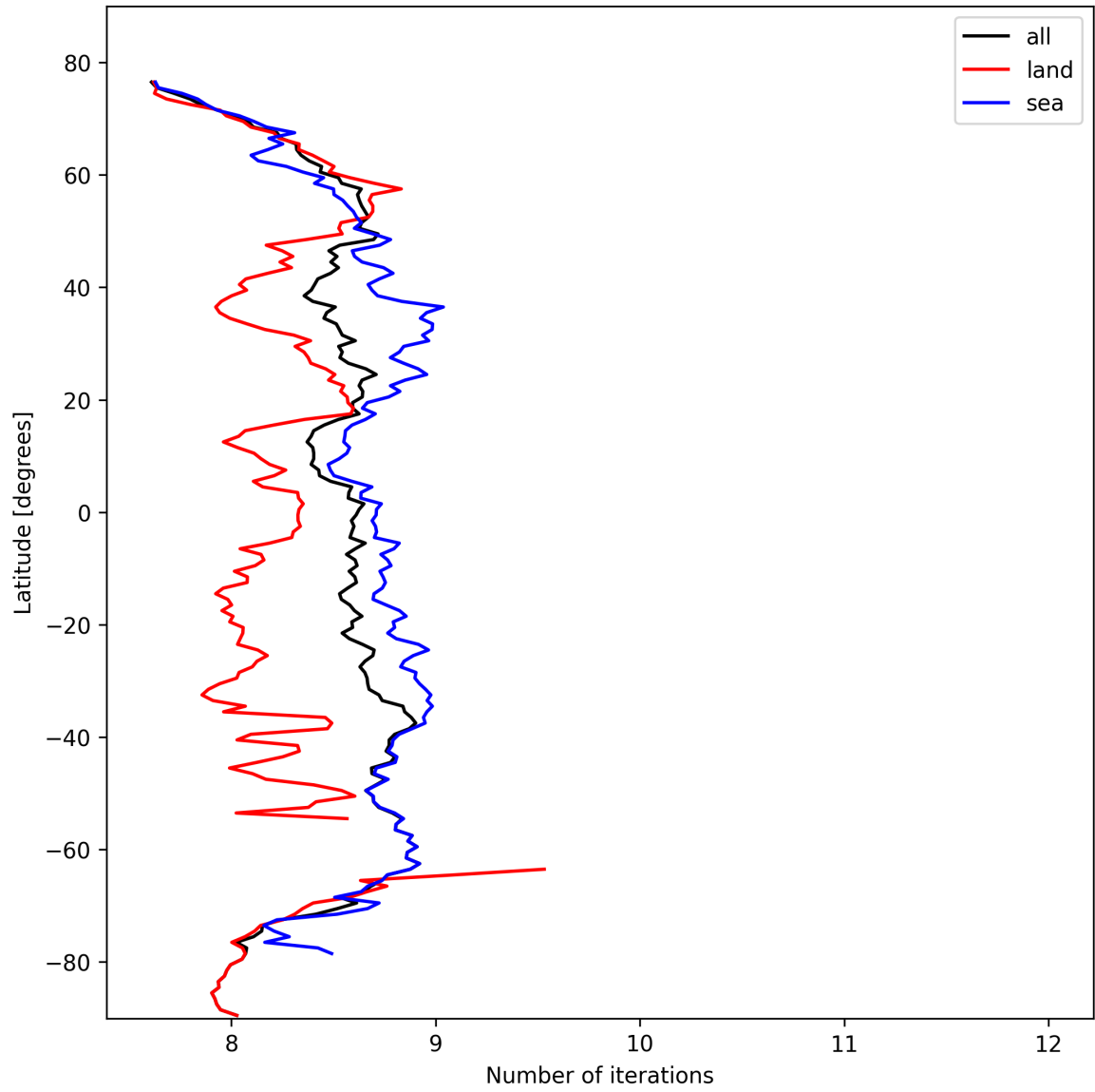
Figure 16: Zonal average of “Number of iterations” for 2025-10-14 to 2025-10-16.
