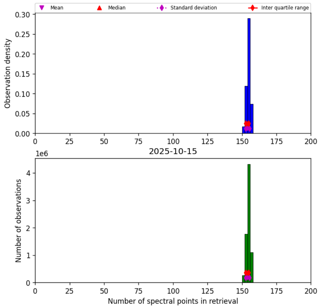
Figure 21: Histogram of “Number of spectral points in retrieval” for 2025-10-14 to 2025-10-16
