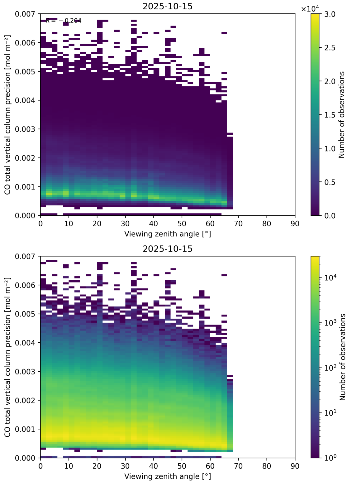
Figure 71: Scatter density plot of “Viewing zenith angle” against “CO total vertical column precision” for 2025-10-14 to 2025-10-16.
