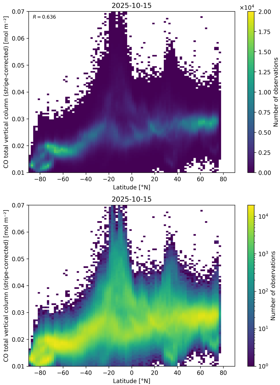
Figure 52: Scatter density plot of “Latitude” against “CO total vertical column (stripe-corrected)” for 2025-10-14 to 2025-10-16.
