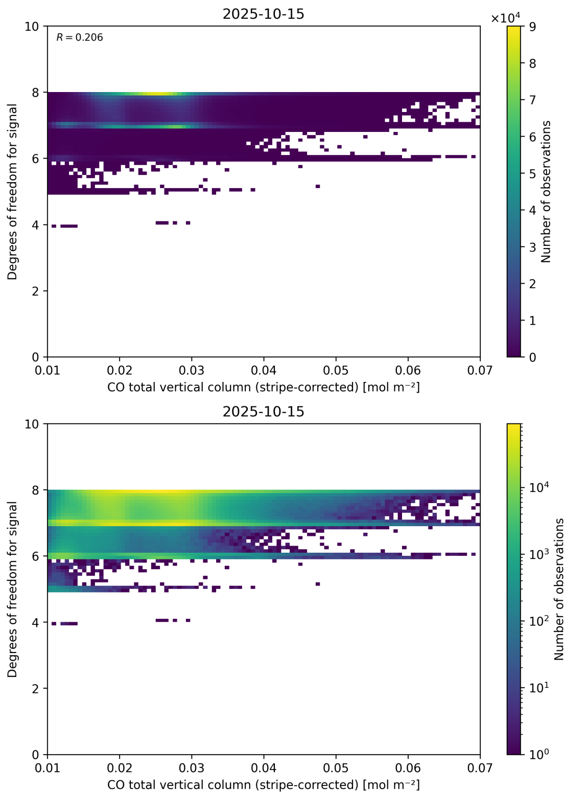
Figure 38: Scatter density plot of “CO total vertical column (stripe-corrected)” against “Degrees of freedom for signal” for 2025-10-14 to 2025-10-16.
