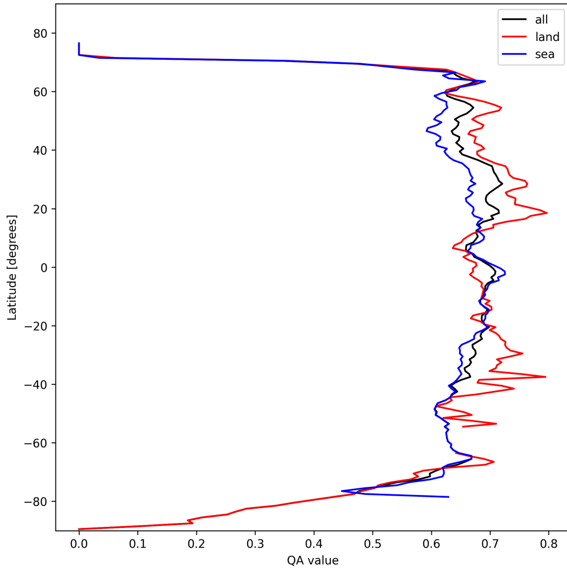
Figure 9: Zonal average of “QA value” for 2025-10-14 to 2025-10-16.
