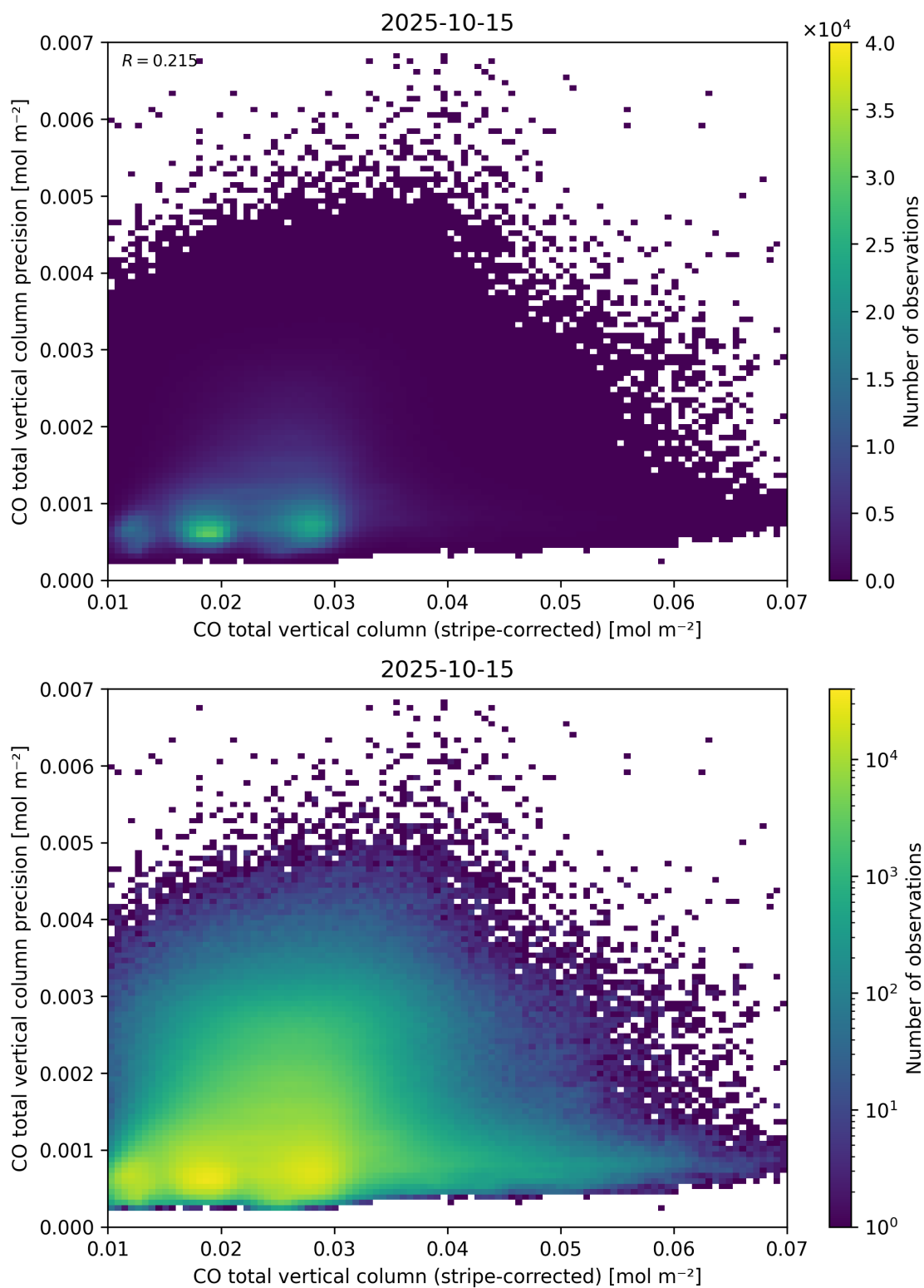
Figure 36: Scatter density plot of “CO total vertical column (stripe-corrected)” against “CO total vertical column precision” for 2025-10-14 to 2025-10-16.
