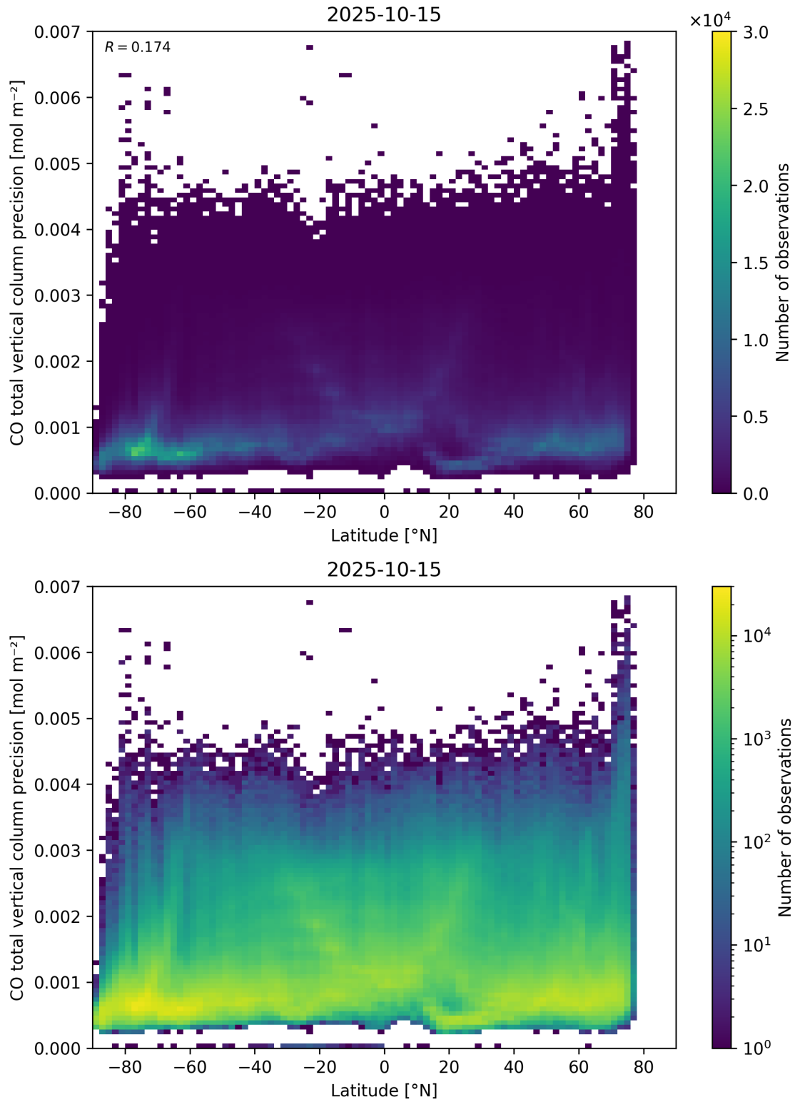
Figure 53: Scatter density plot of “Latitude” against “CO total vertical column precision” for 2025-10-14 to 2025-10-16.
