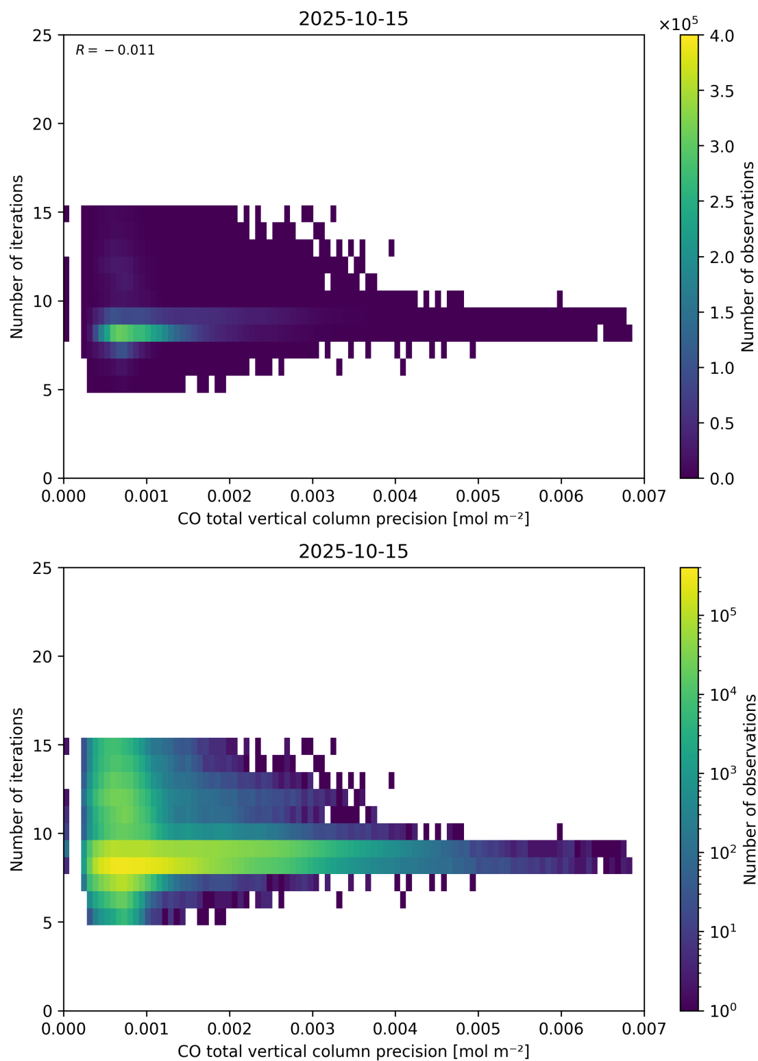
Figure 46: Scatter density plot of “CO total vertical column precision” against “Number of iterations” for 2025-10-14 to 2025-10-16.
