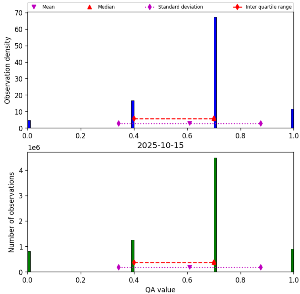
Figure 17: Histogram of “QA value” for 2025-10-14 to 2025-10-16
