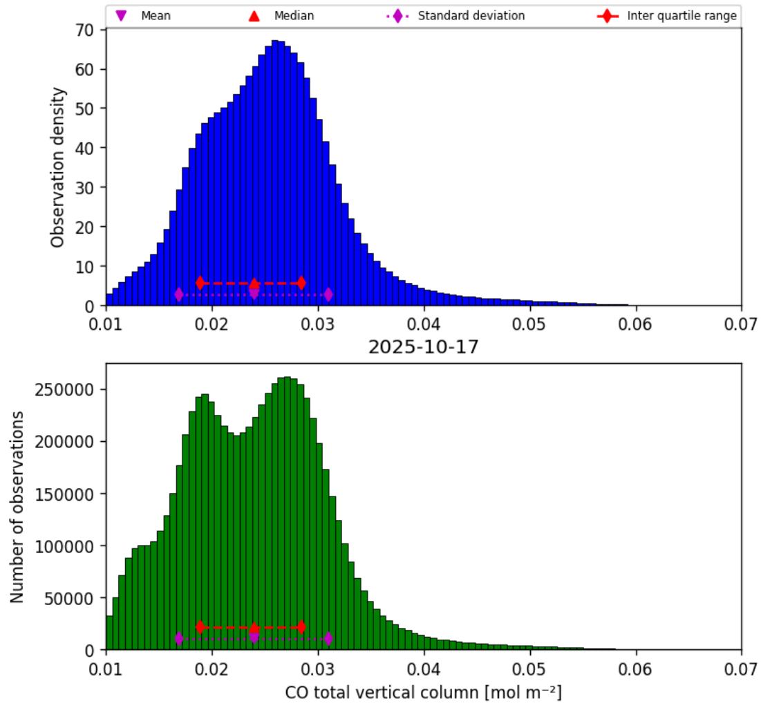
Figure 18: Histogram of “CO total vertical column” for 2025-10-17 to 2025-10-18
