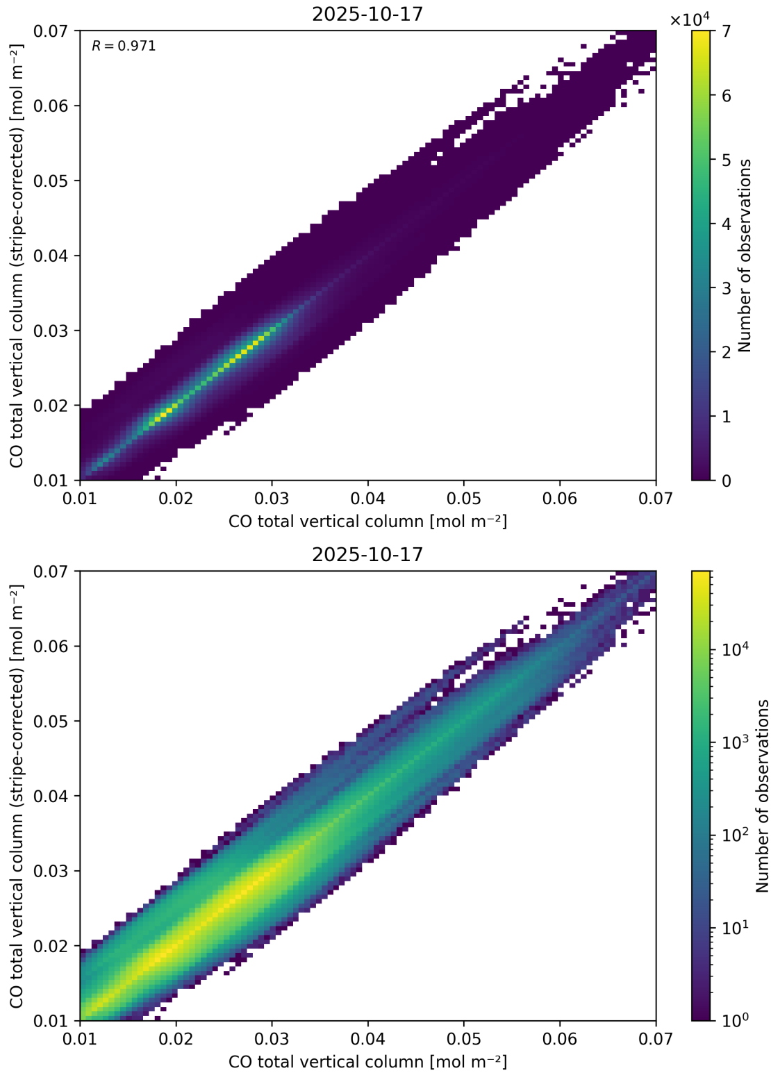
Figure 33: Scatter density plot of “CO total vertical column” against “CO total vertical column (stripe-corrected)” for 2025-10-17 to 2025-10-18.
