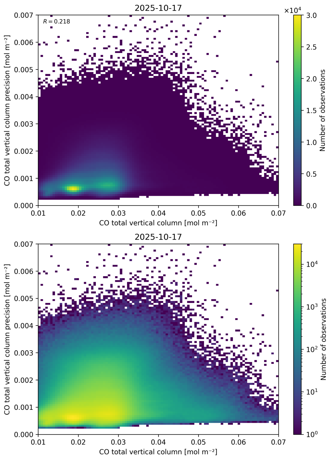
Figure 34: Scatter density plot of “CO total vertical column” against “CO total vertical column precision” for 2025-10-17 to 2025-10-18.
