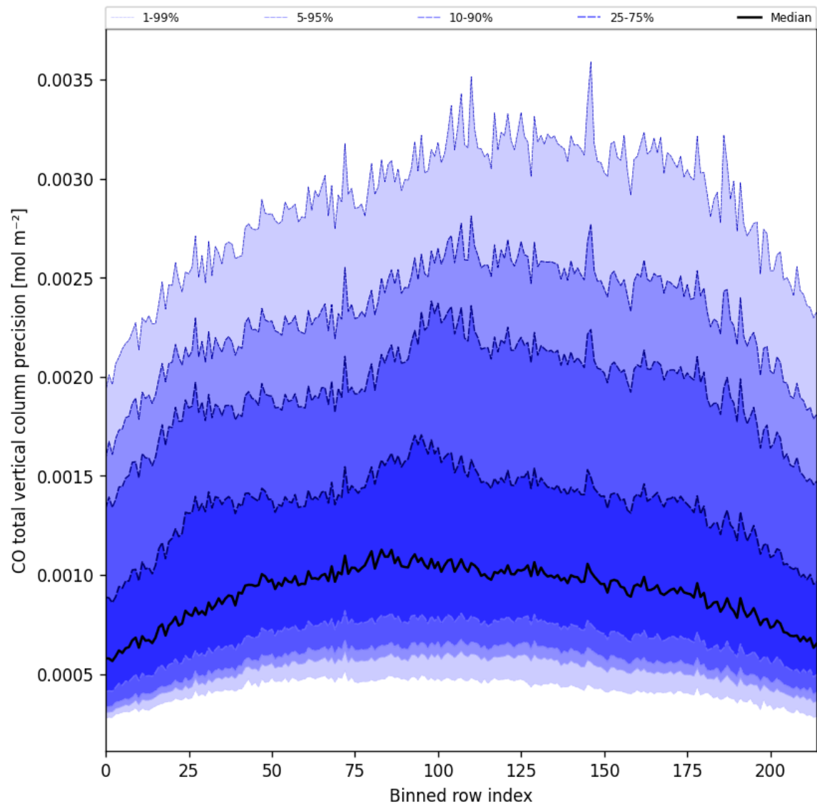
Figure 28: Along track statistics of “CO total vertical column precision” for 2025-10-17 to 2025-10-18
