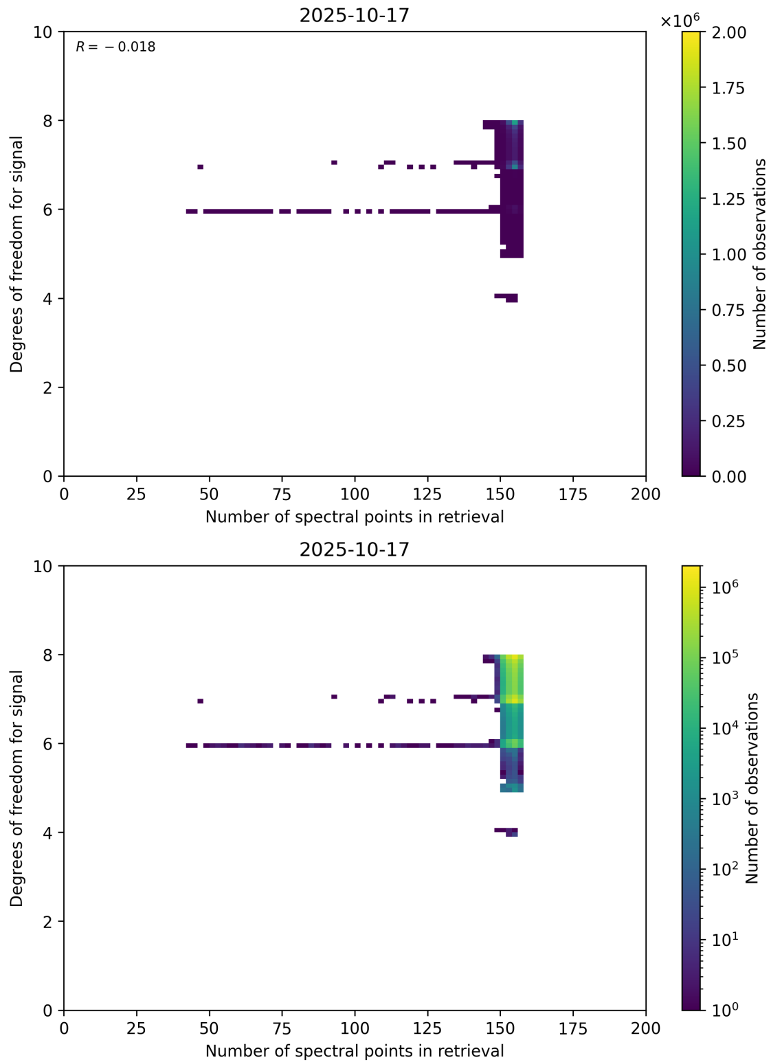
Figure 59: Scatter density plot of “Number of spectral points in retrieval” against “Degrees of freedom for signal” for 2025-10-17 to 2025-10-18.
