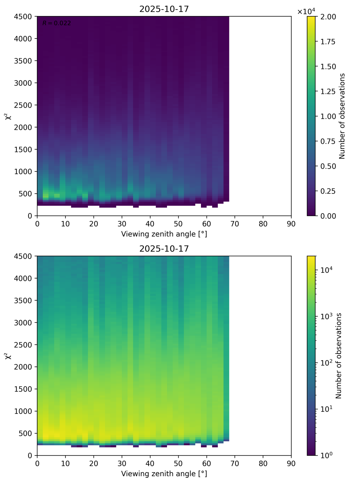
Figure 72: Scatter density plot of “Viewing zenith angle” against “ \chi^2 ” for 2025-10-17 to 2025-10-18.
