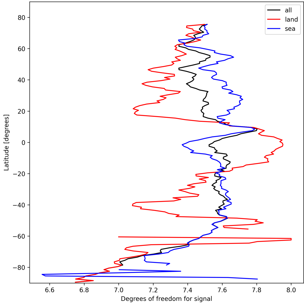
Figure 15: Zonal average of “Degrees of freedom for signal” for 2025-10-17 to 2025-10-18.
