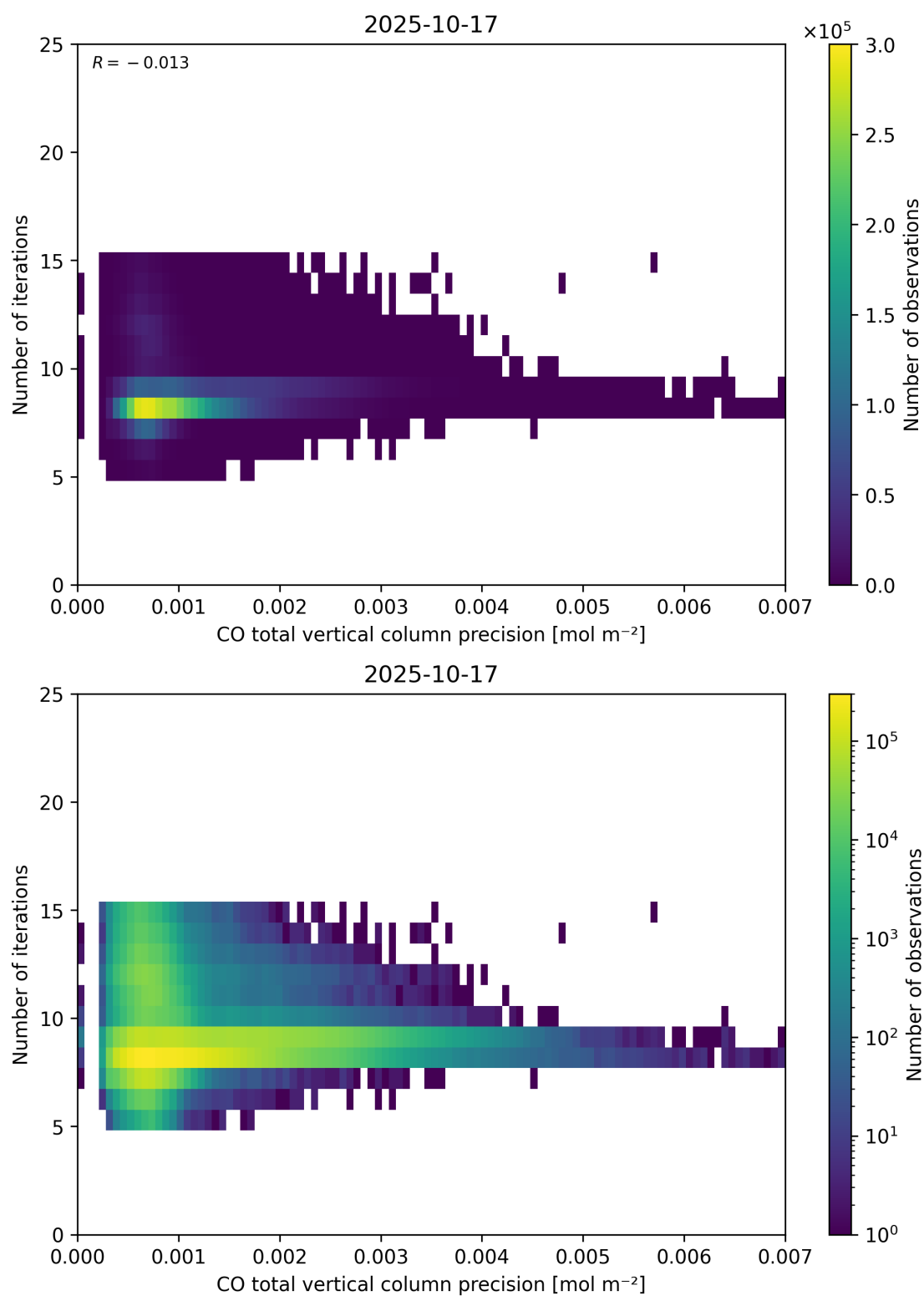
Figure 46: Scatter density plot of “CO total vertical column precision” against “Number of iterations” for 2025-10-17 to 2025-10-18.
