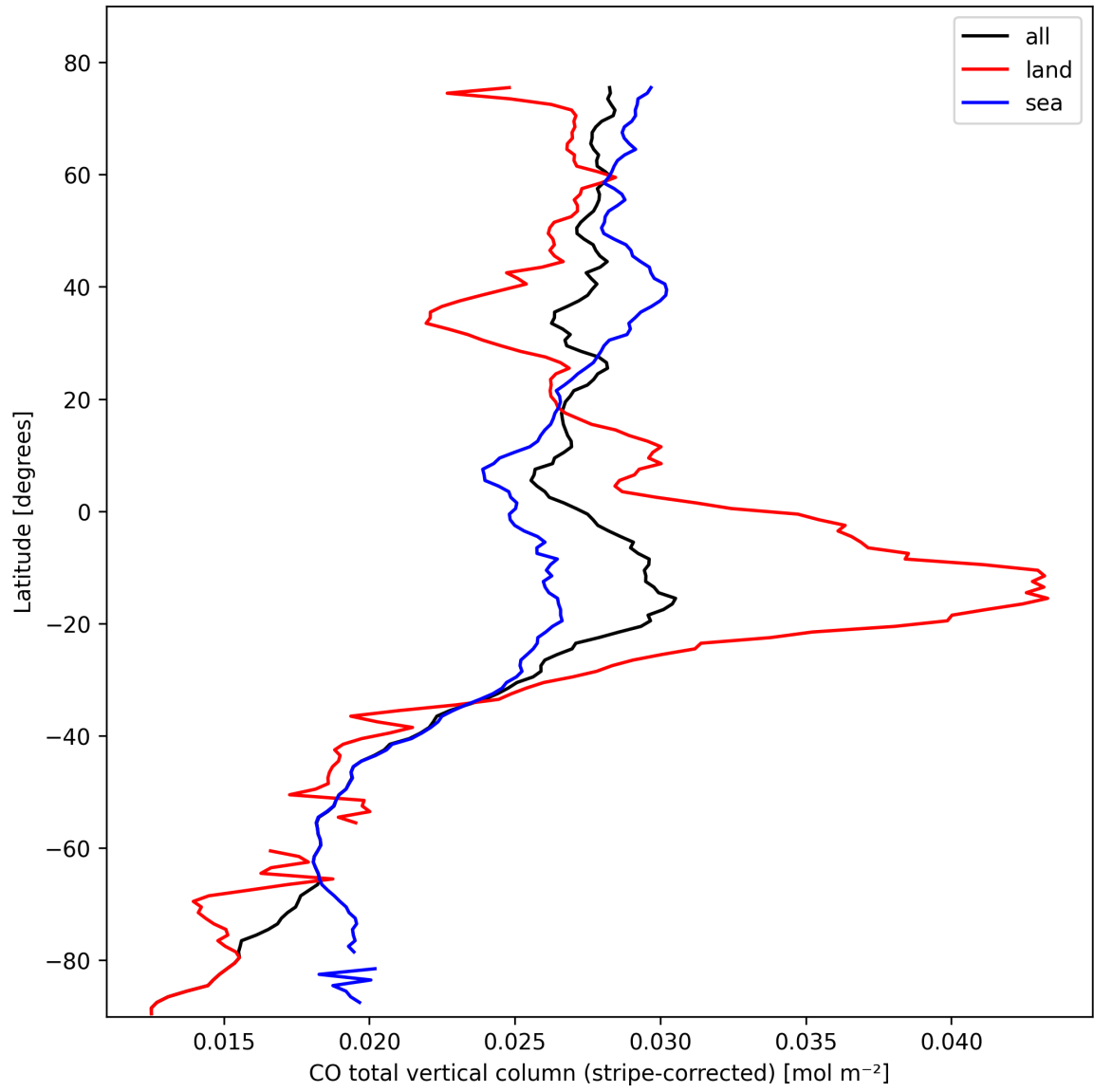
Figure 11: Zonal average of “CO total vertical column (stripe-corrected)” for 2025-10-17 to 2025-10-18.
