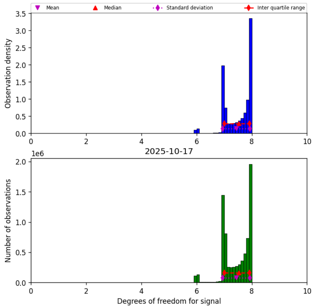
Figure 23: Histogram of “Degrees of freedom for signal” for 2025-10-17 to 2025-10-18
