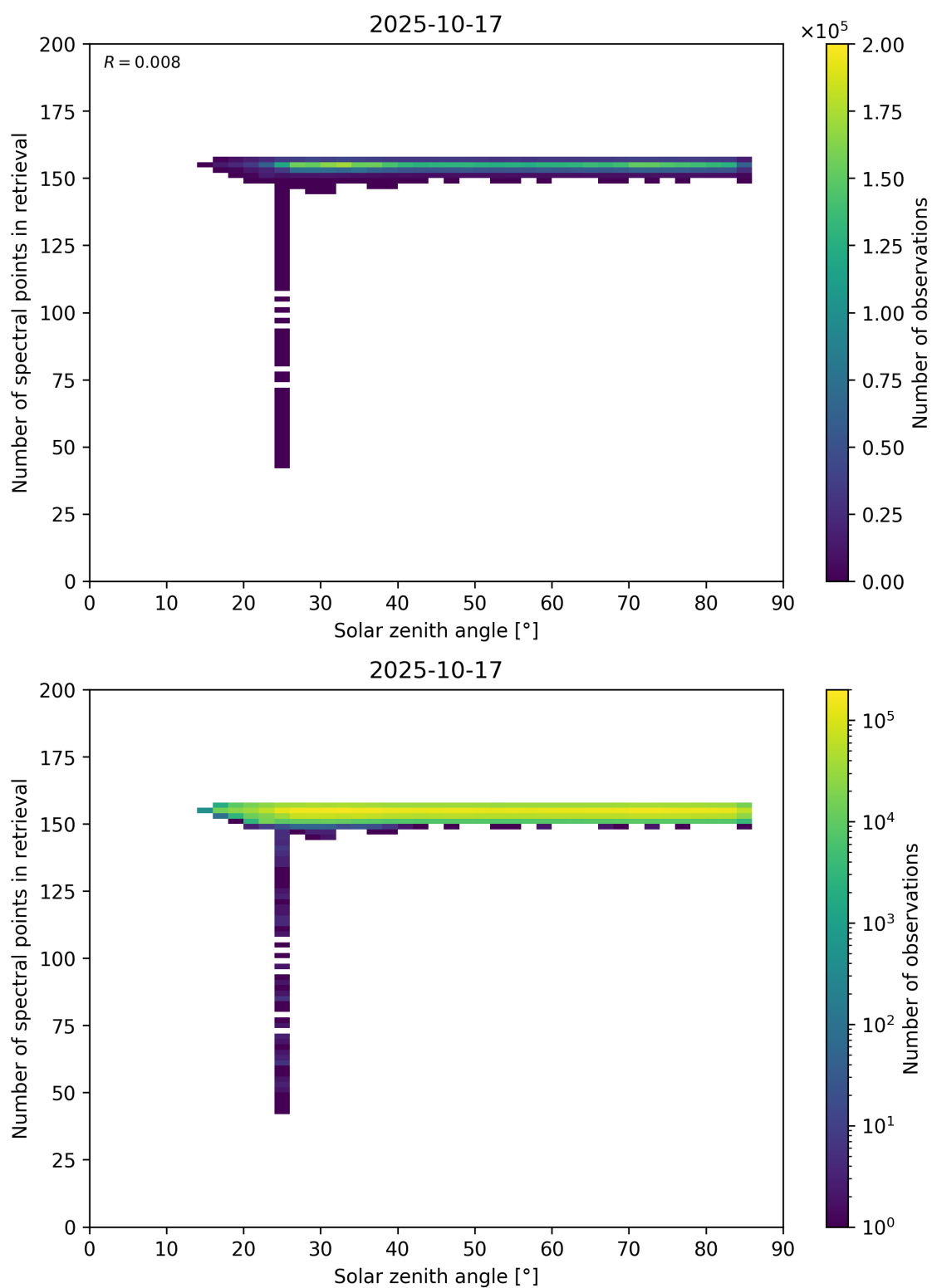
Figure 68: Scatter density plot of “Solar zenith angle” against “Number of spectral points in retrieval” for 2025-10-17 to 2025-10-18.
