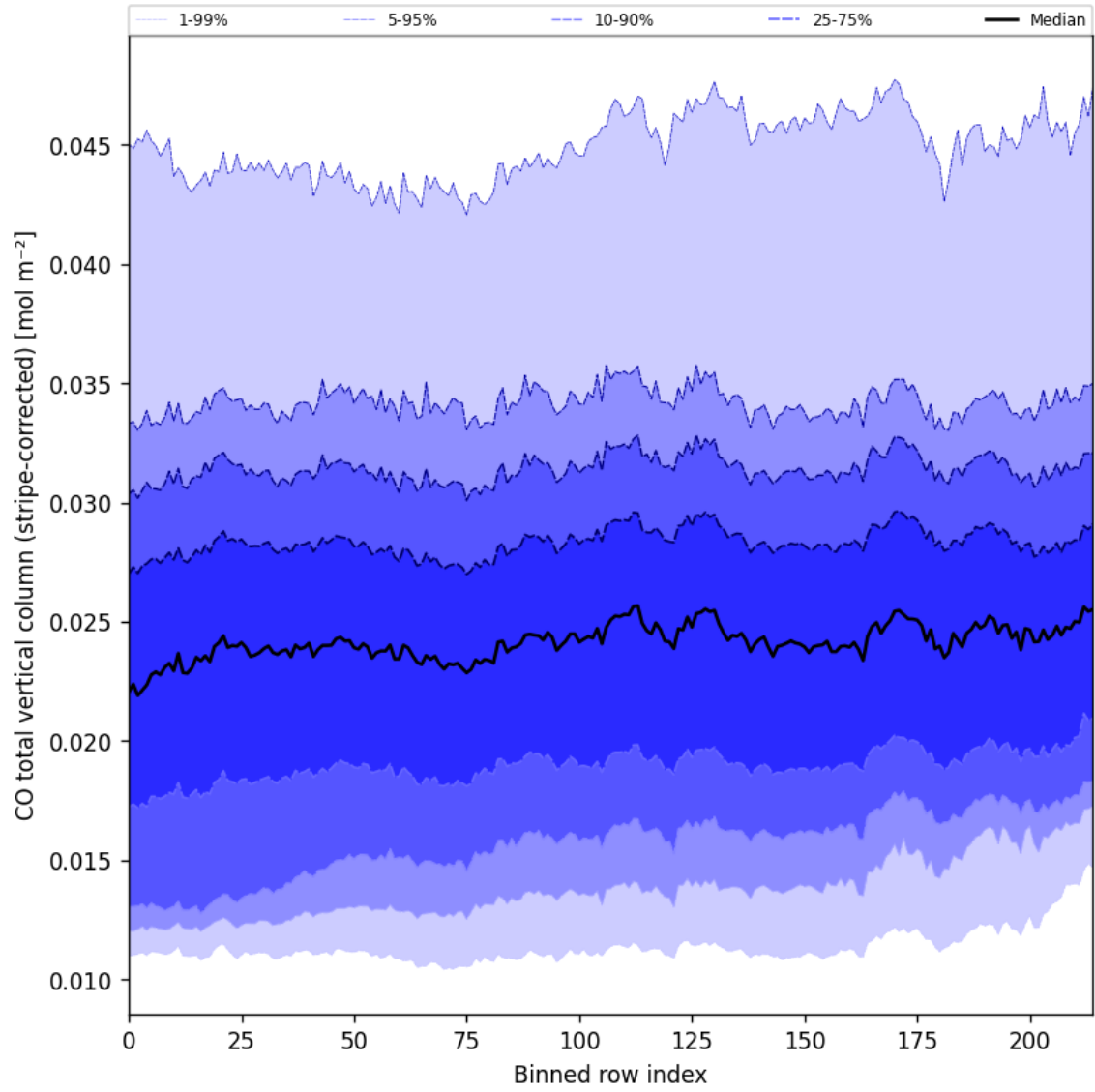
Figure 27: Along track statistics of “CO total vertical column (stripe-corrected)” for 2025-10-17 to 2025-10-18
