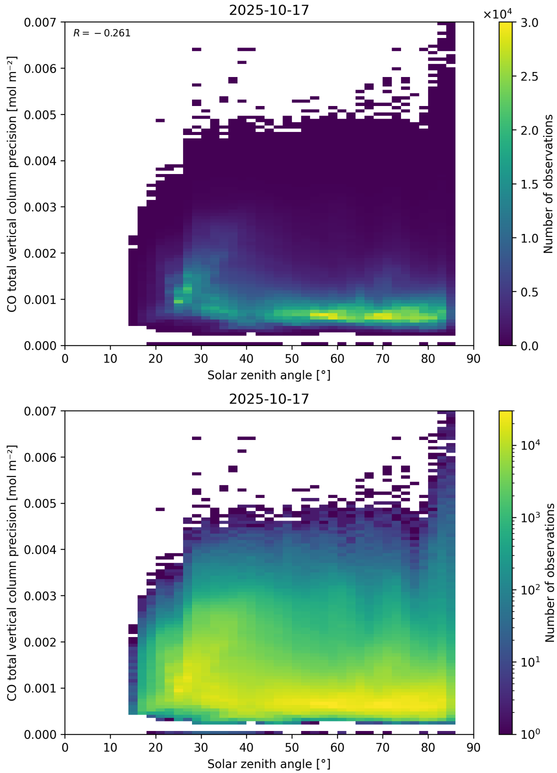
Figure 63: Scatter density plot of “Solar zenith angle” against “CO total vertical column precision” for 2025-10-17 to 2025-10-18.
