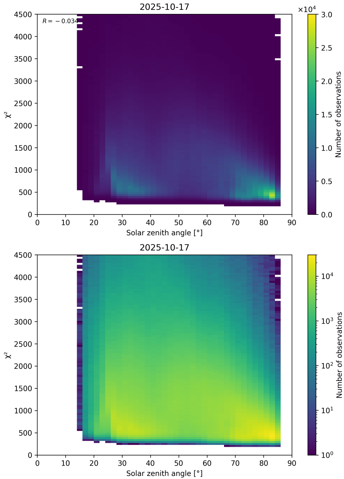
Figure 64: Scatter density plot of “Solar zenith angle” against “ \chi^2 ” for 2025-10-17 to 2025-10-18.
