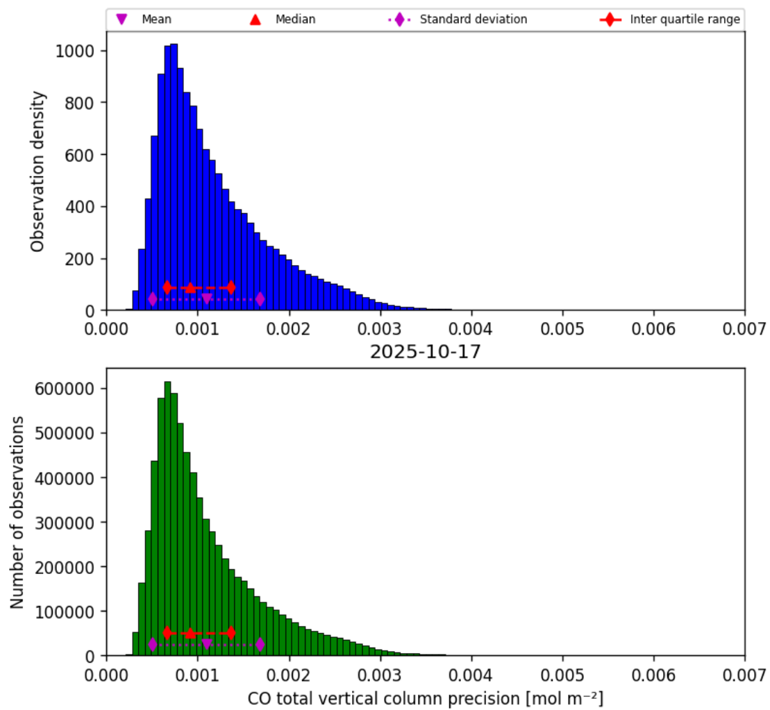
Figure 20: Histogram of “CO total vertical column precision” for 2025-10-17 to 2025-10-18
