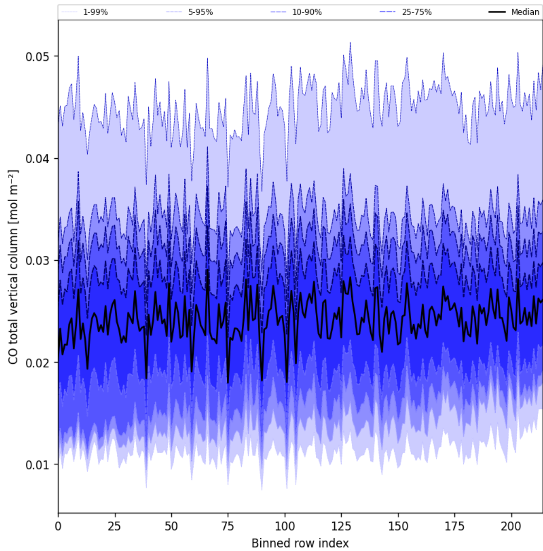
Figure 26: Along track statistics of “CO total vertical column” for 2025-10-17 to 2025-10-18
