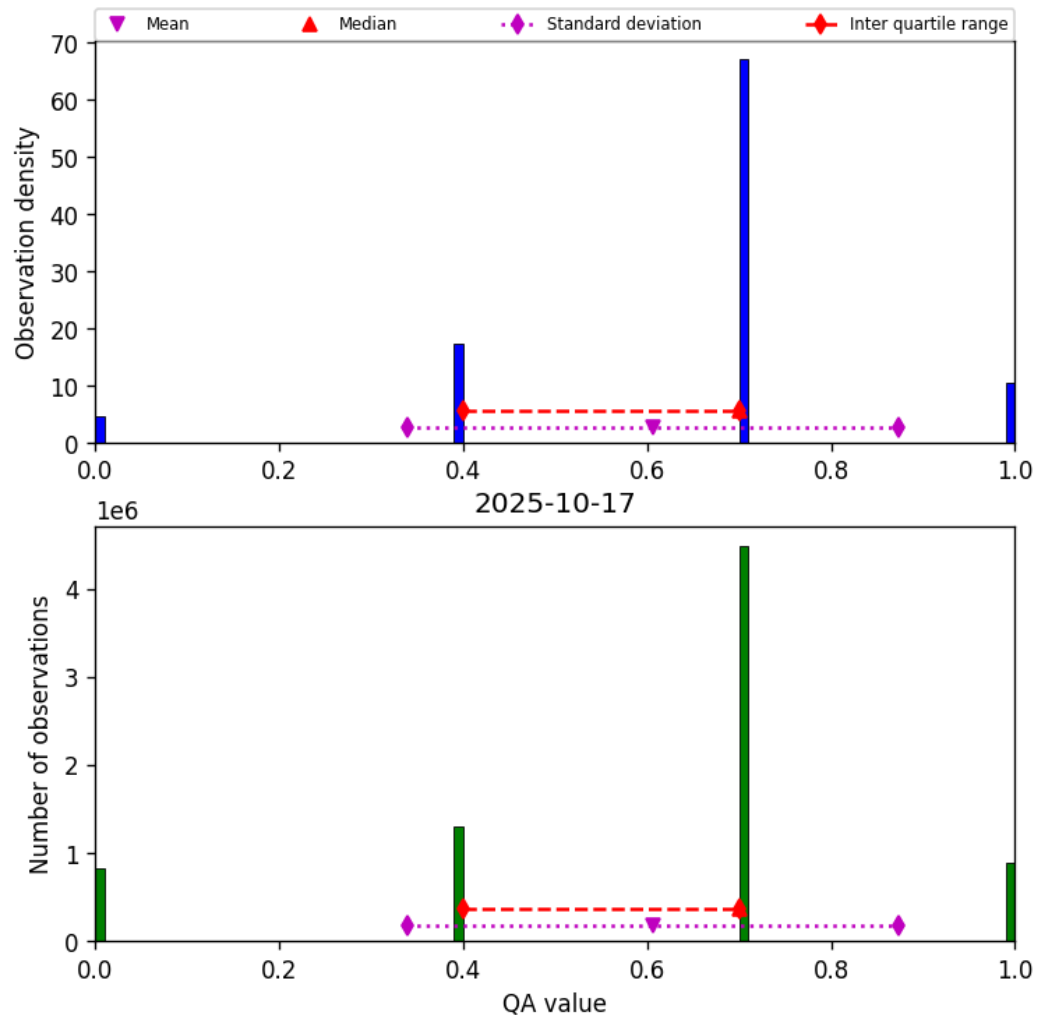
Figure 17: Histogram of “QA value” for 2025-10-17 to 2025-10-18
