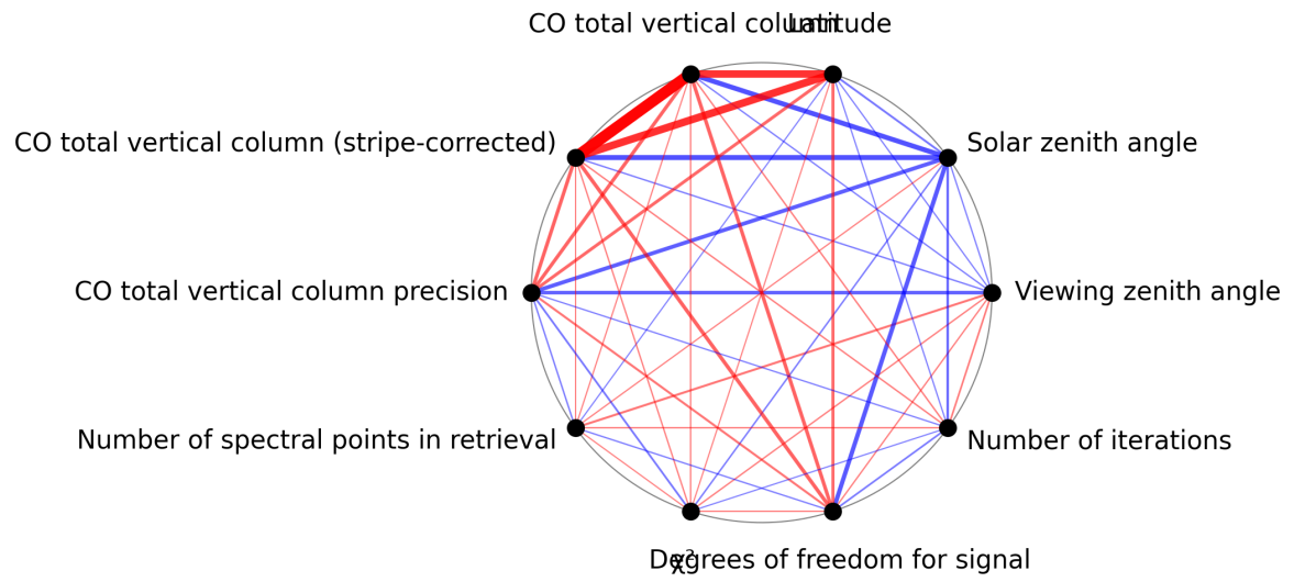
Figure 1: Map of correlation graph for 2025-10-17 to 2025-10-18.
