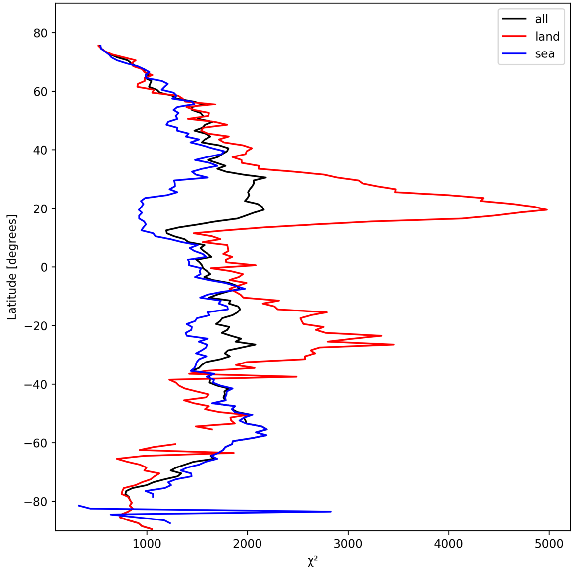
Figure 14: Zonal average of “ \chi^2 ” for 2025-10-17 to 2025-10-18.
