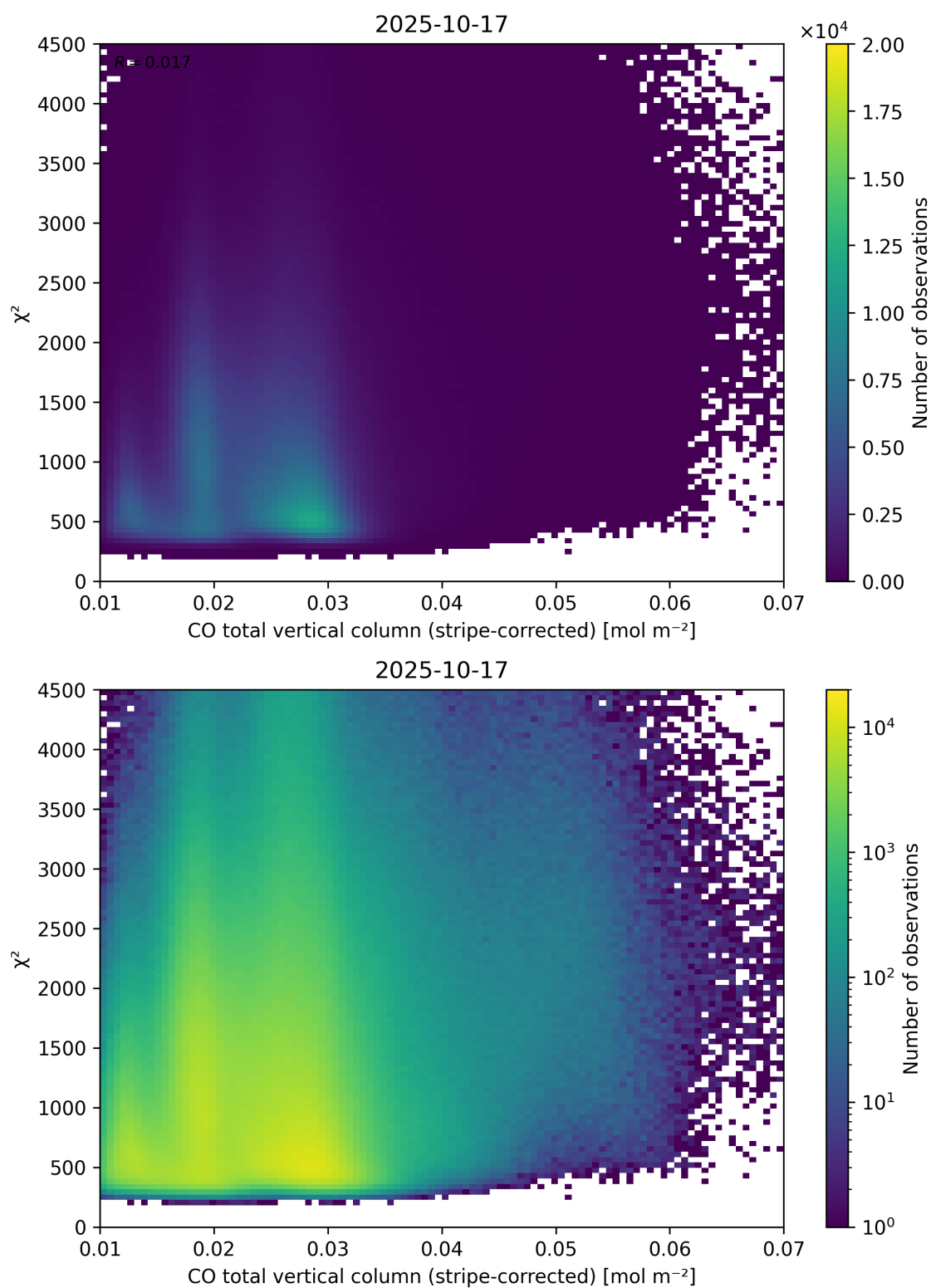
Figure 37: Scatter density plot of “CO total vertical column (stripe-corrected)” against “ \chi^2 ” for 2025-10-17 to 2025-10-18.
