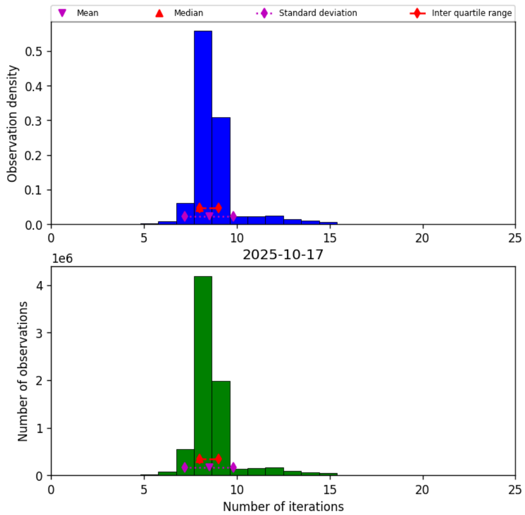
Figure 24: Histogram of “Number of iterations” for 2025-10-17 to 2025-10-18
