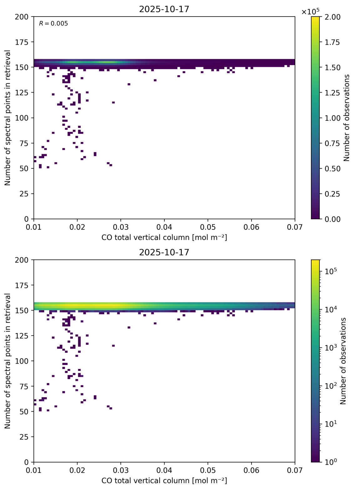
Figure 43: Scatter density plot of “CO total vertical column” against “Number of spectral points in retrieval” for 2025-10-17 to 2025-10-18.
