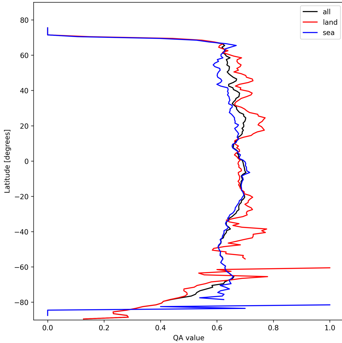
Figure 9: Zonal average of “QA value” for 2025-10-17 to 2025-10-18.
