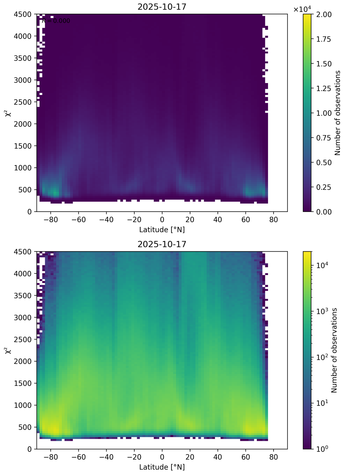
Figure 54: Scatter density plot of “Latitude” against “ \chi^2 ” for 2025-10-17 to 2025-10-18.
