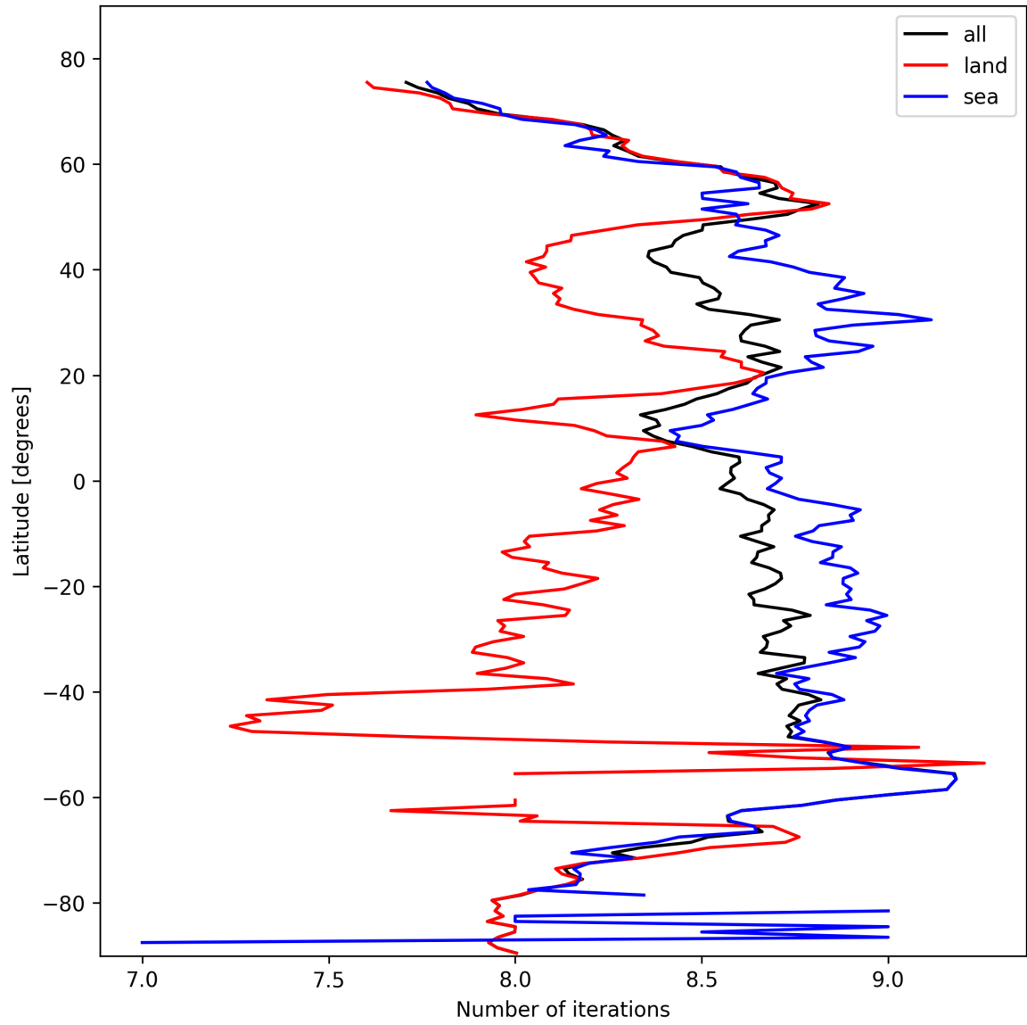
Figure 16: Zonal average of “Number of iterations” for 2025-10-17 to 2025-10-18.
