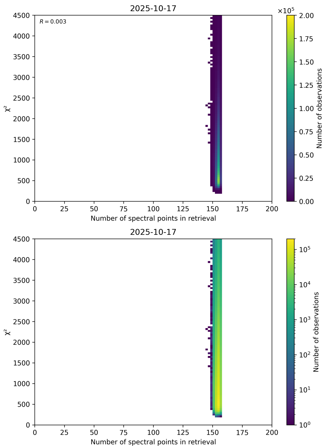
Figure 58: Scatter density plot of “Number of spectral points in retrieval” against “ \chi^2 ” for 2025-10-17 to 2025-10-18.
