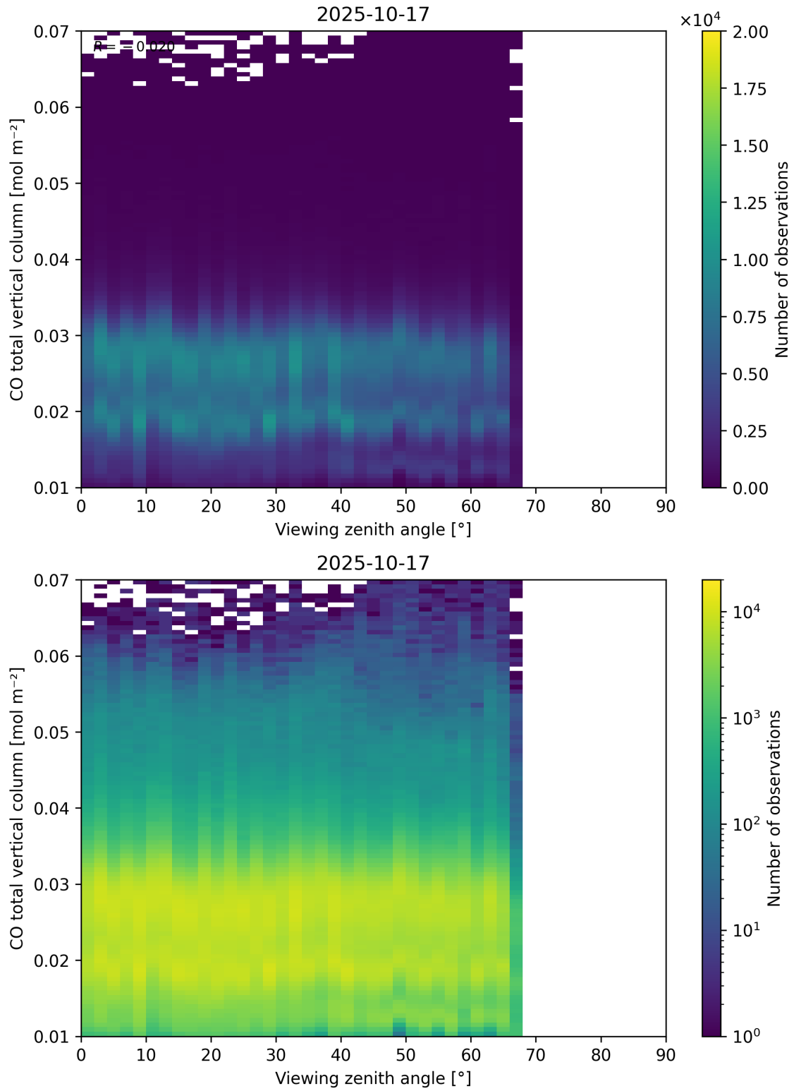
Figure 69: Scatter density plot of “Viewing zenith angle” against “CO total vertical column” for 2025-10-17 to 2025-10-18.
