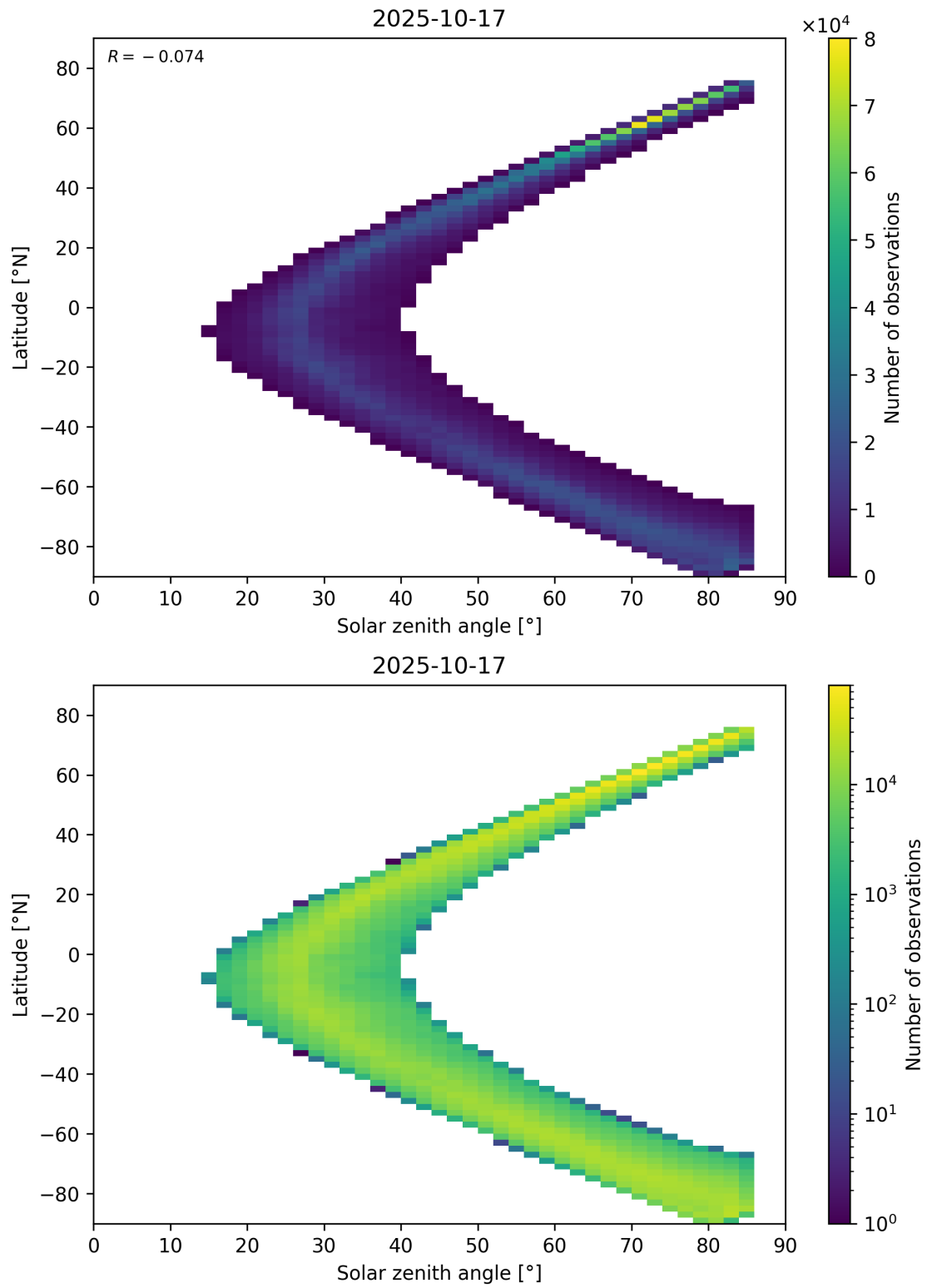
Figure 66: Scatter density plot of “Solar zenith angle” against “Latitude” for 2025-10-17 to 2025-10-18.
