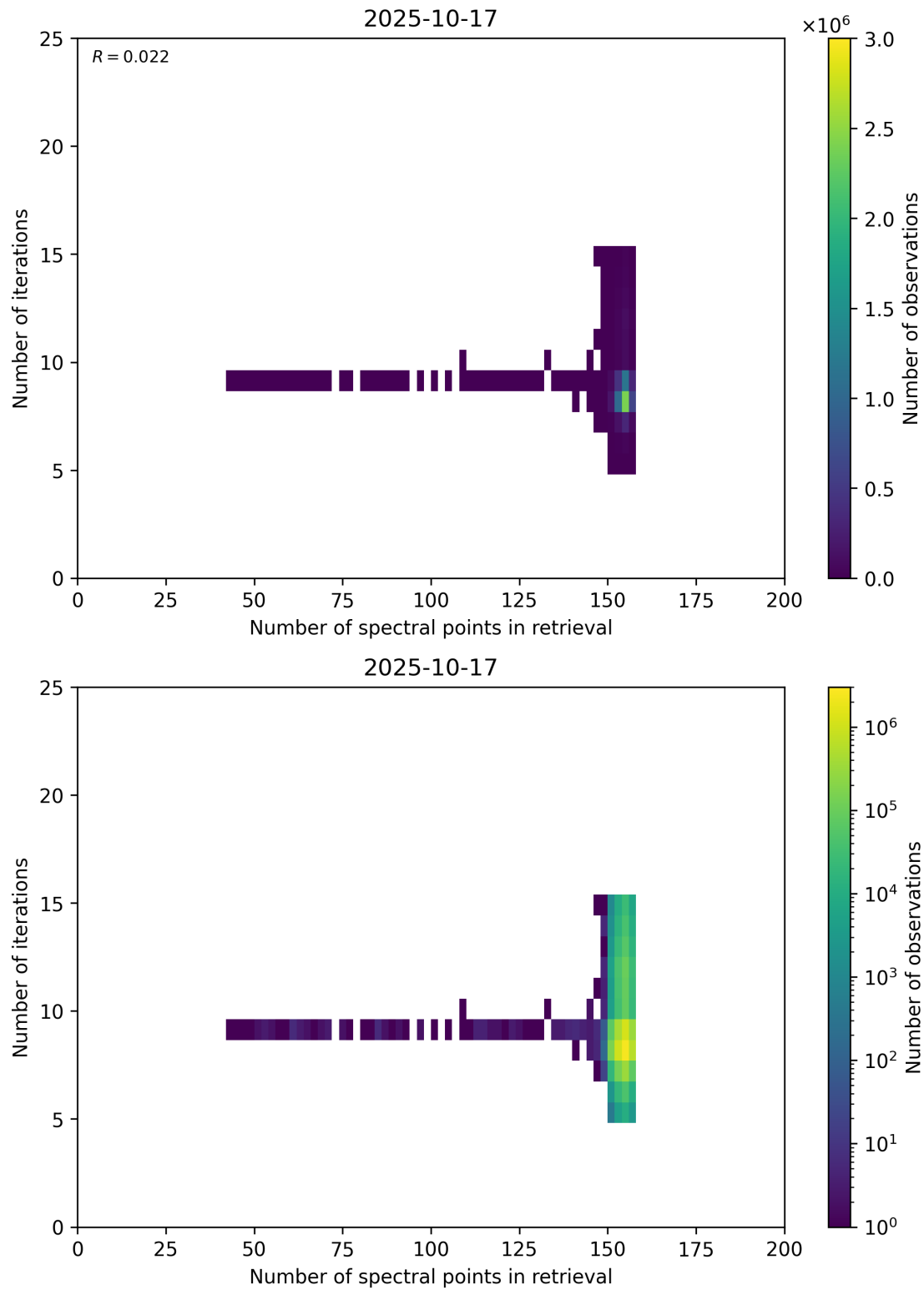
Figure 60: Scatter density plot of “Number of spectral points in retrieval” against “Number of iterations” for 2025-10-17 to 2025-10-18.
