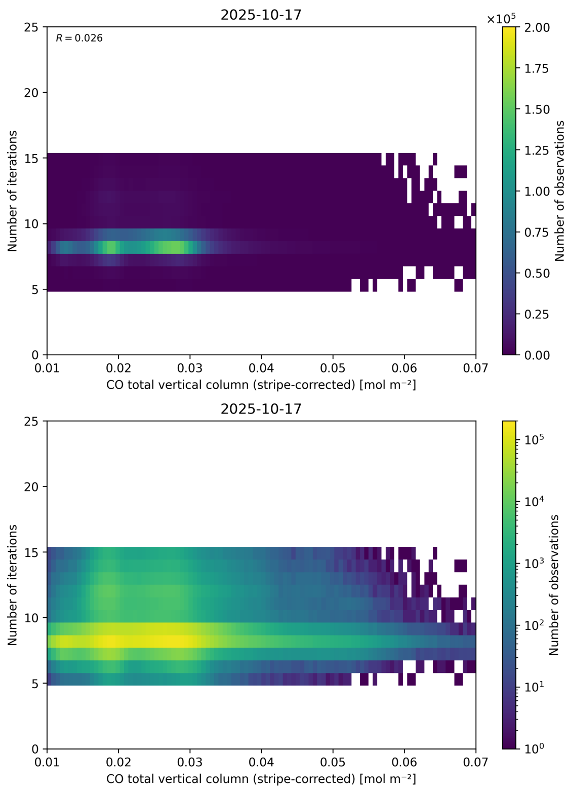
Figure 39: Scatter density plot of “CO total vertical column (stripe-corrected)” against “Number of iterations” for 2025-10-17 to 2025-10-18.
