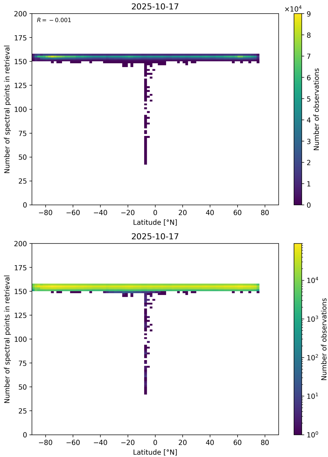
Figure 57: Scatter density plot of “Latitude” against “Number of spectral points in retrieval” for 2025-10-17 to 2025-10-18.
