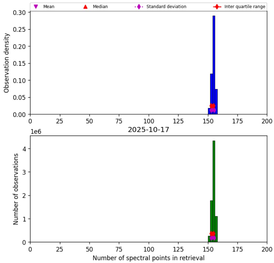
Figure 21: Histogram of “Number of spectral points in retrieval” for 2025-10-17 to 2025-10-18
