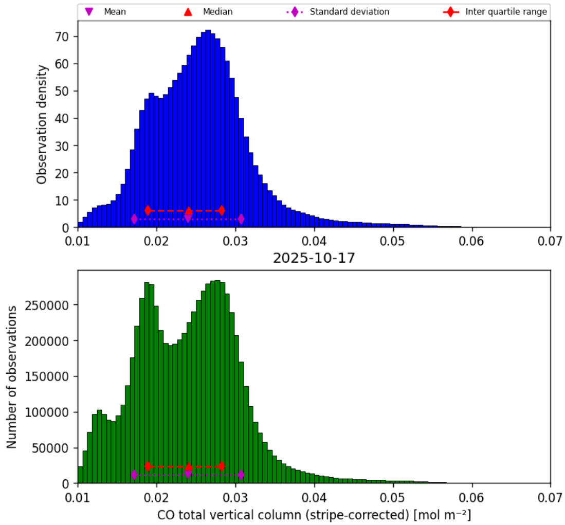
Figure 19: Histogram of “CO total vertical column (stripe-corrected)” for 2025-10-17 to 2025-10-18
