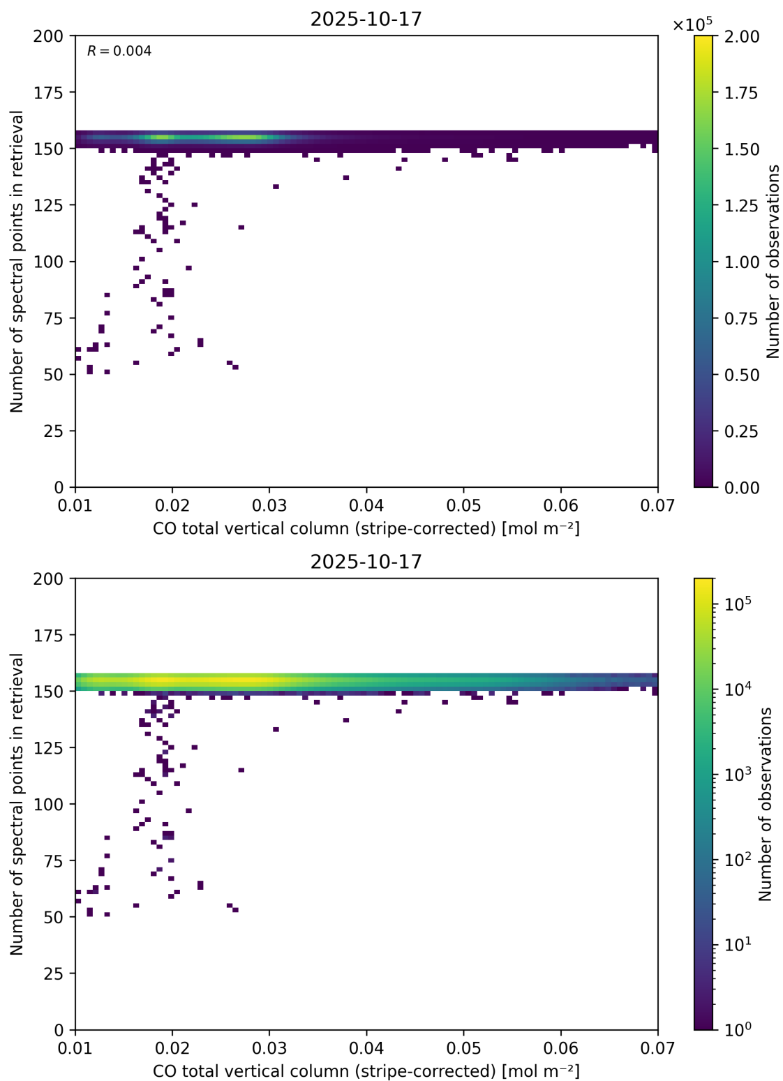
Figure 40: Scatter density plot of “CO total vertical column (stripe-corrected)” against “Number of spectral points in retrieval” for 2025-10-17 to 2025-10-18.
