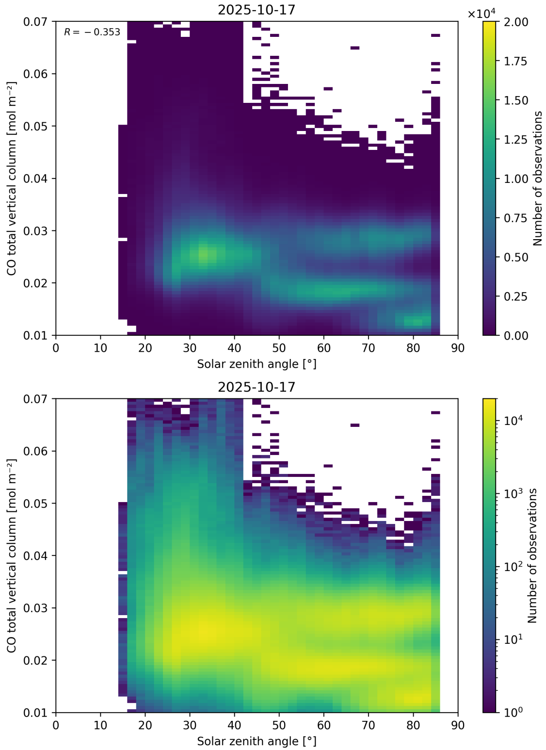
Figure 61: Scatter density plot of “Solar zenith angle” against “CO total vertical column” for 2025-10-17 to 2025-10-18.
