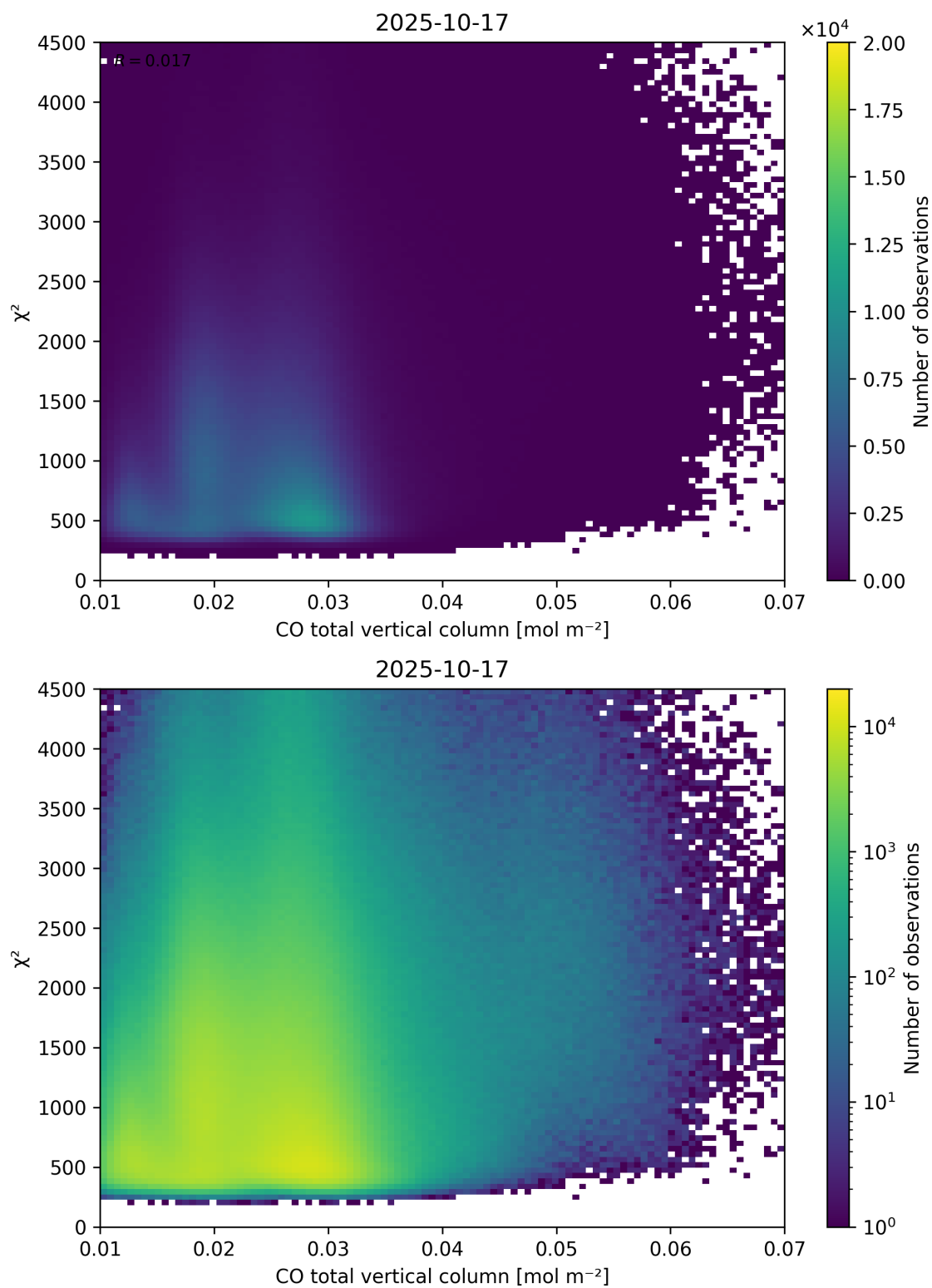
Figure 35: Scatter density plot of “CO total vertical column” against “ \chi^2 ” for 2025-10-17 to 2025-10-18.
