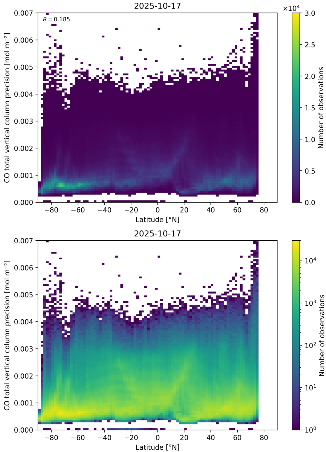
Figure 53: Scatter density plot of “Latitude” against “CO total vertical column precision” for 2025-10-17 to 2025-10-18.
