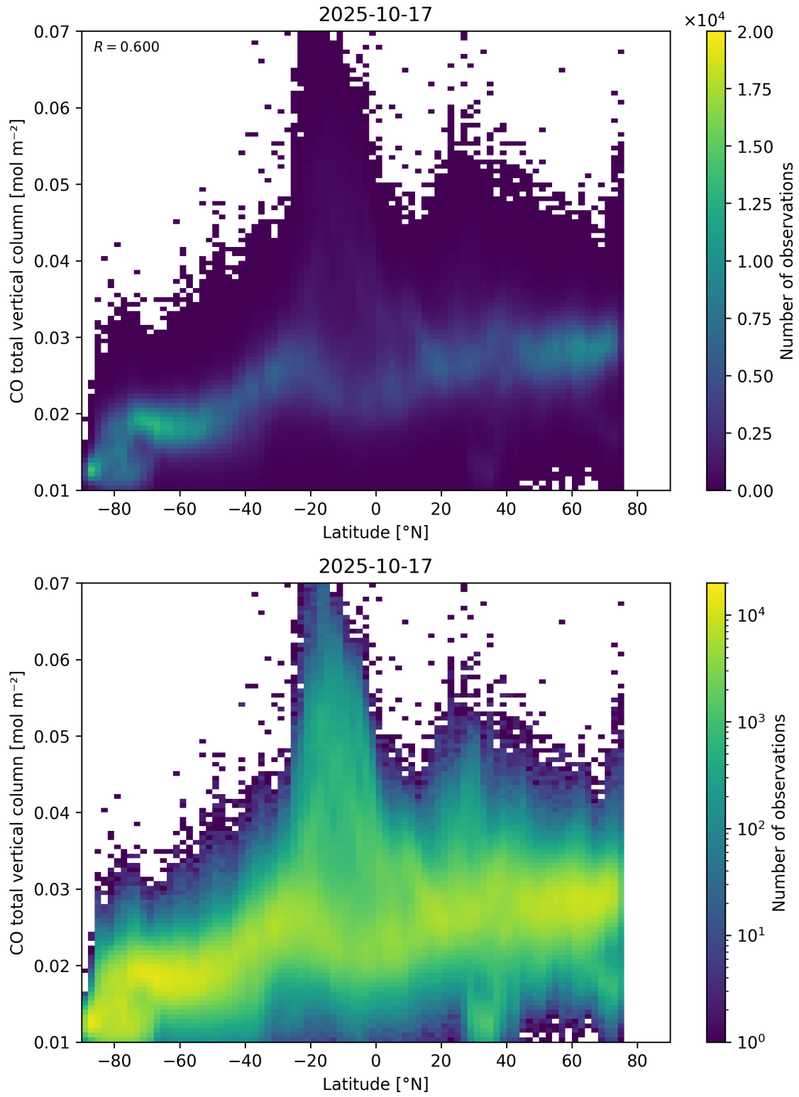
Figure 51: Scatter density plot of “Latitude” against “CO total vertical column” for 2025-10-17 to 2025-10-18.
