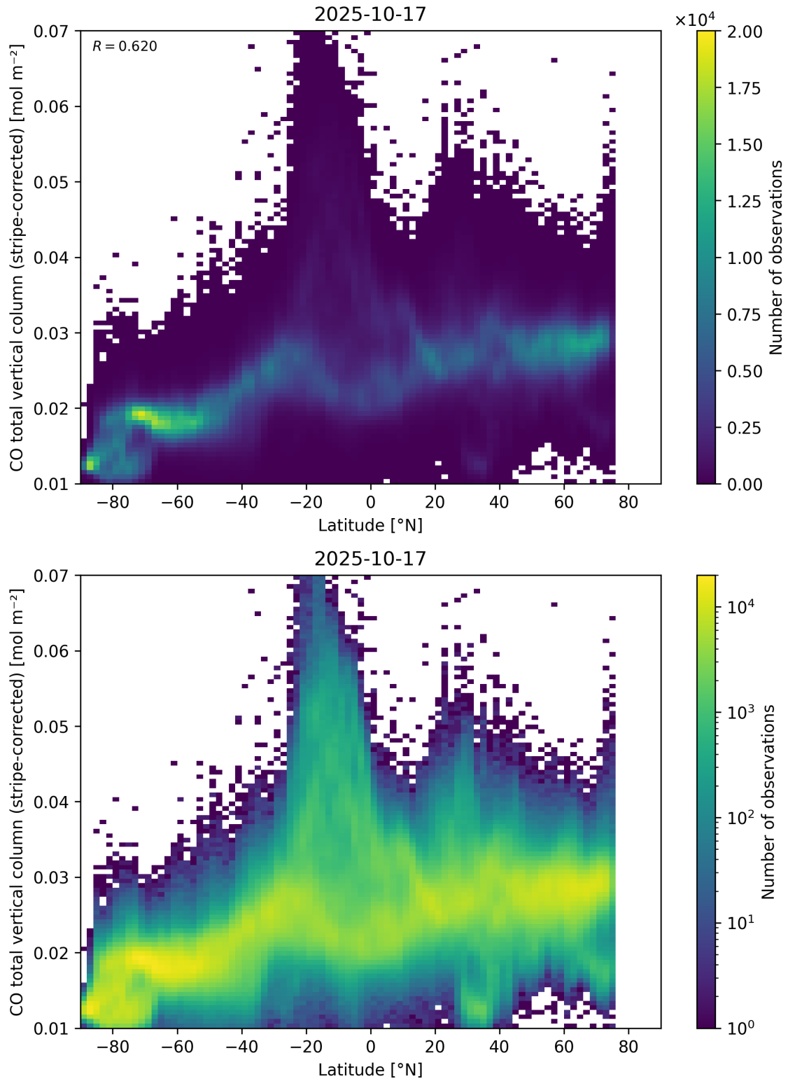
Figure 52: Scatter density plot of “Latitude” against “CO total vertical column (stripe-corrected)” for 2025-10-17 to 2025-10-18.
