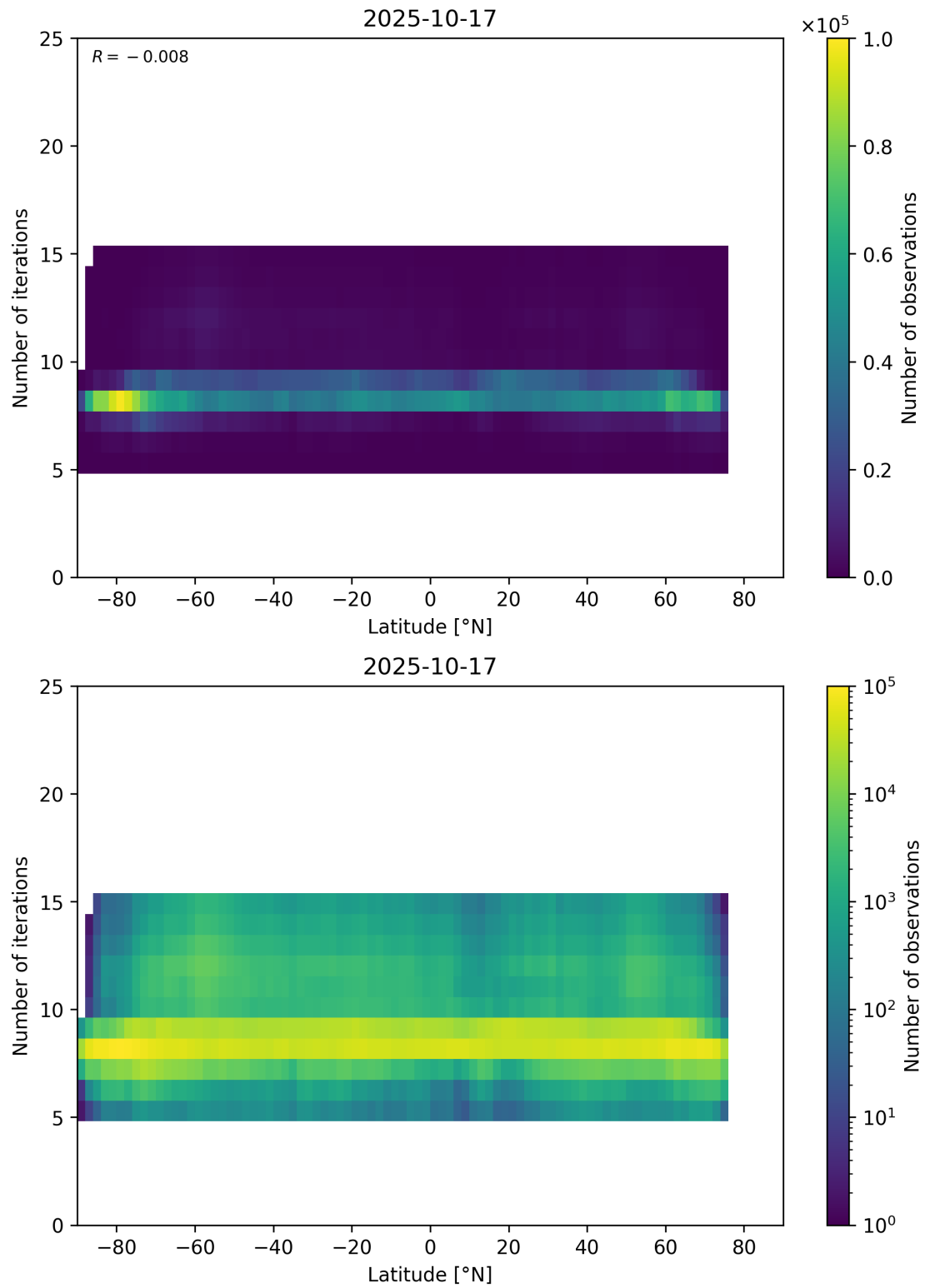
Figure 56: Scatter density plot of “Latitude” against “Number of iterations” for 2025-10-17 to 2025-10-18.
