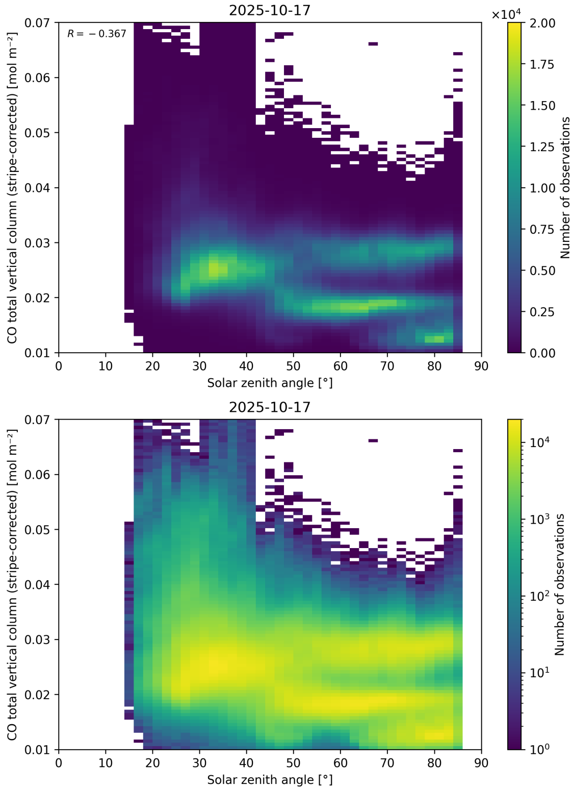
Figure 62: Scatter density plot of “Solar zenith angle” against “CO total vertical column (stripe-corrected)” for 2025-10-17 to 2025-10-18.
