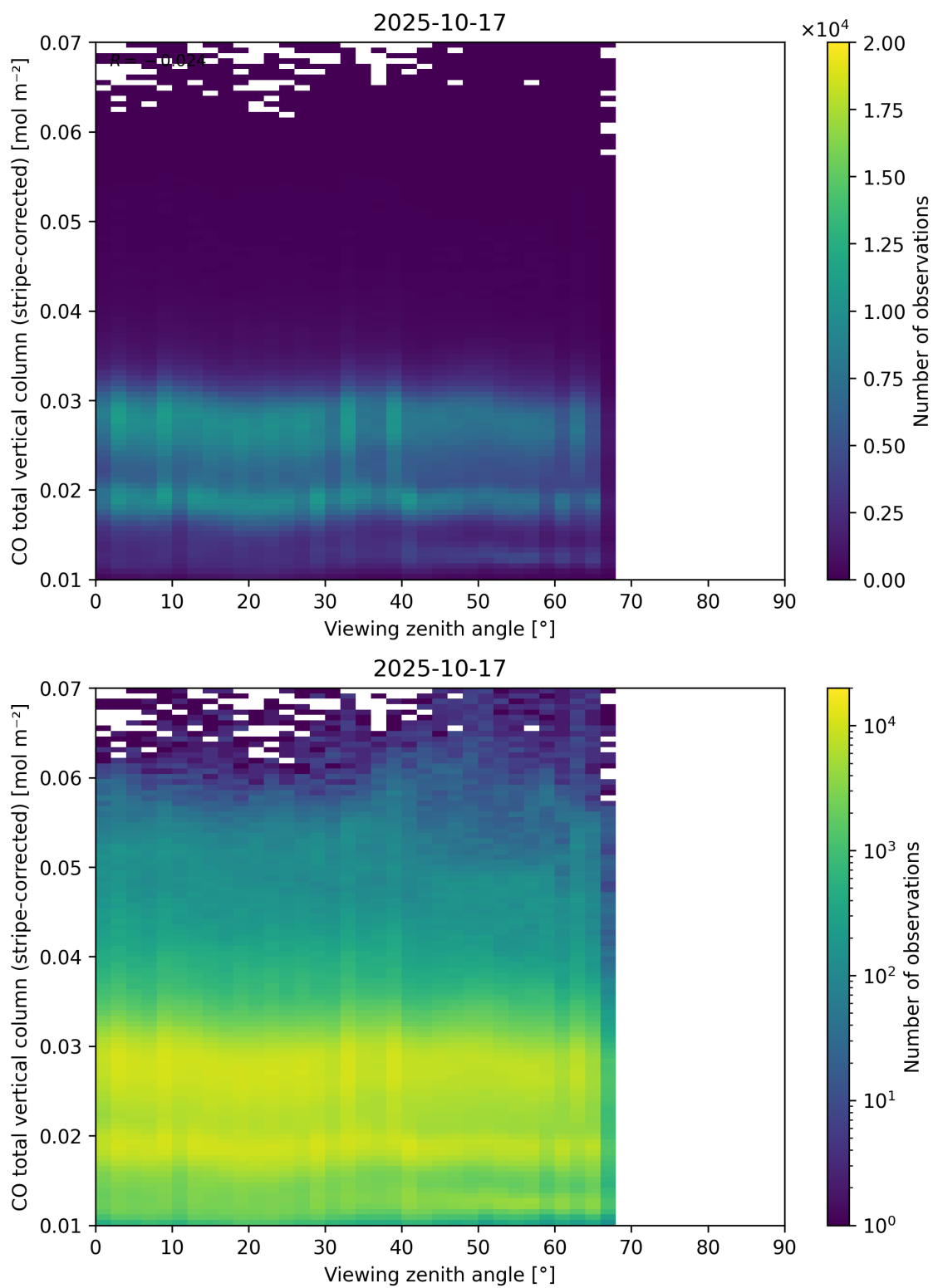
Figure 70: Scatter density plot of “Viewing zenith angle” against “CO total vertical column (stripe-corrected)” for 2025-10-17 to 2025-10-18.
