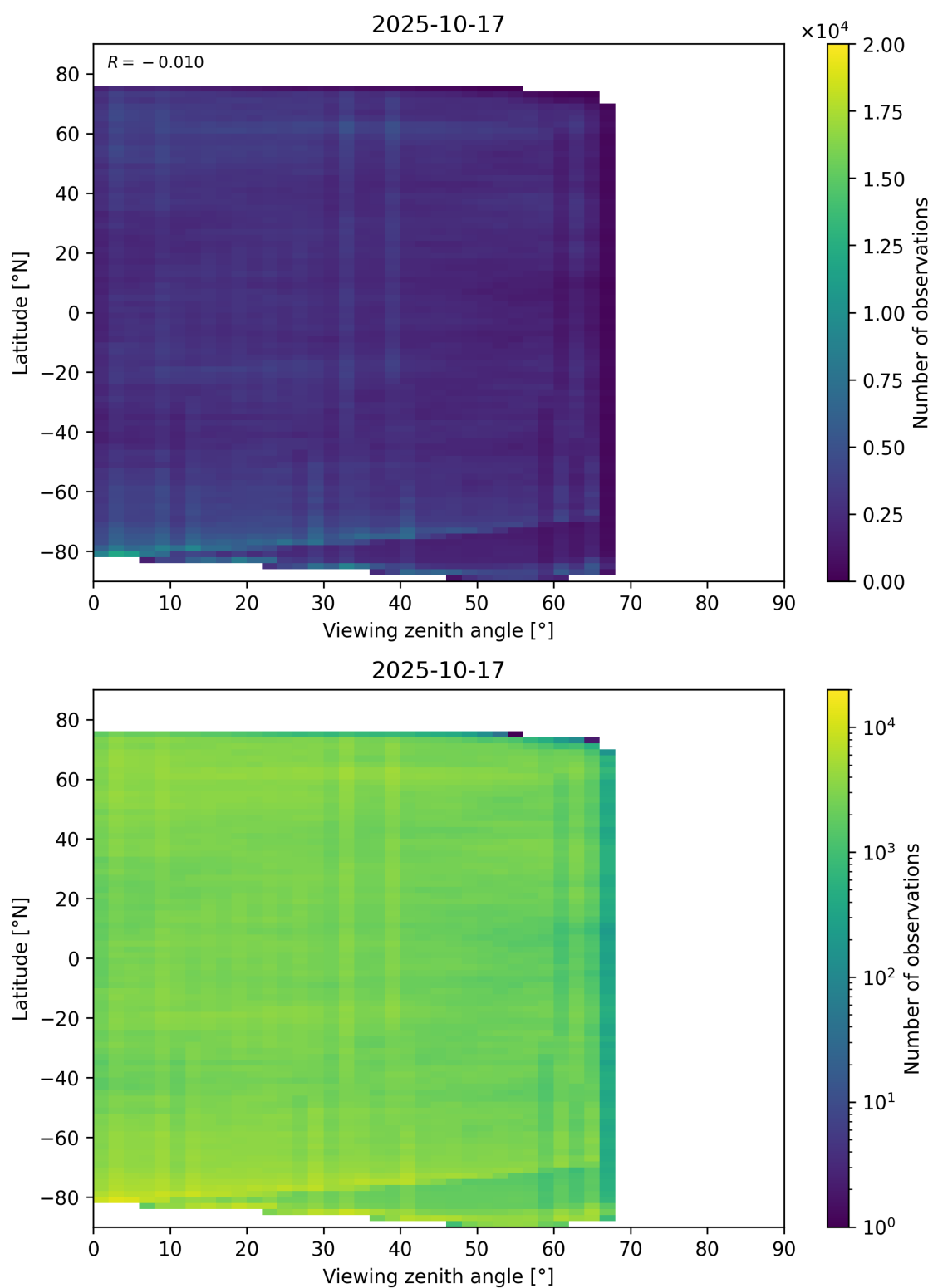
Figure 74: Scatter density plot of “Viewing zenith angle” against “Latitude” for 2025-10-17 to 2025-10-18.
