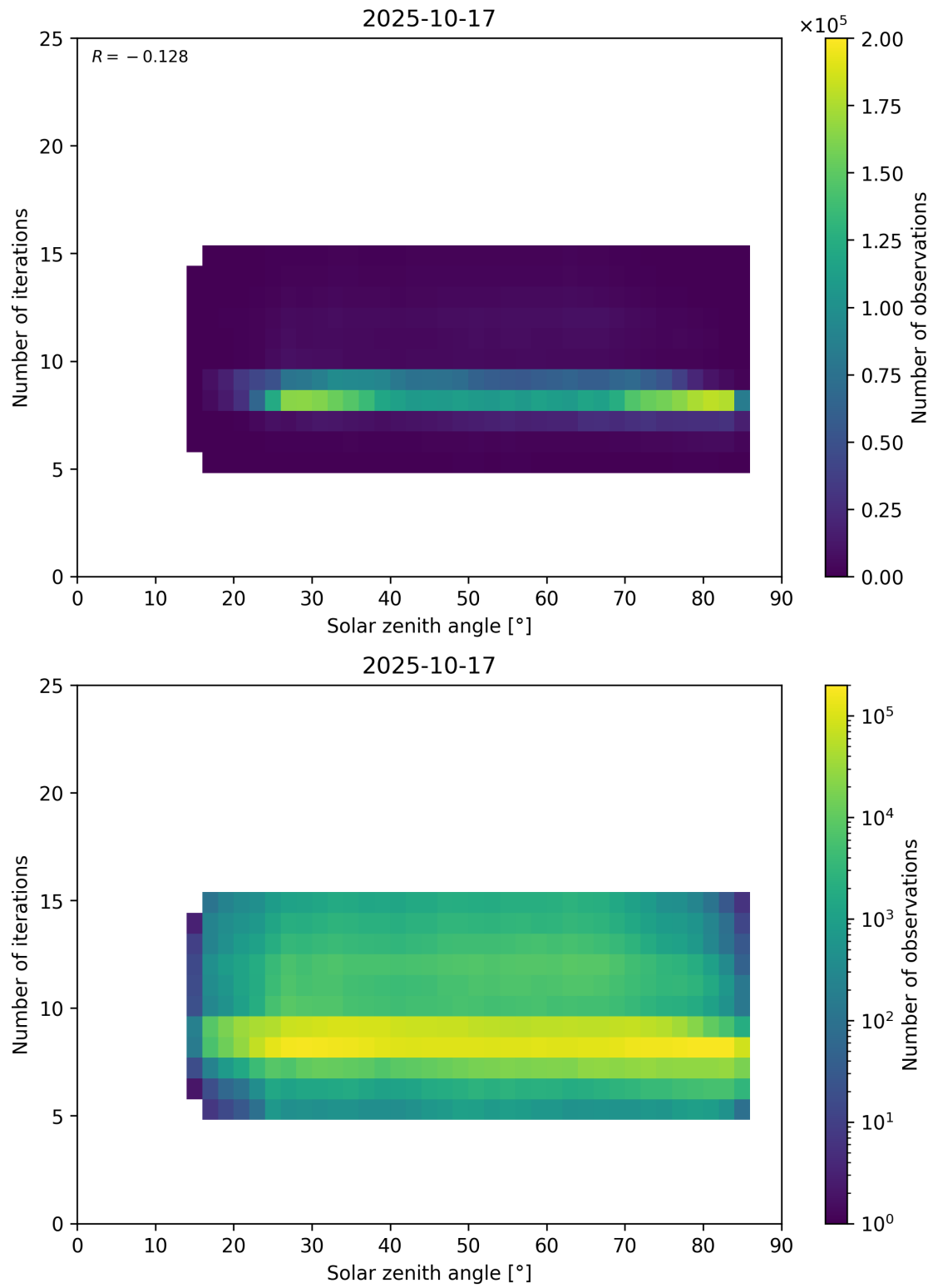
Figure 67: Scatter density plot of “Solar zenith angle” against “Number of iterations” for 2025-10-17 to 2025-10-18.
