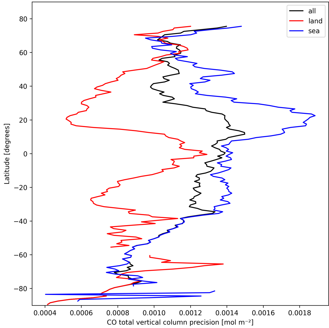
Figure 12: Zonal average of “CO total vertical column precision” for 2025-10-17 to 2025-10-18.
