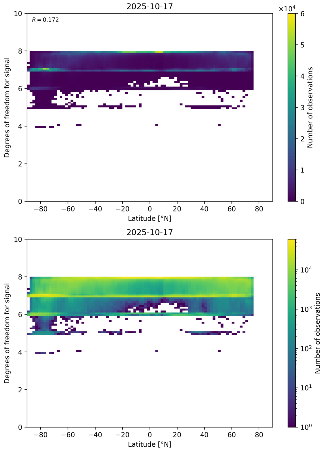
Figure 55: Scatter density plot of “Latitude” against “Degrees of freedom for signal” for 2025-10-17 to 2025-10-18.
