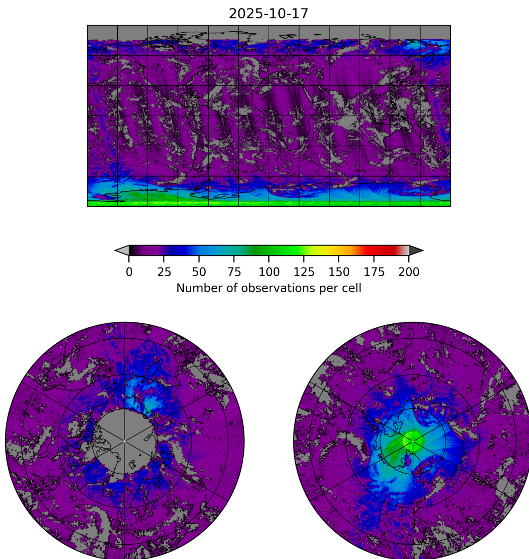
Figure 8: Map of the number of observations for 2025-10-17 to 2025-10-18
