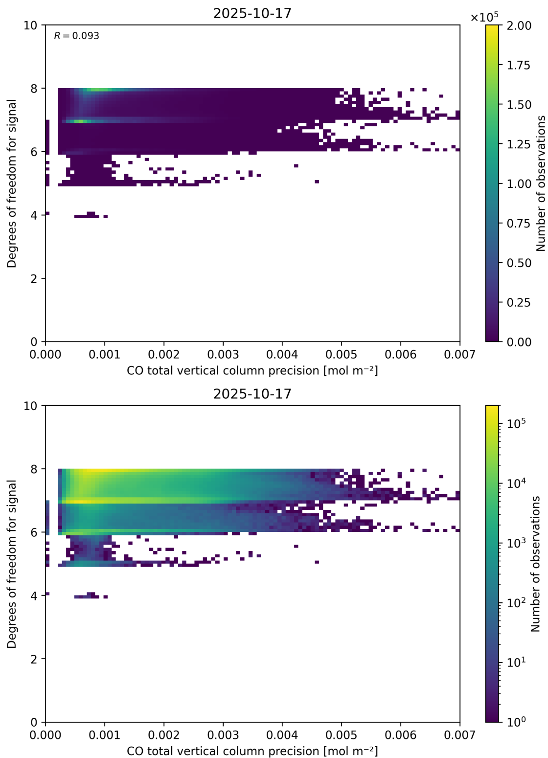
Figure 45: Scatter density plot of “CO total vertical column precision” against “Degrees of freedom for signal” for 2025-10-17 to 2025-10-18.
