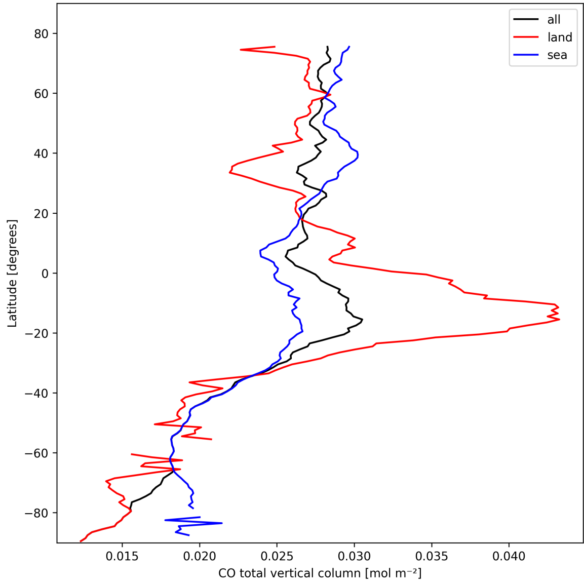
Figure 10: Zonal average of “CO total vertical column” for 2025-10-17 to 2025-10-18.
