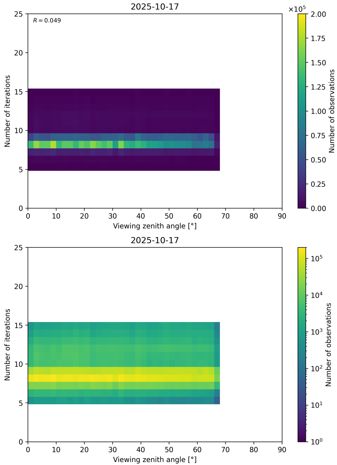
Figure 75: Scatter density plot of “Viewing zenith angle” against “Number of iterations” for 2025-10-17 to 2025-10-18.
