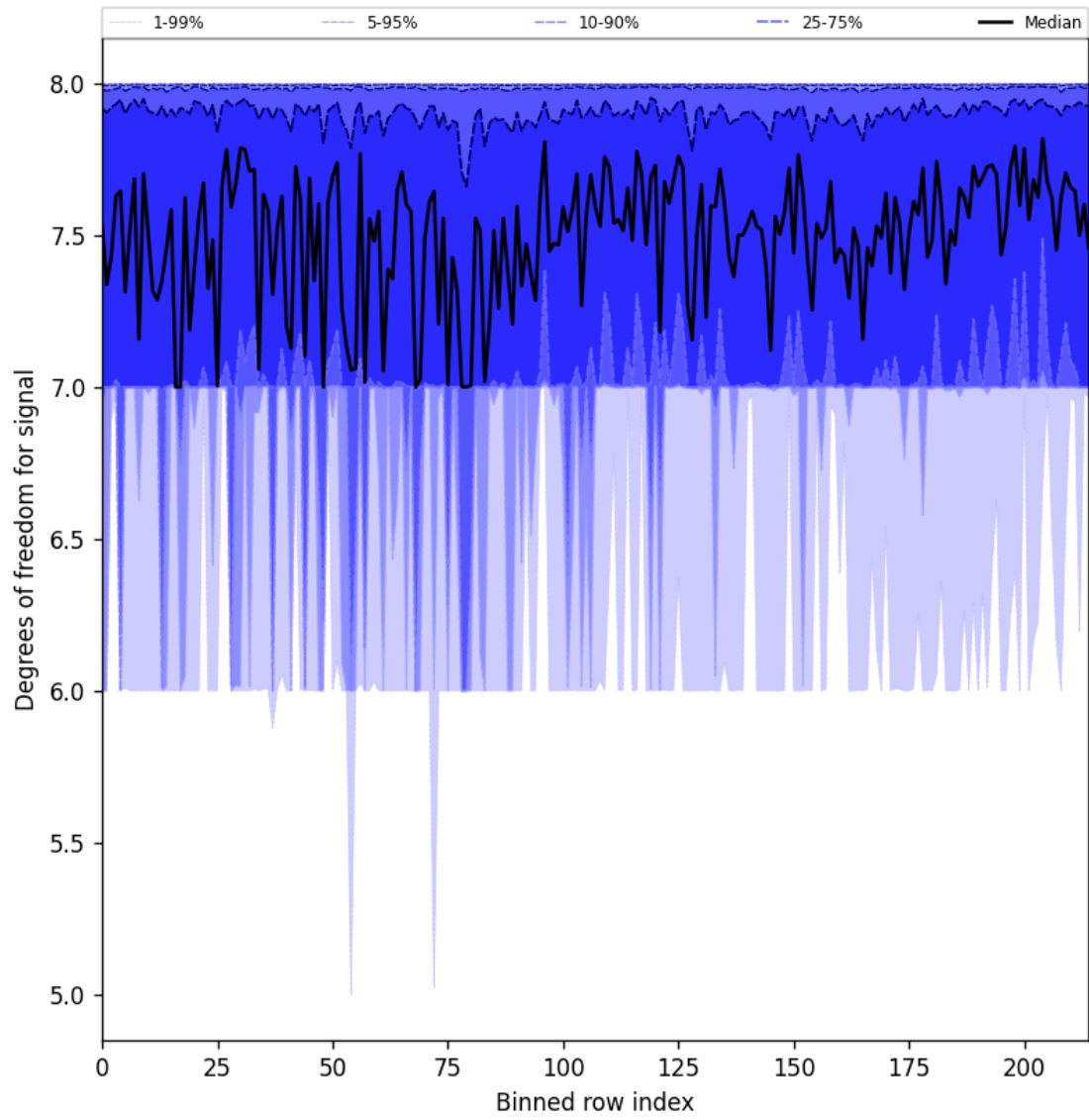
Figure 31: Along track statistics of “Degrees of freedom for signal” for 2025-10-17 to 2025-10-18
