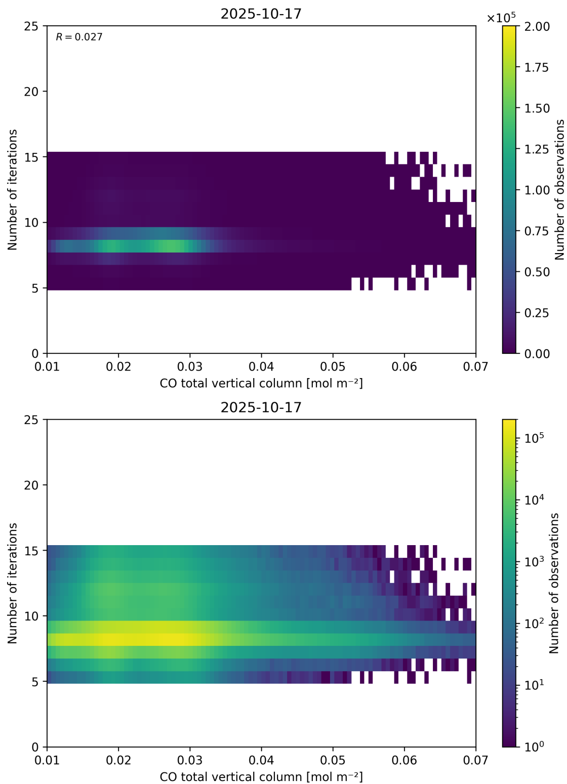
Figure 42: Scatter density plot of “CO total vertical column” against “Number of iterations” for 2025-10-17 to 2025-10-18.
