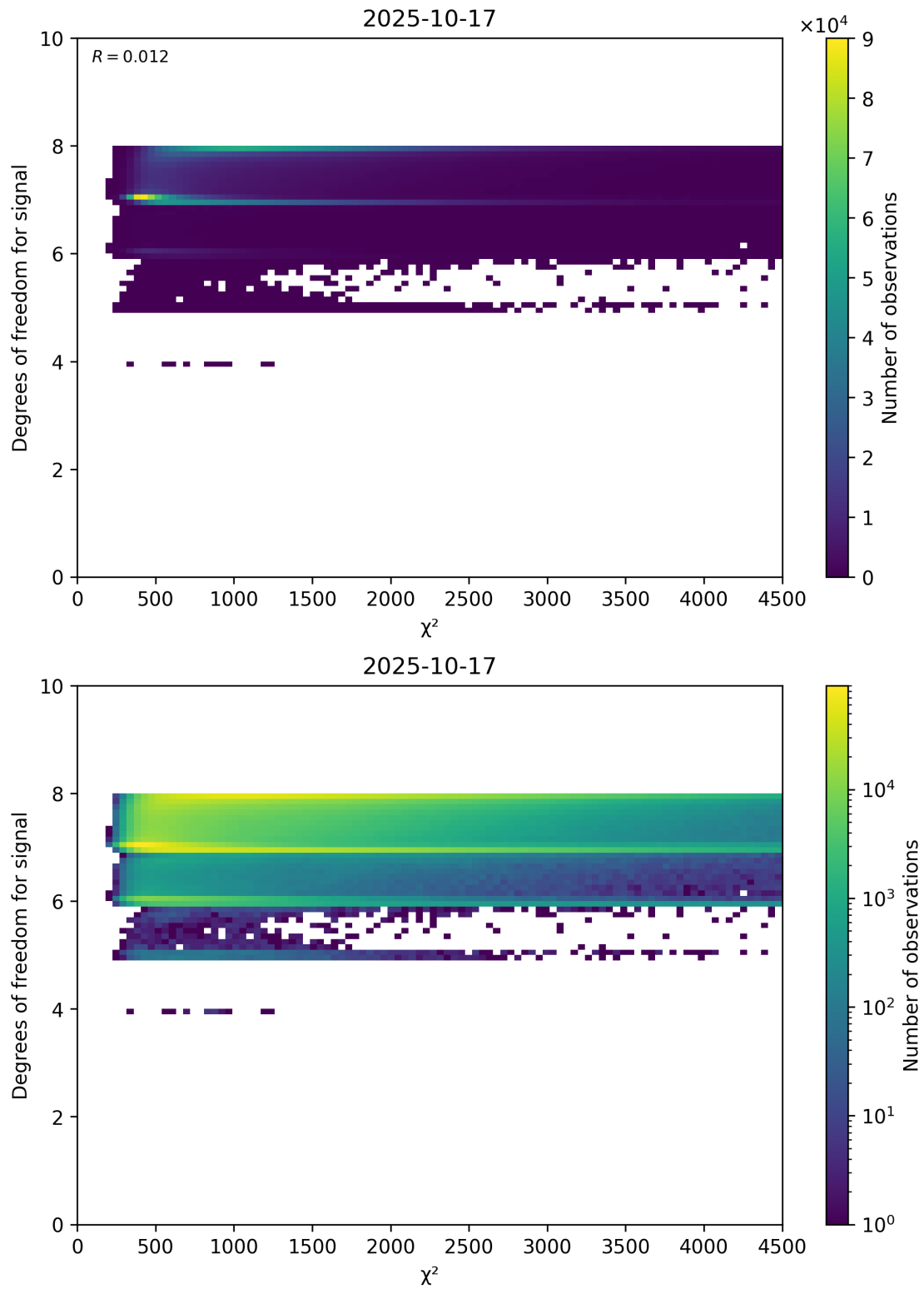
Figure 48: Scatter density plot of “ \chi^2 ” against “Degrees of freedom for signal” for 2025-10-17 to 2025-10-18.
