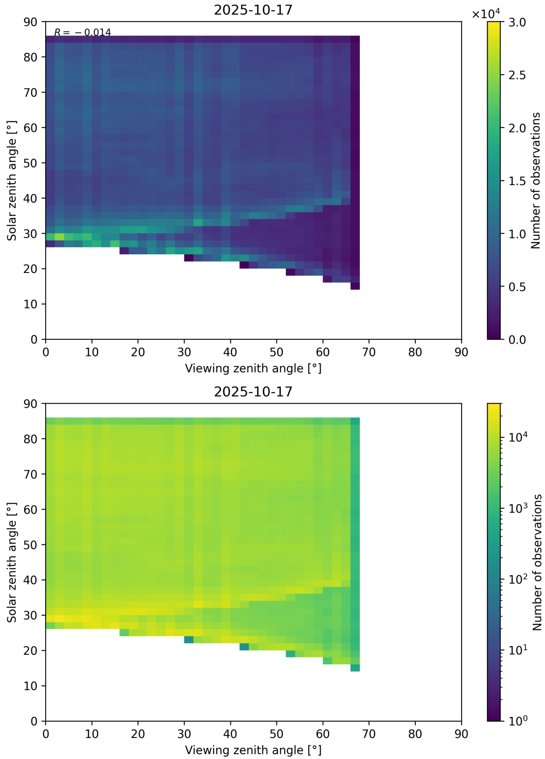
Figure 77: Scatter density plot of “Viewing zenith angle” against “Solar zenith angle” for 2025-10-17 to 2025-10-18.
