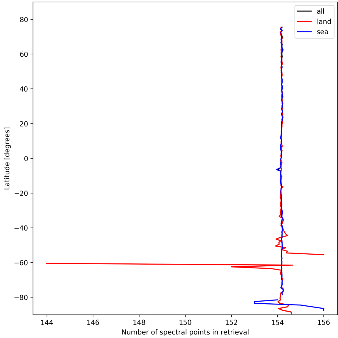
Figure 13: Zonal average of “Number of spectral points in retrieval” for 2025-10-17 to 2025-10-18.
