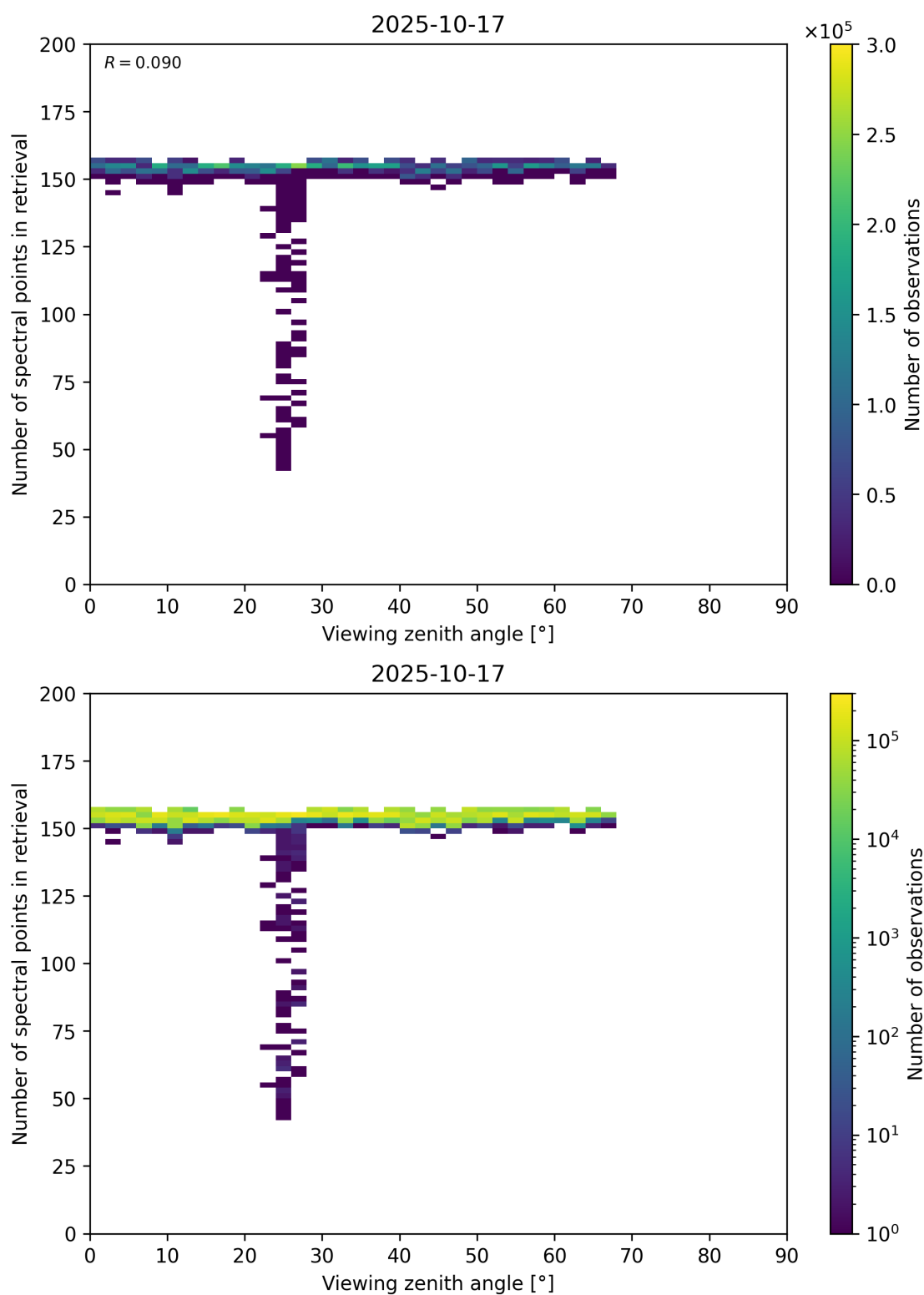
Figure 76: Scatter density plot of “Viewing zenith angle” against “Number of spectral points in retrieval” for 2025-10-17 to 2025-10-18.
