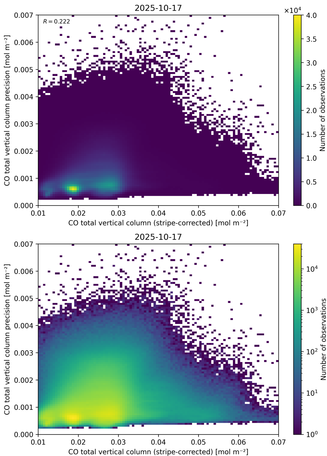
Figure 36: Scatter density plot of “CO total vertical column (stripe-corrected)” against “CO total vertical column precision” for 2025-10-17 to 2025-10-18.
