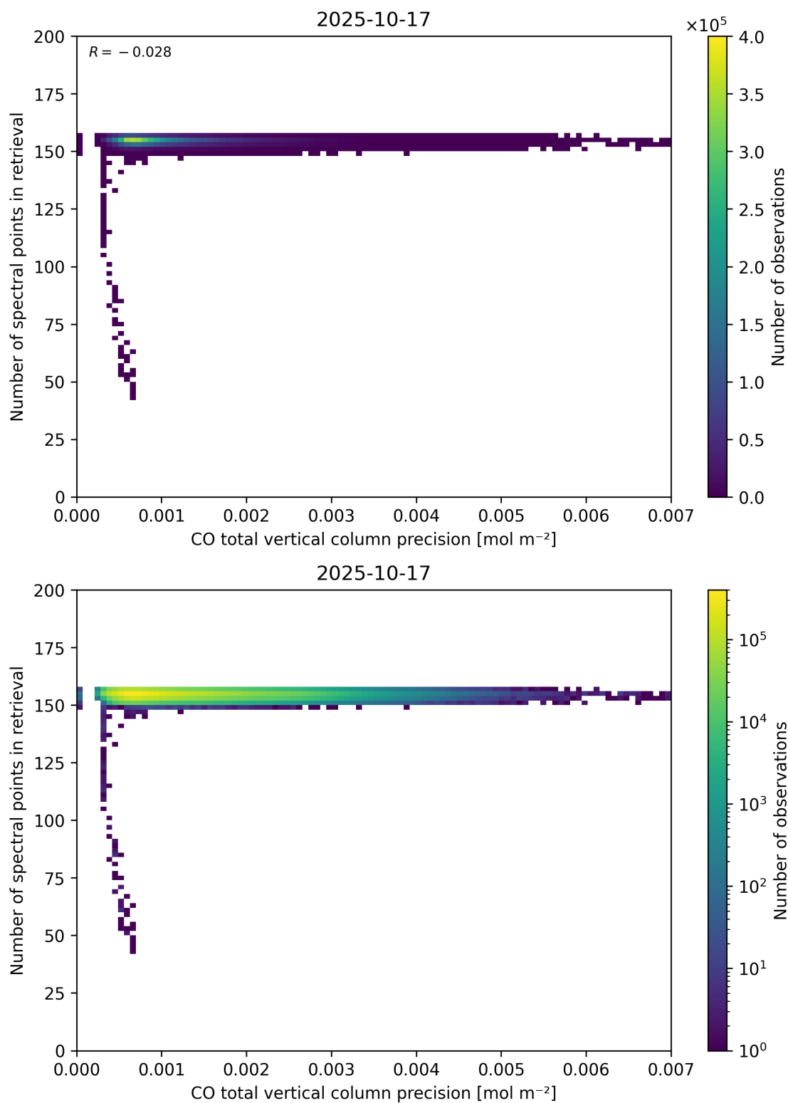
Figure 47: Scatter density plot of “CO total vertical column precision” against “Number of spectral points in retrieval” for 2025-10-17 to 2025-10-18.
