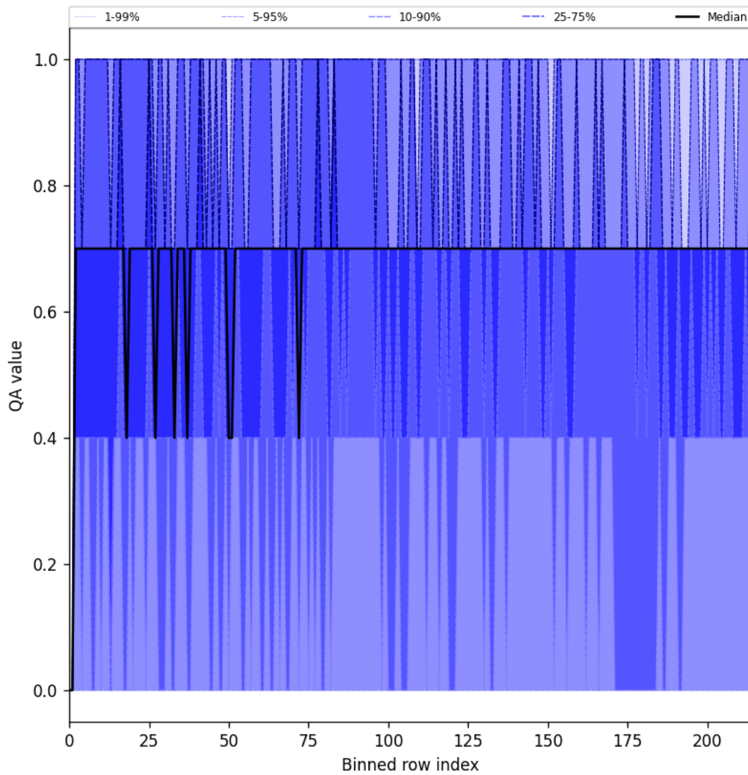
Figure 25: Along track statistics of “QA value” for 2025-10-17 to 2025-10-18
