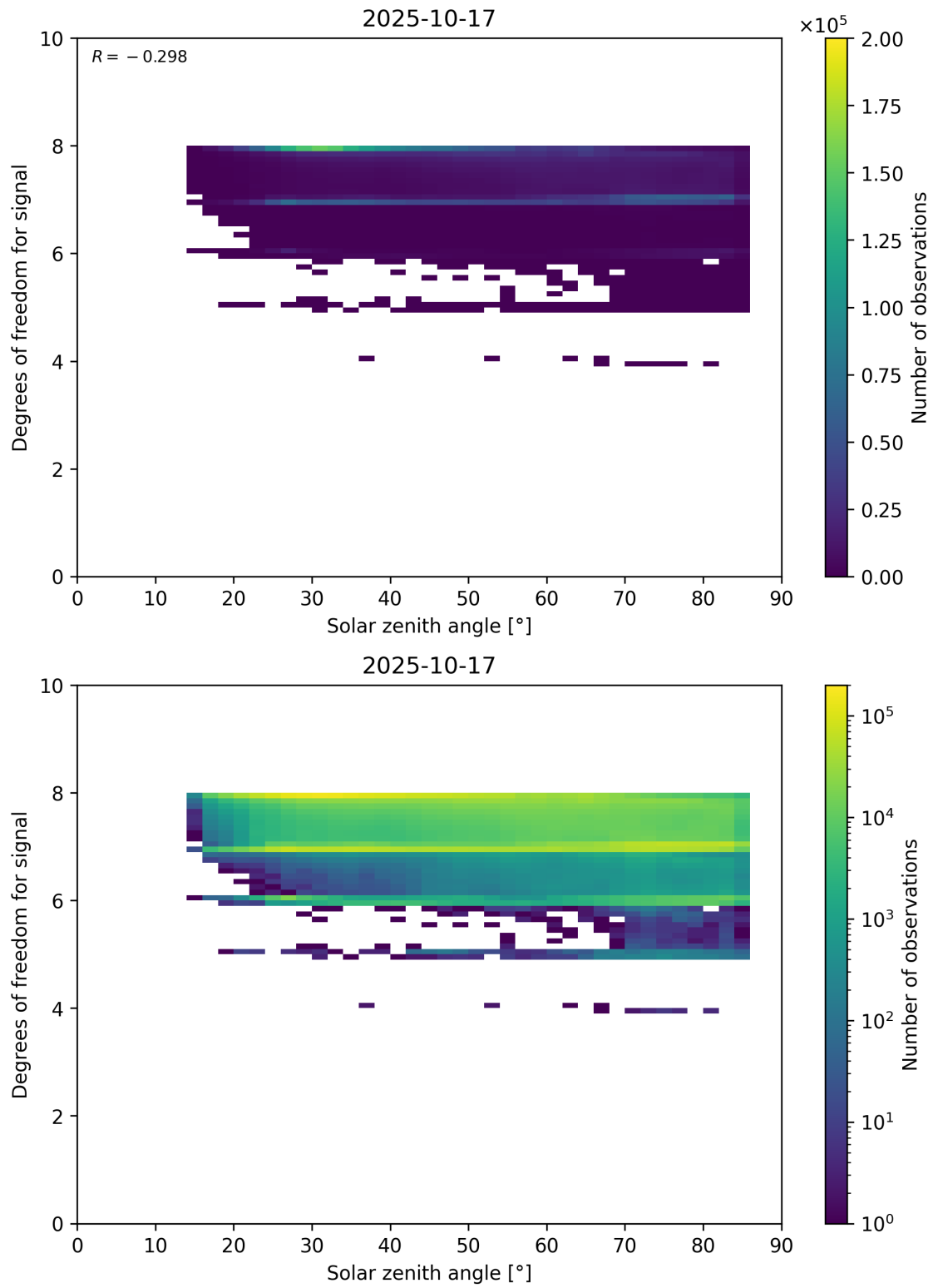
Figure 65: Scatter density plot of “Solar zenith angle” against “Degrees of freedom for signal” for 2025-10-17 to 2025-10-18.
