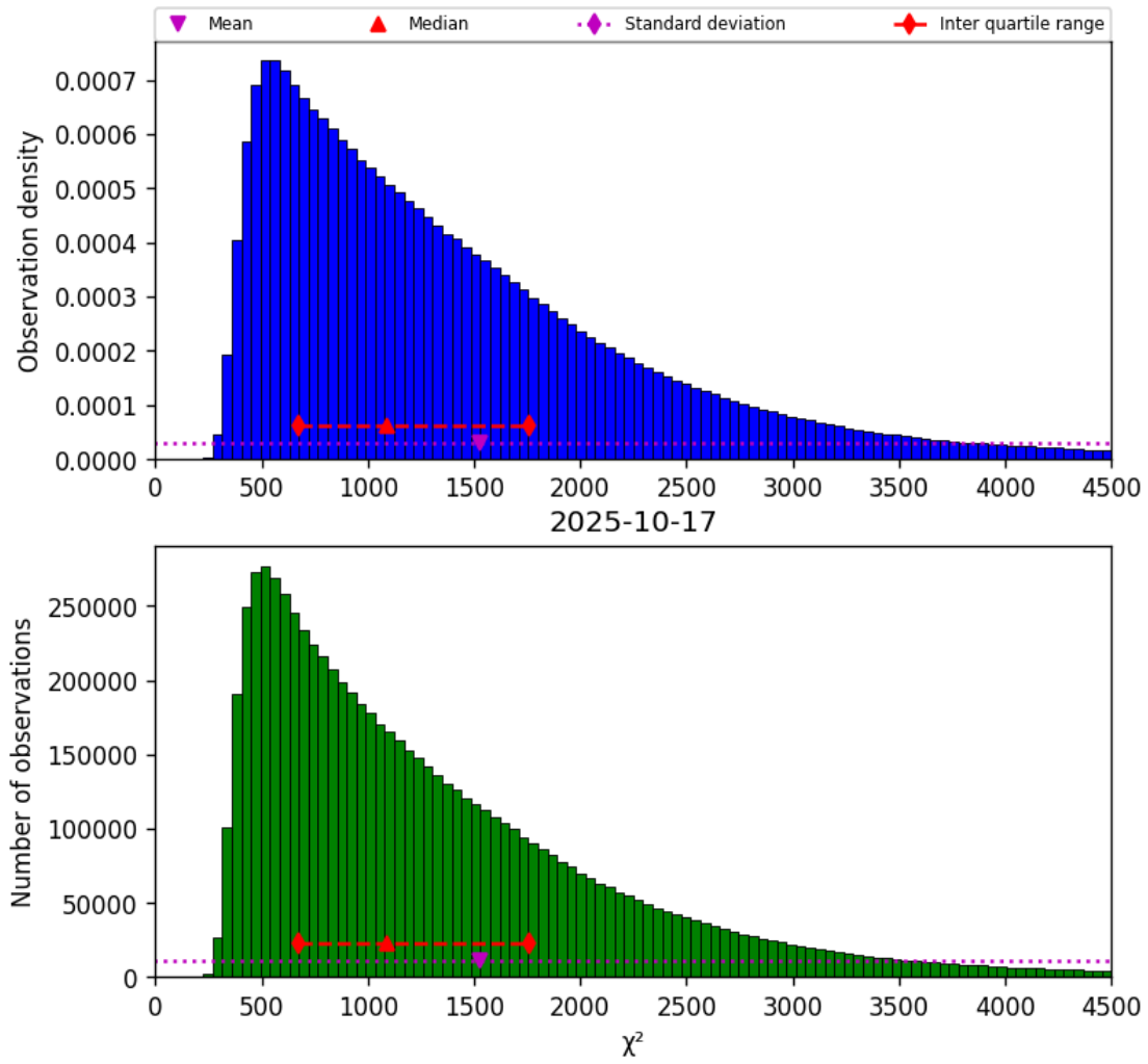
Figure 22: Histogram of “ \chi^2 ” for 2025-10-17 to 2025-10-18
