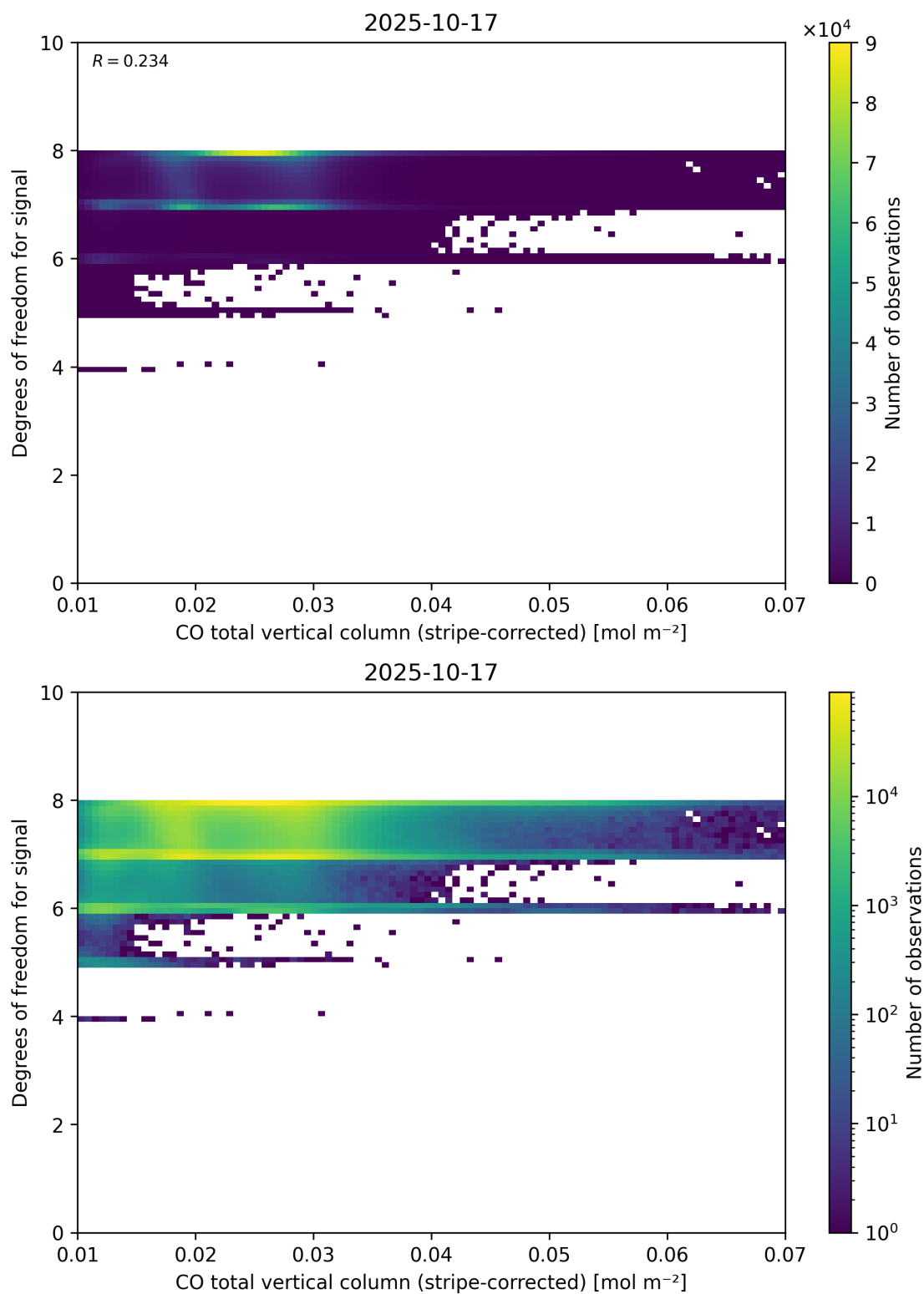
Figure 38: Scatter density plot of “CO total vertical column (stripe-corrected)” against “Degrees of freedom for signal” for 2025-10-17 to 2025-10-18.
