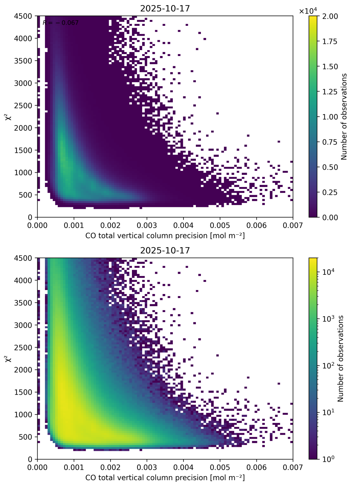
Figure 44: Scatter density plot of “CO total vertical column precision” against “ \chi^2 ” for 2025-10-17 to 2025-10-18.
