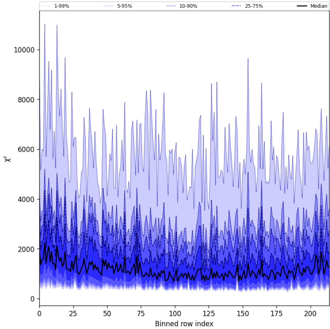
Figure 30: Along track statistics of “ \chi^2 ” for 2025-10-17 to 2025-10-18
