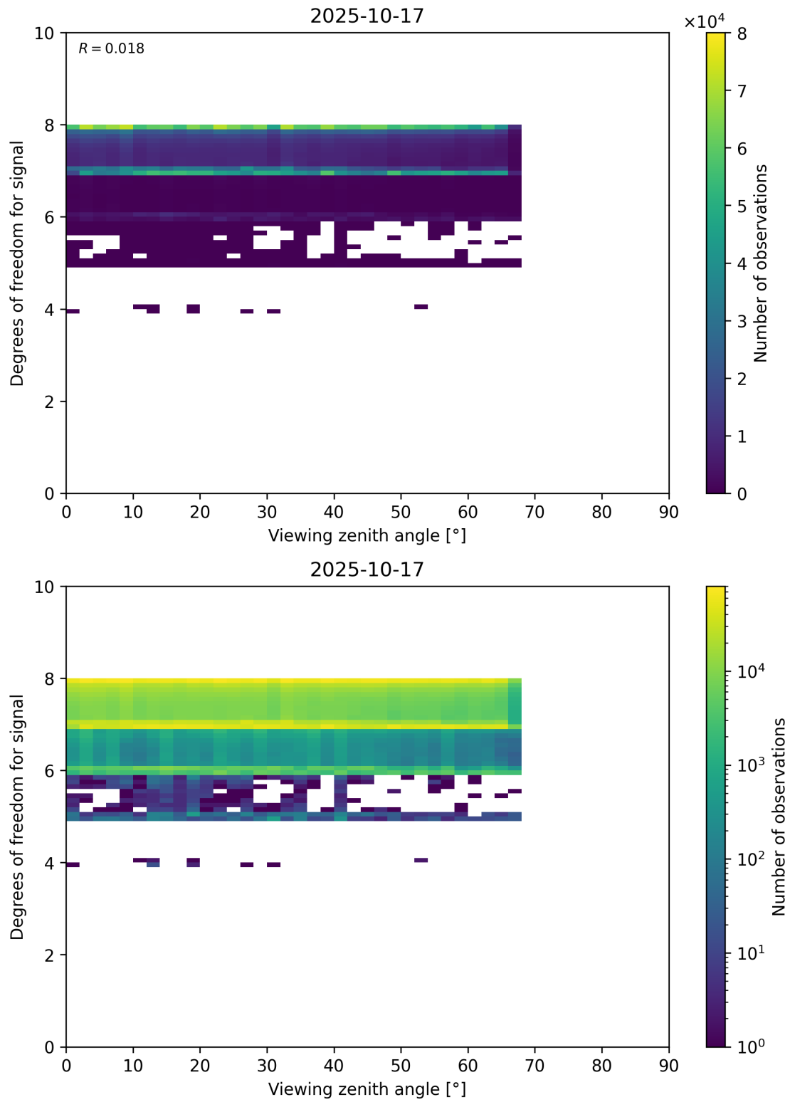
Figure 73: Scatter density plot of “Viewing zenith angle” against “Degrees of freedom for signal” for 2025-10-17 to 2025-10-18.
