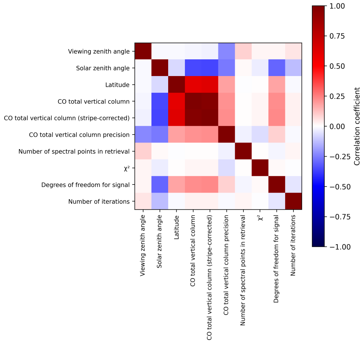
Figure 2: Map of correlation matrix for 2025-10-17 to 2025-10-18.
