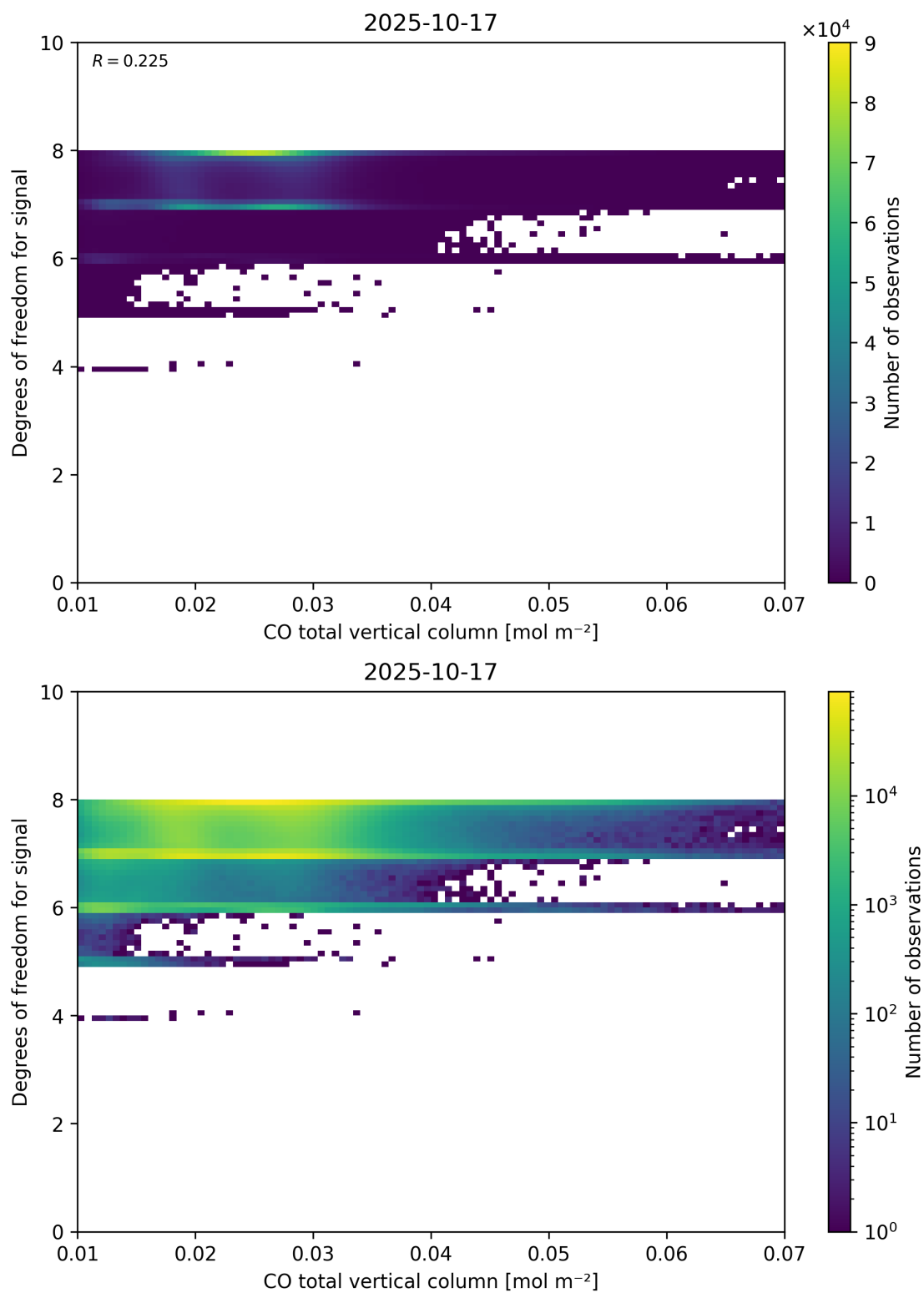
Figure 41: Scatter density plot of “CO total vertical column” against “Degrees of freedom for signal” for 2025-10-17 to 2025-10-18.
