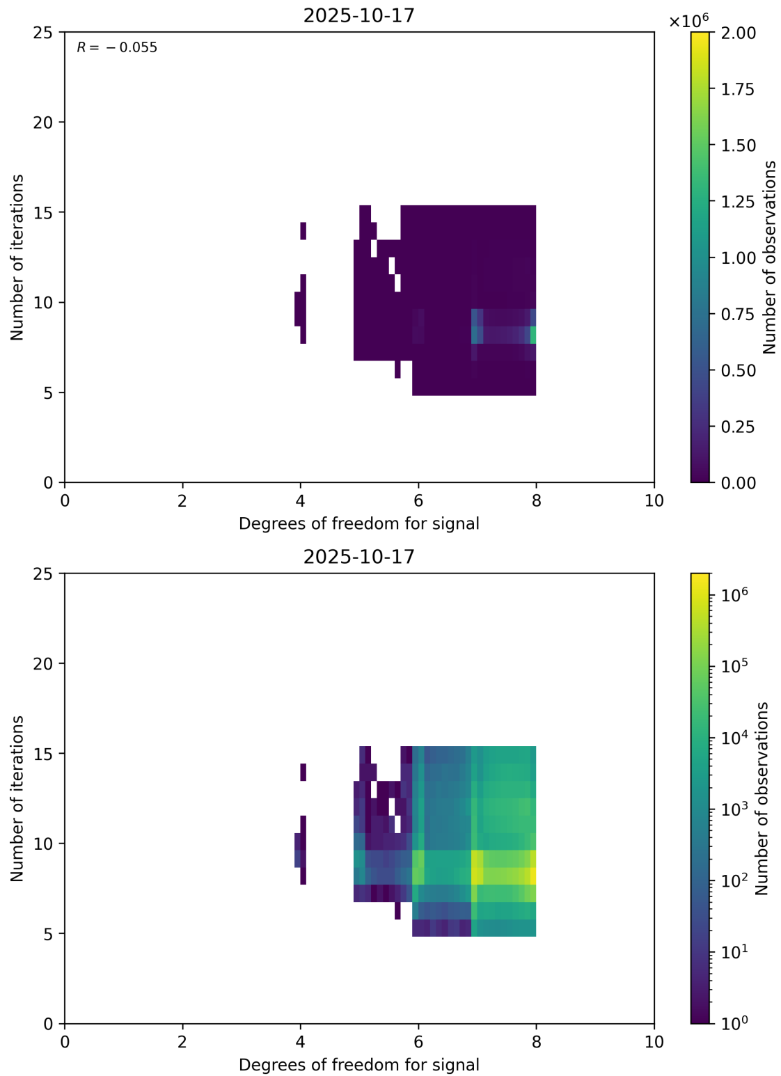
Figure 50: Scatter density plot of “Degrees of freedom for signal” against “Number of iterations” for 2025-10-17 to 2025-10-18.
