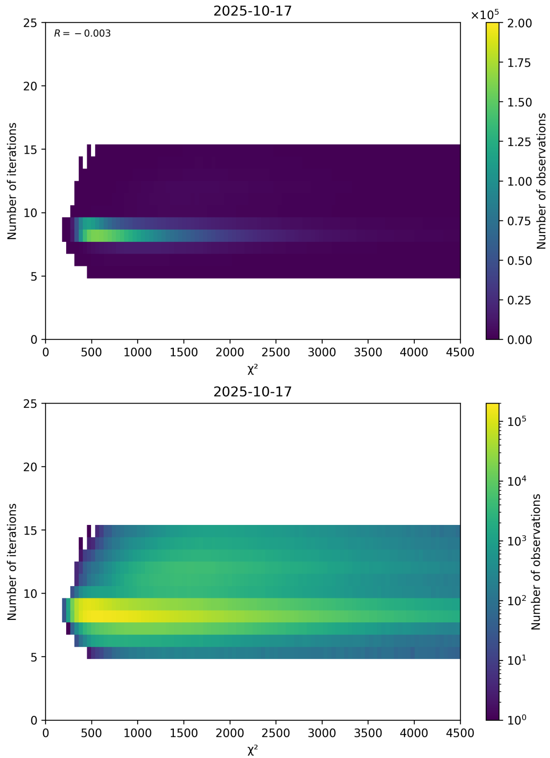
Figure 49: Scatter density plot of “ \chi^2 ” against “Number of iterations” for 2025-10-17 to 2025-10-18.
