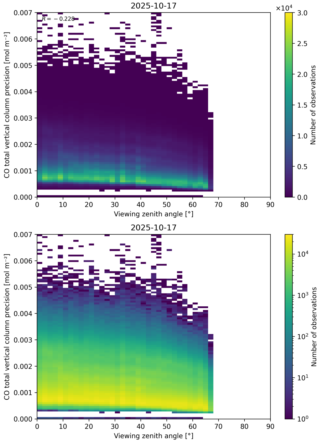
Figure 71: Scatter density plot of “Viewing zenith angle” against “CO total vertical column precision” for 2025-10-17 to 2025-10-18.
