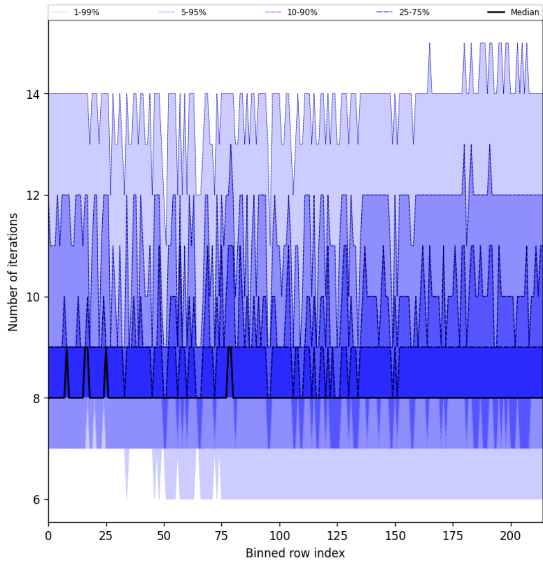
Figure 32: Along track statistics of “Number of iterations” for 2025-10-17 to 2025-10-18
