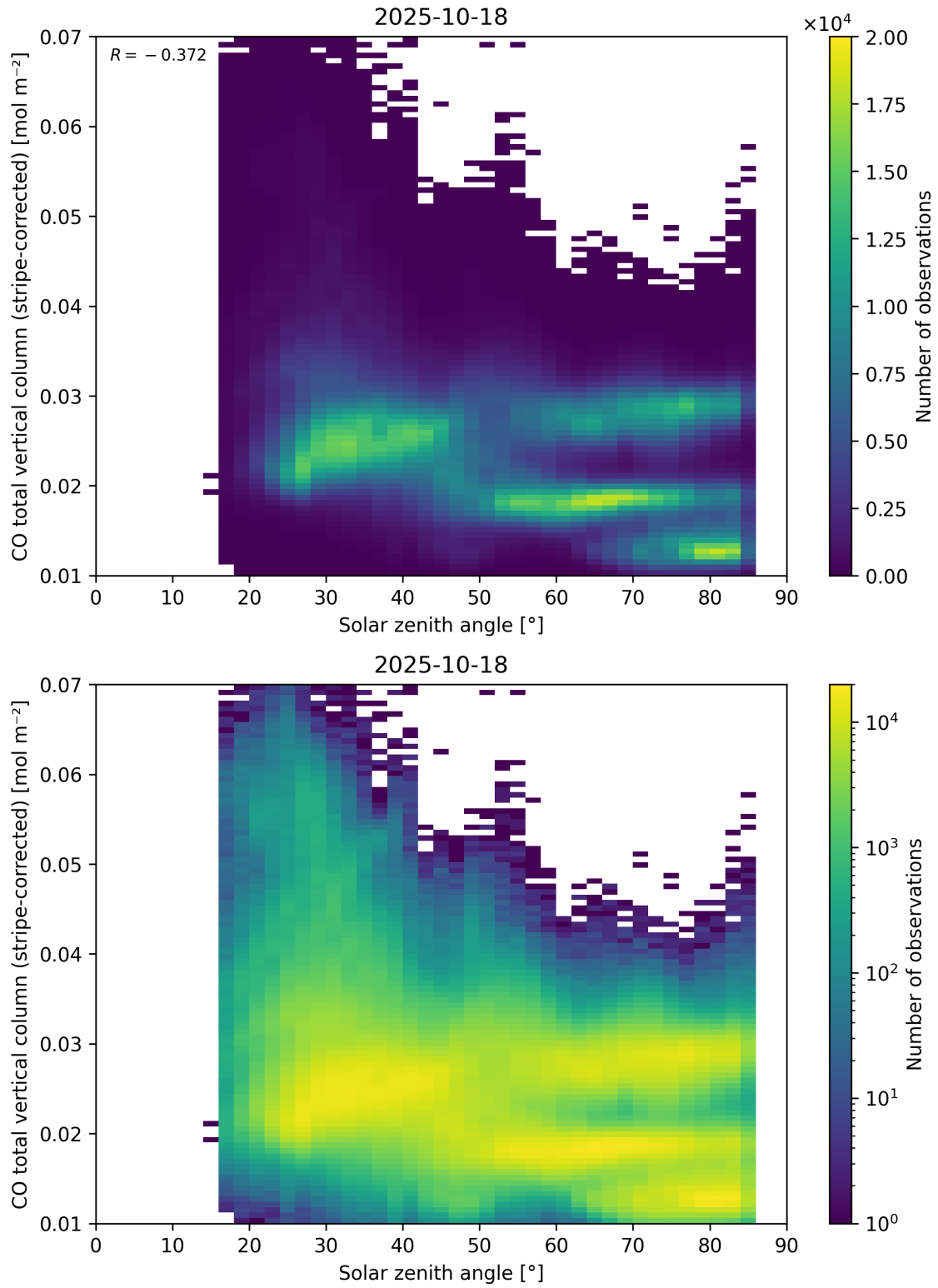
Figure 62: Scatter density plot of “Solar zenith angle” against “CO total vertical column (stripe-corrected)” for 2025-10-17 to 2025-10-19.
