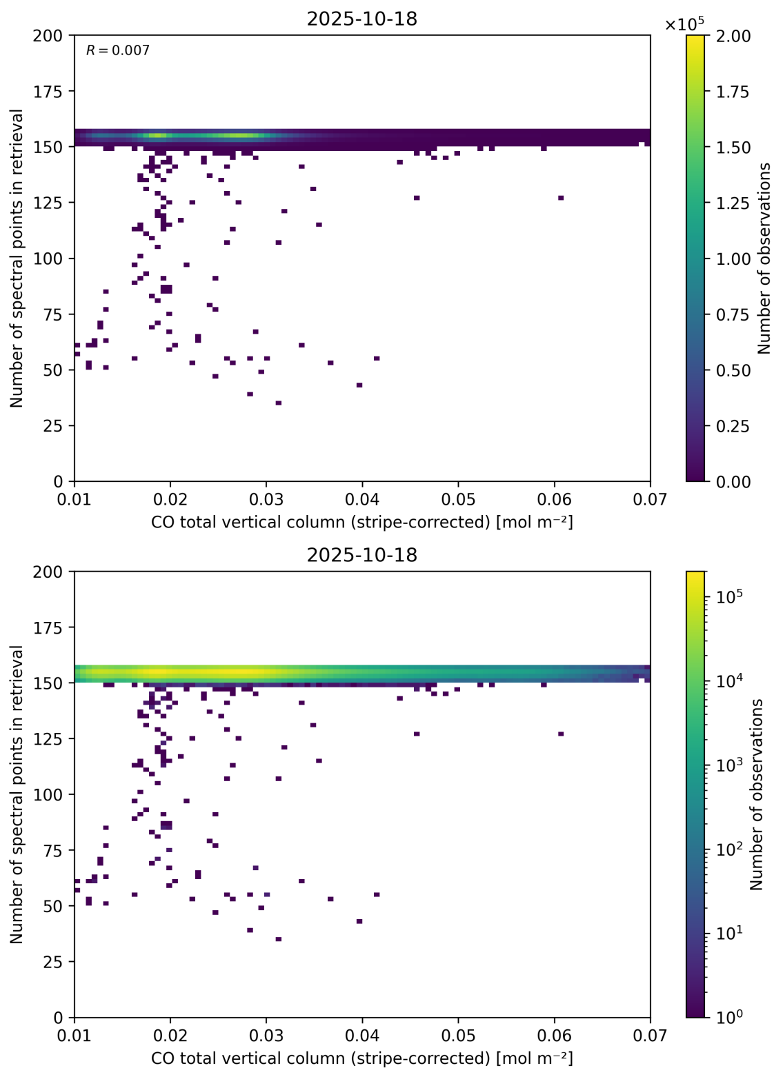
Figure 40: Scatter density plot of “CO total vertical column (stripe-corrected)” against “Number of spectral points in retrieval” for 2025-10-17 to 2025-10-19.
