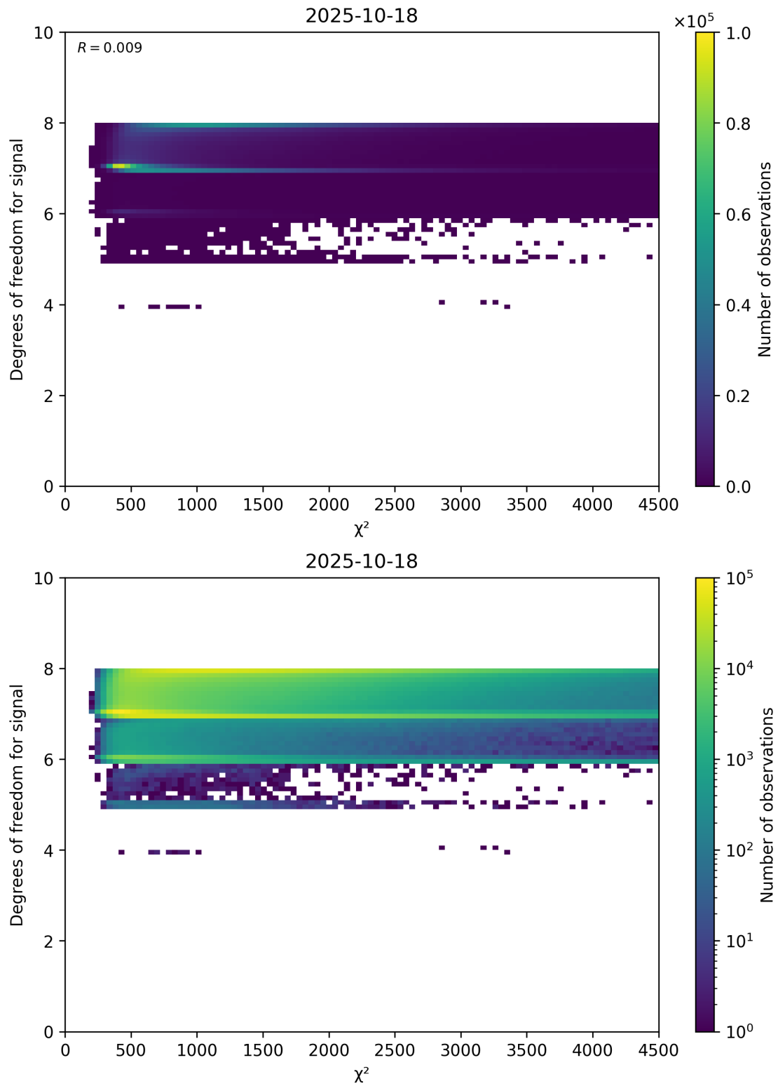
Figure 48: Scatter density plot of “ \chi^2 ” against “Degrees of freedom for signal” for 2025-10-17 to 2025-10-19.
