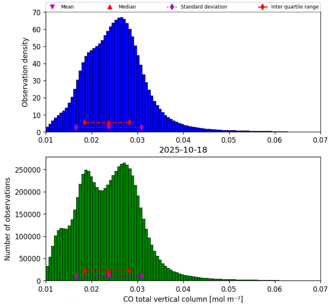
Figure 18: Histogram of “CO total vertical column” for 2025-10-17 to 2025-10-19
