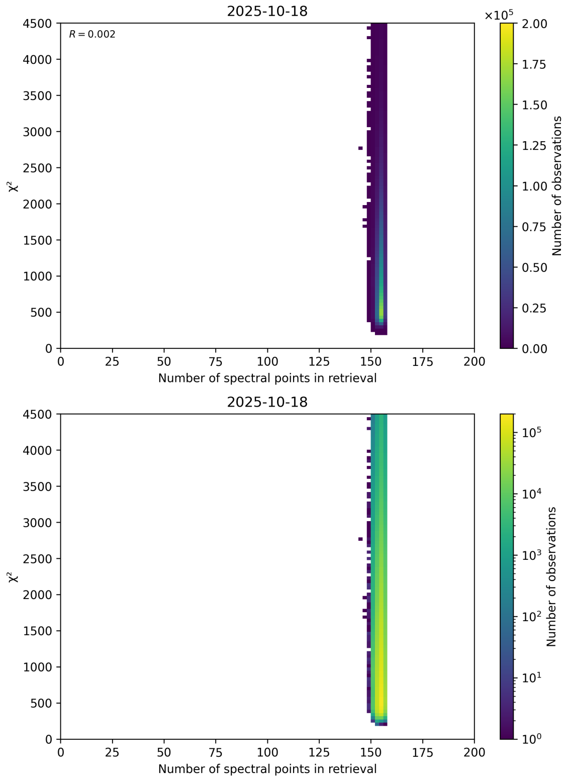
Figure 58: Scatter density plot of “Number of spectral points in retrieval” against “ \chi^2 ” for 2025-10-17 to 2025-10-19.
