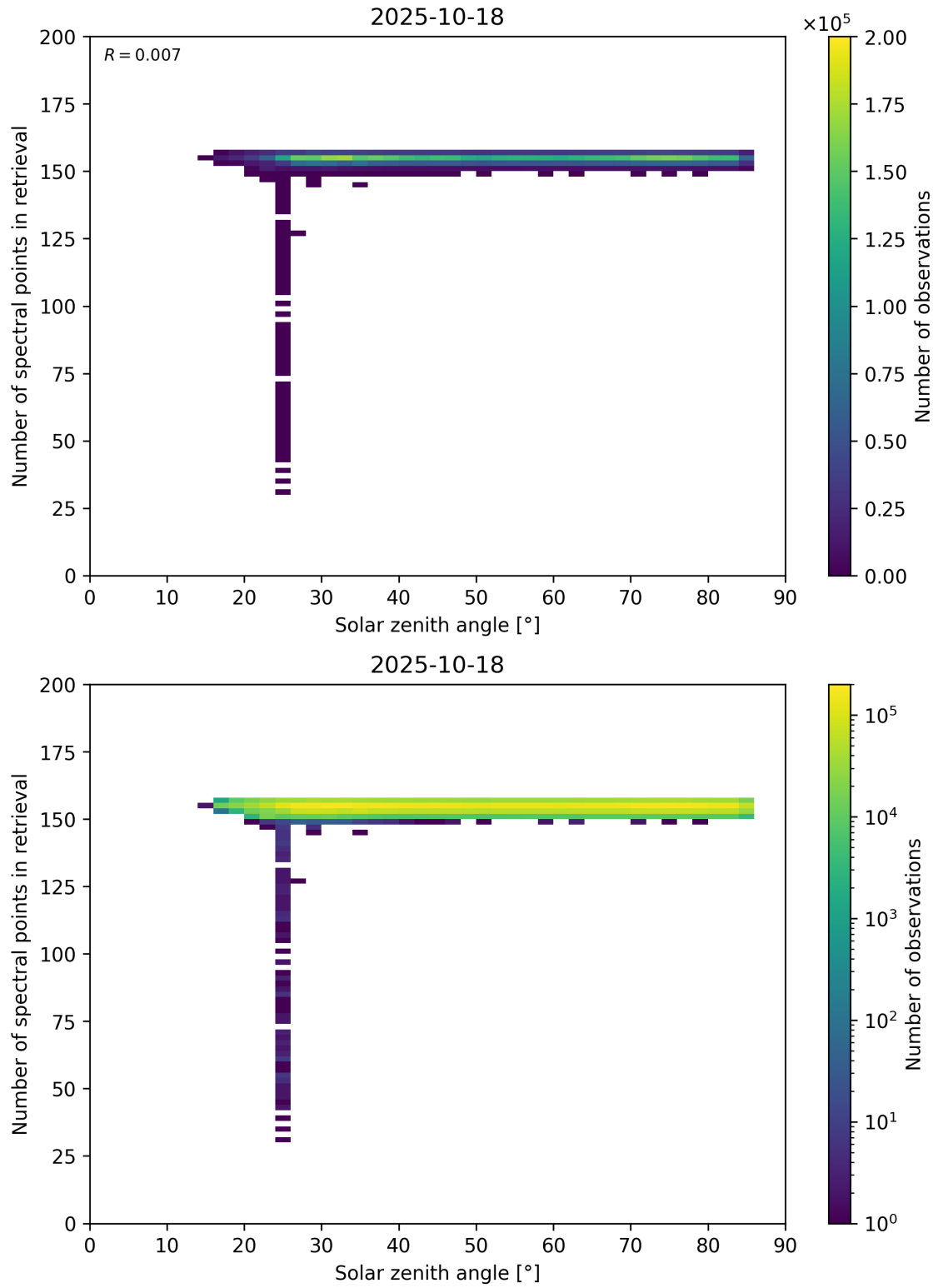
Figure 68: Scatter density plot of “Solar zenith angle” against “Number of spectral points in retrieval” for 2025-10-17 to 2025-10-19.
