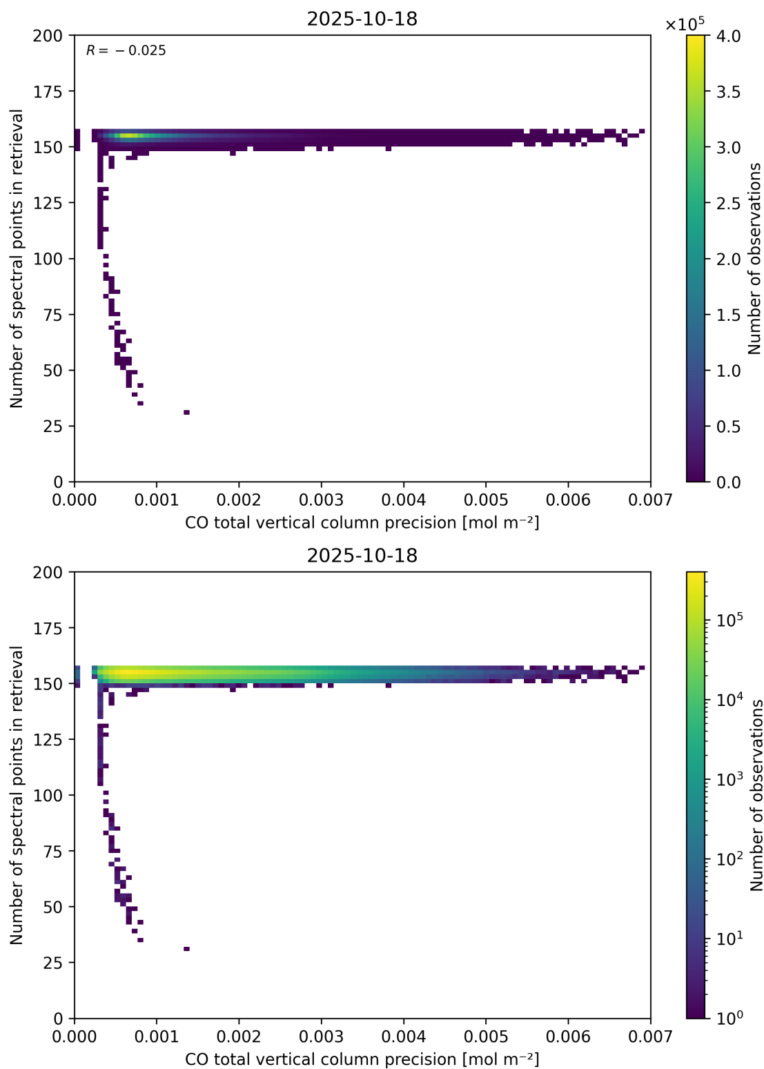
Figure 47: Scatter density plot of “CO total vertical column precision” against “Number of spectral points in retrieval” for 2025-10-17 to 2025-10-19.
