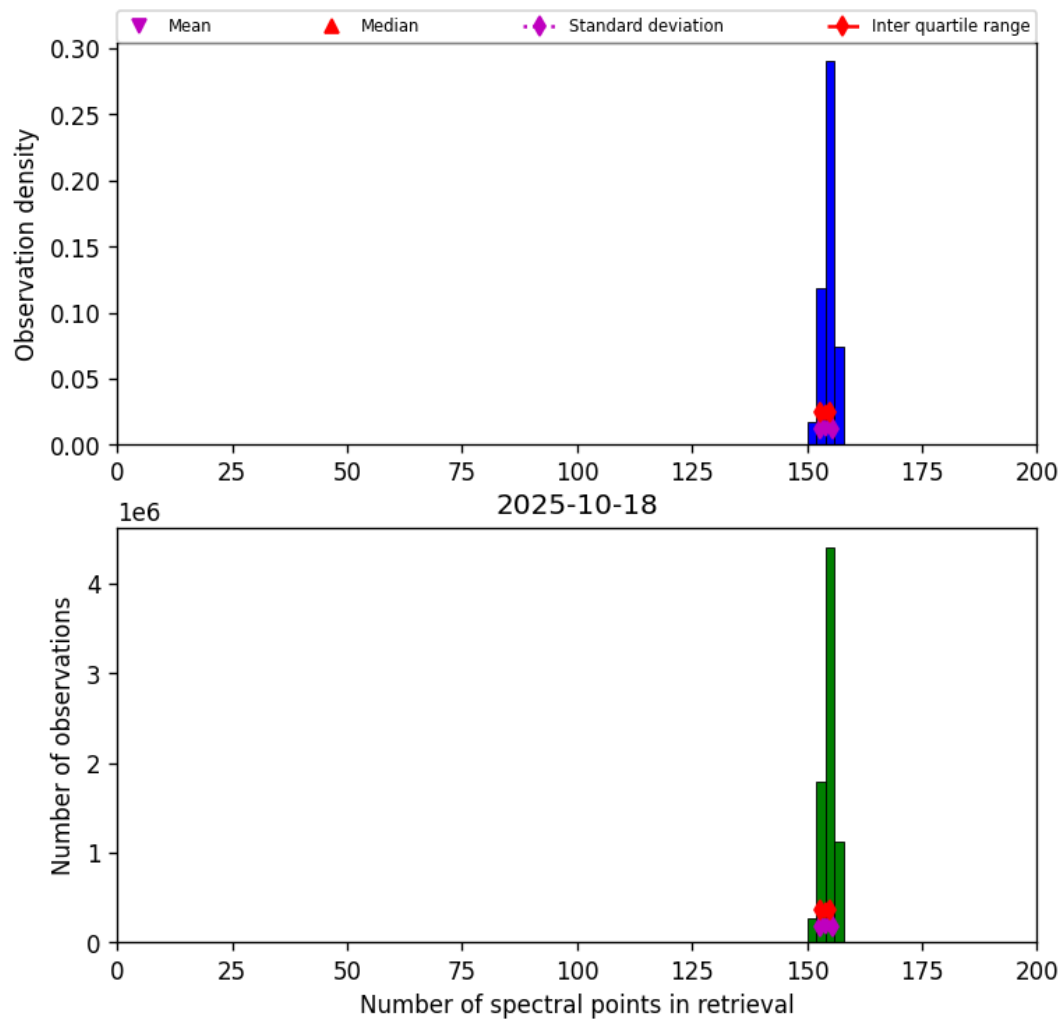
Figure 21: Histogram of “Number of spectral points in retrieval” for 2025-10-17 to 2025-10-19
