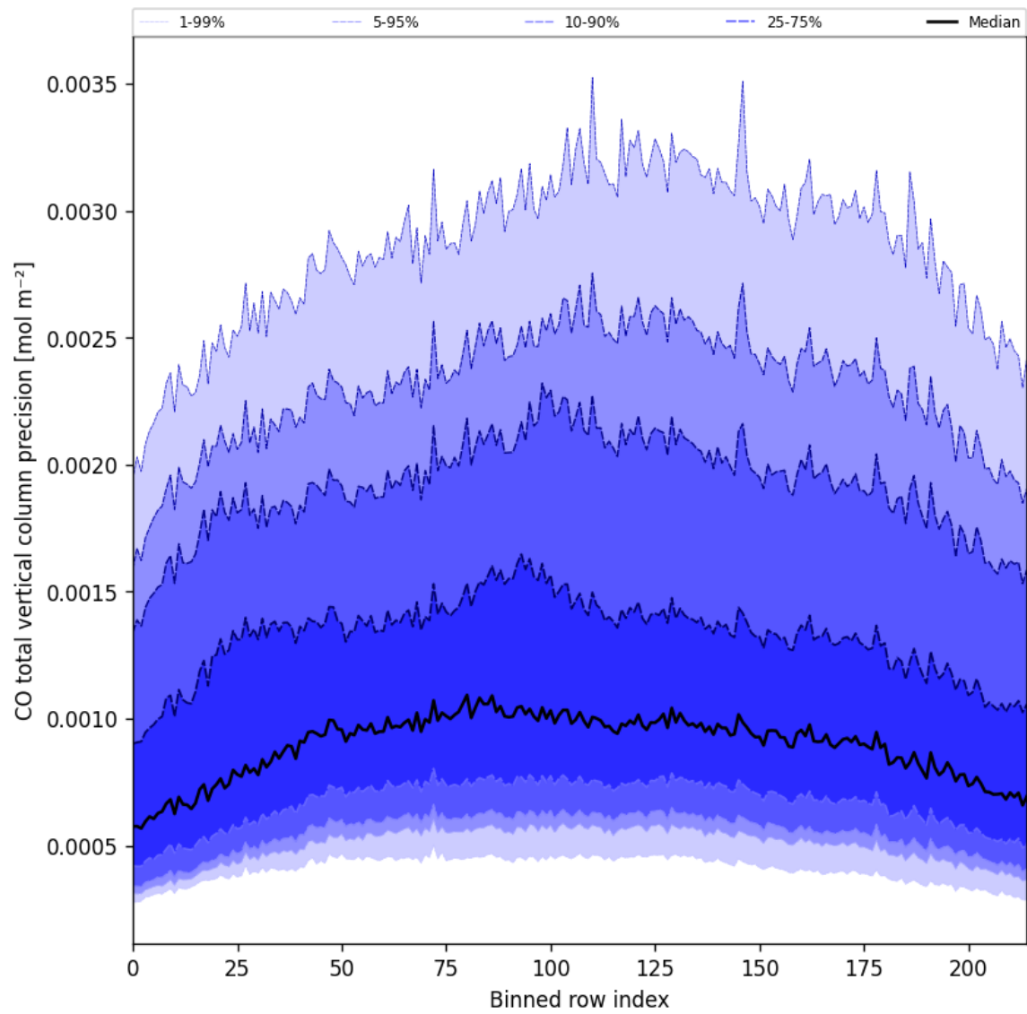
Figure 28: Along track statistics of “CO total vertical column precision” for 2025-10-17 to 2025-10-19
