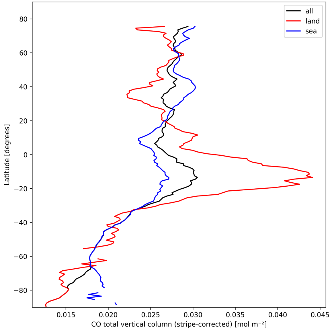
Figure 11: Zonal average of “CO total vertical column (stripe-corrected)” for 2025-10-17 to 2025-10-19.
