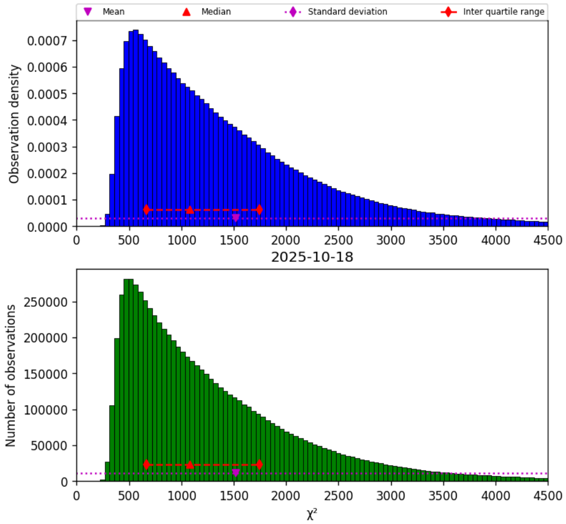
Figure 22: Histogram of “ \chi^2 ” for 2025-10-17 to 2025-10-19
