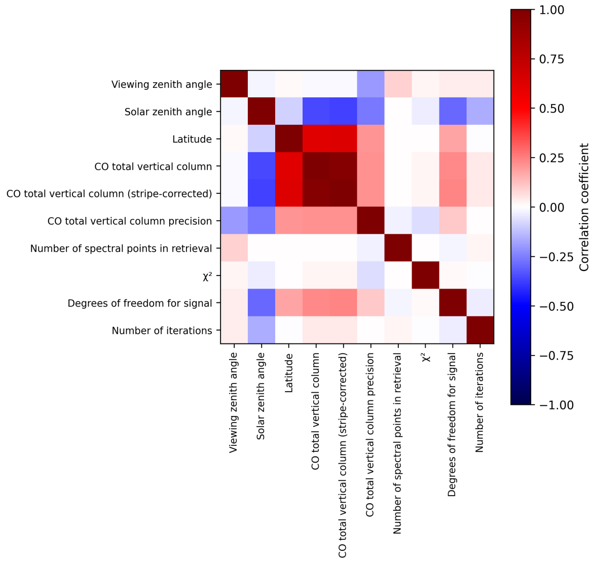
Figure 2: Map of correlation matrix for 2025-10-17 to 2025-10-19.
