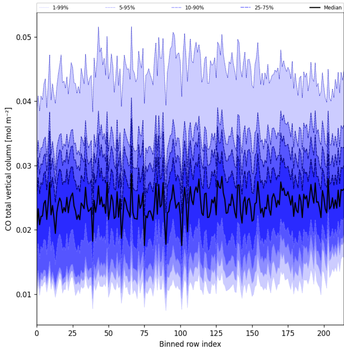
Figure 26: Along track statistics of “CO total vertical column” for 2025-10-17 to 2025-10-19
