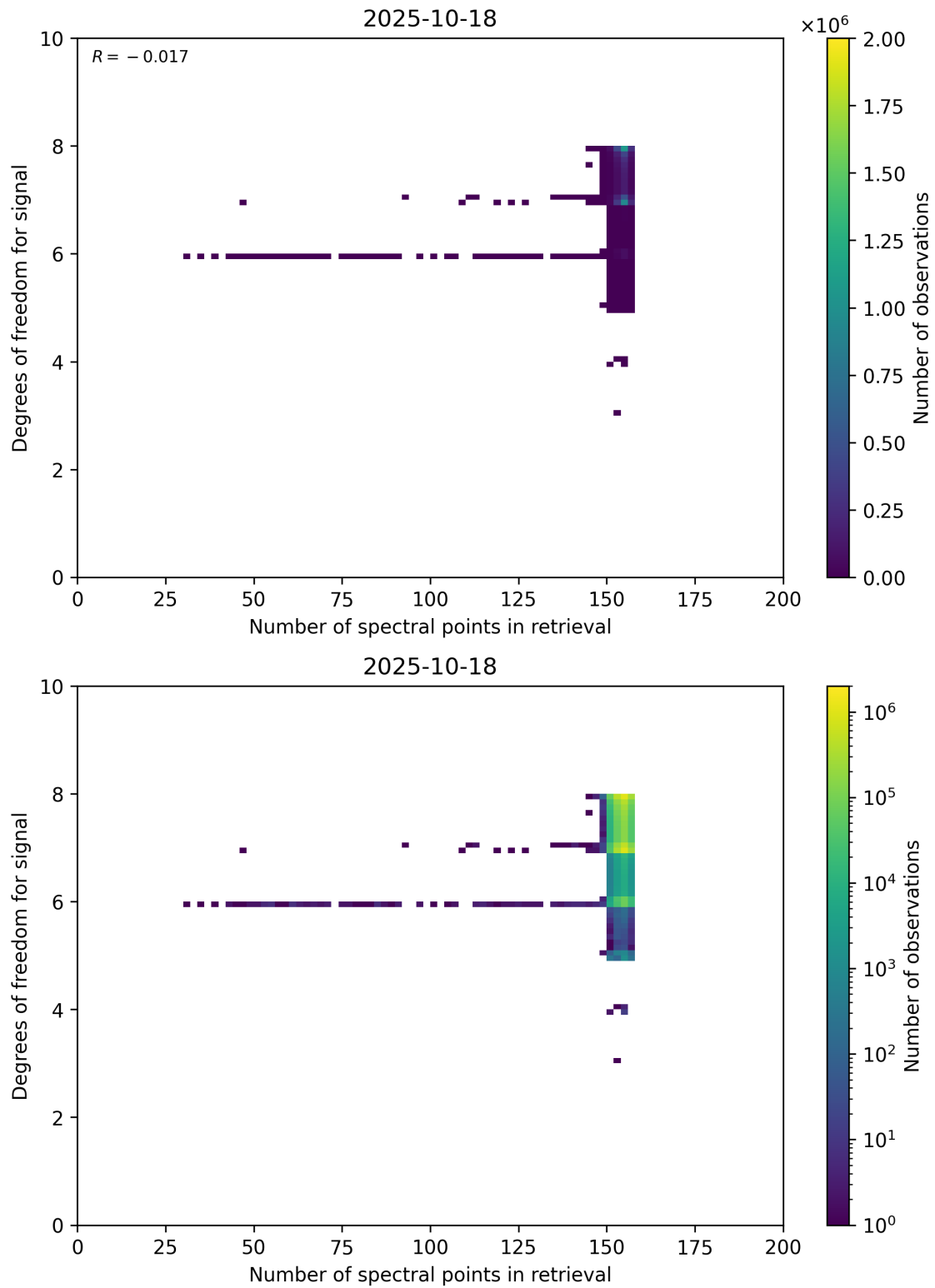
Figure 59: Scatter density plot of “Number of spectral points in retrieval” against “Degrees of freedom for signal” for 2025-10-17 to 2025-10-19.
