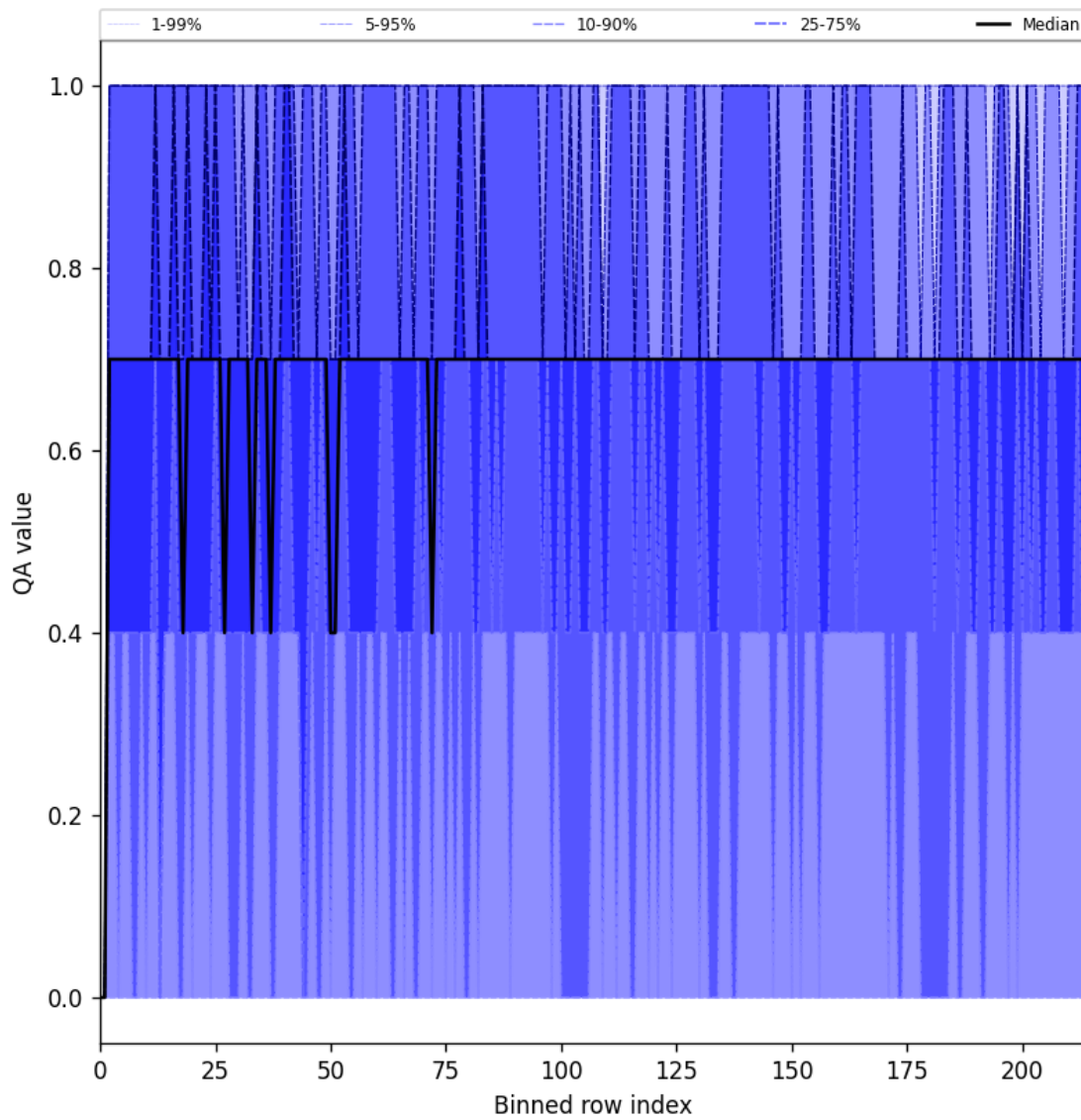
Figure 25: Along track statistics of “QA value” for 2025-10-17 to 2025-10-19
