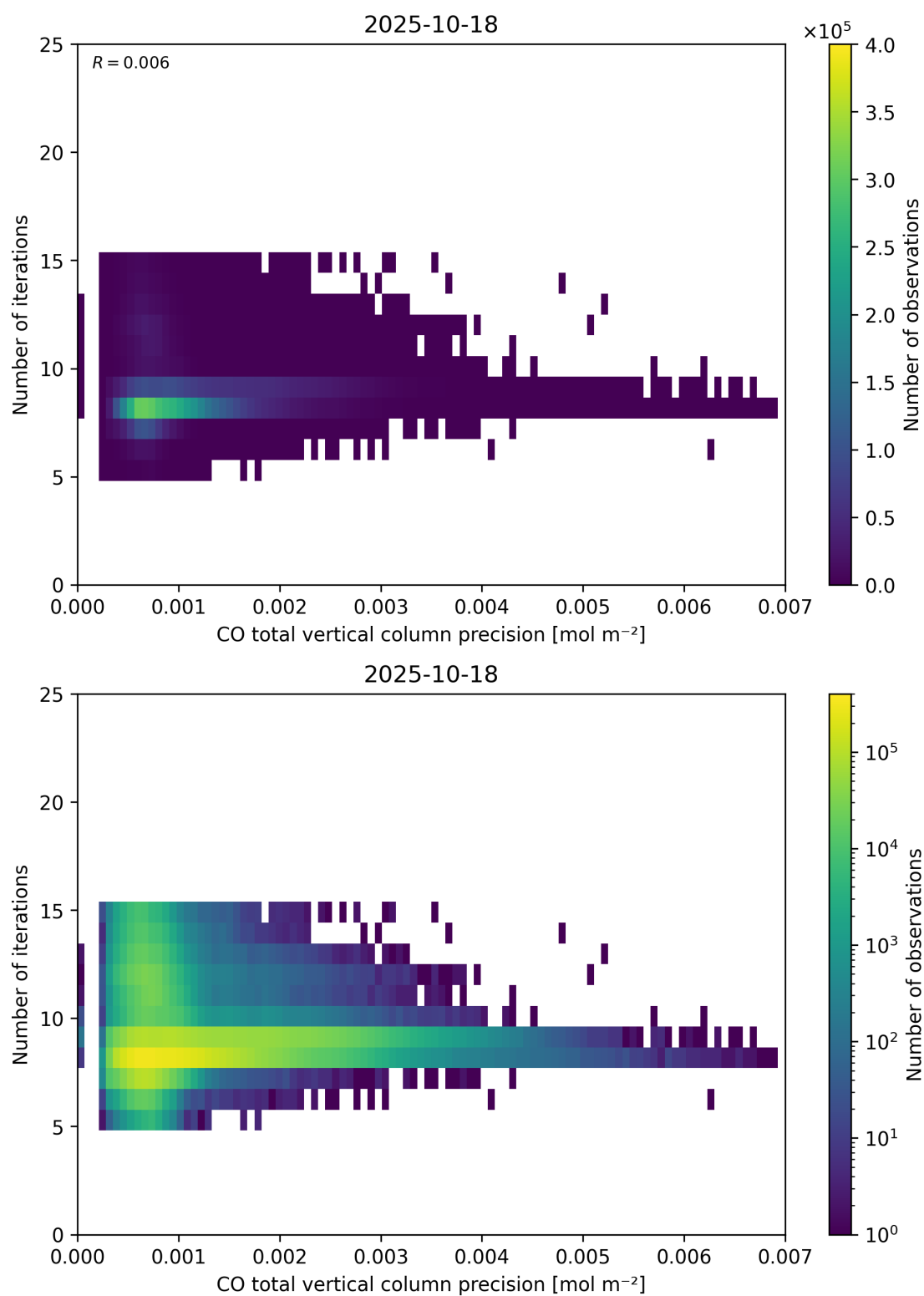
Figure 46: Scatter density plot of “CO total vertical column precision” against “Number of iterations” for 2025-10-17 to 2025-10-19.
