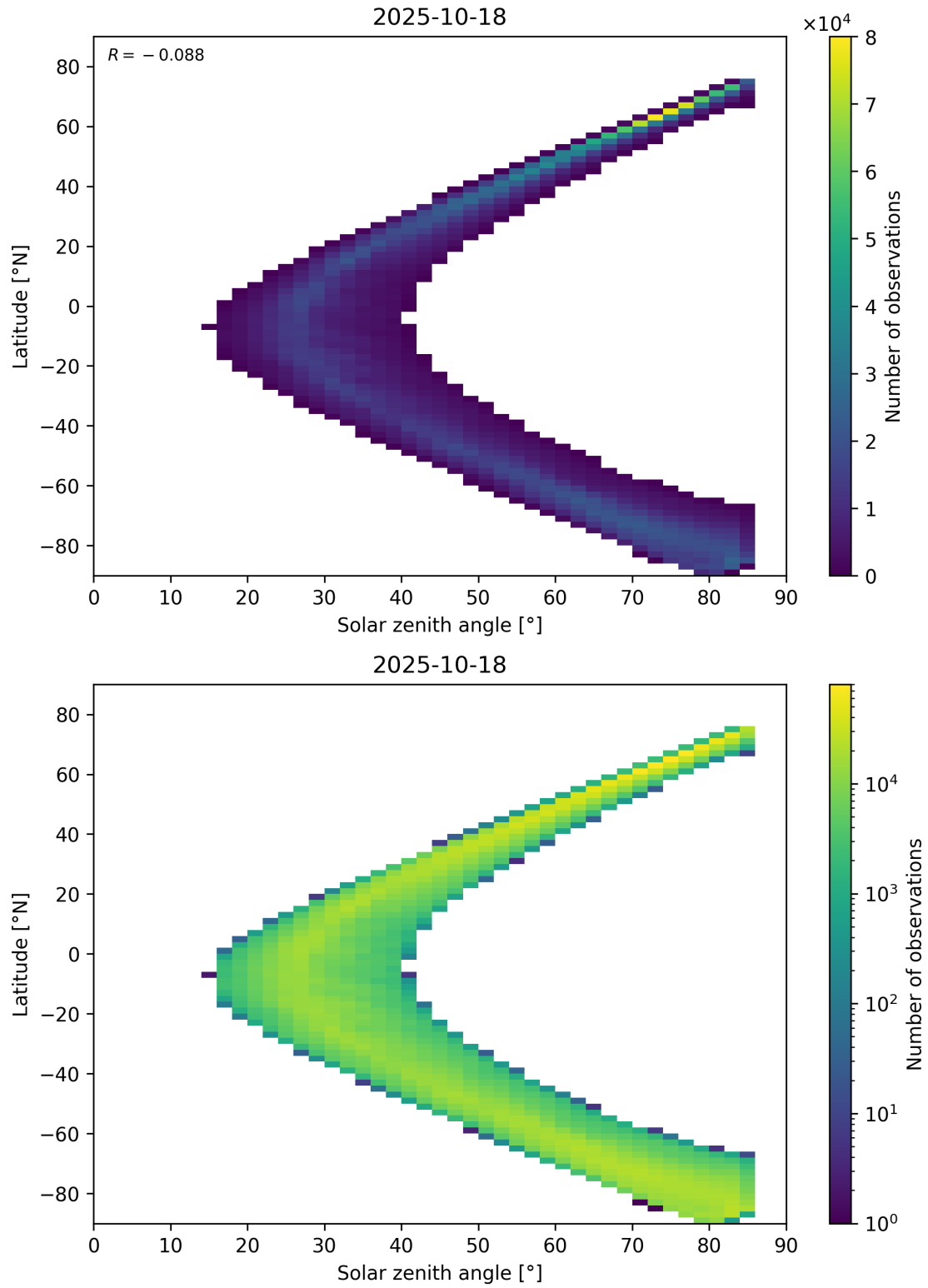
Figure 66: Scatter density plot of “Solar zenith angle” against “Latitude” for 2025-10-17 to 2025-10-19.
