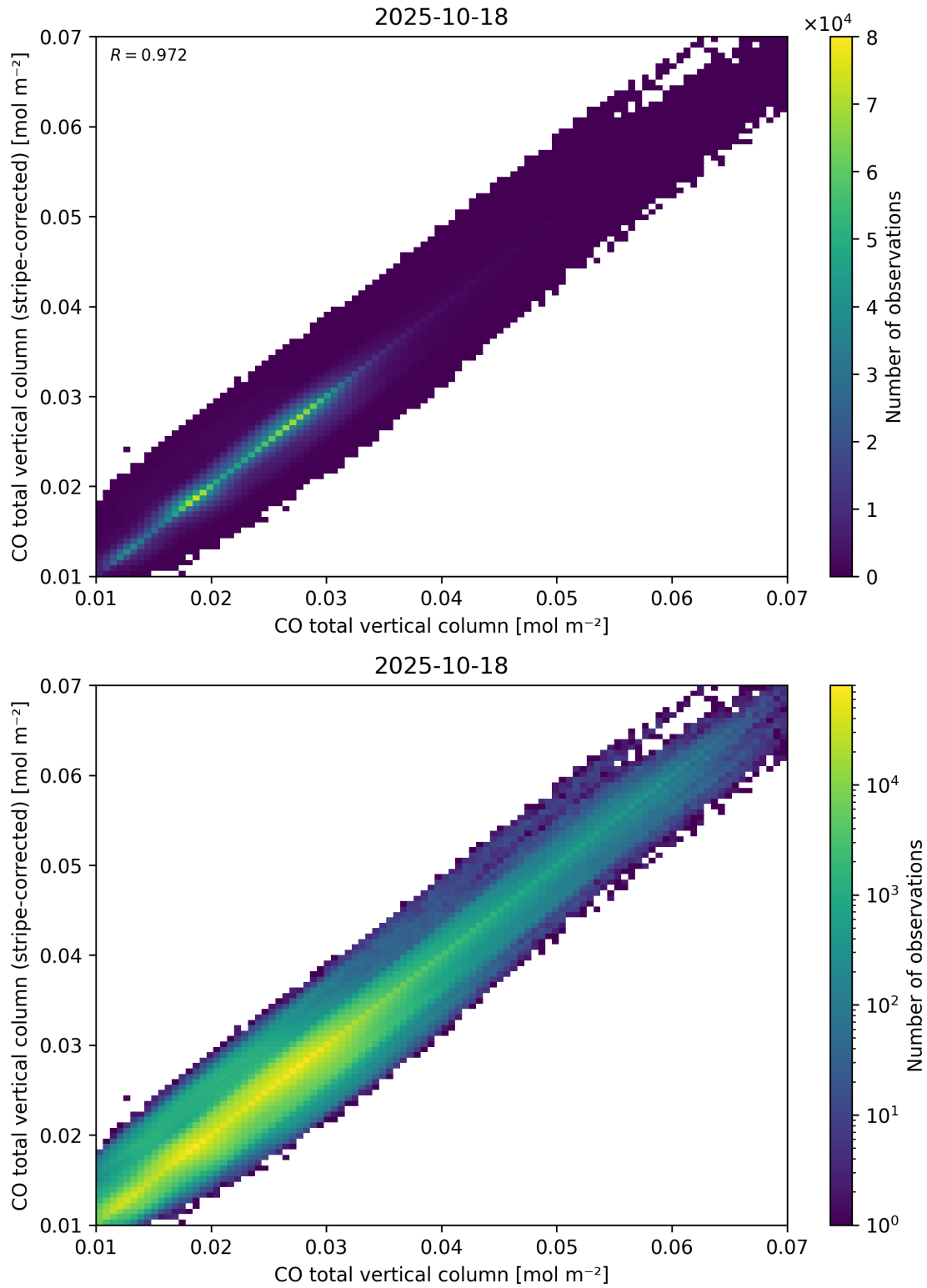
Figure 33: Scatter density plot of “CO total vertical column” against “CO total vertical column (stripe-corrected)” for 2025-10-17 to 2025-10-19.
