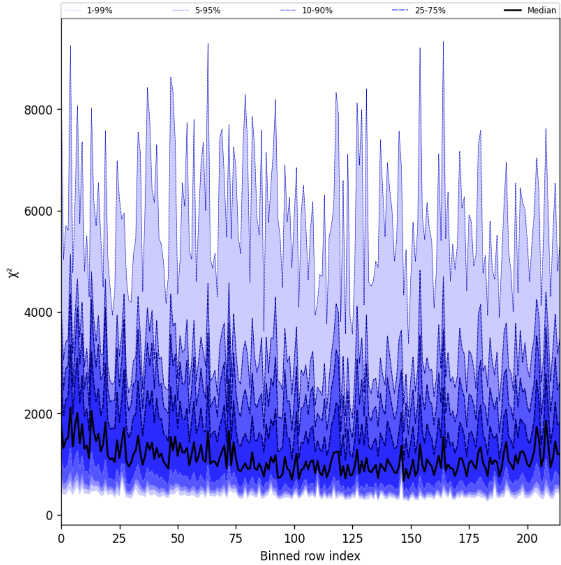
Figure 30: Along track statistics of “ \chi^2 ” for 2025-10-17 to 2025-10-19
