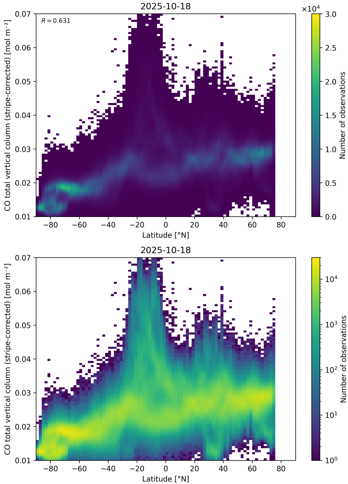
Figure 52: Scatter density plot of “Latitude” against “CO total vertical column (stripe-corrected)” for 2025-10-17 to 2025-10-19.
