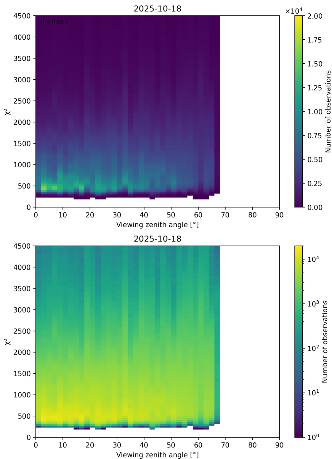
Figure 72: Scatter density plot of “Viewing zenith angle” against “ \chi^2 ” for 2025-10-17 to 2025-10-19.
