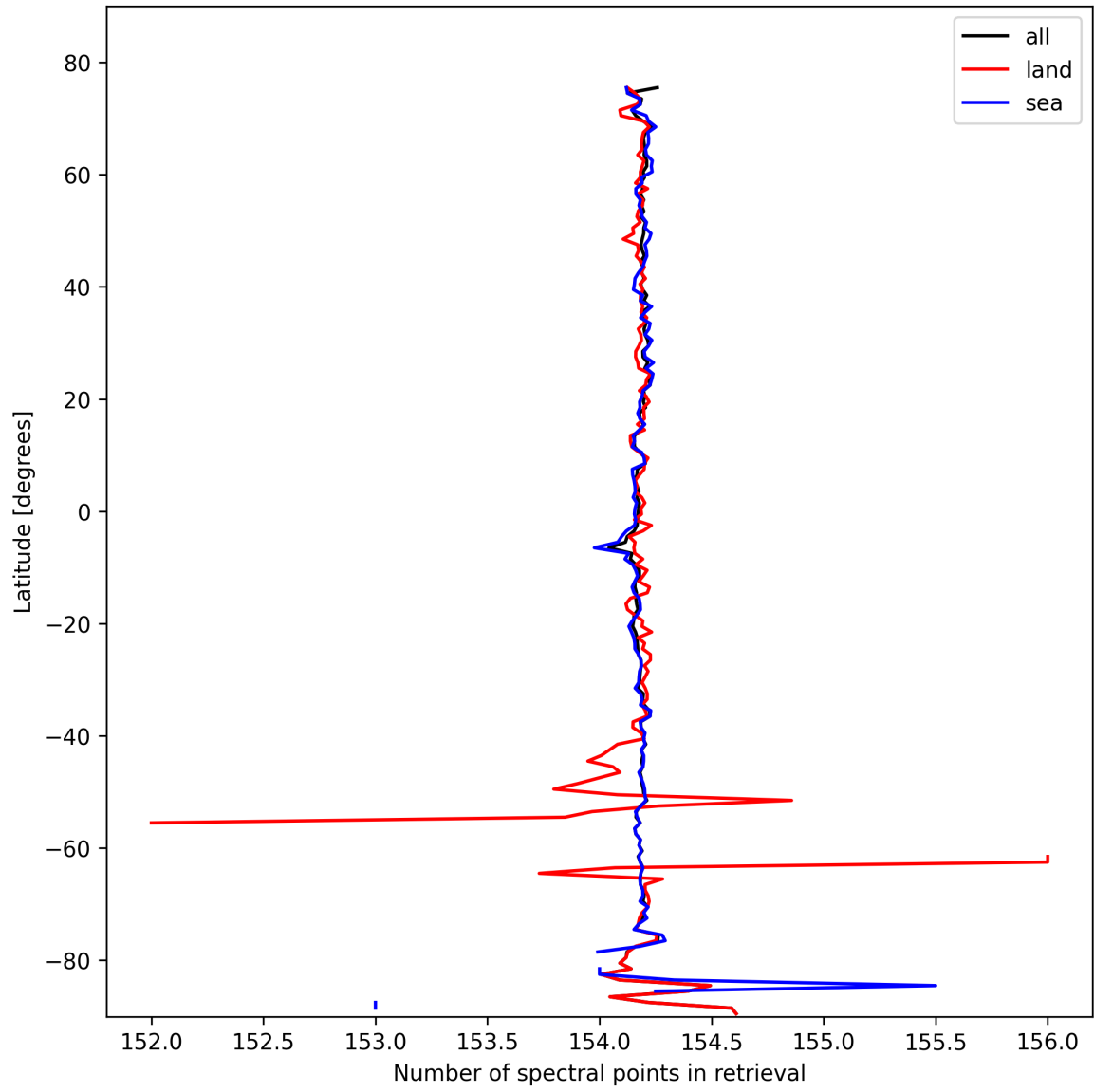
Figure 13: Zonal average of “Number of spectral points in retrieval” for 2025-10-17 to 2025-10-19.
