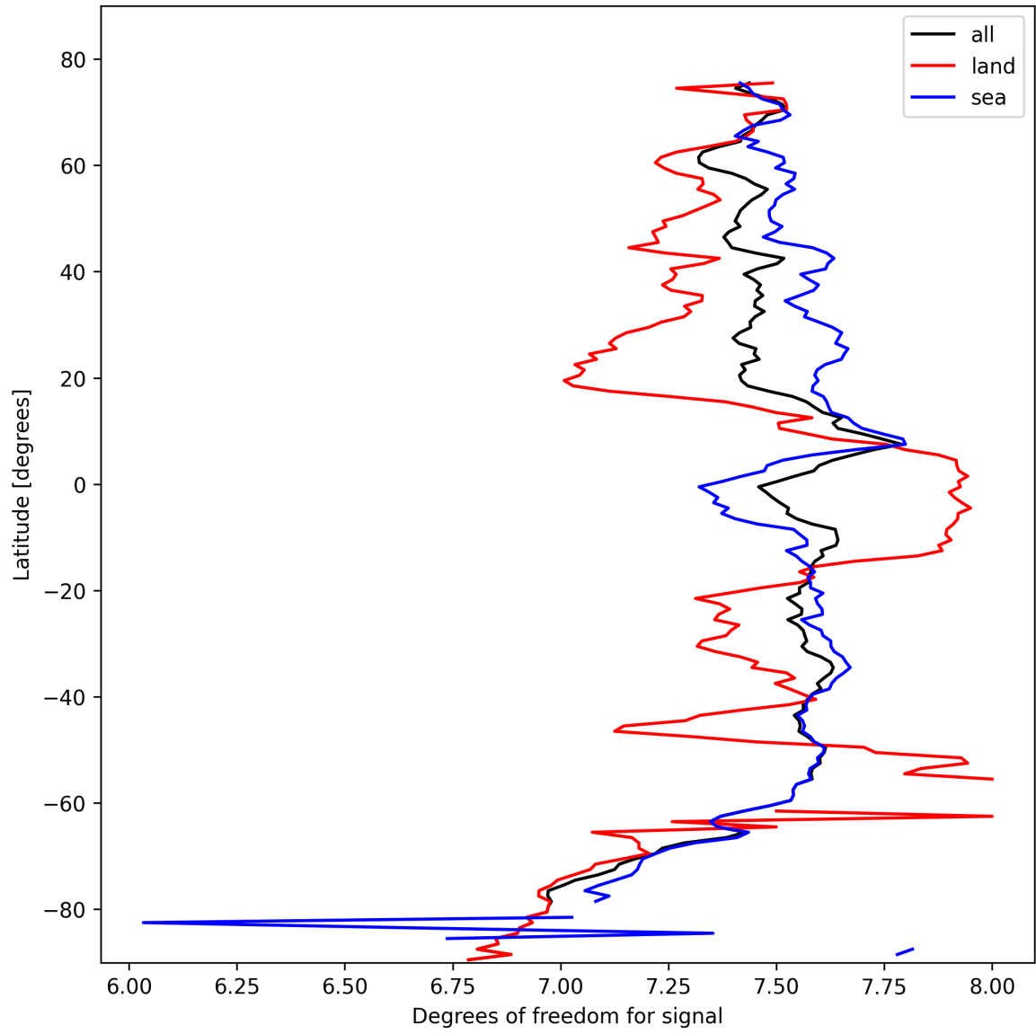
Figure 15: Zonal average of “Degrees of freedom for signal” for 2025-10-17 to 2025-10-19.
