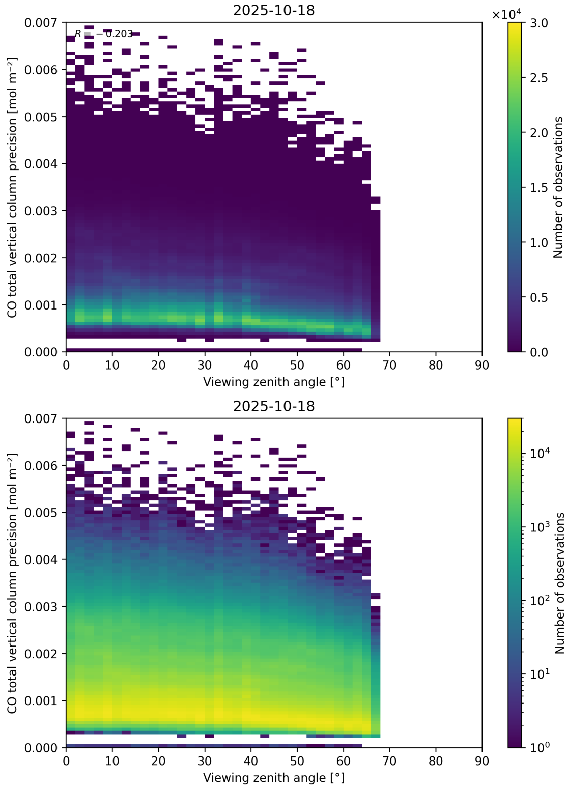
Figure 71: Scatter density plot of “Viewing zenith angle” against “CO total vertical column precision” for 2025-10-17 to 2025-10-19.
