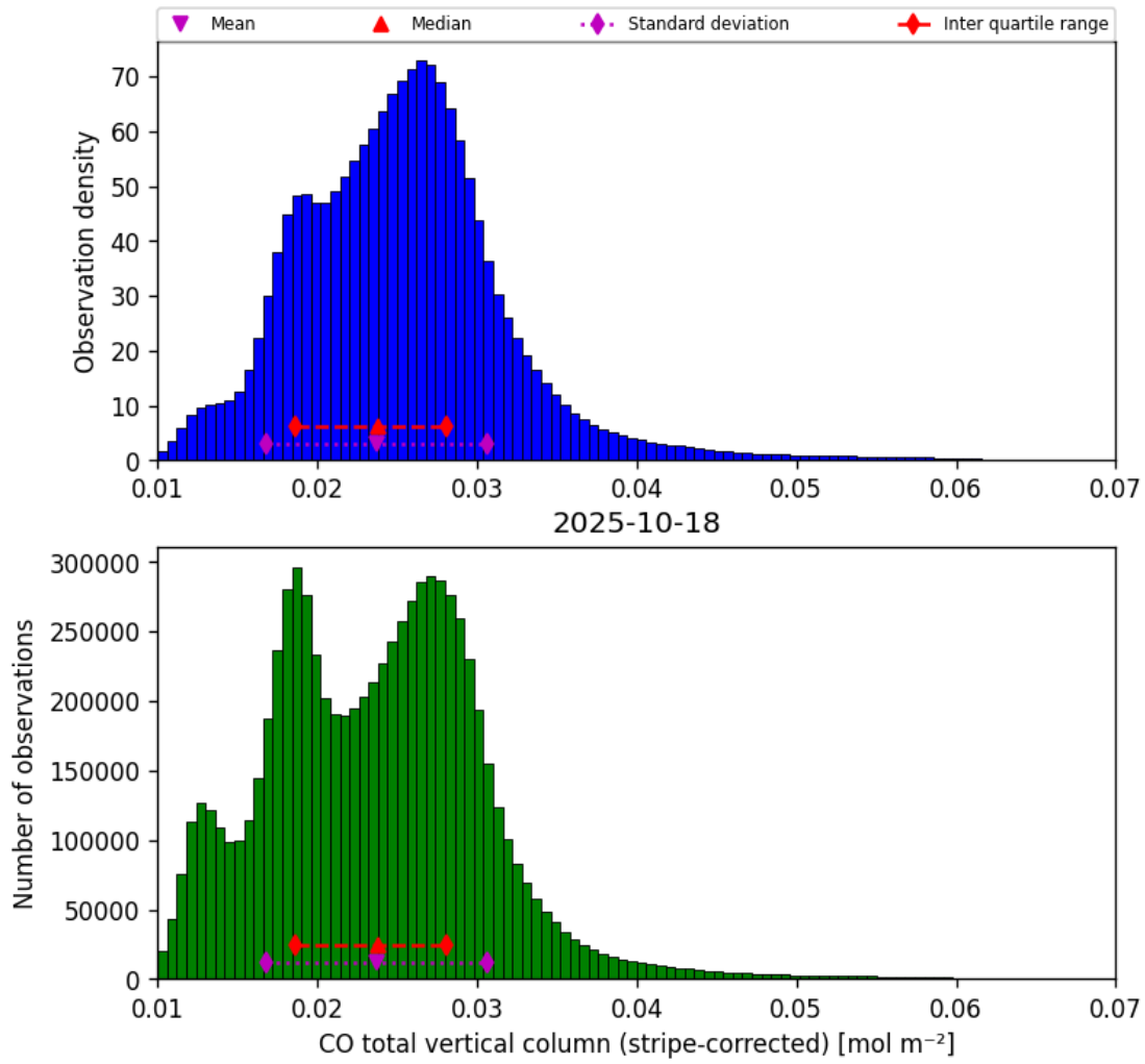
Figure 19: Histogram of “CO total vertical column (stripe-corrected)” for 2025-10-17 to 2025-10-19
