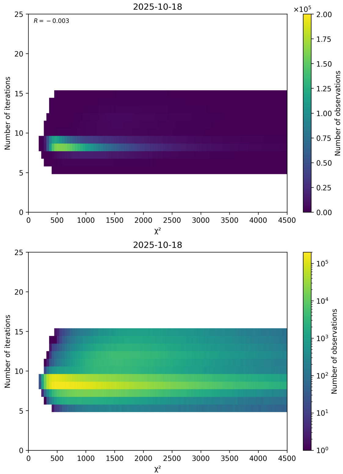
Figure 49: Scatter density plot of “ \chi^2 ” against “Number of iterations” for 2025-10-17 to 2025-10-19.
