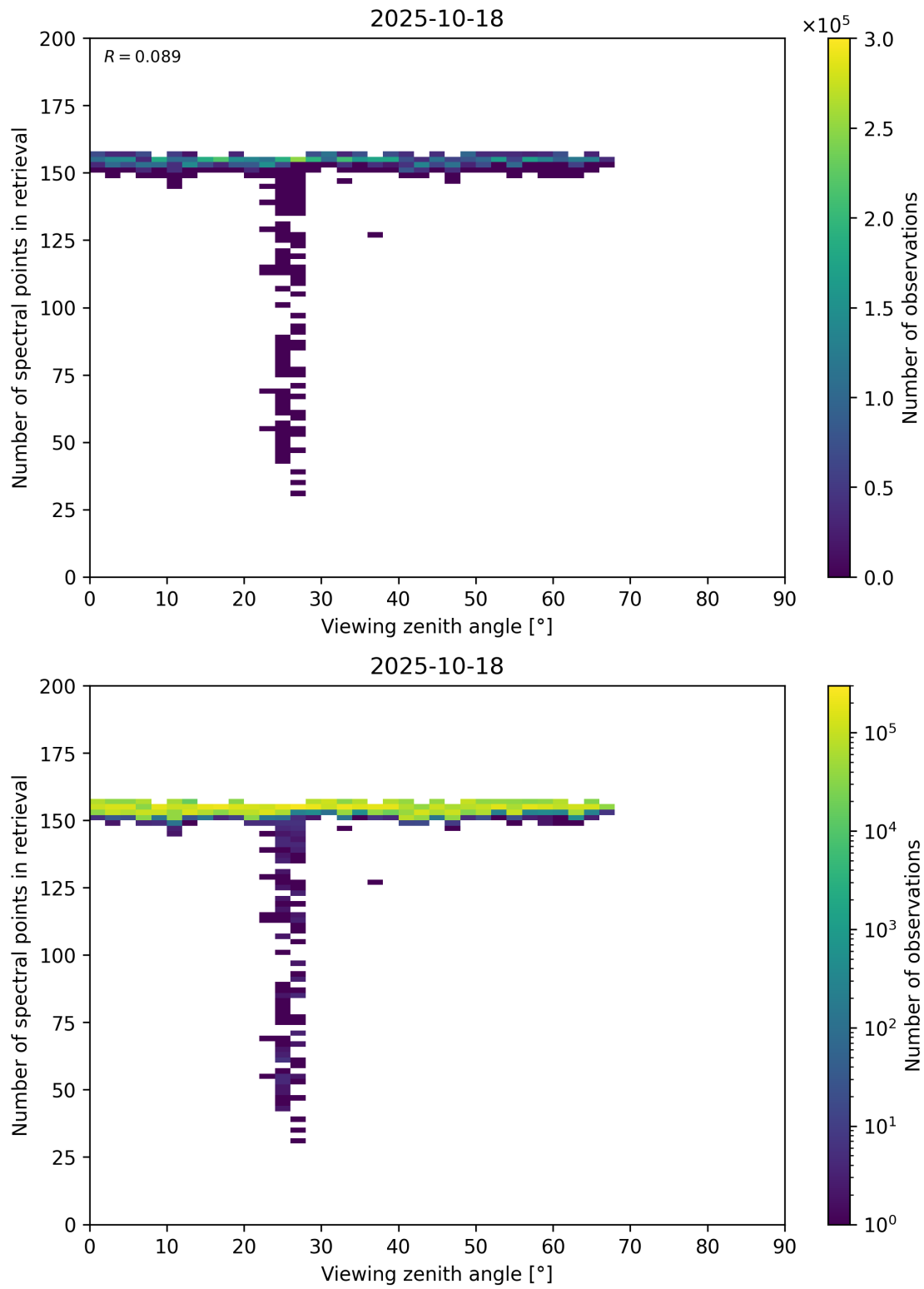
Figure 76: Scatter density plot of “Viewing zenith angle” against “Number of spectral points in retrieval” for 2025-10-17 to 2025-10-19.
