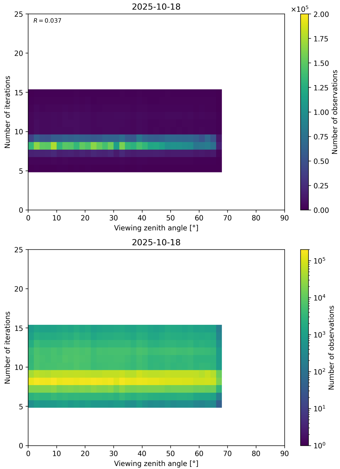
Figure 75: Scatter density plot of “Viewing zenith angle” against “Number of iterations” for 2025-10-17 to 2025-10-19.
