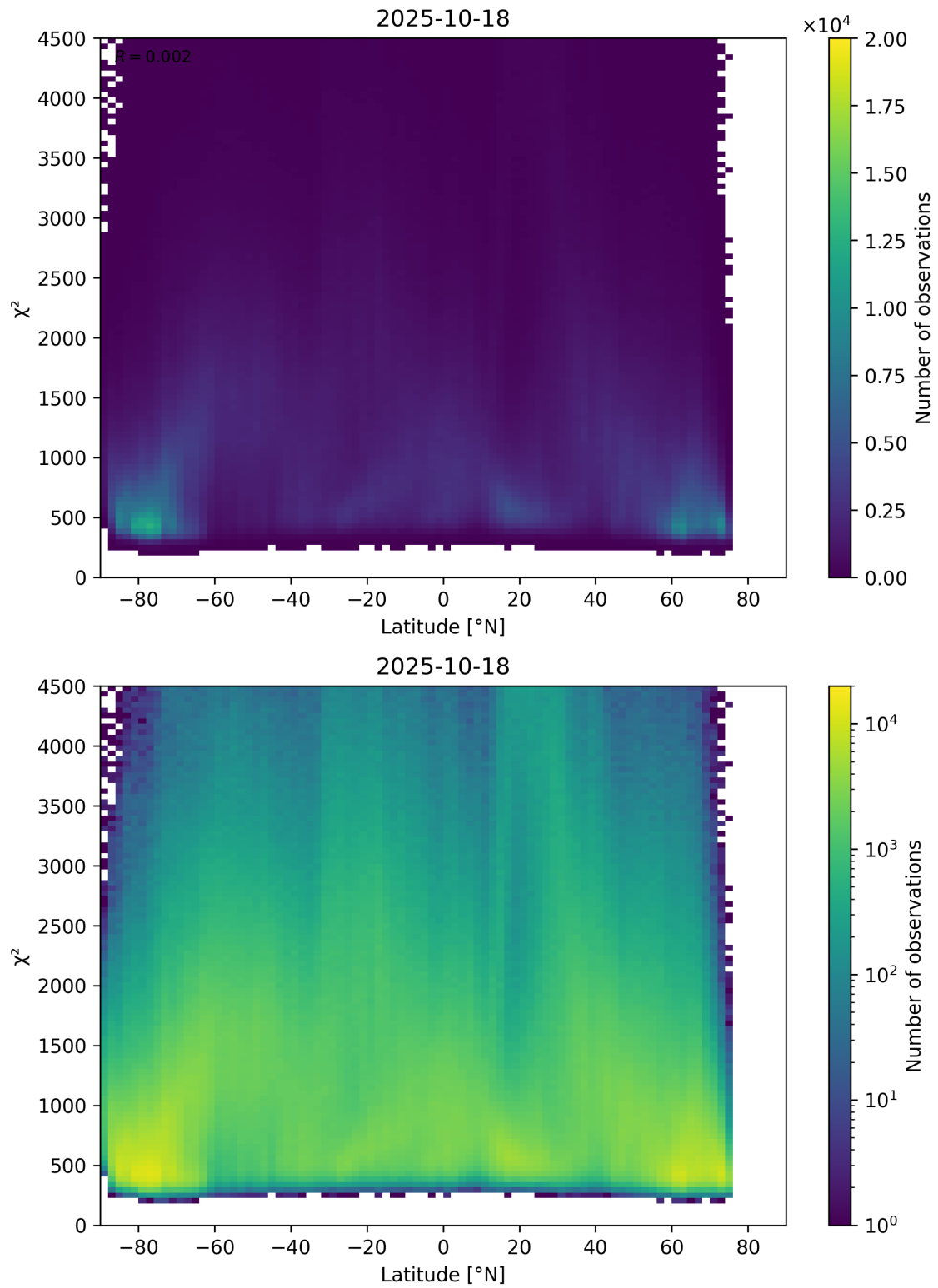
Figure 54: Scatter density plot of “Latitude” against “ \chi^2 ” for 2025-10-17 to 2025-10-19.
