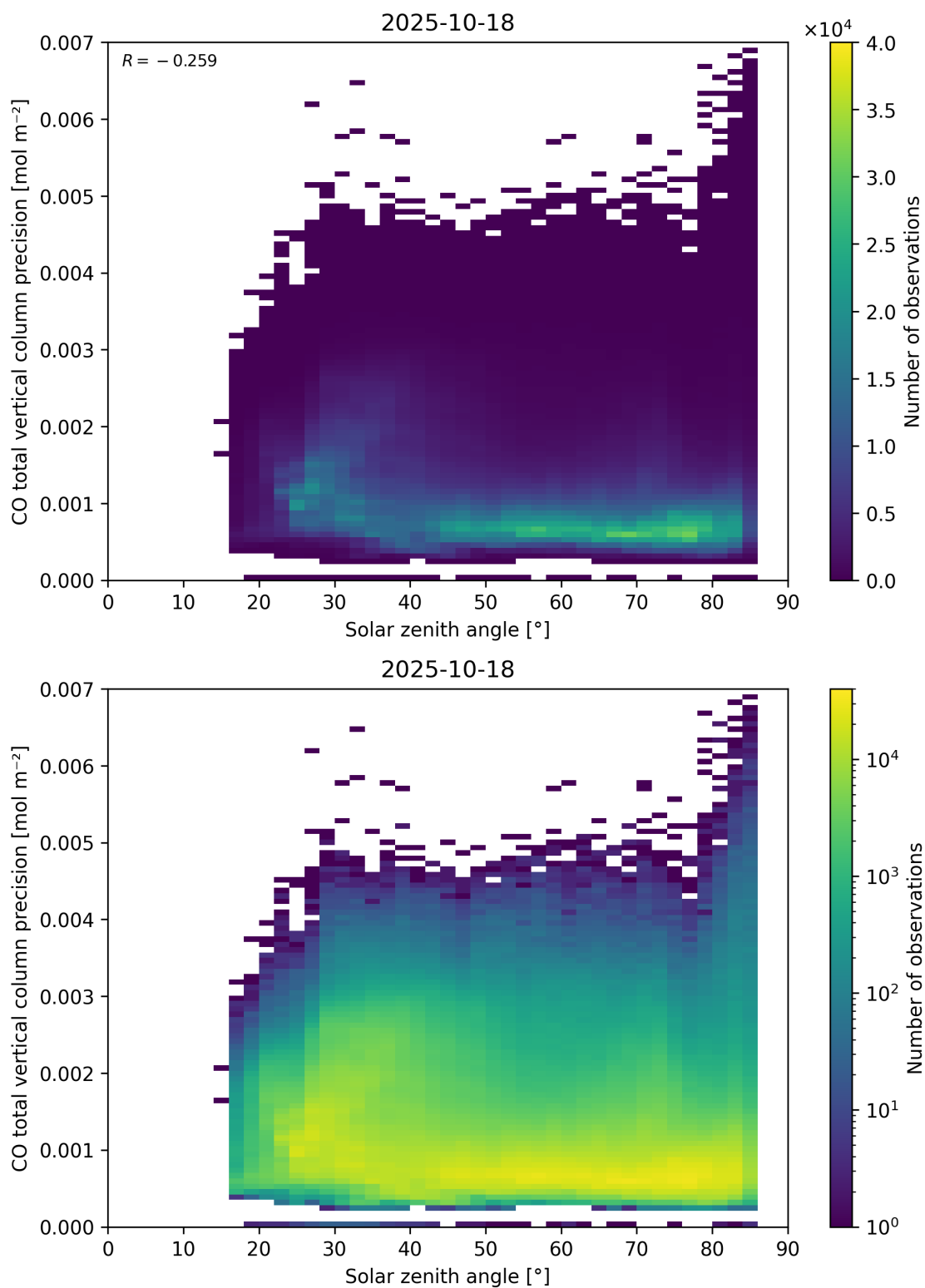
Figure 63: Scatter density plot of “Solar zenith angle” against “CO total vertical column precision” for 2025-10-17 to 2025-10-19.
