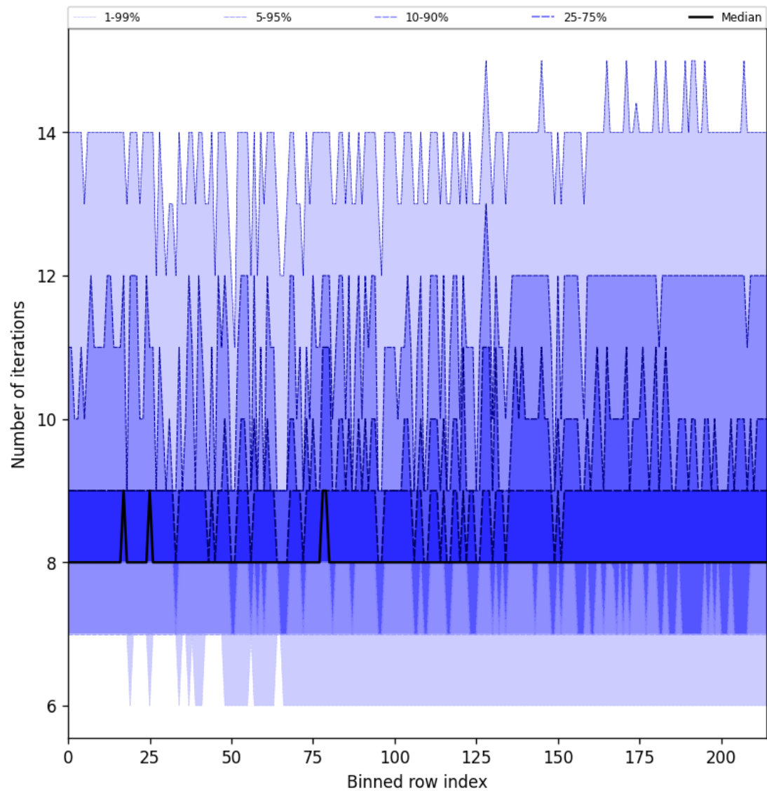
Figure 32: Along track statistics of “Number of iterations” for 2025-10-17 to 2025-10-19
