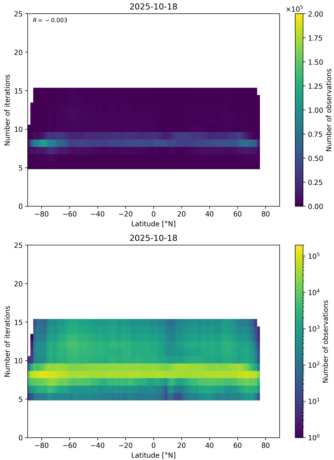
Figure 56: Scatter density plot of “Latitude” against “Number of iterations” for 2025-10-17 to 2025-10-19.
