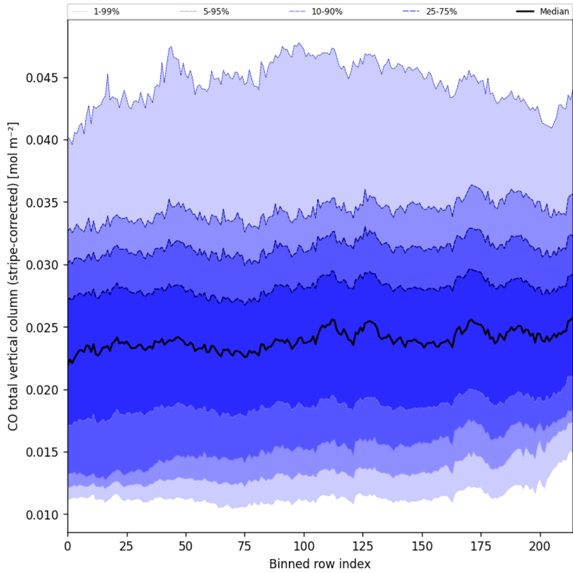
Figure 27: Along track statistics of “CO total vertical column (stripe-corrected)” for 2025-10-17 to 2025-10-19
