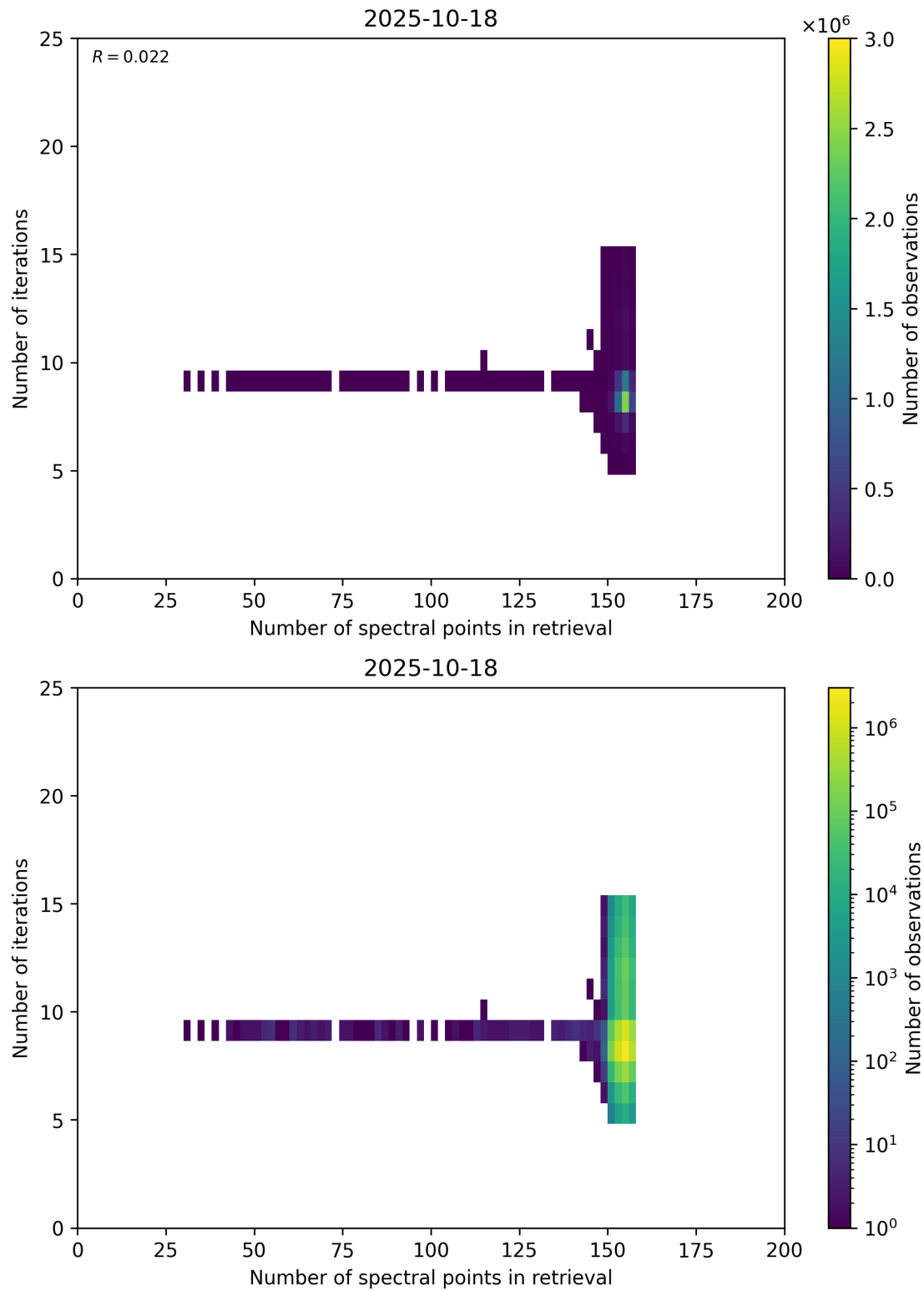
Figure 60: Scatter density plot of “Number of spectral points in retrieval” against “Number of iterations” for 2025-10-17 to 2025-10-19.
