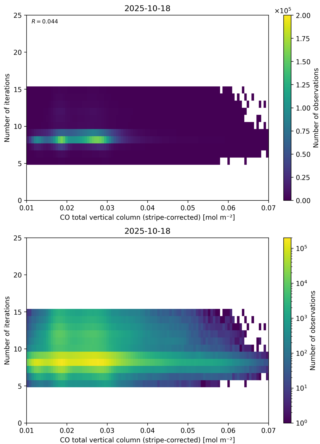
Figure 39: Scatter density plot of “CO total vertical column (stripe-corrected)” against “Number of iterations” for 2025-10-17 to 2025-10-19.
