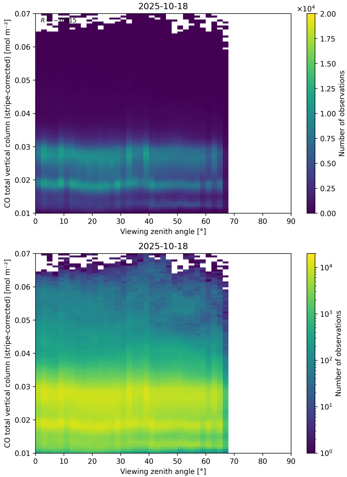
Figure 70: Scatter density plot of “Viewing zenith angle” against “CO total vertical column (stripe-corrected)” for 2025-10-17 to 2025-10-19.
