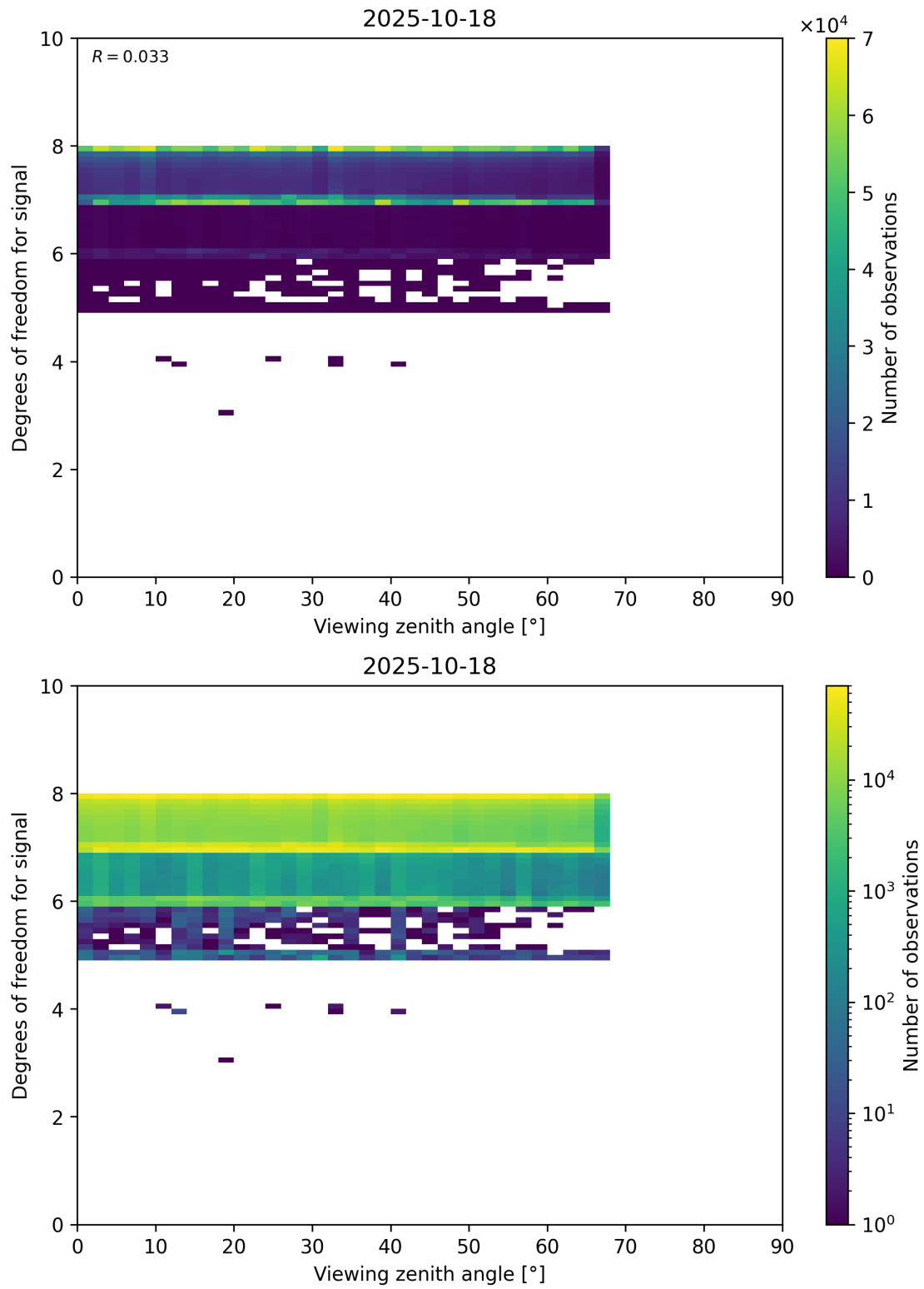
Figure 73: Scatter density plot of “Viewing zenith angle” against “Degrees of freedom for signal” for 2025-10-17 to 2025-10-19.
