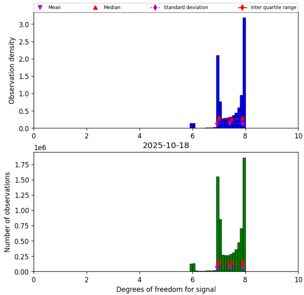
Figure 23: Histogram of “Degrees of freedom for signal” for 2025-10-17 to 2025-10-19
