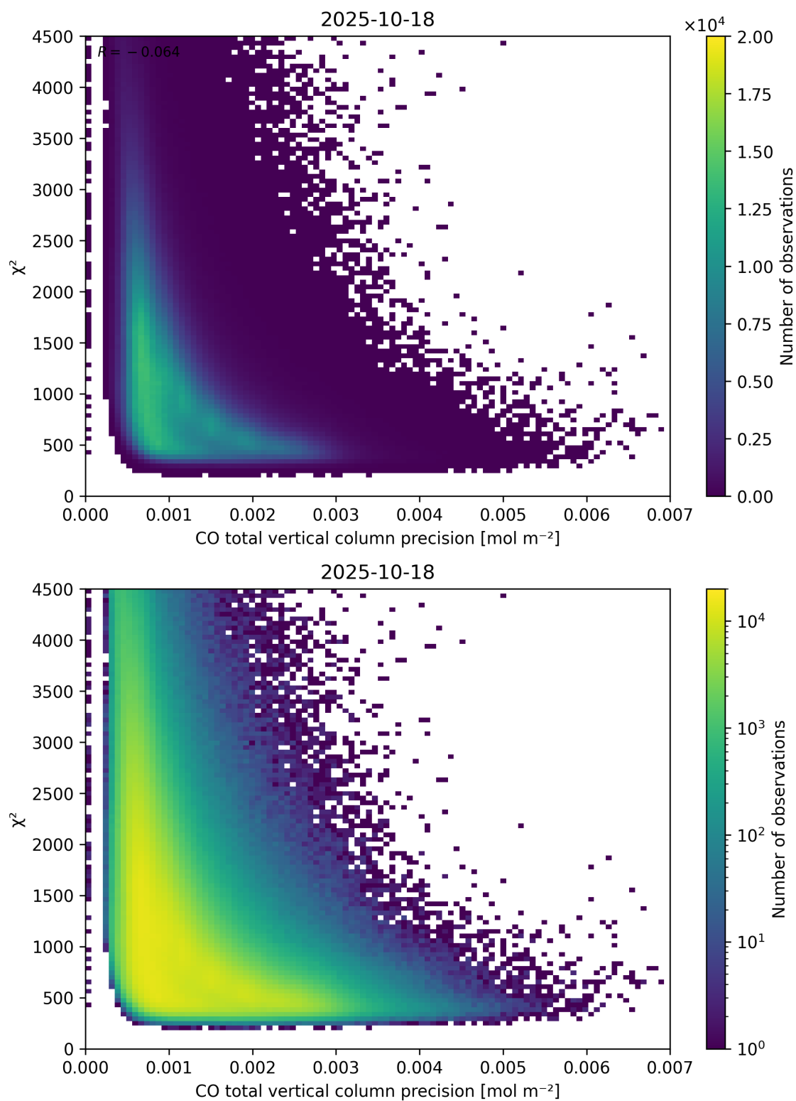
Figure 44: Scatter density plot of “CO total vertical column precision” against “ \chi^2 ” for 2025-10-17 to 2025-10-19.
