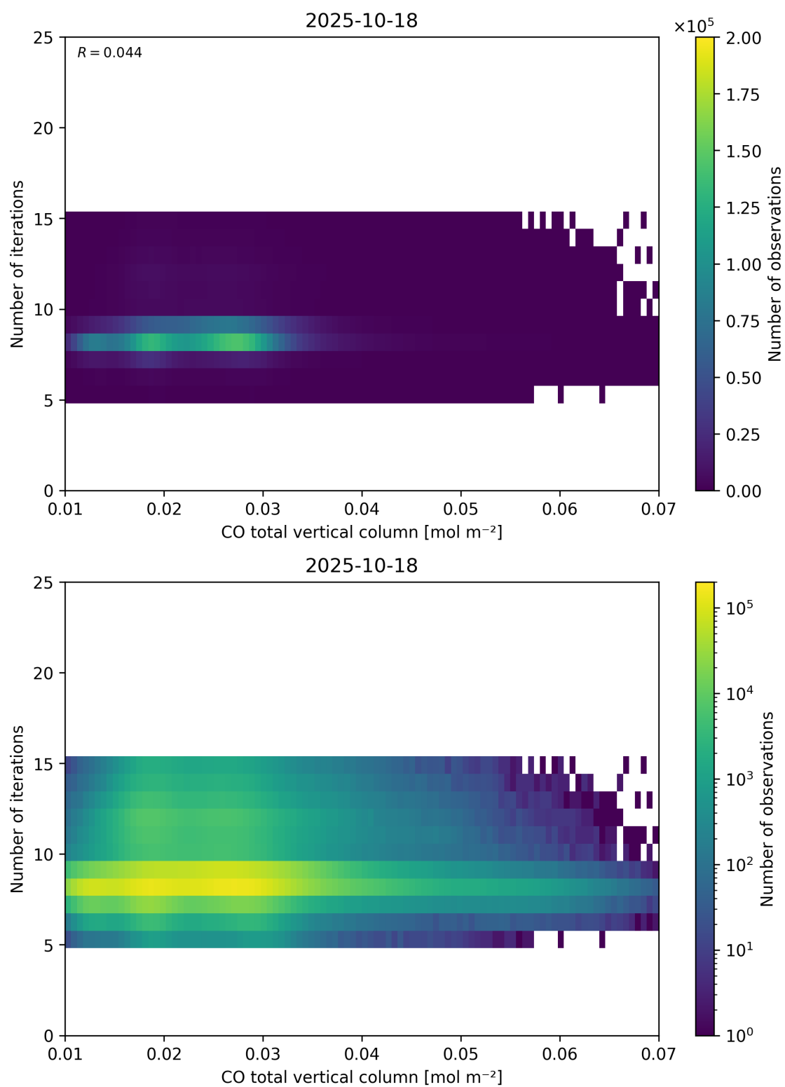
Figure 42: Scatter density plot of “CO total vertical column” against “Number of iterations” for 2025-10-17 to 2025-10-19.
