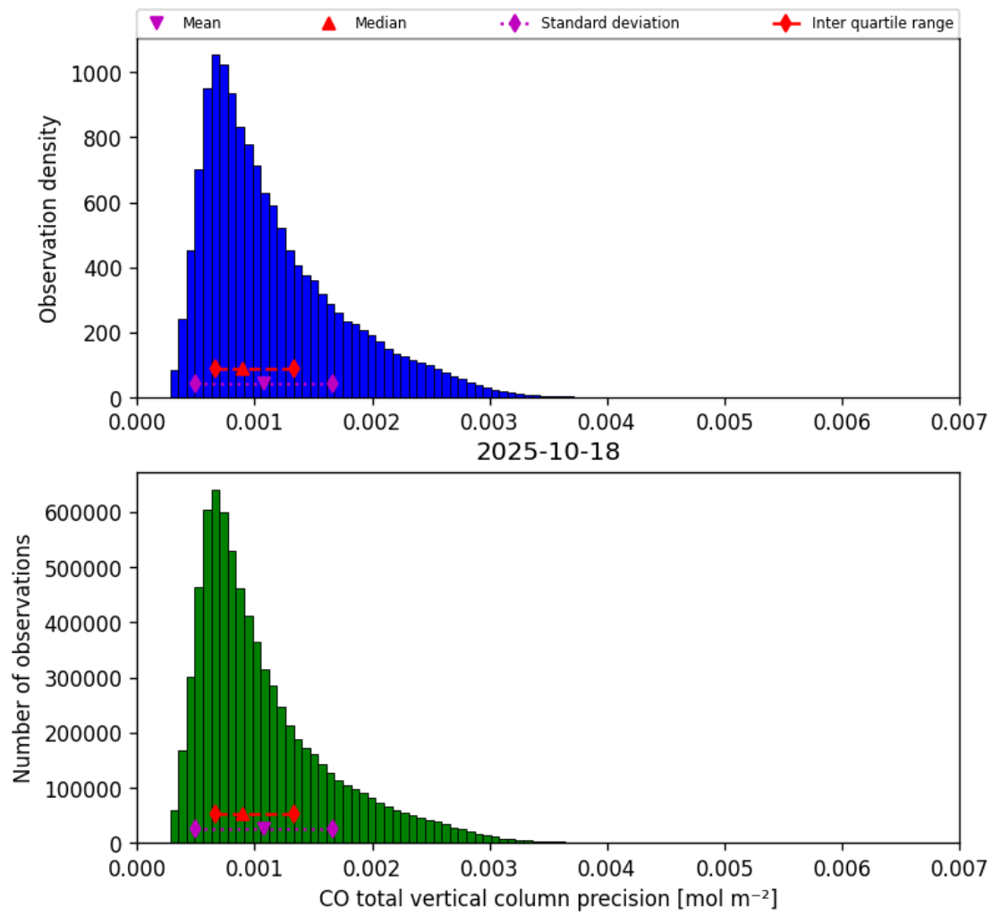
Figure 20: Histogram of “CO total vertical column precision” for 2025-10-17 to 2025-10-19
