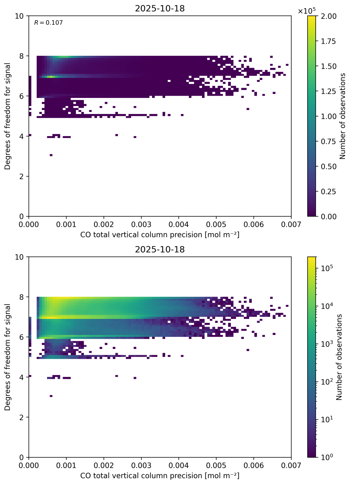
Figure 45: Scatter density plot of “CO total vertical column precision” against “Degrees of freedom for signal” for 2025-10-17 to 2025-10-19.
