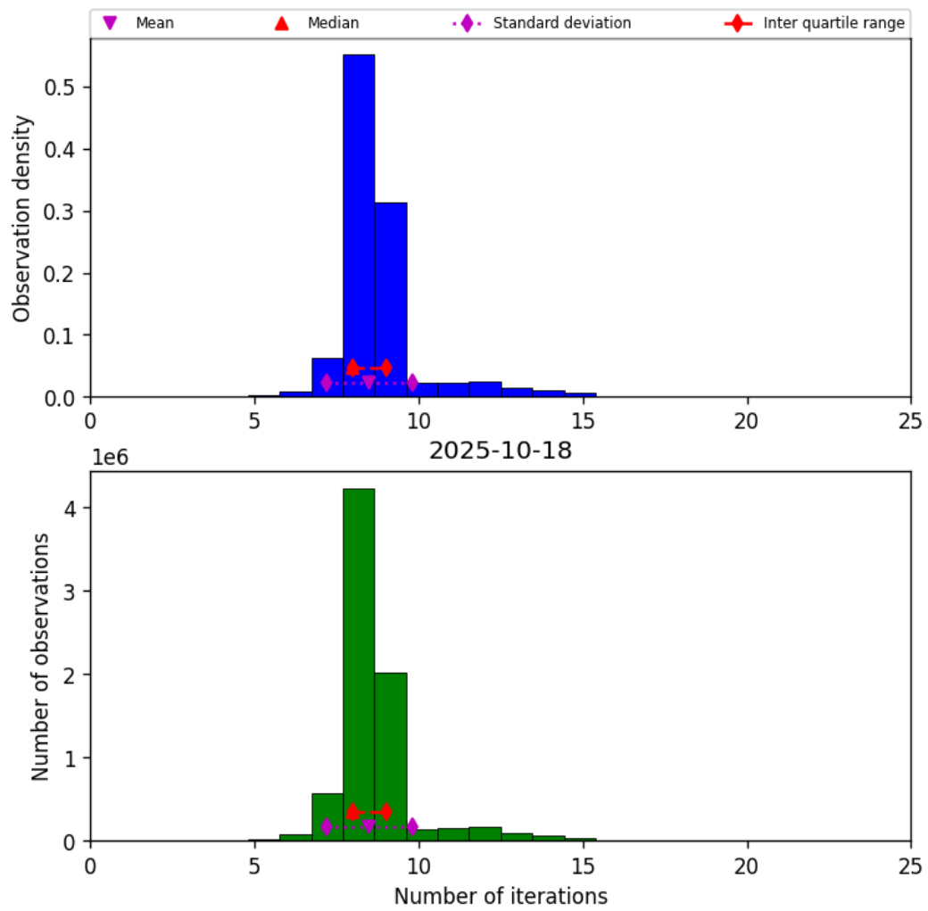
Figure 24: Histogram of “Number of iterations” for 2025-10-17 to 2025-10-19
