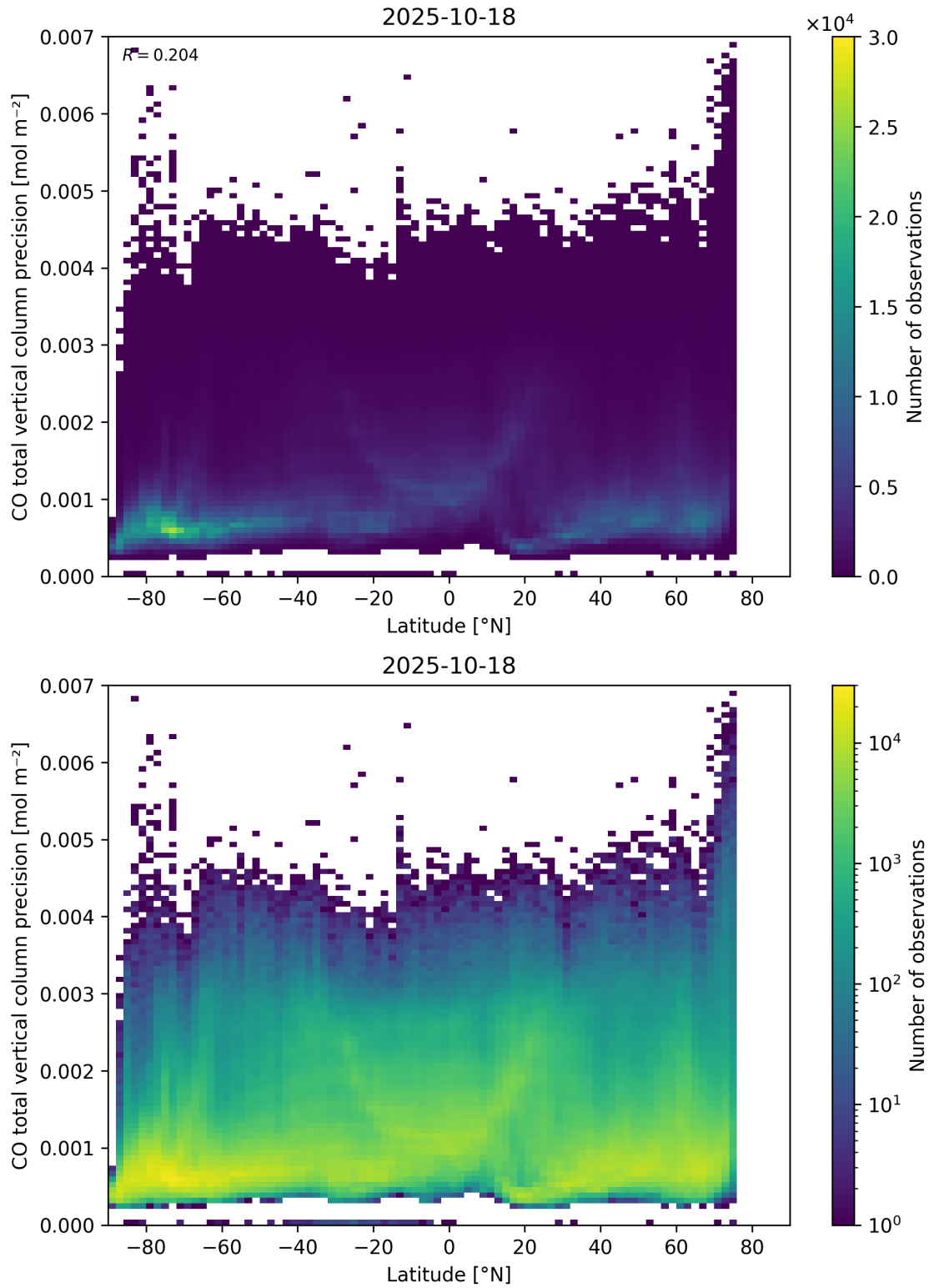
Figure 53: Scatter density plot of “Latitude” against “CO total vertical column precision” for 2025-10-17 to 2025-10-19.
