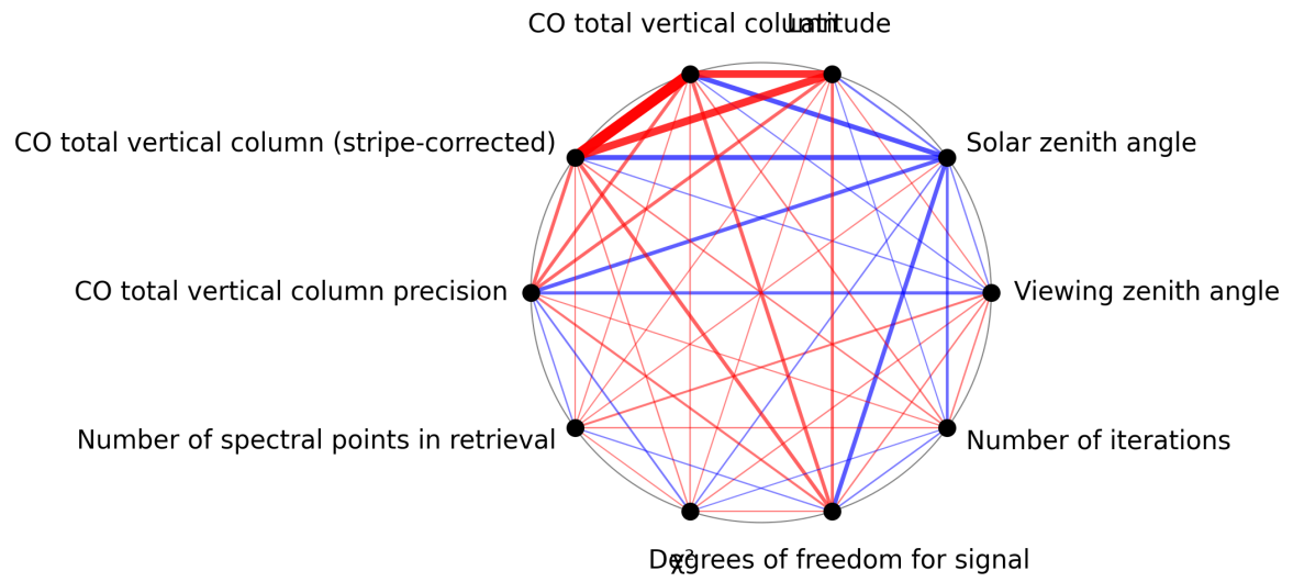
Figure 1: Map of correlation graph for 2025-10-17 to 2025-10-19.
