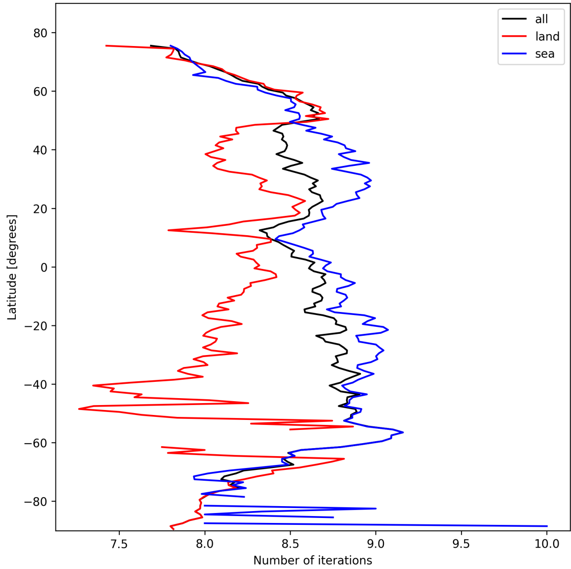
Figure 16: Zonal average of “Number of iterations” for 2025-10-17 to 2025-10-19.
