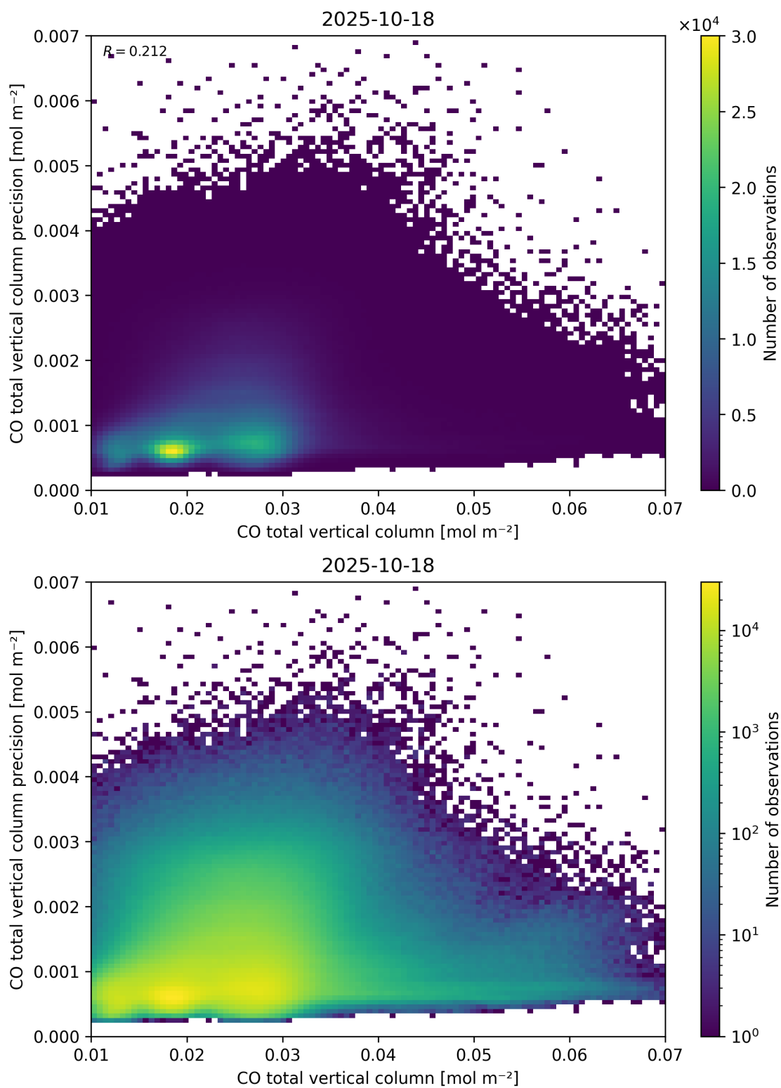
Figure 34: Scatter density plot of “CO total vertical column” against “CO total vertical column precision” for 2025-10-17 to 2025-10-19.
