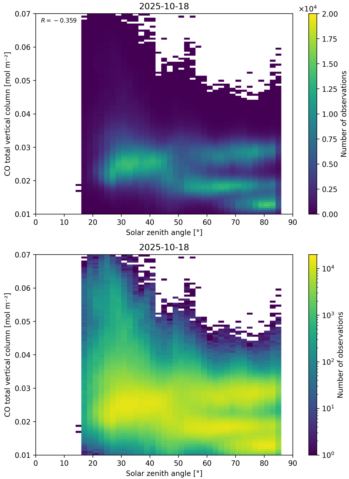
Figure 61: Scatter density plot of “Solar zenith angle” against “CO total vertical column” for 2025-10-17 to 2025-10-19.
