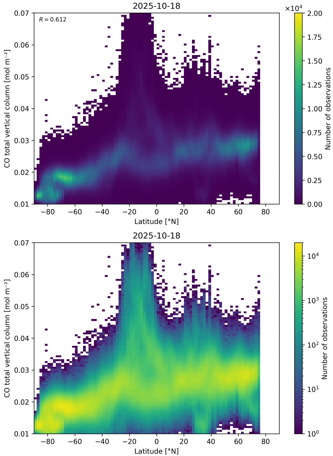
Figure 51: Scatter density plot of “Latitude” against “CO total vertical column” for 2025-10-17 to 2025-10-19.
