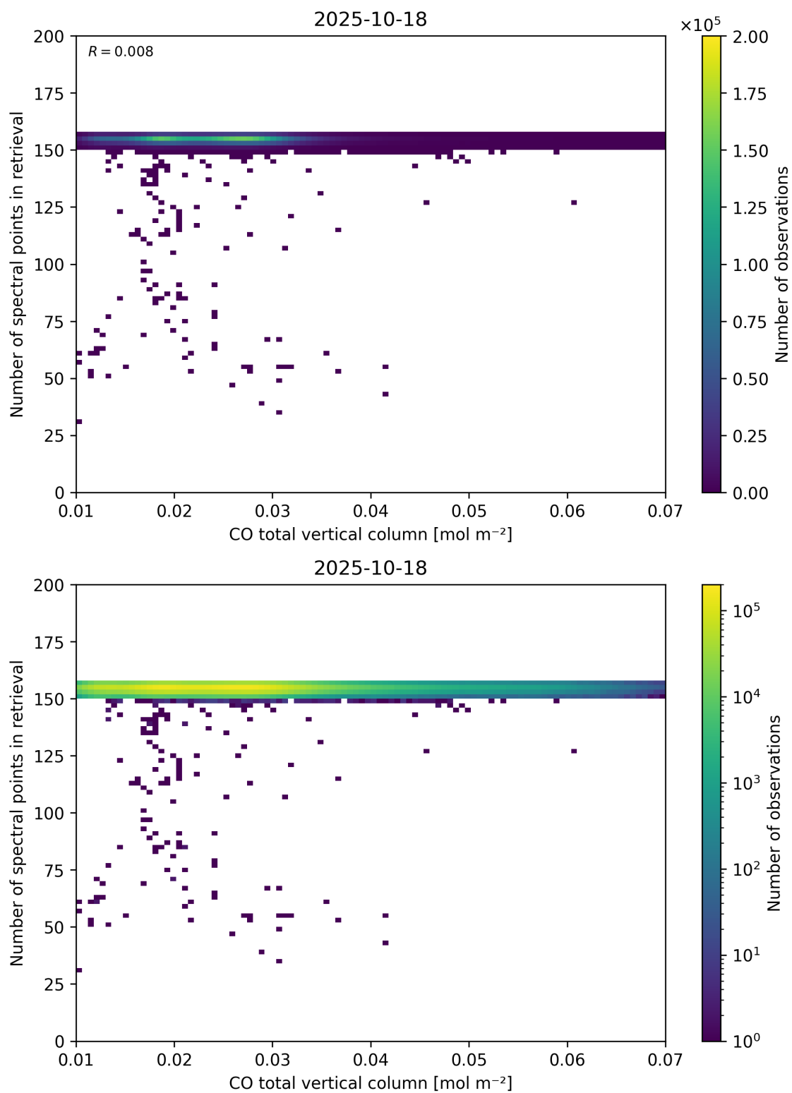
Figure 43: Scatter density plot of “CO total vertical column” against “Number of spectral points in retrieval” for 2025-10-17 to 2025-10-19.
