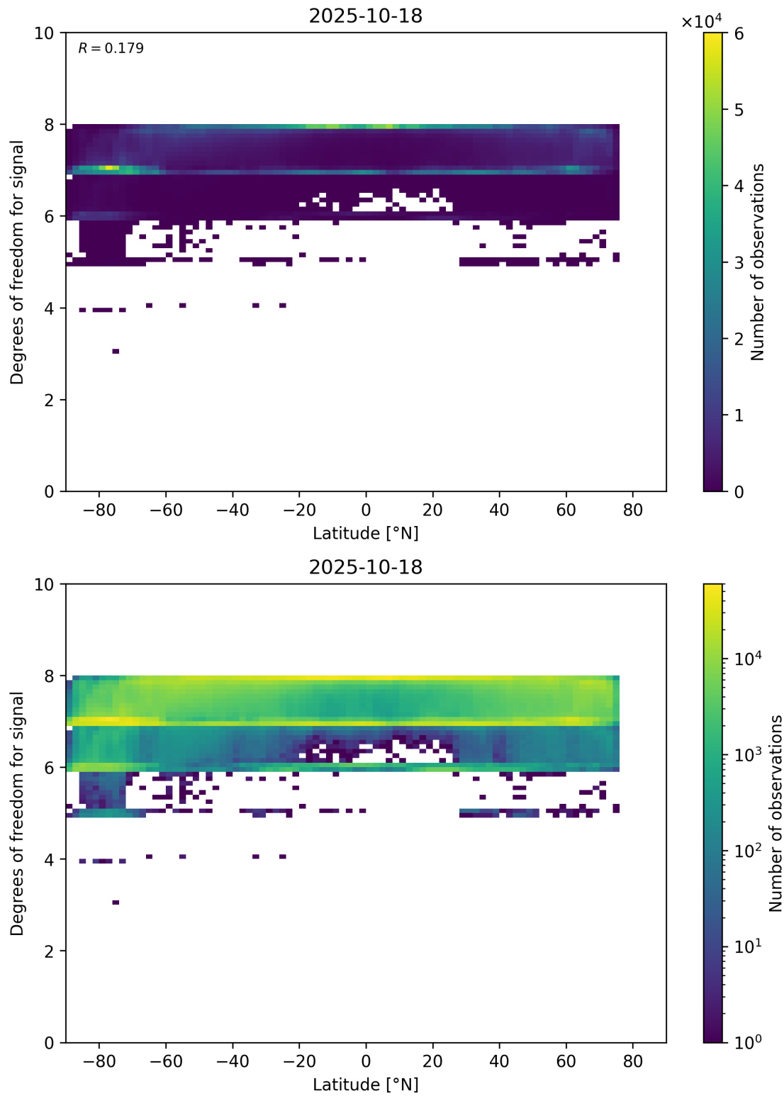
Figure 55: Scatter density plot of “Latitude” against “Degrees of freedom for signal” for 2025-10-17 to 2025-10-19.
