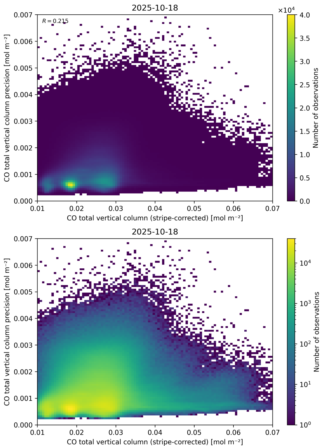
Figure 36: Scatter density plot of “CO total vertical column (stripe-corrected)” against “CO total vertical column precision” for 2025-10-17 to 2025-10-19.
