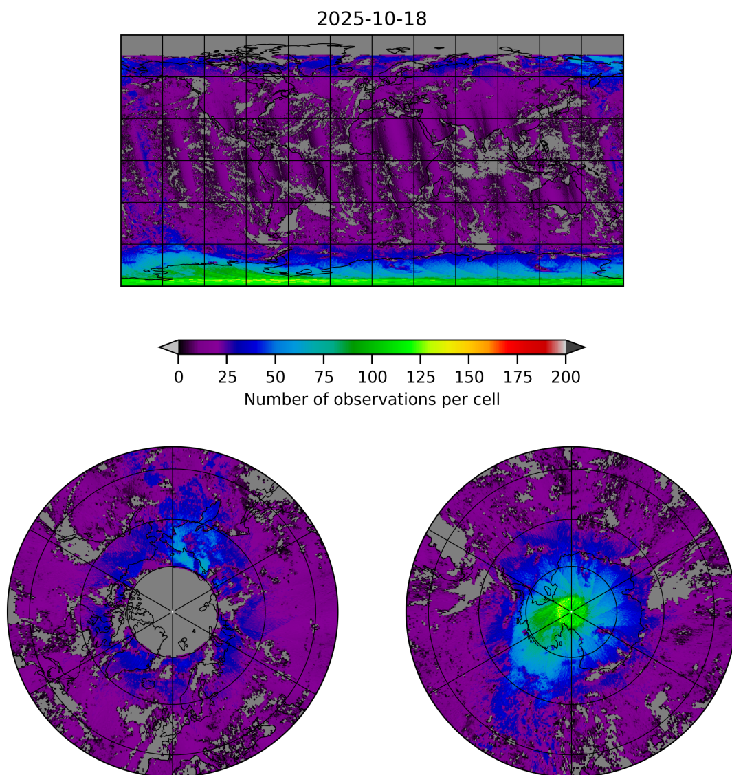
Figure 8: Map of the number of observations for 2025-10-17 to 2025-10-19
