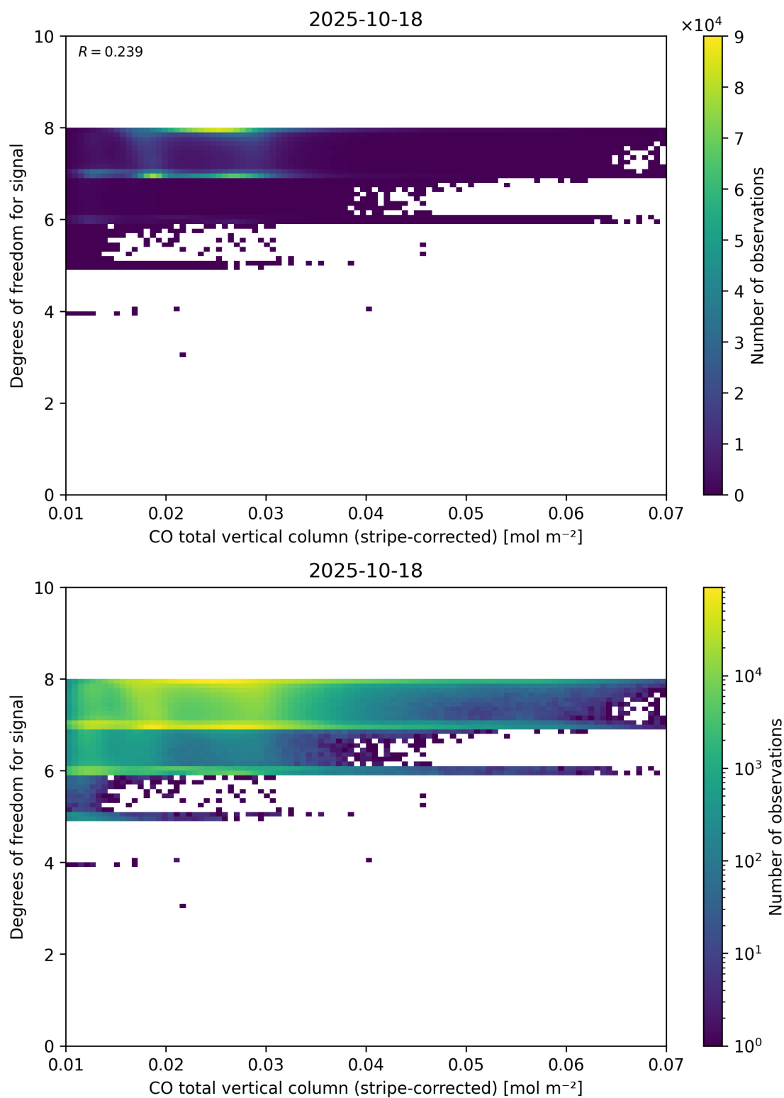
Figure 38: Scatter density plot of “CO total vertical column (stripe-corrected)” against “Degrees of freedom for signal” for 2025-10-17 to 2025-10-19.
