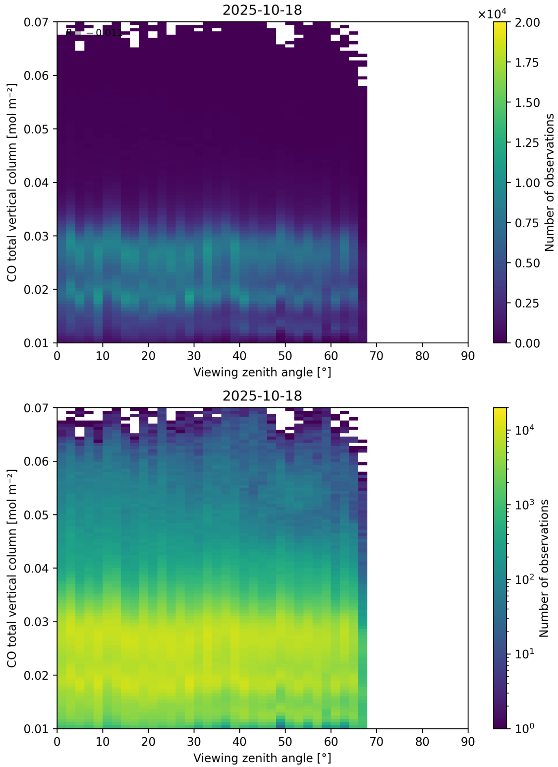
Figure 69: Scatter density plot of “Viewing zenith angle” against “CO total vertical column” for 2025-10-17 to 2025-10-19.
