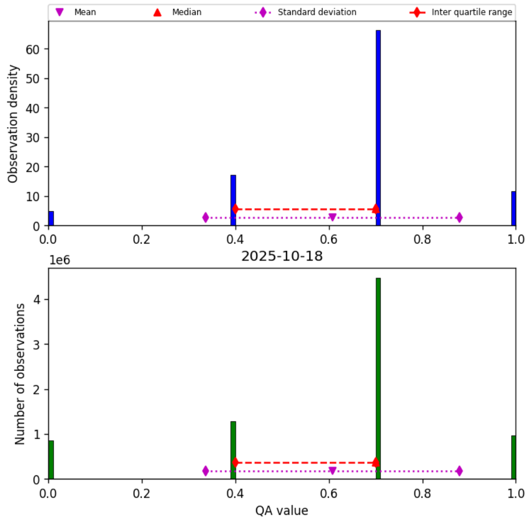
Figure 17: Histogram of “QA value” for 2025-10-17 to 2025-10-19
