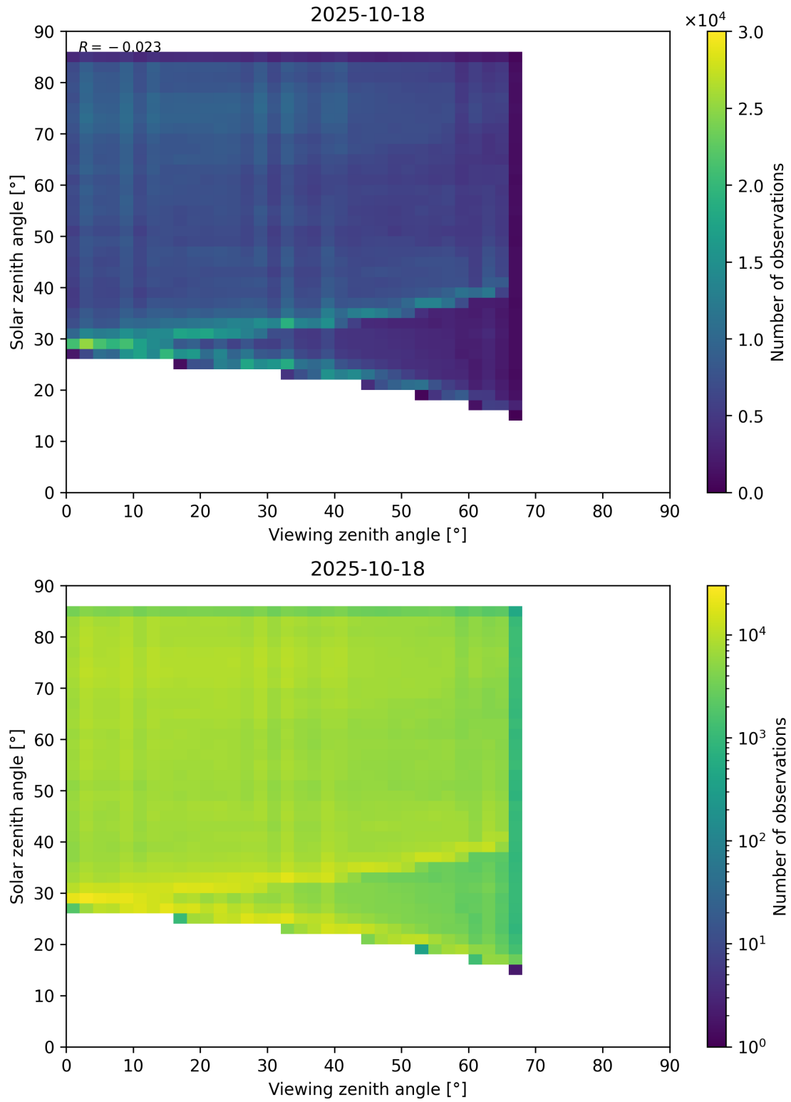
Figure 77: Scatter density plot of “Viewing zenith angle” against “Solar zenith angle” for 2025-10-17 to 2025-10-19.
