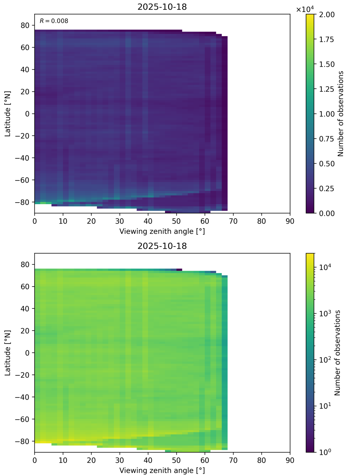
Figure 74: Scatter density plot of “Viewing zenith angle” against “Latitude” for 2025-10-17 to 2025-10-19.
