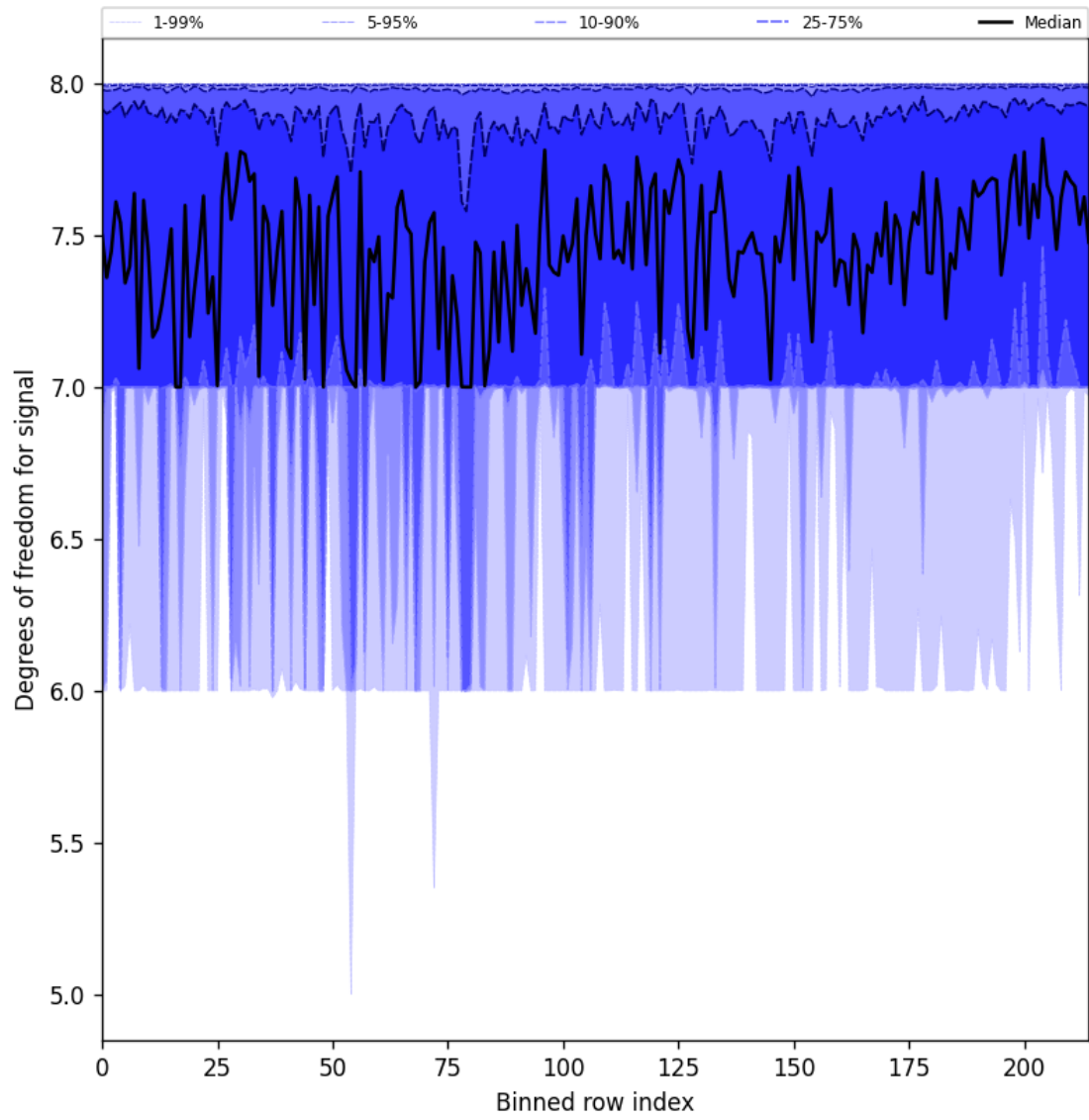
Figure 31: Along track statistics of “Degrees of freedom for signal” for 2025-10-17 to 2025-10-19
