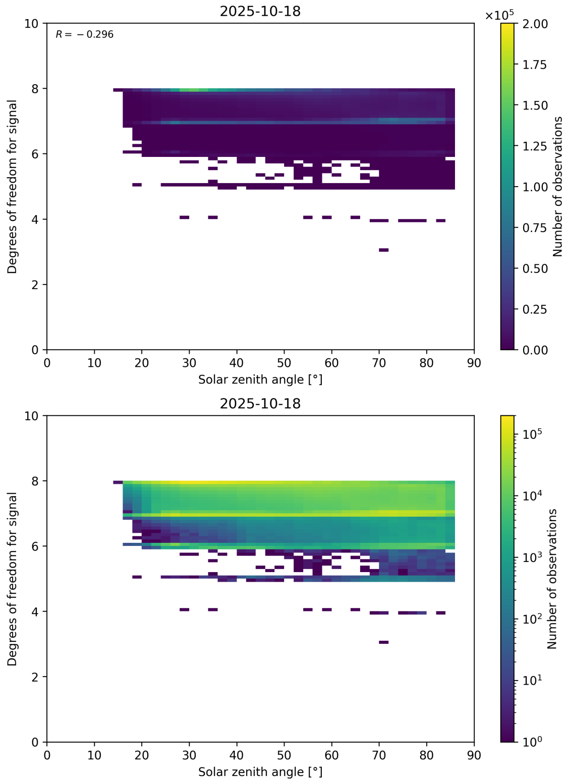
Figure 65: Scatter density plot of “Solar zenith angle” against “Degrees of freedom for signal” for 2025-10-17 to 2025-10-19.
