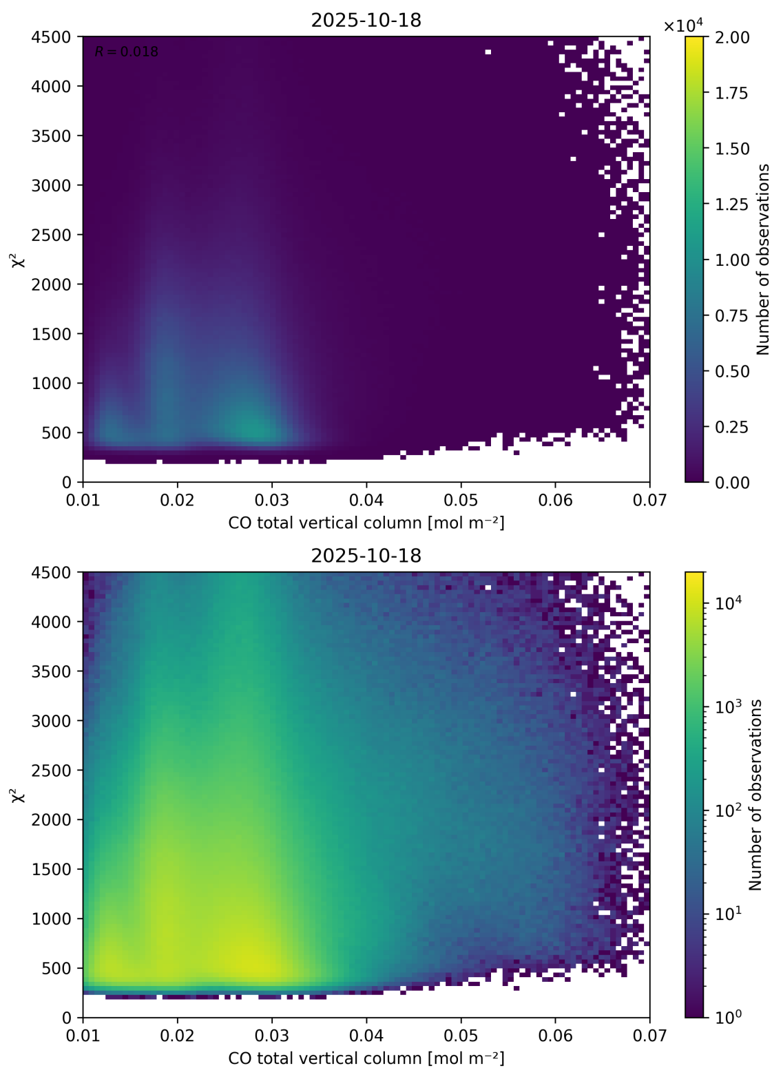
Figure 35: Scatter density plot of “CO total vertical column” against “ \chi^2 ” for 2025-10-17 to 2025-10-19.
