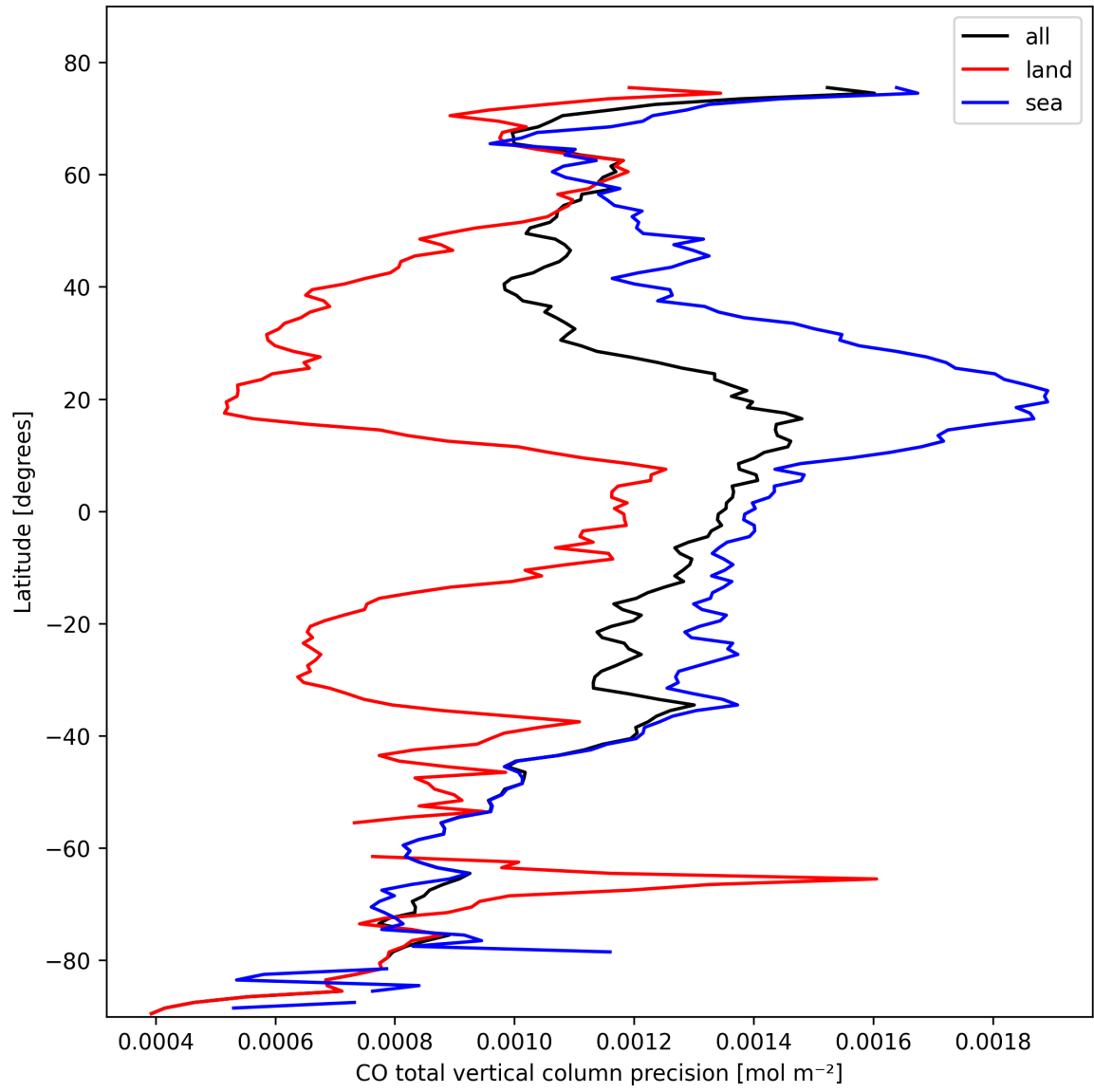
Figure 12: Zonal average of “CO total vertical column precision” for 2025-10-17 to 2025-10-19.
