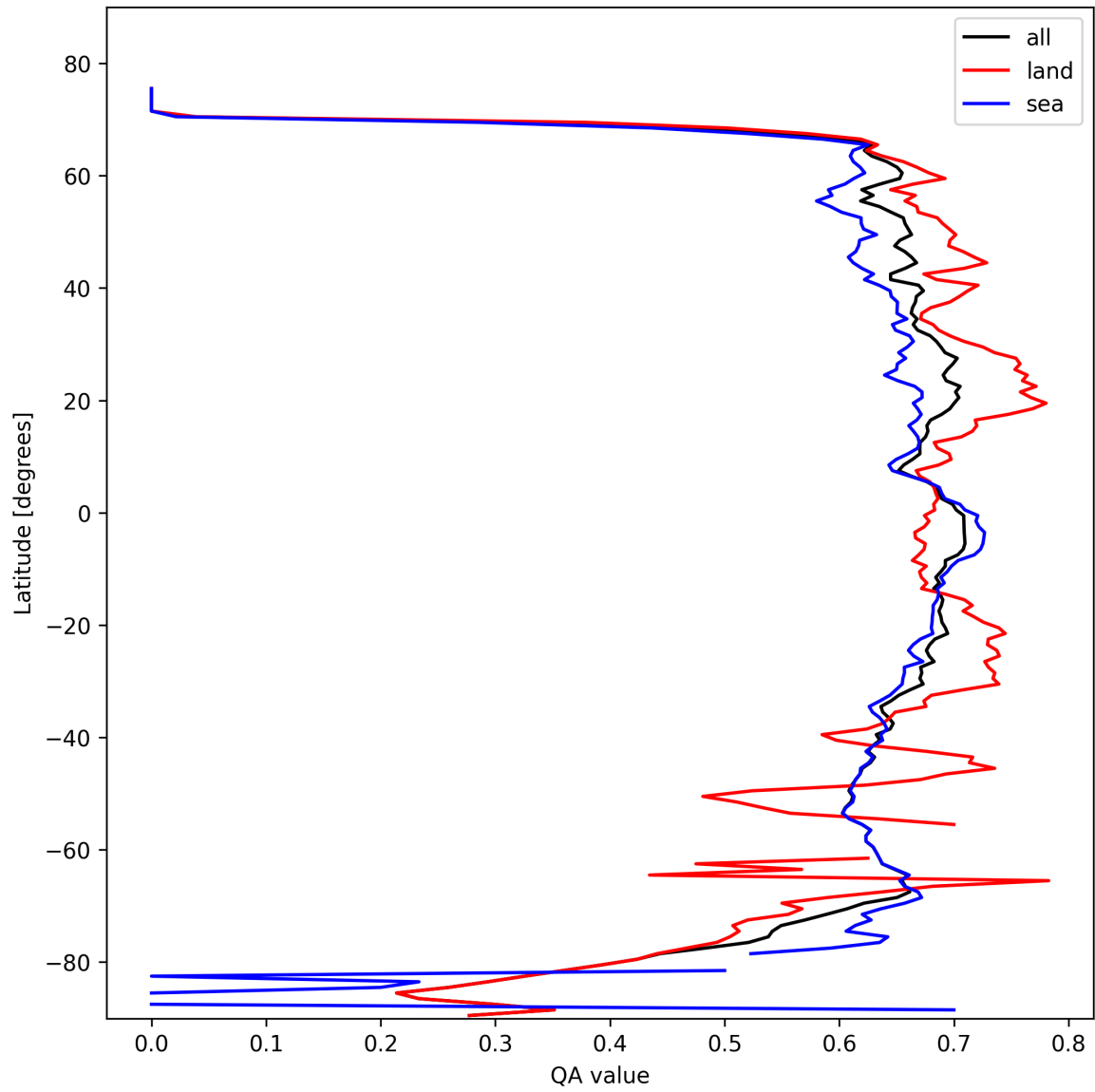
Figure 9: Zonal average of “QA value” for 2025-10-17 to 2025-10-19.
