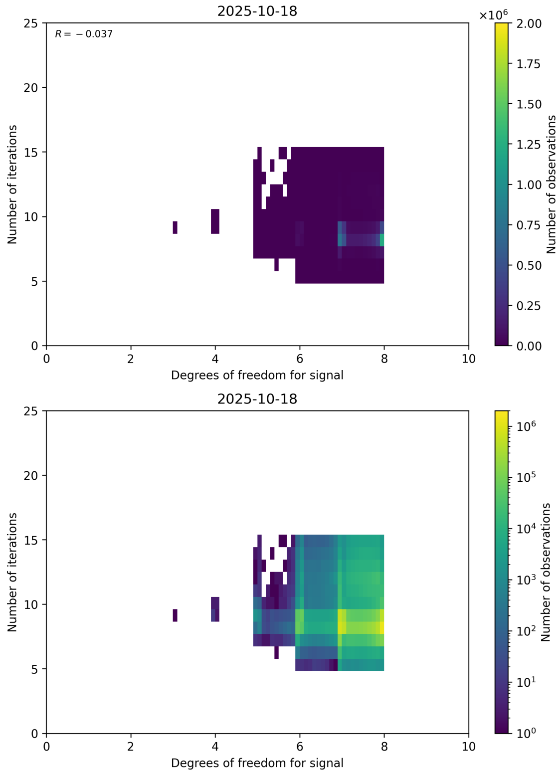
Figure 50: Scatter density plot of “Degrees of freedom for signal” against “Number of iterations” for 2025-10-17 to 2025-10-19.
