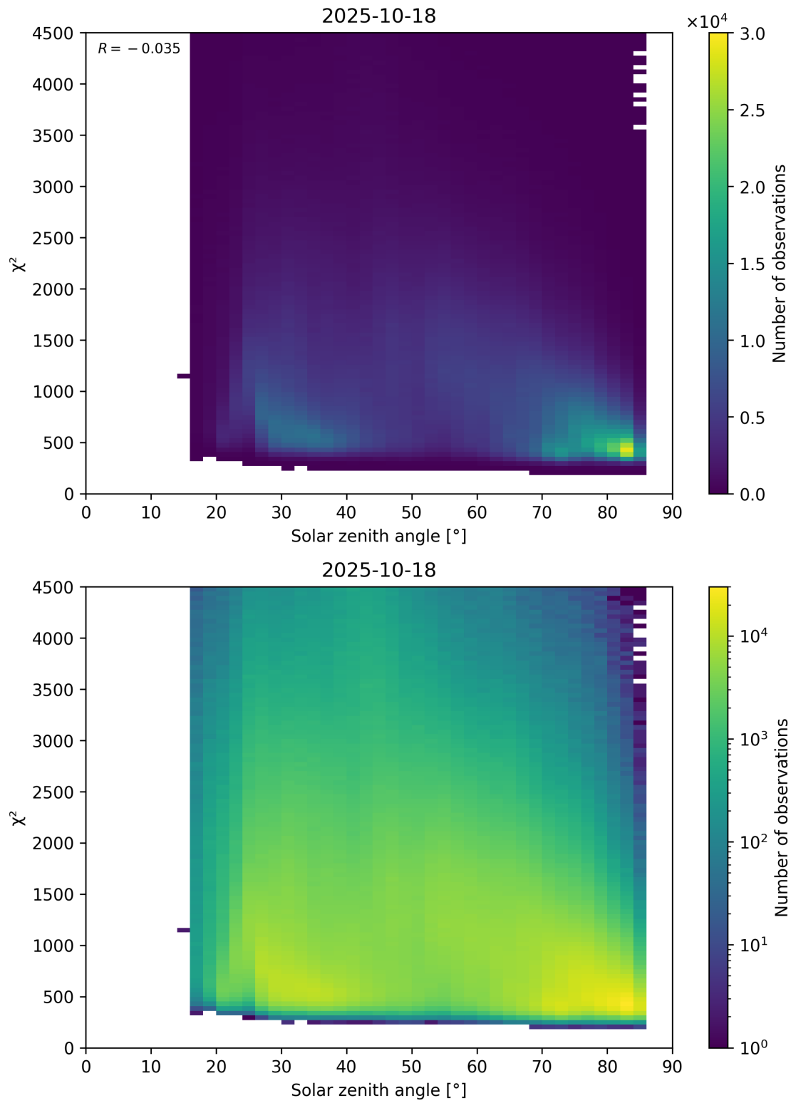
Figure 64: Scatter density plot of “Solar zenith angle” against “ \chi^2 ” for 2025-10-17 to 2025-10-19.
