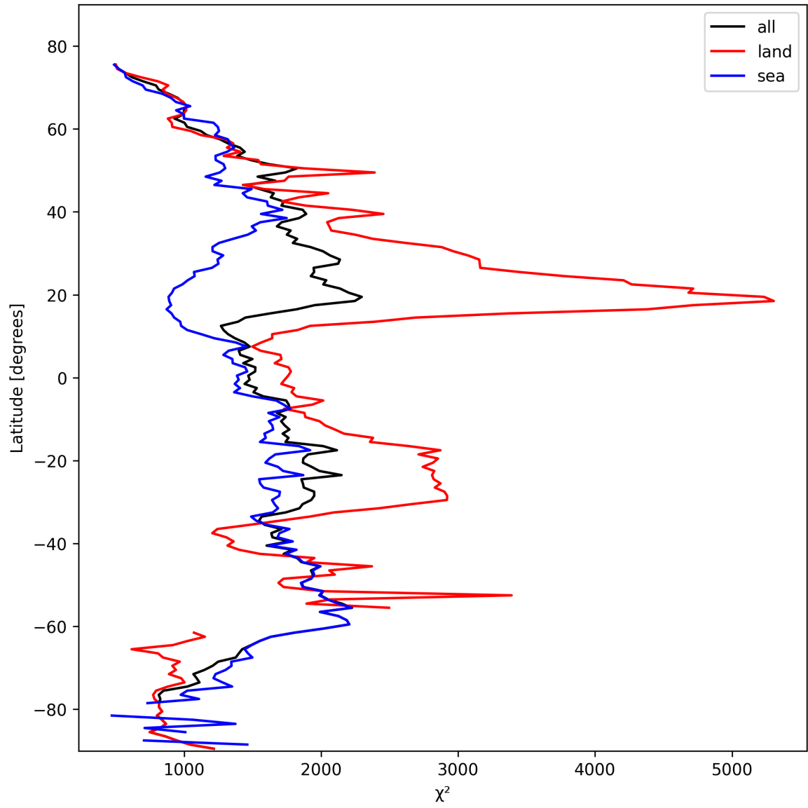
Figure 14: Zonal average of “ \chi^2 ” for 2025-10-17 to 2025-10-19.
