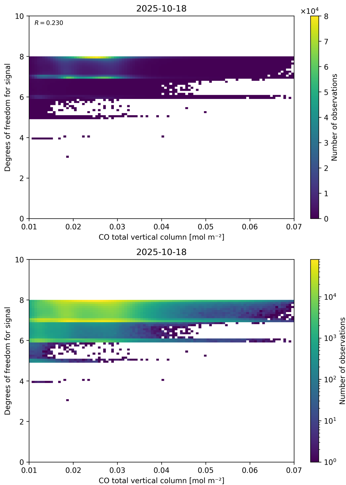
Figure 41: Scatter density plot of “CO total vertical column” against “Degrees of freedom for signal” for 2025-10-17 to 2025-10-19.
