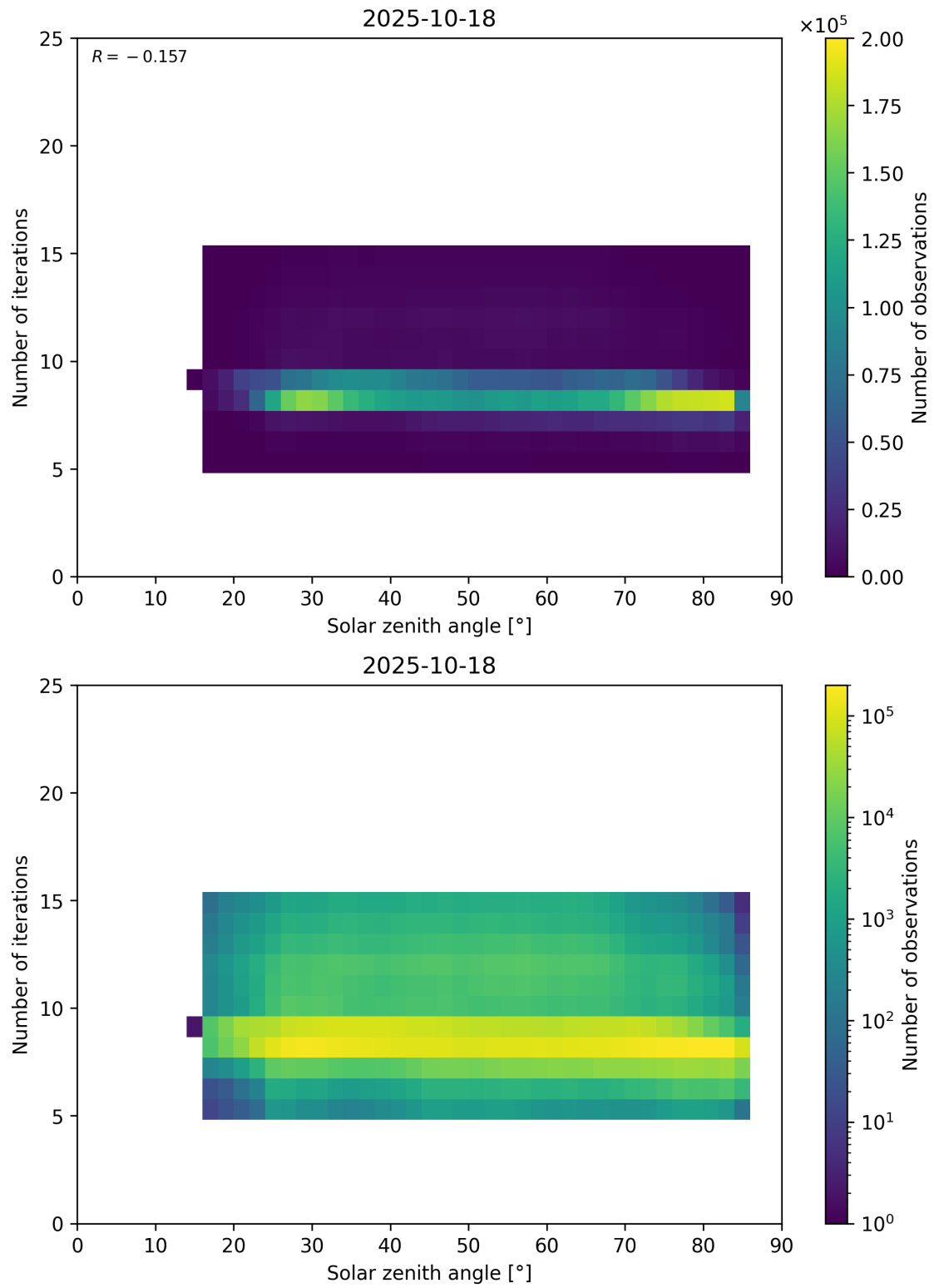
Figure 67: Scatter density plot of “Solar zenith angle” against “Number of iterations” for 2025-10-17 to 2025-10-19.
