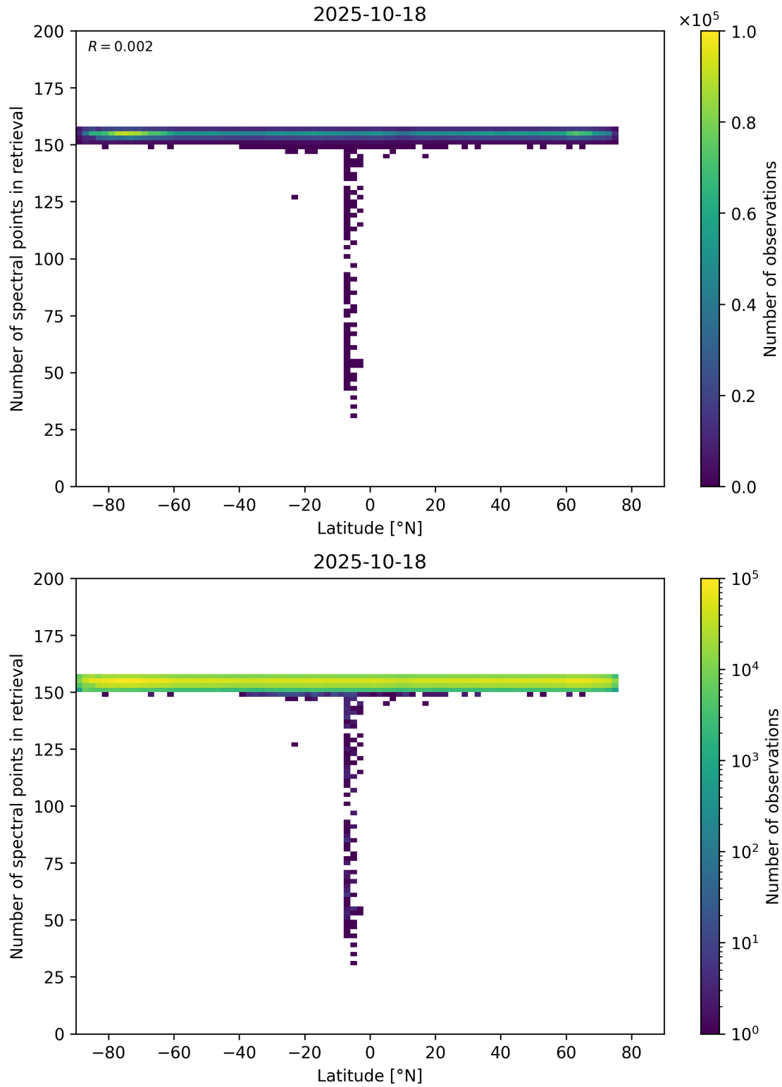
Figure 57: Scatter density plot of “Latitude” against “Number of spectral points in retrieval” for 2025-10-17 to 2025-10-19.
