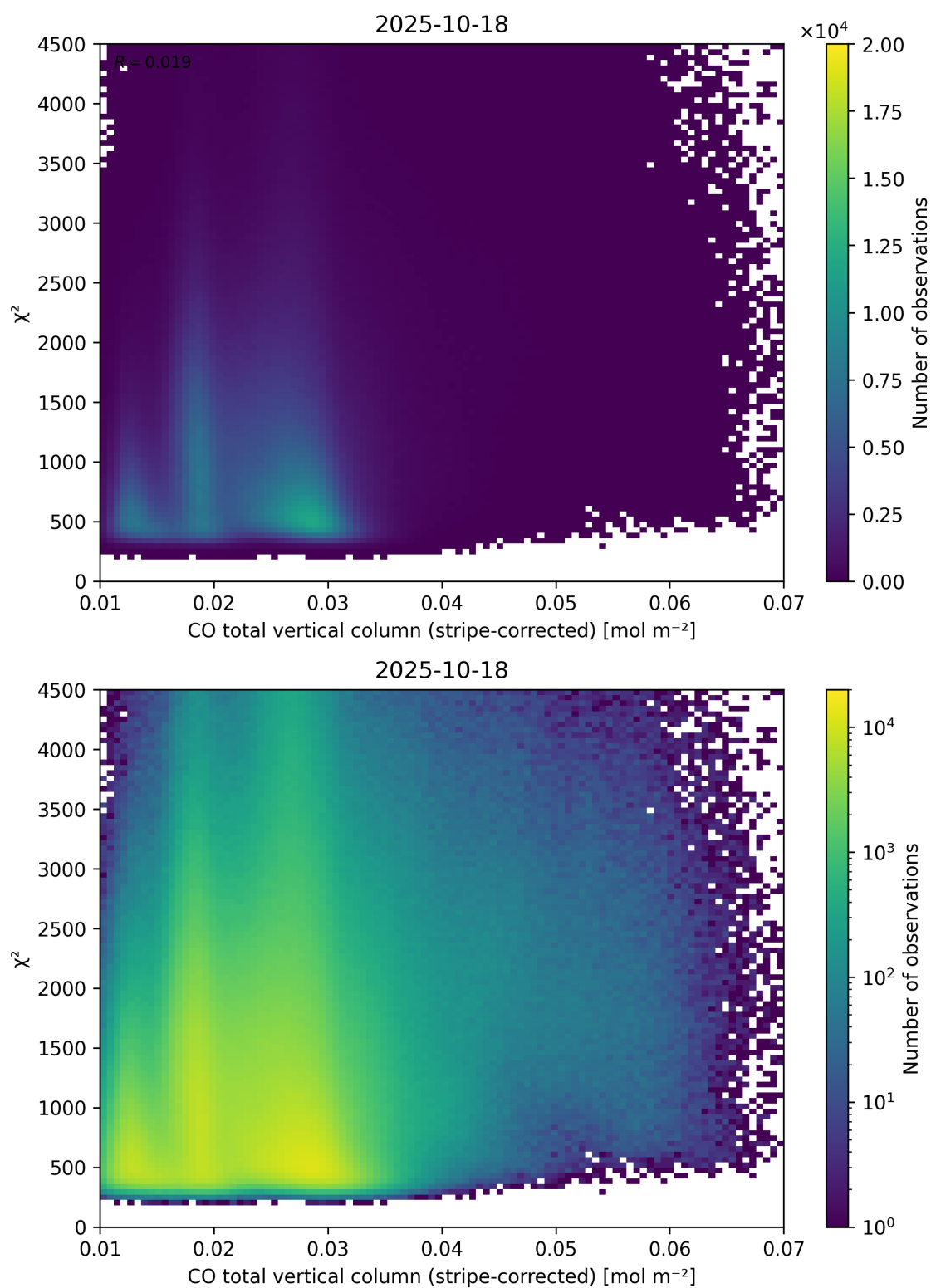
Figure 37: Scatter density plot of “CO total vertical column (stripe-corrected)” against “ \chi^2 ” for 2025-10-17 to 2025-10-19.
