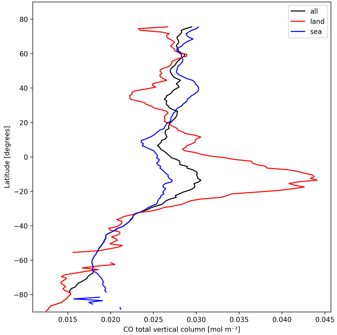
Figure 10: Zonal average of “CO total vertical column” for 2025-10-17 to 2025-10-19.
