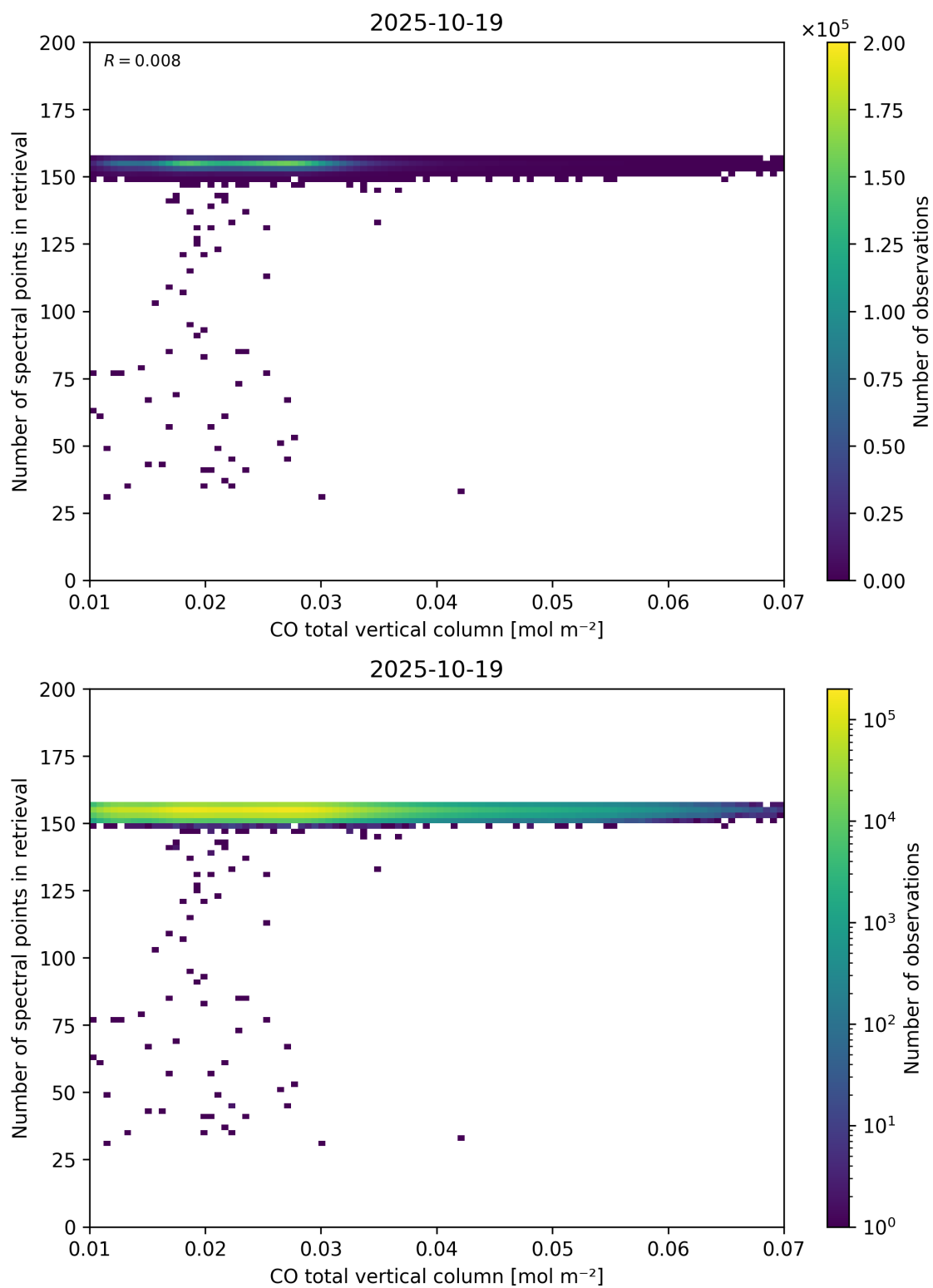
Figure 43: Scatter density plot of “CO total vertical column” against “Number of spectral points in retrieval” for 2025-10-18 to 2025-10-20.
