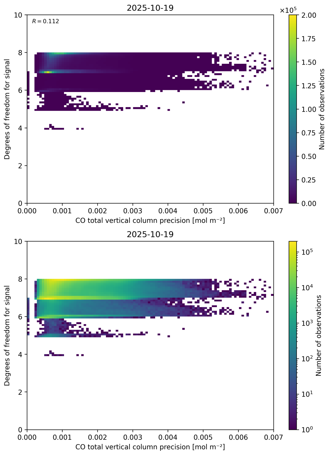
Figure 45: Scatter density plot of “CO total vertical column precision” against “Degrees of freedom for signal” for 2025-10-18 to 2025-10-20.
