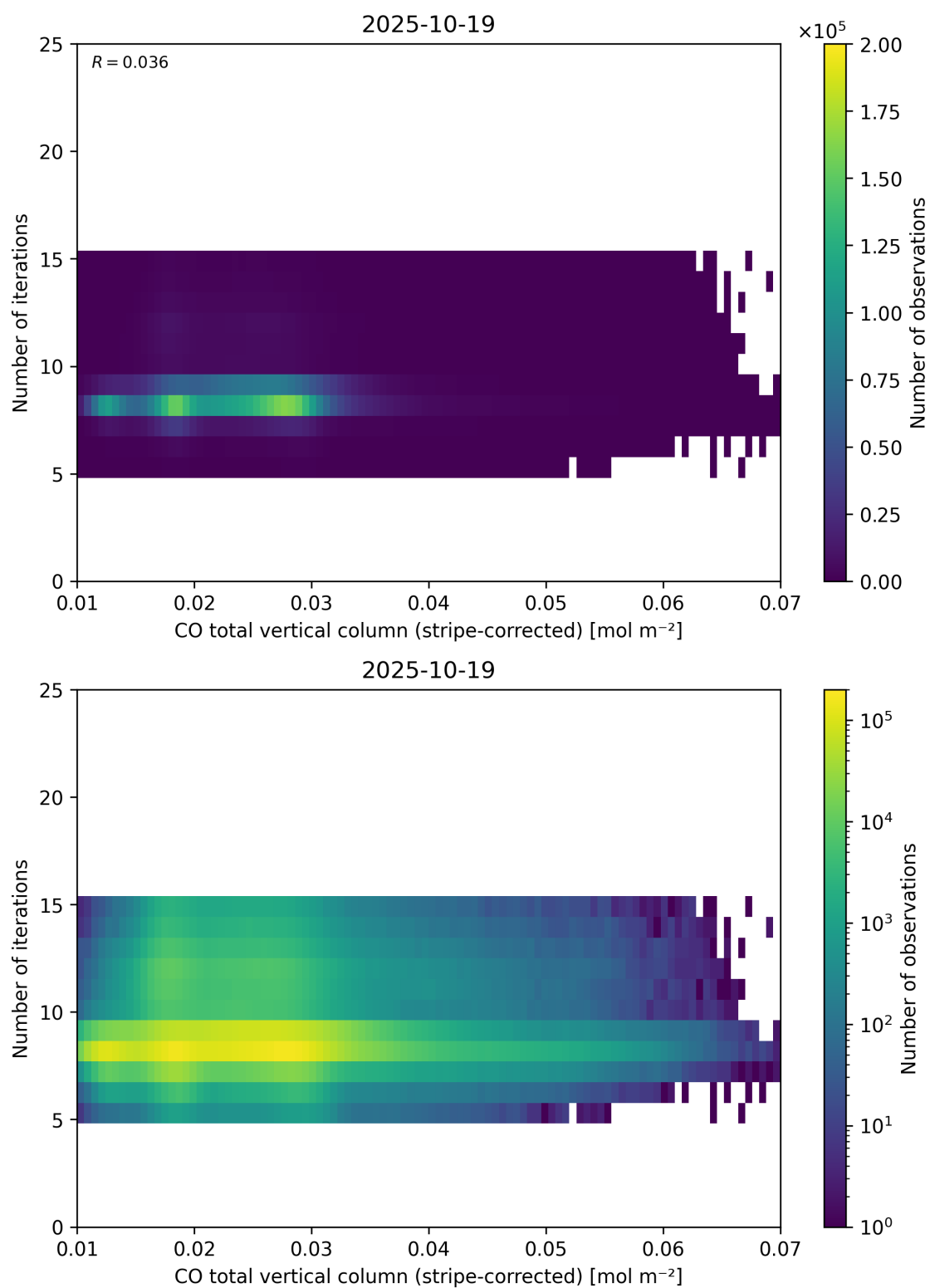
Figure 39: Scatter density plot of “CO total vertical column (stripe-corrected)” against “Number of iterations” for 2025-10-18 to 2025-10-20.
