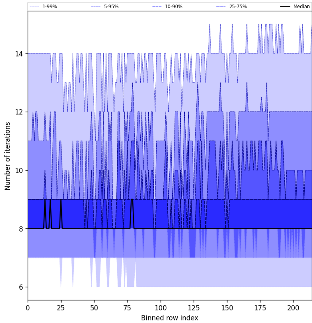
Figure 32: Along track statistics of “Number of iterations” for 2025-10-18 to 2025-10-20
