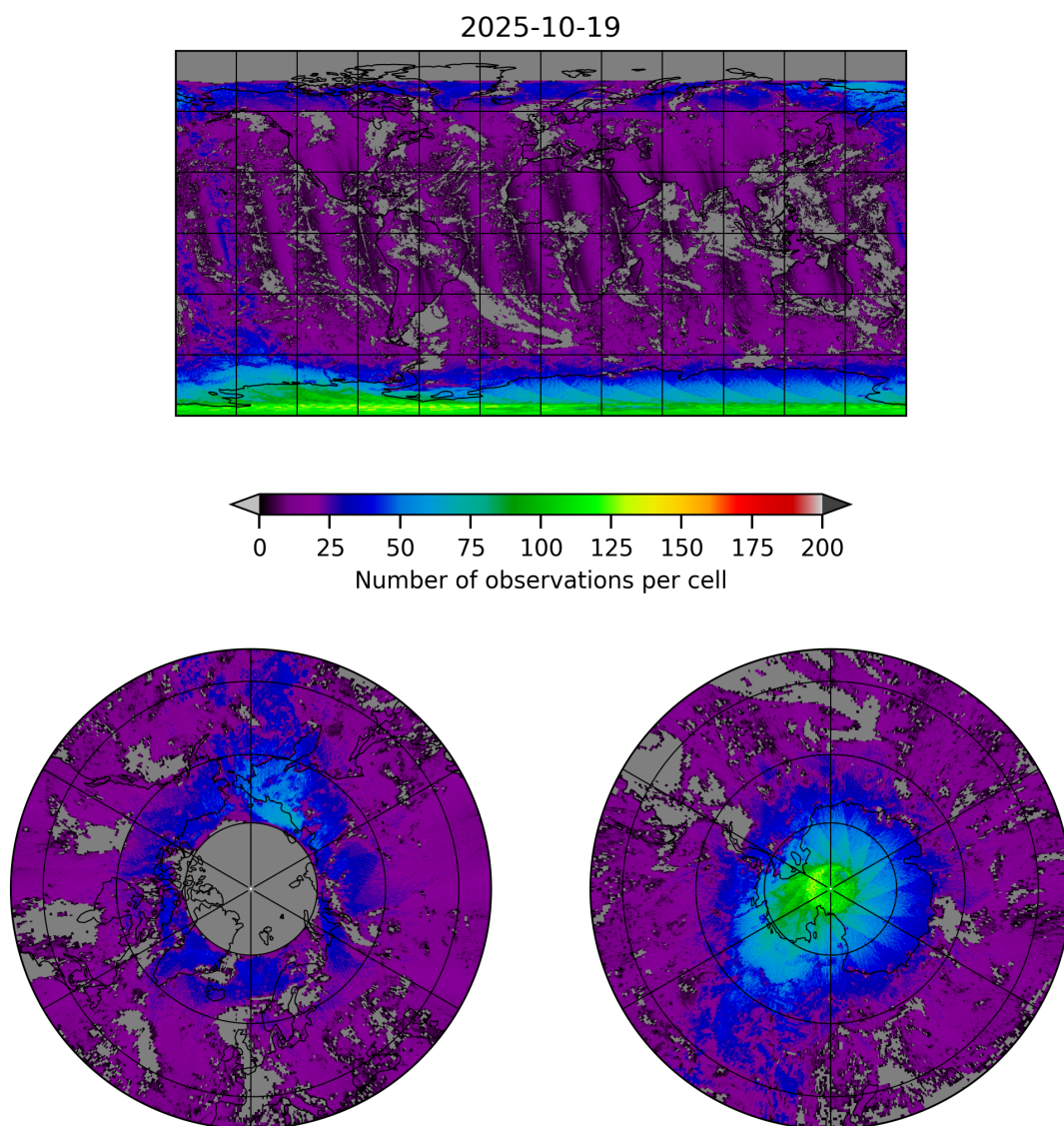
Figure 8: Map of the number of observations for 2025-10-18 to 2025-10-20
