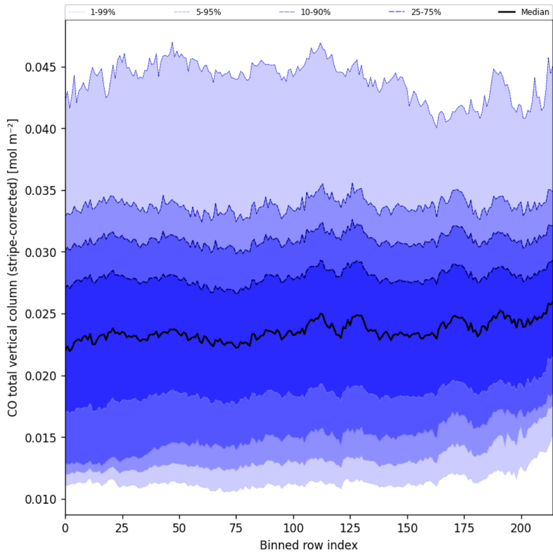
Figure 27: Along track statistics of “CO total vertical column (stripe-corrected)” for 2025-10-18 to 2025-10-20
