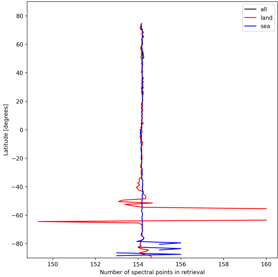
Figure 13: Zonal average of “Number of spectral points in retrieval” for 2025-10-18 to 2025-10-20.
