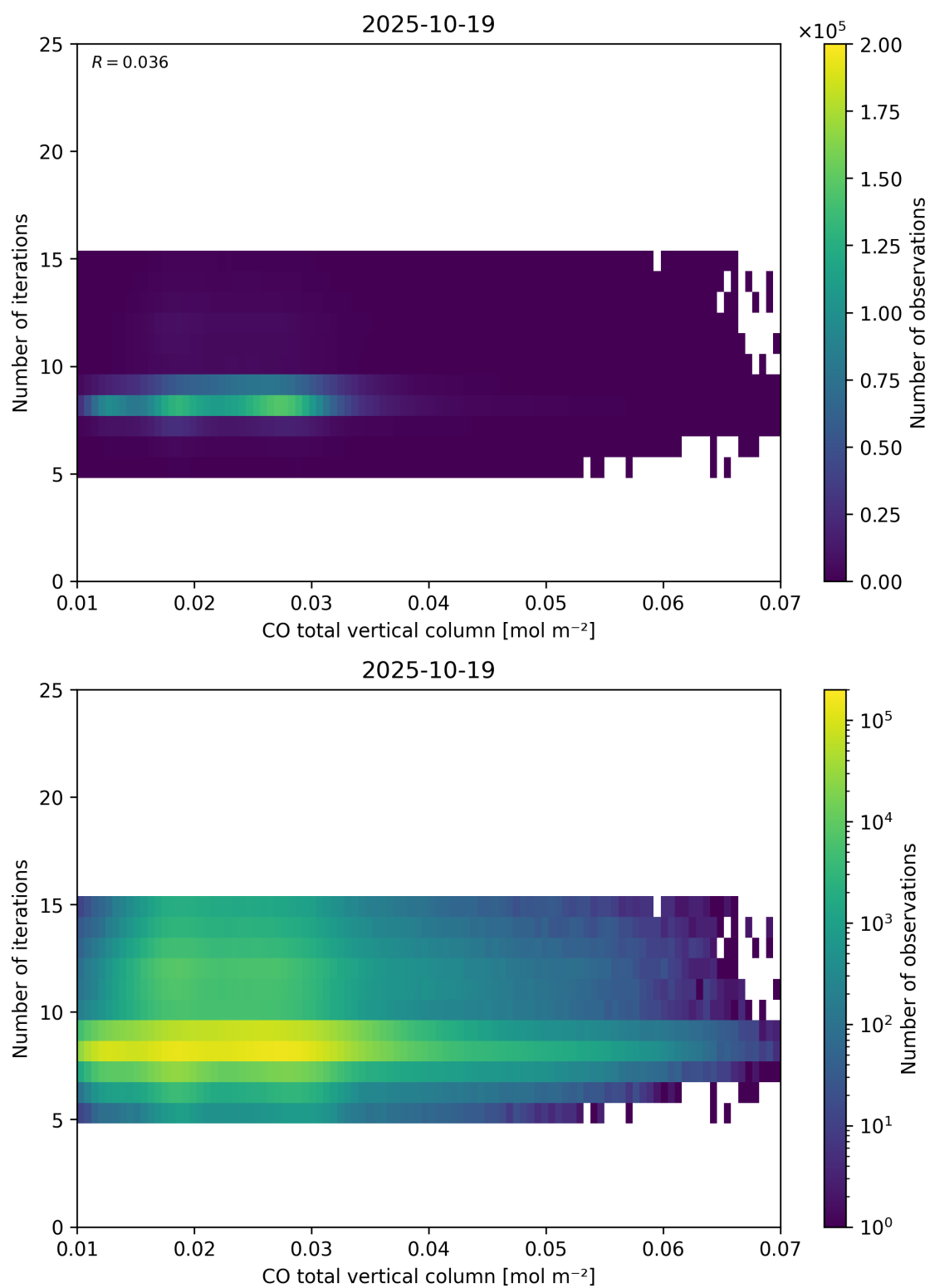
Figure 42: Scatter density plot of “CO total vertical column” against “Number of iterations” for 2025-10-18 to 2025-10-20.
