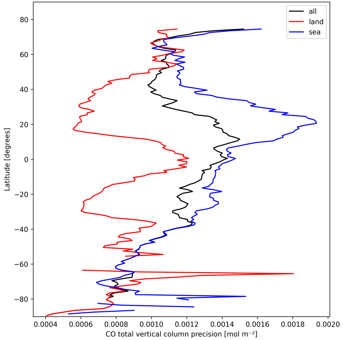
Figure 12: Zonal average of “CO total vertical column precision” for 2025-10-18 to 2025-10-20.
