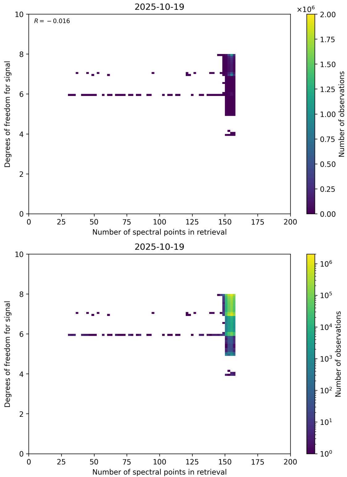
Figure 59: Scatter density plot of “Number of spectral points in retrieval” against “Degrees of freedom for signal” for 2025-10-18 to 2025-10-20.
