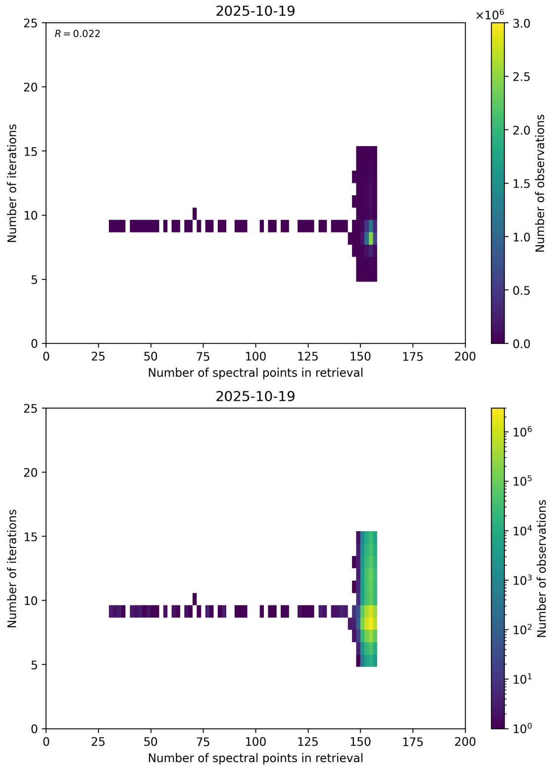
Figure 60: Scatter density plot of “Number of spectral points in retrieval” against “Number of iterations” for 2025-10-18 to 2025-10-20.
