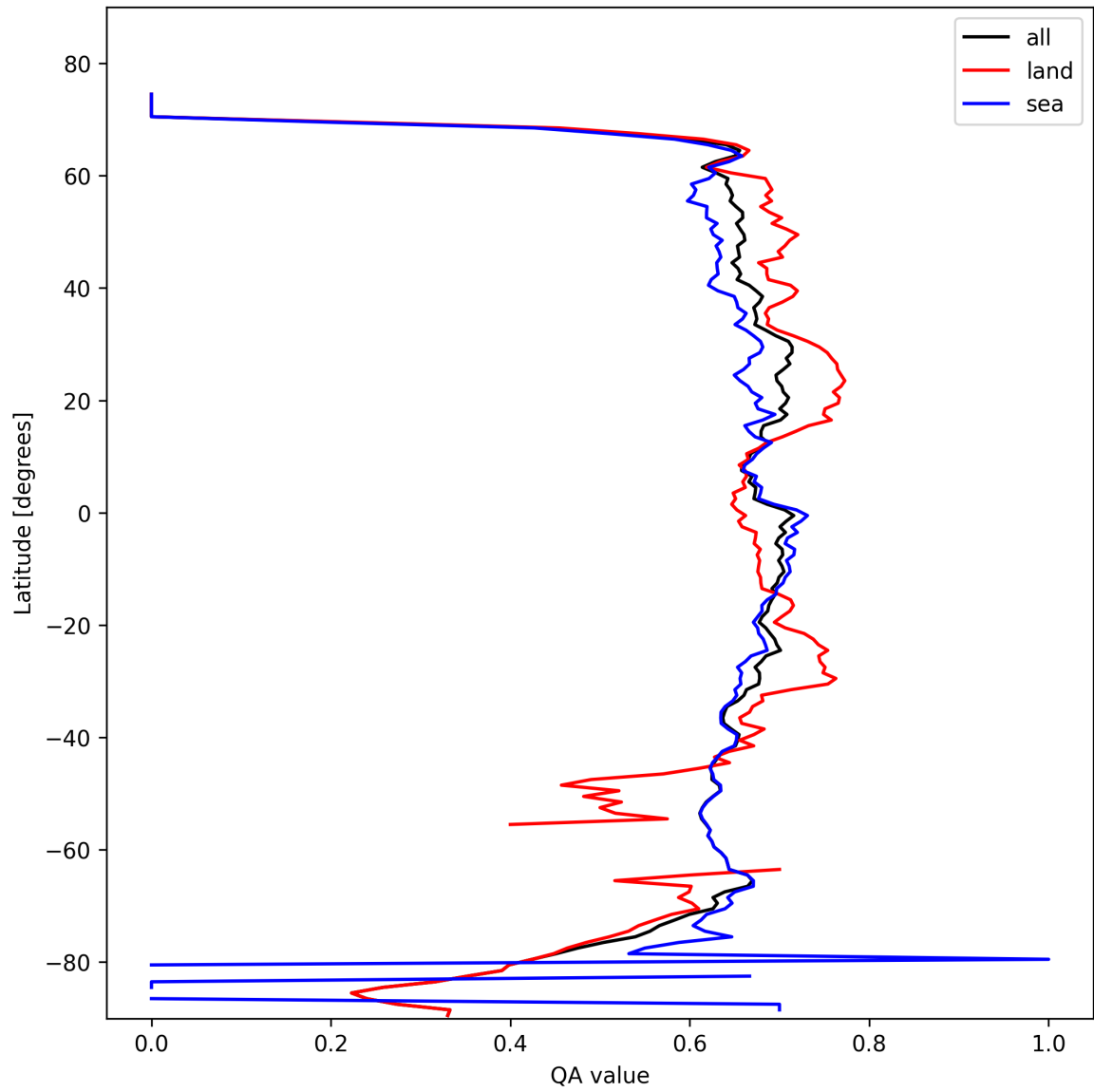
Figure 9: Zonal average of “QA value” for 2025-10-18 to 2025-10-20.
