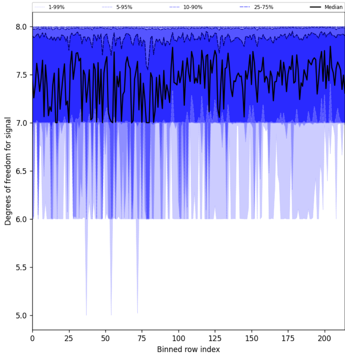
Figure 31: Along track statistics of “Degrees of freedom for signal” for 2025-10-18 to 2025-10-20
