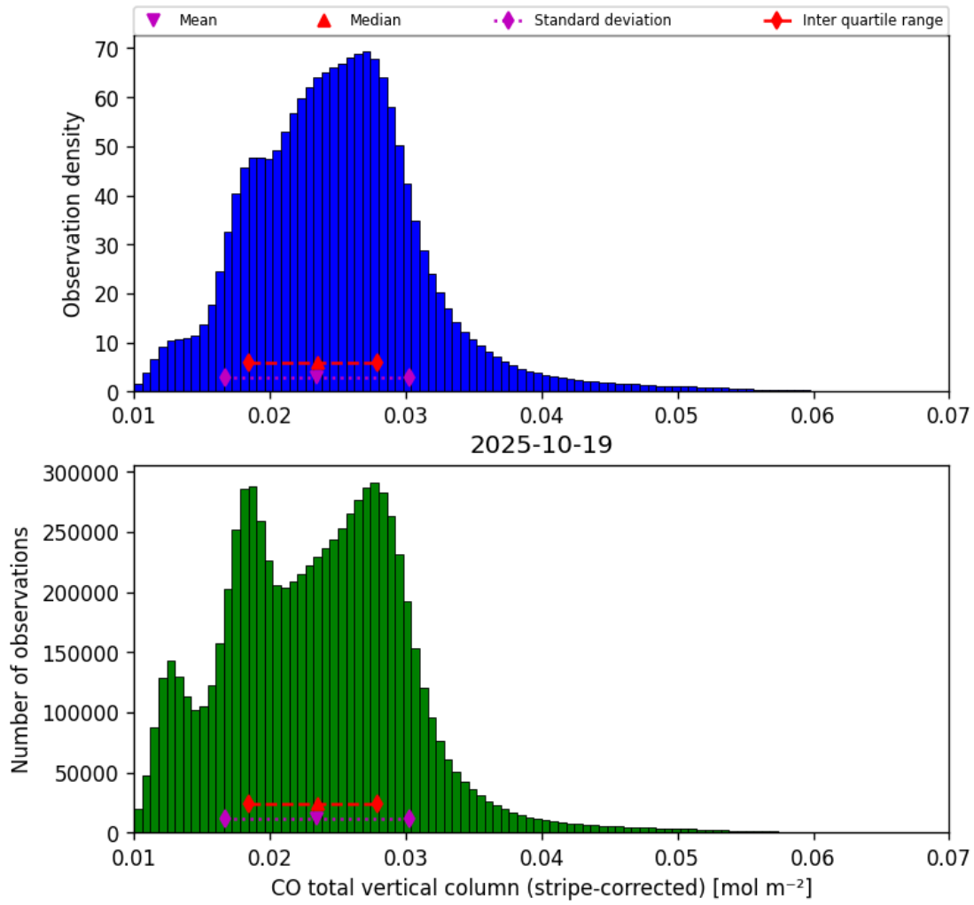
Figure 19: Histogram of “CO total vertical column (stripe-corrected)” for 2025-10-18 to 2025-10-20
