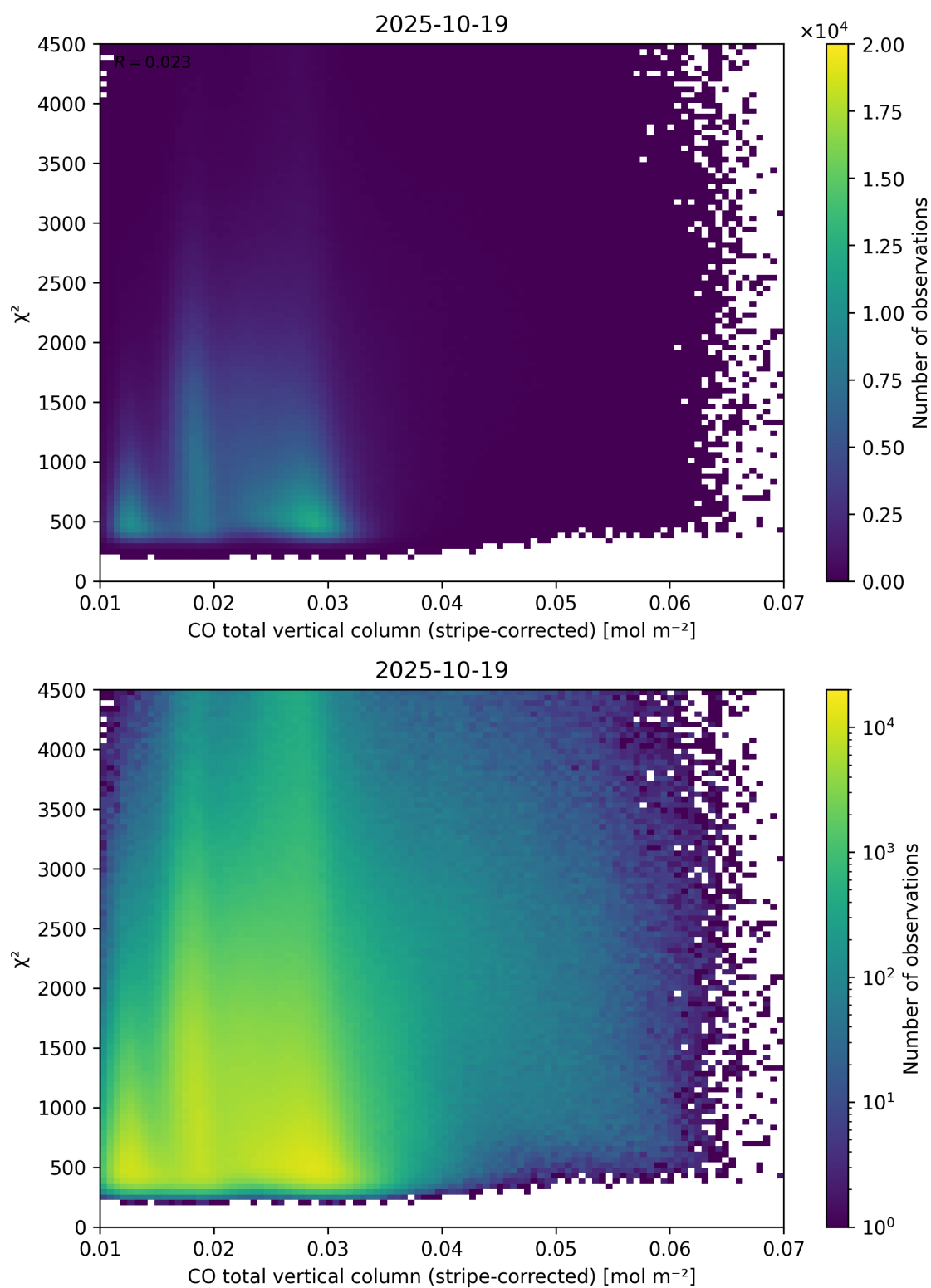
Figure 37: Scatter density plot of “CO total vertical column (stripe-corrected)” against “ \chi^2 ” for 2025-10-18 to 2025-10-20.
