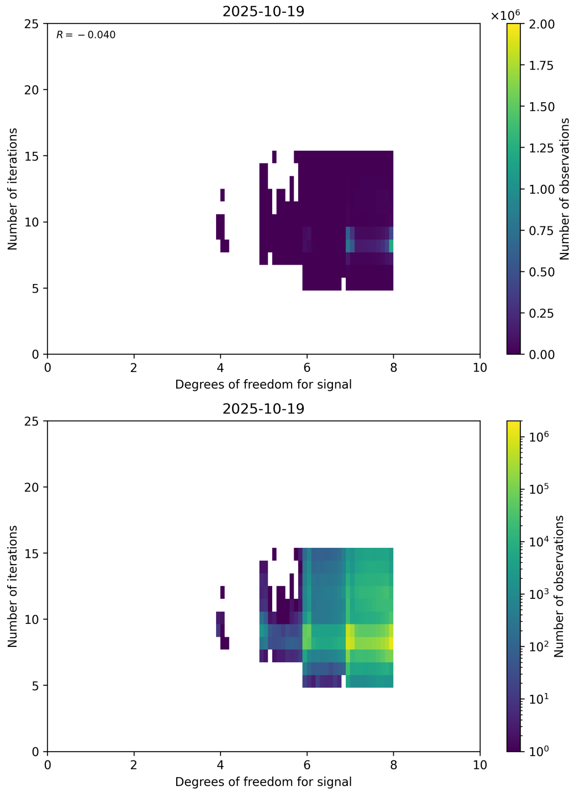
Figure 50: Scatter density plot of “Degrees of freedom for signal” against “Number of iterations” for 2025-10-18 to 2025-10-20.
