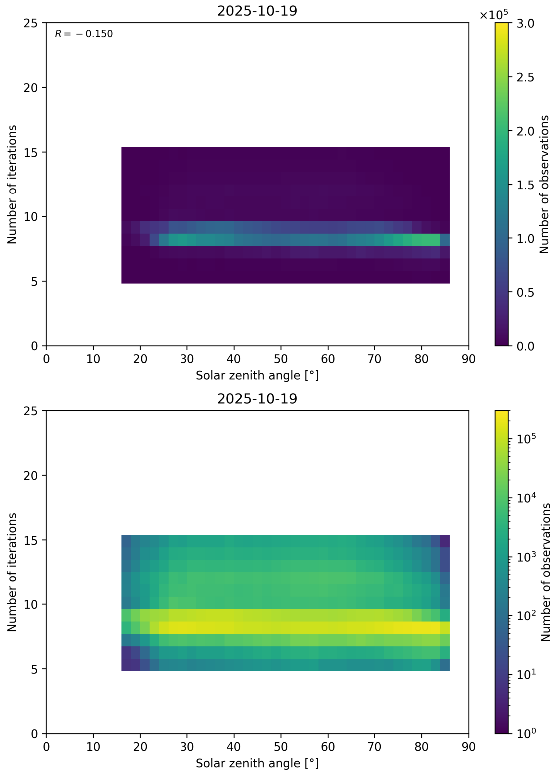
Figure 67: Scatter density plot of “Solar zenith angle” against “Number of iterations” for 2025-10-18 to 2025-10-20.
