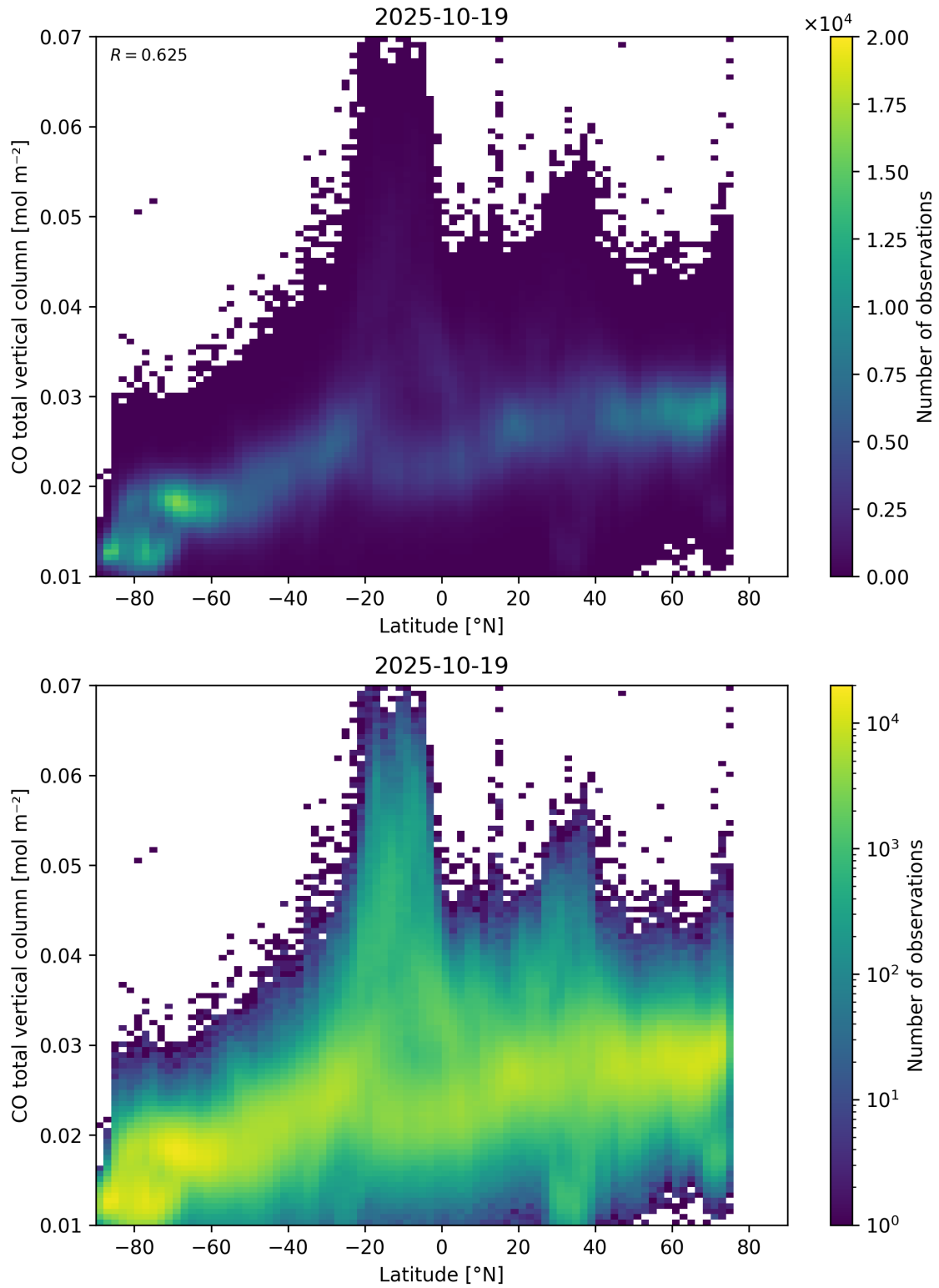
Figure 51: Scatter density plot of “Latitude” against “CO total vertical column” for 2025-10-18 to 2025-10-20.
