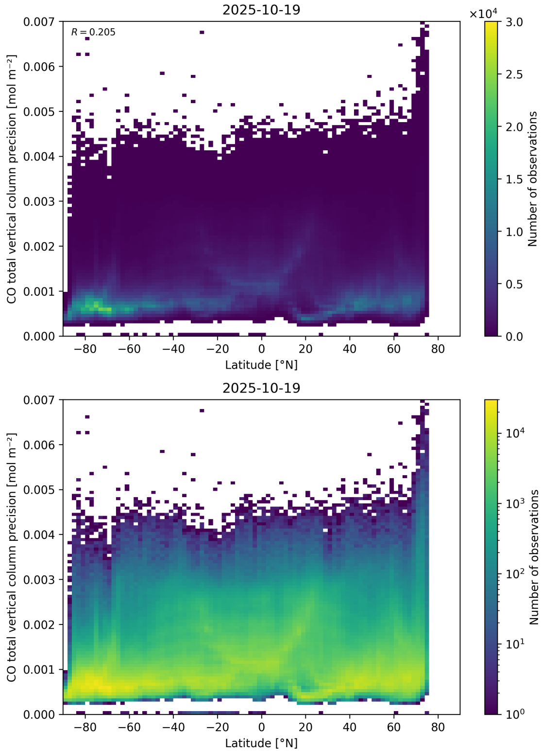
Figure 53: Scatter density plot of “Latitude” against “CO total vertical column precision” for 2025-10-18 to 2025-10-20.
