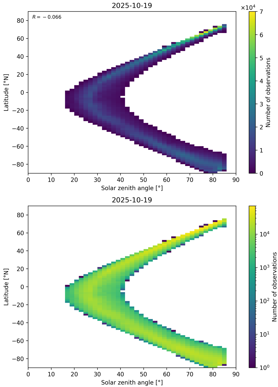
Figure 66: Scatter density plot of “Solar zenith angle” against “Latitude” for 2025-10-18 to 2025-10-20.
