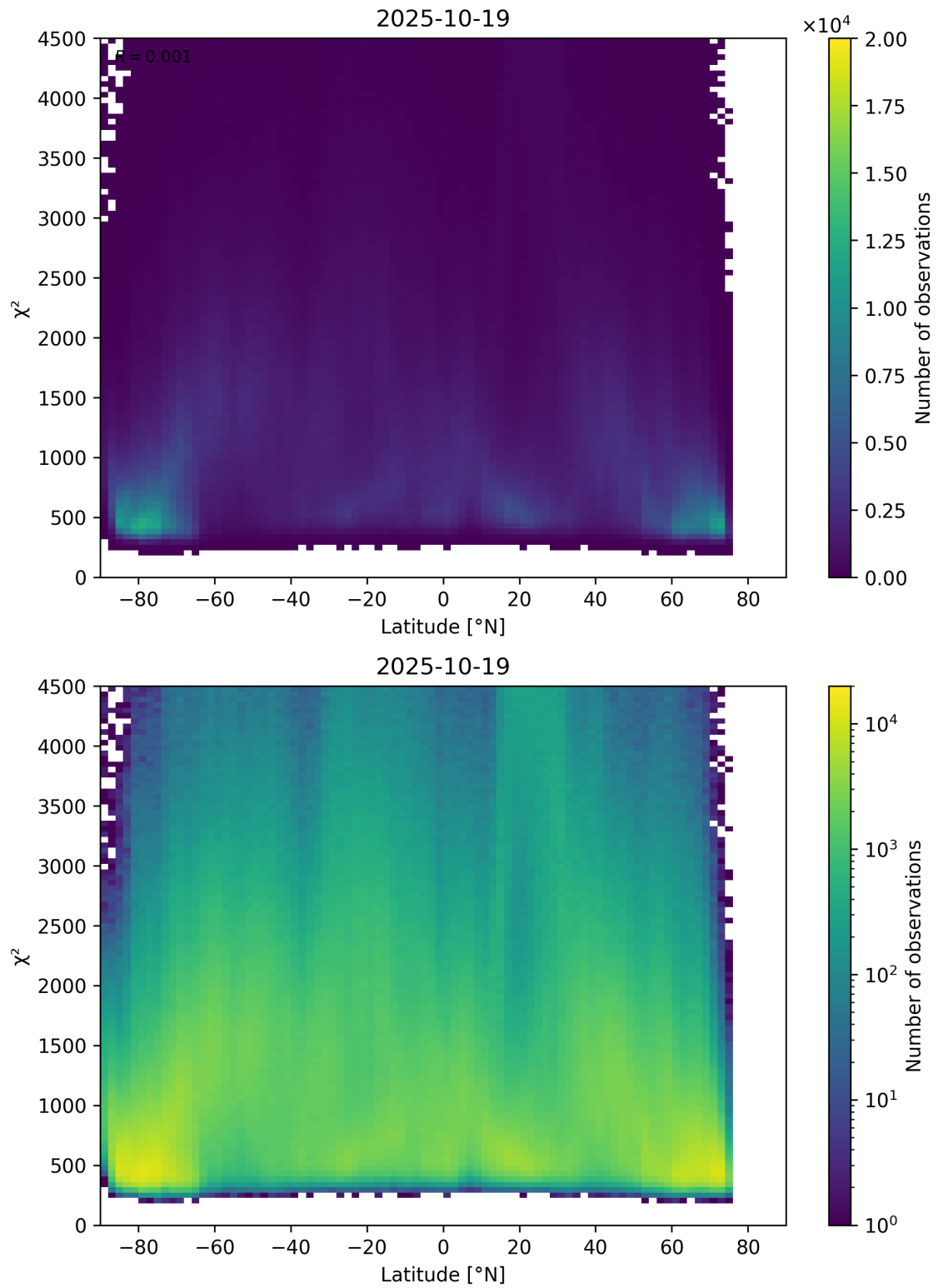
Figure 54: Scatter density plot of “Latitude” against “ \chi^2 ” for 2025-10-18 to 2025-10-20.
