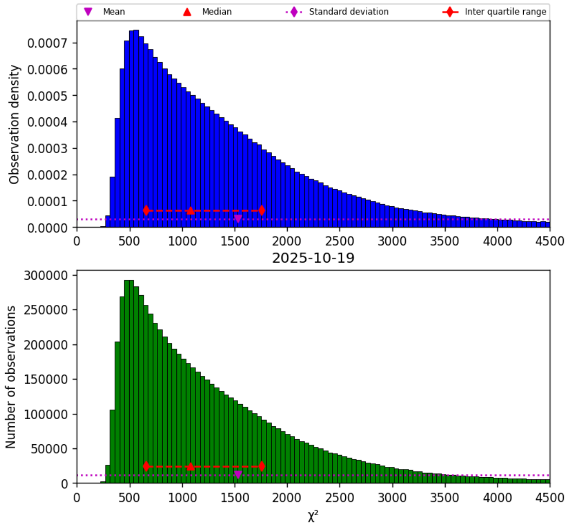
Figure 22: Histogram of “ \chi^2 ” for 2025-10-18 to 2025-10-20
