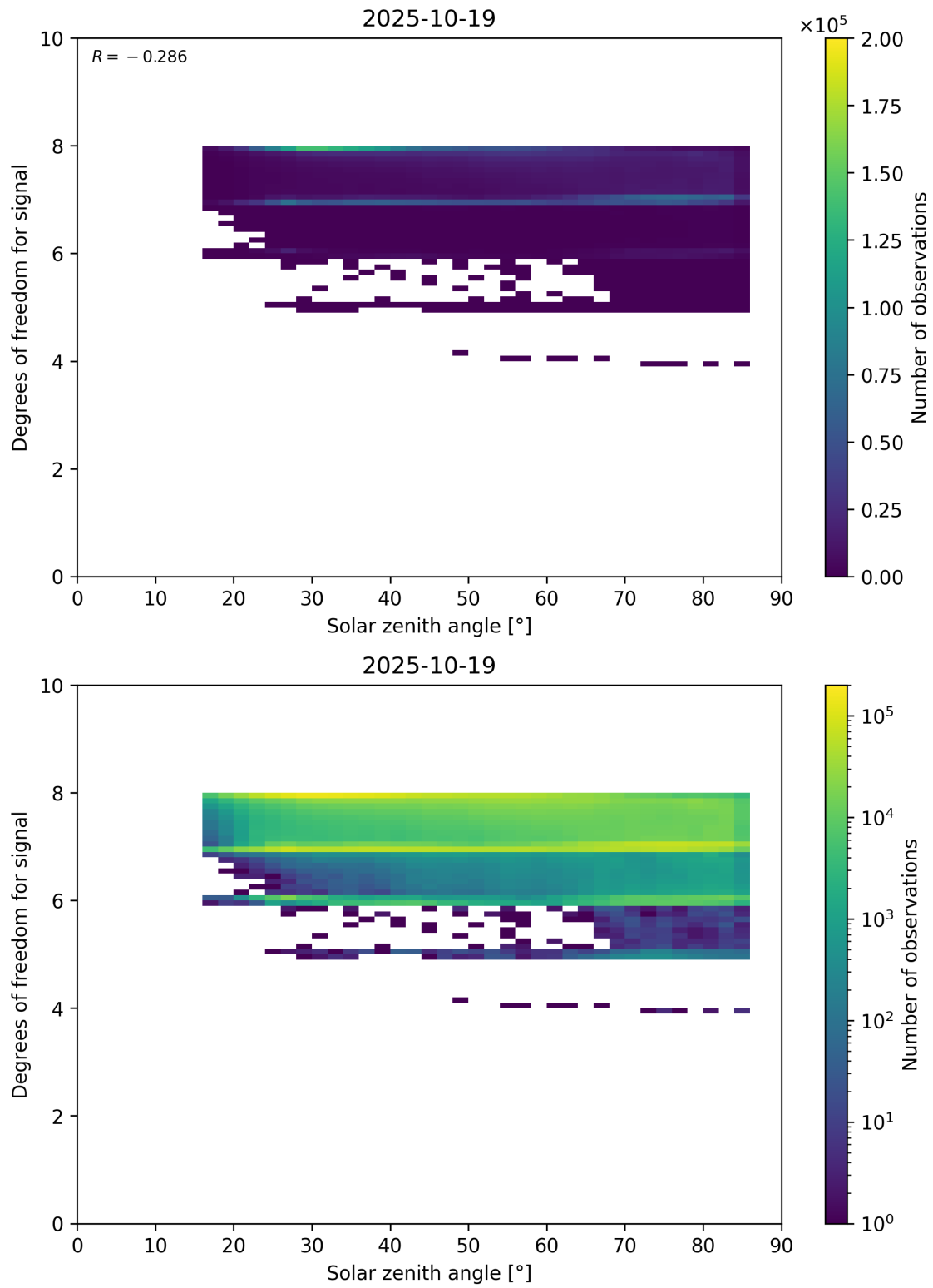
Figure 65: Scatter density plot of “Solar zenith angle” against “Degrees of freedom for signal” for 2025-10-18 to 2025-10-20.
