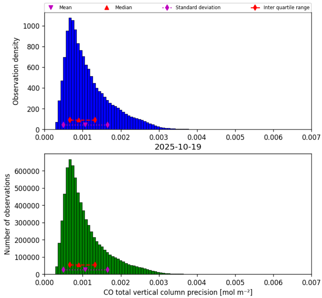
Figure 20: Histogram of “CO total vertical column precision” for 2025-10-18 to 2025-10-20
