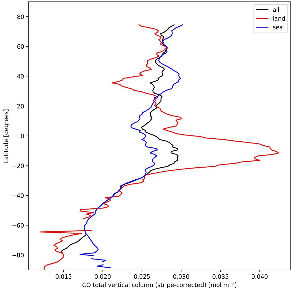
Figure 11: Zonal average of “CO total vertical column (stripe-corrected)” for 2025-10-18 to 2025-10-20.
