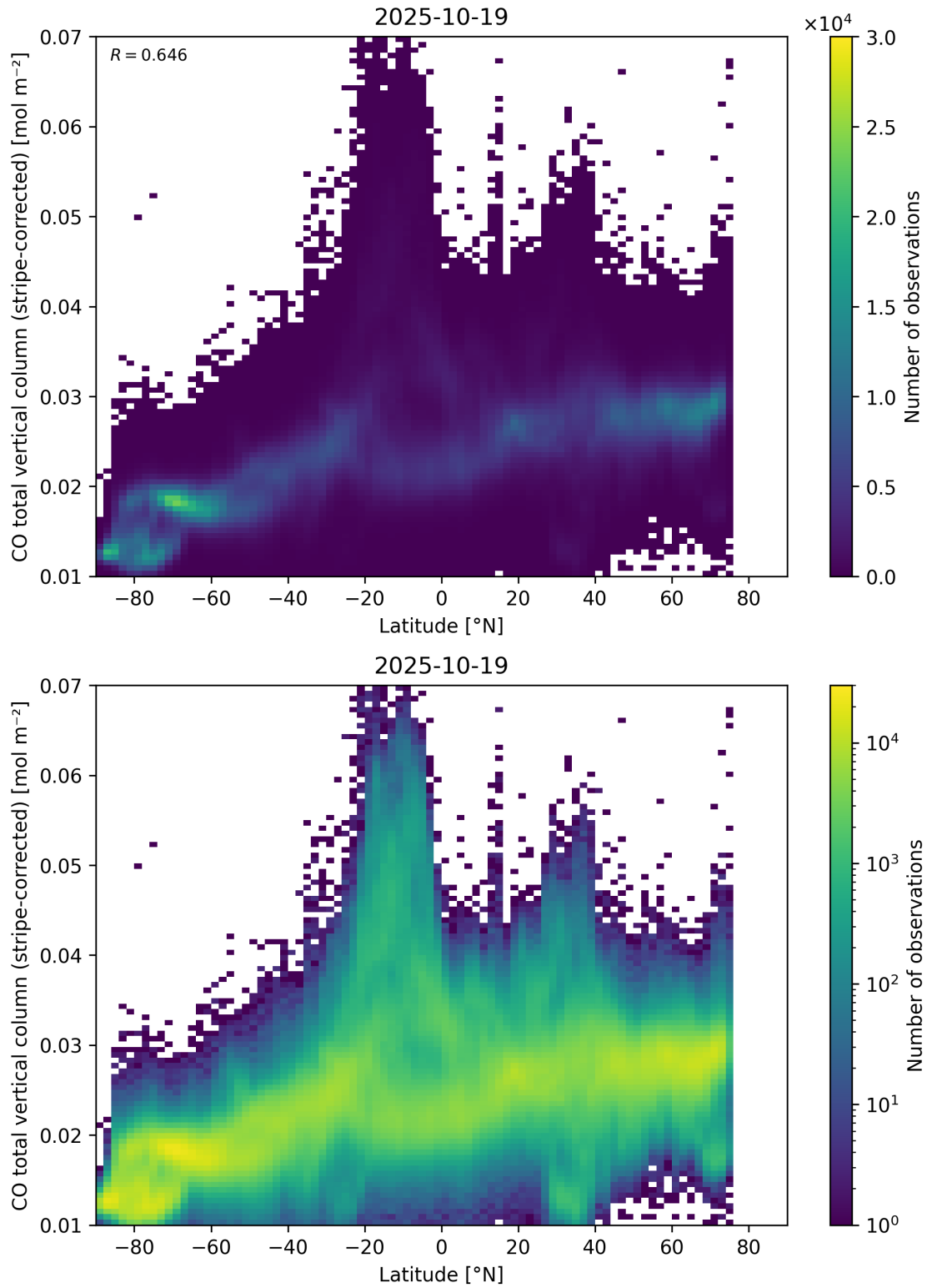
Figure 52: Scatter density plot of “Latitude” against “CO total vertical column (stripe-corrected)” for 2025-10-18 to 2025-10-20.
