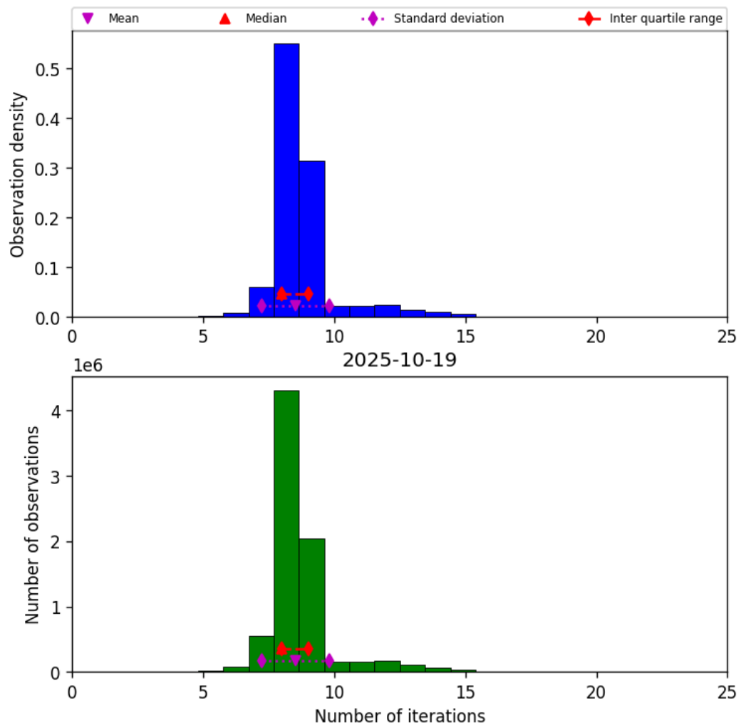
Figure 24: Histogram of “Number of iterations” for 2025-10-18 to 2025-10-20
