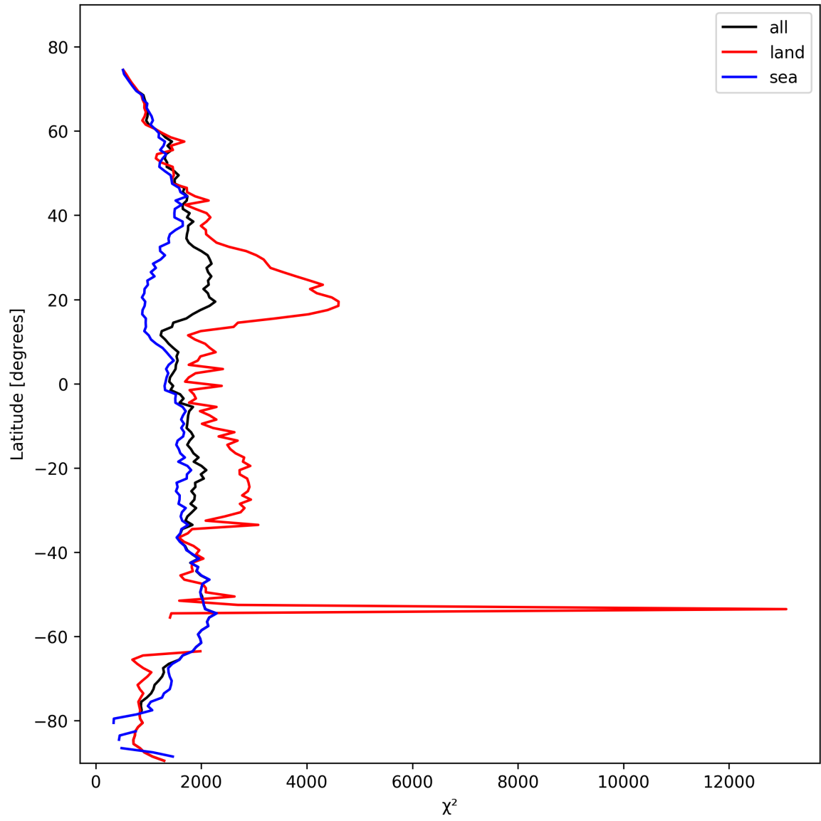
Figure 14: Zonal average of “ \chi^2 ” for 2025-10-18 to 2025-10-20.
