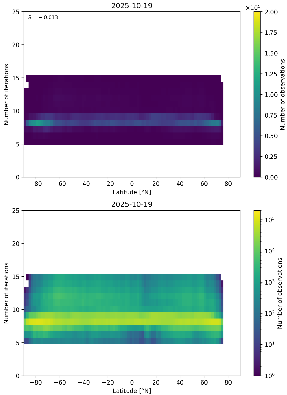
Figure 56: Scatter density plot of “Latitude” against “Number of iterations” for 2025-10-18 to 2025-10-20.
