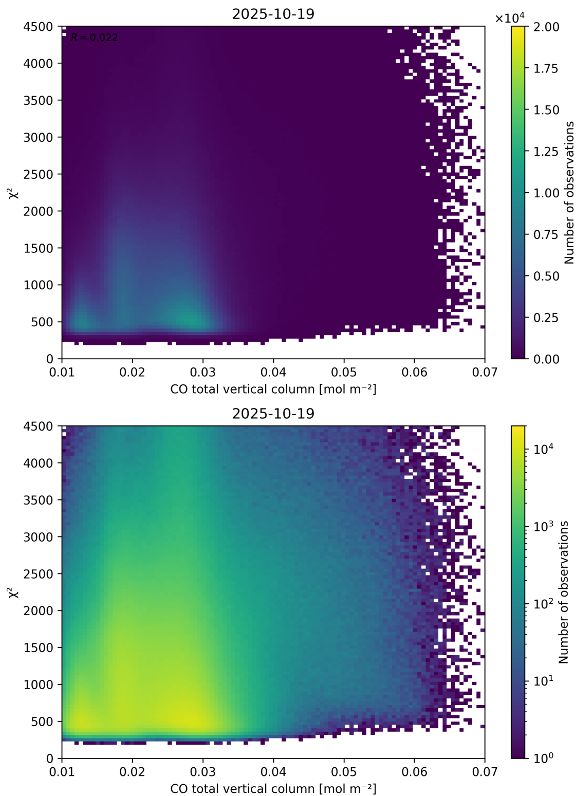
Figure 35: Scatter density plot of “CO total vertical column” against “ \chi^2 ” for 2025-10-18 to 2025-10-20.
