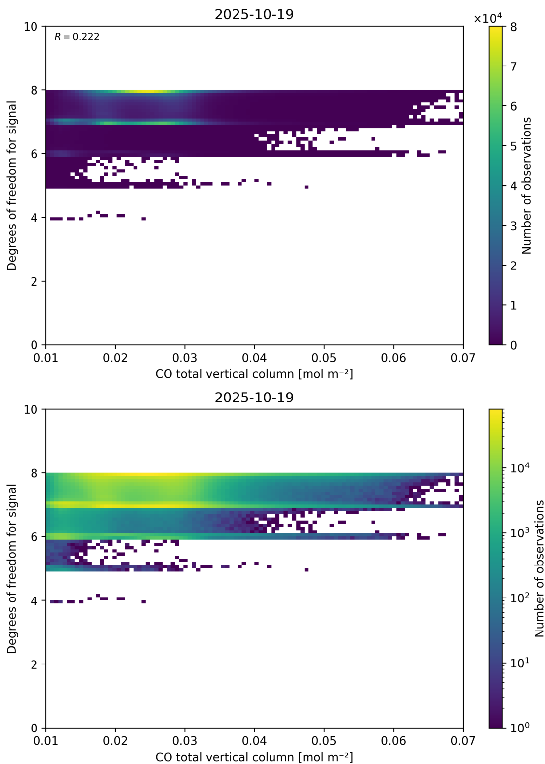
Figure 41: Scatter density plot of “CO total vertical column” against “Degrees of freedom for signal” for 2025-10-18 to 2025-10-20.
