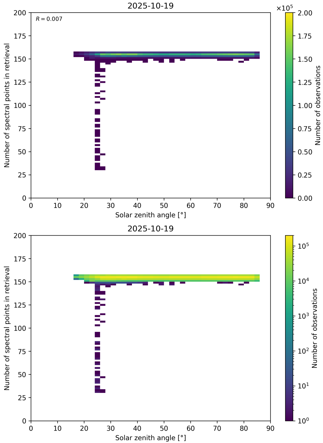
Figure 68: Scatter density plot of “Solar zenith angle” against “Number of spectral points in retrieval” for 2025-10-18 to 2025-10-20.
