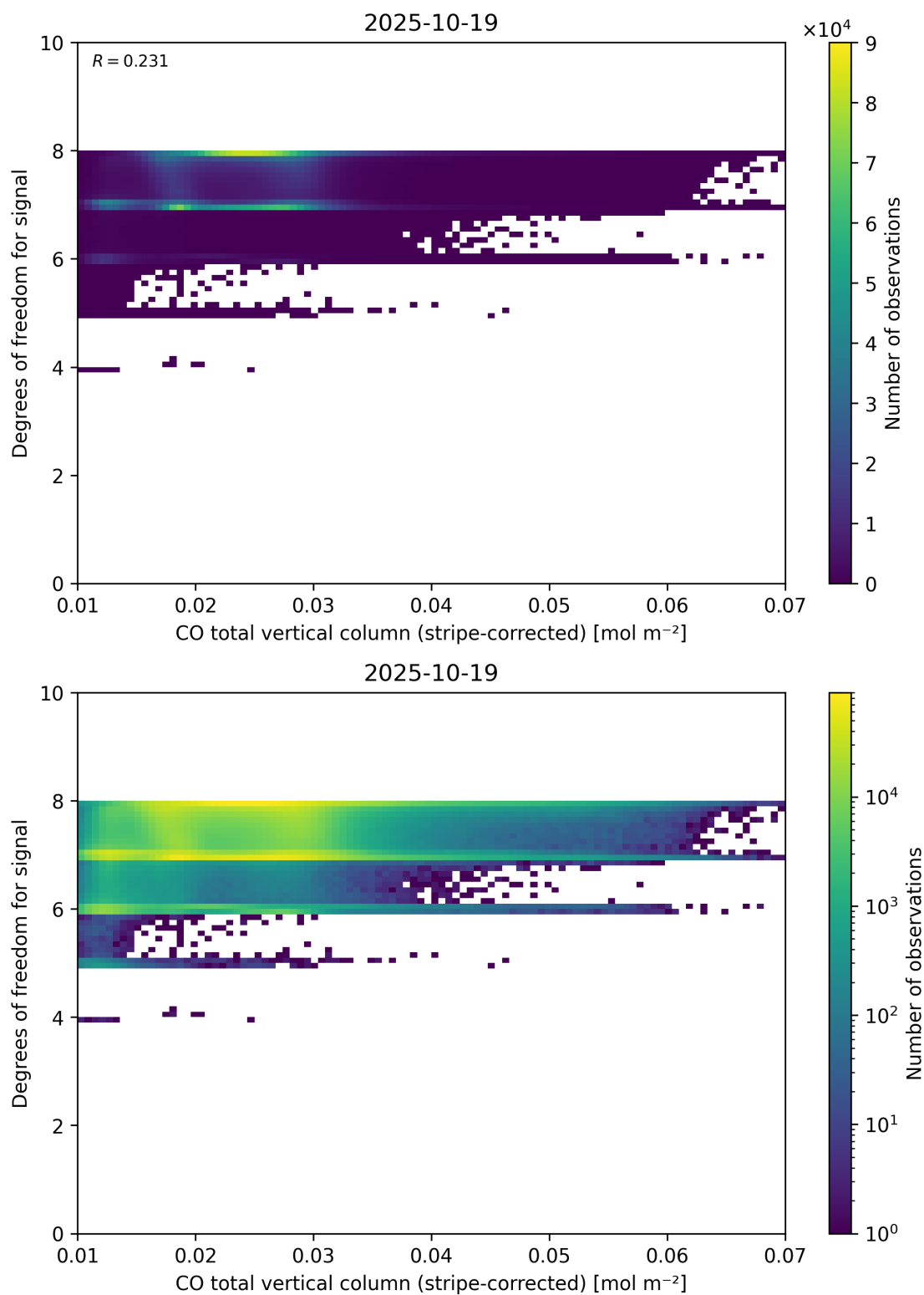
Figure 38: Scatter density plot of “CO total vertical column (stripe-corrected)” against “Degrees of freedom for signal” for 2025-10-18 to 2025-10-20.
