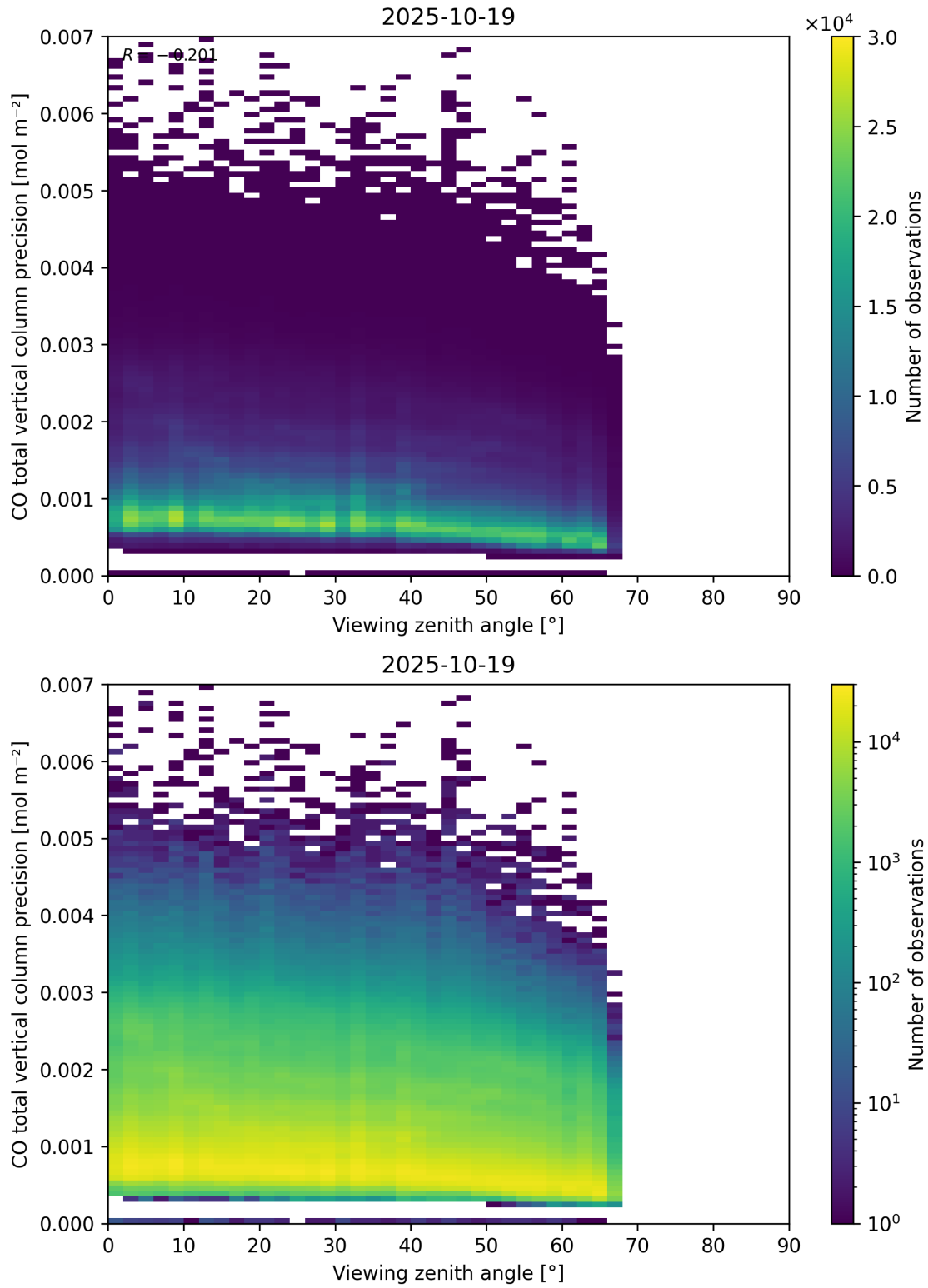
Figure 71: Scatter density plot of “Viewing zenith angle” against “CO total vertical column precision” for 2025-10-18 to 2025-10-20.
