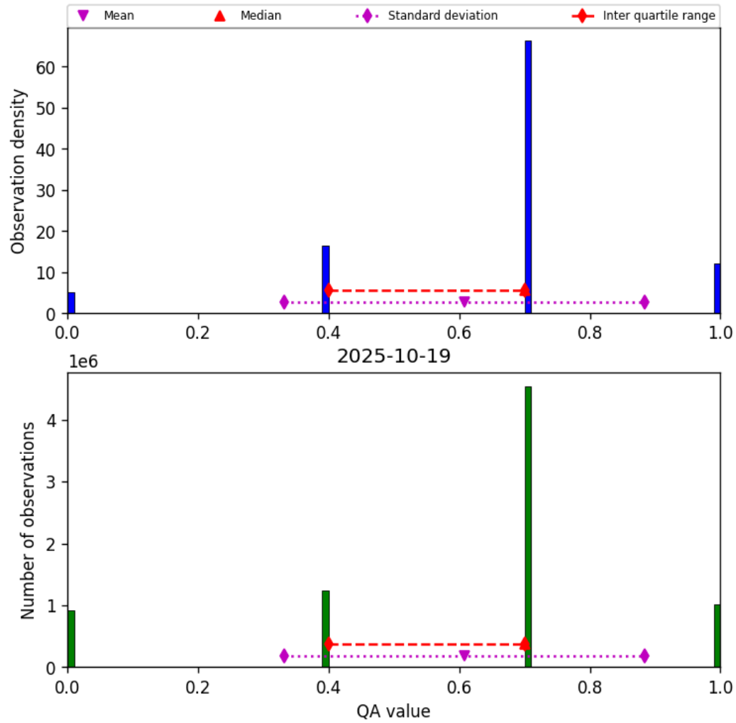
Figure 17: Histogram of “QA value” for 2025-10-18 to 2025-10-20
