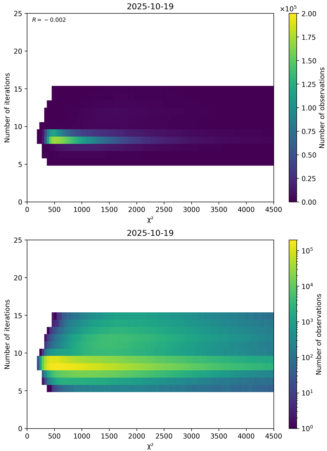
Figure 49: Scatter density plot of “ \chi^2 ” against “Number of iterations” for 2025-10-18 to 2025-10-20.
