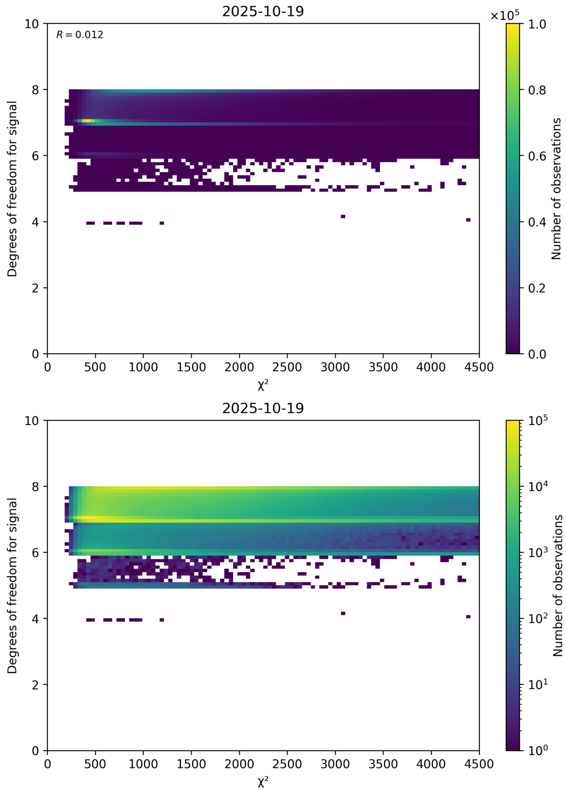
Figure 48: Scatter density plot of “ \chi^2 ” against “Degrees of freedom for signal” for 2025-10-18 to 2025-10-20.
