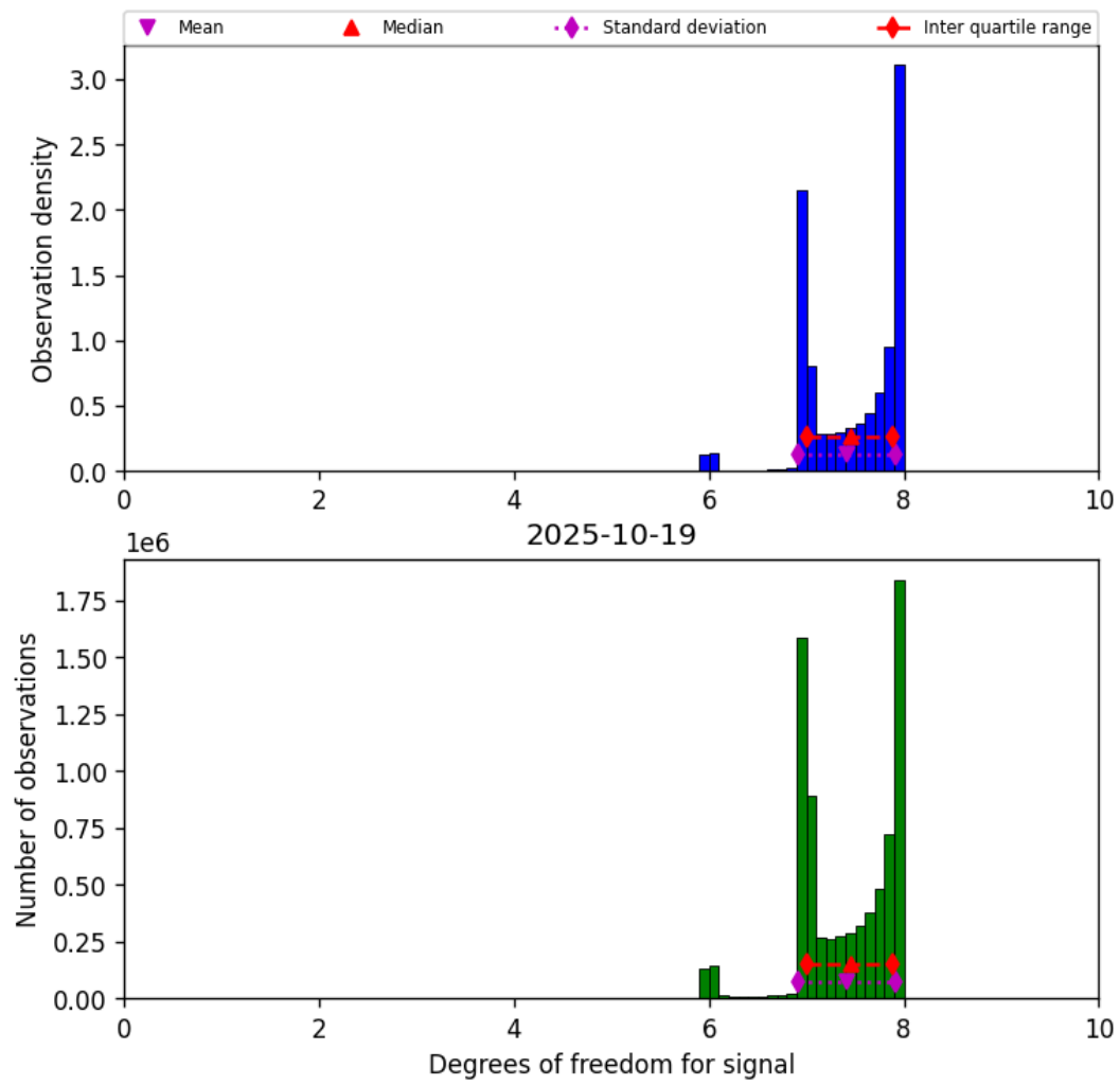
Figure 23: Histogram of “Degrees of freedom for signal” for 2025-10-18 to 2025-10-20
