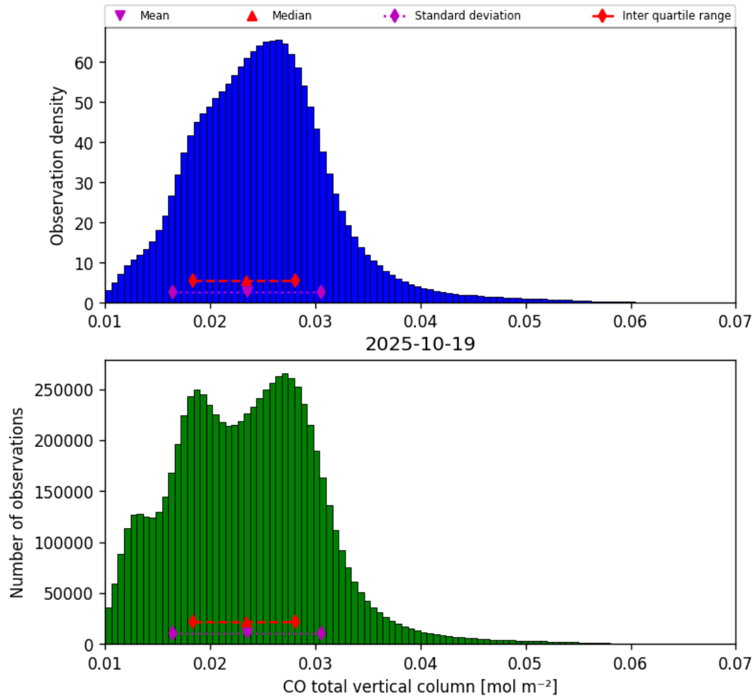
Figure 18: Histogram of “CO total vertical column” for 2025-10-18 to 2025-10-20
