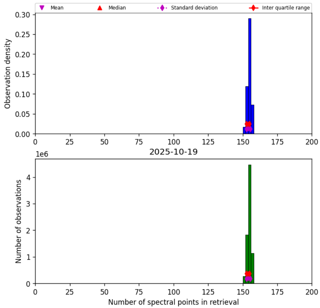
Figure 21: Histogram of “Number of spectral points in retrieval” for 2025-10-18 to 2025-10-20
