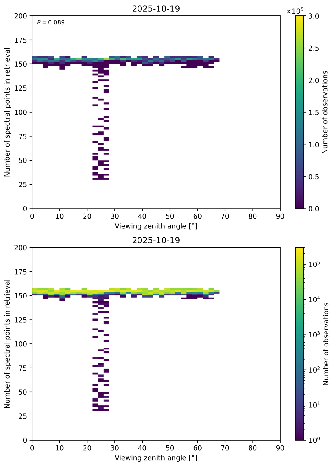
Figure 76: Scatter density plot of “Viewing zenith angle” against “Number of spectral points in retrieval” for 2025-10-18 to 2025-10-20.
