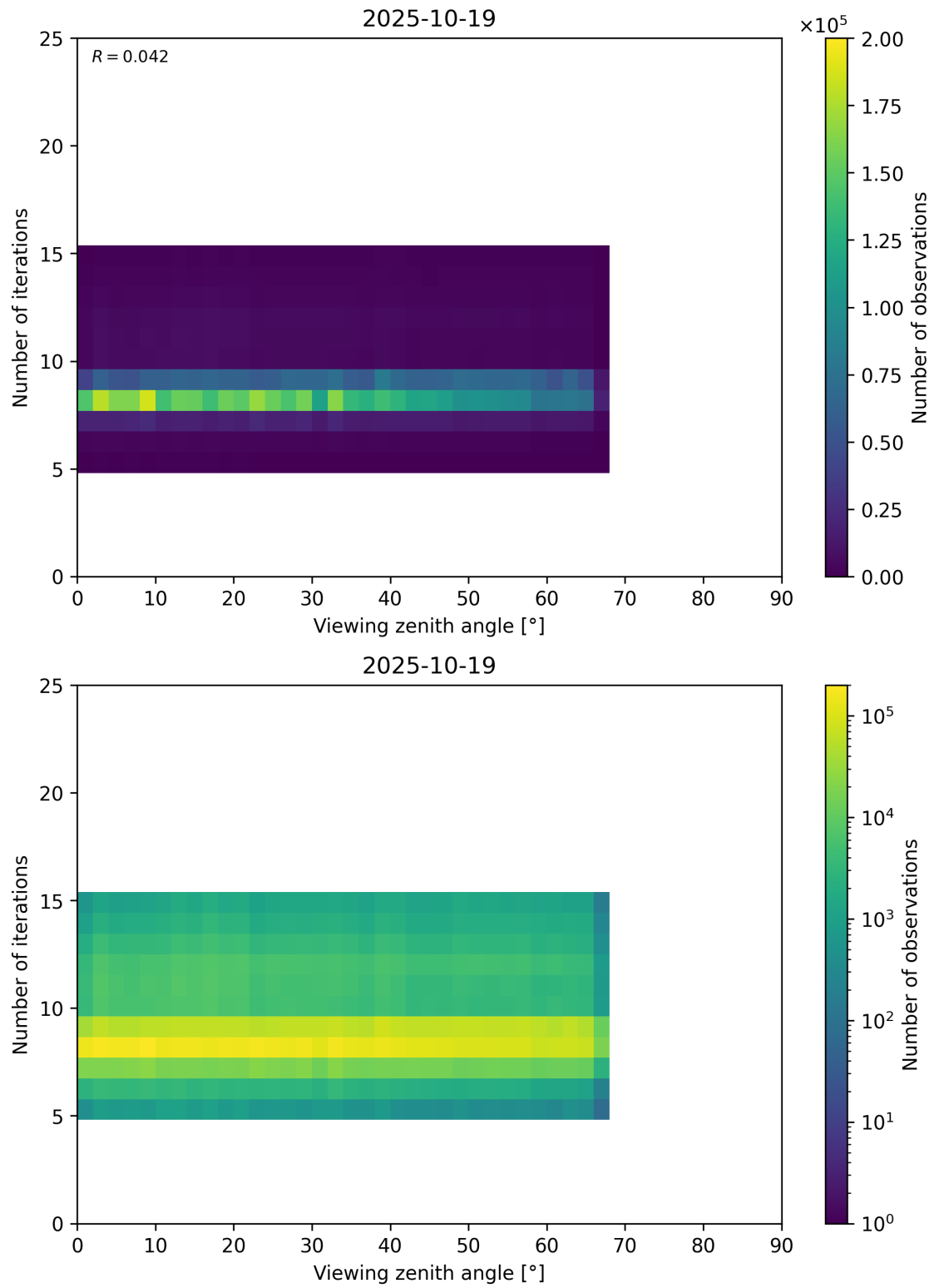
Figure 75: Scatter density plot of “Viewing zenith angle” against “Number of iterations” for 2025-10-18 to 2025-10-20.
