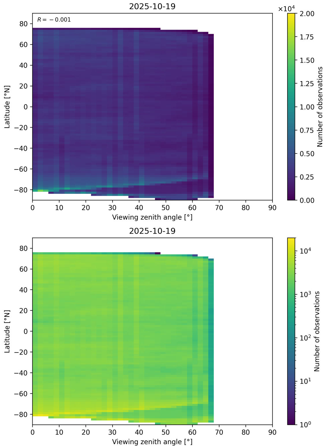
Figure 74: Scatter density plot of “Viewing zenith angle” against “Latitude” for 2025-10-18 to 2025-10-20.
