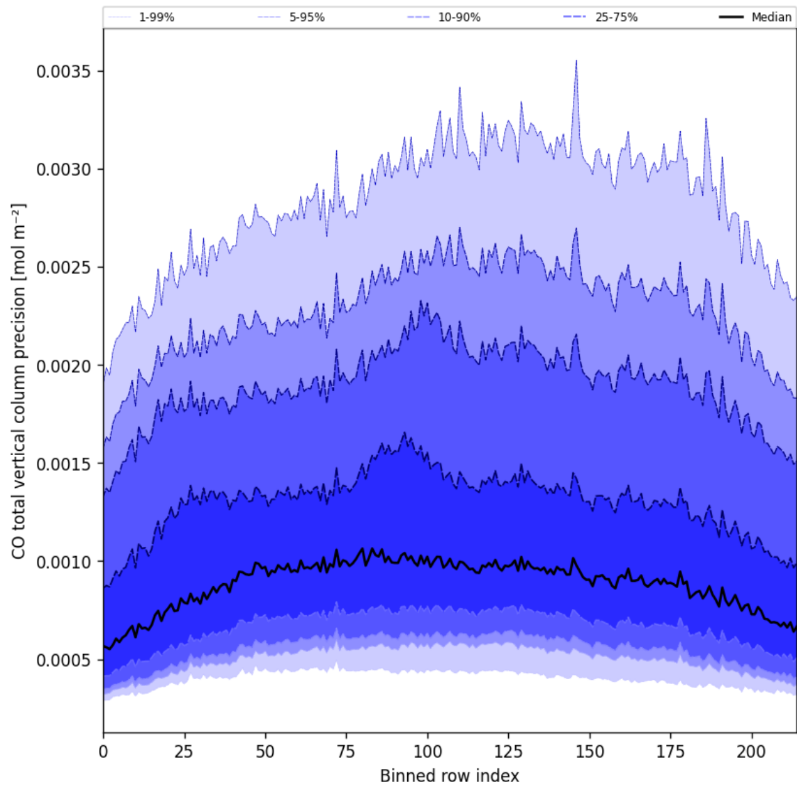
Figure 28: Along track statistics of “CO total vertical column precision” for 2025-10-18 to 2025-10-20
