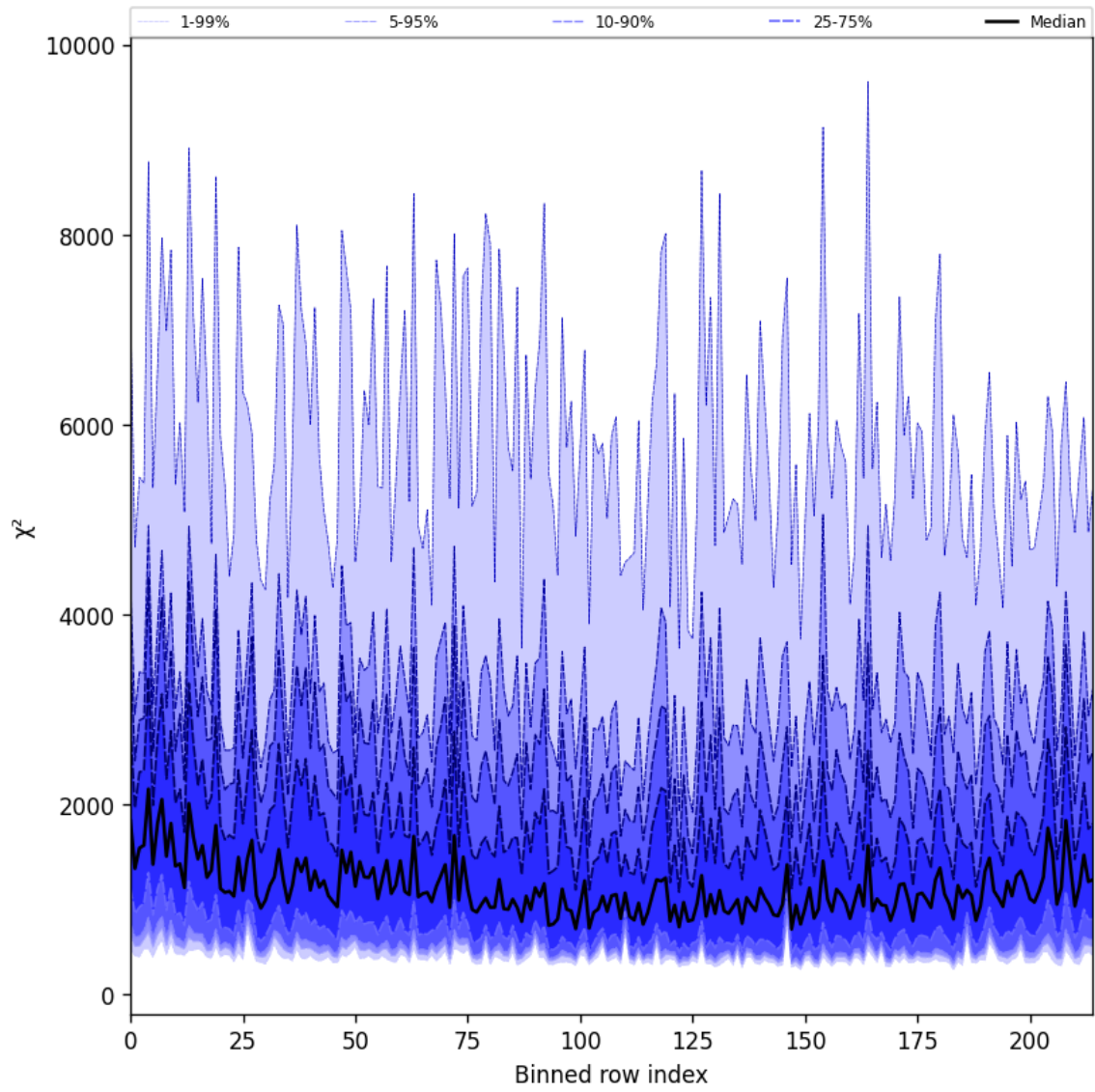
Figure 30: Along track statistics of “ \chi^2 ” for 2025-10-18 to 2025-10-20
