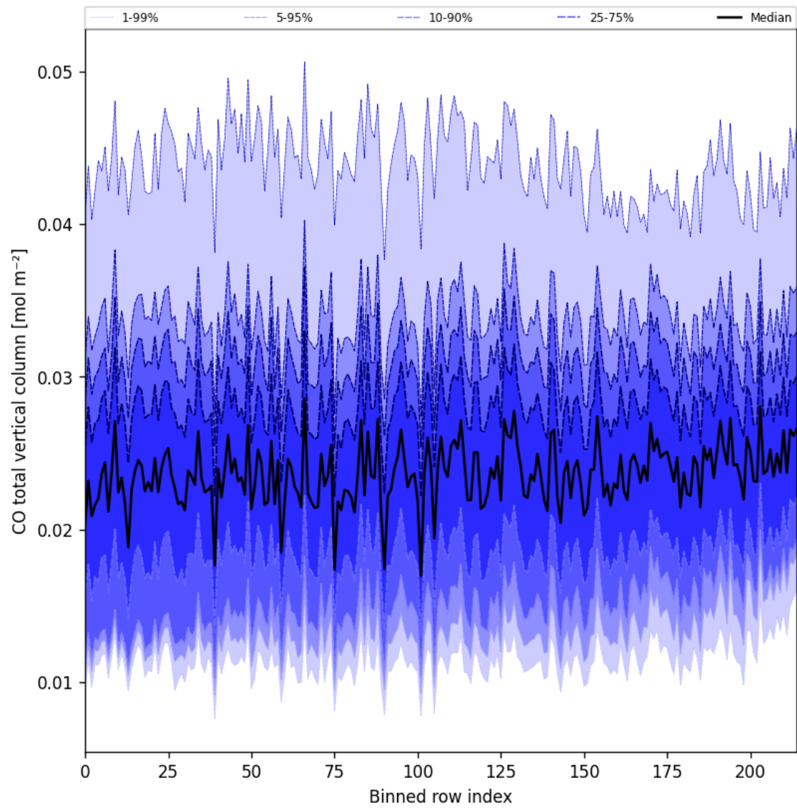
Figure 26: Along track statistics of “CO total vertical column” for 2025-10-18 to 2025-10-20
