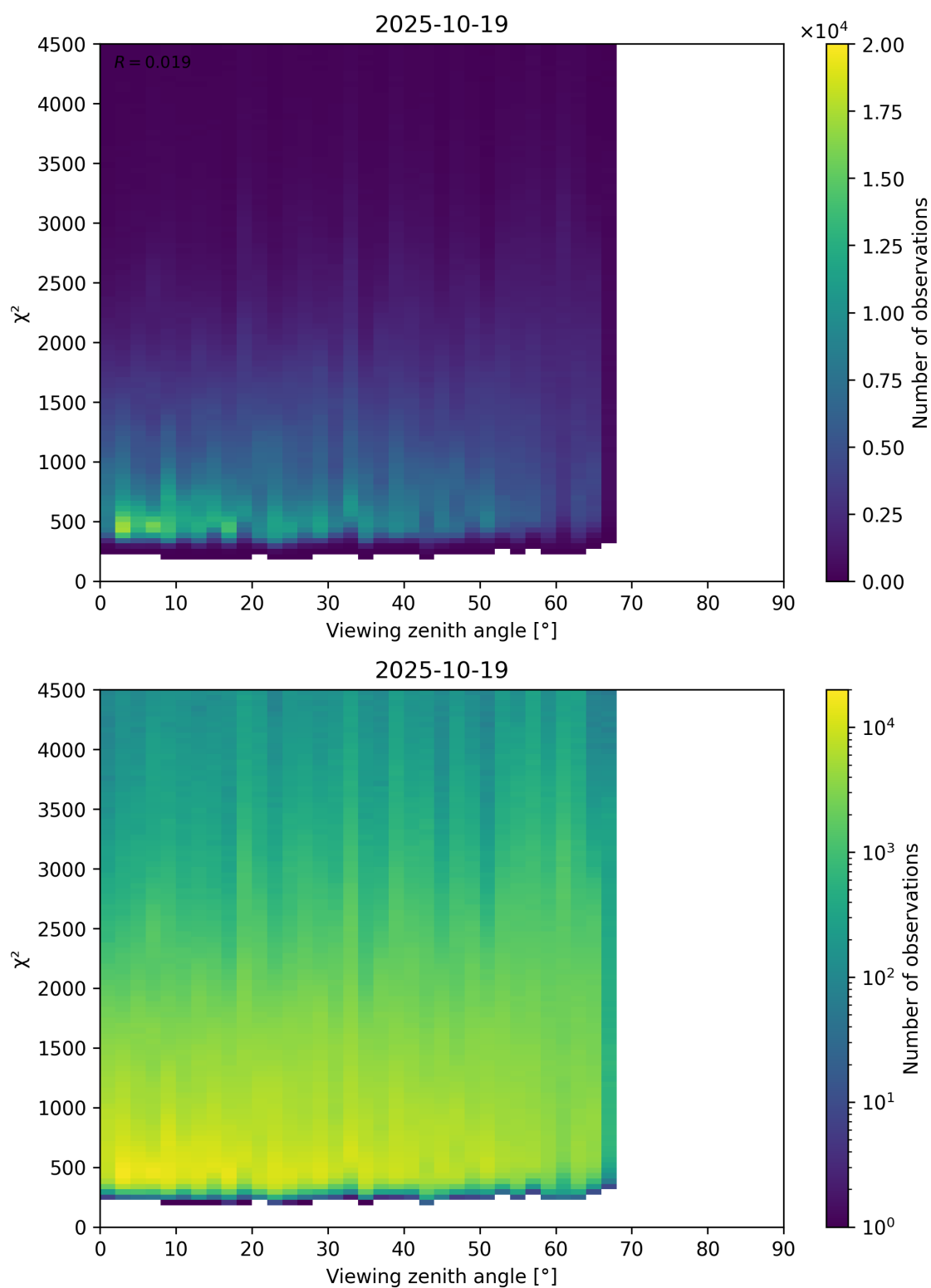
Figure 72: Scatter density plot of “Viewing zenith angle” against “ \chi^2 ” for 2025-10-18 to 2025-10-20.
