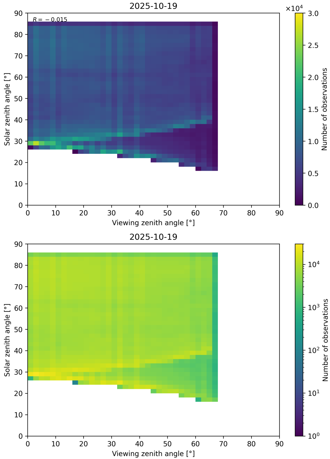
Figure 77: Scatter density plot of “Viewing zenith angle” against “Solar zenith angle” for 2025-10-18 to 2025-10-20.
