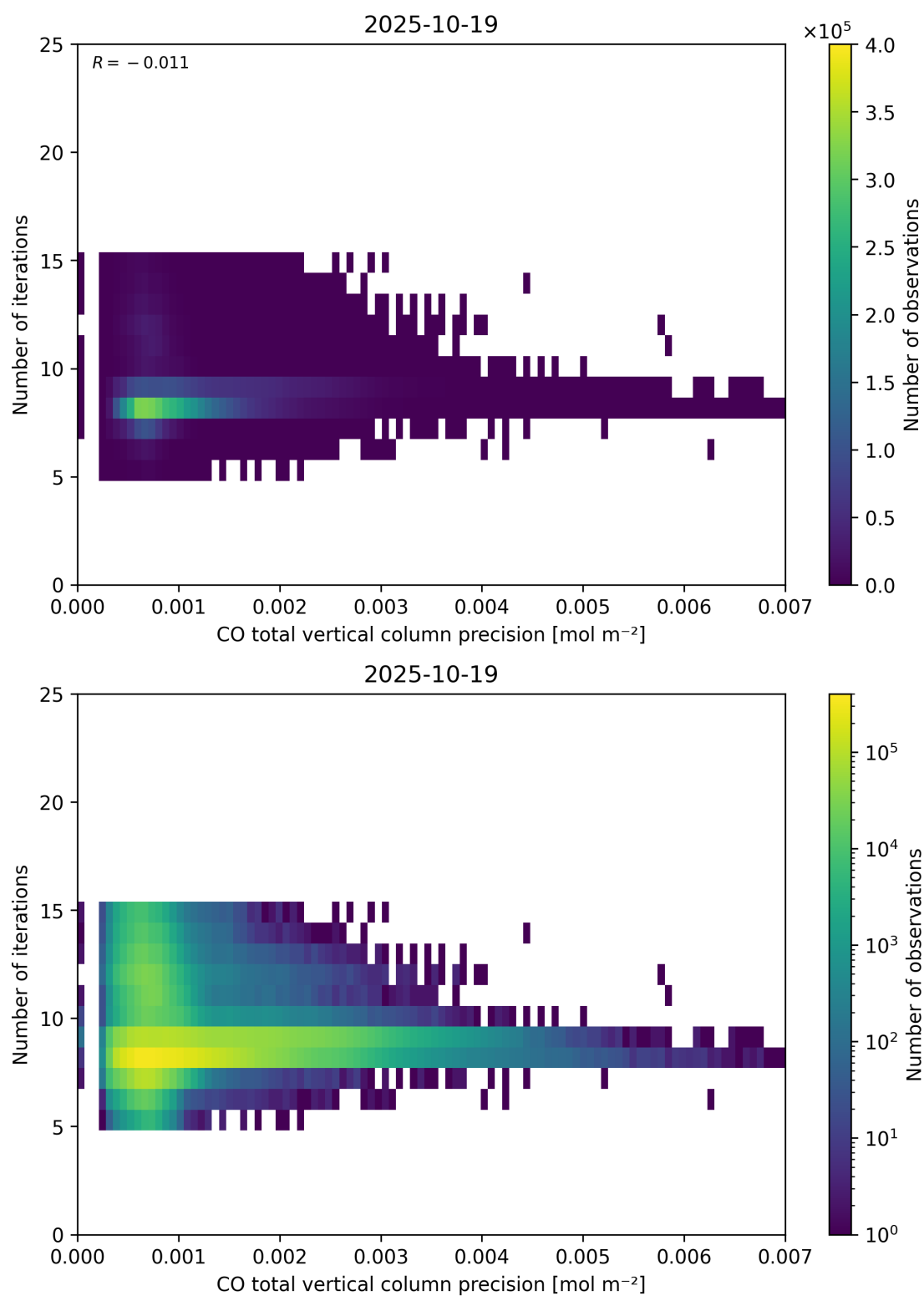
Figure 46: Scatter density plot of “CO total vertical column precision” against “Number of iterations” for 2025-10-18 to 2025-10-20.
