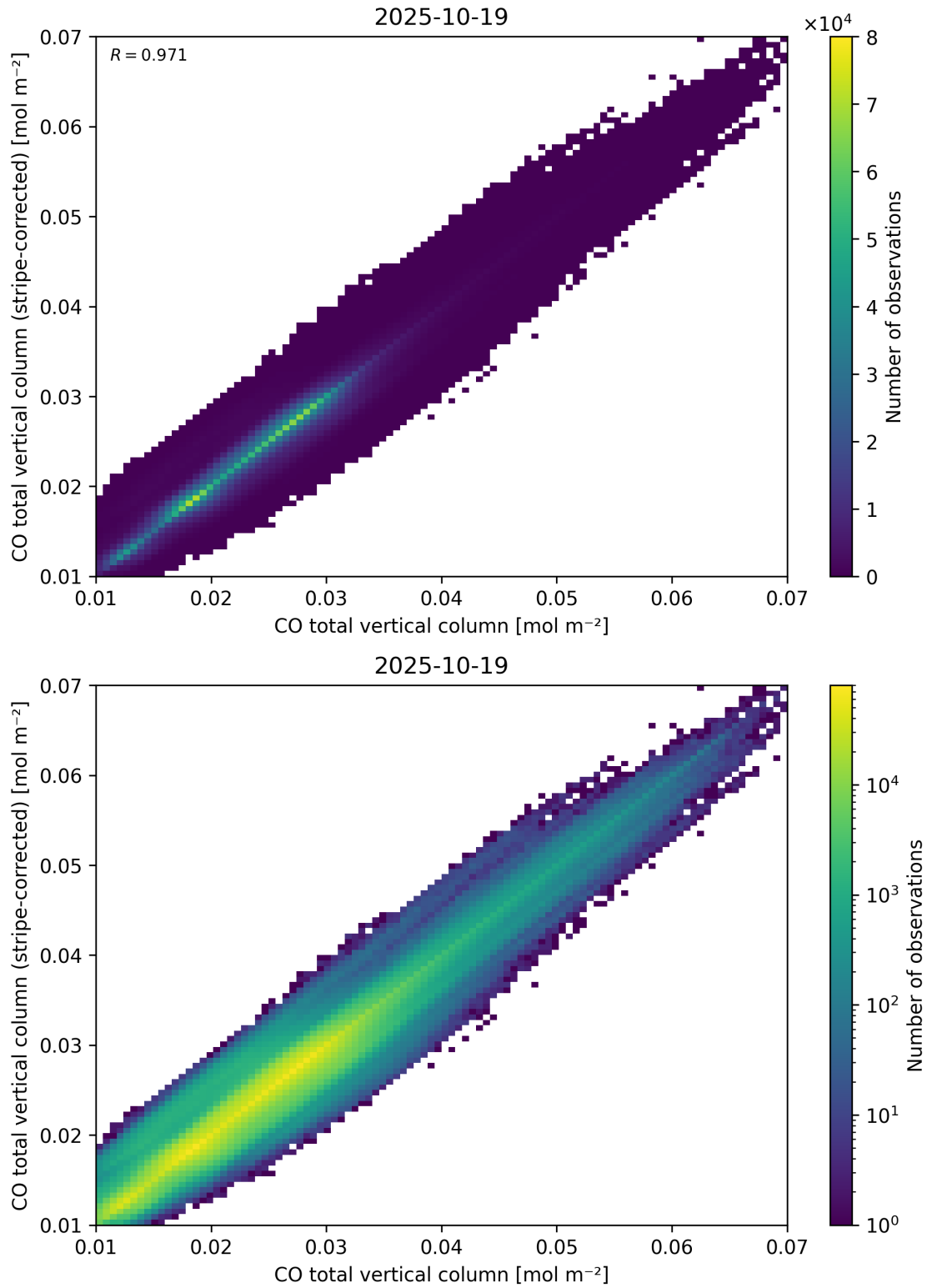
Figure 33: Scatter density plot of “CO total vertical column” against “CO total vertical column (stripe-corrected)” for 2025-10-18 to 2025-10-20.
