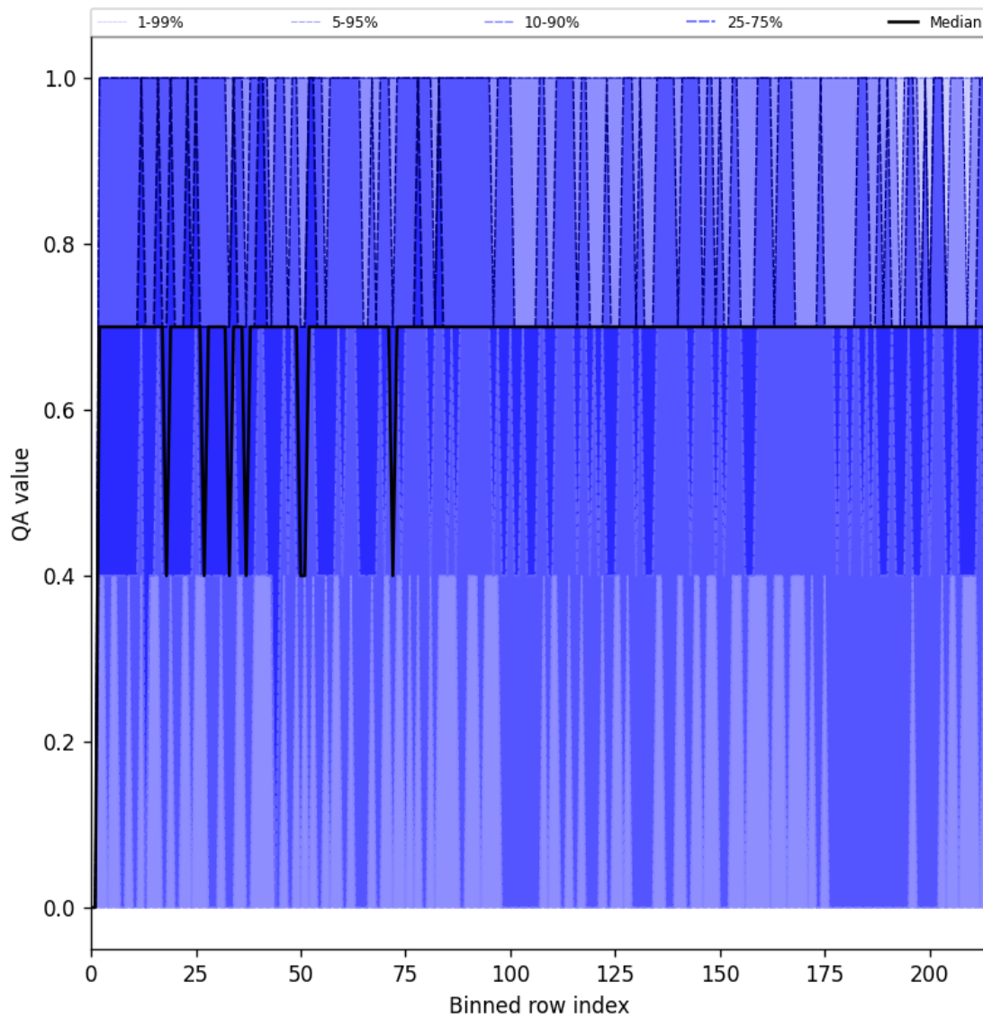
Figure 25: Along track statistics of “QA value” for 2025-10-18 to 2025-10-20
