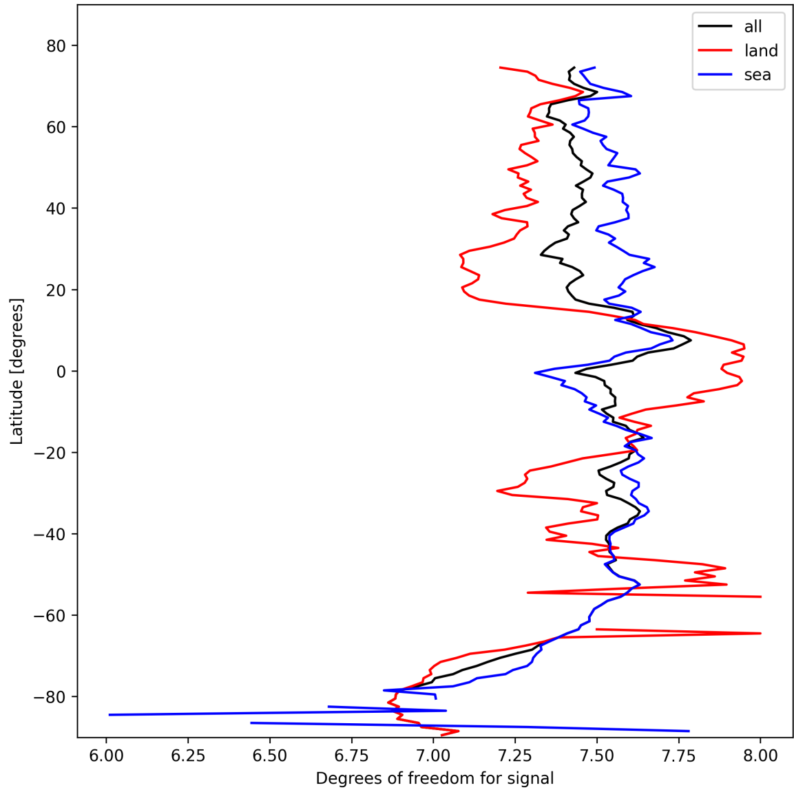
Figure 15: Zonal average of “Degrees of freedom for signal” for 2025-10-18 to 2025-10-20.
