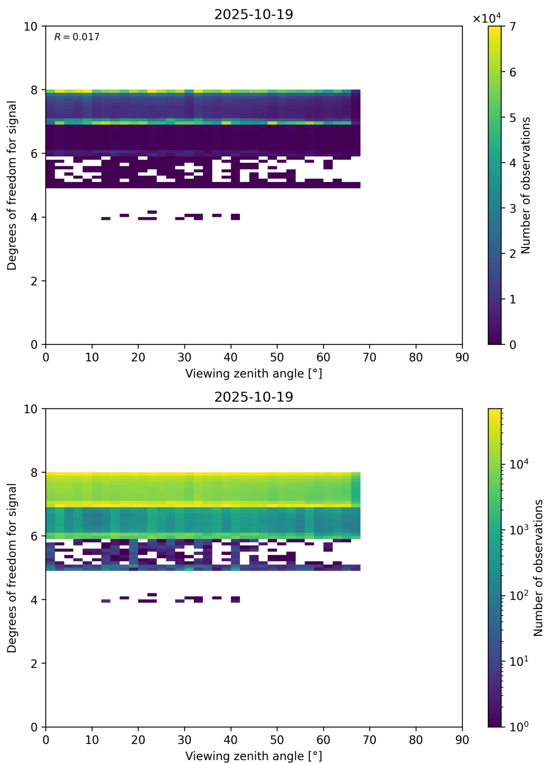
Figure 73: Scatter density plot of “Viewing zenith angle” against “Degrees of freedom for signal” for 2025-10-18 to 2025-10-20.
