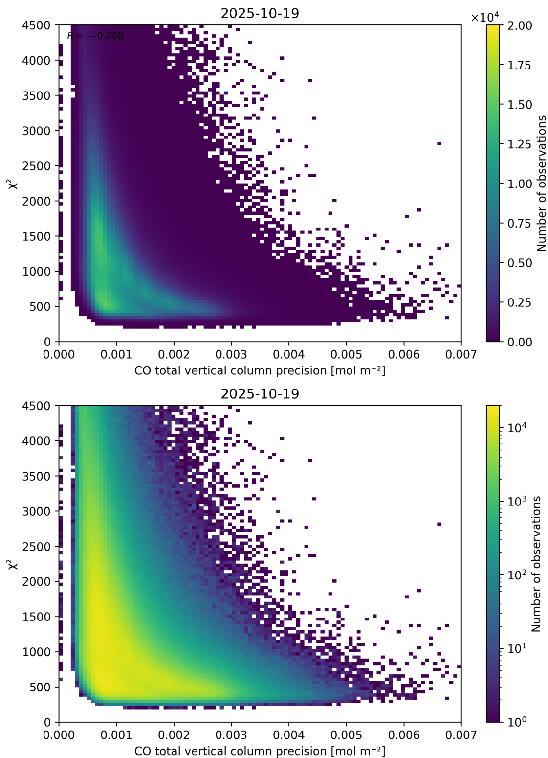
Figure 44: Scatter density plot of “CO total vertical column precision” against “ \chi^2 ” for 2025-10-18 to 2025-10-20.
