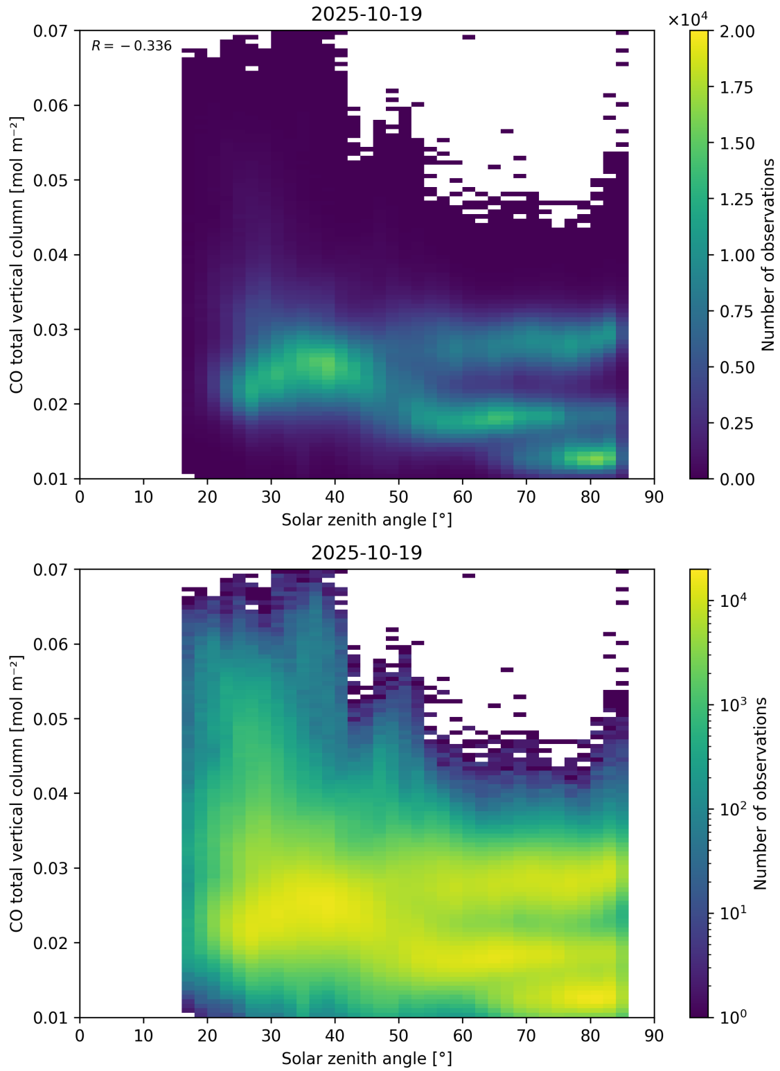
Figure 61: Scatter density plot of “Solar zenith angle” against “CO total vertical column” for 2025-10-18 to 2025-10-20.
