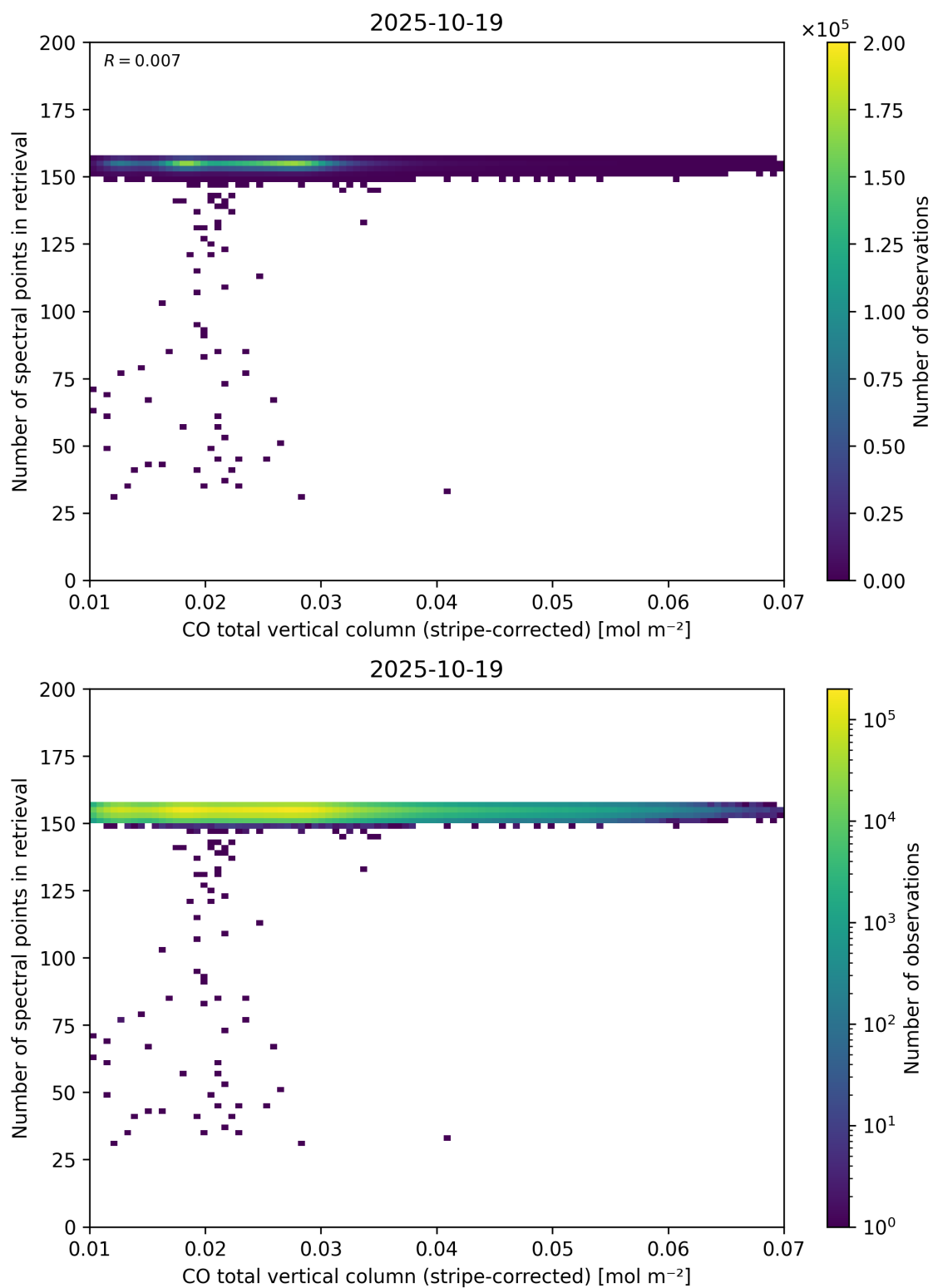
Figure 40: Scatter density plot of “CO total vertical column (stripe-corrected)” against “Number of spectral points in retrieval” for 2025-10-18 to 2025-10-20.
