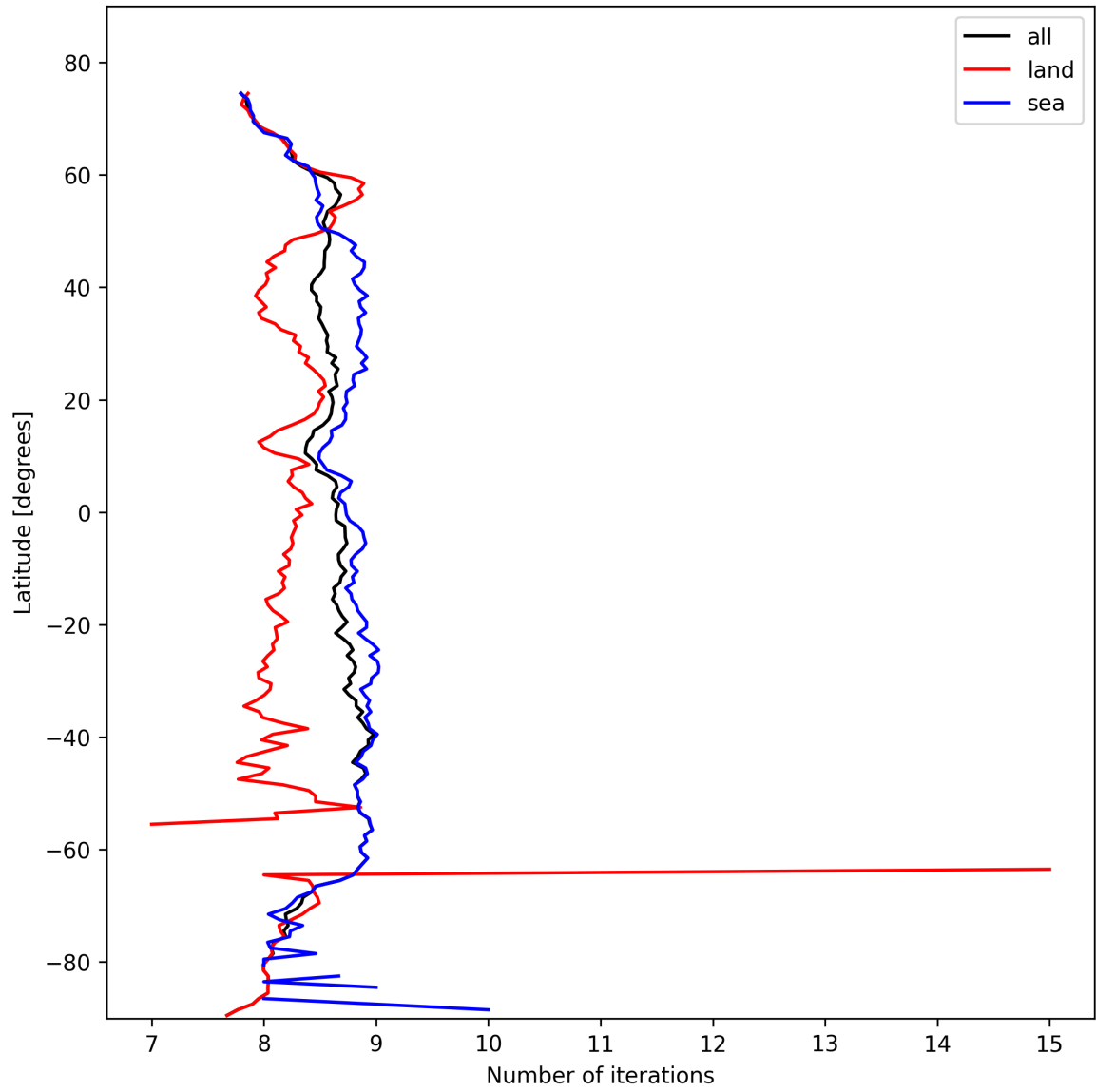
Figure 16: Zonal average of “Number of iterations” for 2025-10-18 to 2025-10-20.
