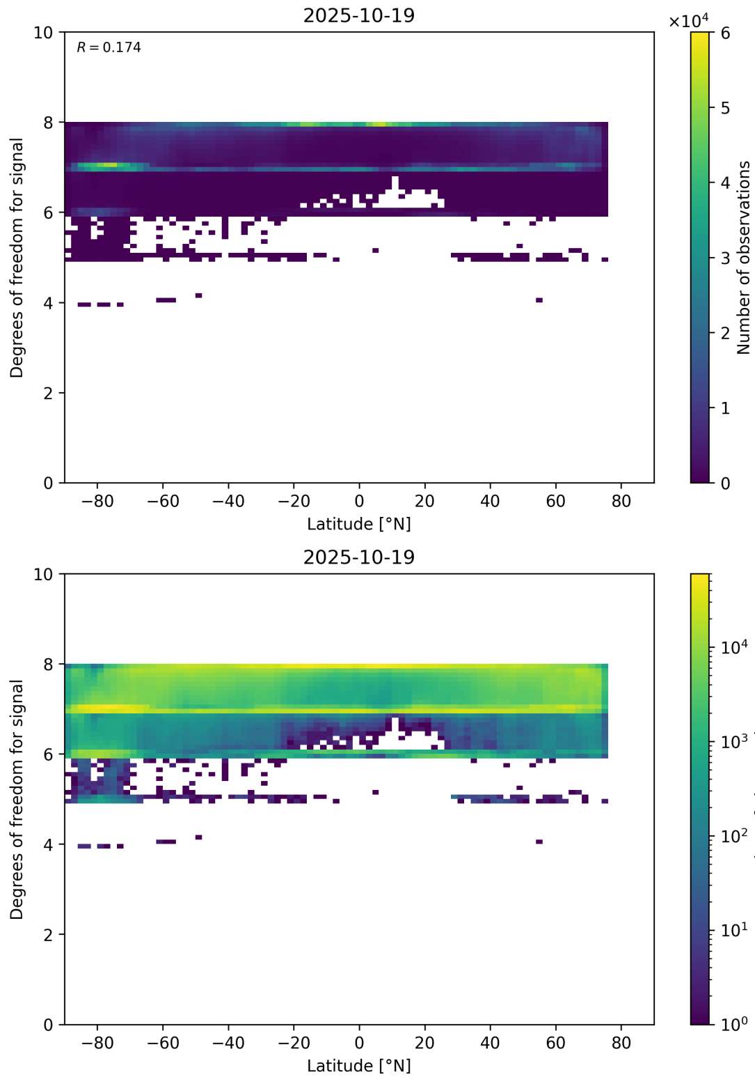
Figure 55: Scatter density plot of “Latitude” against “Degrees of freedom for signal” for 2025-10-18 to 2025-10-20.
