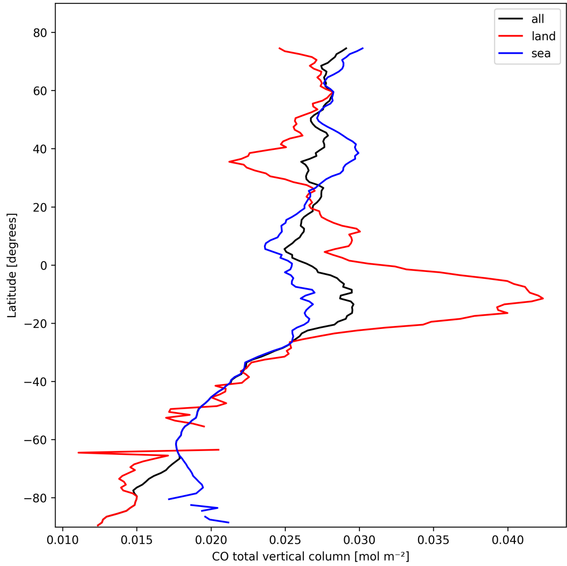
Figure 10: Zonal average of “CO total vertical column” for 2025-10-18 to 2025-10-20.
