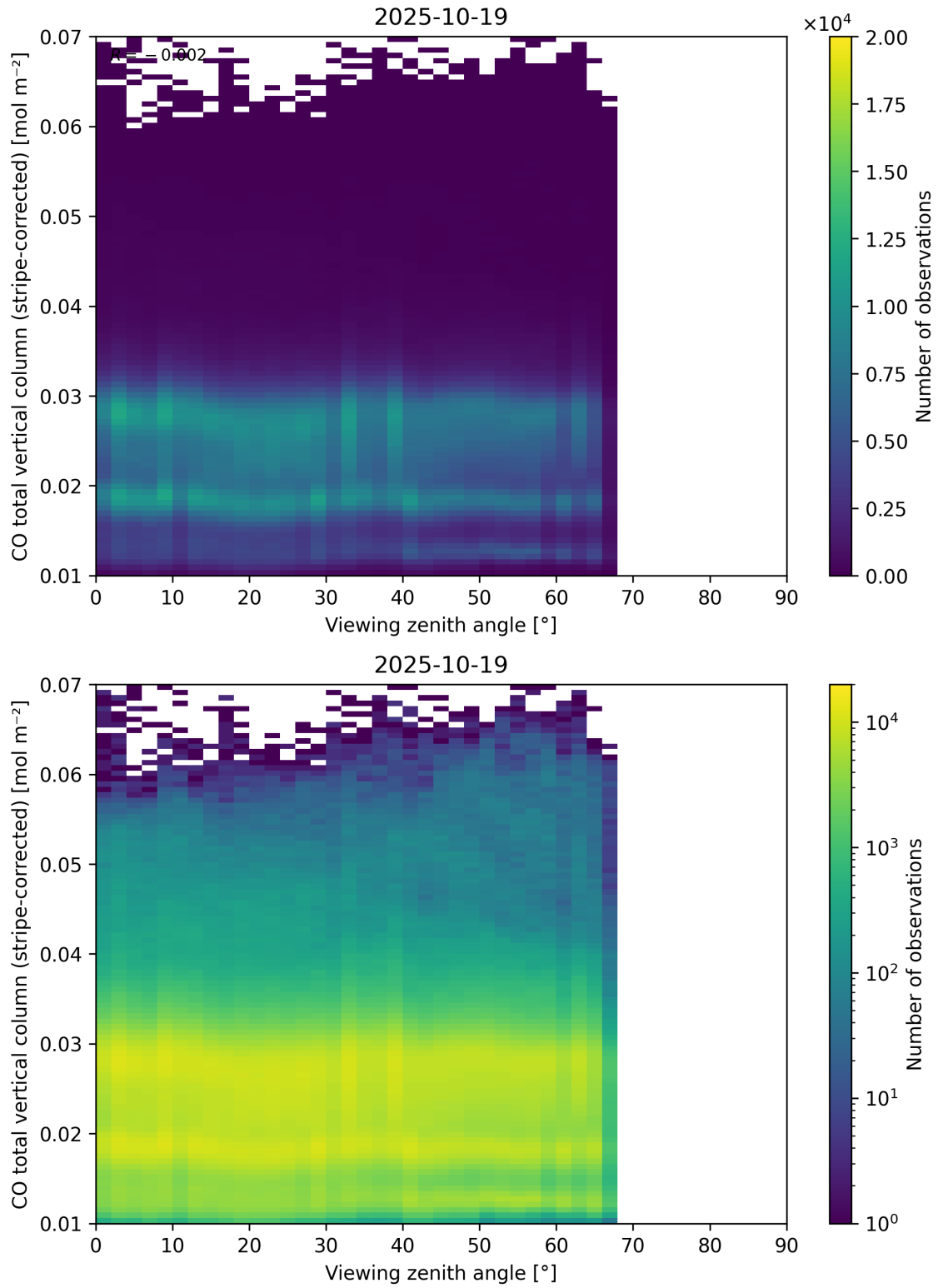
Figure 70: Scatter density plot of “Viewing zenith angle” against “CO total vertical column (stripe-corrected)” for 2025-10-18 to 2025-10-20.
