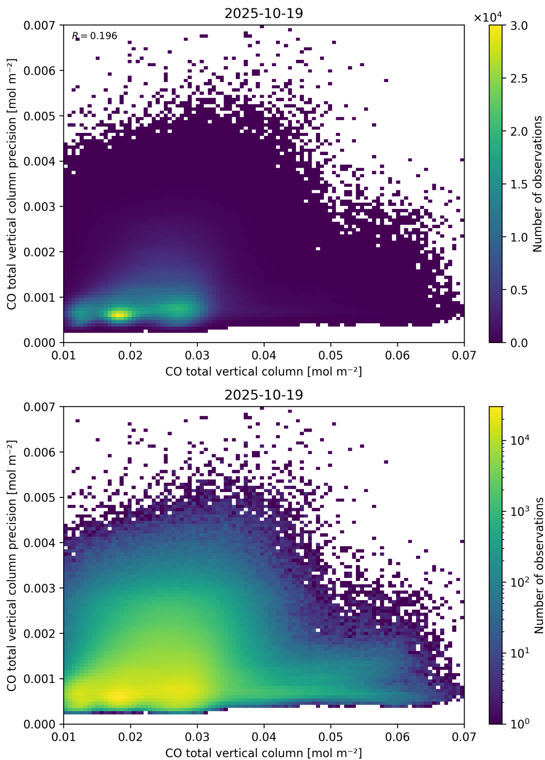
Figure 34: Scatter density plot of “CO total vertical column” against “CO total vertical column precision” for 2025-10-18 to 2025-10-20.
