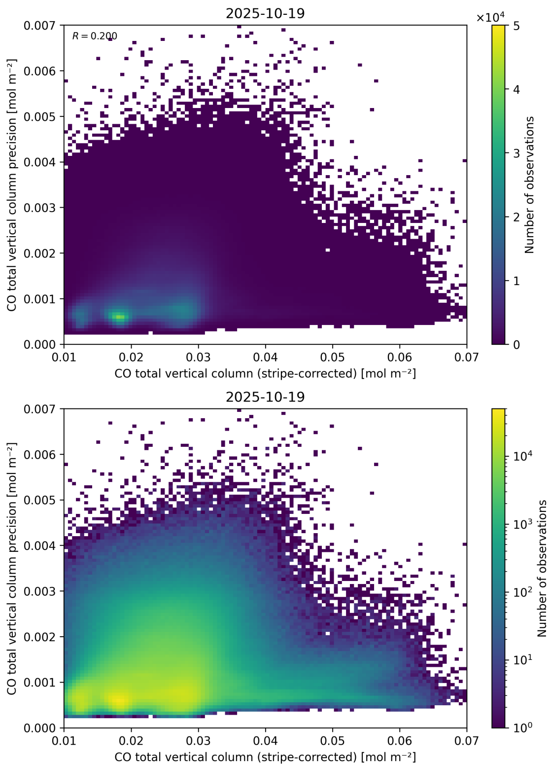
Figure 36: Scatter density plot of “CO total vertical column (stripe-corrected)” against “CO total vertical column precision” for 2025-10-18 to 2025-10-20.
