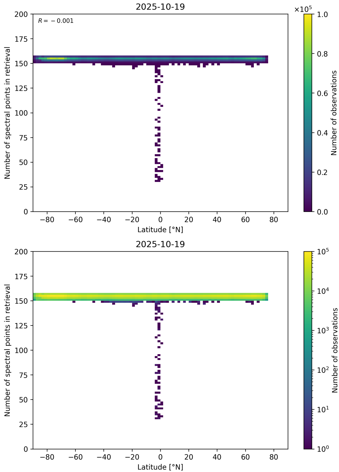
Figure 57: Scatter density plot of “Latitude” against “Number of spectral points in retrieval” for 2025-10-18 to 2025-10-20.
