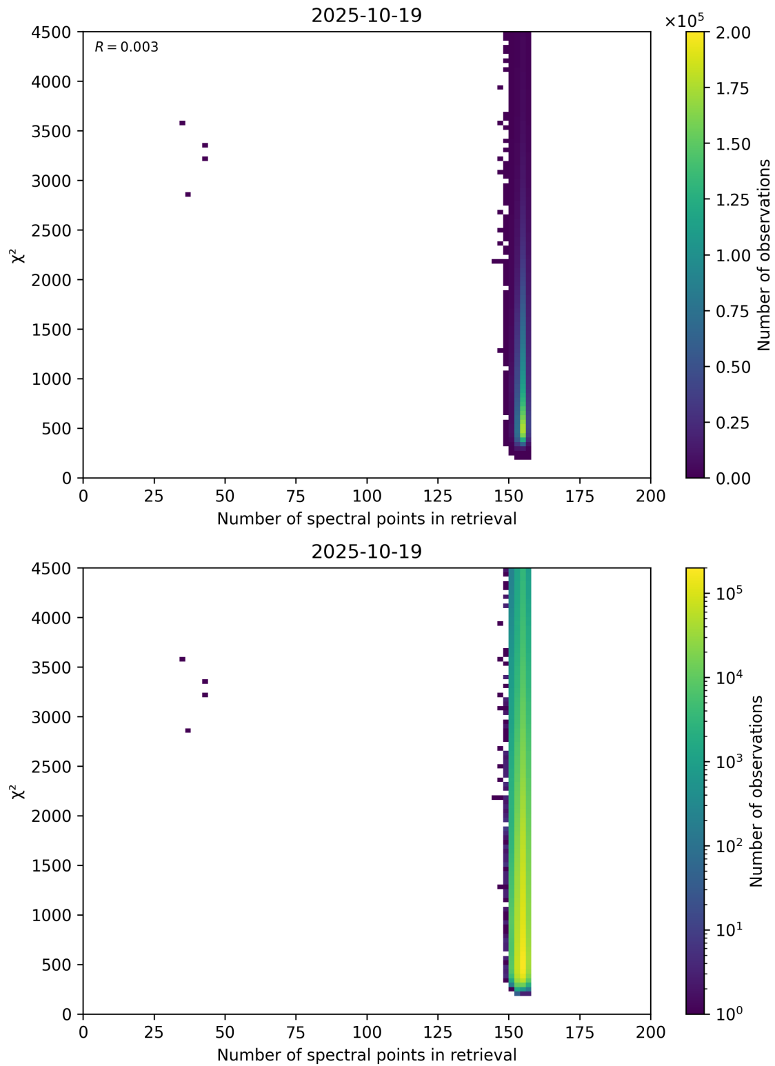
Figure 58: Scatter density plot of “Number of spectral points in retrieval” against “ \chi^2 ” for 2025-10-18 to 2025-10-20.
