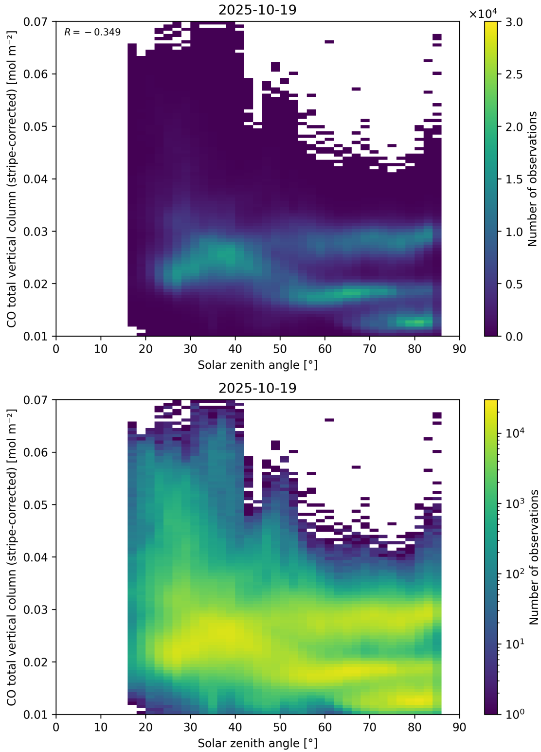
Figure 62: Scatter density plot of “Solar zenith angle” against “CO total vertical column (stripe-corrected)” for 2025-10-18 to 2025-10-20.
