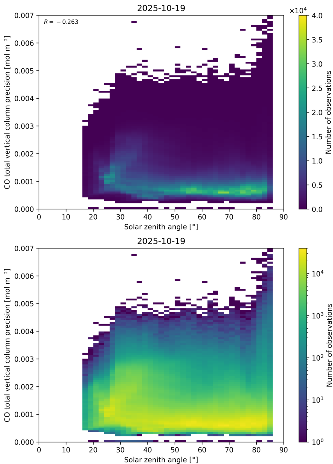
Figure 63: Scatter density plot of “Solar zenith angle” against “CO total vertical column precision” for 2025-10-18 to 2025-10-20.
