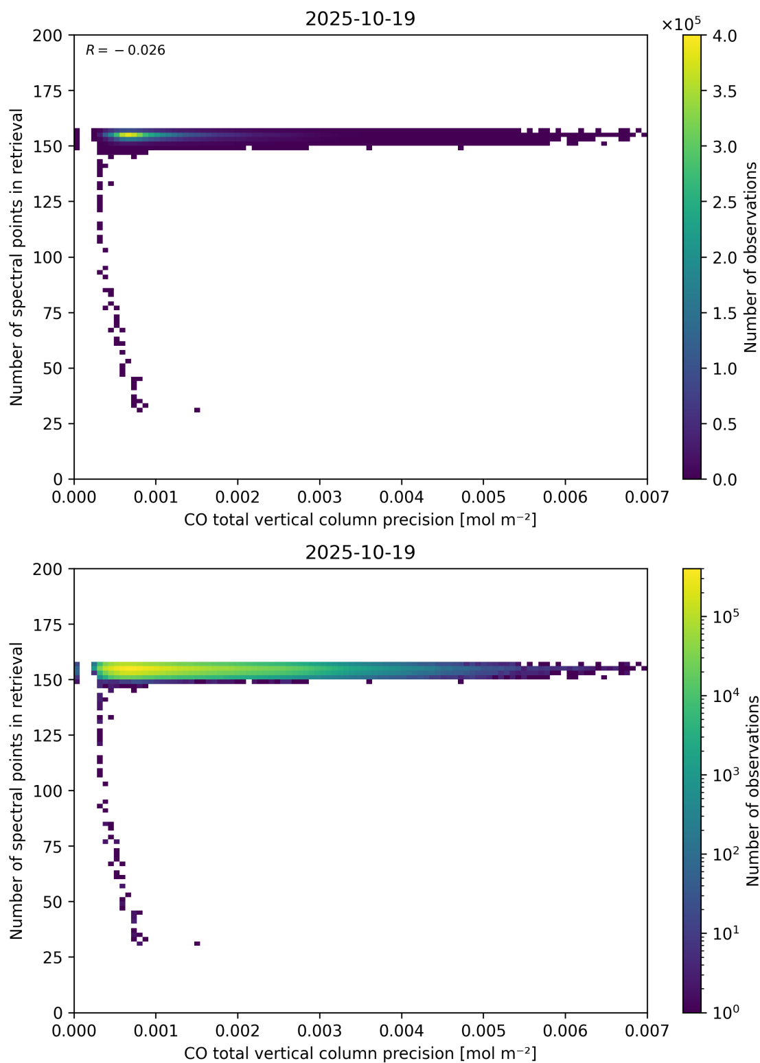
Figure 47: Scatter density plot of “CO total vertical column precision” against “Number of spectral points in retrieval” for 2025-10-18 to 2025-10-20.
