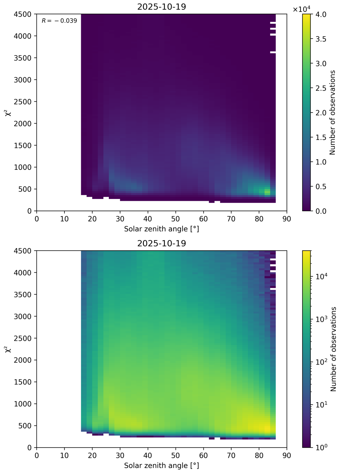
Figure 64: Scatter density plot of “Solar zenith angle” against “ \chi^2 ” for 2025-10-18 to 2025-10-20.
