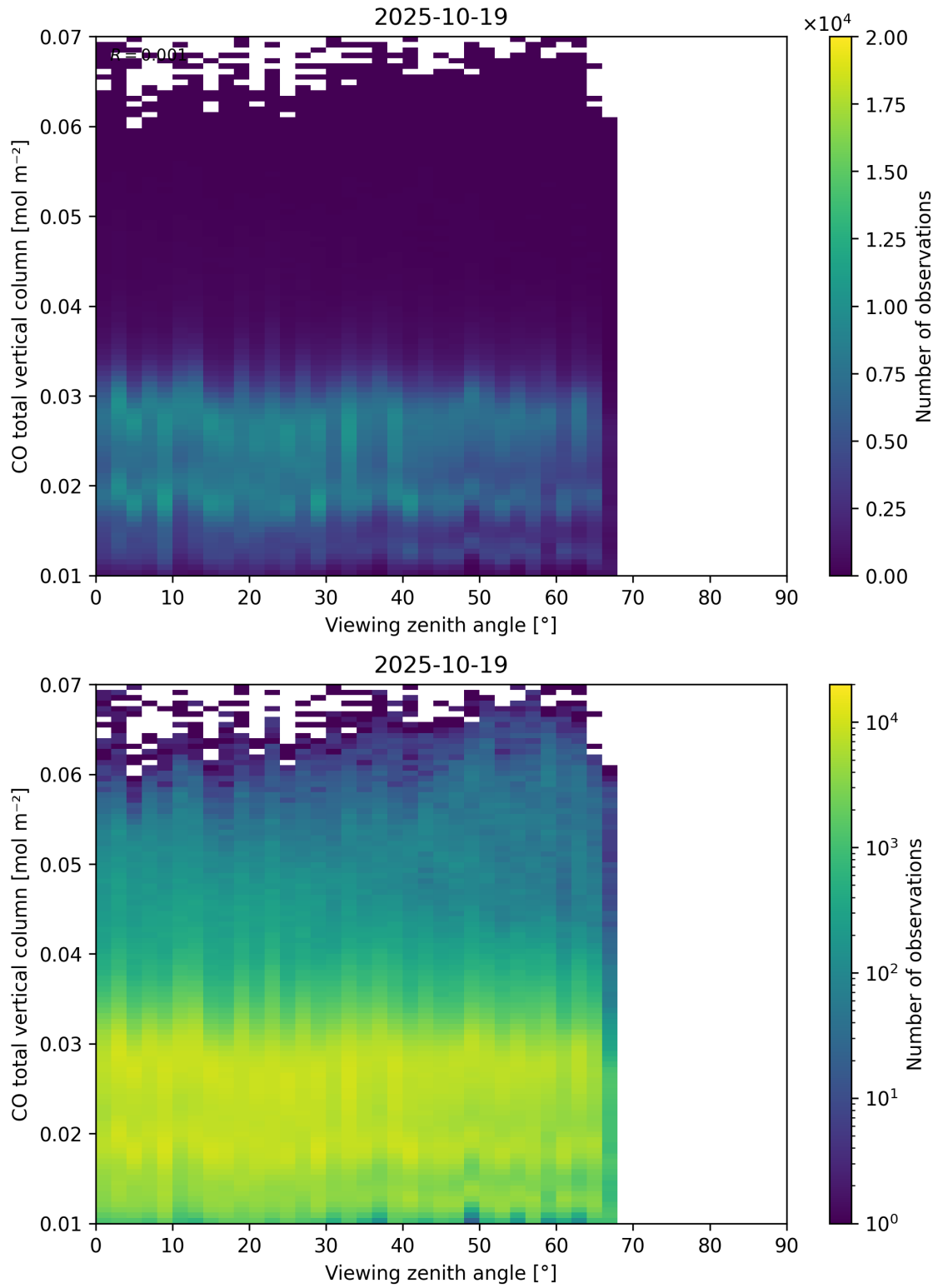
Figure 69: Scatter density plot of “Viewing zenith angle” against “CO total vertical column” for 2025-10-18 to 2025-10-20.
