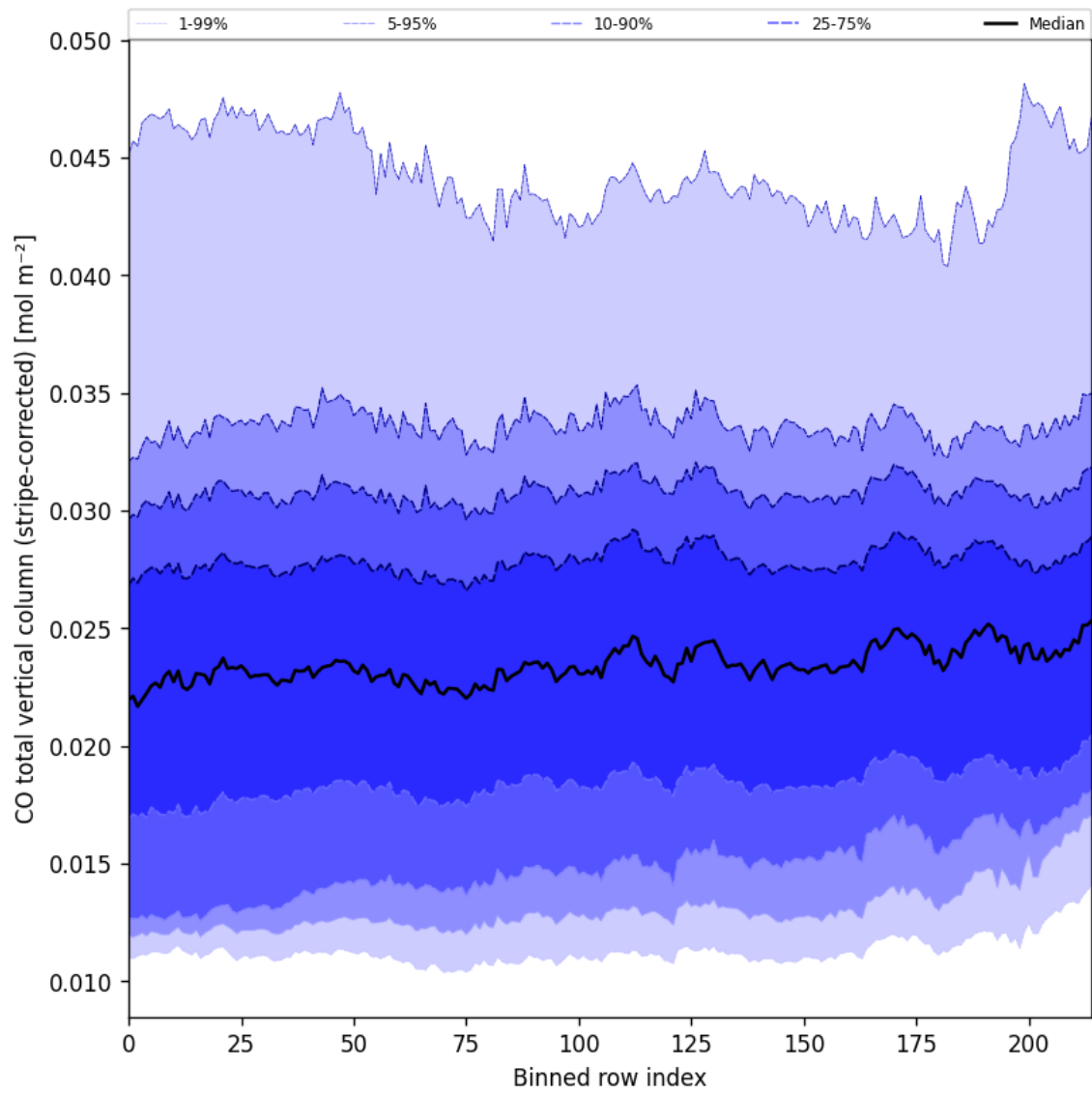
Figure 27: Along track statistics of “CO total vertical column (stripe-corrected)” for 2025-10-19 to 2025-10-21
