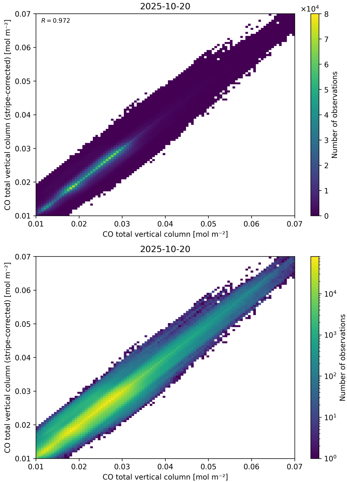
Figure 33: Scatter density plot of “CO total vertical column” against “CO total vertical column (stripe-corrected)” for 2025-10-19 to 2025-10-21.
