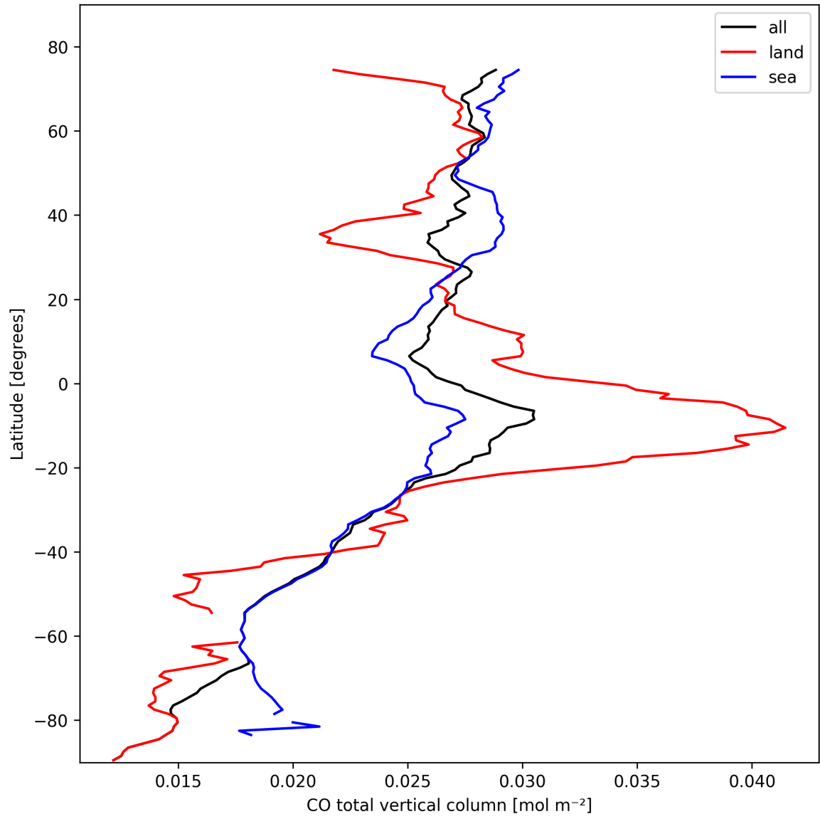
Figure 10: Zonal average of “CO total vertical column” for 2025-10-19 to 2025-10-21.
