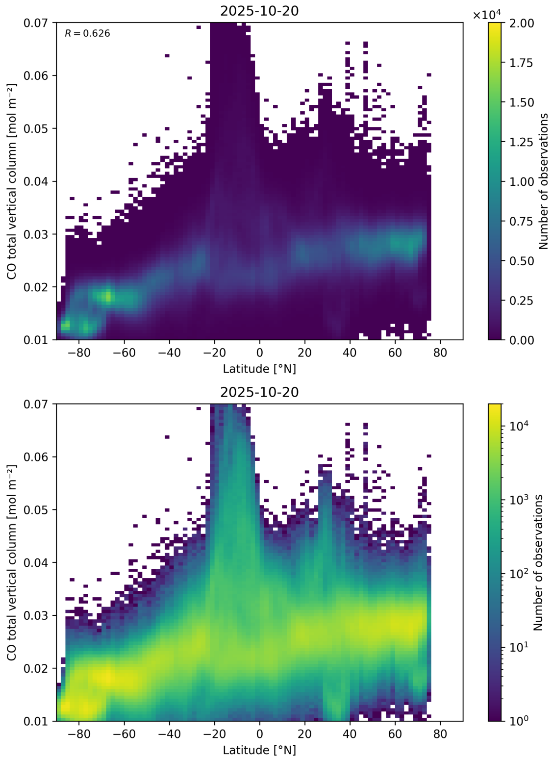
Figure 51: Scatter density plot of “Latitude” against “CO total vertical column” for 2025-10-19 to 2025-10-21.
