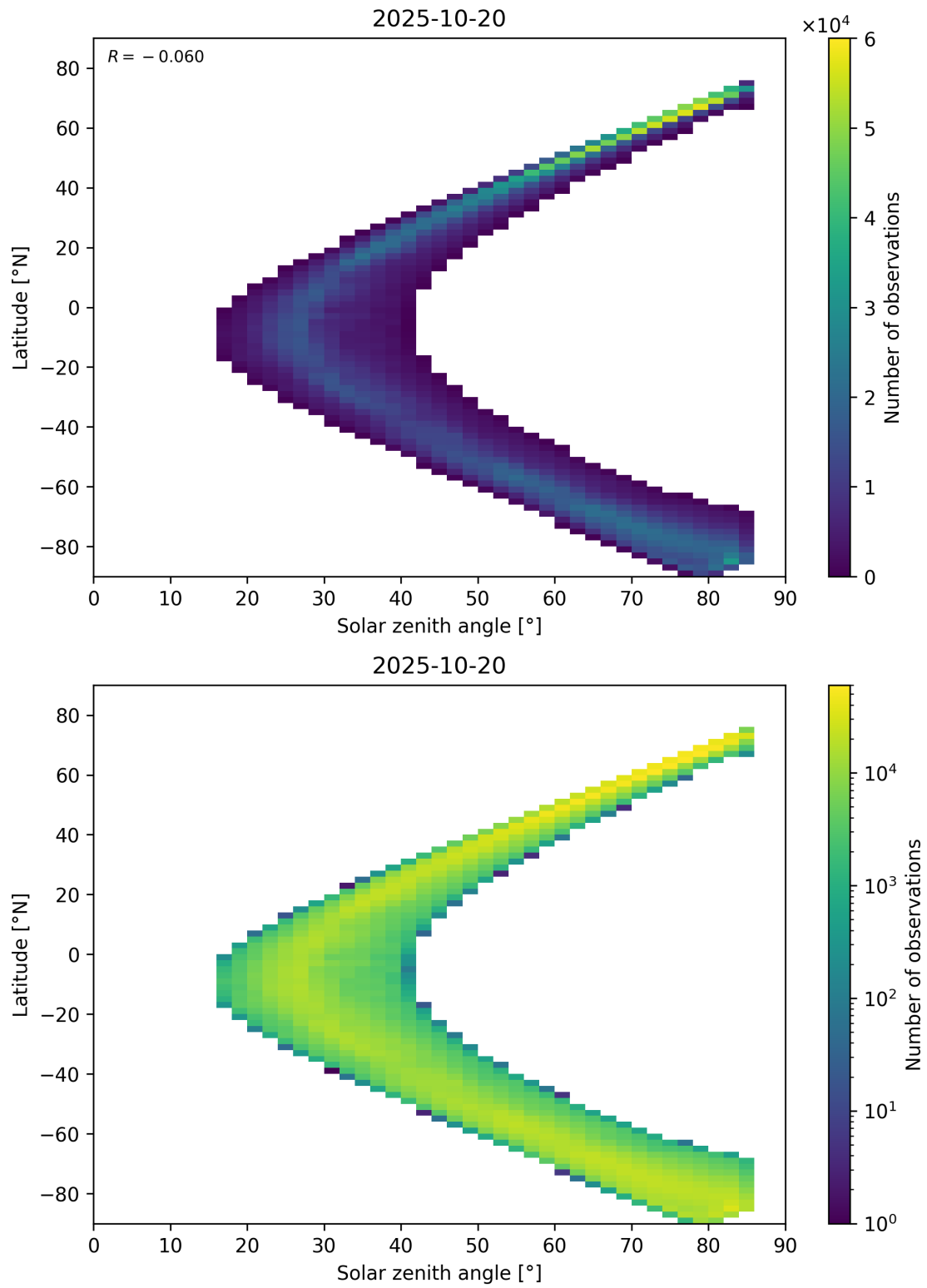
Figure 66: Scatter density plot of “Solar zenith angle” against “Latitude” for 2025-10-19 to 2025-10-21.
