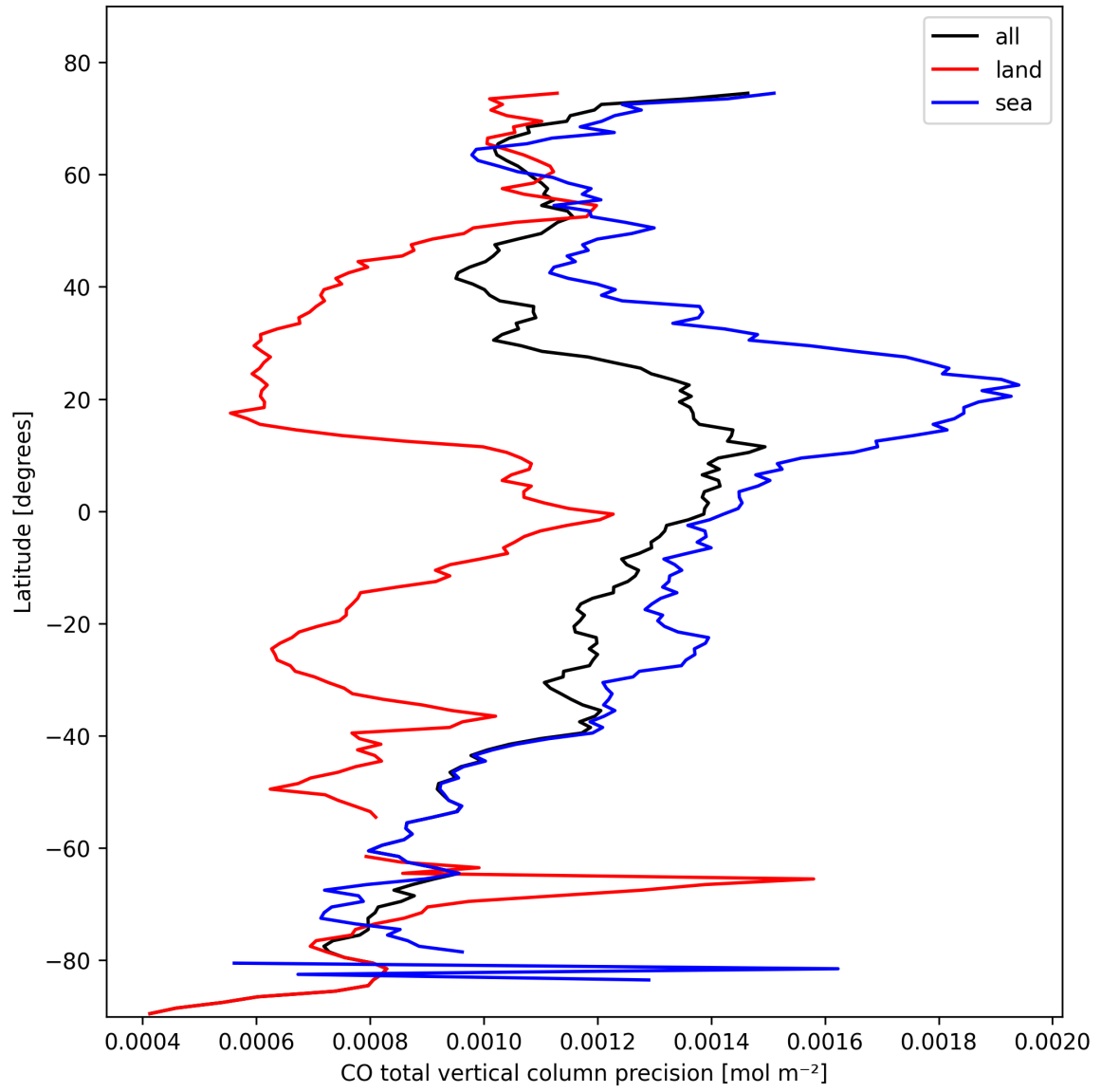
Figure 12: Zonal average of “CO total vertical column precision” for 2025-10-19 to 2025-10-21.
