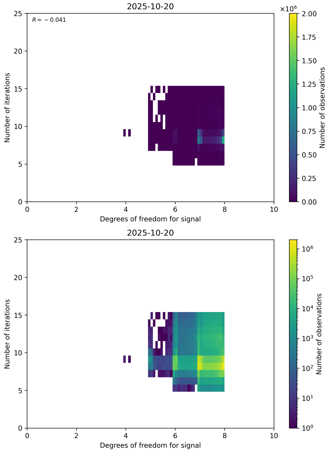
Figure 50: Scatter density plot of “Degrees of freedom for signal” against “Number of iterations” for 2025-10-19 to 2025-10-21.
