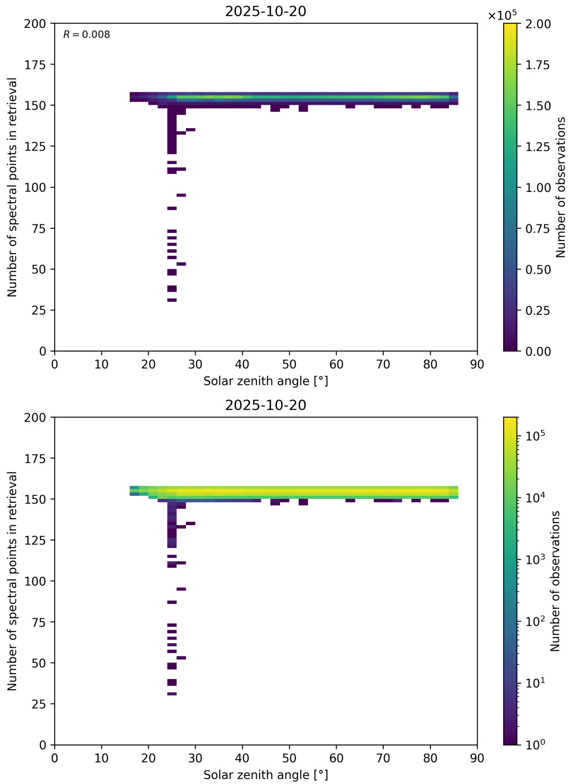
Figure 68: Scatter density plot of “Solar zenith angle” against “Number of spectral points in retrieval” for 2025-10-19 to 2025-10-21.
