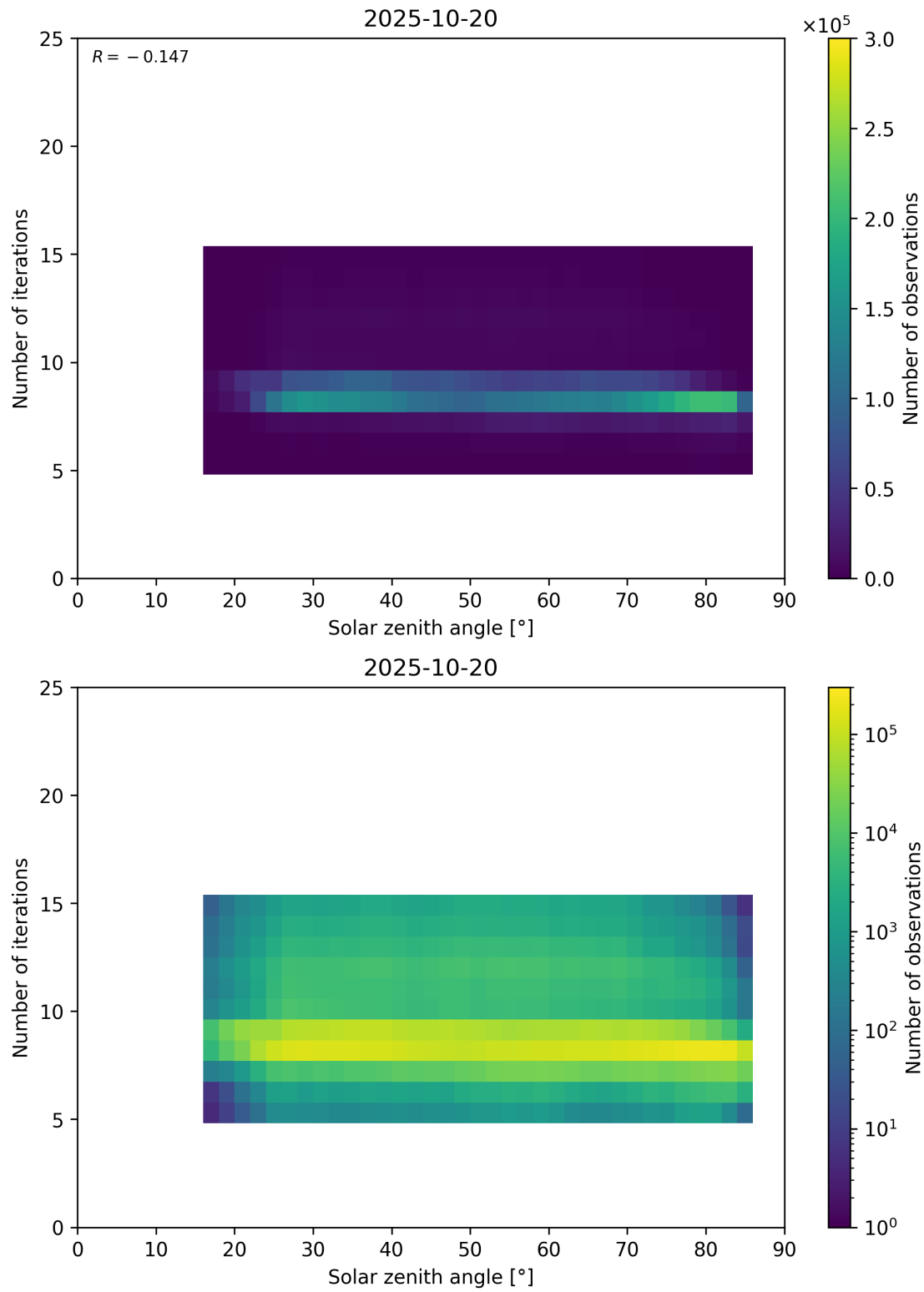
Figure 67: Scatter density plot of “Solar zenith angle” against “Number of iterations” for 2025-10-19 to 2025-10-21.
