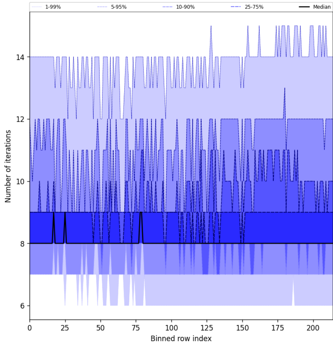
Figure 32: Along track statistics of “Number of iterations” for 2025-10-19 to 2025-10-21
