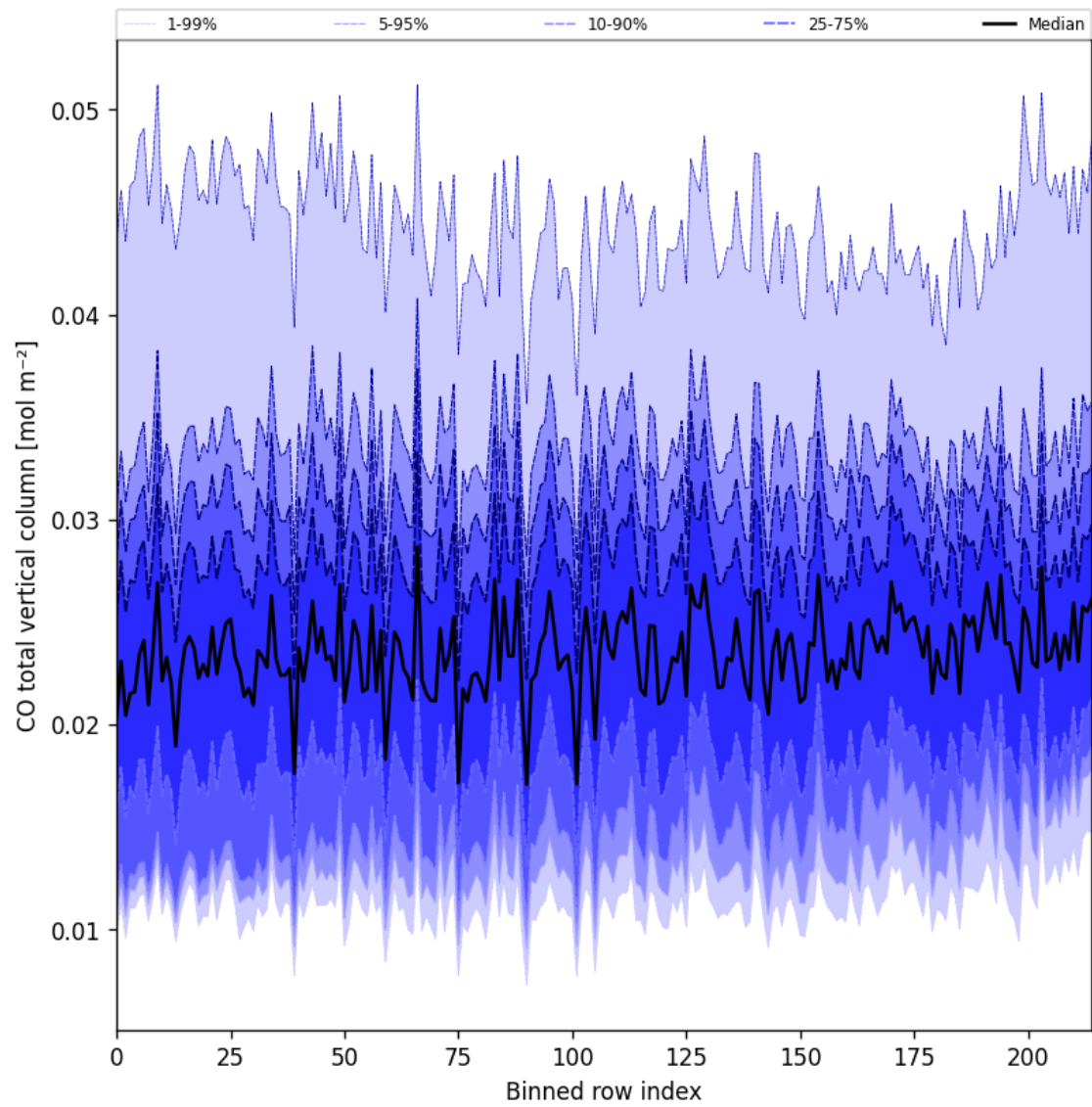
Figure 26: Along track statistics of “CO total vertical column” for 2025-10-19 to 2025-10-21
