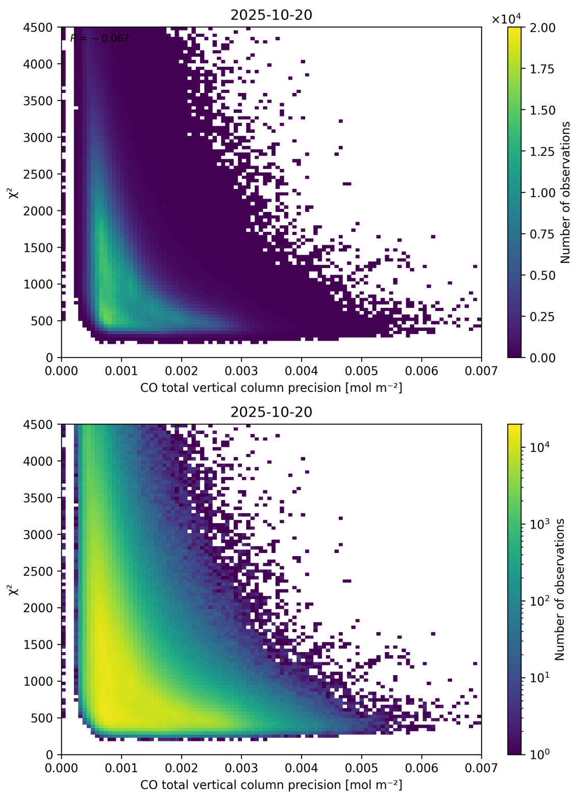
Figure 44: Scatter density plot of “CO total vertical column precision” against “ \chi^2 ” for 2025-10-19 to 2025-10-21.
