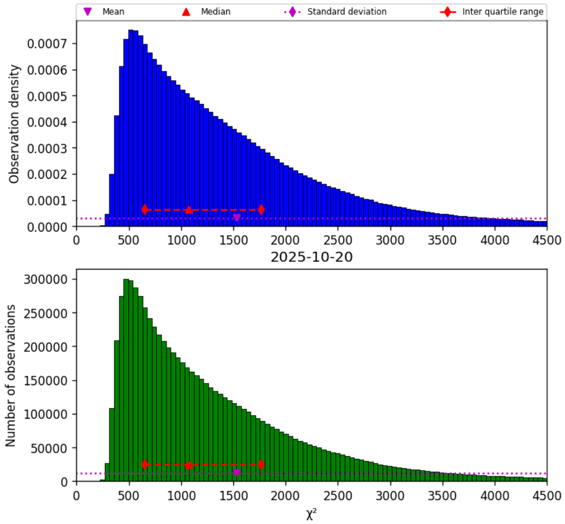
Figure 22: Histogram of “ \chi^2 ” for 2025-10-19 to 2025-10-21
