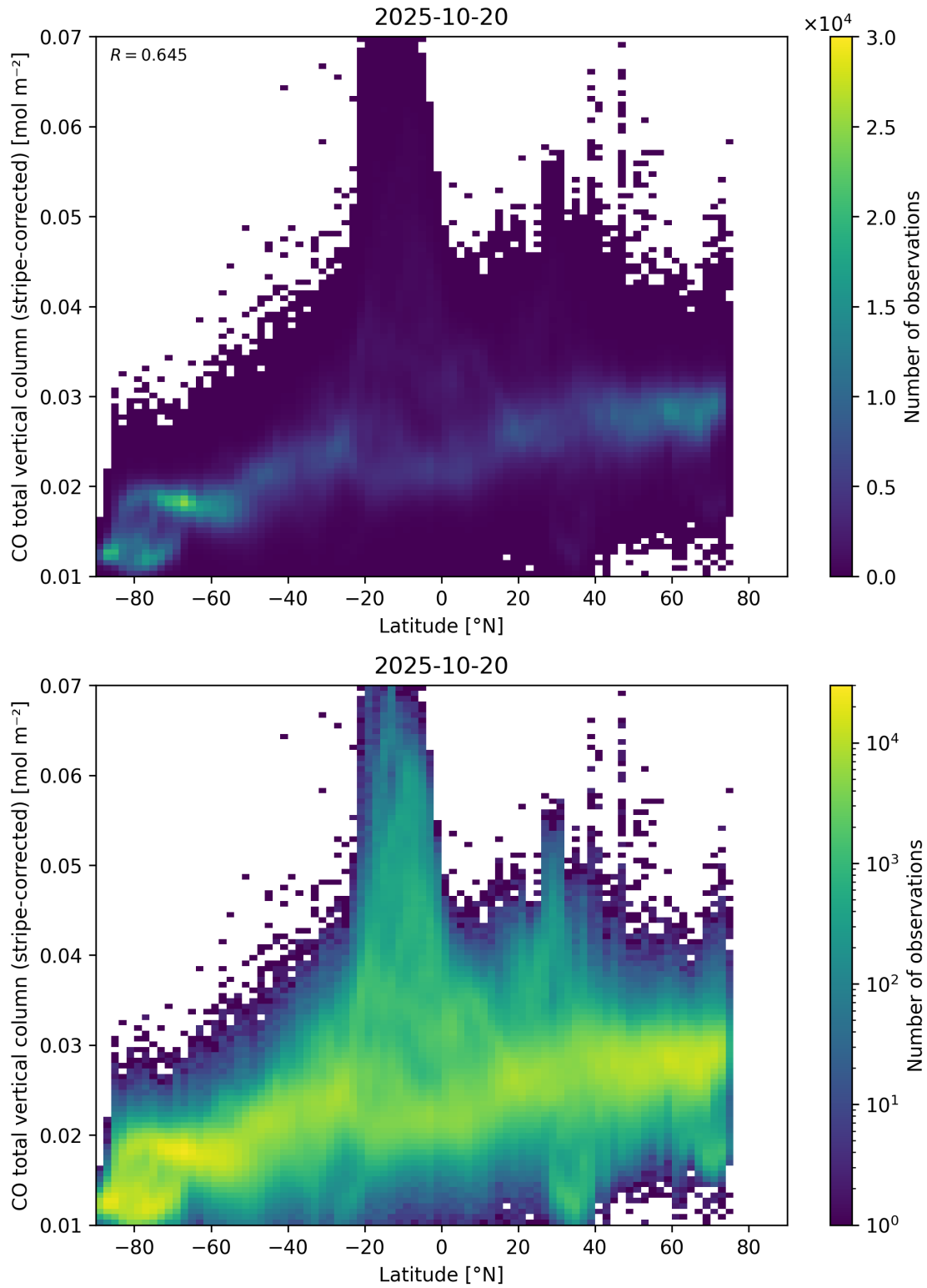
Figure 52: Scatter density plot of “Latitude” against “CO total vertical column (stripe-corrected)” for 2025-10-19 to 2025-10-21.
