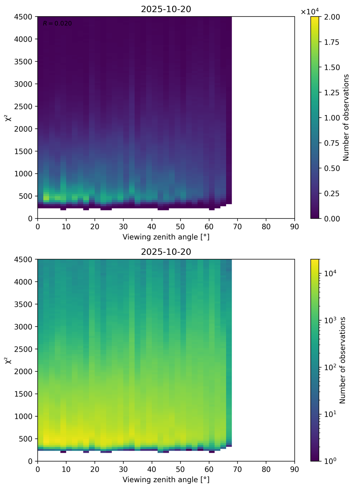
Figure 72: Scatter density plot of “Viewing zenith angle” against “ \chi^2 ” for 2025-10-19 to 2025-10-21.
