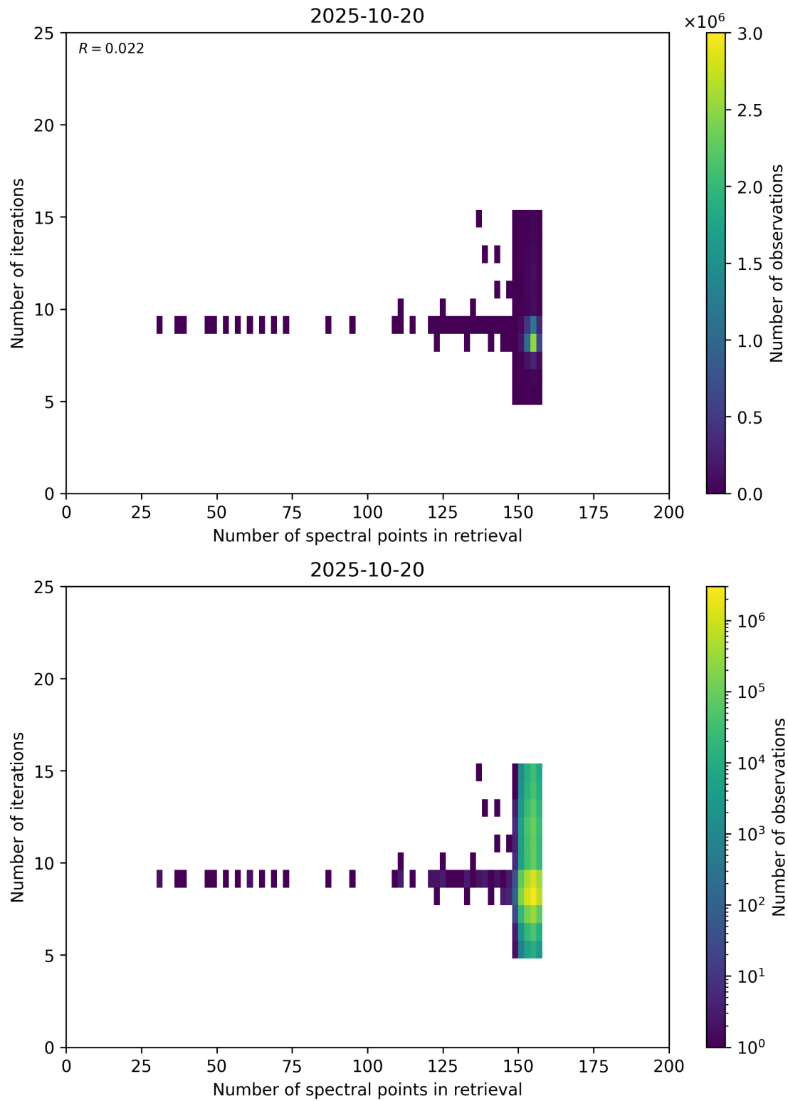
Figure 60: Scatter density plot of “Number of spectral points in retrieval” against “Number of iterations” for 2025-10-19 to 2025-10-21.
