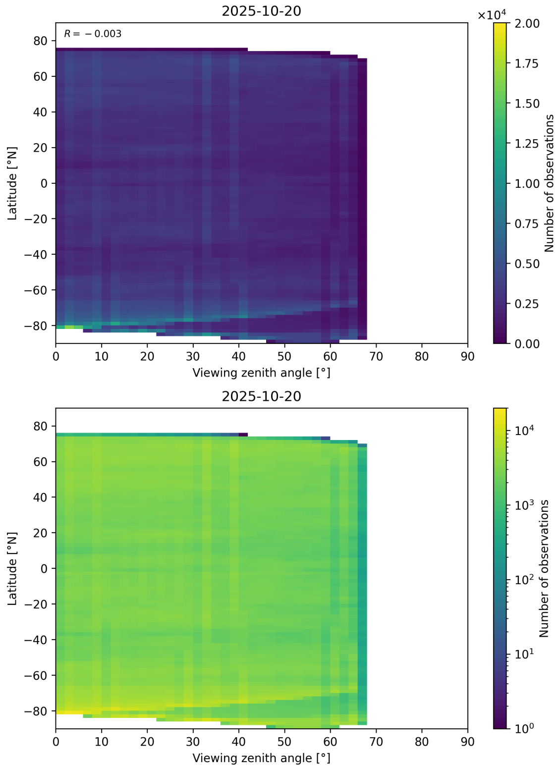
Figure 74: Scatter density plot of “Viewing zenith angle” against “Latitude” for 2025-10-19 to 2025-10-21.
