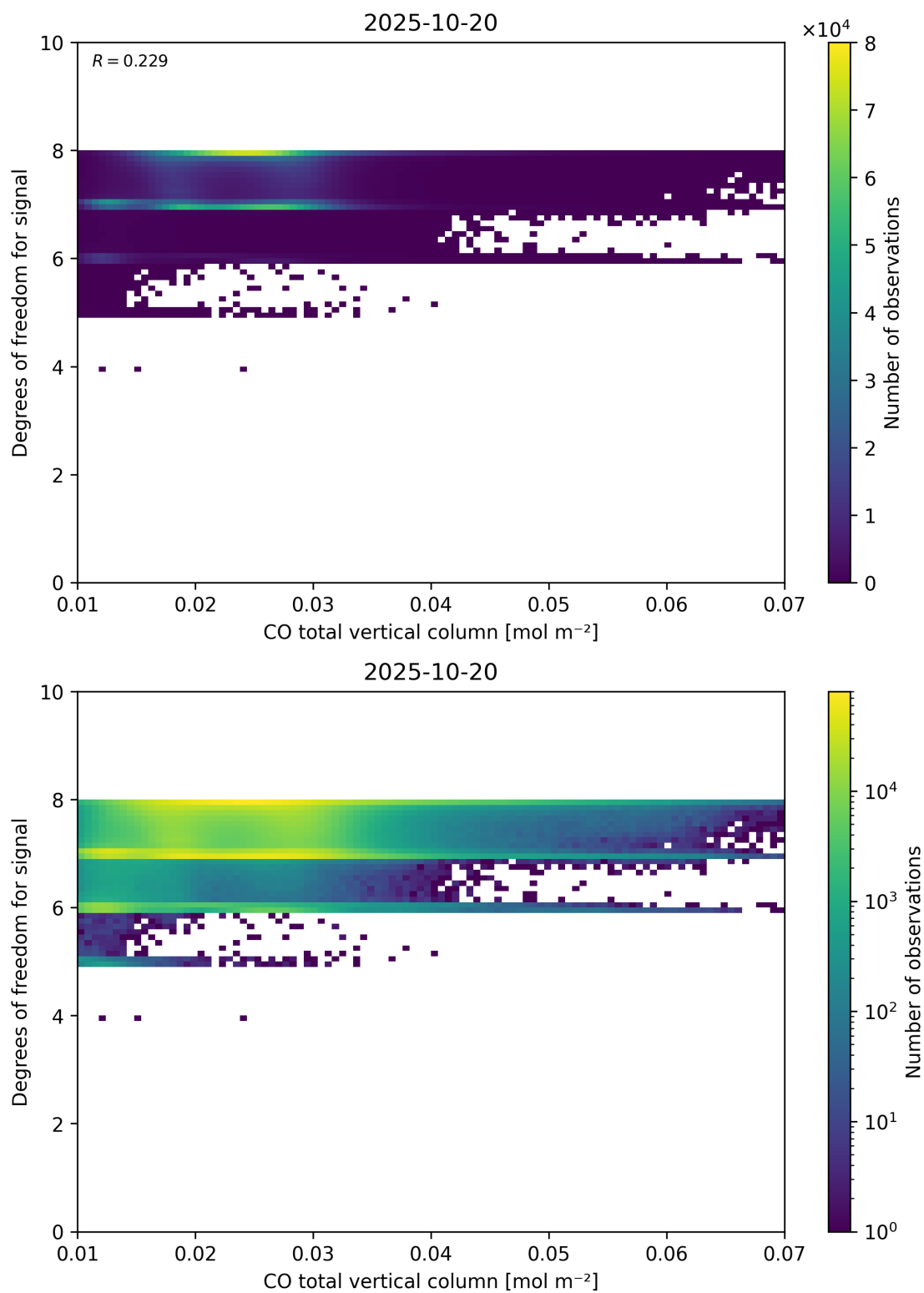
Figure 41: Scatter density plot of “CO total vertical column” against “Degrees of freedom for signal” for 2025-10-19 to 2025-10-21.
