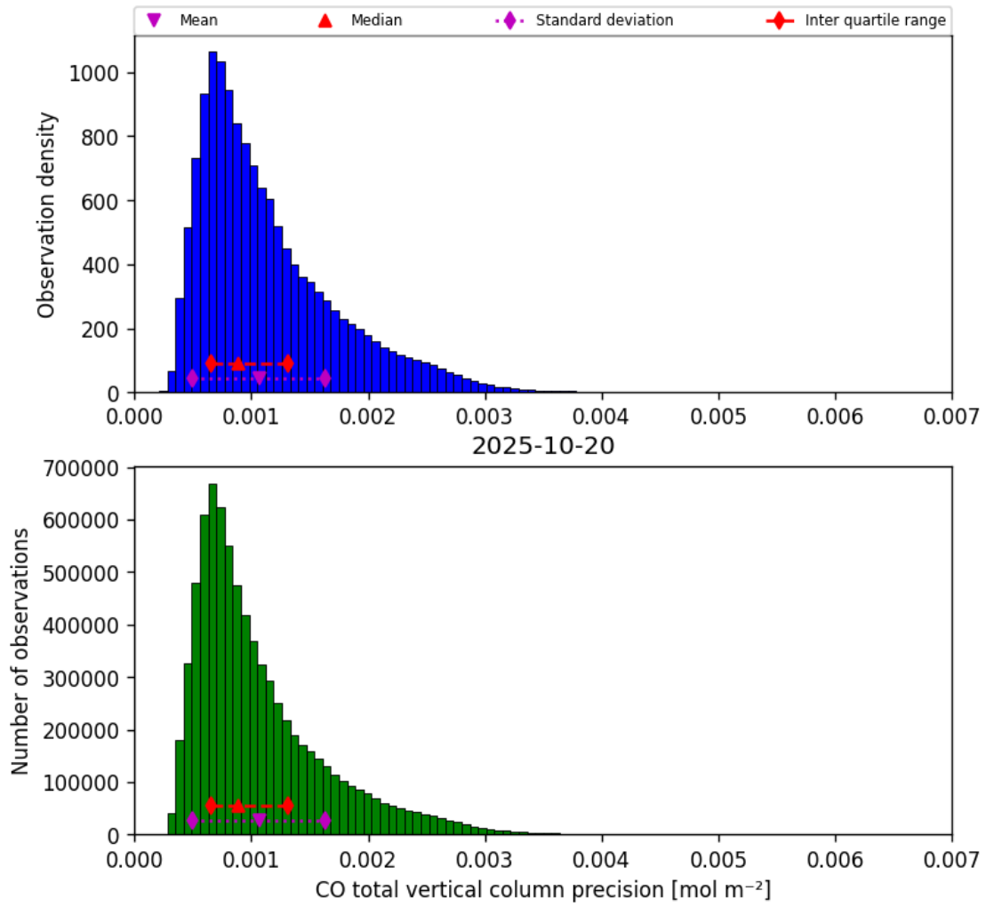
Figure 20: Histogram of “CO total vertical column precision” for 2025-10-19 to 2025-10-21
