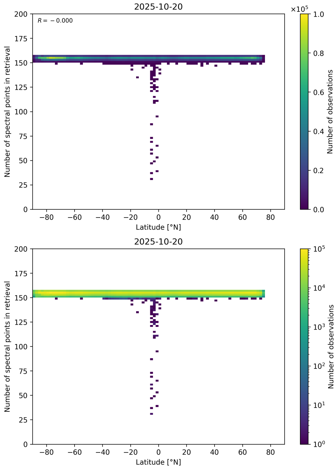
Figure 57: Scatter density plot of “Latitude” against “Number of spectral points in retrieval” for 2025-10-19 to 2025-10-21.
