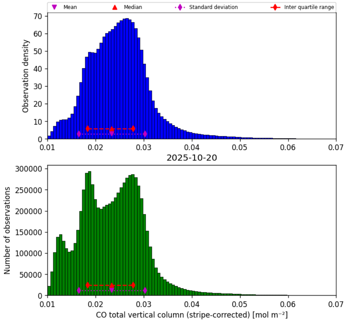
Figure 19: Histogram of “CO total vertical column (stripe-corrected)” for 2025-10-19 to 2025-10-21
