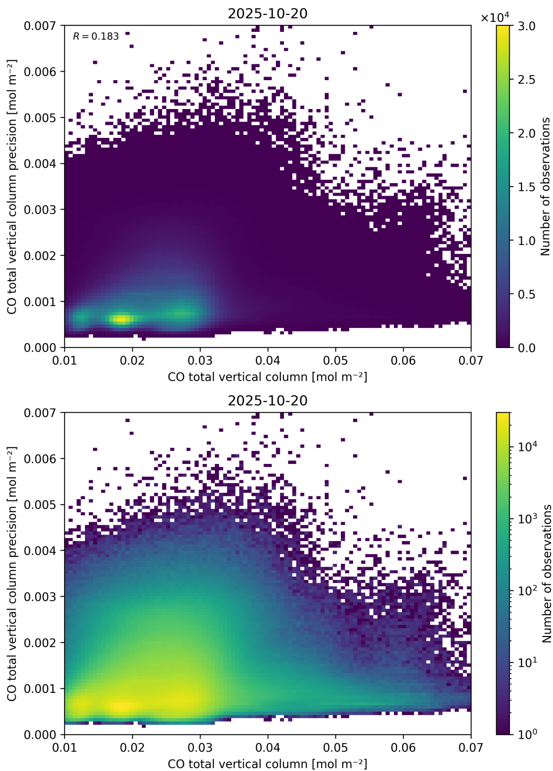
Figure 34: Scatter density plot of “CO total vertical column” against “CO total vertical column precision” for 2025-10-19 to 2025-10-21.
