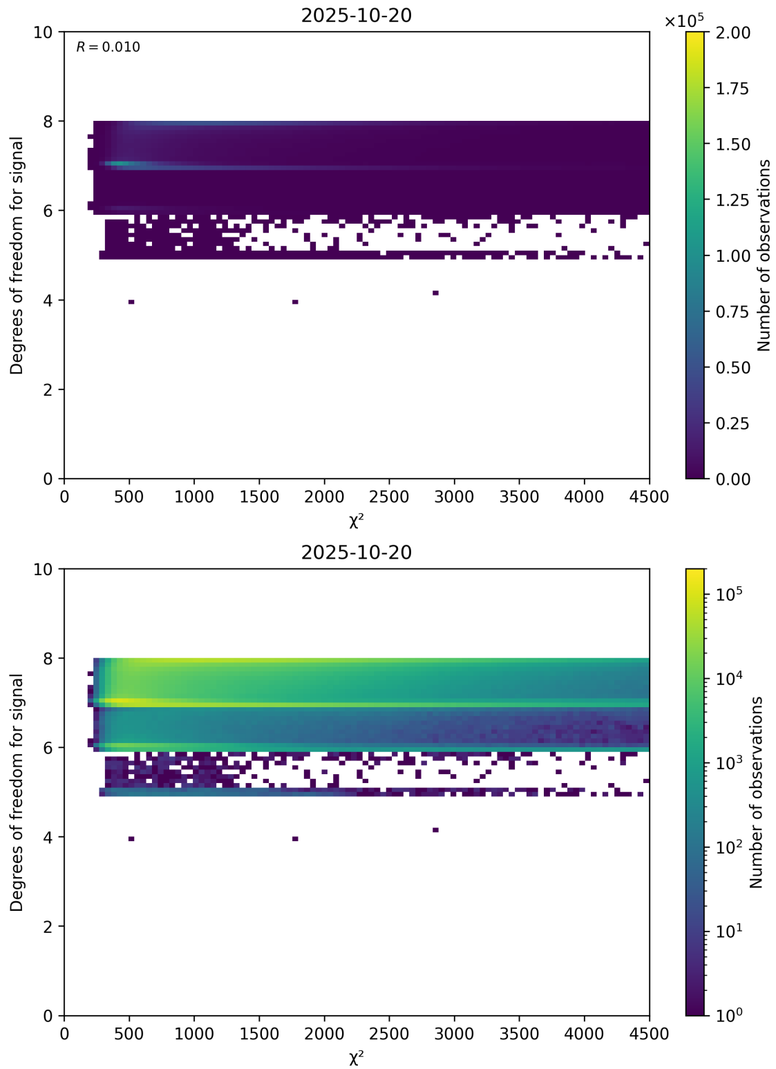
Figure 48: Scatter density plot of “ \chi^2 ” against “Degrees of freedom for signal” for 2025-10-19 to 2025-10-21.
