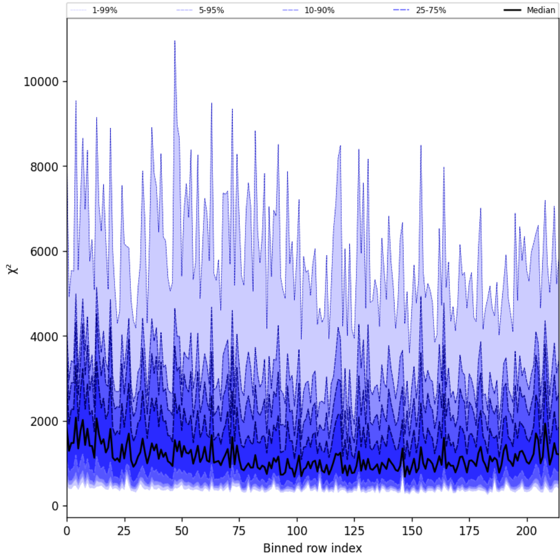
Figure 30: Along track statistics of “ \chi^2 ” for 2025-10-19 to 2025-10-21
