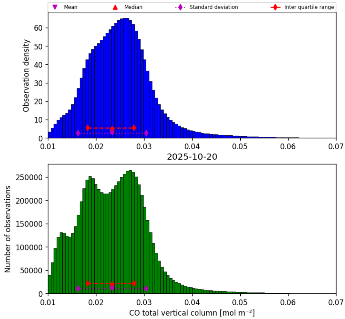
Figure 18: Histogram of “CO total vertical column” for 2025-10-19 to 2025-10-21
