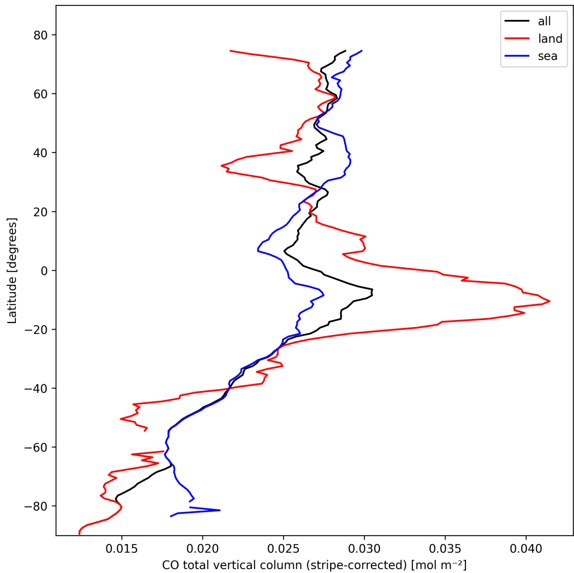
Figure 11: Zonal average of “CO total vertical column (stripe-corrected)” for 2025-10-19 to 2025-10-21.
