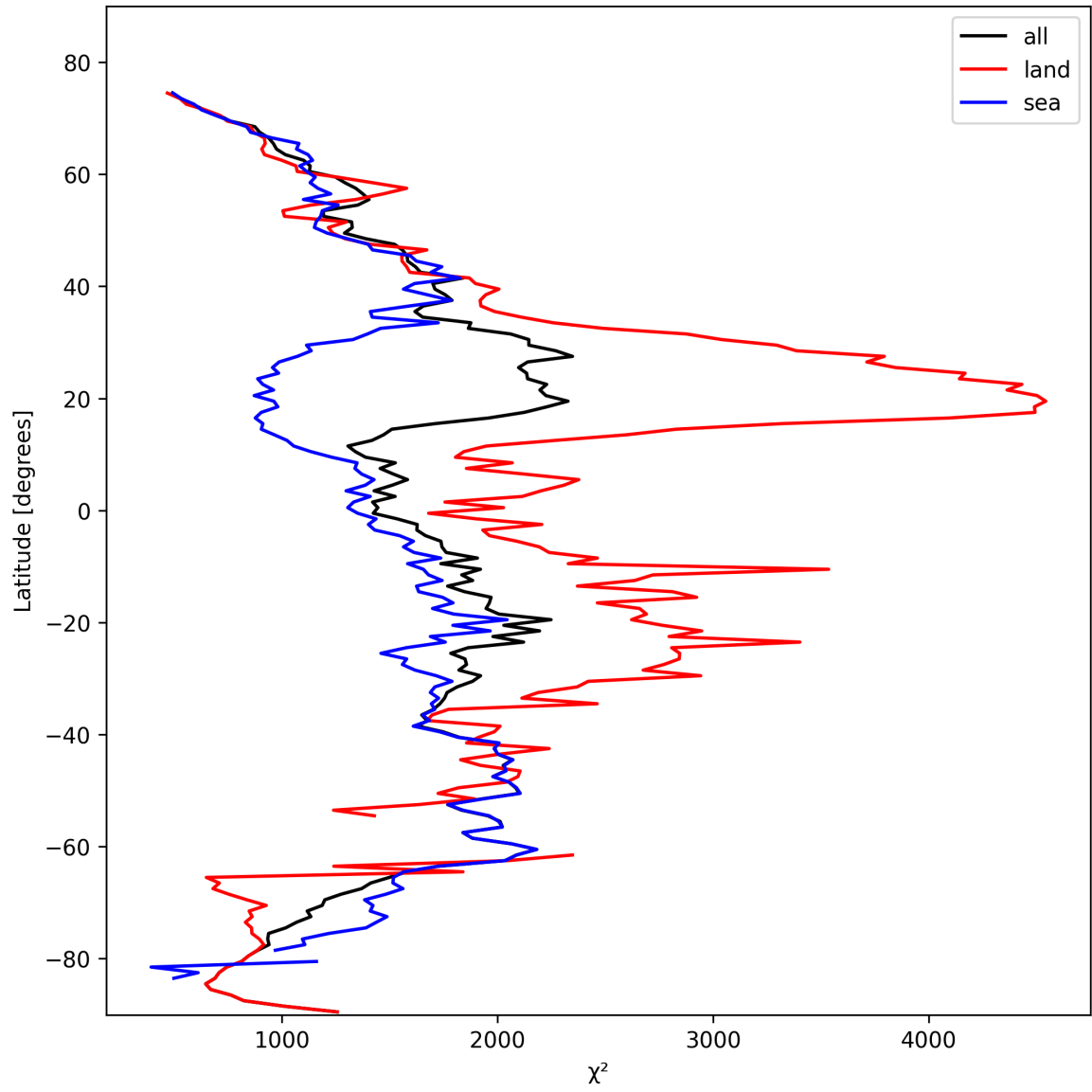
Figure 14: Zonal average of “ \chi^2 ” for 2025-10-19 to 2025-10-21.
