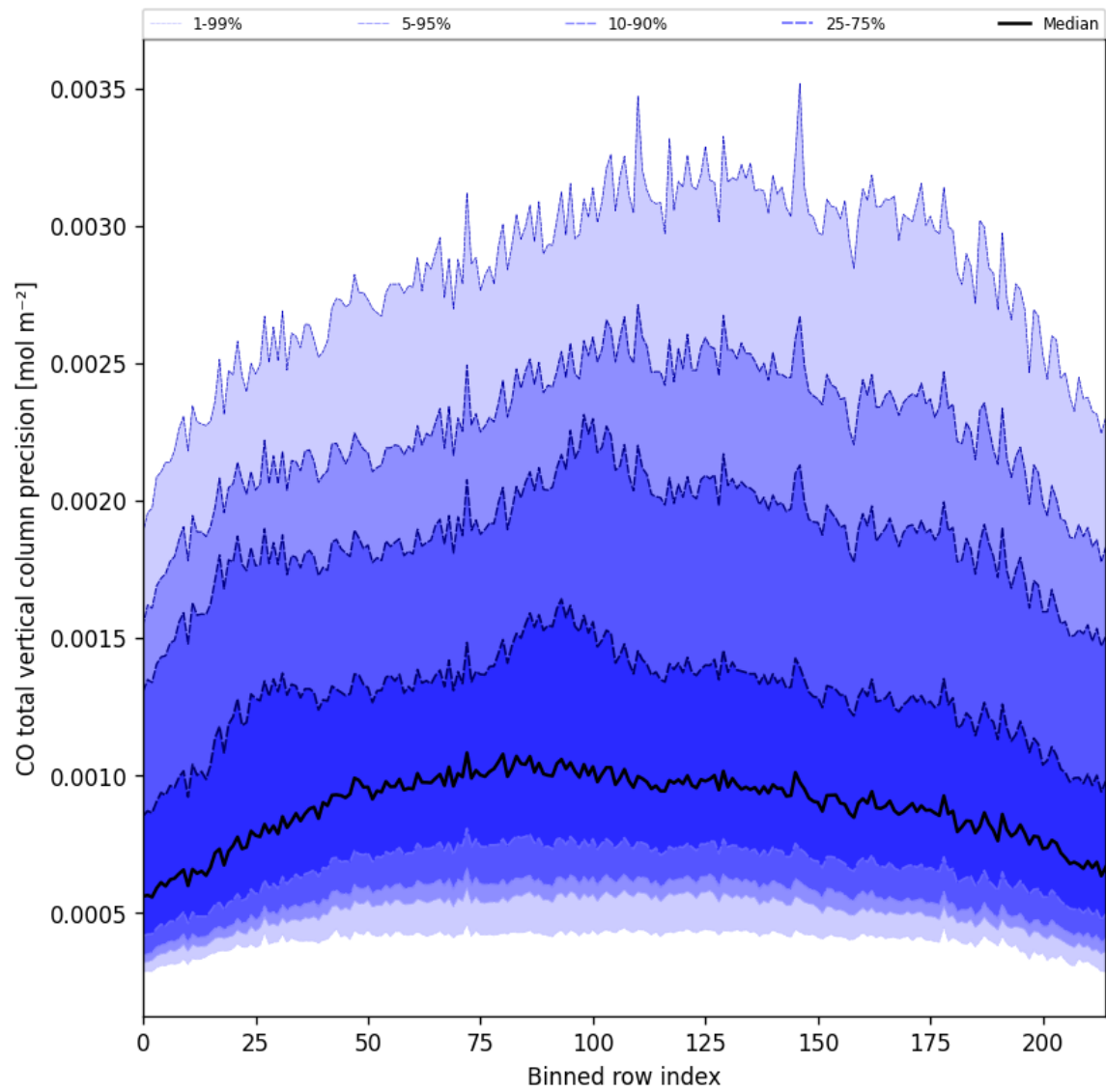
Figure 28: Along track statistics of “CO total vertical column precision” for 2025-10-19 to 2025-10-21
