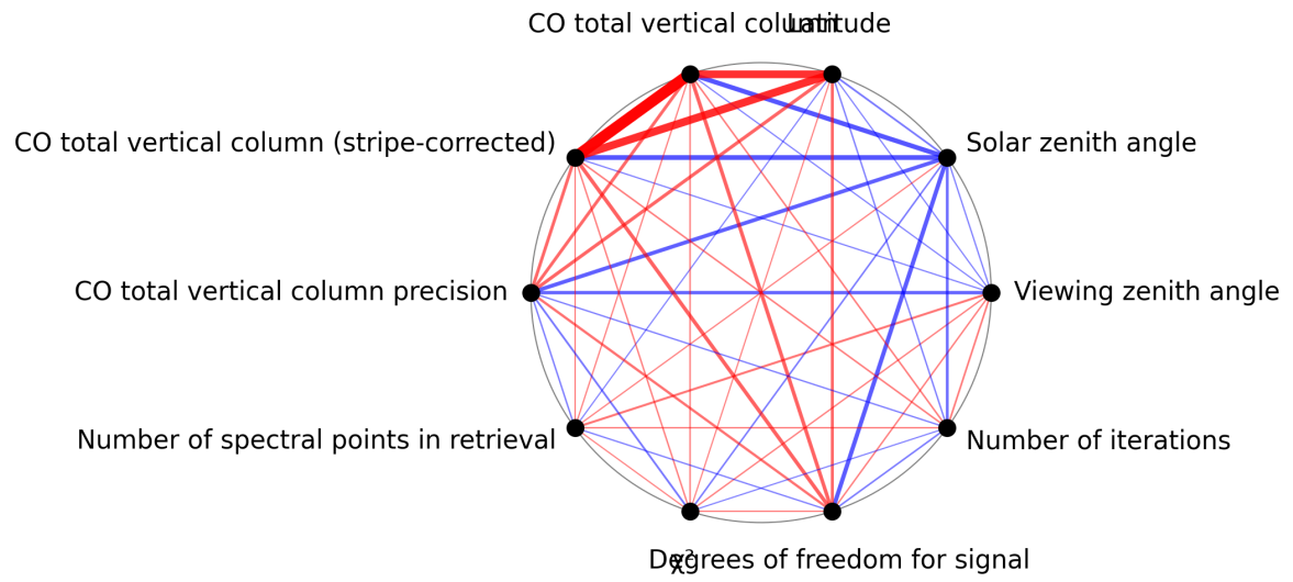
Figure 1: Map of correlation graph for 2025-10-19 to 2025-10-21.
