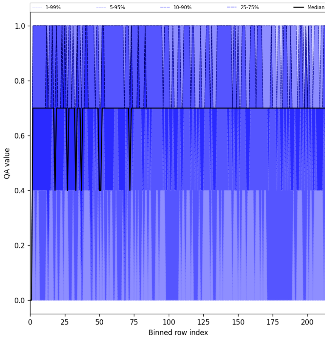
Figure 25: Along track statistics of “QA value” for 2025-10-19 to 2025-10-21
