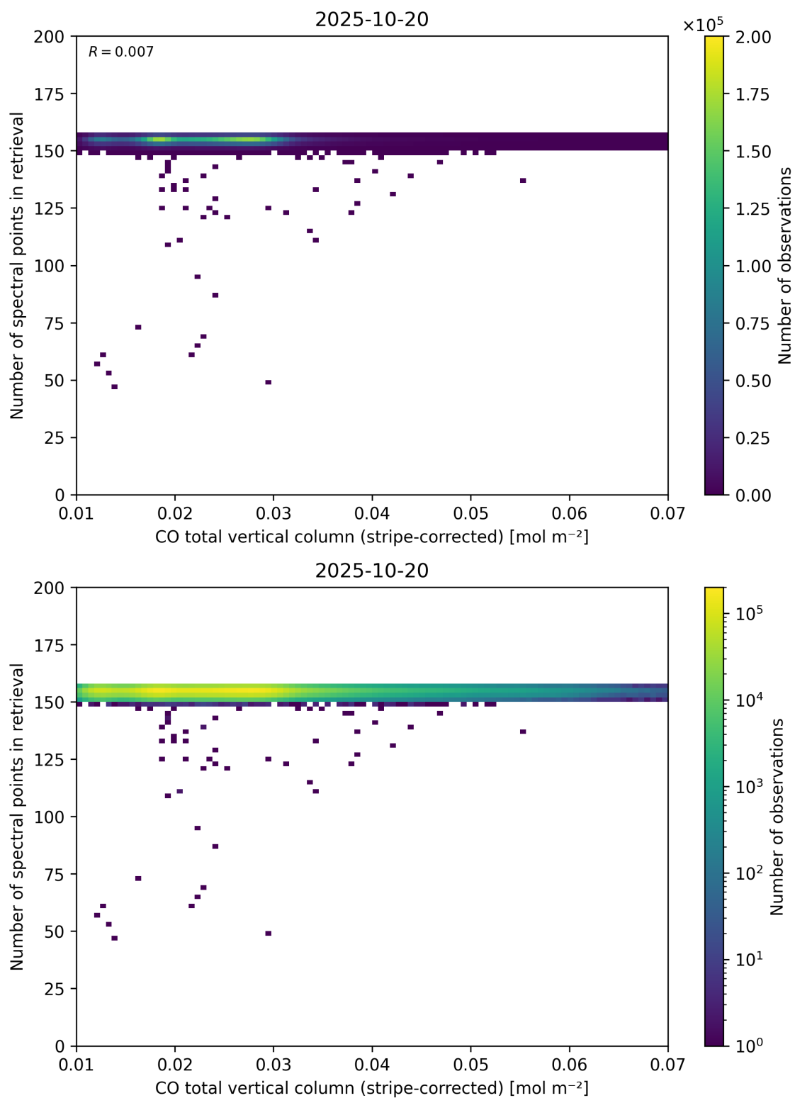
Figure 40: Scatter density plot of “CO total vertical column (stripe-corrected)” against “Number of spectral points in retrieval” for 2025-10-19 to 2025-10-21.
