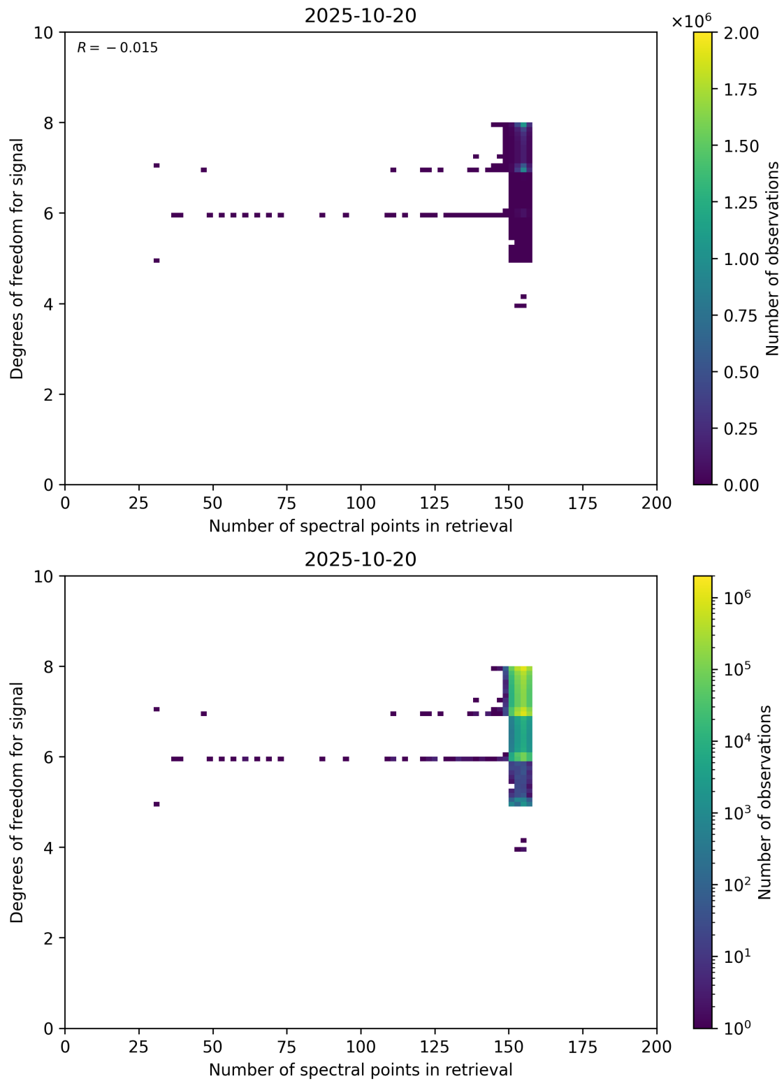
Figure 59: Scatter density plot of “Number of spectral points in retrieval” against “Degrees of freedom for signal” for 2025-10-19 to 2025-10-21.
