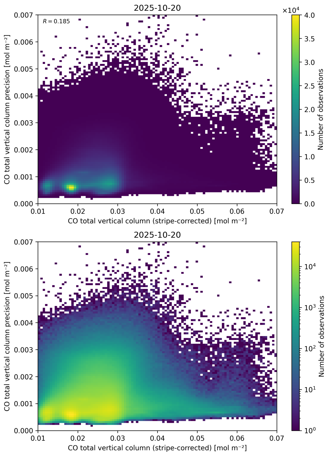
Figure 36: Scatter density plot of “CO total vertical column (stripe-corrected)” against “CO total vertical column precision” for 2025-10-19 to 2025-10-21.
