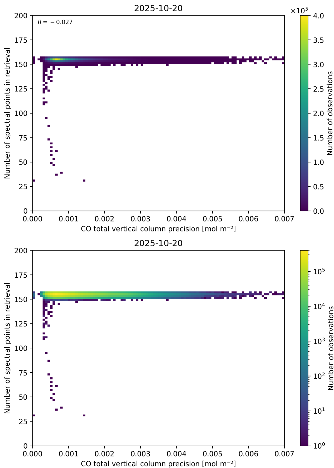
Figure 47: Scatter density plot of “CO total vertical column precision” against “Number of spectral points in retrieval” for 2025-10-19 to 2025-10-21.
