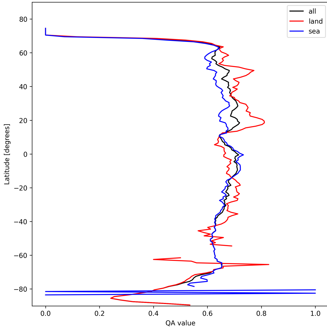
Figure 9: Zonal average of “QA value” for 2025-10-19 to 2025-10-21.
