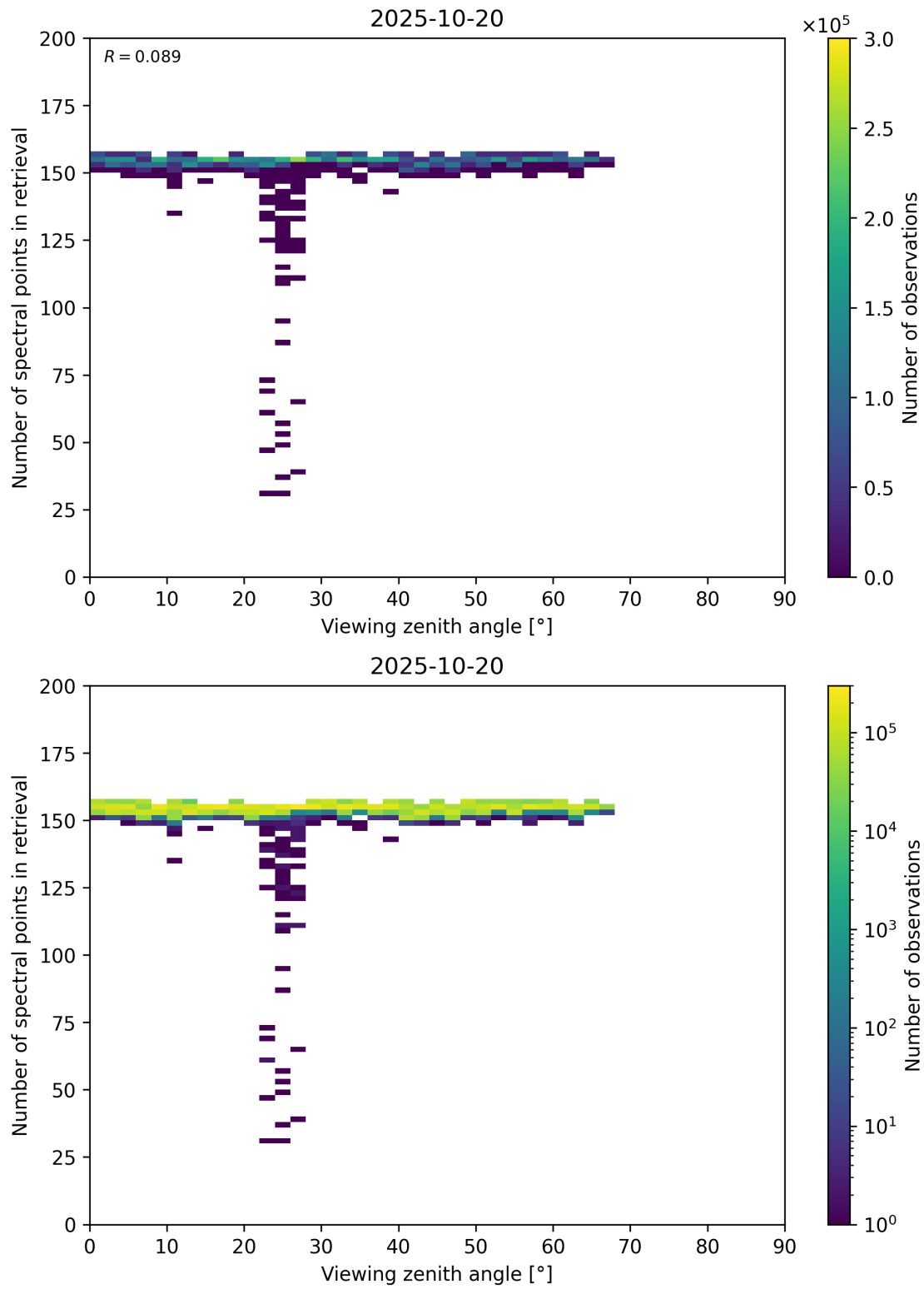
Figure 76: Scatter density plot of “Viewing zenith angle” against “Number of spectral points in retrieval” for 2025-10-19 to 2025-10-21.
