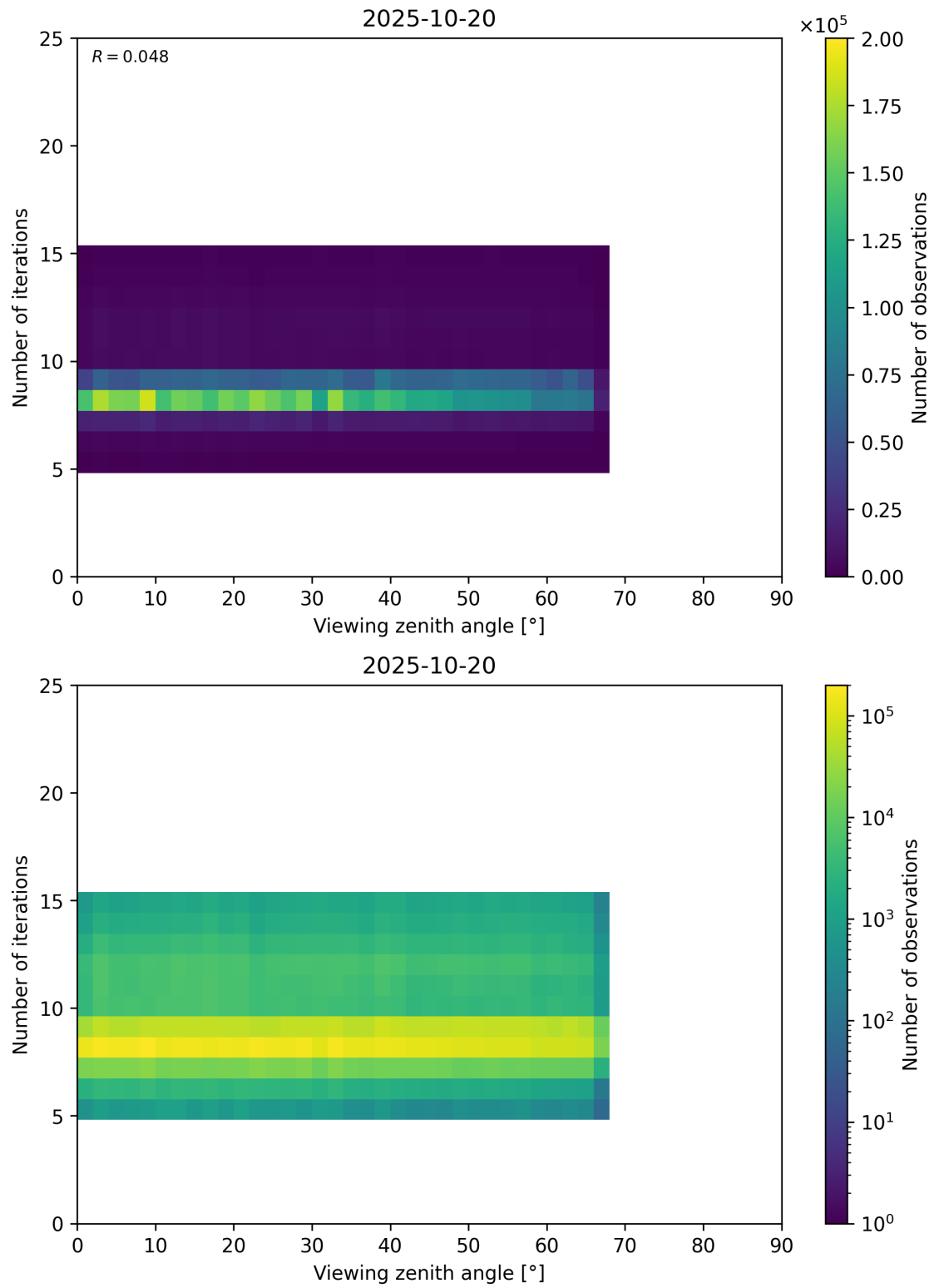
Figure 75: Scatter density plot of “Viewing zenith angle” against “Number of iterations” for 2025-10-19 to 2025-10-21.
