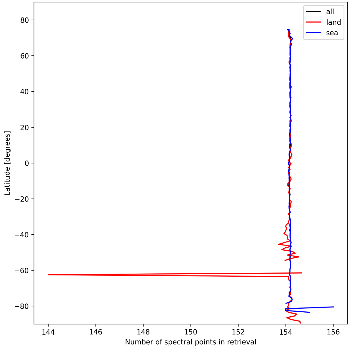
Figure 13: Zonal average of “Number of spectral points in retrieval” for 2025-10-19 to 2025-10-21.
