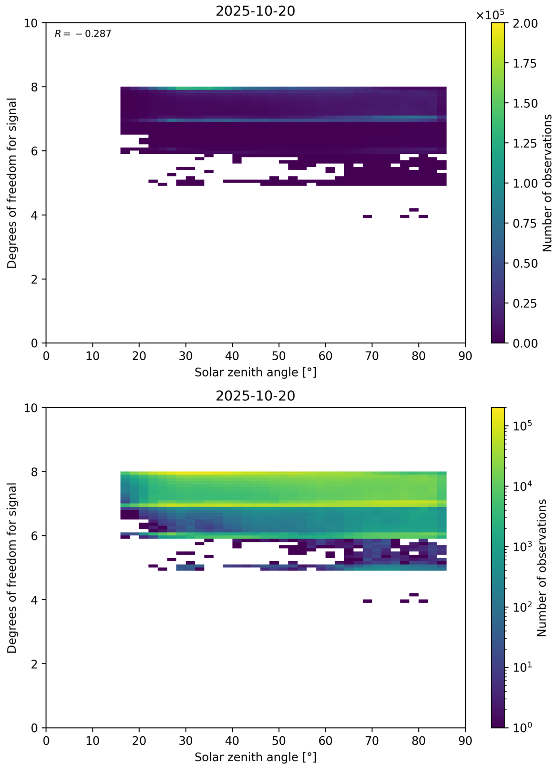
Figure 65: Scatter density plot of “Solar zenith angle” against “Degrees of freedom for signal” for 2025-10-19 to 2025-10-21.
