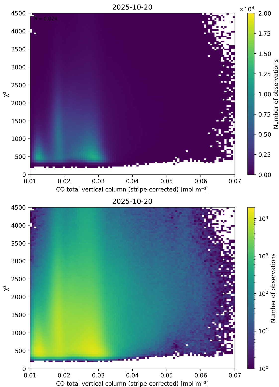
Figure 37: Scatter density plot of “CO total vertical column (stripe-corrected)” against “ \chi^2 ” for 2025-10-19 to 2025-10-21.
