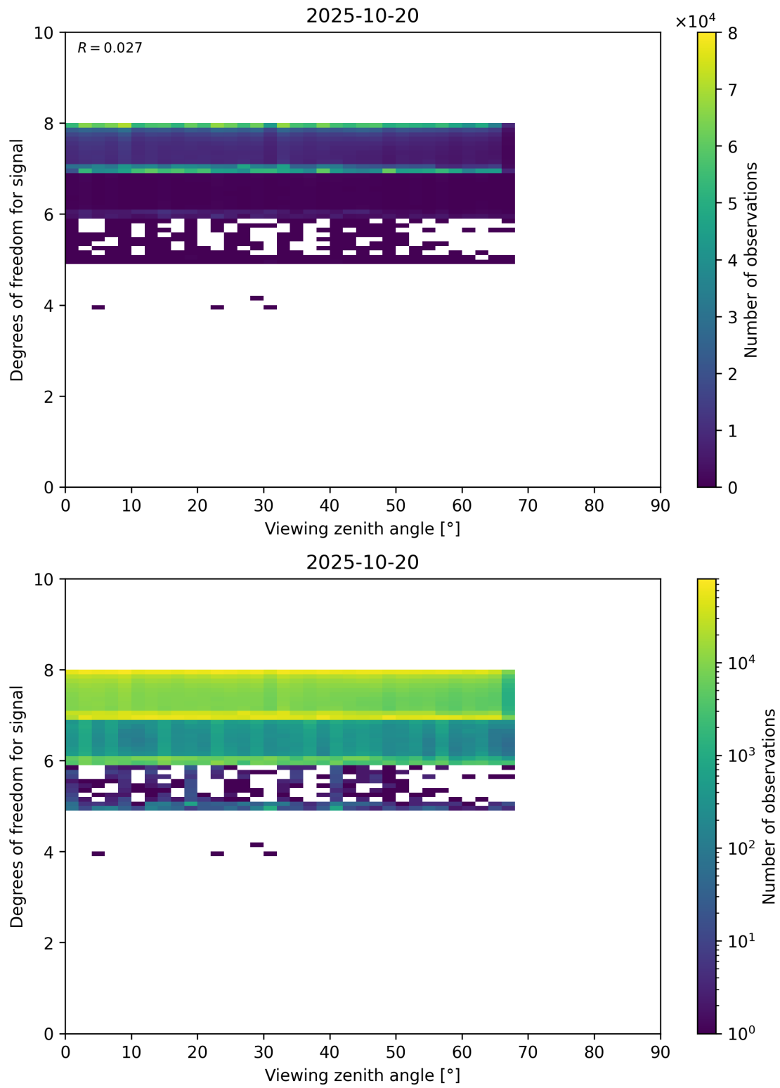
Figure 73: Scatter density plot of “Viewing zenith angle” against “Degrees of freedom for signal” for 2025-10-19 to 2025-10-21.
