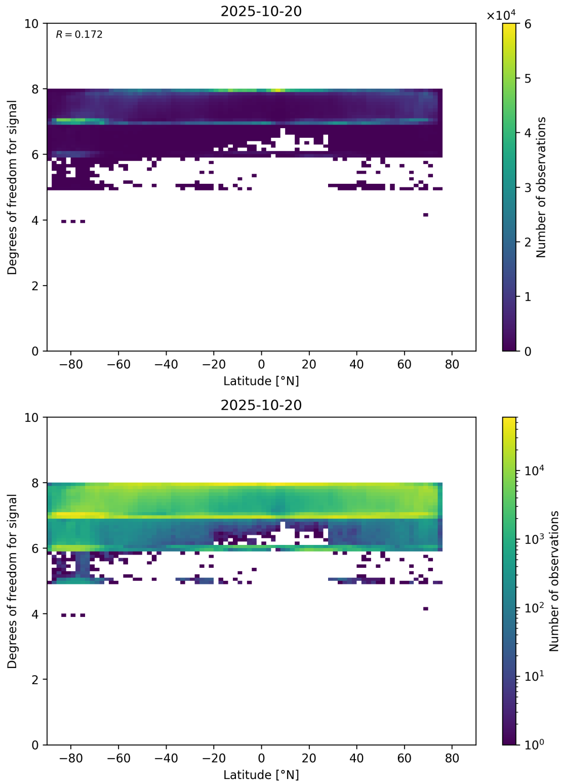
Figure 55: Scatter density plot of “Latitude” against “Degrees of freedom for signal” for 2025-10-19 to 2025-10-21.
