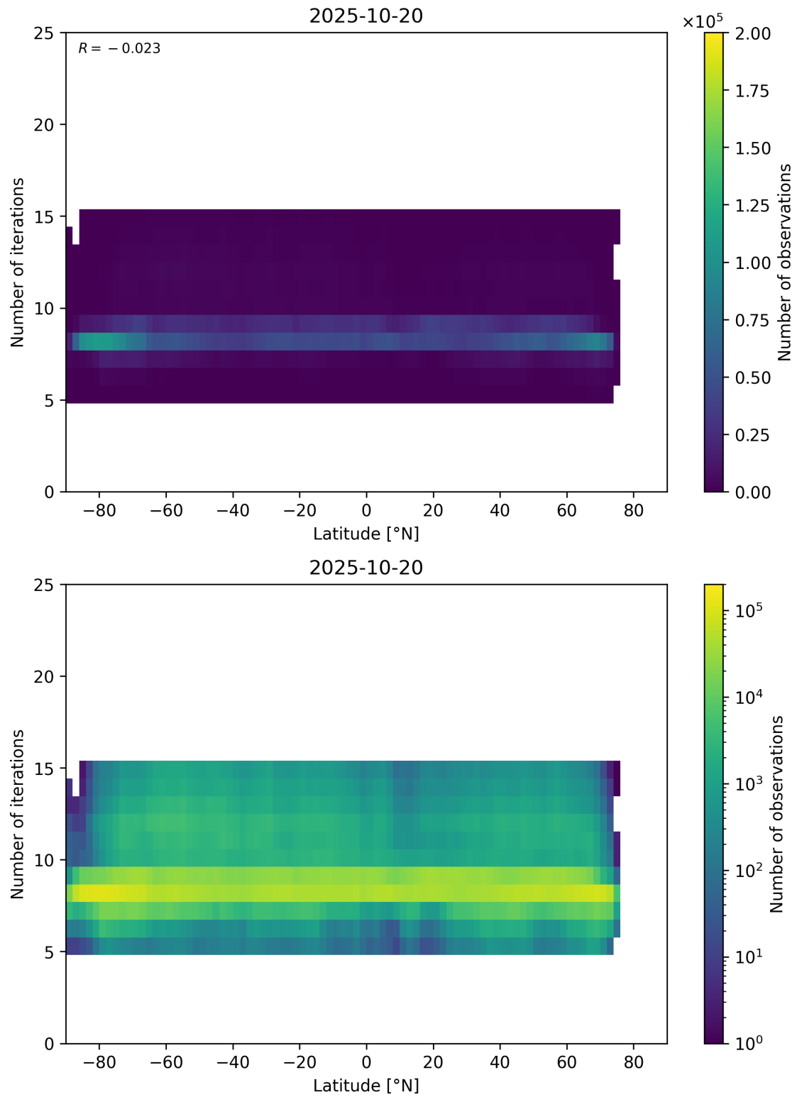
Figure 56: Scatter density plot of “Latitude” against “Number of iterations” for 2025-10-19 to 2025-10-21.
