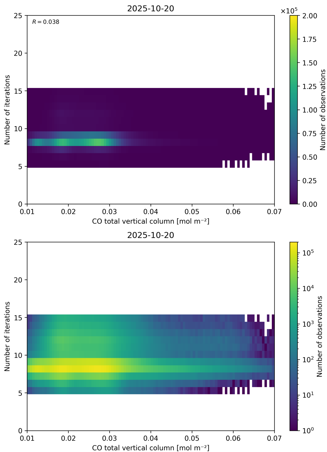
Figure 42: Scatter density plot of “CO total vertical column” against “Number of iterations” for 2025-10-19 to 2025-10-21.
