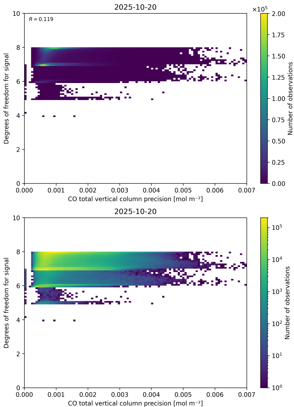
Figure 45: Scatter density plot of “CO total vertical column precision” against “Degrees of freedom for signal” for 2025-10-19 to 2025-10-21.
