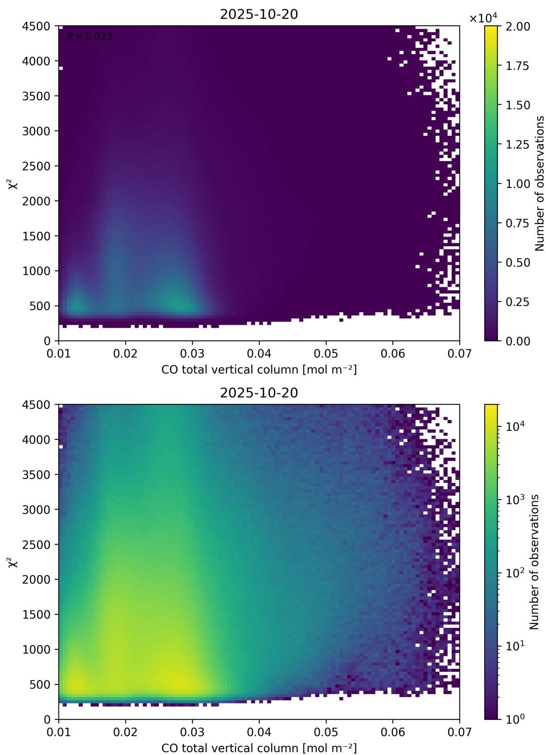
Figure 35: Scatter density plot of “CO total vertical column” against “ \chi^2 ” for 2025-10-19 to 2025-10-21.
