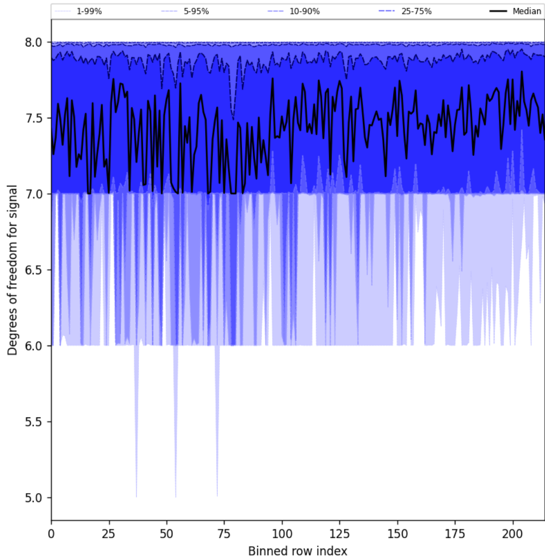
Figure 31: Along track statistics of “Degrees of freedom for signal” for 2025-10-19 to 2025-10-21
