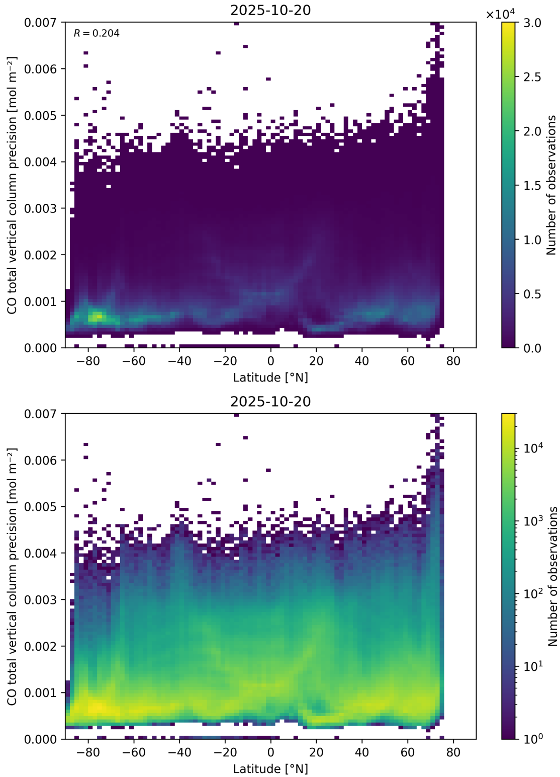
Figure 53: Scatter density plot of “Latitude” against “CO total vertical column precision” for 2025-10-19 to 2025-10-21.
