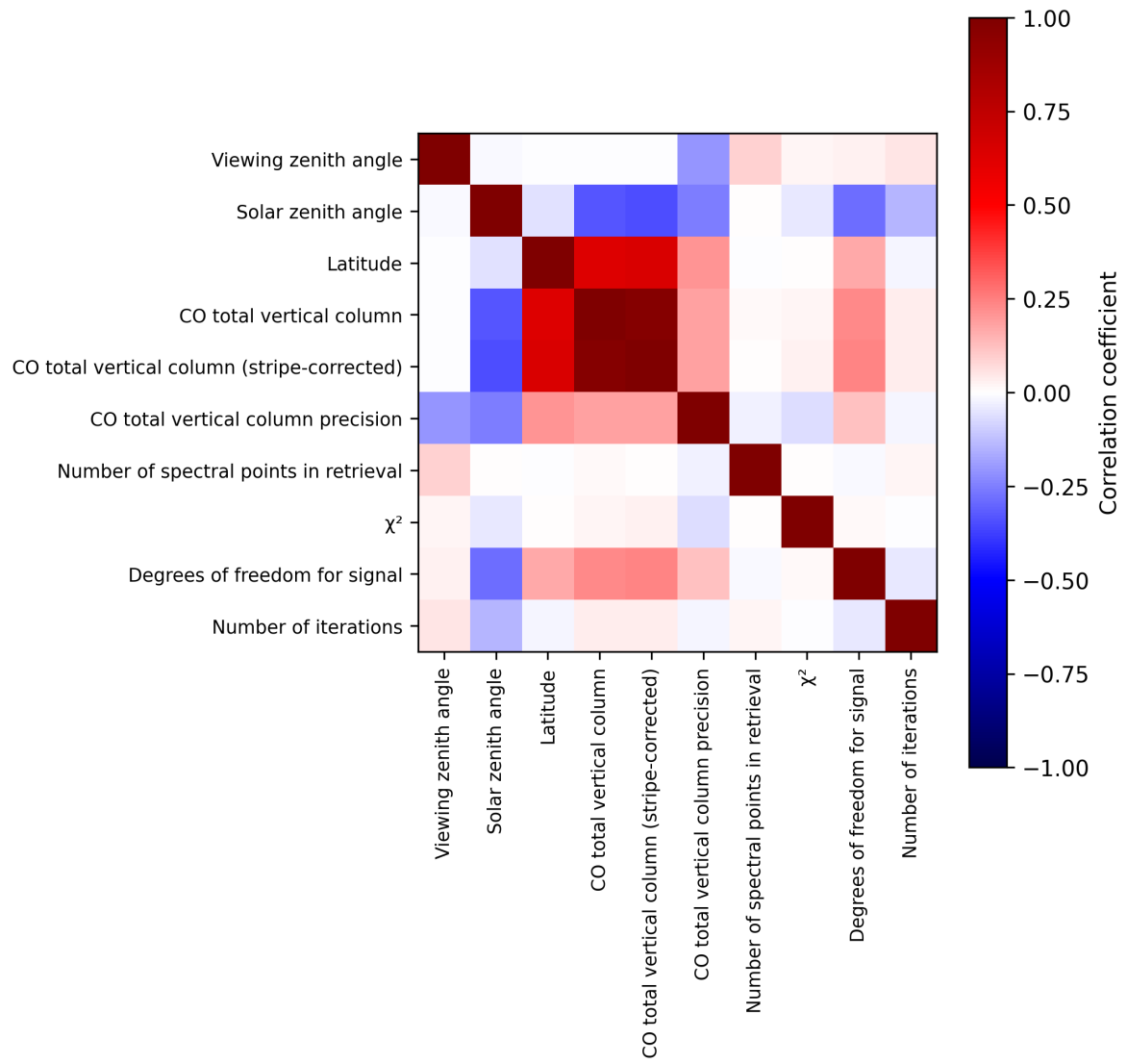
Figure 2: Map of correlation matrix for 2025-10-19 to 2025-10-21.
