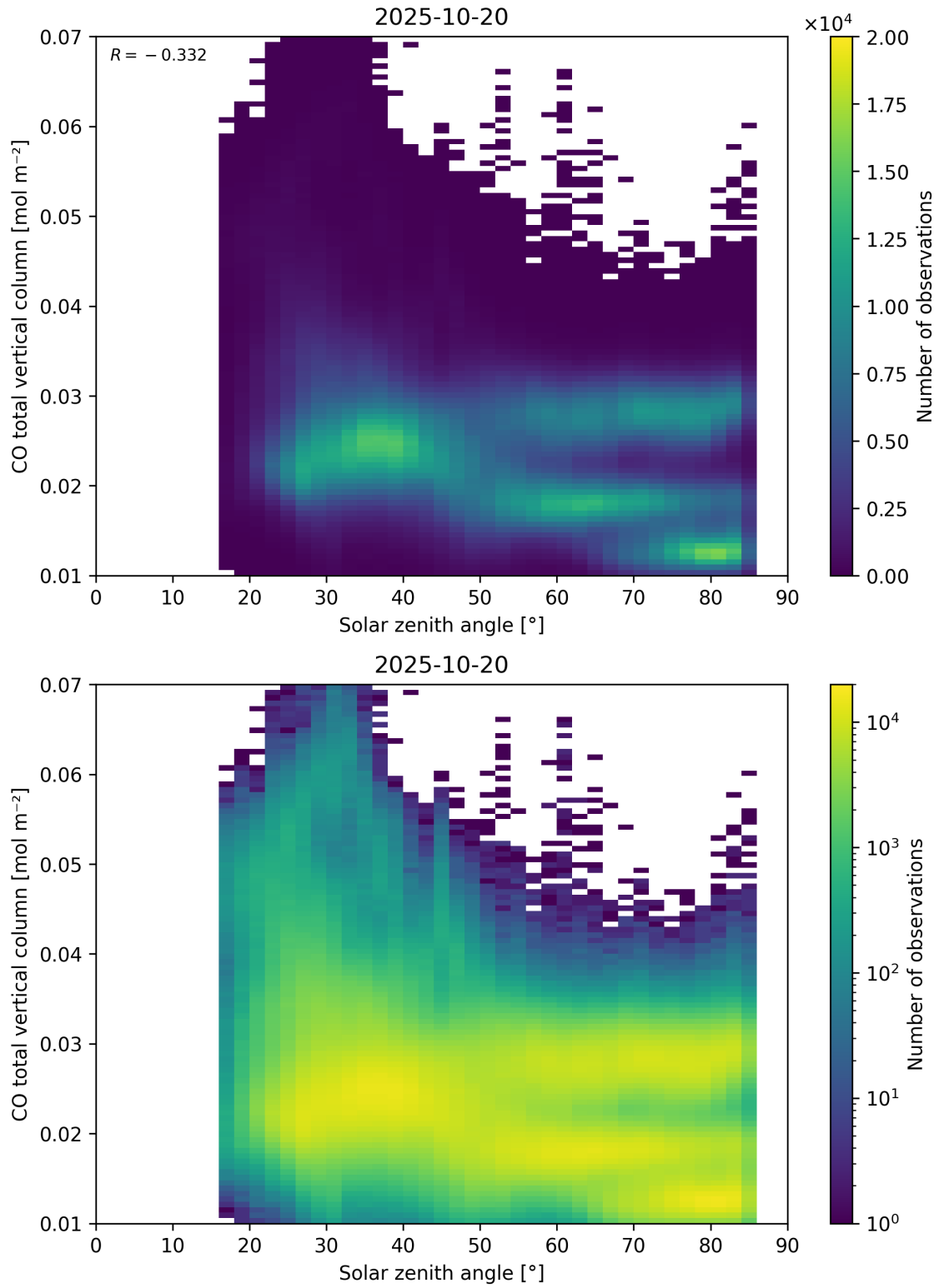
Figure 61: Scatter density plot of “Solar zenith angle” against “CO total vertical column” for 2025-10-19 to 2025-10-21.
