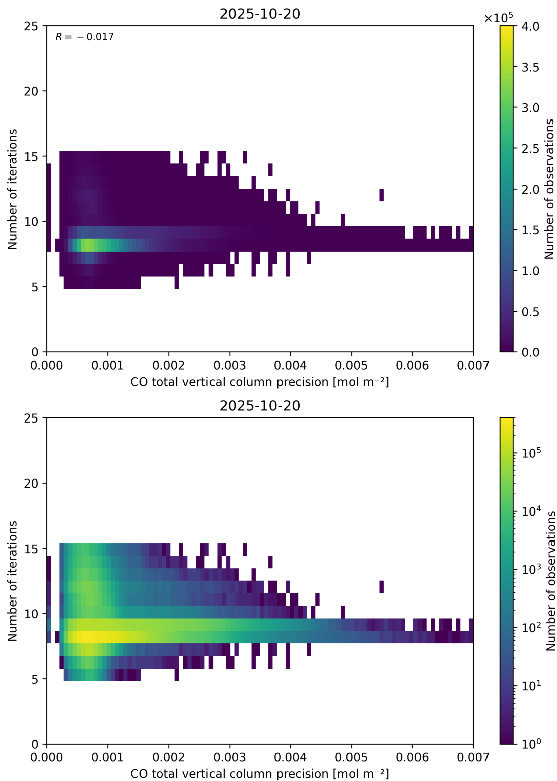
Figure 46: Scatter density plot of “CO total vertical column precision” against “Number of iterations” for 2025-10-19 to 2025-10-21.
