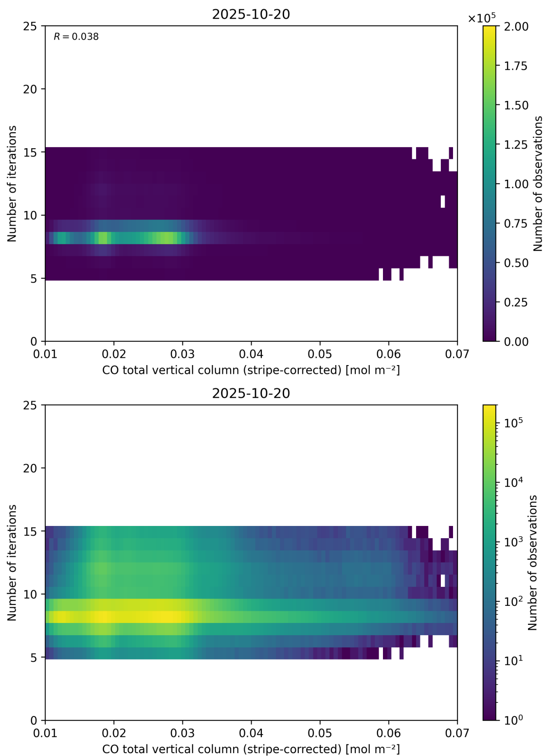
Figure 39: Scatter density plot of “CO total vertical column (stripe-corrected)” against “Number of iterations” for 2025-10-19 to 2025-10-21.
