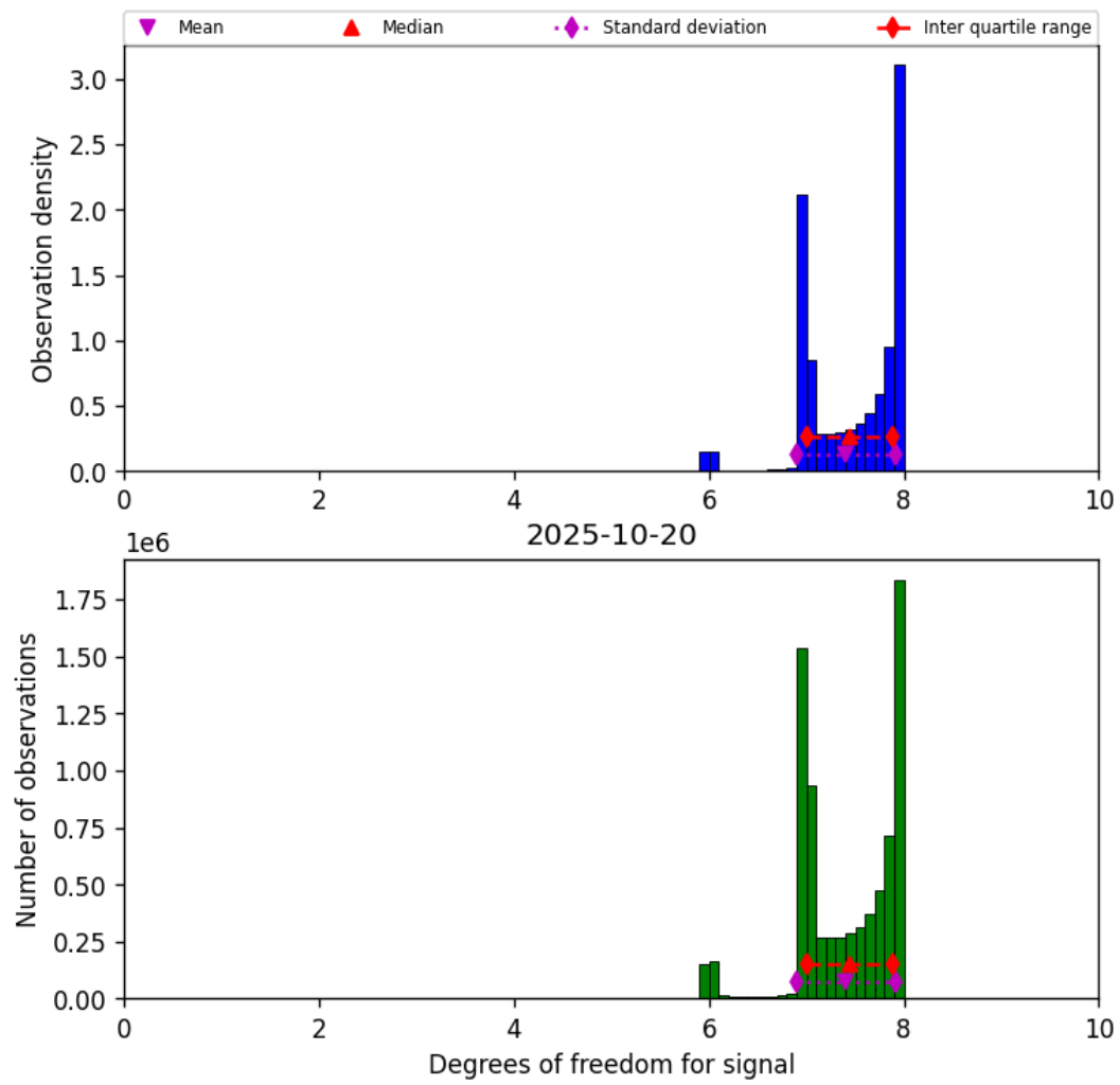
Figure 23: Histogram of “Degrees of freedom for signal” for 2025-10-19 to 2025-10-21
