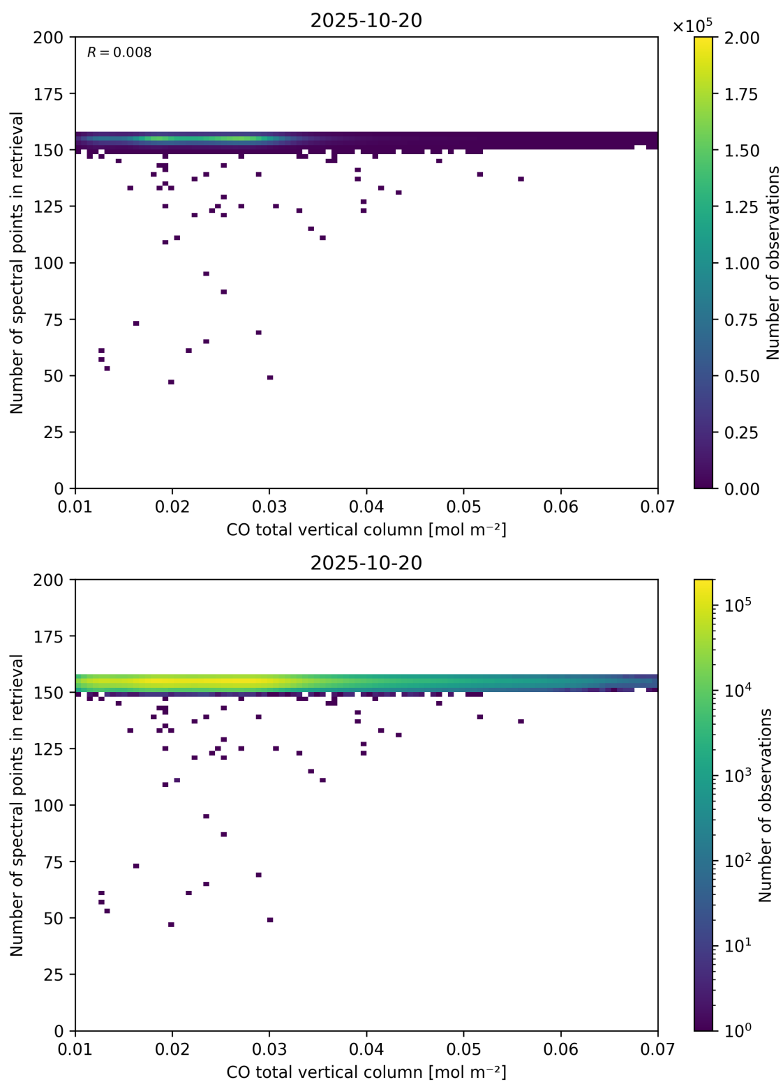
Figure 43: Scatter density plot of “CO total vertical column” against “Number of spectral points in retrieval” for 2025-10-19 to 2025-10-21.
