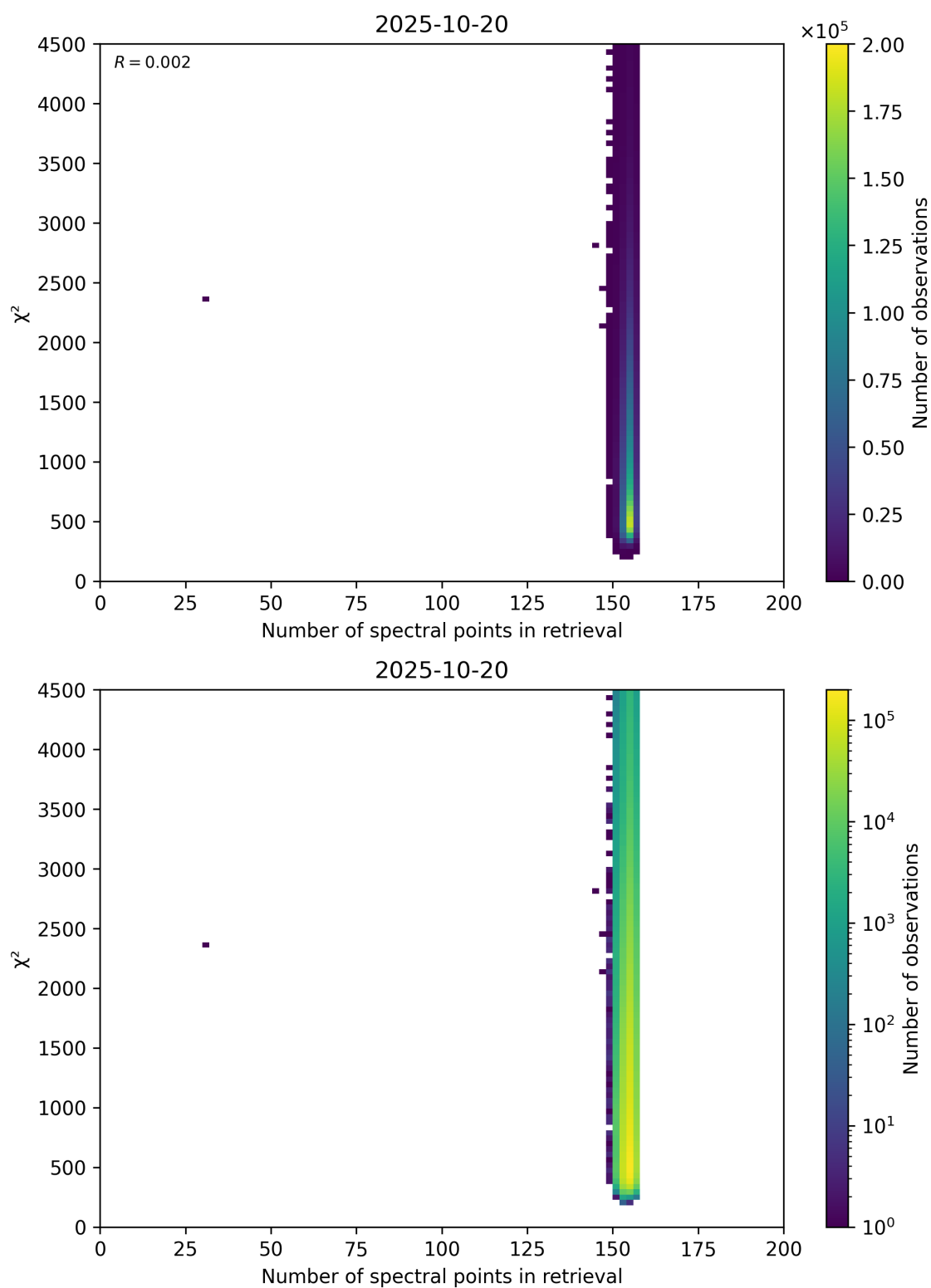
Figure 58: Scatter density plot of “Number of spectral points in retrieval” against “ \chi^2 ” for 2025-10-19 to 2025-10-21.
