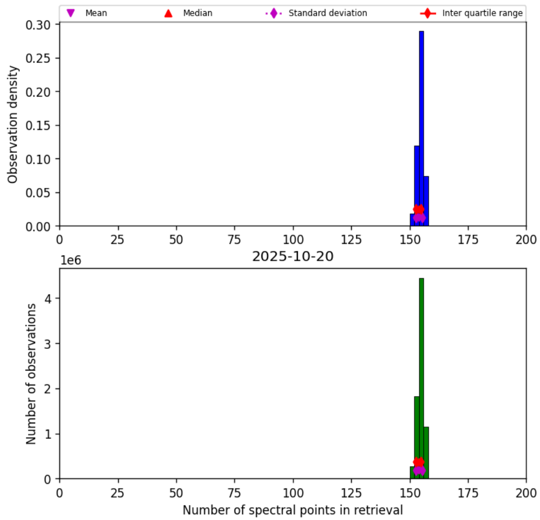
Figure 21: Histogram of “Number of spectral points in retrieval” for 2025-10-19 to 2025-10-21
