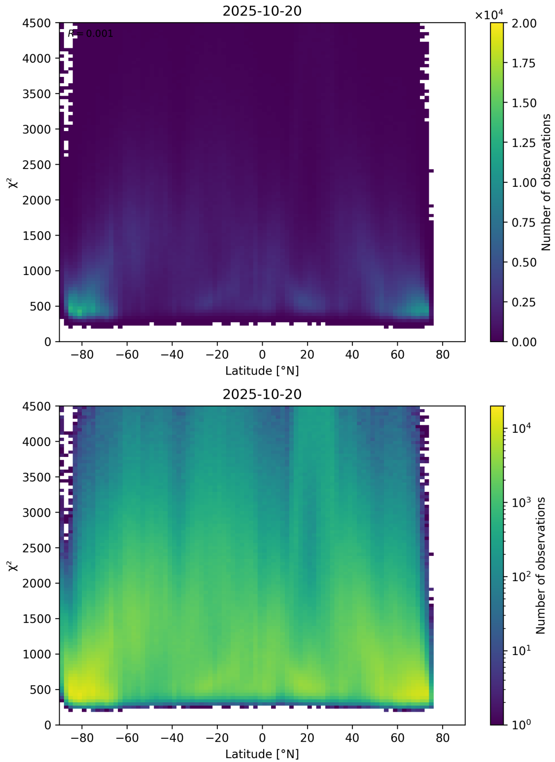
Figure 54: Scatter density plot of “Latitude” against “ \chi^2 ” for 2025-10-19 to 2025-10-21.
