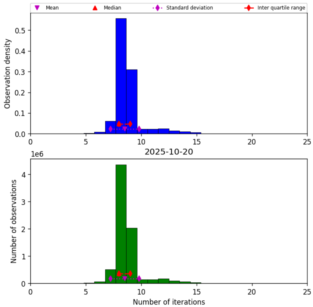
Figure 24: Histogram of “Number of iterations” for 2025-10-19 to 2025-10-21
