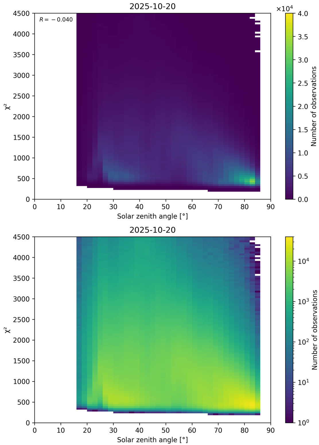
Figure 64: Scatter density plot of “Solar zenith angle” against “ \chi^2 ” for 2025-10-19 to 2025-10-21.
