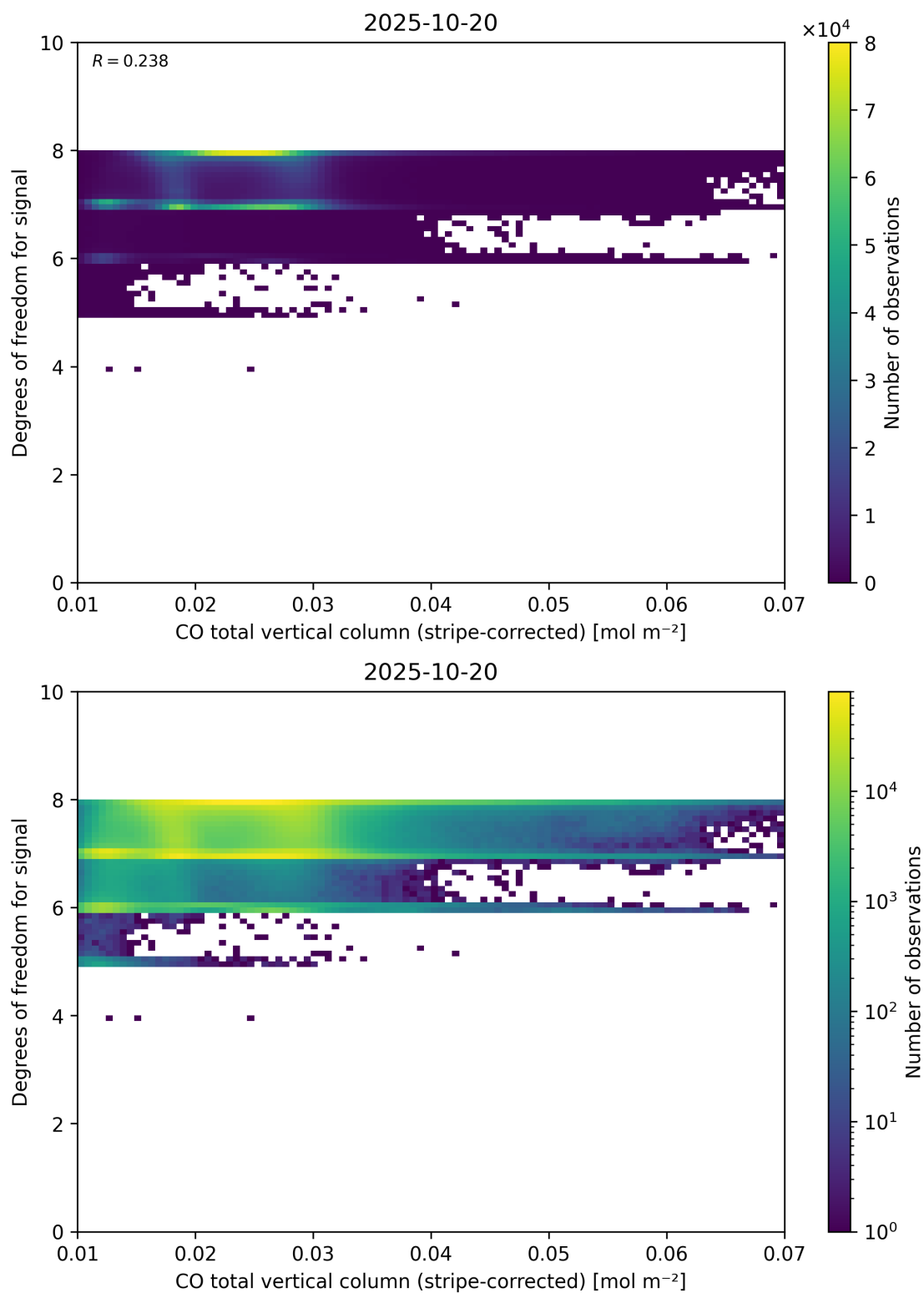
Figure 38: Scatter density plot of “CO total vertical column (stripe-corrected)” against “Degrees of freedom for signal” for 2025-10-19 to 2025-10-21.
