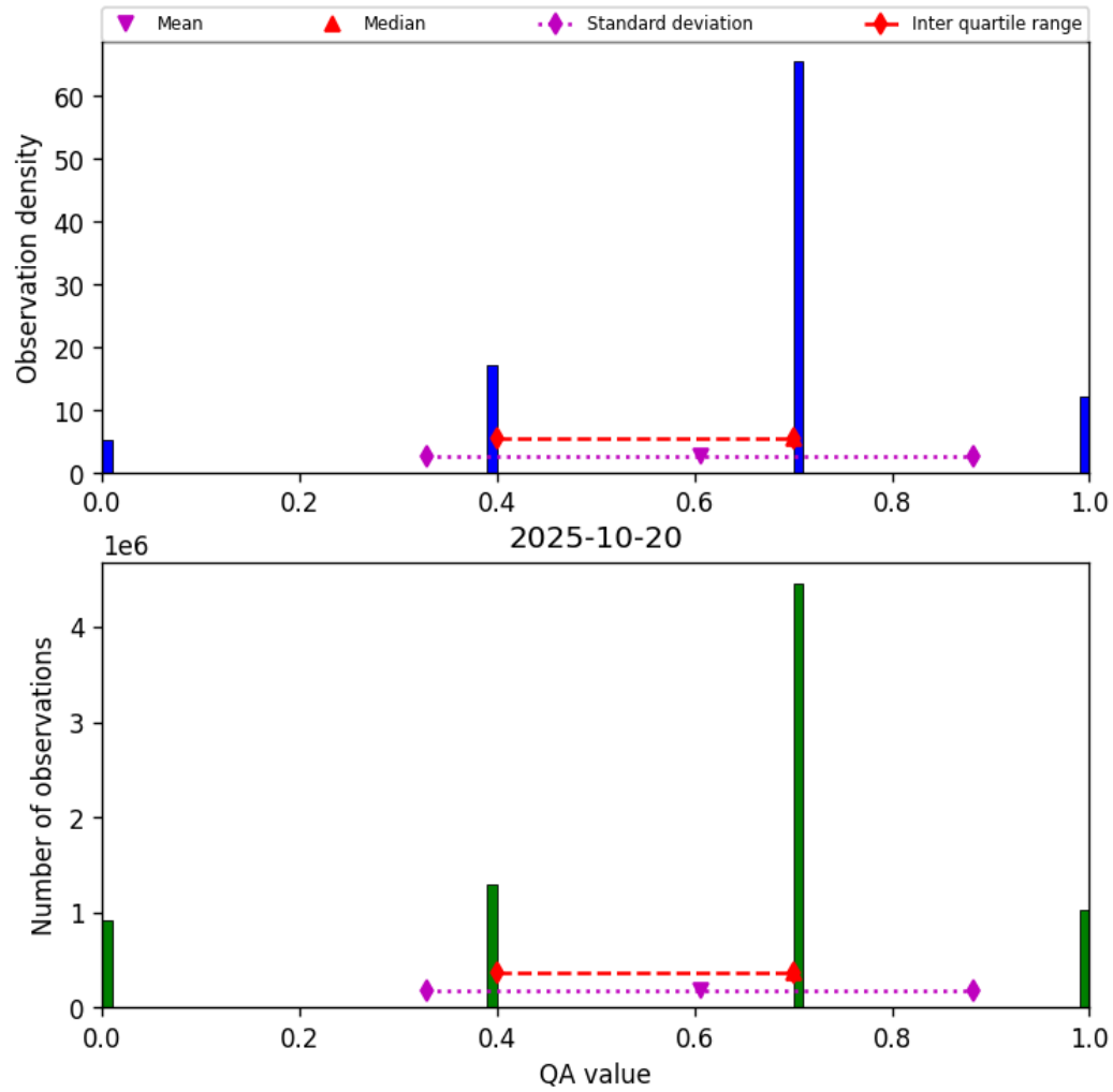
Figure 17: Histogram of “QA value” for 2025-10-19 to 2025-10-21
