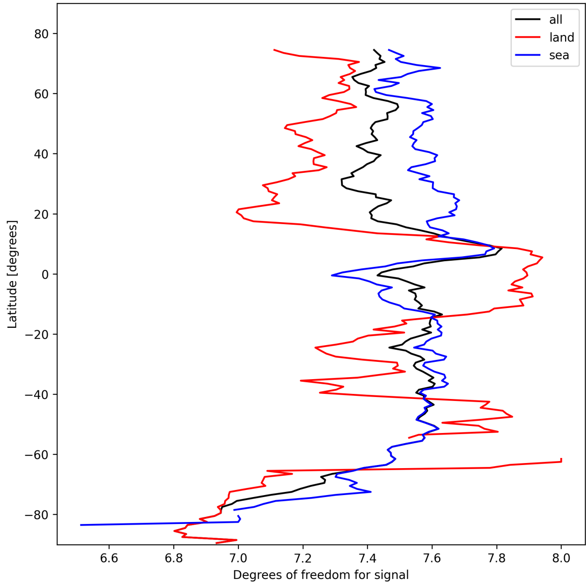
Figure 15: Zonal average of “Degrees of freedom for signal” for 2025-10-19 to 2025-10-21.
