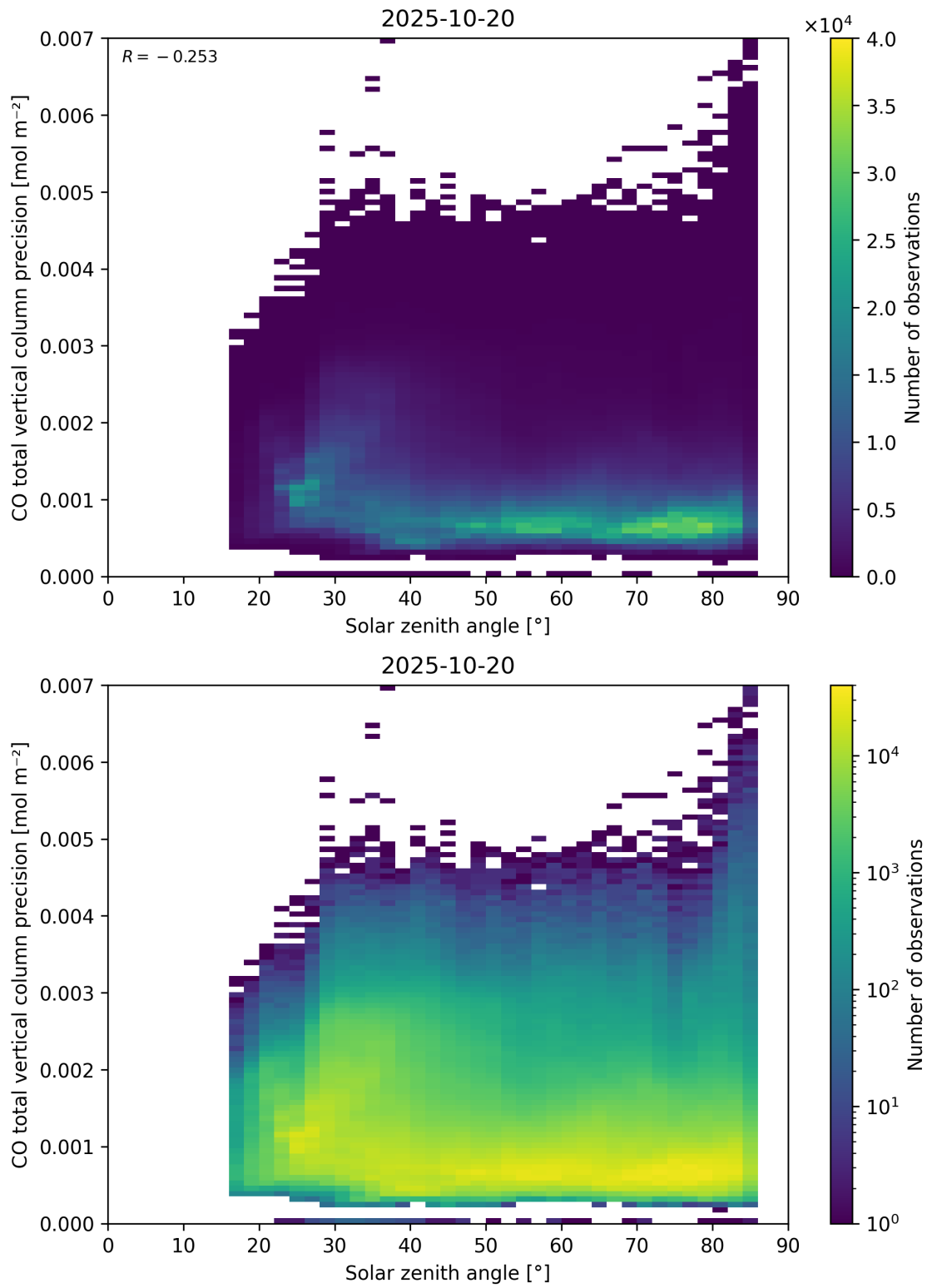
Figure 63: Scatter density plot of “Solar zenith angle” against “CO total vertical column precision” for 2025-10-19 to 2025-10-21.
