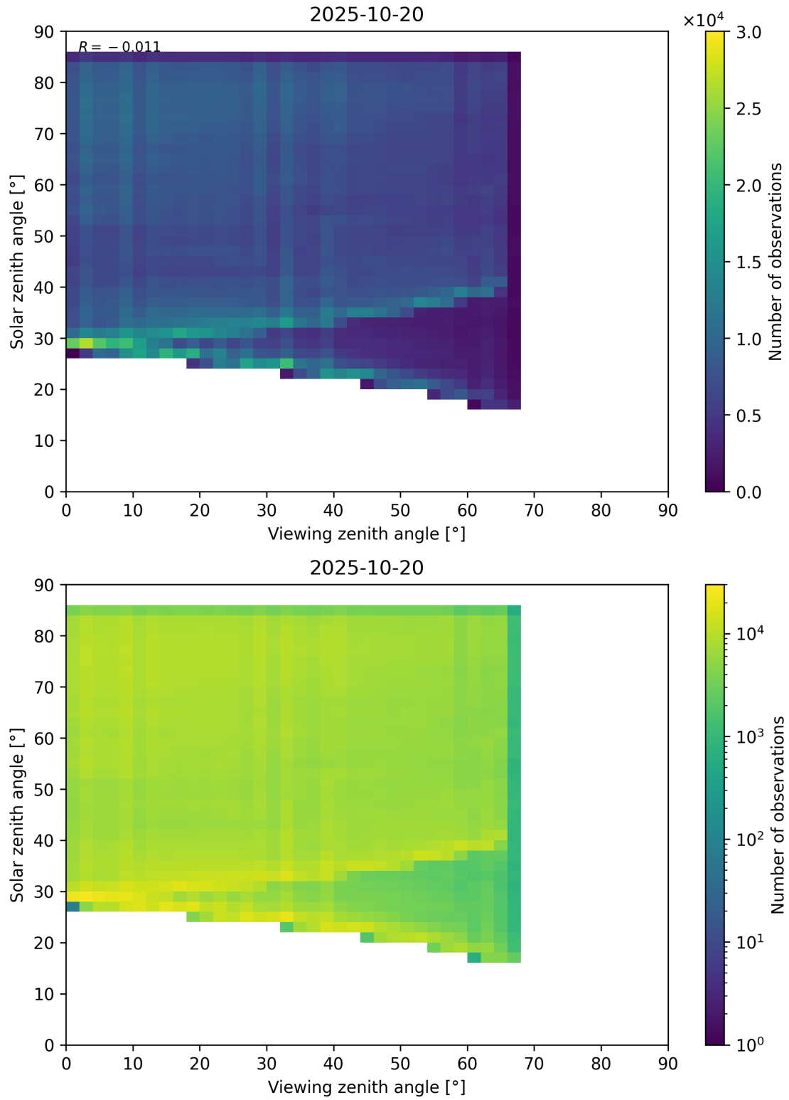
Figure 77: Scatter density plot of “Viewing zenith angle” against “Solar zenith angle” for 2025-10-19 to 2025-10-21.
