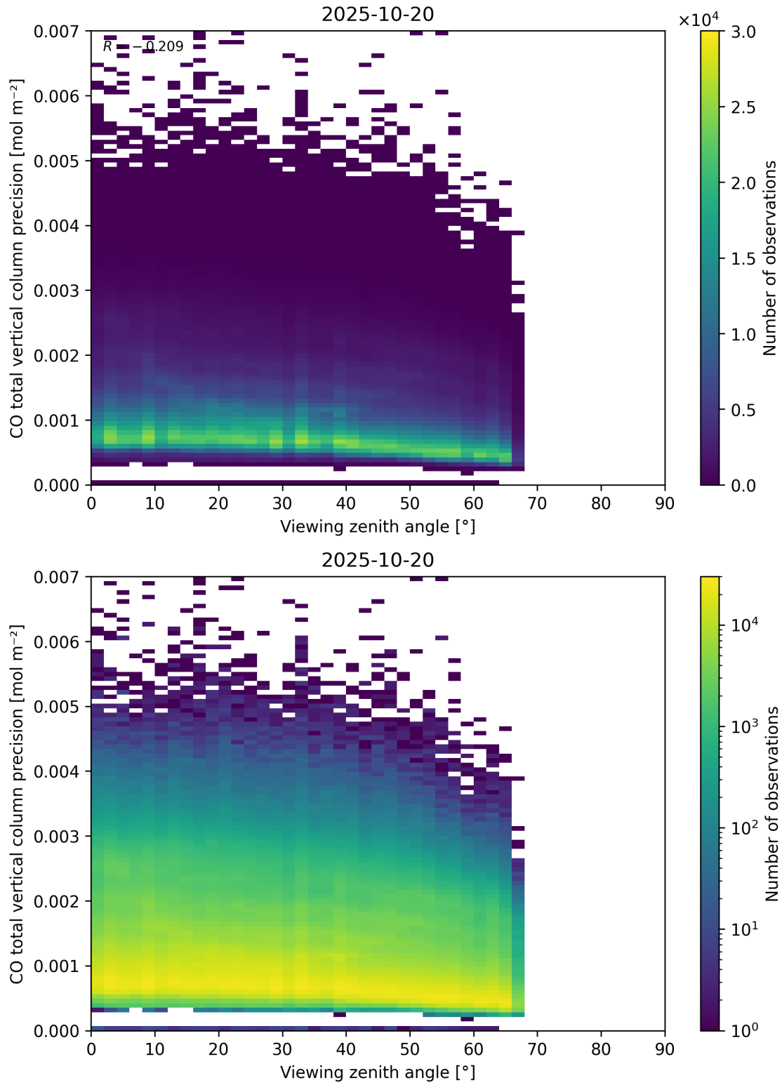
Figure 71: Scatter density plot of “Viewing zenith angle” against “CO total vertical column precision” for 2025-10-19 to 2025-10-21.
