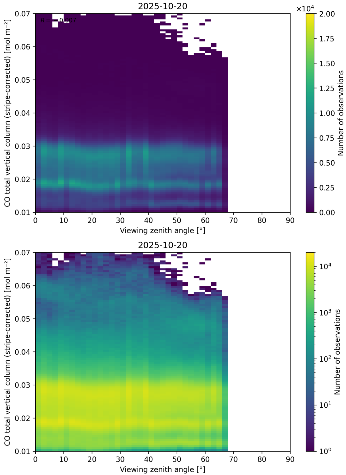
Figure 70: Scatter density plot of “Viewing zenith angle” against “CO total vertical column (stripe-corrected)” for 2025-10-19 to 2025-10-21.
