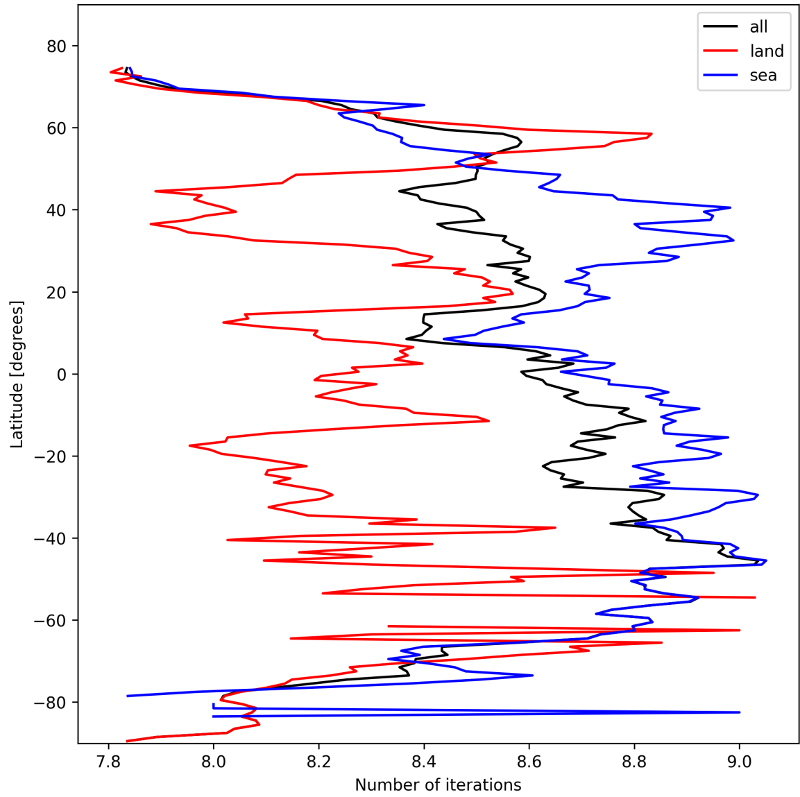
Figure 16: Zonal average of “Number of iterations” for 2025-10-19 to 2025-10-21.
