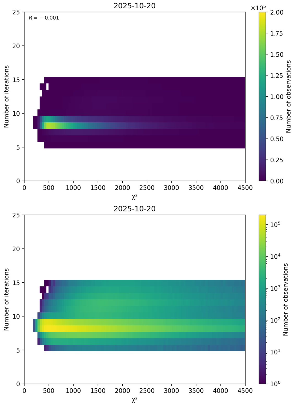
Figure 49: Scatter density plot of “ \chi^2 ” against “Number of iterations” for 2025-10-19 to 2025-10-21.
