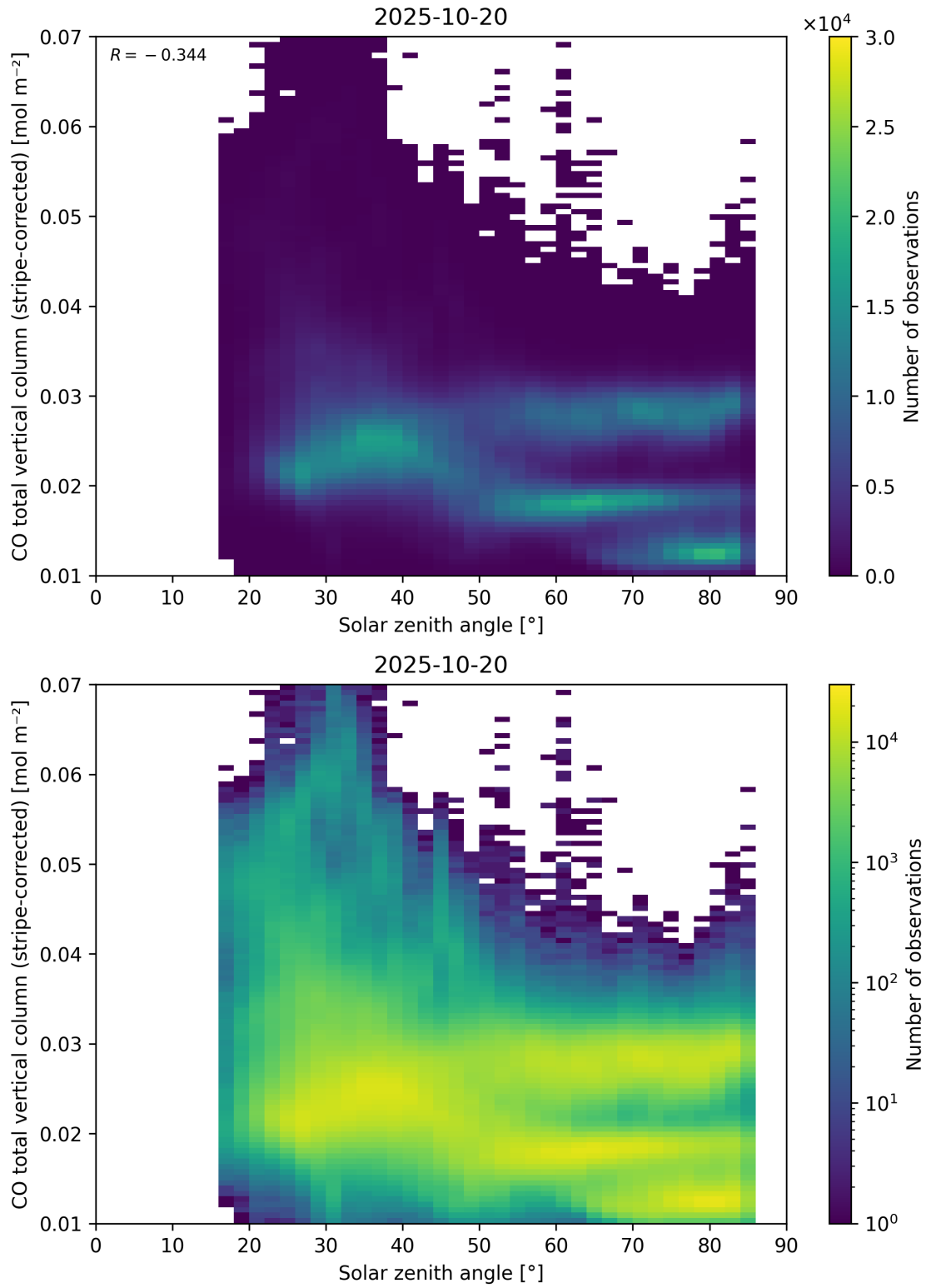
Figure 62: Scatter density plot of “Solar zenith angle” against “CO total vertical column (stripe-corrected)” for 2025-10-19 to 2025-10-21.
