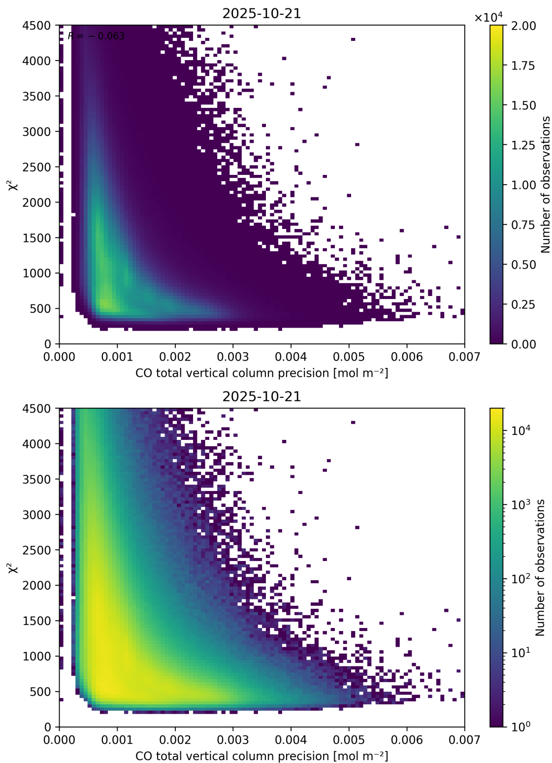
Figure 44: Scatter density plot of “CO total vertical column precision” against “ \chi^2 ” for 2025-10-20 to 2025-10-22.
