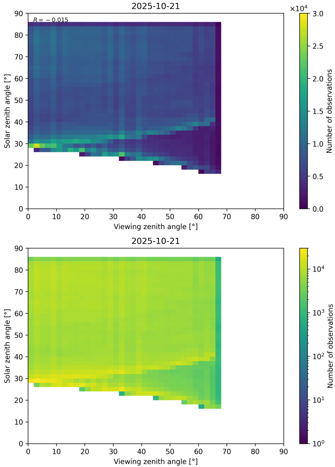
Figure 77: Scatter density plot of “Viewing zenith angle” against “Solar zenith angle” for 2025-10-20 to 2025-10-22.
