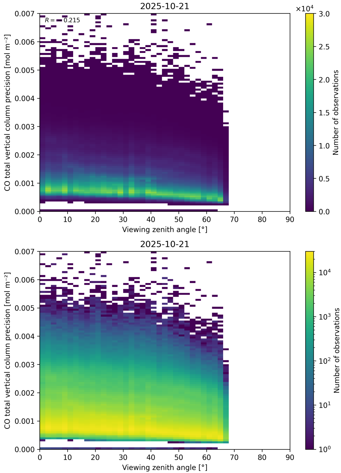
Figure 71: Scatter density plot of “Viewing zenith angle” against “CO total vertical column precision” for 2025-10-20 to 2025-10-22.
