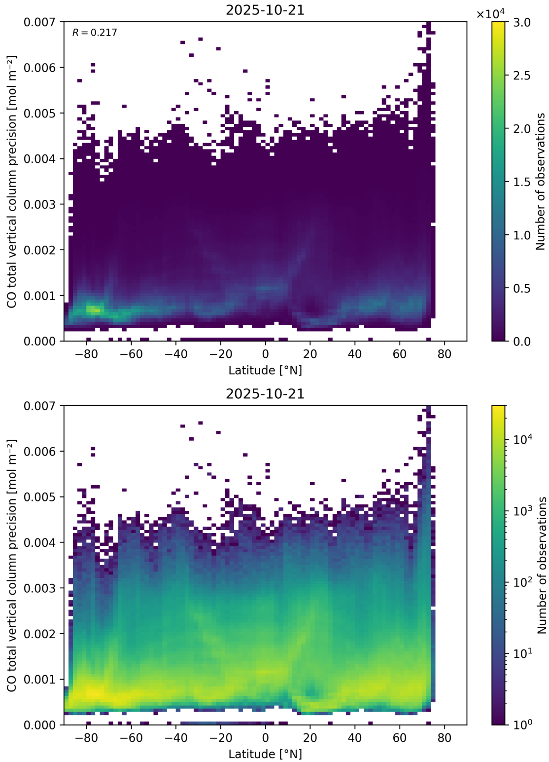
Figure 53: Scatter density plot of “Latitude” against “CO total vertical column precision” for 2025-10-20 to 2025-10-22.
