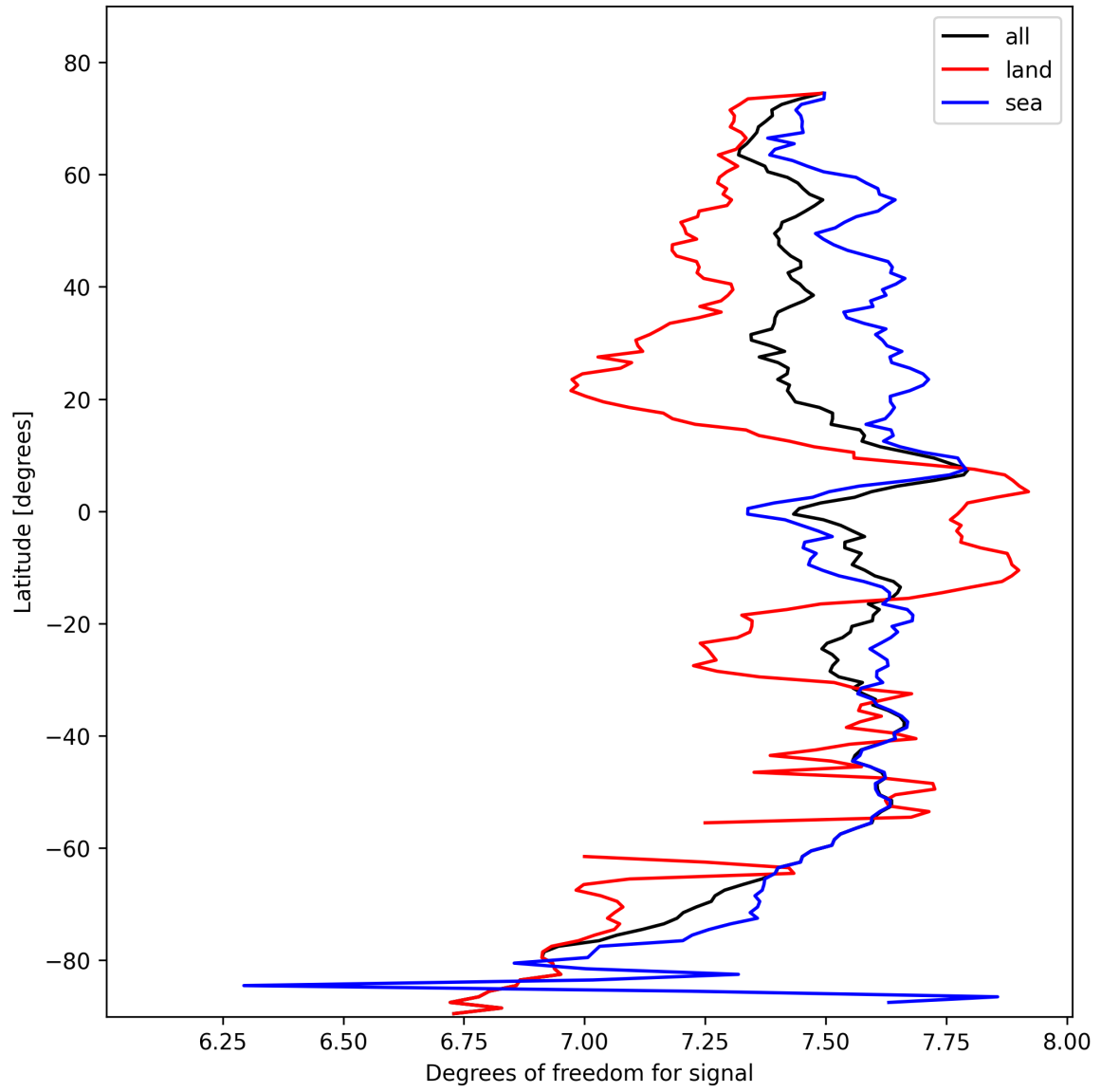
Figure 15: Zonal average of “Degrees of freedom for signal” for 2025-10-20 to 2025-10-22.
