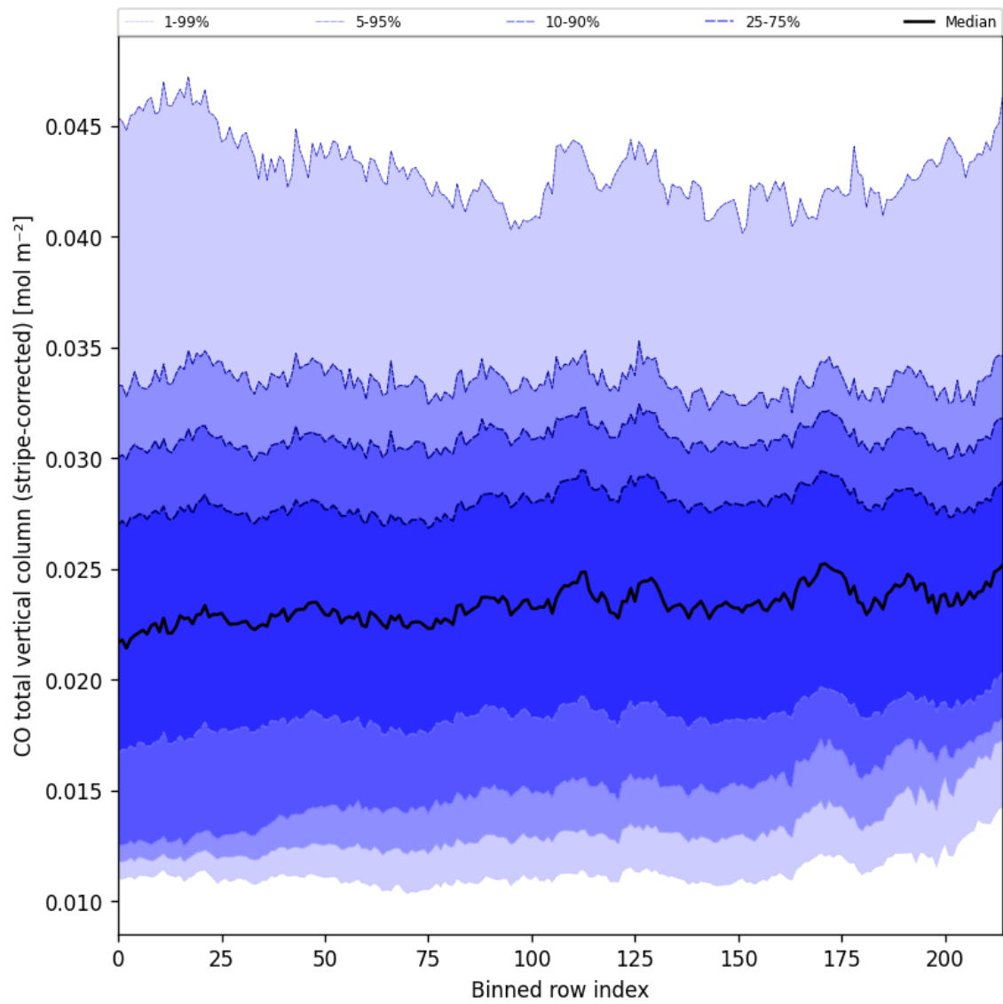
Figure 27: Along track statistics of “CO total vertical column (stripe-corrected)” for 2025-10-20 to 2025-10-22
