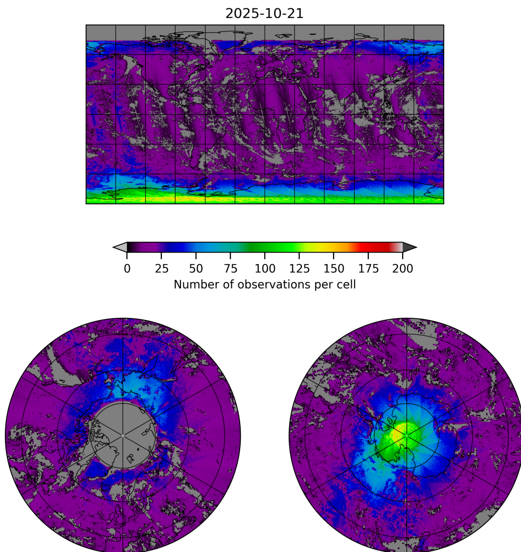
Figure 8: Map of the number of observations for 2025-10-20 to 2025-10-22
