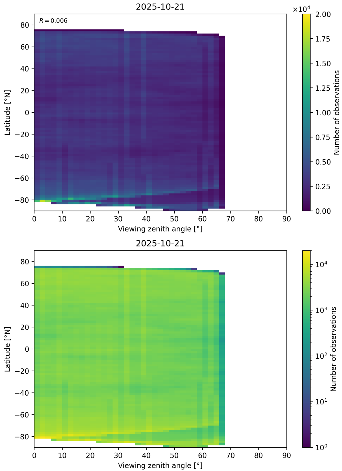
Figure 74: Scatter density plot of “Viewing zenith angle” against “Latitude” for 2025-10-20 to 2025-10-22.
