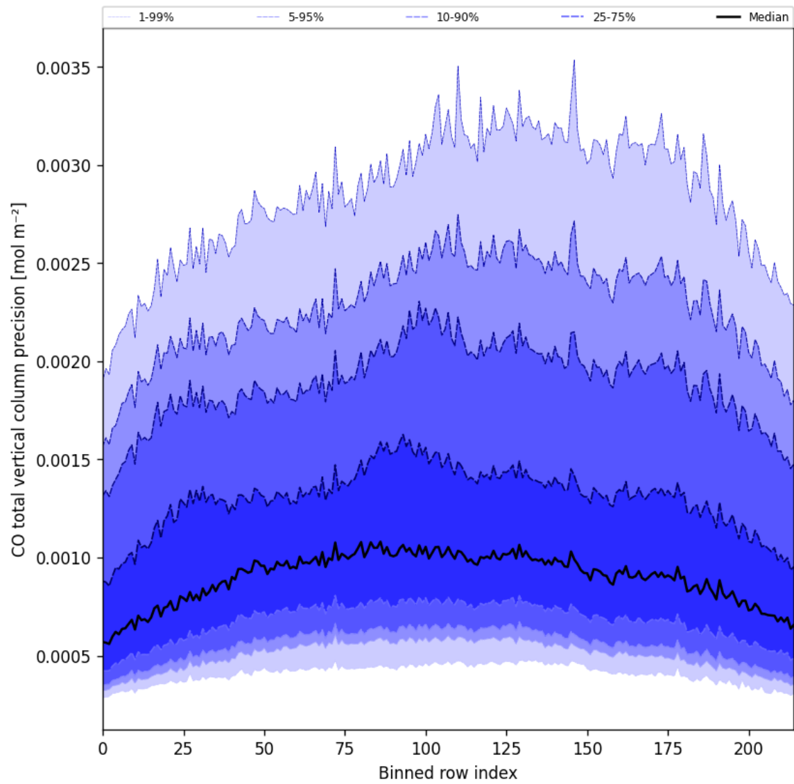
Figure 28: Along track statistics of “CO total vertical column precision” for 2025-10-20 to 2025-10-22
