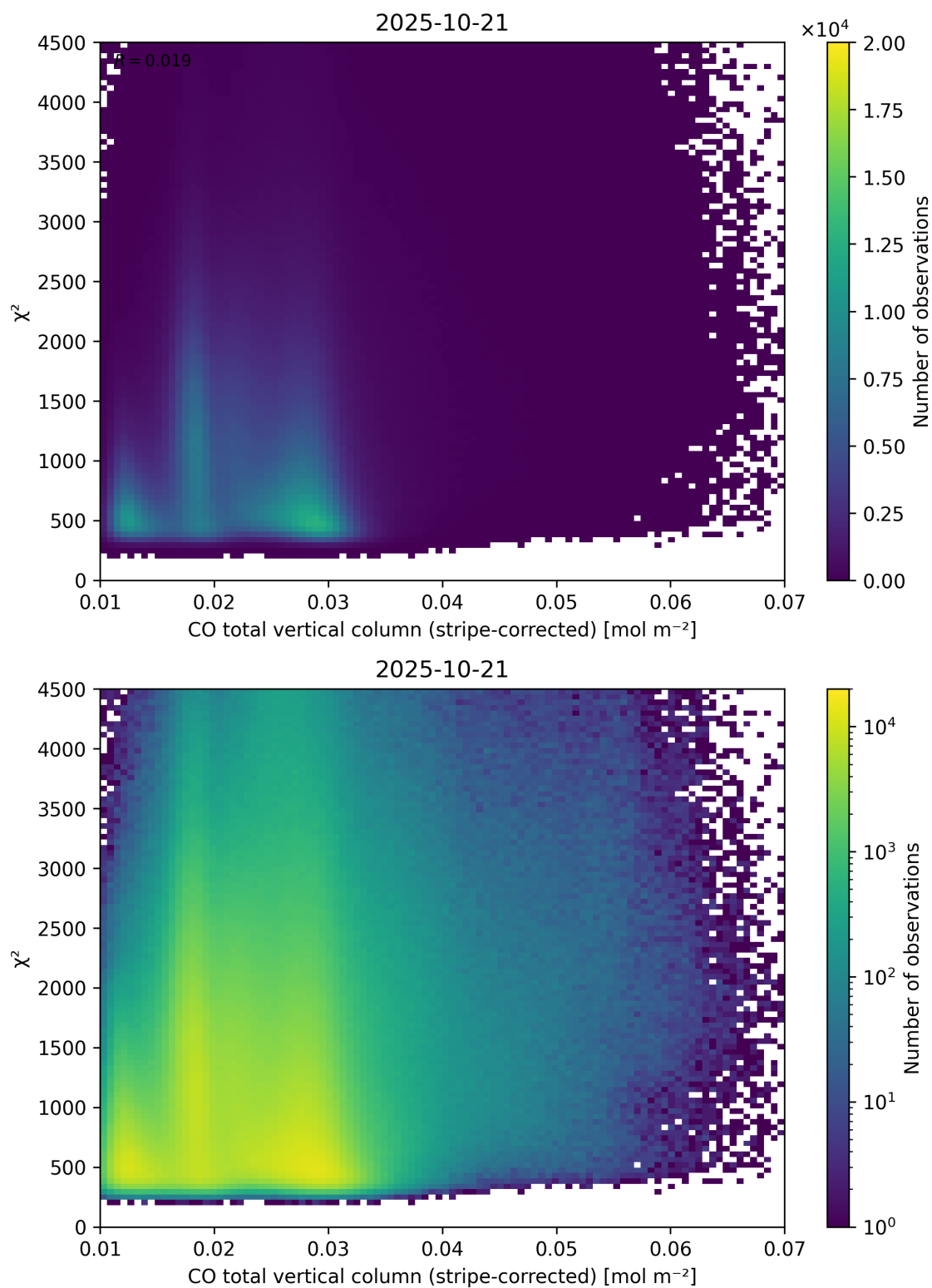
Figure 37: Scatter density plot of “CO total vertical column (stripe-corrected)” against “ \chi^2 ” for 2025-10-20 to 2025-10-22.
