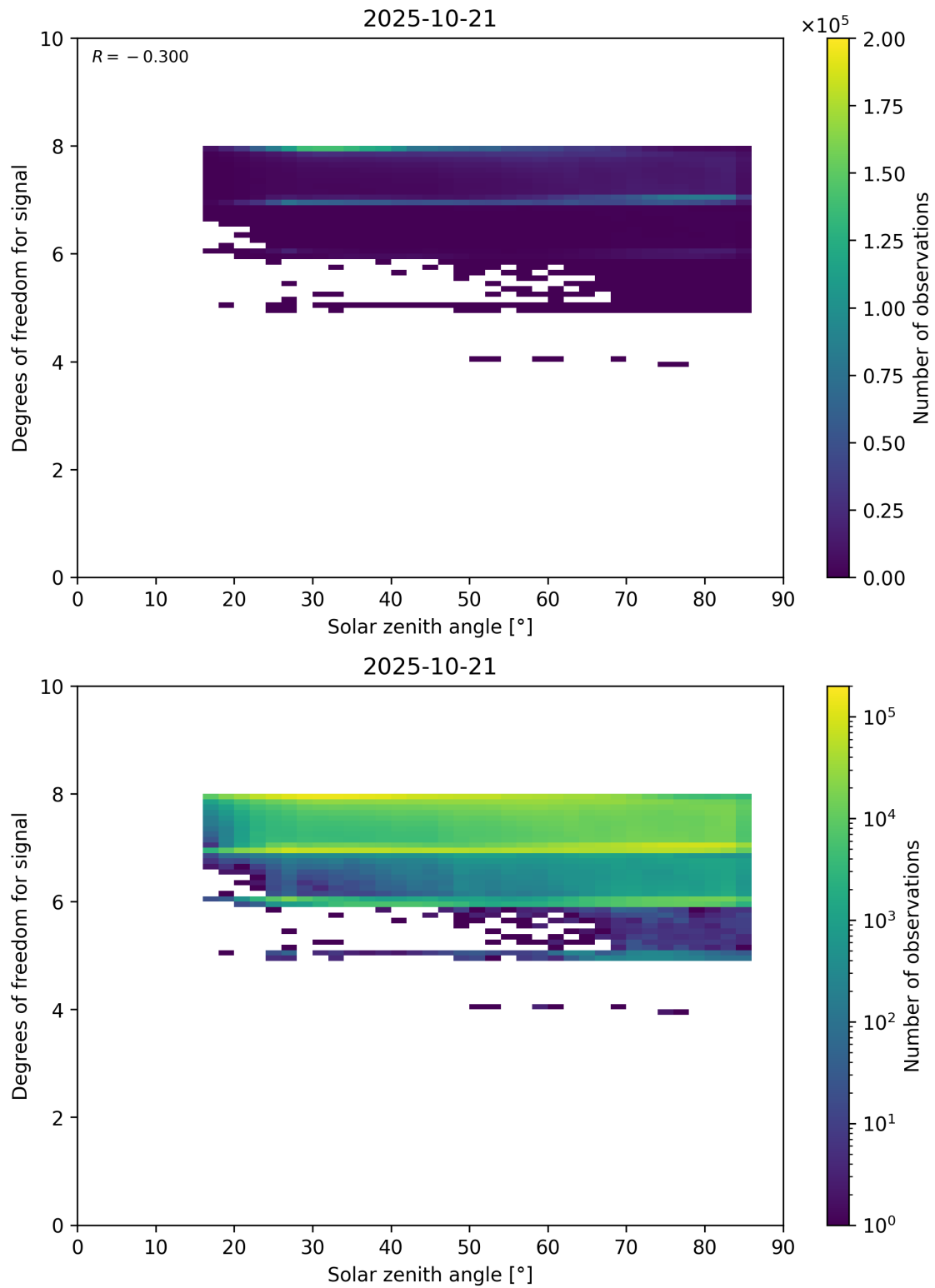
Figure 65: Scatter density plot of “Solar zenith angle” against “Degrees of freedom for signal” for 2025-10-20 to 2025-10-22.
