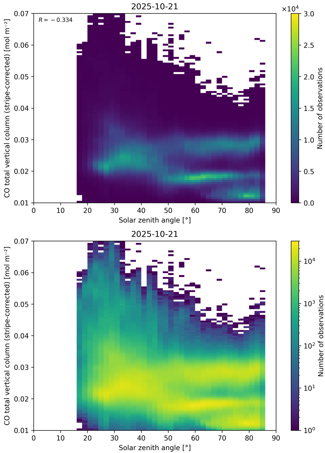
Figure 62: Scatter density plot of “Solar zenith angle” against “CO total vertical column (stripe-corrected)” for 2025-10-20 to 2025-10-22.
