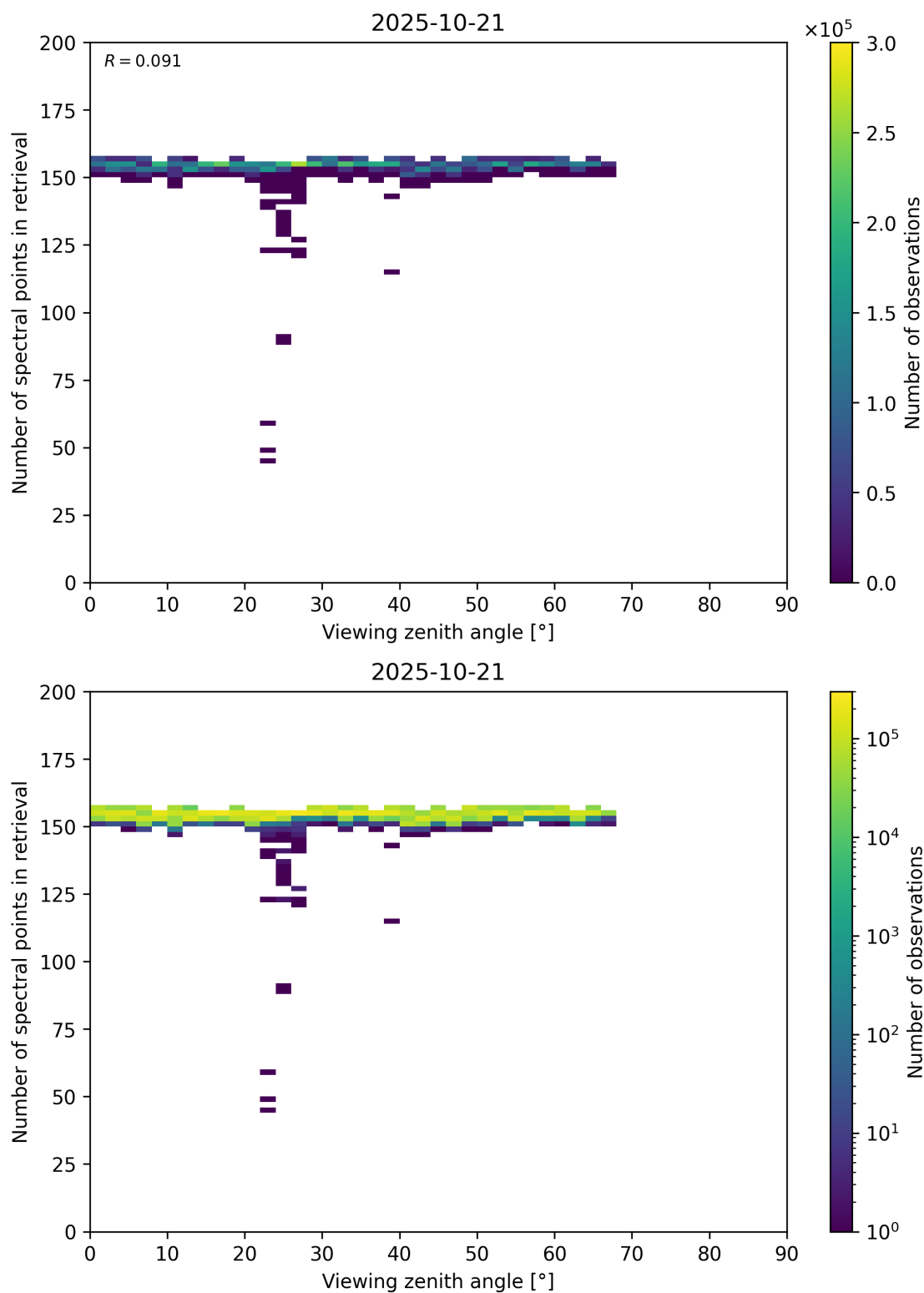
Figure 76: Scatter density plot of “Viewing zenith angle” against “Number of spectral points in retrieval” for 2025-10-20 to 2025-10-22.
