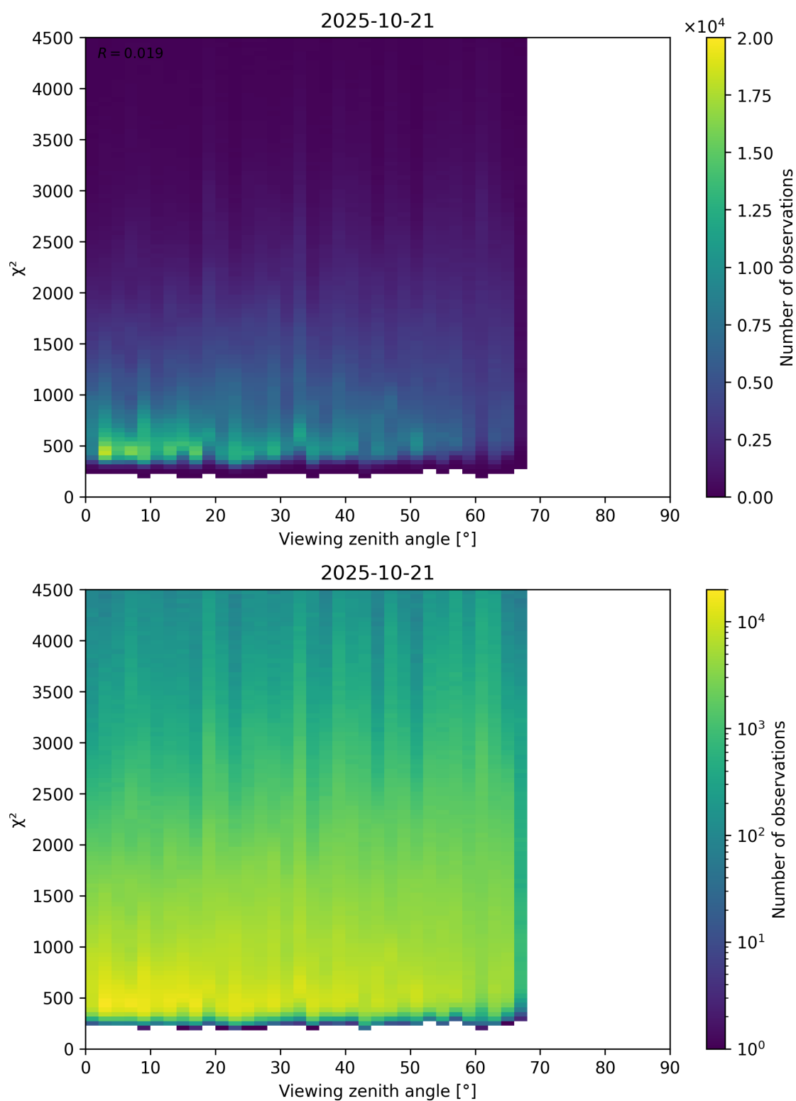
Figure 72: Scatter density plot of “Viewing zenith angle” against “ \chi^2 ” for 2025-10-20 to 2025-10-22.
