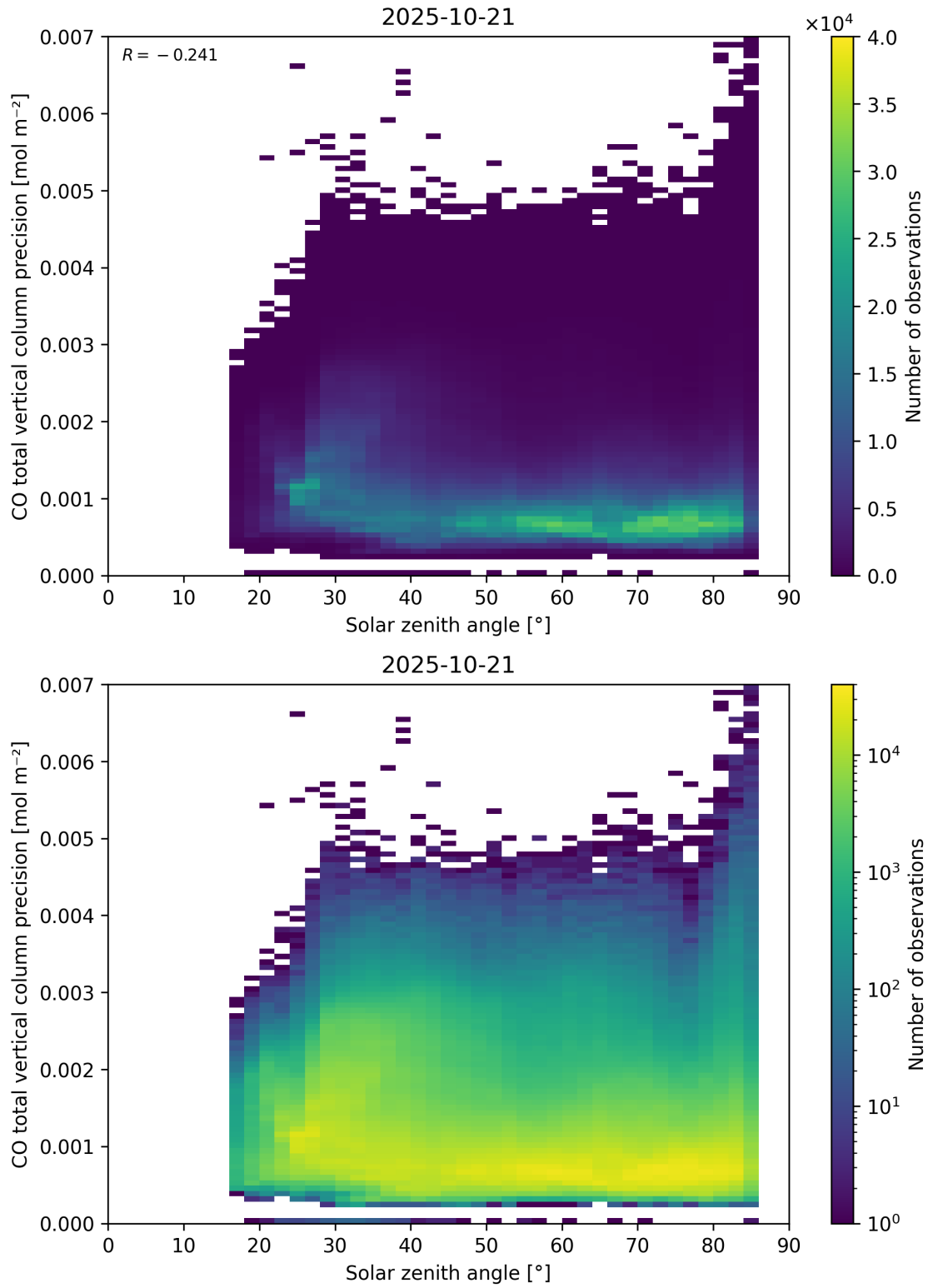
Figure 63: Scatter density plot of “Solar zenith angle” against “CO total vertical column precision” for 2025-10-20 to 2025-10-22.
