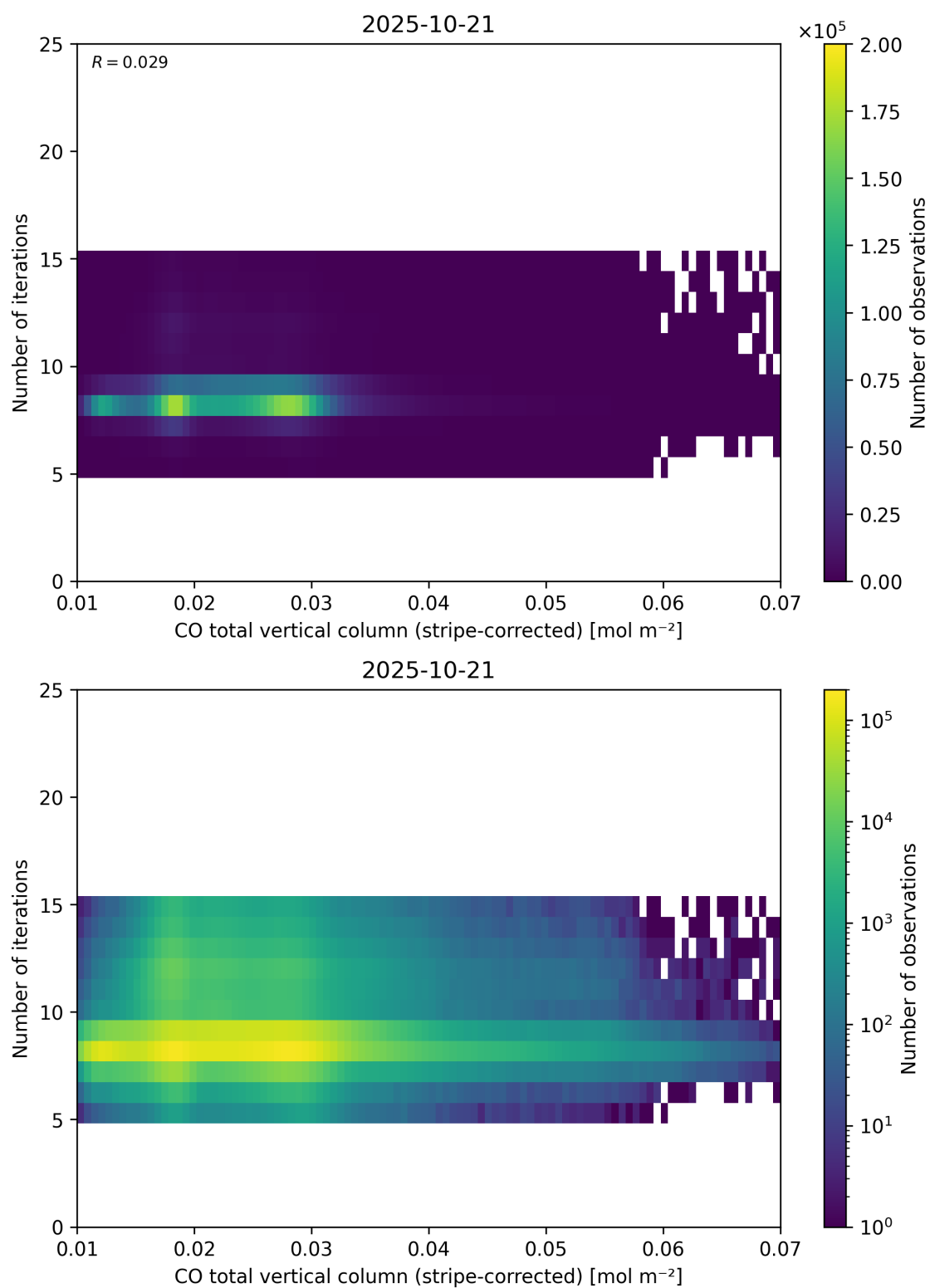
Figure 39: Scatter density plot of “CO total vertical column (stripe-corrected)” against “Number of iterations” for 2025-10-20 to 2025-10-22.
