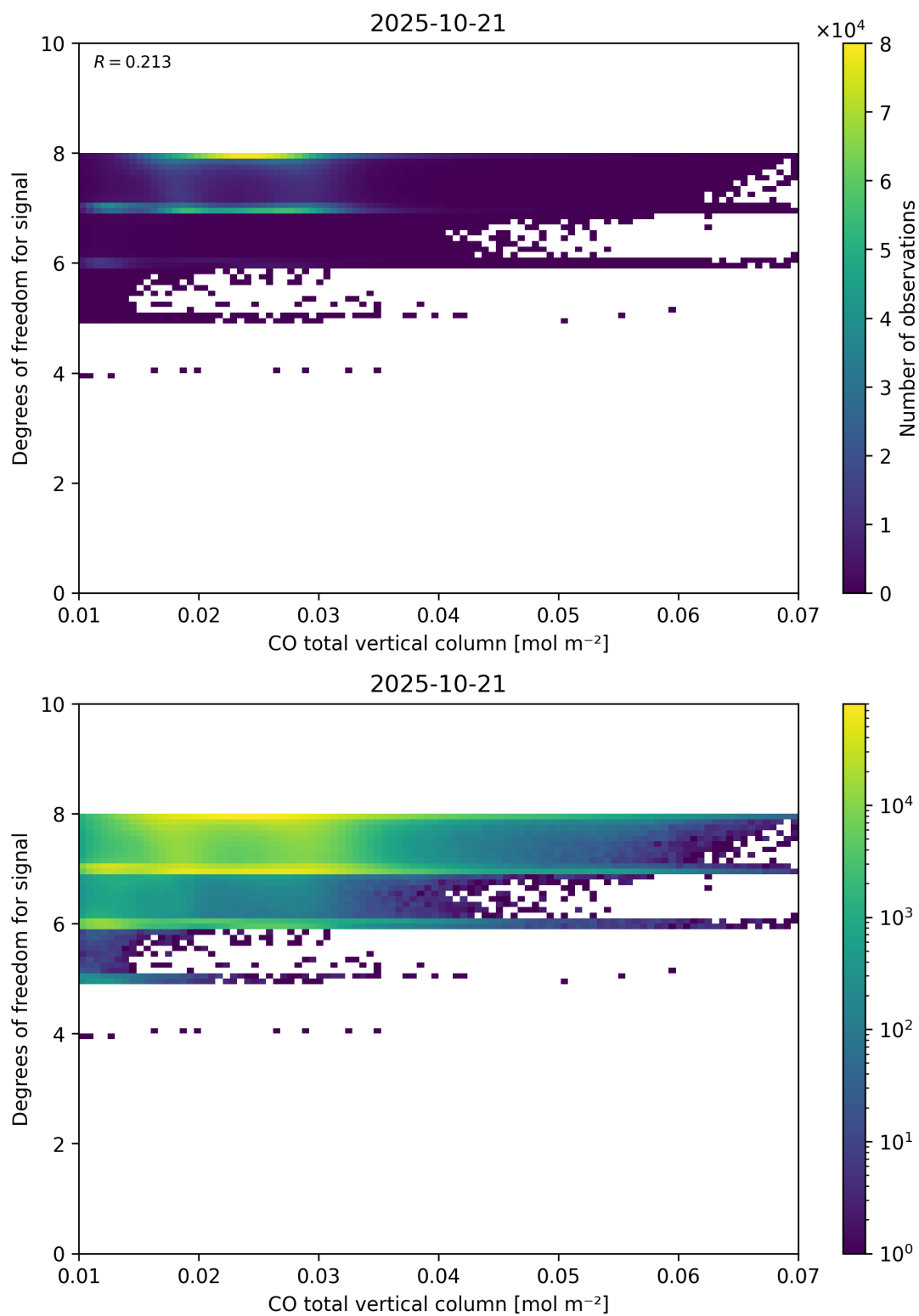
Figure 41: Scatter density plot of “CO total vertical column” against “Degrees of freedom for signal” for 2025-10-20 to 2025-10-22.
