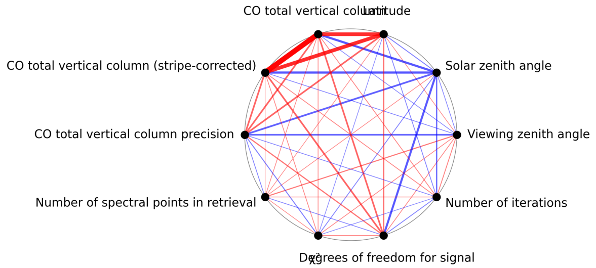
Figure 1: Map of correlation graph for 2025-10-20 to 2025-10-22.
