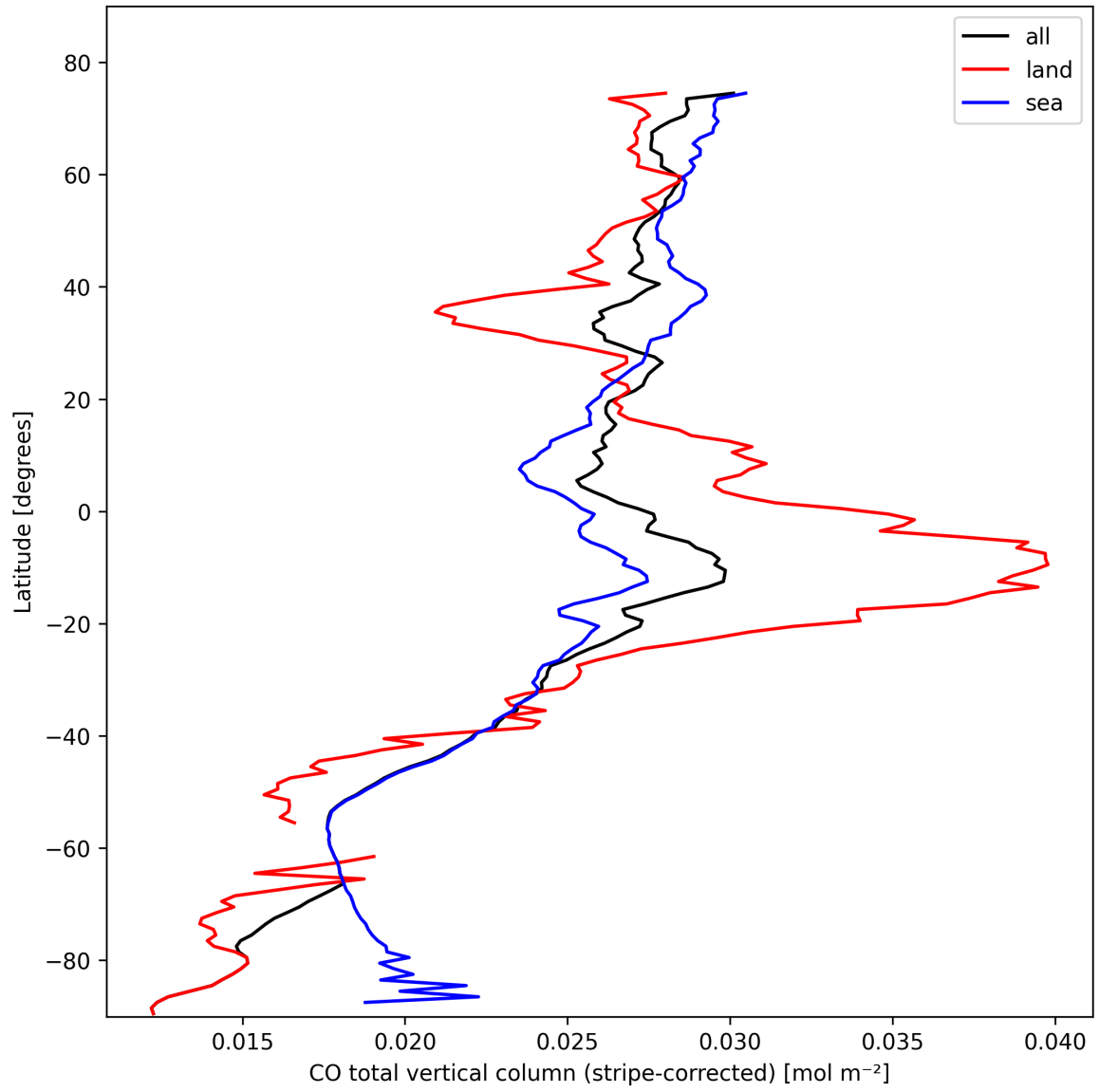
Figure 11: Zonal average of “CO total vertical column (stripe-corrected)” for 2025-10-20 to 2025-10-22.
