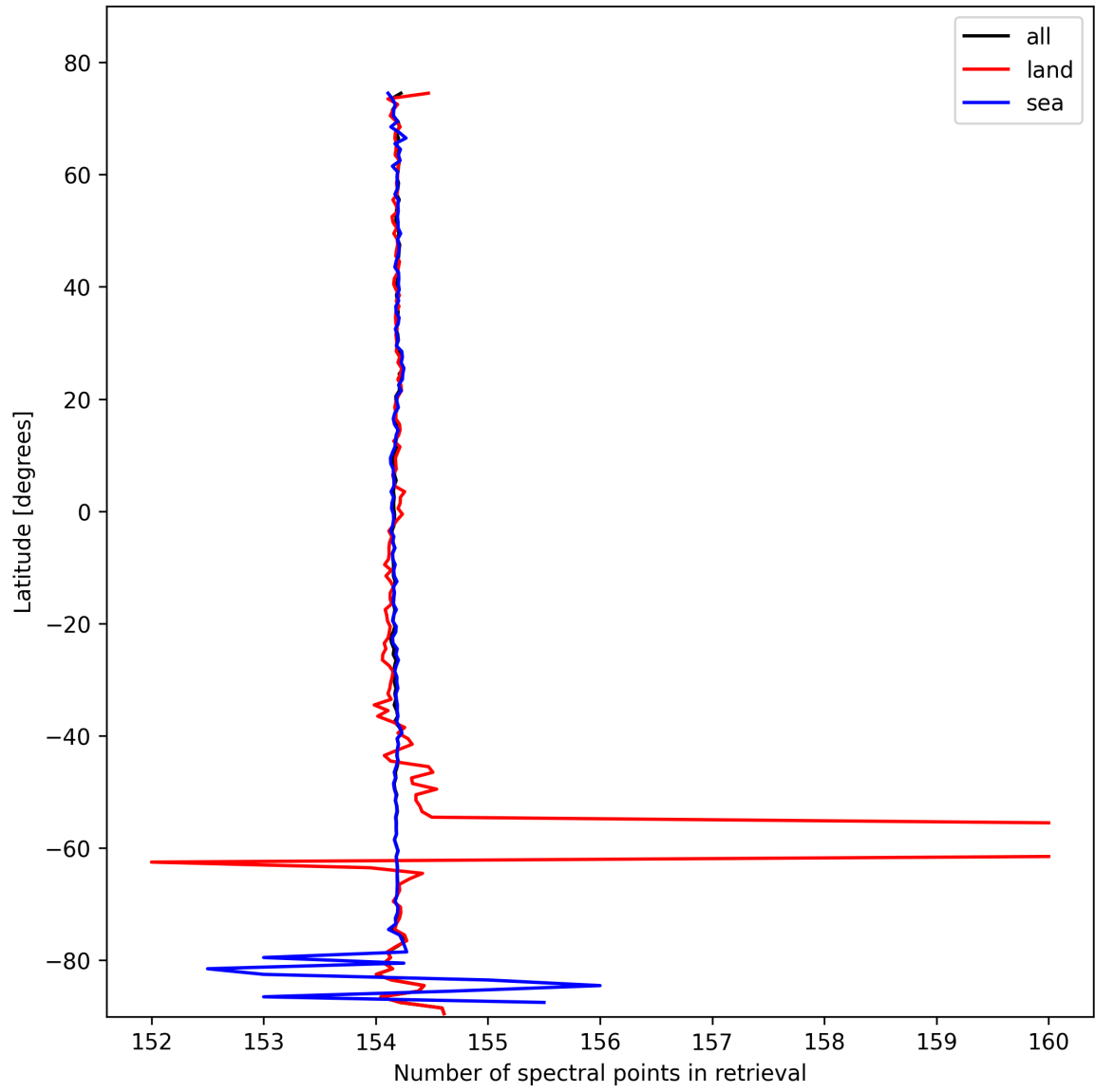
Figure 13: Zonal average of “Number of spectral points in retrieval” for 2025-10-20 to 2025-10-22.
