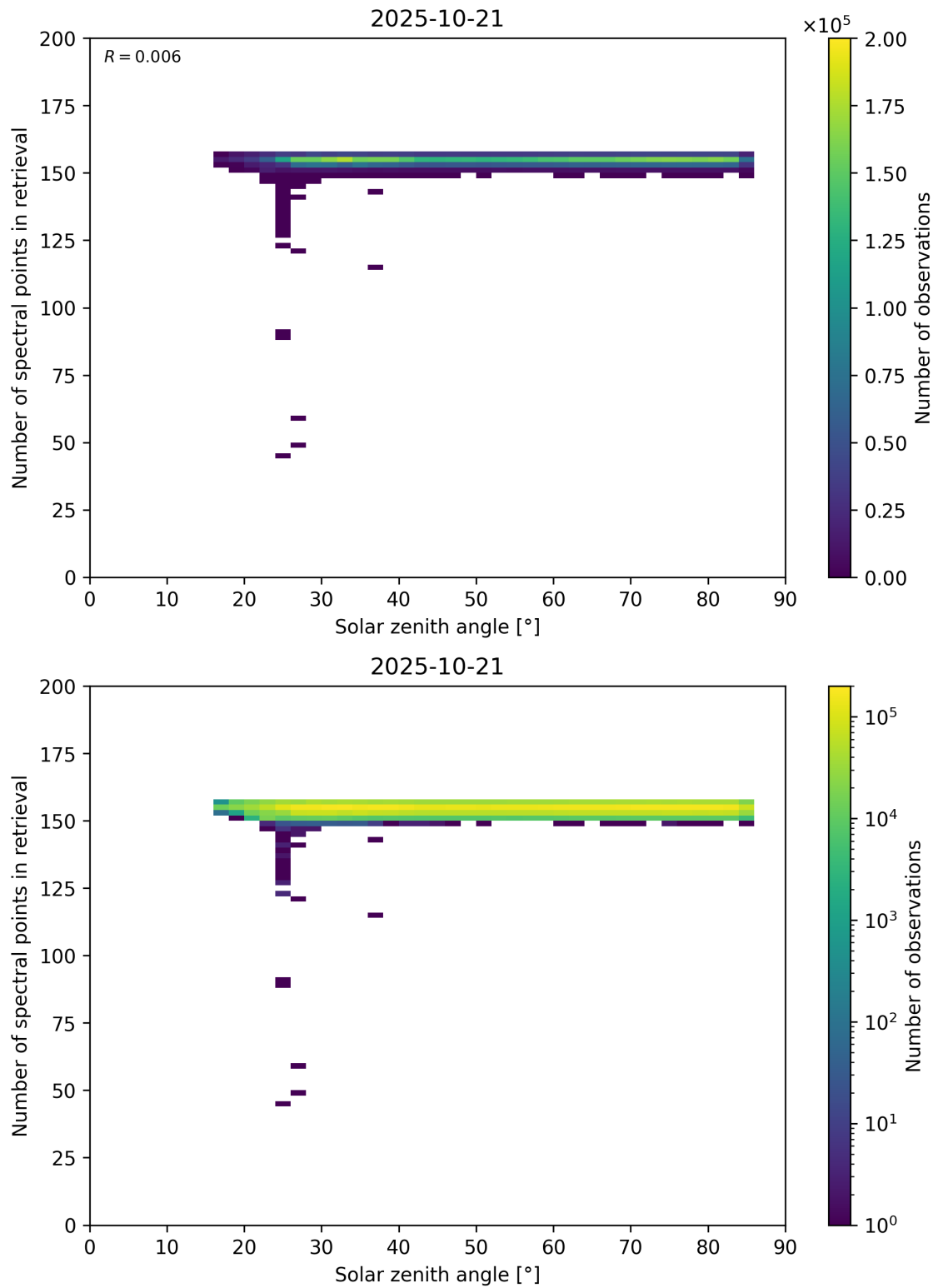
Figure 68: Scatter density plot of “Solar zenith angle” against “Number of spectral points in retrieval” for 2025-10-20 to 2025-10-22.
