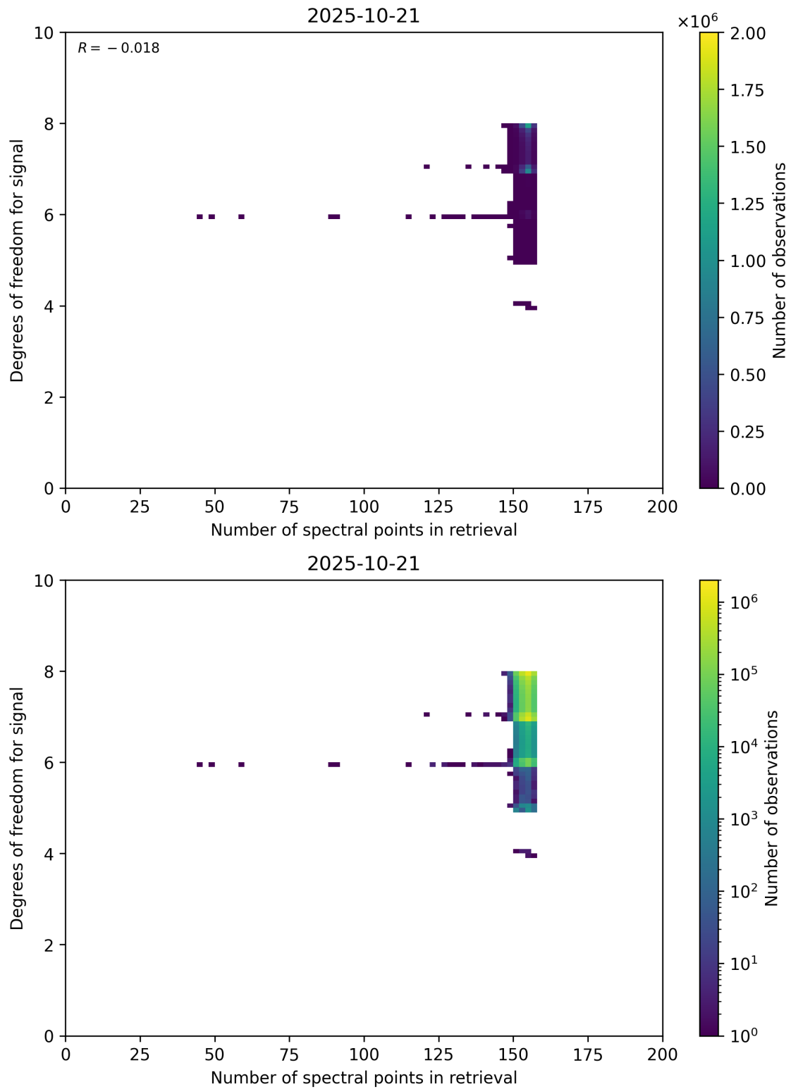
Figure 59: Scatter density plot of “Number of spectral points in retrieval” against “Degrees of freedom for signal” for 2025-10-20 to 2025-10-22.
