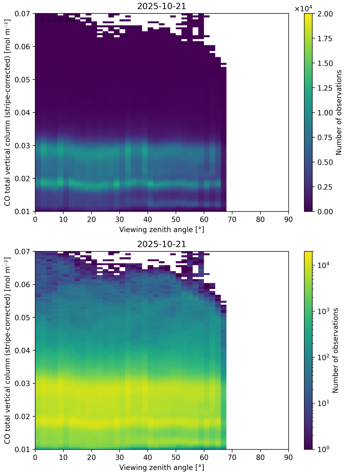
Figure 70: Scatter density plot of “Viewing zenith angle” against “CO total vertical column (stripe-corrected)” for 2025-10-20 to 2025-10-22.
