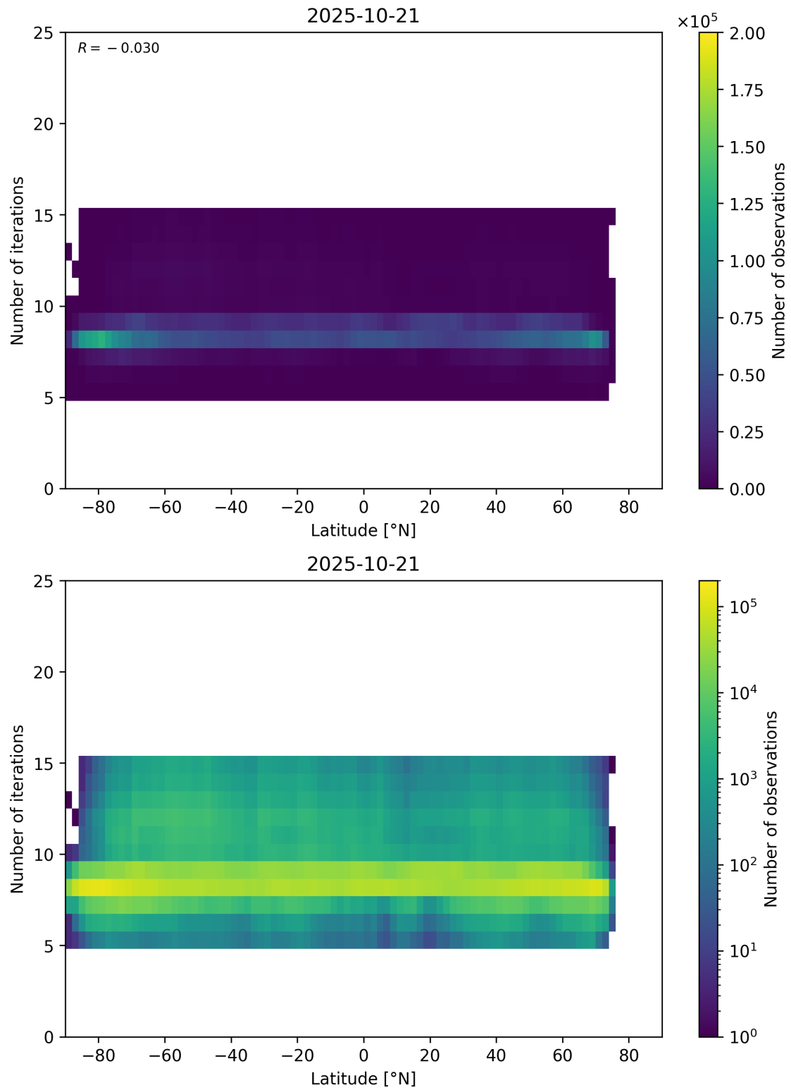
Figure 56: Scatter density plot of “Latitude” against “Number of iterations” for 2025-10-20 to 2025-10-22.
