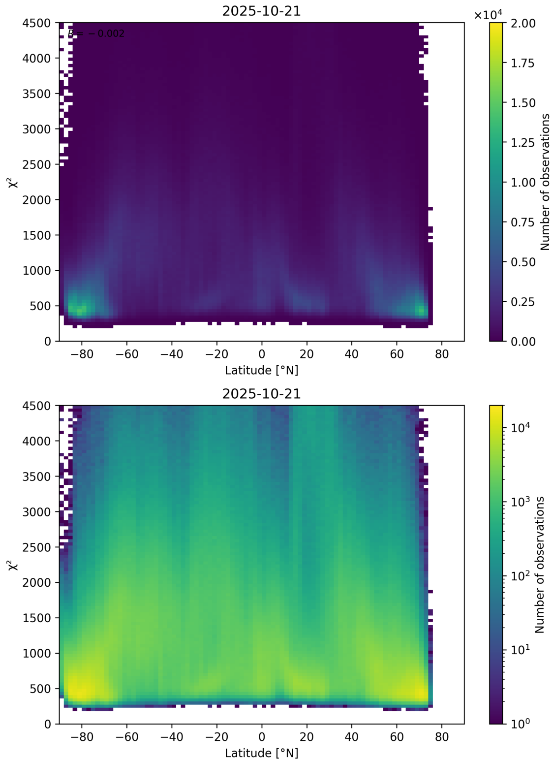
Figure 54: Scatter density plot of “Latitude” against “ \chi^2 ” for 2025-10-20 to 2025-10-22.
