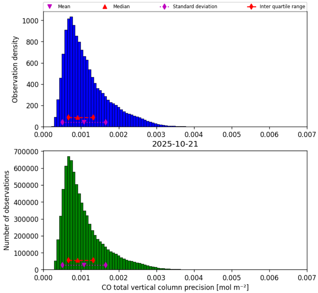
Figure 20: Histogram of “CO total vertical column precision” for 2025-10-20 to 2025-10-22
