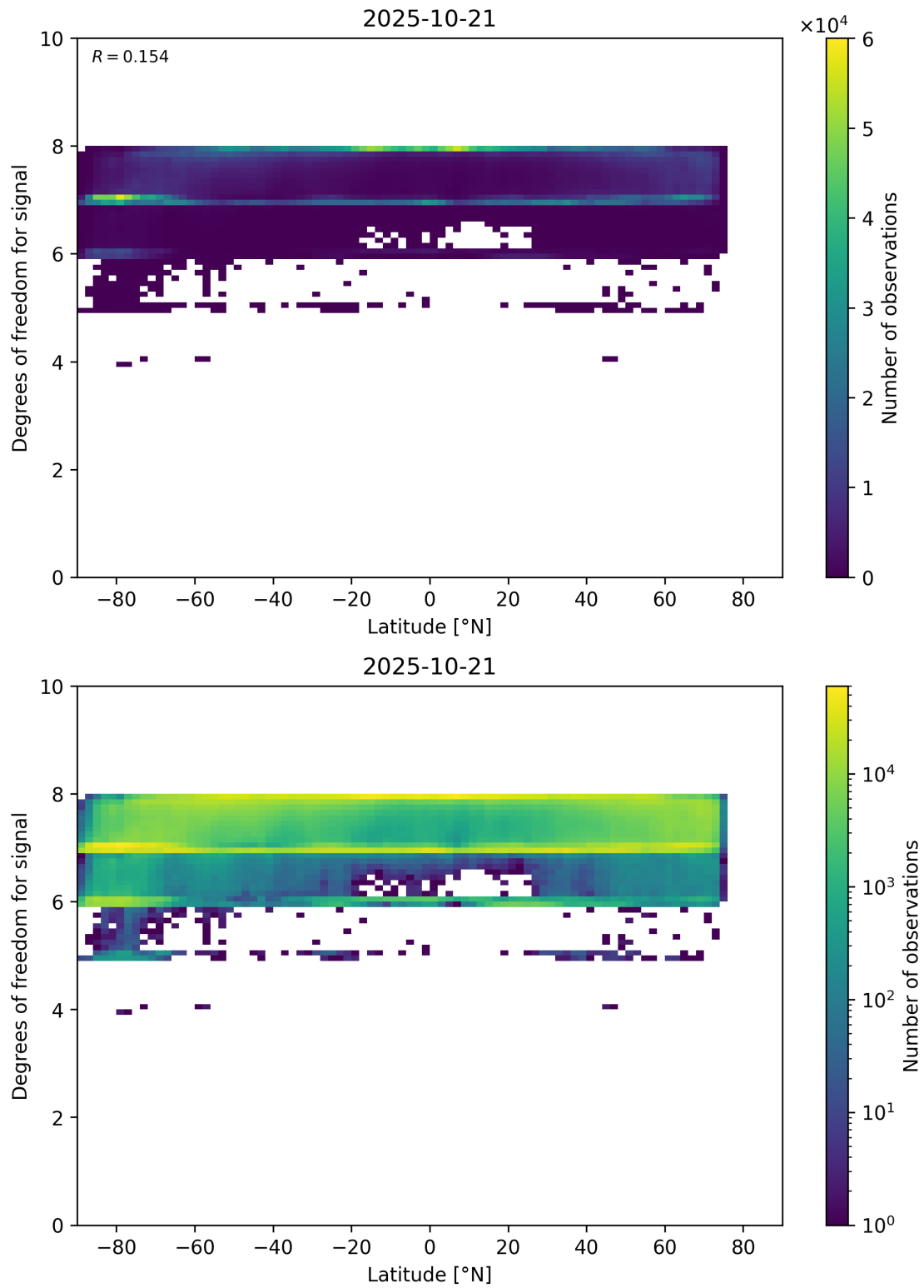
Figure 55: Scatter density plot of “Latitude” against “Degrees of freedom for signal” for 2025-10-20 to 2025-10-22.
