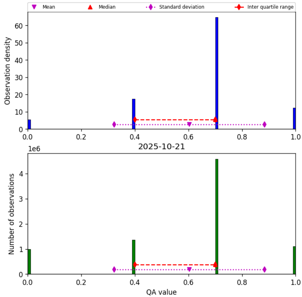
Figure 17: Histogram of “QA value” for 2025-10-20 to 2025-10-22
