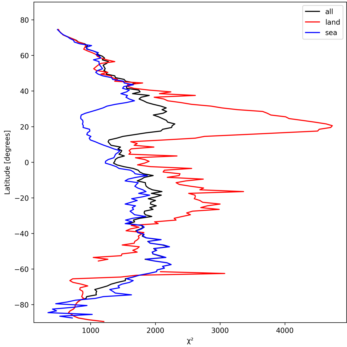
Figure 14: Zonal average of “ \chi^2 ” for 2025-10-20 to 2025-10-22.
