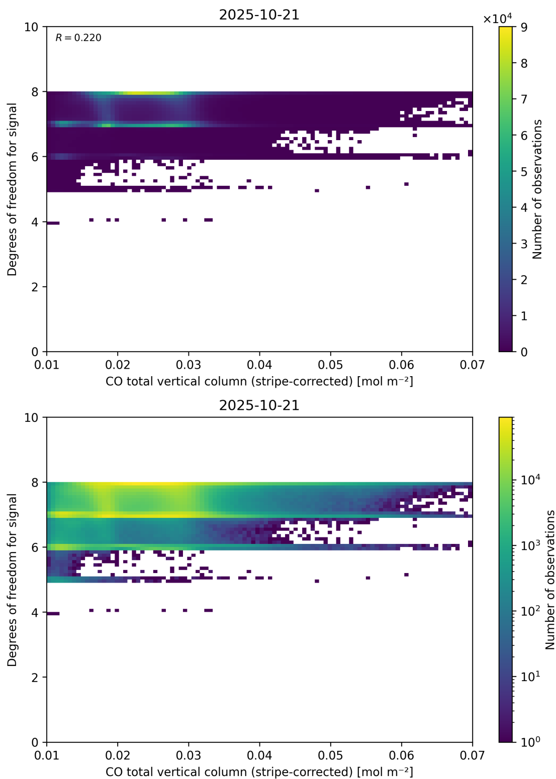
Figure 38: Scatter density plot of “CO total vertical column (stripe-corrected)” against “Degrees of freedom for signal” for 2025-10-20 to 2025-10-22.
