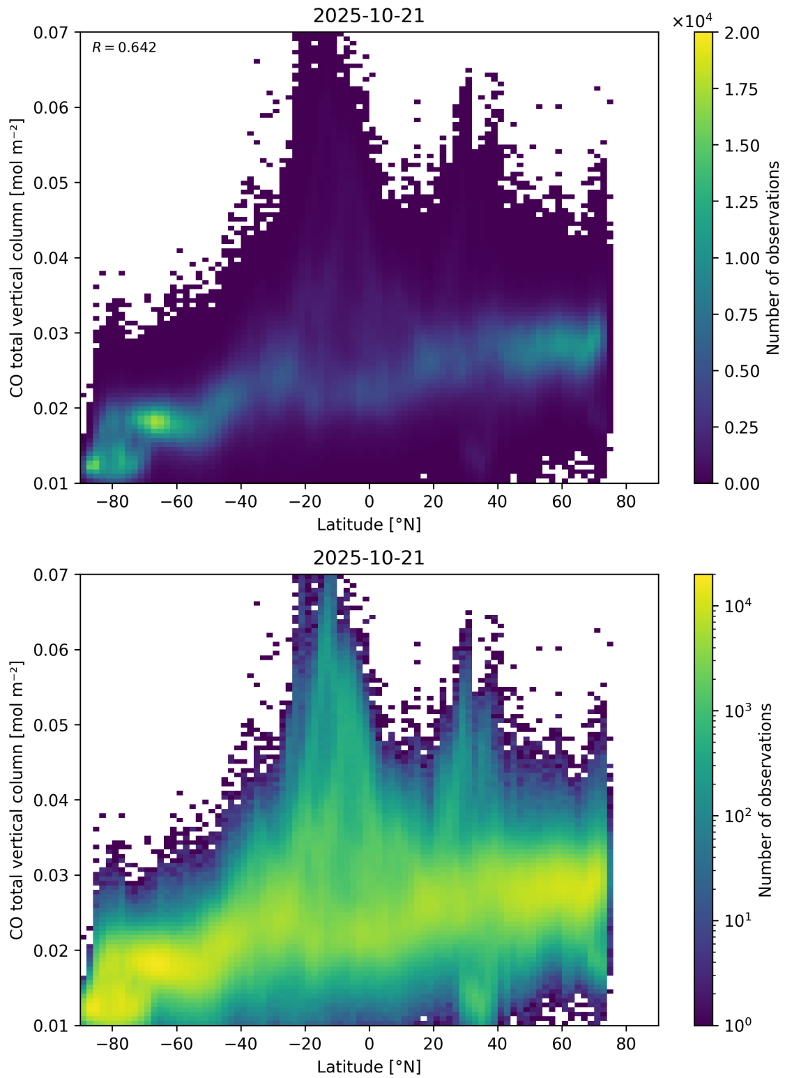
Figure 51: Scatter density plot of “Latitude” against “CO total vertical column” for 2025-10-20 to 2025-10-22.
