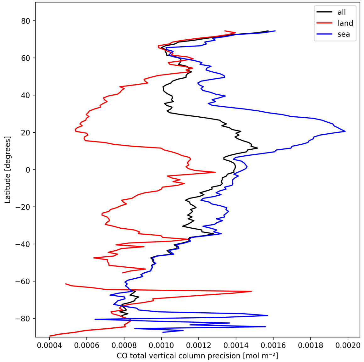
Figure 12: Zonal average of “CO total vertical column precision” for 2025-10-20 to 2025-10-22.
