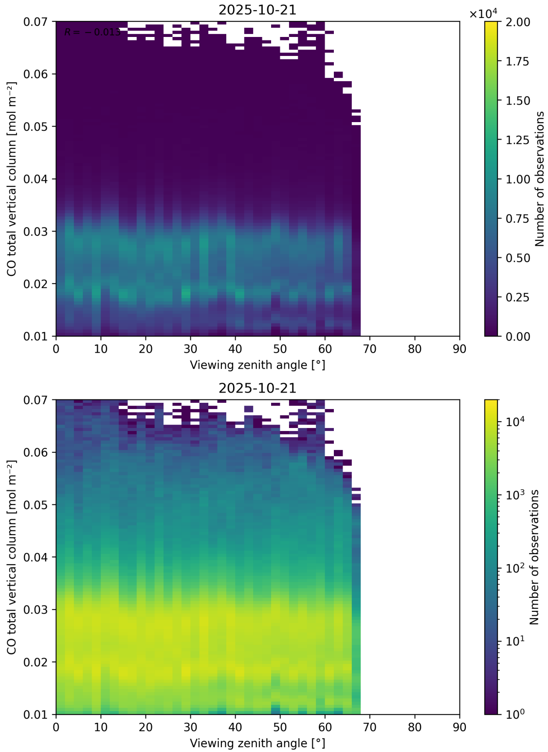
Figure 69: Scatter density plot of “Viewing zenith angle” against “CO total vertical column” for 2025-10-20 to 2025-10-22.
