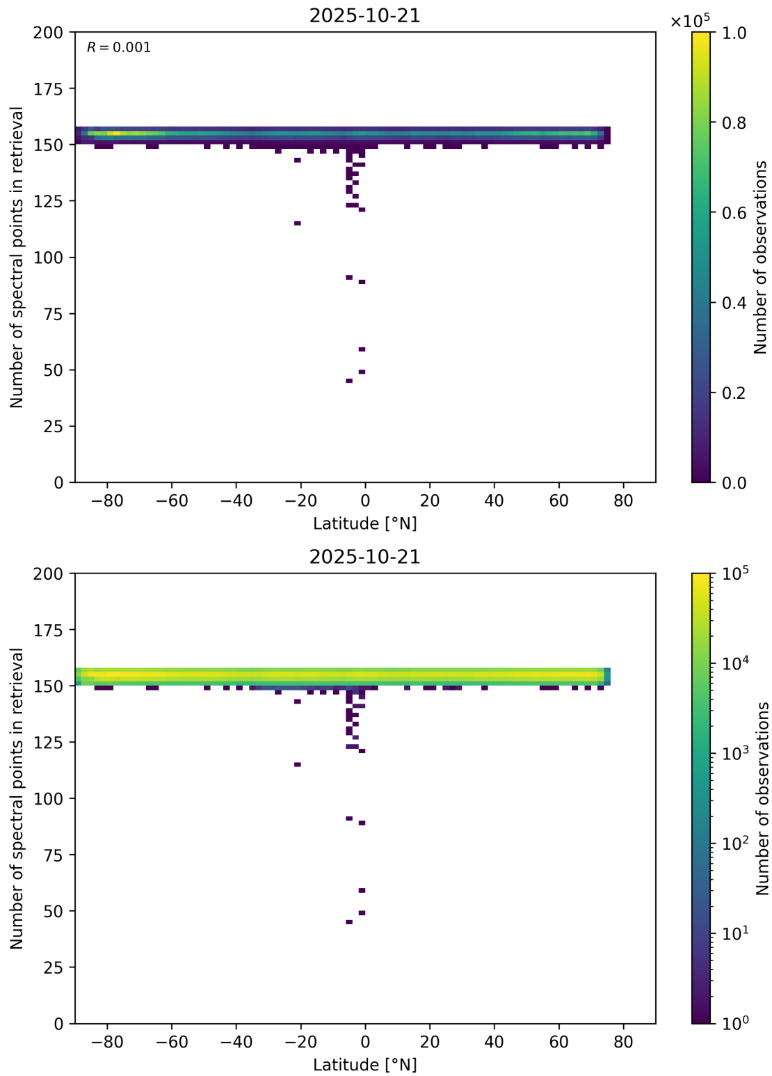
Figure 57: Scatter density plot of “Latitude” against “Number of spectral points in retrieval” for 2025-10-20 to 2025-10-22.
