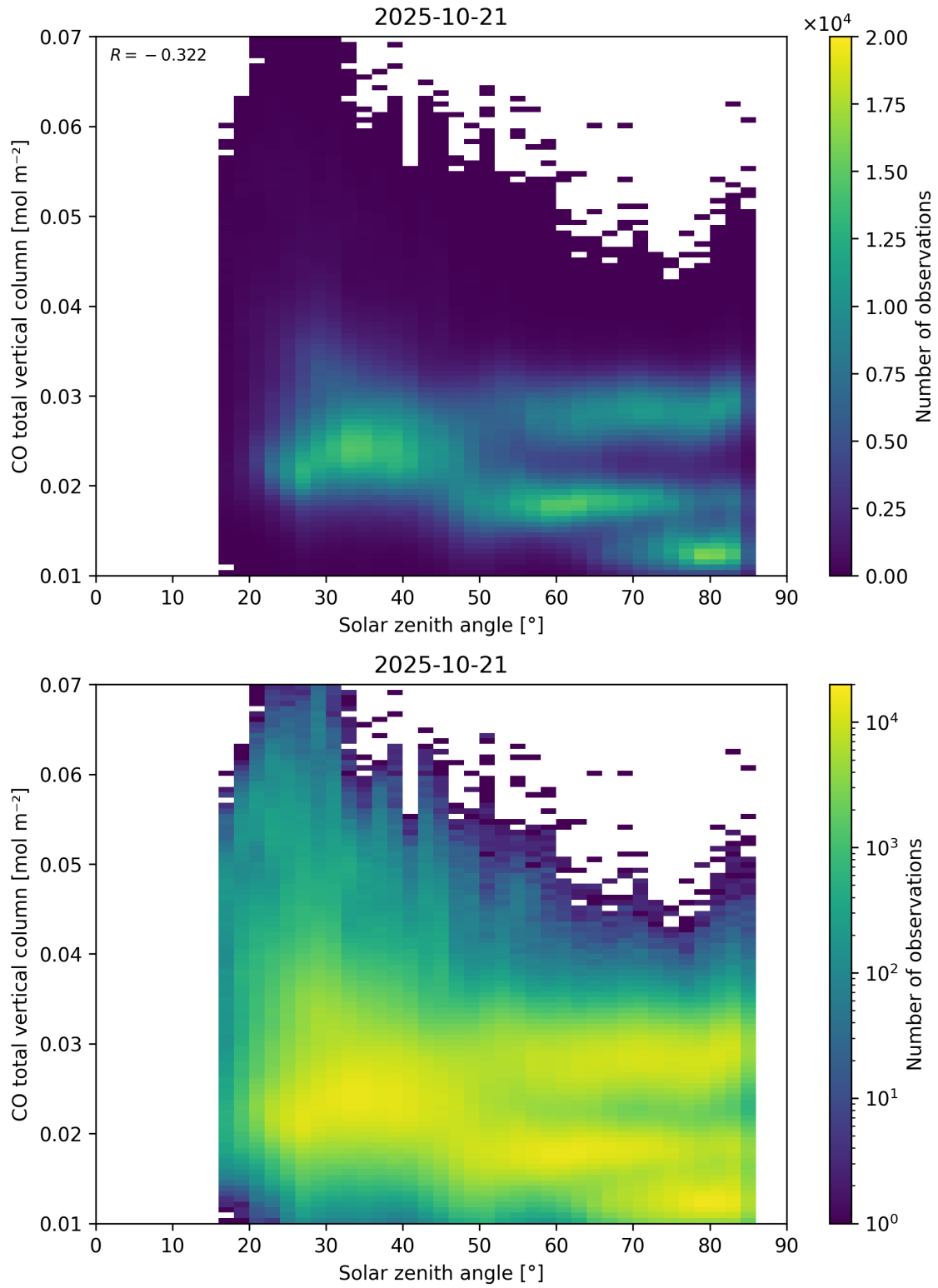
Figure 61: Scatter density plot of “Solar zenith angle” against “CO total vertical column” for 2025-10-20 to 2025-10-22.
