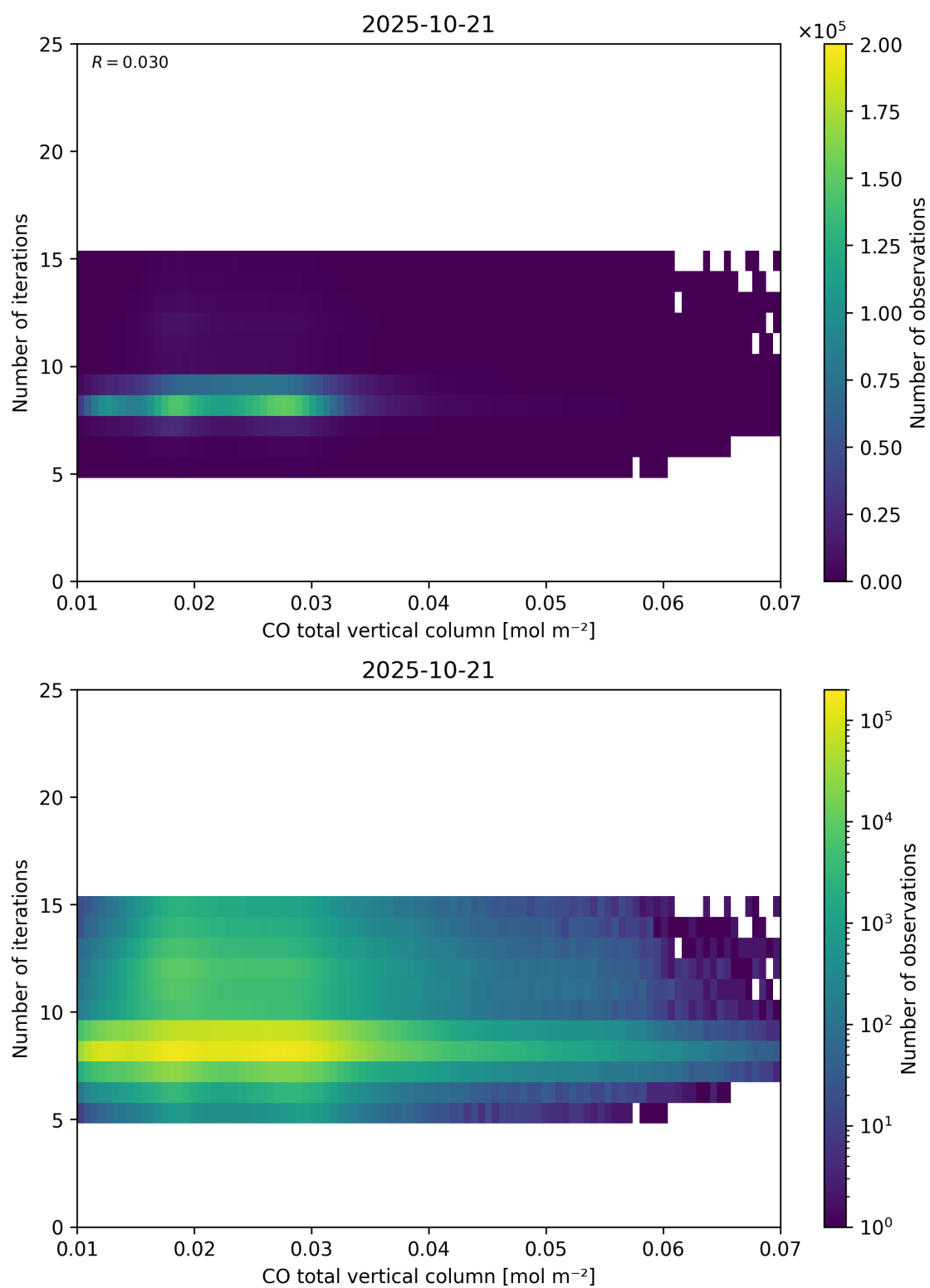
Figure 42: Scatter density plot of “CO total vertical column” against “Number of iterations” for 2025-10-20 to 2025-10-22.
