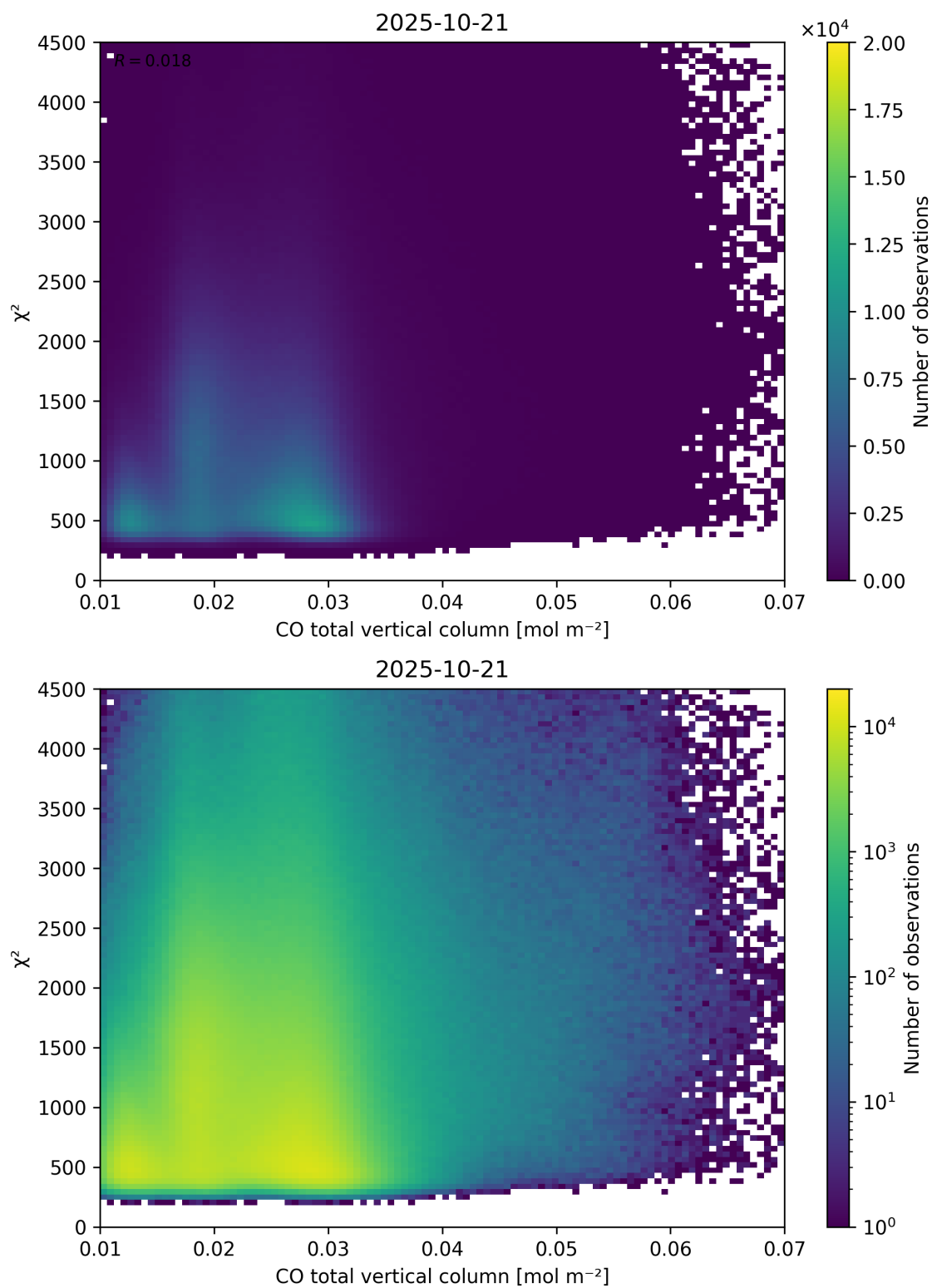
Figure 35: Scatter density plot of “CO total vertical column” against “ \chi^2 ” for 2025-10-20 to 2025-10-22.
