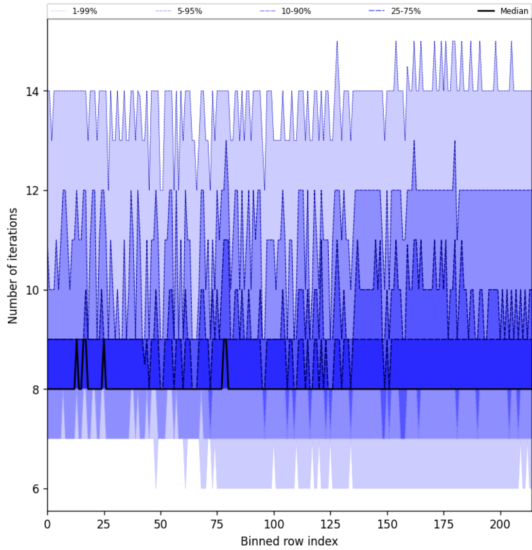
Figure 32: Along track statistics of “Number of iterations” for 2025-10-20 to 2025-10-22
