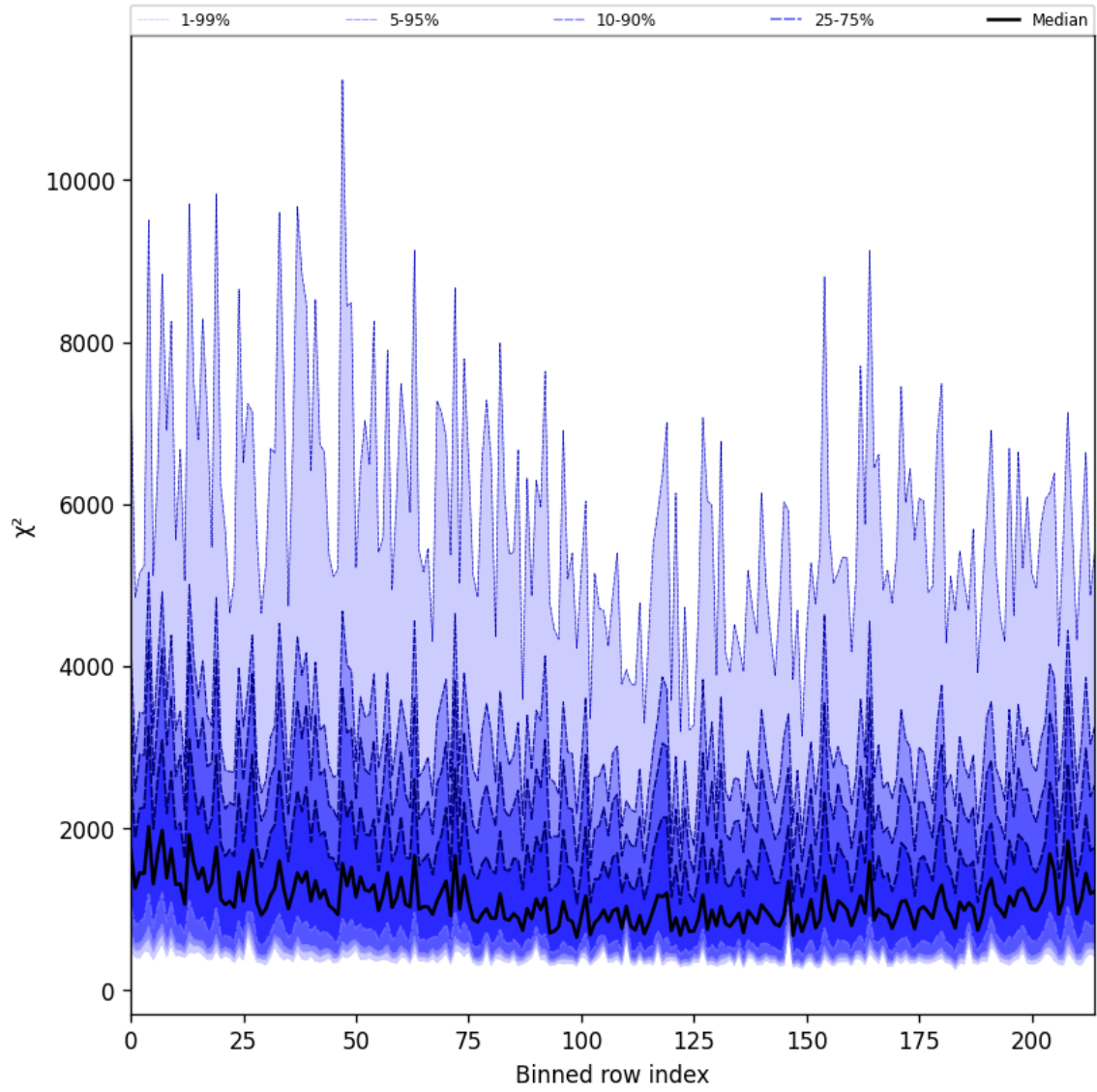
Figure 30: Along track statistics of “ \chi^2 ” for 2025-10-20 to 2025-10-22
