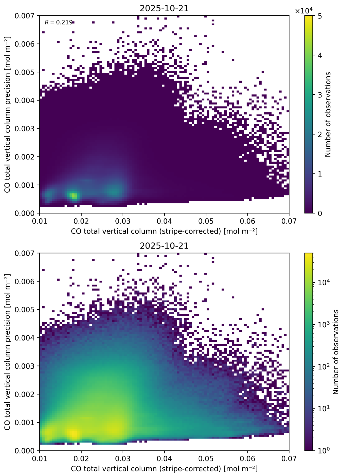
Figure 36: Scatter density plot of “CO total vertical column (stripe-corrected)” against “CO total vertical column precision” for 2025-10-20 to 2025-10-22.
