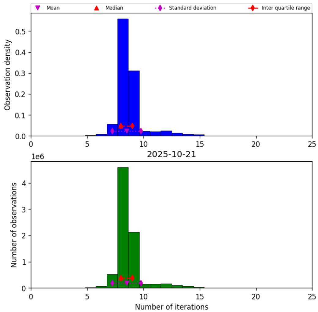
Figure 24: Histogram of “Number of iterations” for 2025-10-20 to 2025-10-22
