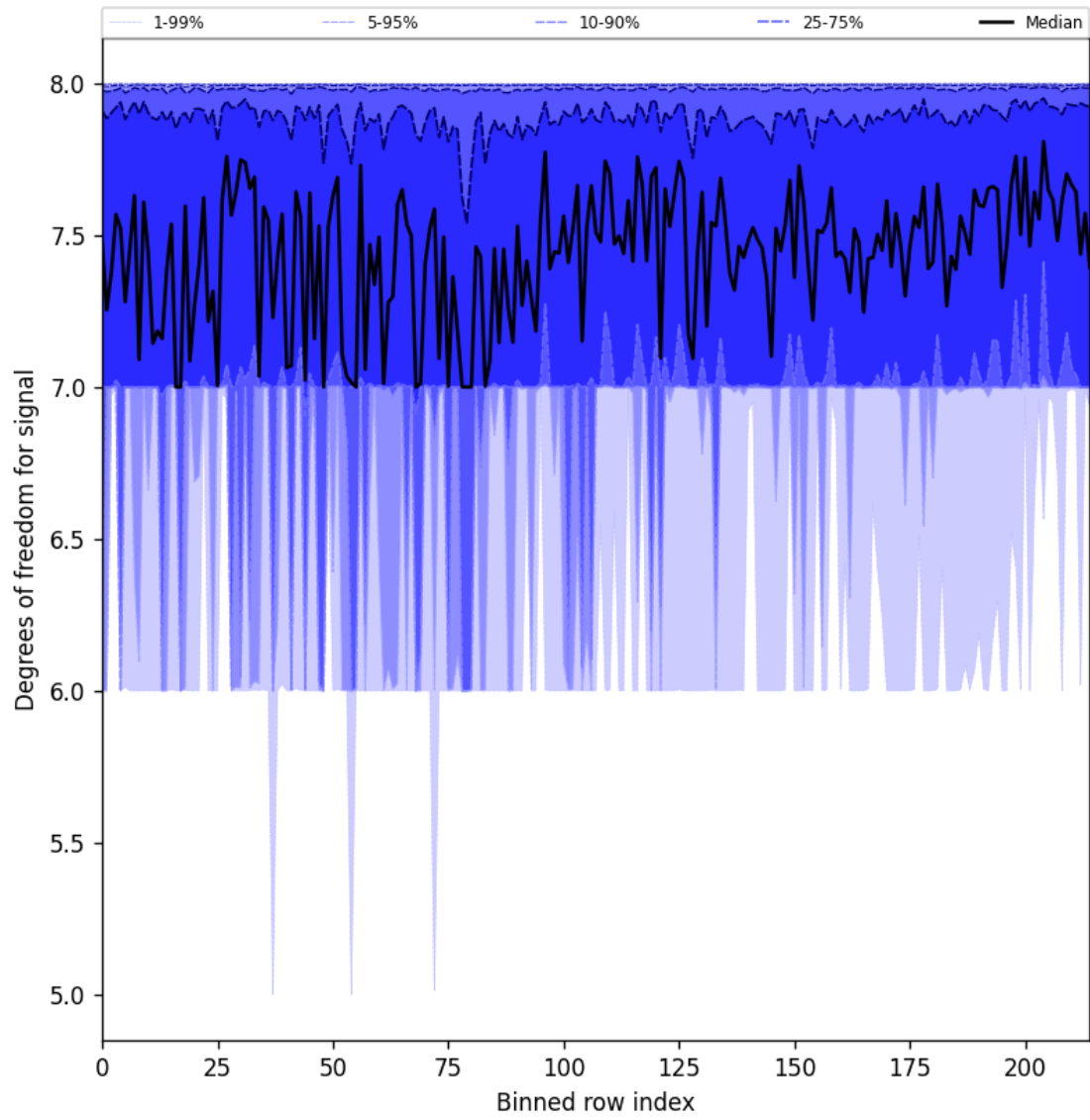
Figure 31: Along track statistics of “Degrees of freedom for signal” for 2025-10-20 to 2025-10-22
