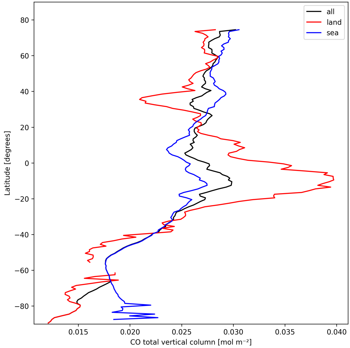
Figure 10: Zonal average of “CO total vertical column” for 2025-10-20 to 2025-10-22.
