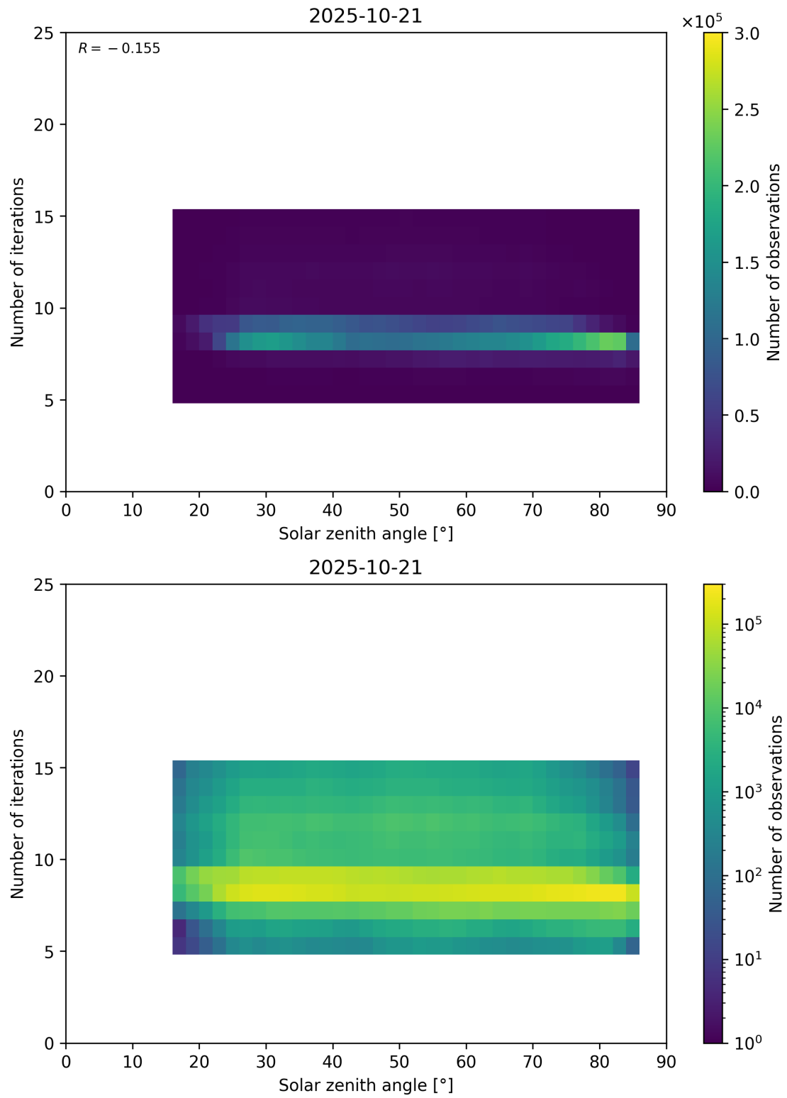
Figure 67: Scatter density plot of “Solar zenith angle” against “Number of iterations” for 2025-10-20 to 2025-10-22.
