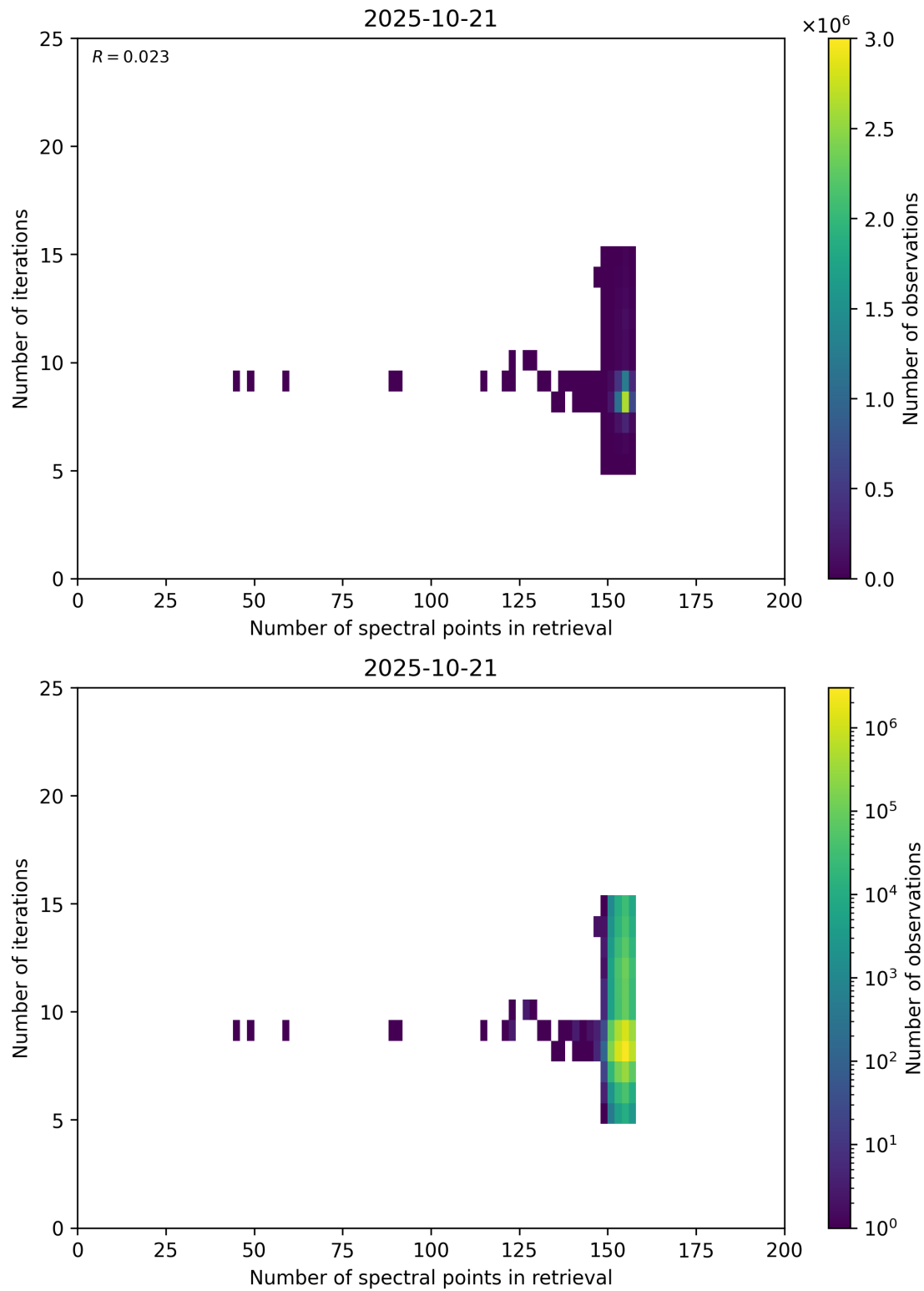
Figure 60: Scatter density plot of “Number of spectral points in retrieval” against “Number of iterations” for 2025-10-20 to 2025-10-22.
