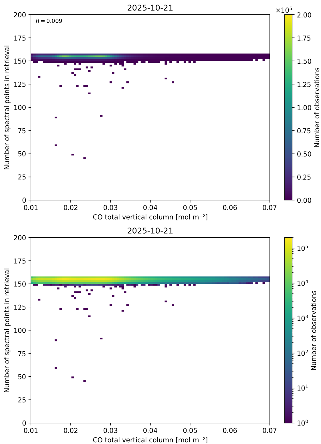
Figure 43: Scatter density plot of “CO total vertical column” against “Number of spectral points in retrieval” for 2025-10-20 to 2025-10-22.
