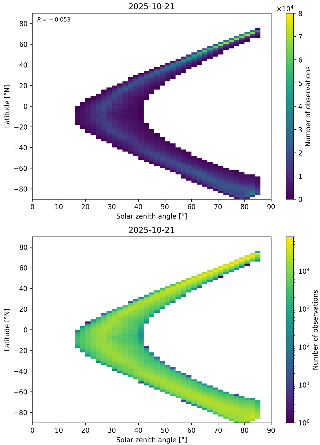
Figure 66: Scatter density plot of “Solar zenith angle” against “Latitude” for 2025-10-20 to 2025-10-22.
