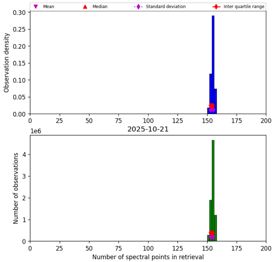
Figure 21: Histogram of “Number of spectral points in retrieval” for 2025-10-20 to 2025-10-22
