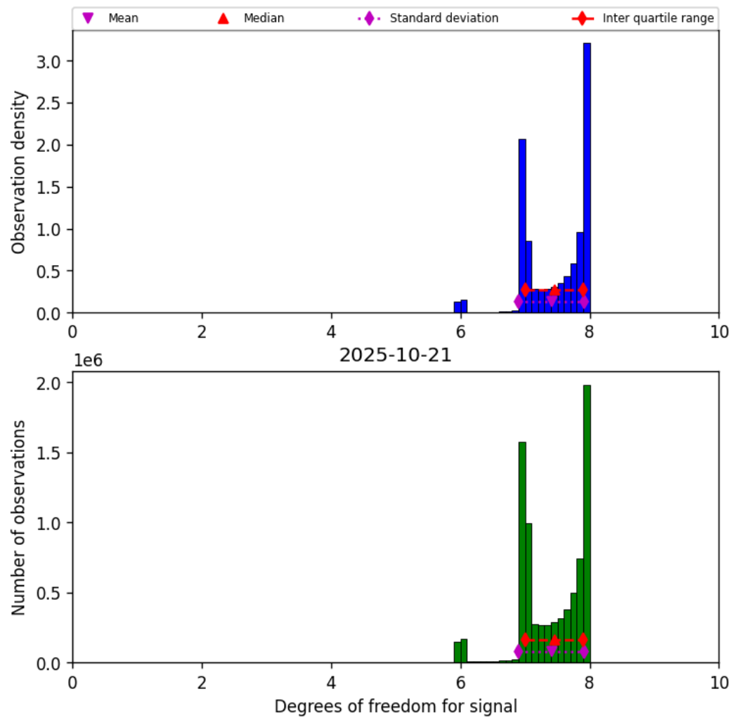
Figure 23: Histogram of “Degrees of freedom for signal” for 2025-10-20 to 2025-10-22
