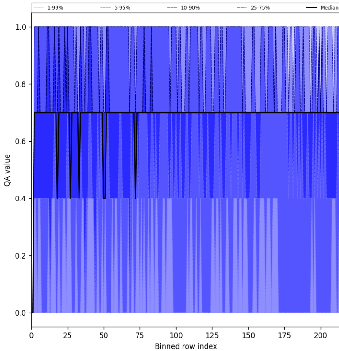
Figure 25: Along track statistics of “QA value” for 2025-10-20 to 2025-10-22
