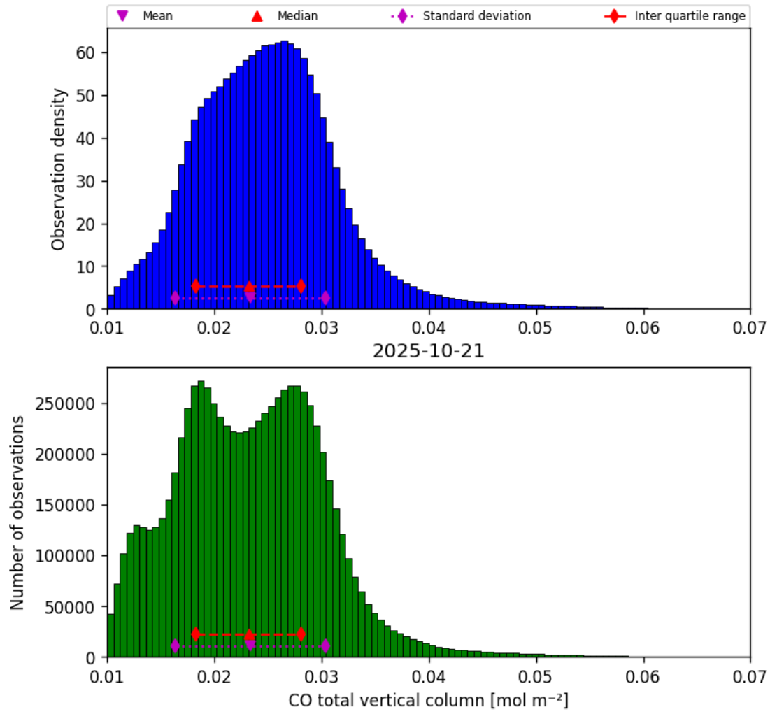
Figure 18: Histogram of “CO total vertical column” for 2025-10-20 to 2025-10-22
