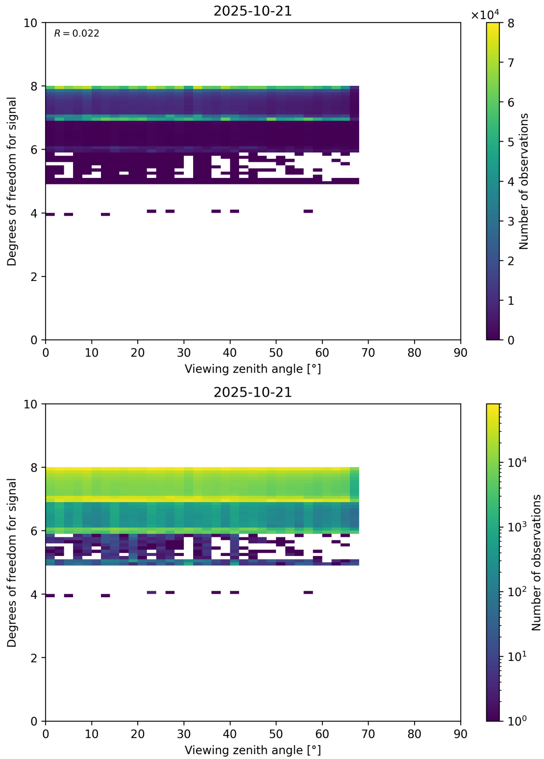
Figure 73: Scatter density plot of “Viewing zenith angle” against “Degrees of freedom for signal” for 2025-10-20 to 2025-10-22.
