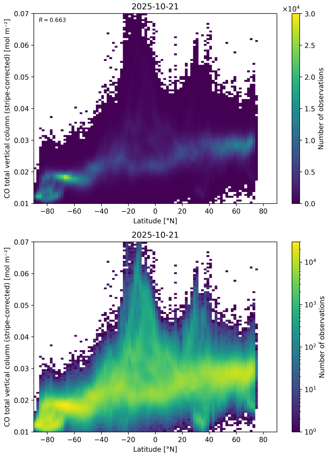
Figure 52: Scatter density plot of “Latitude” against “CO total vertical column (stripe-corrected)” for 2025-10-20 to 2025-10-22.
