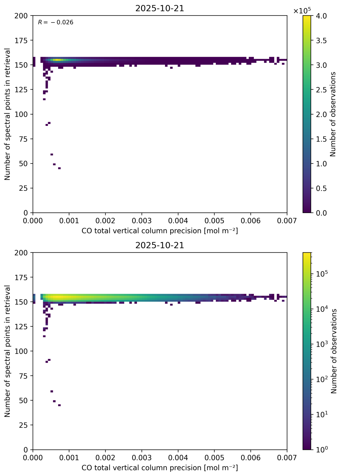
Figure 47: Scatter density plot of “CO total vertical column precision” against “Number of spectral points in retrieval” for 2025-10-20 to 2025-10-22.
