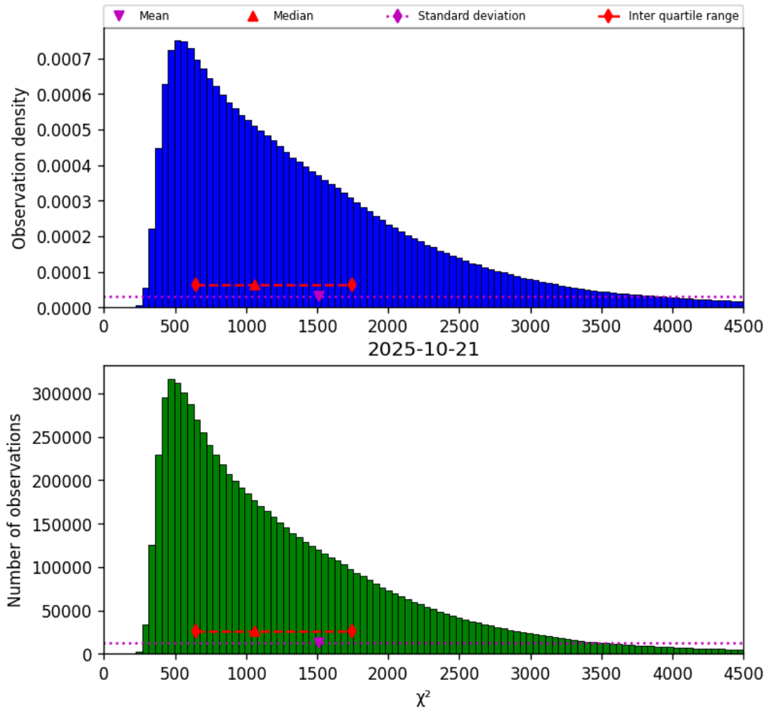
Figure 22: Histogram of “ \chi^2 ” for 2025-10-20 to 2025-10-22
