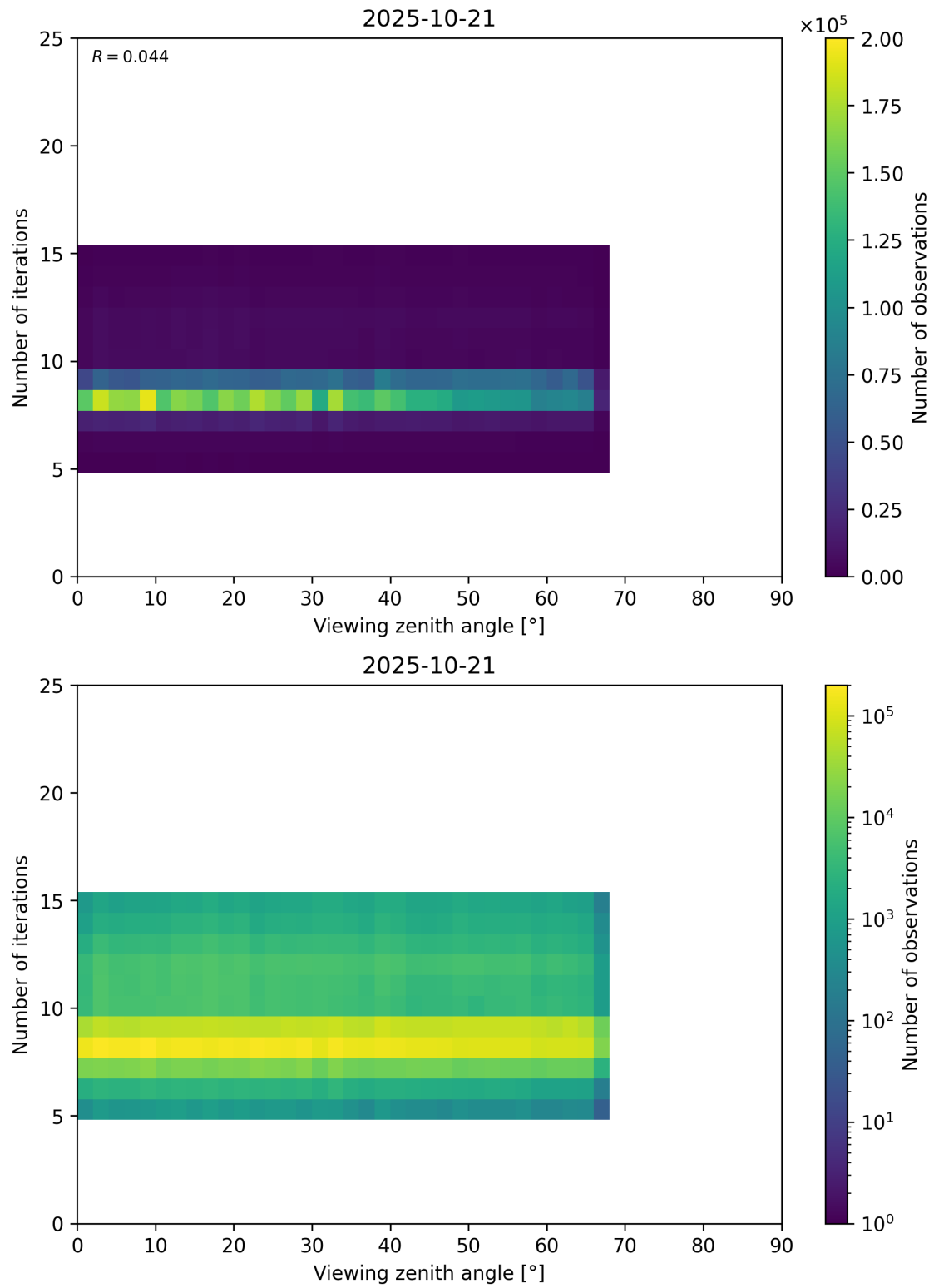
Figure 75: Scatter density plot of “Viewing zenith angle” against “Number of iterations” for 2025-10-20 to 2025-10-22.
