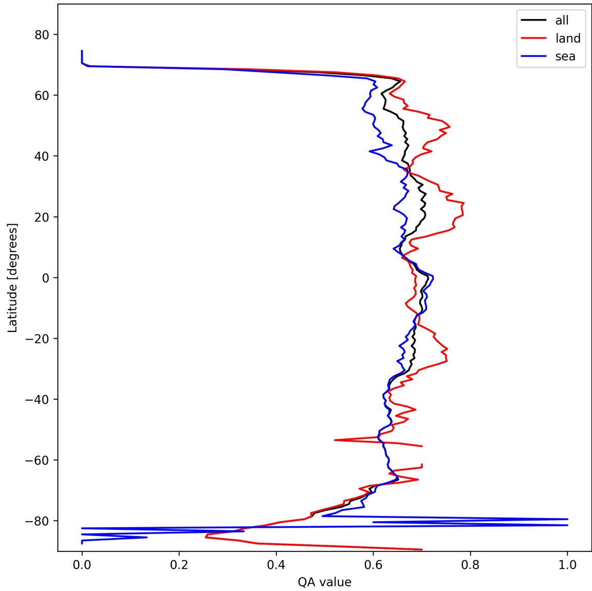
Figure 9: Zonal average of “QA value” for 2025-10-20 to 2025-10-22.
