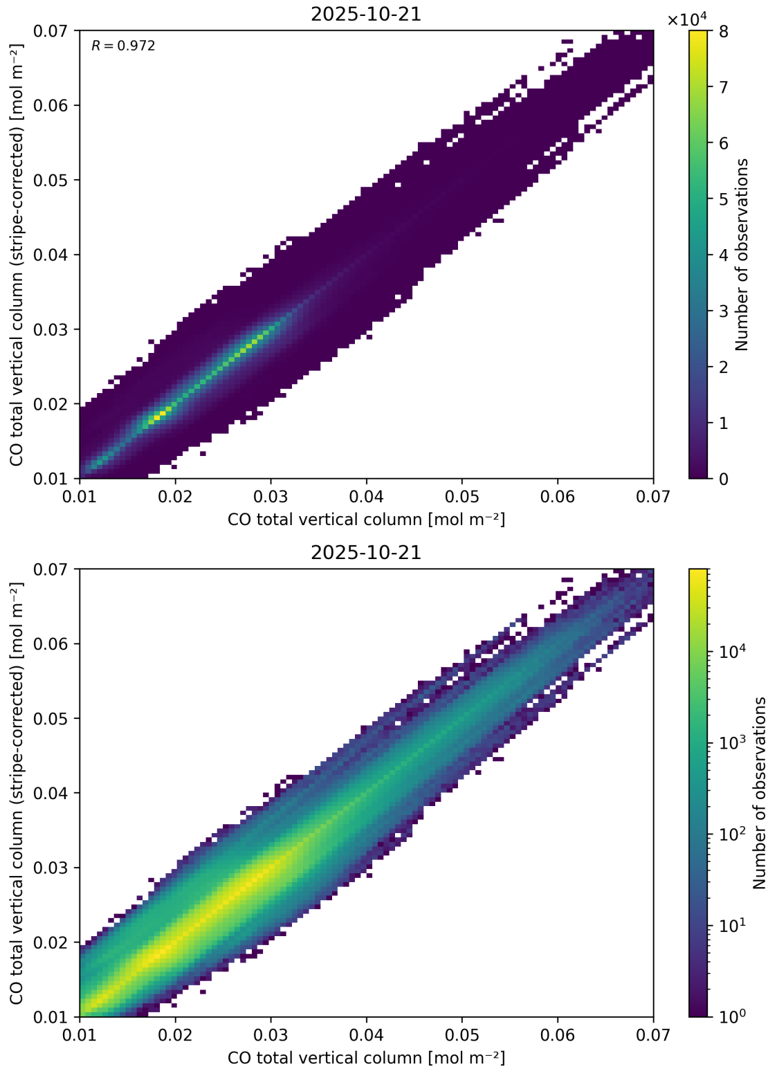
Figure 33: Scatter density plot of “CO total vertical column” against “CO total vertical column (stripe-corrected)” for 2025-10-20 to 2025-10-22.
