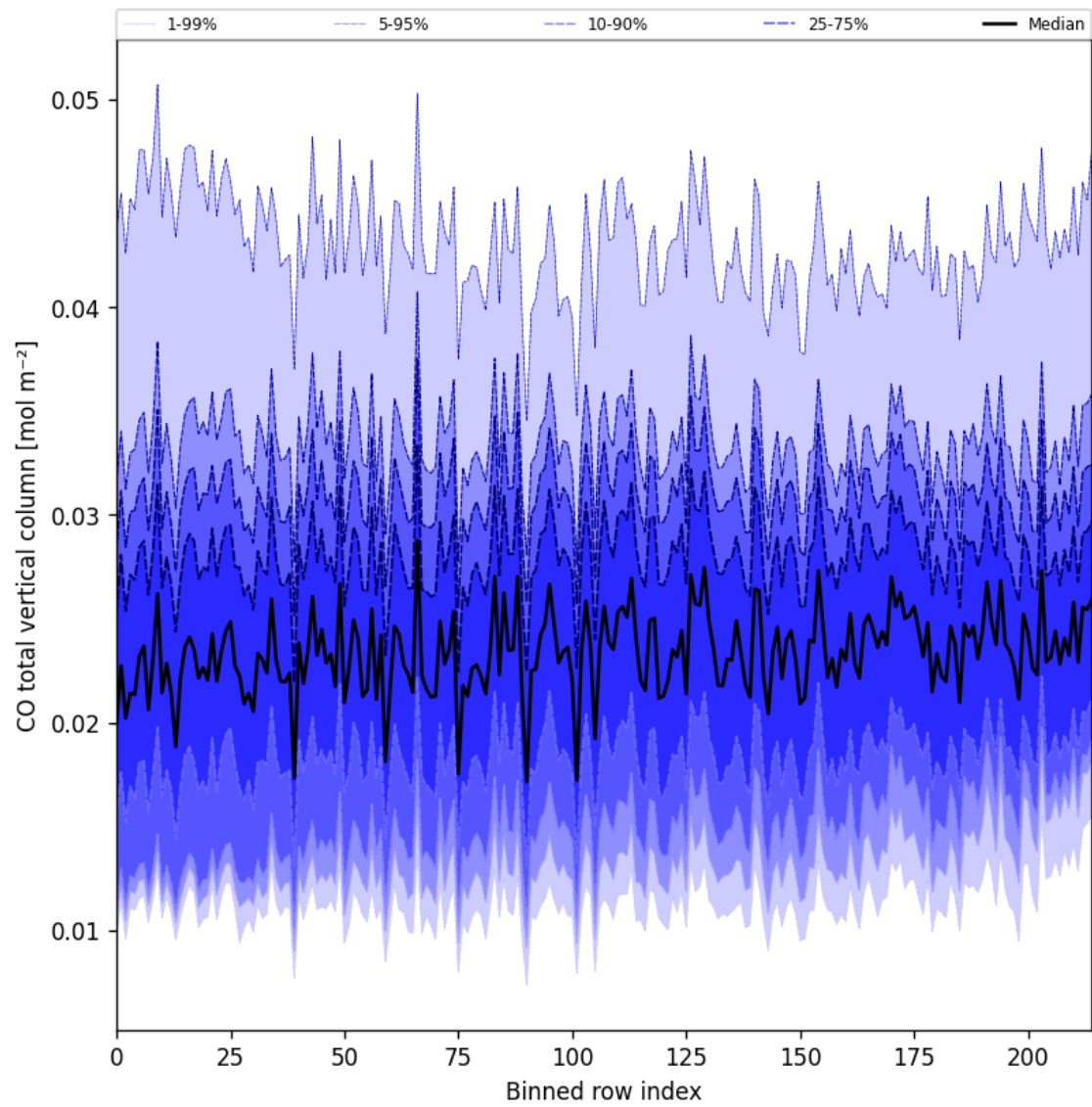
Figure 26: Along track statistics of “CO total vertical column” for 2025-10-20 to 2025-10-22
