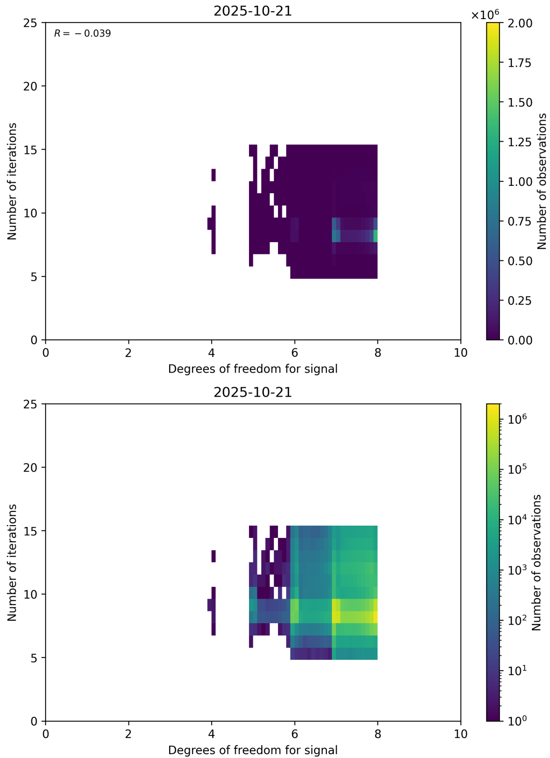
Figure 50: Scatter density plot of “Degrees of freedom for signal” against “Number of iterations” for 2025-10-20 to 2025-10-22.
