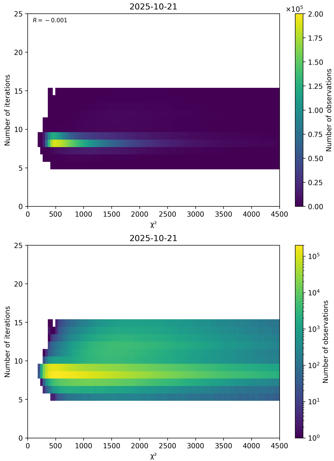
Figure 49: Scatter density plot of “ \chi^2 ” against “Number of iterations” for 2025-10-20 to 2025-10-22.
