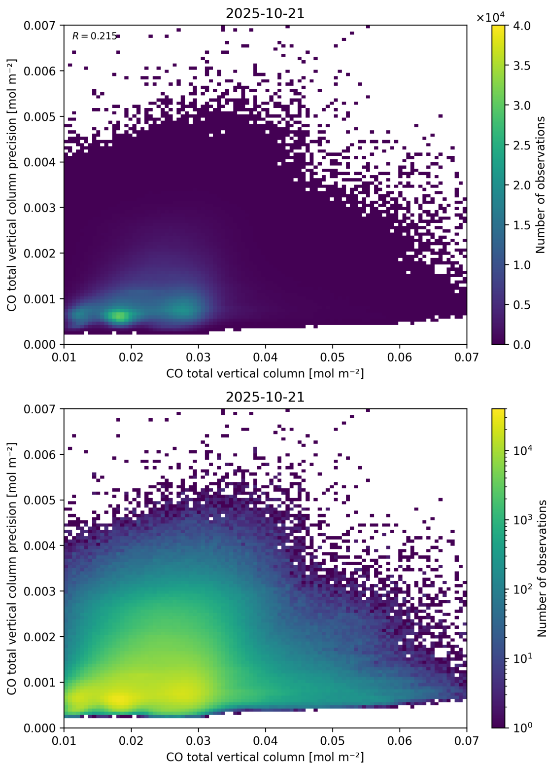
Figure 34: Scatter density plot of “CO total vertical column” against “CO total vertical column precision” for 2025-10-20 to 2025-10-22.
