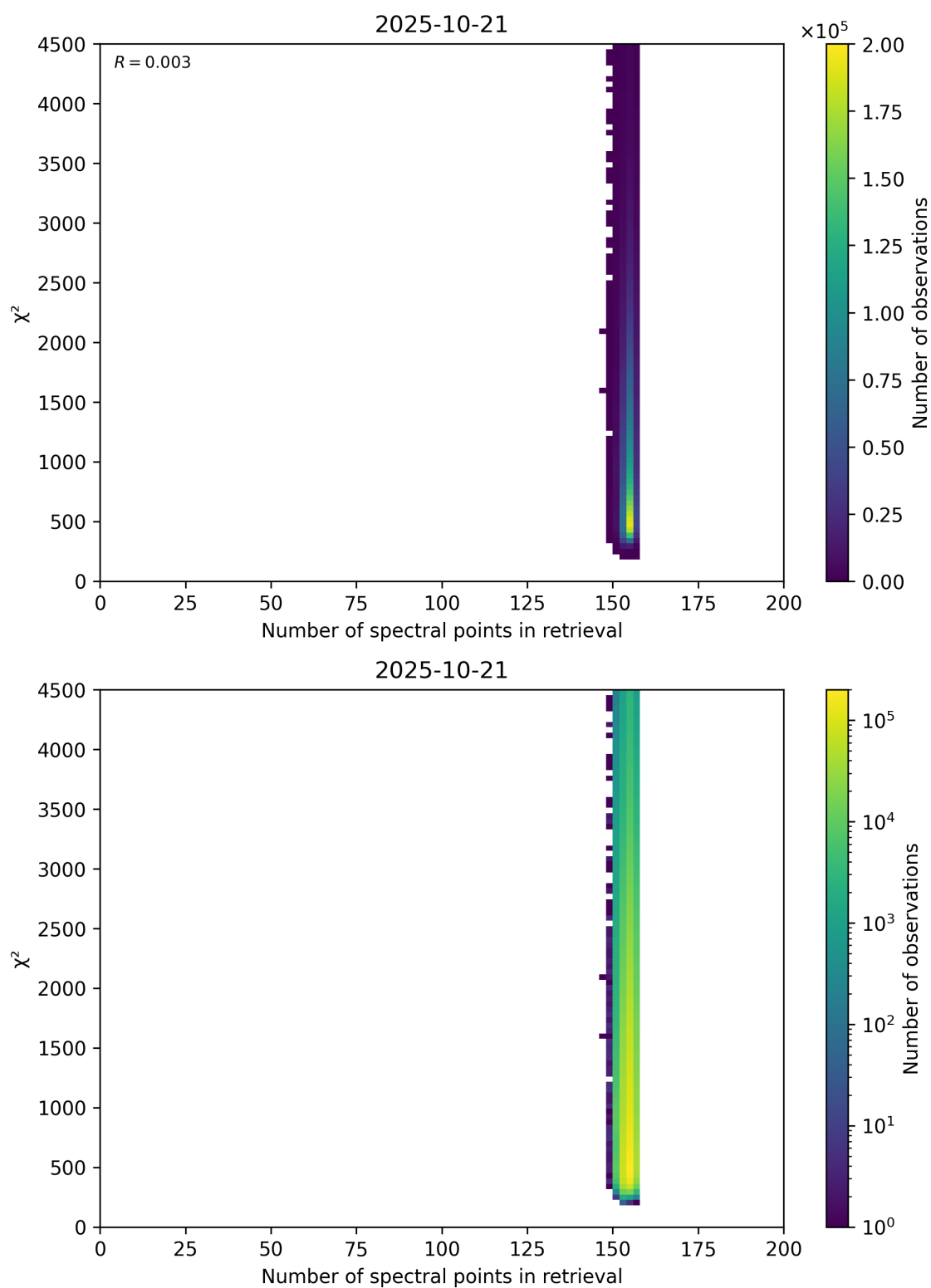
Figure 58: Scatter density plot of “Number of spectral points in retrieval” against “ \chi^2 ” for 2025-10-20 to 2025-10-22.
