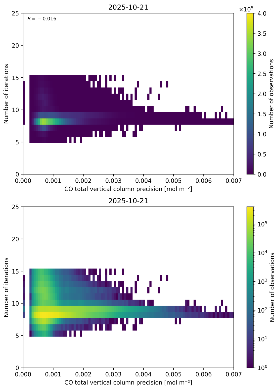
Figure 46: Scatter density plot of “CO total vertical column precision” against “Number of iterations” for 2025-10-20 to 2025-10-22.
