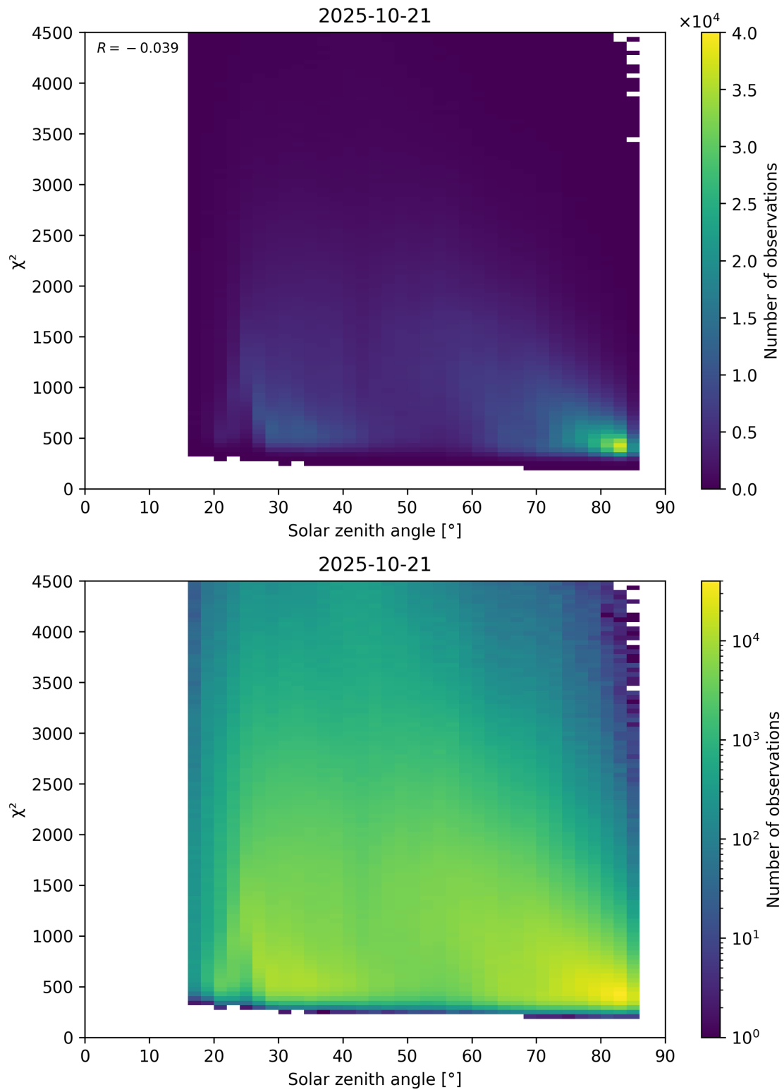
Figure 64: Scatter density plot of “Solar zenith angle” against “ \chi^2 ” for 2025-10-20 to 2025-10-22.
