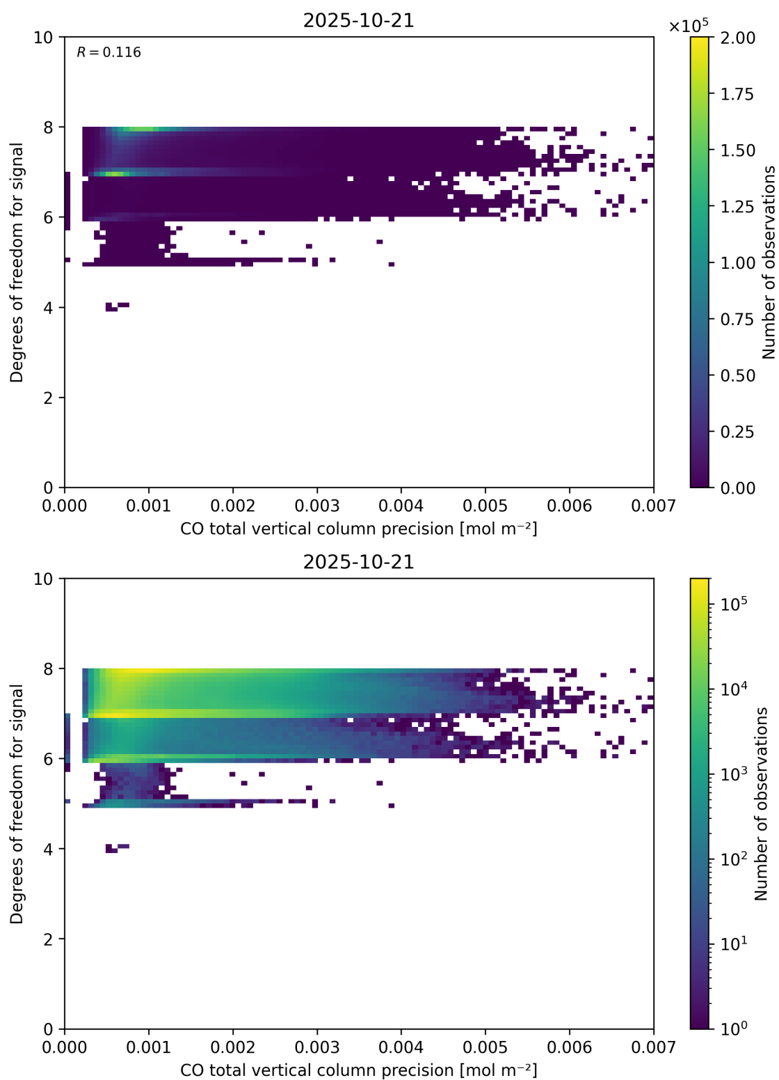
Figure 45: Scatter density plot of “CO total vertical column precision” against “Degrees of freedom for signal” for 2025-10-20 to 2025-10-22.
