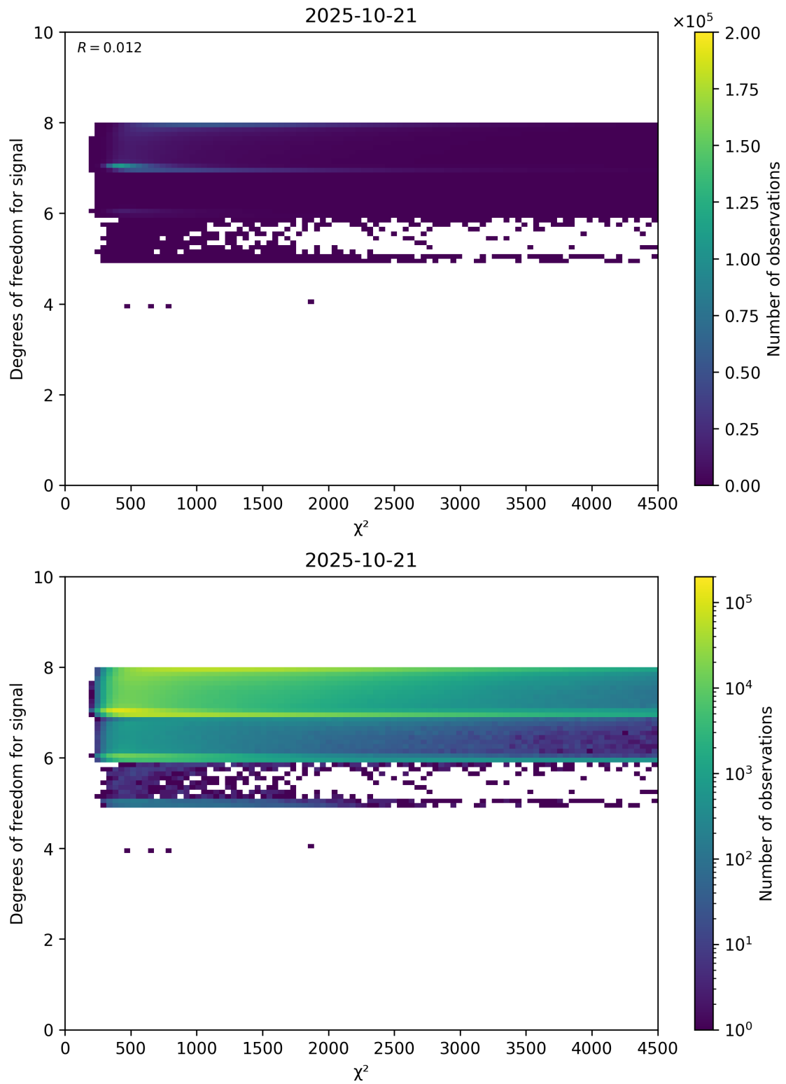
Figure 48: Scatter density plot of “ \chi^2 ” against “Degrees of freedom for signal” for 2025-10-20 to 2025-10-22.
