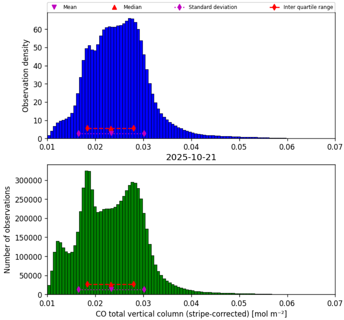
Figure 19: Histogram of “CO total vertical column (stripe-corrected)” for 2025-10-20 to 2025-10-22
