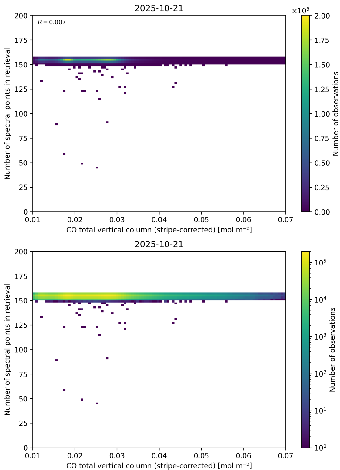
Figure 40: Scatter density plot of “CO total vertical column (stripe-corrected)” against “Number of spectral points in retrieval” for 2025-10-20 to 2025-10-22.
