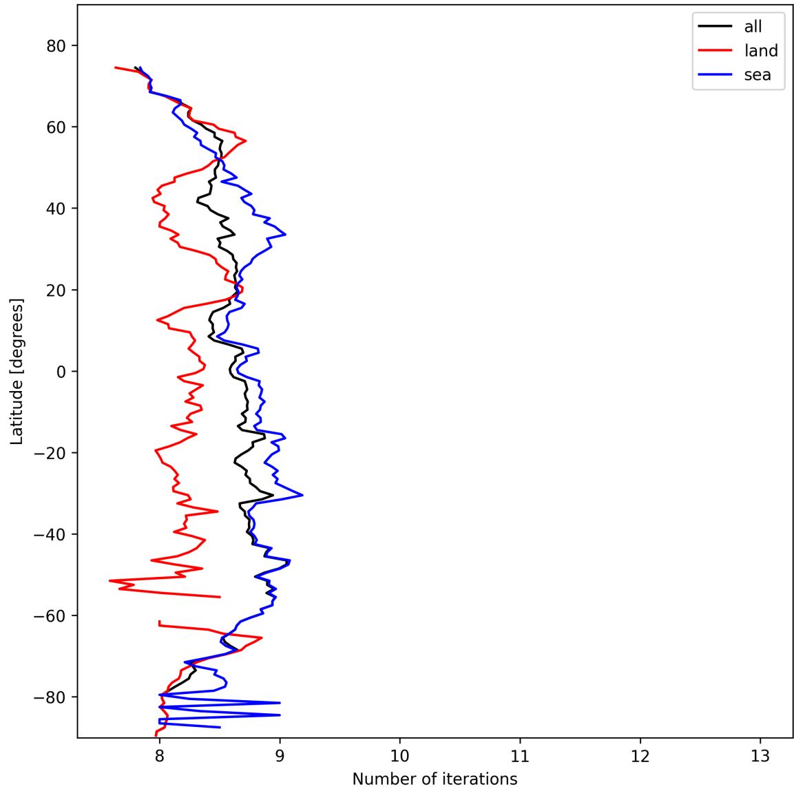
Figure 16: Zonal average of “Number of iterations” for 2025-10-20 to 2025-10-22.
