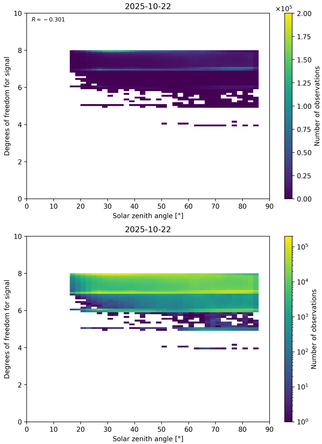
Figure 65: Scatter density plot of “Solar zenith angle” against “Degrees of freedom for signal” for 2025-10-22 to 2025-10-23.
