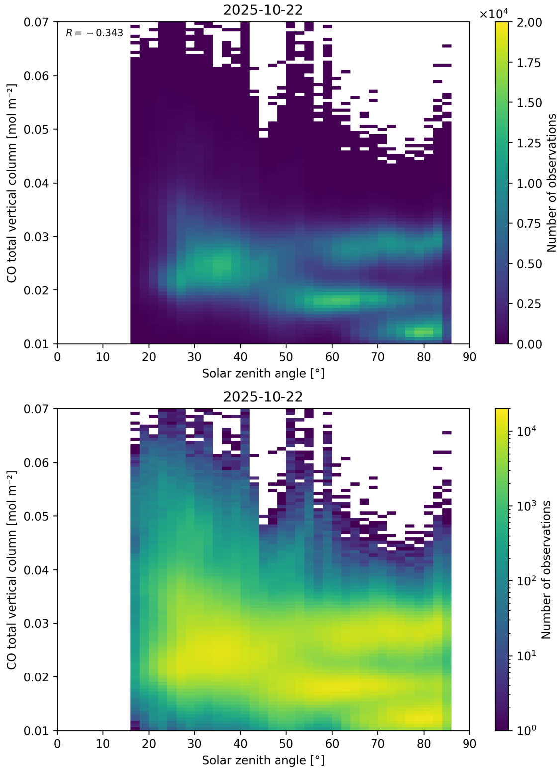
Figure 61: Scatter density plot of “Solar zenith angle” against “CO total vertical column” for 2025-10-22 to 2025-10-23.
