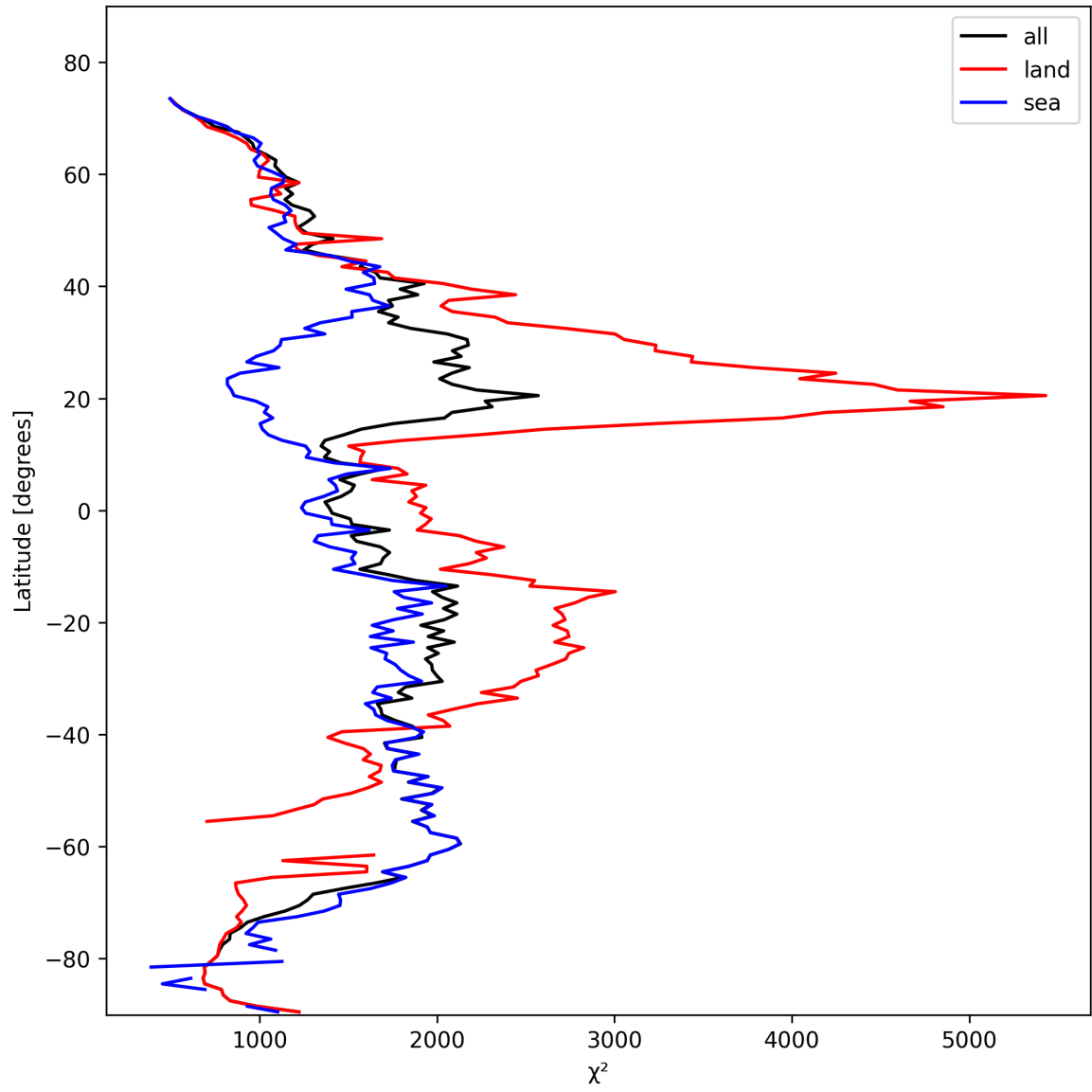
Figure 14: Zonal average of “ \chi^2 ” for 2025-10-22 to 2025-10-23.
