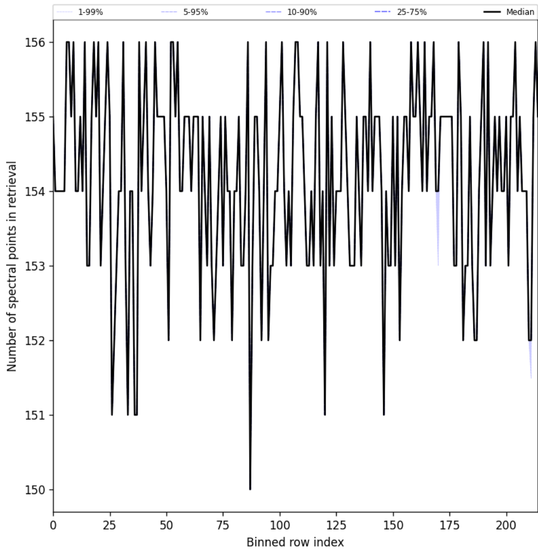
Figure 29: Along track statistics of “Number of spectral points in retrieval” for 2025-10-22 to 2025-10-23
