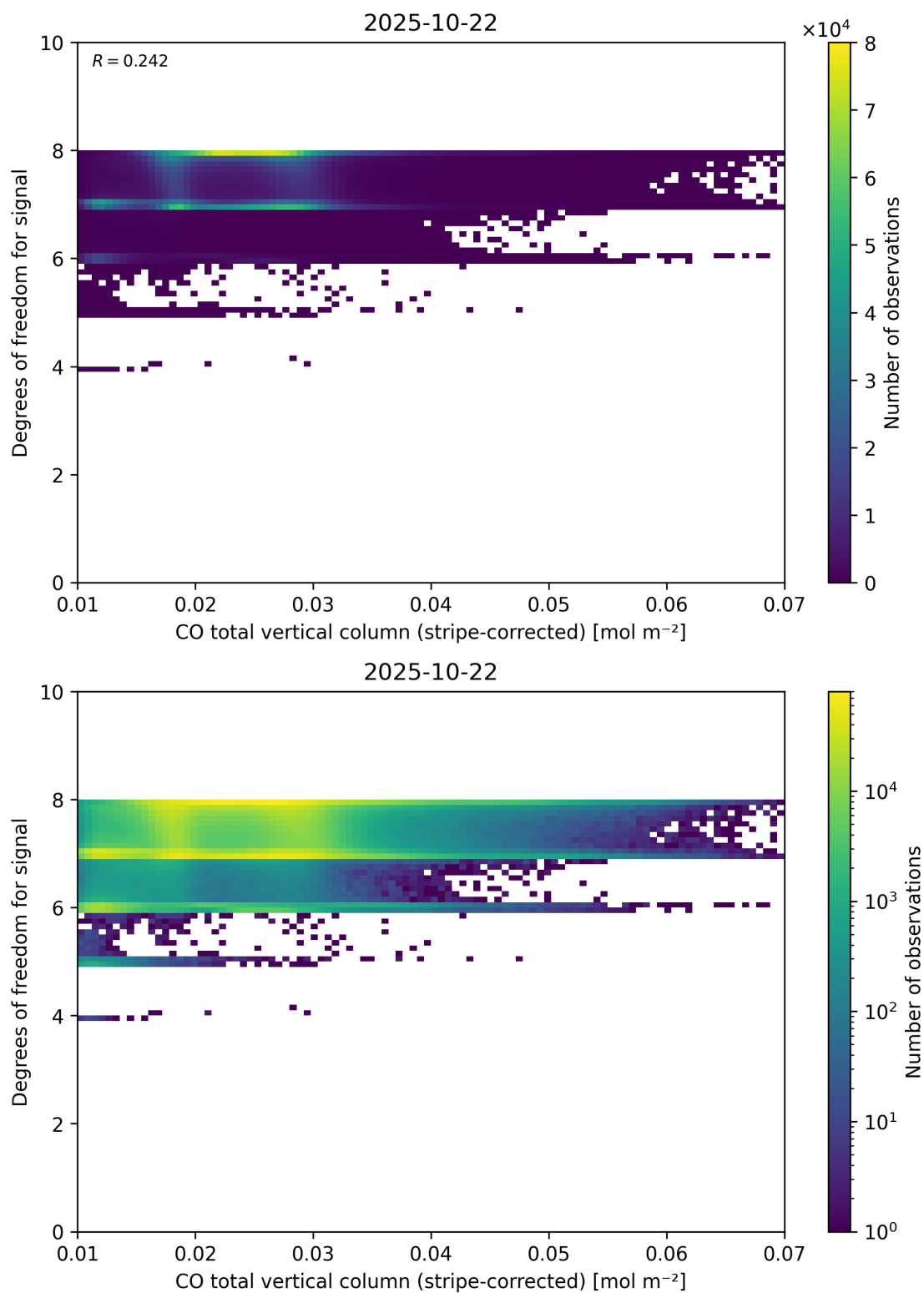
Figure 38: Scatter density plot of “CO total vertical column (stripe-corrected)” against “Degrees of freedom for signal” for 2025-10-22 to 2025-10-23.
