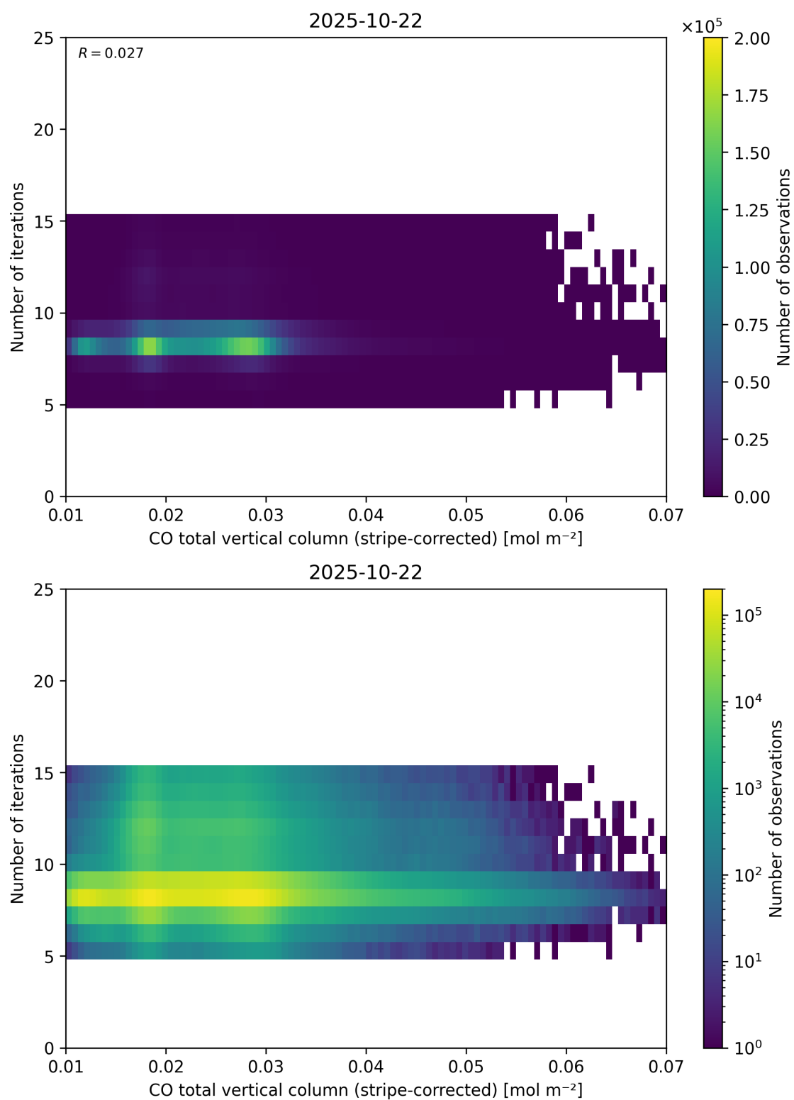
Figure 39: Scatter density plot of “CO total vertical column (stripe-corrected)” against “Number of iterations” for 2025-10-22 to 2025-10-23.
