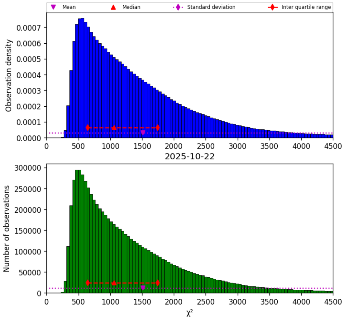
Figure 22: Histogram of “ \chi^2 ” for 2025-10-22 to 2025-10-23
