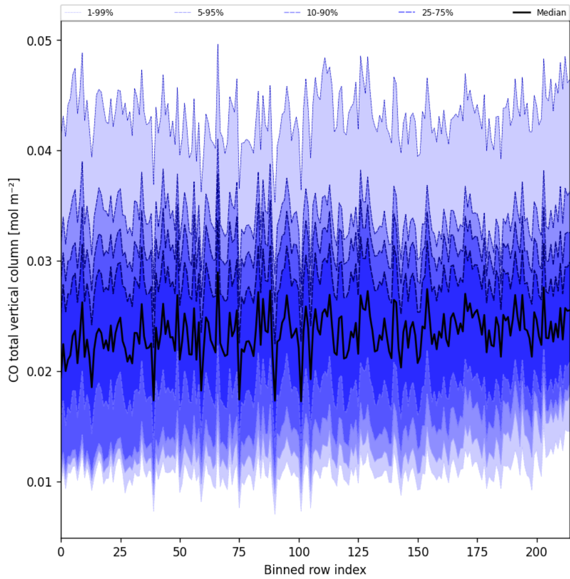
Figure 26: Along track statistics of “CO total vertical column” for 2025-10-22 to 2025-10-23
