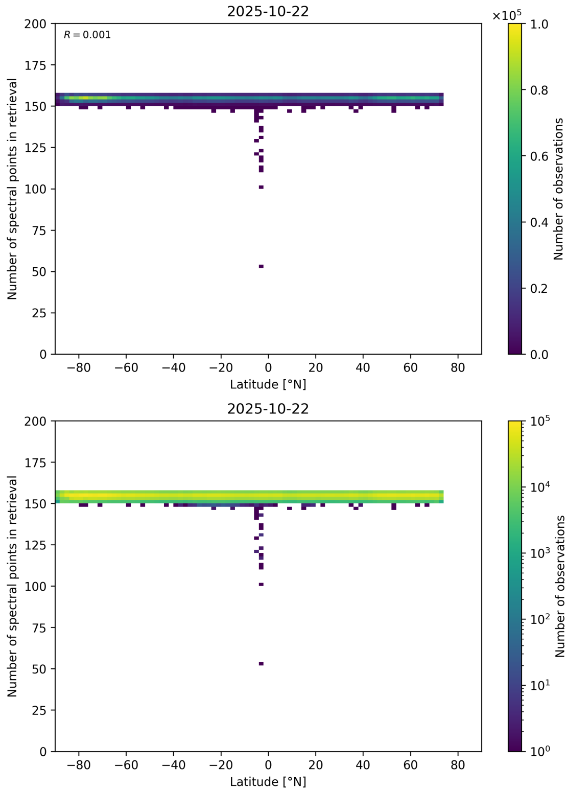
Figure 57: Scatter density plot of “Latitude” against “Number of spectral points in retrieval” for 2025-10-22 to 2025-10-23.
