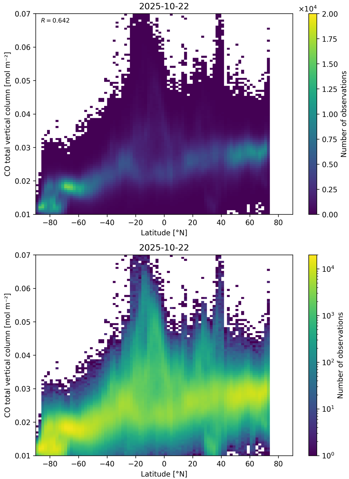
Figure 51: Scatter density plot of “Latitude” against “CO total vertical column” for 2025-10-22 to 2025-10-23.
