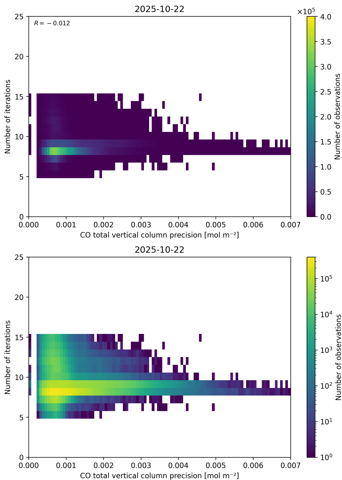
Figure 46: Scatter density plot of “CO total vertical column precision” against “Number of iterations” for 2025-10-22 to 2025-10-23.
