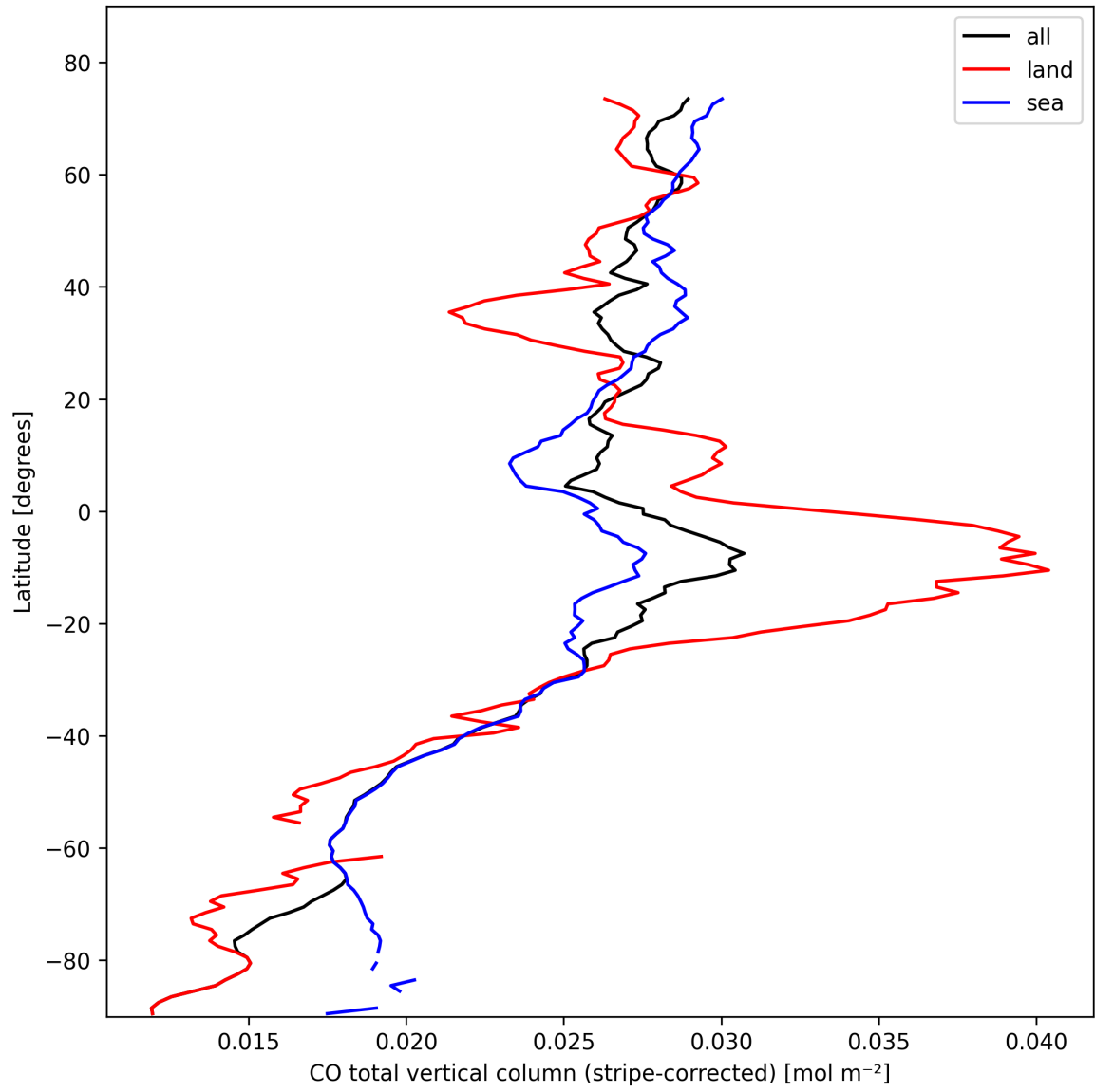
Figure 11: Zonal average of “CO total vertical column (stripe-corrected)” for 2025-10-22 to 2025-10-23.
