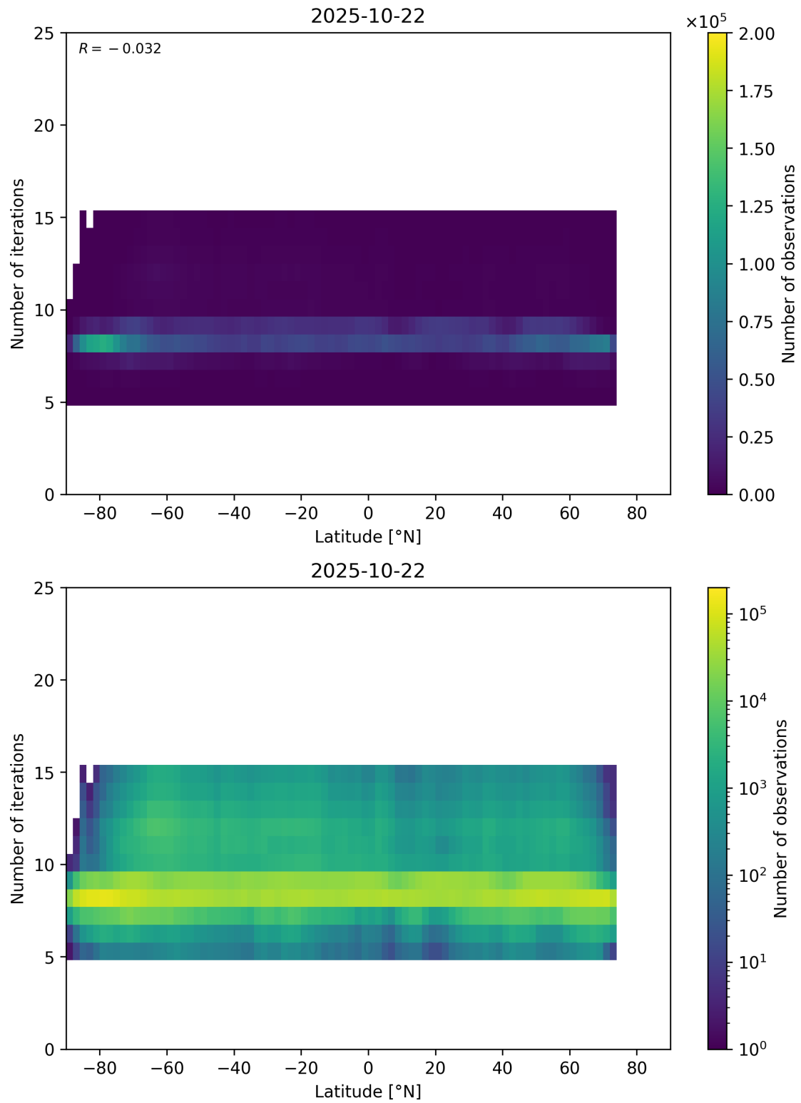
Figure 56: Scatter density plot of “Latitude” against “Number of iterations” for 2025-10-22 to 2025-10-23.
