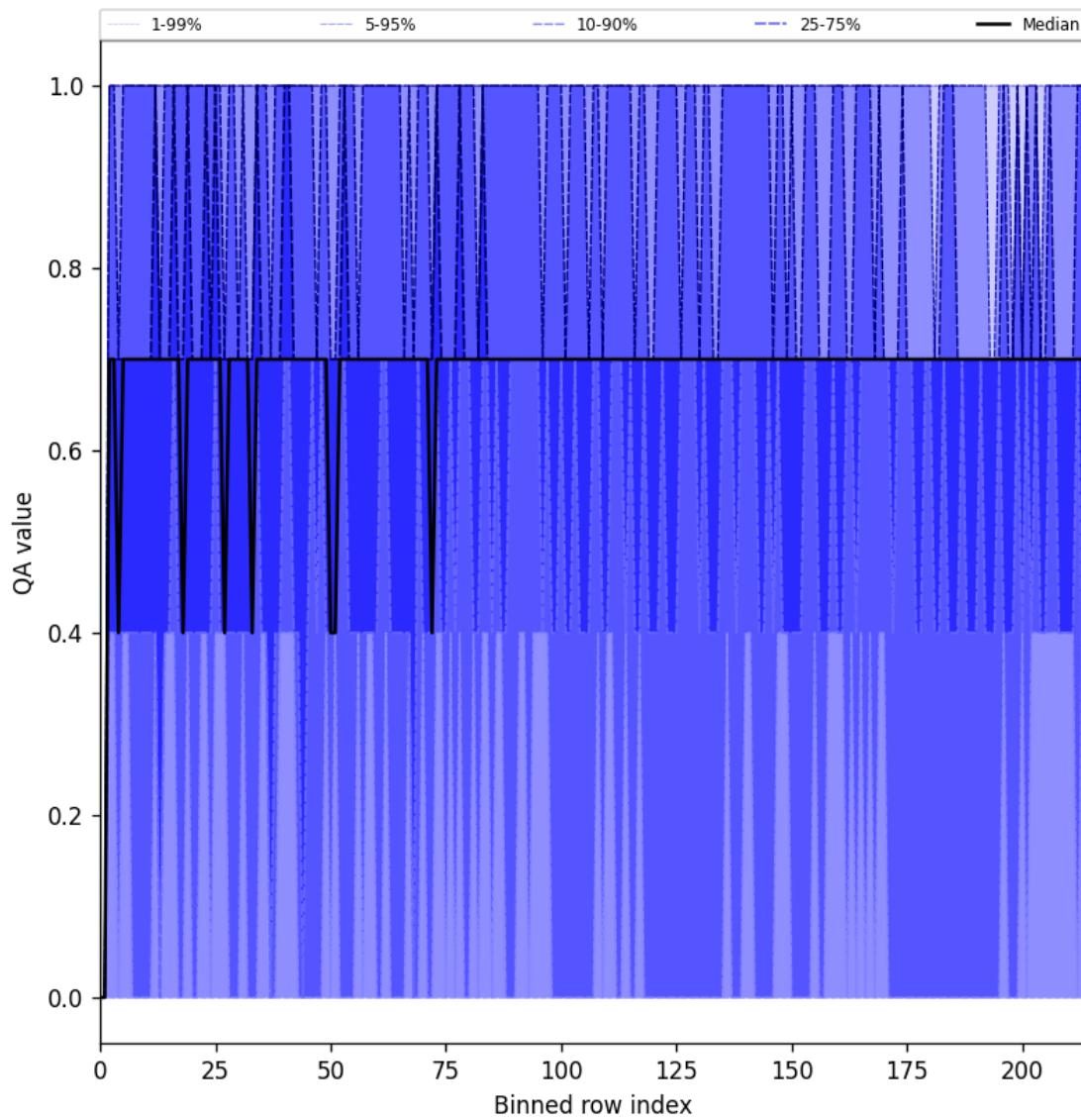
Figure 25: Along track statistics of “QA value” for 2025-10-22 to 2025-10-23
