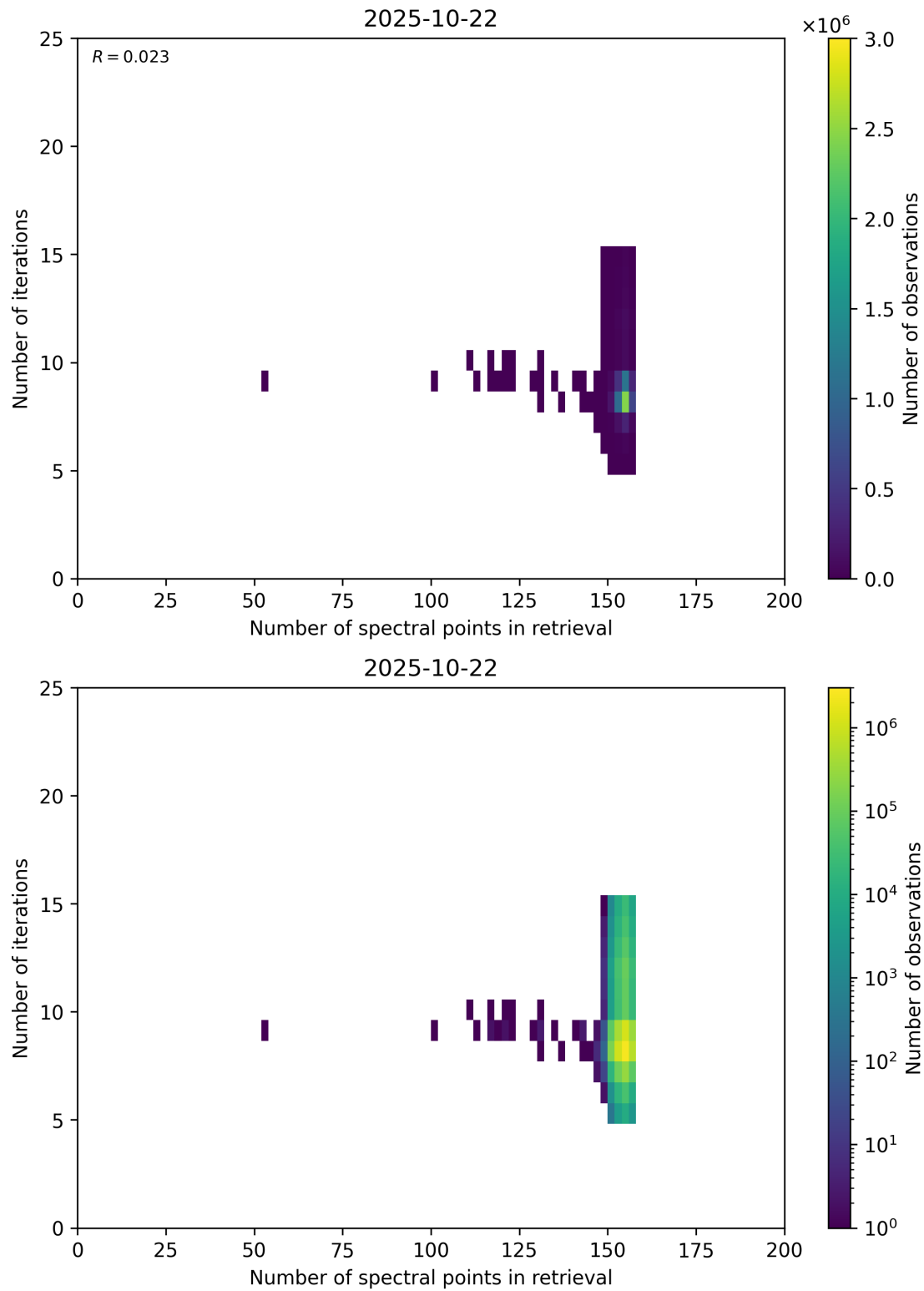
Figure 60: Scatter density plot of “Number of spectral points in retrieval” against “Number of iterations” for 2025-10-22 to 2025-10-23.
