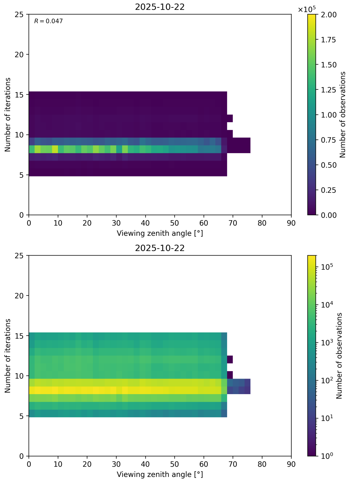
Figure 75: Scatter density plot of “Viewing zenith angle” against “Number of iterations” for 2025-10-22 to 2025-10-23.
