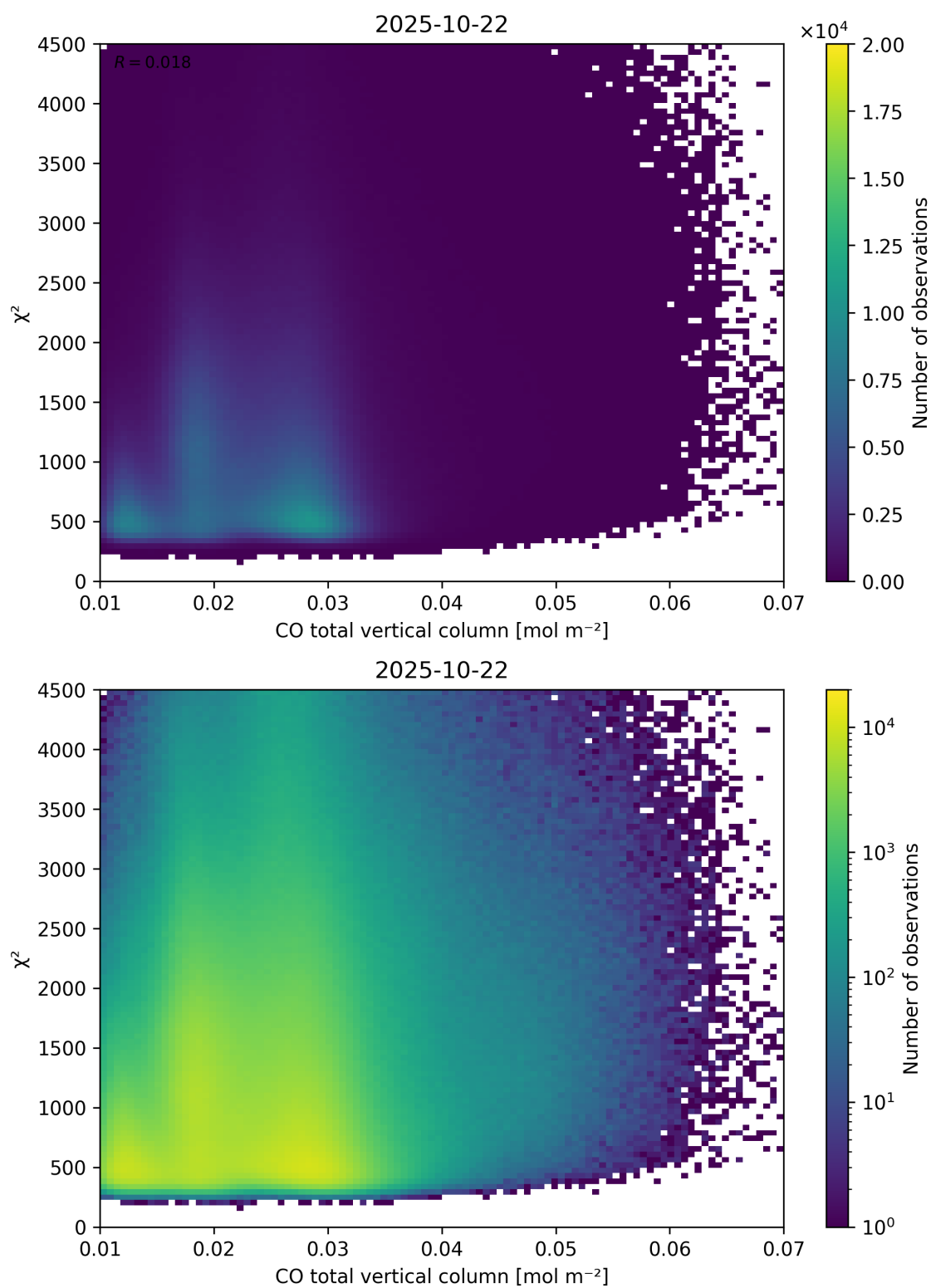
Figure 35: Scatter density plot of “CO total vertical column” against “ \chi^2 ” for 2025-10-22 to 2025-10-23.
