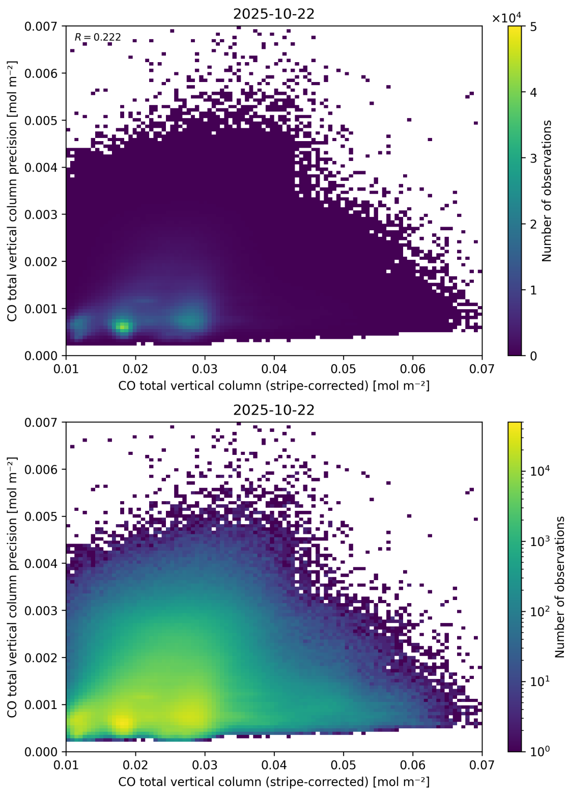
Figure 36: Scatter density plot of “CO total vertical column (stripe-corrected)” against “CO total vertical column precision” for 2025-10-22 to 2025-10-23.
