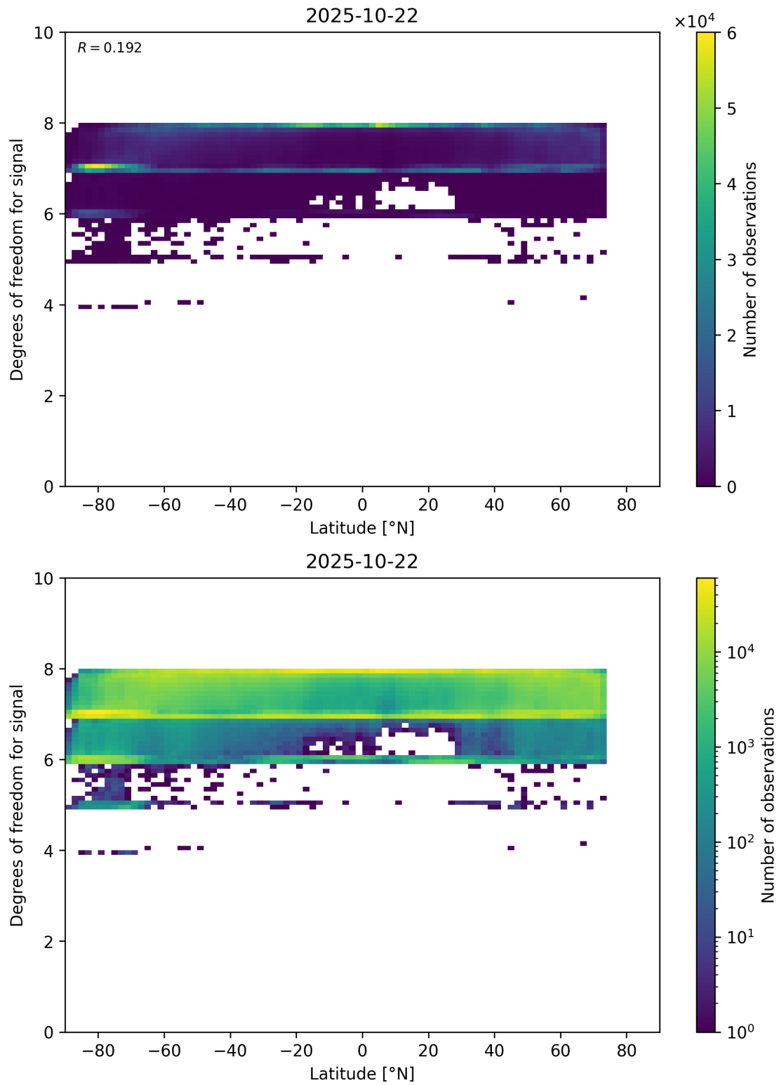
Figure 55: Scatter density plot of “Latitude” against “Degrees of freedom for signal” for 2025-10-22 to 2025-10-23.
