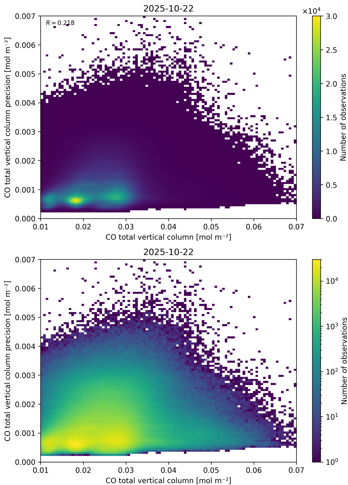
Figure 34: Scatter density plot of “CO total vertical column” against “CO total vertical column precision” for 2025-10-22 to 2025-10-23.
