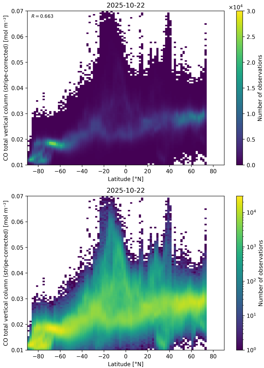
Figure 52: Scatter density plot of “Latitude” against “CO total vertical column (stripe-corrected)” for 2025-10-22 to 2025-10-23.
