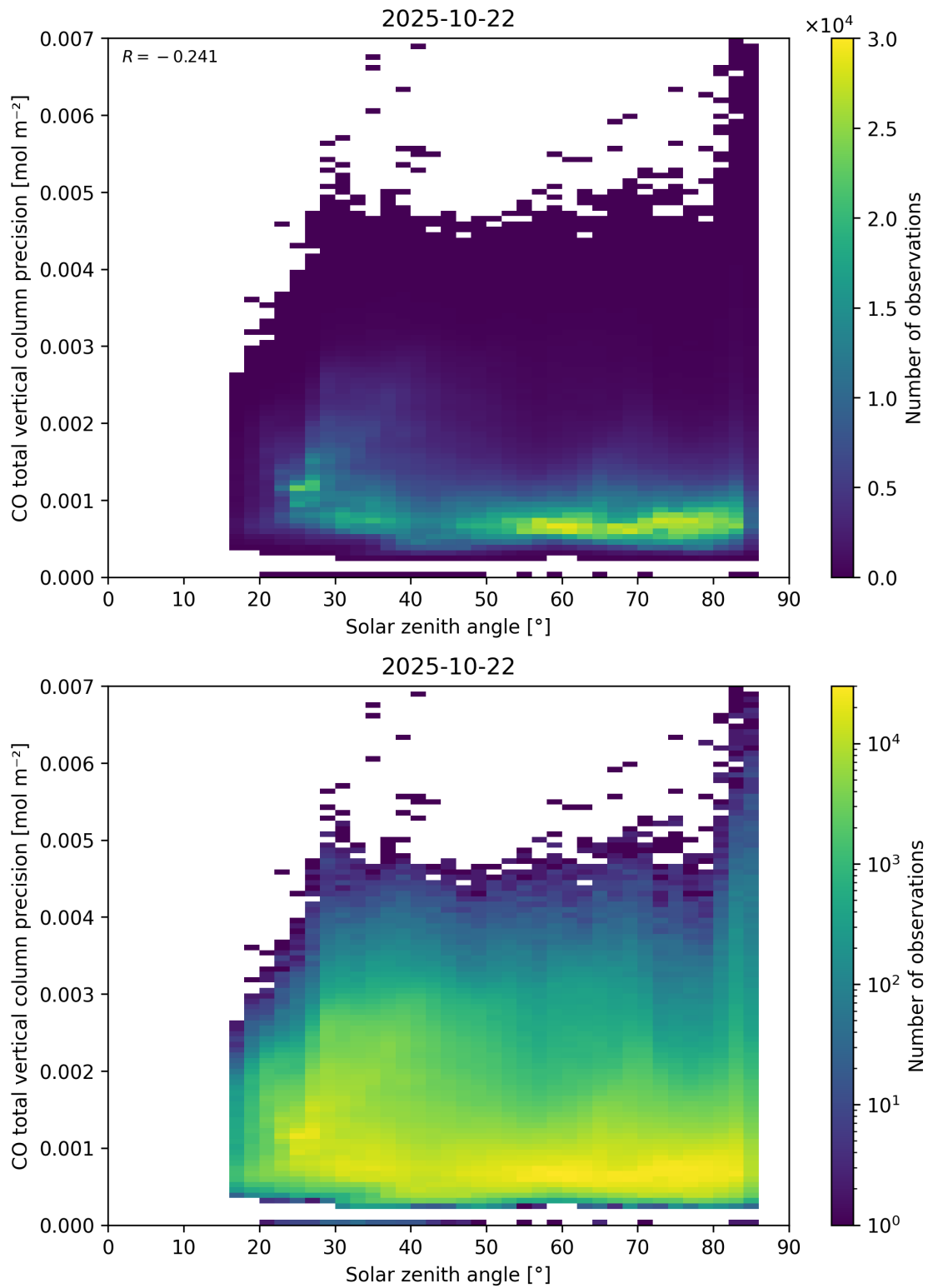
Figure 63: Scatter density plot of “Solar zenith angle” against “CO total vertical column precision” for 2025-10-22 to 2025-10-23.
