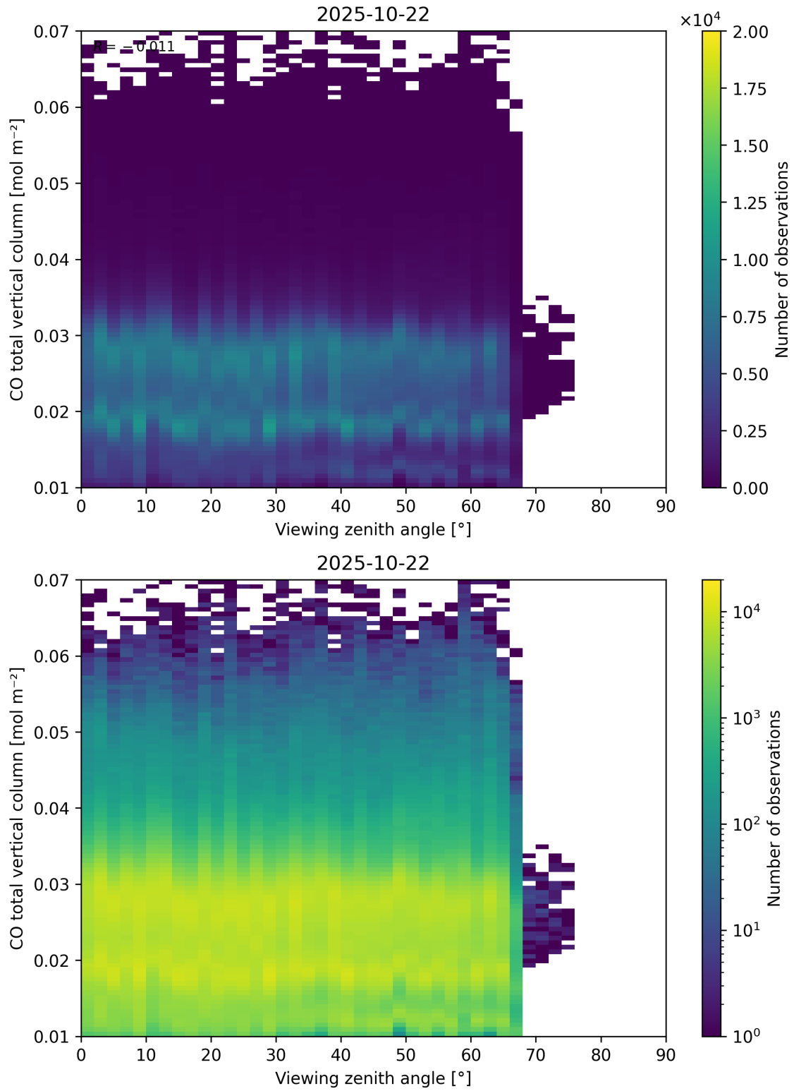
Figure 69: Scatter density plot of “Viewing zenith angle” against “CO total vertical column” for 2025-10-22 to 2025-10-23.
