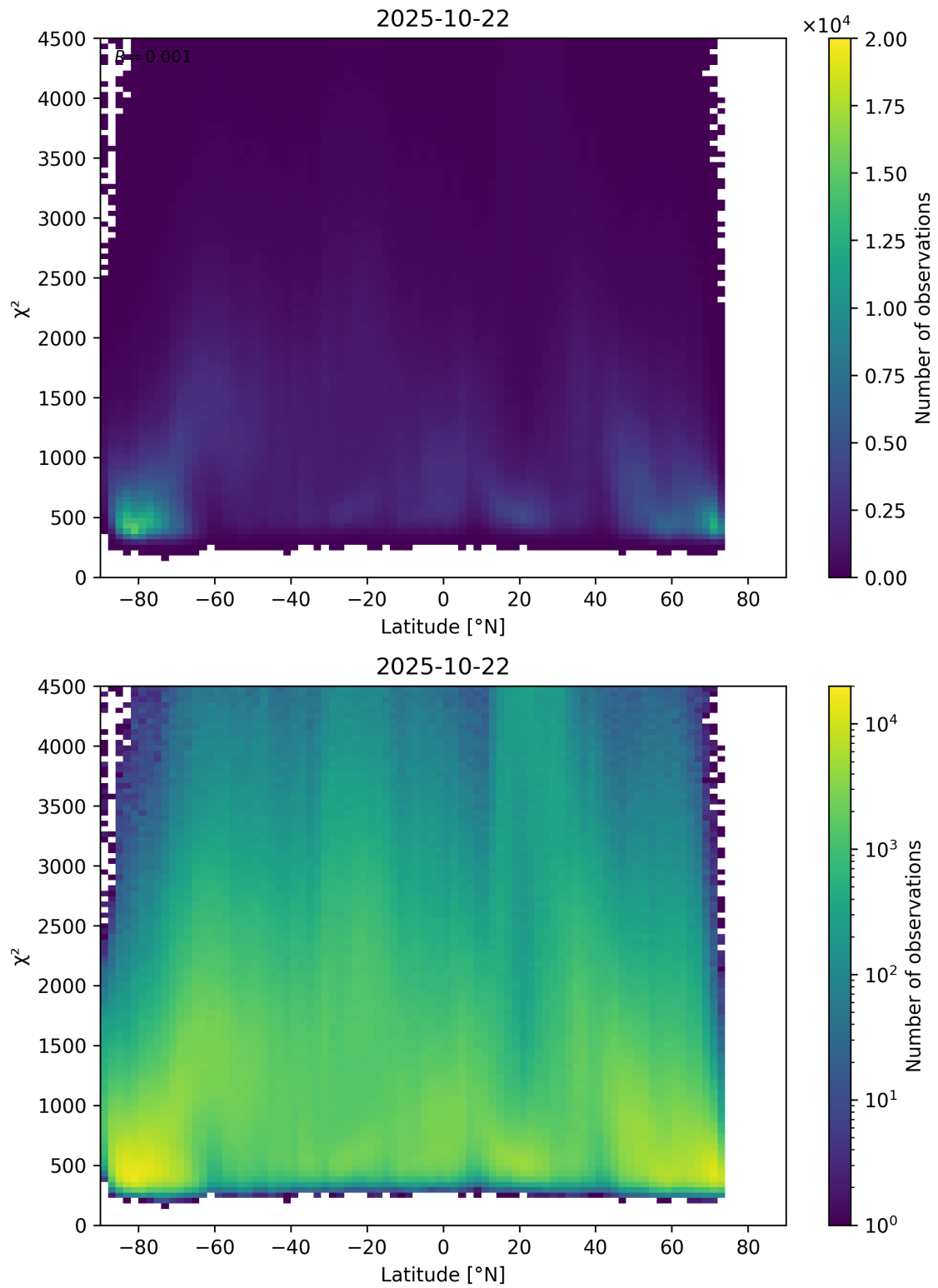
Figure 54: Scatter density plot of “Latitude” against “ \chi^2 ” for 2025-10-22 to 2025-10-23.
