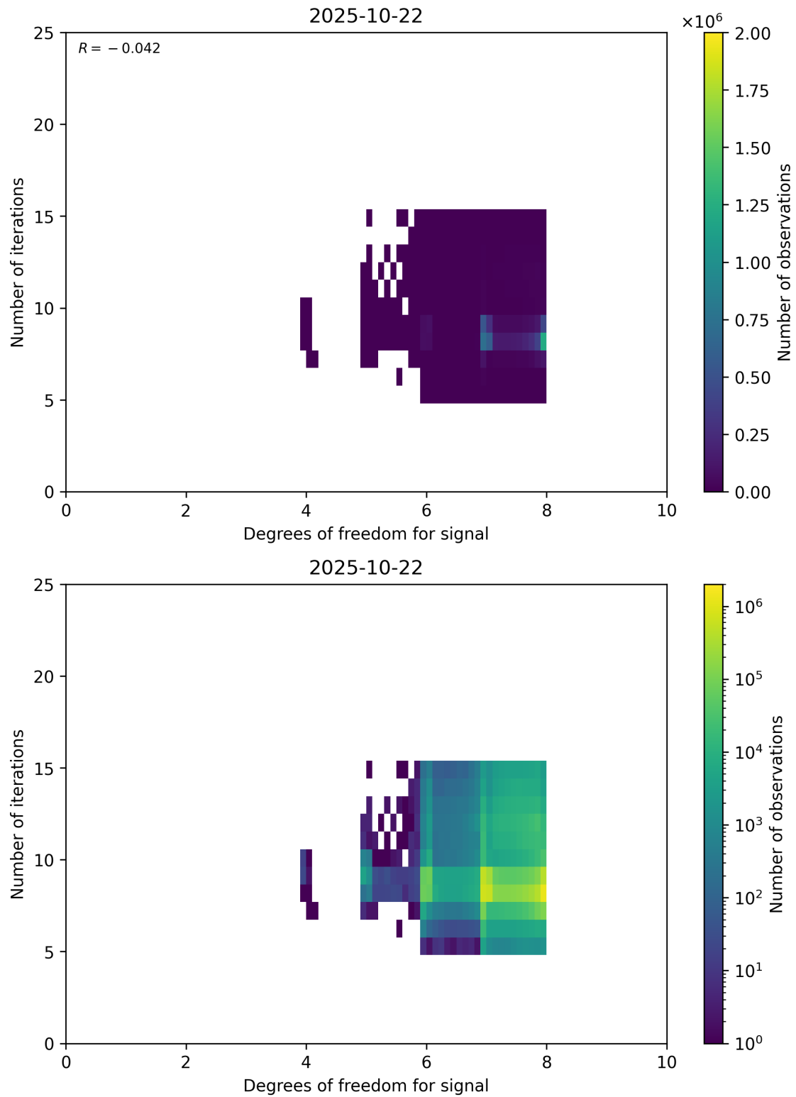
Figure 50: Scatter density plot of “Degrees of freedom for signal” against “Number of iterations” for 2025-10-22 to 2025-10-23.
