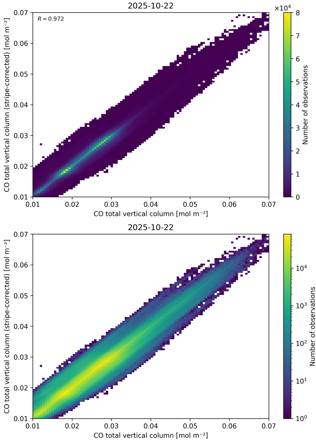
Figure 33: Scatter density plot of “CO total vertical column” against “CO total vertical column (stripe-corrected)” for 2025-10-22 to 2025-10-23.
