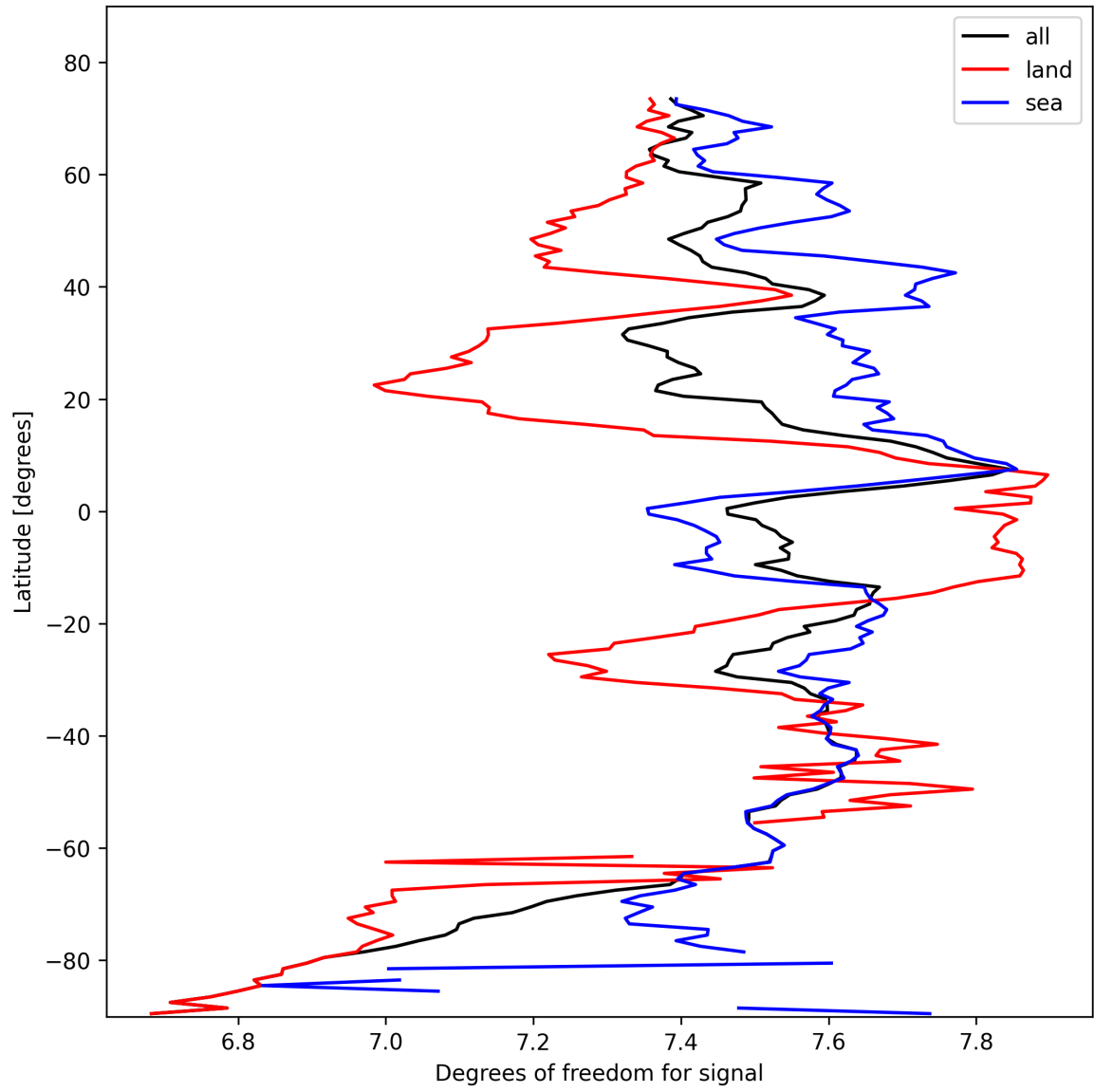
Figure 15: Zonal average of “Degrees of freedom for signal” for 2025-10-22 to 2025-10-23.
