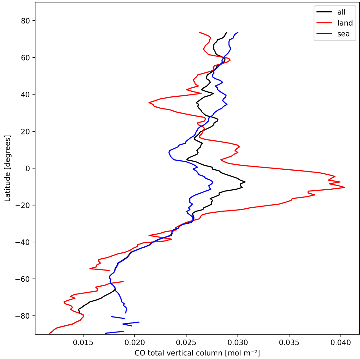
Figure 10: Zonal average of “CO total vertical column” for 2025-10-22 to 2025-10-23.
