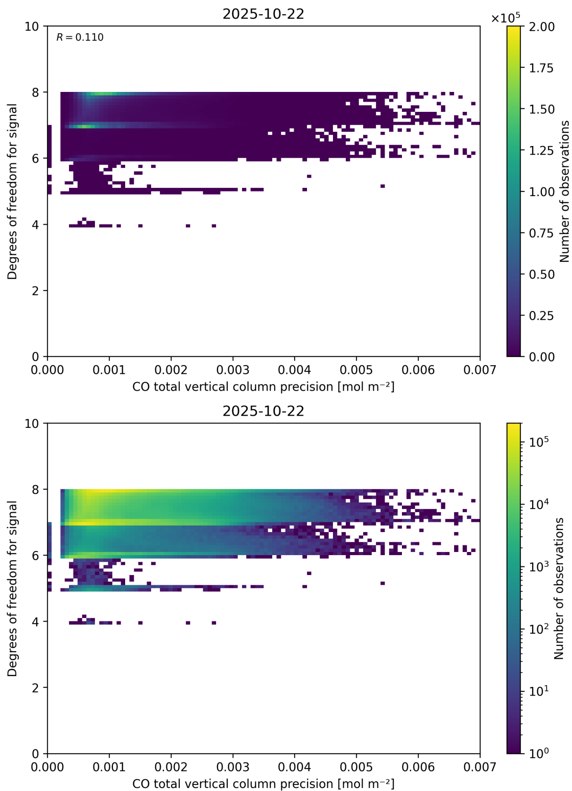
Figure 45: Scatter density plot of “CO total vertical column precision” against “Degrees of freedom for signal” for 2025-10-22 to 2025-10-23.
