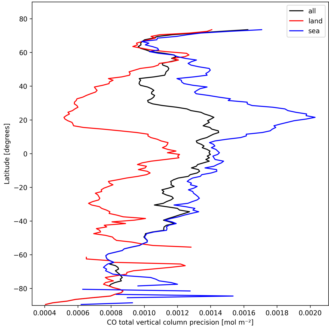
Figure 12: Zonal average of “CO total vertical column precision” for 2025-10-22 to 2025-10-23.
