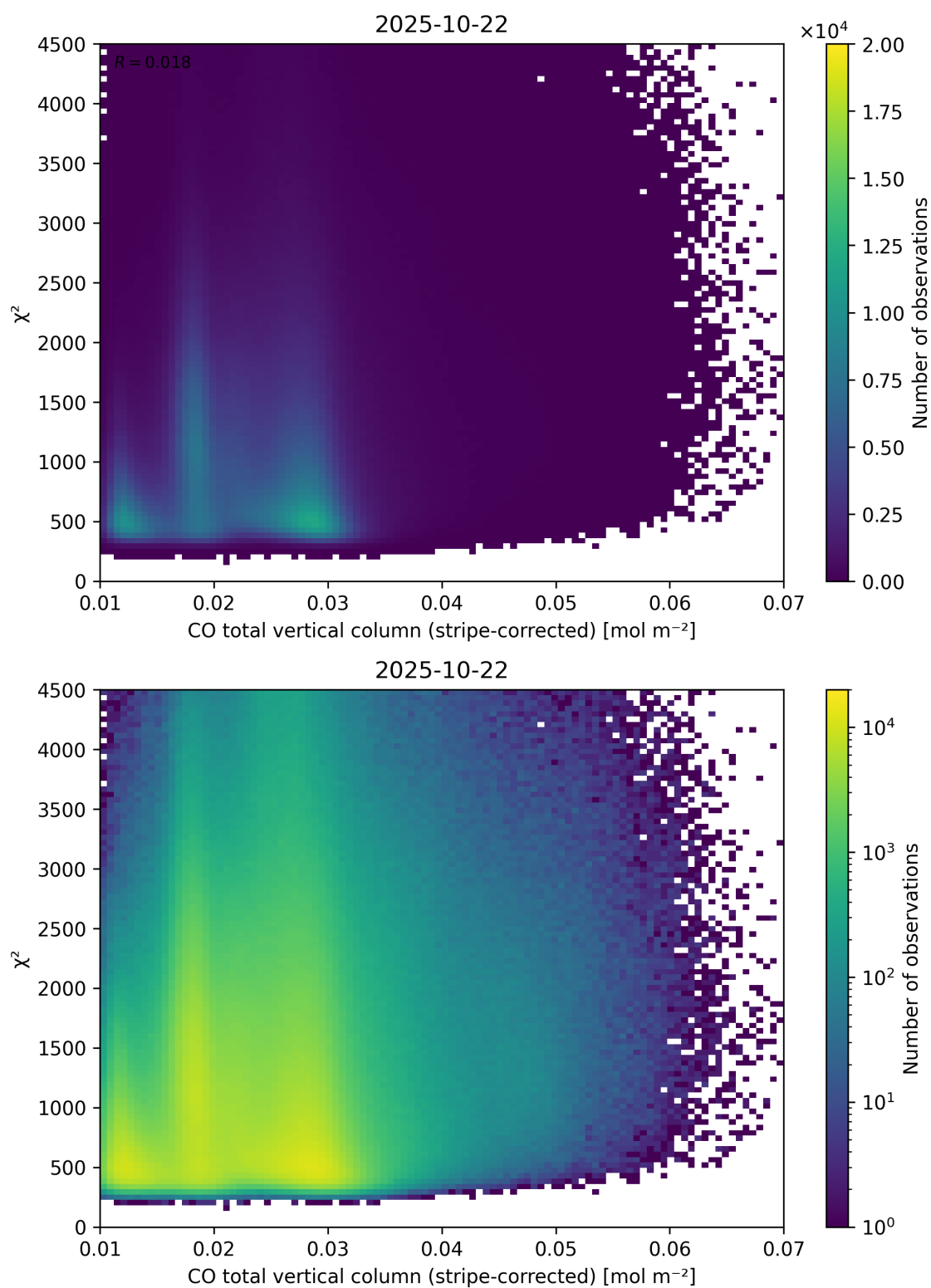
Figure 37: Scatter density plot of “CO total vertical column (stripe-corrected)” against “ \chi^2 ” for 2025-10-22 to 2025-10-23.
