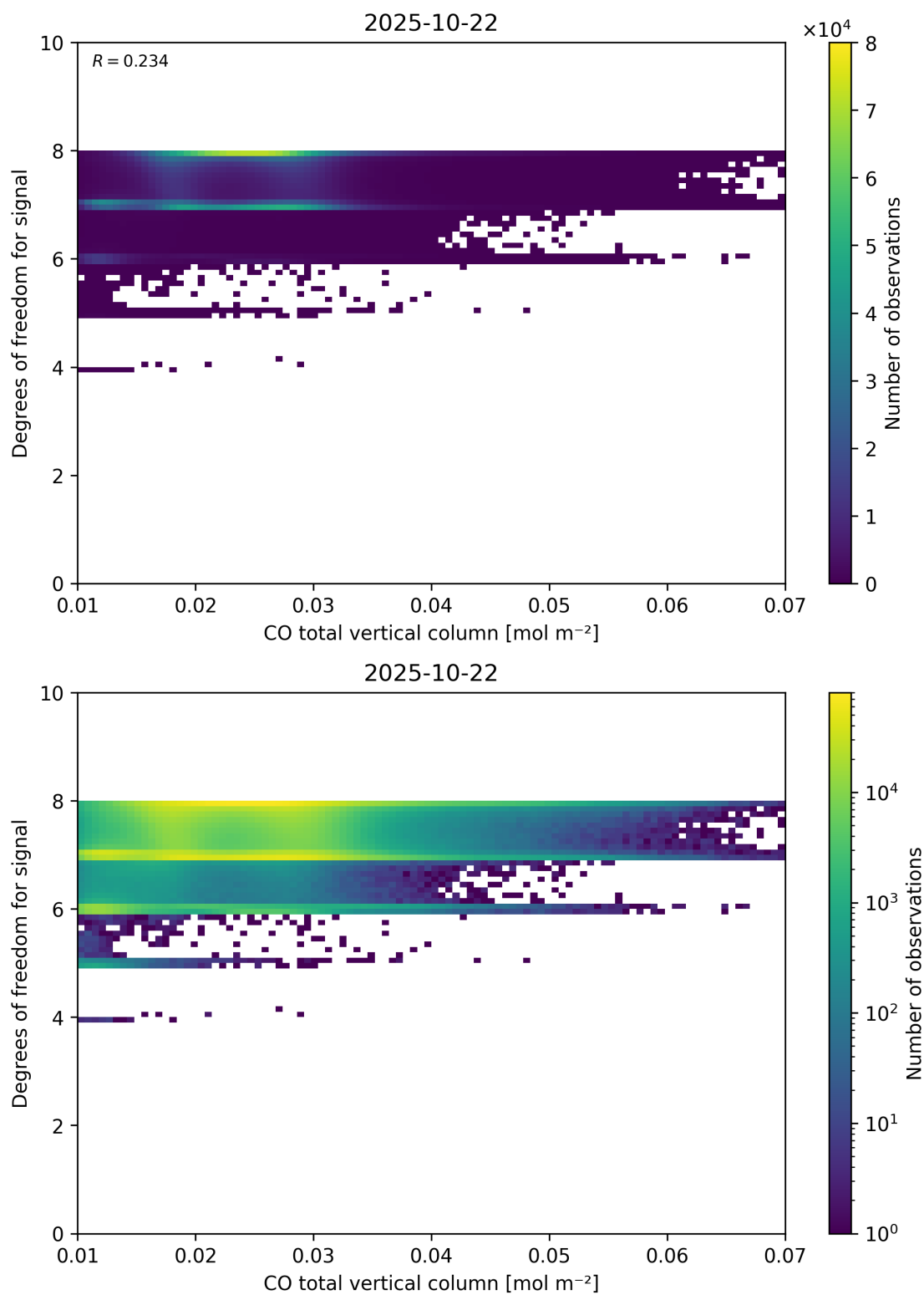
Figure 41: Scatter density plot of “CO total vertical column” against “Degrees of freedom for signal” for 2025-10-22 to 2025-10-23.
