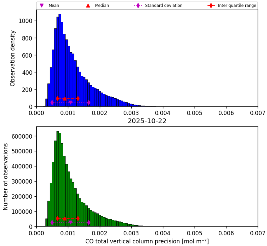
Figure 20: Histogram of “CO total vertical column precision” for 2025-10-22 to 2025-10-23
