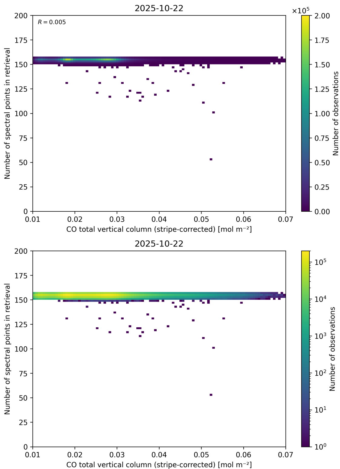
Figure 40: Scatter density plot of “CO total vertical column (stripe-corrected)” against “Number of spectral points in retrieval” for 2025-10-22 to 2025-10-23.
