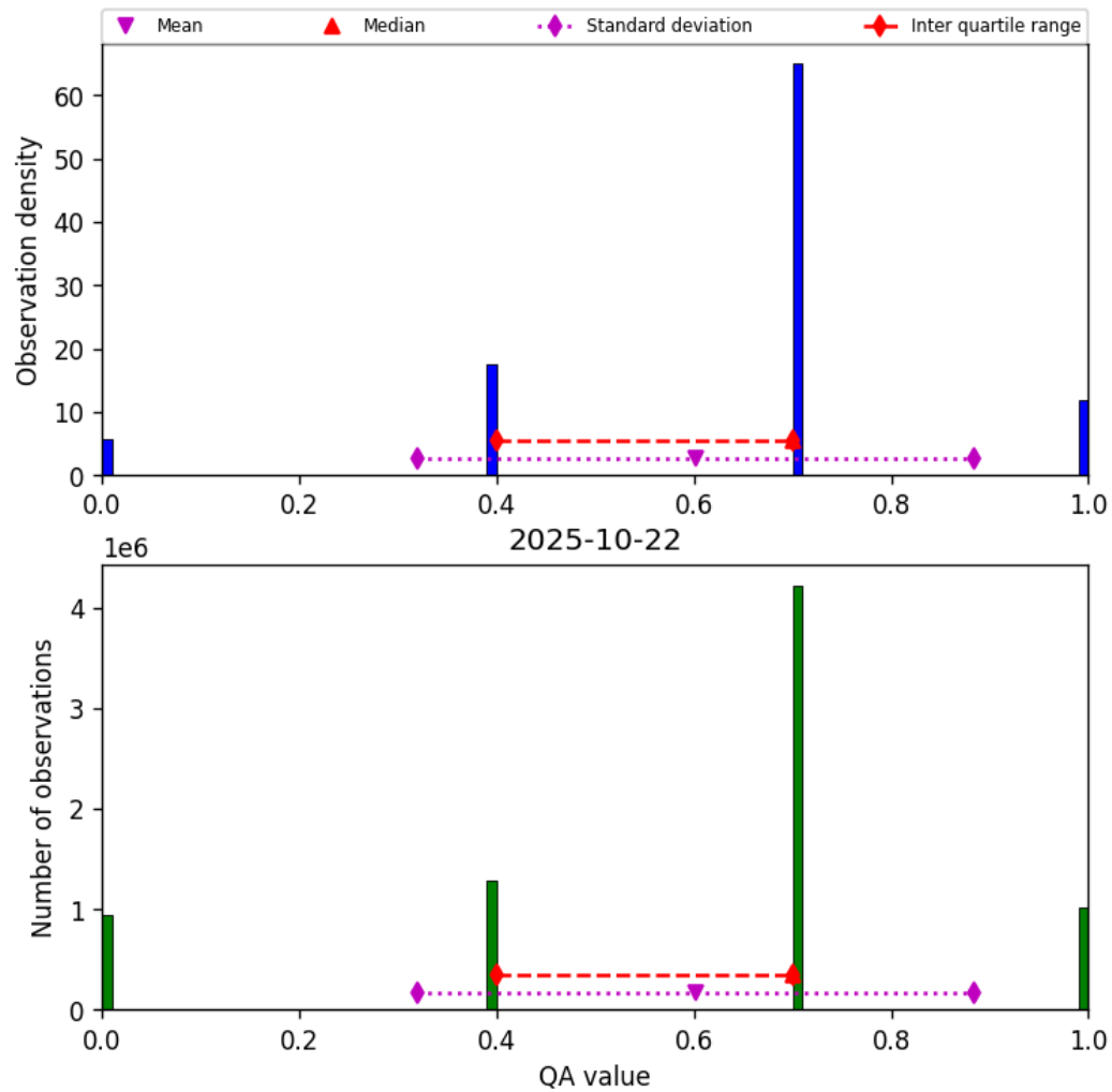
Figure 17: Histogram of “QA value” for 2025-10-22 to 2025-10-23
