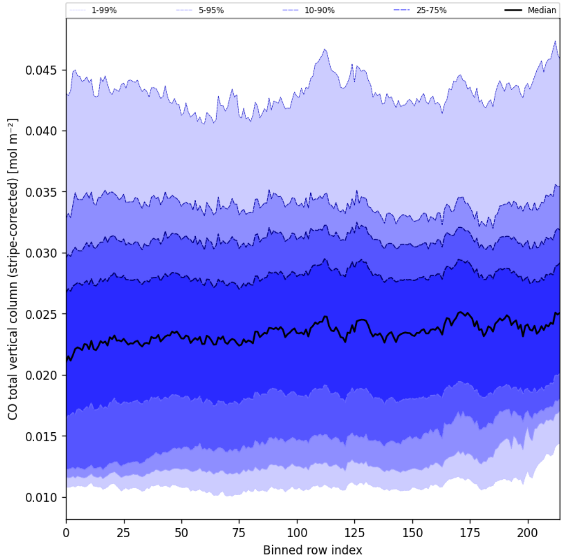
Figure 27: Along track statistics of “CO total vertical column (stripe-corrected)” for 2025-10-22 to 2025-10-23
