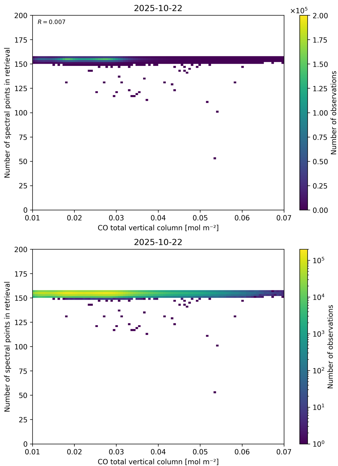
Figure 43: Scatter density plot of “CO total vertical column” against “Number of spectral points in retrieval” for 2025-10-22 to 2025-10-23.
