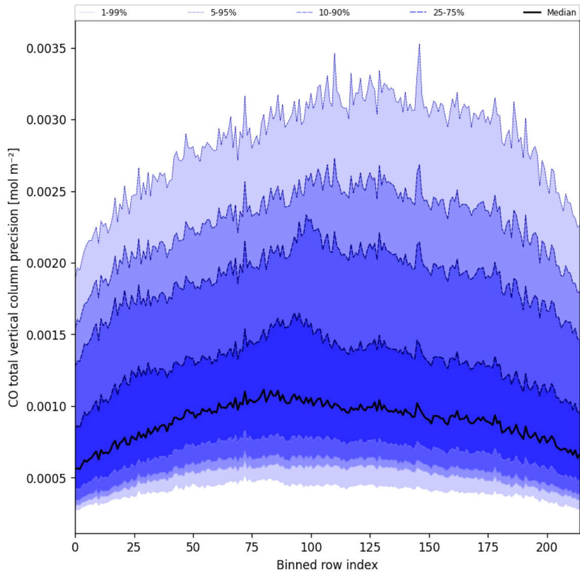
Figure 28: Along track statistics of “CO total vertical column precision” for 2025-10-22 to 2025-10-23
