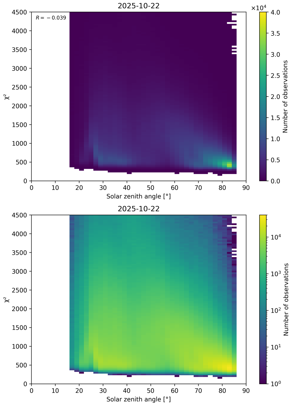
Figure 64: Scatter density plot of “Solar zenith angle” against “ \chi^2 ” for 2025-10-22 to 2025-10-23.
