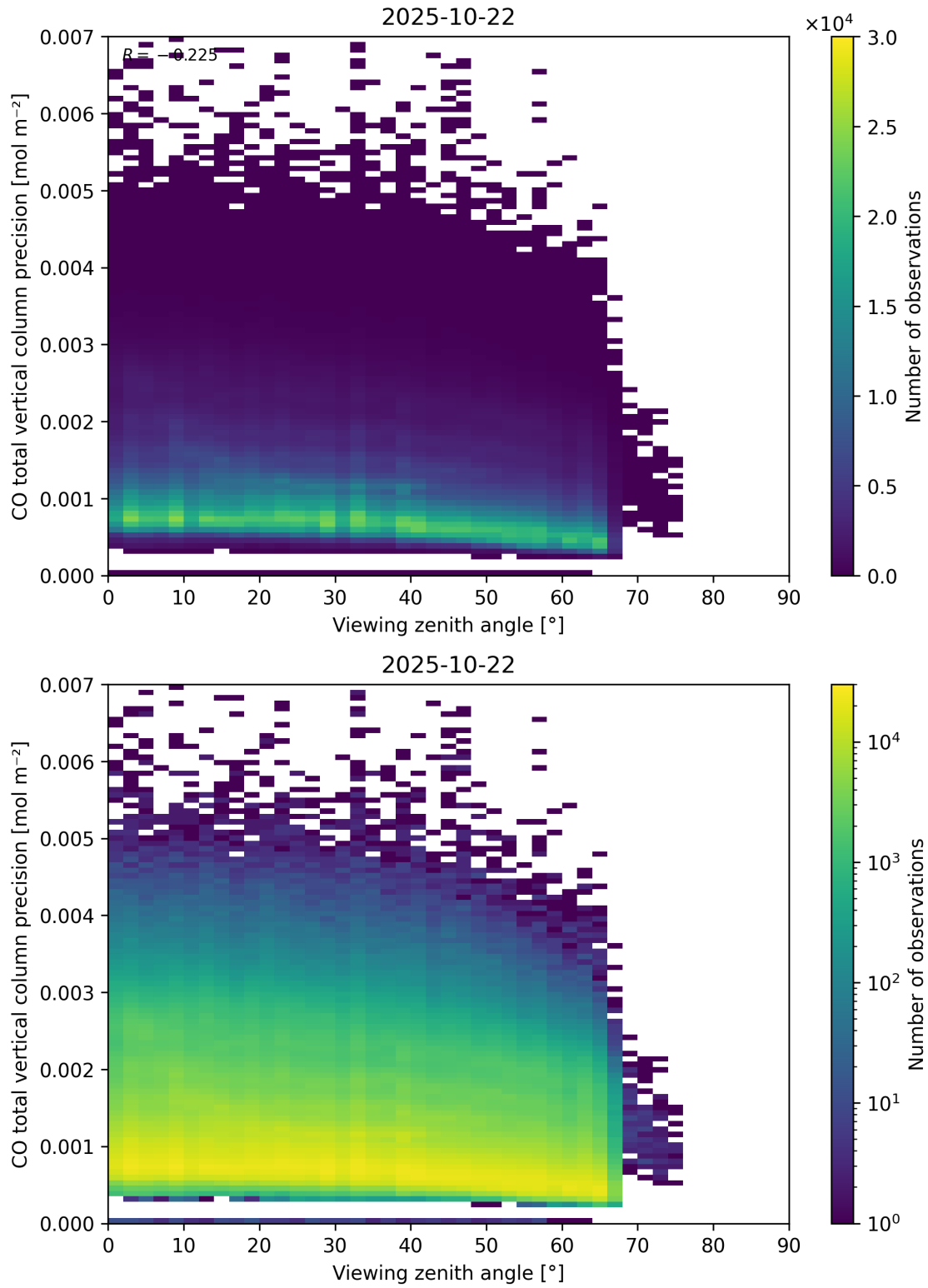
Figure 71: Scatter density plot of “Viewing zenith angle” against “CO total vertical column precision” for 2025-10-22 to 2025-10-23.
