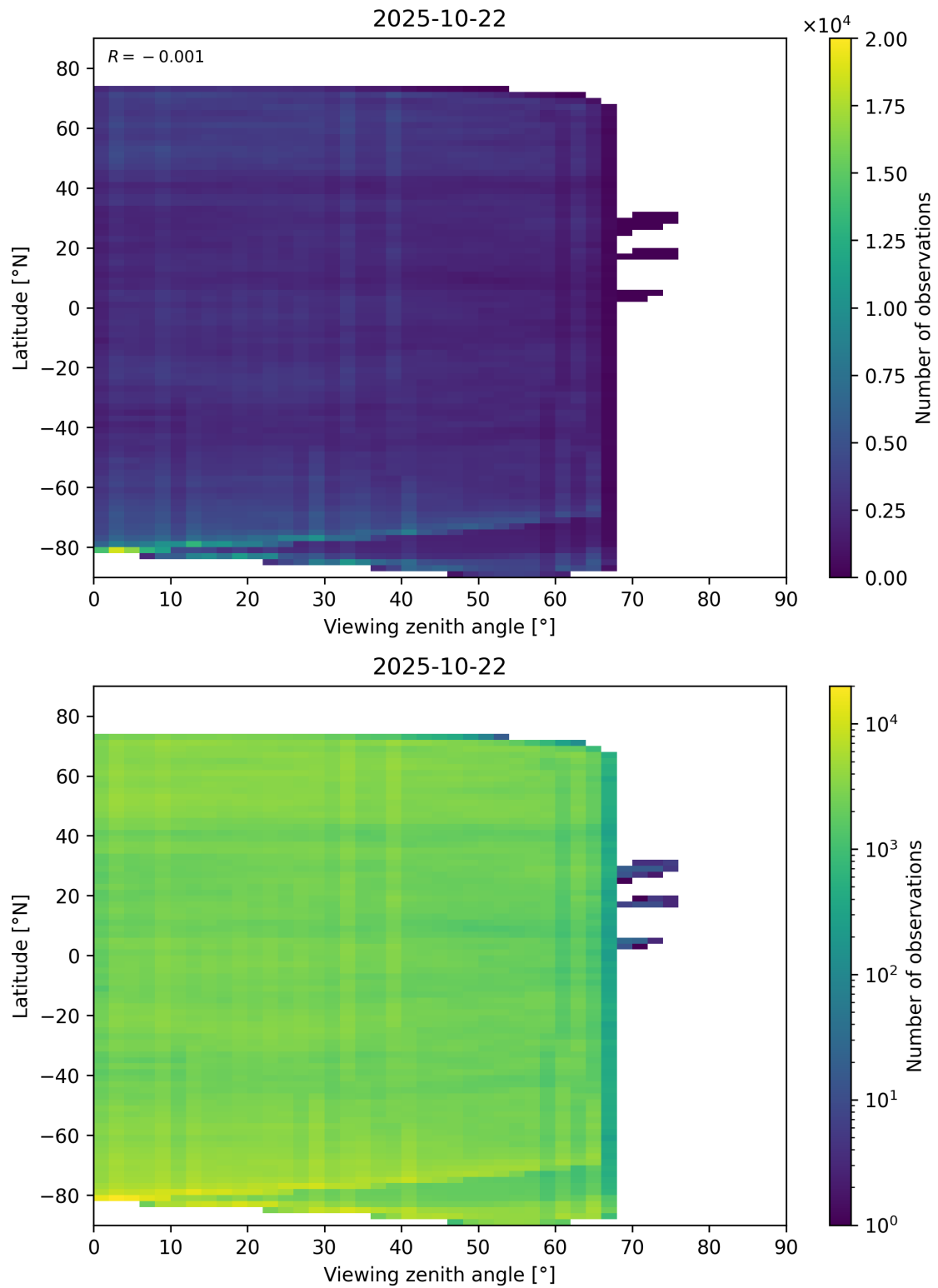
Figure 74: Scatter density plot of “Viewing zenith angle” against “Latitude” for 2025-10-22 to 2025-10-23.
