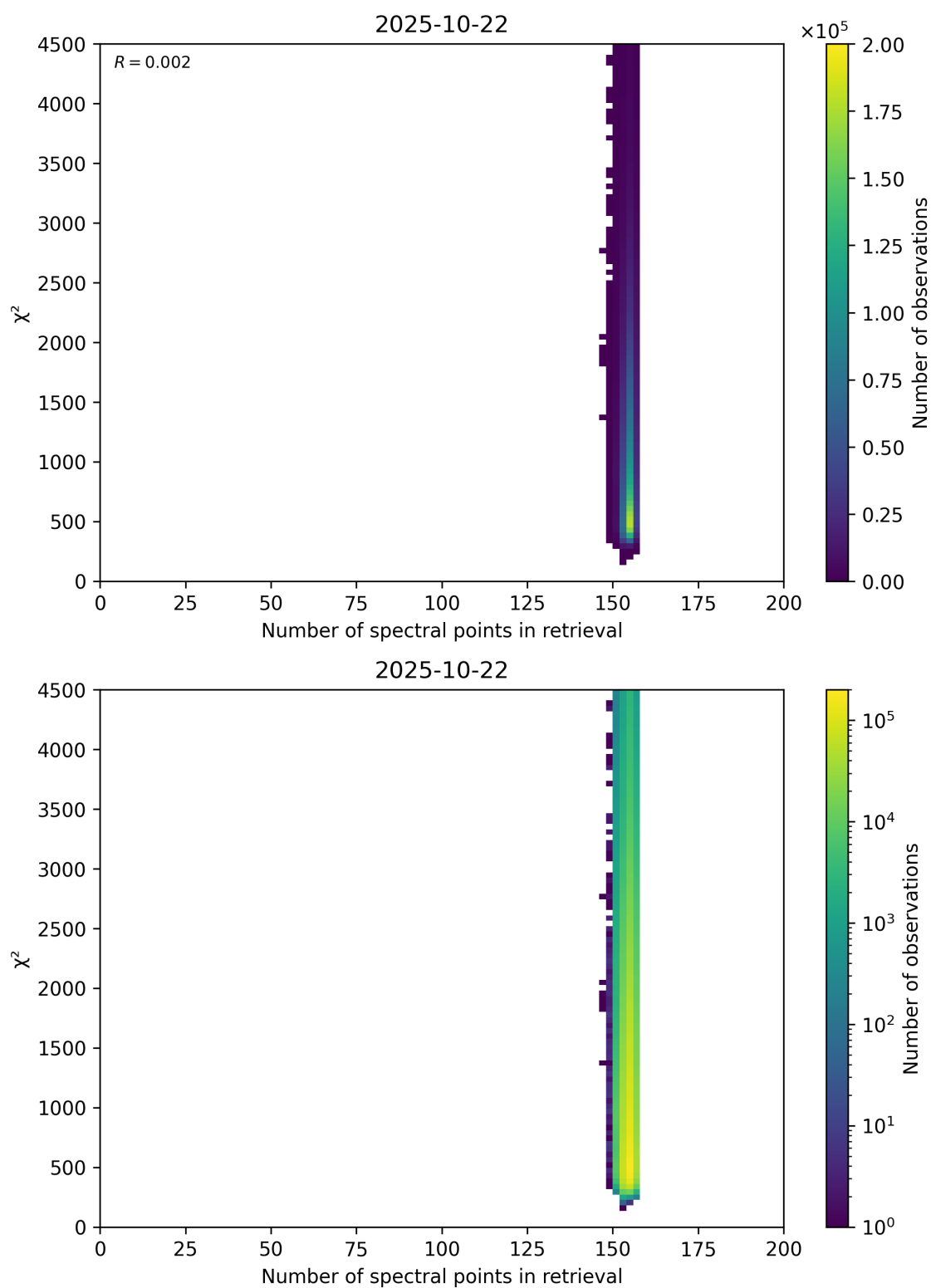
Figure 58: Scatter density plot of “Number of spectral points in retrieval” against “ \chi^2 ” for 2025-10-22 to 2025-10-23.
