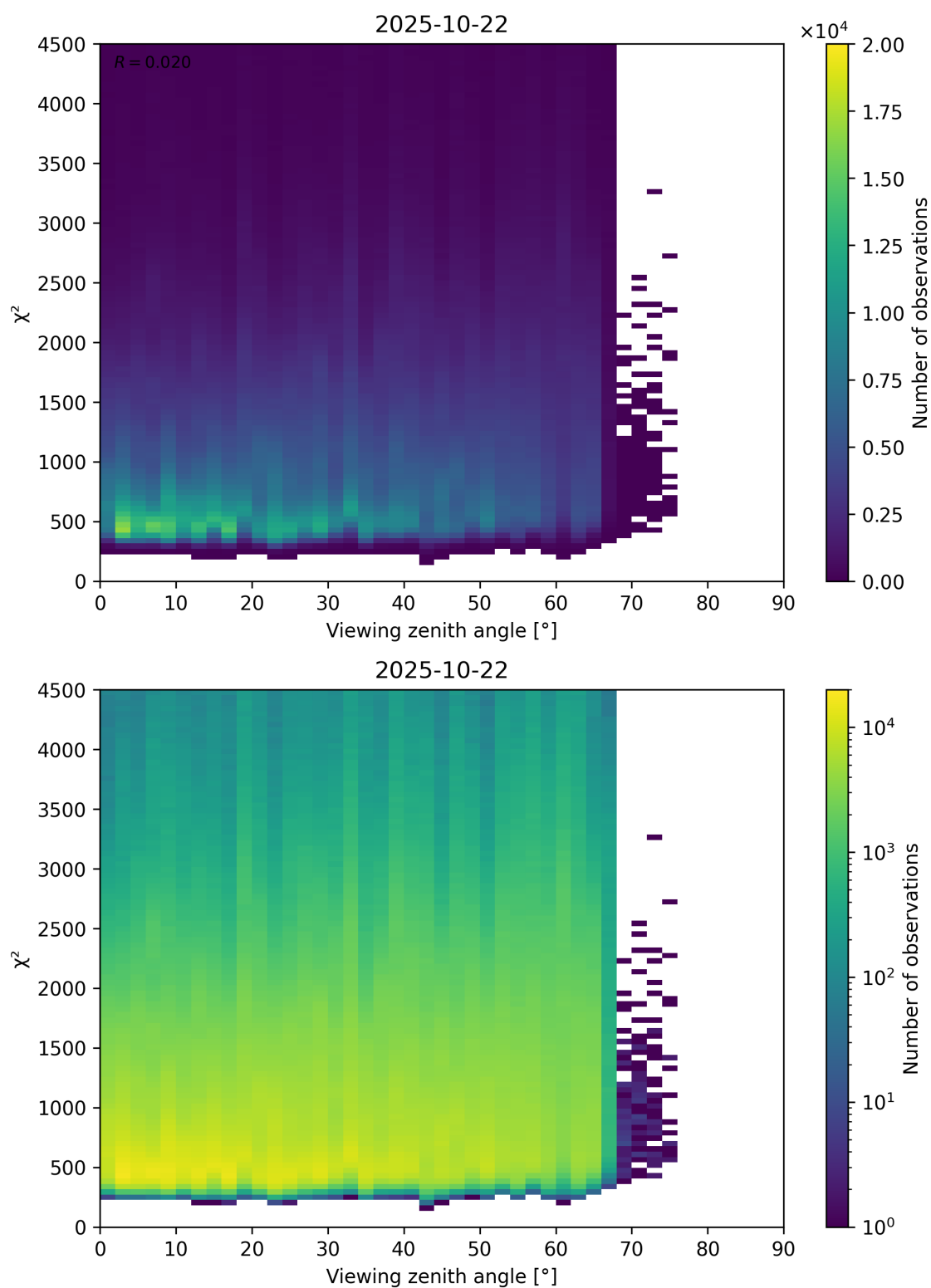
Figure 72: Scatter density plot of “Viewing zenith angle” against “ \chi^2 ” for 2025-10-22 to 2025-10-23.
