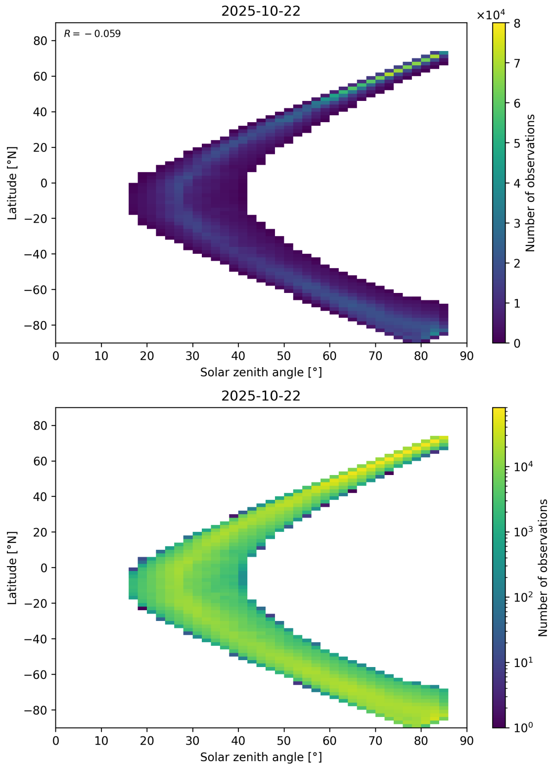
Figure 66: Scatter density plot of “Solar zenith angle” against “Latitude” for 2025-10-22 to 2025-10-23.
