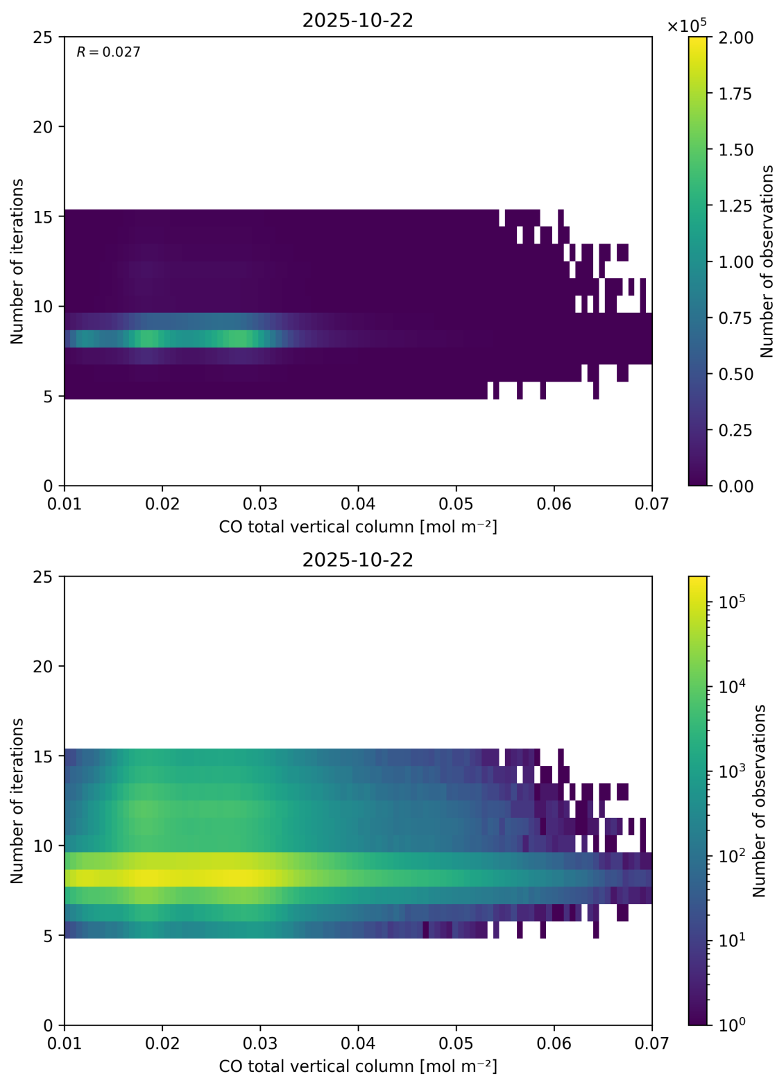
Figure 42: Scatter density plot of “CO total vertical column” against “Number of iterations” for 2025-10-22 to 2025-10-23.
