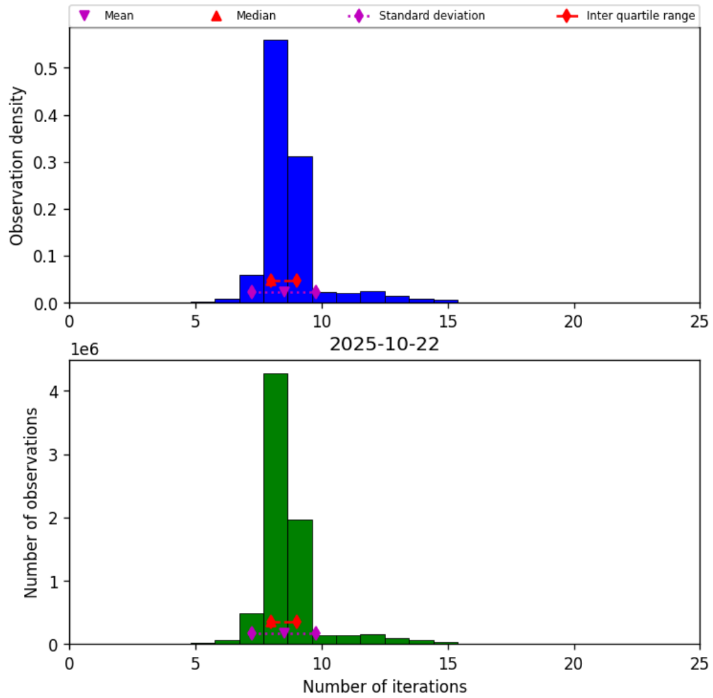
Figure 24: Histogram of “Number of iterations” for 2025-10-22 to 2025-10-23
