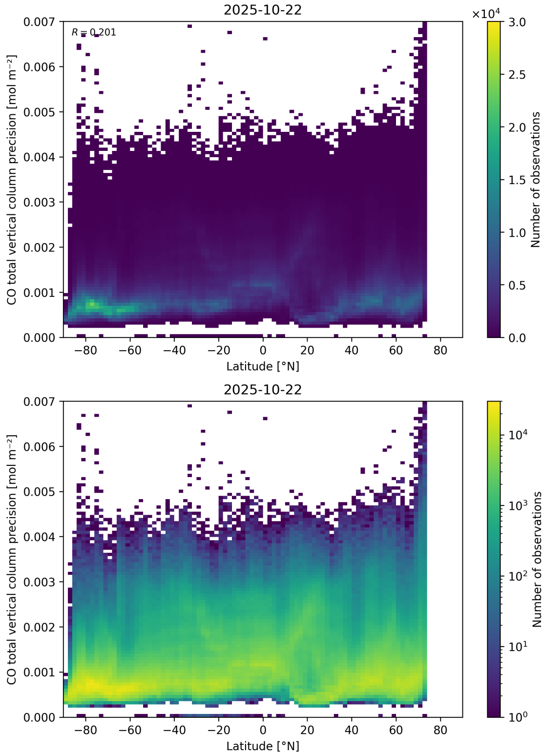
Figure 53: Scatter density plot of “Latitude” against “CO total vertical column precision” for 2025-10-22 to 2025-10-23.
