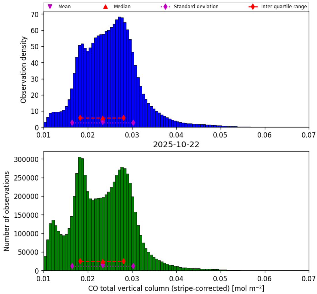
Figure 19: Histogram of “CO total vertical column (stripe-corrected)” for 2025-10-22 to 2025-10-23
