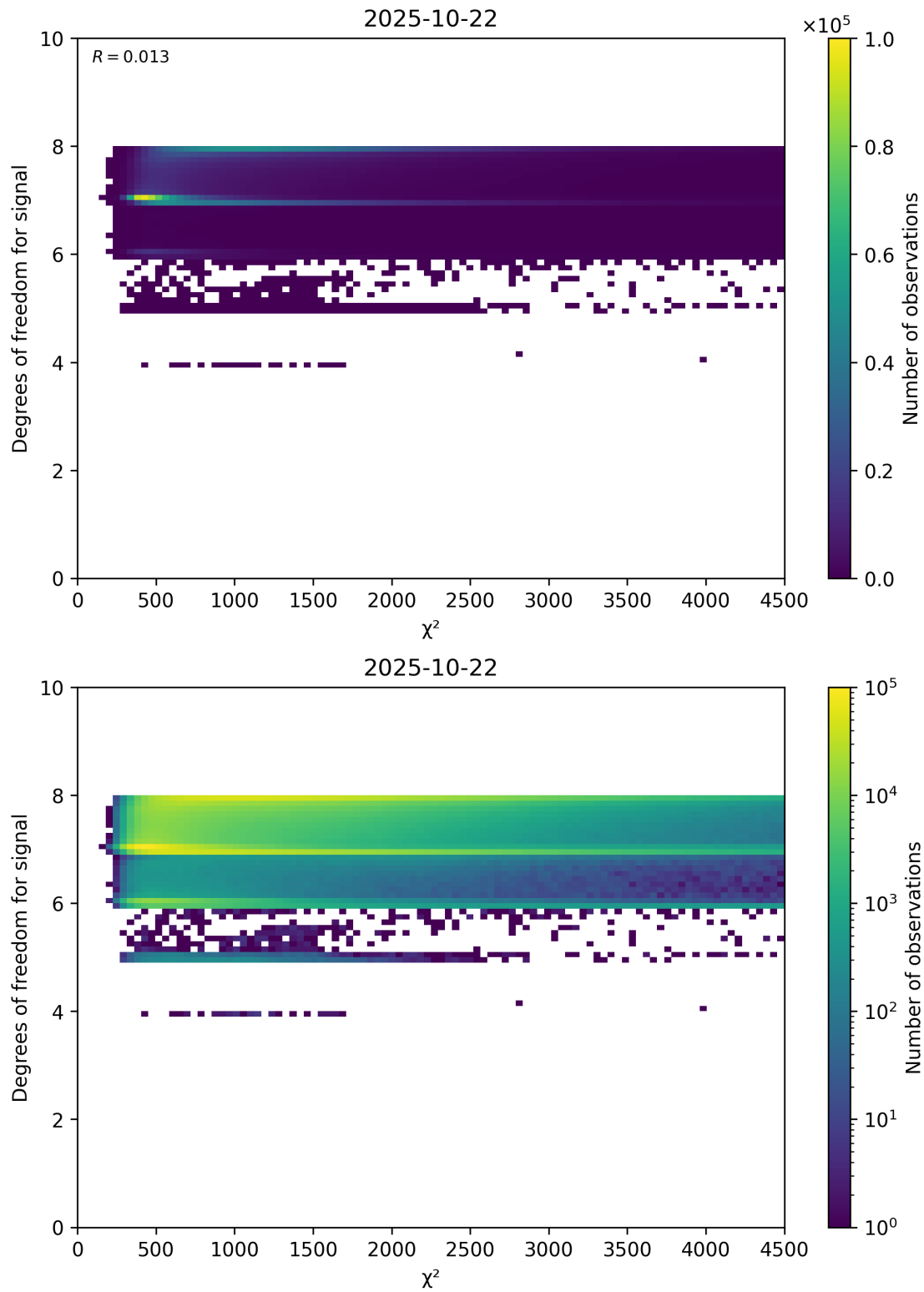
Figure 48: Scatter density plot of “ \chi^2 ” against “Degrees of freedom for signal” for 2025-10-22 to 2025-10-23.
