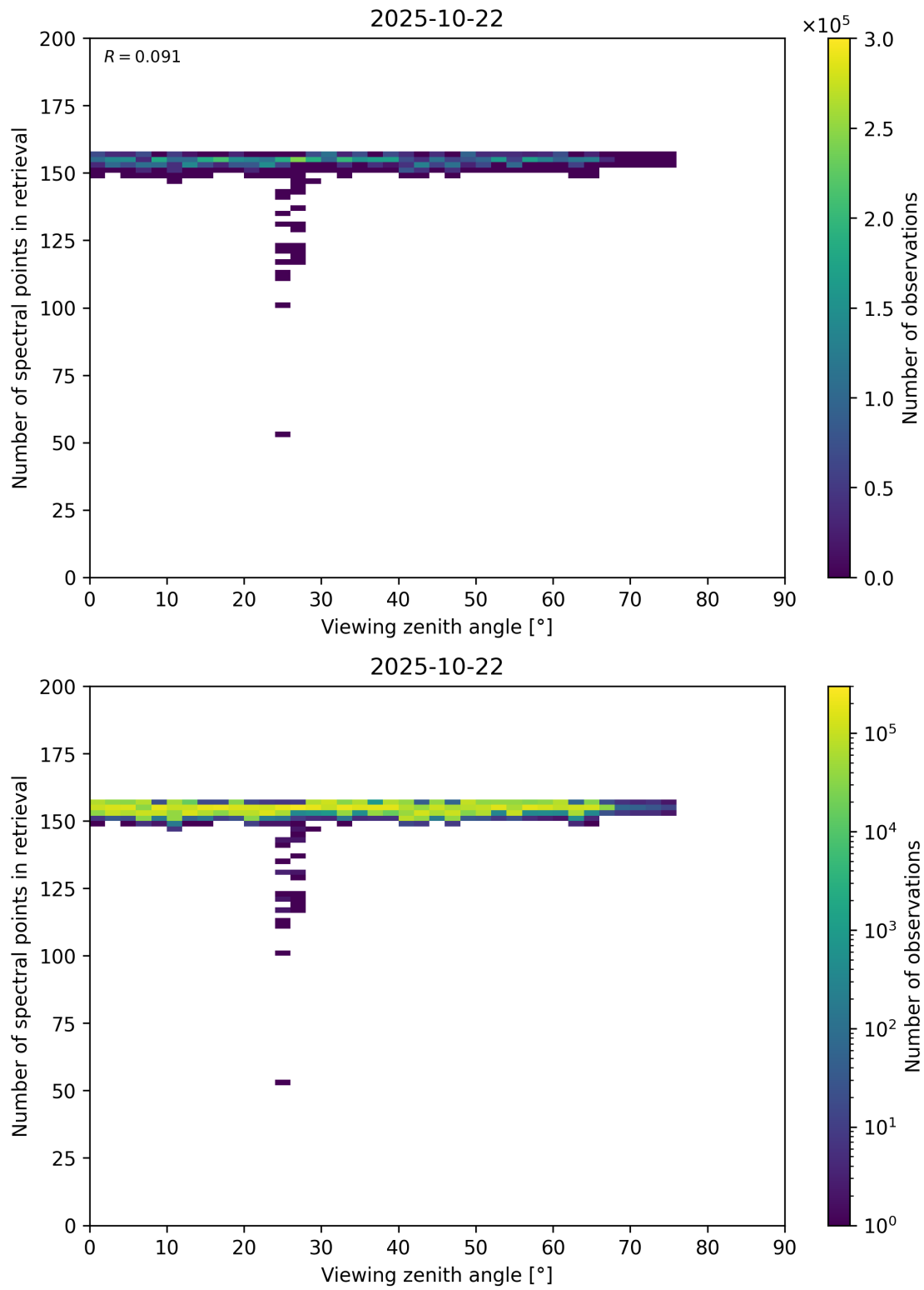
Figure 76: Scatter density plot of “Viewing zenith angle” against “Number of spectral points in retrieval” for 2025-10-22 to 2025-10-23.
