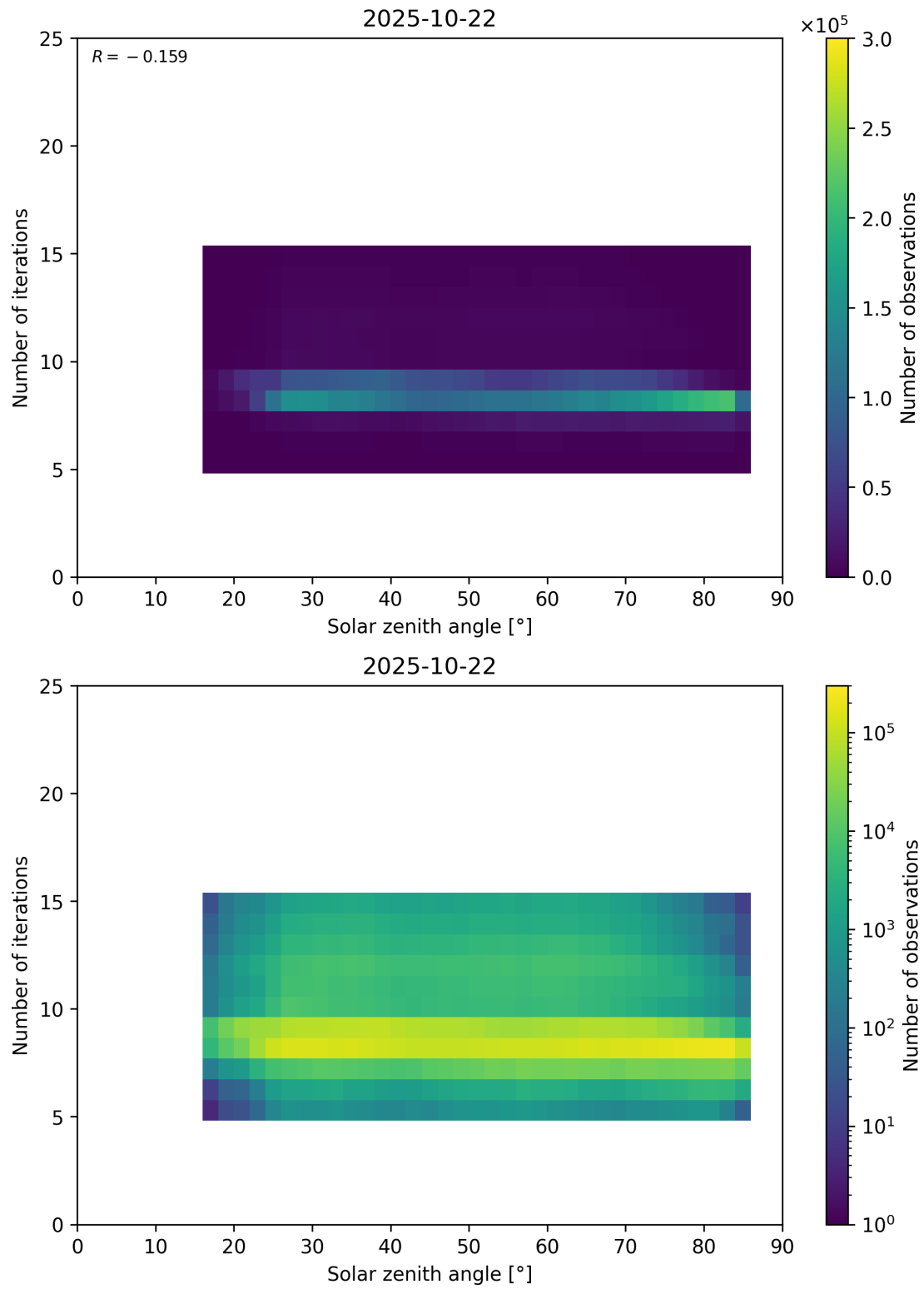
Figure 67: Scatter density plot of “Solar zenith angle” against “Number of iterations” for 2025-10-22 to 2025-10-23.
