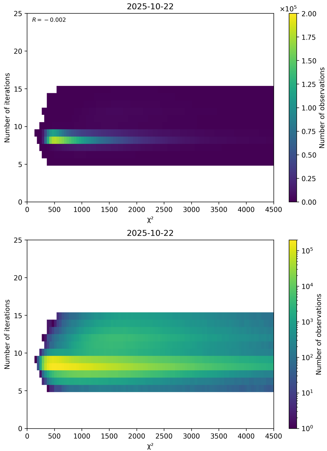
Figure 49: Scatter density plot of “ \chi^2 ” against “Number of iterations” for 2025-10-22 to 2025-10-23.
