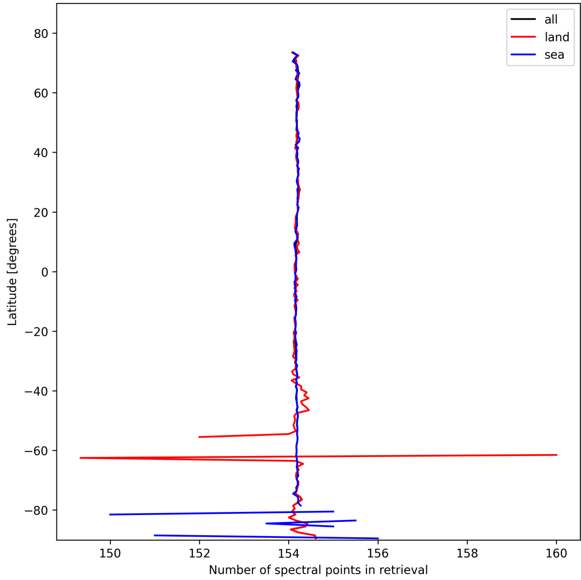
Figure 13: Zonal average of “Number of spectral points in retrieval” for 2025-10-22 to 2025-10-23.
