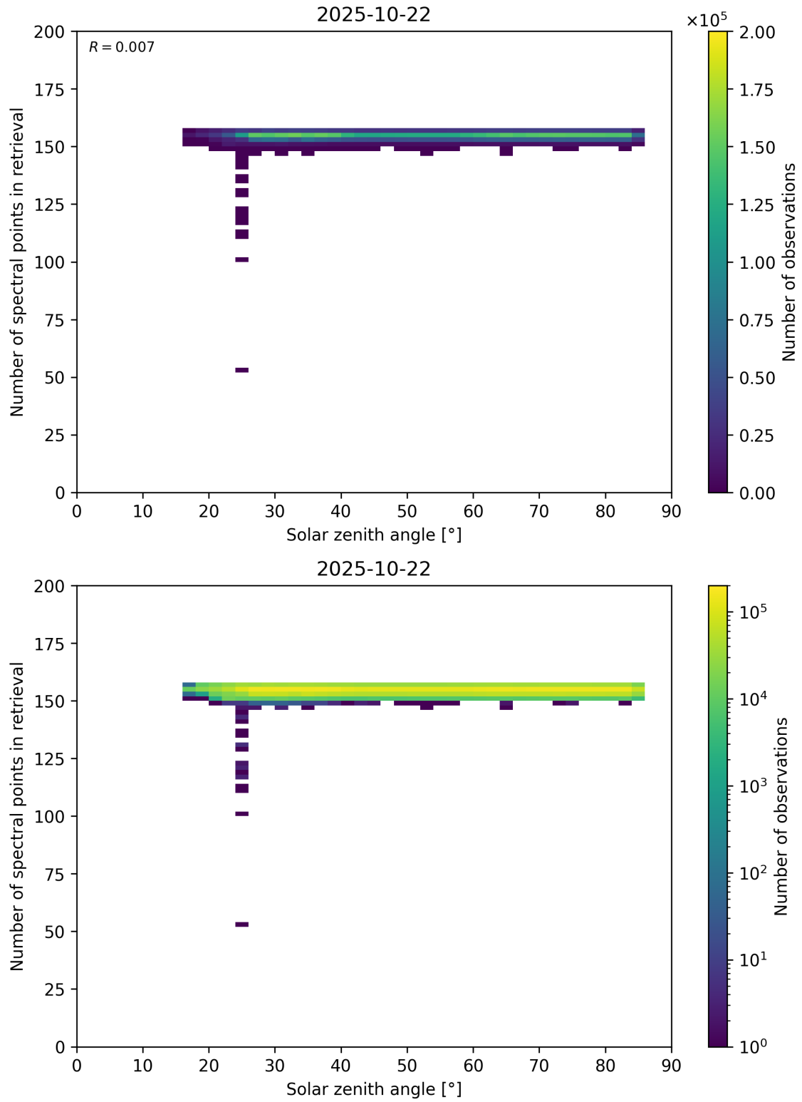
Figure 68: Scatter density plot of “Solar zenith angle” against “Number of spectral points in retrieval” for 2025-10-22 to 2025-10-23.
