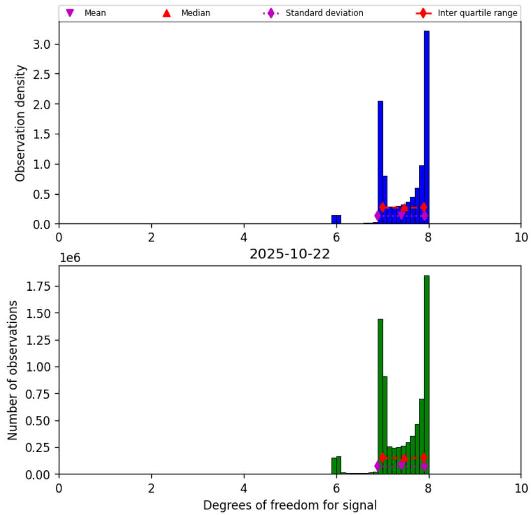
Figure 23: Histogram of “Degrees of freedom for signal” for 2025-10-22 to 2025-10-23
