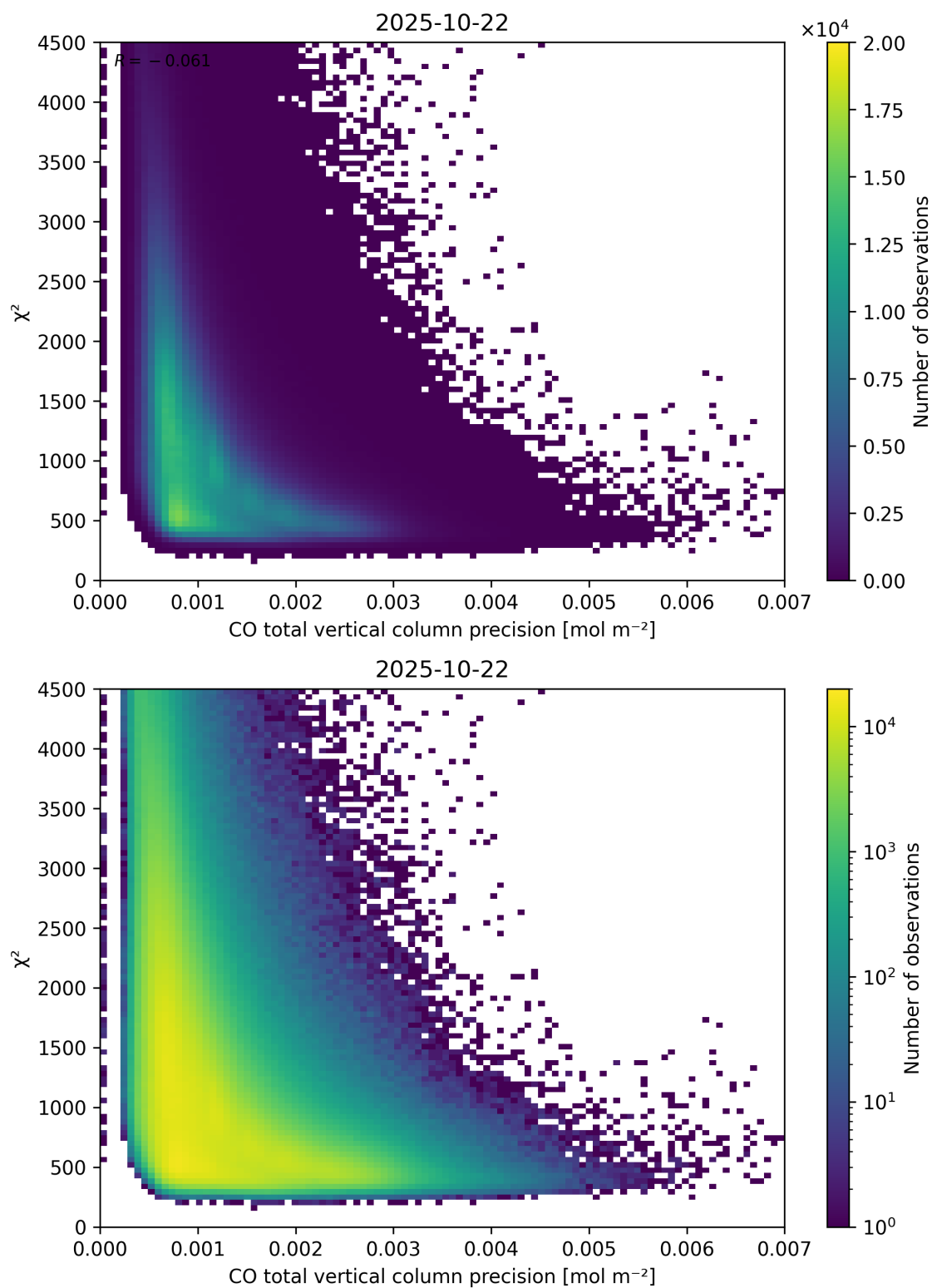
Figure 44: Scatter density plot of “CO total vertical column precision” against “ \chi^2 ” for 2025-10-22 to 2025-10-23.
