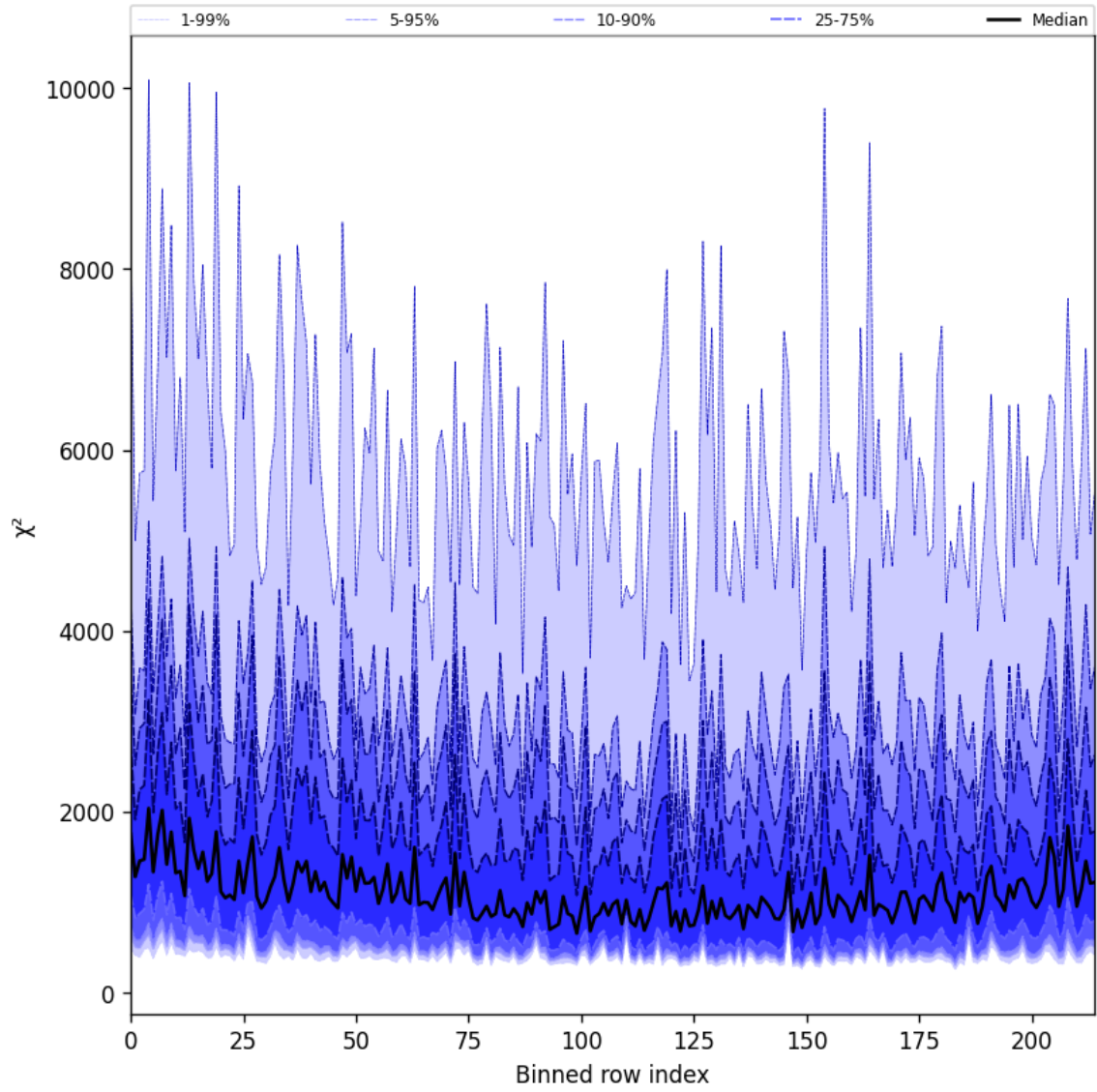
Figure 30: Along track statistics of “ \chi^2 ” for 2025-10-22 to 2025-10-23
