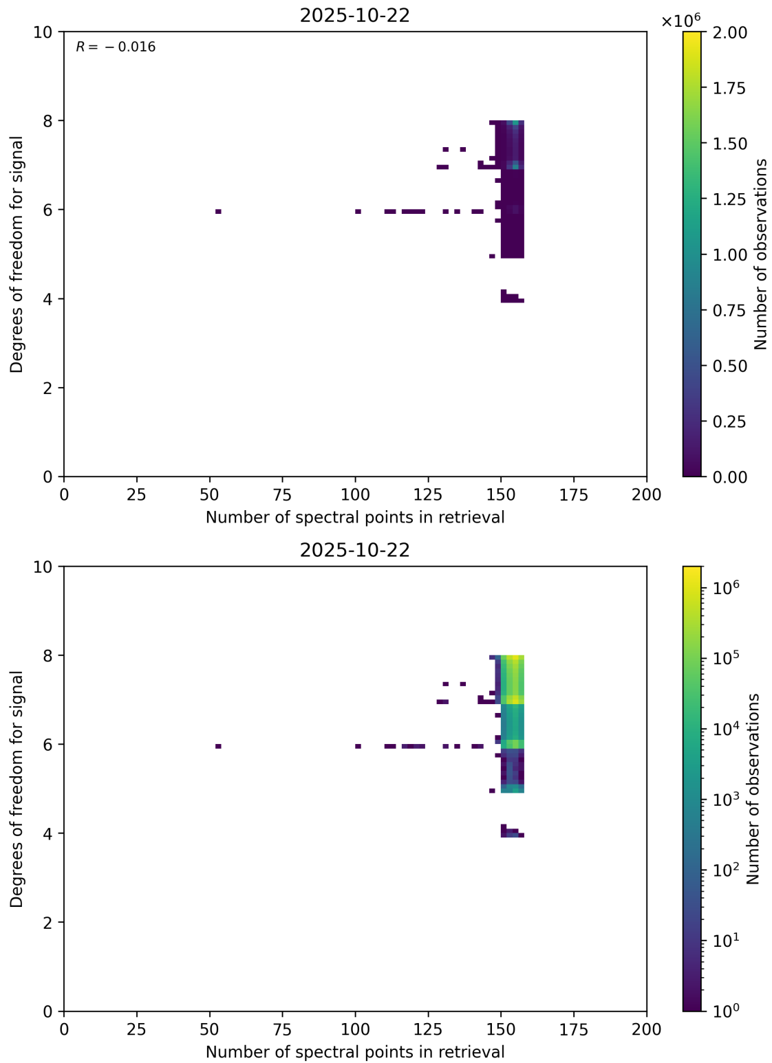
Figure 59: Scatter density plot of “Number of spectral points in retrieval” against “Degrees of freedom for signal” for 2025-10-22 to 2025-10-23.
