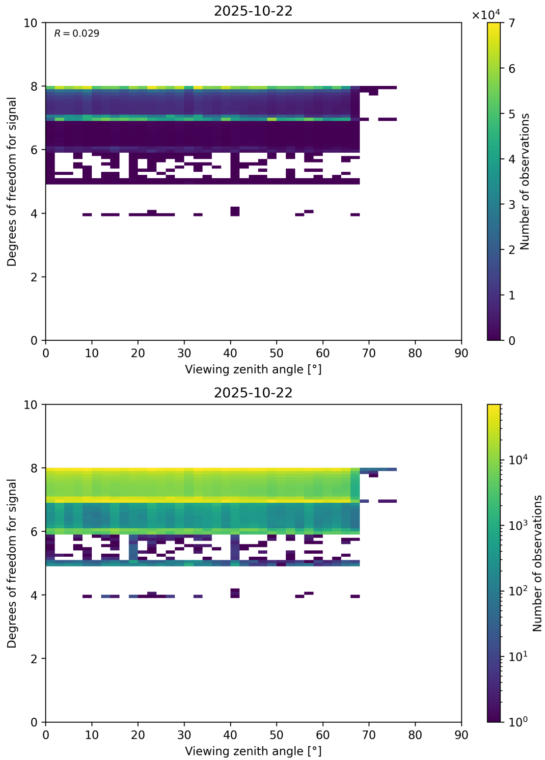
Figure 73: Scatter density plot of “Viewing zenith angle” against “Degrees of freedom for signal” for 2025-10-22 to 2025-10-23.
