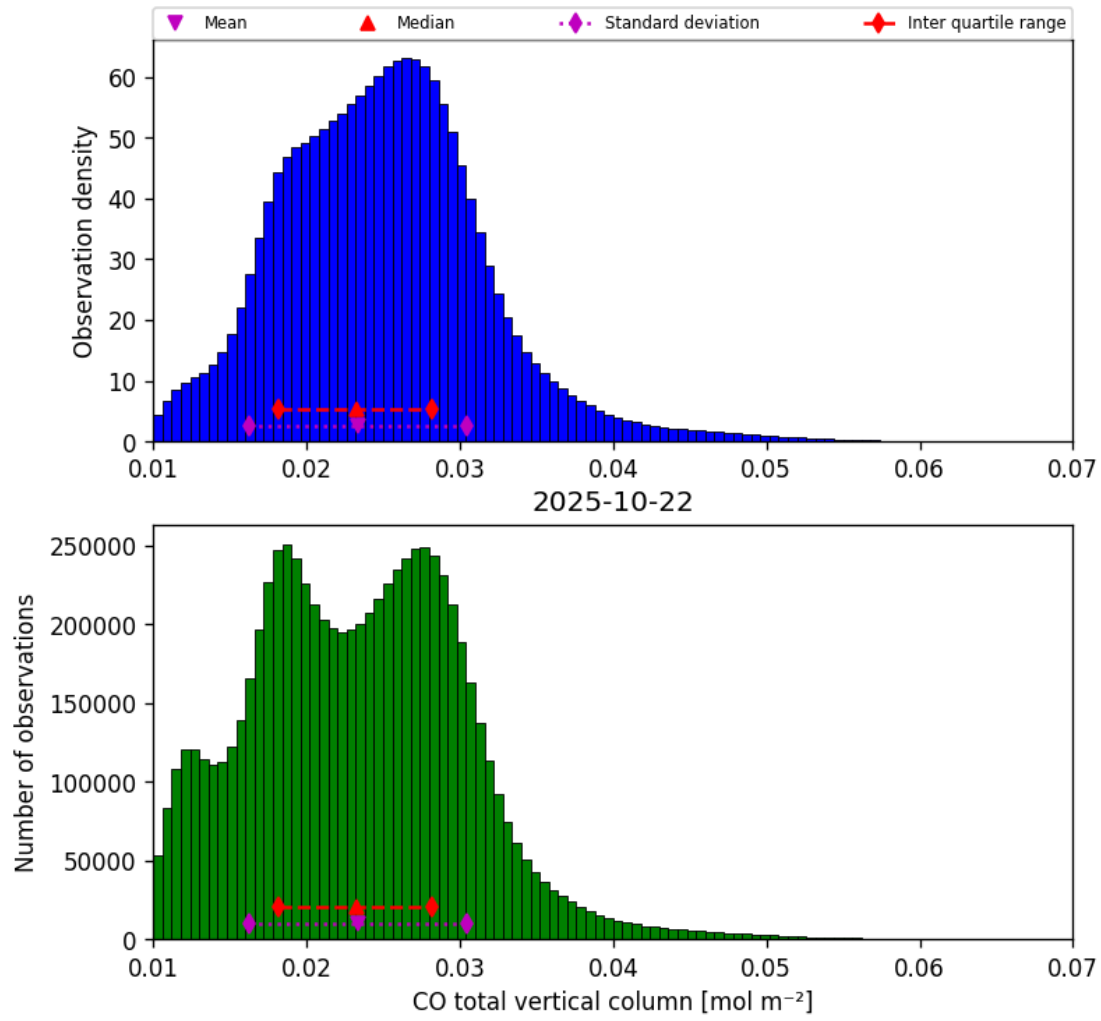
Figure 18: Histogram of “CO total vertical column” for 2025-10-22 to 2025-10-23
