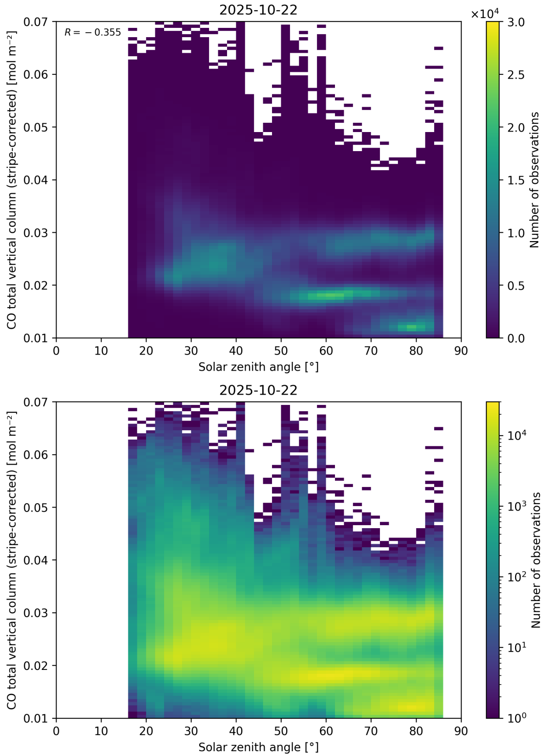
Figure 62: Scatter density plot of “Solar zenith angle” against “CO total vertical column (stripe-corrected)” for 2025-10-22 to 2025-10-23.
