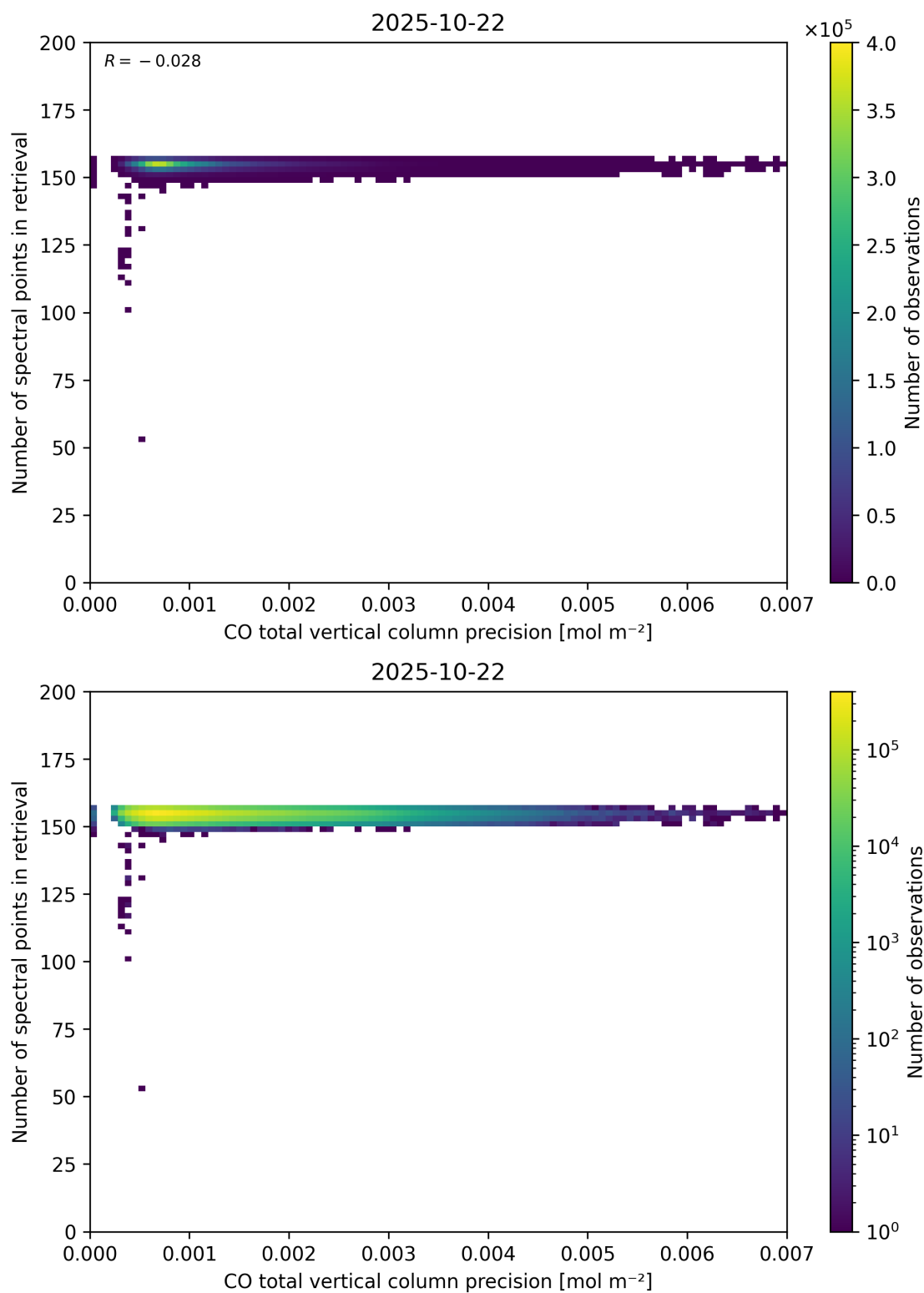
Figure 47: Scatter density plot of “CO total vertical column precision” against “Number of spectral points in retrieval” for 2025-10-22 to 2025-10-23.
