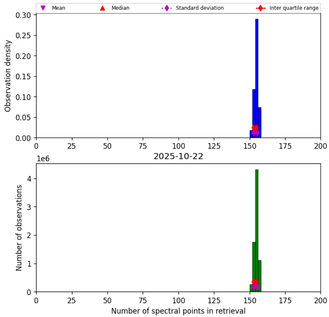
Figure 21: Histogram of “Number of spectral points in retrieval” for 2025-10-22 to 2025-10-23
