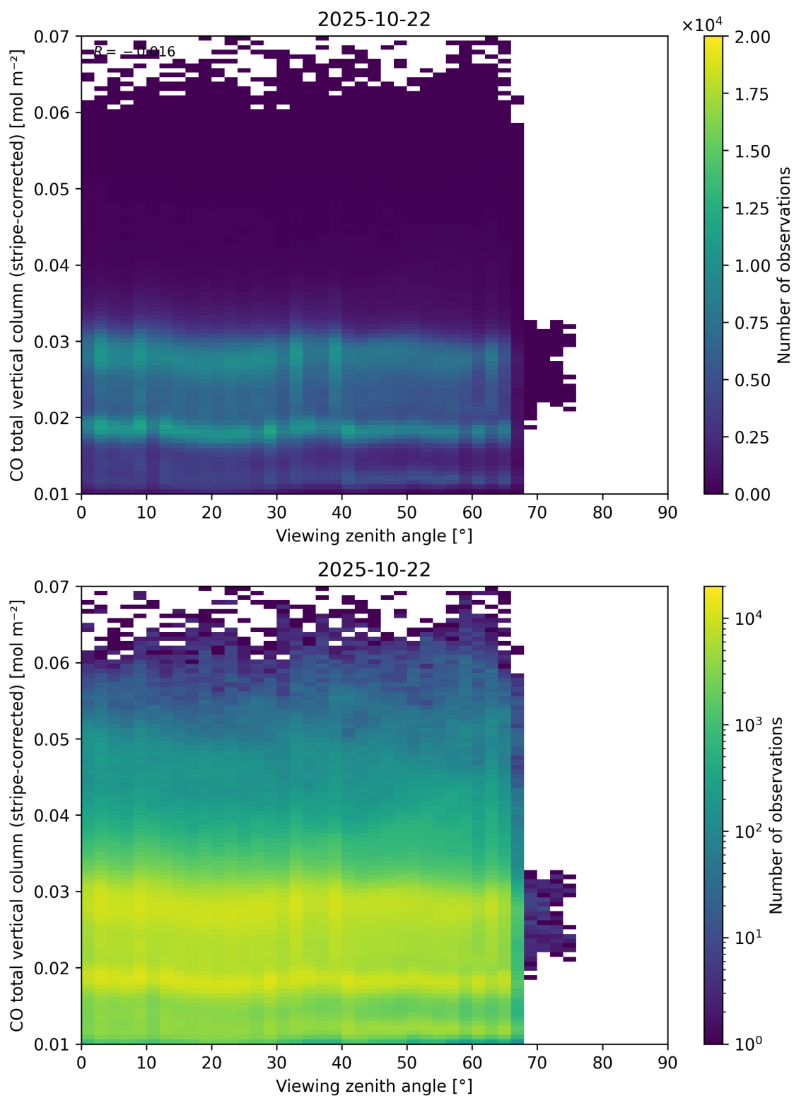
Figure 70: Scatter density plot of “Viewing zenith angle” against “CO total vertical column (stripe-corrected)” for 2025-10-22 to 2025-10-23.
