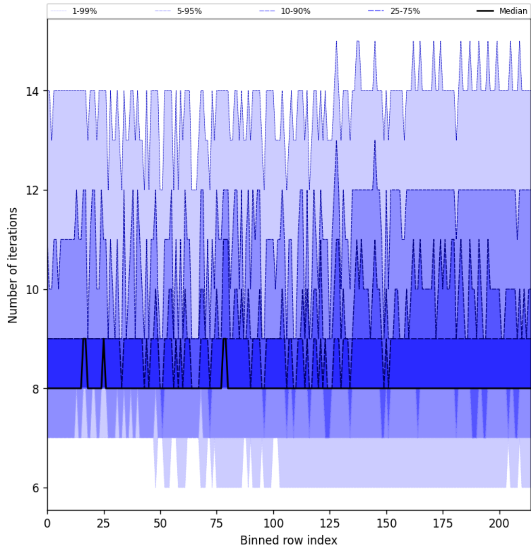
Figure 32: Along track statistics of “Number of iterations” for 2025-10-22 to 2025-10-23
