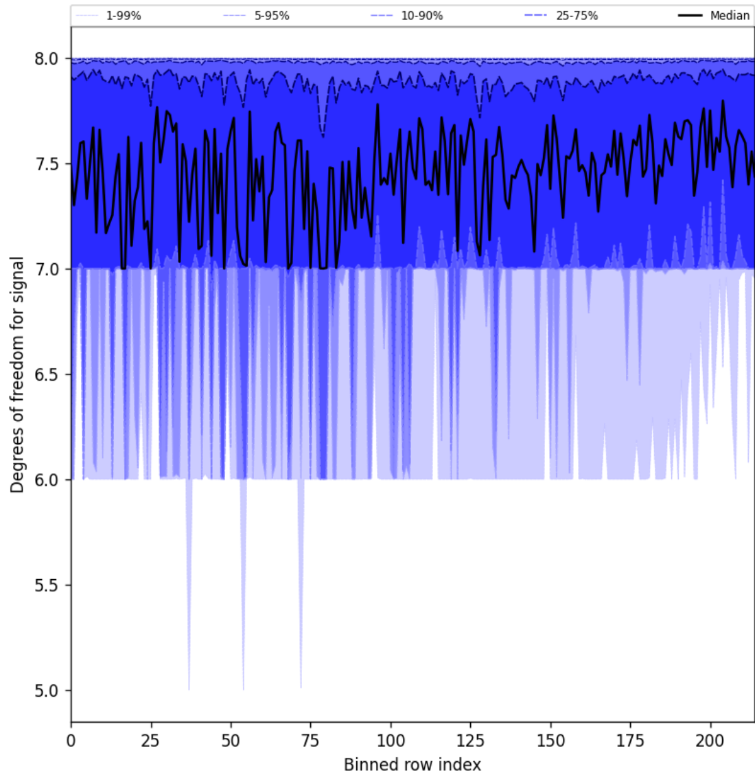
Figure 31: Along track statistics of “Degrees of freedom for signal” for 2025-10-22 to 2025-10-23
