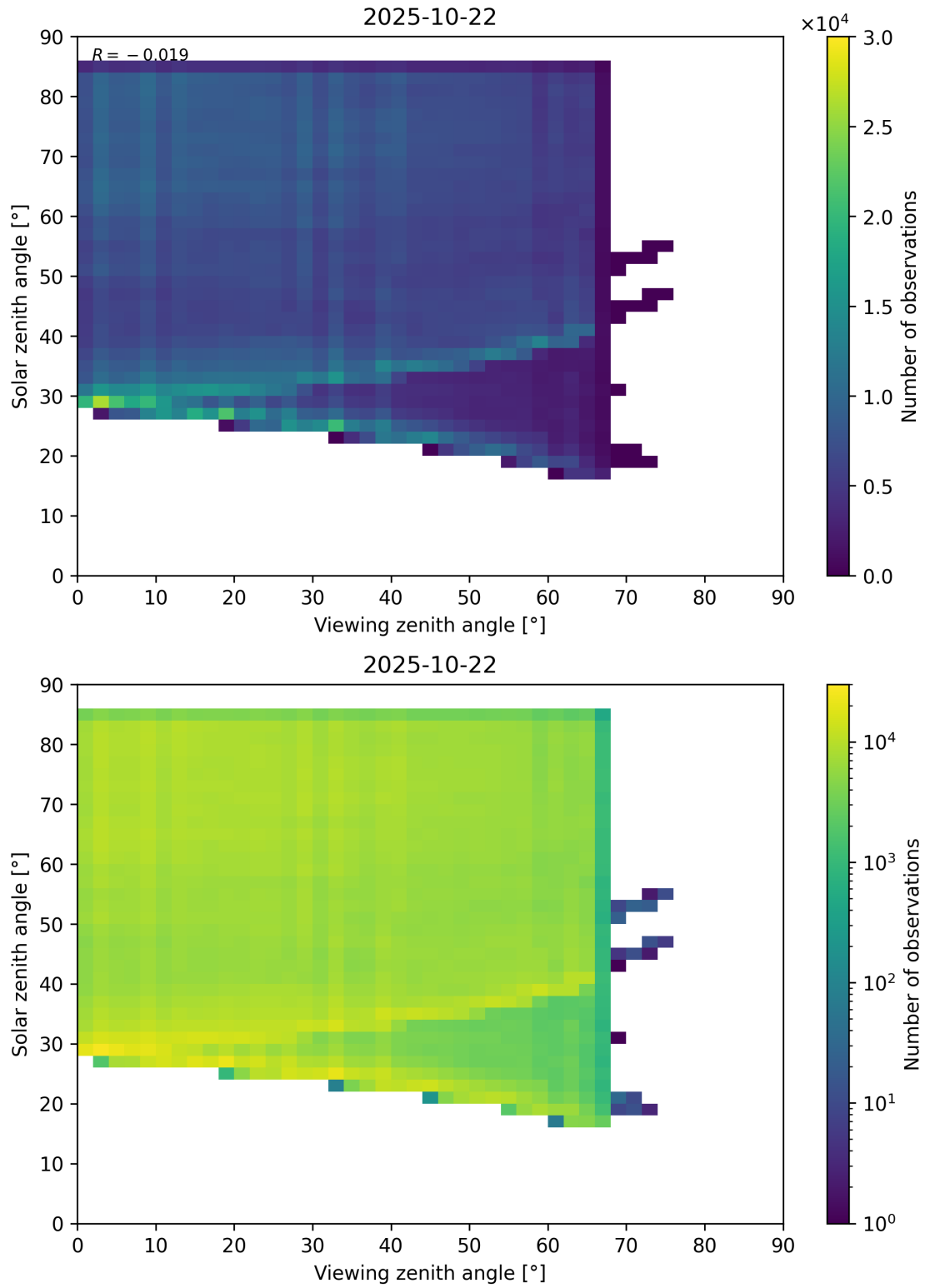
Figure 77: Scatter density plot of “Viewing zenith angle” against “Solar zenith angle” for 2025-10-22 to 2025-10-23.
