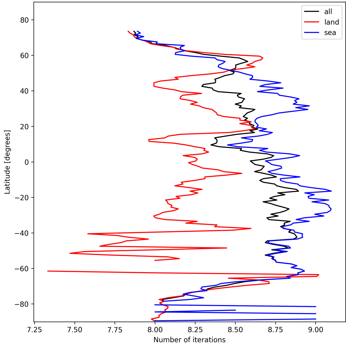
Figure 16: Zonal average of “Number of iterations” for 2025-10-22 to 2025-10-23.
