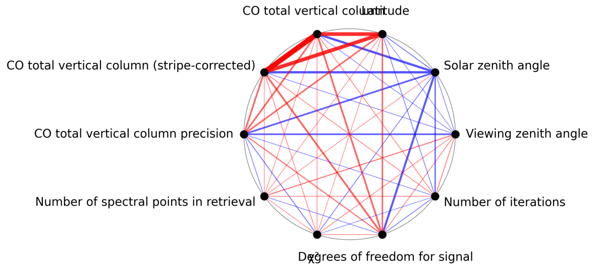
Figure 1: Map of correlation graph for 2025-10-22 to 2025-10-23.
