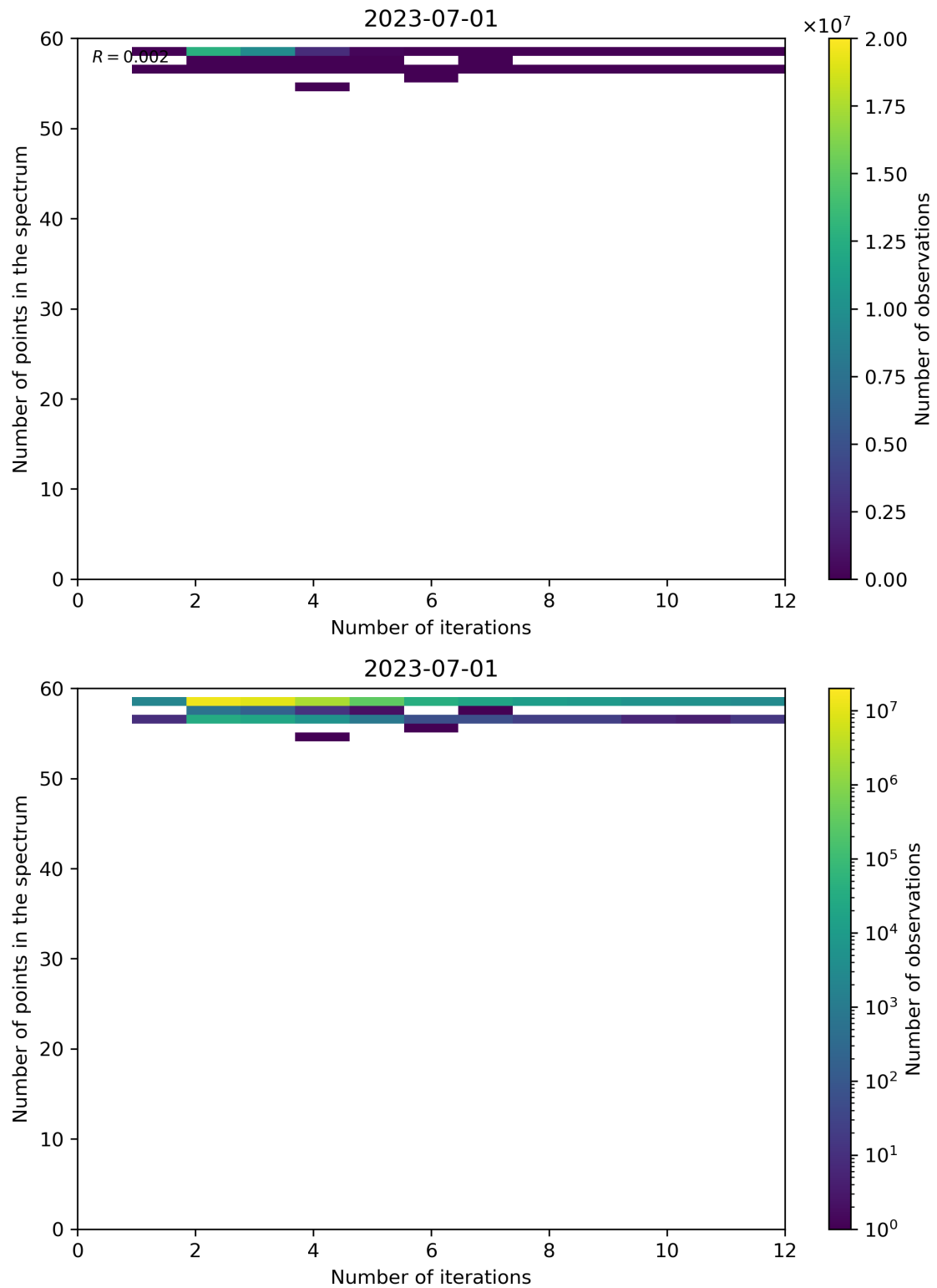
Figure 108: Scatter density plot of “Number of iterations” against “Number of points in the spectrum” for 2023-06-30 to 2023-07-02.
