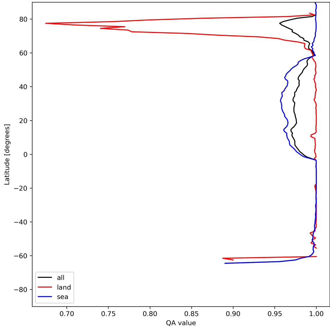
Figure 12: Zonal average of “QA value” for 2023-06-30 to 2023-07-02.
