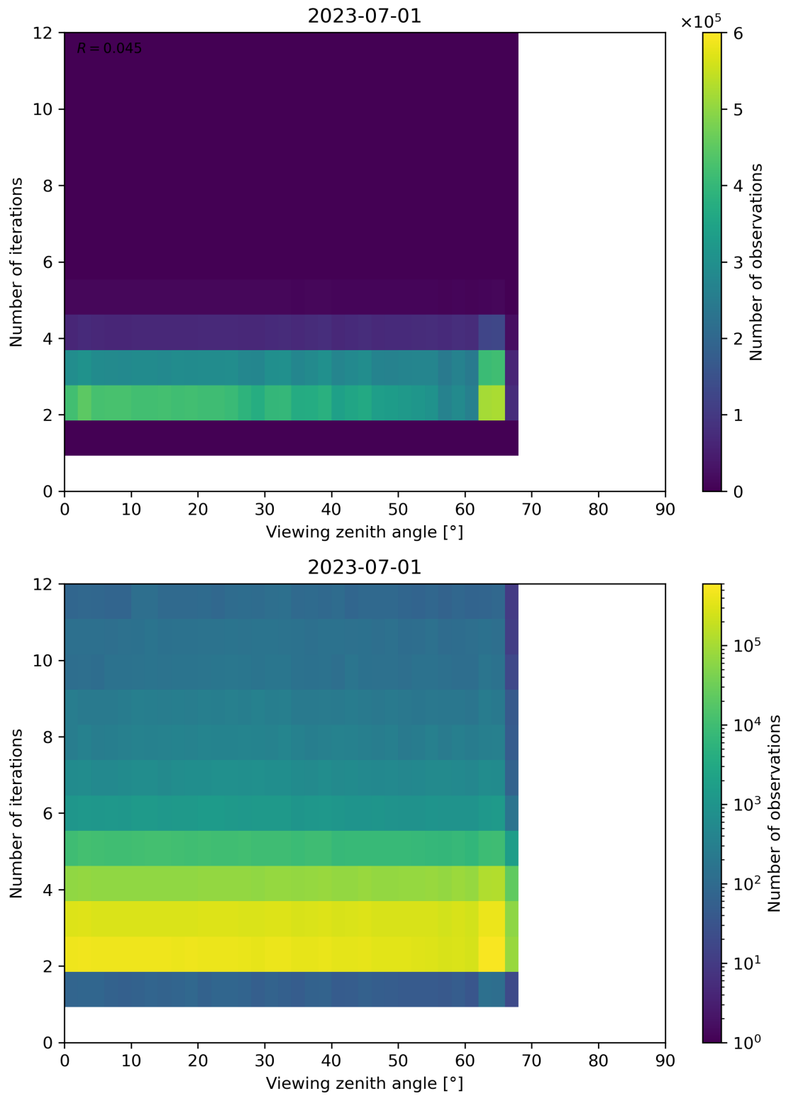
Figure 136: Scatter density plot of “Viewing zenith angle” against “Number of iterations” for 2023-06-30 to 2023-07-02.
