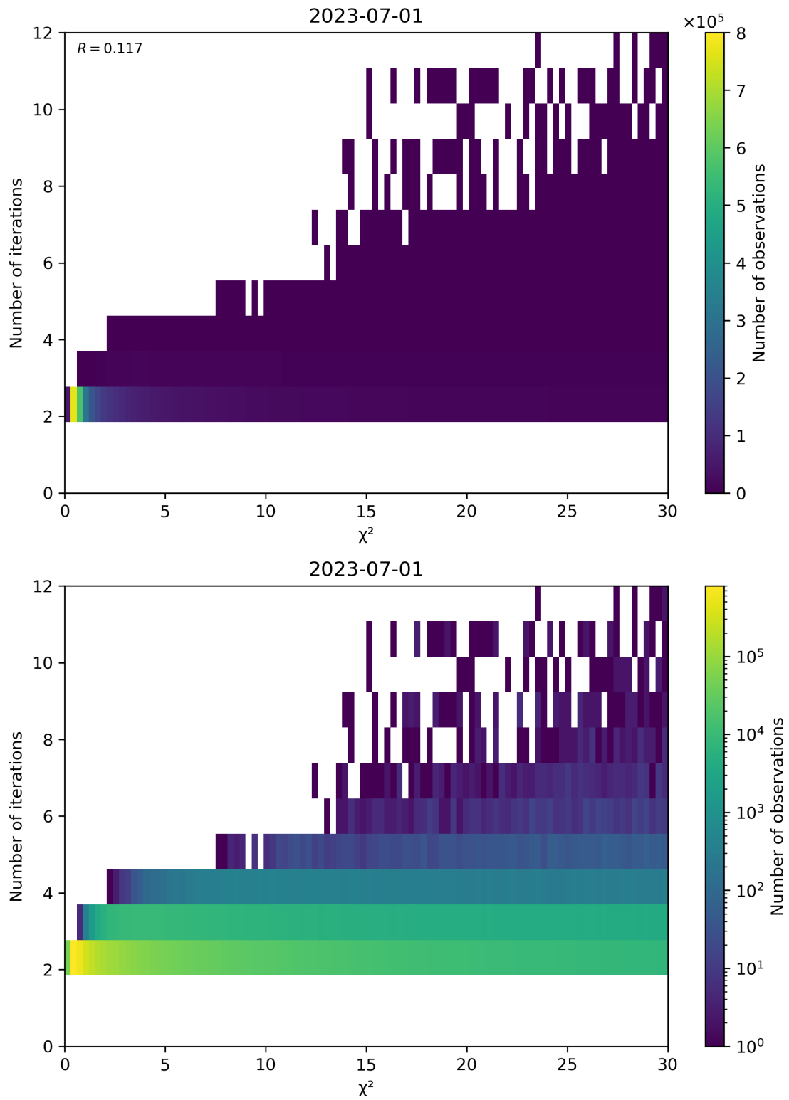
Figure 73: Scatter density plot of “ \chi^2 ” against “Number of iterations” for 2023-06-30 to 2023-07-02.
