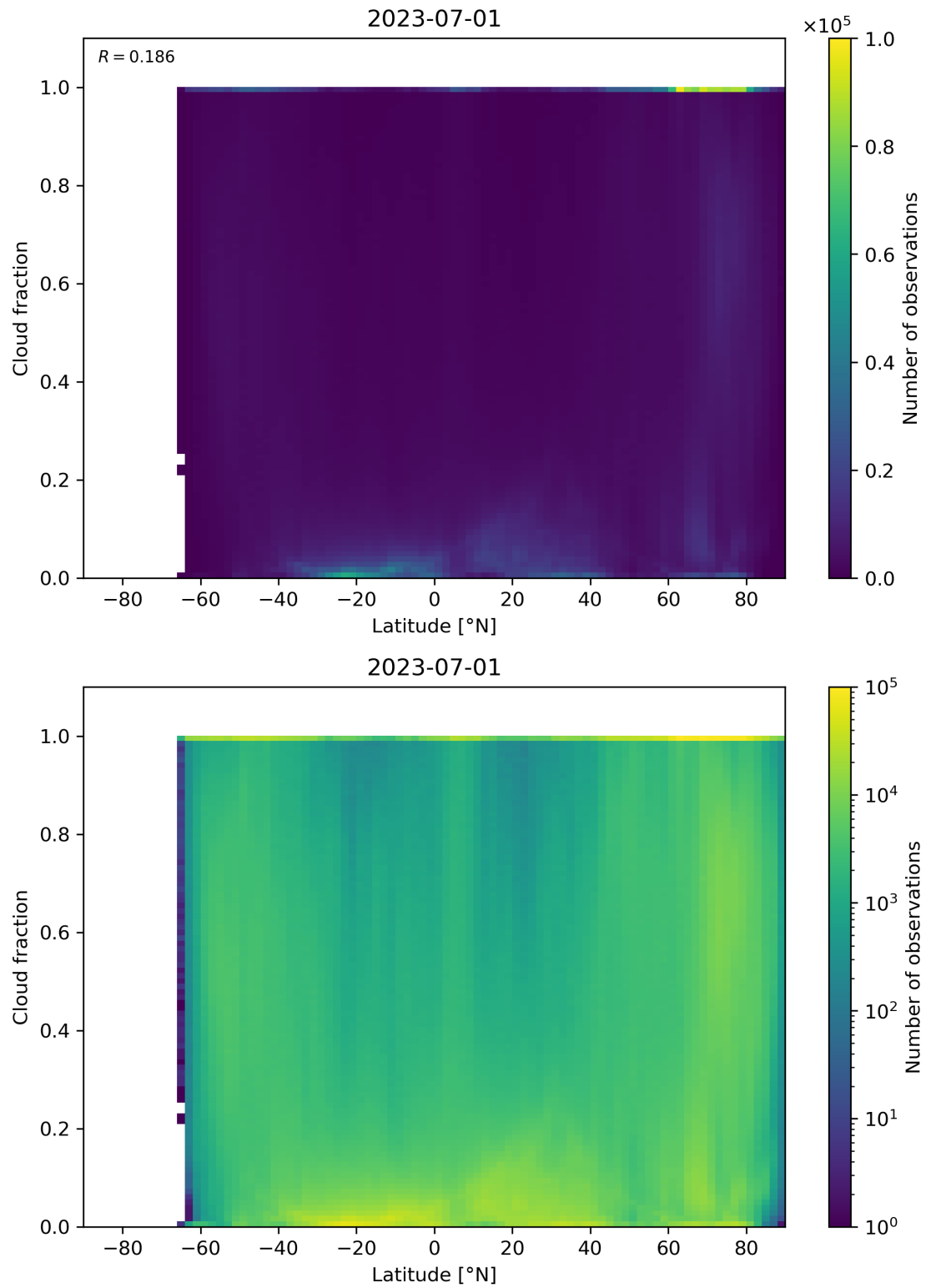
Figure 99: Scatter density plot of “Latitude” against “Cloud fraction” for 2023-06-30 to 2023-07-02.
