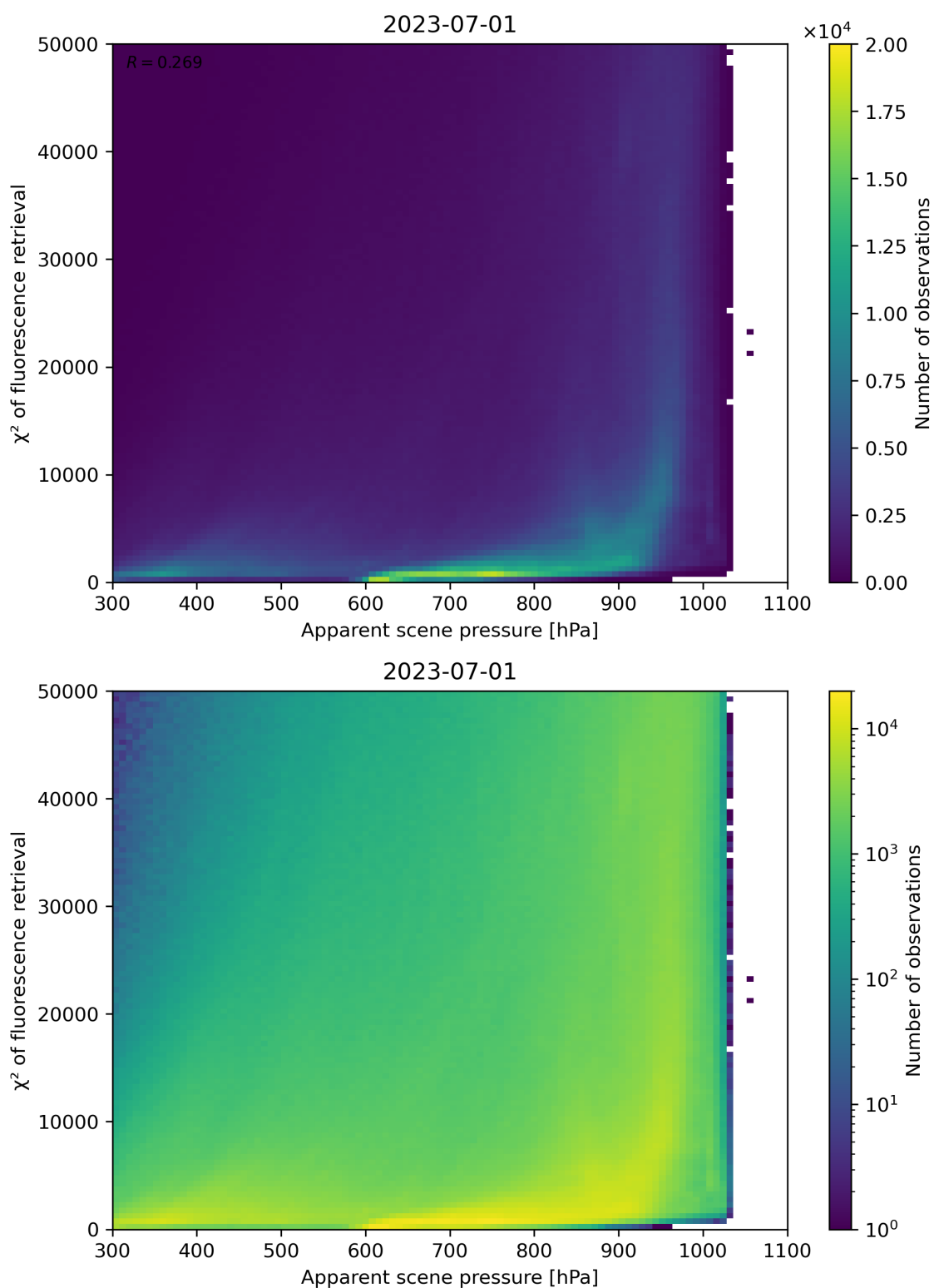
Figure 64: Scatter density plot of “Apparent scene pressure” against “ \chi^2 of fluorescence retrieval” for 2023-06-30 to 2023-07-02.
