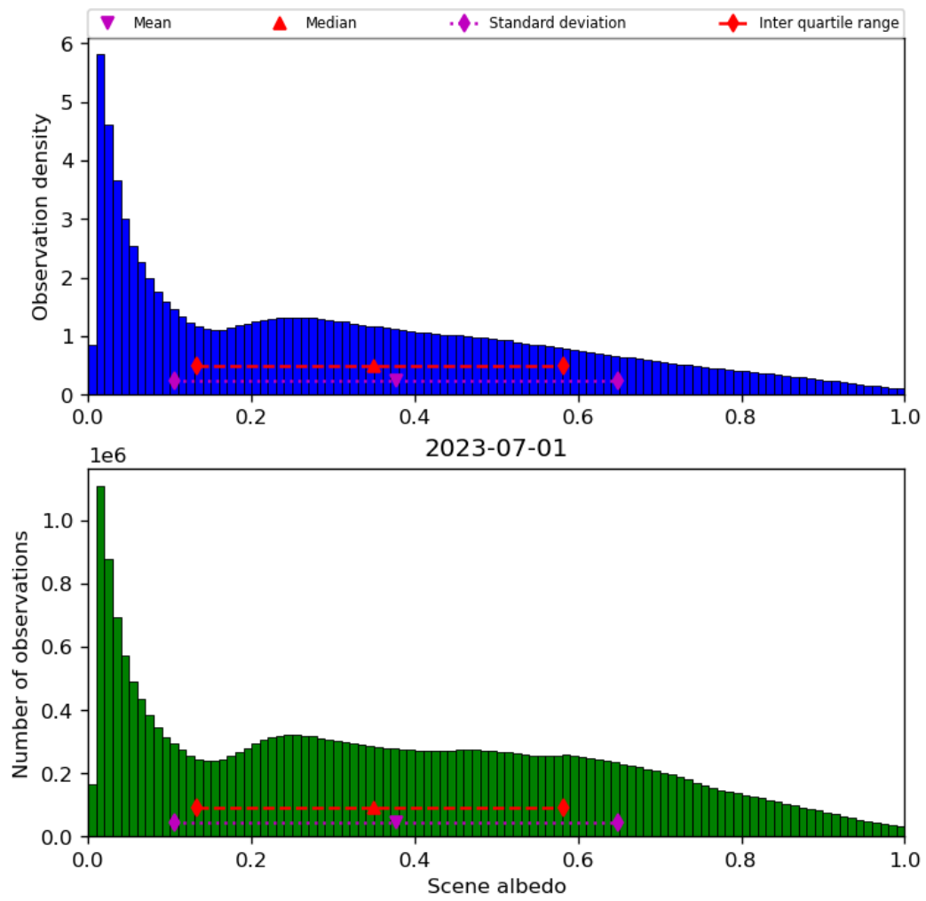
Figure 34: Histogram of “Scene albedo” for 2023-06-30 to 2023-07-02
