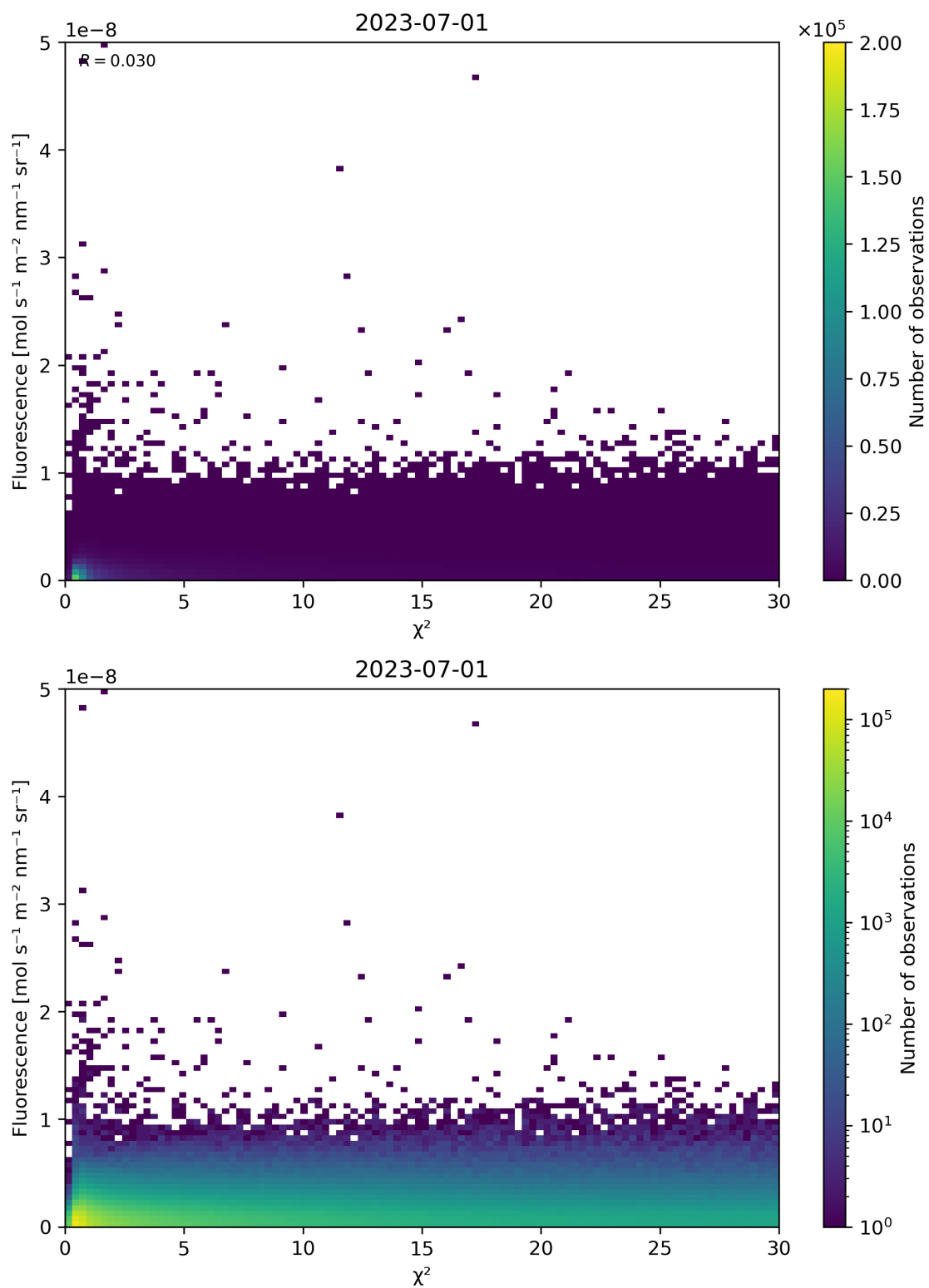
Figure 70: Scatter density plot of “ \chi^2 ” against “Fluorescence” for 2023-06-30 to 2023-07-02.
