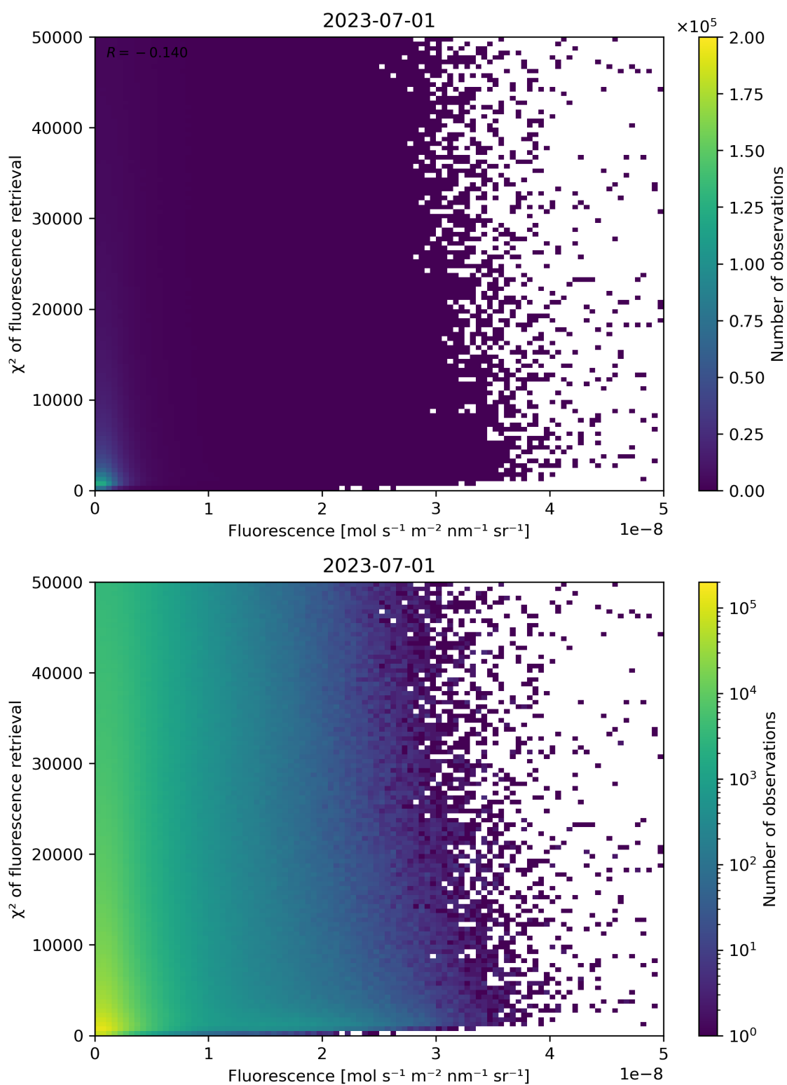
Figure 93: Scatter density plot of “Fluorescence” against “ \chi^2 of fluorescence retrieval” for 2023-06-30 to 2023-07-02.
