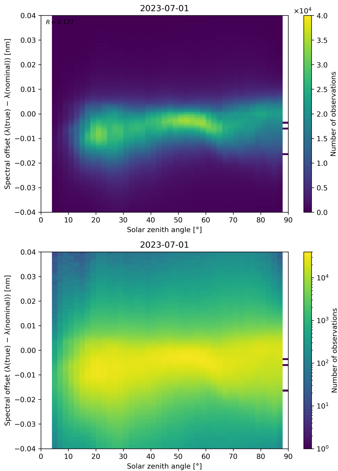
Figure 128: Scatter density plot of “Solar zenith angle” against “Spectral offset ( \lambda(\text{true}) - \lambda(\text{nominal}) )” for 2023-06-30 to 2023-07-02.
