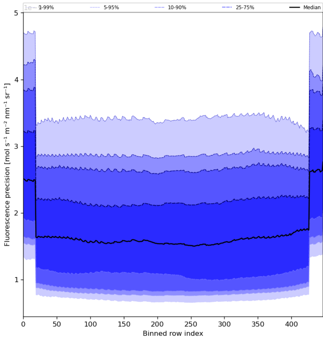
Figure 58: Along track statistics of “Fluorescence precision” for 2023-06-30 to 2023-07-02
