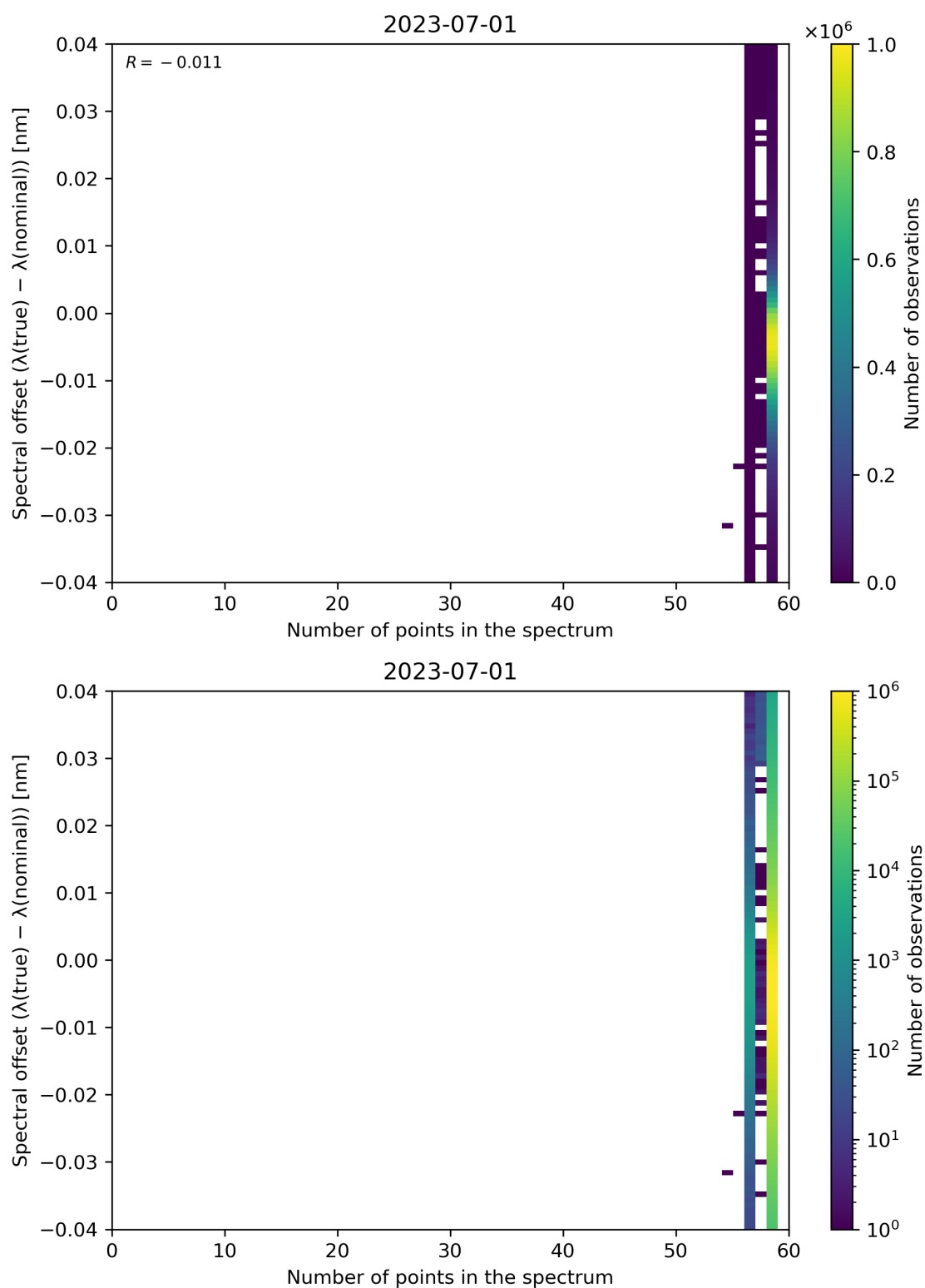
Figure 110: Scatter density plot of “Number of points in the spectrum” against “Spectral offset ( \lambda(\text{true}) - \lambda(\text{nominal}) )” for 2023-06-30 to 2023-07-02.
