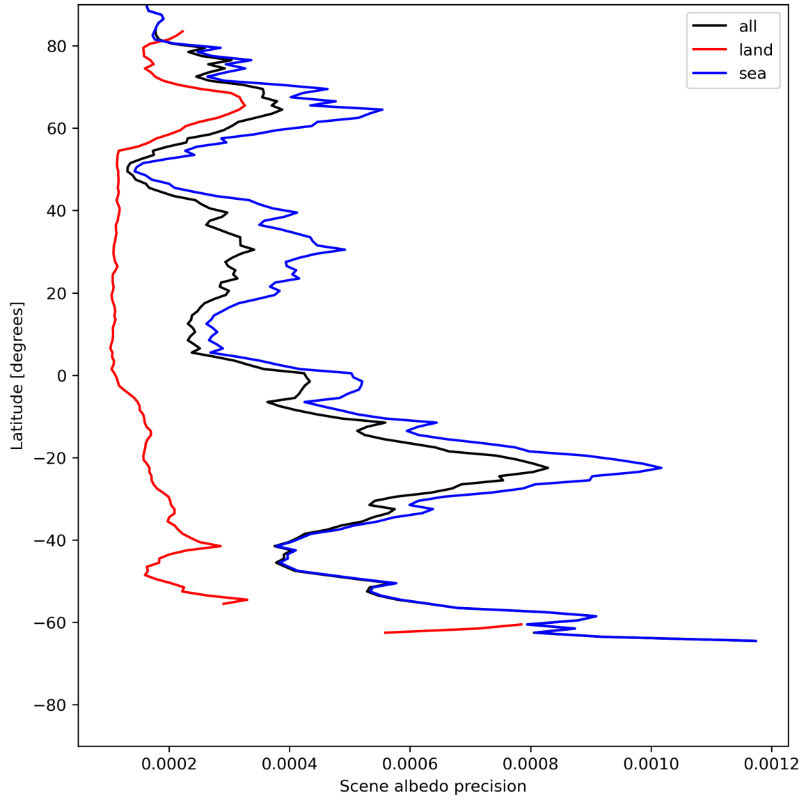
Figure 18: Zonal average of “Scene albedo precision” for 2023-06-30 to 2023-07-02.
