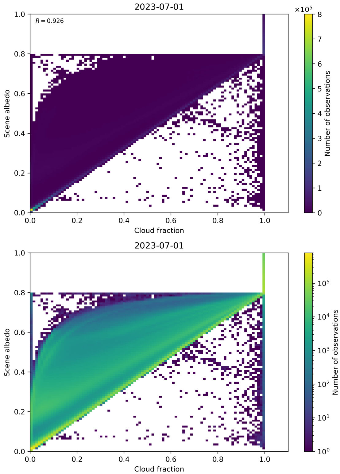
Figure 82: Scatter density plot of “Cloud fraction” against “Scene albedo” for 2023-06-30 to 2023-07-02.
