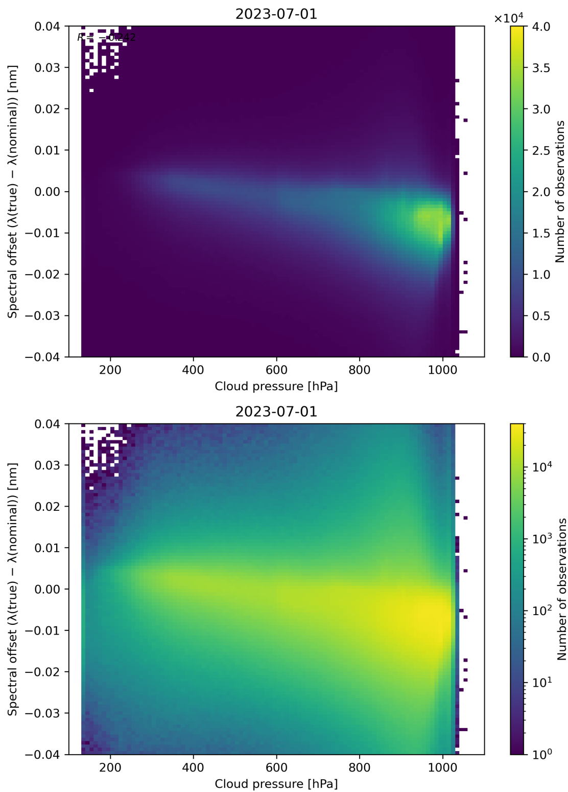
Figure 92: Scatter density plot of “Cloud pressure” against “Spectral offset ( \lambda(\text{true}) - \lambda(\text{nominal}) )” for 2023-06-30 to 2023-07-02.
