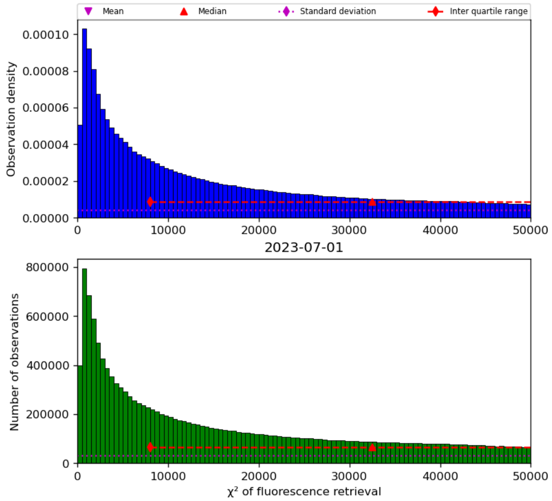
Figure 42: Histogram of “ \chi^2 of fluorescence retrieval” for 2023-06-30 to 2023-07-02
