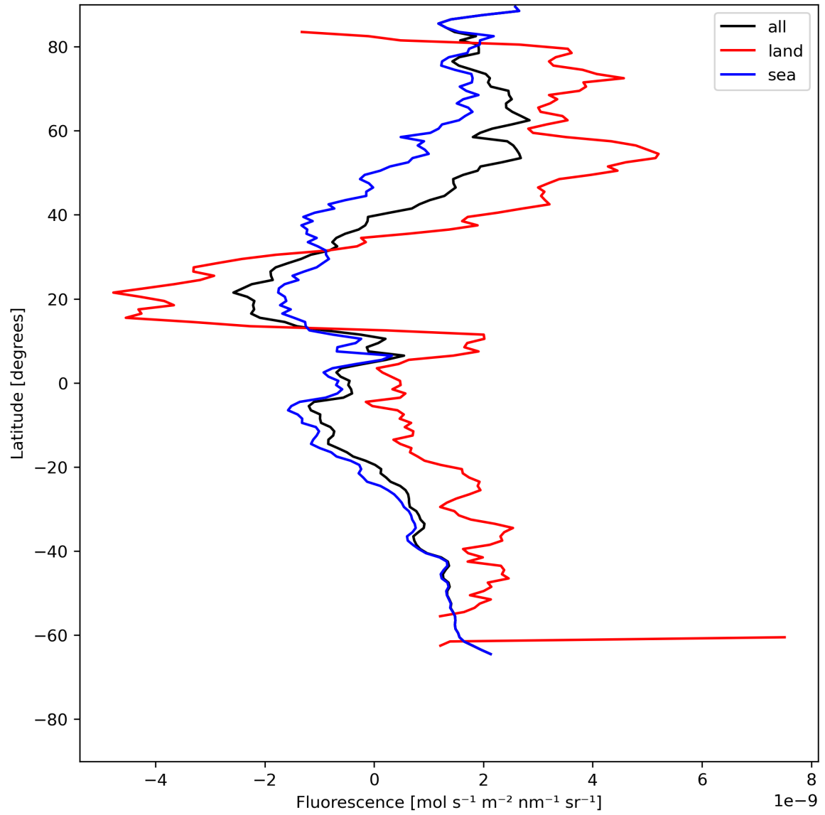
Figure 23: Zonal average of “Fluorescence” for 2023-06-30 to 2023-07-02.
