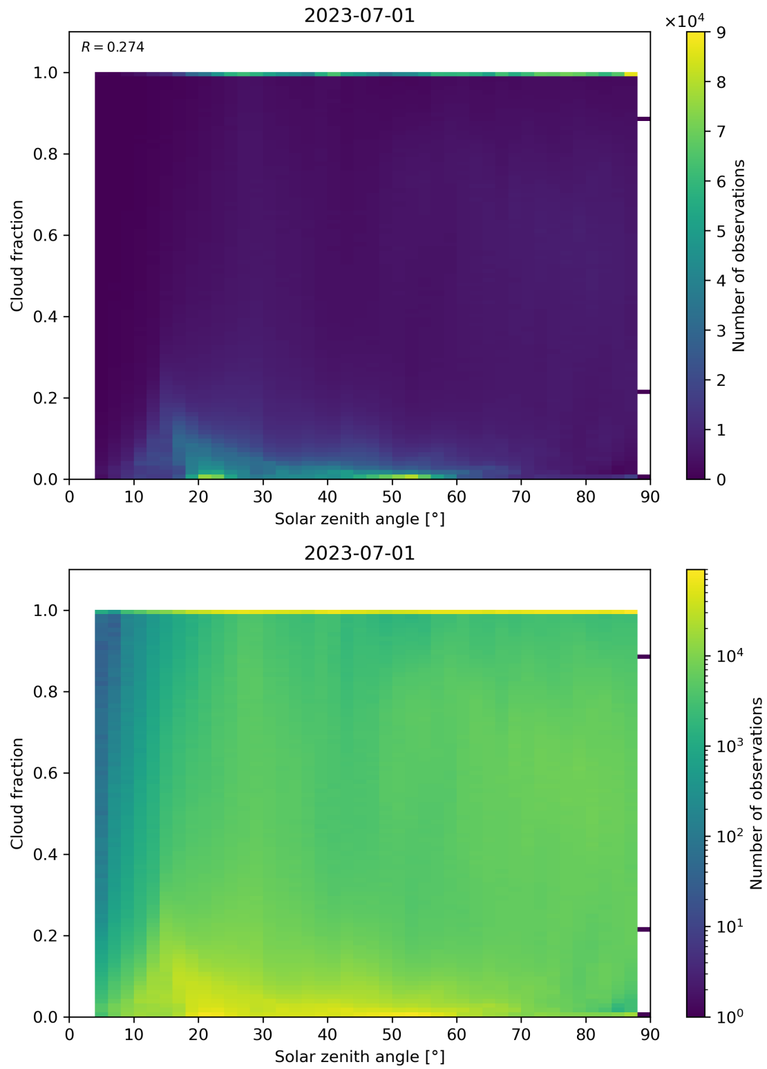
Figure 121: Scatter density plot of “Solar zenith angle” against “Cloud fraction” for 2023-06-30 to 2023-07-02.
