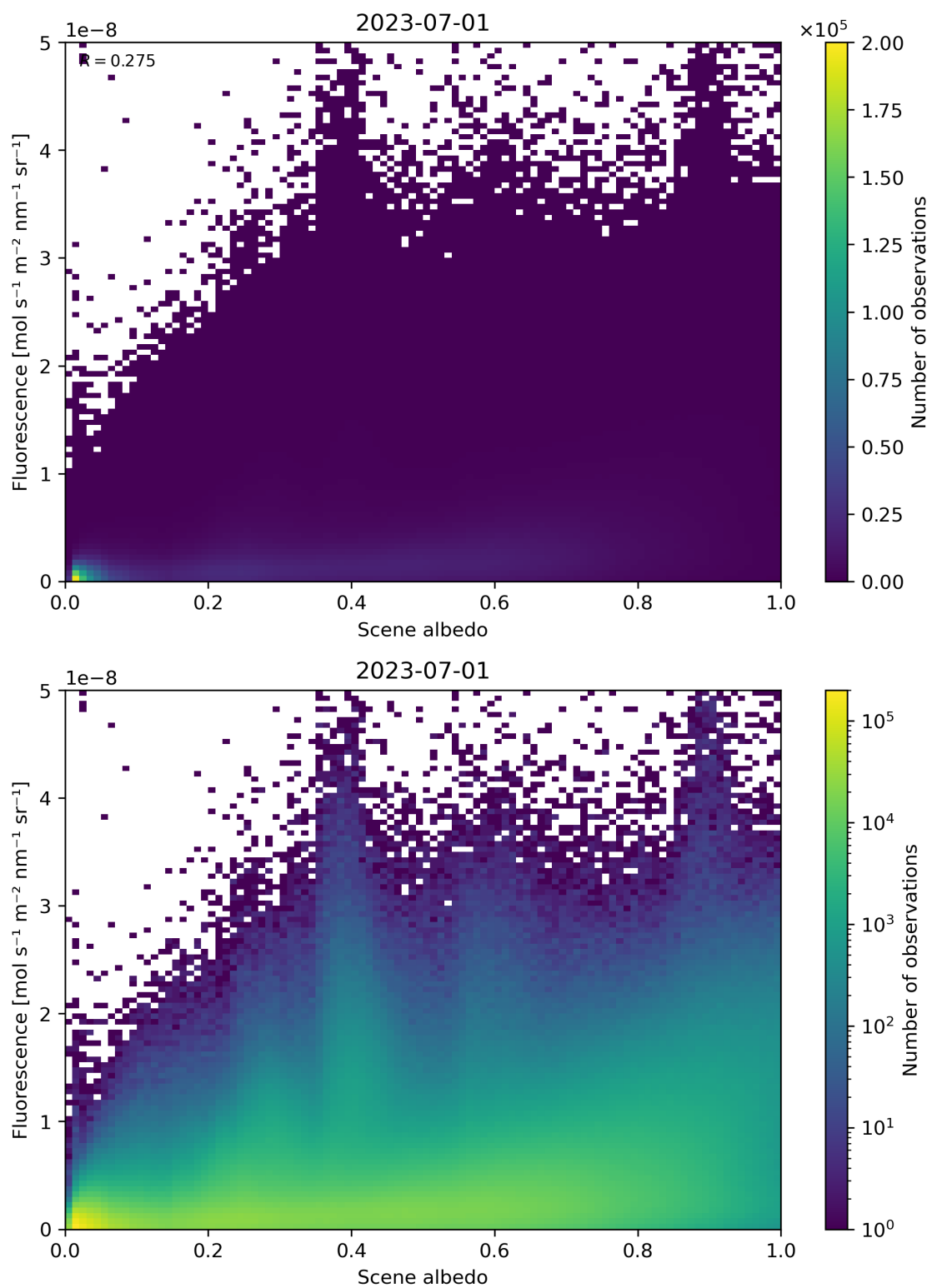
Figure 114: Scatter density plot of “Scene albedo” against “Fluorescence” for 2023-06-30 to 2023-07-02.
