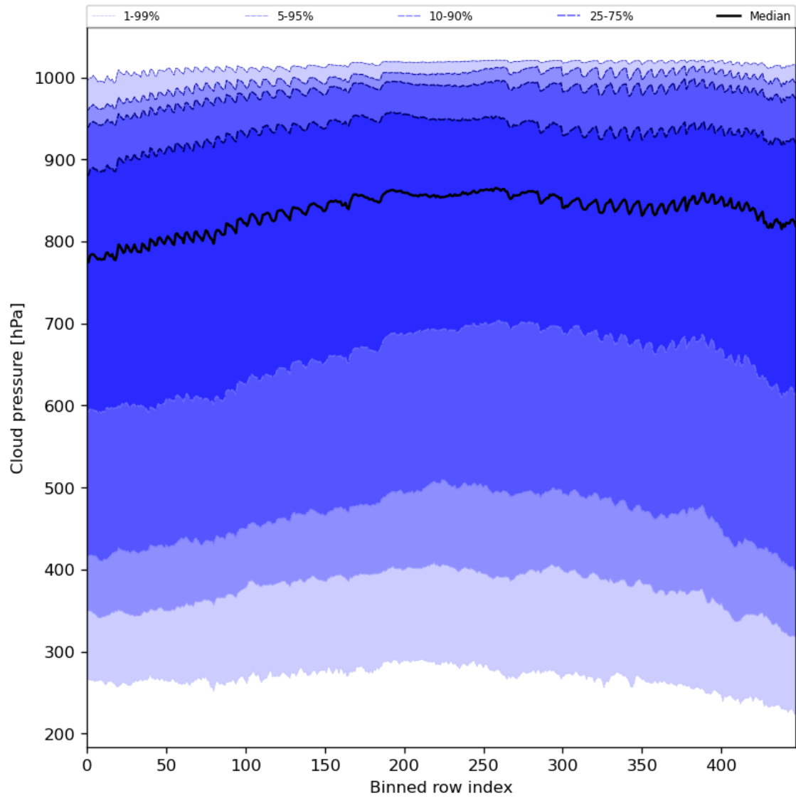
Figure 47: Along track statistics of “Cloud pressure” for 2023-06-30 to 2023-07-02
