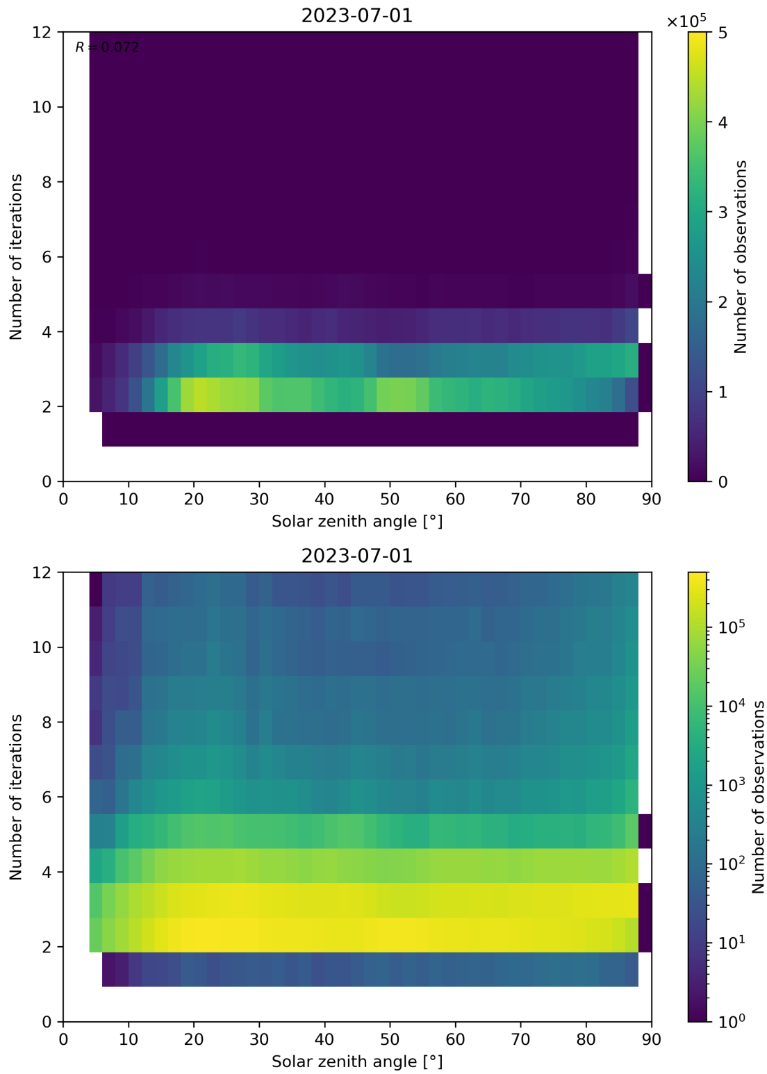
Figure 125: Scatter density plot of “Solar zenith angle” against “Number of iterations” for 2023-06-30 to 2023-07-02.
