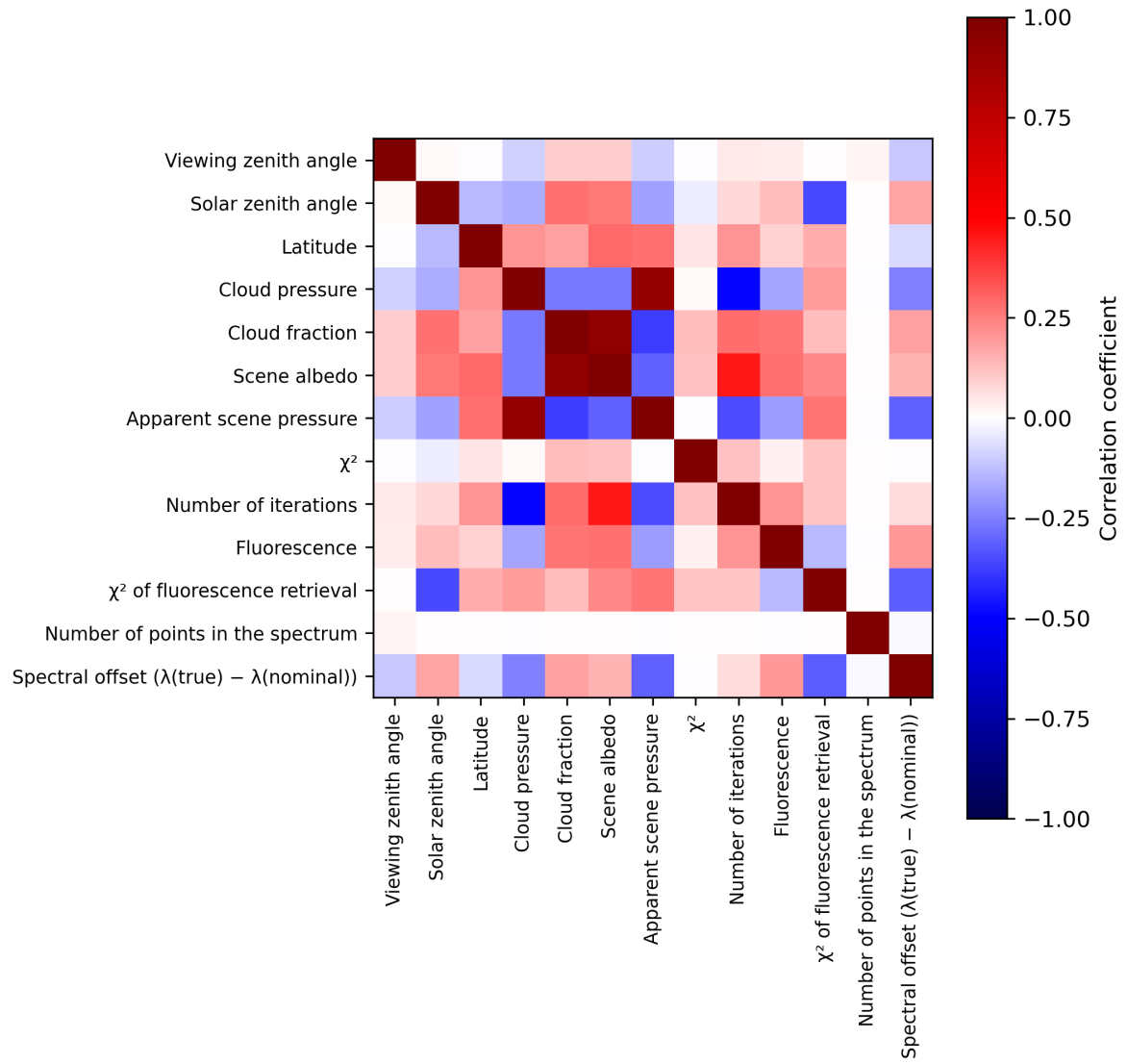
Figure 2: Map of correlation matrix for 2023-06-30 to 2023-07-02.
