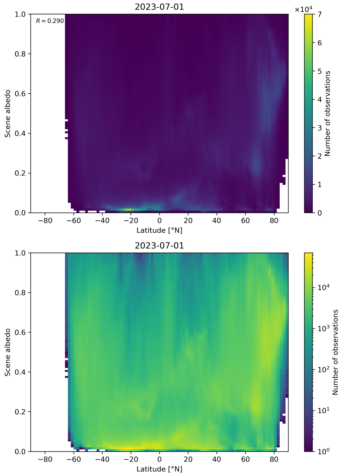
Figure 104: Scatter density plot of “Latitude” against “Scene albedo” for 2023-06-30 to 2023-07-02.
