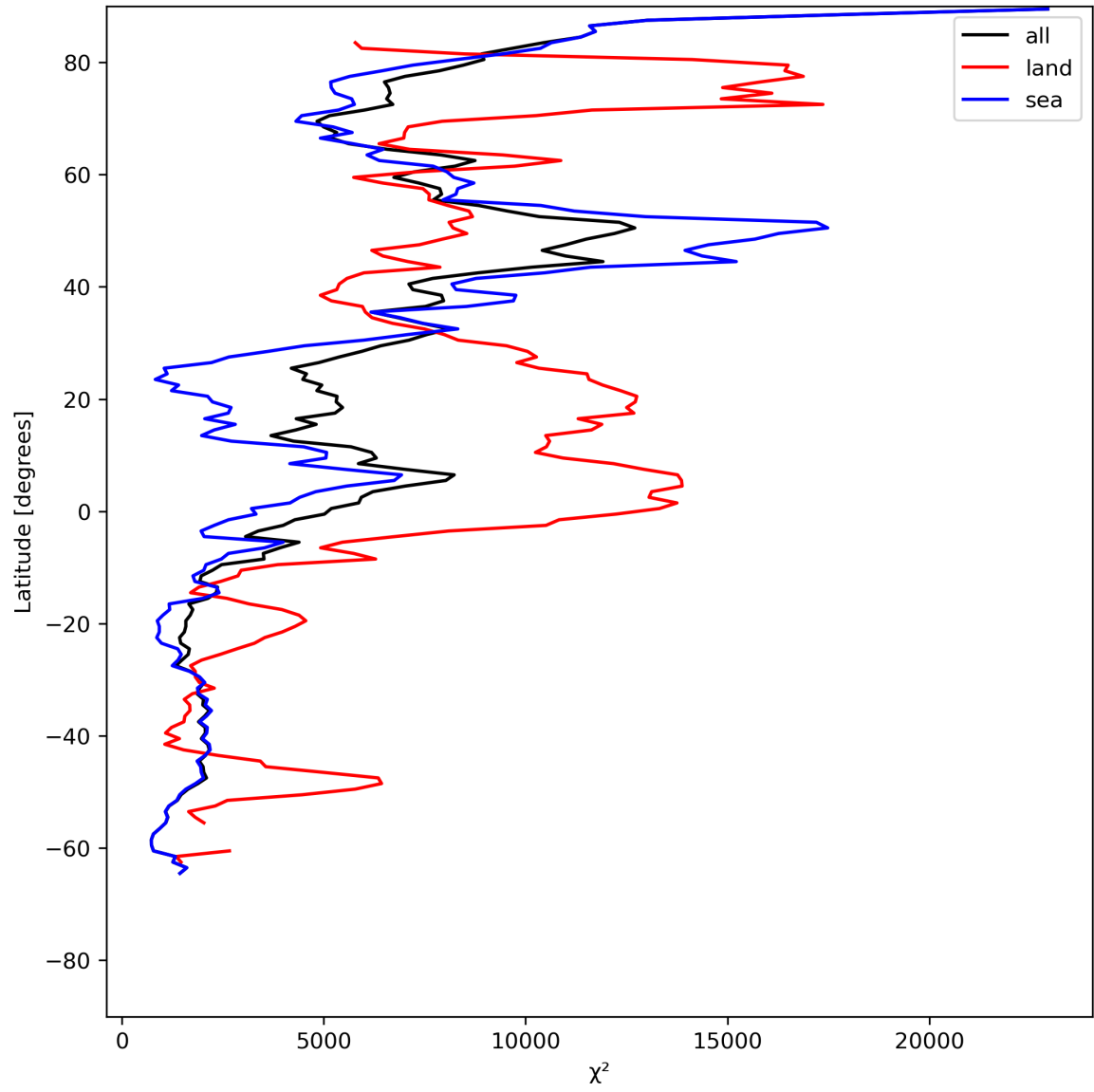
Figure 21: Zonal average of “ \chi^2 ” for 2023-06-30 to 2023-07-02.
