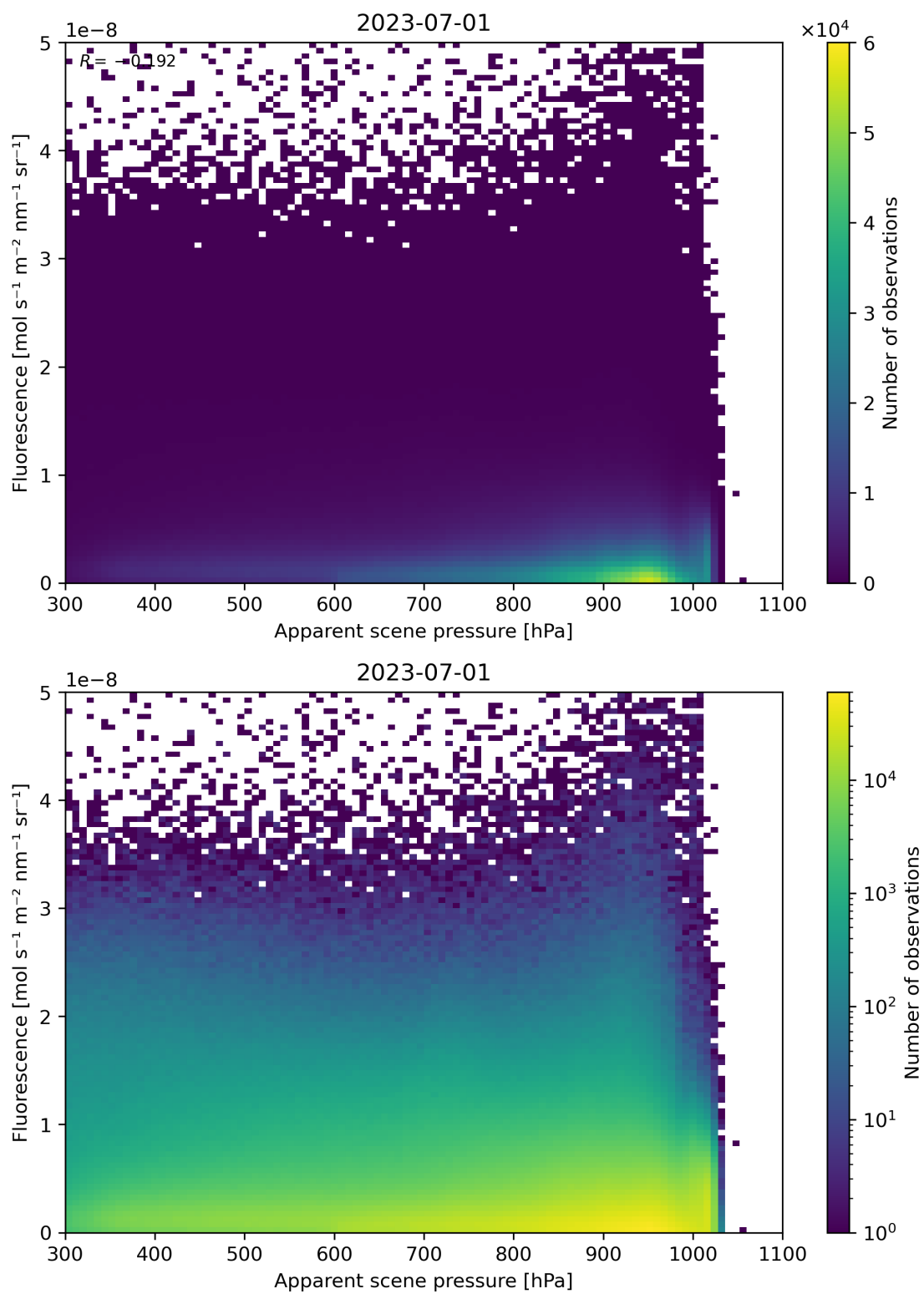
Figure 65: Scatter density plot of “Apparent scene pressure” against “Fluorescence” for 2023-06-30 to 2023-07-02.
