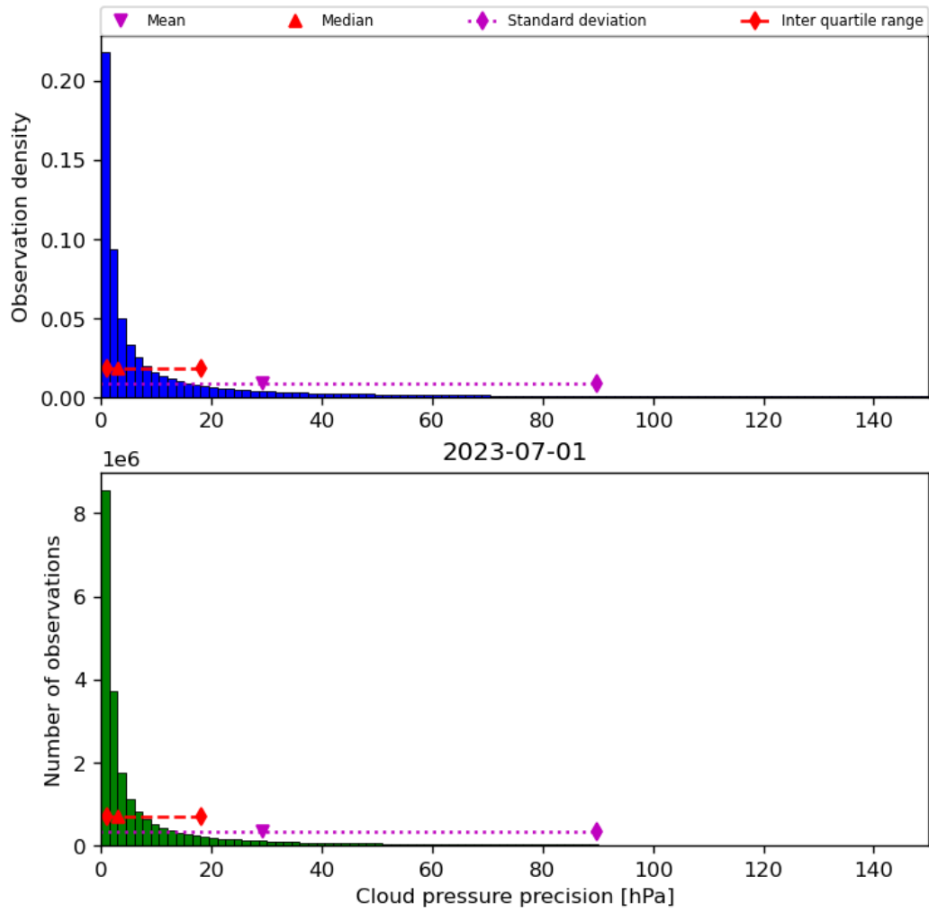
Figure 31: Histogram of “Cloud pressure precision” for 2023-06-30 to 2023-07-02
