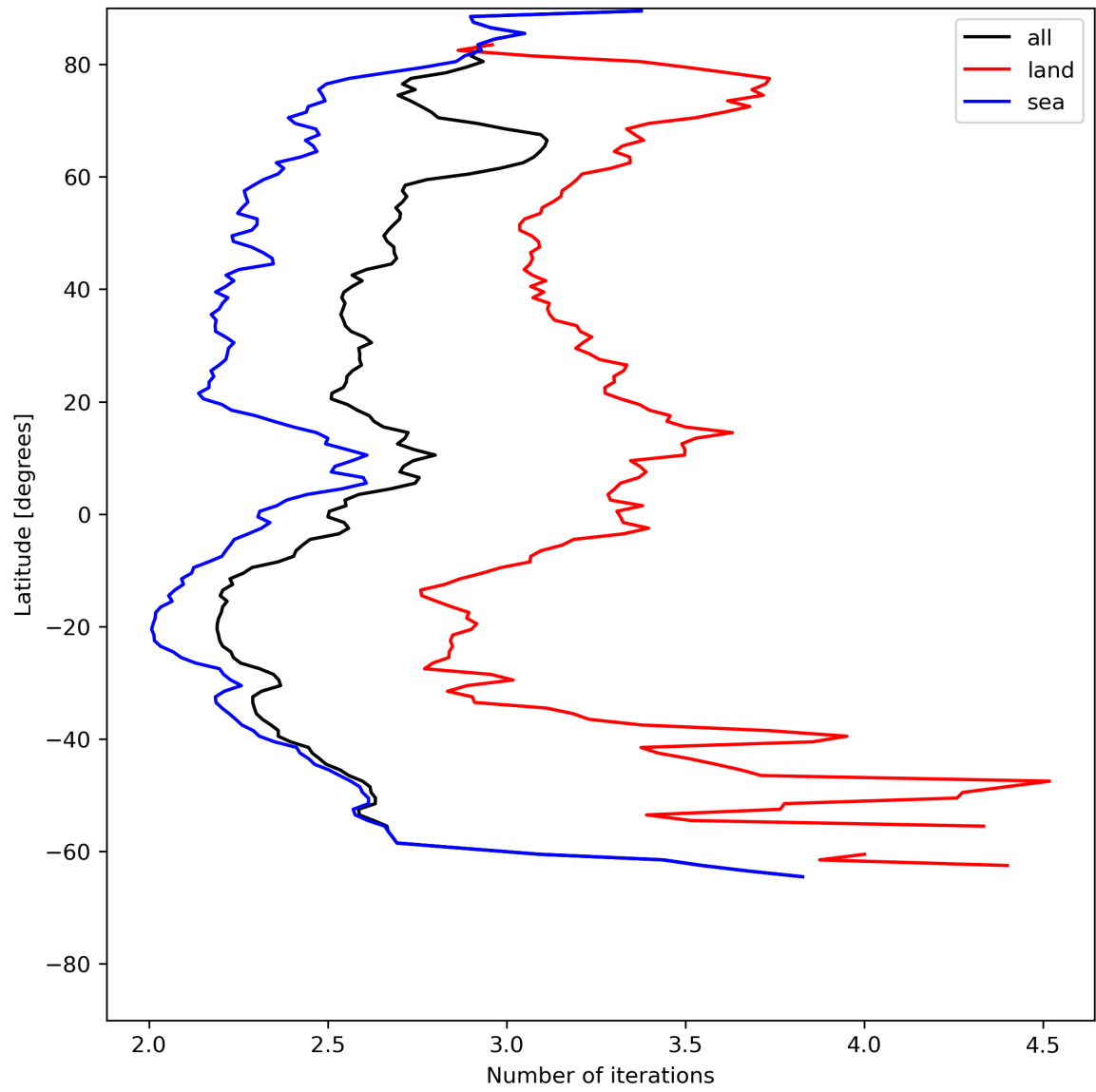
Figure 22: Zonal average of “Number of iterations” for 2023-06-30 to 2023-07-02.
