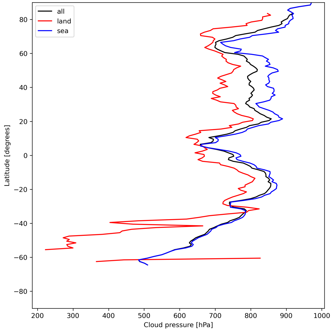
Figure 13: Zonal average of “Cloud pressure” for 2023-06-30 to 2023-07-02.
