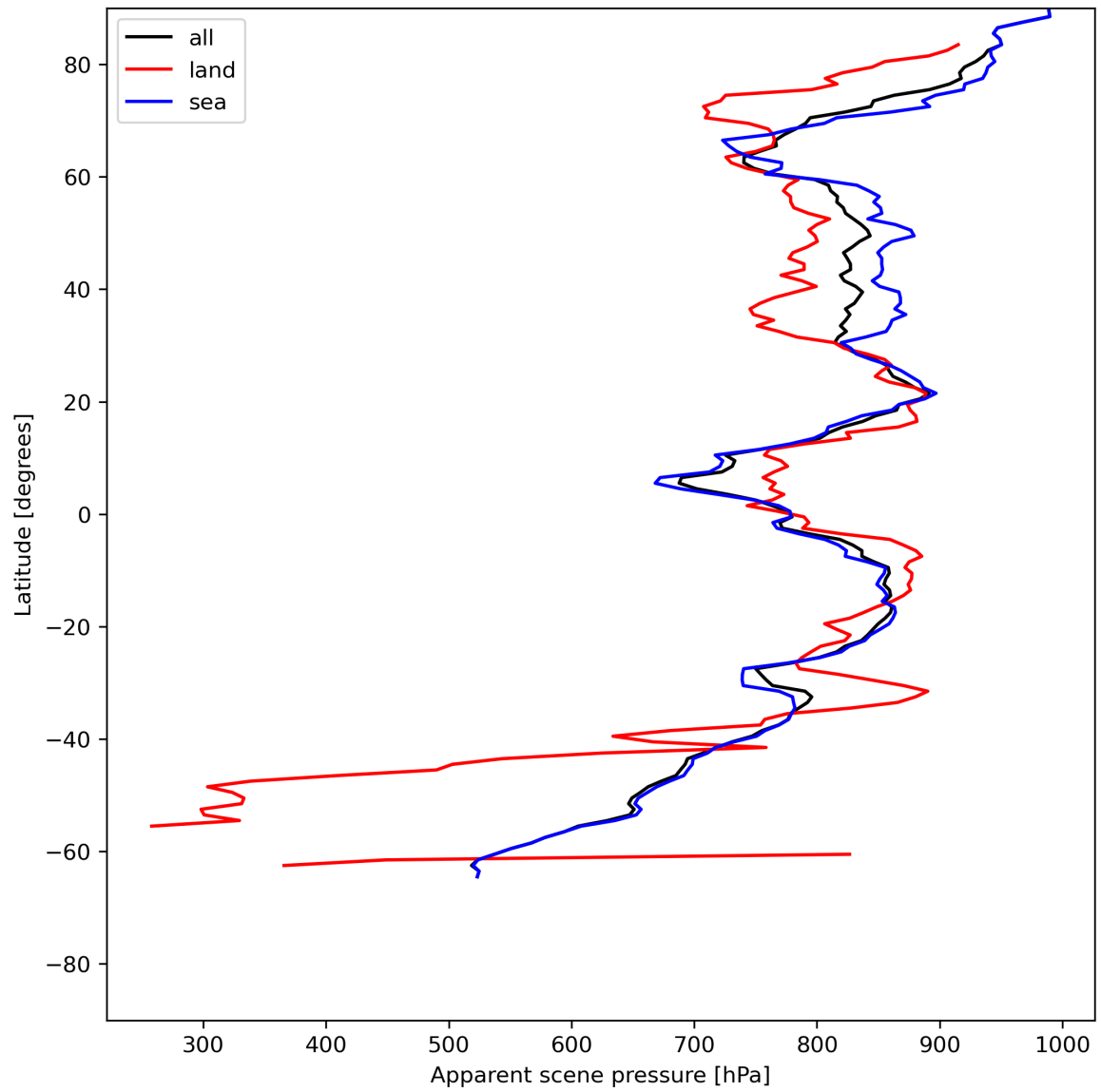
Figure 19: Zonal average of “Apparent scene pressure” for 2023-06-30 to 2023-07-02.
