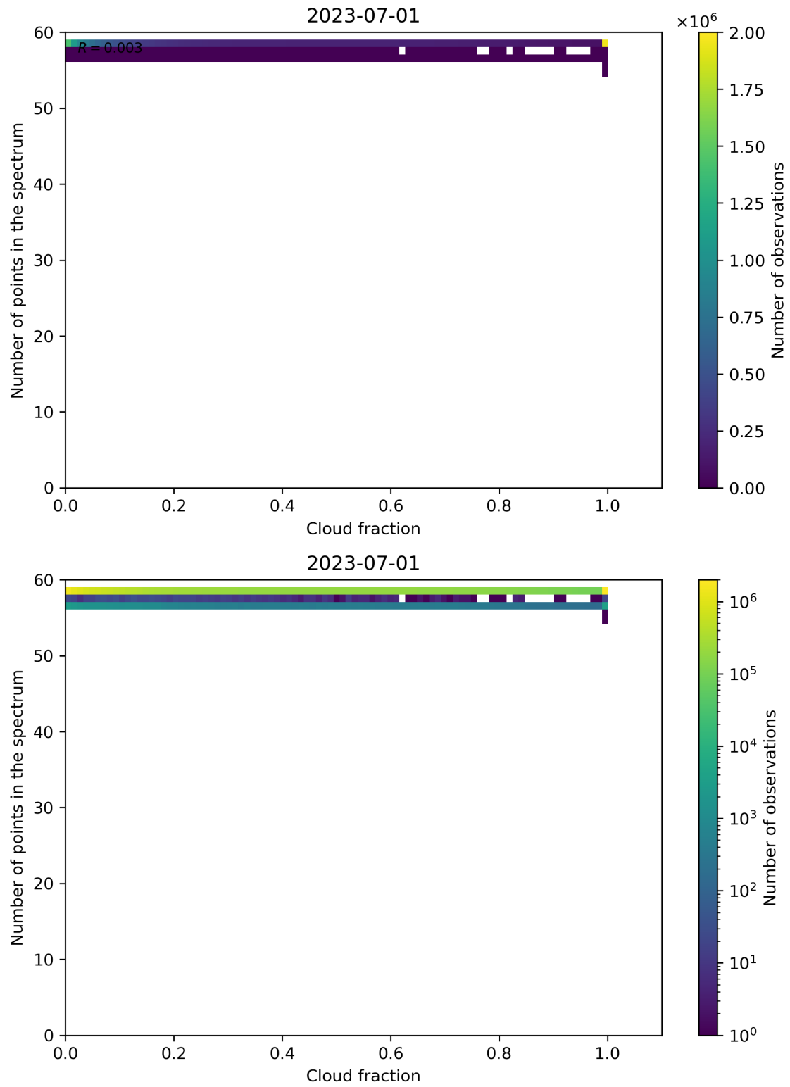
Figure 81: Scatter density plot of “Cloud fraction” against “Number of points in the spectrum” for 2023-06-30 to 2023-07-02.
