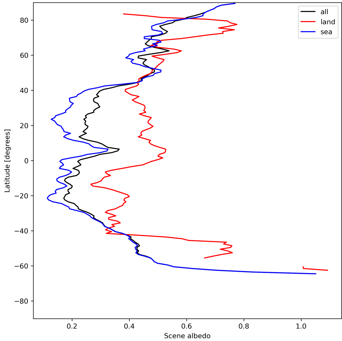
Figure 17: Zonal average of “Scene albedo” for 2023-06-30 to 2023-07-02.
