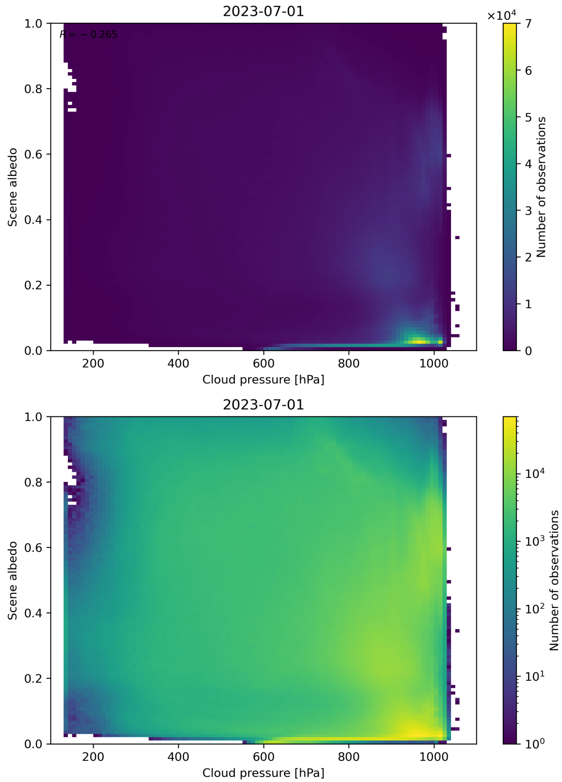
Figure 91: Scatter density plot of “Cloud pressure” against “Scene albedo” for 2023-06-30 to 2023-07-02.
