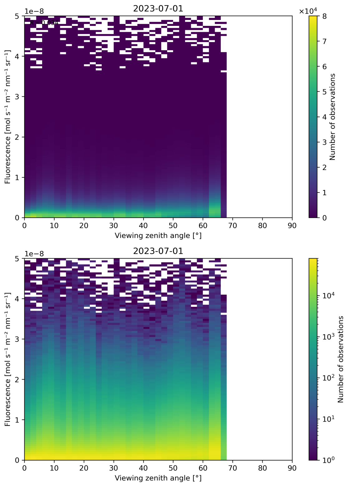
Figure 134: Scatter density plot of “Viewing zenith angle” against “Fluorescence” for 2023-06-30 to 2023-07-02.
