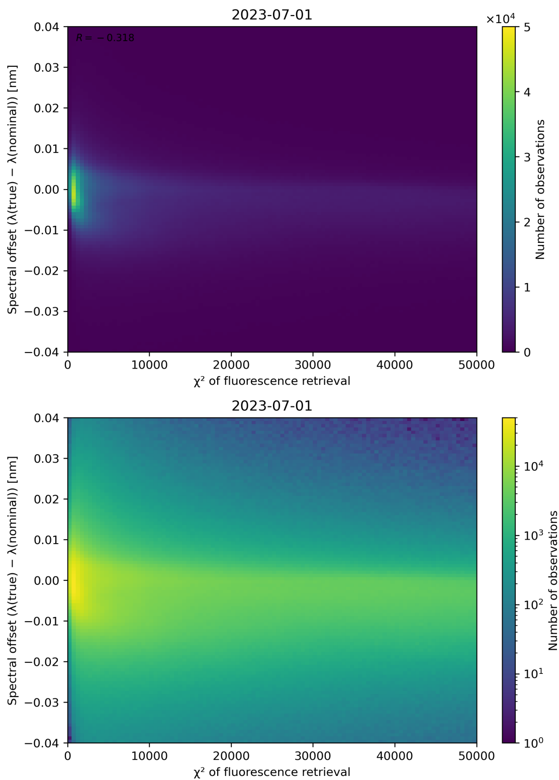
Figure 72: Scatter density plot of " \chi^2 of fluorescence retrieval" against "Spectral offset ( \lambda(\text{true}) - \lambda(\text{nominal})) " for 2023-06-30 to 2023-07-02.
