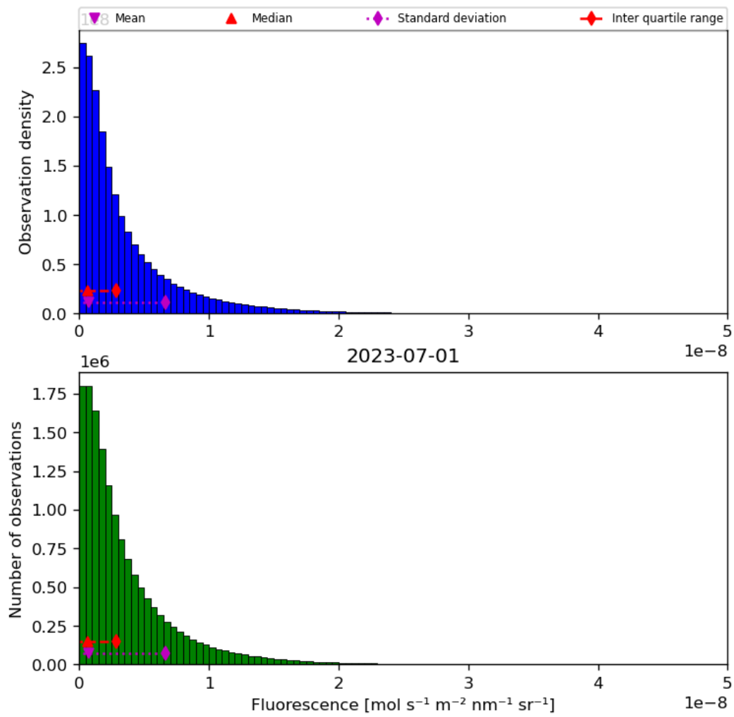
Figure 40: Histogram of “Fluorescence” for 2023-06-30 to 2023-07-02
