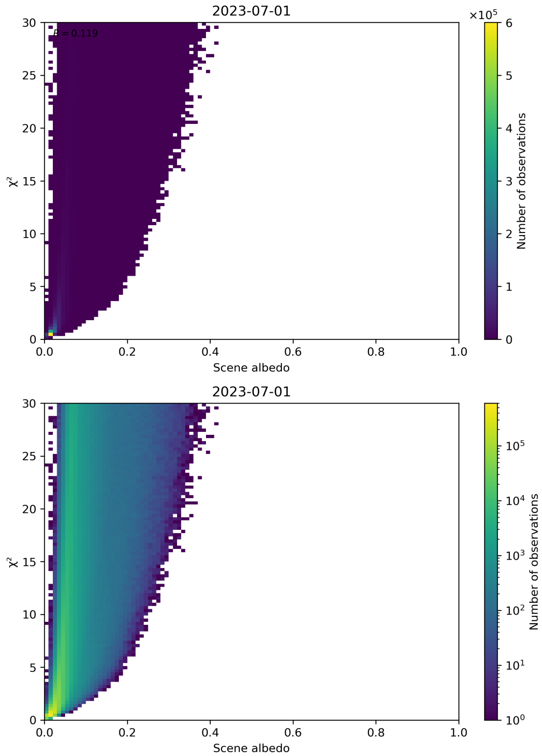
Figure 112: Scatter density plot of “Scene albedo” against “ \chi^2 ” for 2023-06-30 to 2023-07-02.
