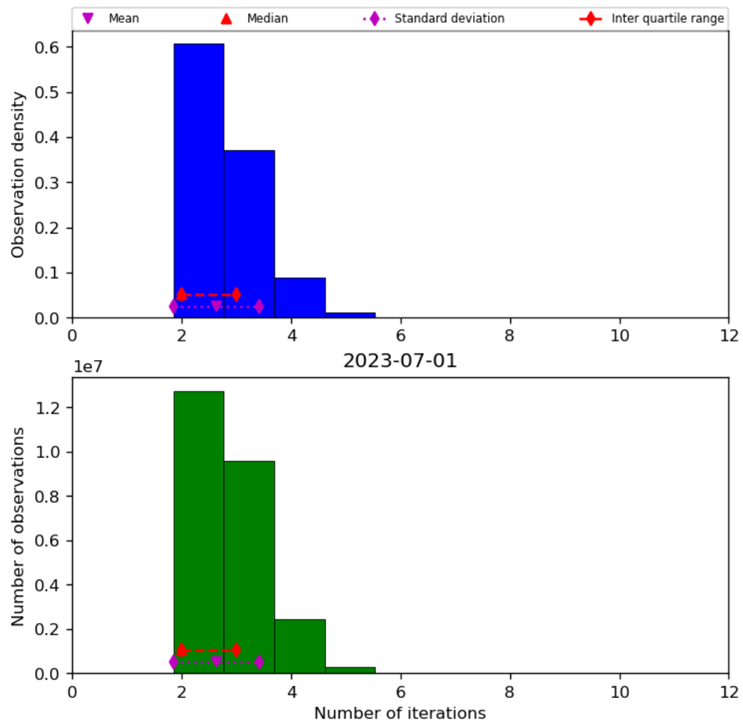
Figure 39: Histogram of “Number of iterations” for 2023-06-30 to 2023-07-02
