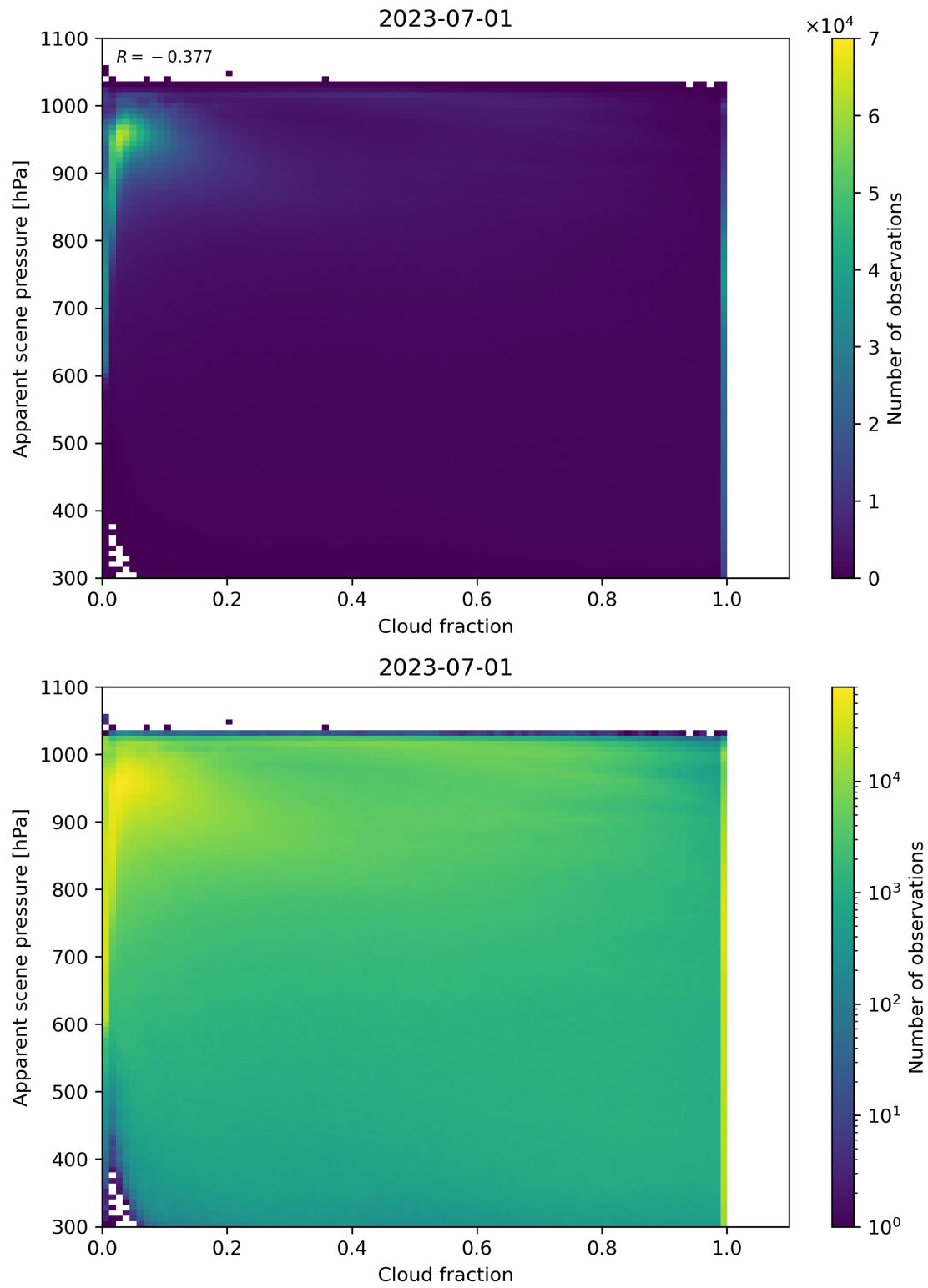
Figure 76: Scatter density plot of “Cloud fraction” against “Apparent scene pressure” for 2023-06-30 to 2023-07-02.
