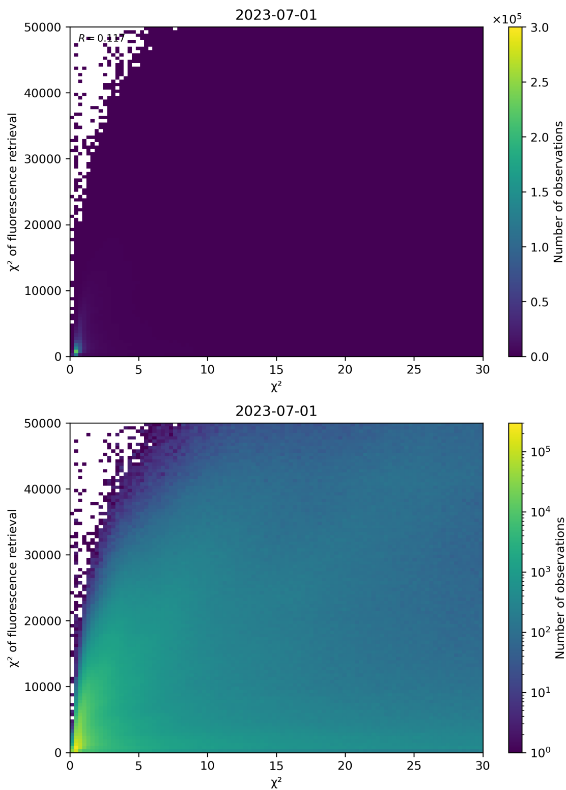
Figure 69: Scatter density plot of “ \chi^2 ” against “ \chi^2 of fluorescence retrieval” for 2023-06-30 to 2023-07-02.
