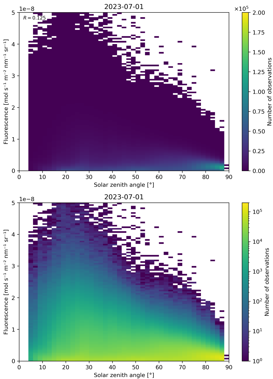
Figure 123: Scatter density plot of “Solar zenith angle” against “Fluorescence” for 2023-06-30 to 2023-07-02.
