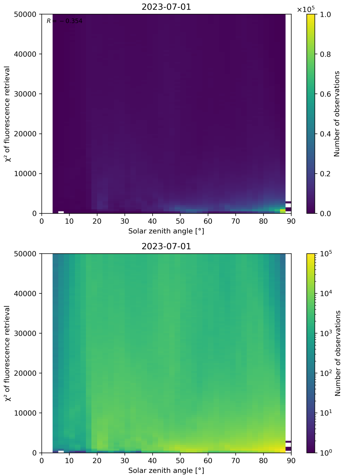
Figure 120: Scatter density plot of “Solar zenith angle” against “ \chi^2 of fluorescence retrieval” for 2023-06-30 to 2023-07-02.
