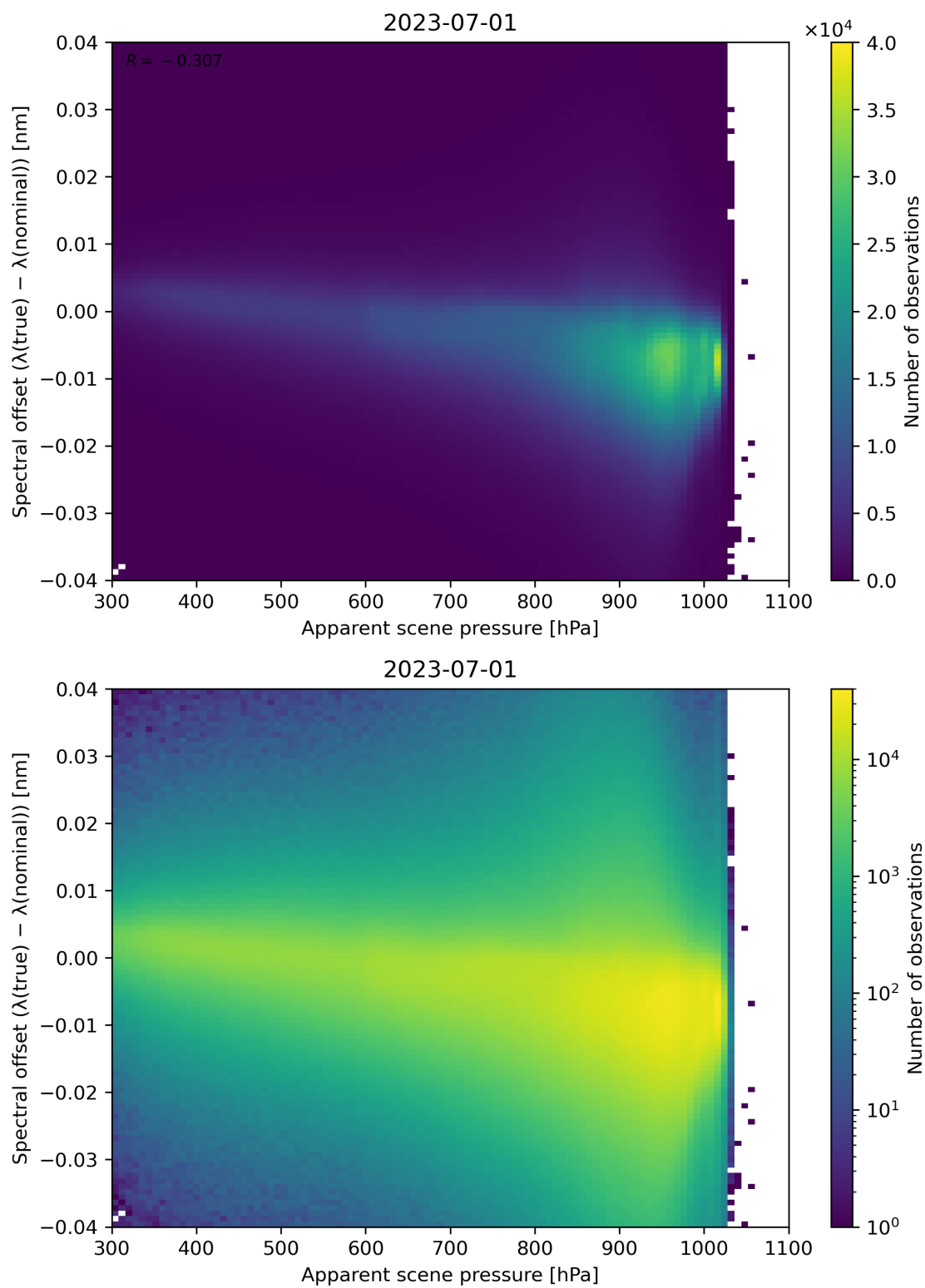
Figure 68: Scatter density plot of “Apparent scene pressure” against “Spectral offset ( \lambda(\text{true}) - \lambda(\text{nominal}) )” for 2023-06-30 to 2023-07-02.
