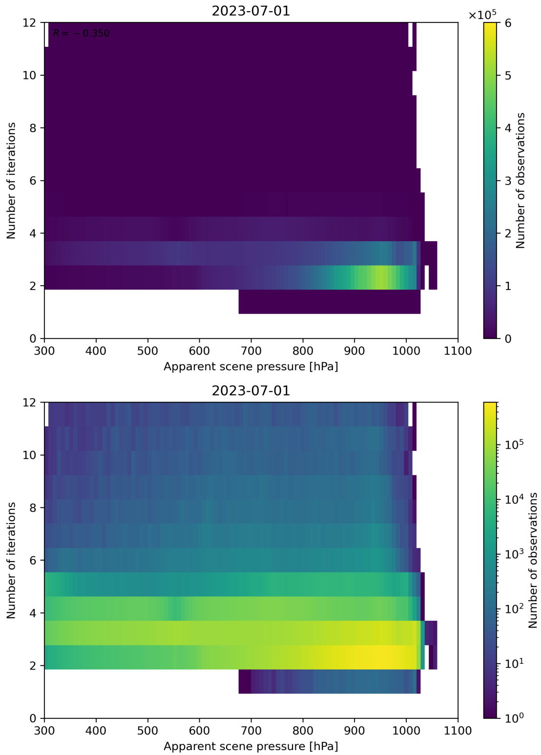
Figure 66: Scatter density plot of “Apparent scene pressure” against “Number of iterations” for 2023-06-30 to 2023-07-02.
