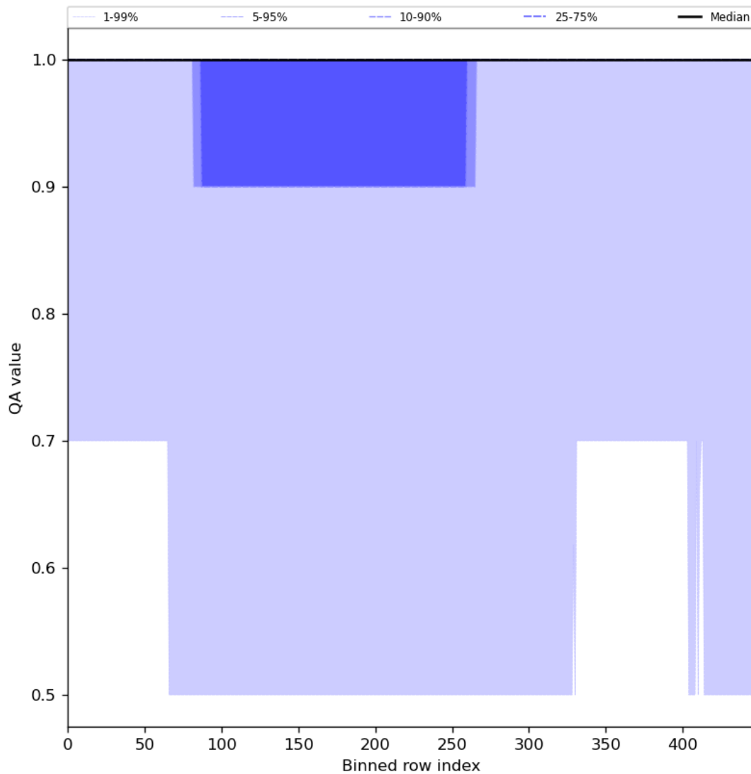
Figure 46: Along track statistics of “QA value” for 2023-06-30 to 2023-07-02
