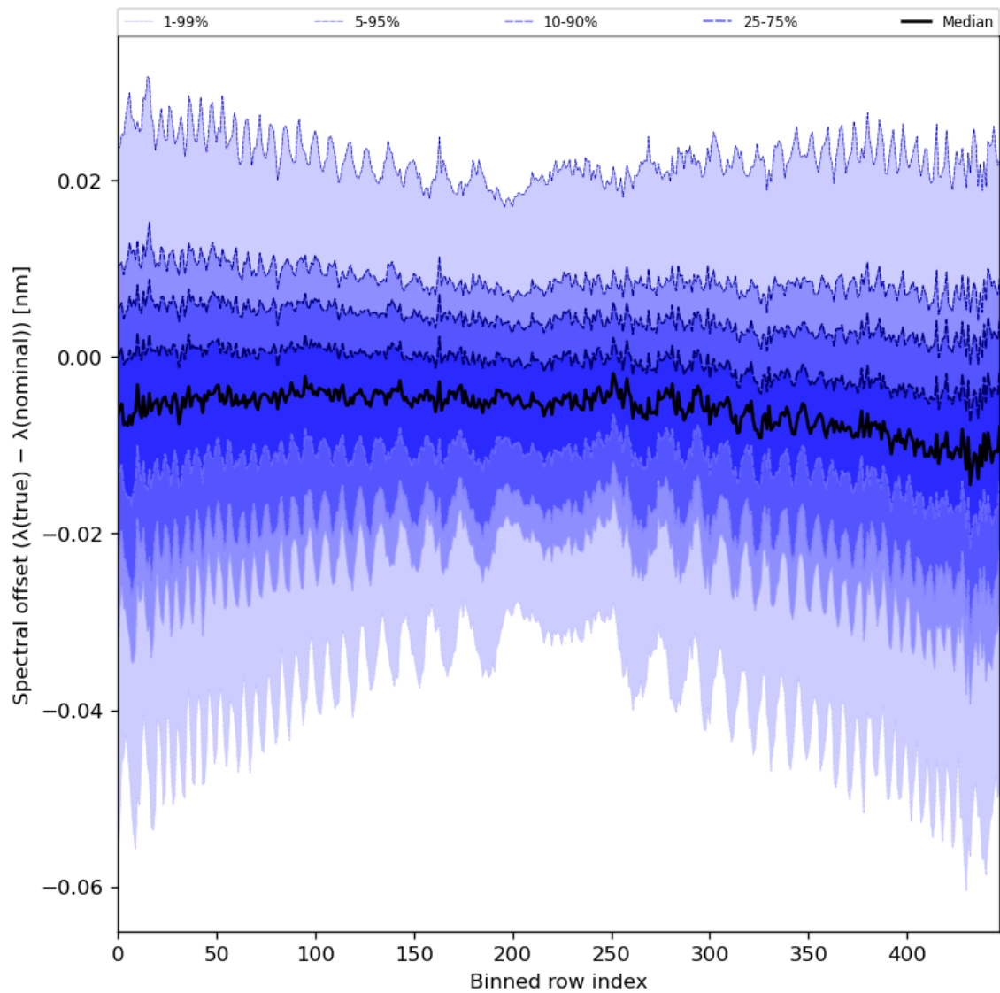
Figure 62: Along track statistics of “Spectral offset ( \lambda(\text{true}) - \lambda(\text{nominal}) )” for 2023-06-30 to 2023-07-02
