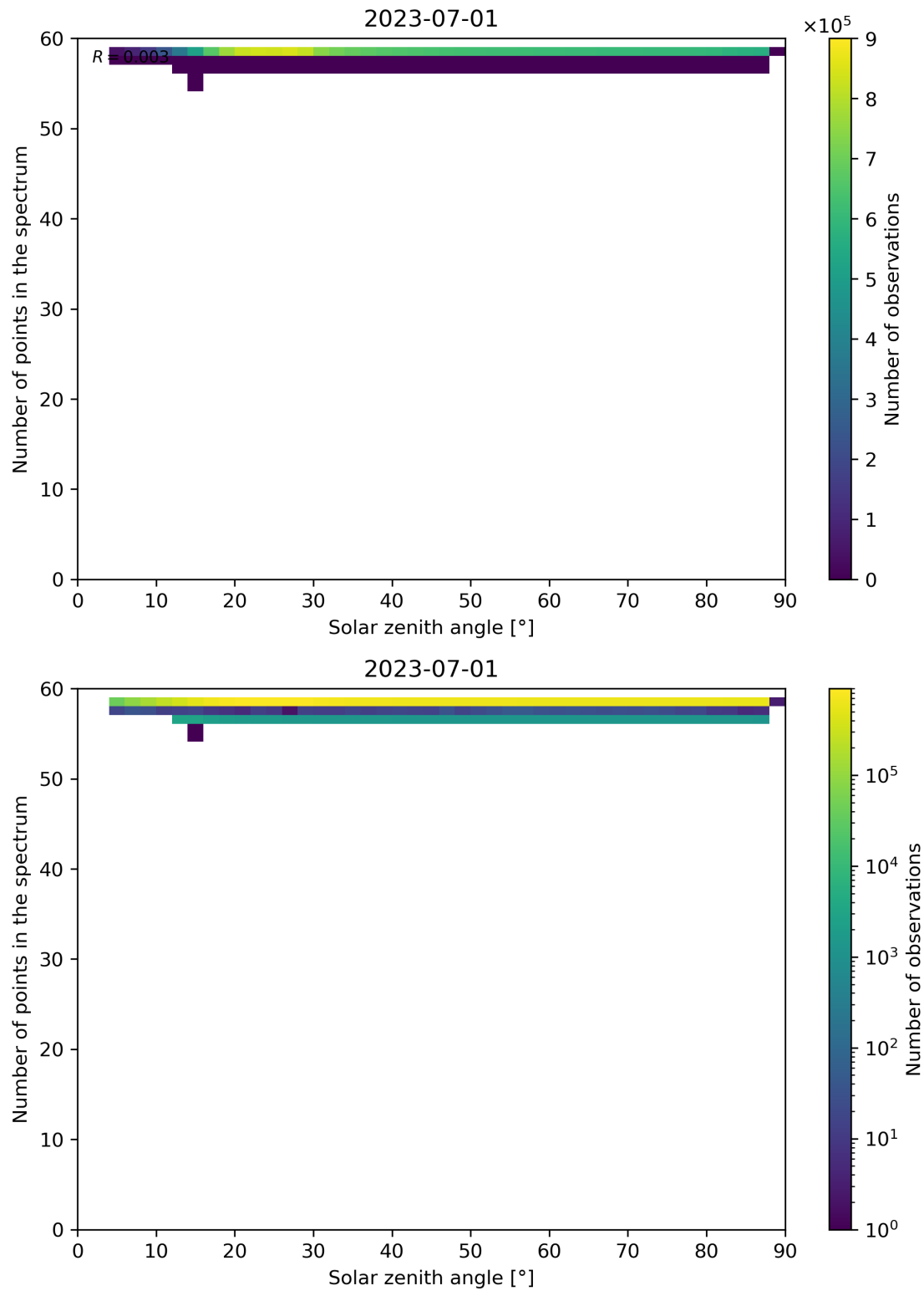
Figure 126: Scatter density plot of “Solar zenith angle” against “Number of points in the spectrum” for 2023-06-30 to 2023-07-02.
