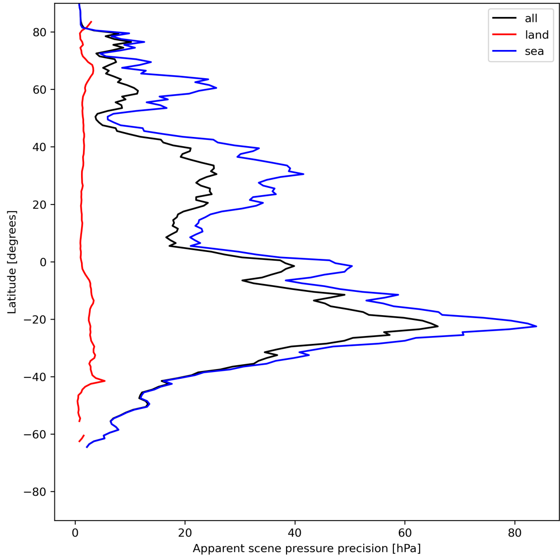
Figure 20: Zonal average of “Apparent scene pressure precision” for 2023-06-30 to 2023-07-02.
