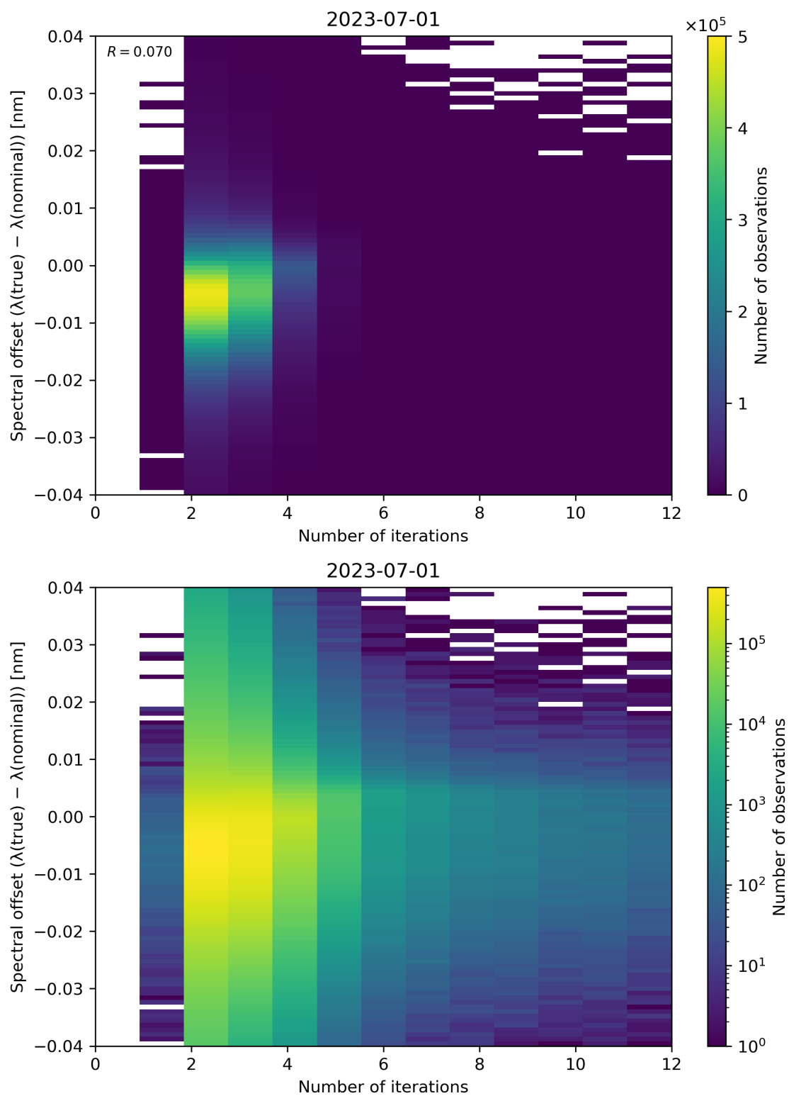
Figure 109: Scatter density plot of “Number of iterations” against “Spectral offset ( \lambda(\text{true}) - \lambda(\text{nominal}) )” for 2023-06-30 to 2023-07-02.
