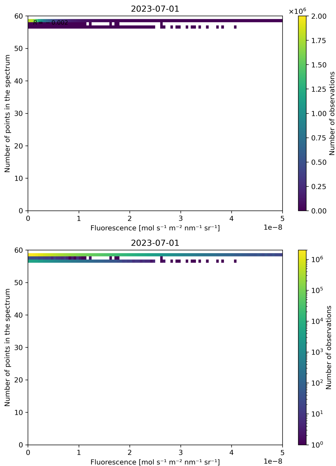
Figure 94: Scatter density plot of “Fluorescence” against “Number of points in the spectrum” for 2023-06-30 to 2023-07-02.
