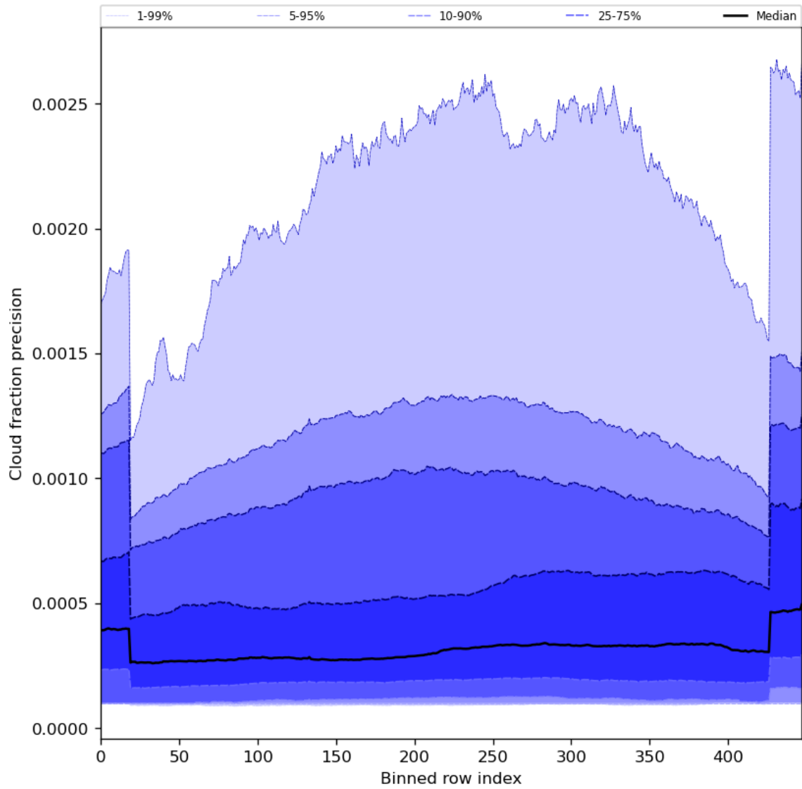
Figure 50: Along track statistics of “Cloud fraction precision” for 2023-06-30 to 2023-07-02
