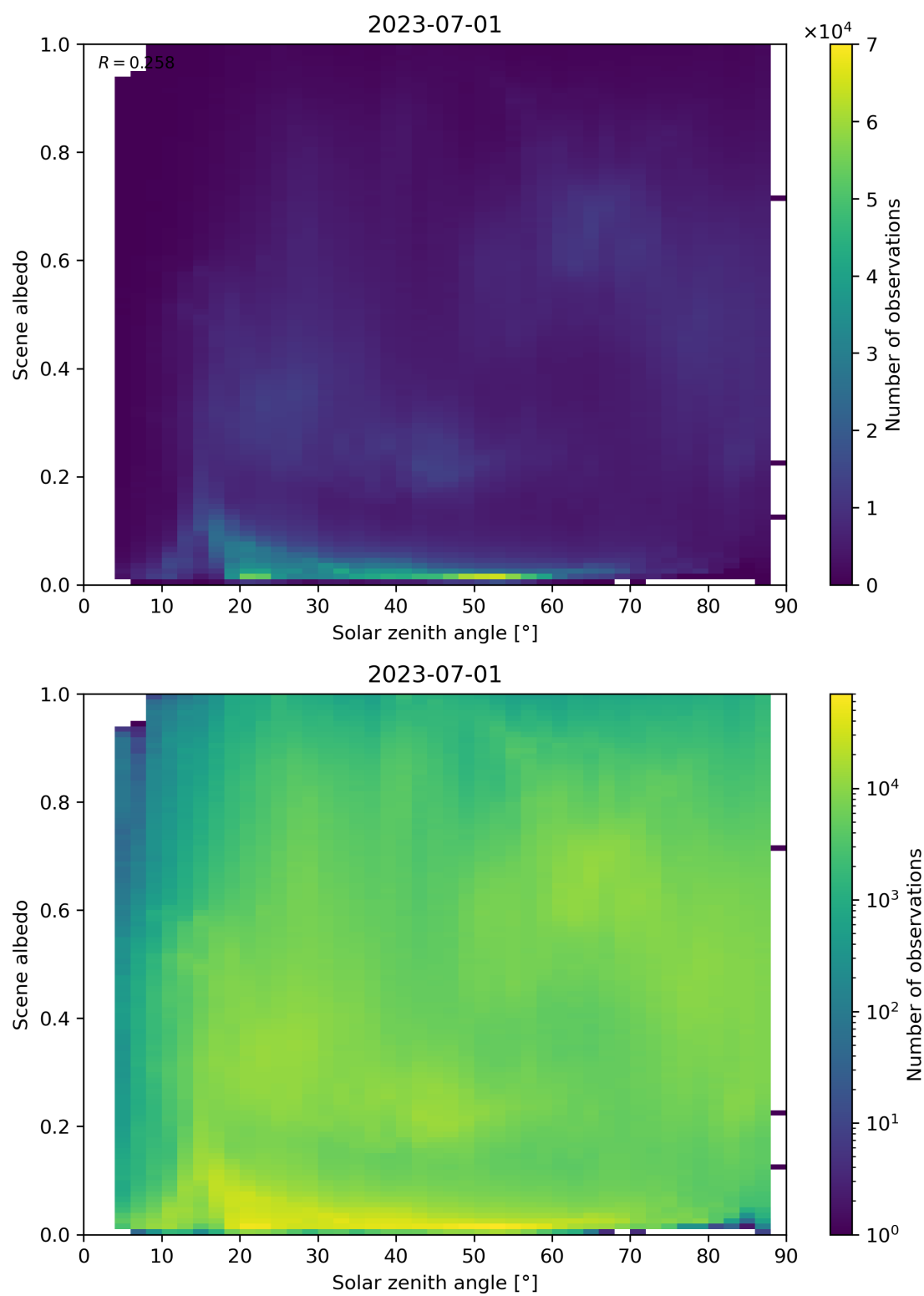
Figure 127: Scatter density plot of “Solar zenith angle” against “Scene albedo” for 2023-06-30 to 2023-07-02.
