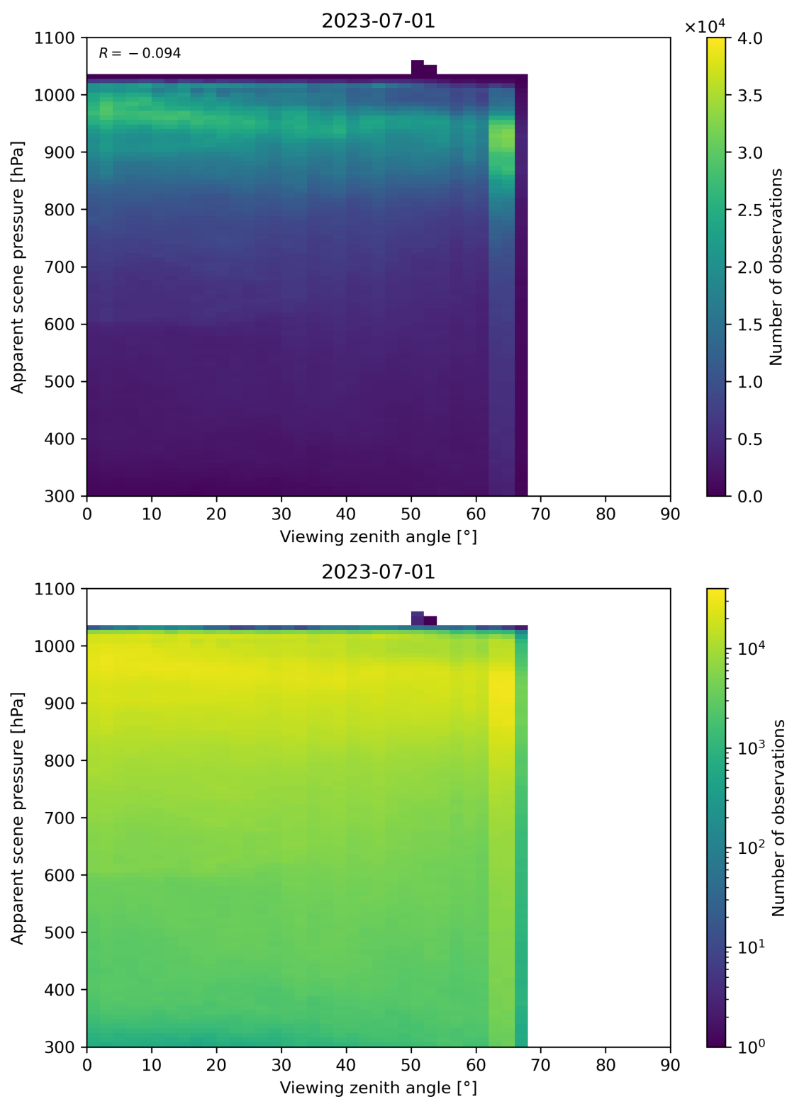
Figure 129: Scatter density plot of “Viewing zenith angle” against “Apparent scene pressure” for 2023-06-30 to 2023-07-02.
