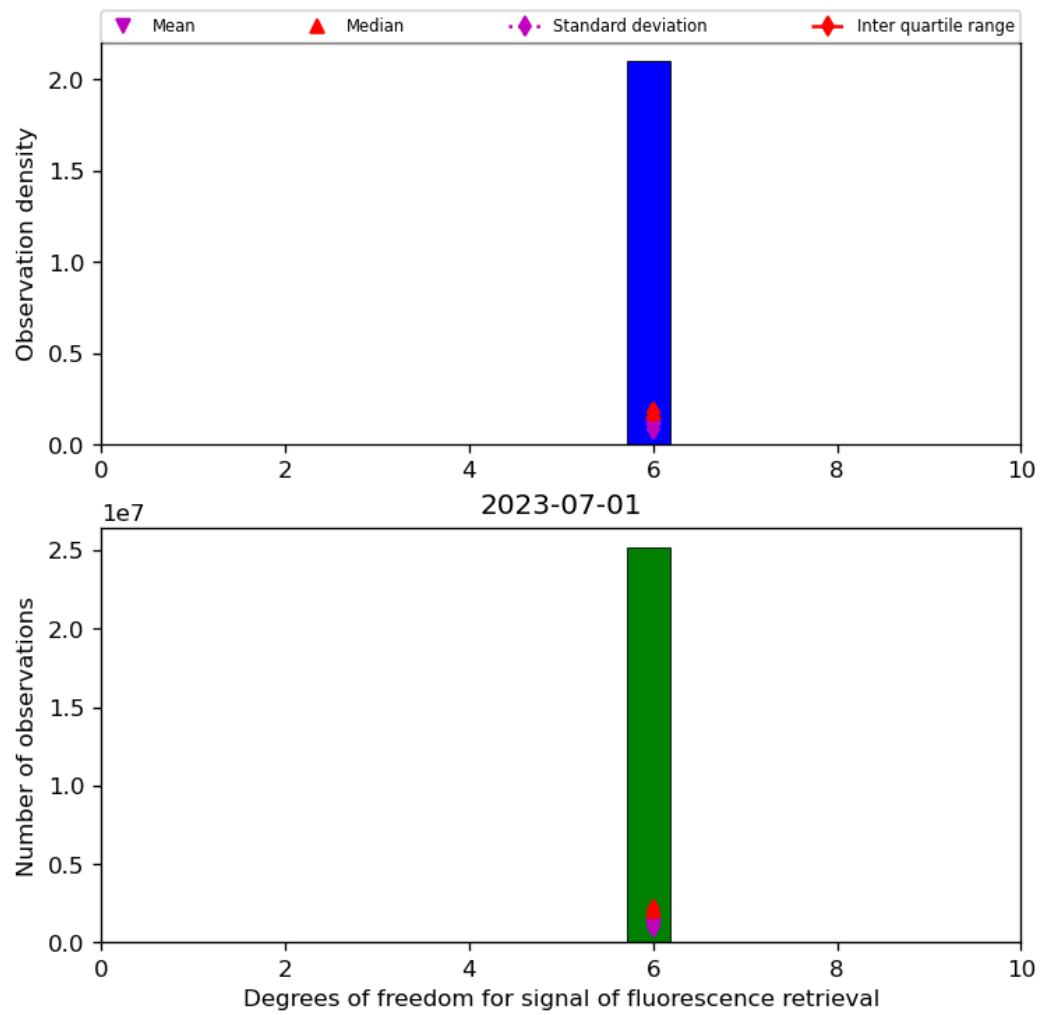
Figure 43: Histogram of “Degrees of freedom for signal of fluorescence retrieval” for 2023-06-30 to 2023-07-02
