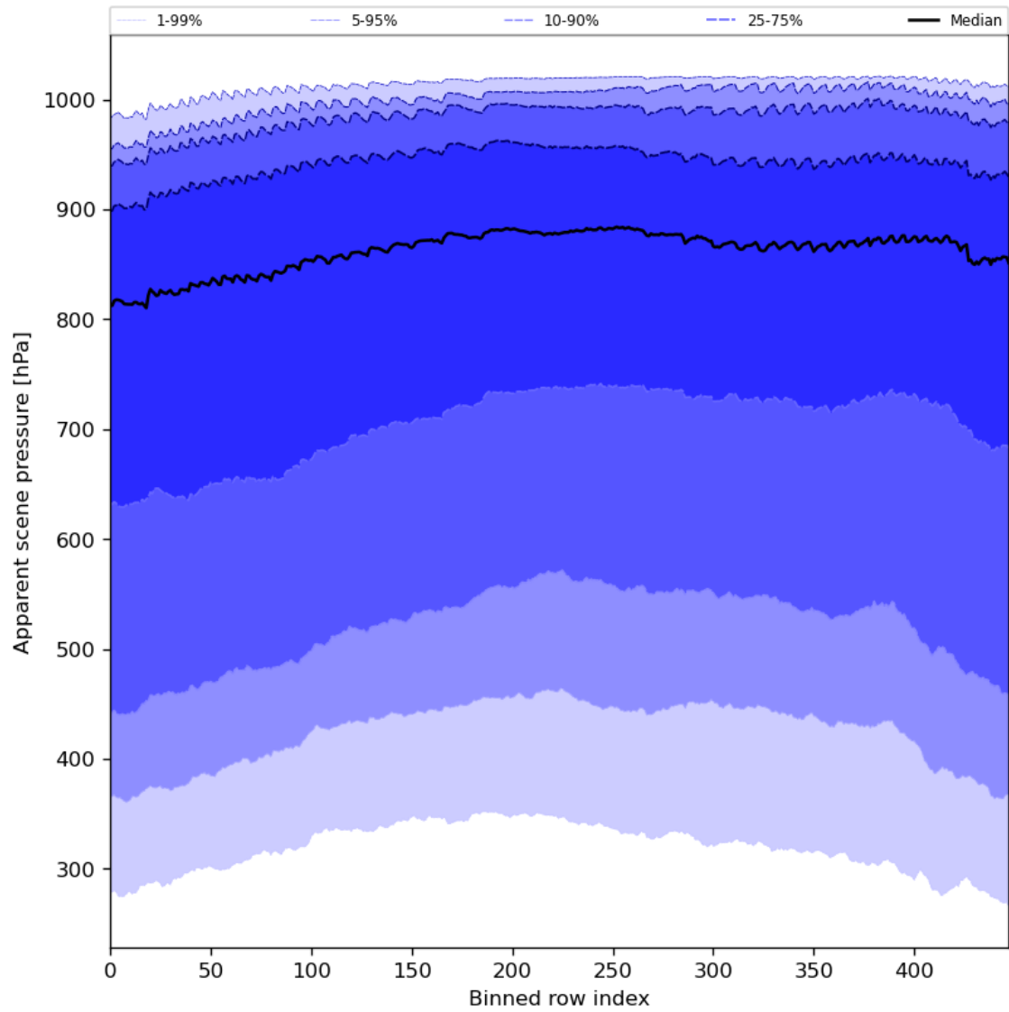
Figure 53: Along track statistics of “Apparent scene pressure” for 2023-06-30 to 2023-07-02
