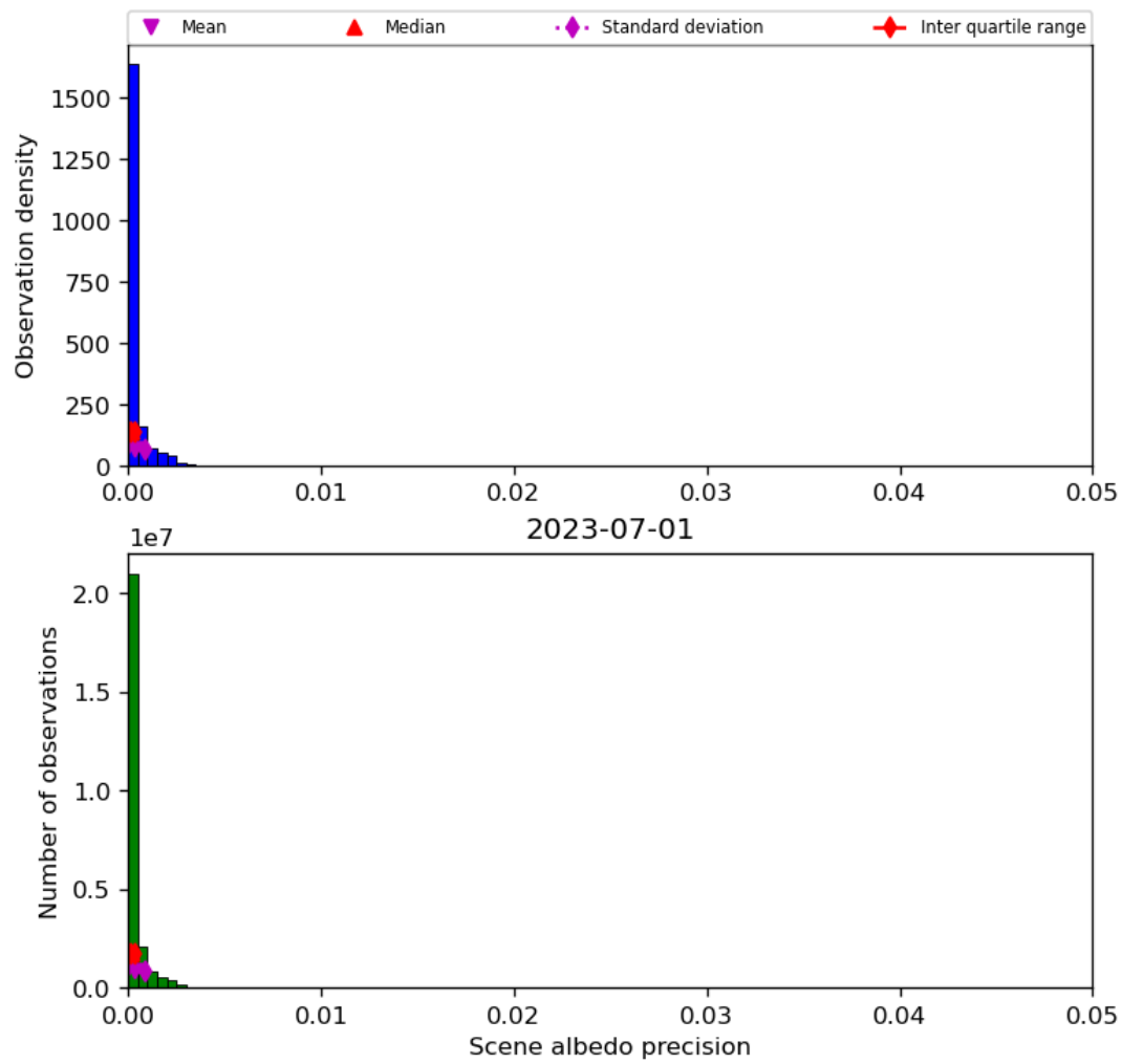
Figure 35: Histogram of “Scene albedo precision” for 2023-06-30 to 2023-07-02
