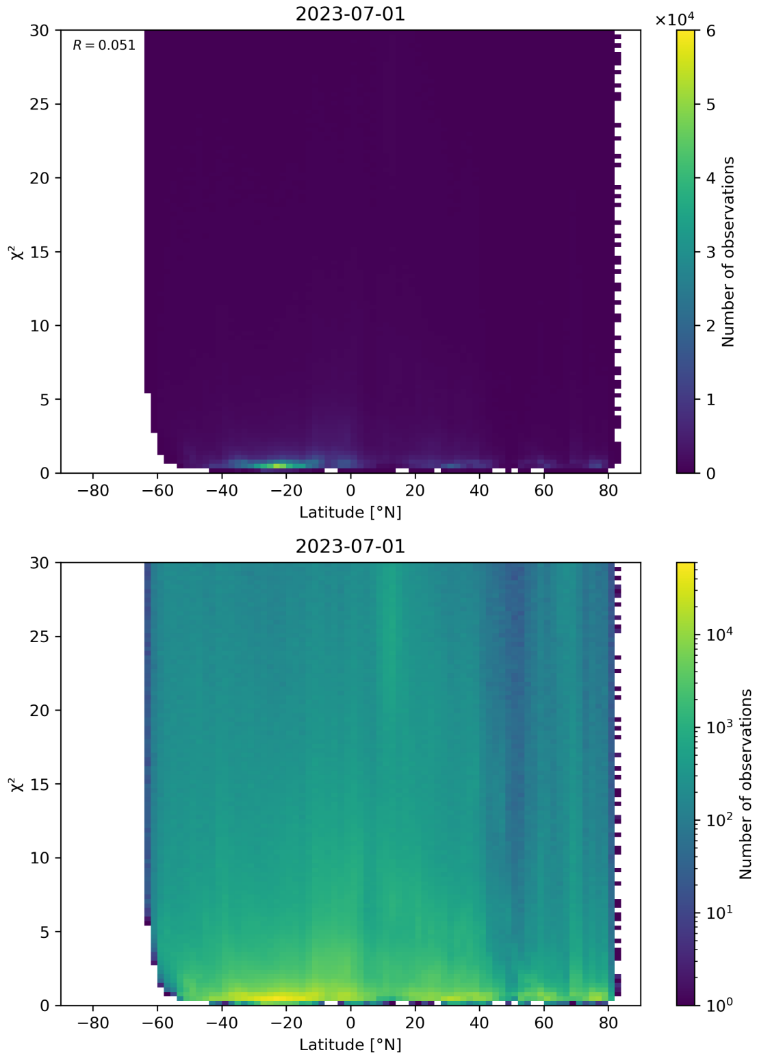
Figure 97: Scatter density plot of “Latitude” against “ \chi^2 ” for 2023-06-30 to 2023-07-02.
