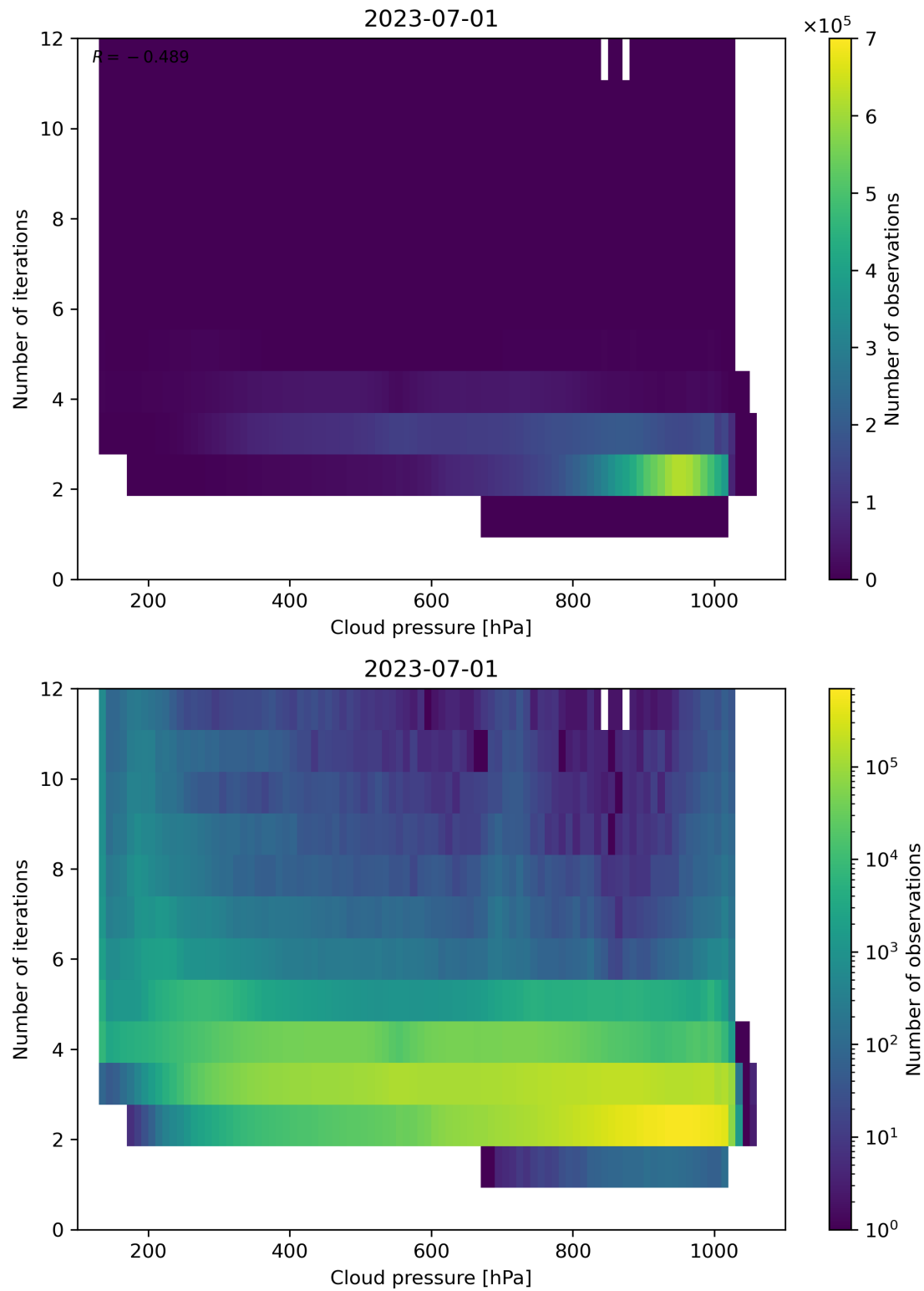
Figure 89: Scatter density plot of “Cloud pressure” against “Number of iterations” for 2023-06-30 to 2023-07-02.
