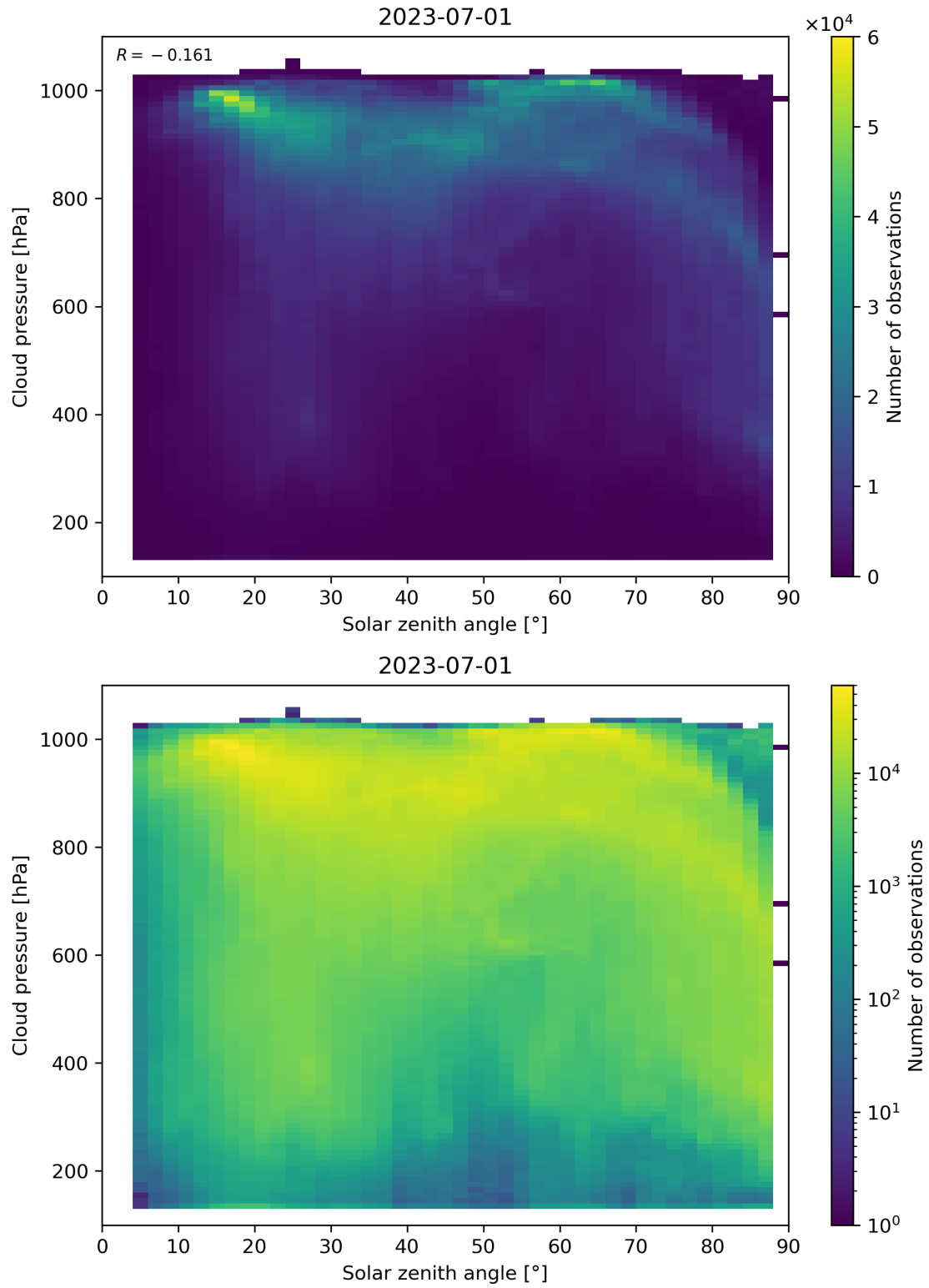
Figure 122: Scatter density plot of “Solar zenith angle” against “Cloud pressure” for 2023-06-30 to 2023-07-02.
