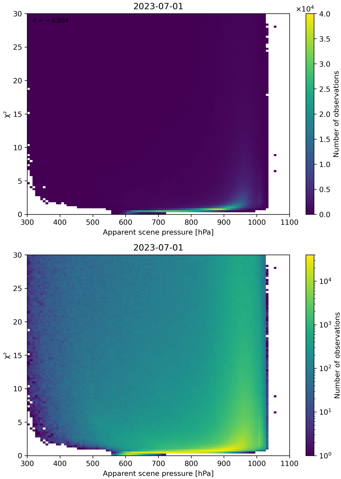
Figure 63: Scatter density plot of “Apparent scene pressure” against “ \chi^2 ” for 2023-06-30 to 2023-07-02.
