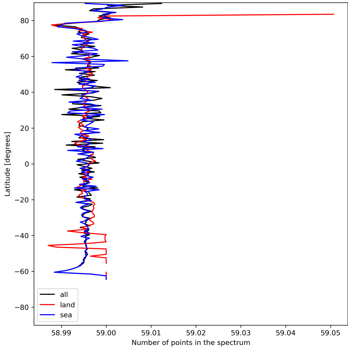
Figure 27: Zonal average of “Number of points in the spectrum” for 2023-06-30 to 2023-07-02.
