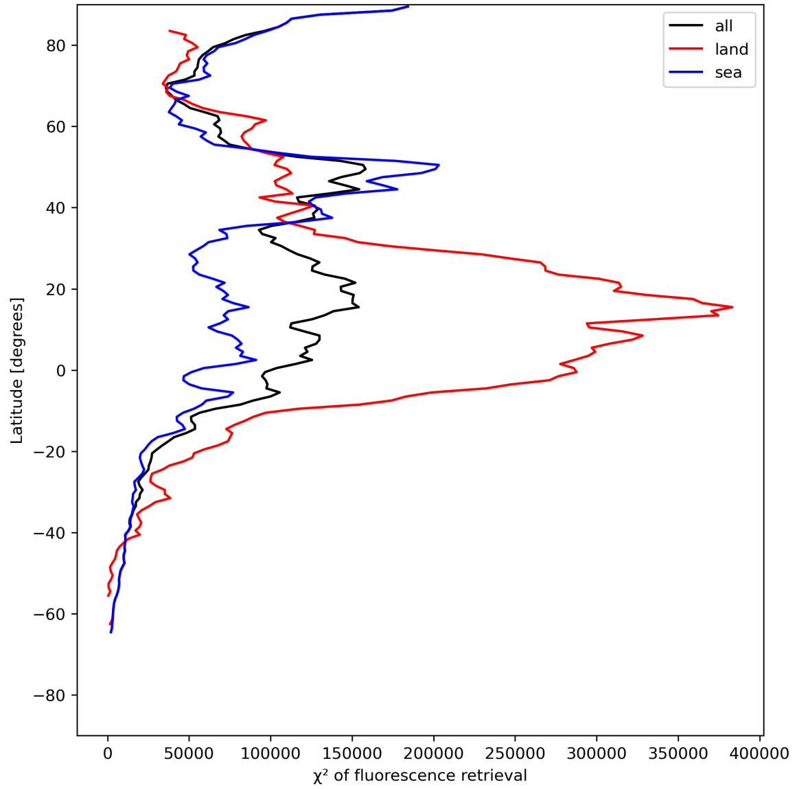
Figure 25: Zonal average of “ \chi^2 of fluorescence retrieval” for 2023-06-30 to 2023-07-02.
