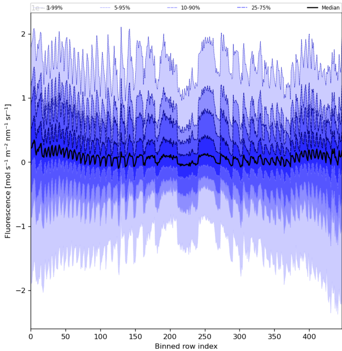
Figure 57: Along track statistics of “Fluorescence” for 2023-06-30 to 2023-07-02
