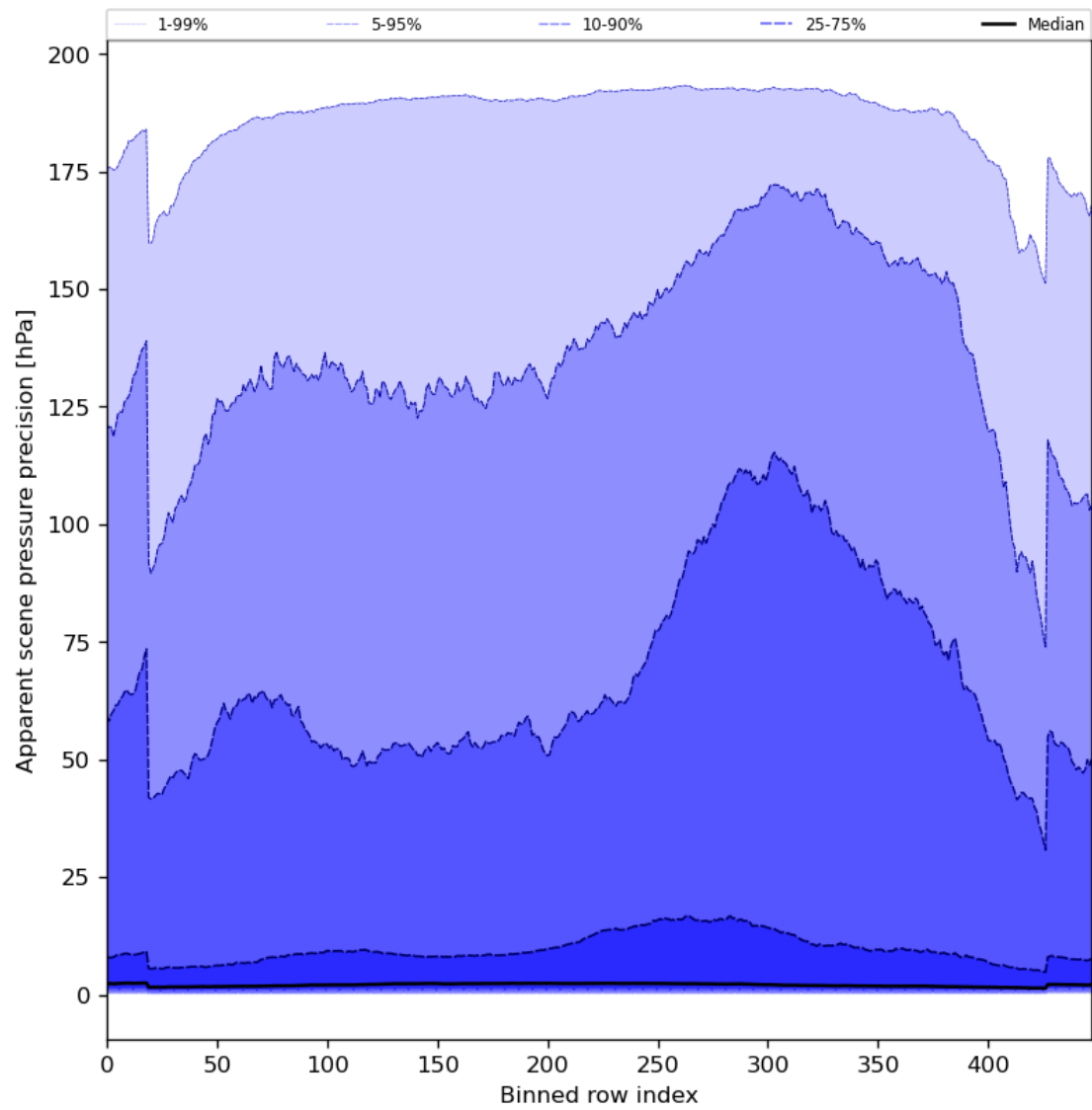
Figure 54: Along track statistics of “Apparent scene pressure precision” for 2023-06-30 to 2023-07-02
