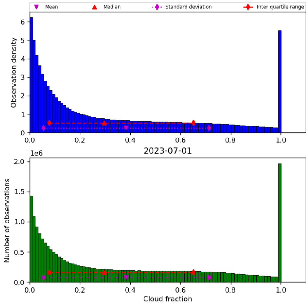
Figure 32: Histogram of “Cloud fraction” for 2023-06-30 to 2023-07-02
