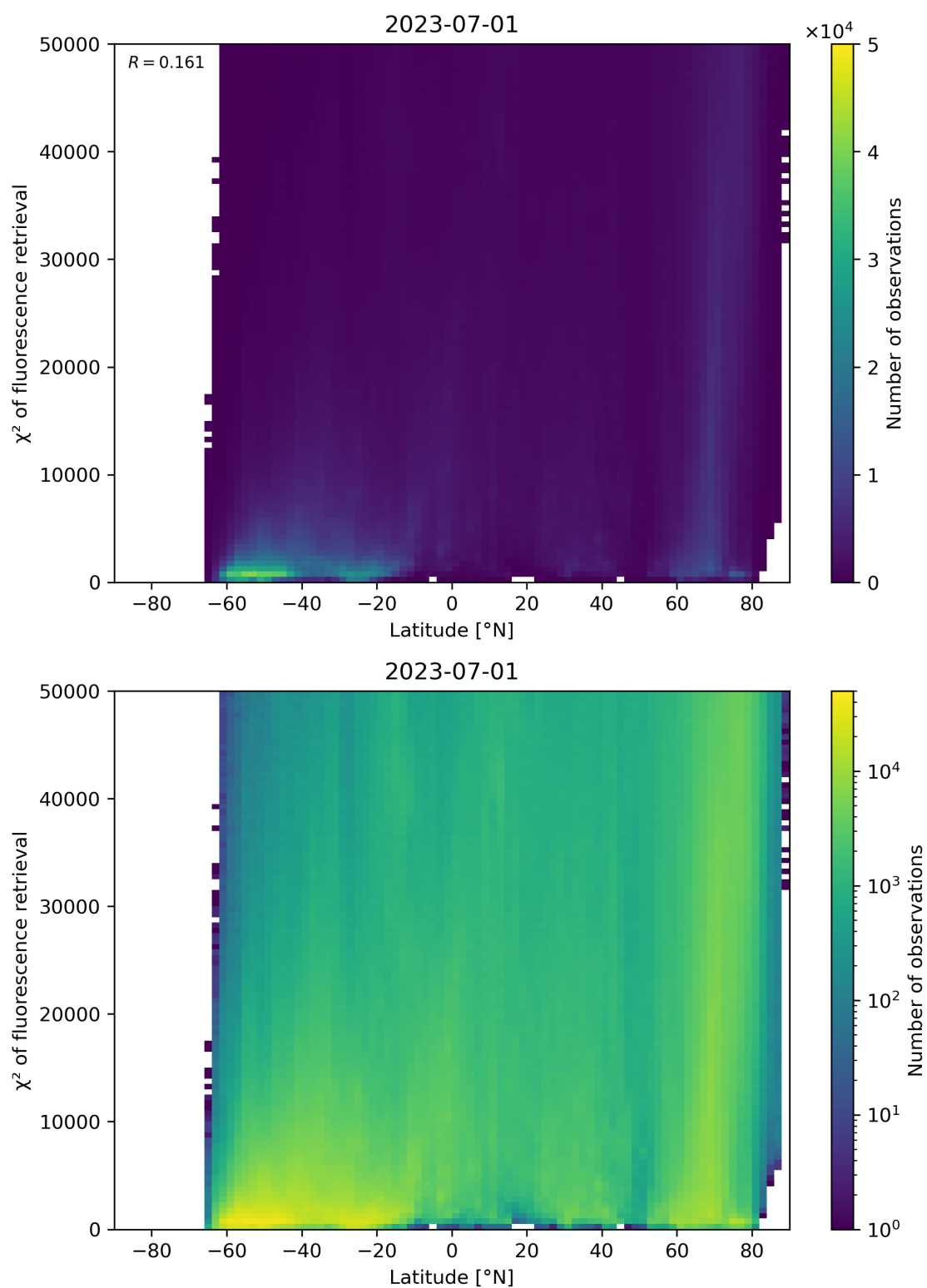
Figure 98: Scatter density plot of “Latitude” against “ \chi^2 of fluorescence retrieval” for 2023-06-30 to 2023-07-02.
