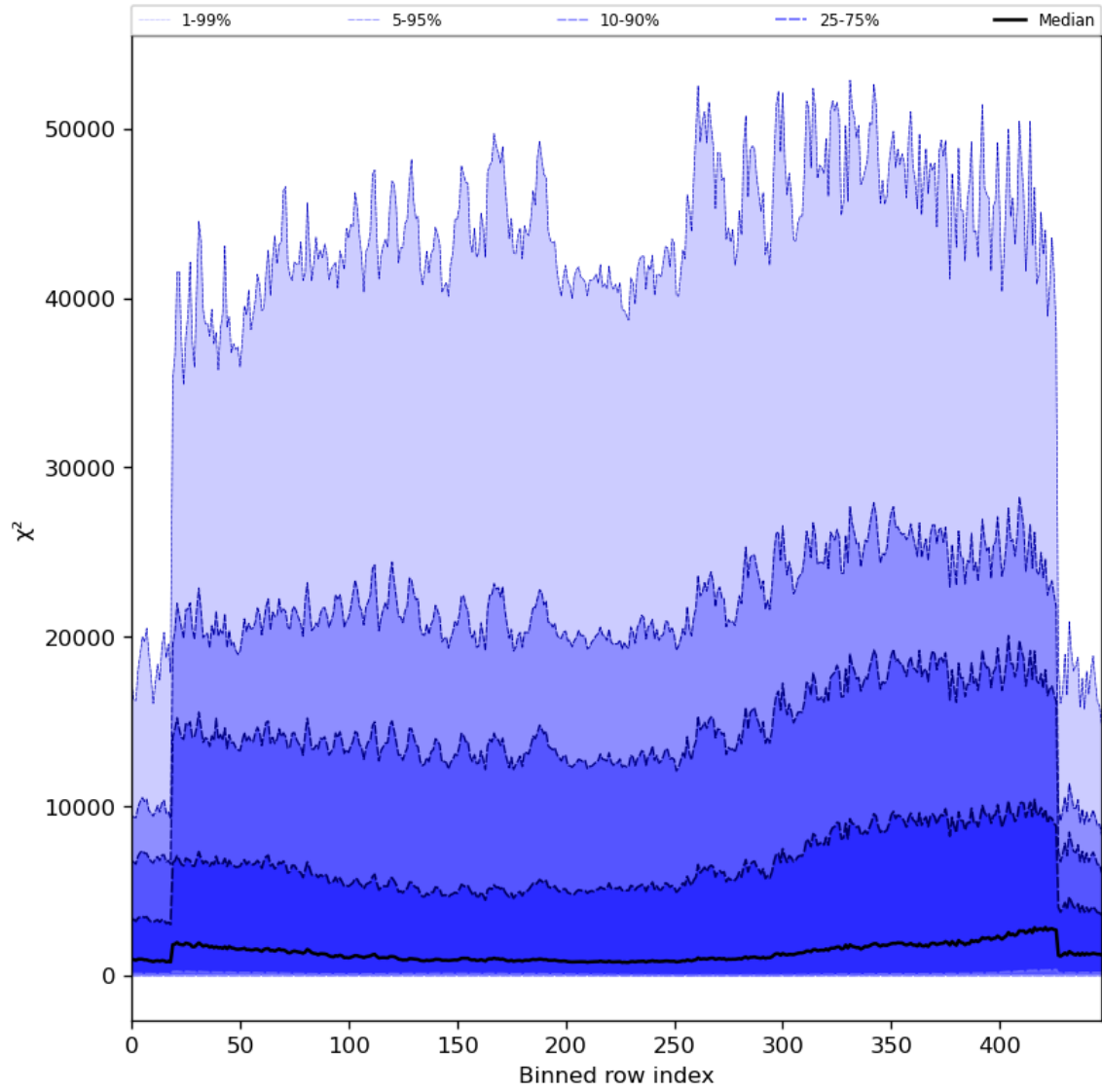
Figure 55: Along track statistics of “ \chi^2 ” for 2023-06-30 to 2023-07-02
