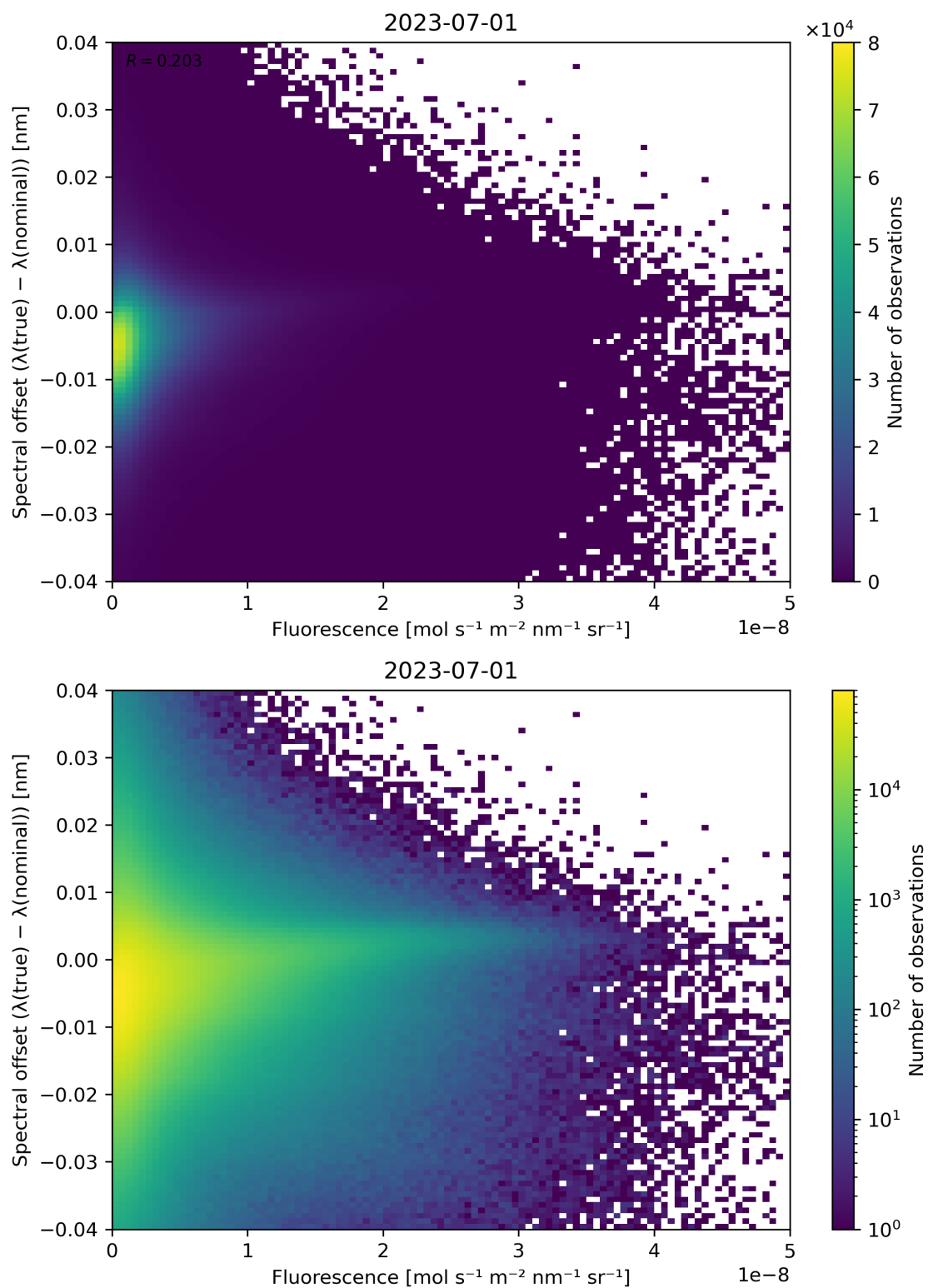
Figure 95: Scatter density plot of “Fluorescence” against “Spectral offset ( \lambda(\text{true}) - \lambda(\text{nominal}) )” for 2023-06-30 to 2023-07-02.
