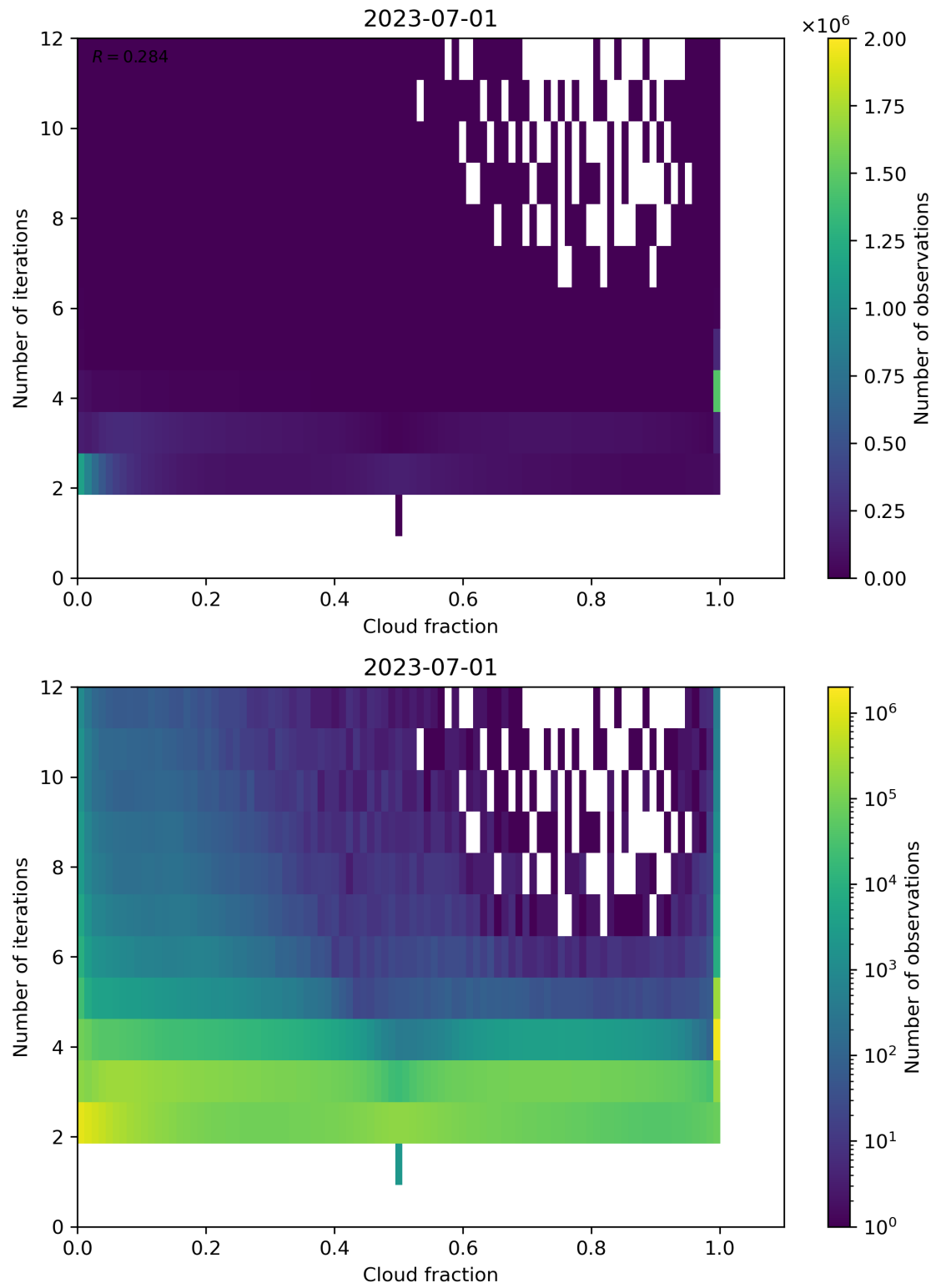
Figure 80: Scatter density plot of “Cloud fraction” against “Number of iterations” for 2023-06-30 to 2023-07-02.
