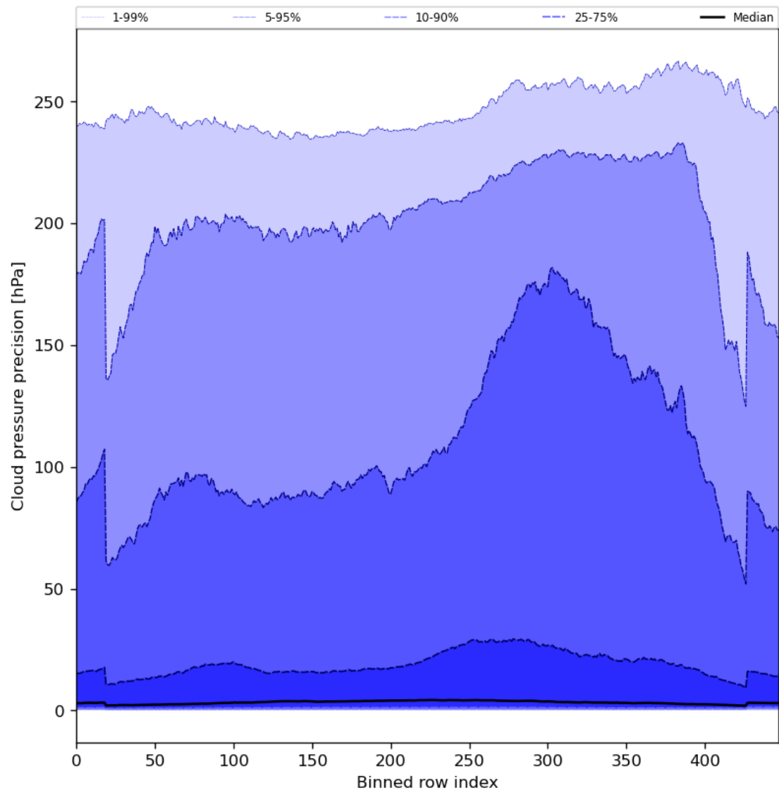
Figure 48: Along track statistics of “Cloud pressure precision” for 2023-06-30 to 2023-07-02
