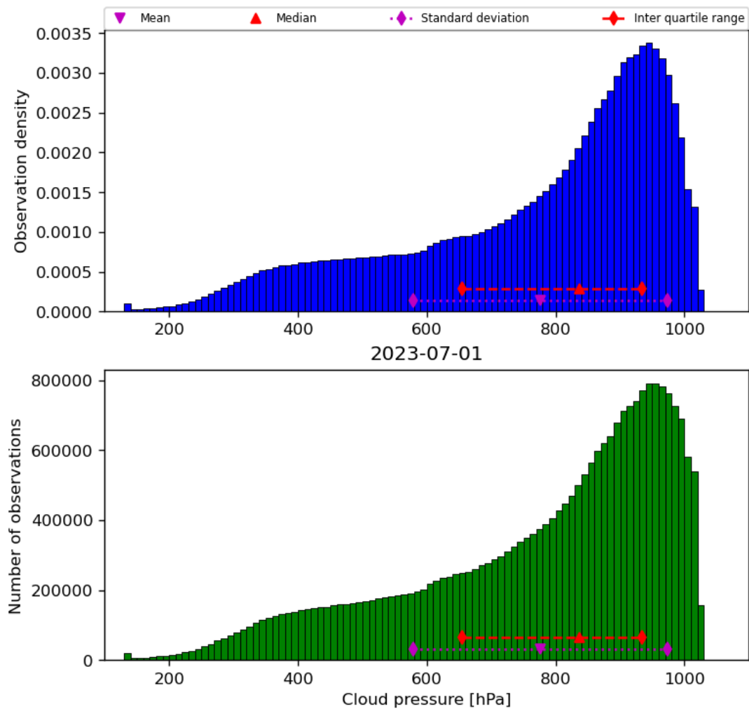
Figure 30: Histogram of “Cloud pressure” for 2023-06-30 to 2023-07-02
