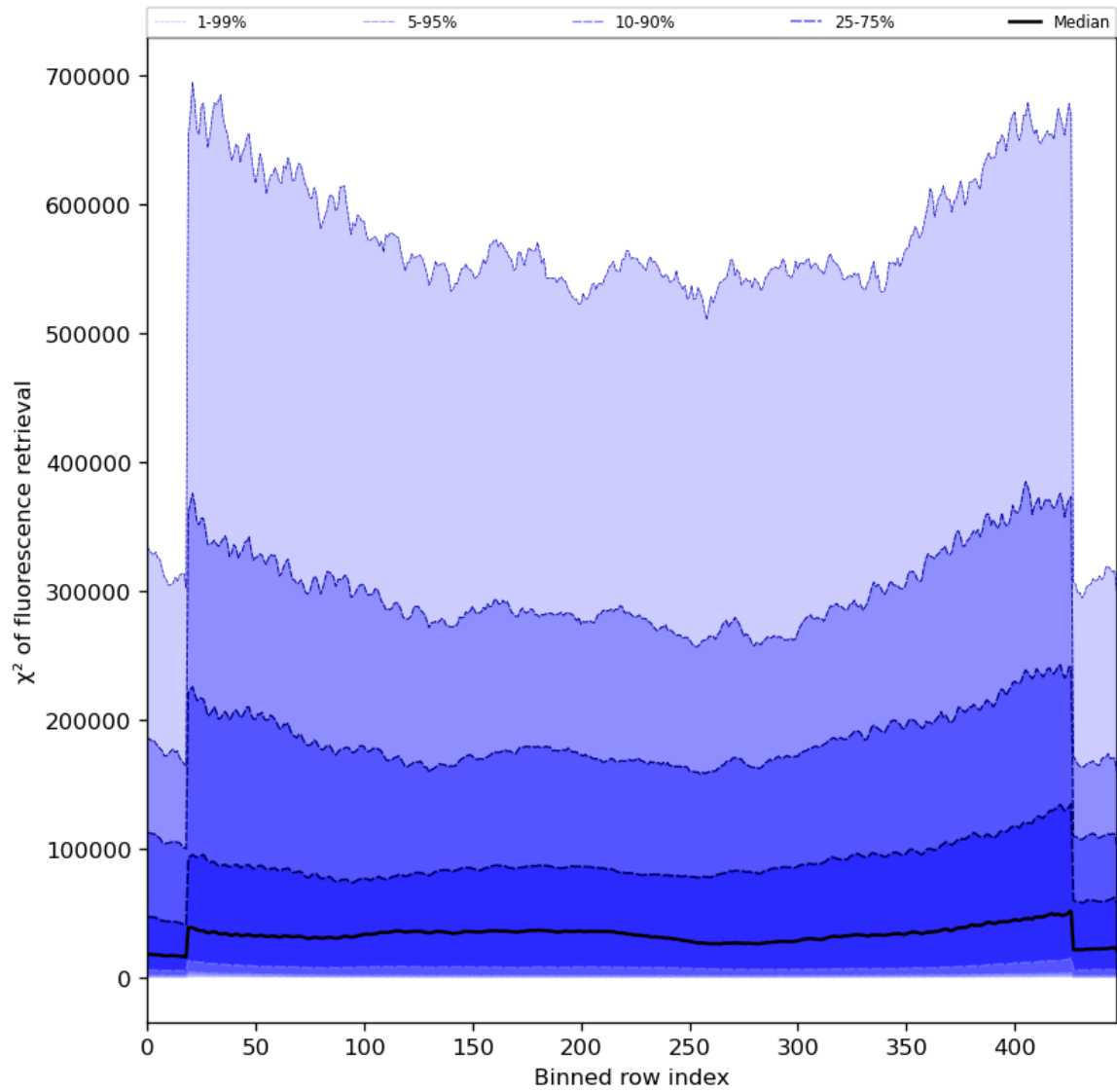
Figure 59: Along track statistics of “ \chi^2 of fluorescence retrieval” for 2023-06-30 to 2023-07-02
