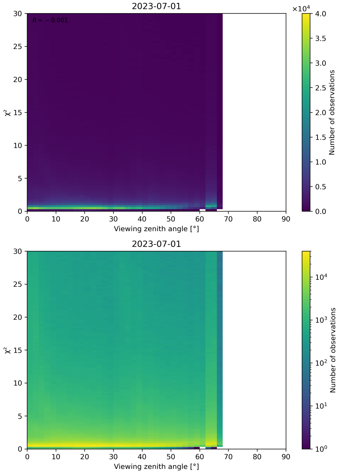
Figure 130: Scatter density plot of “Viewing zenith angle” against “ \chi^2 ” for 2023-06-30 to 2023-07-02.
