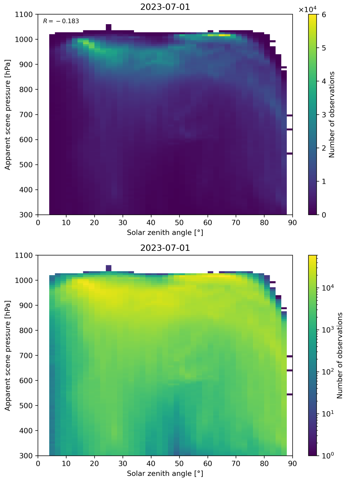
Figure 118: Scatter density plot of “Solar zenith angle” against “Apparent scene pressure” for 2023-06-30 to 2023-07-02.
