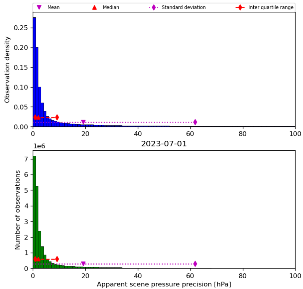
Figure 37: Histogram of “Apparent scene pressure precision” for 2023-06-30 to 2023-07-02
