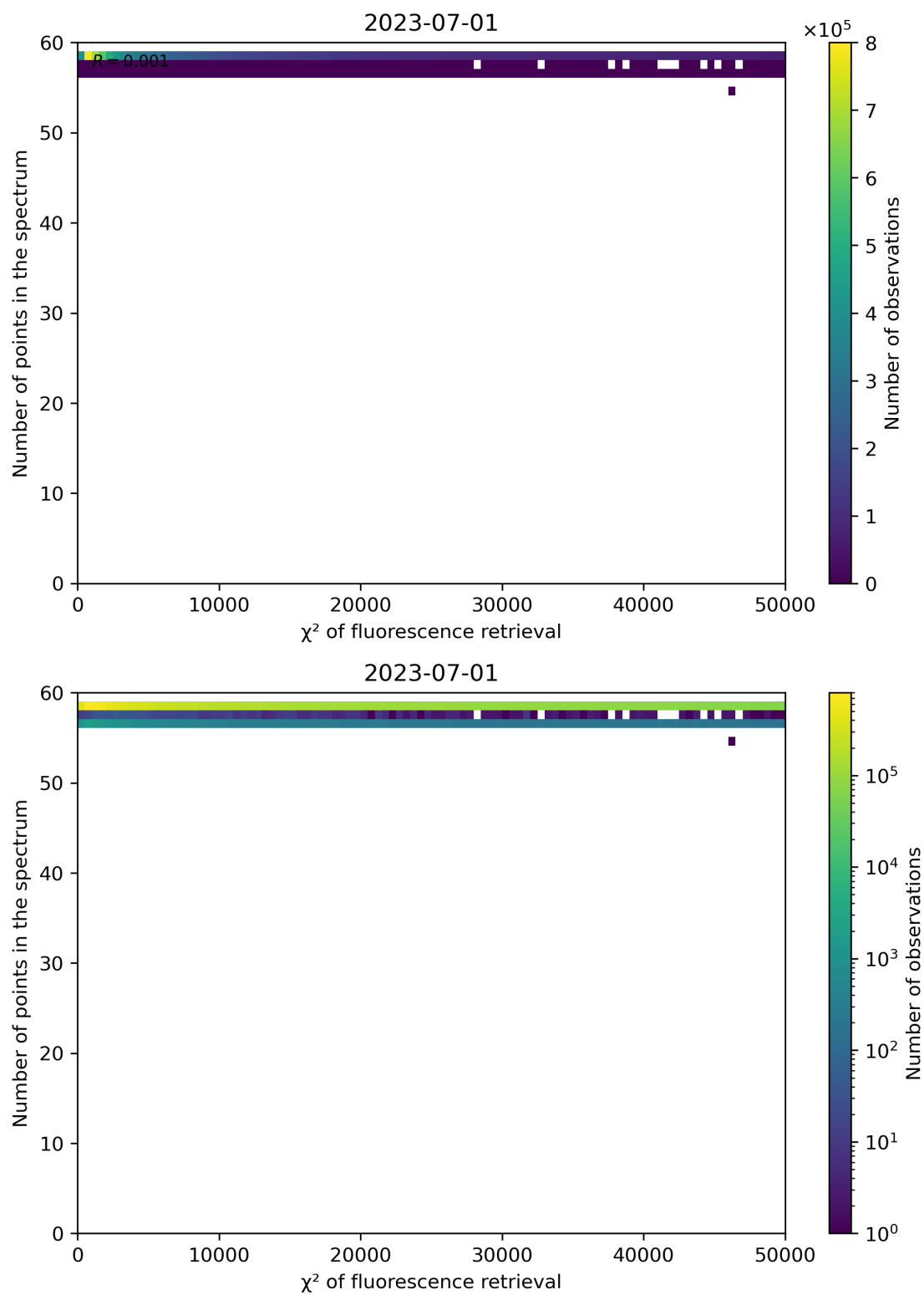
Figure 71: Scatter density plot of “ \chi^2 of fluorescence retrieval” against “Number of points in the spectrum” for 2023-06-30 to 2023-07-02.
