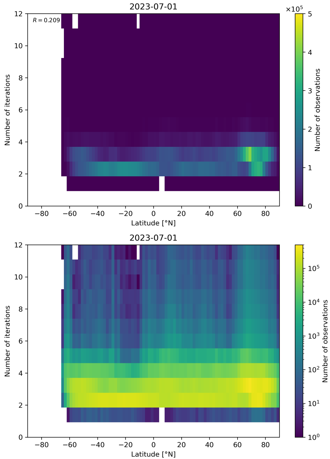
Figure 102: Scatter density plot of “Latitude” against “Number of iterations” for 2023-06-30 to 2023-07-02.
