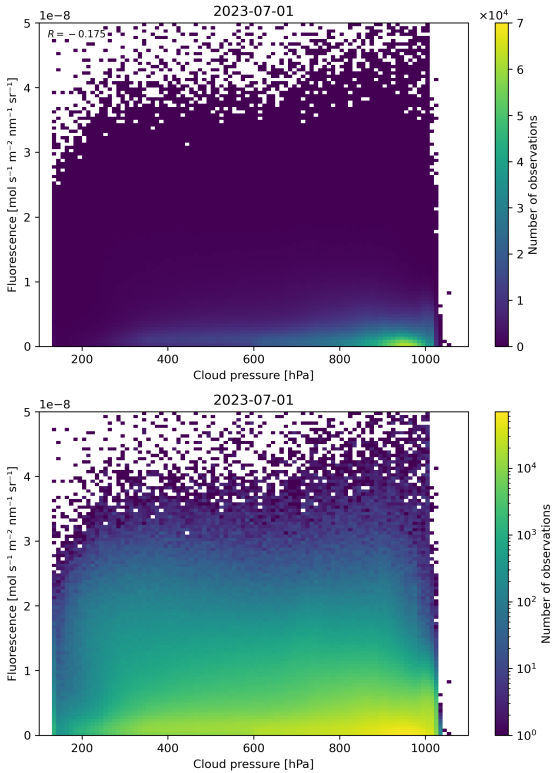
Figure 88: Scatter density plot of “Cloud pressure” against “Fluorescence” for 2023-06-30 to 2023-07-02.
