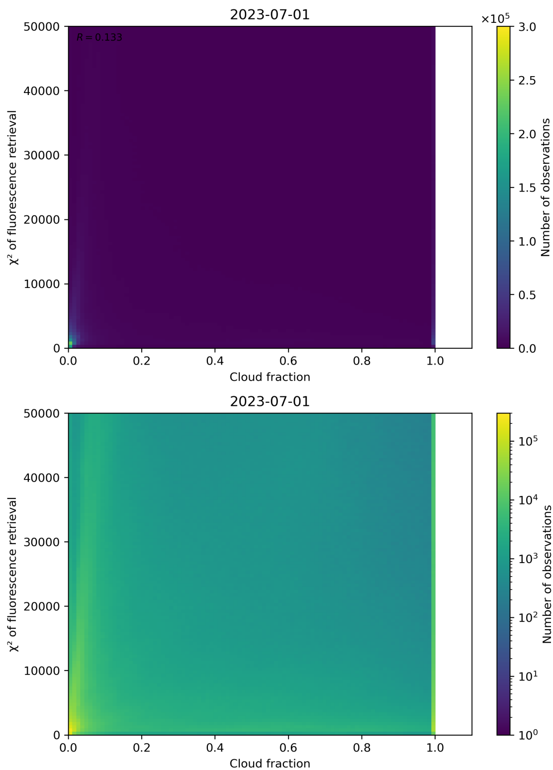
Figure 78: Scatter density plot of “Cloud fraction” against “ \chi^2 of fluorescence retrieval” for 2023-06-30 to 2023-07-02.
