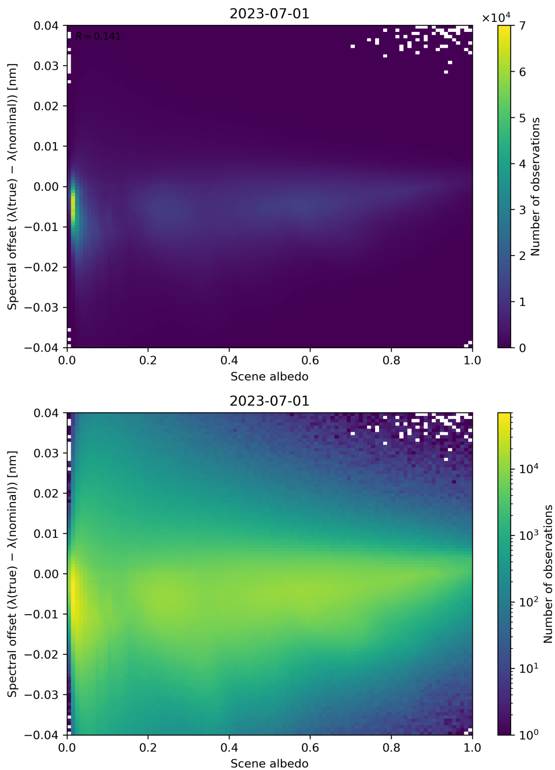
Figure 117: Scatter density plot of “Scene albedo” against “Spectral offset ( \lambda(\text{true}) - \lambda(\text{nominal}) )” for 2023-06-30 to 2023-07-02.
