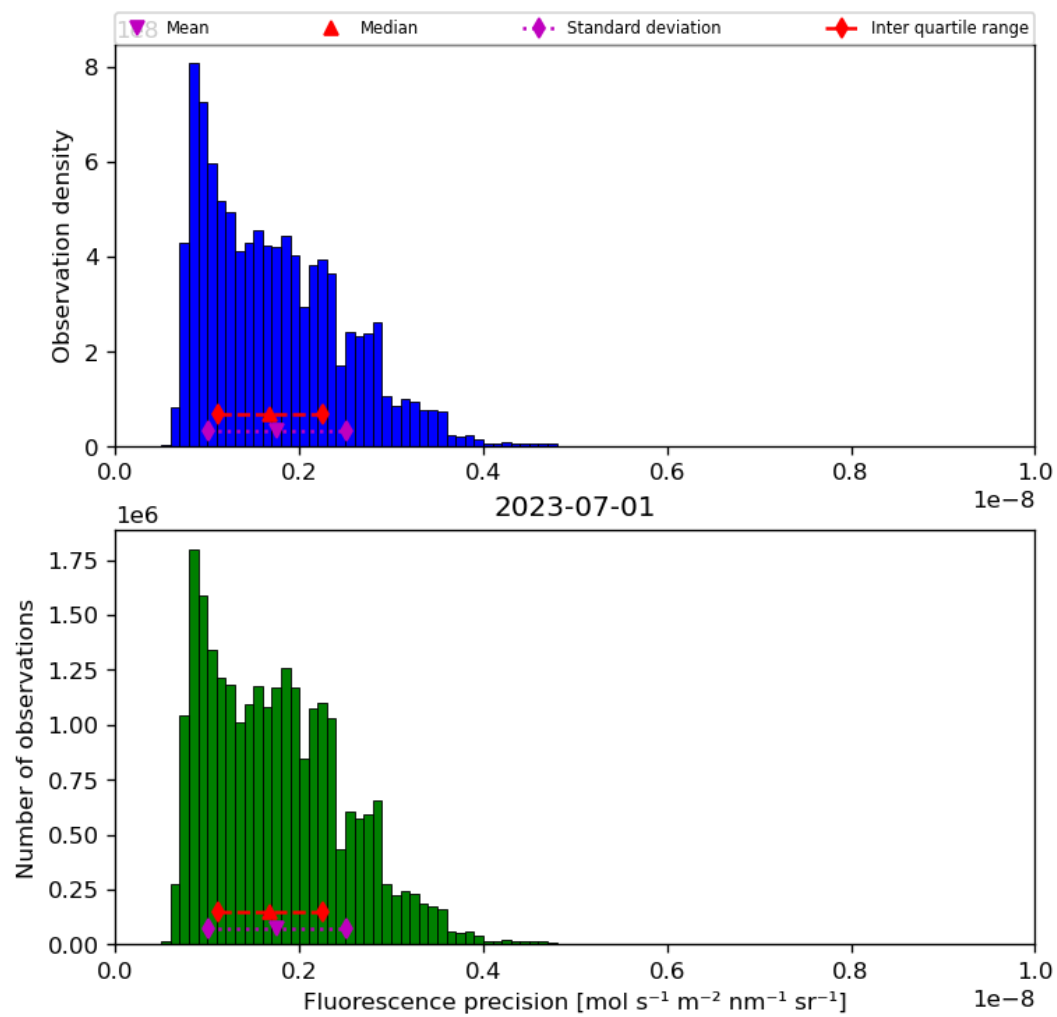
Figure 41: Histogram of “Fluorescence precision” for 2023-06-30 to 2023-07-02
