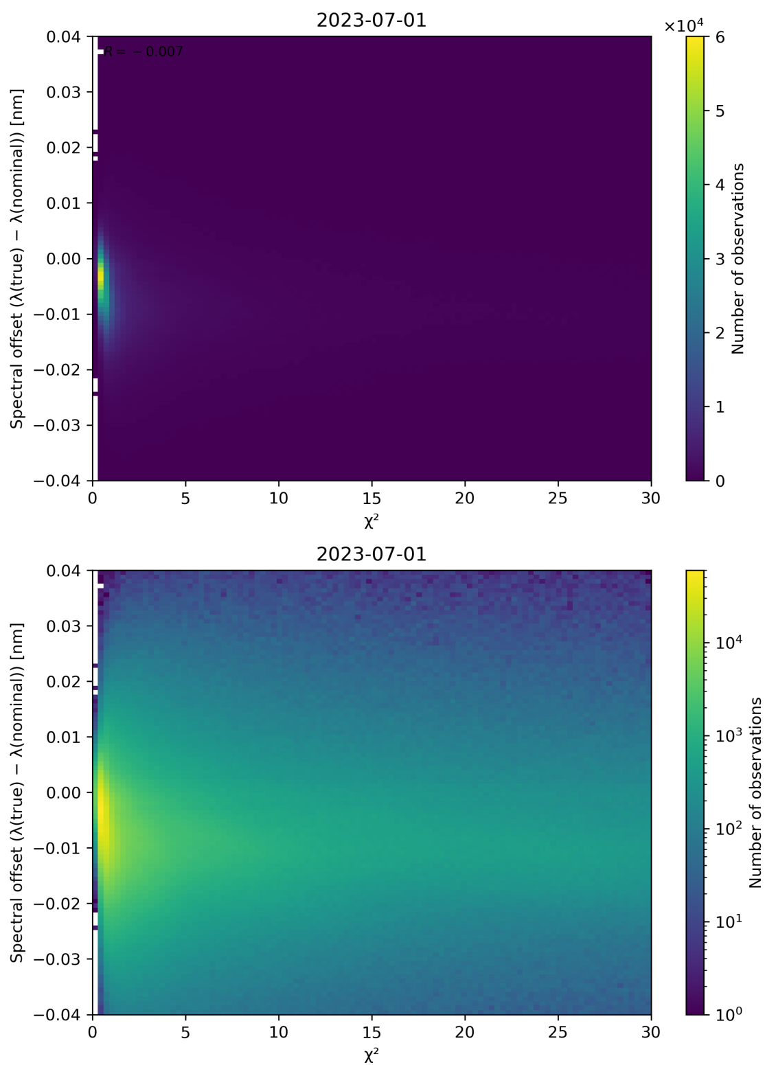
Figure 75: Scatter density plot of “ \chi^2 ” against “Spectral offset ( \lambda(\text{true}) - \lambda(\text{nominal}) )” for 2023-06-30 to 2023-07-02.
