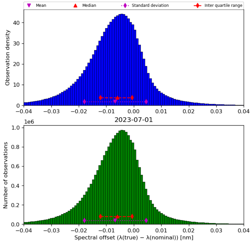
Figure 45: Histogram of “Spectral offset ( \lambda(\text{true}) - \lambda(\text{nominal}) )” for 2023-06-30 to 2023-07-02
