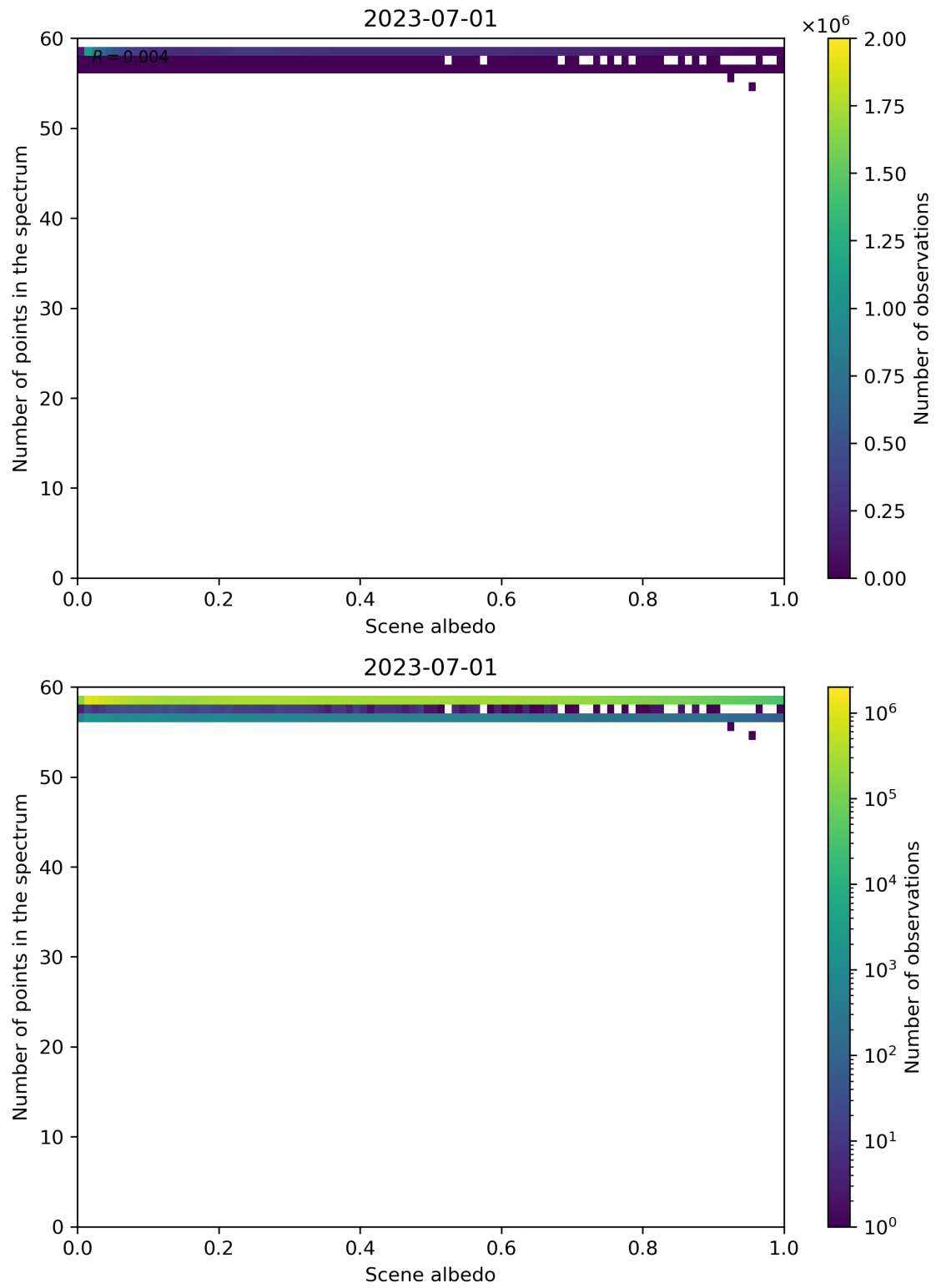
Figure 116: Scatter density plot of “Scene albedo” against “Number of points in the spectrum” for 2023-06-30 to 2023-07-02.
