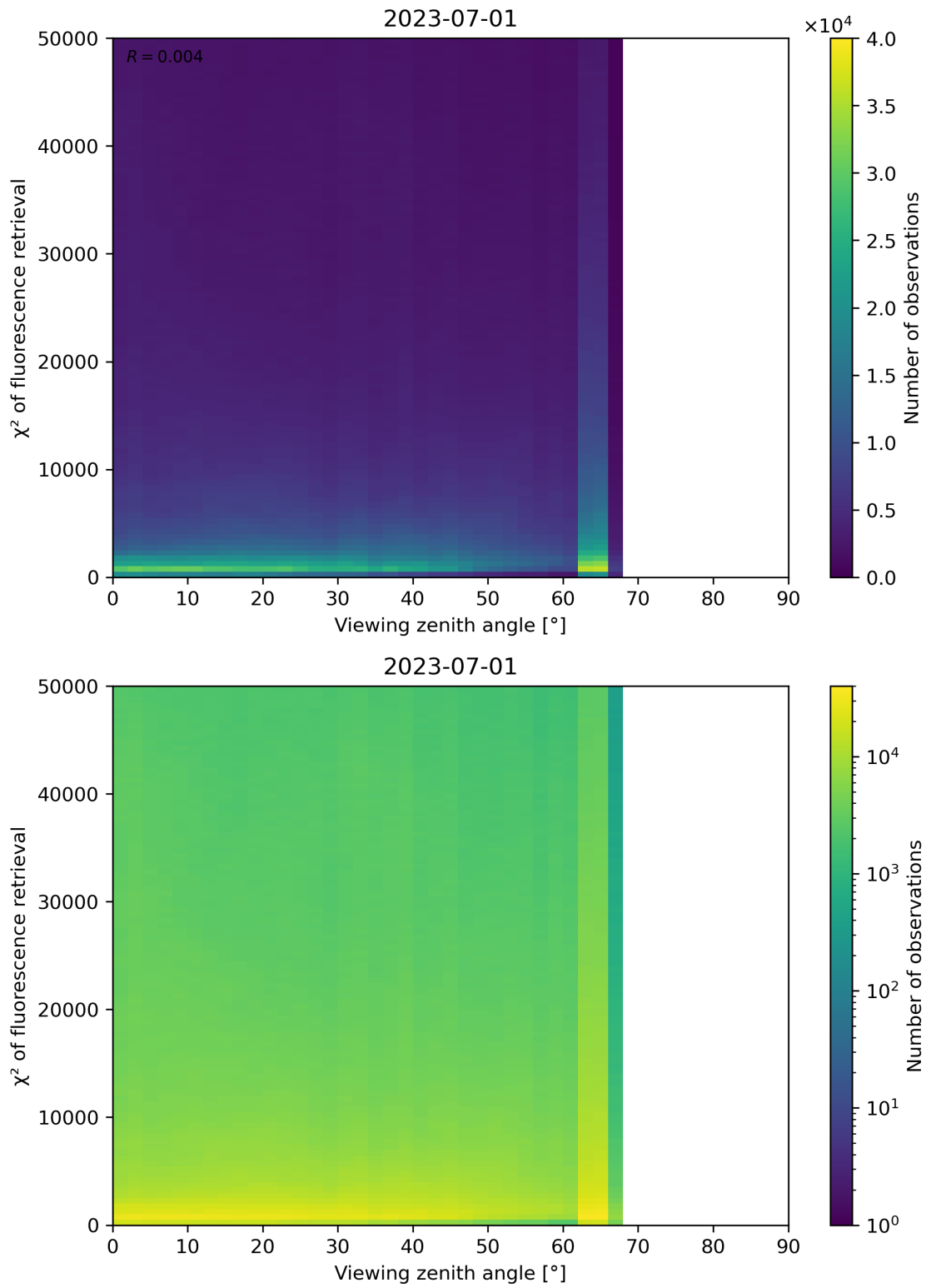
Figure 131: Scatter density plot of “Viewing zenith angle” against “ \chi^2 of fluorescence retrieval” for 2023-06-30 to 2023-07-02.
