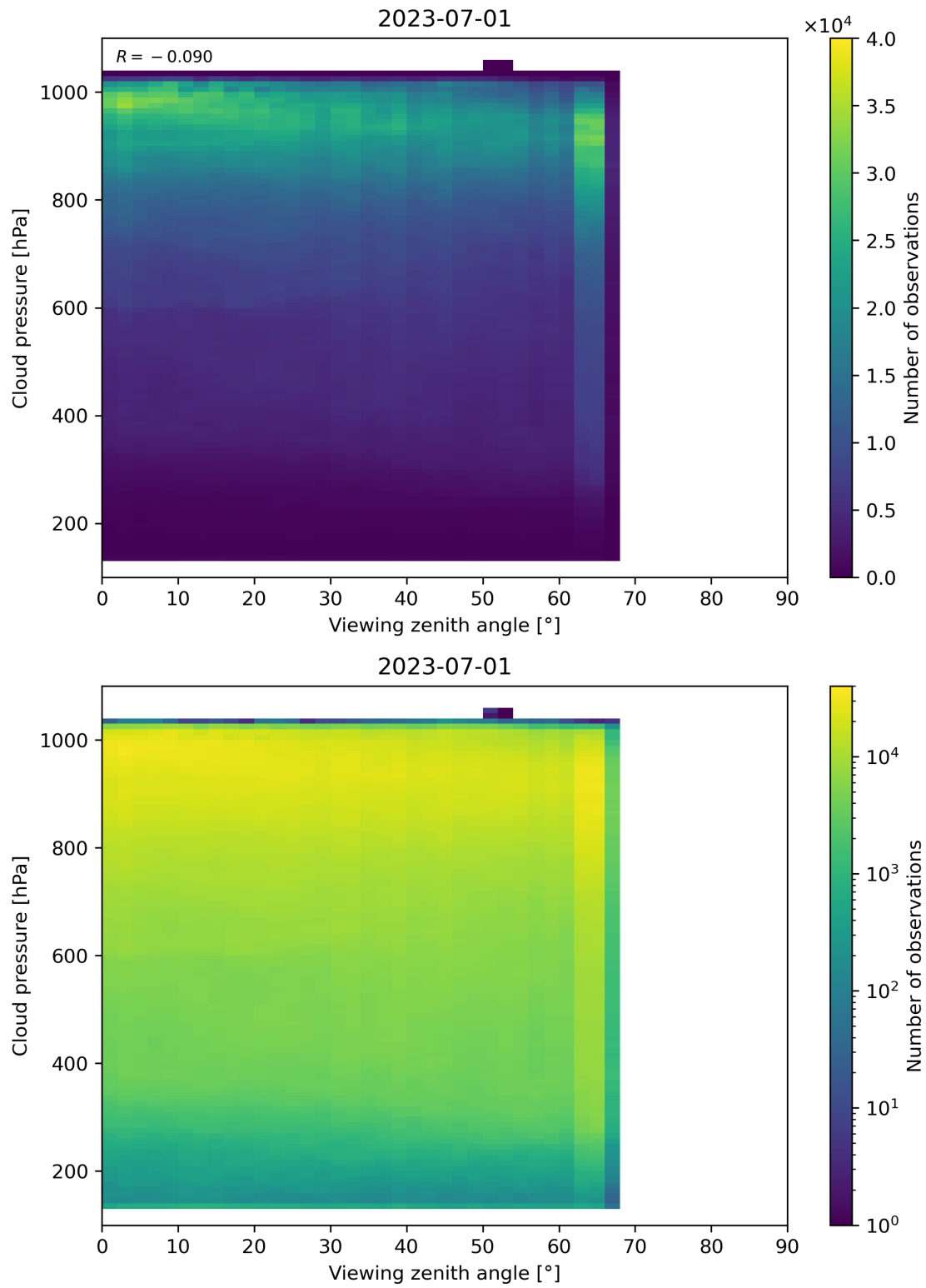
Figure 133: Scatter density plot of “Viewing zenith angle” against “Cloud pressure” for 2023-06-30 to 2023-07-02.
