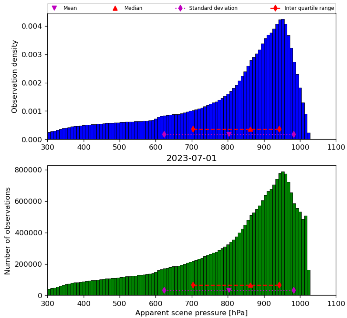
Figure 36: Histogram of “Apparent scene pressure” for 2023-06-30 to 2023-07-02
