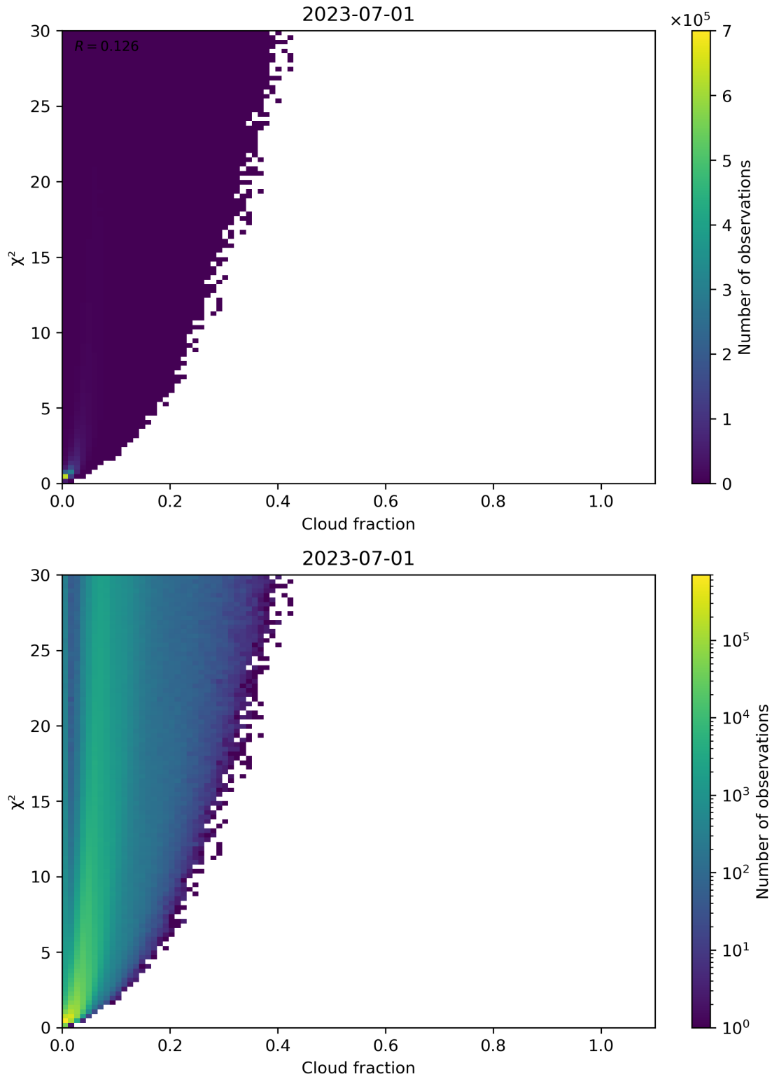
Figure 77: Scatter density plot of “Cloud fraction” against “ \chi^2 ” for 2023-06-30 to 2023-07-02.
