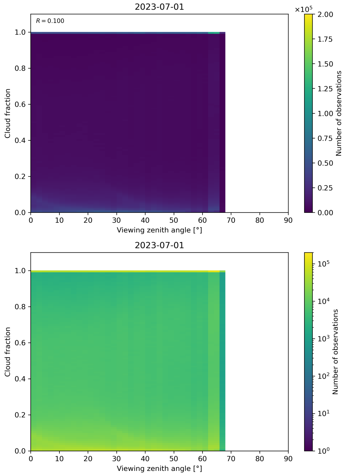
Figure 132: Scatter density plot of “Viewing zenith angle” against “Cloud fraction” for 2023-06-30 to 2023-07-02.
