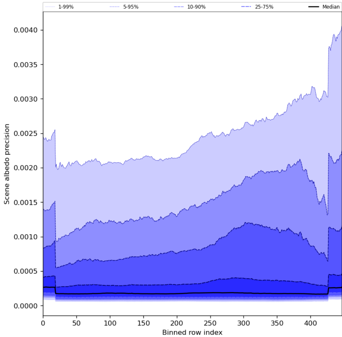
Figure 52: Along track statistics of “Scene albedo precision” for 2023-06-30 to 2023-07-02
