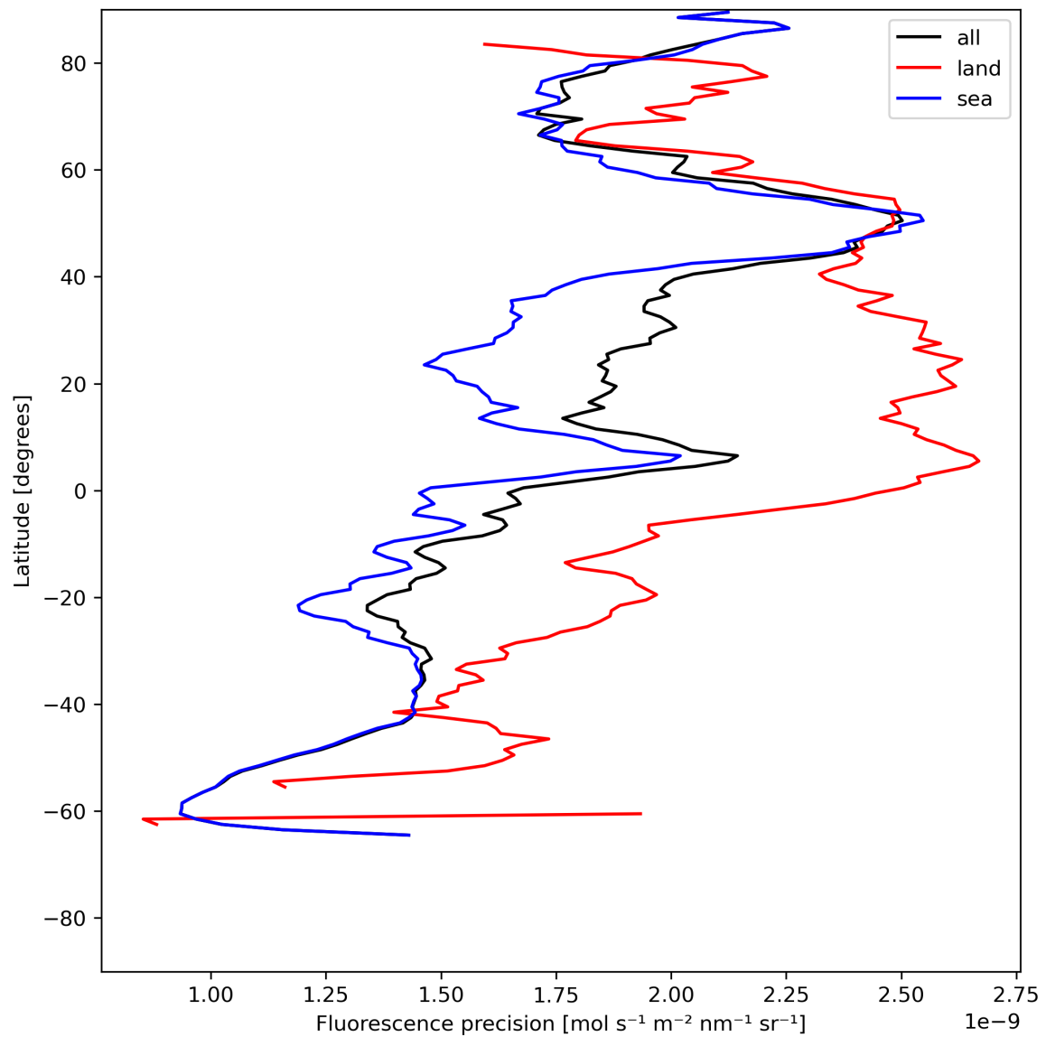
Figure 24: Zonal average of “Fluorescence precision” for 2023-06-30 to 2023-07-02.
