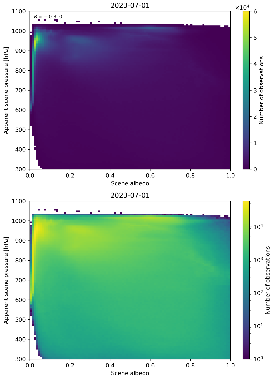
Figure 111: Scatter density plot of “Scene albedo” against “Apparent scene pressure” for 2023-06-30 to 2023-07-02.
