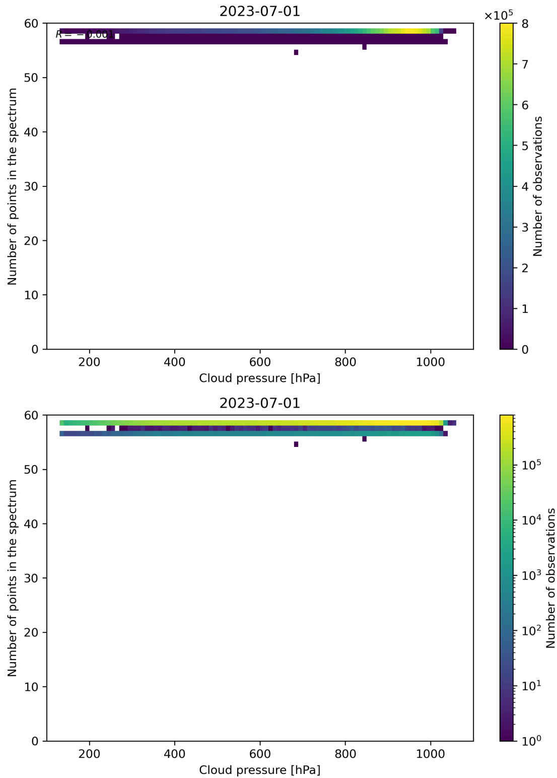
Figure 90: Scatter density plot of “Cloud pressure” against “Number of points in the spectrum” for 2023-06-30 to 2023-07-02.
