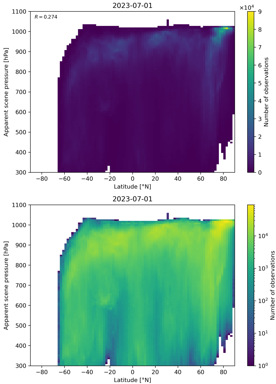
Figure 96: Scatter density plot of “Latitude” against “Apparent scene pressure” for 2023-06-30 to 2023-07-02.
