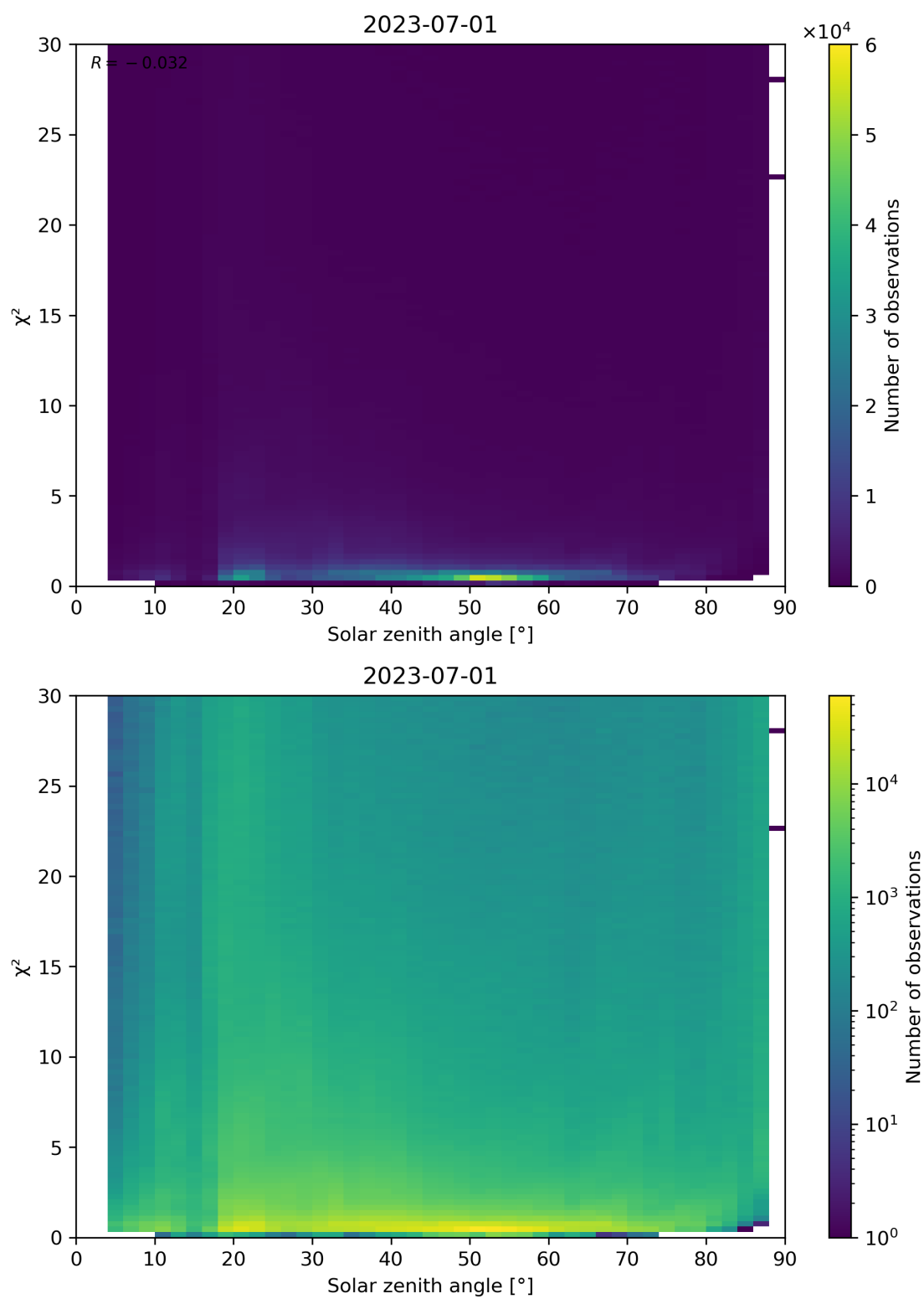
Figure 119: Scatter density plot of “Solar zenith angle” against “ \chi^2 ” for 2023-06-30 to 2023-07-02.
