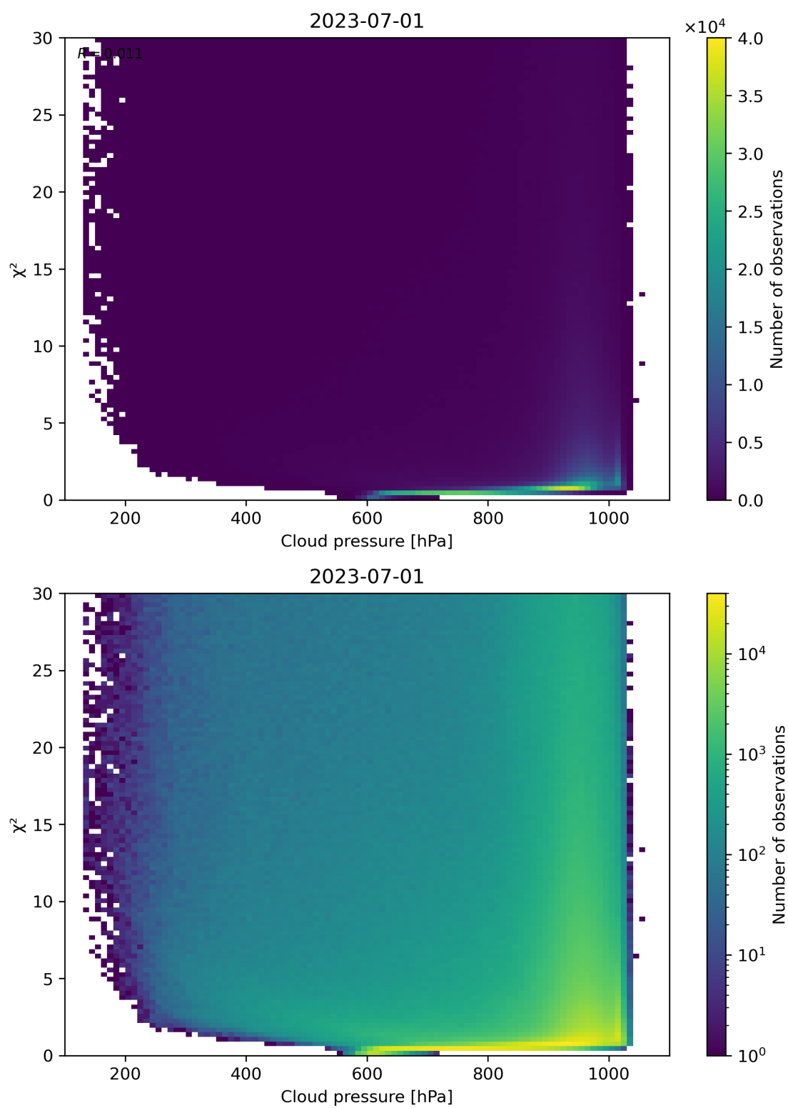
Figure 85: Scatter density plot of “Cloud pressure” against “ \chi^2 ” for 2023-06-30 to 2023-07-02.
