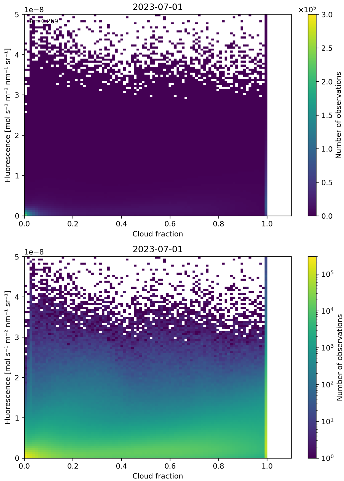
Figure 79: Scatter density plot of “Cloud fraction” against “Fluorescence” for 2023-06-30 to 2023-07-02.
