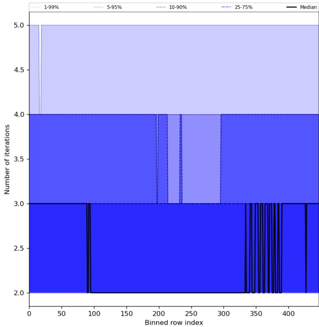
Figure 56: Along track statistics of “Number of iterations” for 2023-06-30 to 2023-07-02
