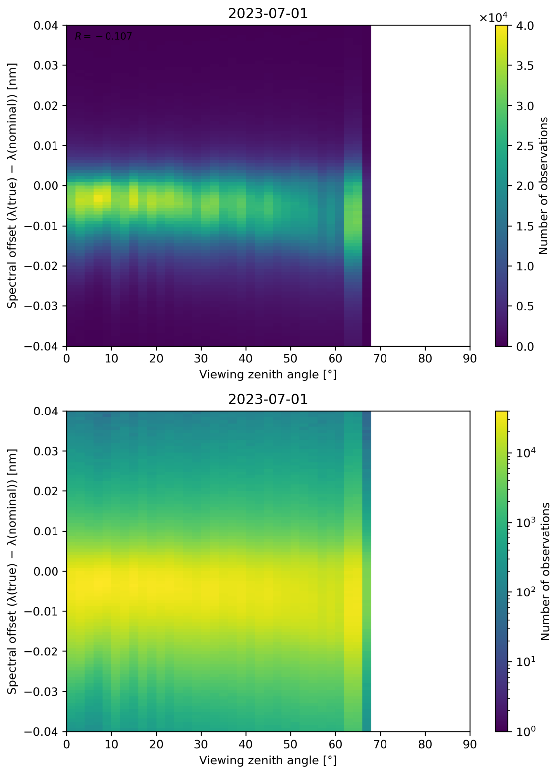
Figure 140: Scatter density plot of “Viewing zenith angle” against “Spectral offset ( \lambda(\text{true}) - \lambda(\text{nominal}) )” for 2023-06-30 to 2023-07-02.
