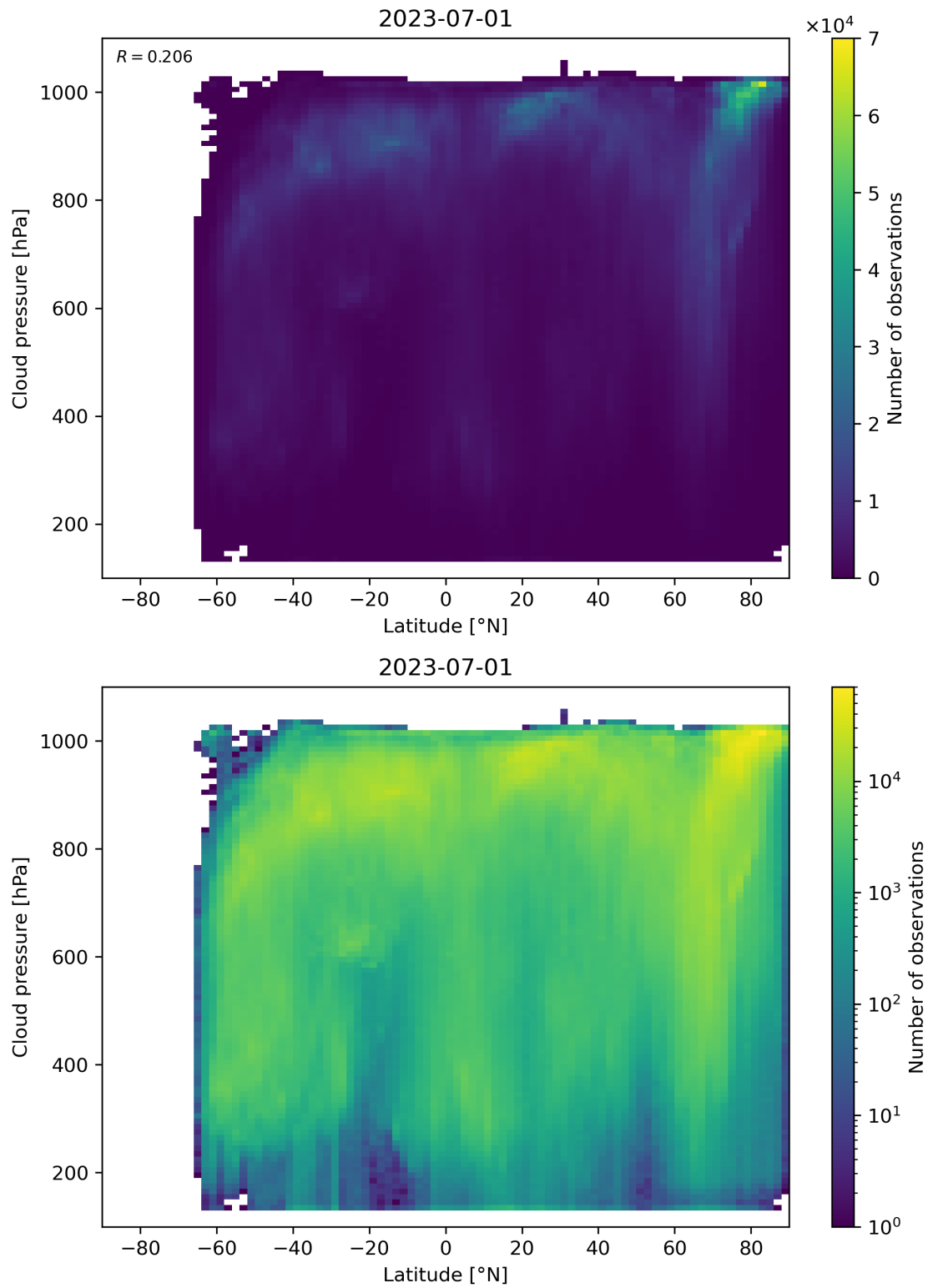
Figure 100: Scatter density plot of “Latitude” against “Cloud pressure” for 2023-06-30 to 2023-07-02.
