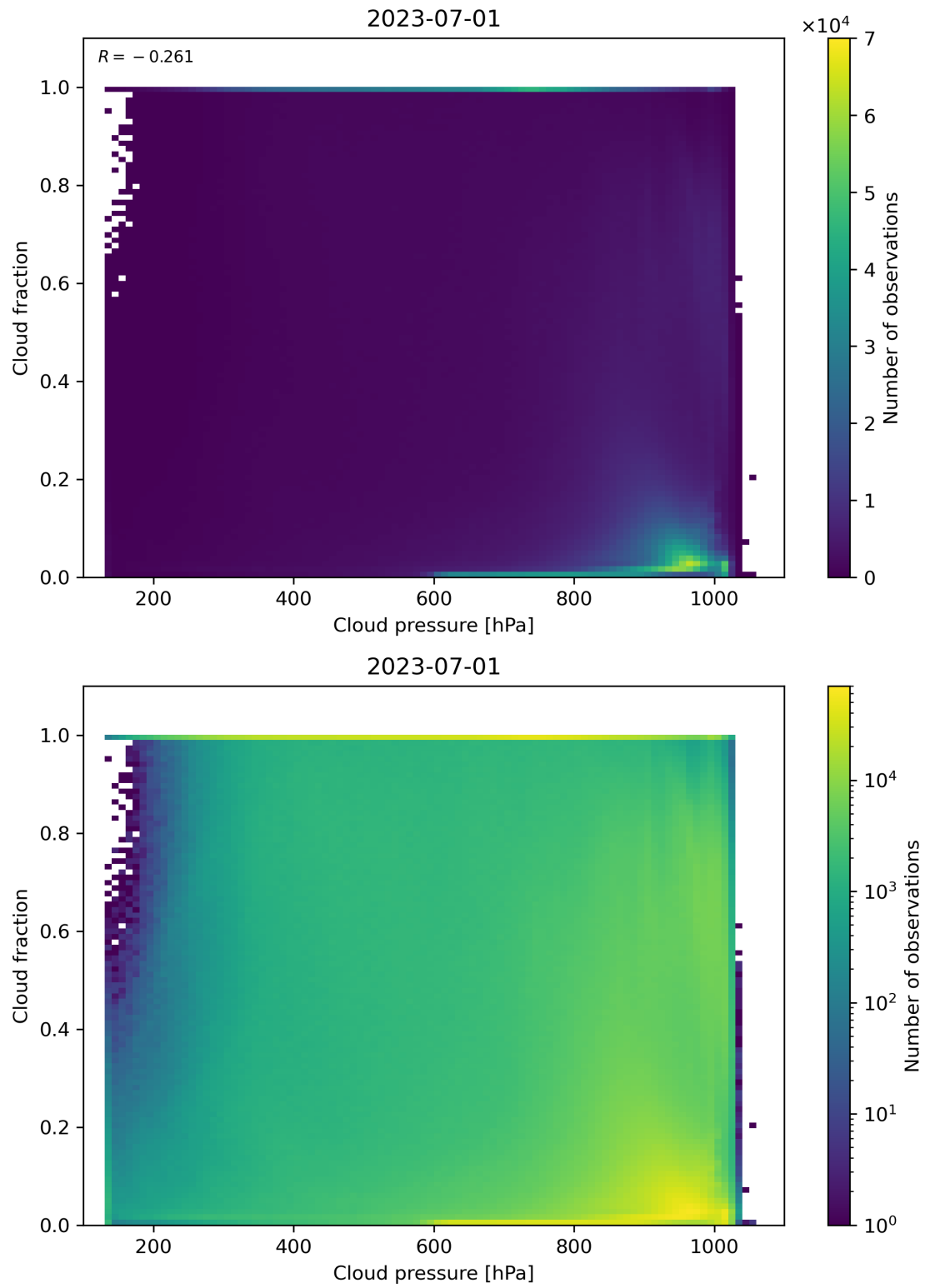
Figure 87: Scatter density plot of “Cloud pressure” against “Cloud fraction” for 2023-06-30 to 2023-07-02.
