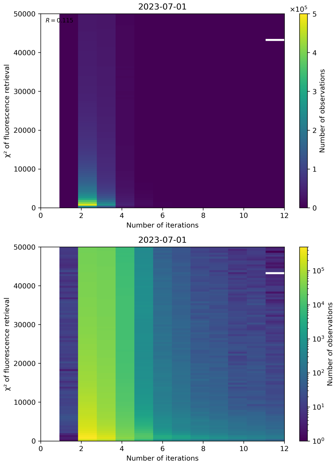
Figure 106: Scatter density plot of “Number of iterations” against “ \chi^2 of fluorescence retrieval” for 2023-06-30 to 2023-07-02.
