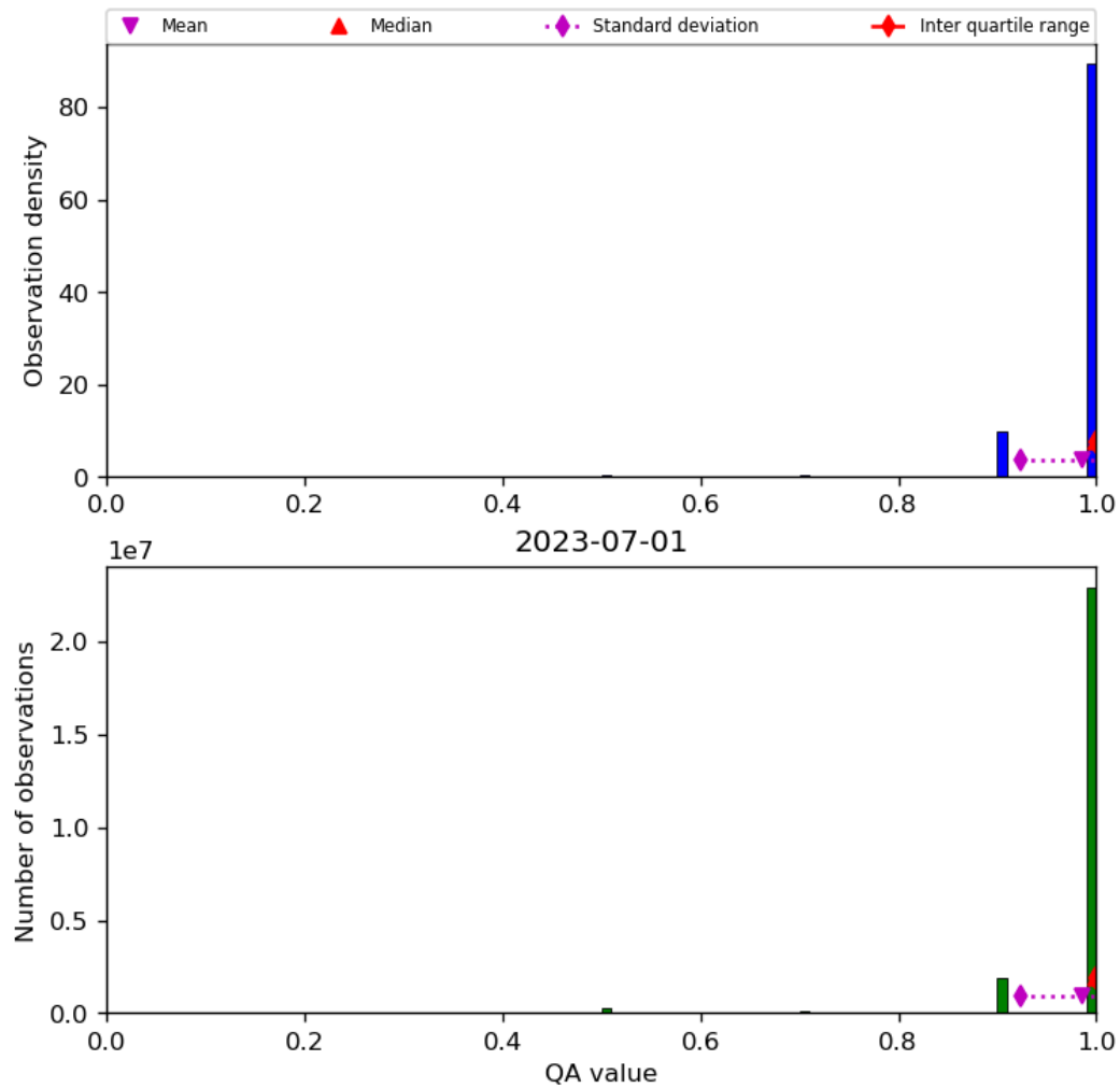
Figure 29: Histogram of “QA value” for 2023-06-30 to 2023-07-02
