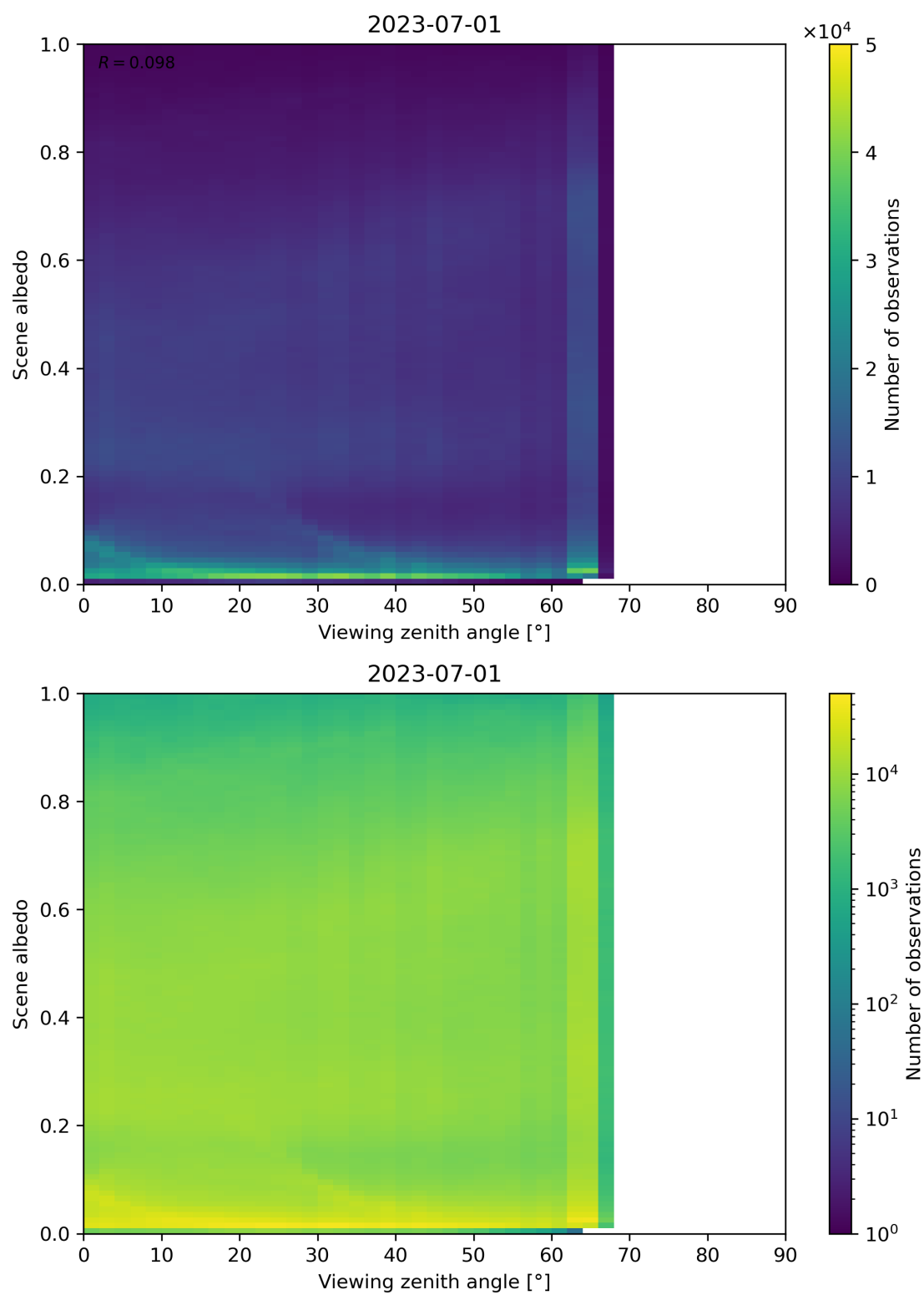
Figure 138: Scatter density plot of “Viewing zenith angle” against “Scene albedo” for 2023-06-30 to 2023-07-02.
