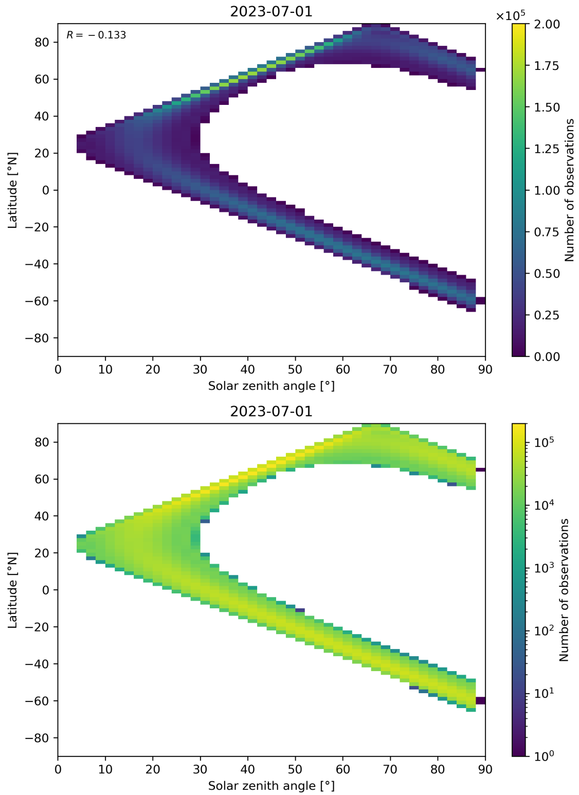
Figure 124: Scatter density plot of “Solar zenith angle” against “Latitude” for 2023-06-30 to 2023-07-02.
