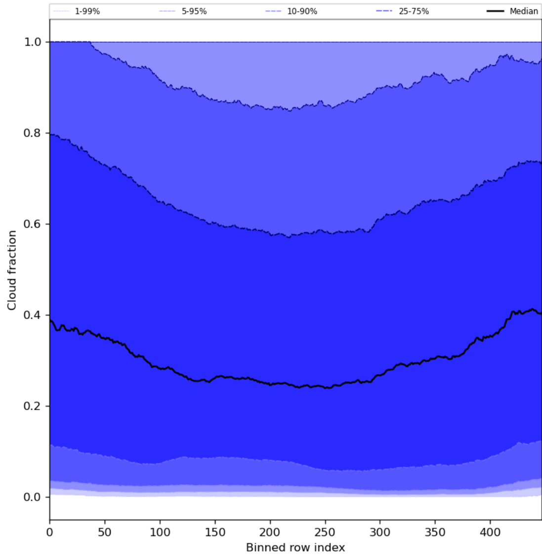
Figure 49: Along track statistics of “Cloud fraction” for 2023-06-30 to 2023-07-02
