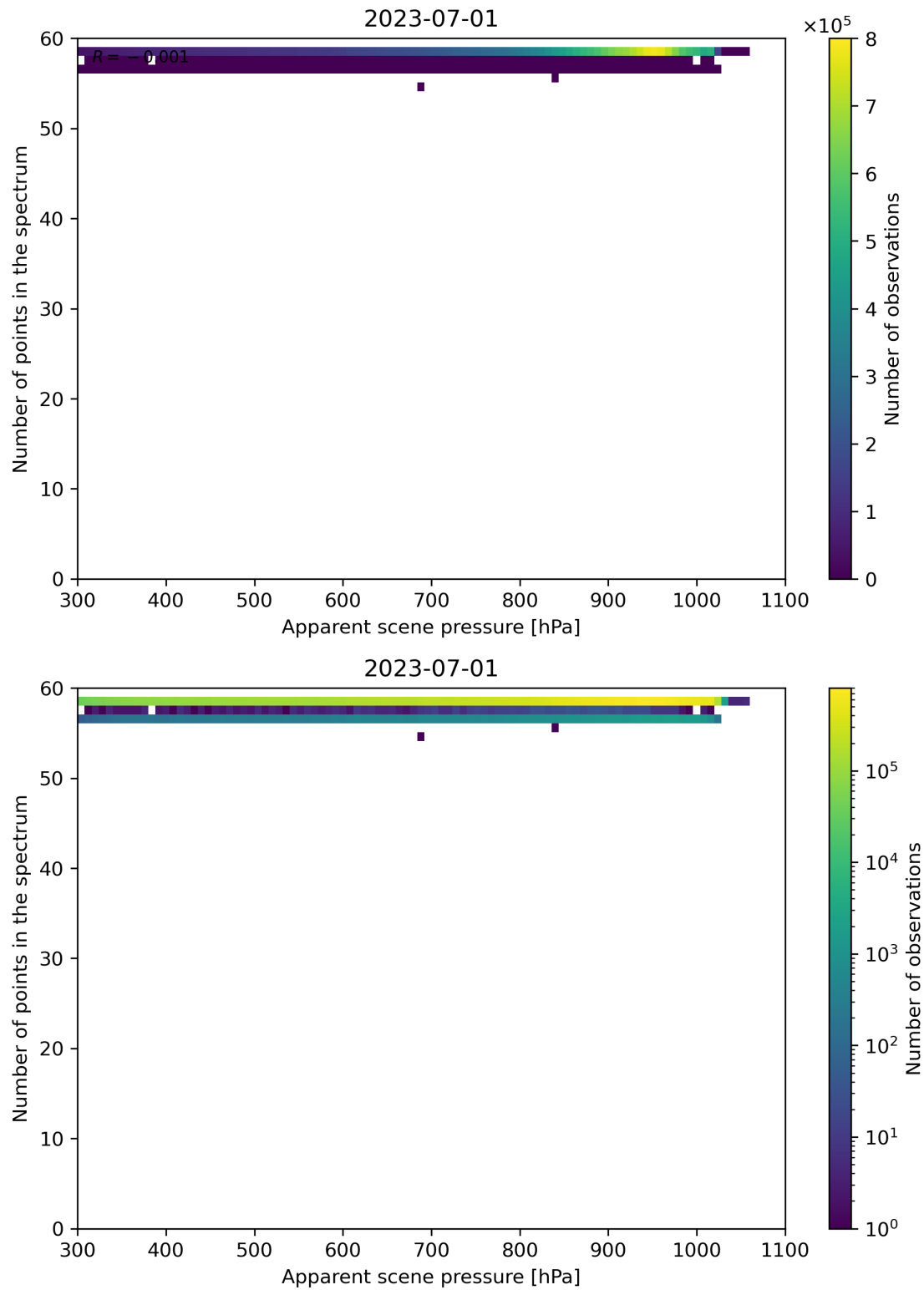
Figure 67: Scatter density plot of “Apparent scene pressure” against “Number of points in the spectrum” for 2023-06-30 to 2023-07-02.
