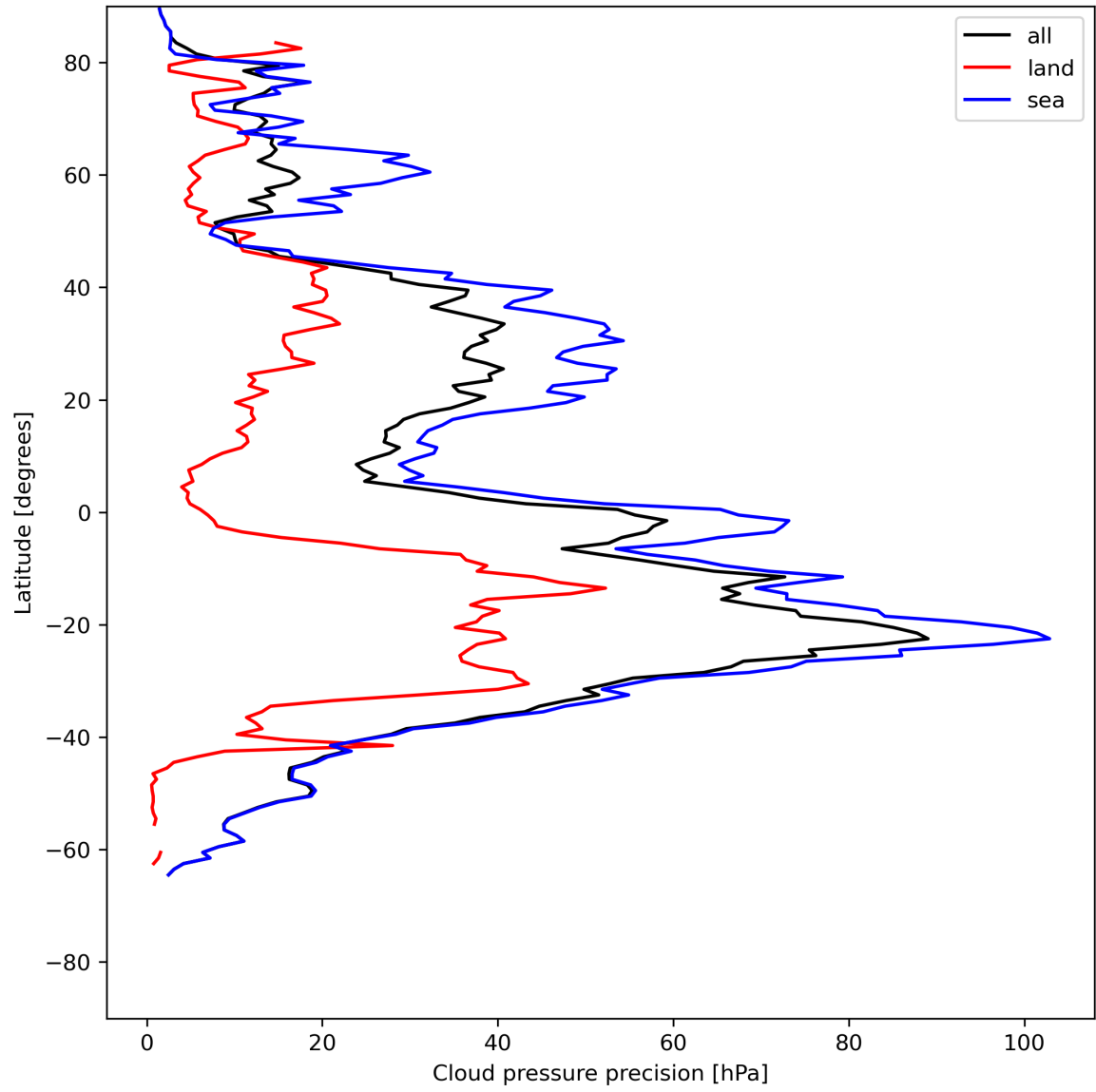
Figure 14: Zonal average of “Cloud pressure precision” for 2023-06-30 to 2023-07-02.
