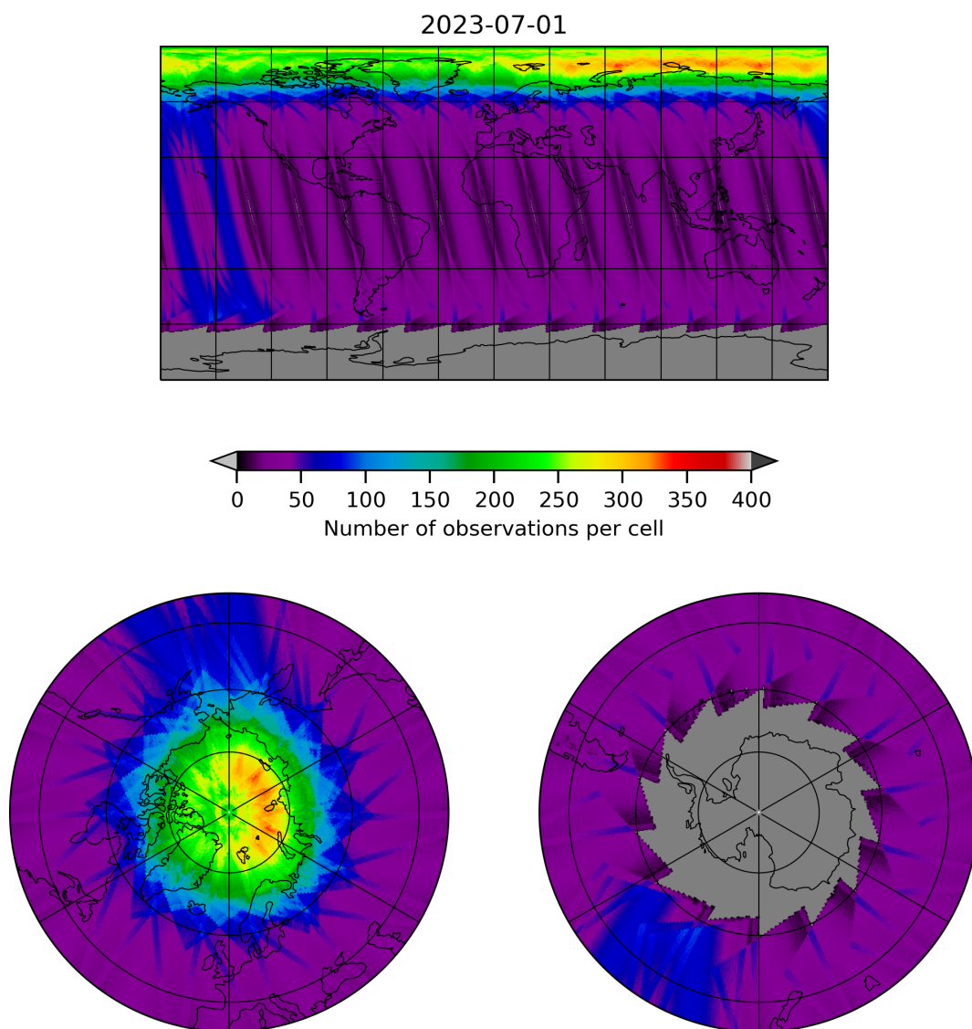
Figure 11: Map of the number of observations for 2023-06-30 to 2023-07-02
