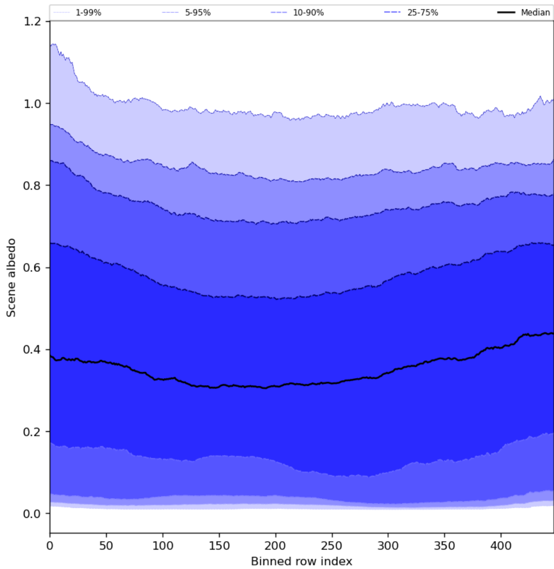
Figure 51: Along track statistics of “Scene albedo” for 2023-06-30 to 2023-07-02
