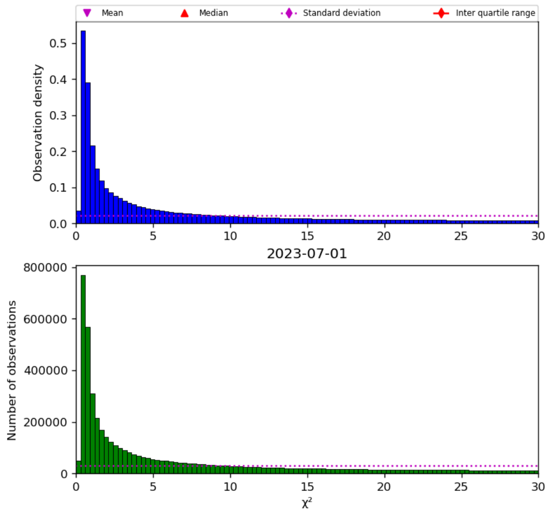
Figure 38: Histogram of “ \chi^2 ” for 2023-06-30 to 2023-07-02
