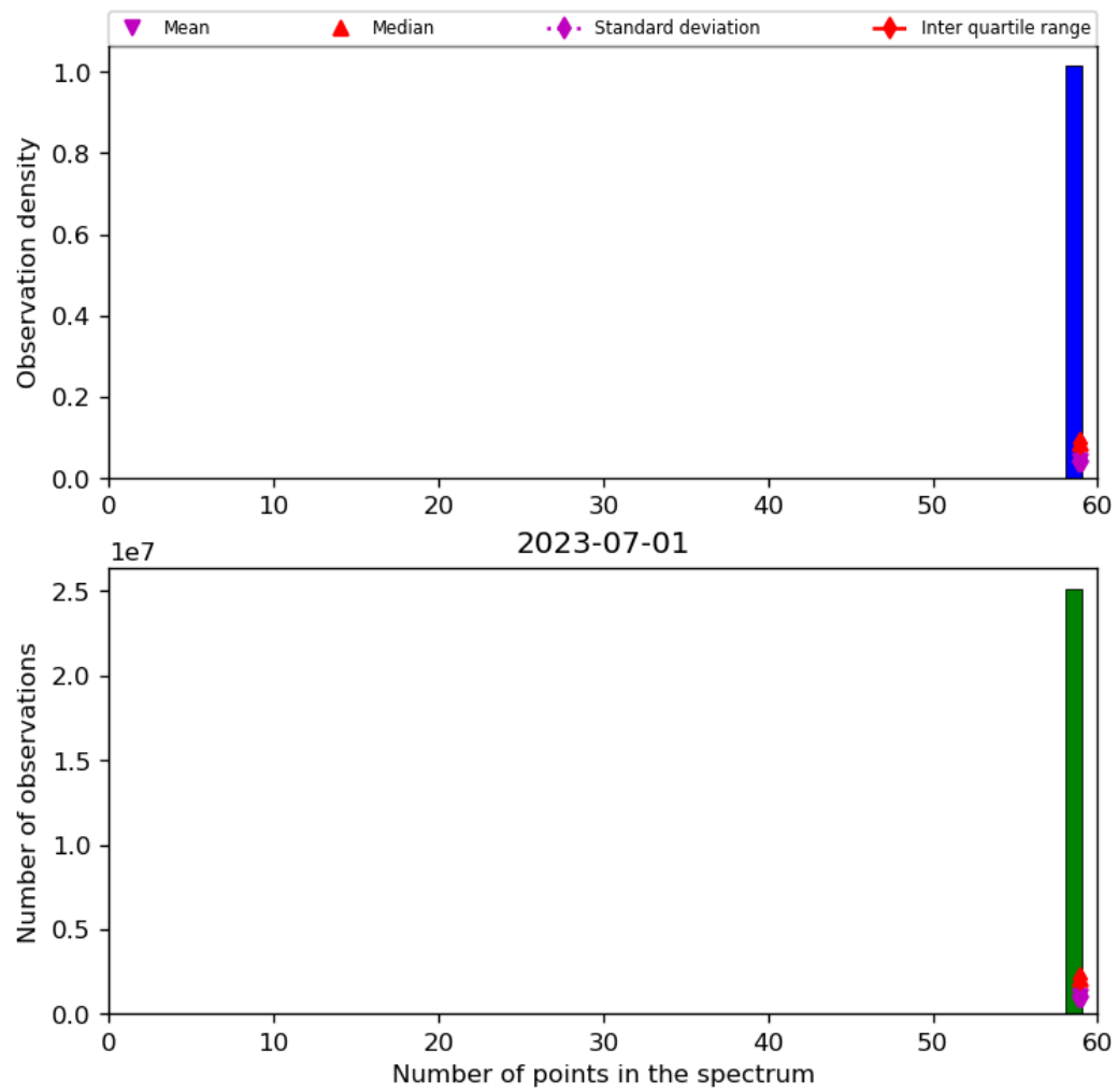
Figure 44: Histogram of “Number of points in the spectrum” for 2023-06-30 to 2023-07-02
