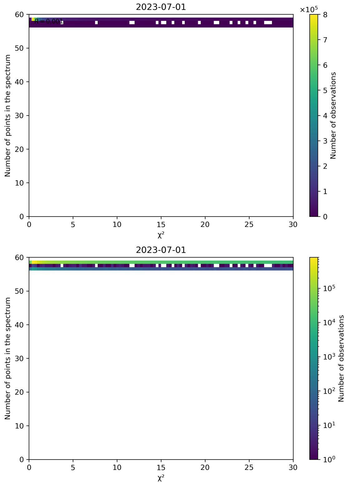
Figure 74: Scatter density plot of “ \chi^2 ” against “Number of points in the spectrum” for 2023-06-30 to 2023-07-02.
