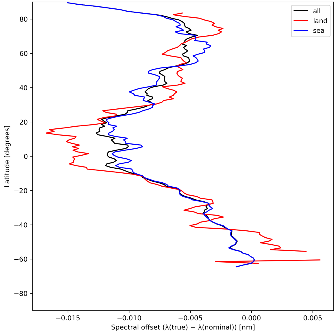
Figure 28: Zonal average of “Spectral offset ( \lambda(\text{true}) - \lambda(\text{nominal}) )” for 2023-06-30 to 2023-07-02.
