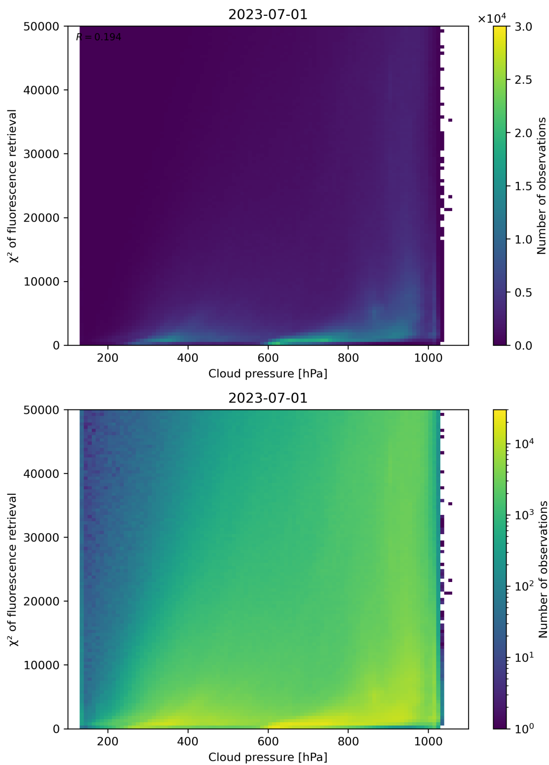
Figure 86: Scatter density plot of “Cloud pressure” against “ \chi^2 of fluorescence retrieval” for 2023-06-30 to 2023-07-02.
