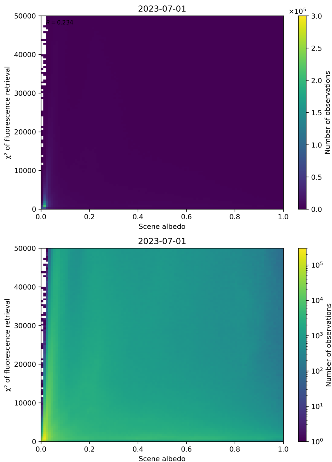
Figure 113: Scatter density plot of “Scene albedo” against “ \chi^2 of fluorescence retrieval” for 2023-06-30 to 2023-07-02.
