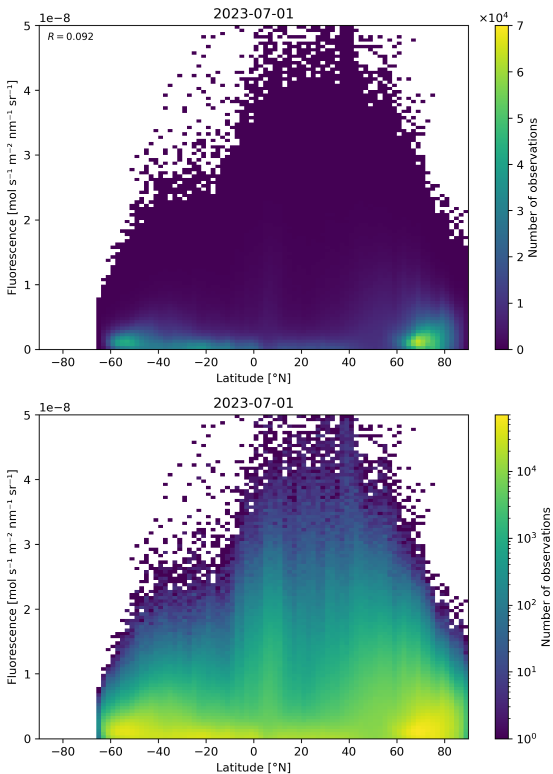
Figure 101: Scatter density plot of “Latitude” against “Fluorescence” for 2023-06-30 to 2023-07-02.
