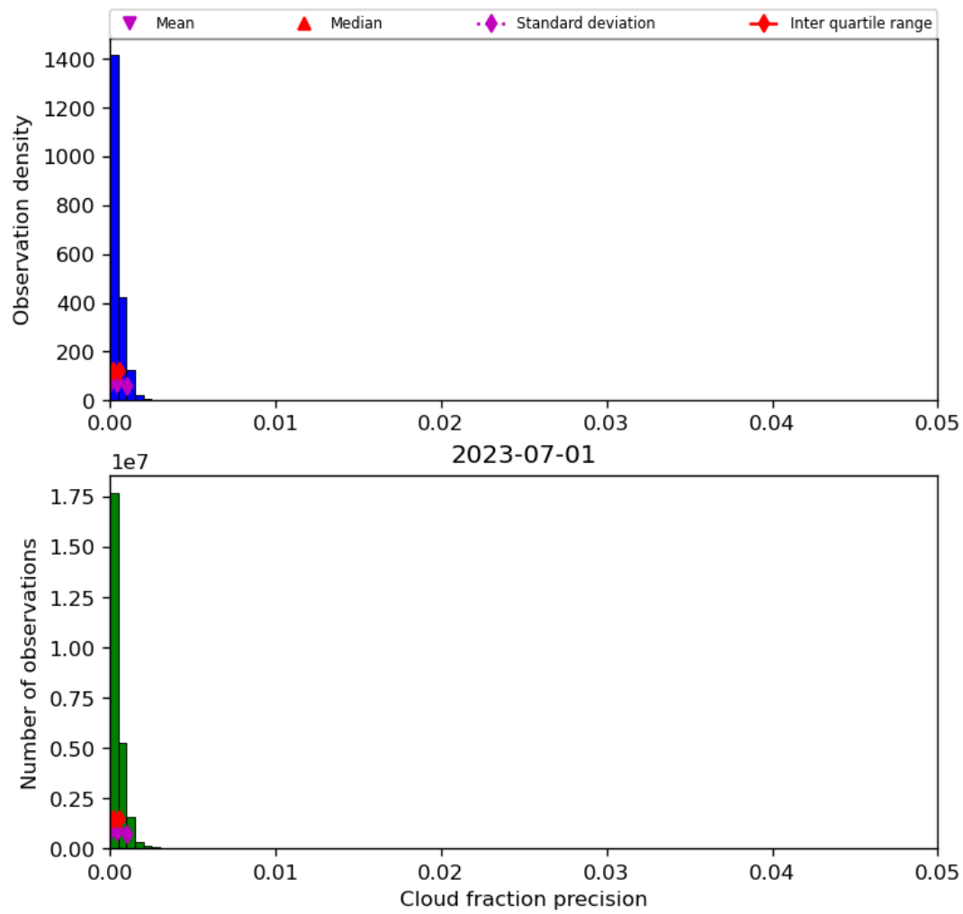
Figure 33: Histogram of “Cloud fraction precision” for 2023-06-30 to 2023-07-02
