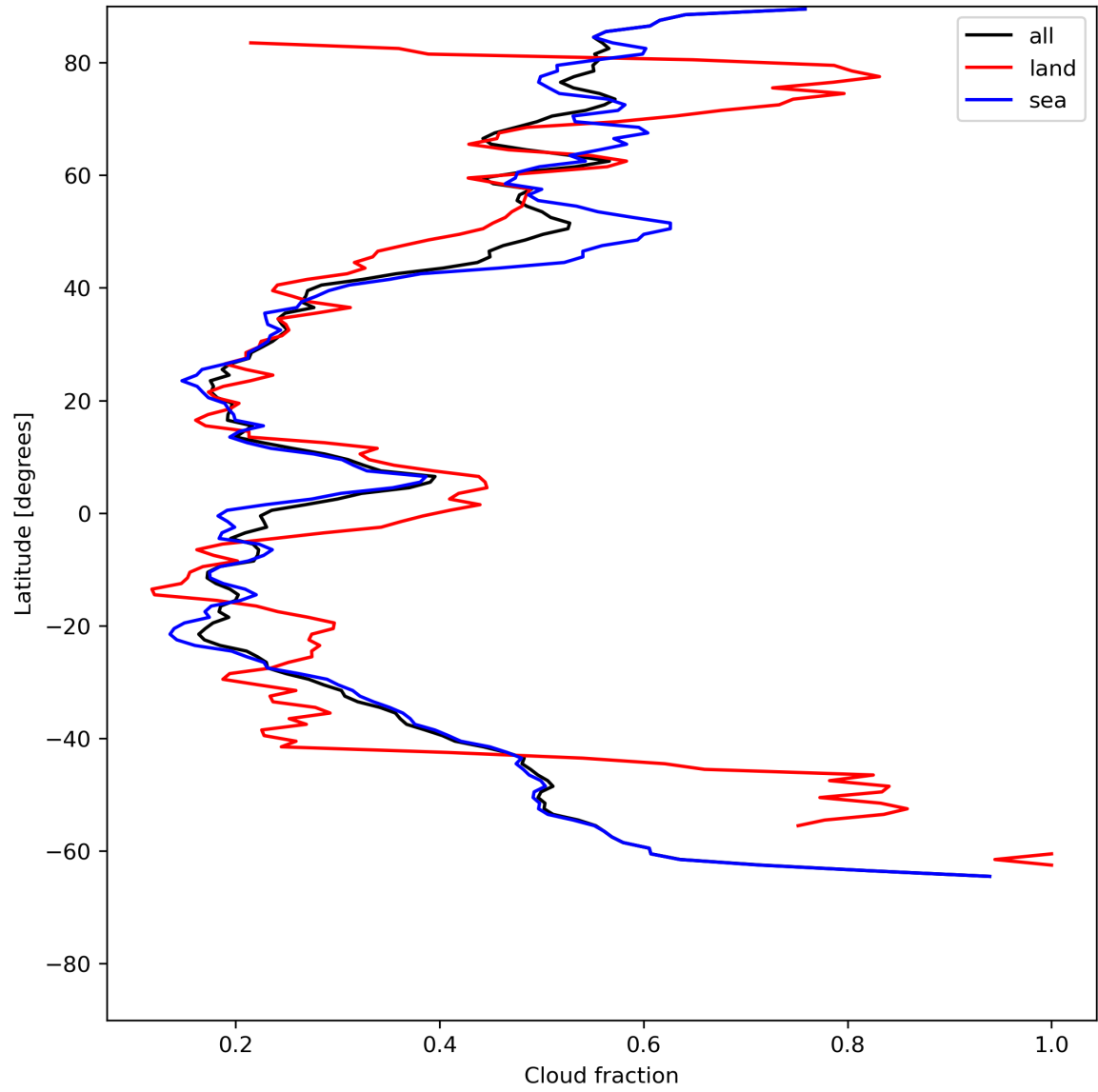
Figure 15: Zonal average of “Cloud fraction” for 2023-06-30 to 2023-07-02.
