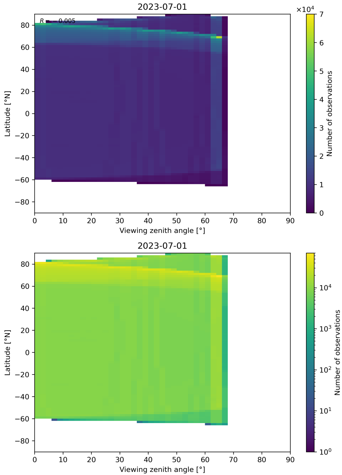
Figure 135: Scatter density plot of “Viewing zenith angle” against “Latitude” for 2023-06-30 to 2023-07-02.
