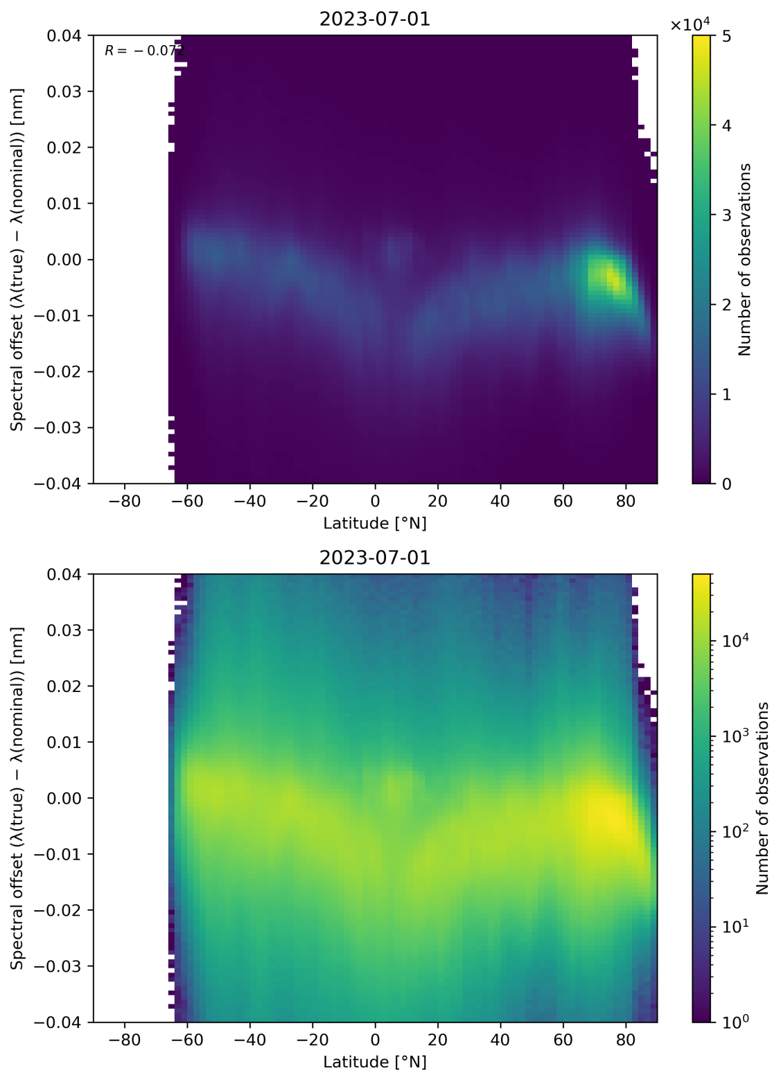
Figure 105: Scatter density plot of “Latitude” against “Spectral offset ( \lambda(\text{true}) - \lambda(\text{nominal}) )” for 2023-06-30 to 2023-07-02.
