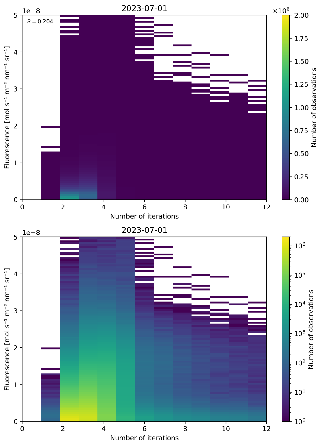
Figure 107: Scatter density plot of “Number of iterations” against “Fluorescence” for 2023-06-30 to 2023-07-02.
