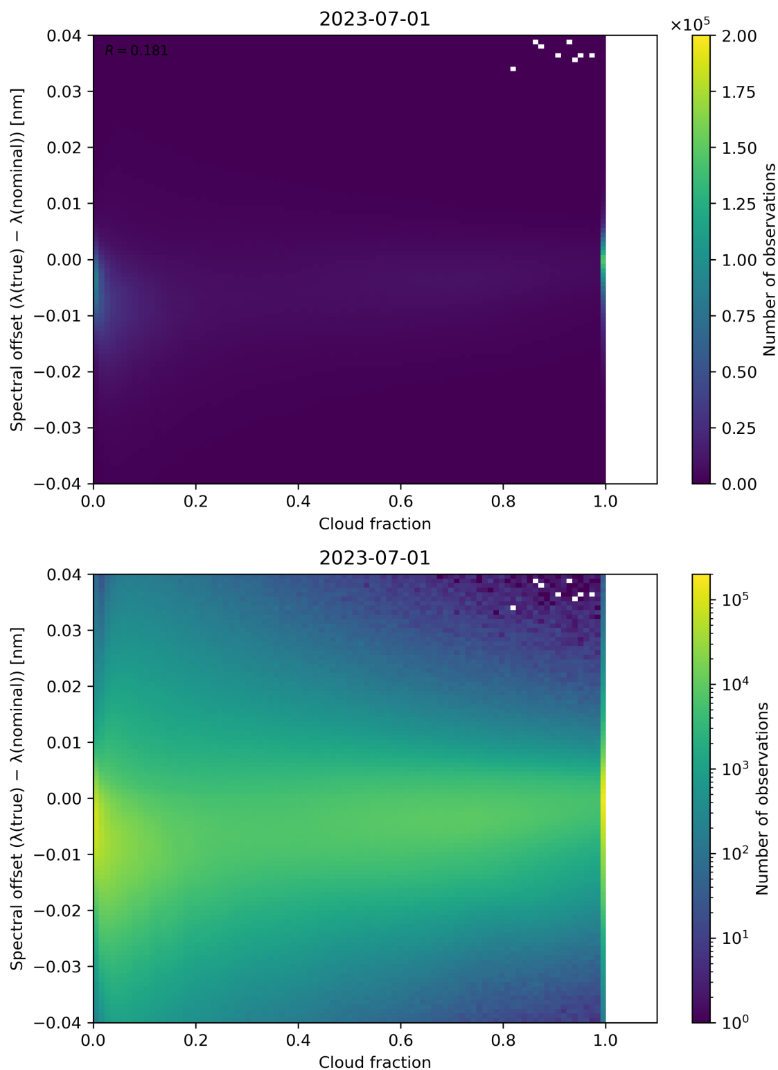
Figure 83: Scatter density plot of “Cloud fraction” against “Spectral offset ( \lambda(\text{true}) - \lambda(\text{nominal}) )” for 2023-06-30 to 2023-07-02.
