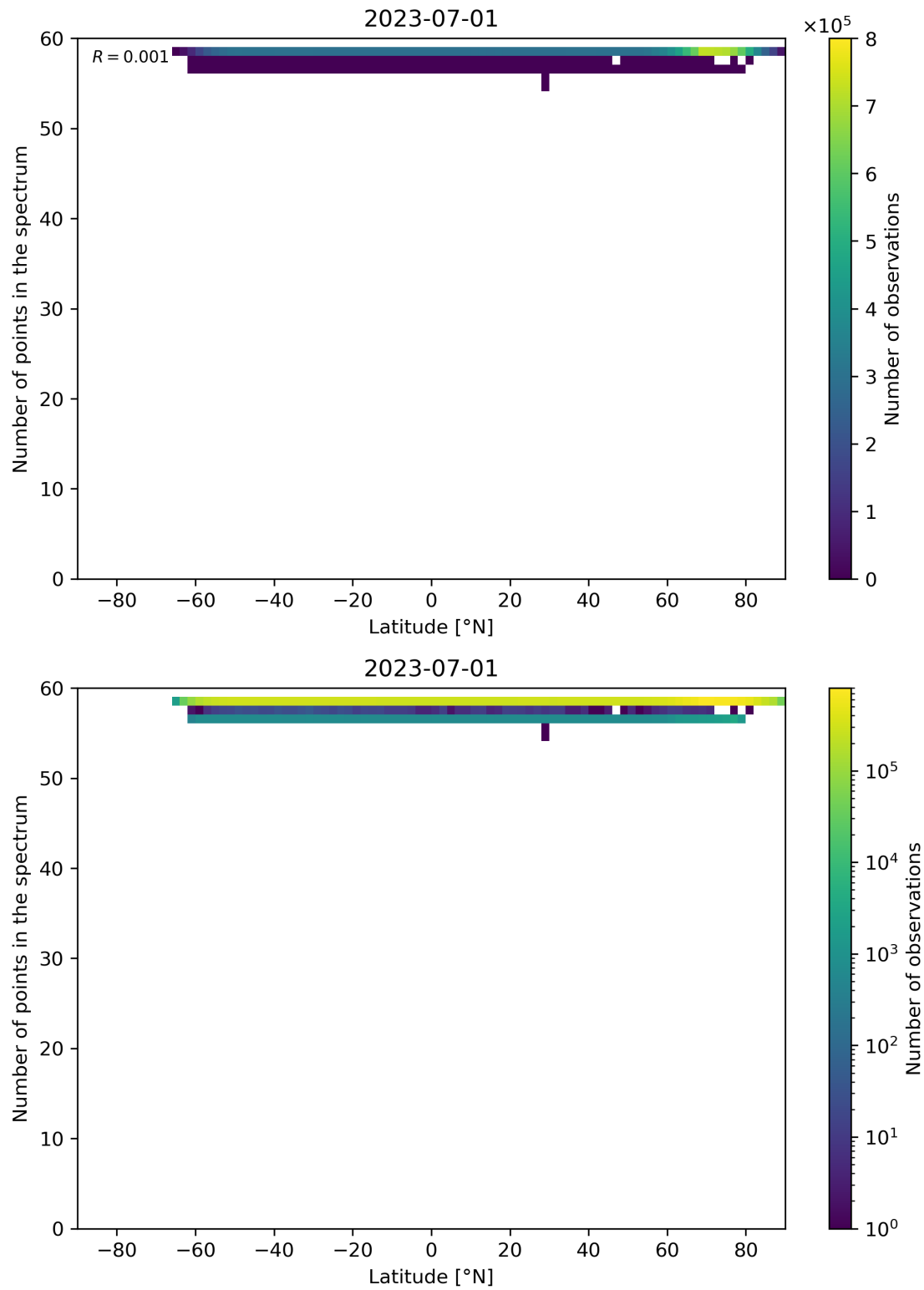
Figure 103: Scatter density plot of “Latitude” against “Number of points in the spectrum” for 2023-06-30 to 2023-07-02.
