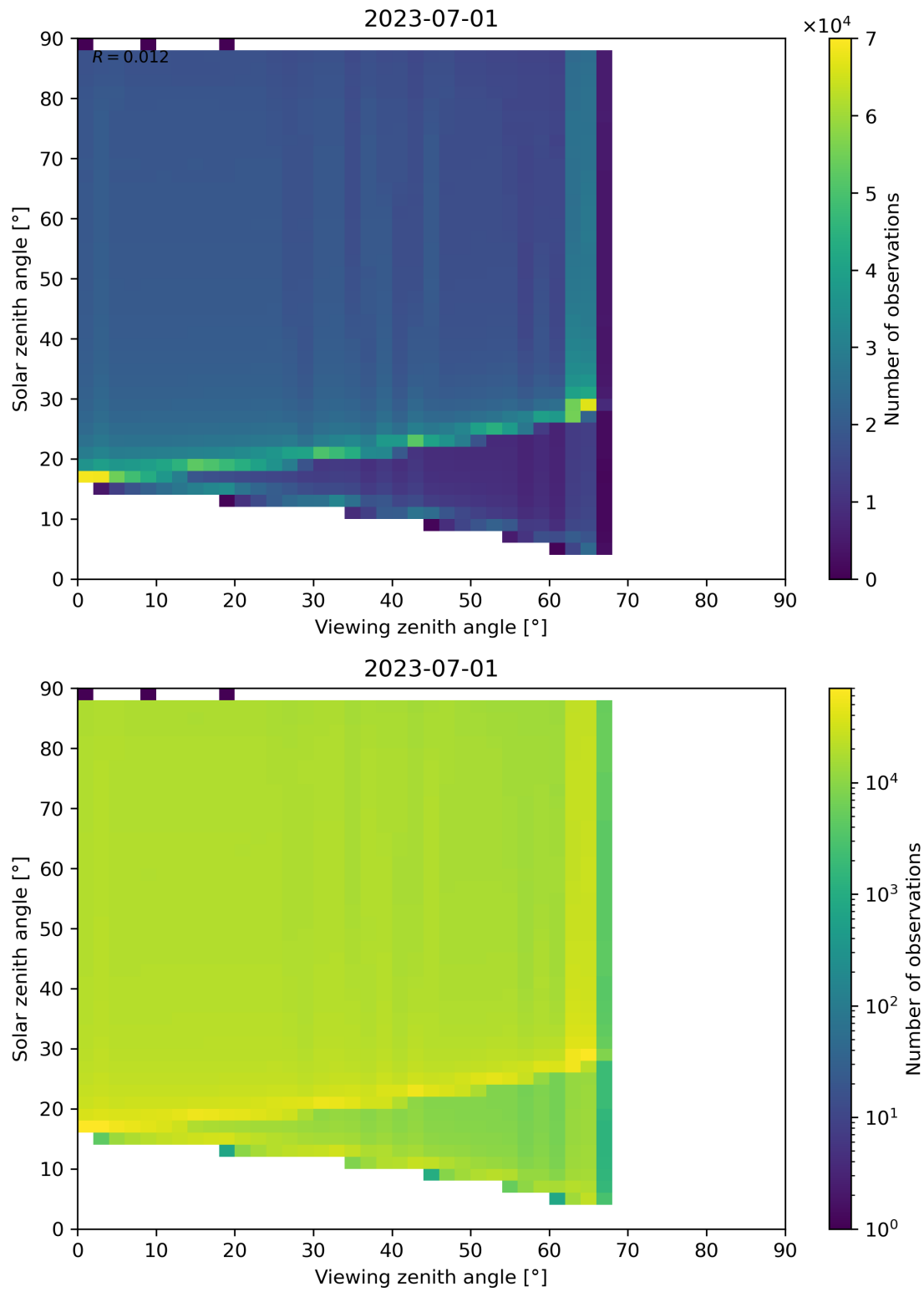
Figure 139: Scatter density plot of “Viewing zenith angle” against “Solar zenith angle” for 2023-06-30 to 2023-07-02.
