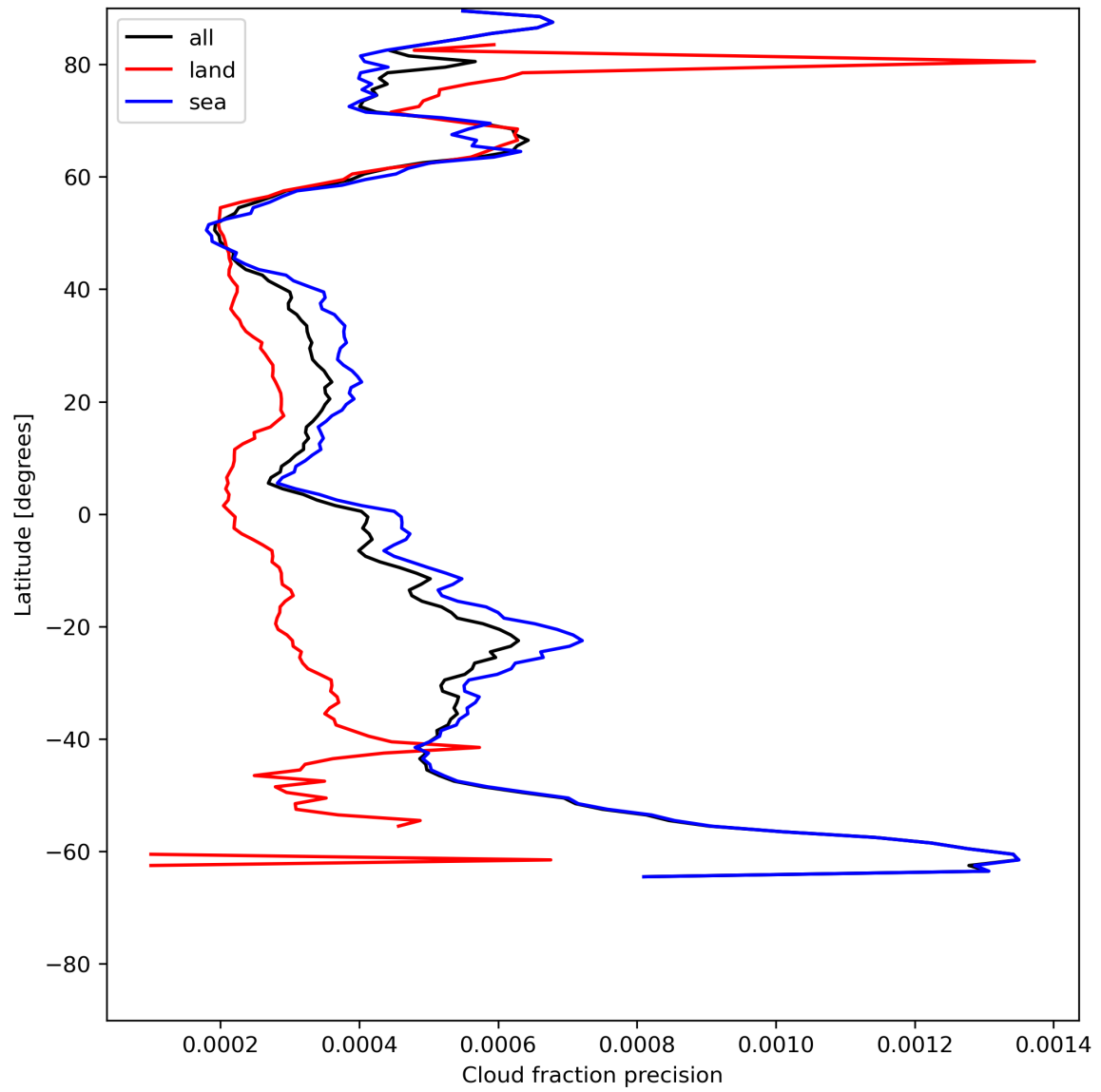
Figure 16: Zonal average of “Cloud fraction precision” for 2023-06-30 to 2023-07-02.
