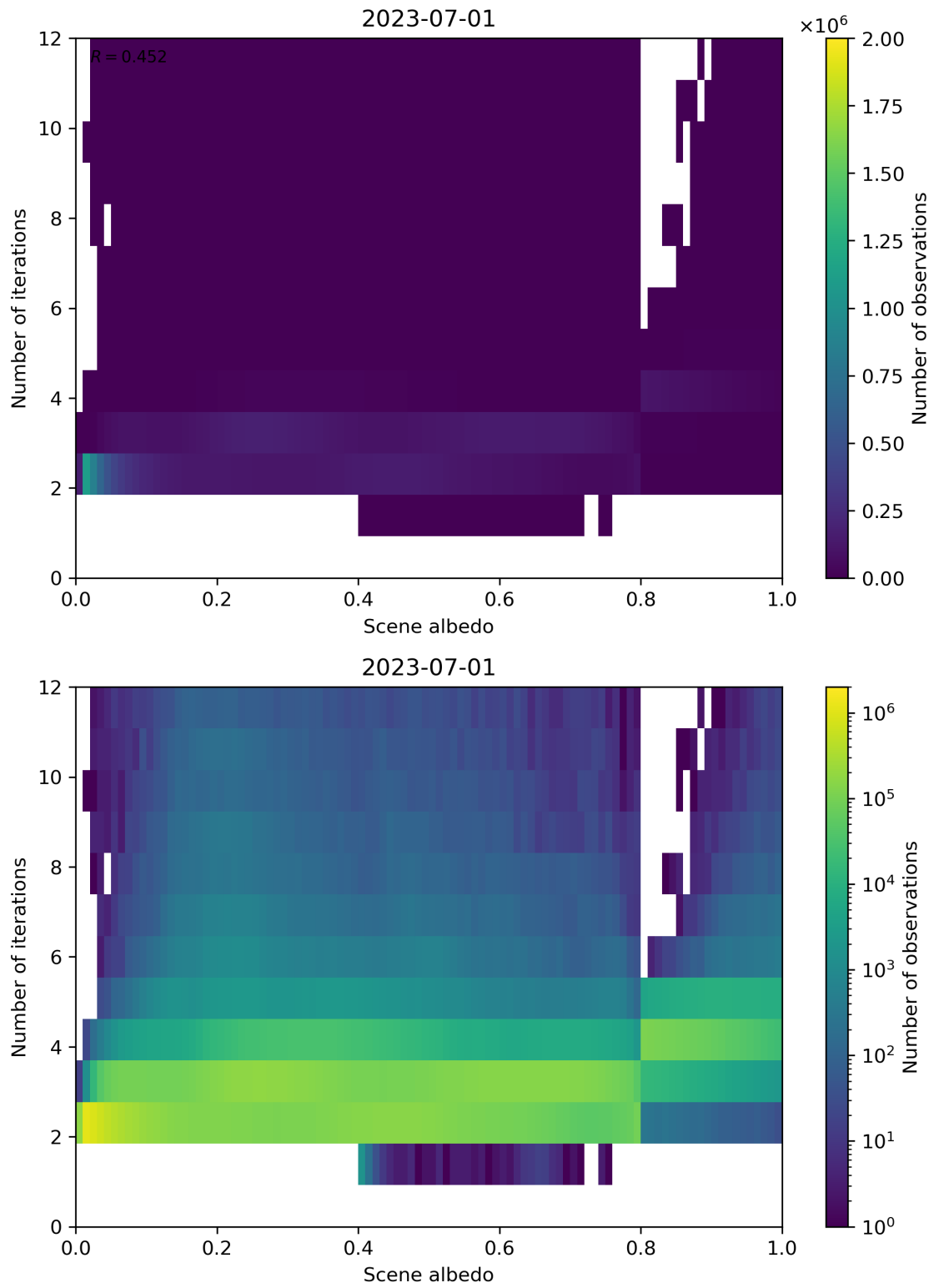
Figure 115: Scatter density plot of “Scene albedo” against “Number of iterations” for 2023-06-30 to 2023-07-02.
