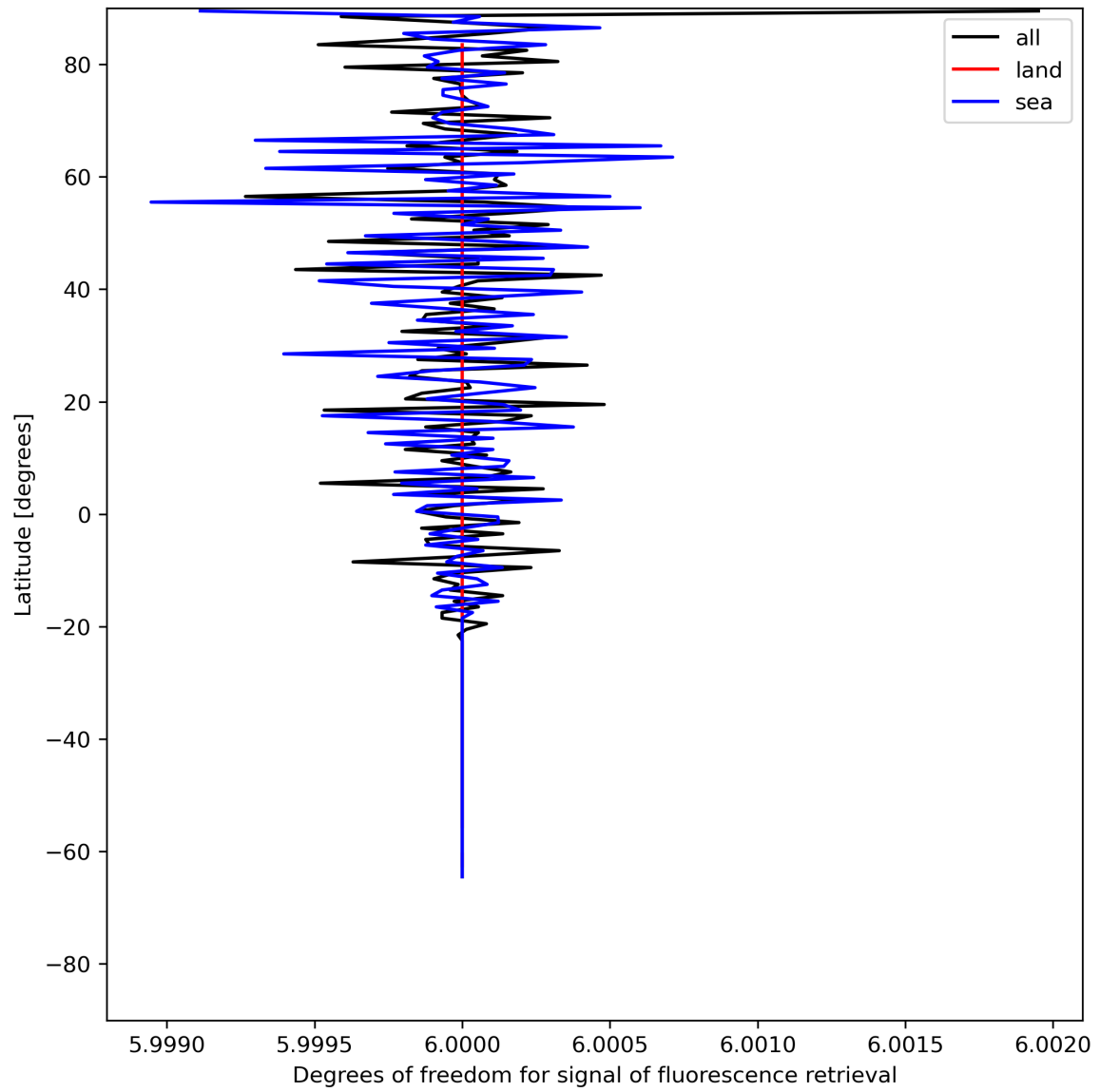
Figure 26: Zonal average of “Degrees of freedom for signal of fluorescence retrieval” for 2023-06-30 to 2023-07-02.
