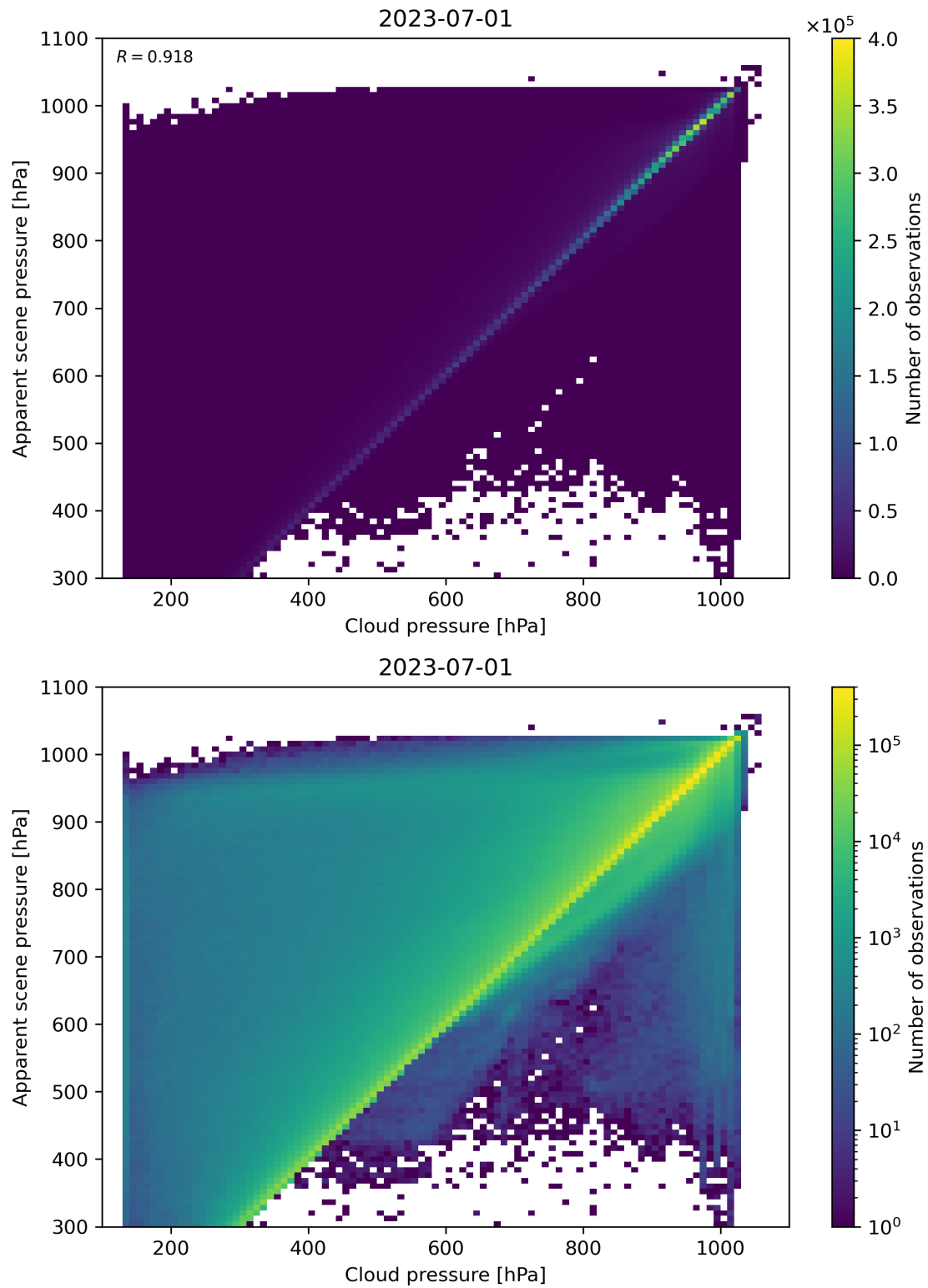
Figure 84: Scatter density plot of “Cloud pressure” against “Apparent scene pressure” for 2023-06-30 to 2023-07-02.
