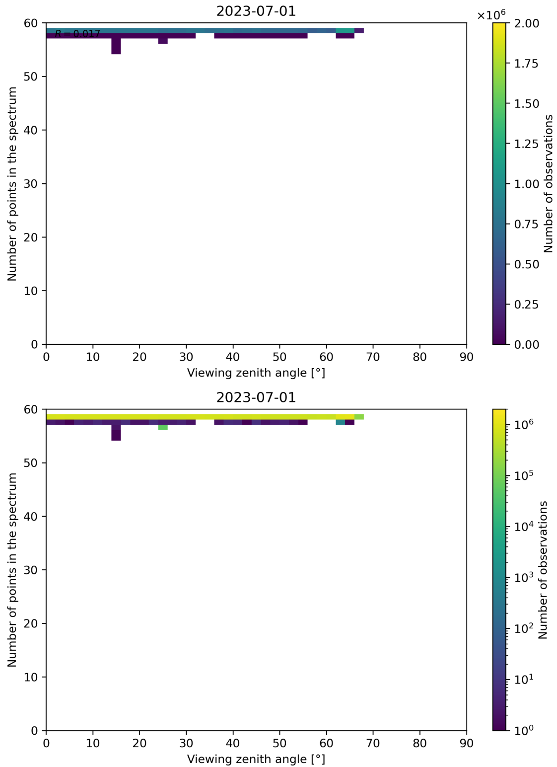
Figure 137: Scatter density plot of “Viewing zenith angle” against “Number of points in the spectrum” for 2023-06-30 to 2023-07-02.
