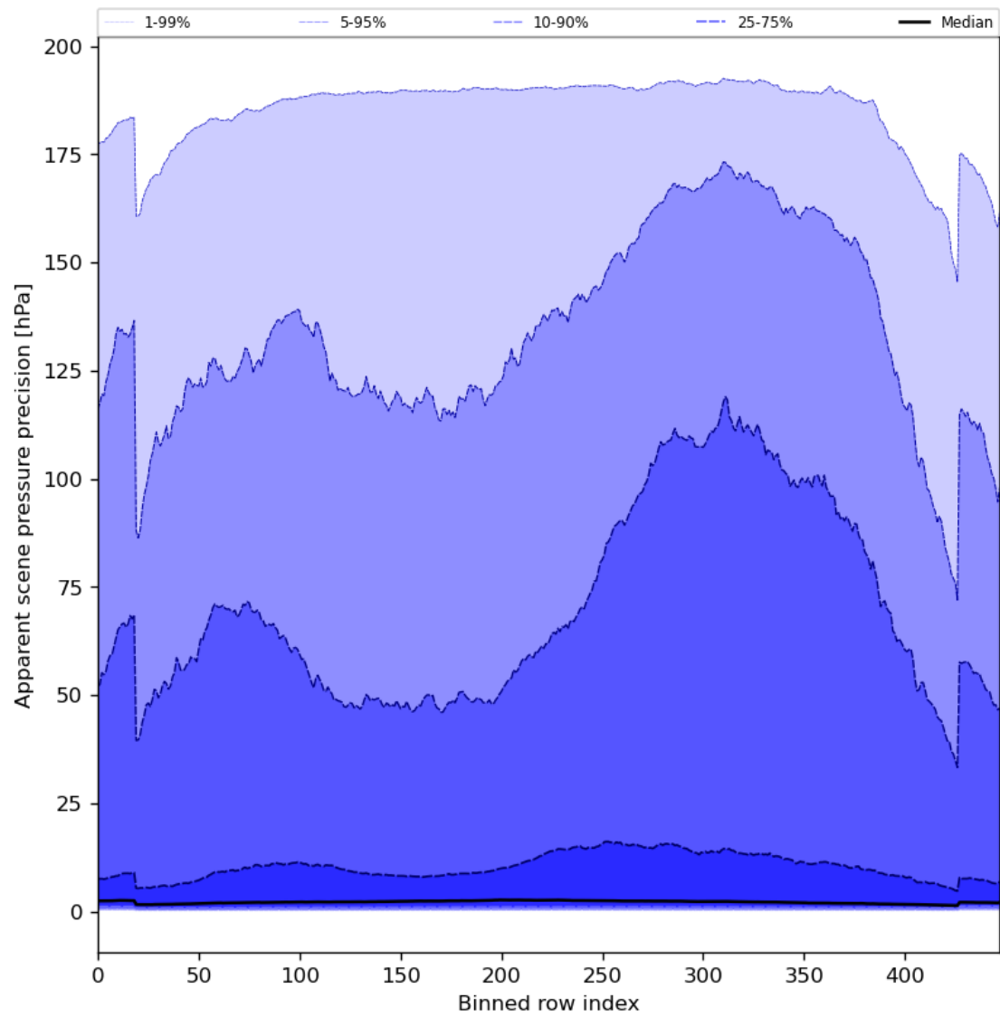
Figure 54: Along track statistics of “Apparent scene pressure precision” for 2023-07-01 to 2023-07-03
