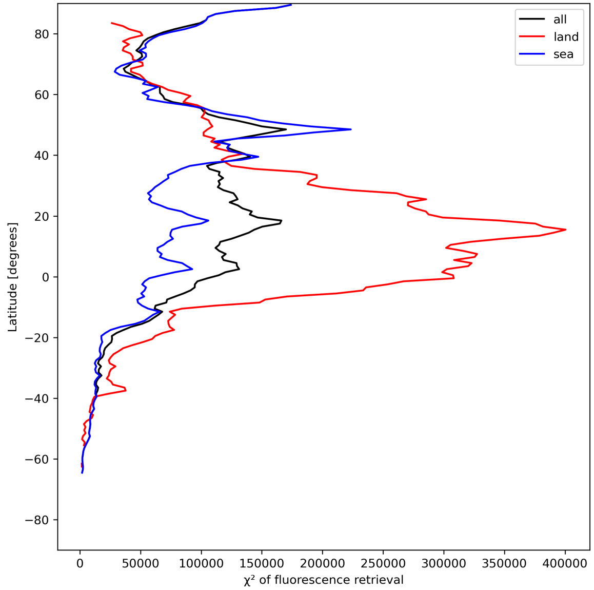
Figure 25: Zonal average of “ \chi^2 of fluorescence retrieval” for 2023-07-01 to 2023-07-03.
