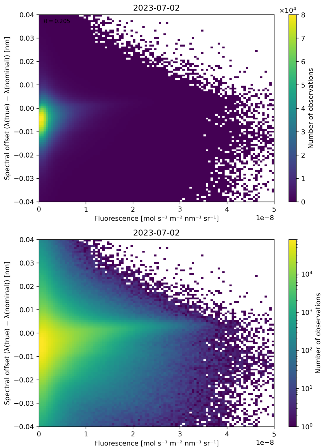
Figure 95: Scatter density plot of “Fluorescence” against “Spectral offset ( \lambda(\text{true}) - \lambda(\text{nominal}) )” for 2023-07-01 to 2023-07-03.
