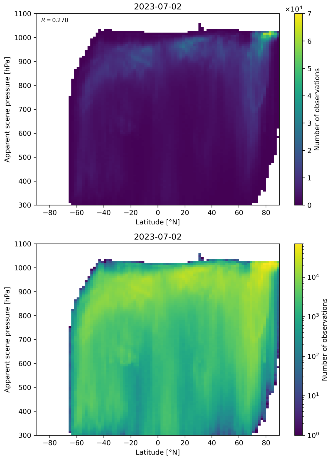
Figure 96: Scatter density plot of “Latitude” against “Apparent scene pressure” for 2023-07-01 to 2023-07-03.
