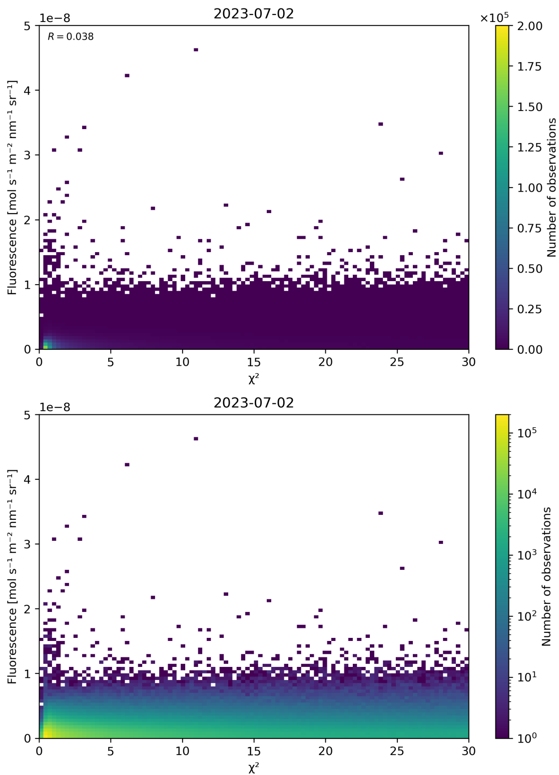
Figure 70: Scatter density plot of “ \chi^2 ” against “Fluorescence” for 2023-07-01 to 2023-07-03.
