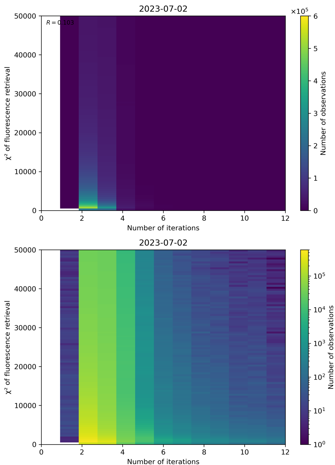
Figure 106: Scatter density plot of “Number of iterations” against “ \chi^2 of fluorescence retrieval” for 2023-07-01 to 2023-07-03.
