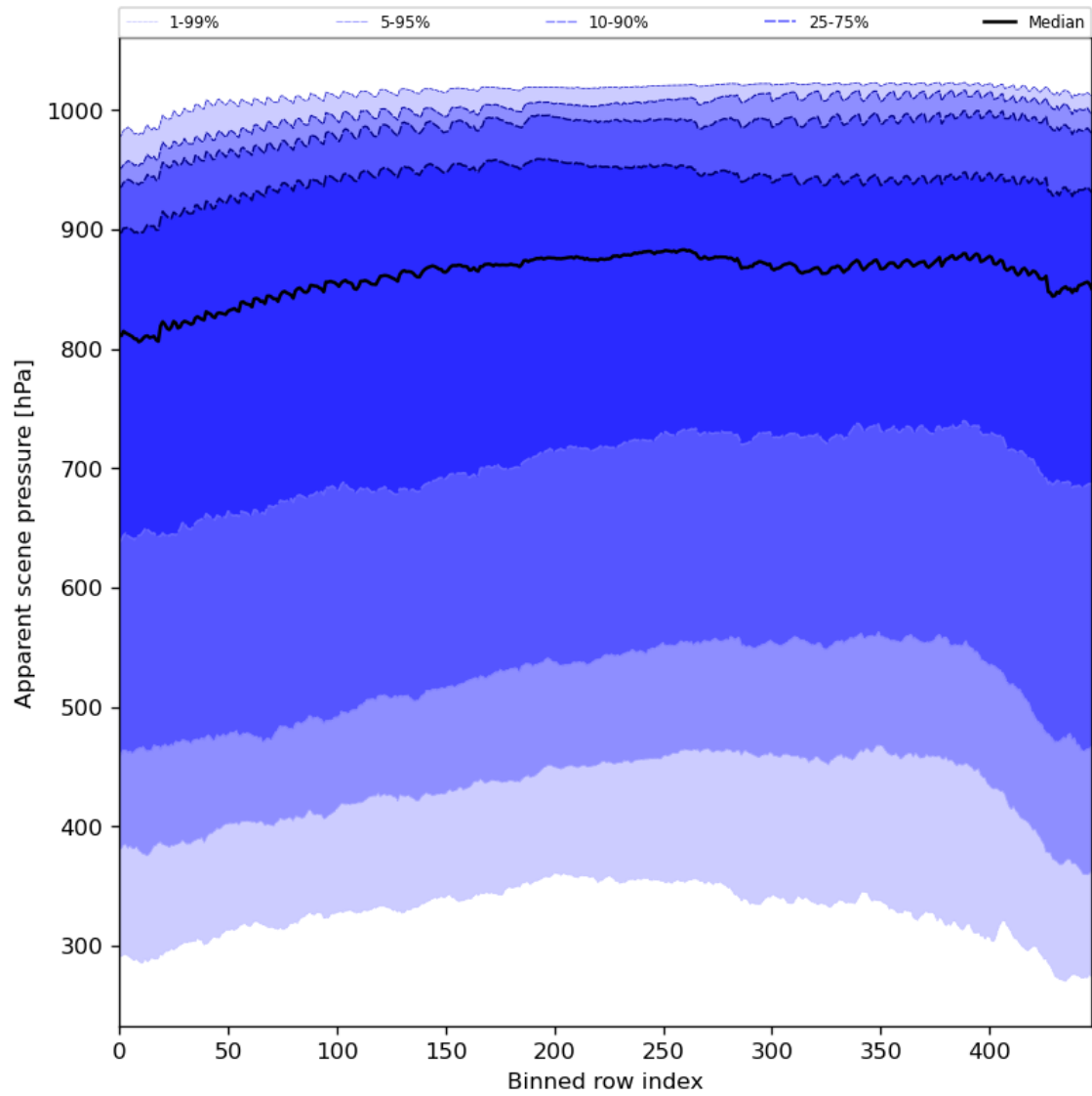
Figure 53: Along track statistics of “Apparent scene pressure” for 2023-07-01 to 2023-07-03
