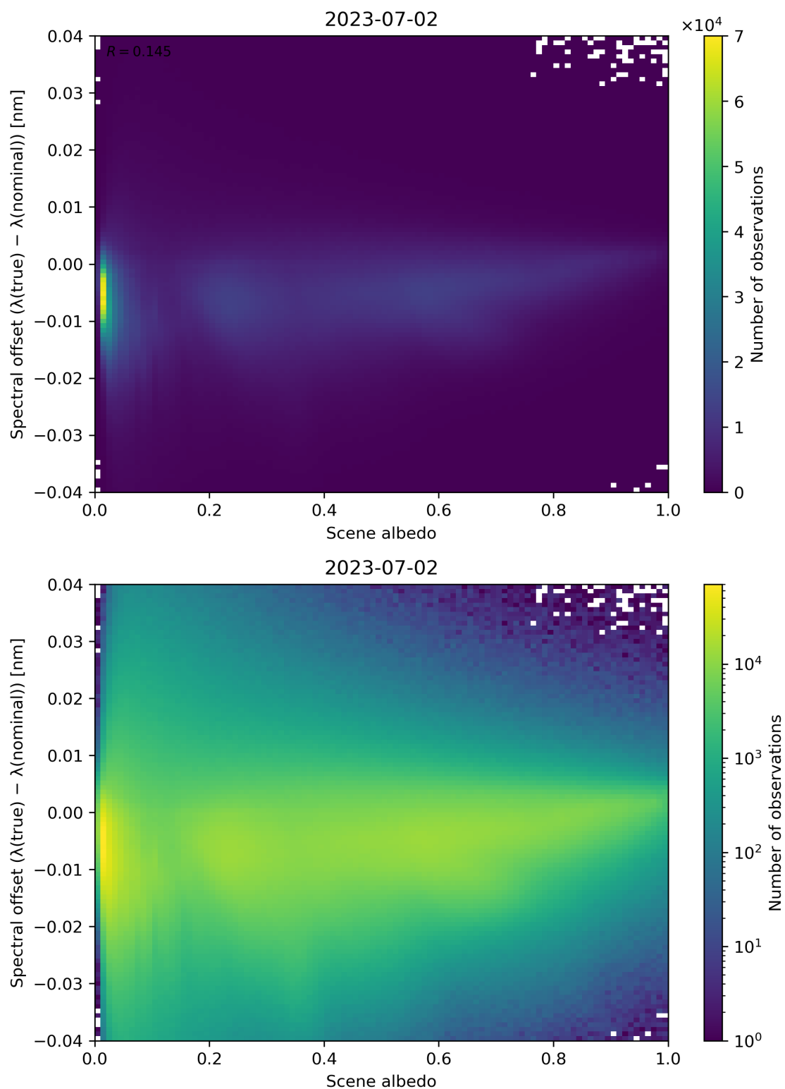
Figure 117: Scatter density plot of “Scene albedo” against “Spectral offset ( \lambda(\text{true}) - \lambda(\text{nominal}) )” for 2023-07-01 to 2023-07-03.
