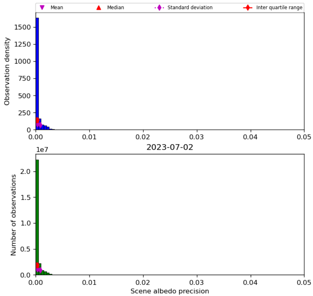
Figure 35: Histogram of “Scene albedo precision” for 2023-07-01 to 2023-07-03
