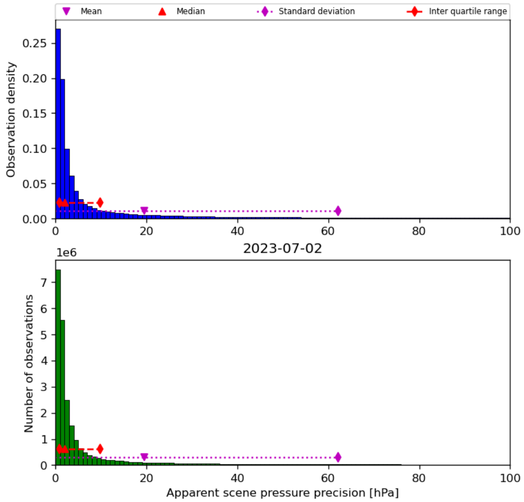
Figure 37: Histogram of “Apparent scene pressure precision” for 2023-07-01 to 2023-07-03
