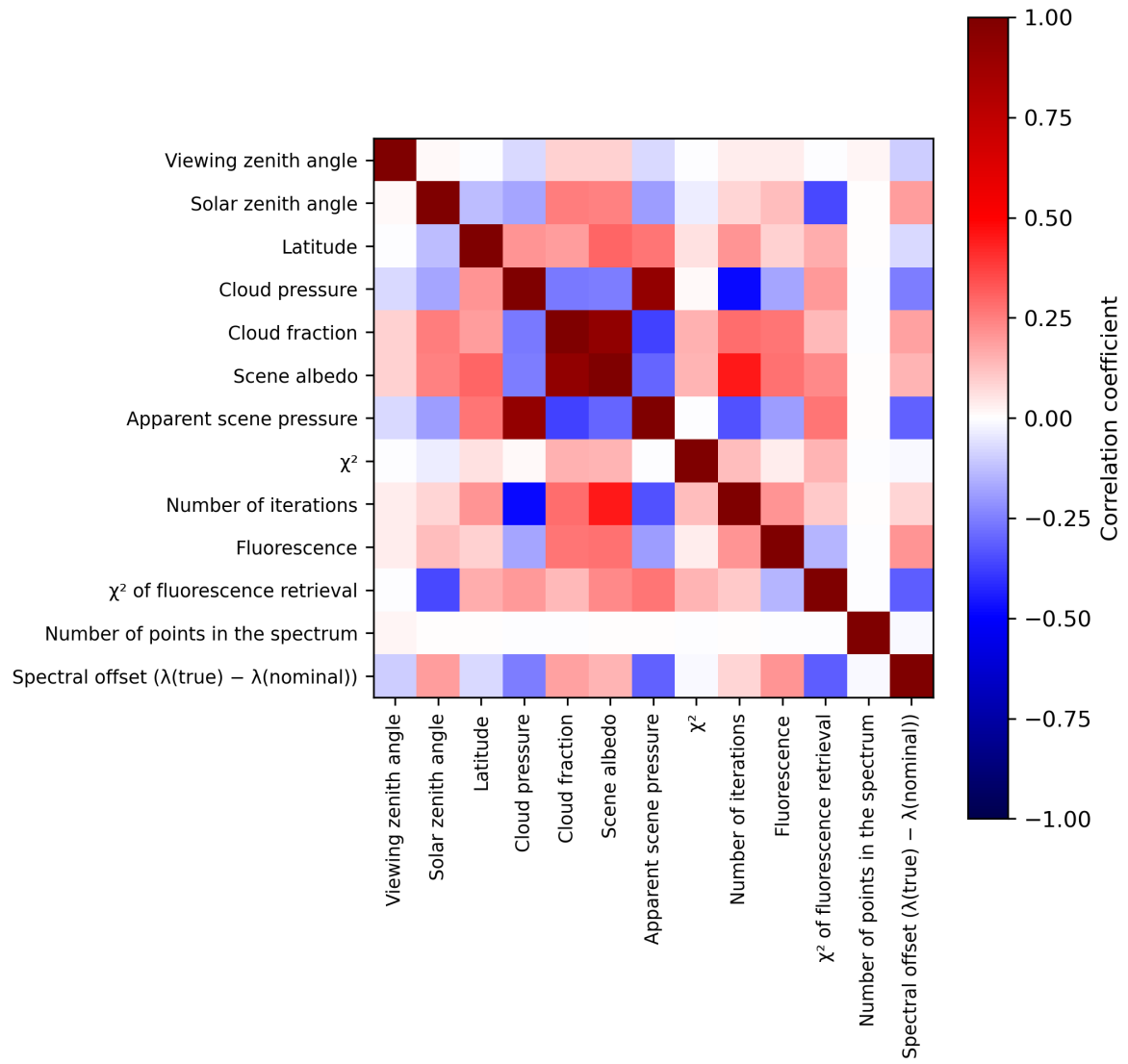
Figure 2: Map of correlation matrix for 2023-07-01 to 2023-07-03.
