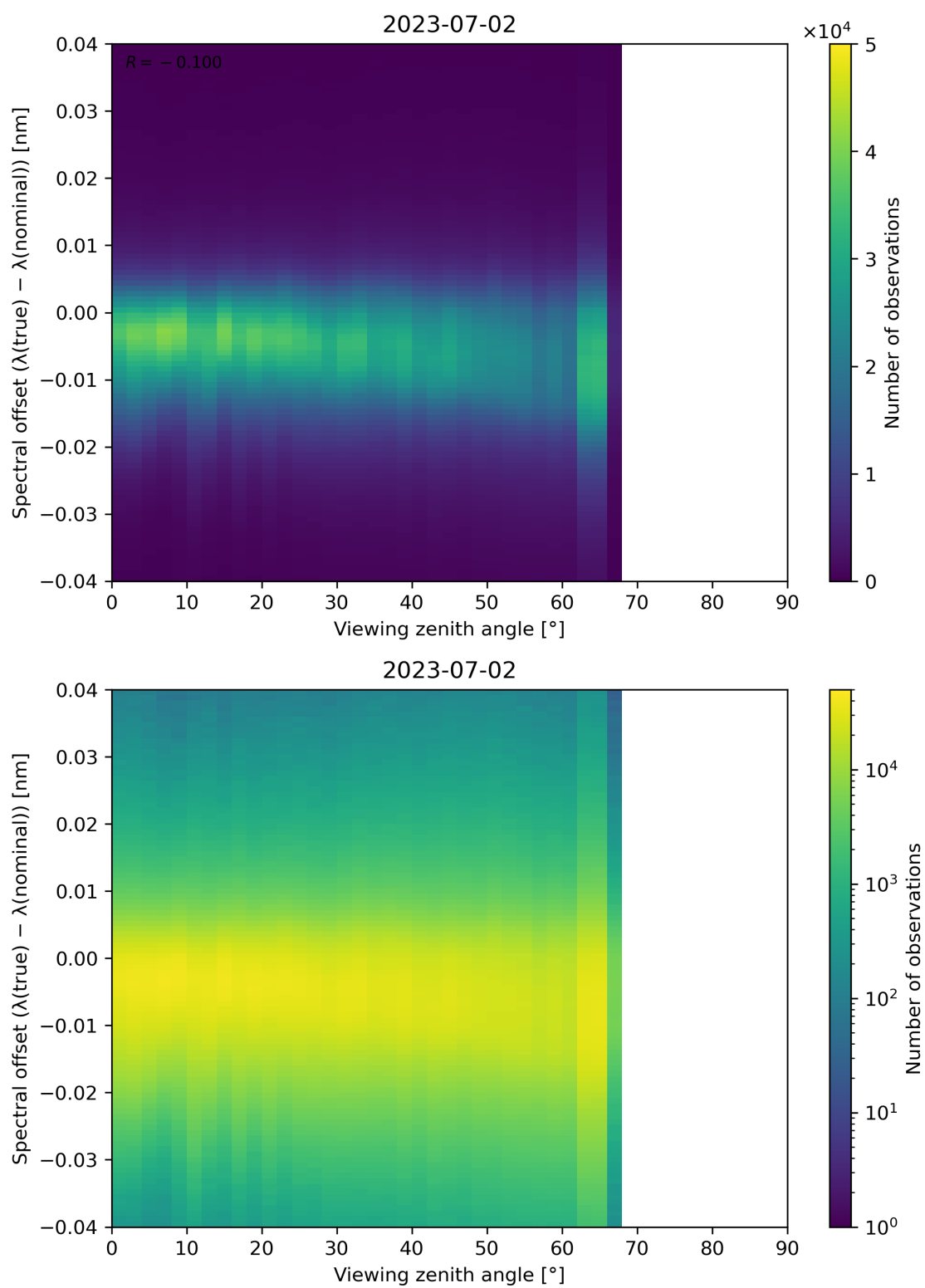
Figure 140: Scatter density plot of “Viewing zenith angle” against “Spectral offset ( \lambda(\text{true}) - \lambda(\text{nominal}) )” for 2023-07-01 to 2023-07-03.
