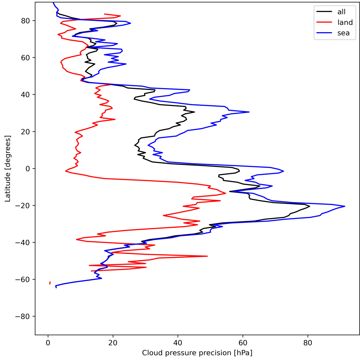
Figure 14: Zonal average of “Cloud pressure precision” for 2023-07-01 to 2023-07-03.
