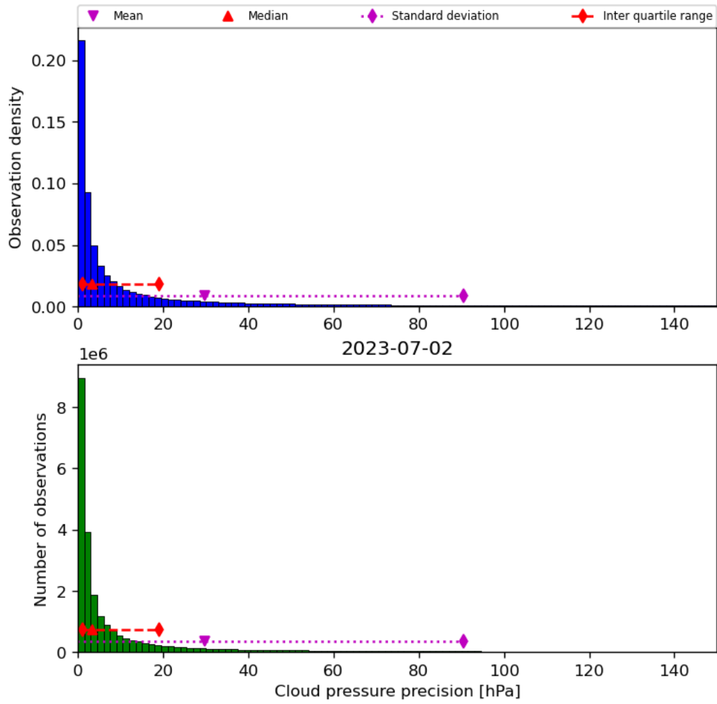
Figure 31: Histogram of “Cloud pressure precision” for 2023-07-01 to 2023-07-03
