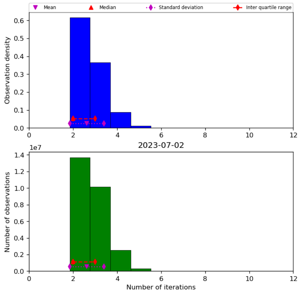
Figure 39: Histogram of “Number of iterations” for 2023-07-01 to 2023-07-03
