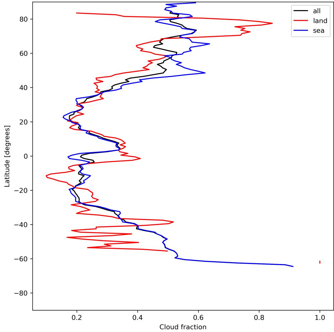
Figure 15: Zonal average of “Cloud fraction” for 2023-07-01 to 2023-07-03.
