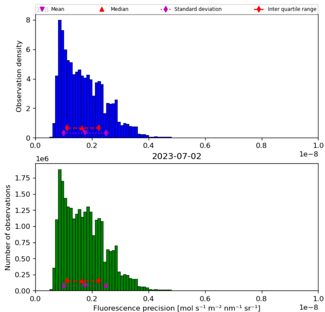
Figure 41: Histogram of “Fluorescence precision” for 2023-07-01 to 2023-07-03
