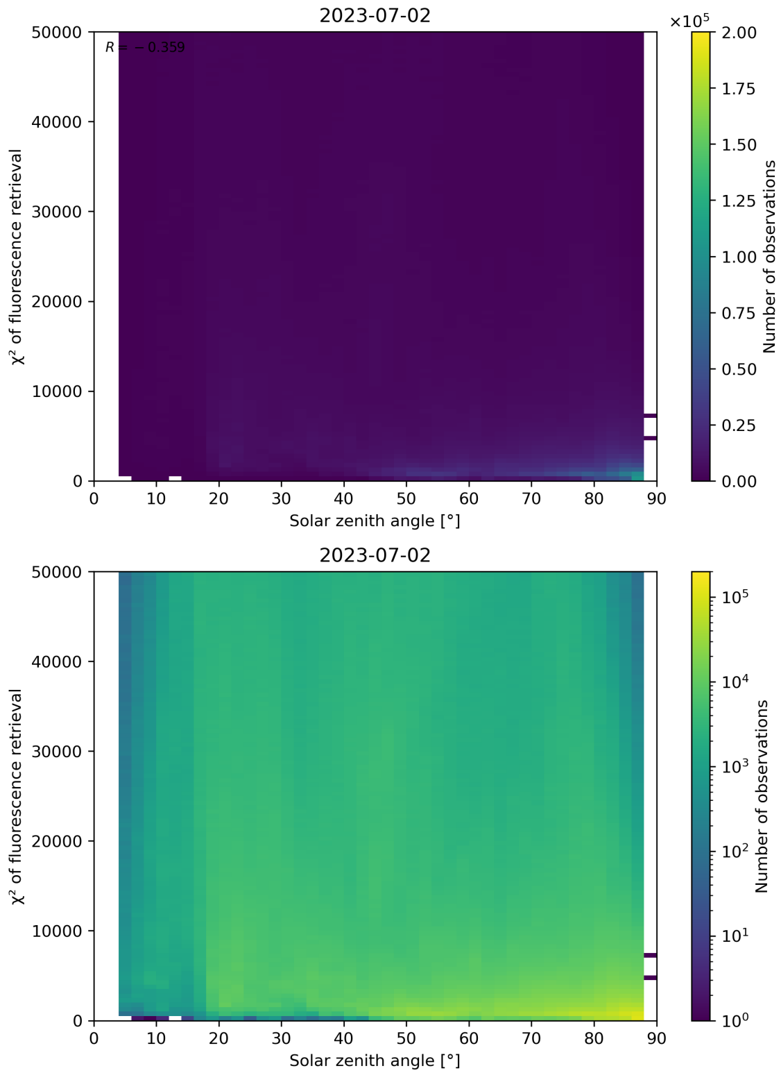
Figure 120: Scatter density plot of “Solar zenith angle” against “ \chi^2 of fluorescence retrieval” for 2023-07-01 to 2023-07-03.
