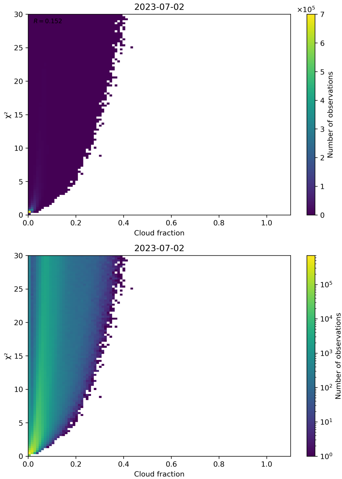
Figure 77: Scatter density plot of “Cloud fraction” against “ \chi^2 ” for 2023-07-01 to 2023-07-03.
