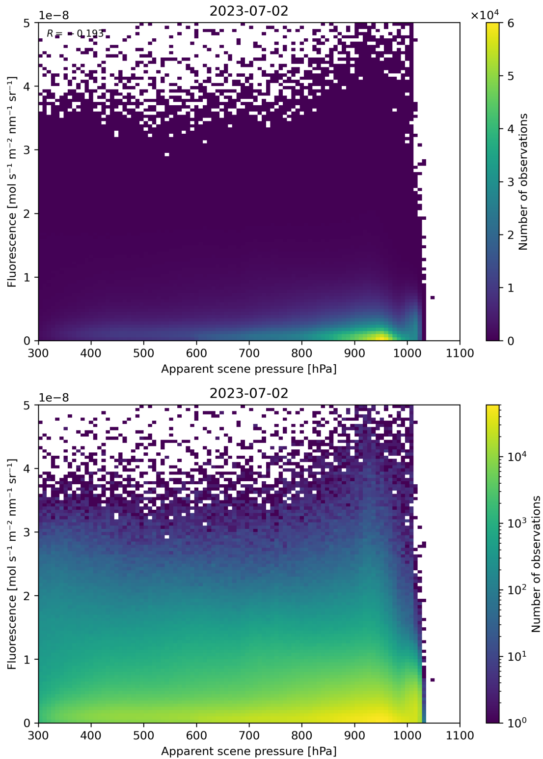
Figure 65: Scatter density plot of “Apparent scene pressure” against “Fluorescence” for 2023-07-01 to 2023-07-03.
