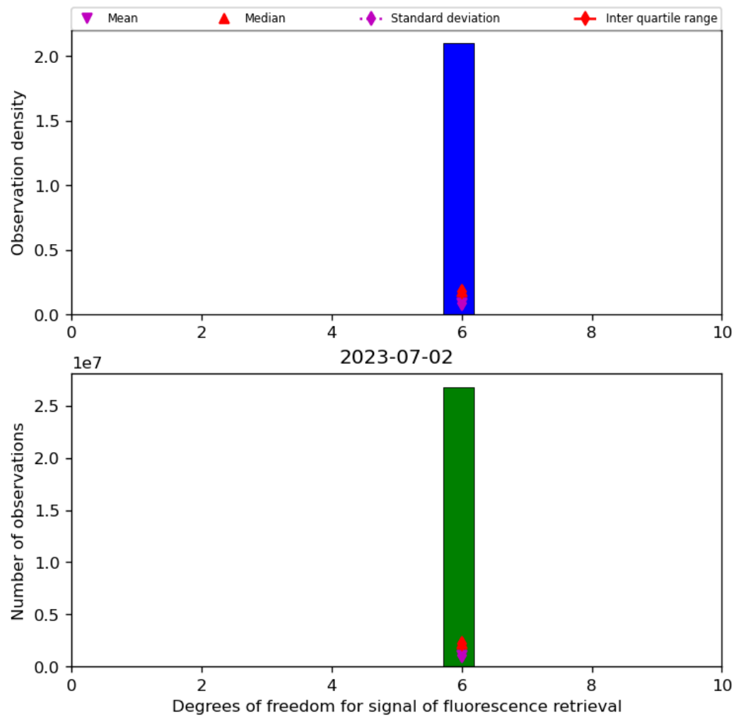
Figure 43: Histogram of “Degrees of freedom for signal of fluorescence retrieval” for 2023-07-01 to 2023-07-03
