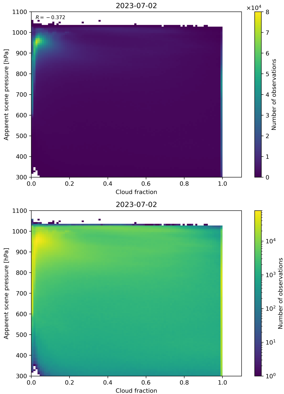
Figure 76: Scatter density plot of “Cloud fraction” against “Apparent scene pressure” for 2023-07-01 to 2023-07-03.
