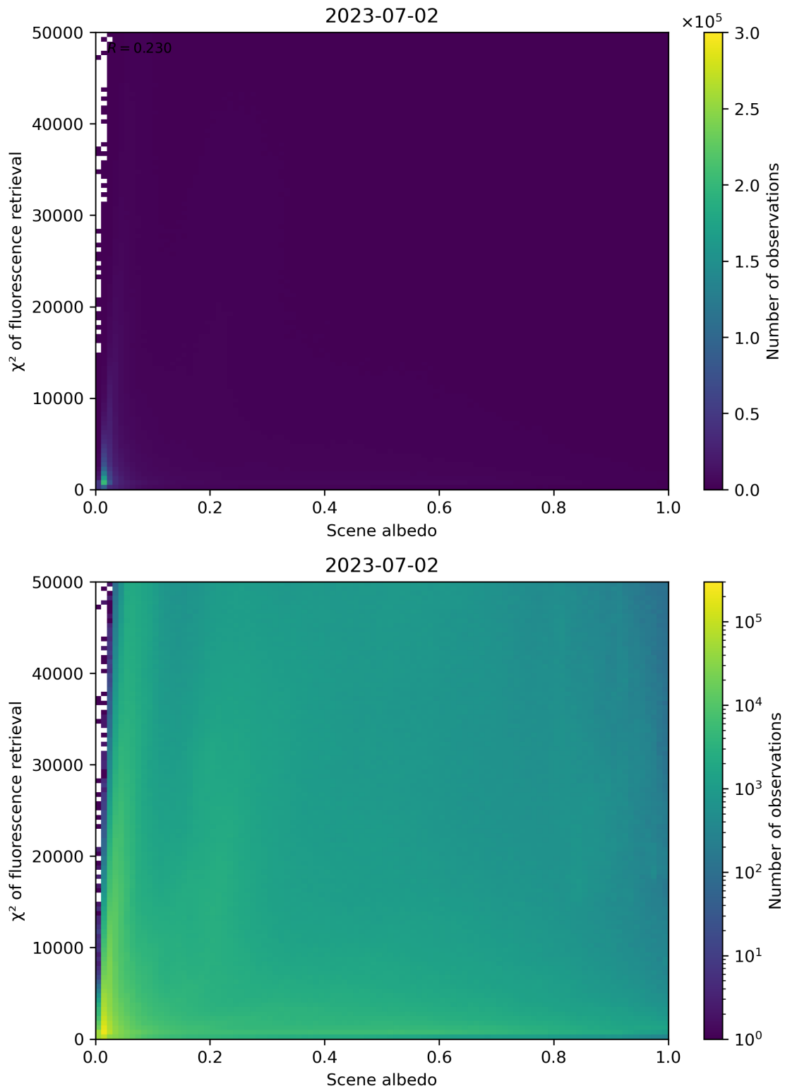
Figure 113: Scatter density plot of “Scene albedo” against “ \chi^2 of fluorescence retrieval” for 2023-07-01 to 2023-07-03.
