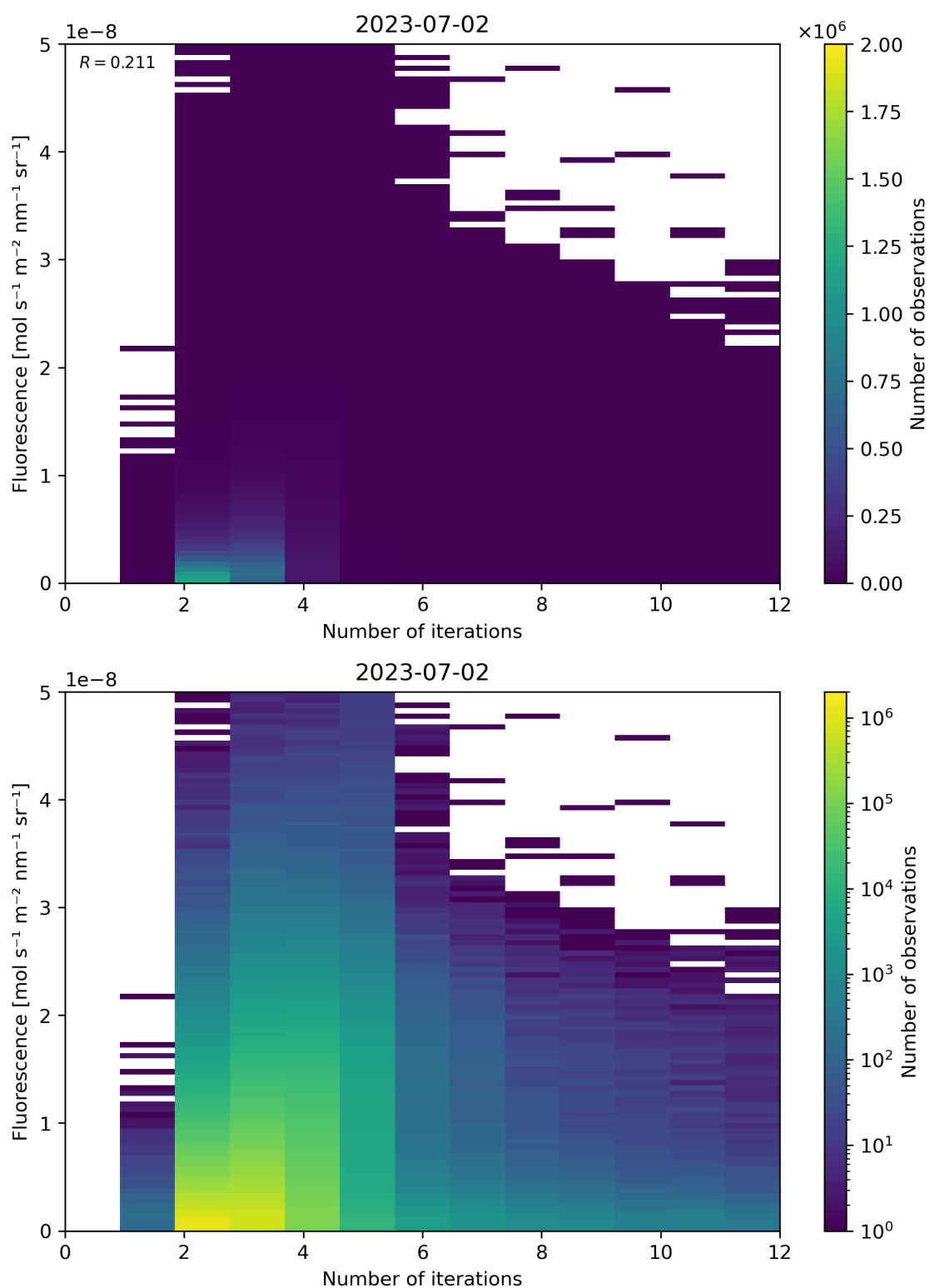
Figure 107: Scatter density plot of “Number of iterations” against “Fluorescence” for 2023-07-01 to 2023-07-03.
