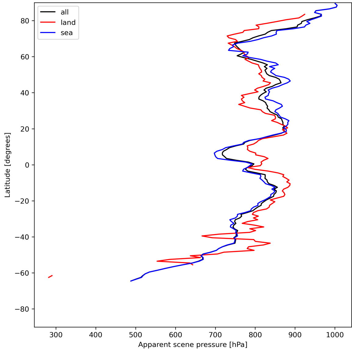
Figure 19: Zonal average of “Apparent scene pressure” for 2023-07-01 to 2023-07-03.
