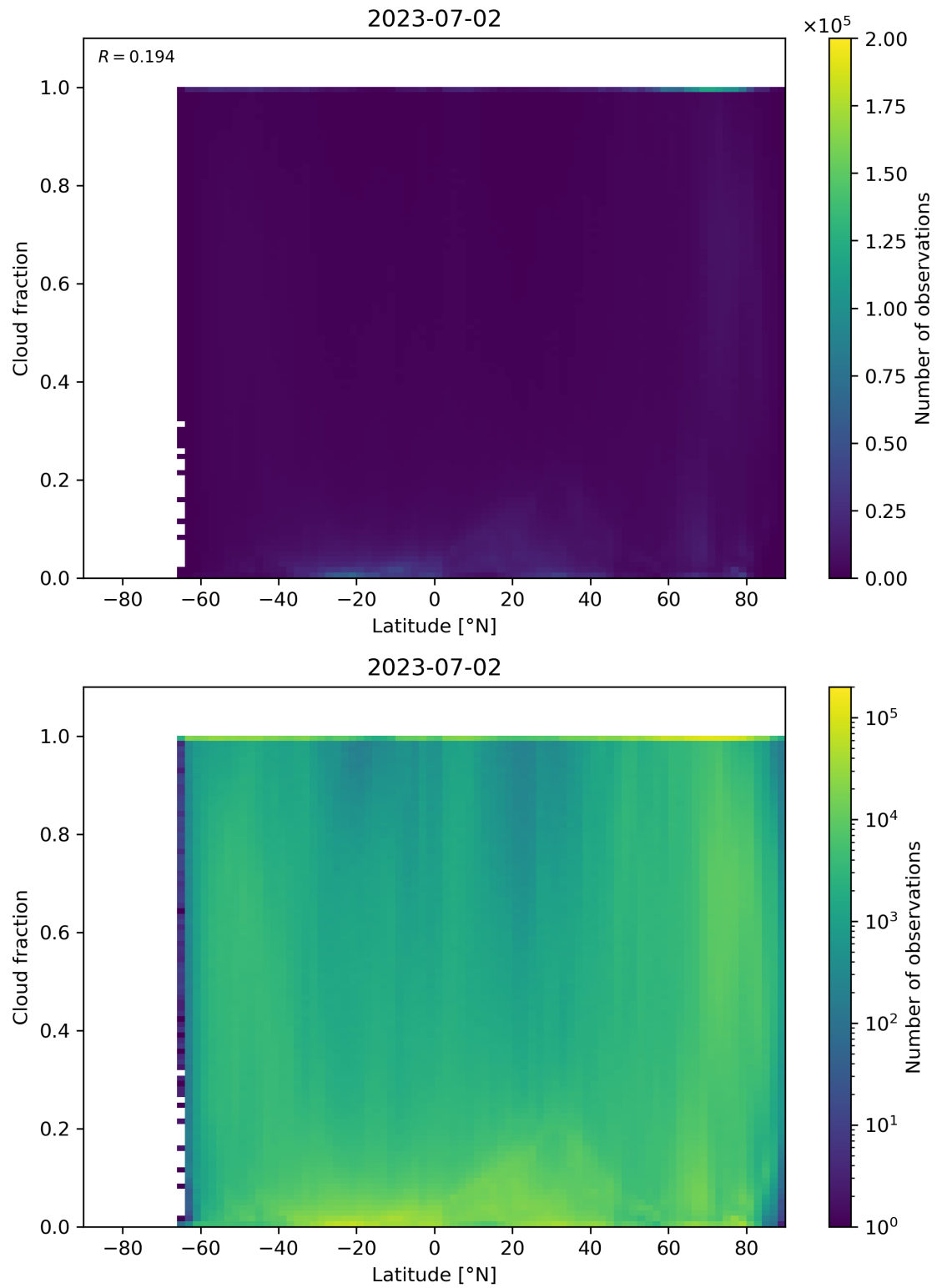
Figure 99: Scatter density plot of “Latitude” against “Cloud fraction” for 2023-07-01 to 2023-07-03.
