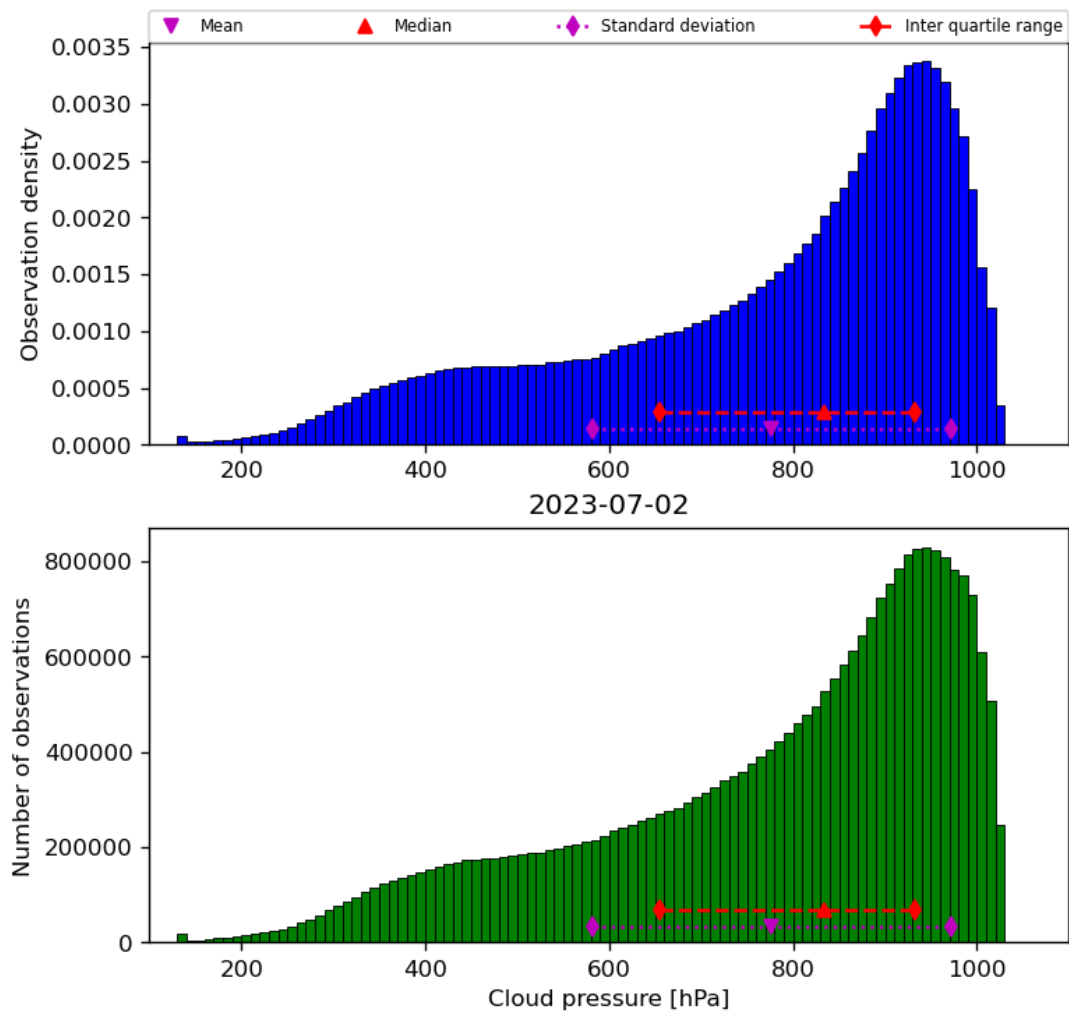
Figure 30: Histogram of “Cloud pressure” for 2023-07-01 to 2023-07-03
