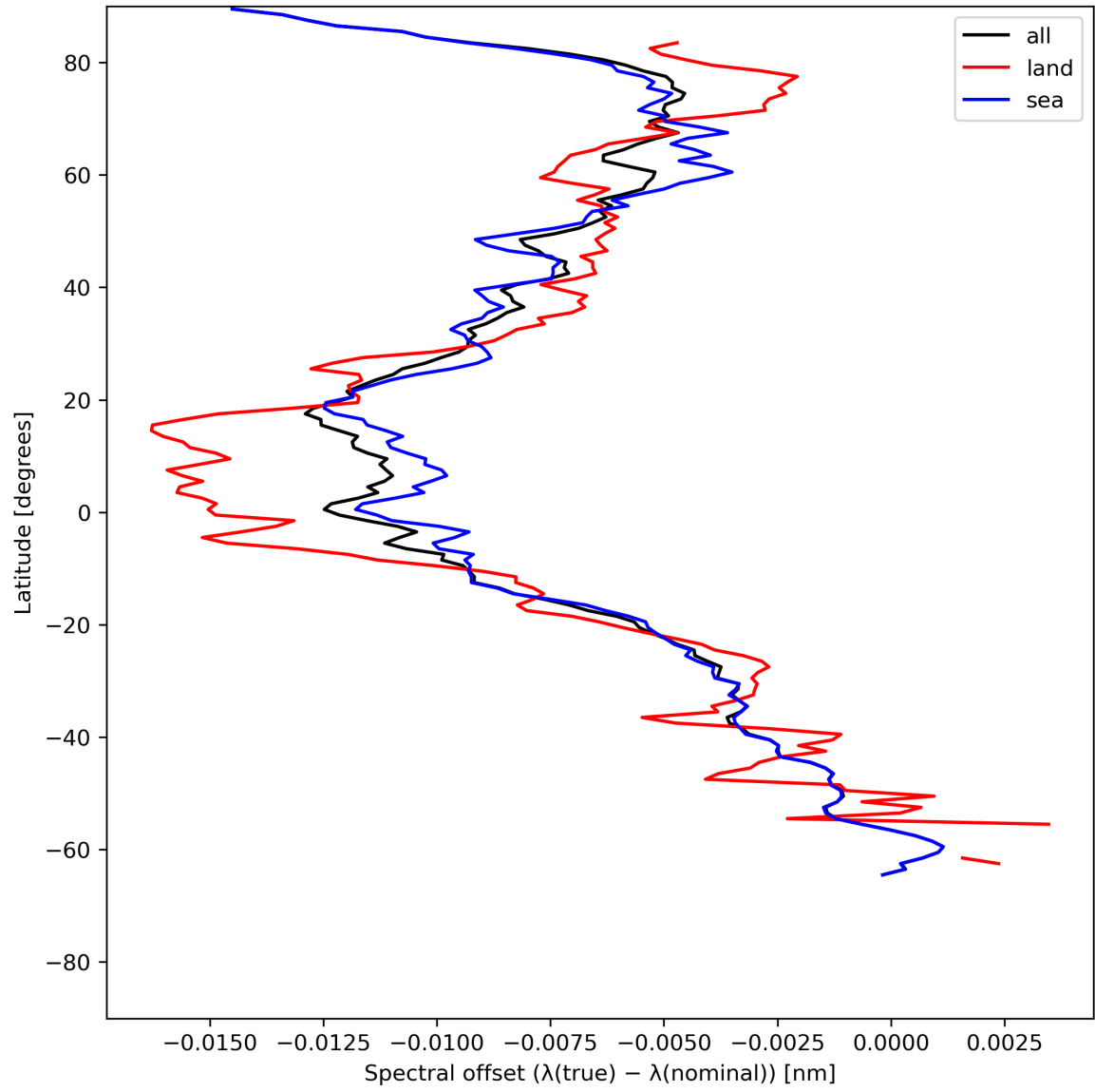
Figure 28: Zonal average of “Spectral offset ( \lambda(\text{true}) - \lambda(\text{nominal}) )” for 2023-07-01 to 2023-07-03.
