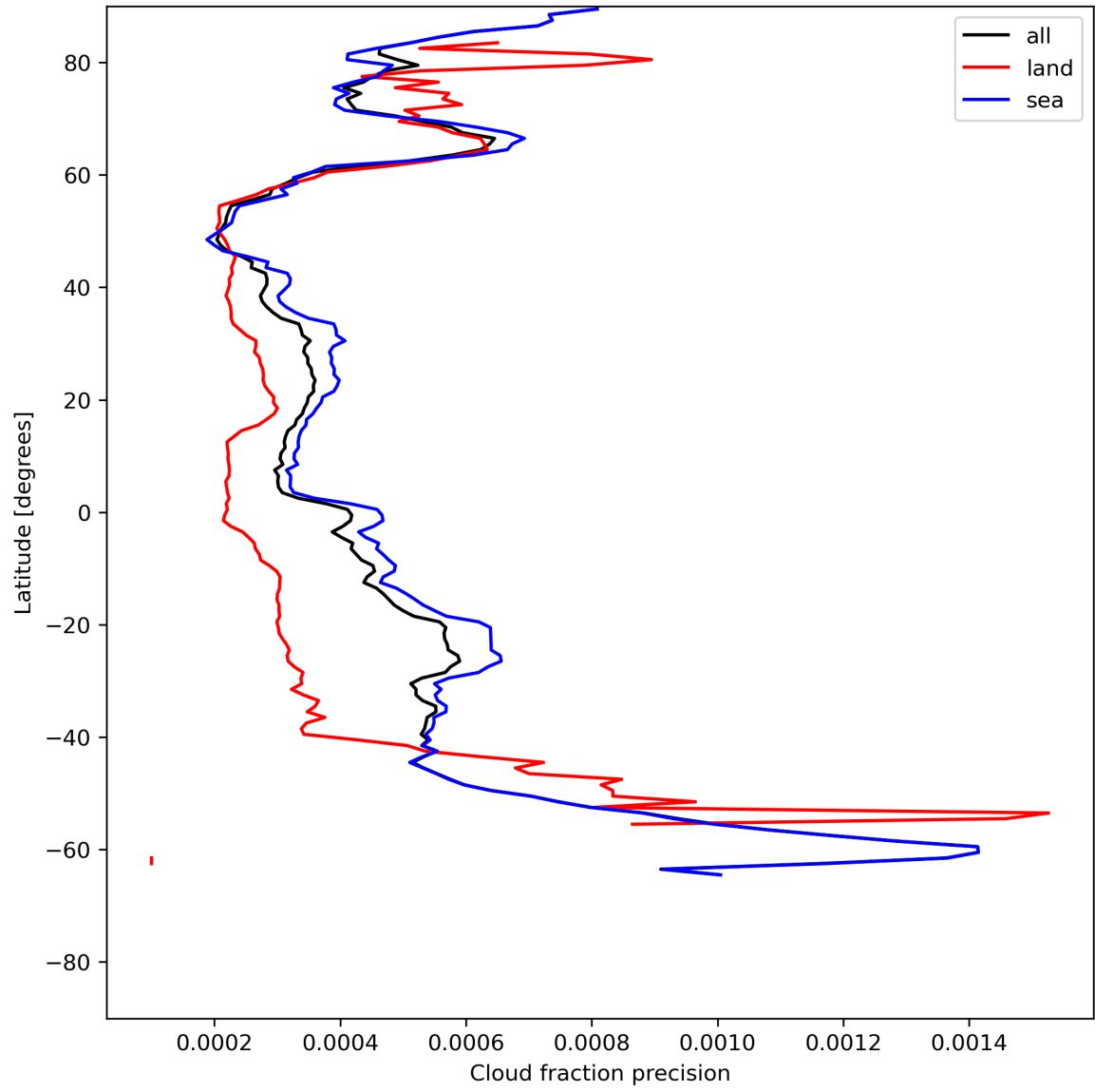
Figure 16: Zonal average of “Cloud fraction precision” for 2023-07-01 to 2023-07-03.
