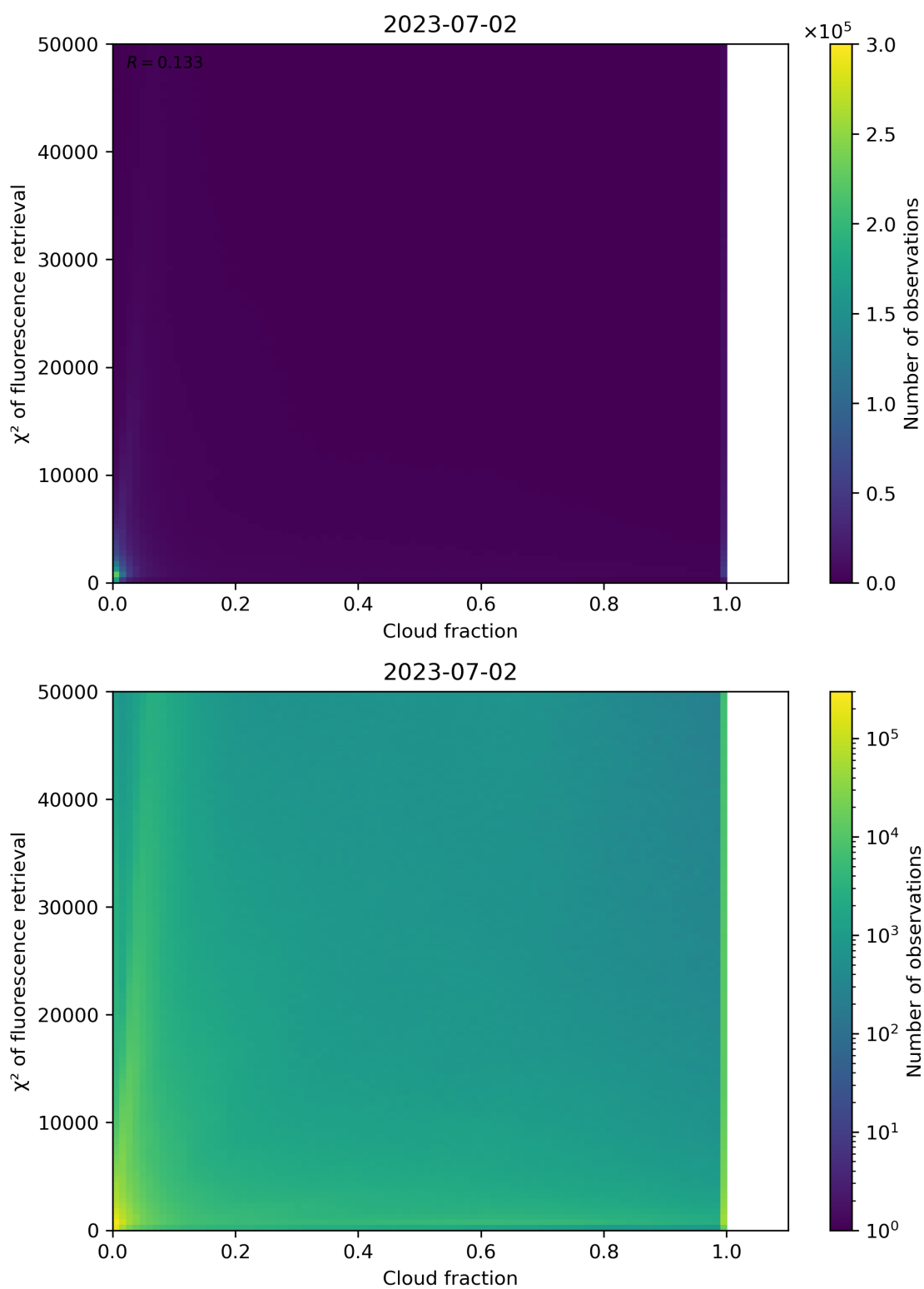
Figure 78: Scatter density plot of “Cloud fraction” against “ \chi^2 of fluorescence retrieval” for 2023-07-01 to 2023-07-03.
