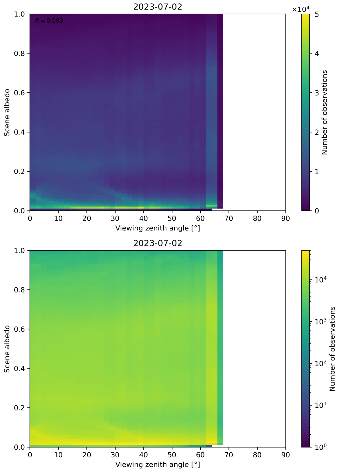
Figure 138: Scatter density plot of “Viewing zenith angle” against “Scene albedo” for 2023-07-01 to 2023-07-03.
