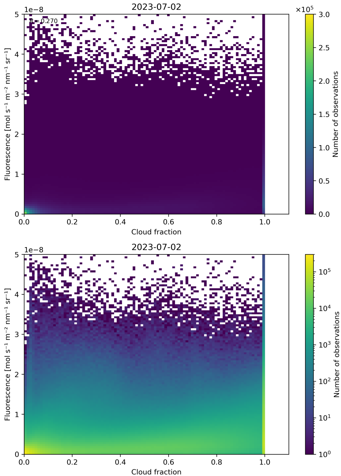
Figure 79: Scatter density plot of “Cloud fraction” against “Fluorescence” for 2023-07-01 to 2023-07-03.
