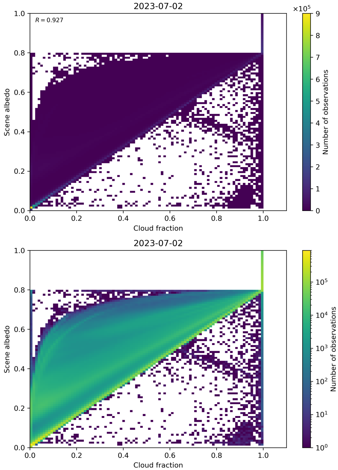
Figure 82: Scatter density plot of “Cloud fraction” against “Scene albedo” for 2023-07-01 to 2023-07-03.
