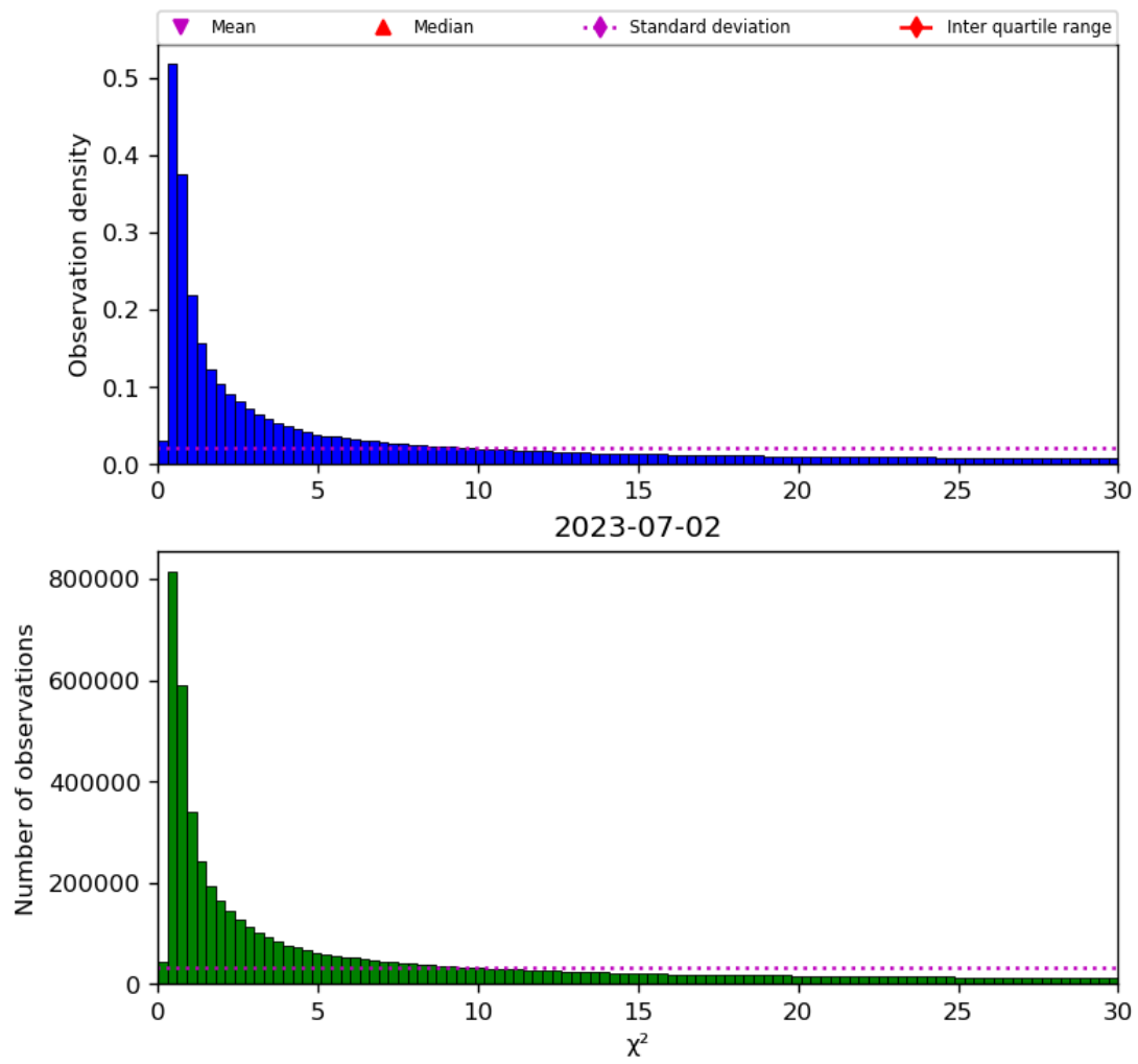
Figure 38: Histogram of " \chi^2 " for 2023-07-01 to 2023-07-03
