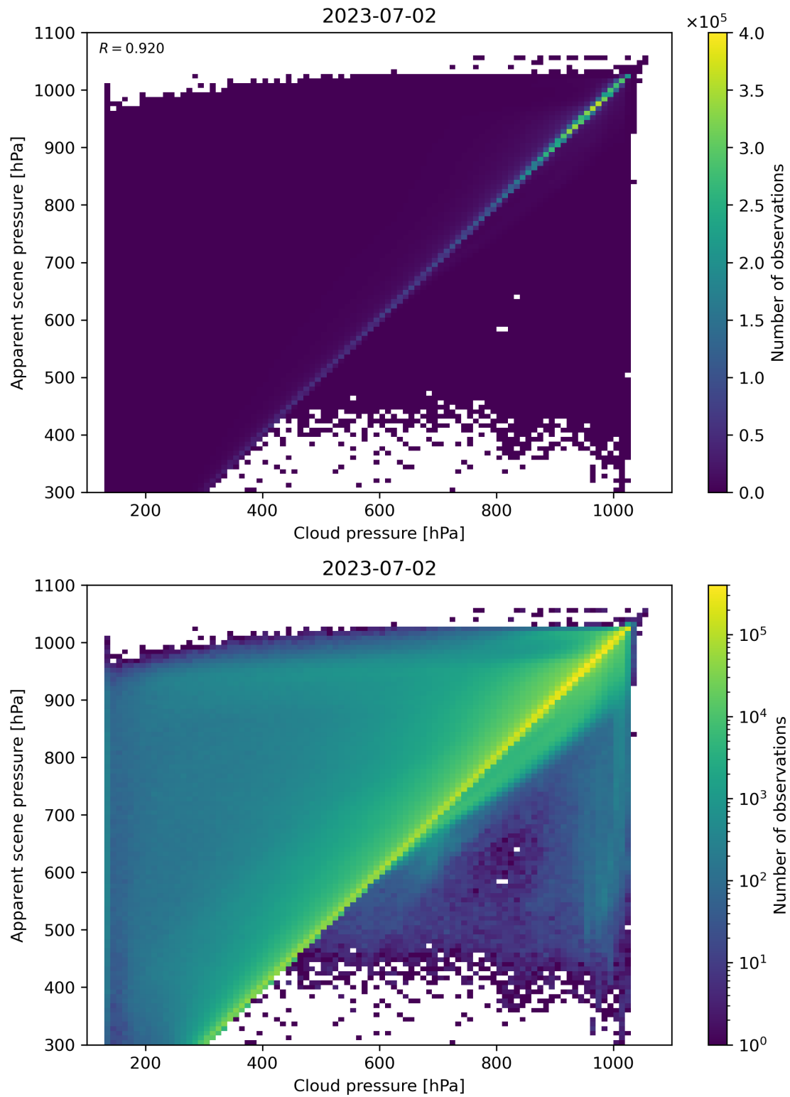
Figure 84: Scatter density plot of “Cloud pressure” against “Apparent scene pressure” for 2023-07-01 to 2023-07-03.
