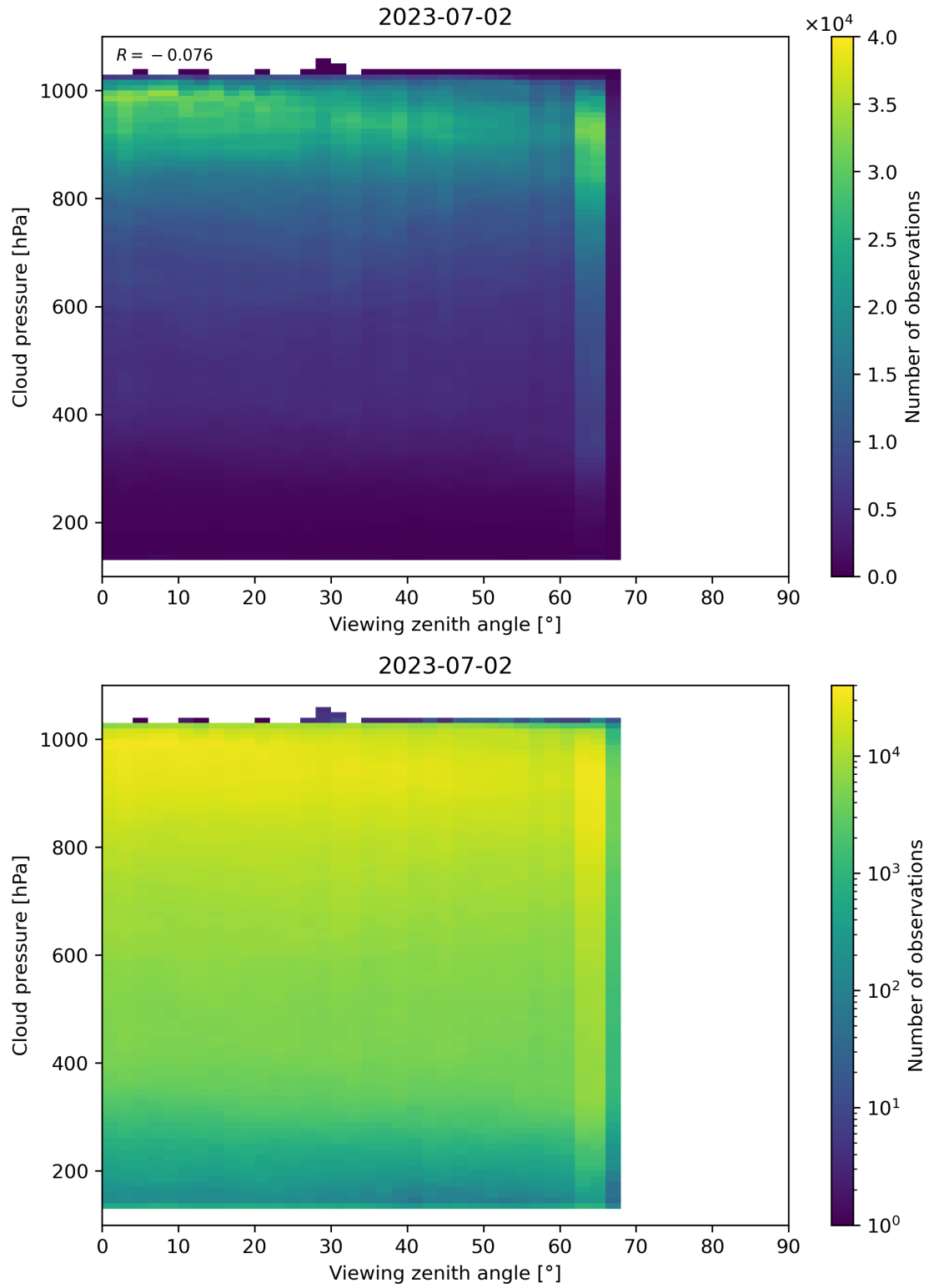
Figure 133: Scatter density plot of “Viewing zenith angle” against “Cloud pressure” for 2023-07-01 to 2023-07-03.
