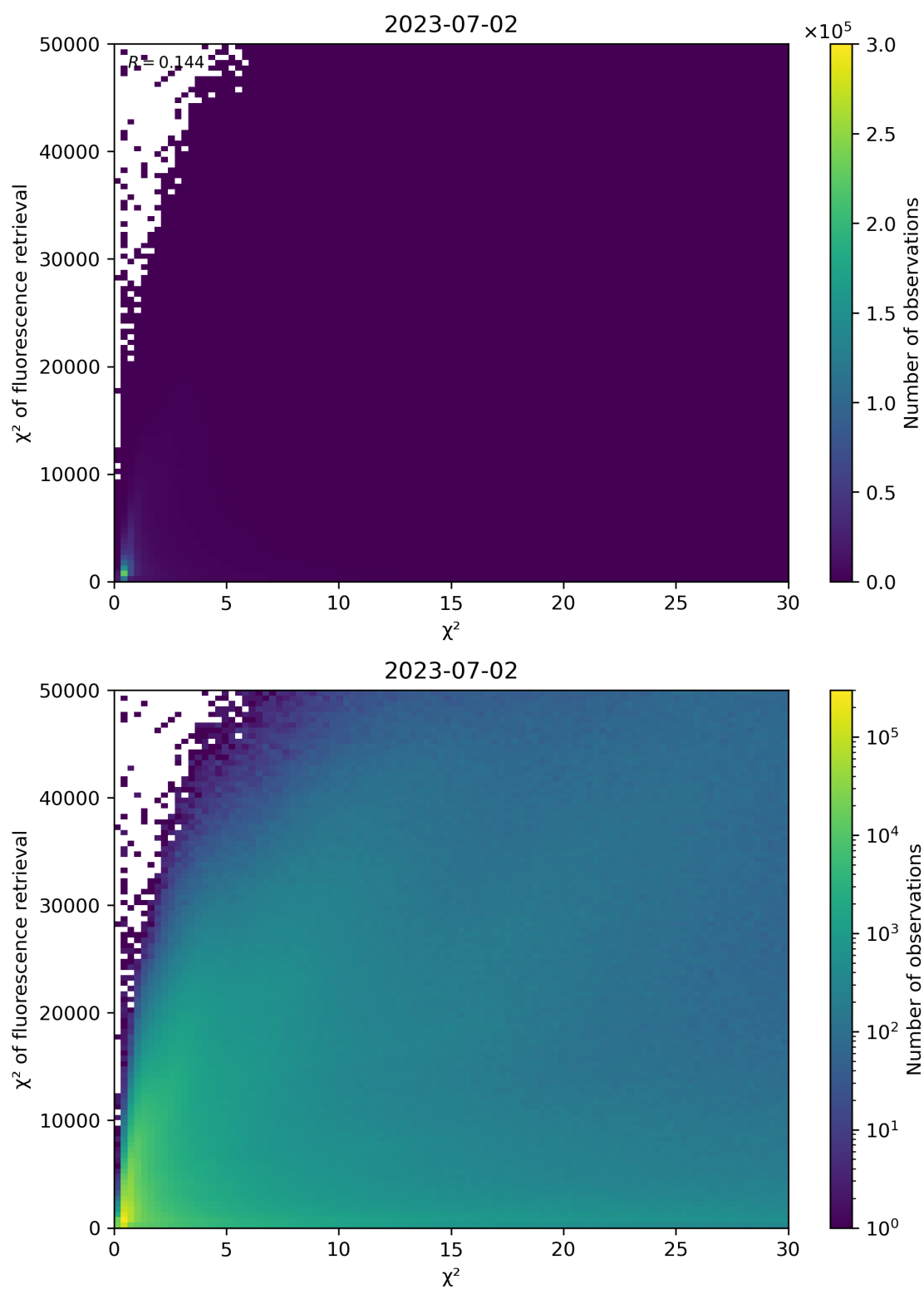
Figure 69: Scatter density plot of “ \chi^2 ” against “ \chi^2 of fluorescence retrieval” for 2023-07-01 to 2023-07-03.
