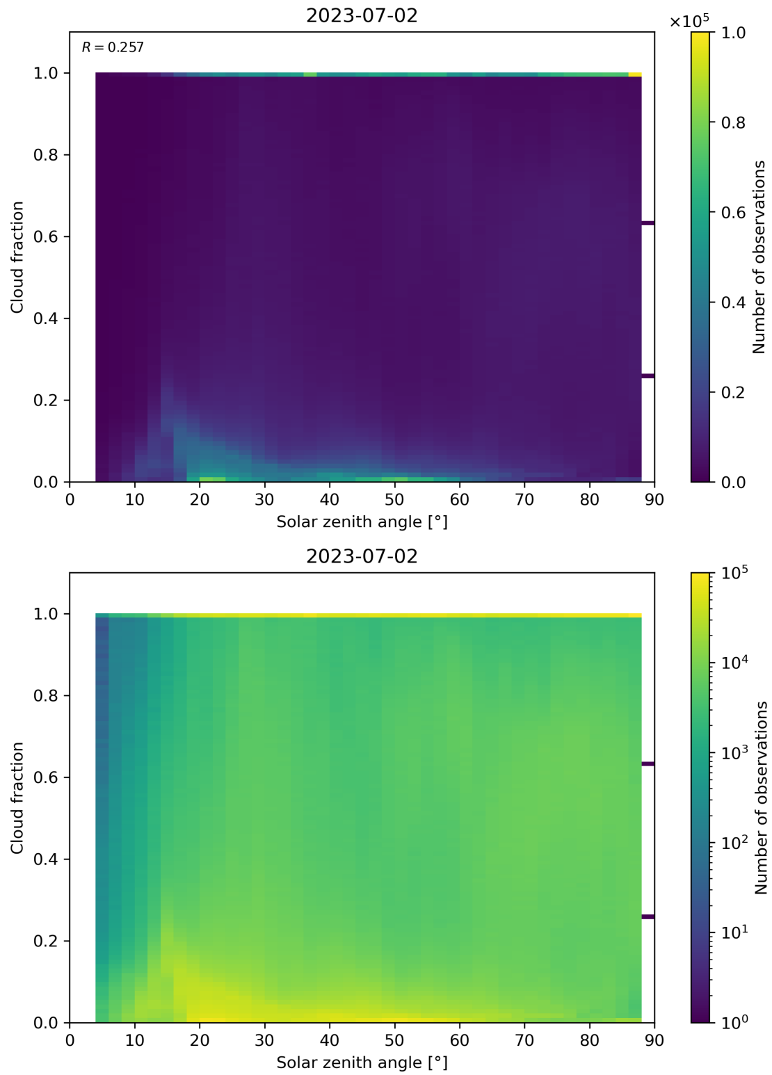
Figure 121: Scatter density plot of “Solar zenith angle” against “Cloud fraction” for 2023-07-01 to 2023-07-03.
