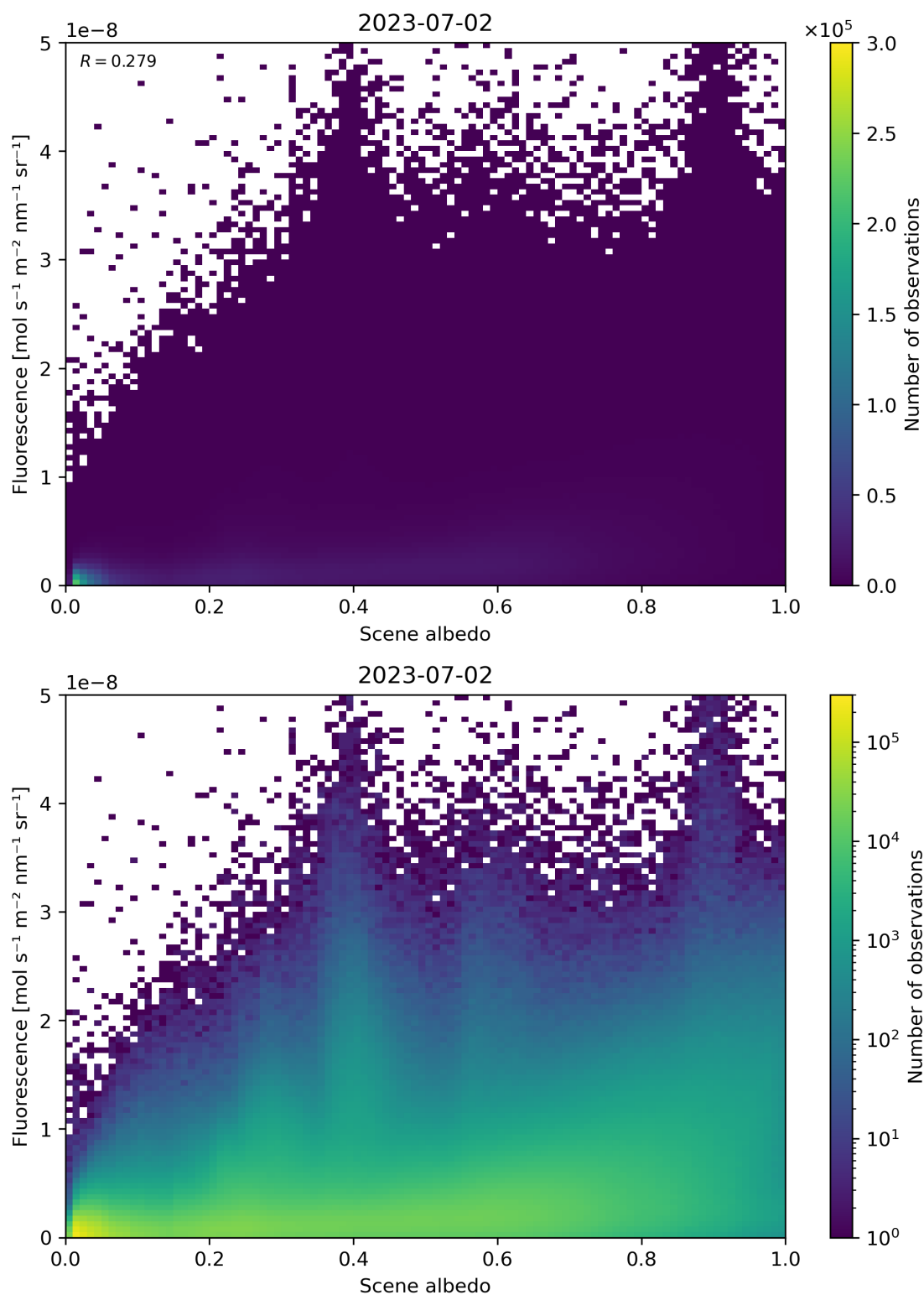
Figure 114: Scatter density plot of “Scene albedo” against “Fluorescence” for 2023-07-01 to 2023-07-03.
