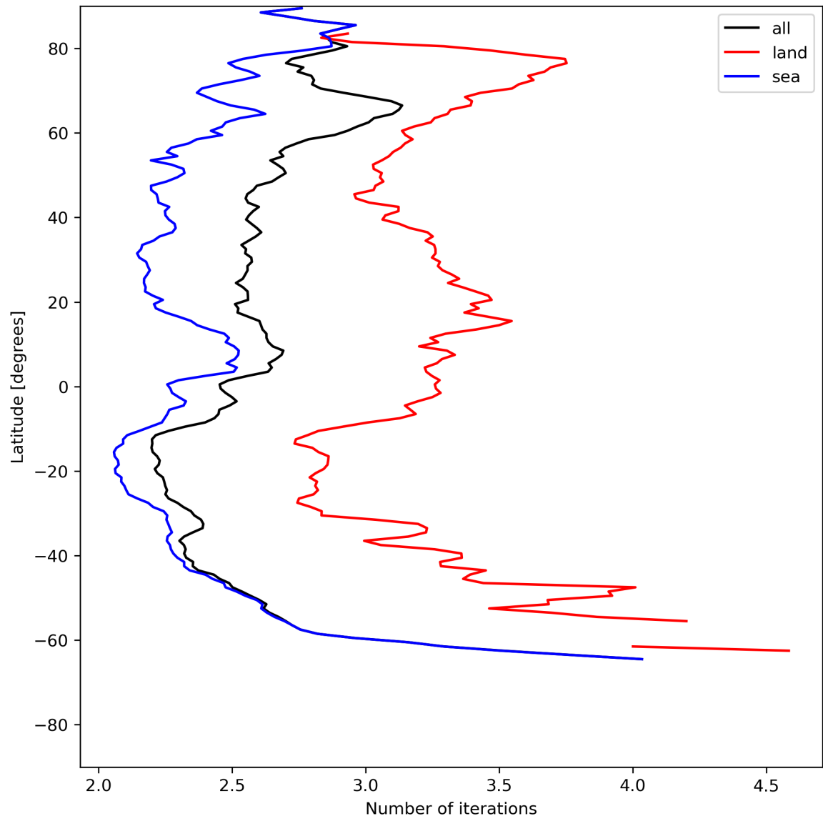
Figure 22: Zonal average of “Number of iterations” for 2023-07-01 to 2023-07-03.
