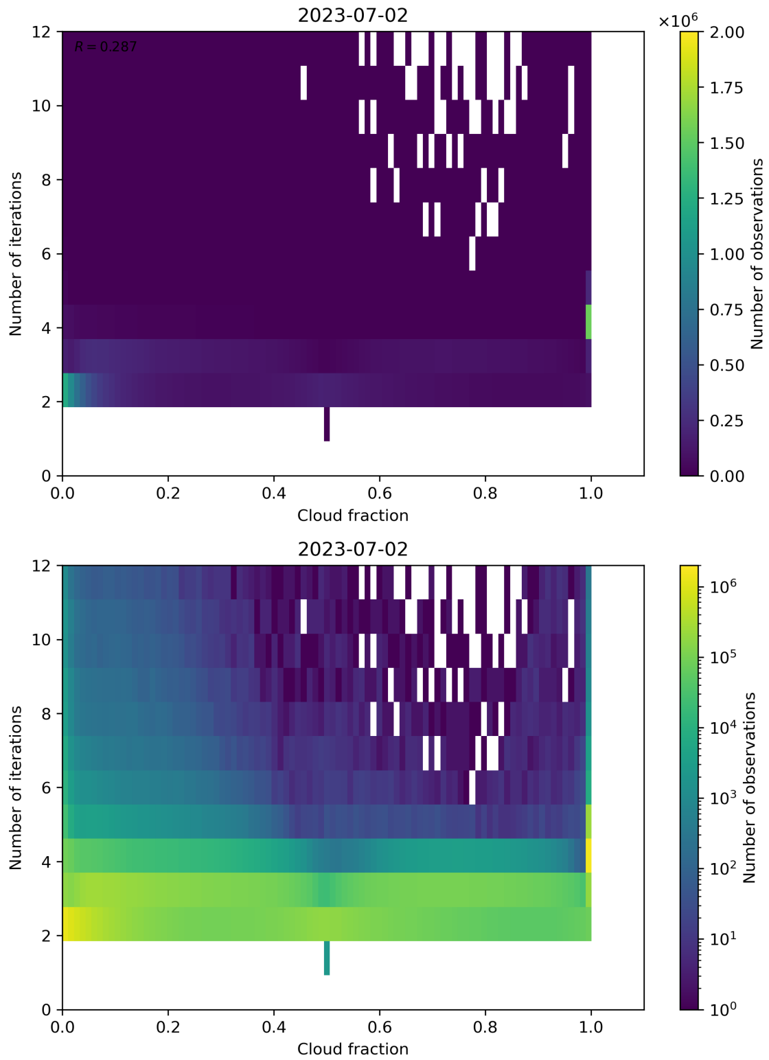
Figure 80: Scatter density plot of “Cloud fraction” against “Number of iterations” for 2023-07-01 to 2023-07-03.
