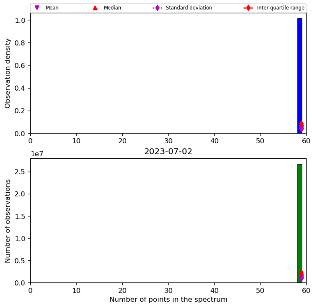
Figure 44: Histogram of “Number of points in the spectrum” for 2023-07-01 to 2023-07-03
