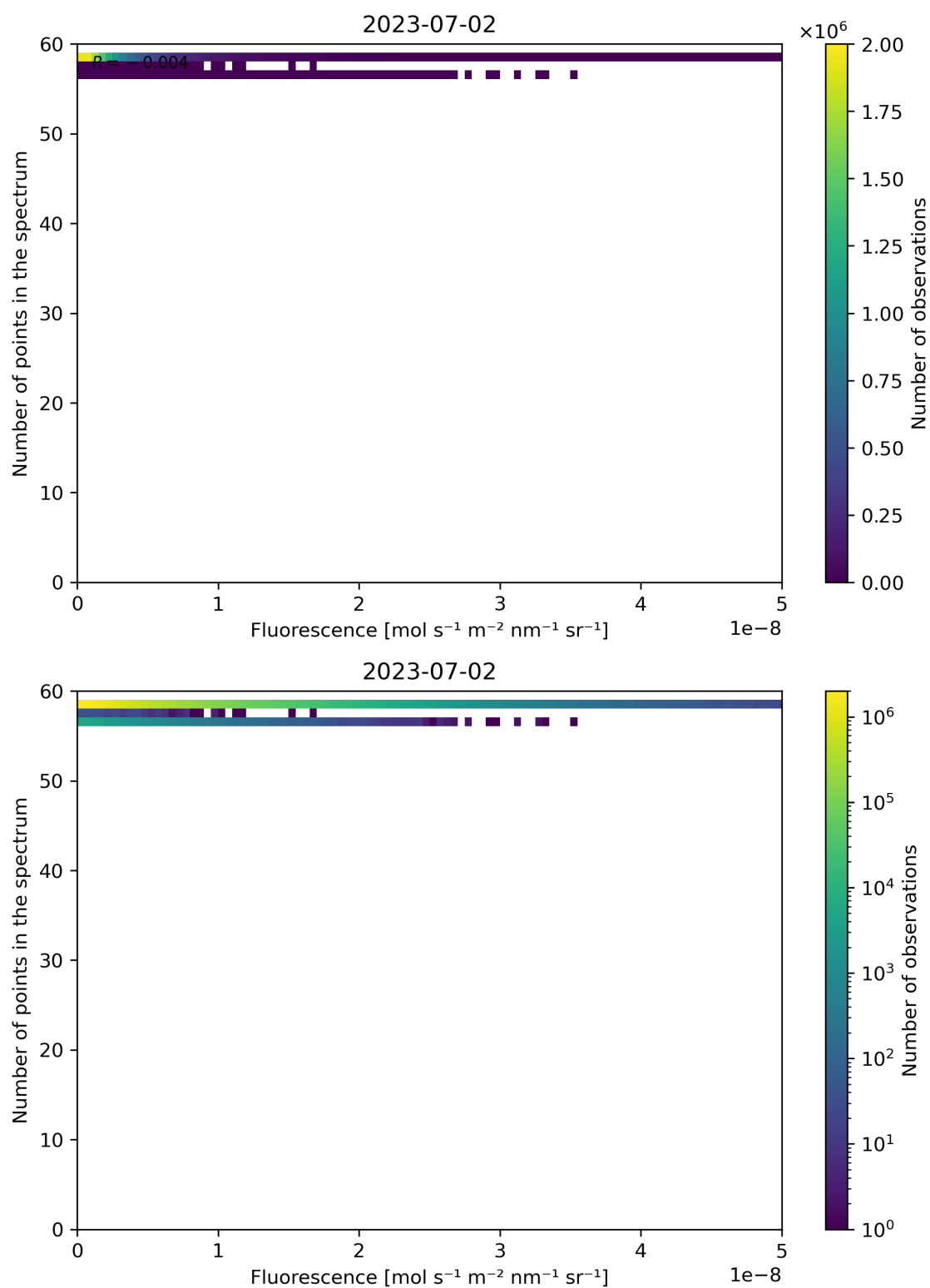
Figure 94: Scatter density plot of “Fluorescence” against “Number of points in the spectrum” for 2023-07-01 to 2023-07-03.
