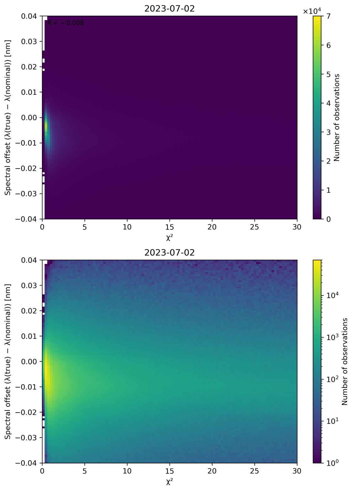
Figure 75: Scatter density plot of “ \chi^2 ” against “Spectral offset ( \lambda(\text{true}) - \lambda(\text{nominal}) )” for 2023-07-01 to 2023-07-03.
