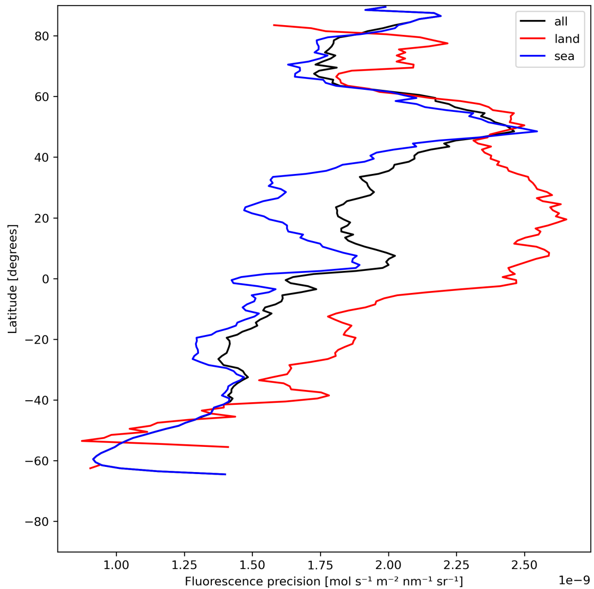
Figure 24: Zonal average of “Fluorescence precision” for 2023-07-01 to 2023-07-03.
