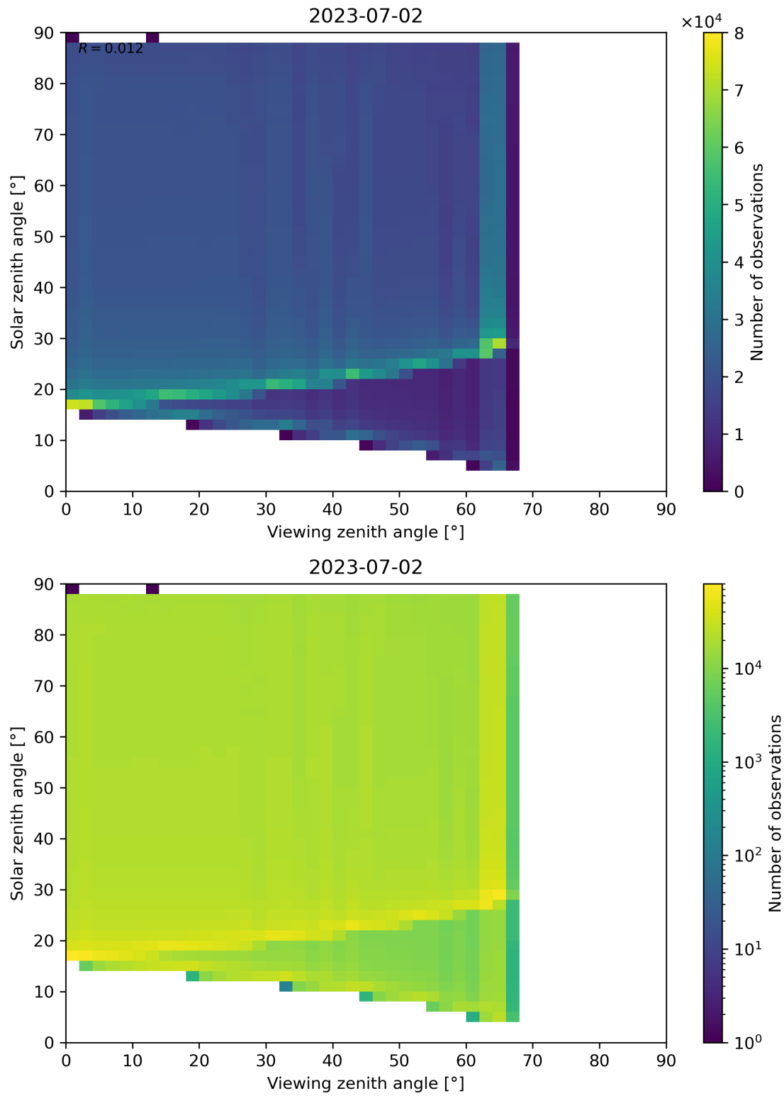
Figure 139: Scatter density plot of “Viewing zenith angle” against “Solar zenith angle” for 2023-07-01 to 2023-07-03.
