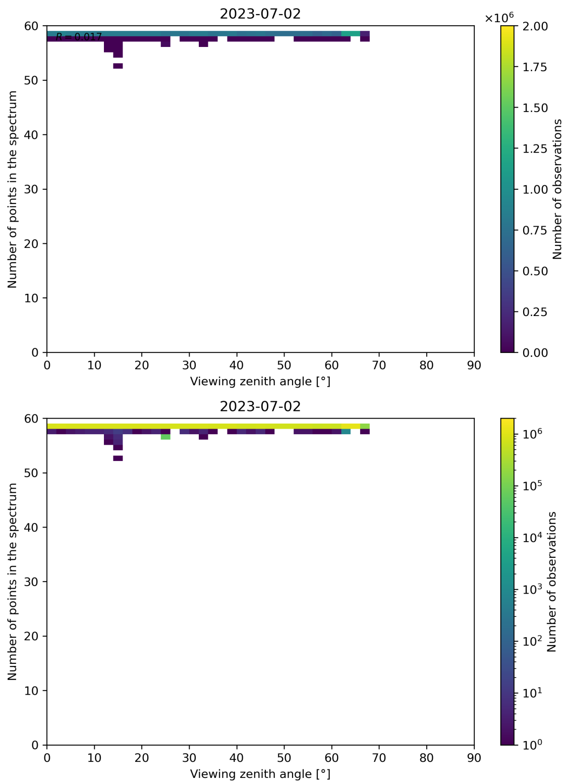
Figure 137: Scatter density plot of “Viewing zenith angle” against “Number of points in the spectrum” for 2023-07-01 to 2023-07-03.
