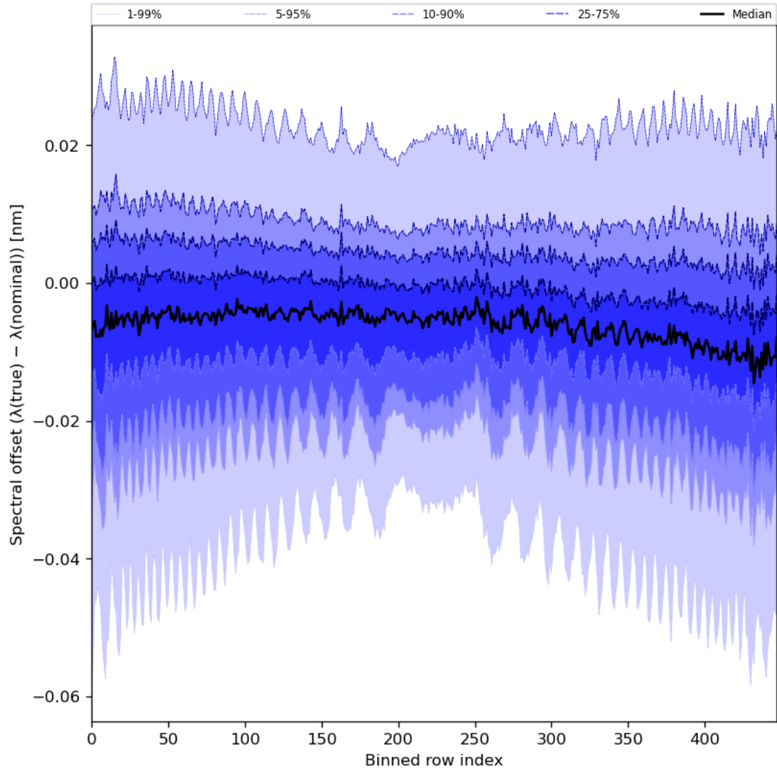
Figure 62: Along track statistics of “Spectral offset ( \lambda(\text{true}) - \lambda(\text{nominal}) )” for 2023-07-01 to 2023-07-03
