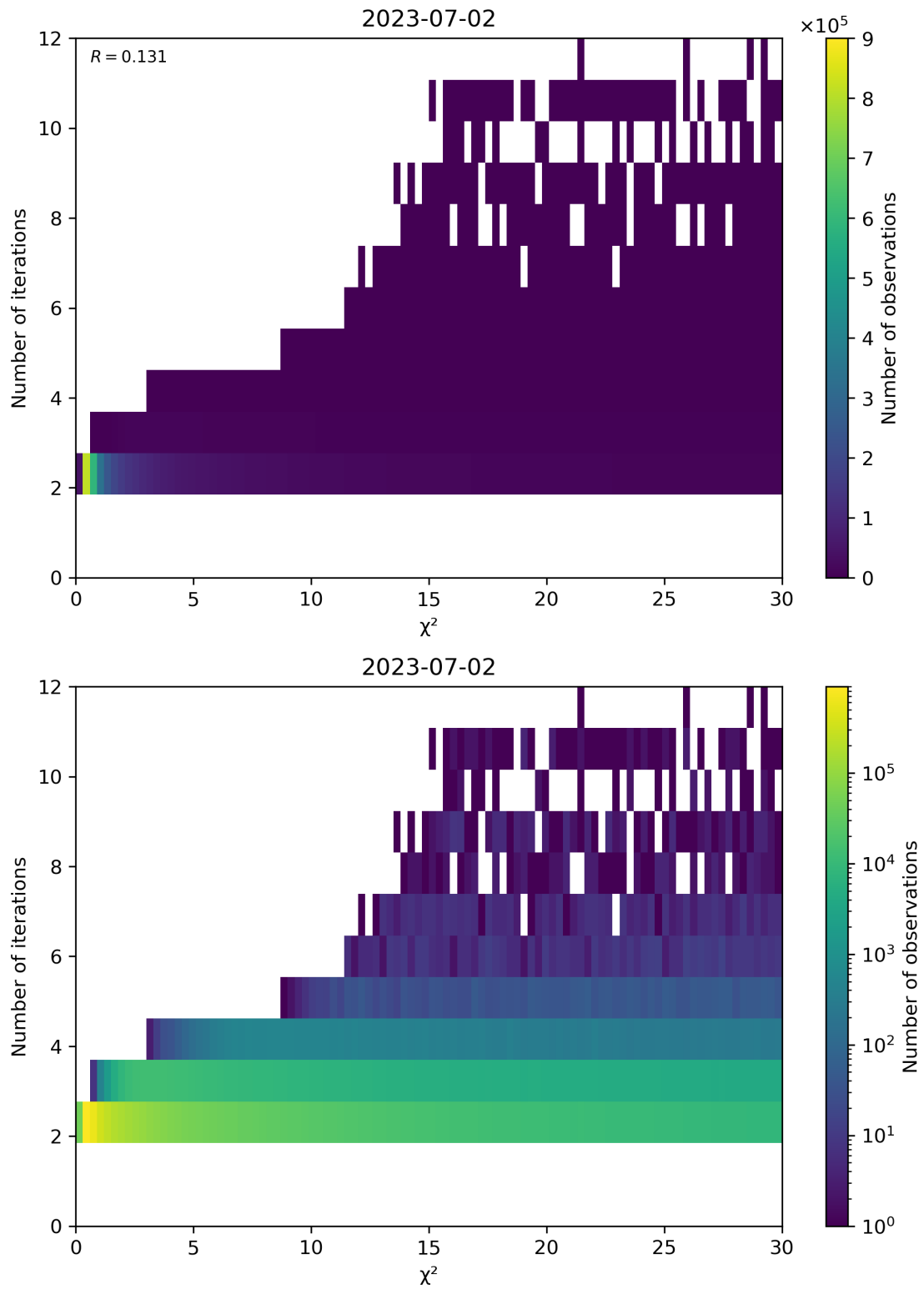
Figure 73: Scatter density plot of “ \chi^2 ” against “Number of iterations” for 2023-07-01 to 2023-07-03.
