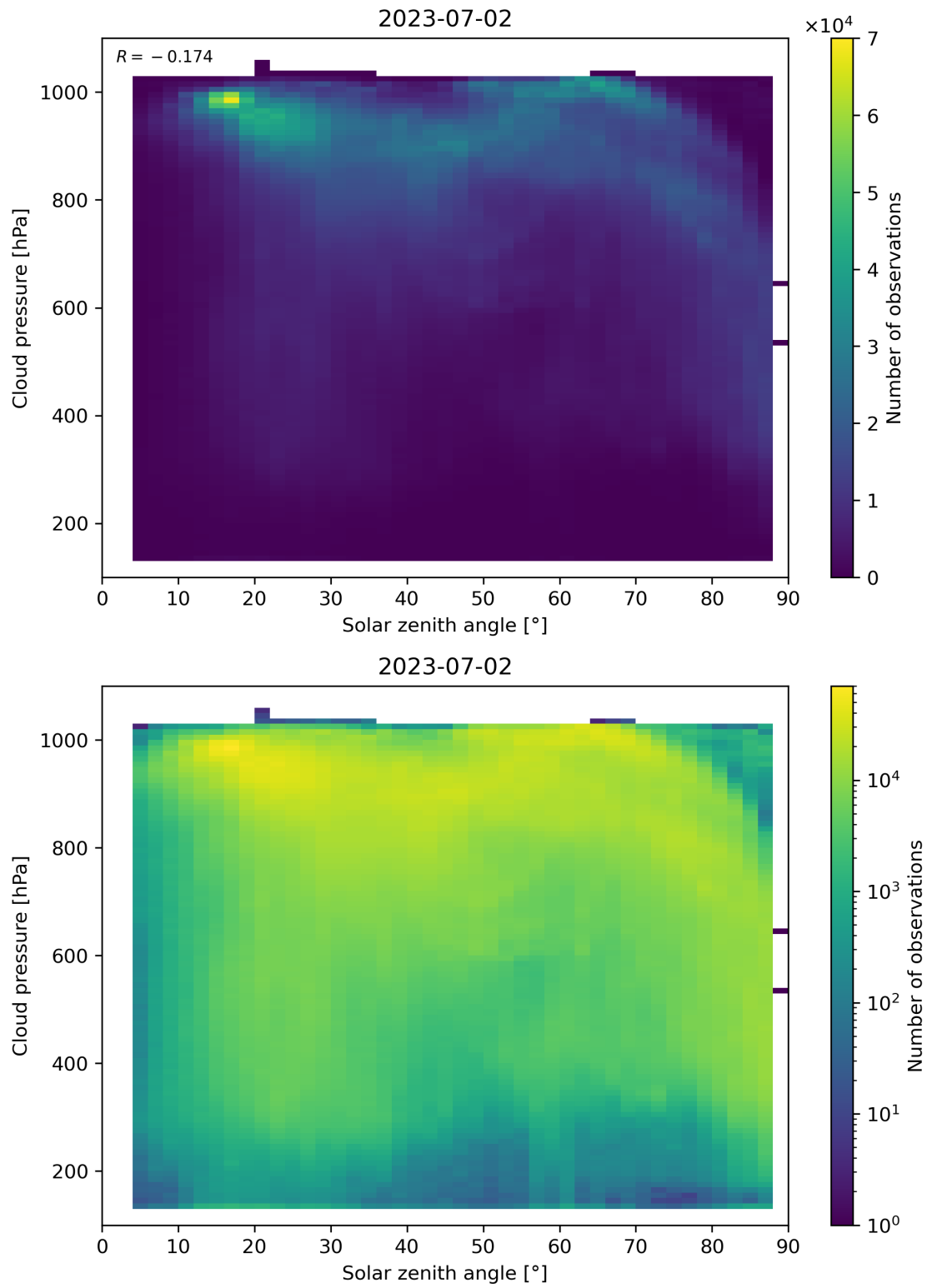
Figure 122: Scatter density plot of “Solar zenith angle” against “Cloud pressure” for 2023-07-01 to 2023-07-03.
