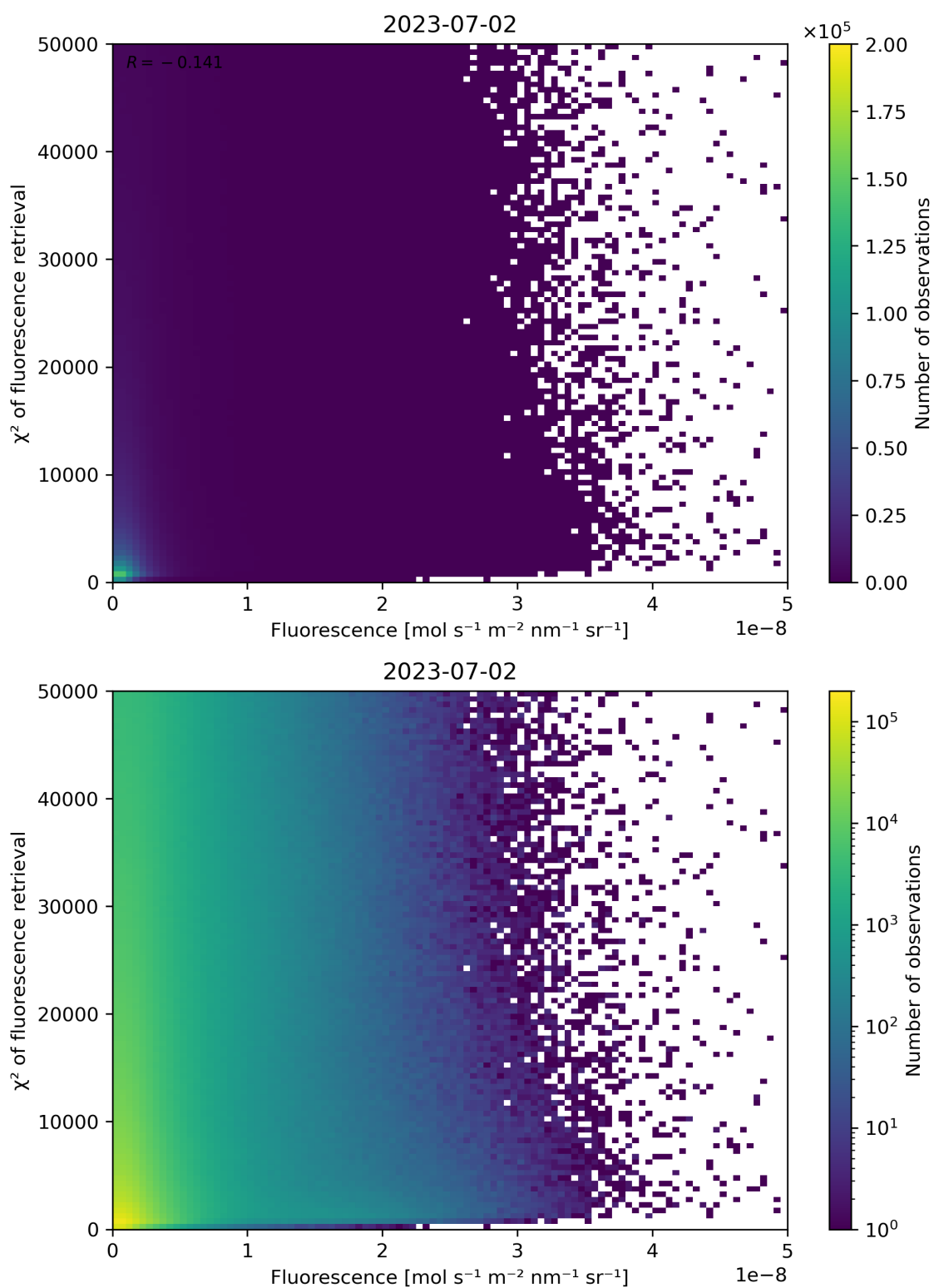
Figure 93: Scatter density plot of “Fluorescence” against “ \chi^2 of fluorescence retrieval” for 2023-07-01 to 2023-07-03.
