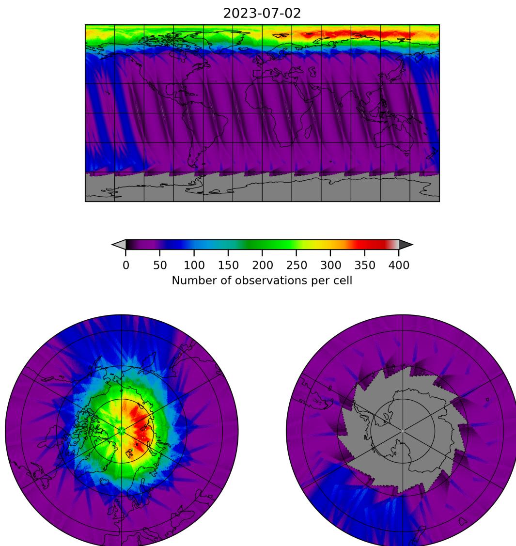
Figure 11: Map of the number of observations for 2023-07-01 to 2023-07-03
