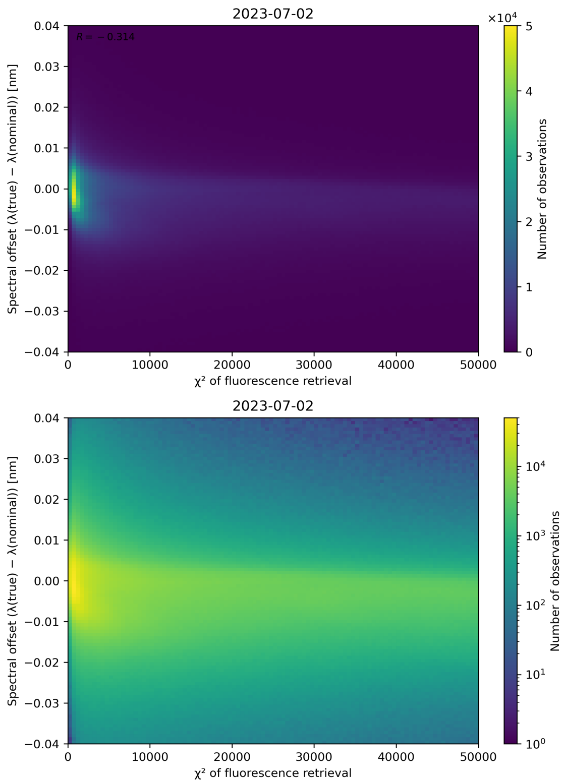
Figure 72: Scatter density plot of " \chi^2 of fluorescence retrieval" against "Spectral offset ( \lambda(\text{true}) - \lambda(\text{nominal}) )" for 2023-07-01 to 2023-07-03.
