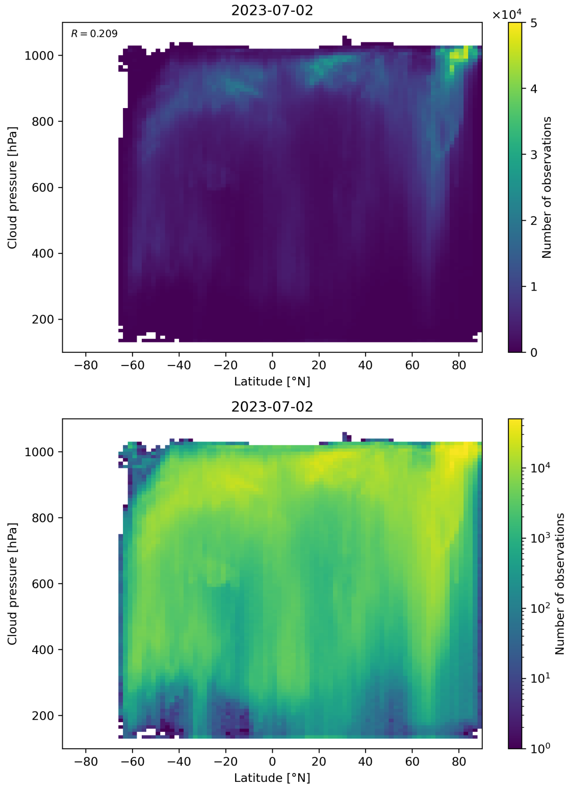
Figure 100: Scatter density plot of “Latitude” against “Cloud pressure” for 2023-07-01 to 2023-07-03.
