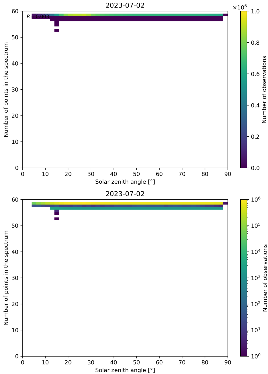
Figure 126: Scatter density plot of “Solar zenith angle” against “Number of points in the spectrum” for 2023-07-01 to 2023-07-03.
