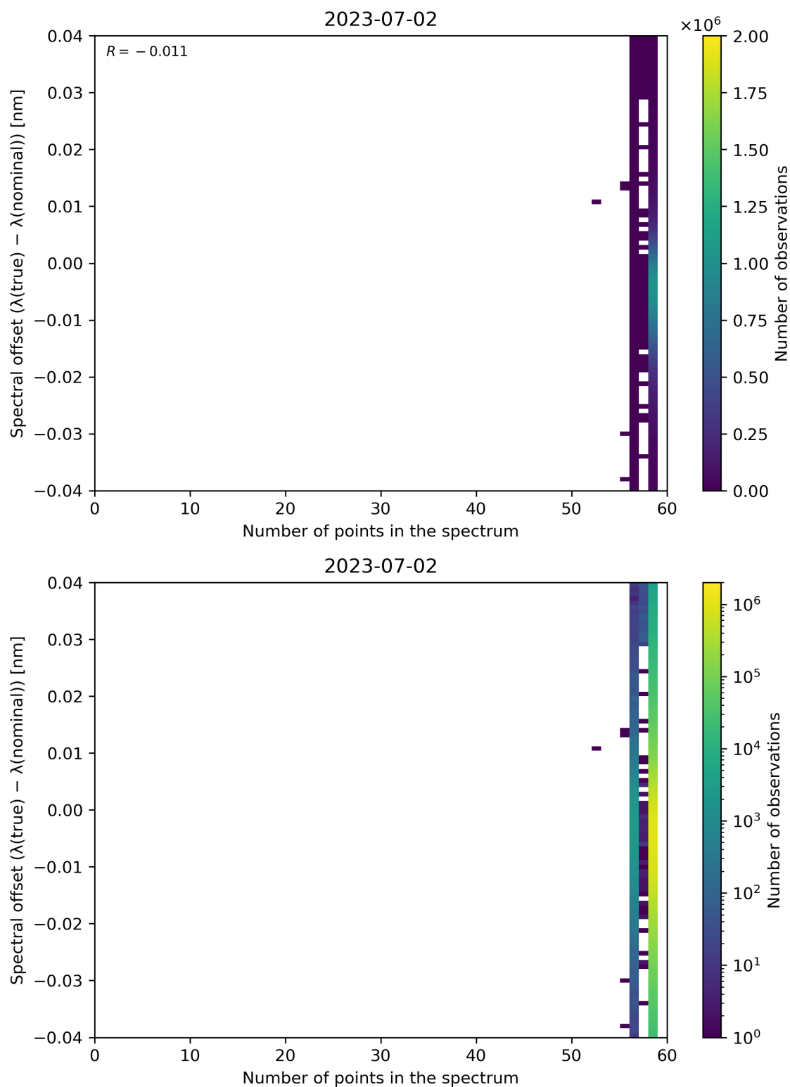
Figure 110: Scatter density plot of “Number of points in the spectrum” against “Spectral offset ( \lambda(\text{true}) - \lambda(\text{nominal}) )” for 2023-07-01 to 2023-07-03.
