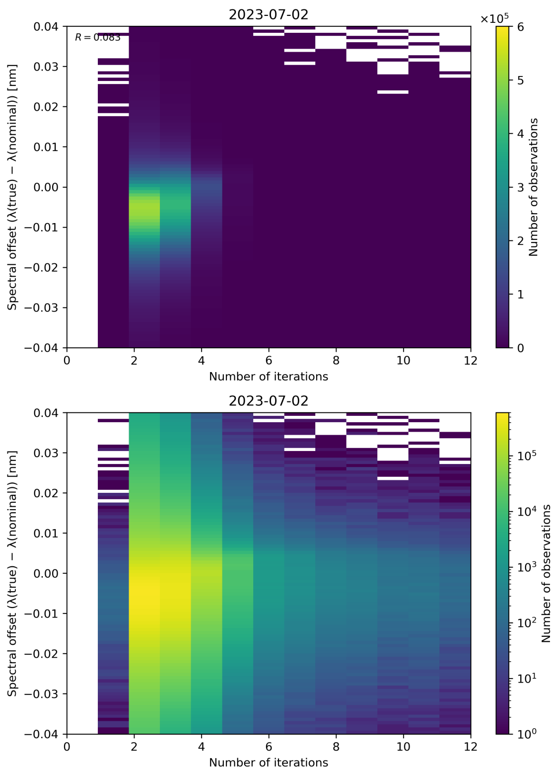
Figure 109: Scatter density plot of “Number of iterations” against “Spectral offset ( \lambda(\text{true}) - \lambda(\text{nominal}) )” for 2023-07-01 to 2023-07-03.
