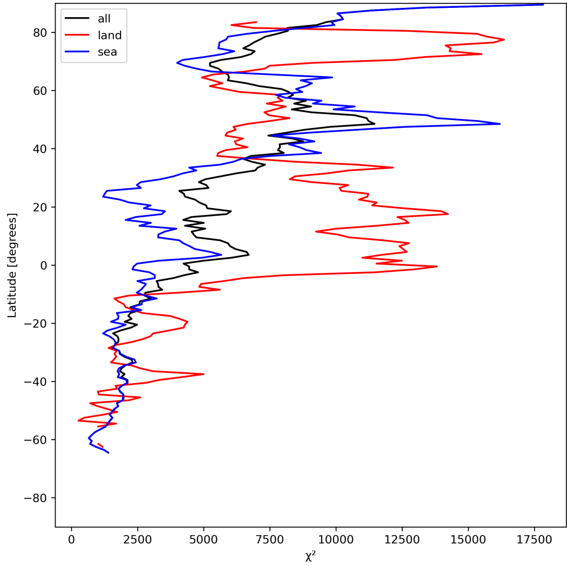
Figure 21: Zonal average of “ \chi^2 ” for 2023-07-01 to 2023-07-03.
