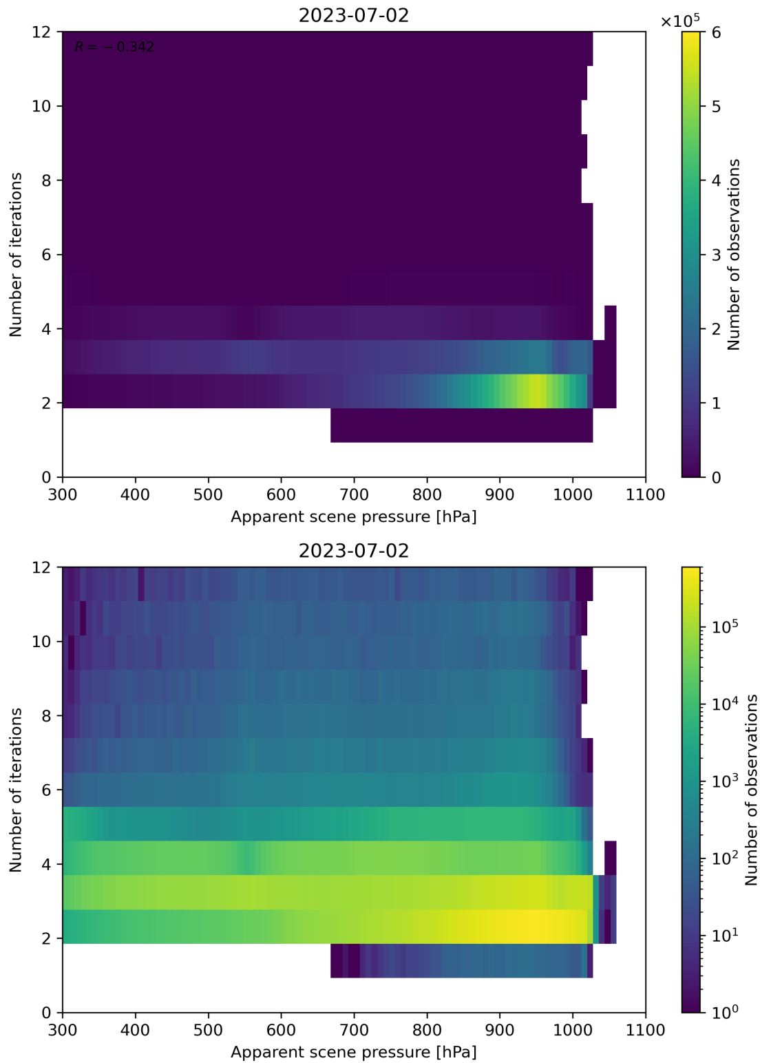
Figure 66: Scatter density plot of “Apparent scene pressure” against “Number of iterations” for 2023-07-01 to 2023-07-03.
