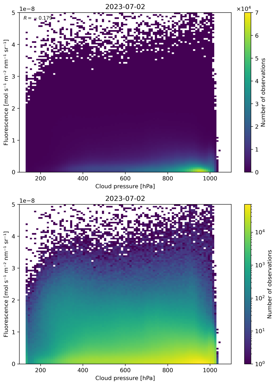
Figure 88: Scatter density plot of “Cloud pressure” against “Fluorescence” for 2023-07-01 to 2023-07-03.
