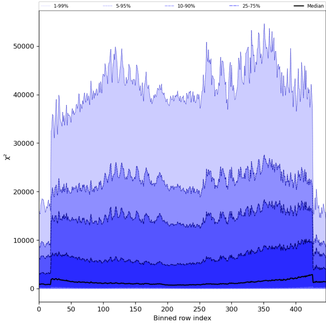
Figure 55: Along track statistics of “ \chi^2 ” for 2023-07-01 to 2023-07-03
