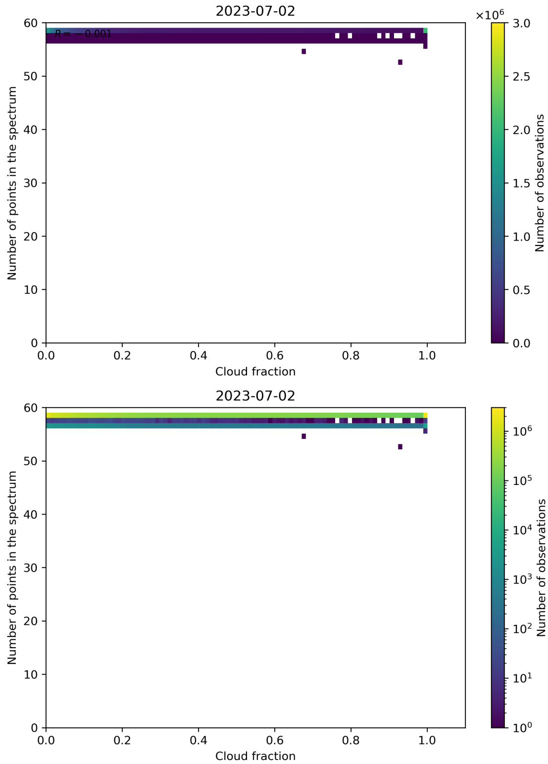
Figure 81: Scatter density plot of “Cloud fraction” against “Number of points in the spectrum” for 2023-07-01 to 2023-07-03.
