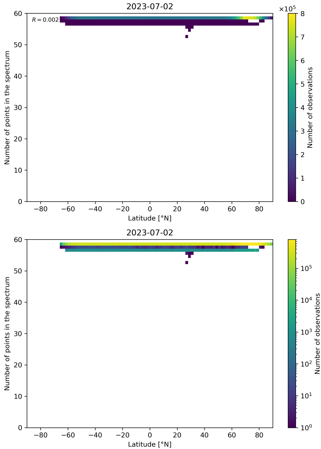
Figure 103: Scatter density plot of “Latitude” against “Number of points in the spectrum” for 2023-07-01 to 2023-07-03.
