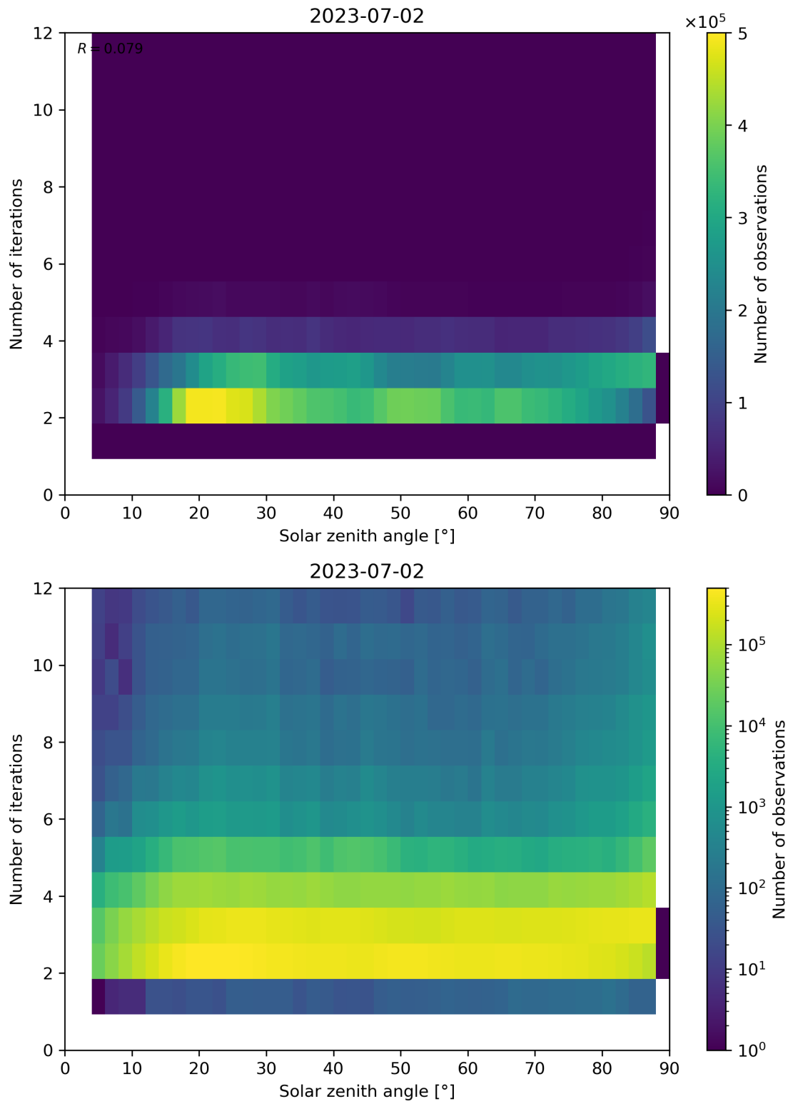
Figure 125: Scatter density plot of “Solar zenith angle” against “Number of iterations” for 2023-07-01 to 2023-07-03.
