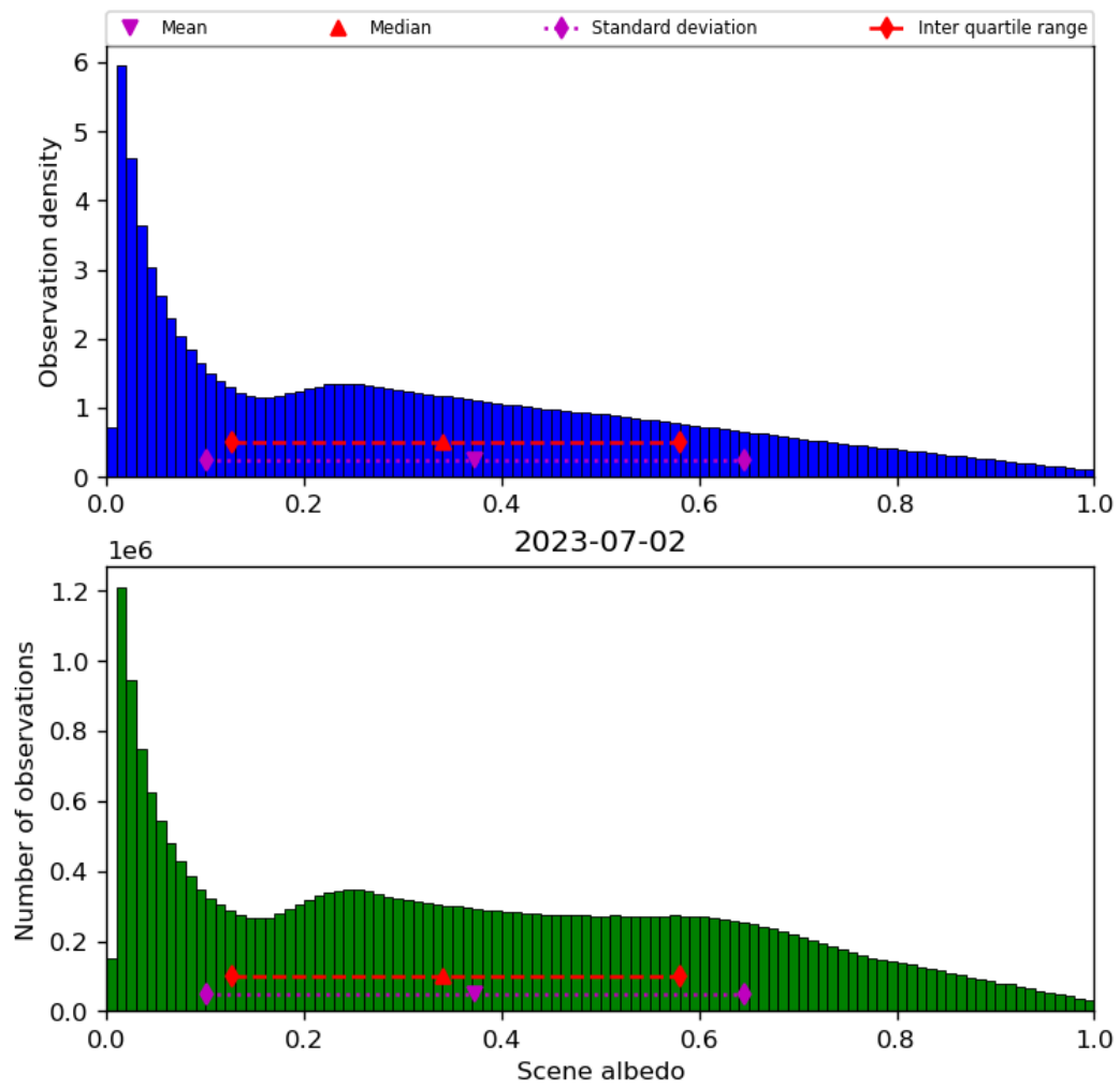
Figure 34: Histogram of “Scene albedo” for 2023-07-01 to 2023-07-03
