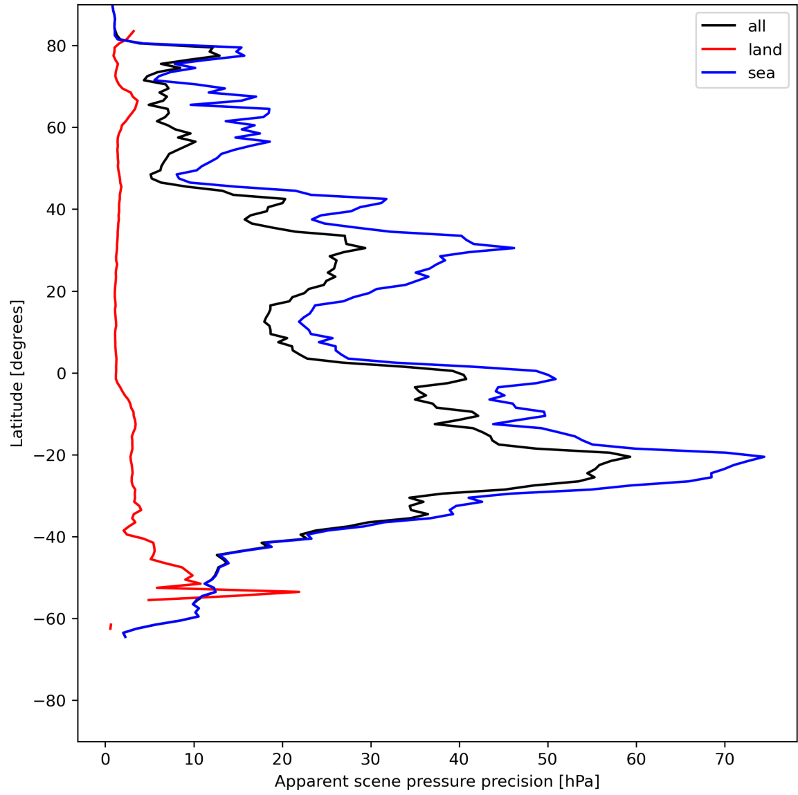
Figure 20: Zonal average of “Apparent scene pressure precision” for 2023-07-01 to 2023-07-03.
