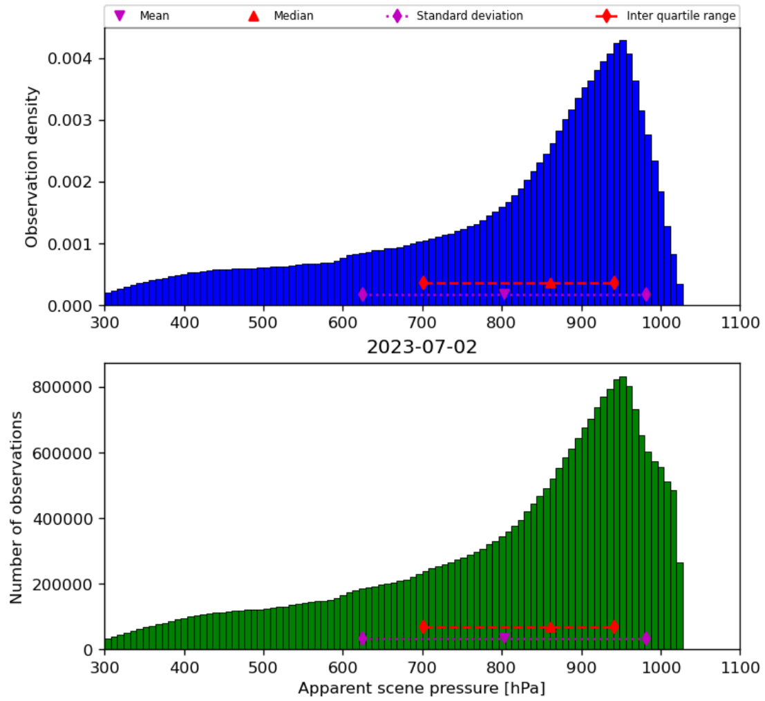
Figure 36: Histogram of “Apparent scene pressure” for 2023-07-01 to 2023-07-03
