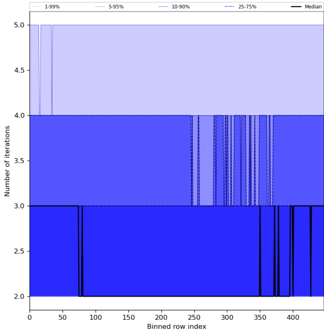
Figure 56: Along track statistics of “Number of iterations” for 2023-07-01 to 2023-07-03
