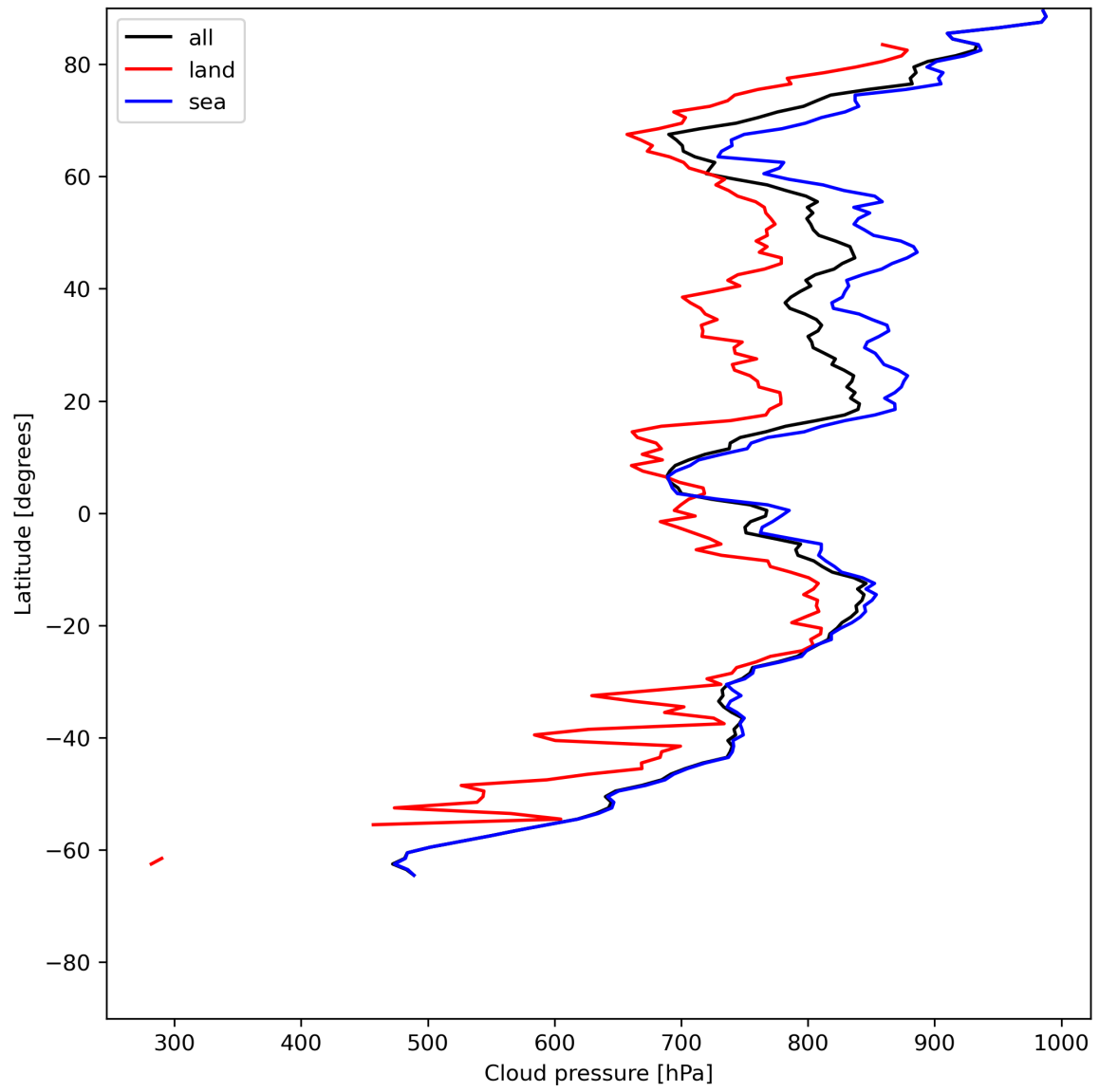
Figure 13: Zonal average of “Cloud pressure” for 2023-07-01 to 2023-07-03.
