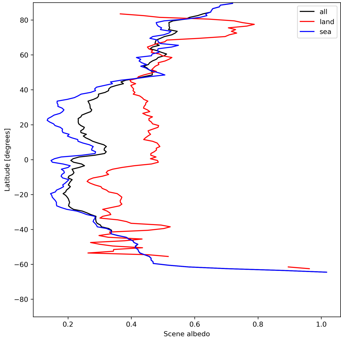
Figure 17: Zonal average of “Scene albedo” for 2023-07-01 to 2023-07-03.
