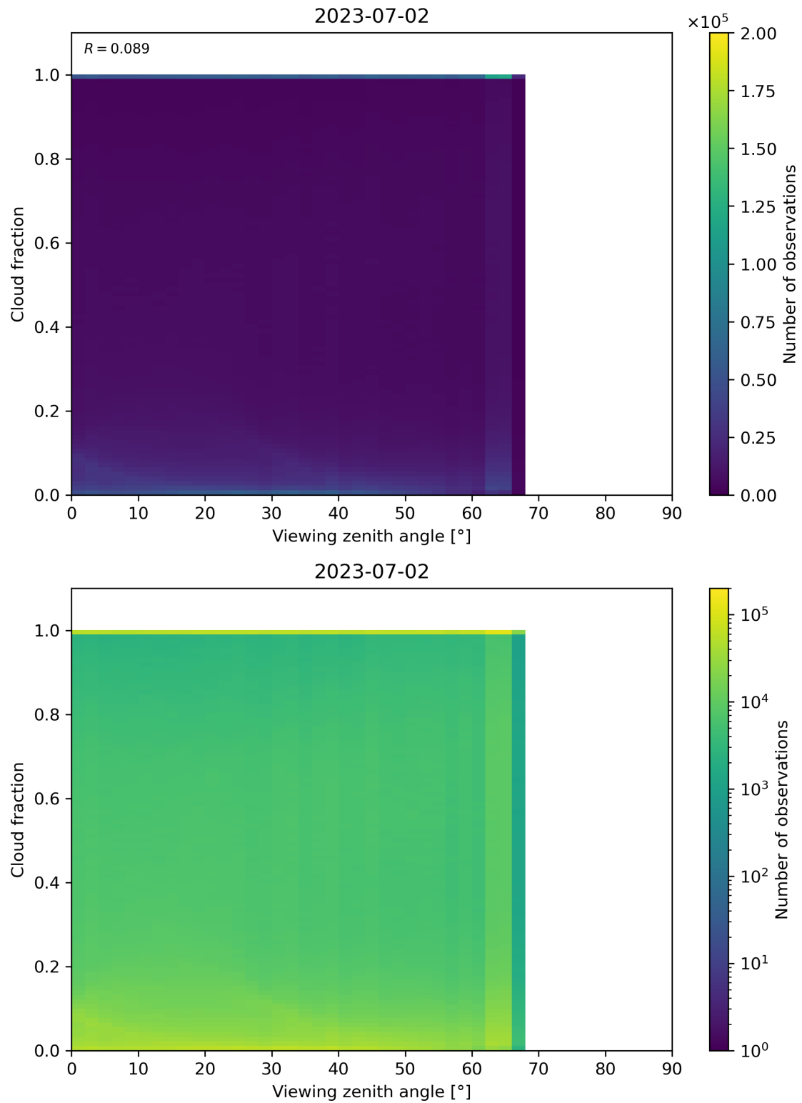
Figure 132: Scatter density plot of “Viewing zenith angle” against “Cloud fraction” for 2023-07-01 to 2023-07-03.
