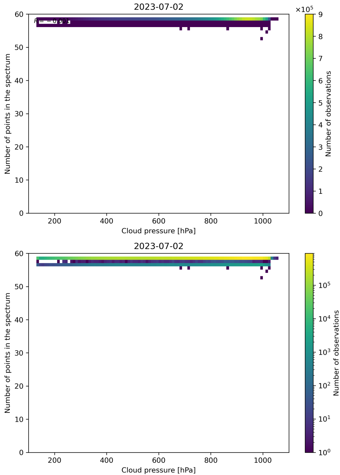
Figure 90: Scatter density plot of “Cloud pressure” against “Number of points in the spectrum” for 2023-07-01 to 2023-07-03.
