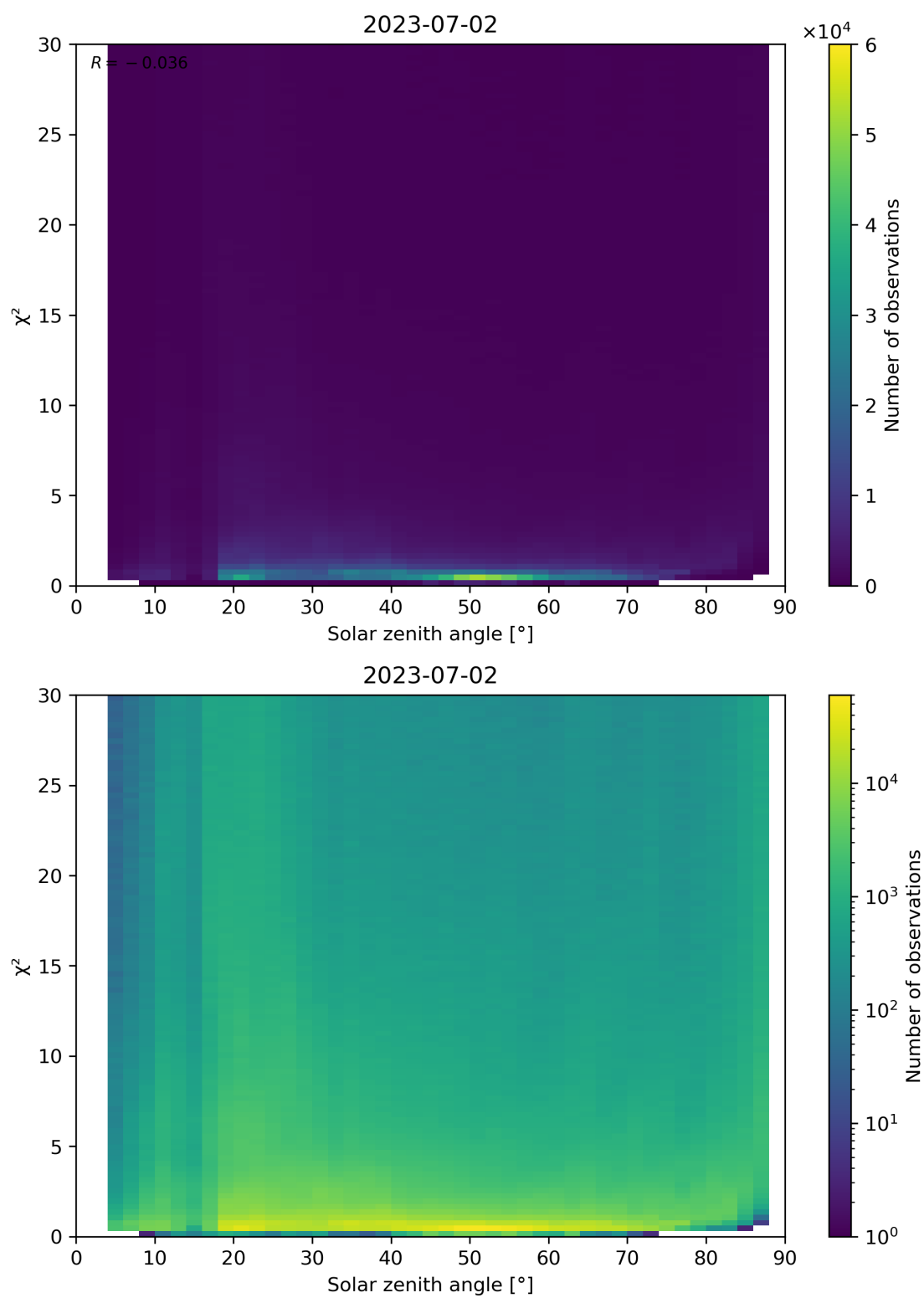
Figure 119: Scatter density plot of “Solar zenith angle” against “ \chi^2 ” for 2023-07-01 to 2023-07-03.
