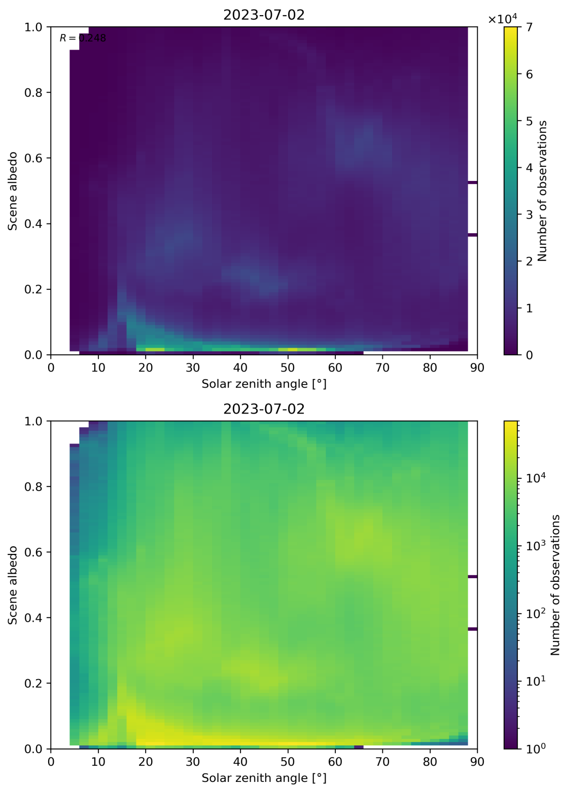
Figure 127: Scatter density plot of “Solar zenith angle” against “Scene albedo” for 2023-07-01 to 2023-07-03.
