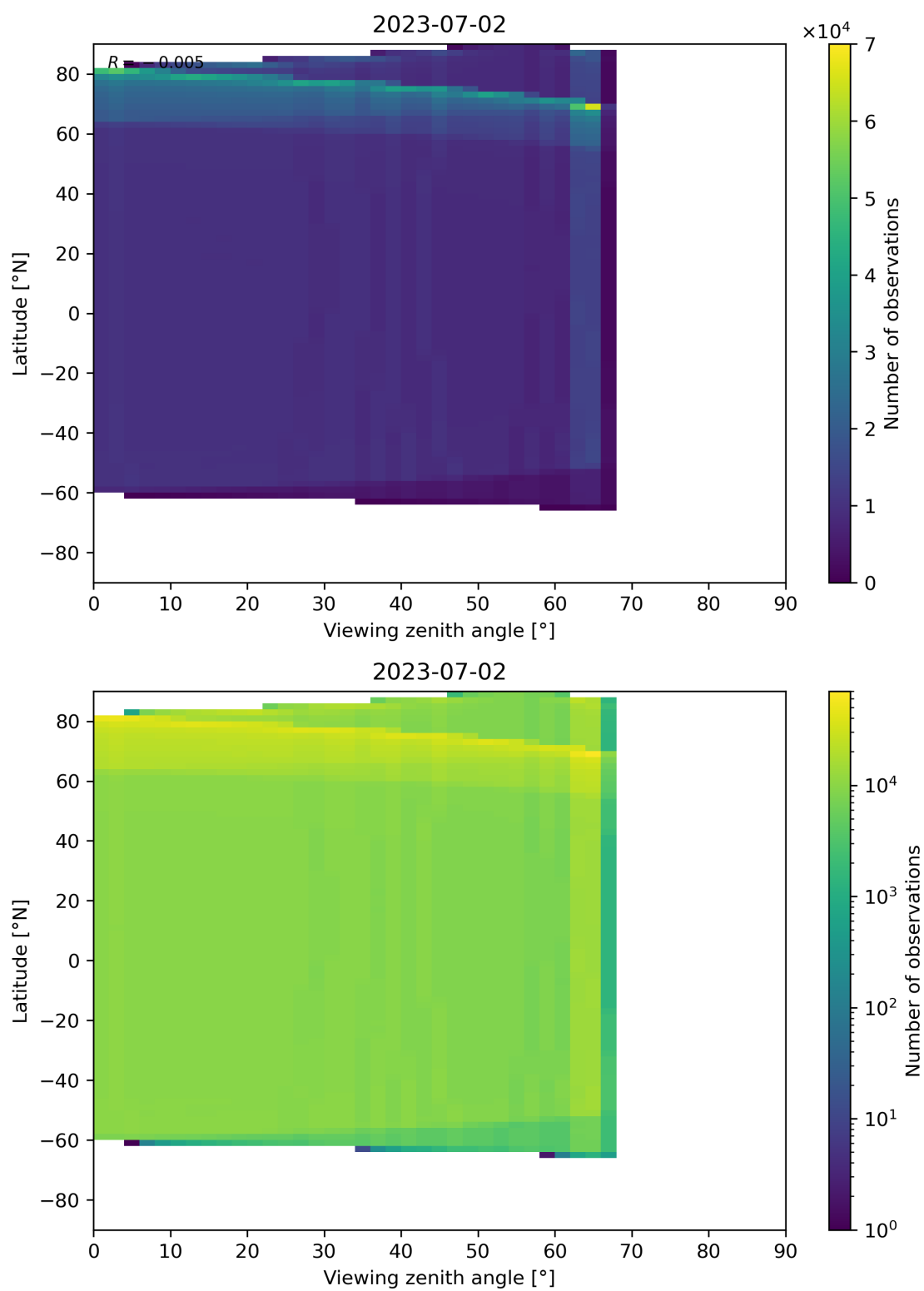
Figure 135: Scatter density plot of “Viewing zenith angle” against “Latitude” for 2023-07-01 to 2023-07-03.
