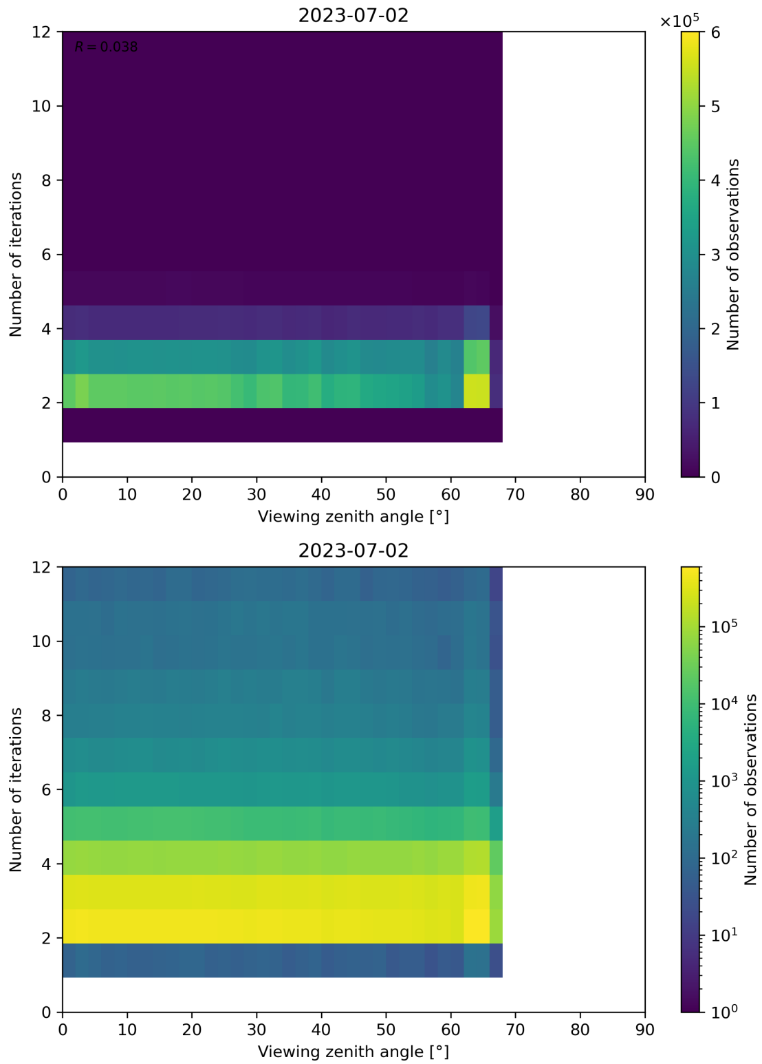
Figure 136: Scatter density plot of “Viewing zenith angle” against “Number of iterations” for 2023-07-01 to 2023-07-03.
