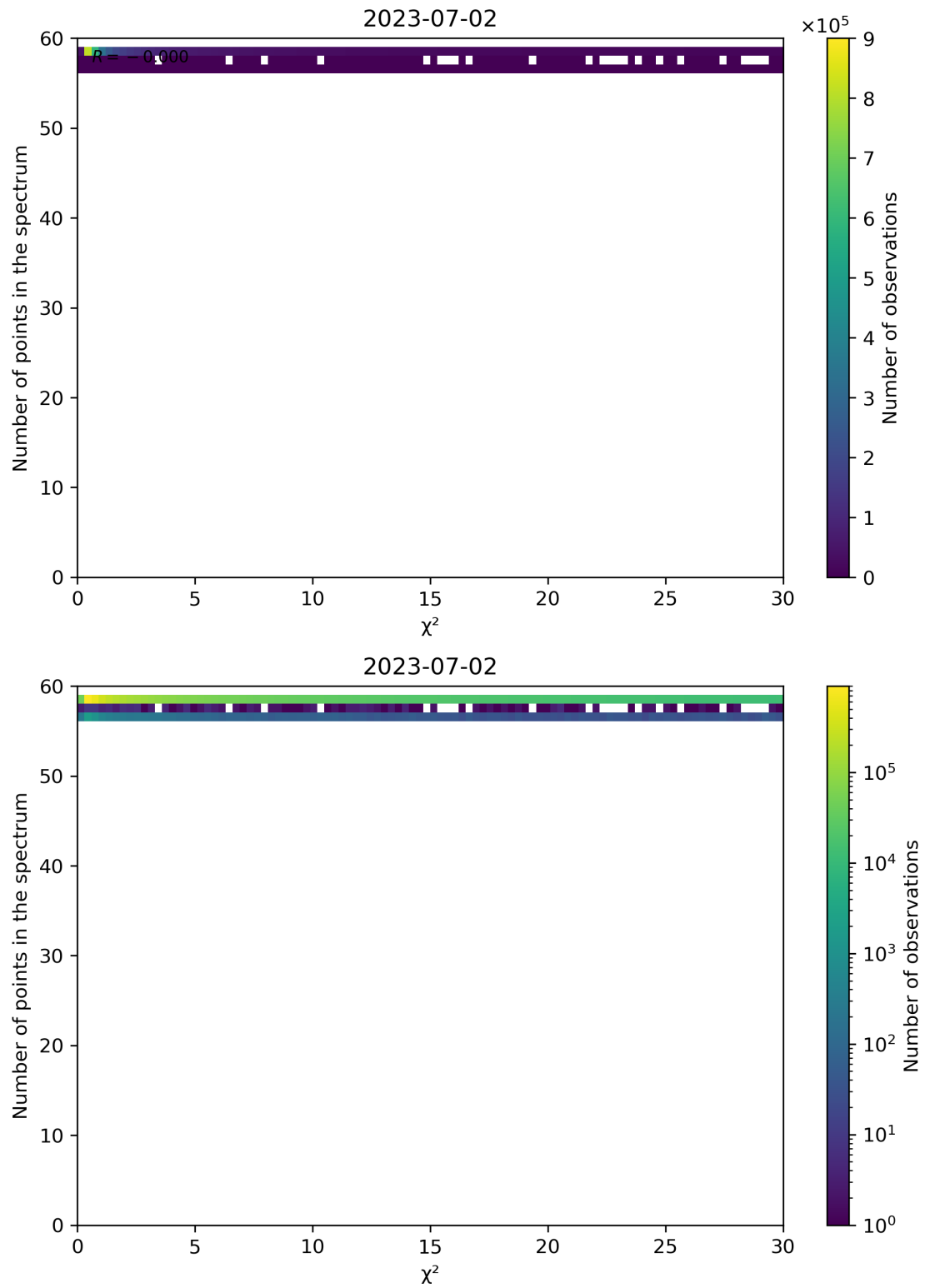
Figure 74: Scatter density plot of “ \chi^2 ” against “Number of points in the spectrum” for 2023-07-01 to 2023-07-03.
