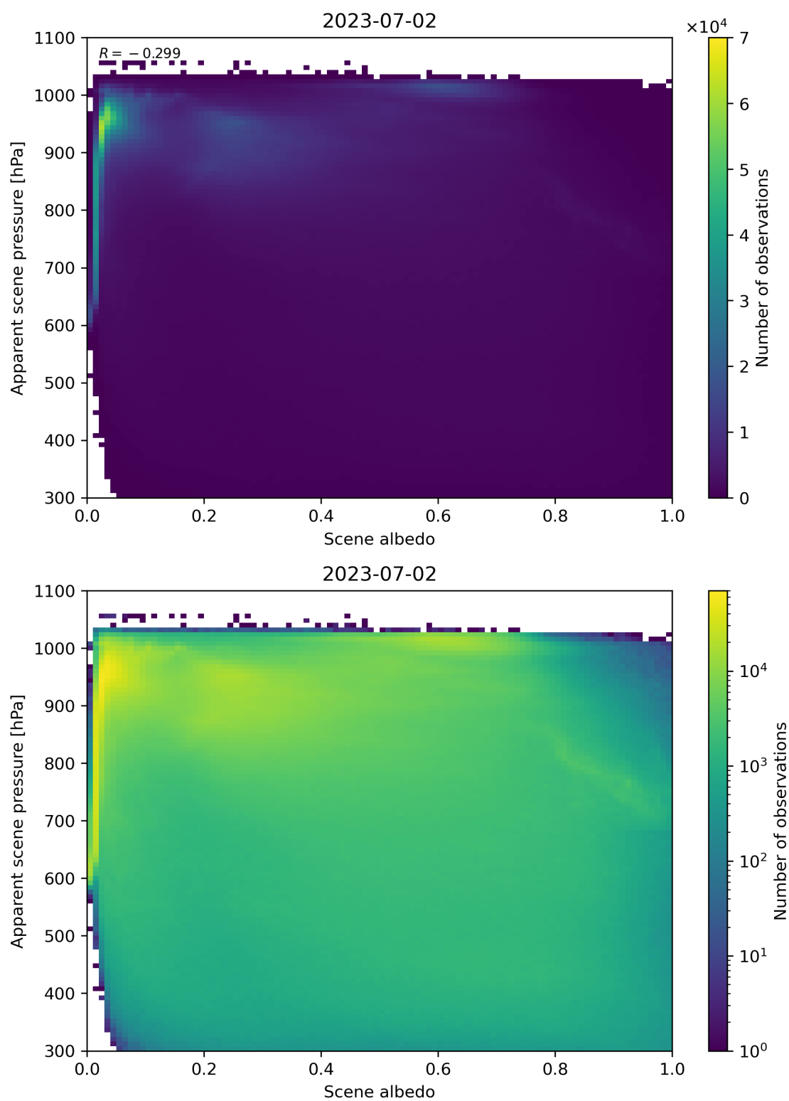
Figure 111: Scatter density plot of “Scene albedo” against “Apparent scene pressure” for 2023-07-01 to 2023-07-03.
