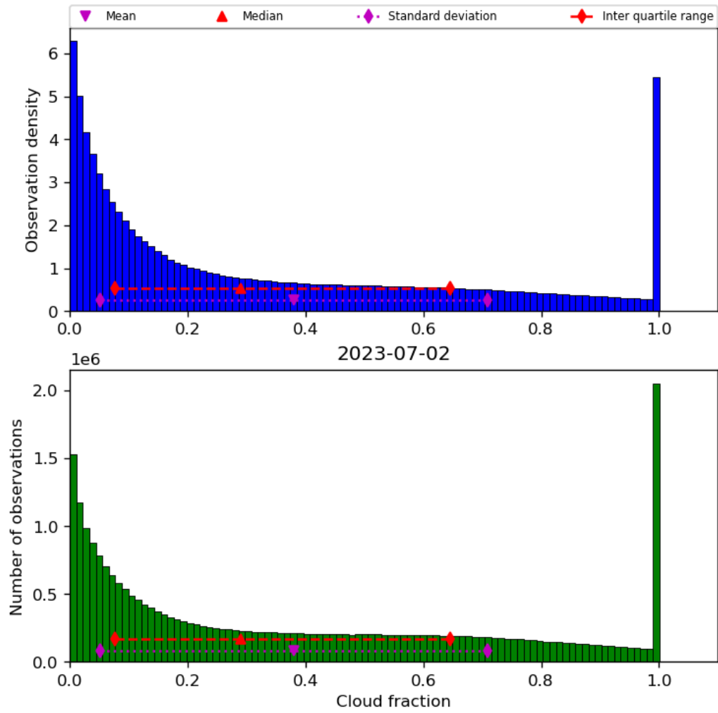
Figure 32: Histogram of “Cloud fraction” for 2023-07-01 to 2023-07-03
