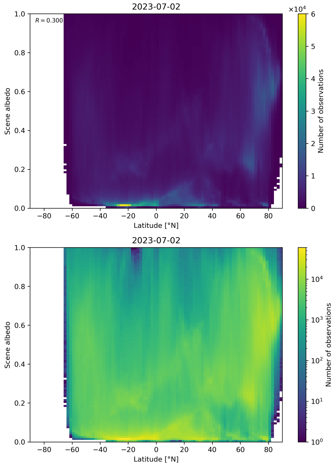
Figure 104: Scatter density plot of “Latitude” against “Scene albedo” for 2023-07-01 to 2023-07-03.
