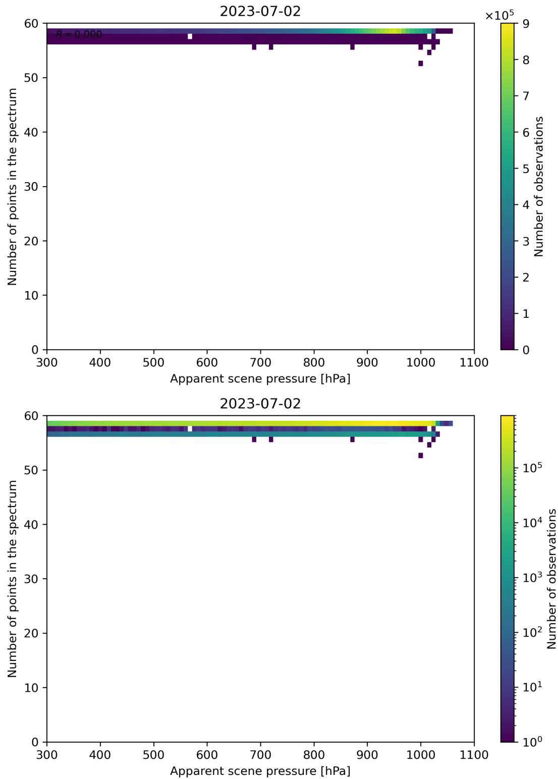
Figure 67: Scatter density plot of “Apparent scene pressure” against “Number of points in the spectrum” for 2023-07-01 to 2023-07-03.
