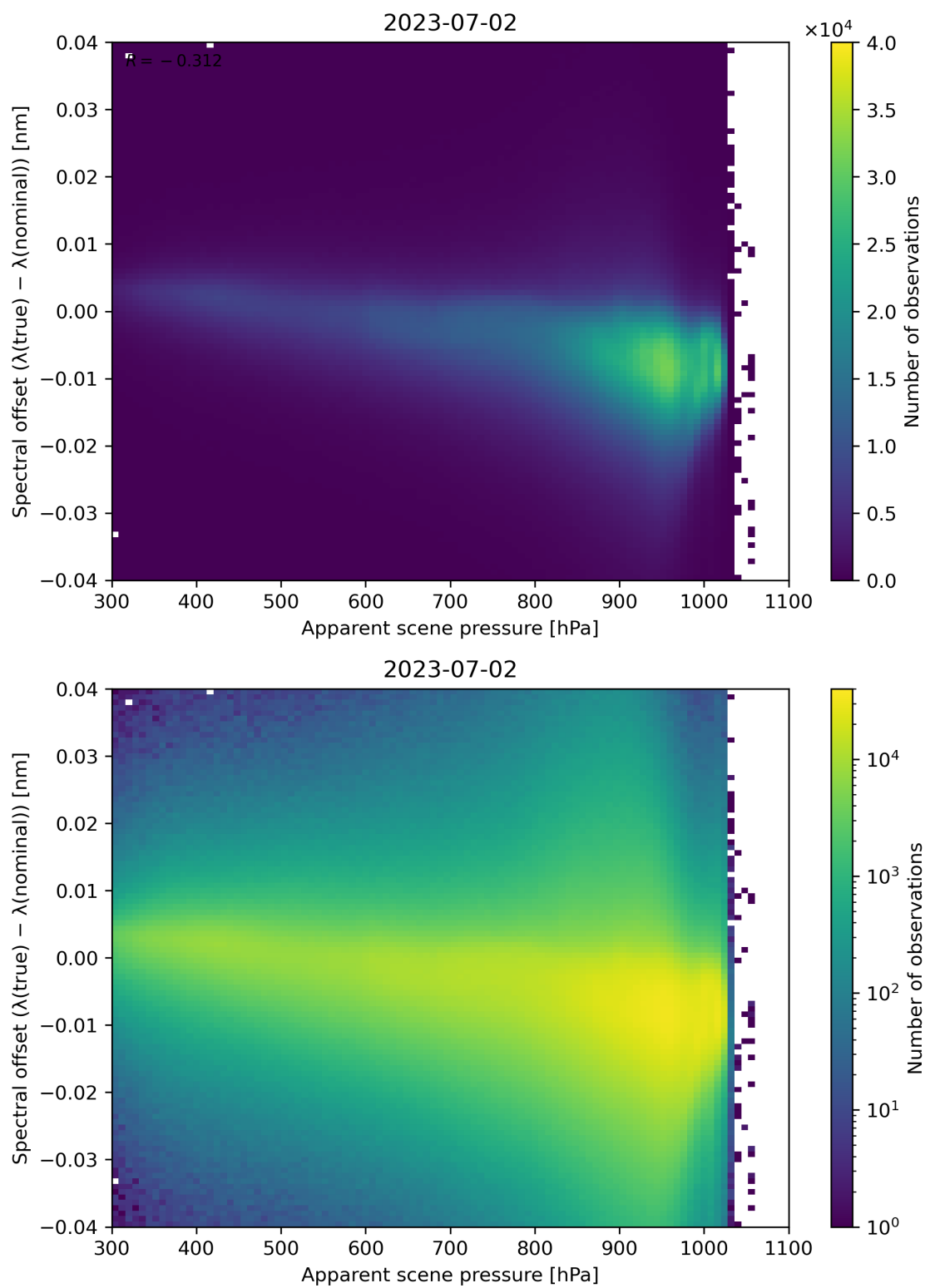
Figure 68: Scatter density plot of “Apparent scene pressure” against “Spectral offset ( \lambda(\text{true}) - \lambda(\text{nominal}) )” for 2023-07-01 to 2023-07-03.
