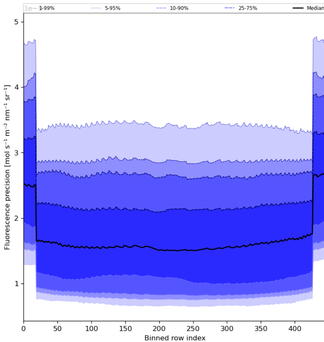
Figure 58: Along track statistics of “Fluorescence precision” for 2023-07-01 to 2023-07-03
