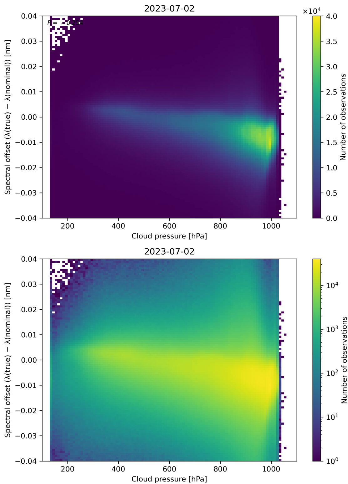
Figure 92: Scatter density plot of “Cloud pressure” against “Spectral offset ( \lambda(\text{true}) - \lambda(\text{nominal}) )” for 2023-07-01 to 2023-07-03.
