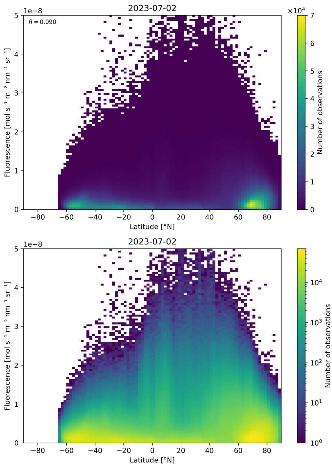
Figure 101: Scatter density plot of “Latitude” against “Fluorescence” for 2023-07-01 to 2023-07-03.
