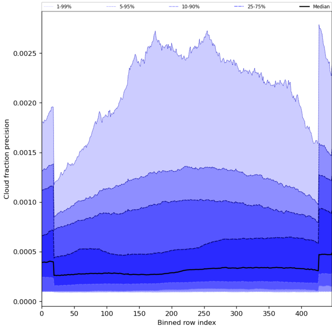
Figure 50: Along track statistics of “Cloud fraction precision” for 2023-07-01 to 2023-07-03
