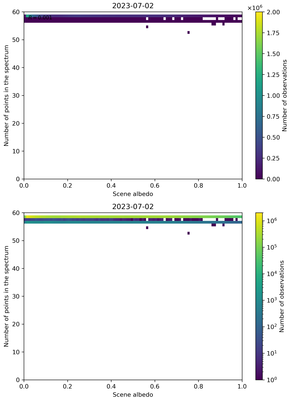
Figure 116: Scatter density plot of “Scene albedo” against “Number of points in the spectrum” for 2023-07-01 to 2023-07-03.
