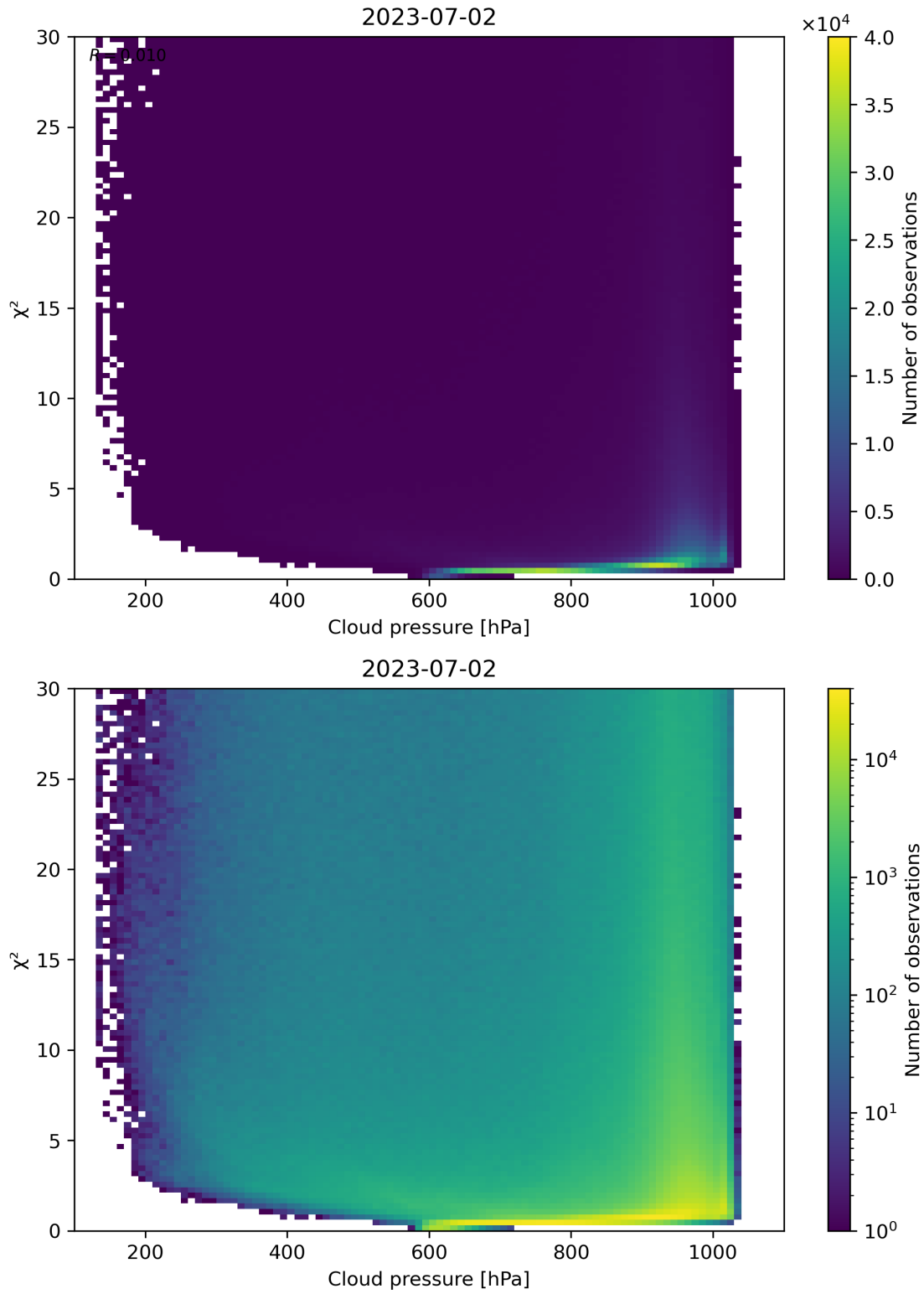
Figure 85: Scatter density plot of “Cloud pressure” against “ \chi^2 ” for 2023-07-01 to 2023-07-03.
