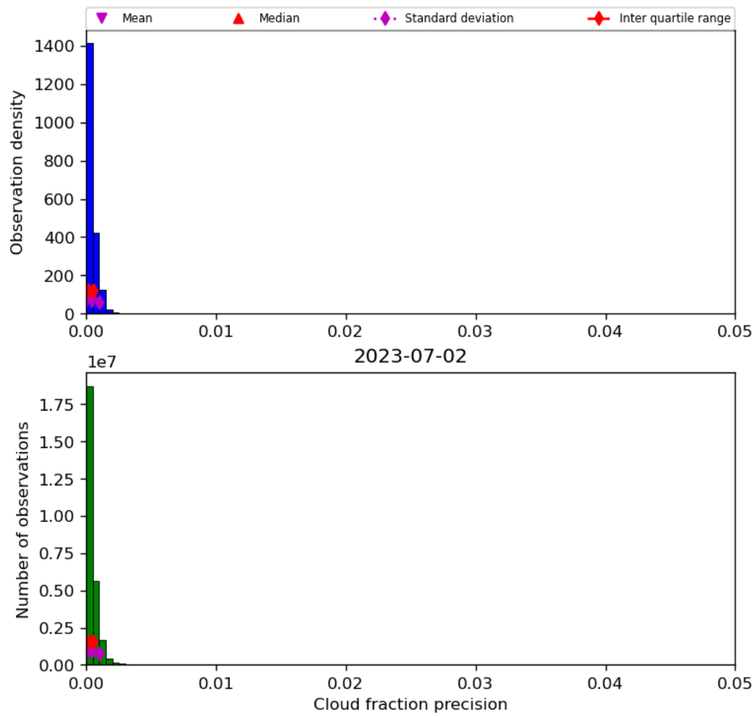
Figure 33: Histogram of “Cloud fraction precision” for 2023-07-01 to 2023-07-03
