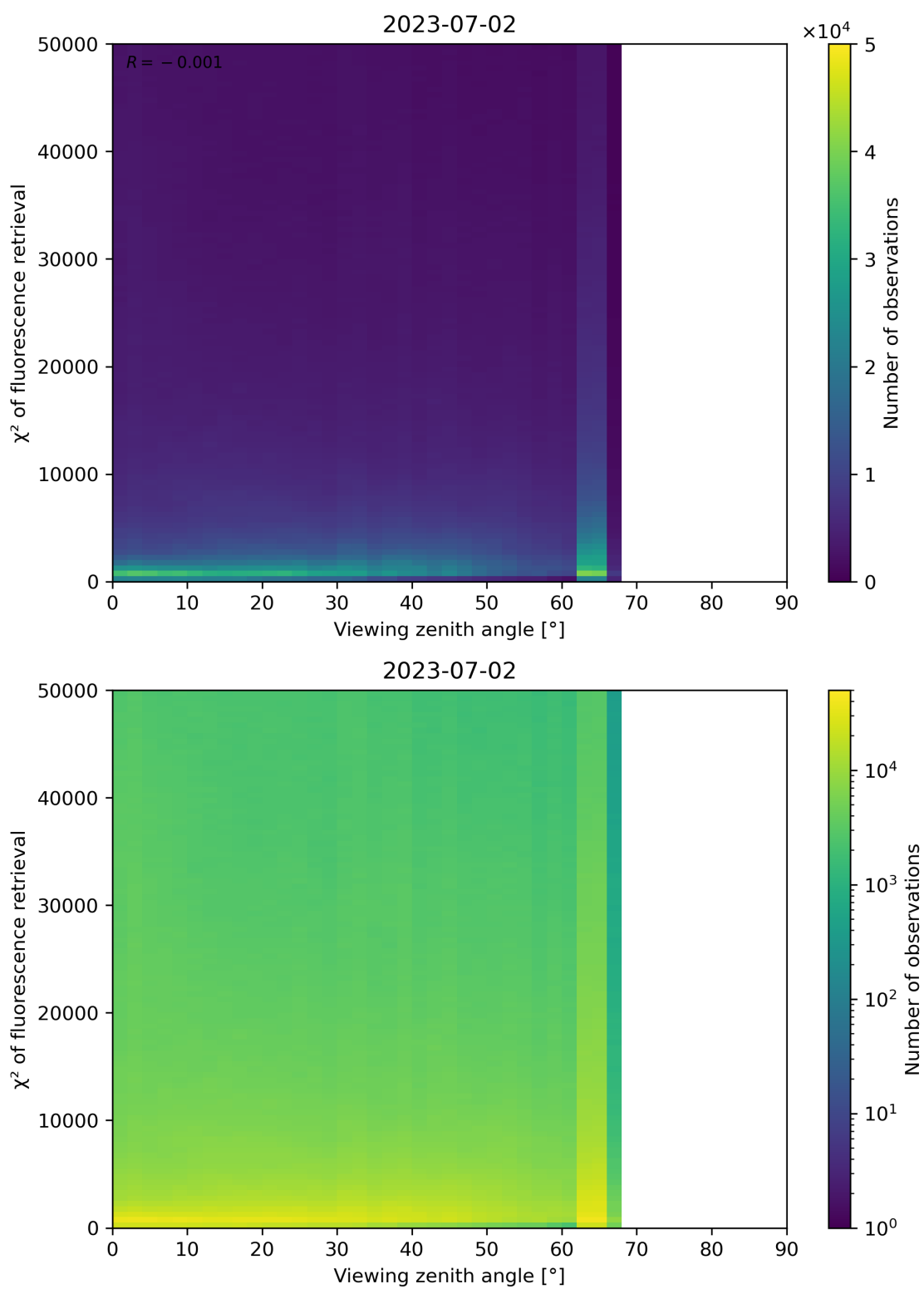
Figure 131: Scatter density plot of “Viewing zenith angle” against “ \chi^2 of fluorescence retrieval” for 2023-07-01 to 2023-07-03.
