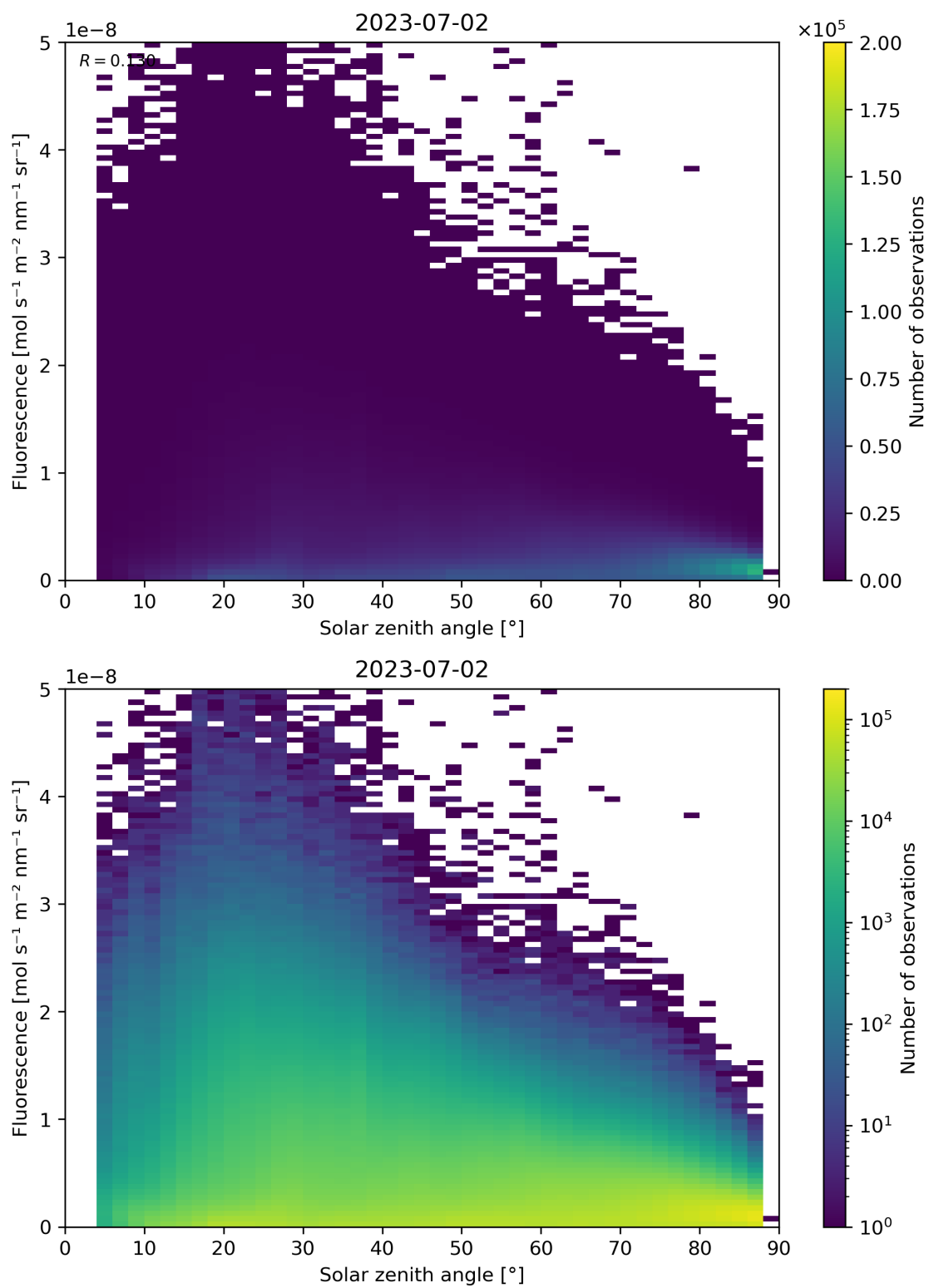
Figure 123: Scatter density plot of “Solar zenith angle” against “Fluorescence” for 2023-07-01 to 2023-07-03.
