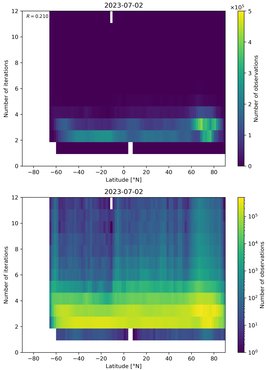
Figure 102: Scatter density plot of “Latitude” against “Number of iterations” for 2023-07-01 to 2023-07-03.
