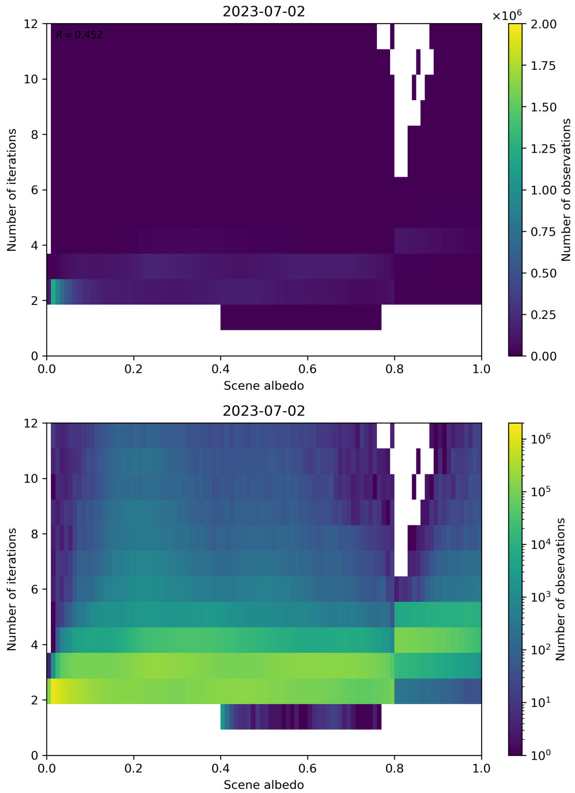
Figure 115: Scatter density plot of “Scene albedo” against “Number of iterations” for 2023-07-01 to 2023-07-03.
