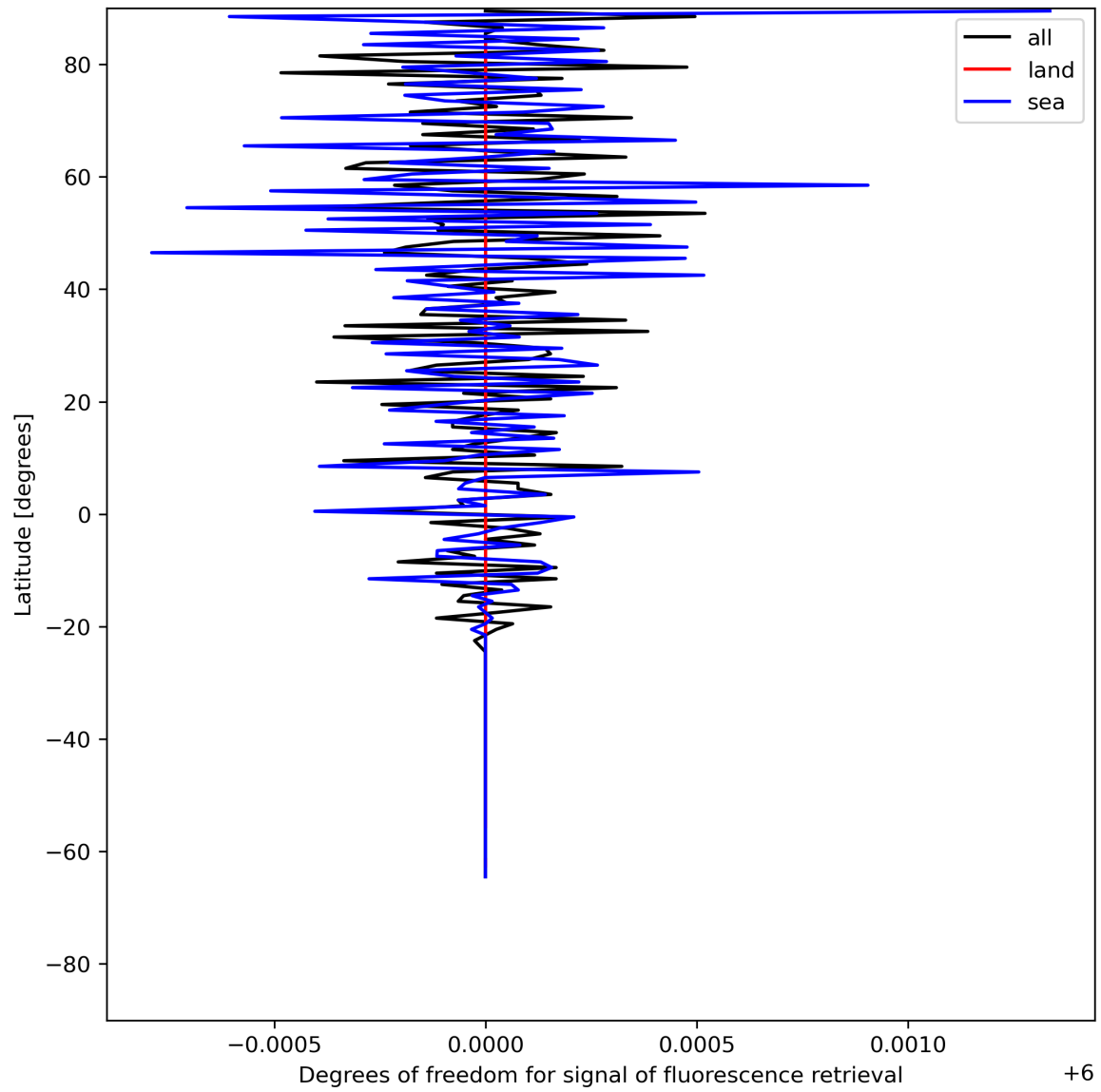
Figure 26: Zonal average of “Degrees of freedom for signal of fluorescence retrieval” for 2023-07-01 to 2023-07-03.
