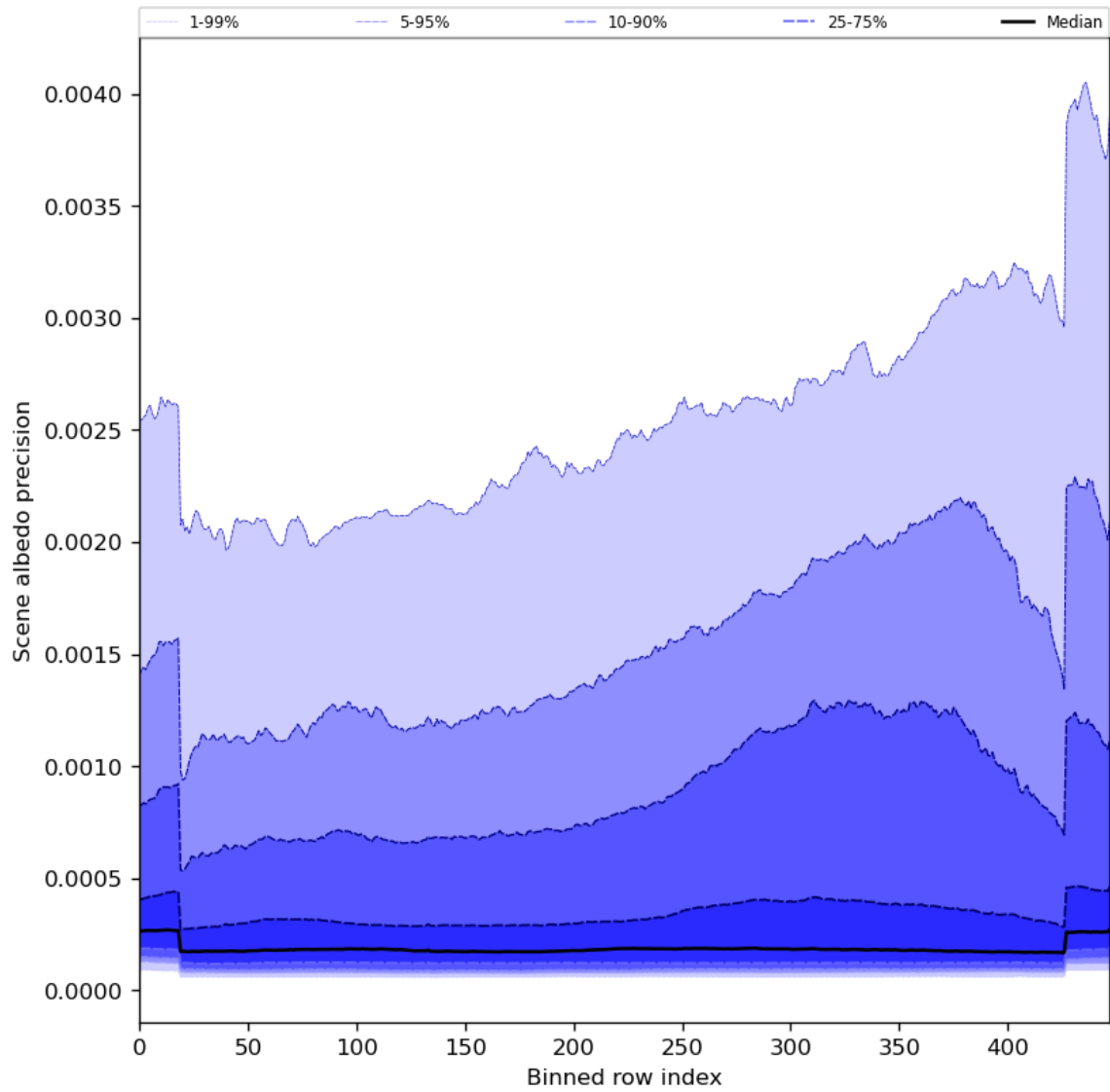
Figure 52: Along track statistics of “Scene albedo precision” for 2023-07-01 to 2023-07-03
