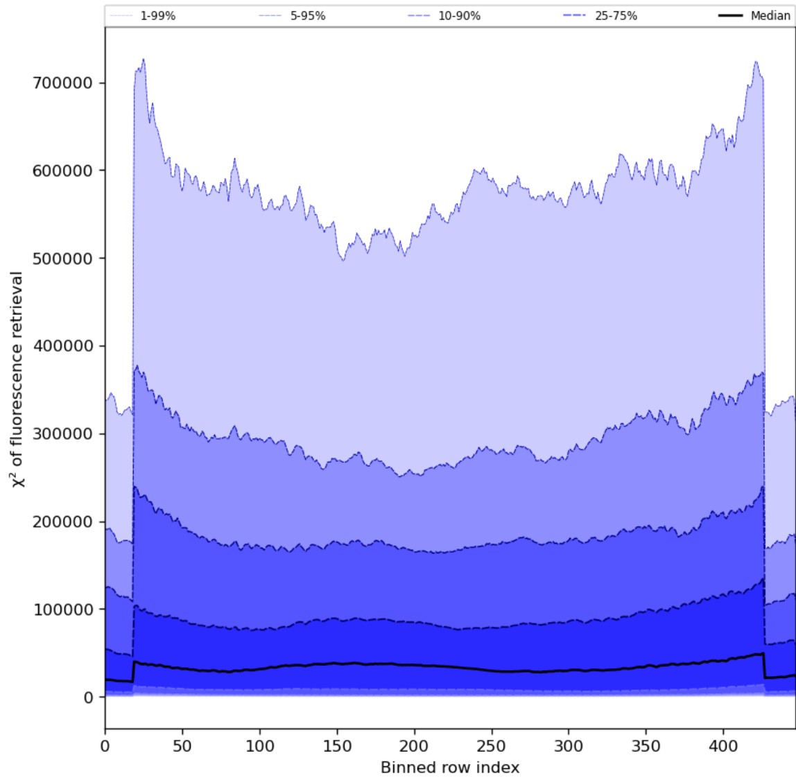
Figure 59: Along track statistics of “ \chi^2 of fluorescence retrieval” for 2023-07-01 to 2023-07-03
