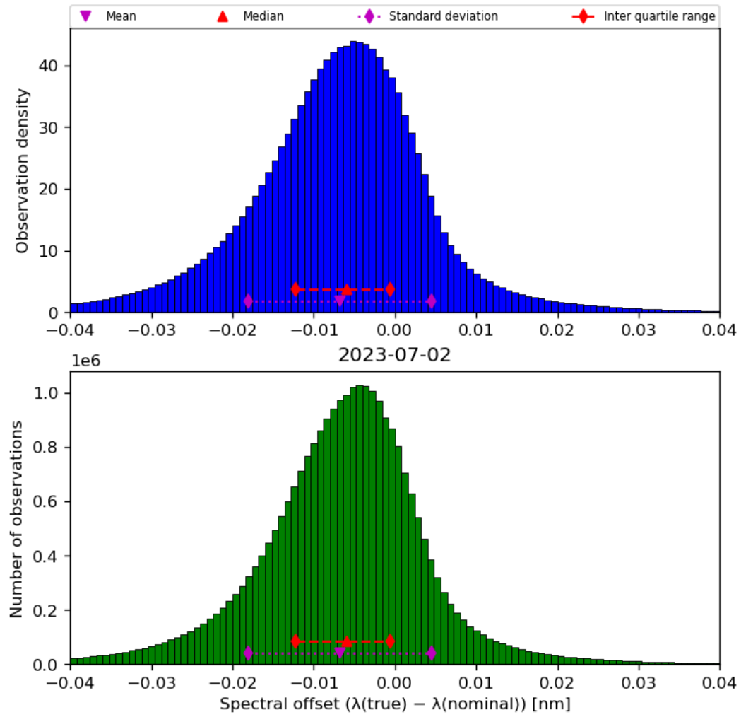
Figure 45: Histogram of “Spectral offset ( \lambda(\text{true}) - \lambda(\text{nominal}) )” for 2023-07-01 to 2023-07-03
