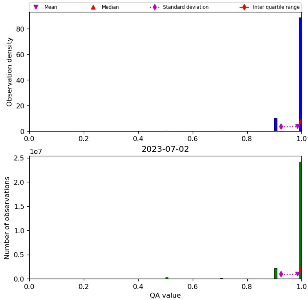
Figure 29: Histogram of “QA value” for 2023-07-01 to 2023-07-03
