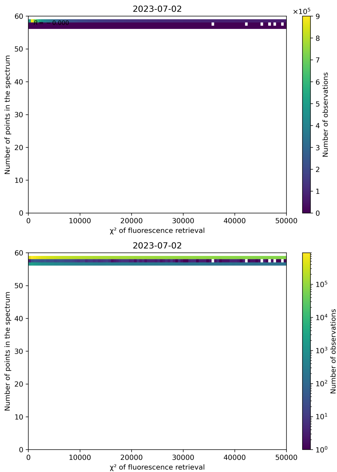
Figure 71: Scatter density plot of " \chi^2 of fluorescence retrieval" against "Number of points in the spectrum" for 2023-07-01 to 2023-07-03.
