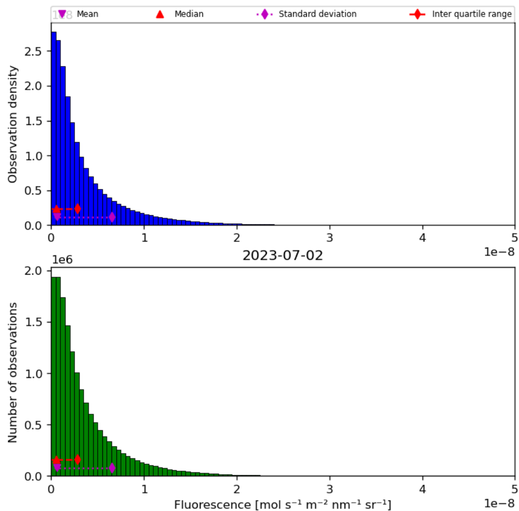
Figure 40: Histogram of “Fluorescence” for 2023-07-01 to 2023-07-03
