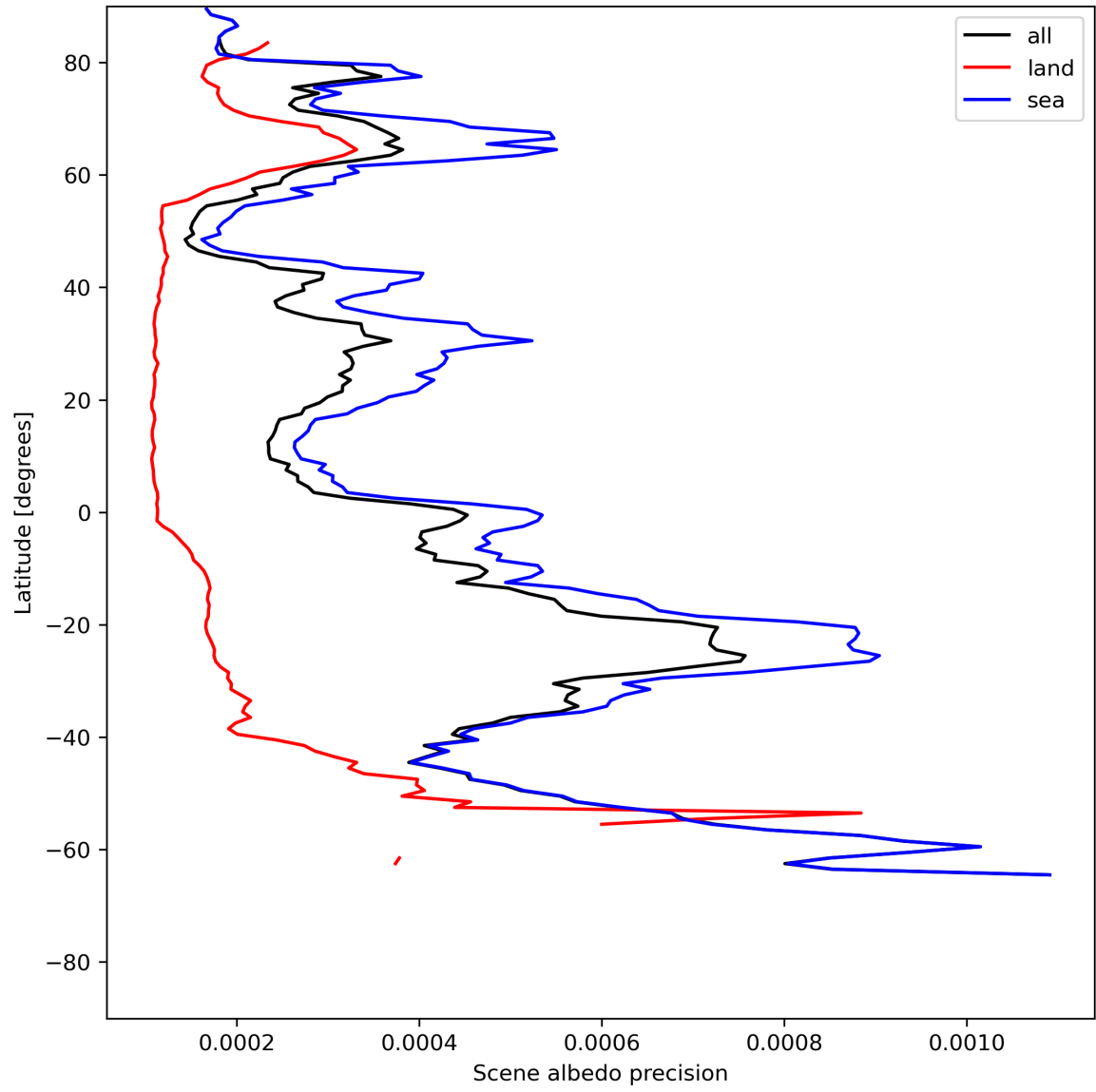
Figure 18: Zonal average of “Scene albedo precision” for 2023-07-01 to 2023-07-03.
