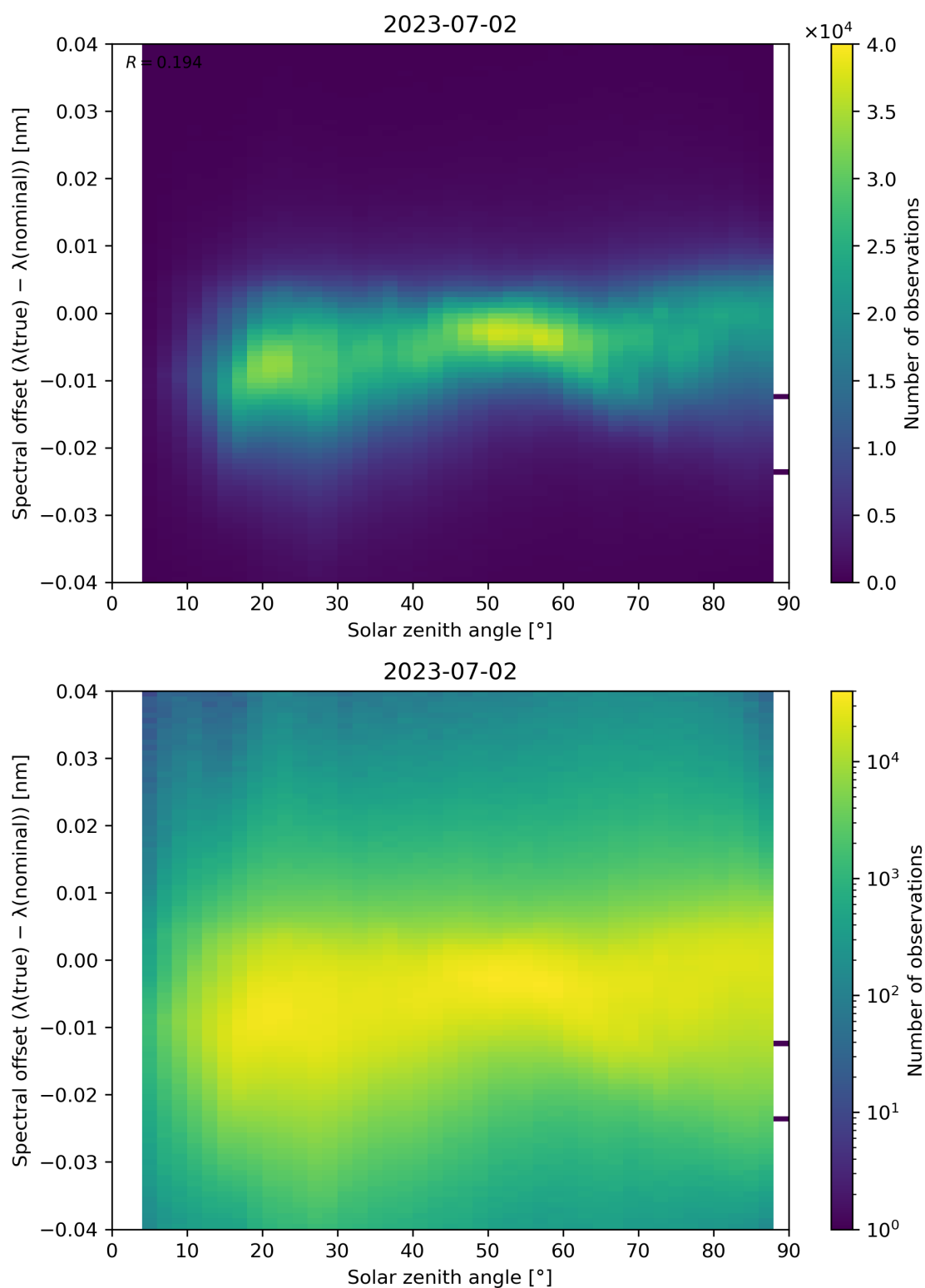
Figure 128: Scatter density plot of “Solar zenith angle” against “Spectral offset ( \lambda(\text{true}) - \lambda(\text{nominal}) )” for 2023-07-01 to 2023-07-03.
