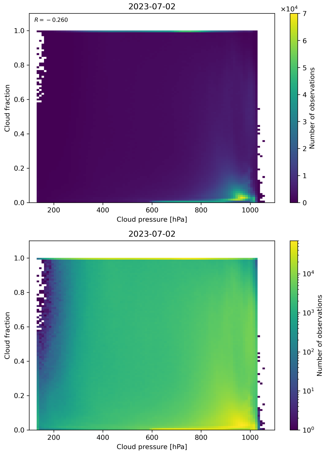
Figure 87: Scatter density plot of “Cloud pressure” against “Cloud fraction” for 2023-07-01 to 2023-07-03.
