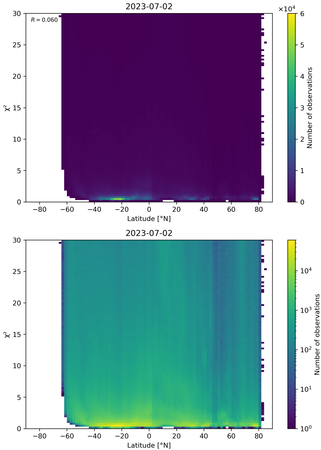
Figure 97: Scatter density plot of “Latitude” against “ \chi^2 ” for 2023-07-01 to 2023-07-03.
