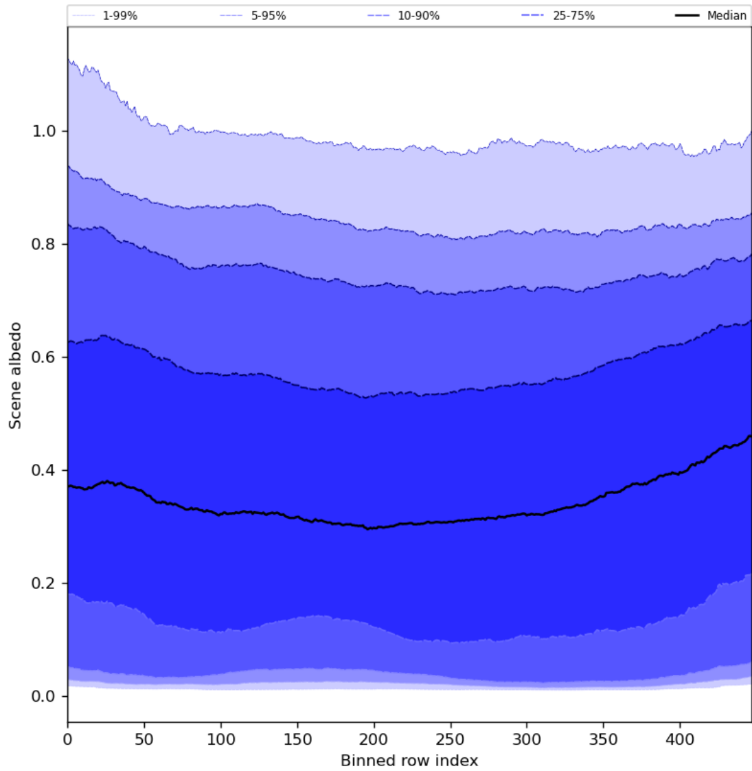
Figure 51: Along track statistics of “Scene albedo” for 2023-07-01 to 2023-07-03
