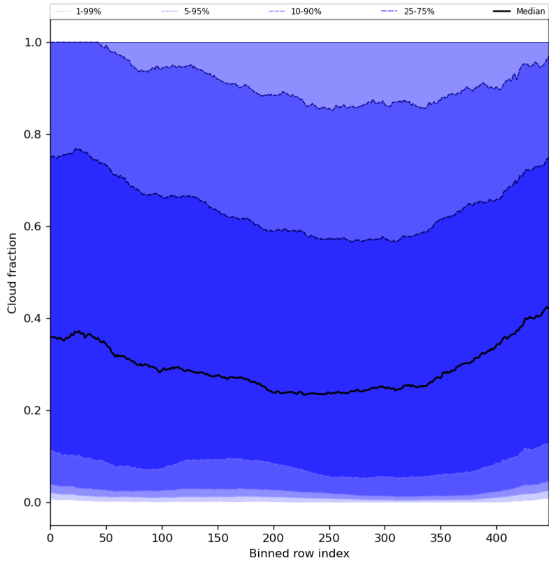
Figure 49: Along track statistics of “Cloud fraction” for 2023-07-01 to 2023-07-03
