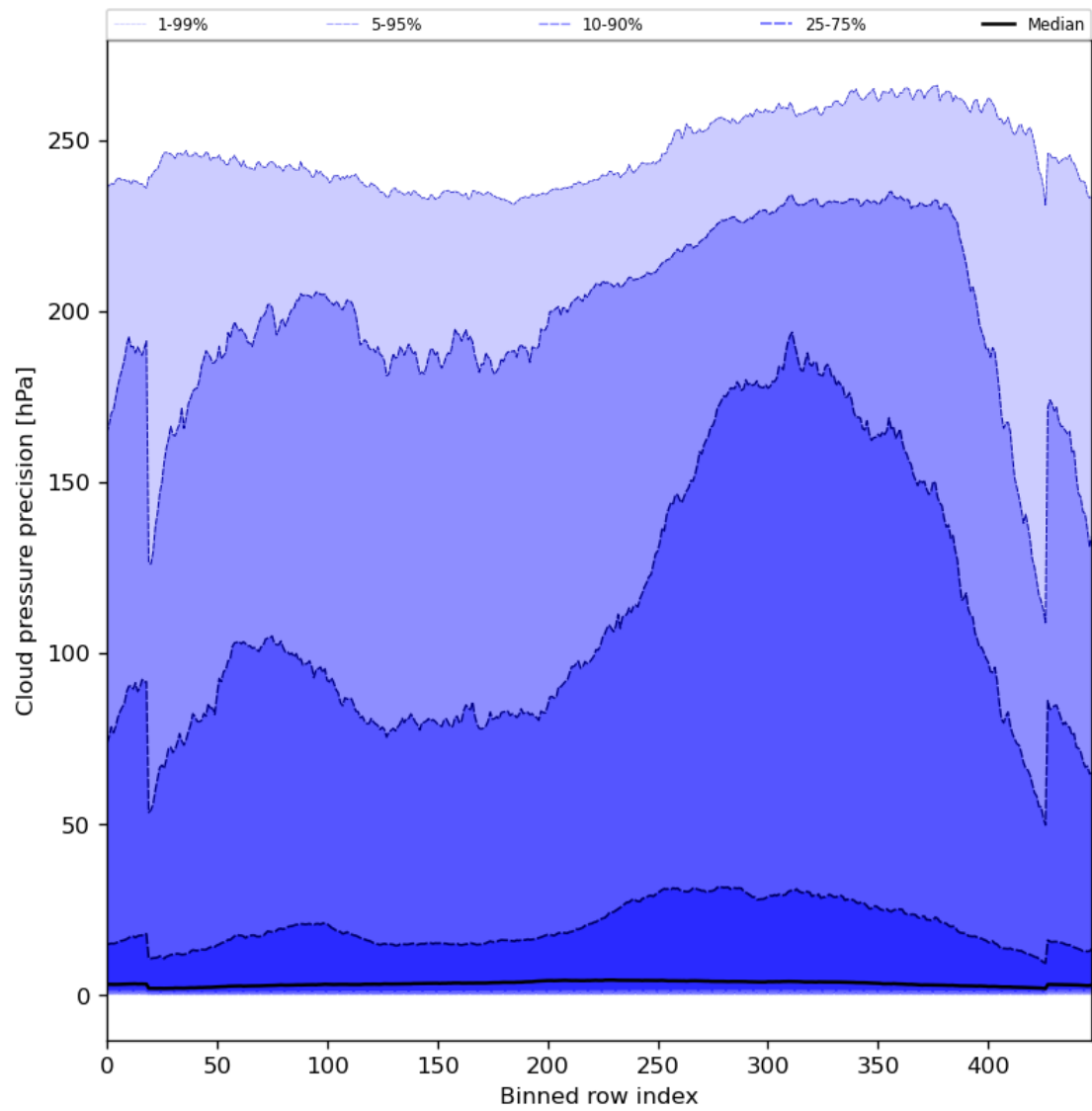
Figure 48: Along track statistics of “Cloud pressure precision” for 2023-07-01 to 2023-07-03
