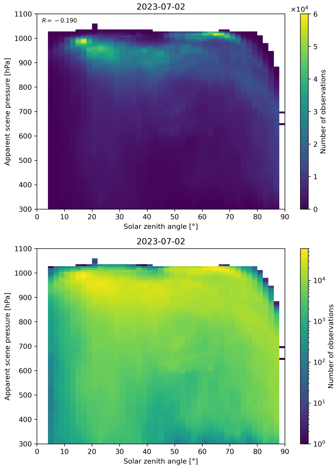
Figure 118: Scatter density plot of “Solar zenith angle” against “Apparent scene pressure” for 2023-07-01 to 2023-07-03.
