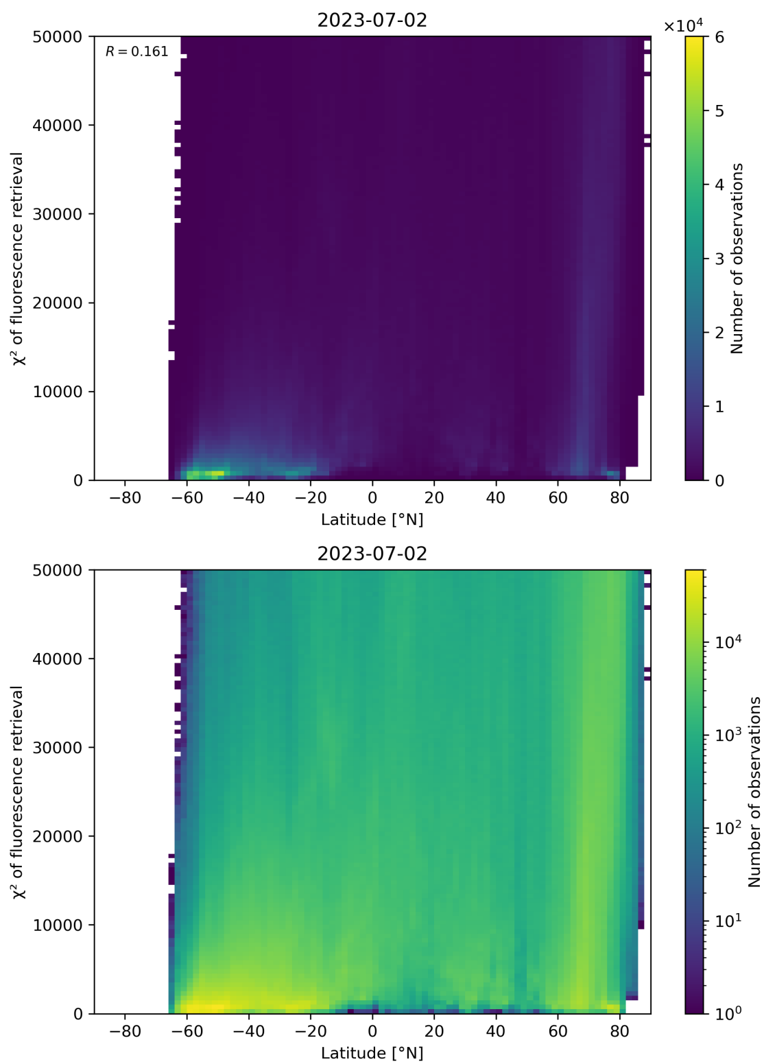
Figure 98: Scatter density plot of “Latitude” against “ \chi^2 of fluorescence retrieval” for 2023-07-01 to 2023-07-03.
