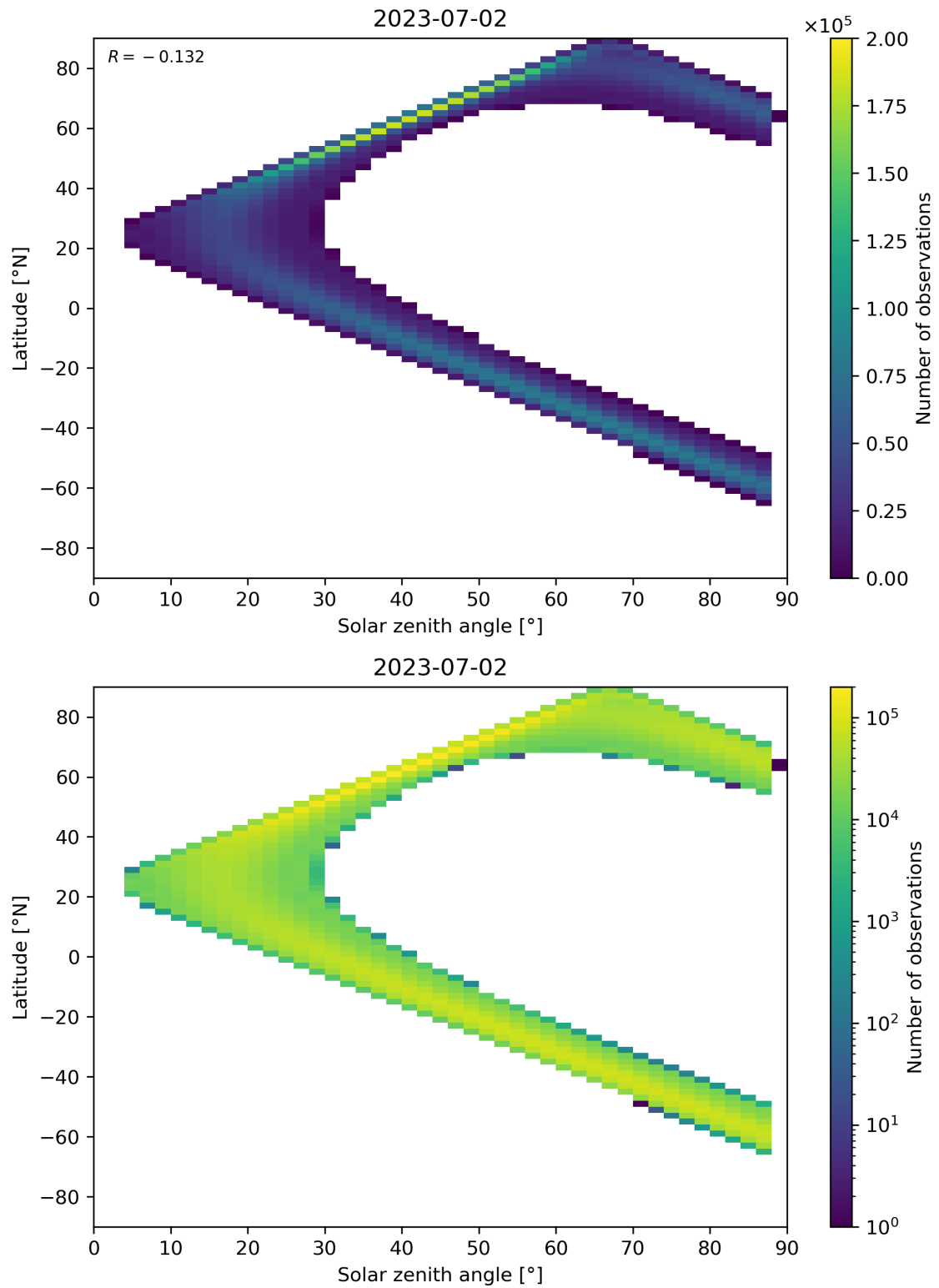
Figure 124: Scatter density plot of “Solar zenith angle” against “Latitude” for 2023-07-01 to 2023-07-03.
