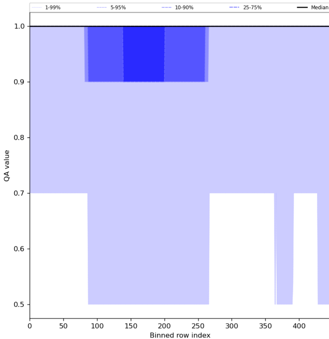
Figure 46: Along track statistics of “QA value” for 2023-07-01 to 2023-07-03
