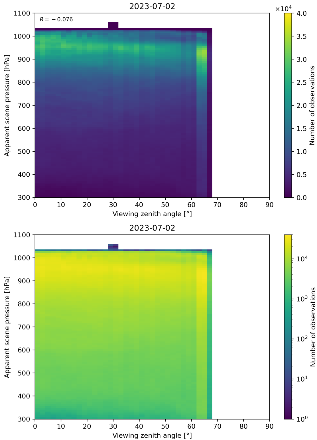
Figure 129: Scatter density plot of “Viewing zenith angle” against “Apparent scene pressure” for 2023-07-01 to 2023-07-03.
