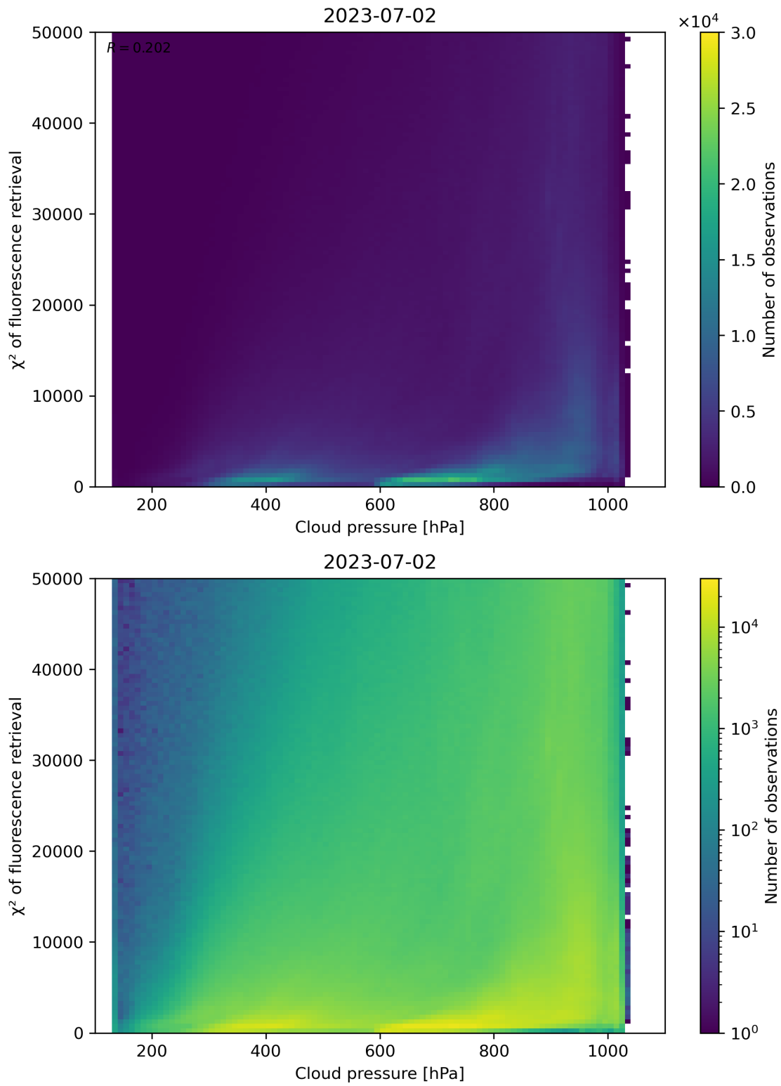
Figure 86: Scatter density plot of “Cloud pressure” against “ \chi^2 of fluorescence retrieval” for 2023-07-01 to 2023-07-03.
