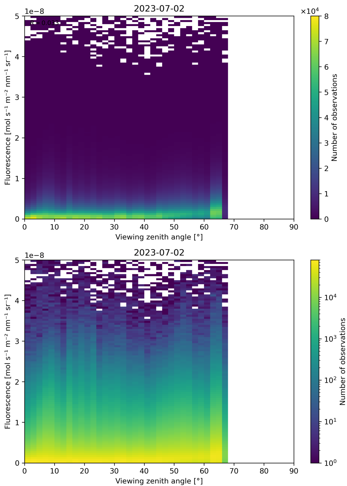
Figure 134: Scatter density plot of “Viewing zenith angle” against “Fluorescence” for 2023-07-01 to 2023-07-03.
