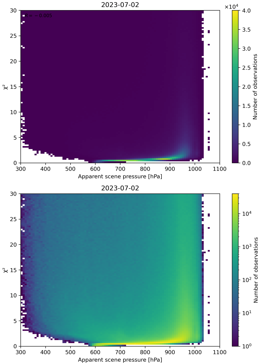
Figure 63: Scatter density plot of “Apparent scene pressure” against “ \chi^2 ” for 2023-07-01 to 2023-07-03.
