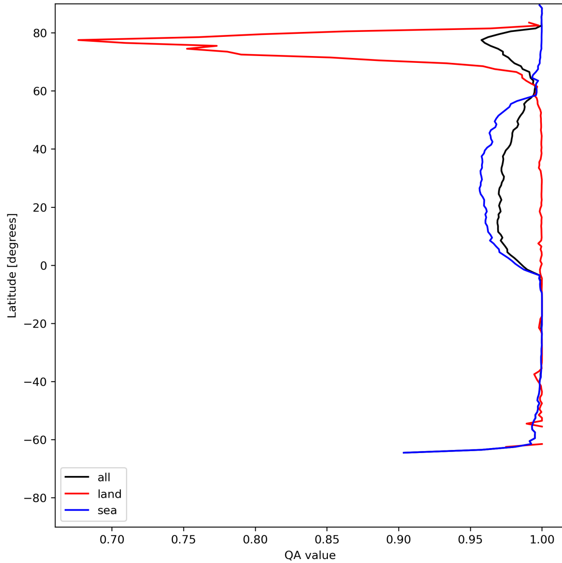
Figure 12: Zonal average of “QA value” for 2023-07-01 to 2023-07-03.
