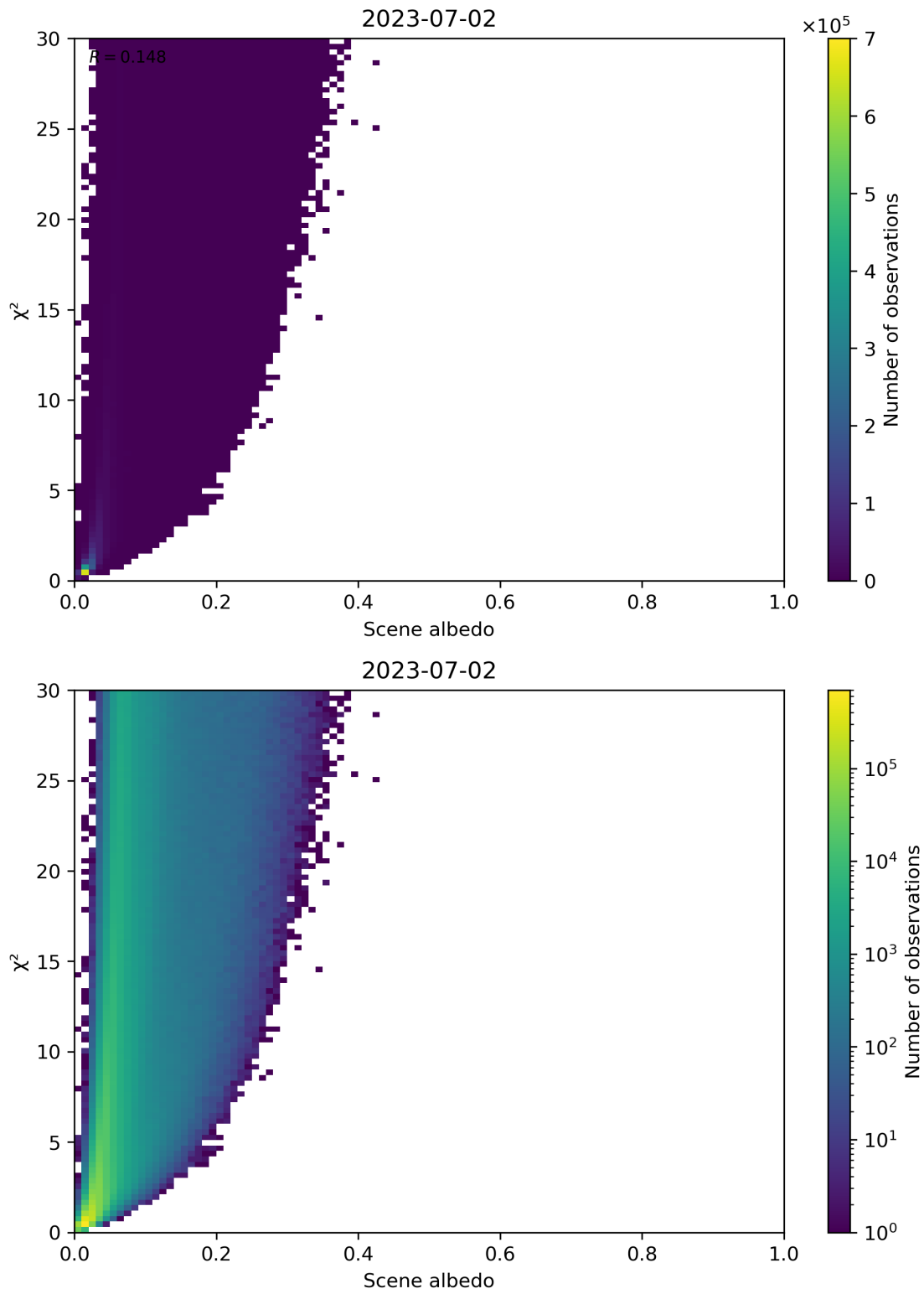
Figure 112: Scatter density plot of “Scene albedo” against “ \chi^2 ” for 2023-07-01 to 2023-07-03.
