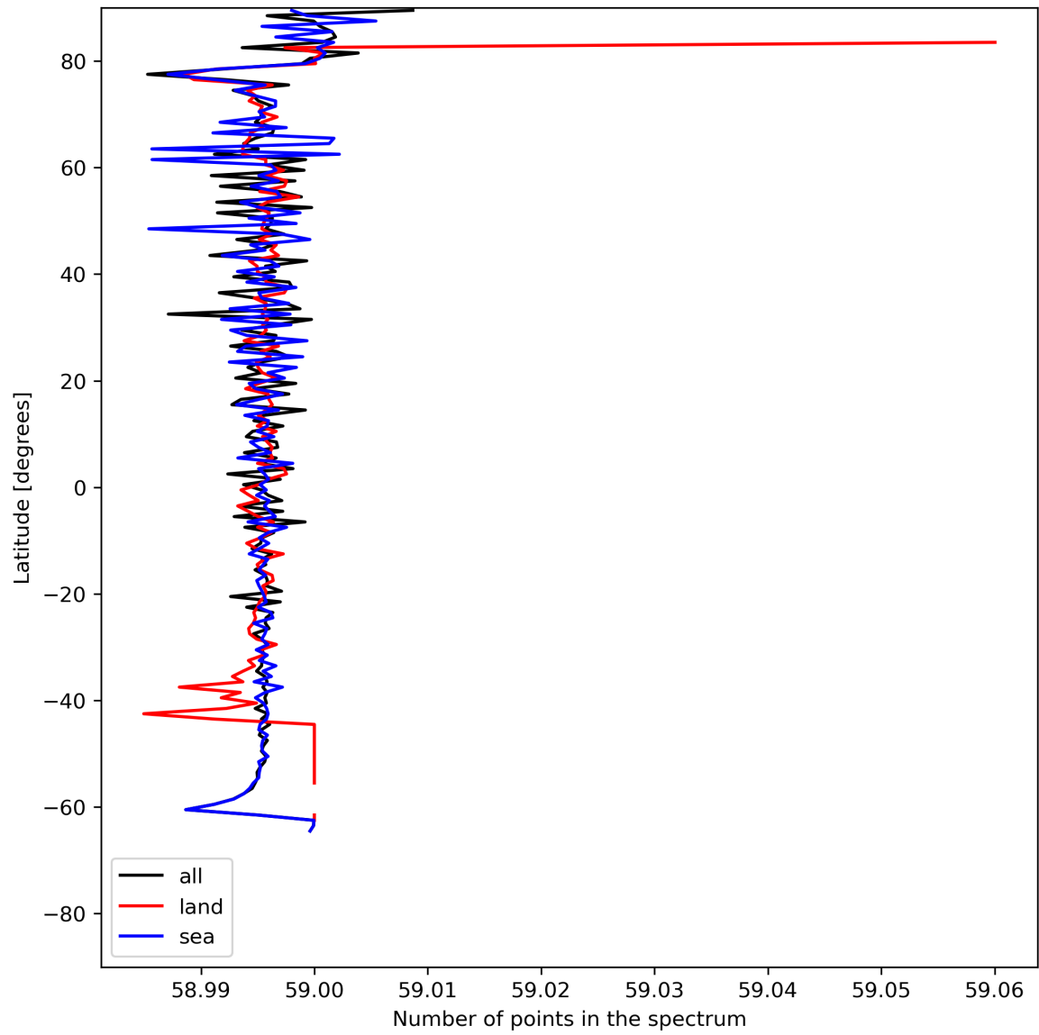
Figure 27: Zonal average of “Number of points in the spectrum” for 2023-07-01 to 2023-07-03.
