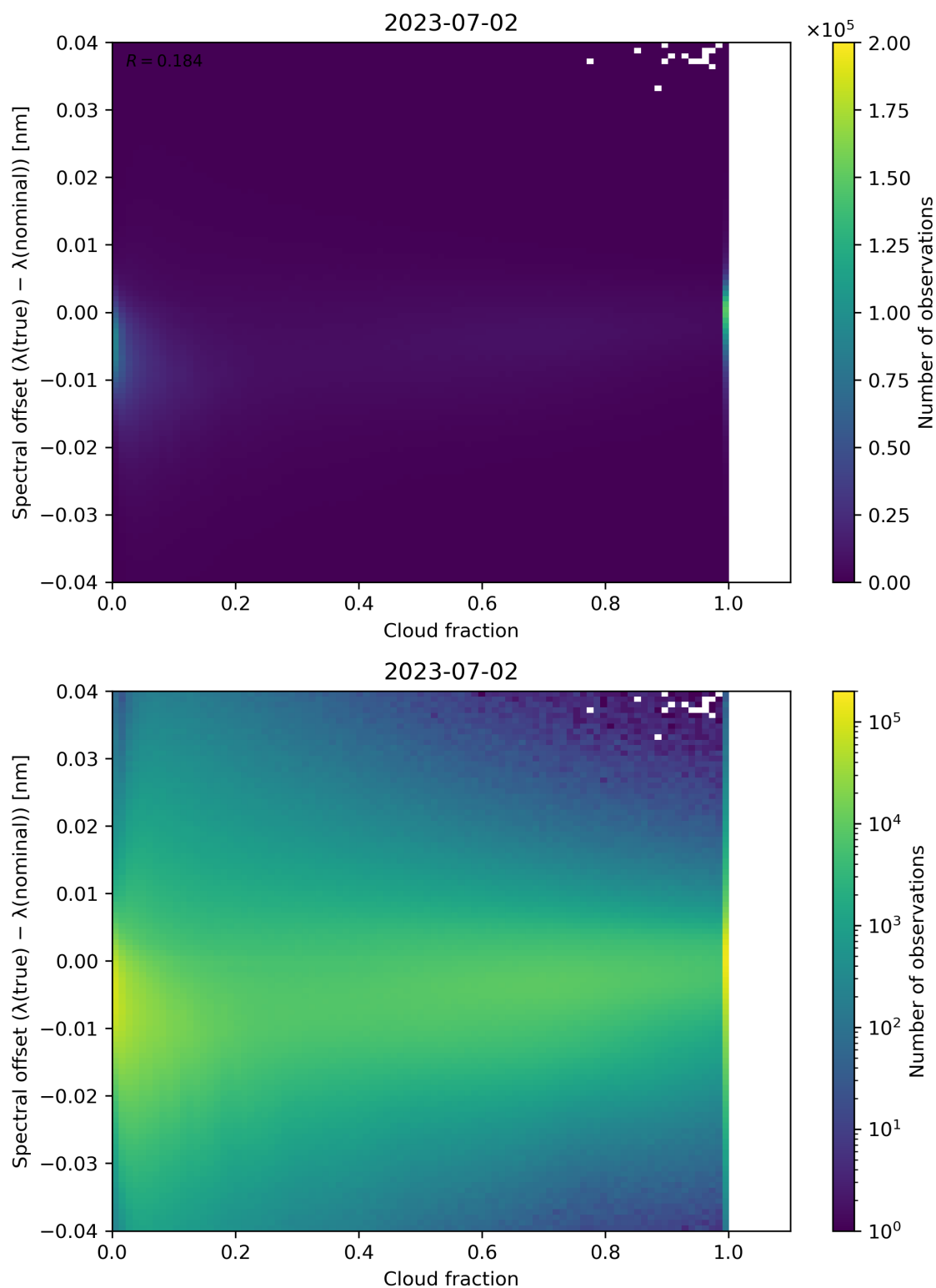
Figure 83: Scatter density plot of “Cloud fraction” against “Spectral offset ( \lambda(\text{true}) - \lambda(\text{nominal}) )” for 2023-07-01 to 2023-07-03.
