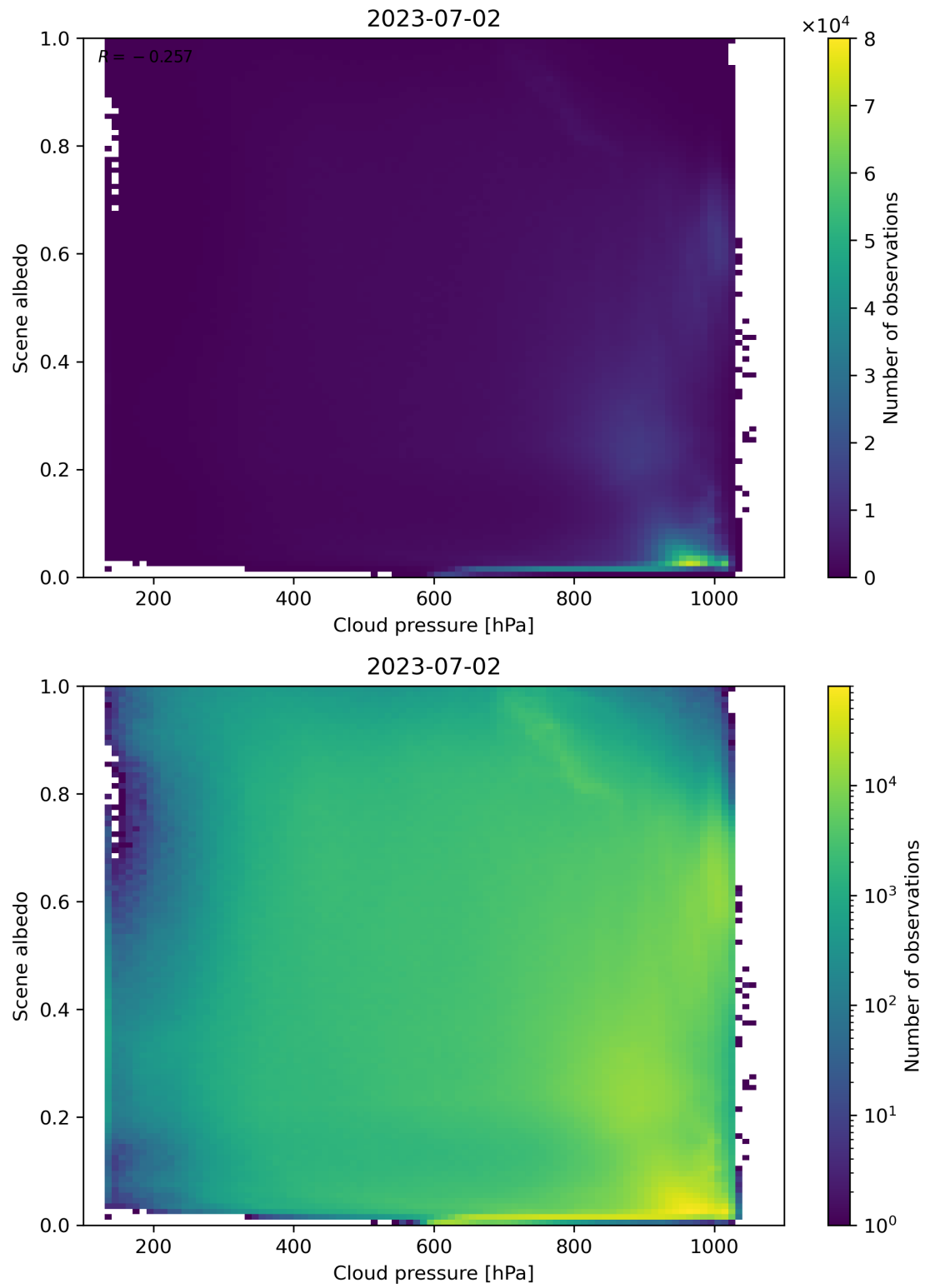
Figure 91: Scatter density plot of “Cloud pressure” against “Scene albedo” for 2023-07-01 to 2023-07-03.
