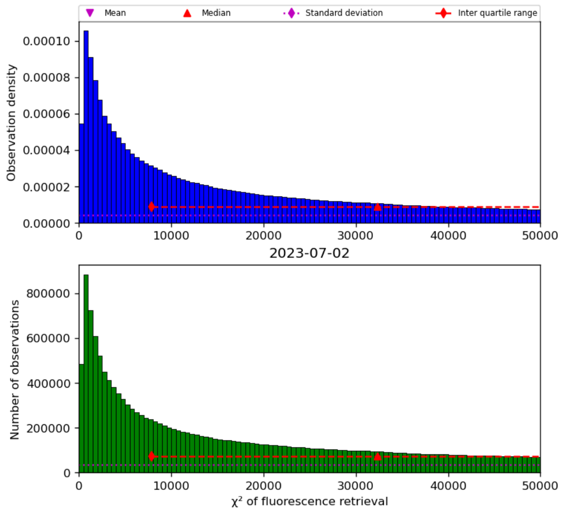
Figure 42: Histogram of “ \chi^2 of fluorescence retrieval” for 2023-07-01 to 2023-07-03
