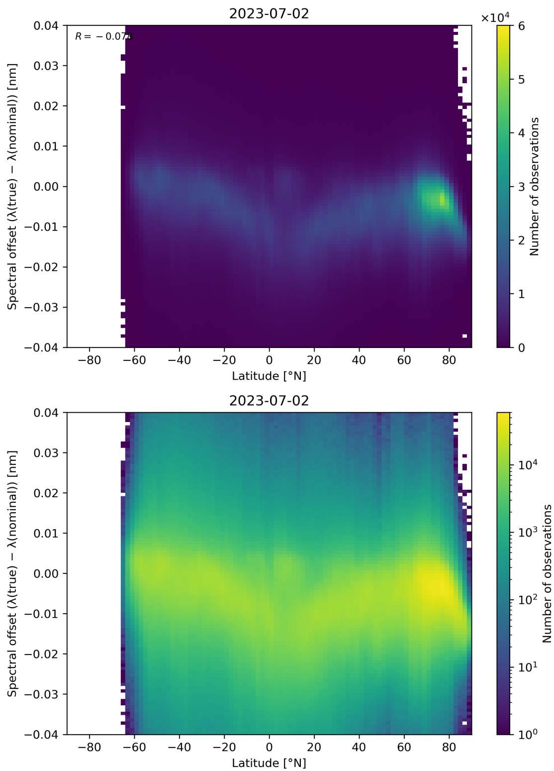
Figure 105: Scatter density plot of “Latitude” against “Spectral offset ( \lambda(\text{true}) - \lambda(\text{nominal}) )” for 2023-07-01 to 2023-07-03.
