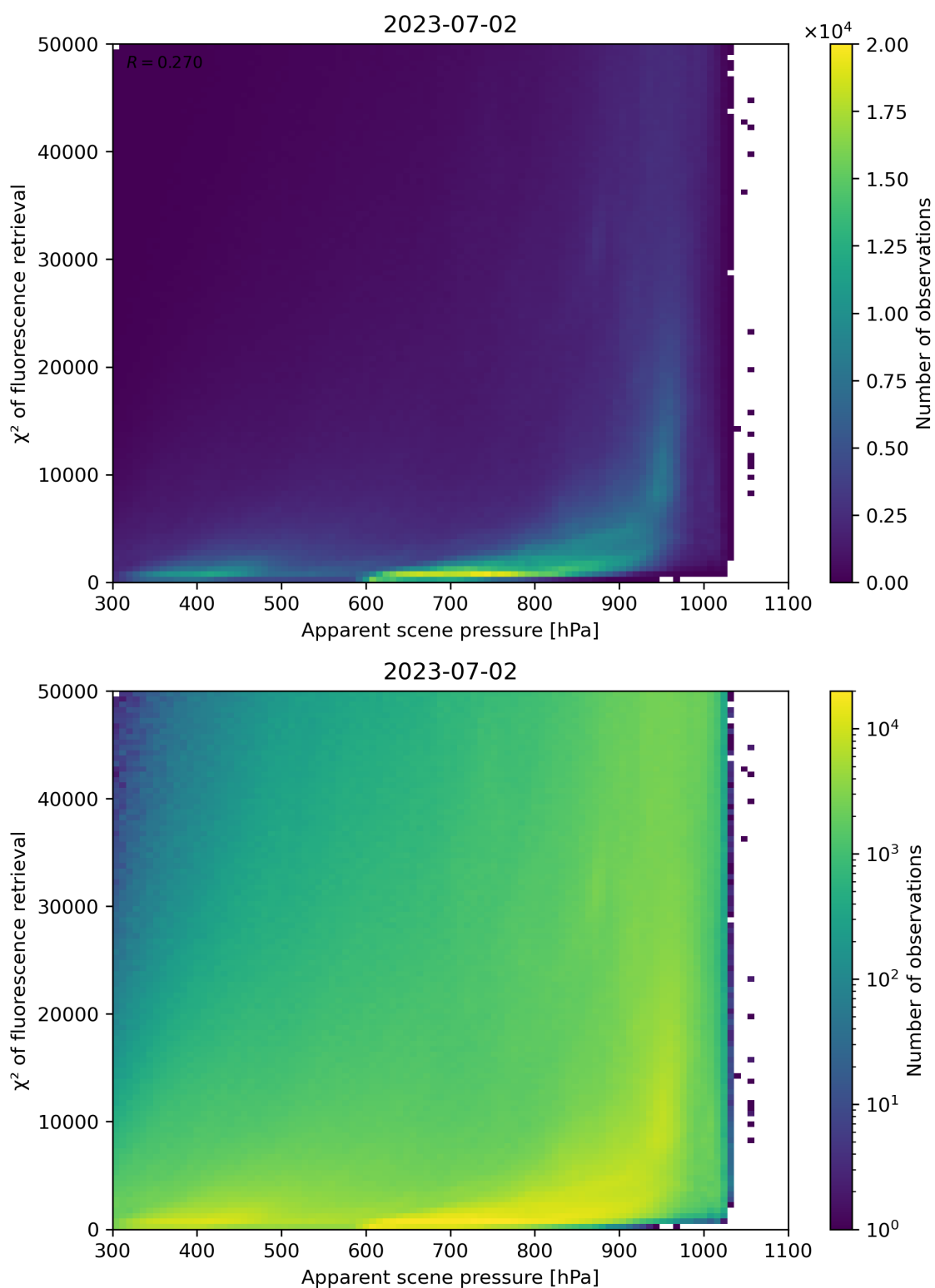
Figure 64: Scatter density plot of “Apparent scene pressure” against “ \chi^2 of fluorescence retrieval” for 2023-07-01 to 2023-07-03.
