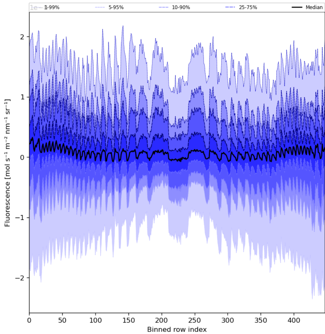
Figure 57: Along track statistics of “Fluorescence” for 2023-07-01 to 2023-07-03
