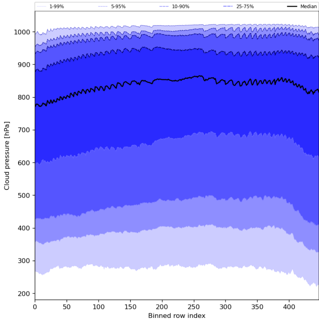
Figure 47: Along track statistics of “Cloud pressure” for 2023-07-01 to 2023-07-03
