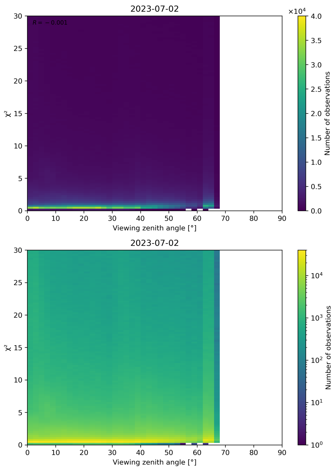
Figure 130: Scatter density plot of “Viewing zenith angle” against “ \chi^2 ” for 2023-07-01 to 2023-07-03.
