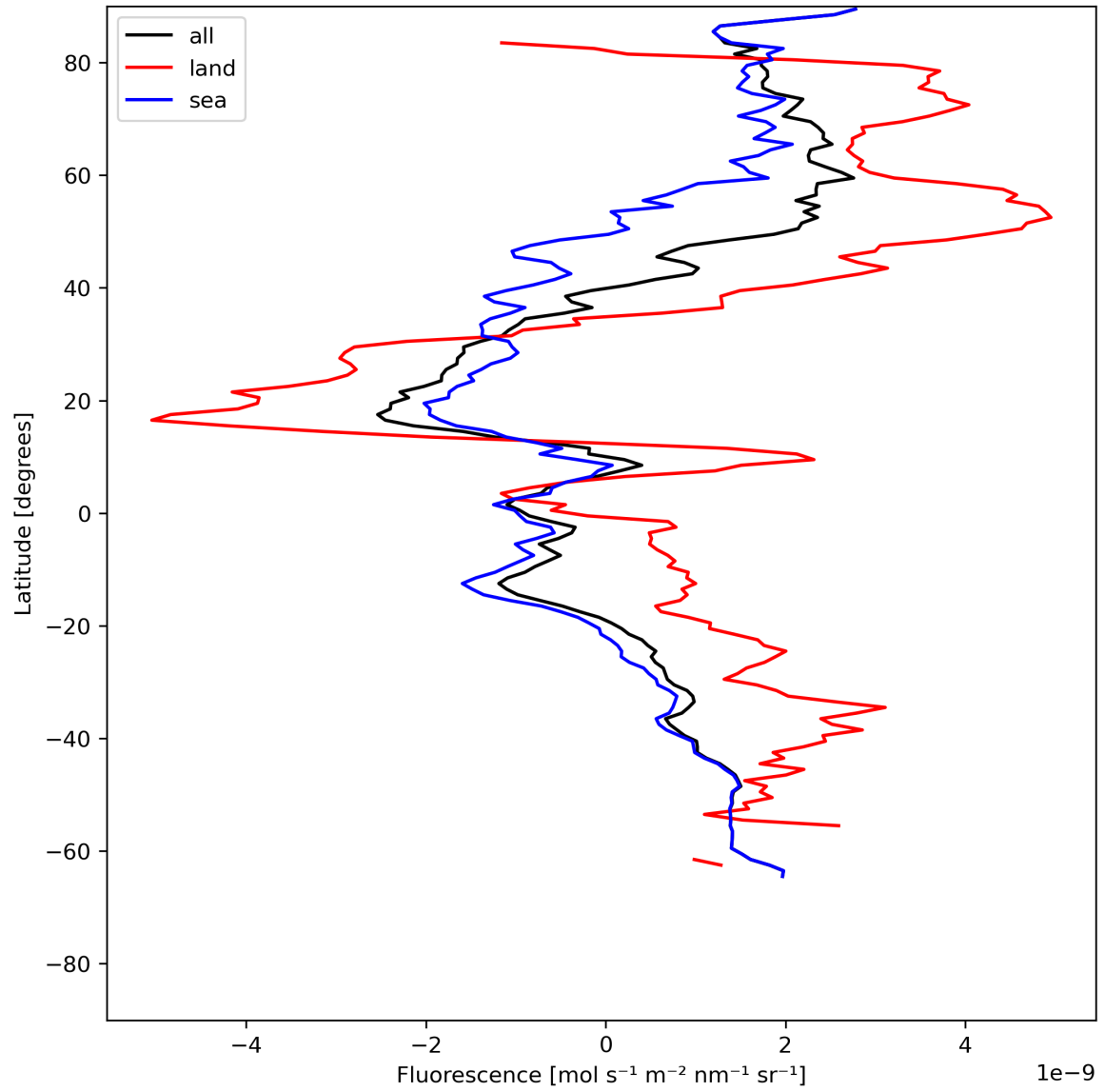
Figure 23: Zonal average of “Fluorescence” for 2023-07-01 to 2023-07-03.
