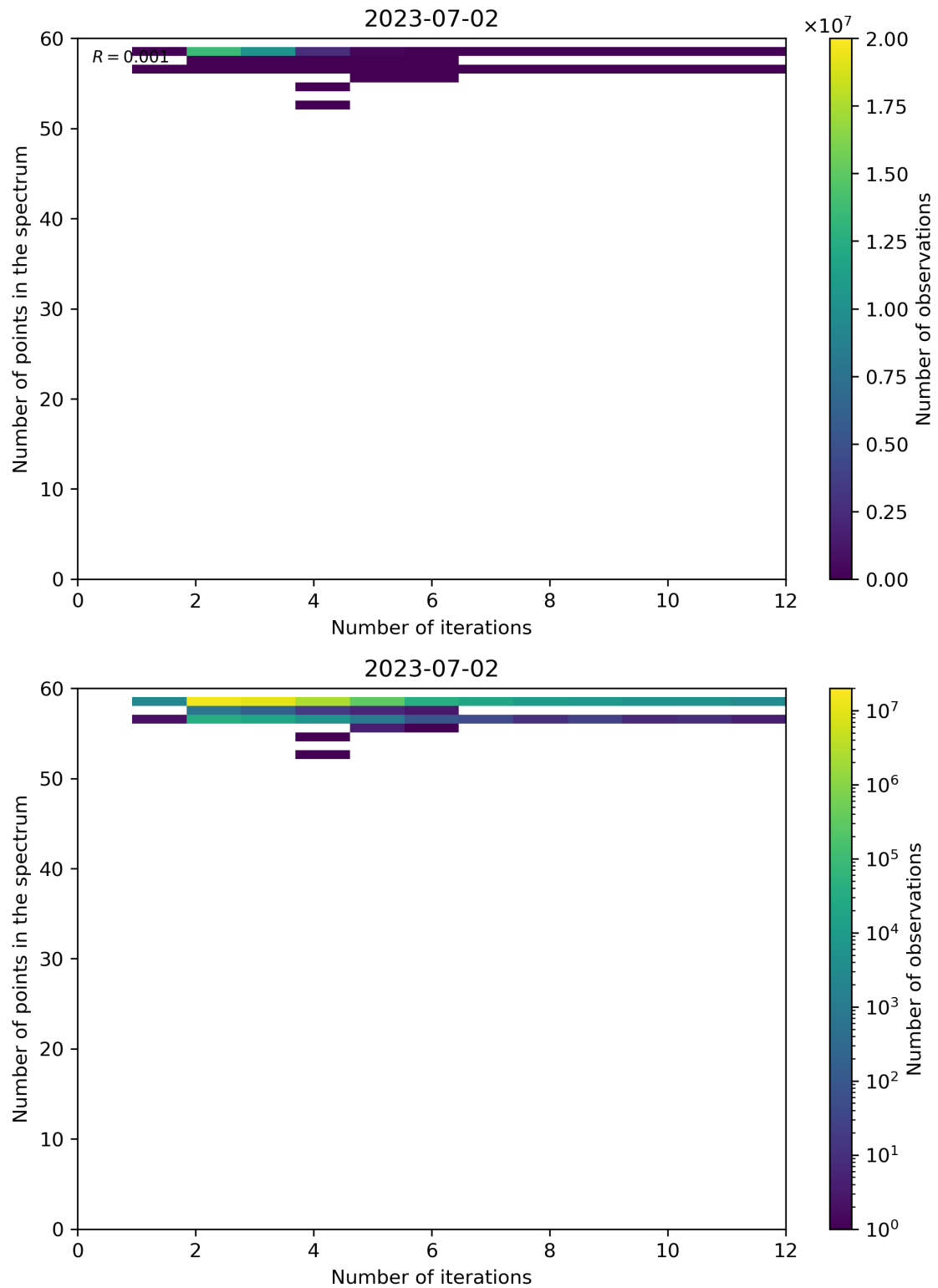
Figure 108: Scatter density plot of “Number of iterations” against “Number of points in the spectrum” for 2023-07-01 to 2023-07-03.
