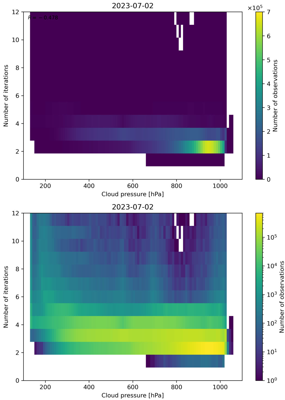
Figure 89: Scatter density plot of “Cloud pressure” against “Number of iterations” for 2023-07-01 to 2023-07-03.
