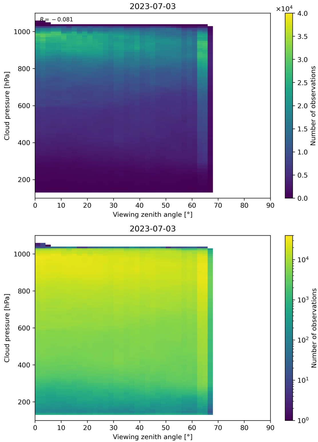
Figure 133: Scatter density plot of “Viewing zenith angle” against “Cloud pressure” for 2023-07-03 to 2023-07-04.
