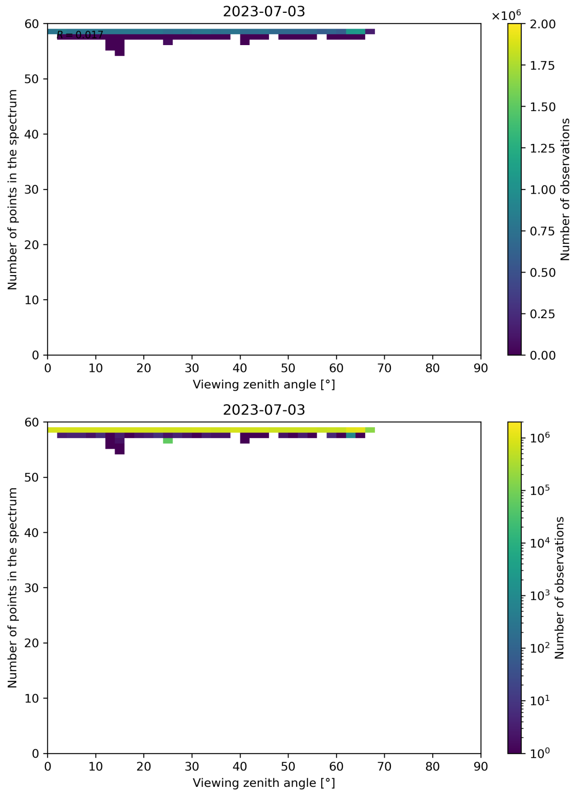
Figure 137: Scatter density plot of “Viewing zenith angle” against “Number of points in the spectrum” for 2023-07-03 to 2023-07-04.
