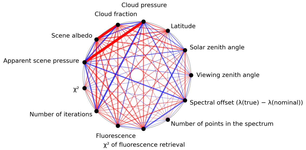
Figure 1: Map of correlation graph for 2023-07-03 to 2023-07-04.
