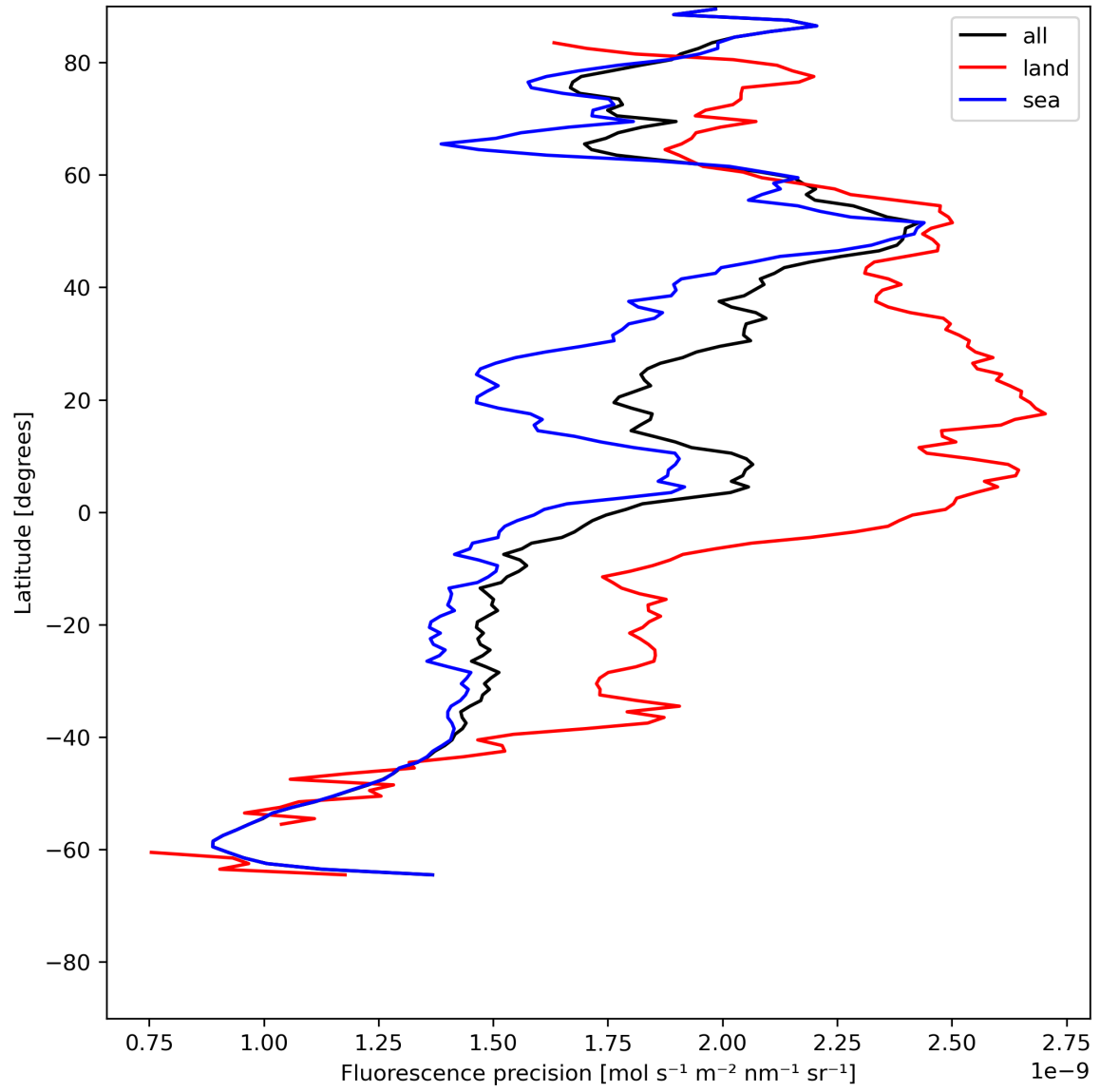
Figure 24: Zonal average of “Fluorescence precision” for 2023-07-03 to 2023-07-04.
