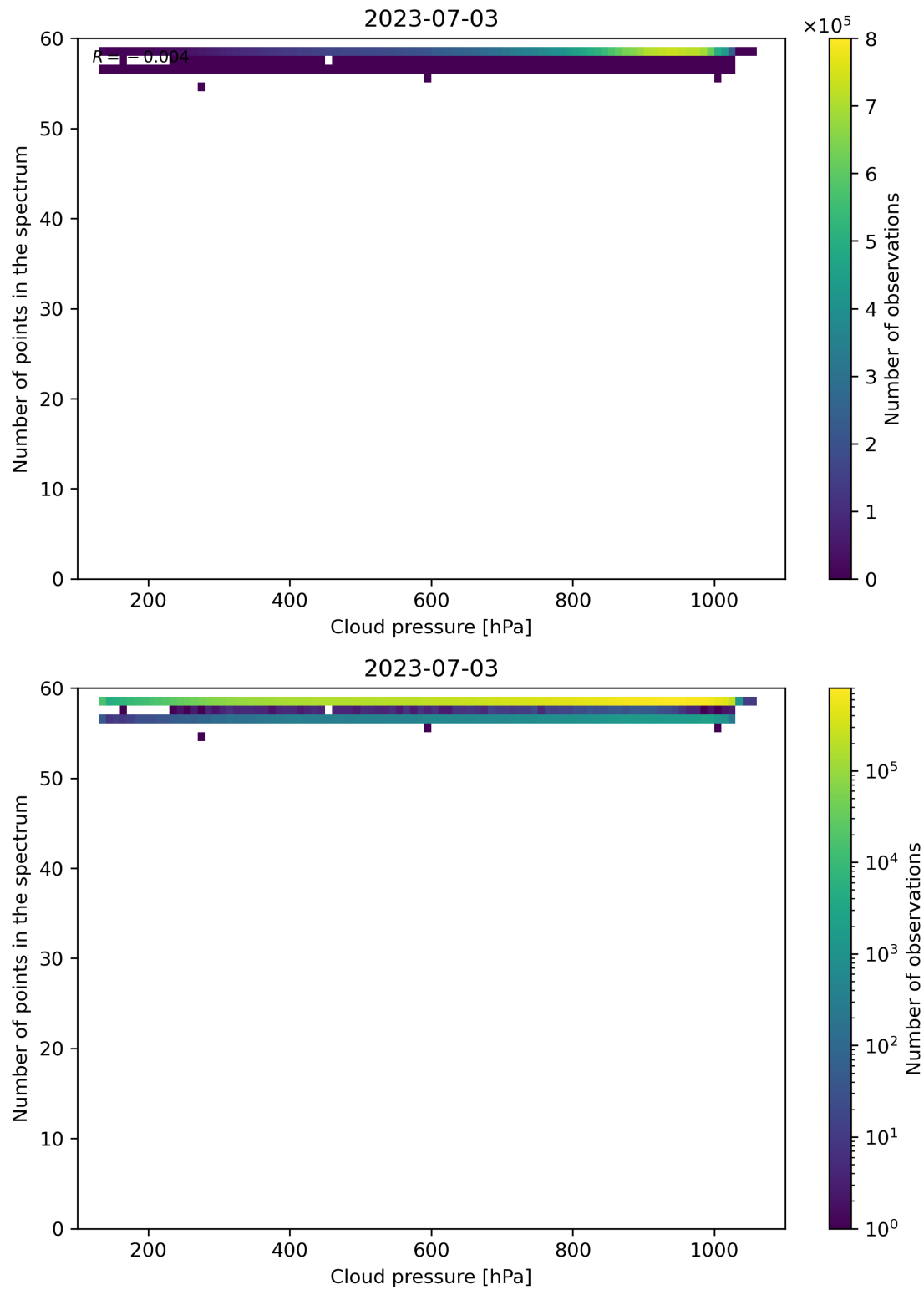
Figure 90: Scatter density plot of “Cloud pressure” against “Number of points in the spectrum” for 2023-07-03 to 2023-07-04.
