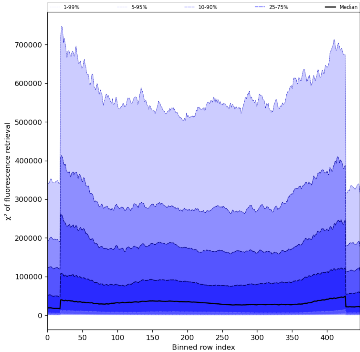
Figure 59: Along track statistics of “ \chi^2 of fluorescence retrieval” for 2023-07-03 to 2023-07-04
