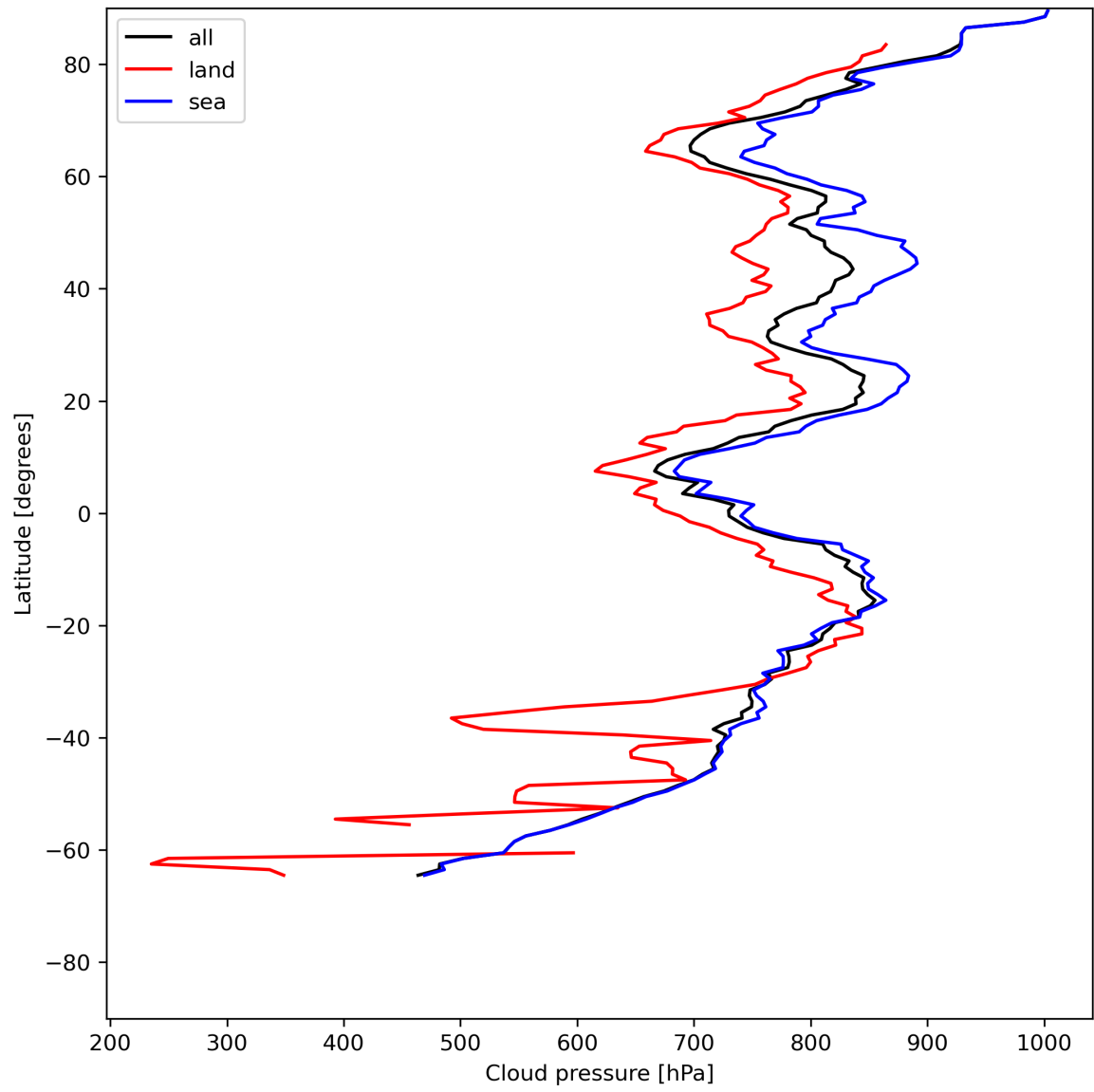
Figure 13: Zonal average of “Cloud pressure” for 2023-07-03 to 2023-07-04.
