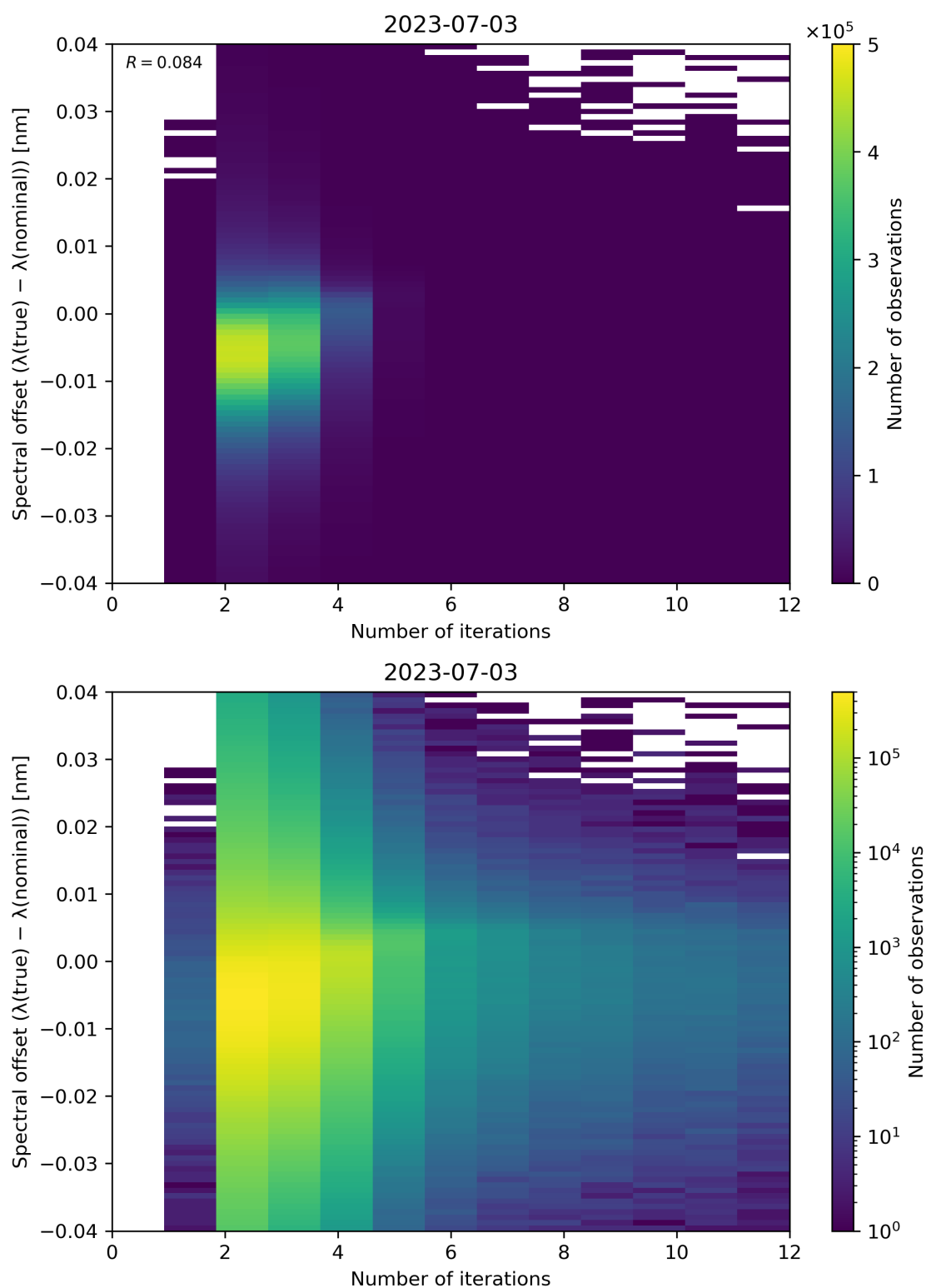
Figure 109: Scatter density plot of “Number of iterations” against “Spectral offset ( \lambda(\text{true}) - \lambda(\text{nominal}) )” for 2023-07-03 to 2023-07-04.
