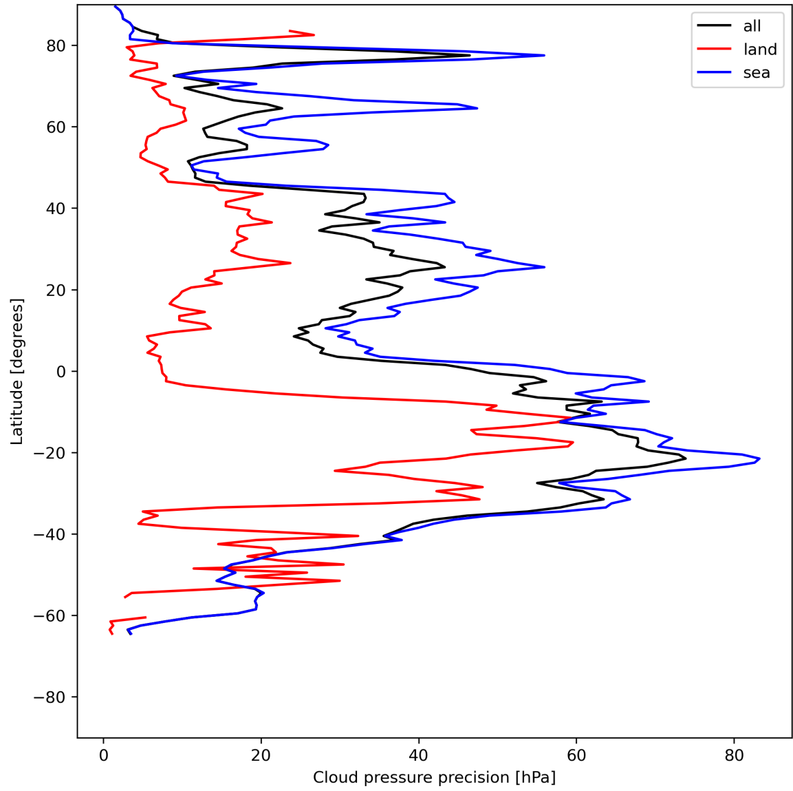
Figure 14: Zonal average of “Cloud pressure precision” for 2023-07-03 to 2023-07-04.
