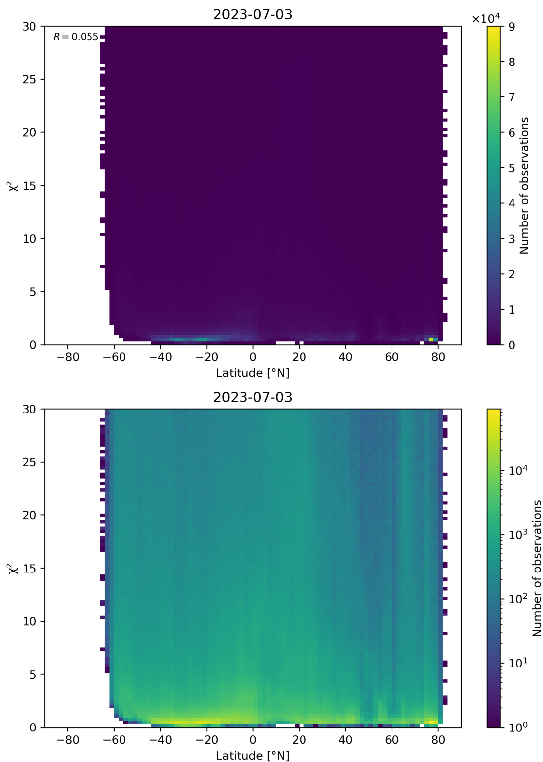
Figure 97: Scatter density plot of “Latitude” against “ \chi^2 ” for 2023-07-03 to 2023-07-04.
