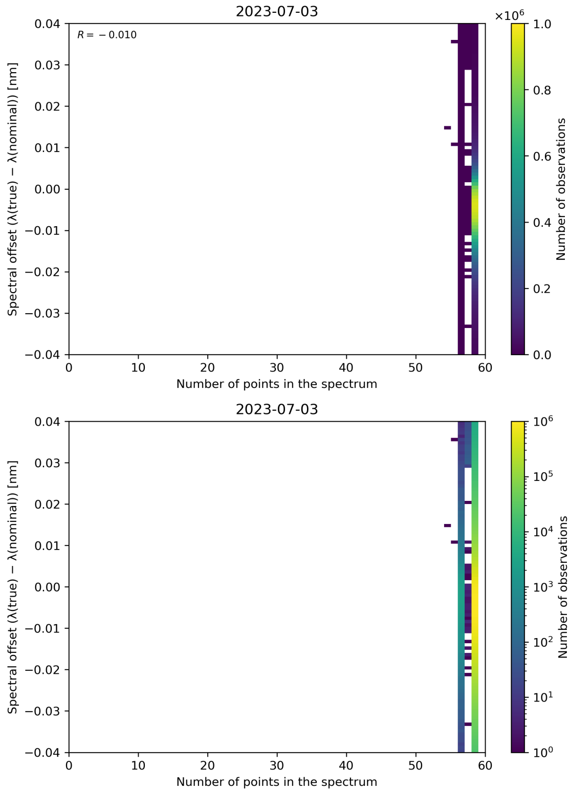
Figure 110: Scatter density plot of “Number of points in the spectrum” against “Spectral offset ( \lambda(\text{true}) - \lambda(\text{nominal}) )” for 2023-07-03 to 2023-07-04.
