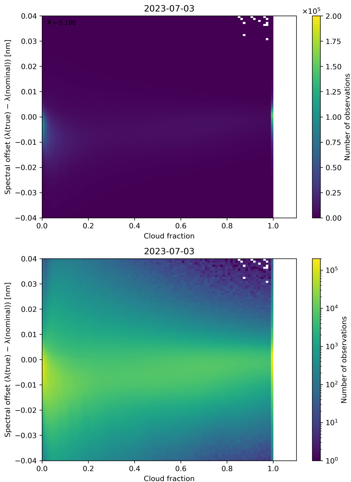
Figure 83: Scatter density plot of “Cloud fraction” against “Spectral offset ( \lambda(\text{true}) - \lambda(\text{nominal}) )” for 2023-07-03 to 2023-07-04.
