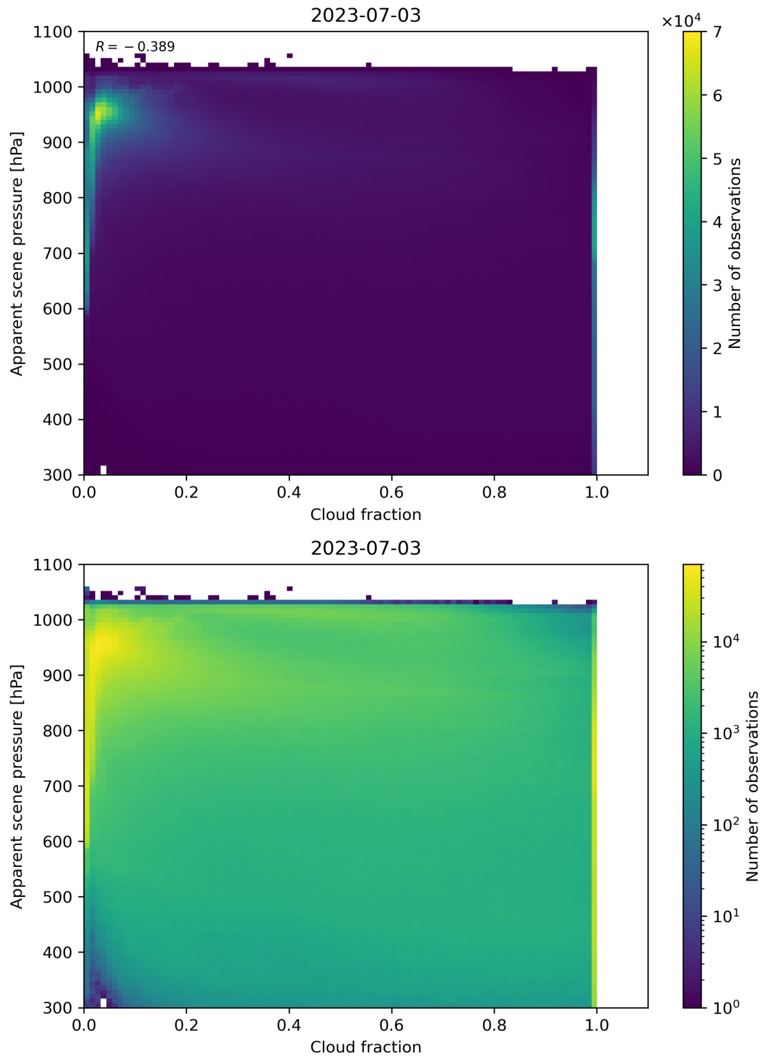
Figure 76: Scatter density plot of “Cloud fraction” against “Apparent scene pressure” for 2023-07-03 to 2023-07-04.
