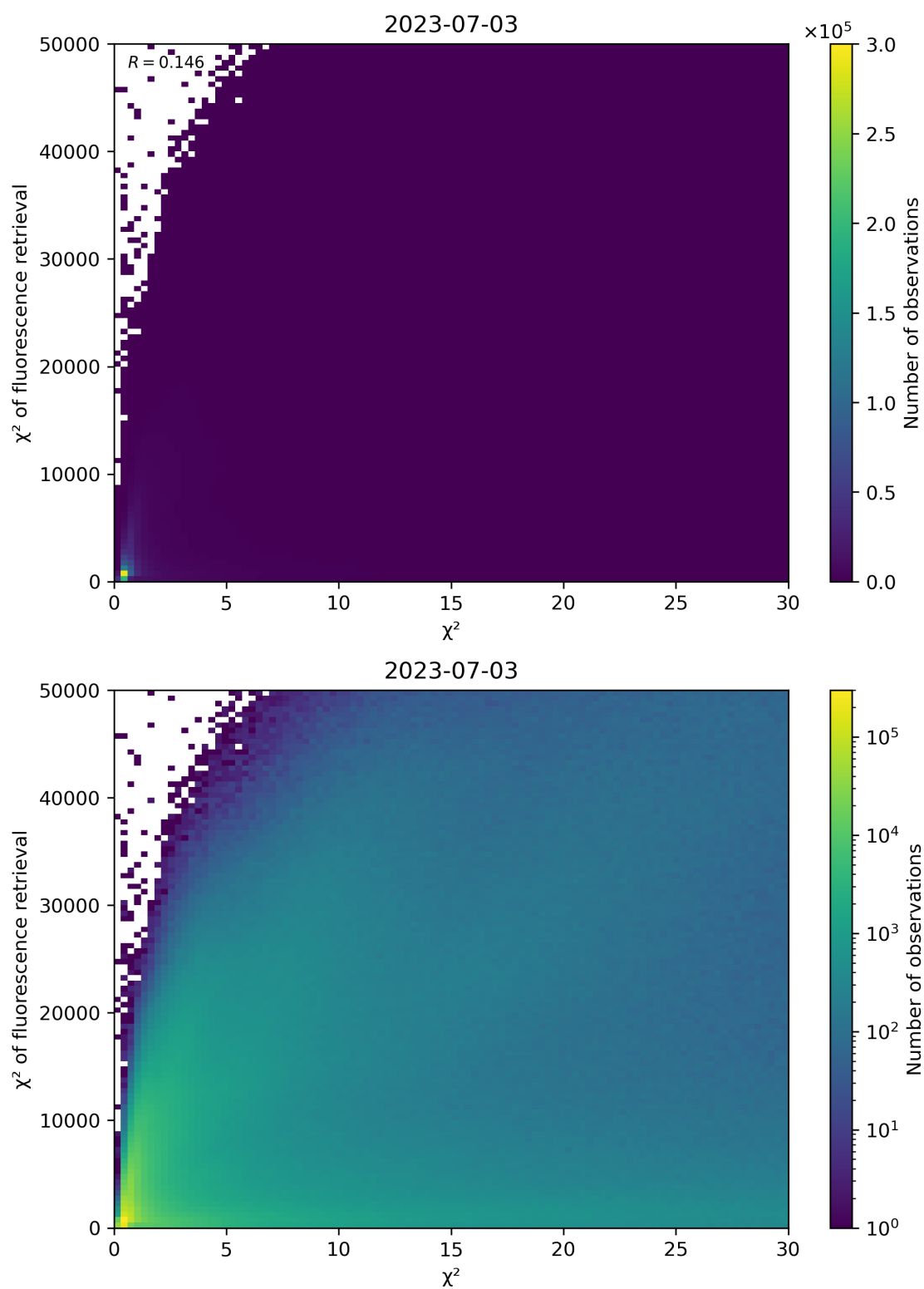
Figure 69: Scatter density plot of “ \chi^2 ” against “ \chi^2 of fluorescence retrieval” for 2023-07-03 to 2023-07-04.
