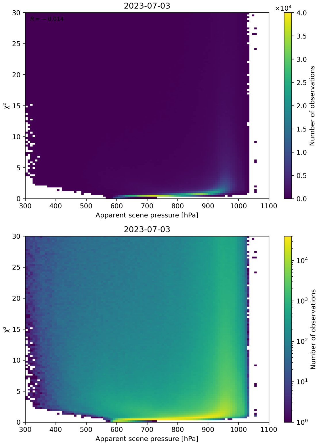
Figure 63: Scatter density plot of “Apparent scene pressure” against “ \chi^2 ” for 2023-07-03 to 2023-07-04.
