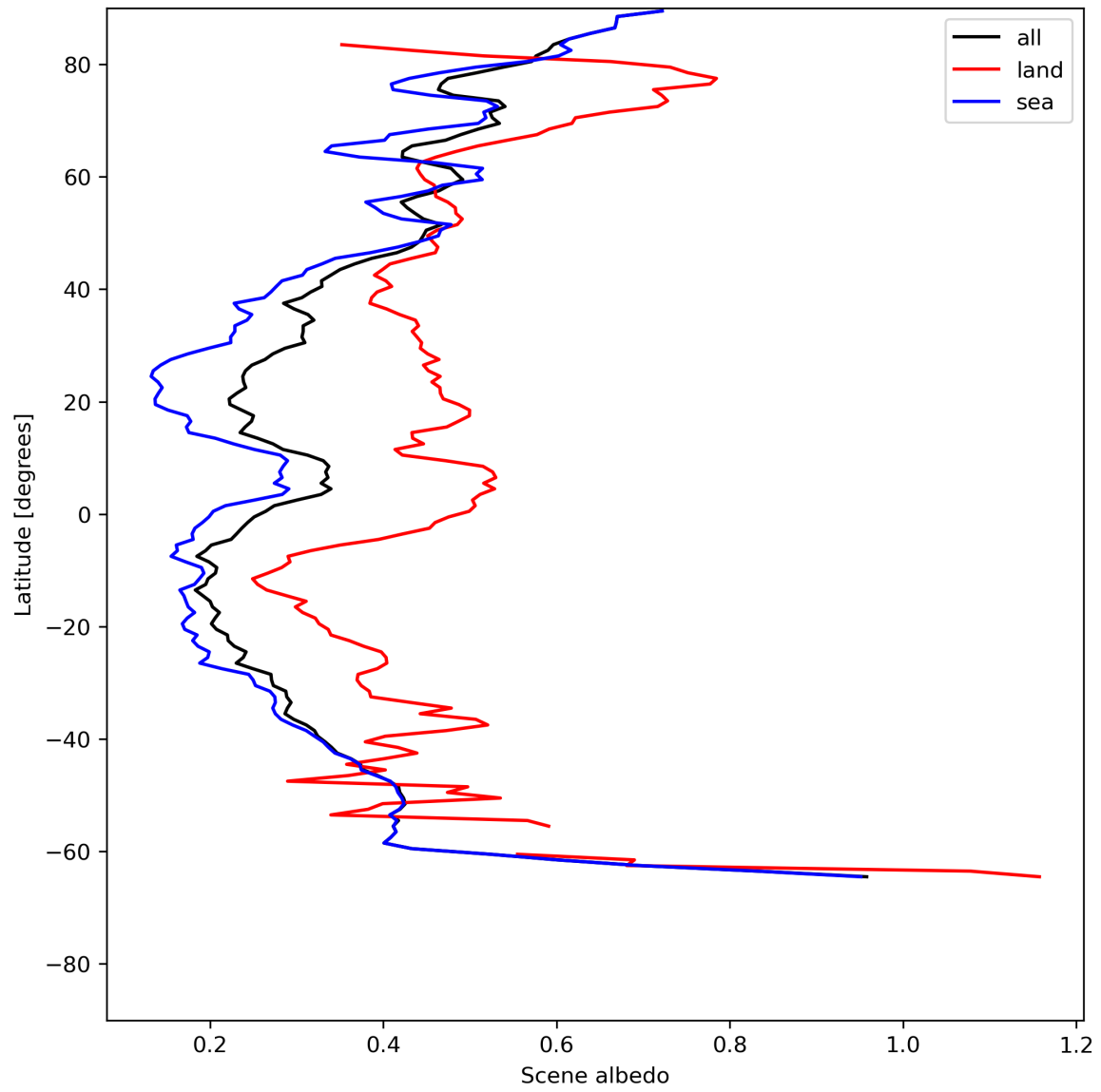
Figure 17: Zonal average of “Scene albedo” for 2023-07-03 to 2023-07-04.
