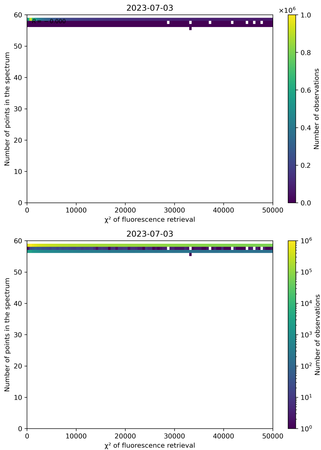
Figure 71: Scatter density plot of " \chi^2 of fluorescence retrieval" against "Number of points in the spectrum" for 2023-07-03 to 2023-07-04.
