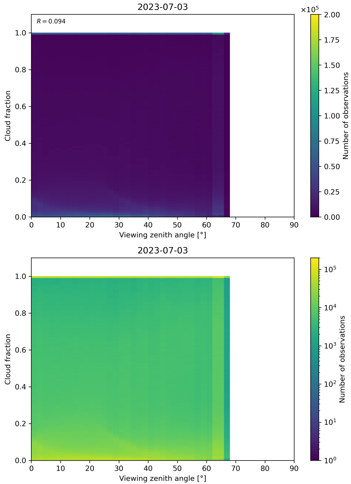
Figure 132: Scatter density plot of “Viewing zenith angle” against “Cloud fraction” for 2023-07-03 to 2023-07-04.
