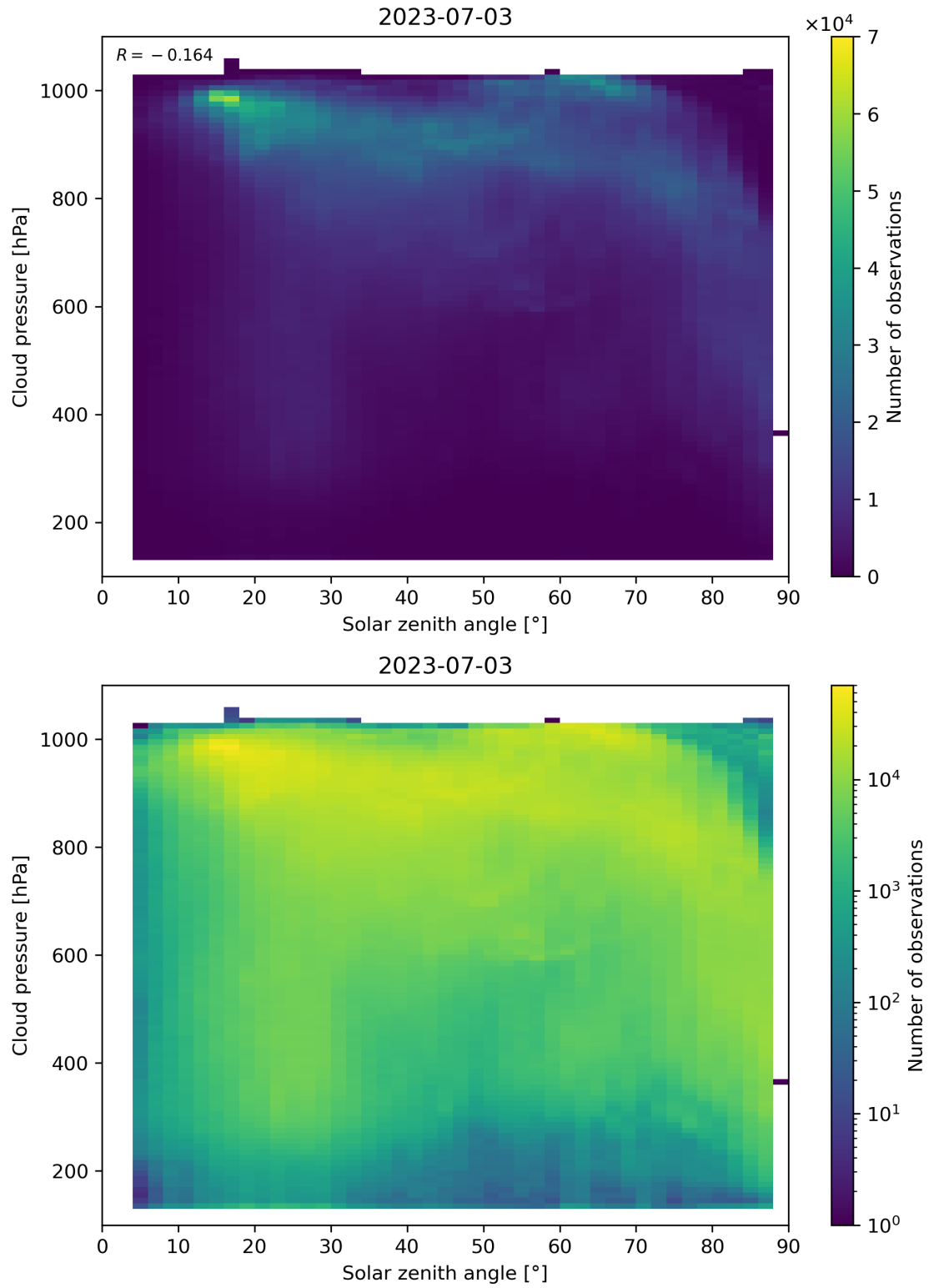
Figure 122: Scatter density plot of “Solar zenith angle” against “Cloud pressure” for 2023-07-03 to 2023-07-04.
