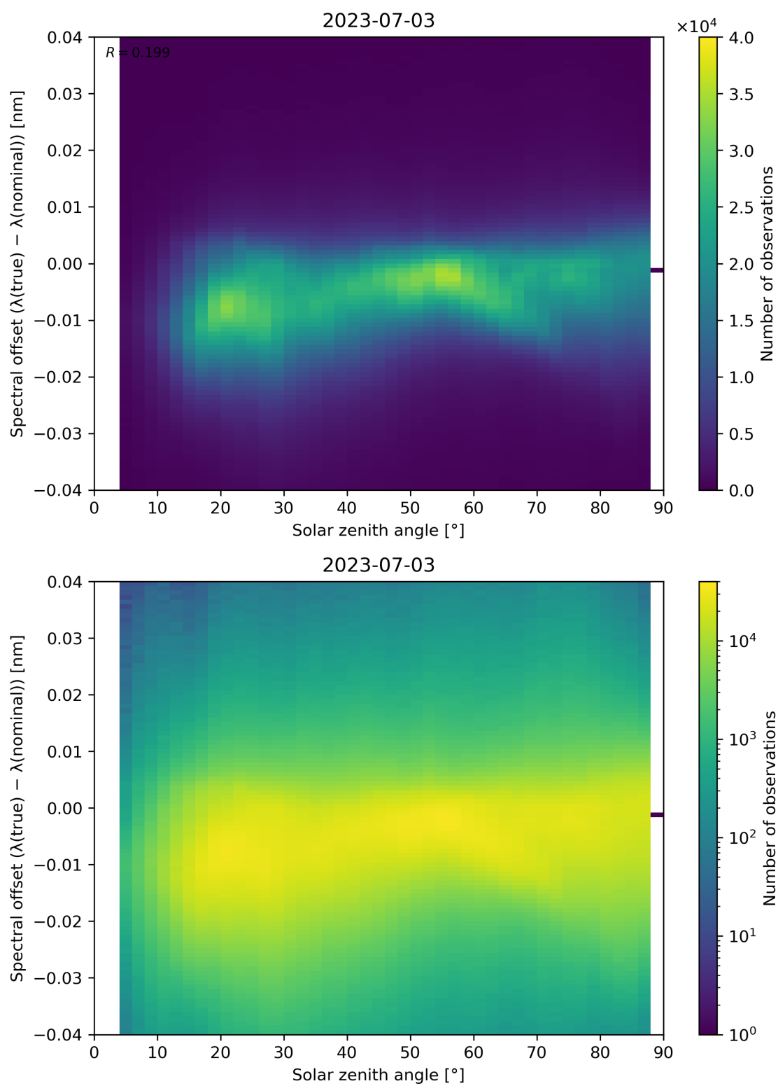
Figure 128: Scatter density plot of “Solar zenith angle” against “Spectral offset ( \lambda(\text{true}) - \lambda(\text{nominal}) )” for 2023-07-03 to 2023-07-04.
