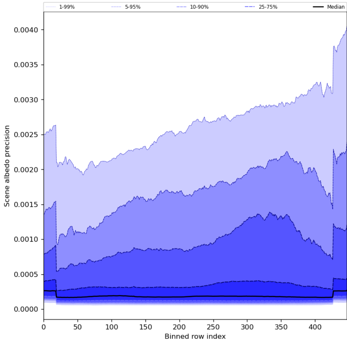
Figure 52: Along track statistics of “Scene albedo precision” for 2023-07-03 to 2023-07-04
