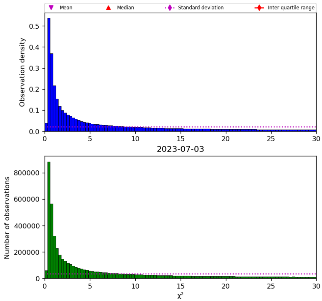
Figure 38: Histogram of " \chi^2 " for 2023-07-03 to 2023-07-04
