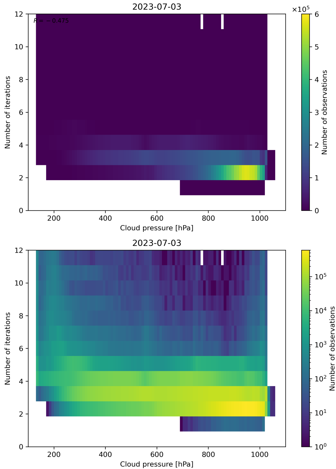
Figure 89: Scatter density plot of “Cloud pressure” against “Number of iterations” for 2023-07-03 to 2023-07-04.
