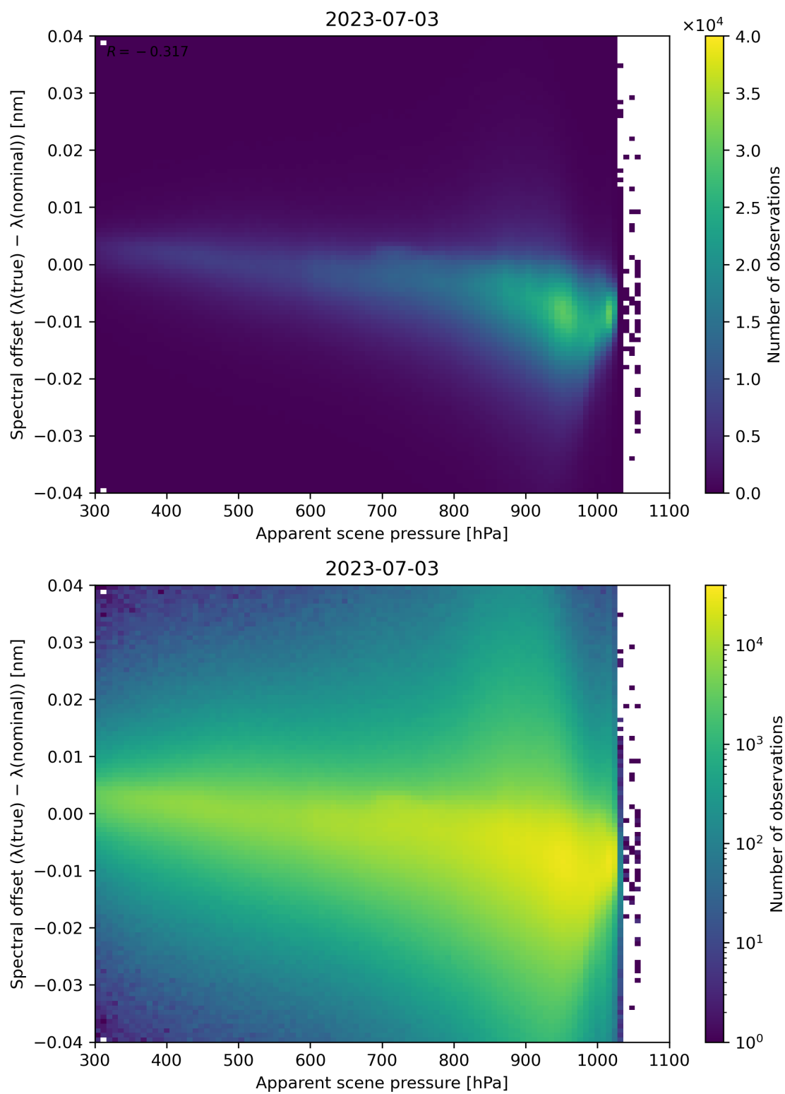
Figure 68: Scatter density plot of “Apparent scene pressure” against “Spectral offset ( \lambda(\text{true}) - \lambda(\text{nominal}) )” for 2023-07-03 to 2023-07-04.
