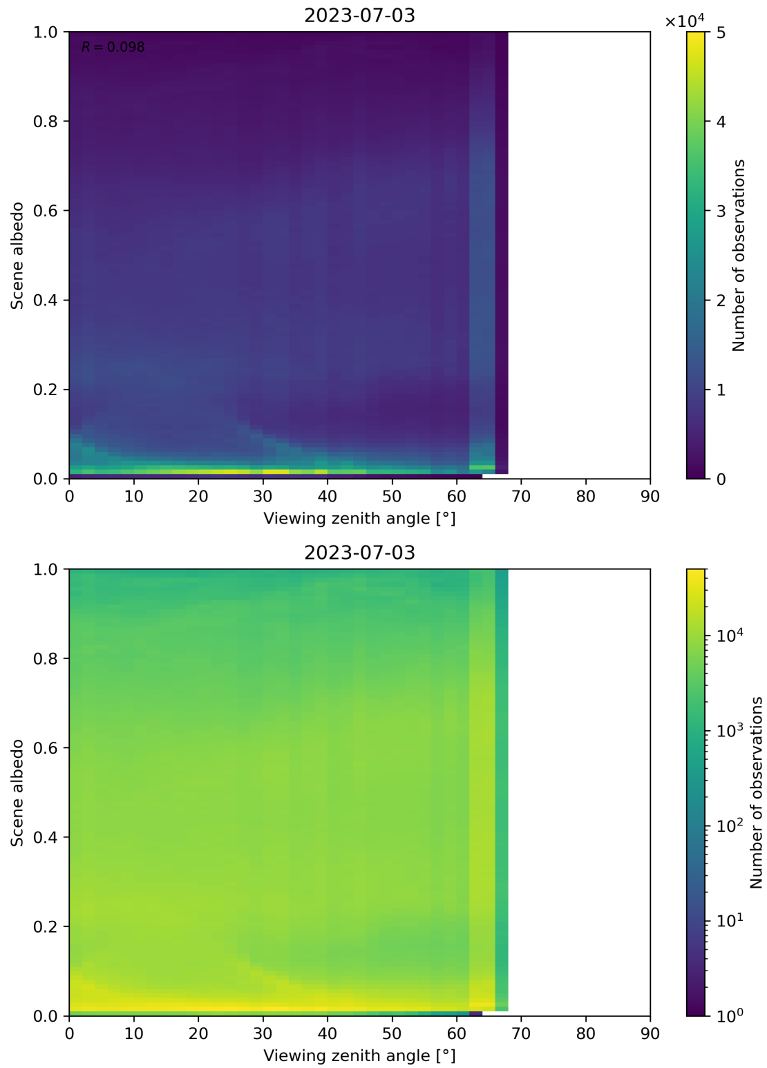
Figure 138: Scatter density plot of “Viewing zenith angle” against “Scene albedo” for 2023-07-03 to 2023-07-04.
