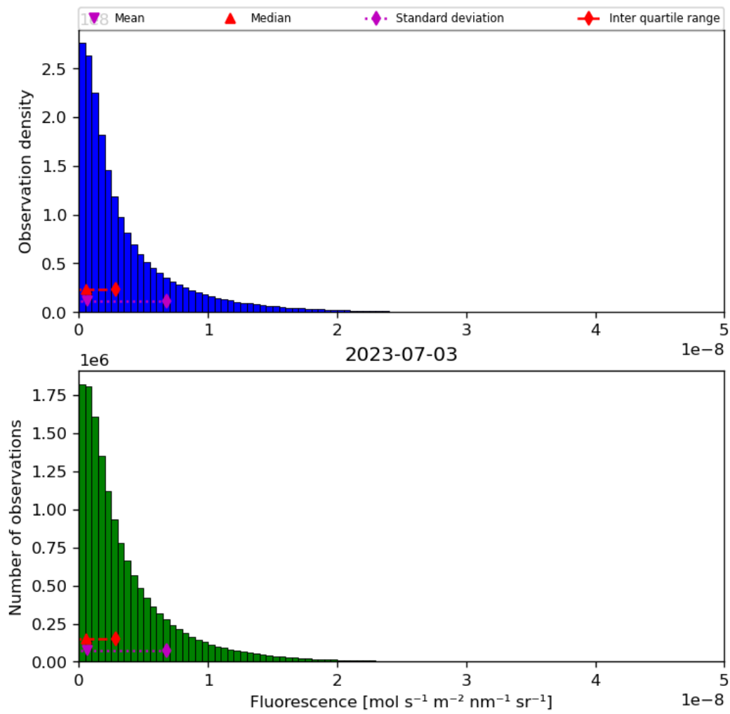
Figure 40: Histogram of “Fluorescence” for 2023-07-03 to 2023-07-04
