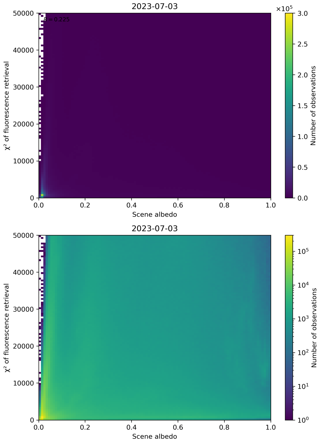
Figure 113: Scatter density plot of “Scene albedo” against “ \chi^2 of fluorescence retrieval” for 2023-07-03 to 2023-07-04.
