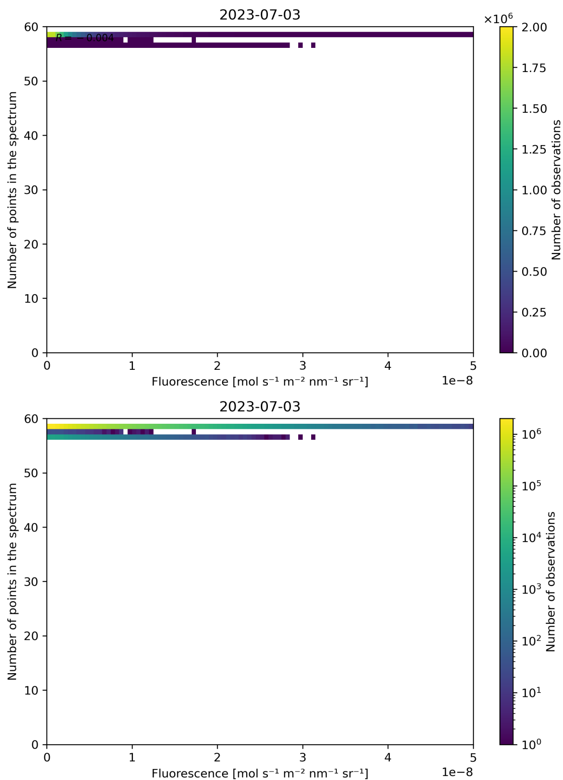
Figure 94: Scatter density plot of “Fluorescence” against “Number of points in the spectrum” for 2023-07-03 to 2023-07-04.
