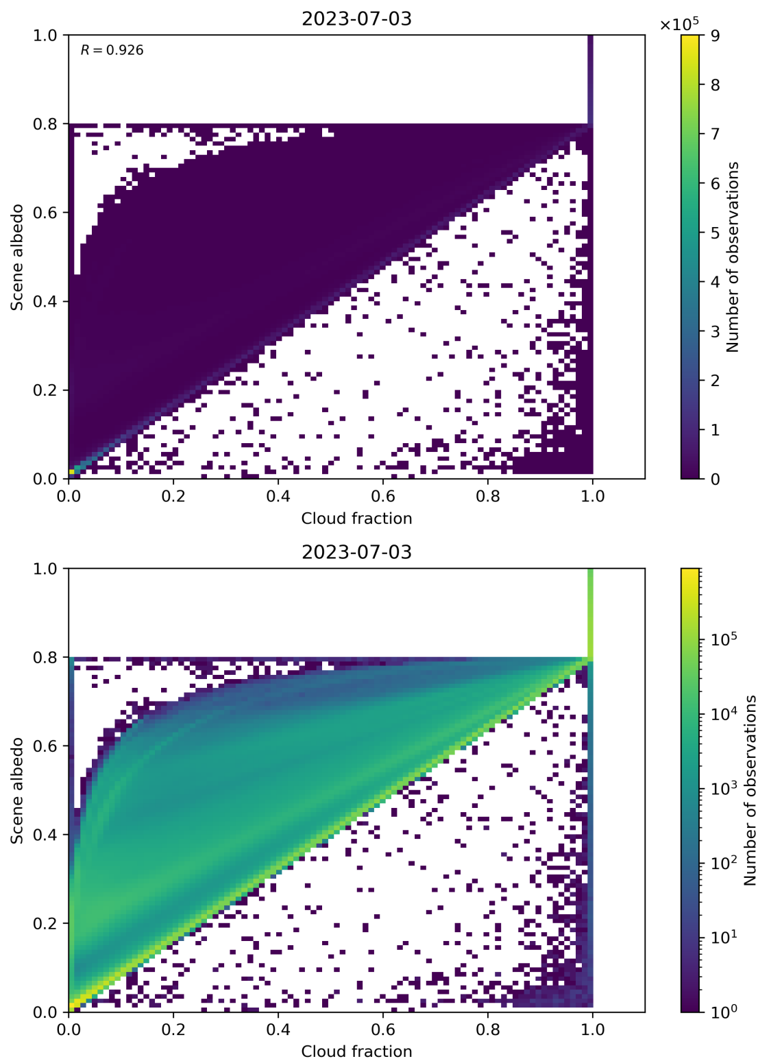
Figure 82: Scatter density plot of “Cloud fraction” against “Scene albedo” for 2023-07-03 to 2023-07-04.
