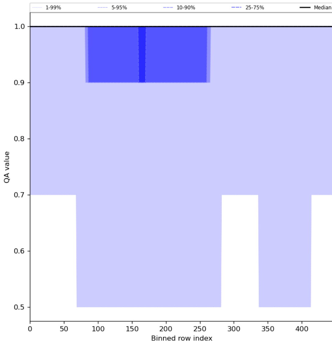
Figure 46: Along track statistics of “QA value” for 2023-07-03 to 2023-07-04
