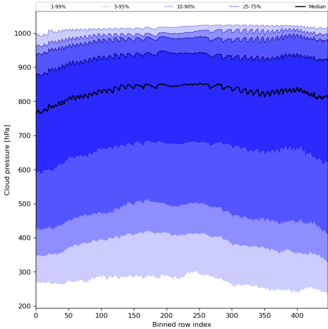
Figure 47: Along track statistics of “Cloud pressure” for 2023-07-03 to 2023-07-04
