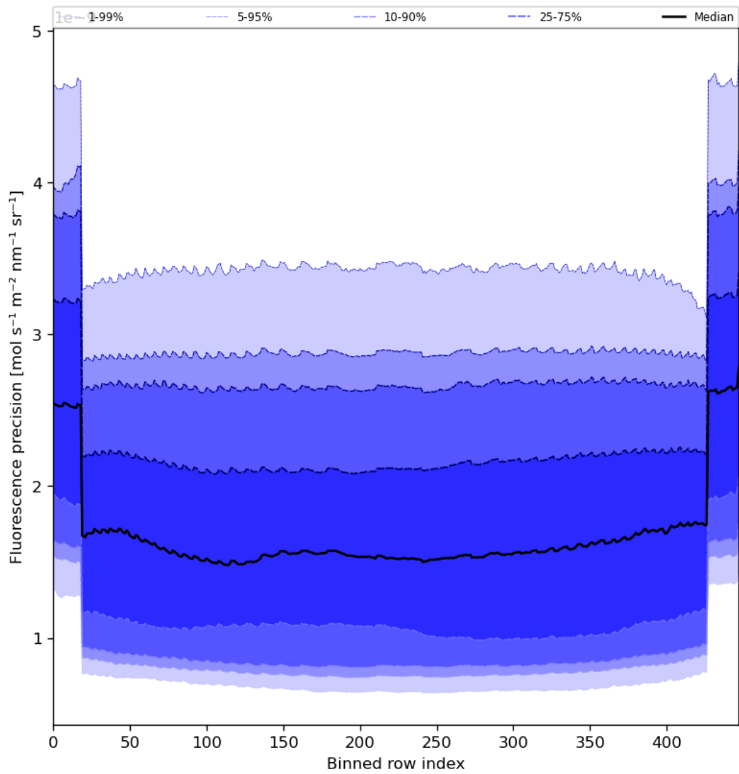
Figure 58: Along track statistics of “Fluorescence precision” for 2023-07-03 to 2023-07-04
