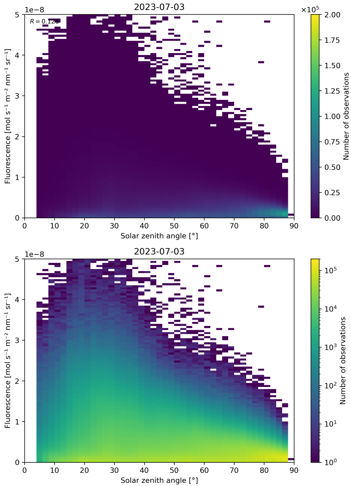
Figure 123: Scatter density plot of “Solar zenith angle” against “Fluorescence” for 2023-07-03 to 2023-07-04.
