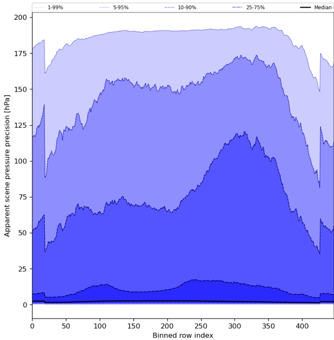
Figure 54: Along track statistics of “Apparent scene pressure precision” for 2023-07-03 to 2023-07-04
