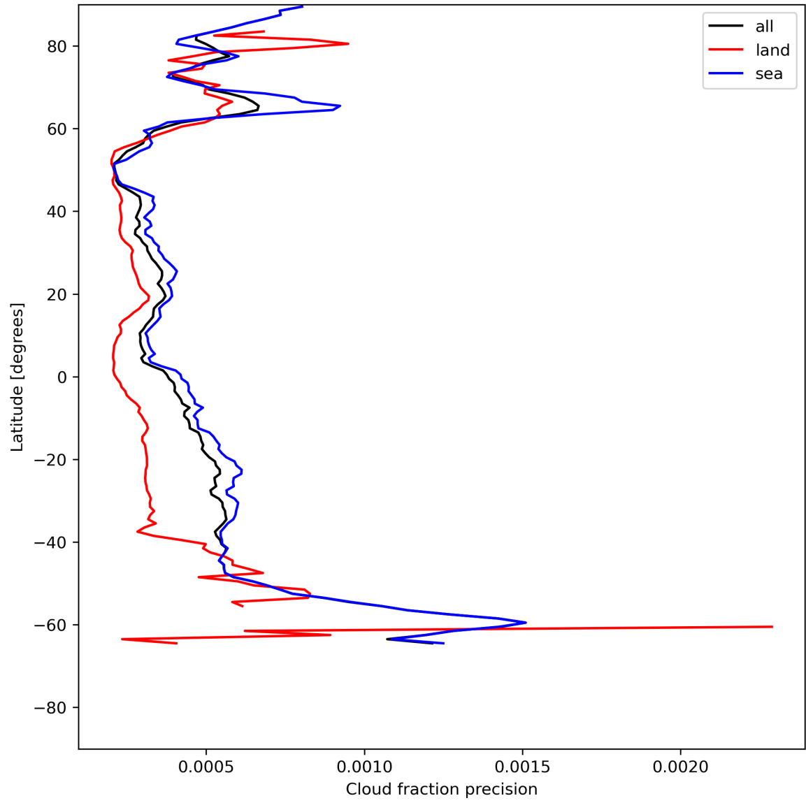
Figure 16: Zonal average of “Cloud fraction precision” for 2023-07-03 to 2023-07-04.
