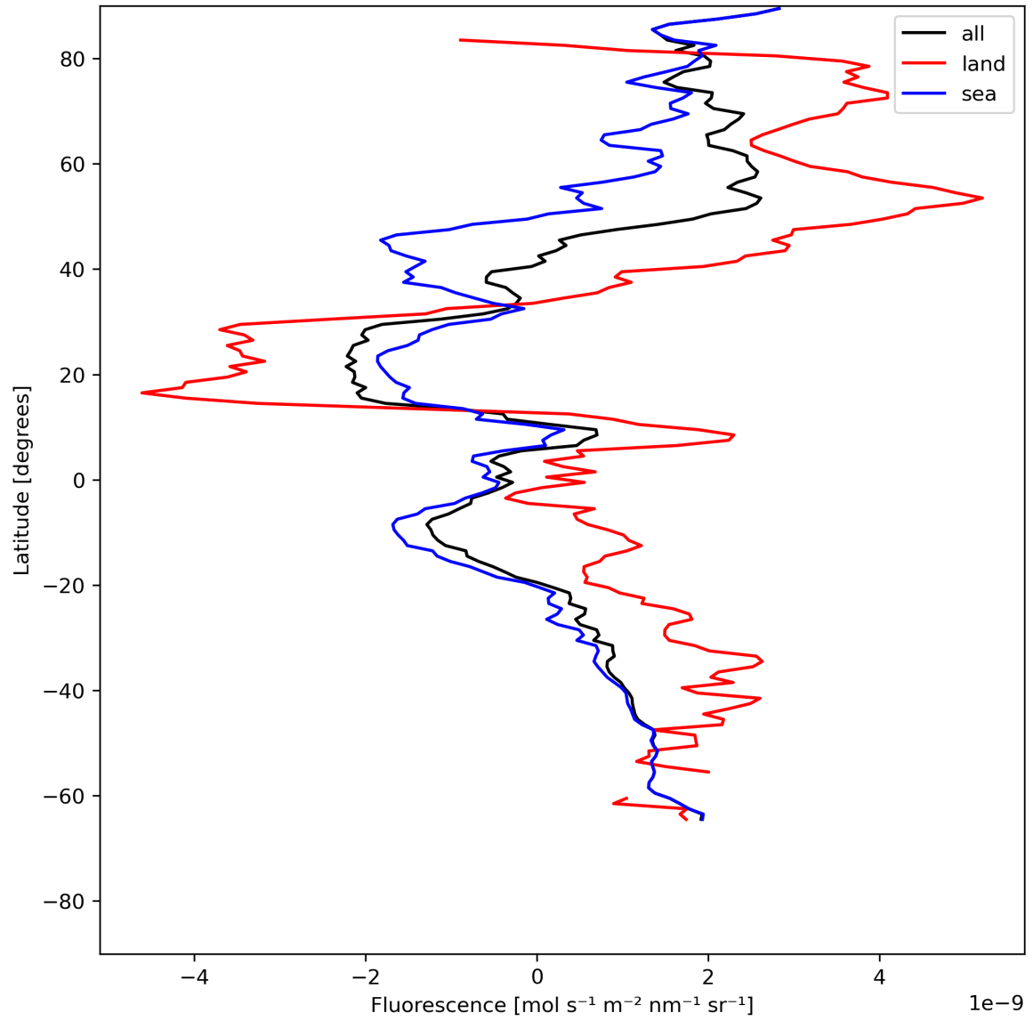
Figure 23: Zonal average of “Fluorescence” for 2023-07-03 to 2023-07-04.
