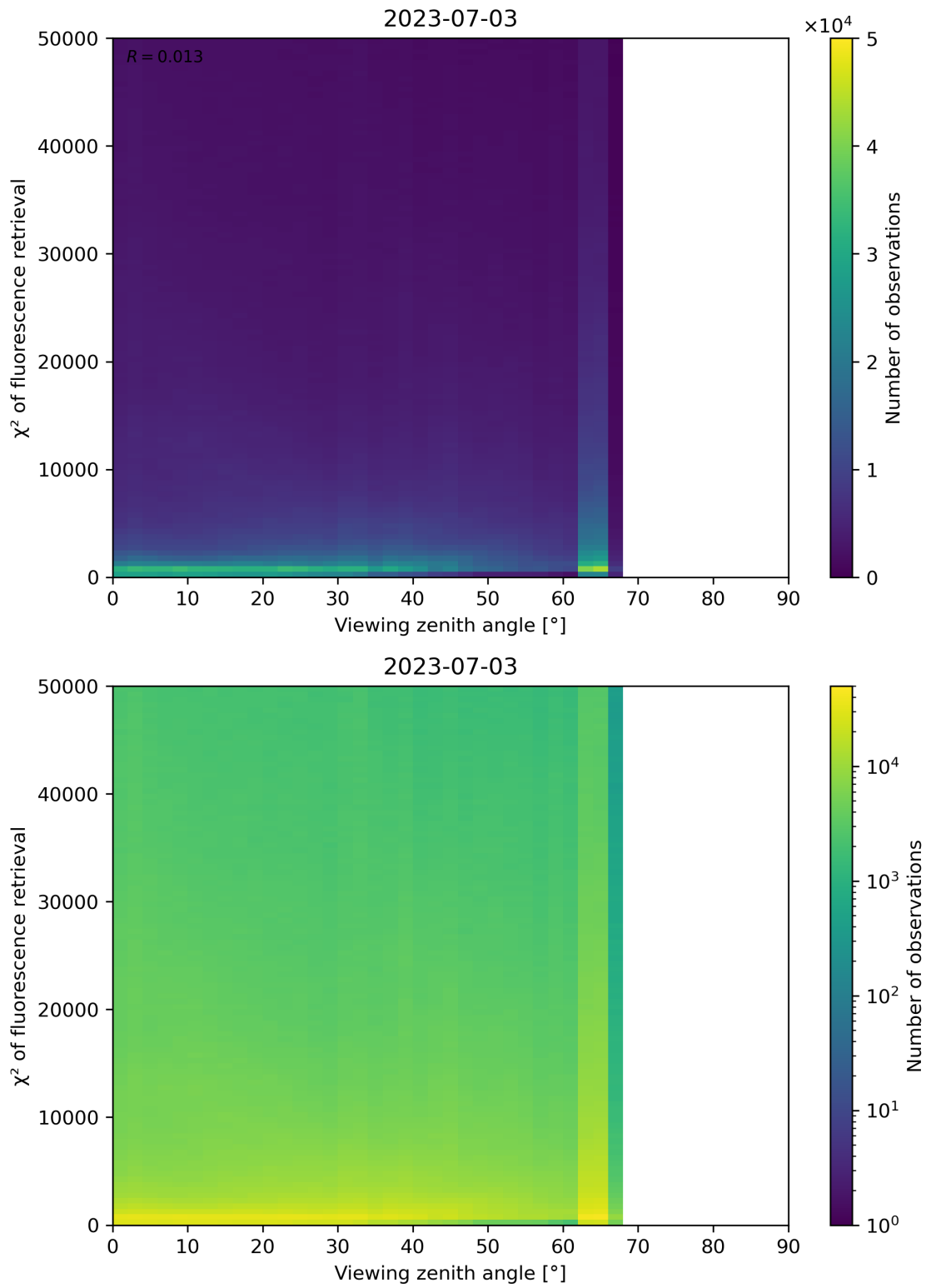
Figure 131: Scatter density plot of “Viewing zenith angle” against “ \chi^2 of fluorescence retrieval” for 2023-07-03 to 2023-07-04.
