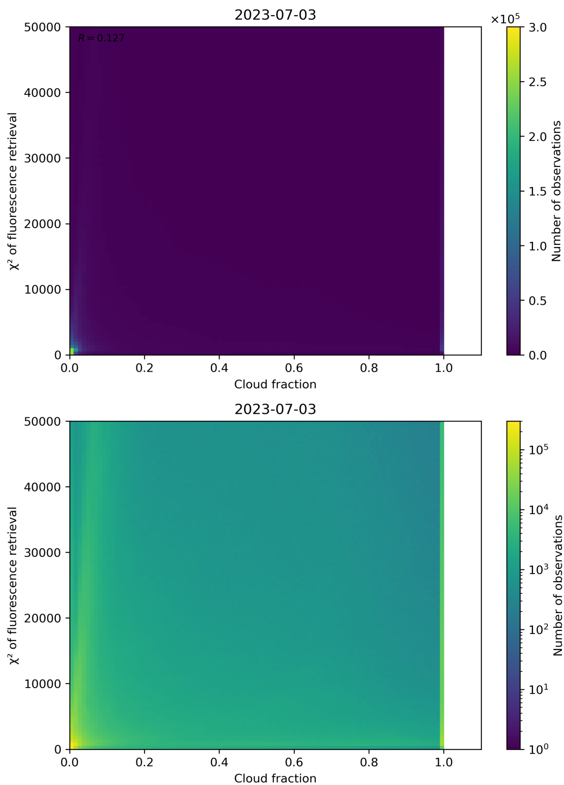
Figure 78: Scatter density plot of “Cloud fraction” against “ \chi^2 of fluorescence retrieval” for 2023-07-03 to 2023-07-04.
