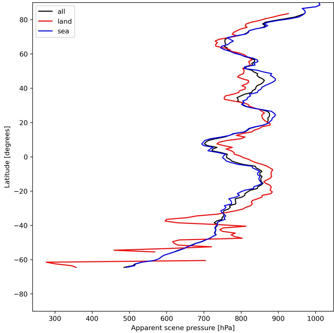
Figure 19: Zonal average of “Apparent scene pressure” for 2023-07-03 to 2023-07-04.
