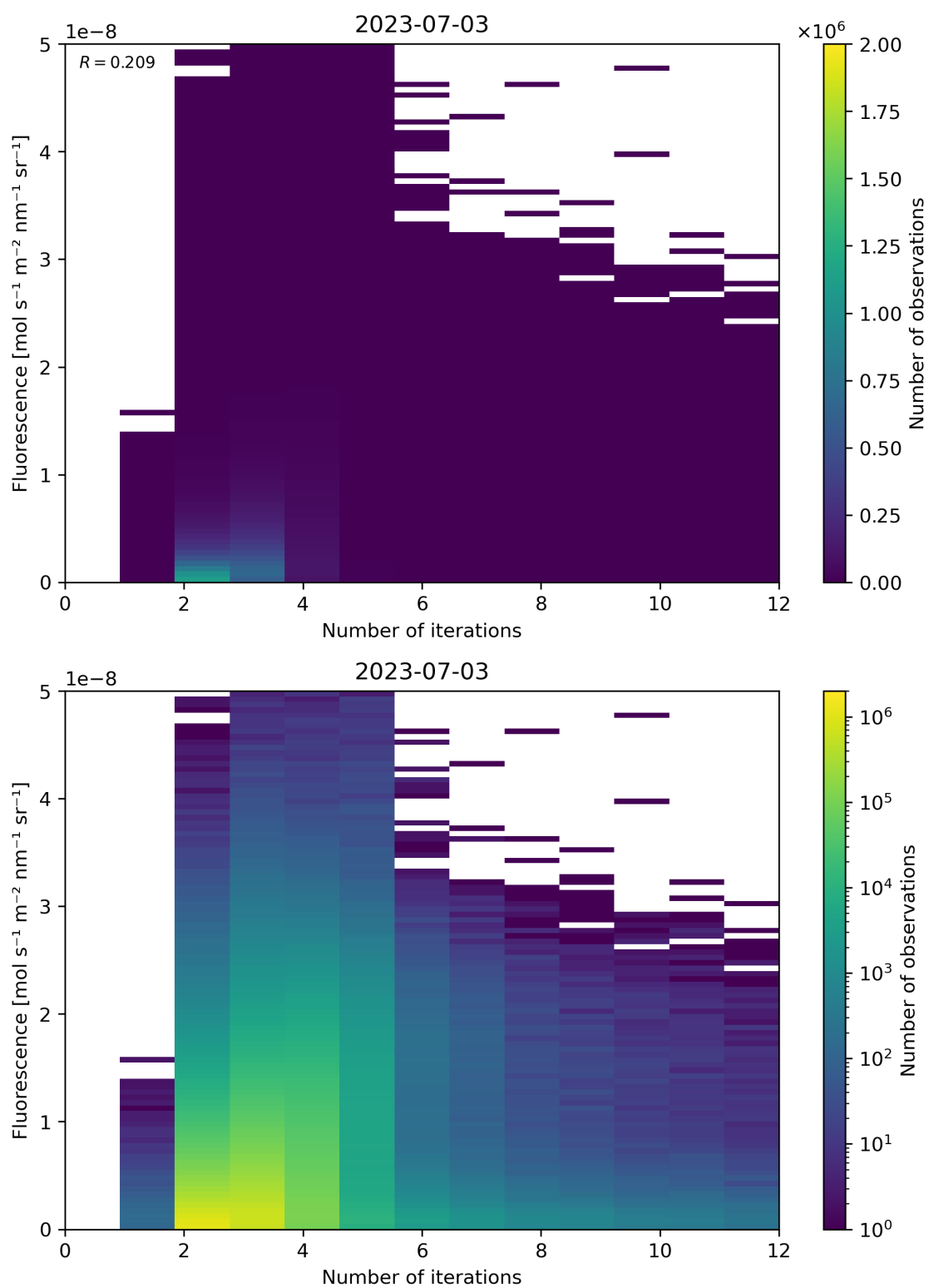
Figure 107: Scatter density plot of “Number of iterations” against “Fluorescence” for 2023-07-03 to 2023-07-04.
