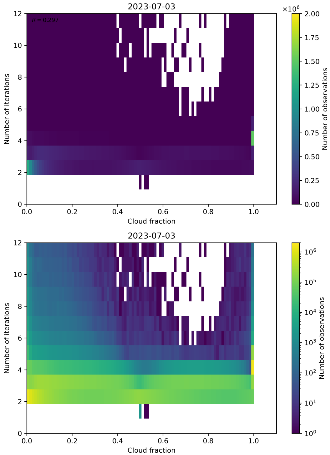
Figure 80: Scatter density plot of “Cloud fraction” against “Number of iterations” for 2023-07-03 to 2023-07-04.
