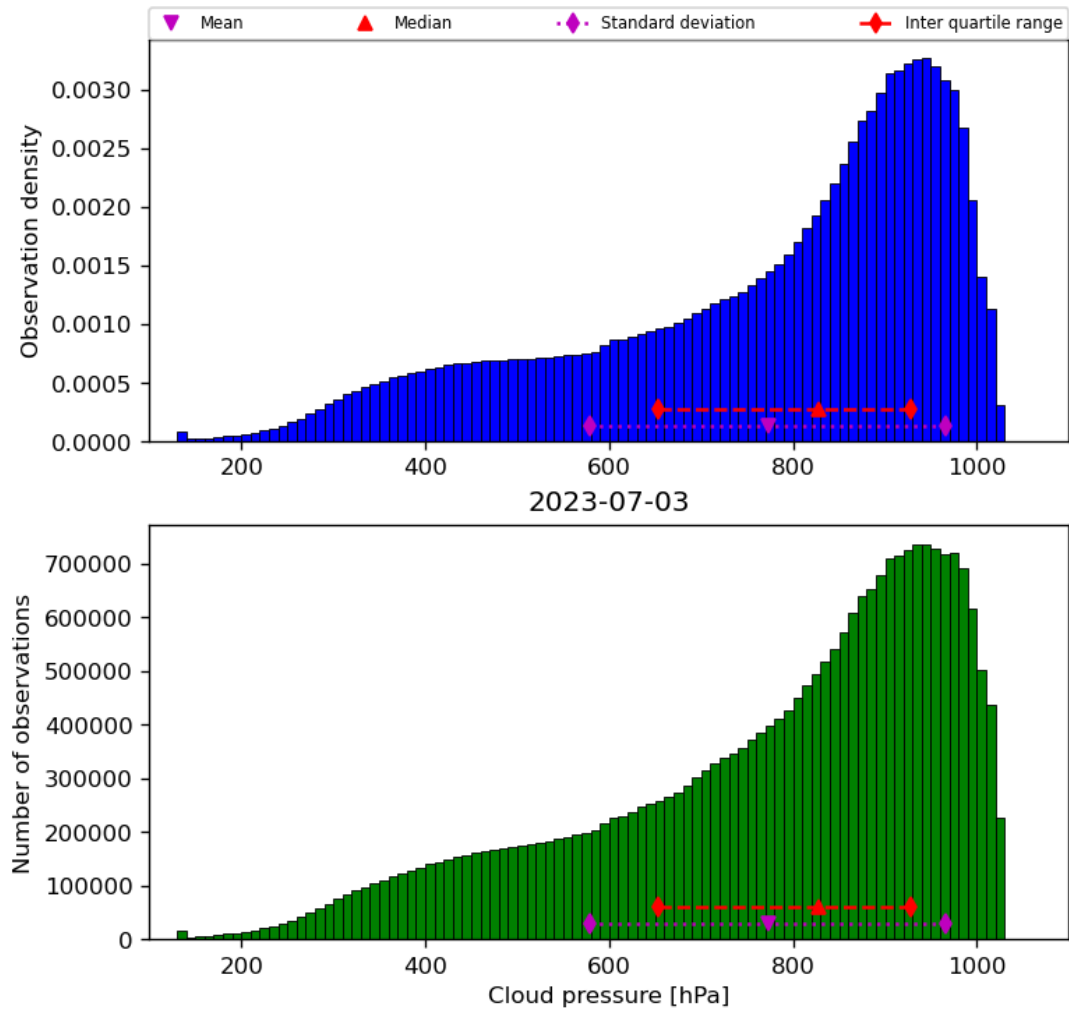
Figure 30: Histogram of “Cloud pressure” for 2023-07-03 to 2023-07-04
