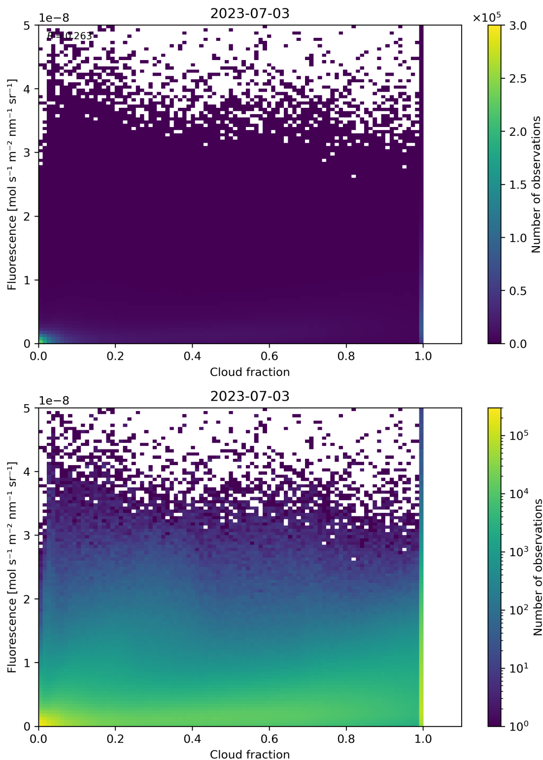
Figure 79: Scatter density plot of “Cloud fraction” against “Fluorescence” for 2023-07-03 to 2023-07-04.
