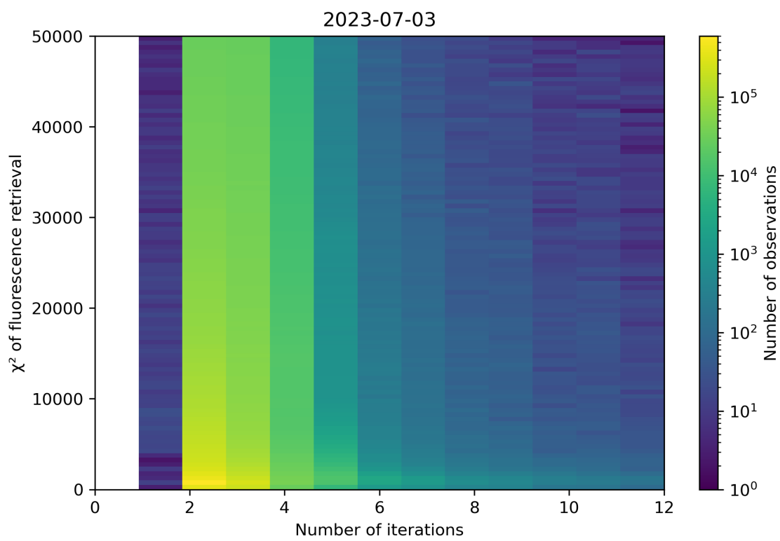
Figure 106: Scatter density plot of “Number of iterations” against “ \chi^2 of fluorescence retrieval” for 2023-07-03 to 2023-07-04.
