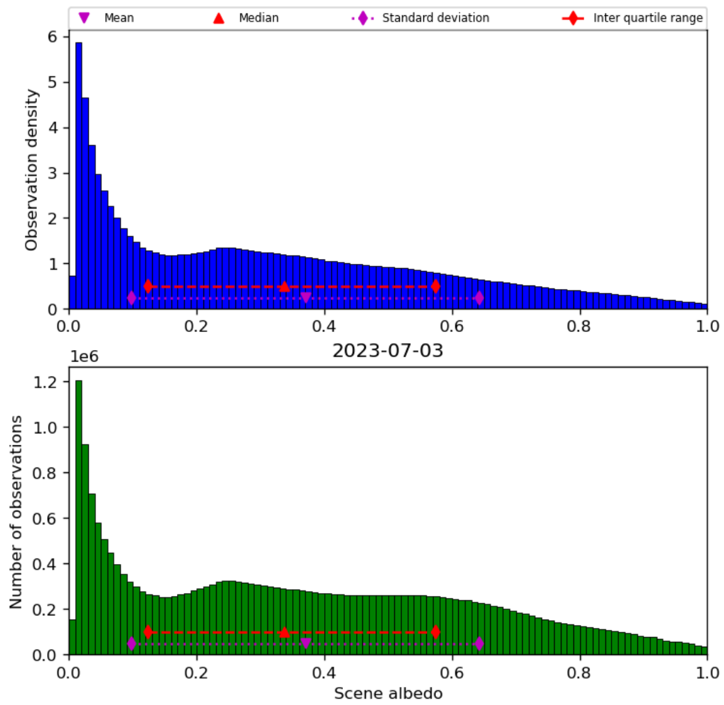
Figure 34: Histogram of “Scene albedo” for 2023-07-03 to 2023-07-04
