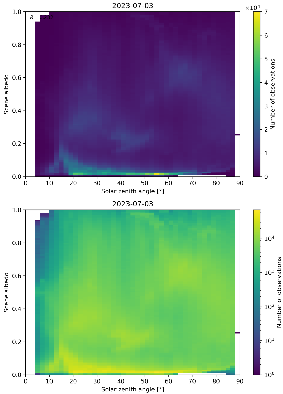
Figure 127: Scatter density plot of “Solar zenith angle” against “Scene albedo” for 2023-07-03 to 2023-07-04.
