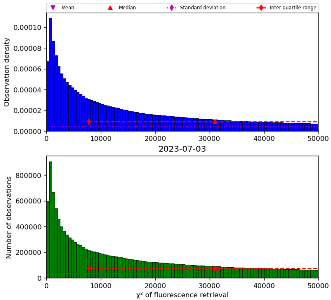
Figure 42: Histogram of “ \chi^2 of fluorescence retrieval” for 2023-07-03 to 2023-07-04
