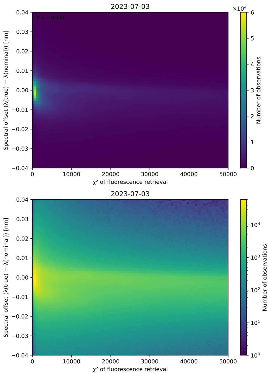
Figure 72: Scatter density plot of " \chi^2 of fluorescence retrieval" against "Spectral offset ( \lambda(\text{true}) - \lambda(\text{nominal})) " for 2023-07-03 to 2023-07-04.
