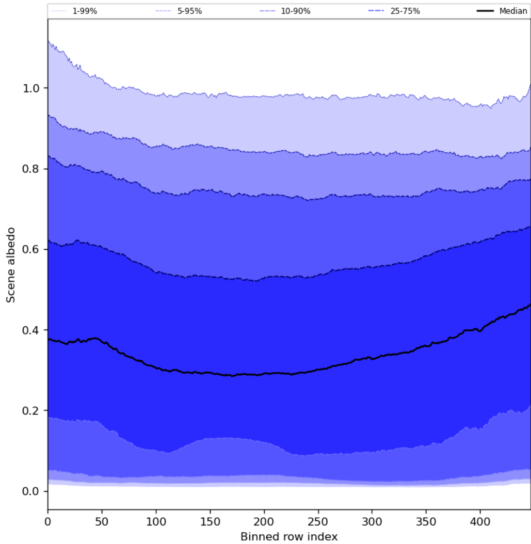
Figure 51: Along track statistics of “Scene albedo” for 2023-07-03 to 2023-07-04
