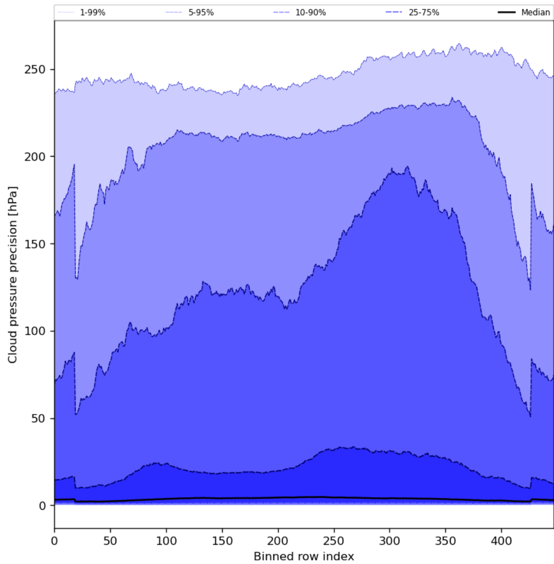
Figure 48: Along track statistics of “Cloud pressure precision” for 2023-07-03 to 2023-07-04
