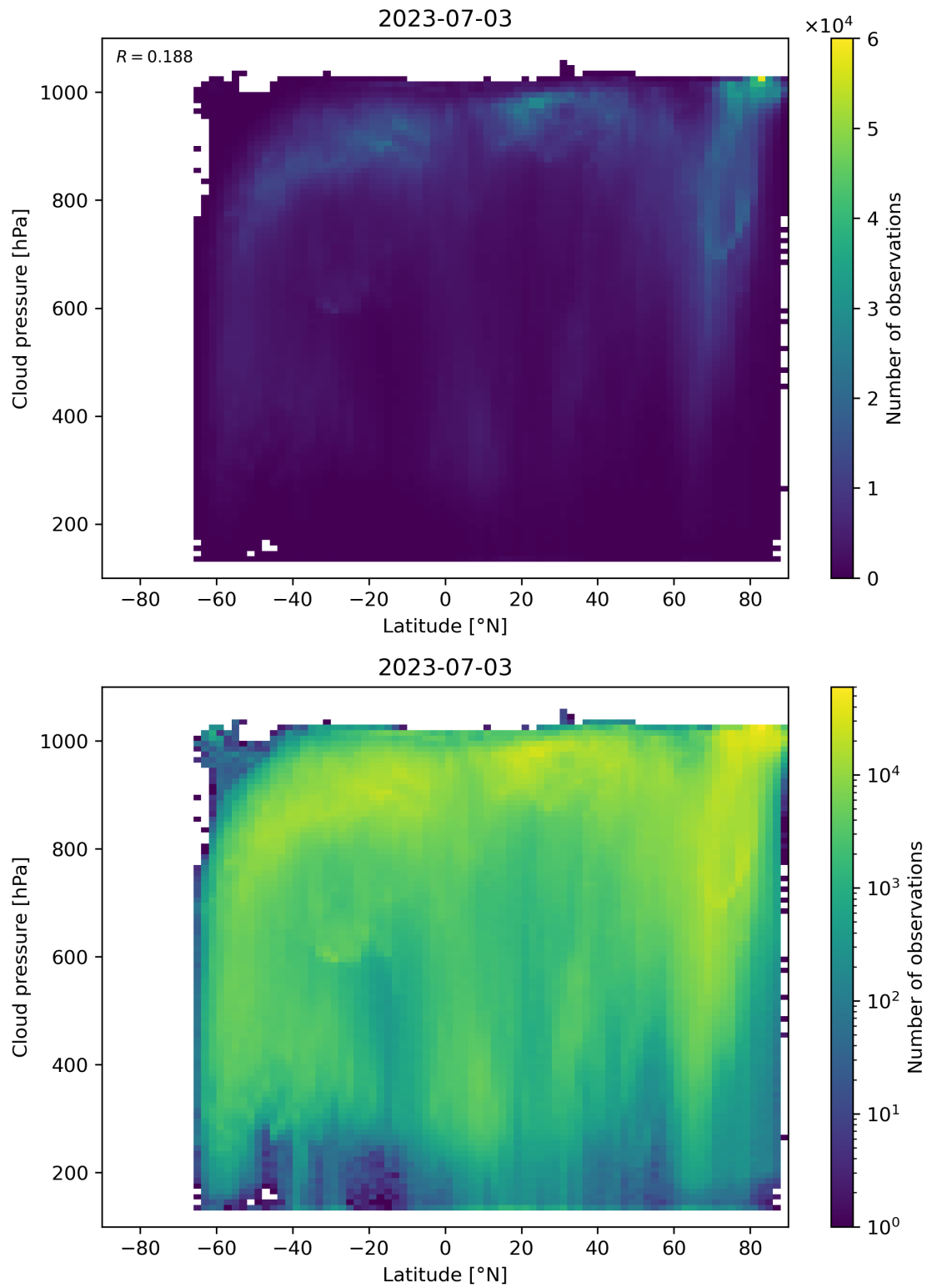
Figure 100: Scatter density plot of “Latitude” against “Cloud pressure” for 2023-07-03 to 2023-07-04.
