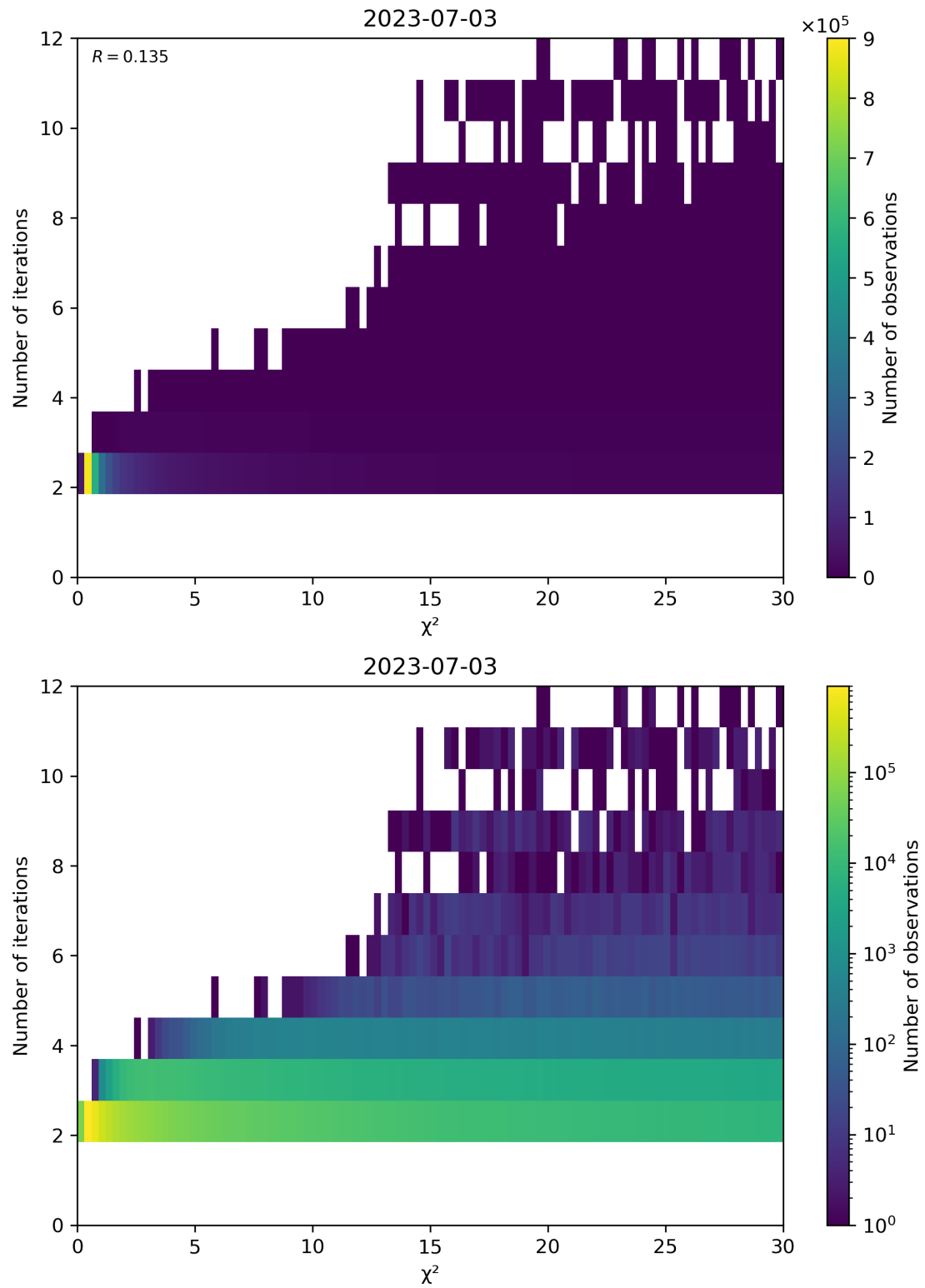
Figure 73: Scatter density plot of “ \chi^2 ” against “Number of iterations” for 2023-07-03 to 2023-07-04.
