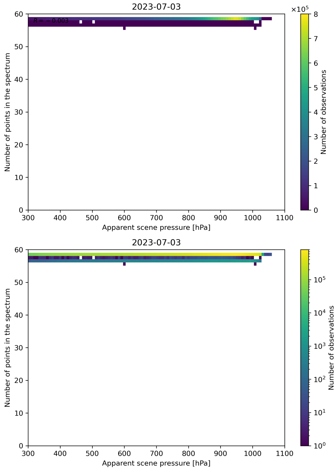
Figure 67: Scatter density plot of “Apparent scene pressure” against “Number of points in the spectrum” for 2023-07-03 to 2023-07-04.
