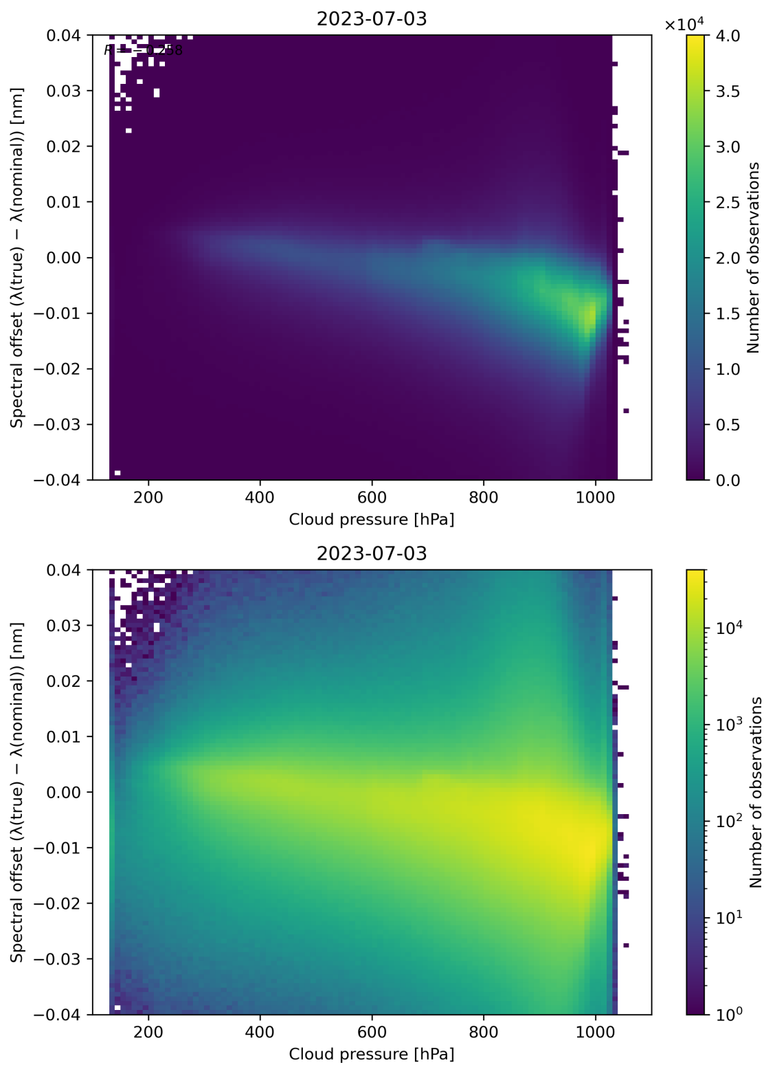
Figure 92: Scatter density plot of “Cloud pressure” against “Spectral offset ( \lambda(\text{true}) - \lambda(\text{nominal}) )” for 2023-07-03 to 2023-07-04.
