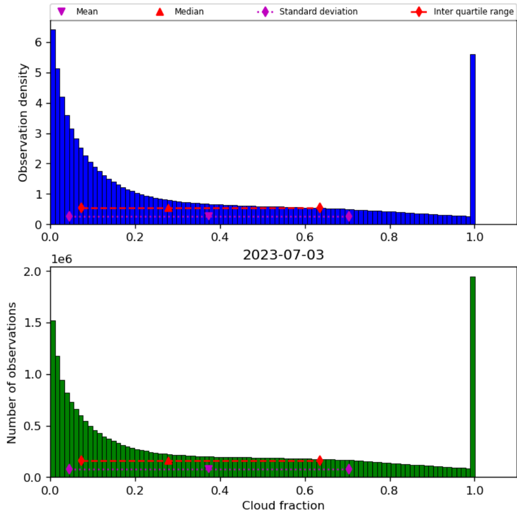
Figure 32: Histogram of “Cloud fraction” for 2023-07-03 to 2023-07-04
