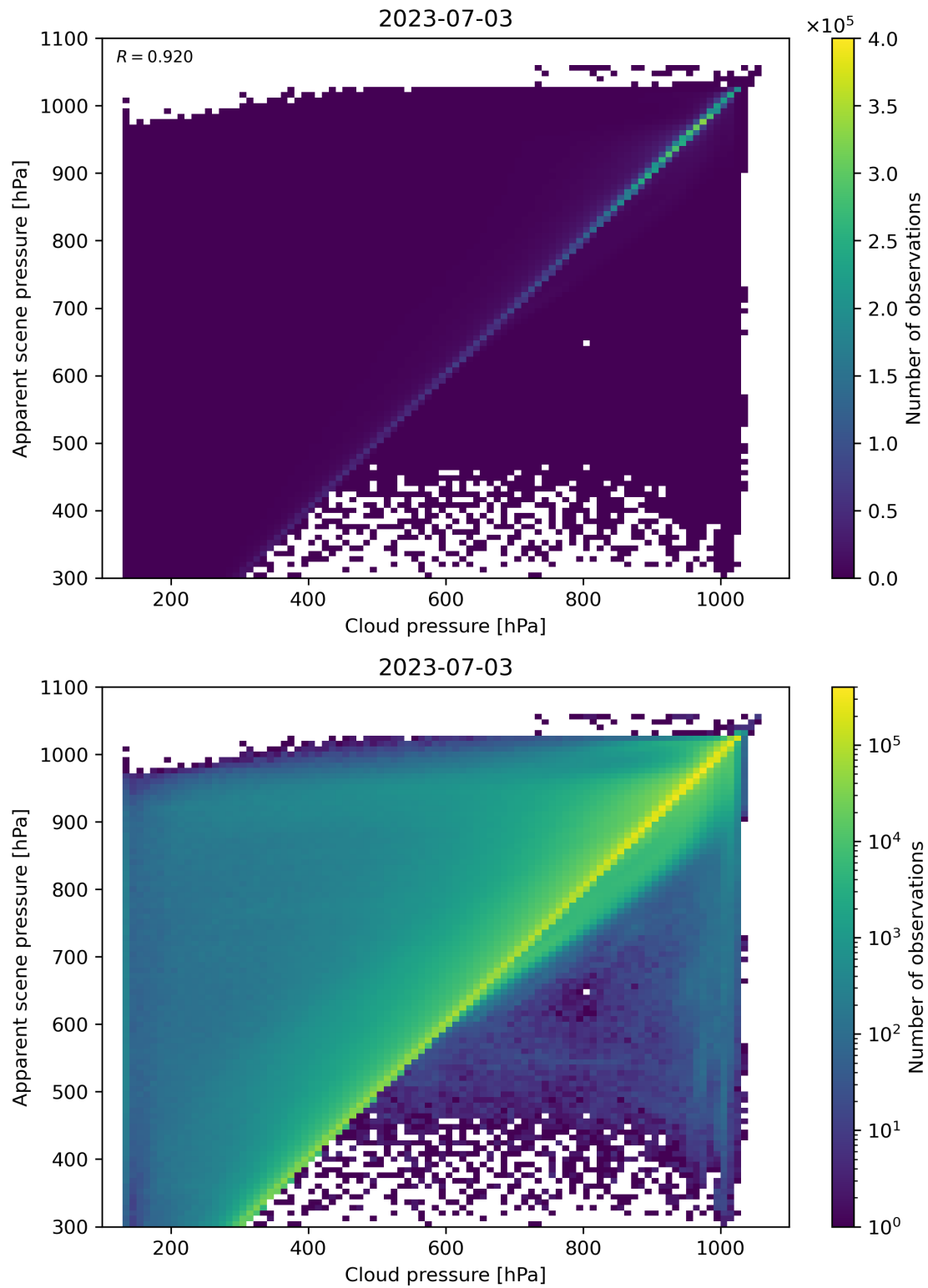
Figure 84: Scatter density plot of “Cloud pressure” against “Apparent scene pressure” for 2023-07-03 to 2023-07-04.
