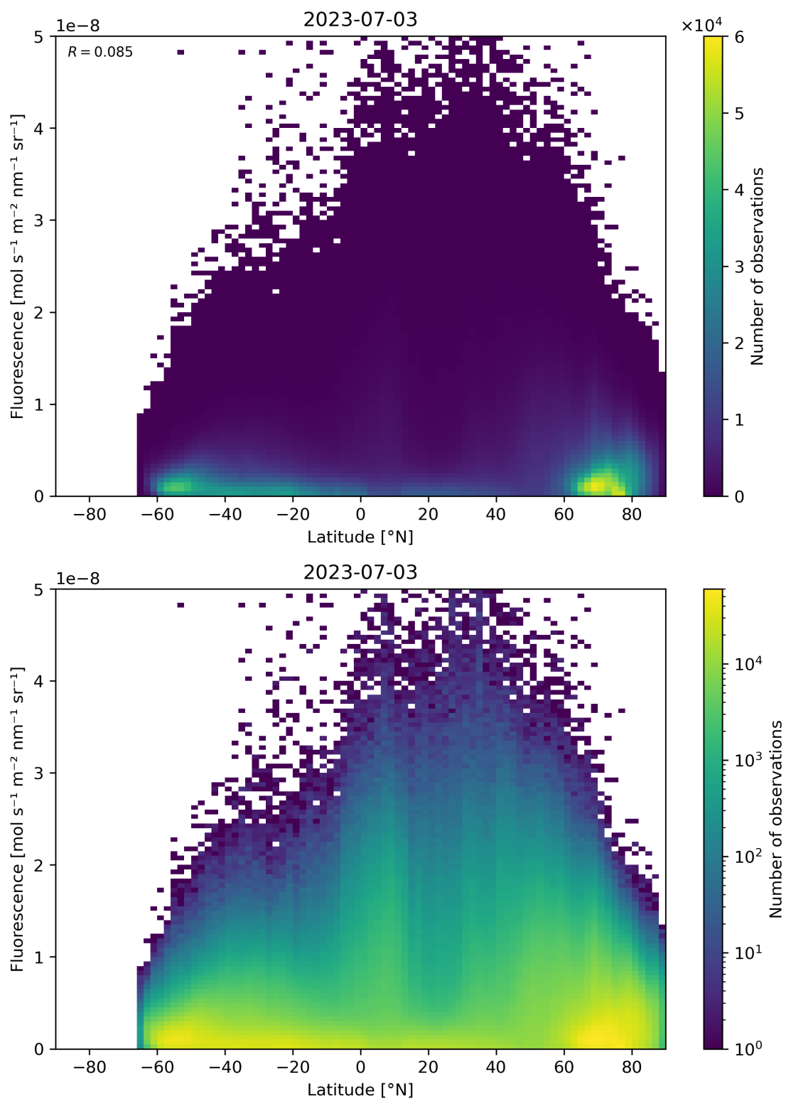
Figure 101: Scatter density plot of “Latitude” against “Fluorescence” for 2023-07-03 to 2023-07-04.
