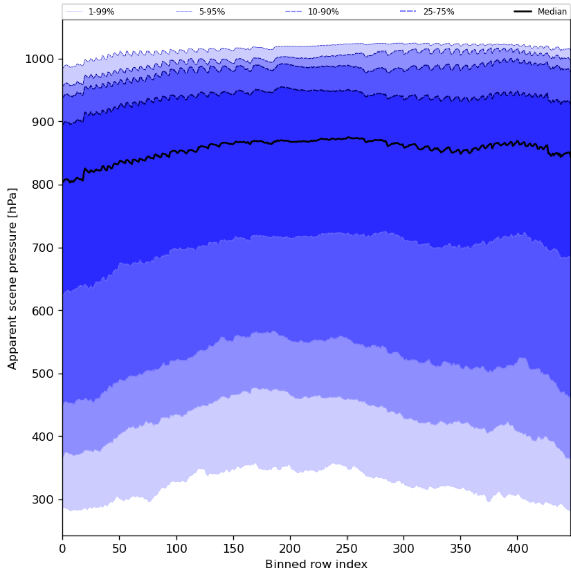
Figure 53: Along track statistics of “Apparent scene pressure” for 2023-07-03 to 2023-07-04
