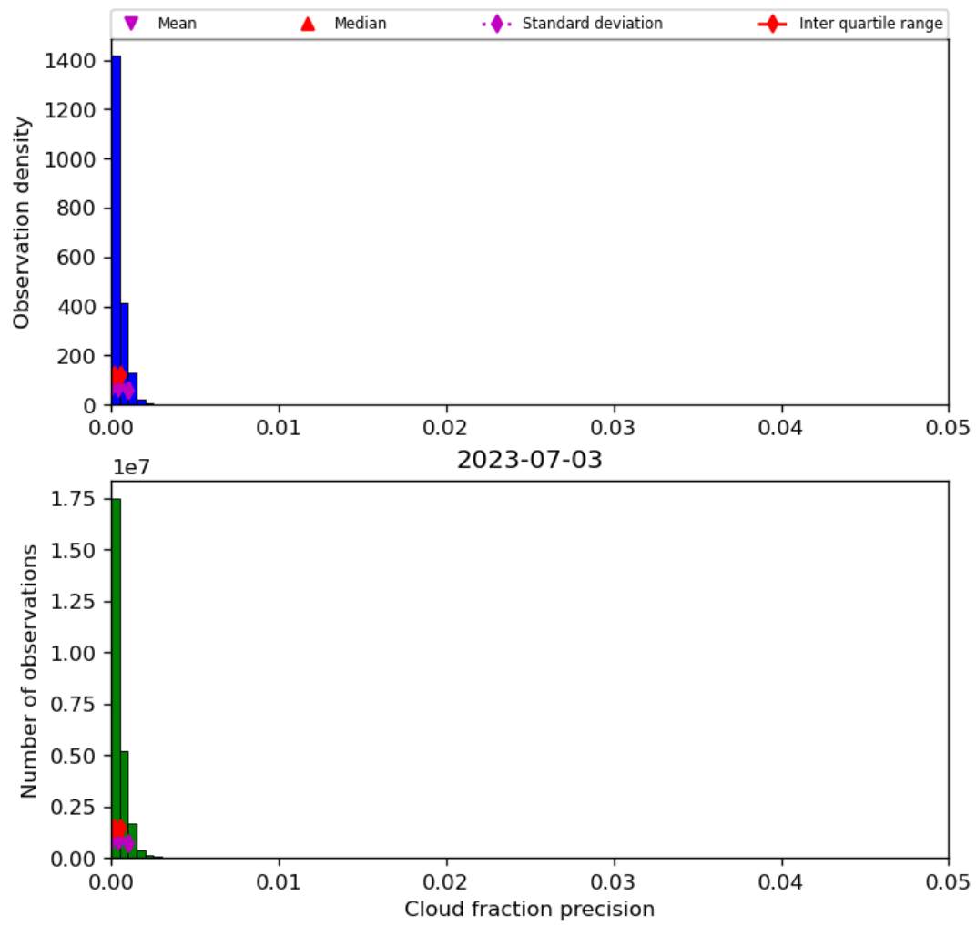
Figure 33: Histogram of “Cloud fraction precision” for 2023-07-03 to 2023-07-04
