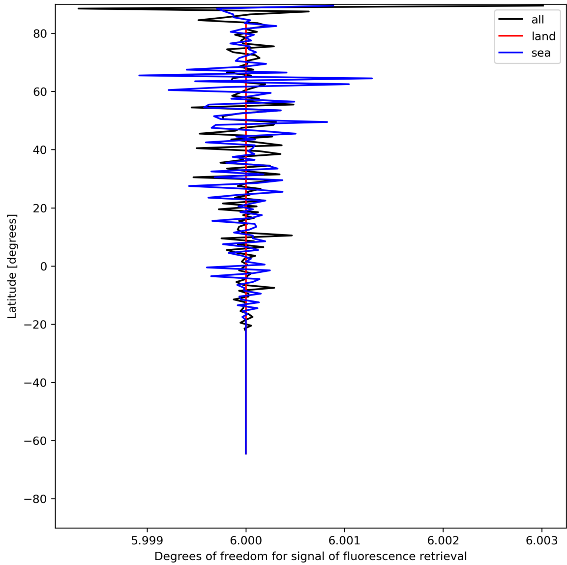
Figure 26: Zonal average of “Degrees of freedom for signal of fluorescence retrieval” for 2023-07-03 to 2023-07-04.
