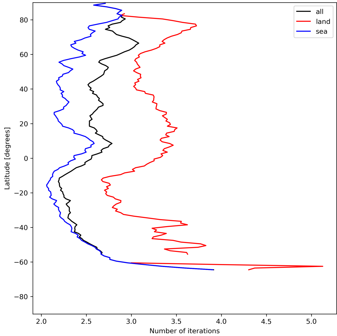
Figure 22: Zonal average of “Number of iterations” for 2023-07-03 to 2023-07-04.
