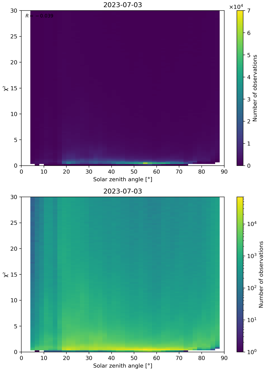
Figure 119: Scatter density plot of “Solar zenith angle” against “ \chi^2 ” for 2023-07-03 to 2023-07-04.
