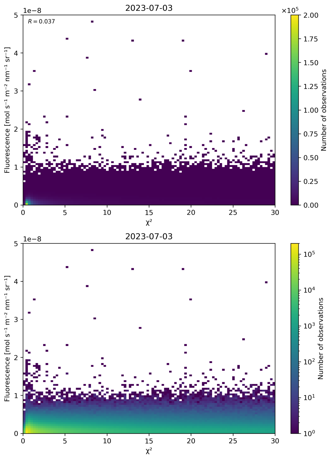
Figure 70: Scatter density plot of “ \chi^2 ” against “Fluorescence” for 2023-07-03 to 2023-07-04.
