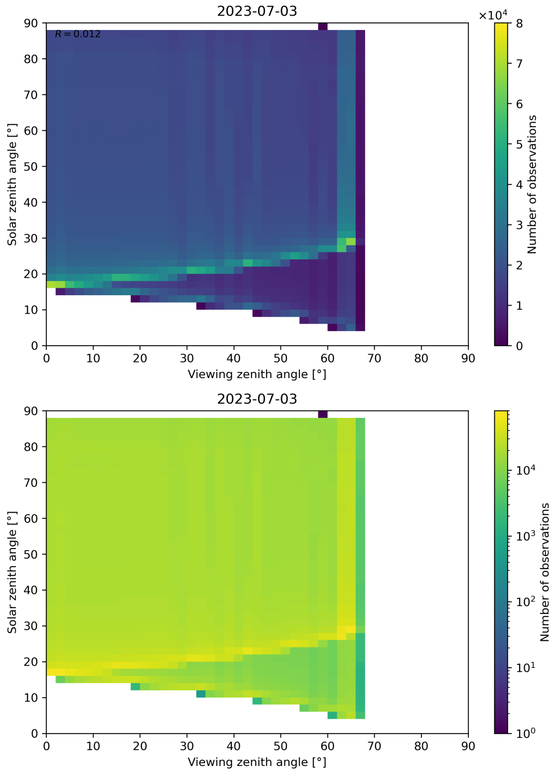
Figure 139: Scatter density plot of “Viewing zenith angle” against “Solar zenith angle” for 2023-07-03 to 2023-07-04.
