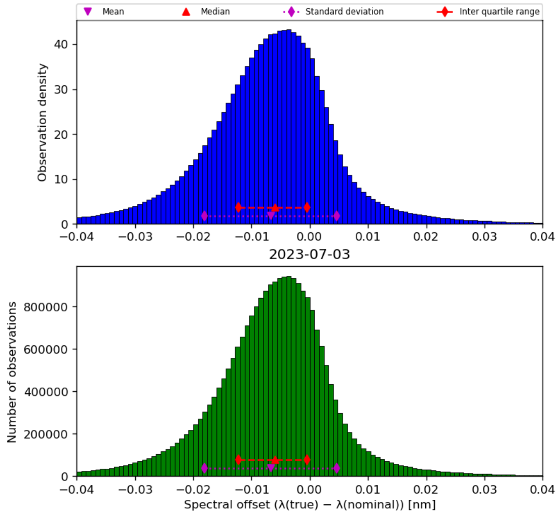
Figure 45: Histogram of “Spectral offset ( \lambda(\text{true}) - \lambda(\text{nominal}) )” for 2023-07-03 to 2023-07-04
