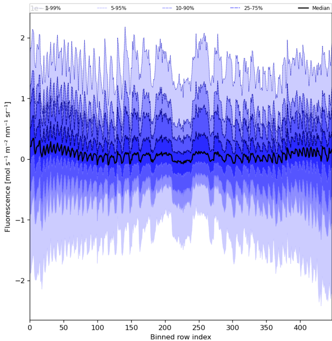
Figure 57: Along track statistics of “Fluorescence” for 2023-07-03 to 2023-07-04
