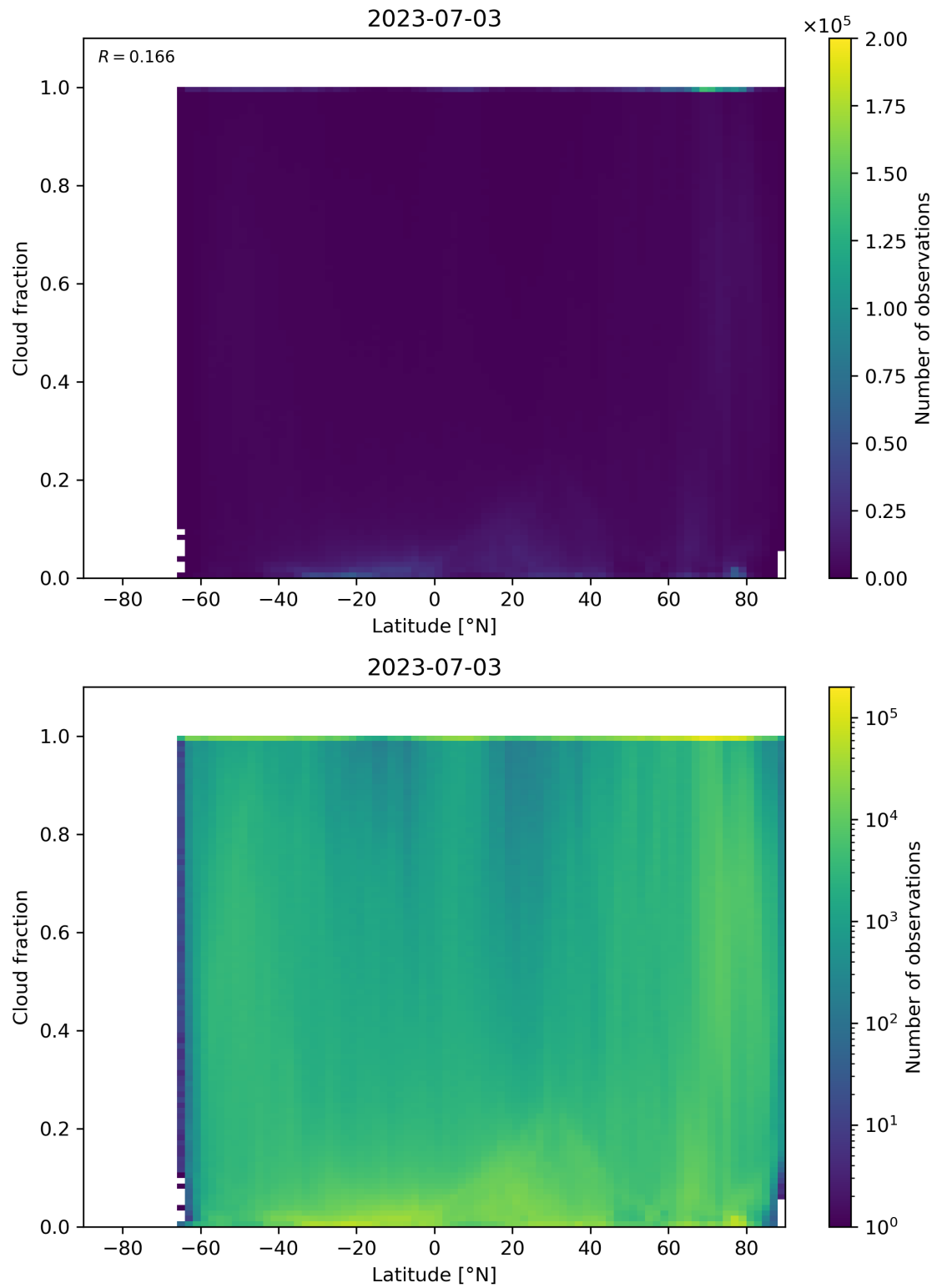
Figure 99: Scatter density plot of “Latitude” against “Cloud fraction” for 2023-07-03 to 2023-07-04.
