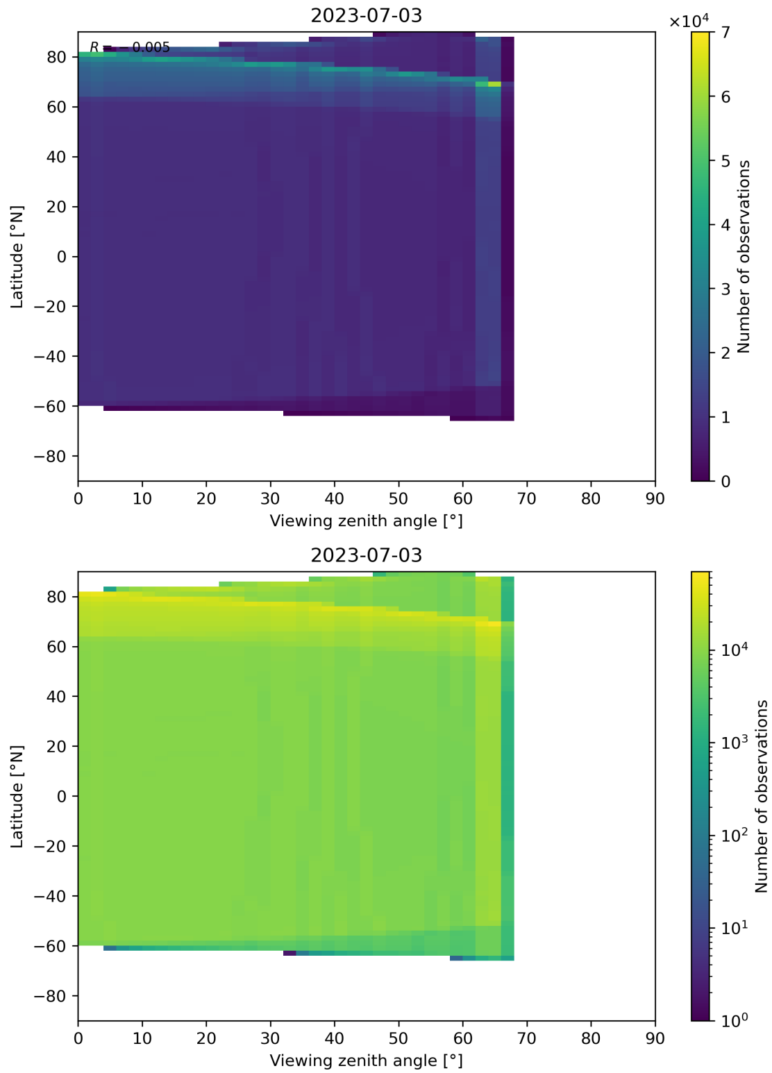
Figure 135: Scatter density plot of “Viewing zenith angle” against “Latitude” for 2023-07-03 to 2023-07-04.
