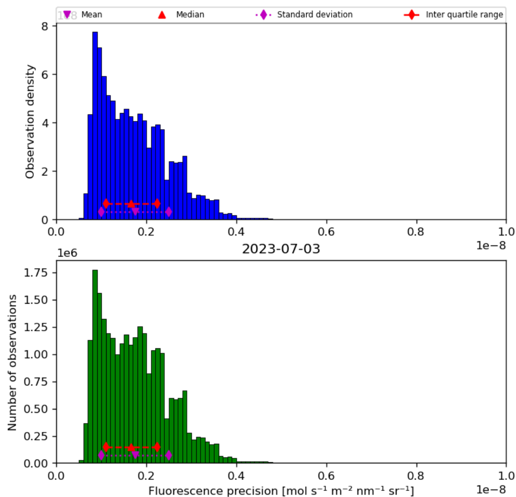
Figure 41: Histogram of “Fluorescence precision” for 2023-07-03 to 2023-07-04
