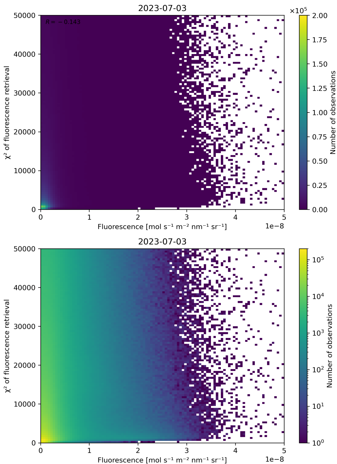
Figure 93: Scatter density plot of “Fluorescence” against “ \chi^2 of fluorescence retrieval” for 2023-07-03 to 2023-07-04.
