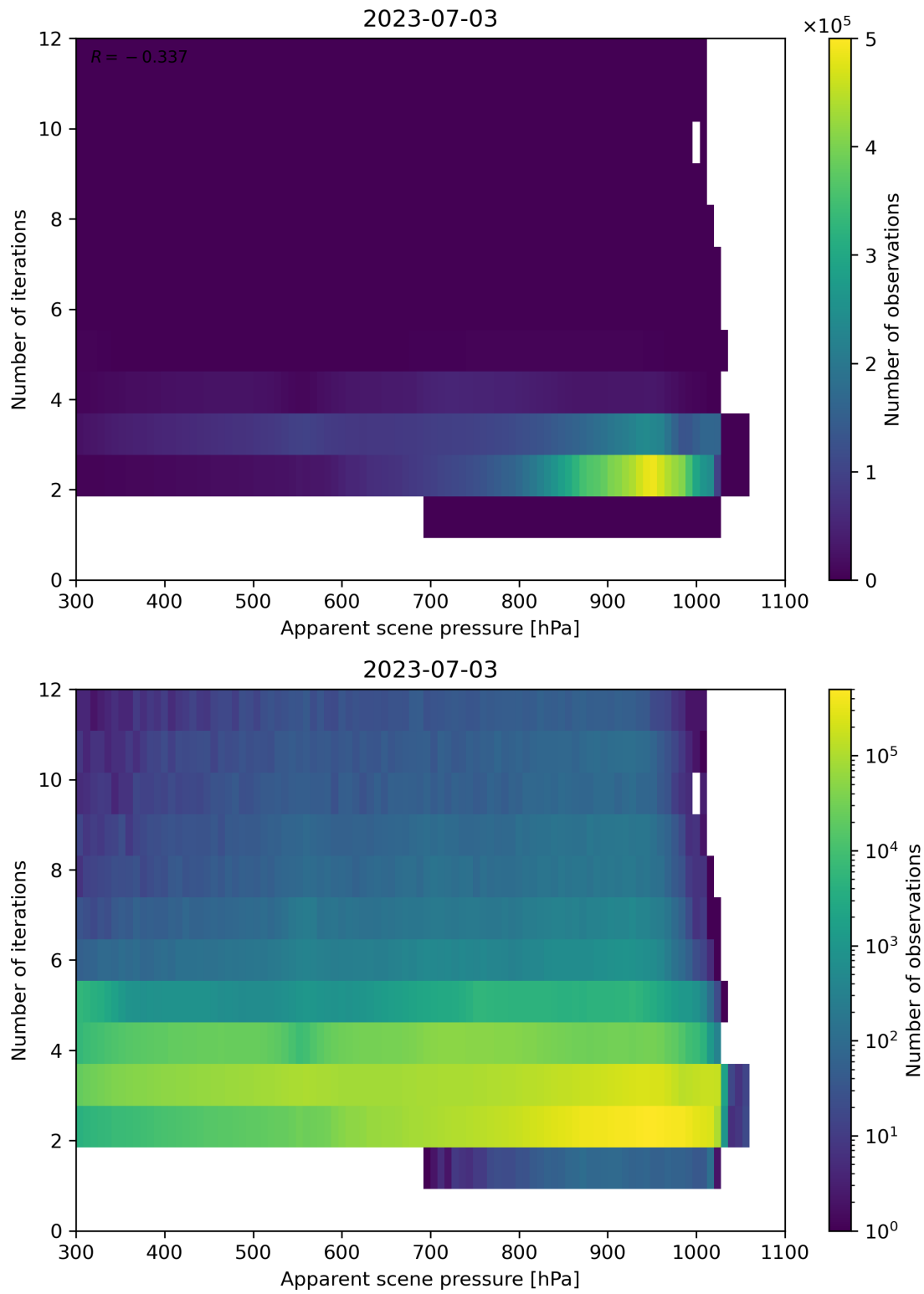
Figure 66: Scatter density plot of “Apparent scene pressure” against “Number of iterations” for 2023-07-03 to 2023-07-04.
