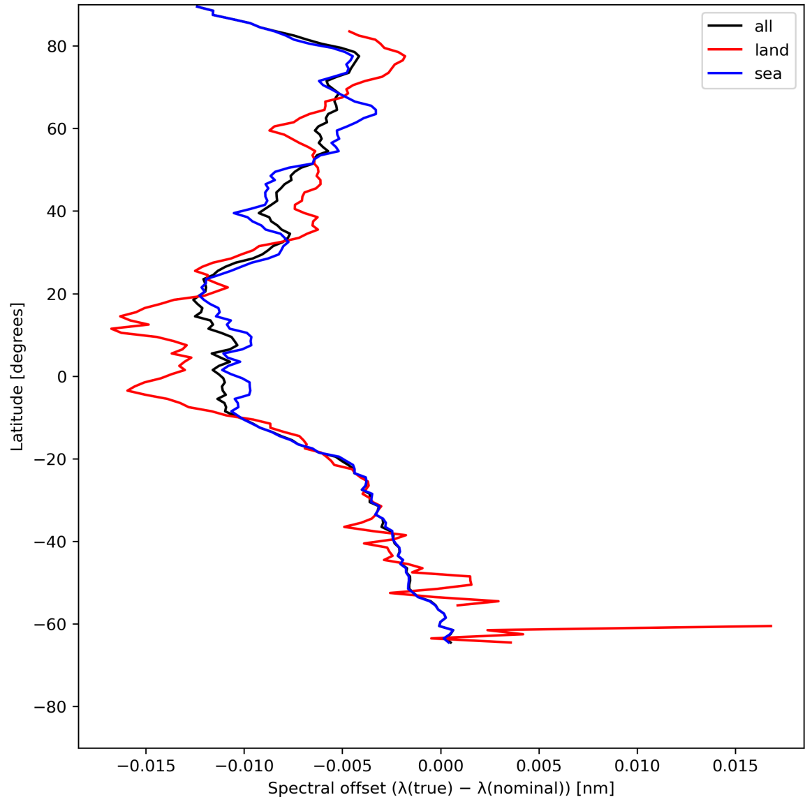
Figure 28: Zonal average of “Spectral offset ( \lambda(\text{true}) - \lambda(\text{nominal}) )” for 2023-07-03 to 2023-07-04.
