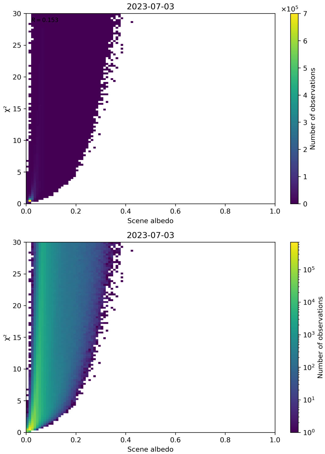
Figure 112: Scatter density plot of “Scene albedo” against “ \chi^2 ” for 2023-07-03 to 2023-07-04.
