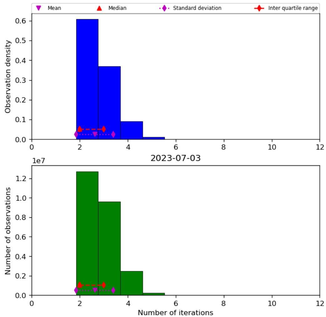
Figure 39: Histogram of “Number of iterations” for 2023-07-03 to 2023-07-04
