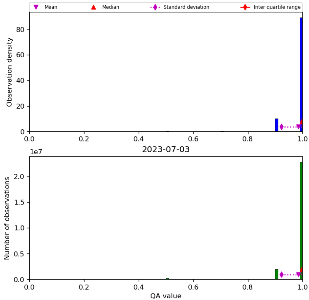
Figure 29: Histogram of “QA value” for 2023-07-03 to 2023-07-04
