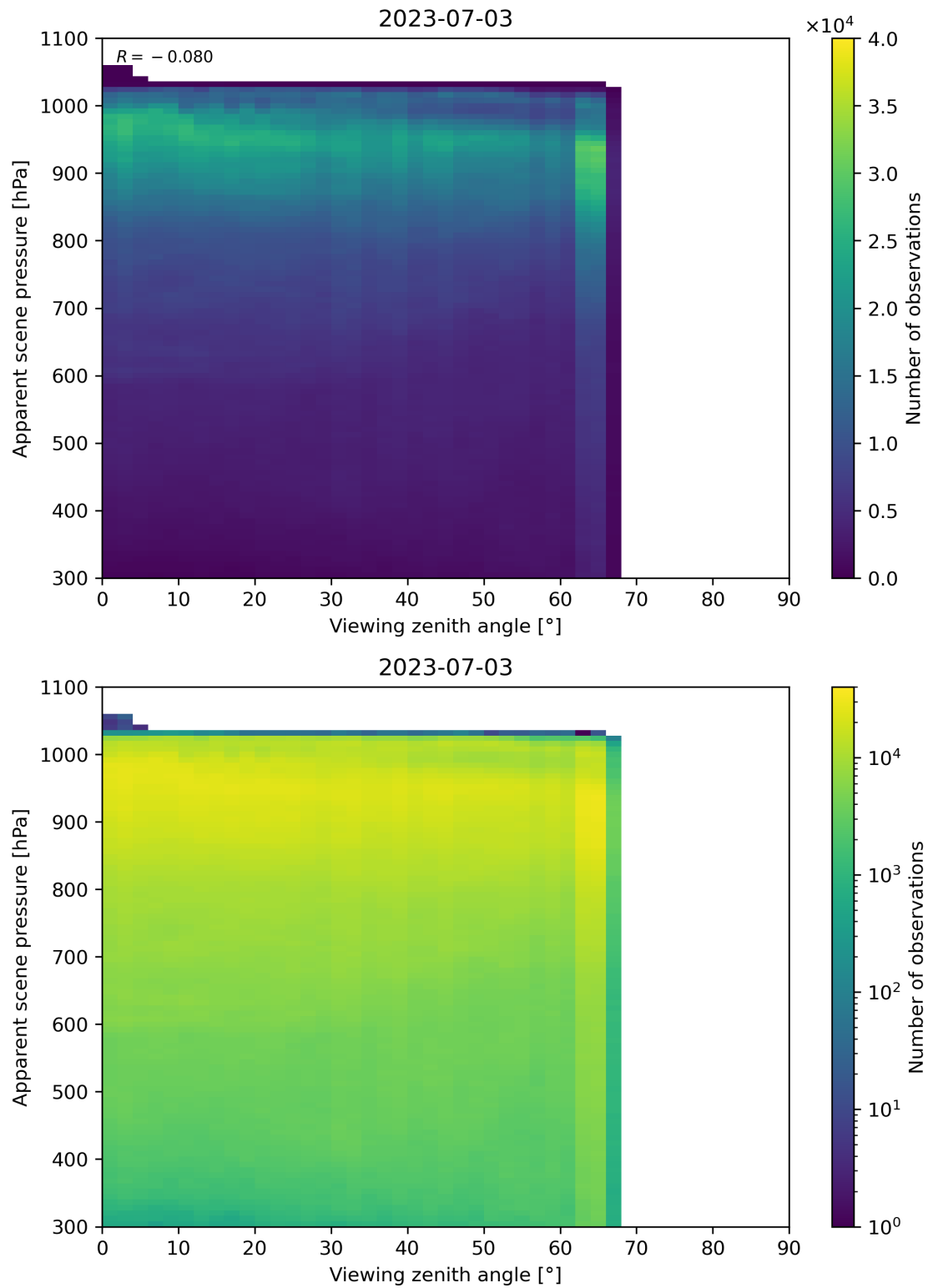
Figure 129: Scatter density plot of “Viewing zenith angle” against “Apparent scene pressure” for 2023-07-03 to 2023-07-04.
