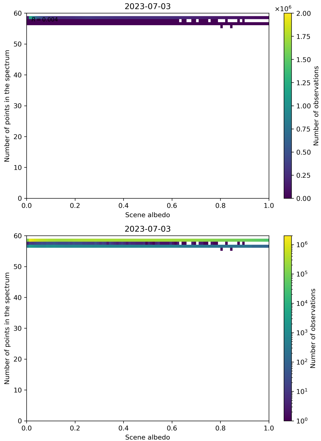
Figure 116: Scatter density plot of “Scene albedo” against “Number of points in the spectrum” for 2023-07-03 to 2023-07-04.
