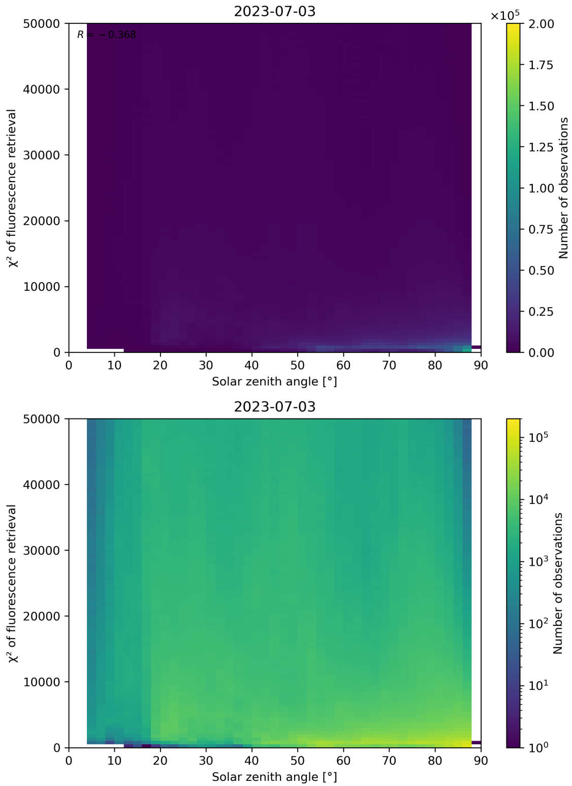
Figure 120: Scatter density plot of “Solar zenith angle” against “ \chi^2 of fluorescence retrieval” for 2023-07-03 to 2023-07-04.
