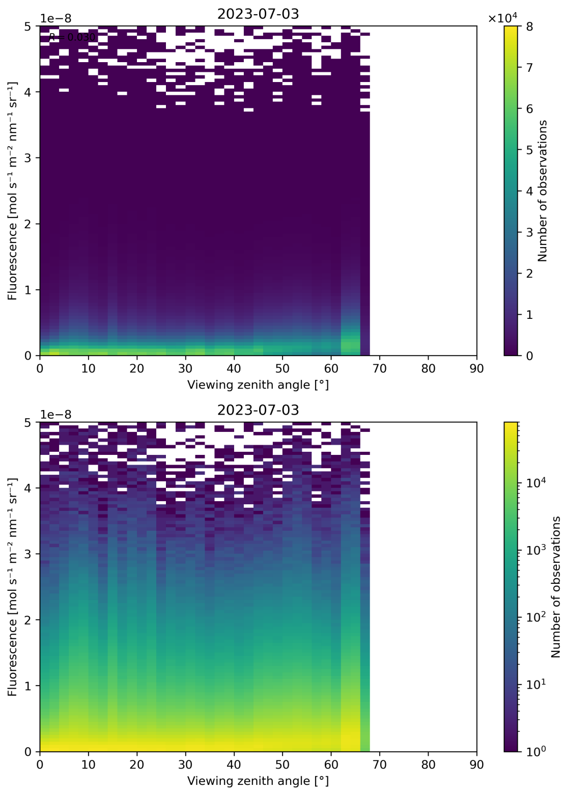
Figure 134: Scatter density plot of “Viewing zenith angle” against “Fluorescence” for 2023-07-03 to 2023-07-04.
