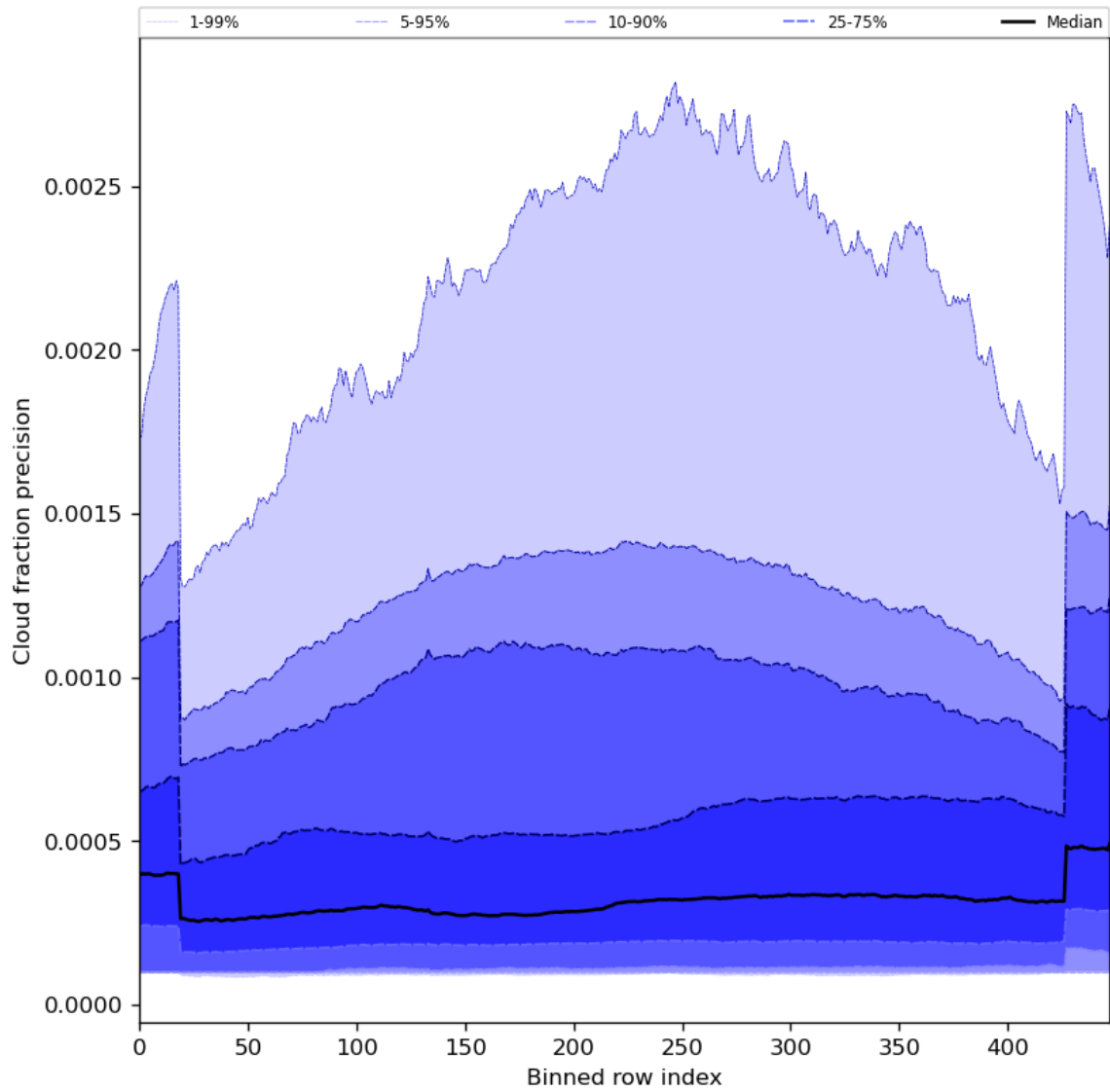
Figure 50: Along track statistics of “Cloud fraction precision” for 2023-07-03 to 2023-07-04
