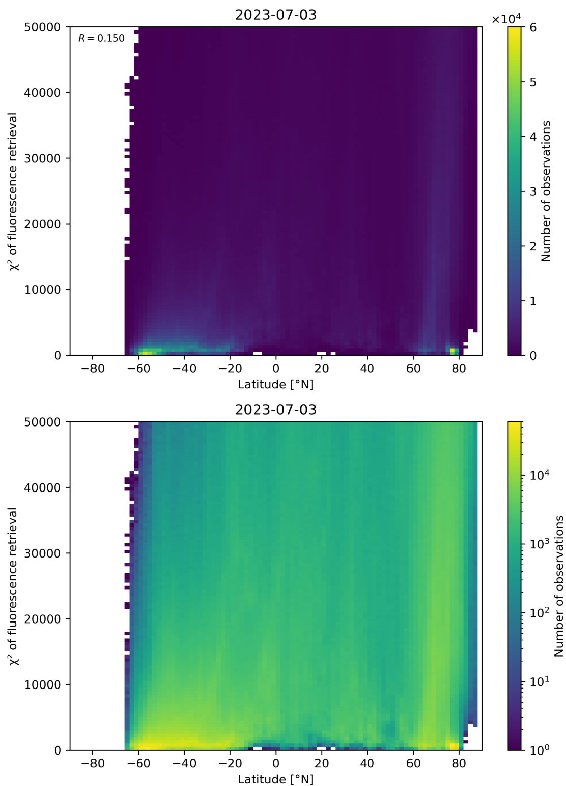
Figure 98: Scatter density plot of “Latitude” against “ \chi^2 of fluorescence retrieval” for 2023-07-03 to 2023-07-04.
