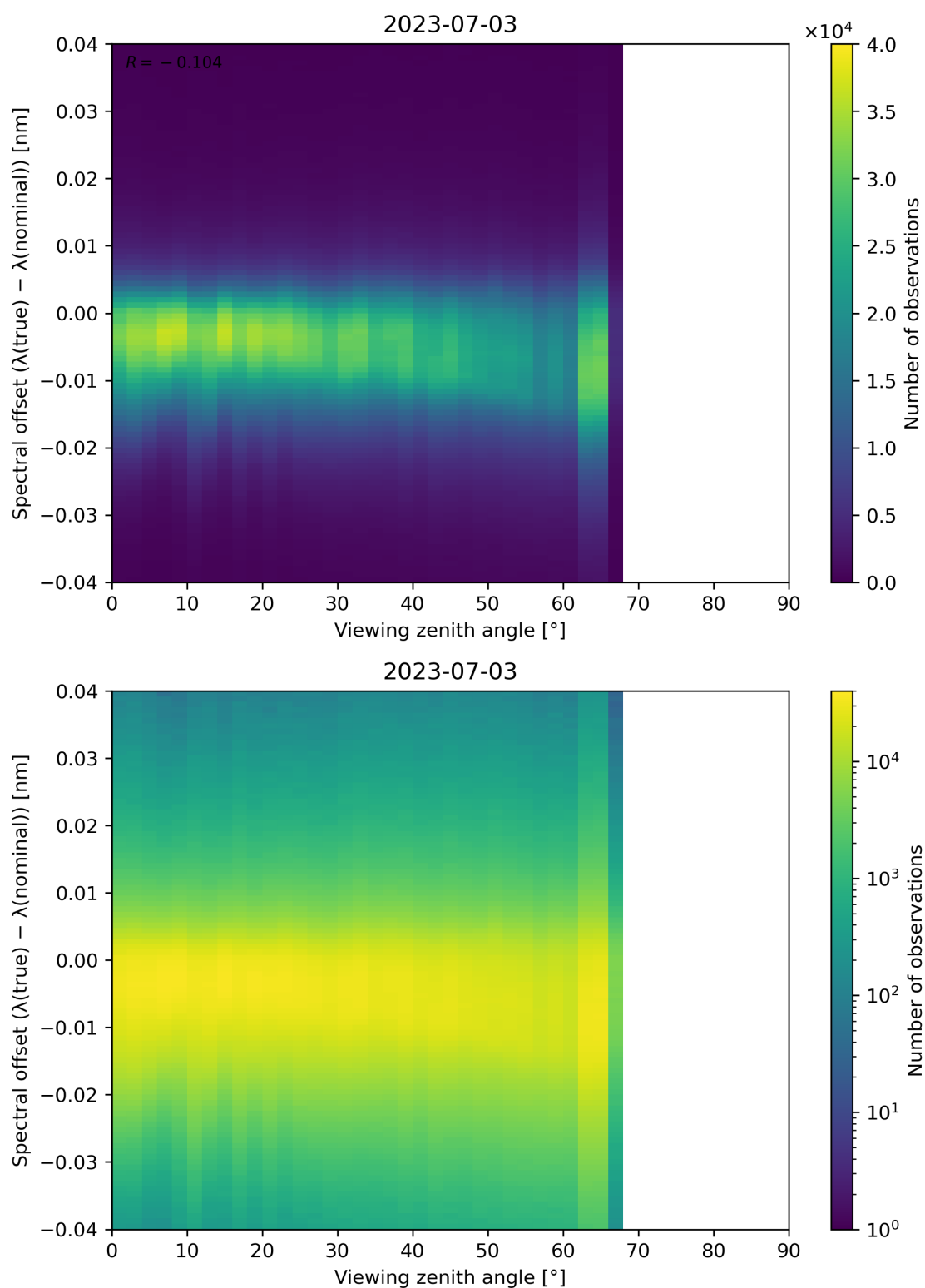
Figure 140: Scatter density plot of “Viewing zenith angle” against “Spectral offset ( \lambda(\text{true}) - \lambda(\text{nominal}) )” for 2023-07-03 to 2023-07-04.
