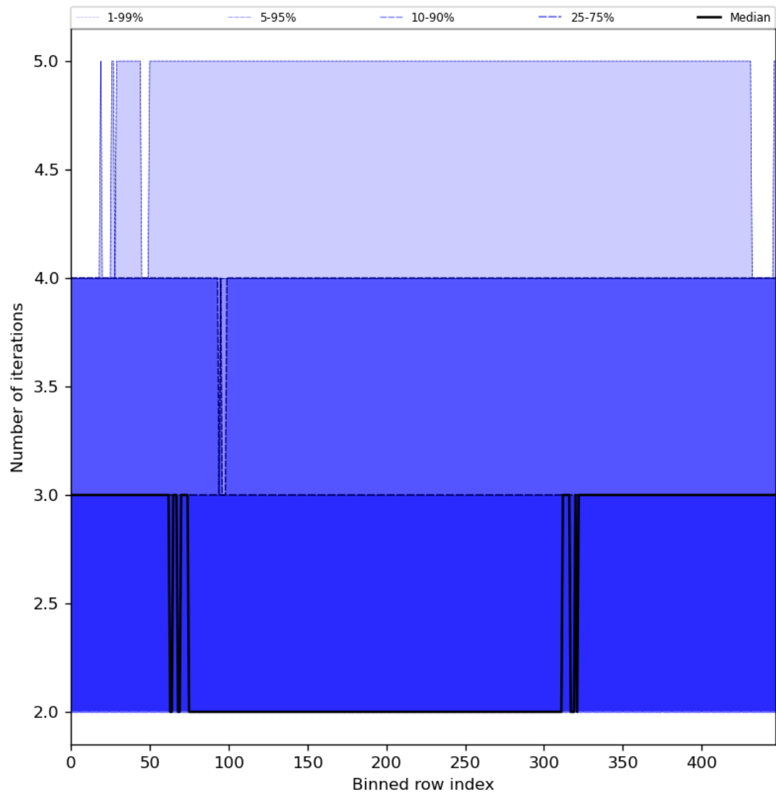
Figure 56: Along track statistics of “Number of iterations” for 2023-07-03 to 2023-07-04
