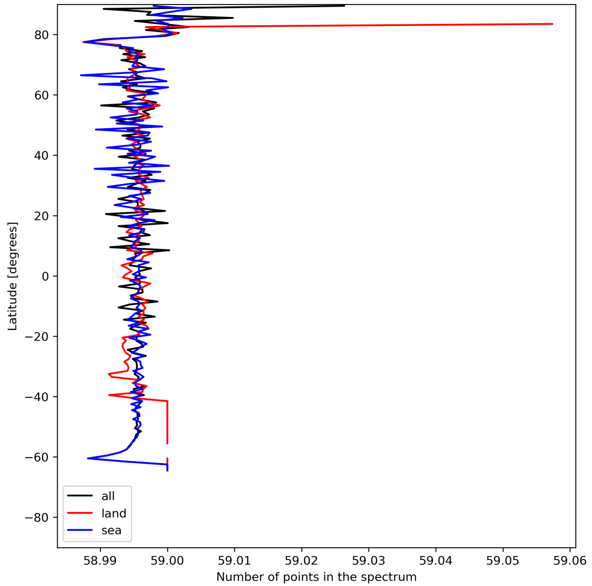
Figure 27: Zonal average of “Number of points in the spectrum” for 2023-07-03 to 2023-07-04.
