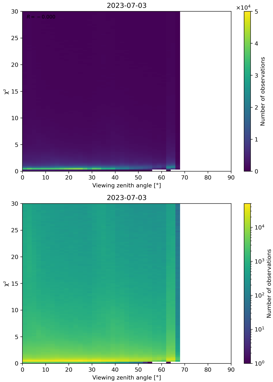
Figure 130: Scatter density plot of “Viewing zenith angle” against “ \chi^2 ” for 2023-07-03 to 2023-07-04.
