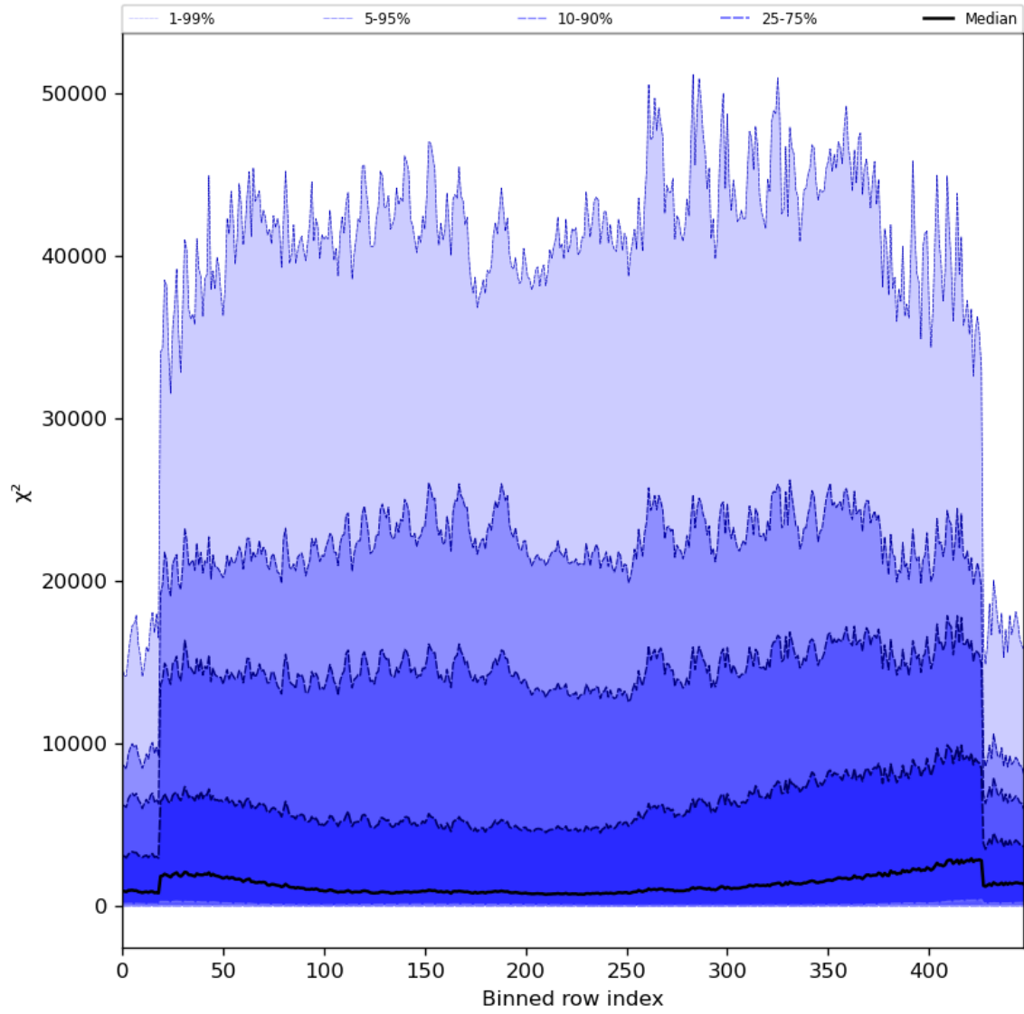
Figure 55: Along track statistics of “ \chi^2 ” for 2023-07-03 to 2023-07-04
