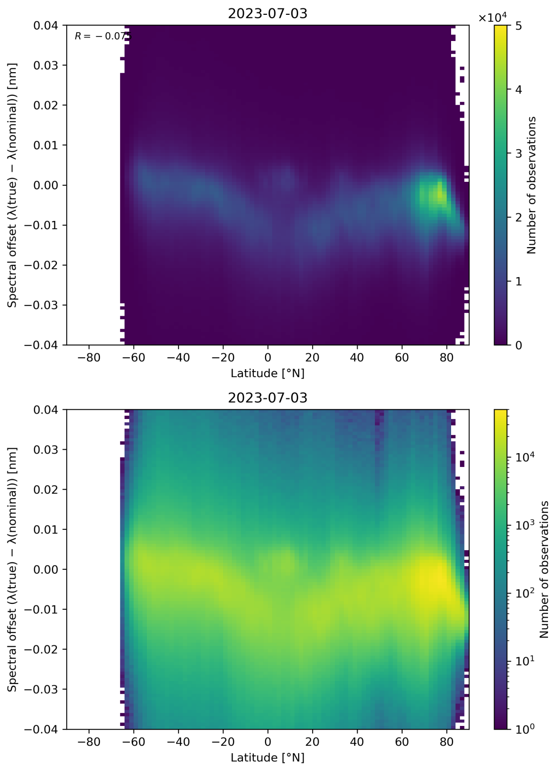
Figure 105: Scatter density plot of “Latitude” against “Spectral offset ( \lambda(\text{true}) - \lambda(\text{nominal}) )” for 2023-07-03 to 2023-07-04.
