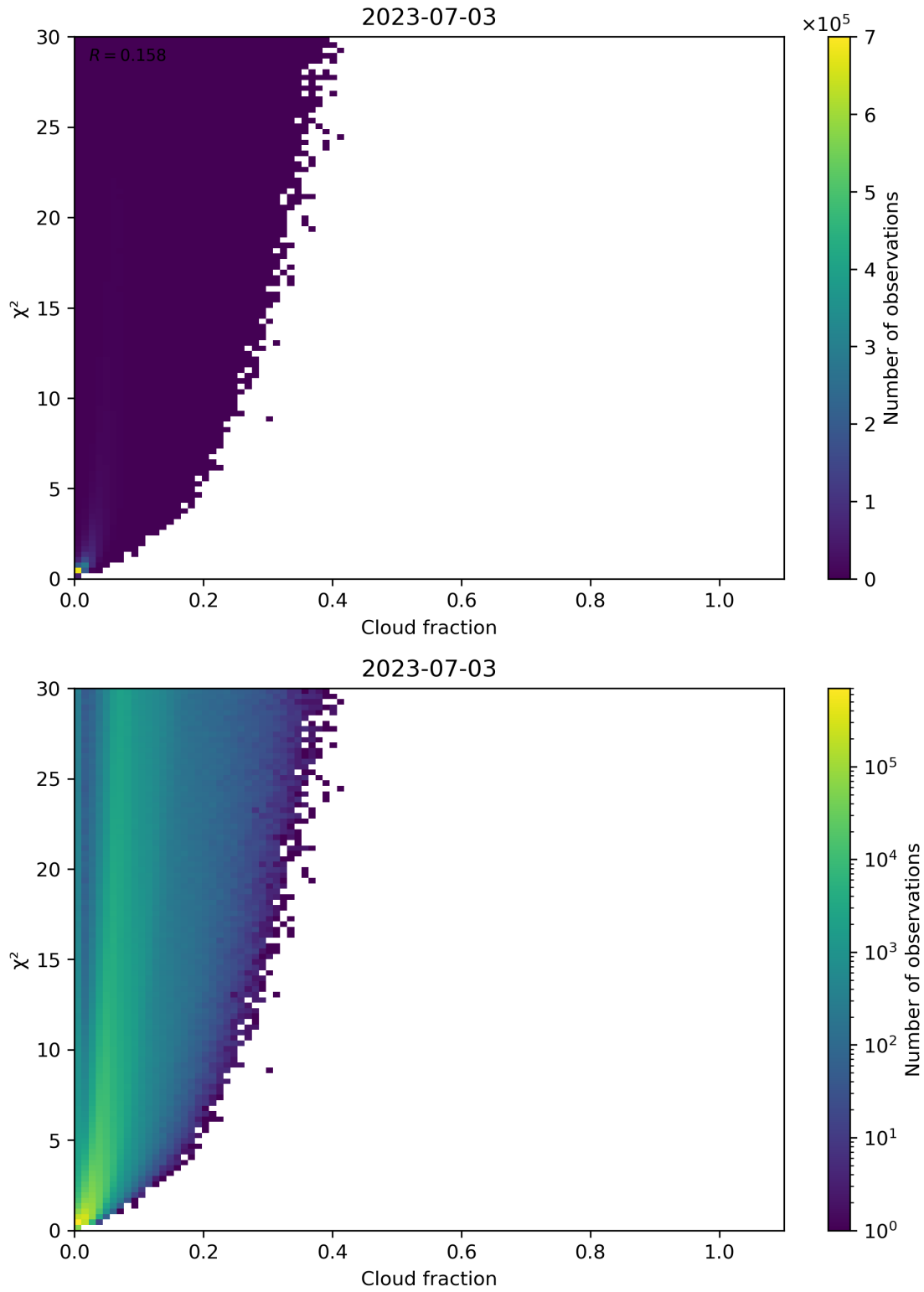
Figure 77: Scatter density plot of “Cloud fraction” against “ \chi^2 ” for 2023-07-03 to 2023-07-04.
