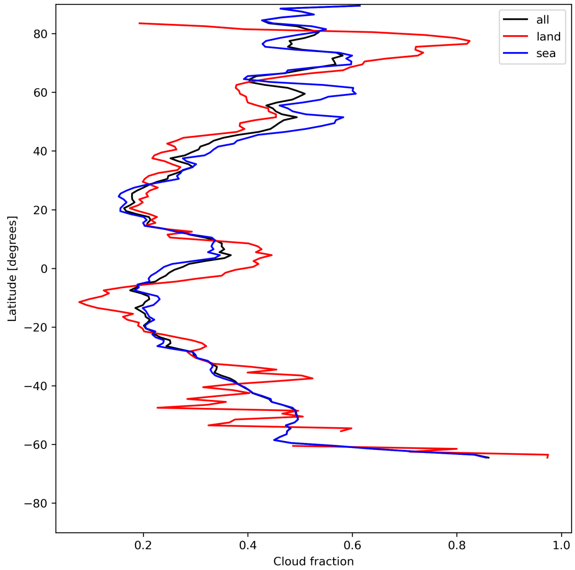
Figure 15: Zonal average of “Cloud fraction” for 2023-07-03 to 2023-07-04.
