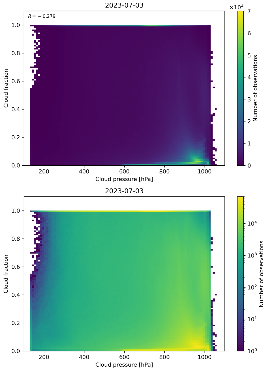
Figure 87: Scatter density plot of “Cloud pressure” against “Cloud fraction” for 2023-07-03 to 2023-07-04.
