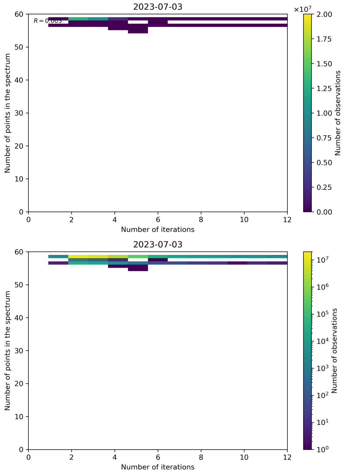
Figure 108: Scatter density plot of “Number of iterations” against “Number of points in the spectrum” for 2023-07-03 to 2023-07-04.
