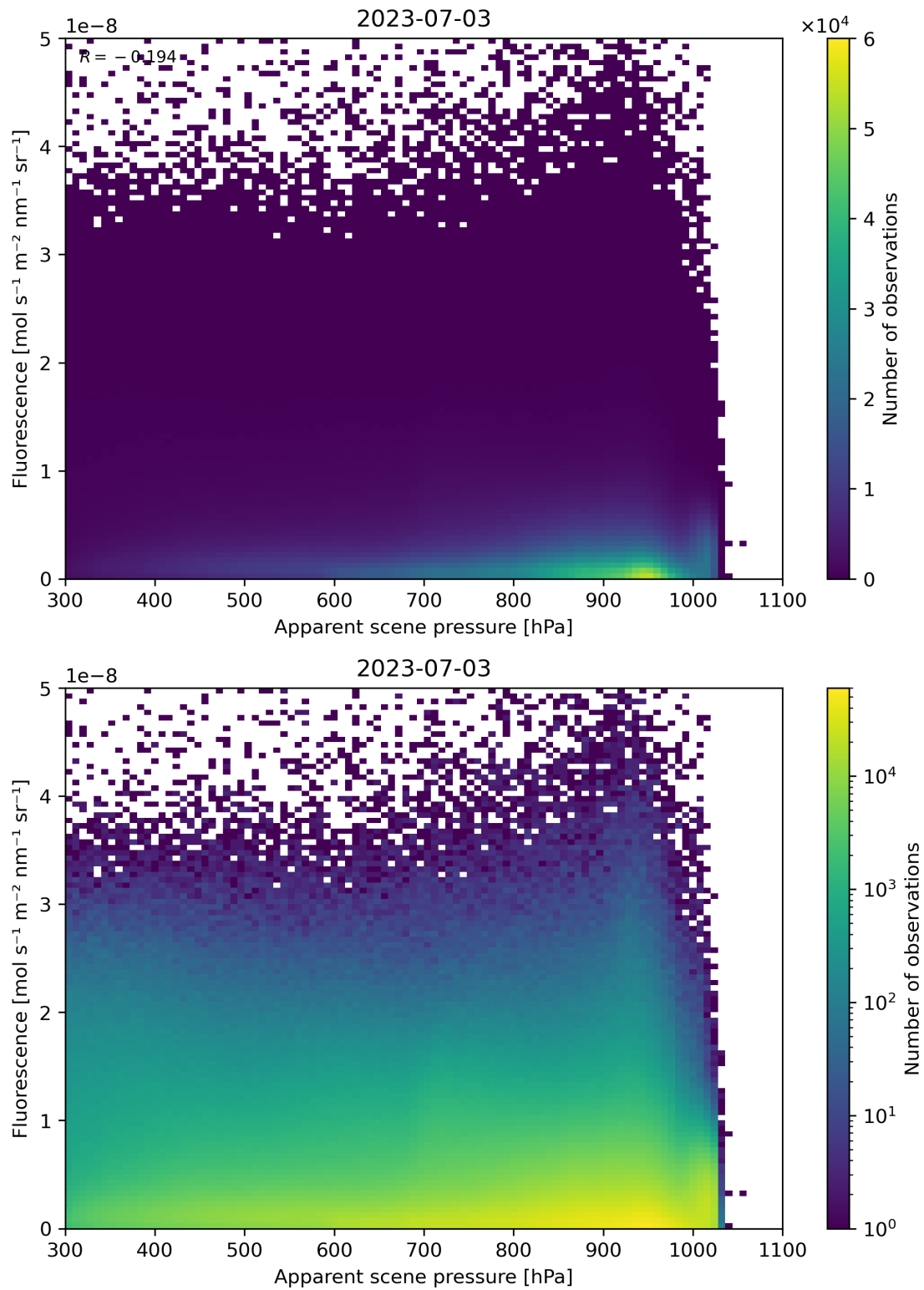
Figure 65: Scatter density plot of “Apparent scene pressure” against “Fluorescence” for 2023-07-03 to 2023-07-04.
