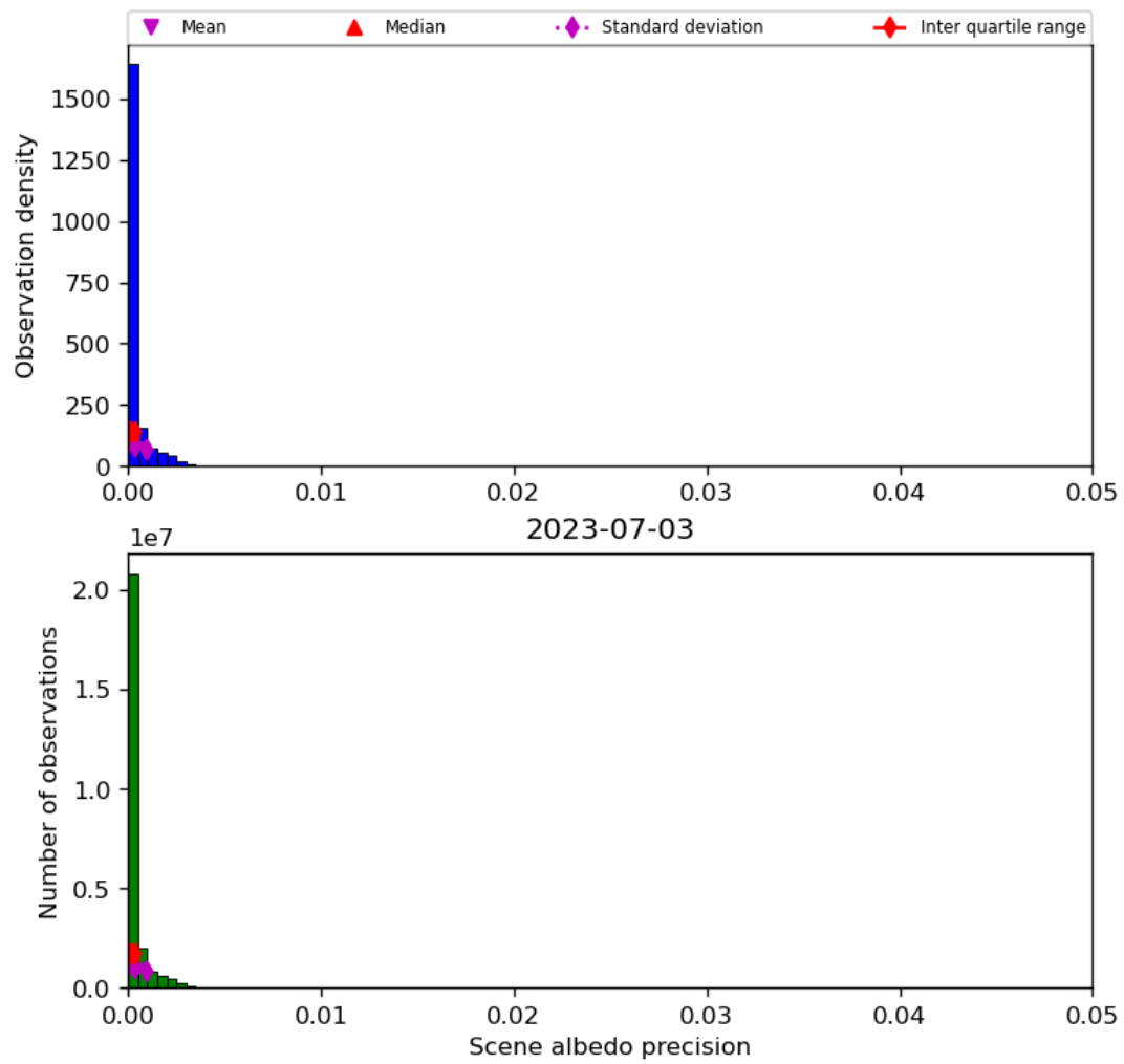
Figure 35: Histogram of “Scene albedo precision” for 2023-07-03 to 2023-07-04
