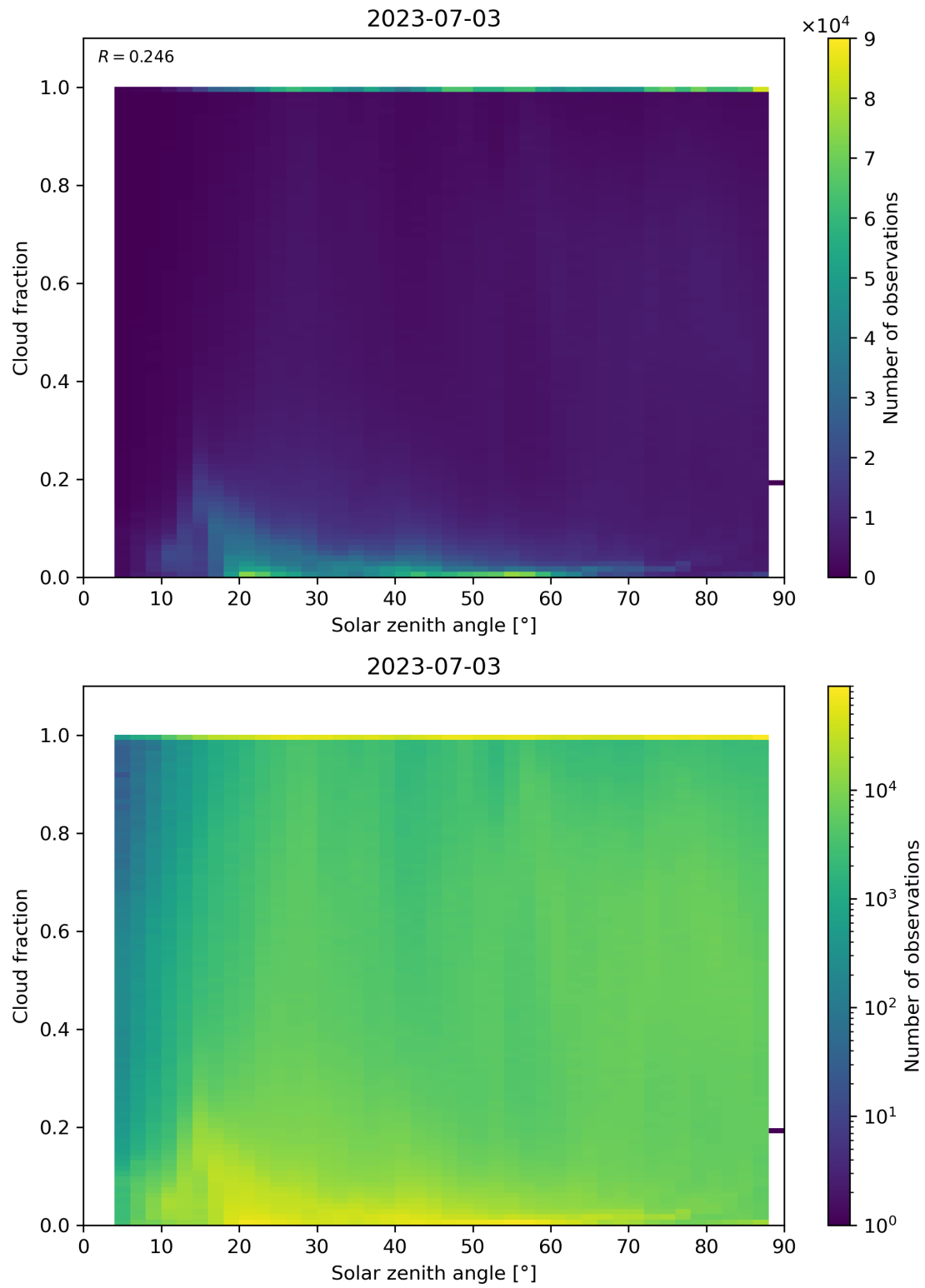
Figure 121: Scatter density plot of “Solar zenith angle” against “Cloud fraction” for 2023-07-03 to 2023-07-04.
