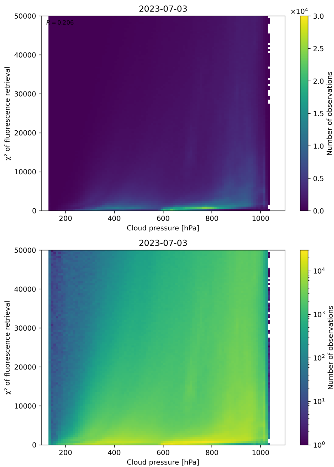
Figure 86: Scatter density plot of “Cloud pressure” against “ \chi^2 of fluorescence retrieval” for 2023-07-03 to 2023-07-04.
