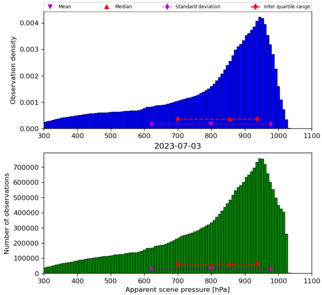
Figure 36: Histogram of “Apparent scene pressure” for 2023-07-03 to 2023-07-04
