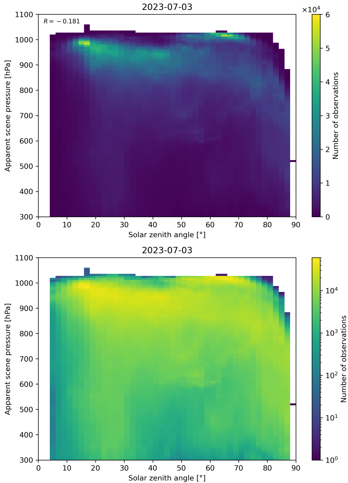
Figure 118: Scatter density plot of “Solar zenith angle” against “Apparent scene pressure” for 2023-07-03 to 2023-07-04.
