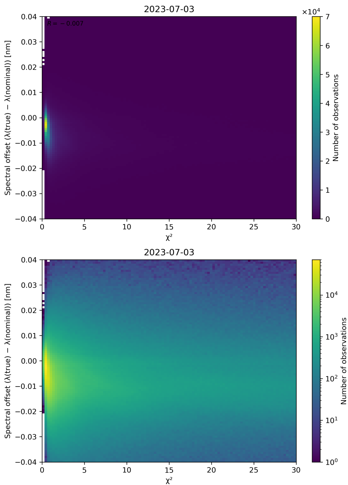
Figure 75: Scatter density plot of “ \chi^2 ” against “Spectral offset ( \lambda(\text{true}) - \lambda(\text{nominal}) )” for 2023-07-03 to 2023-07-04.
