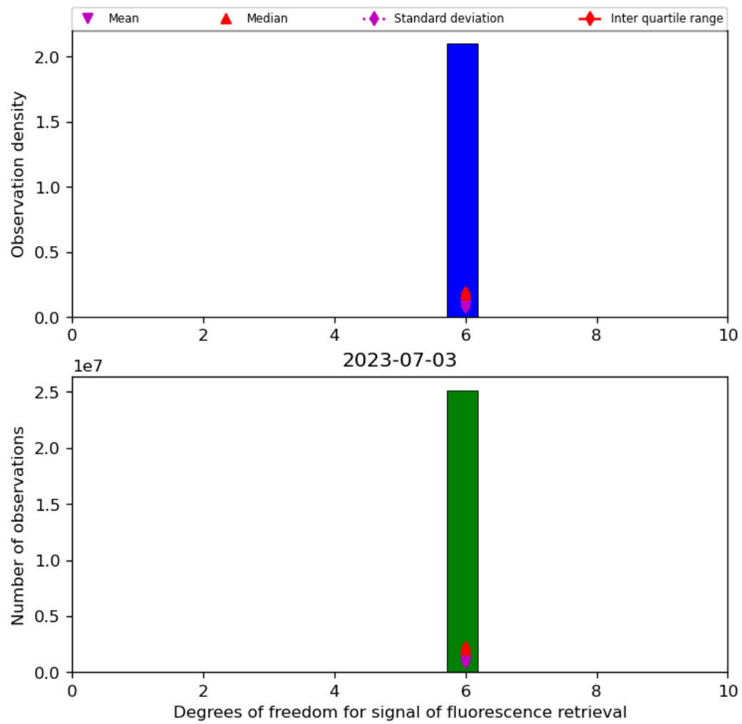
Figure 43: Histogram of “Degrees of freedom for signal of fluorescence retrieval” for 2023-07-03 to 2023-07-04
