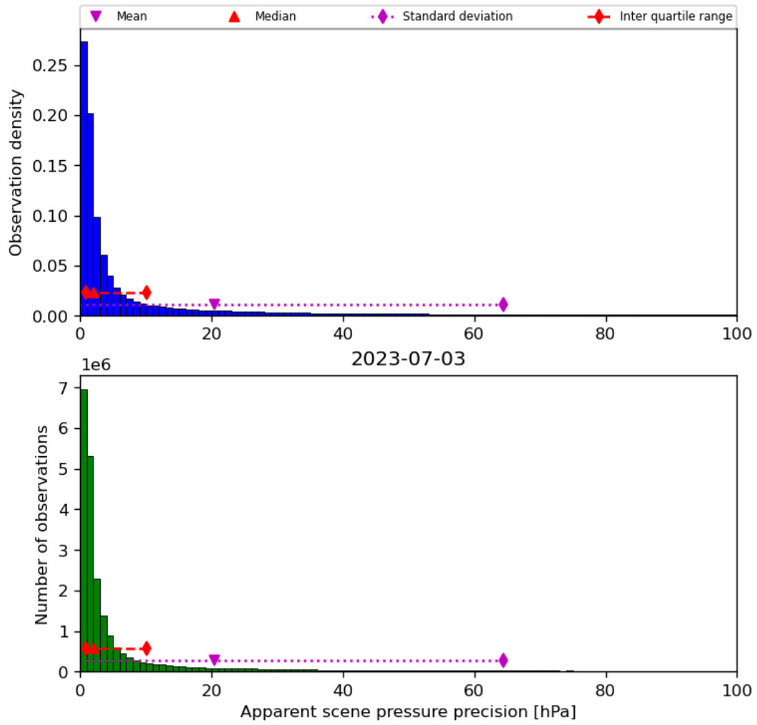
Figure 37: Histogram of “Apparent scene pressure precision” for 2023-07-03 to 2023-07-04
