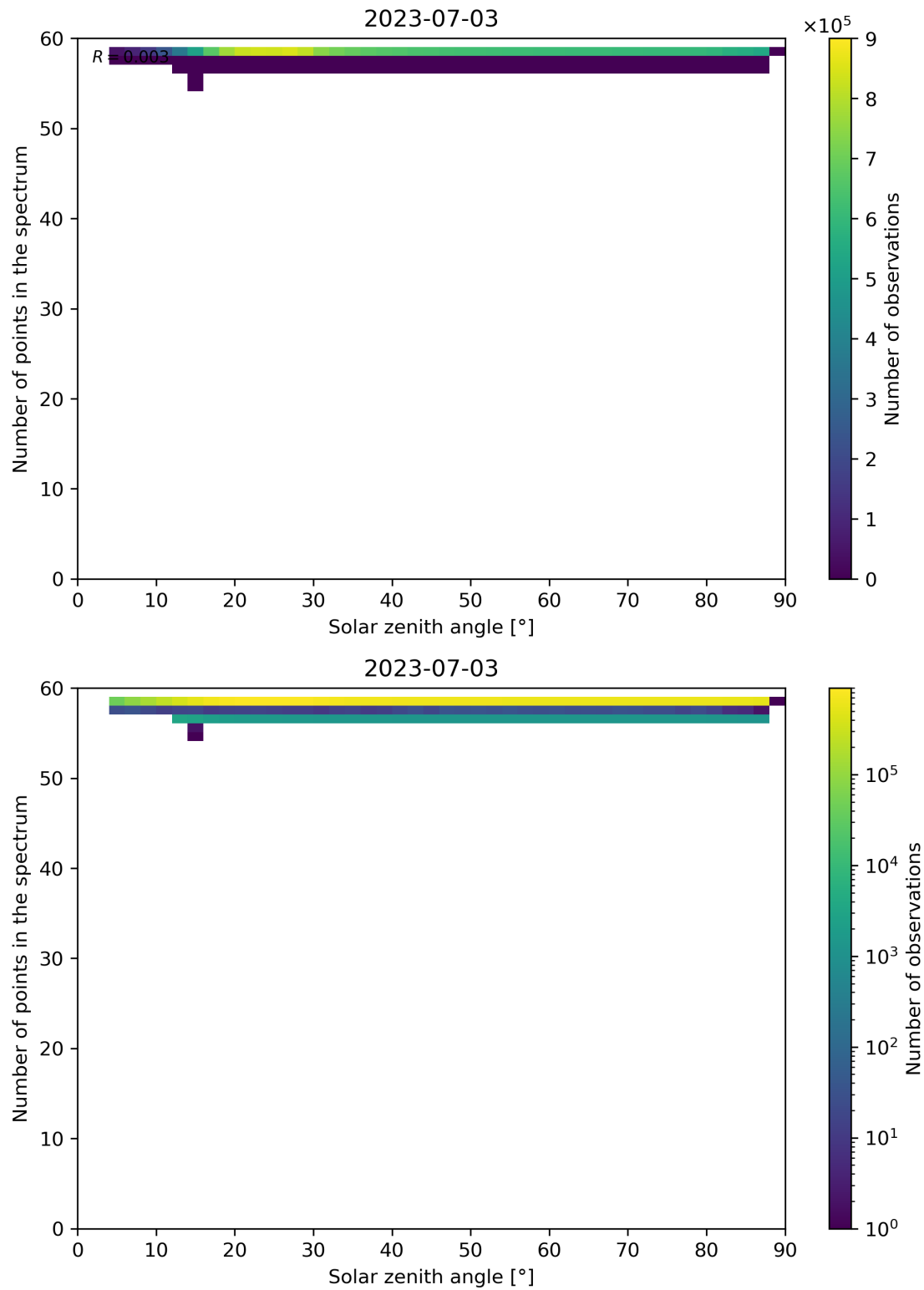
Figure 126: Scatter density plot of “Solar zenith angle” against “Number of points in the spectrum” for 2023-07-03 to 2023-07-04.
