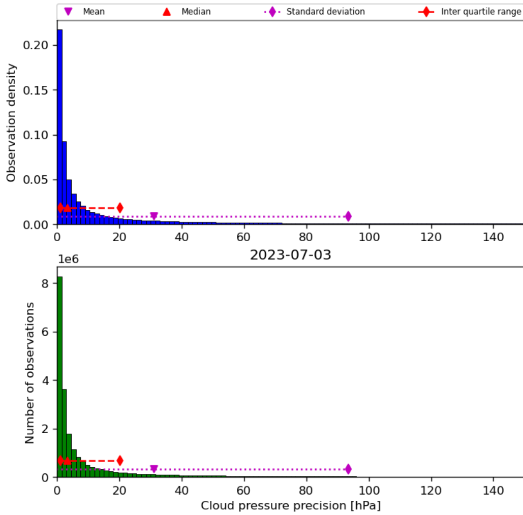
Figure 31: Histogram of “Cloud pressure precision” for 2023-07-03 to 2023-07-04
