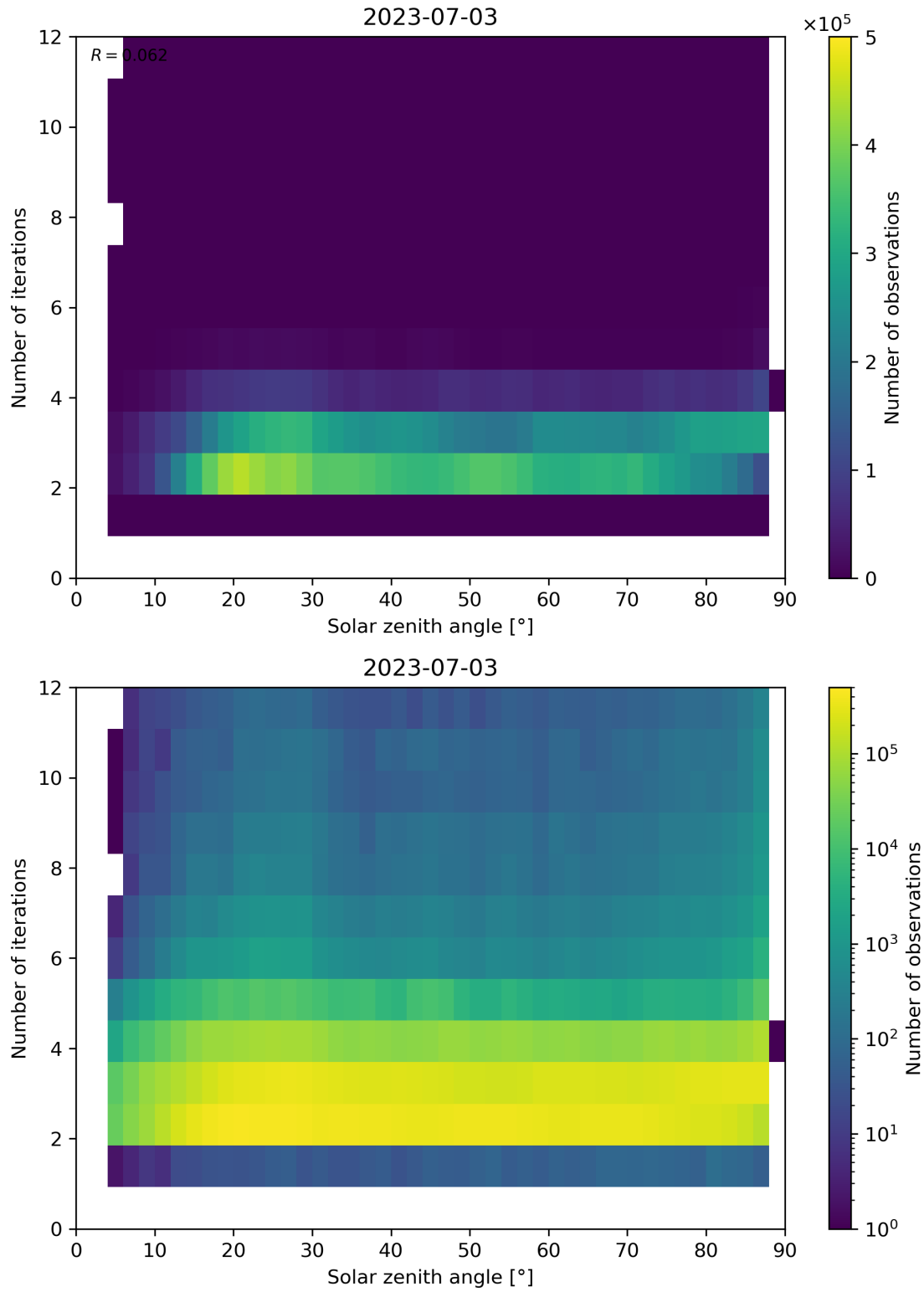
Figure 125: Scatter density plot of “Solar zenith angle” against “Number of iterations” for 2023-07-03 to 2023-07-04.
