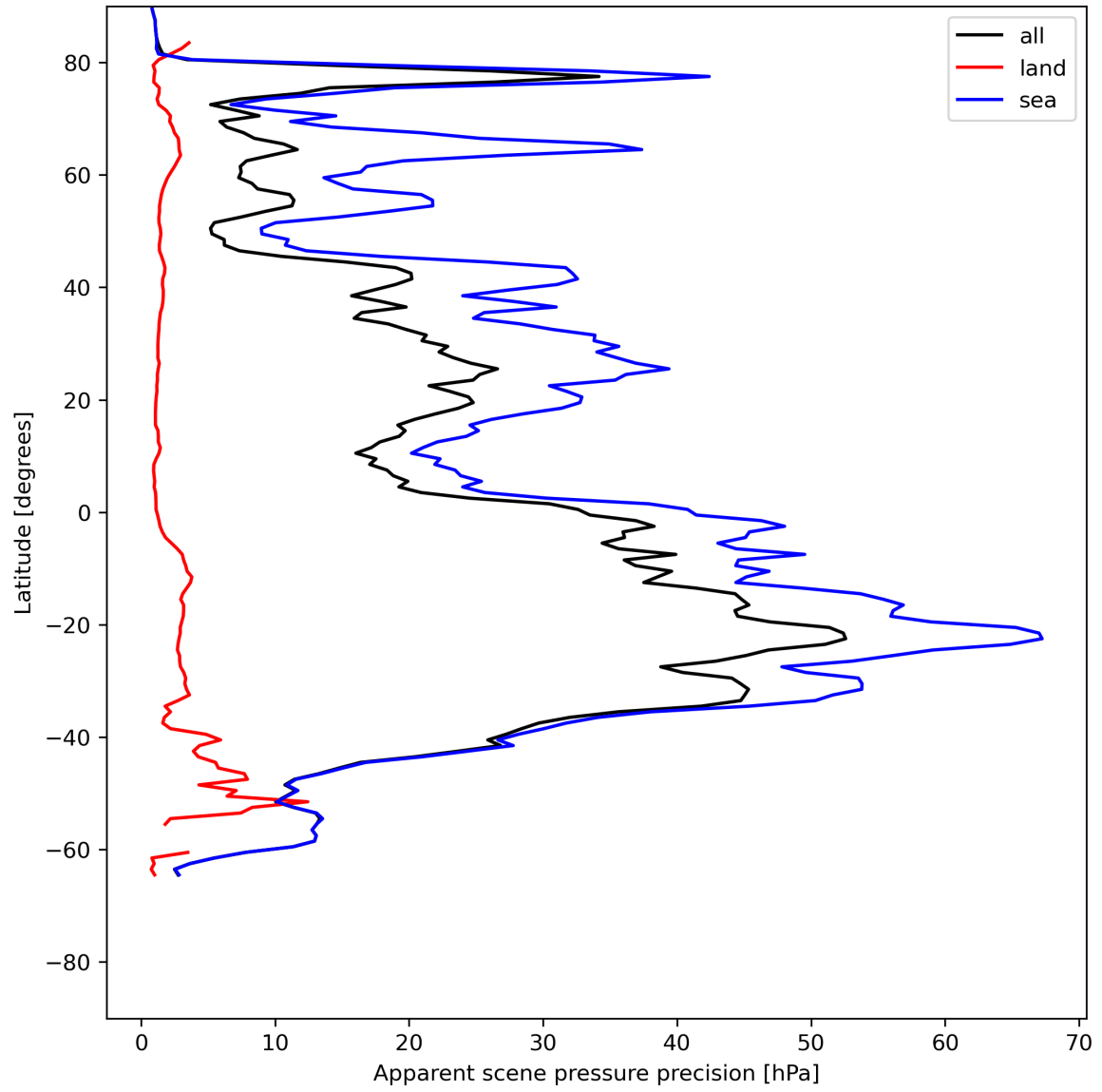
Figure 20: Zonal average of “Apparent scene pressure precision” for 2023-07-03 to 2023-07-04.
