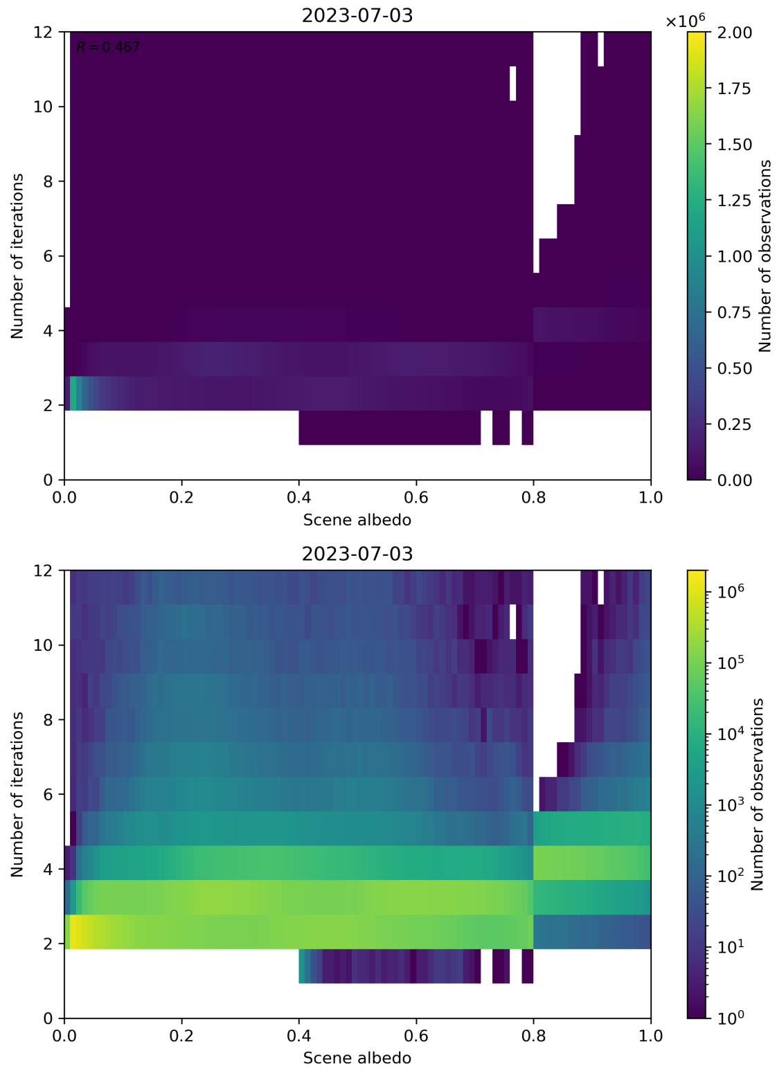
Figure 115: Scatter density plot of “Scene albedo” against “Number of iterations” for 2023-07-03 to 2023-07-04.
