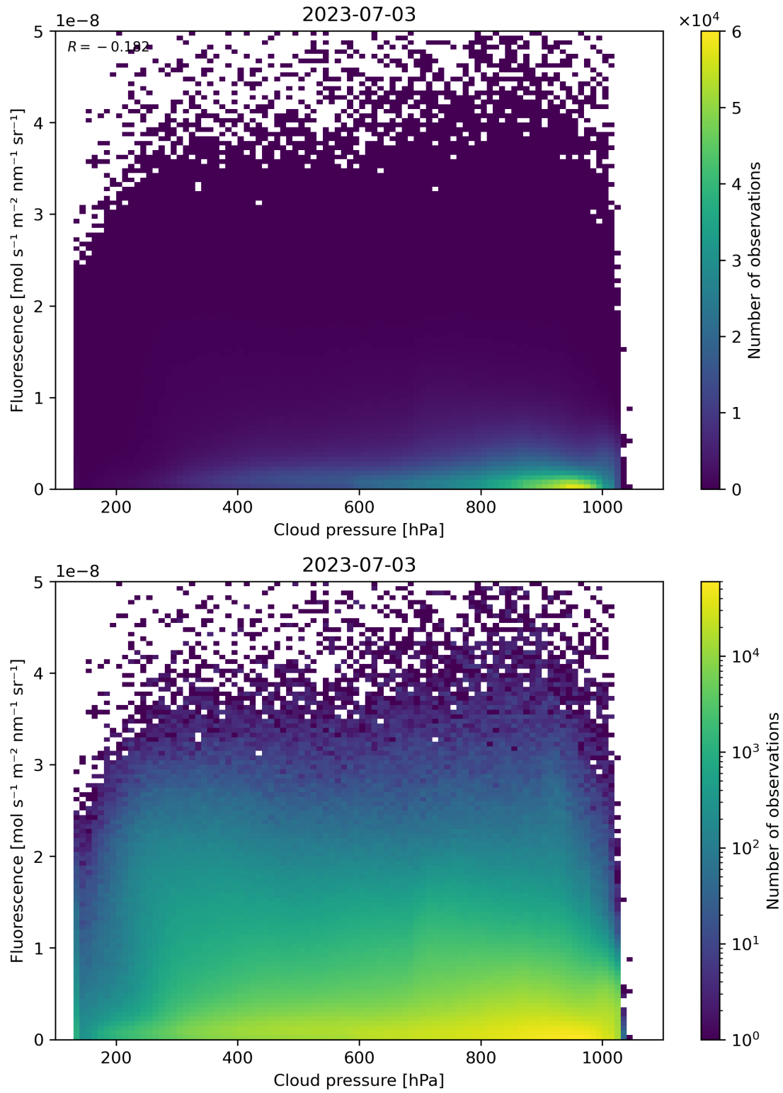
Figure 88: Scatter density plot of “Cloud pressure” against “Fluorescence” for 2023-07-03 to 2023-07-04.
