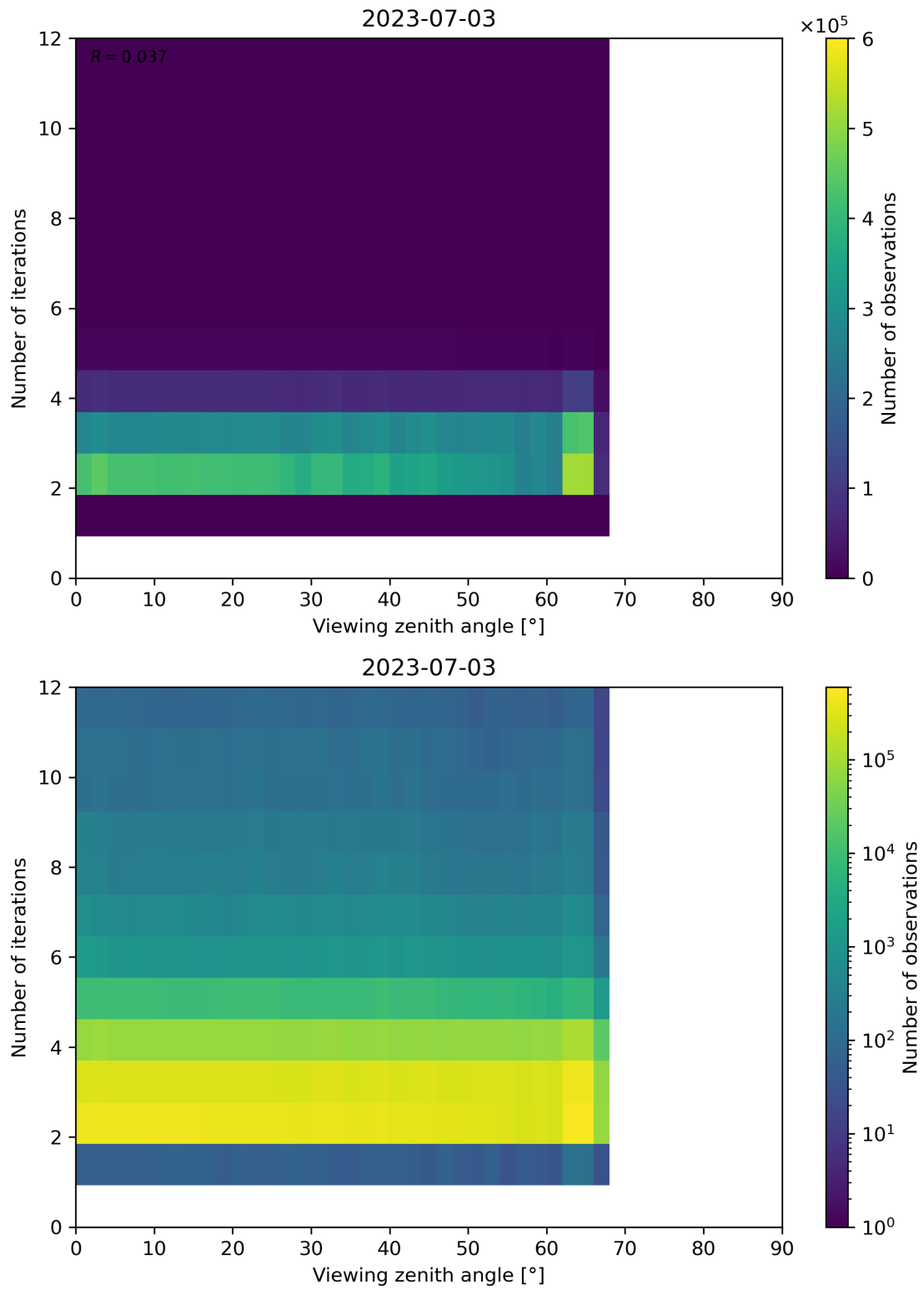
Figure 136: Scatter density plot of “Viewing zenith angle” against “Number of iterations” for 2023-07-03 to 2023-07-04.
