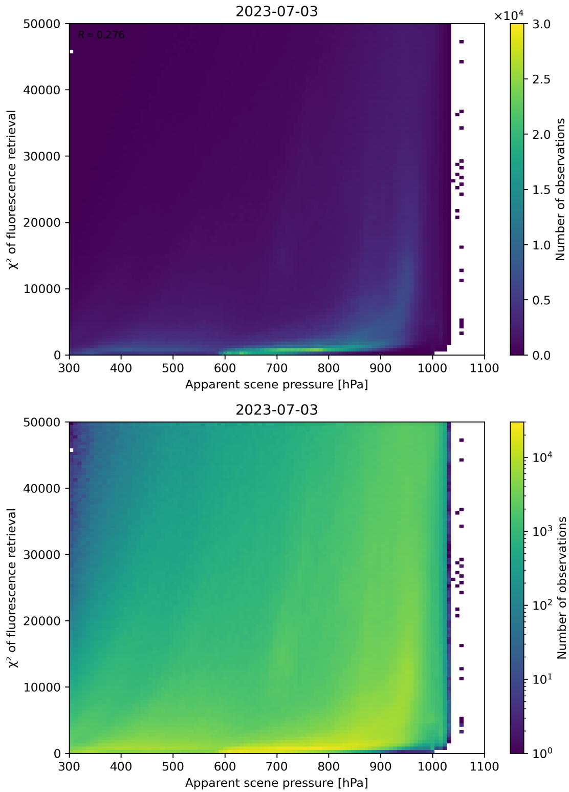
Figure 64: Scatter density plot of “Apparent scene pressure” against “ \chi^2 of fluorescence retrieval” for 2023-07-03 to 2023-07-04.
