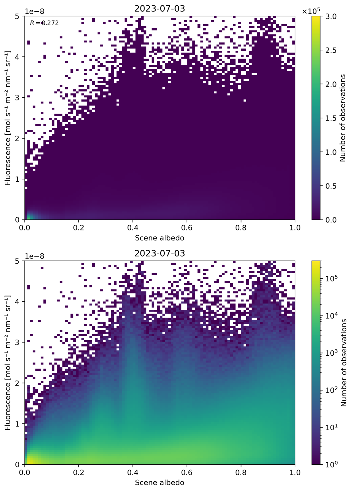
Figure 114: Scatter density plot of “Scene albedo” against “Fluorescence” for 2023-07-03 to 2023-07-04.
