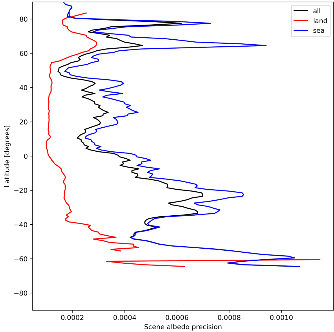
Figure 18: Zonal average of "Scene albedo precision" for 2023-07-03 to 2023-07-04.
