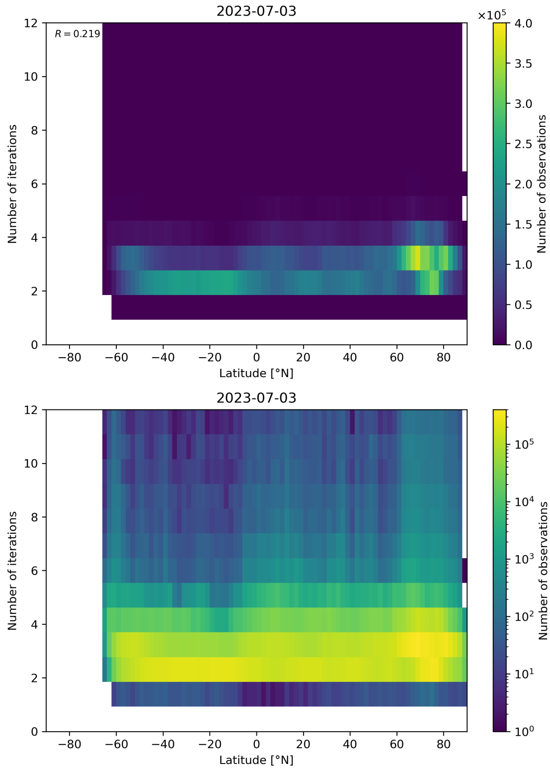
Figure 102: Scatter density plot of “Latitude” against “Number of iterations” for 2023-07-03 to 2023-07-04.
