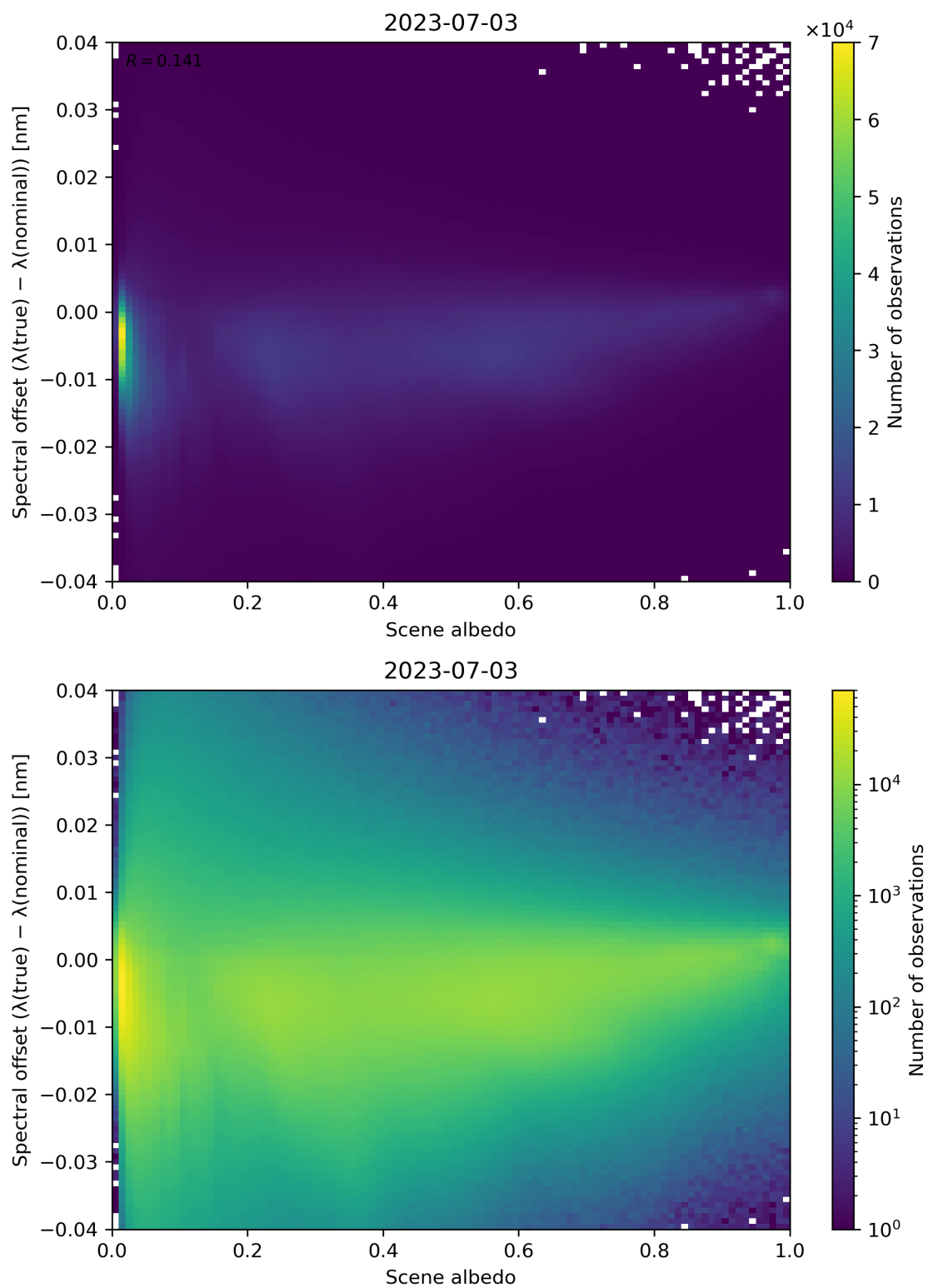
Figure 117: Scatter density plot of “Scene albedo” against “Spectral offset ( \lambda(\text{true}) - \lambda(\text{nominal}) )” for 2023-07-03 to 2023-07-04.
