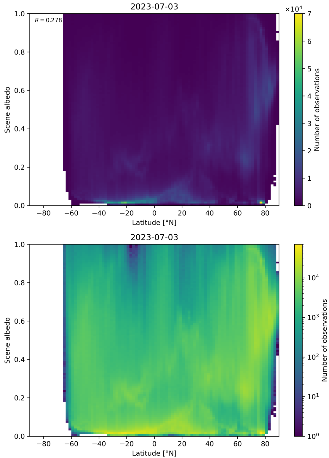
Figure 104: Scatter density plot of “Latitude” against “Scene albedo” for 2023-07-03 to 2023-07-04.
