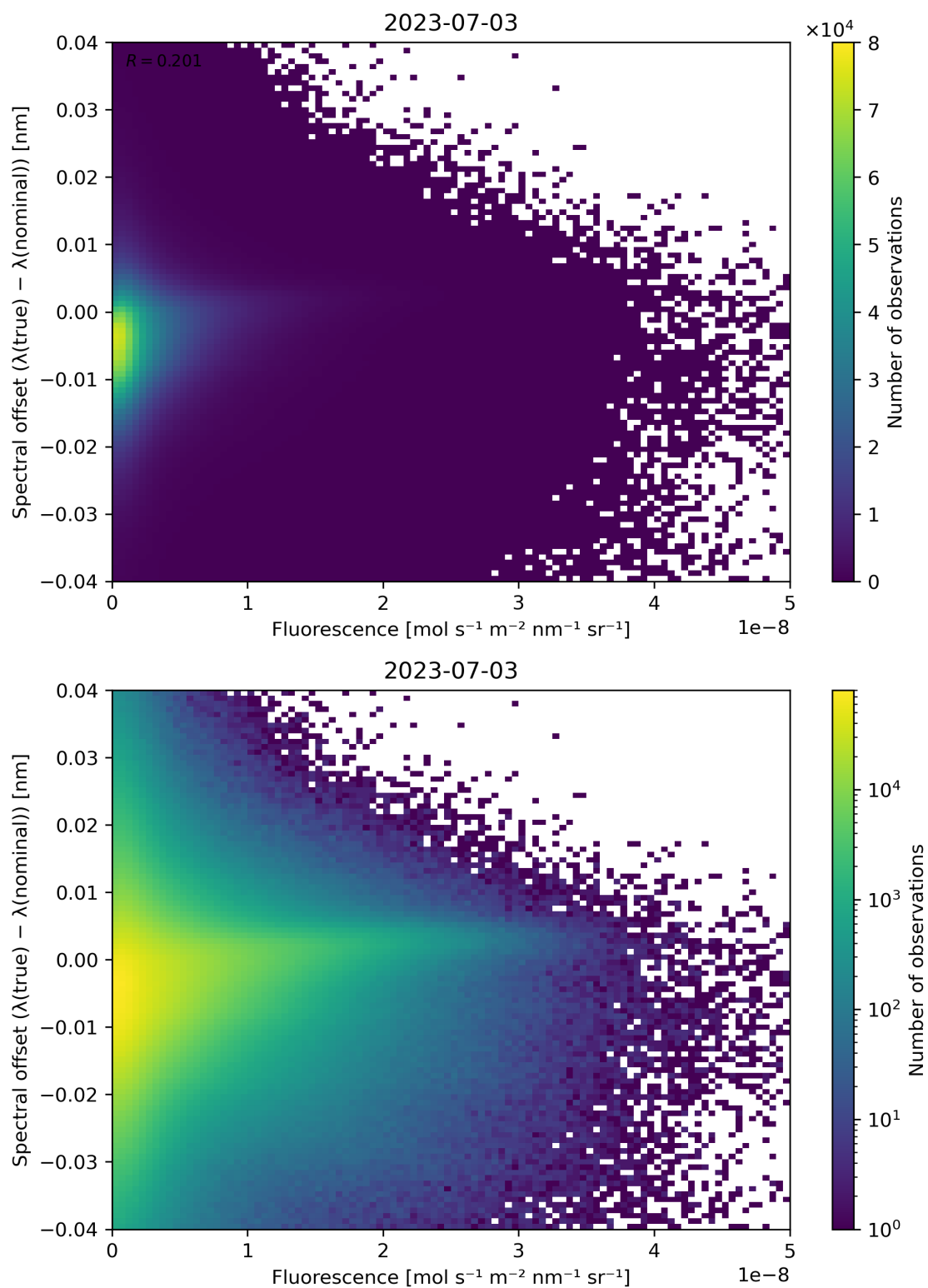
Figure 95: Scatter density plot of “Fluorescence” against “Spectral offset ( \lambda(\text{true}) - \lambda(\text{nominal}) )” for 2023-07-03 to 2023-07-04.
