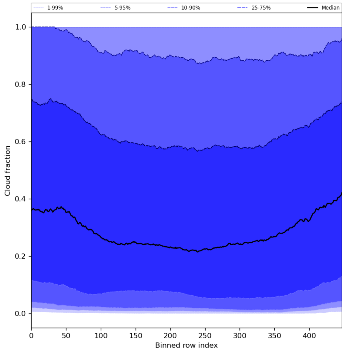
Figure 49: Along track statistics of “Cloud fraction” for 2023-07-03 to 2023-07-04
