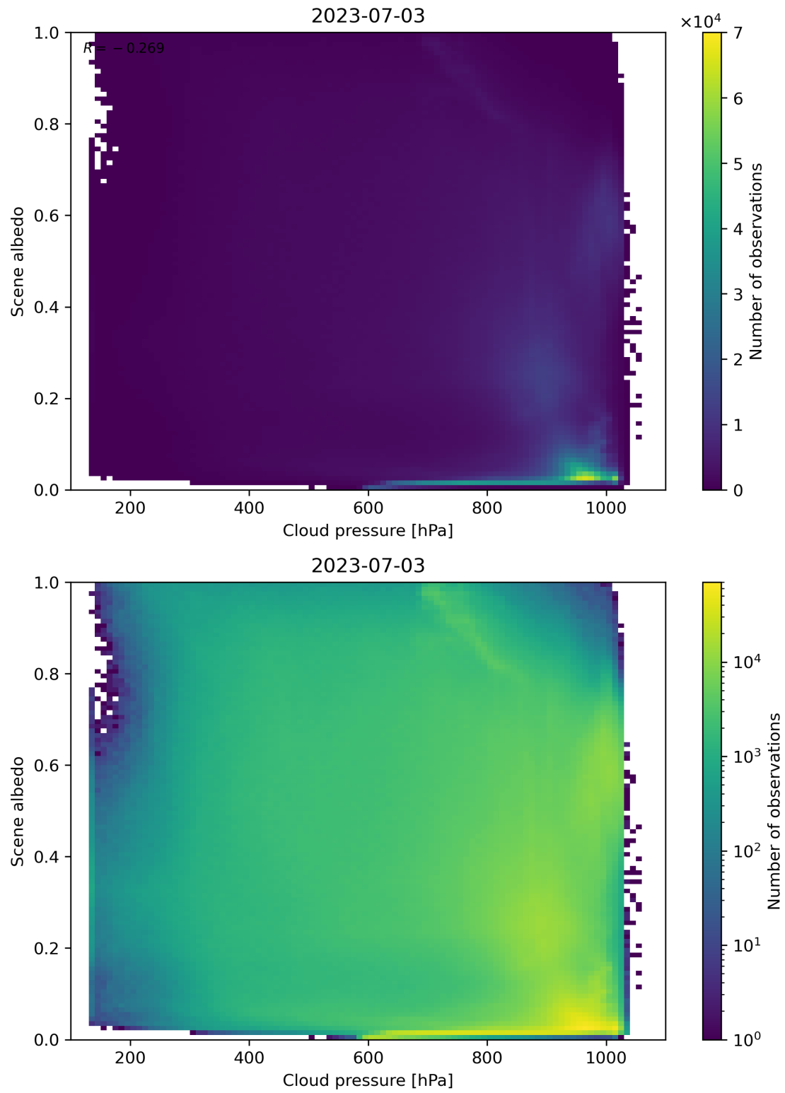
Figure 91: Scatter density plot of “Cloud pressure” against “Scene albedo” for 2023-07-03 to 2023-07-04.
