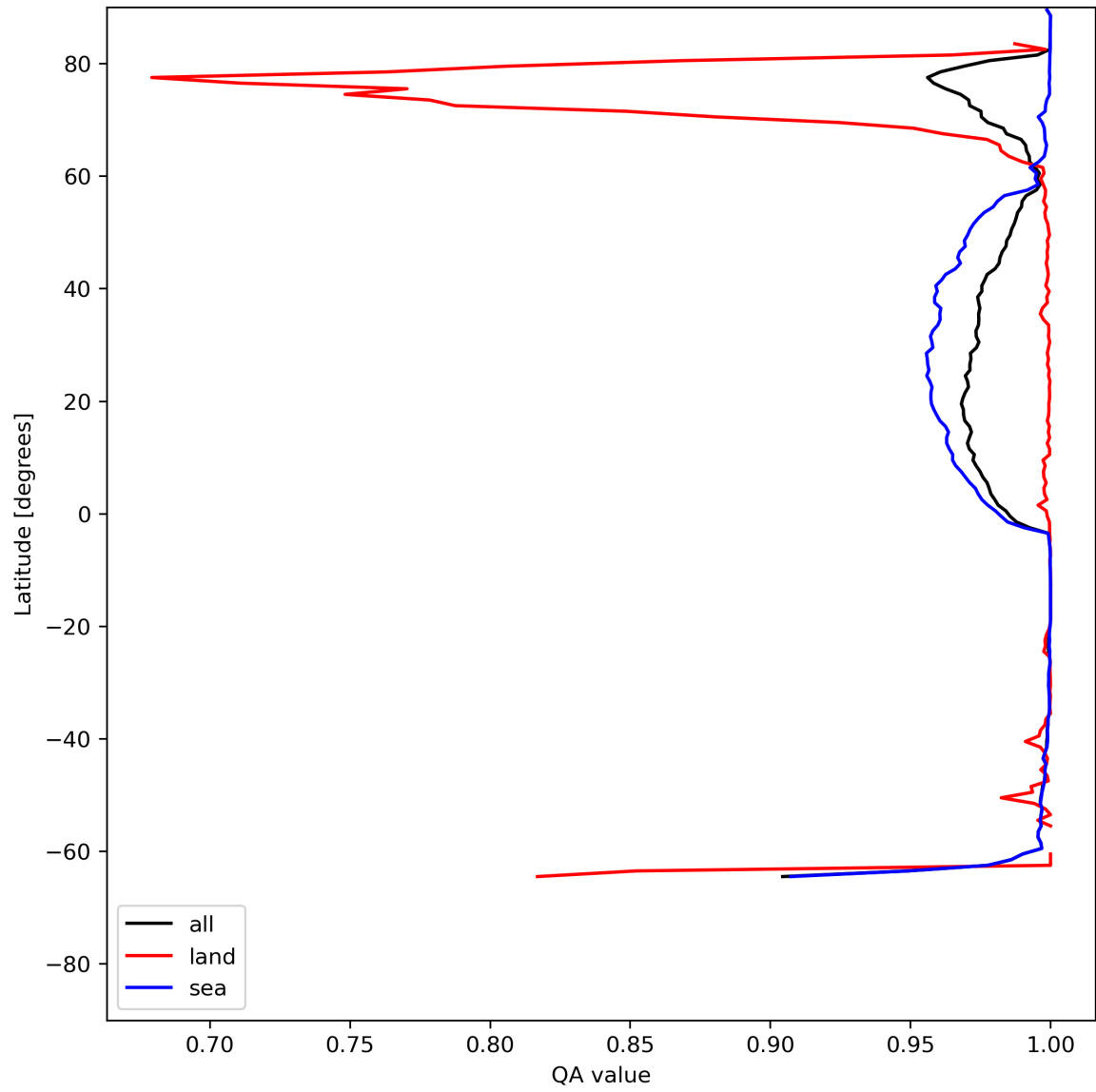
Figure 12: Zonal average of “QA value” for 2023-07-03 to 2023-07-04.
