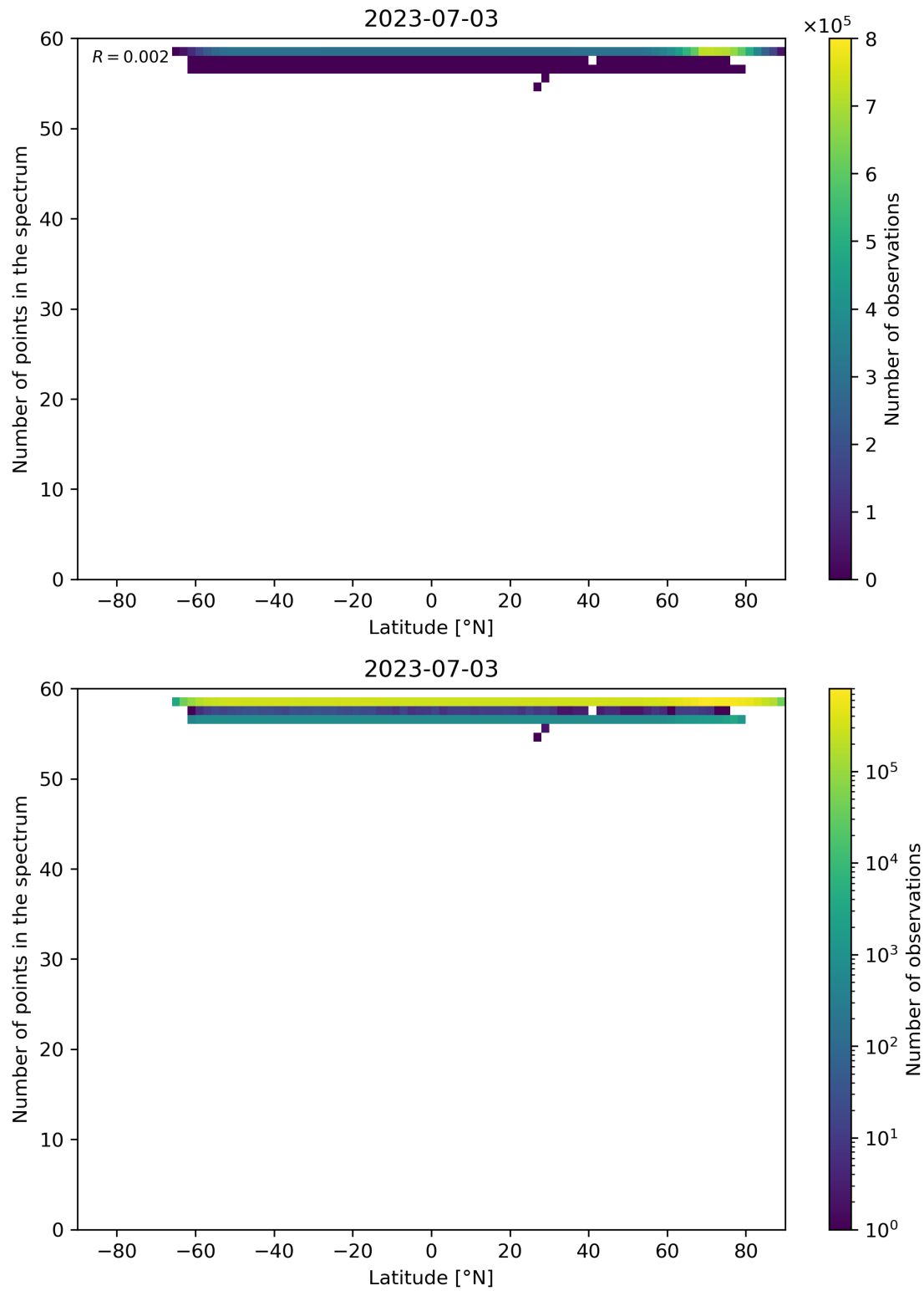
Figure 103: Scatter density plot of “Latitude” against “Number of points in the spectrum” for 2023-07-03 to 2023-07-04.
