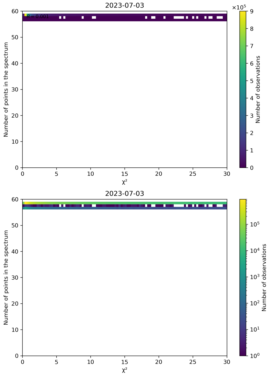
Figure 74: Scatter density plot of " \chi^2 " against "Number of points in the spectrum" for 2023-07-03 to 2023-07-04.
