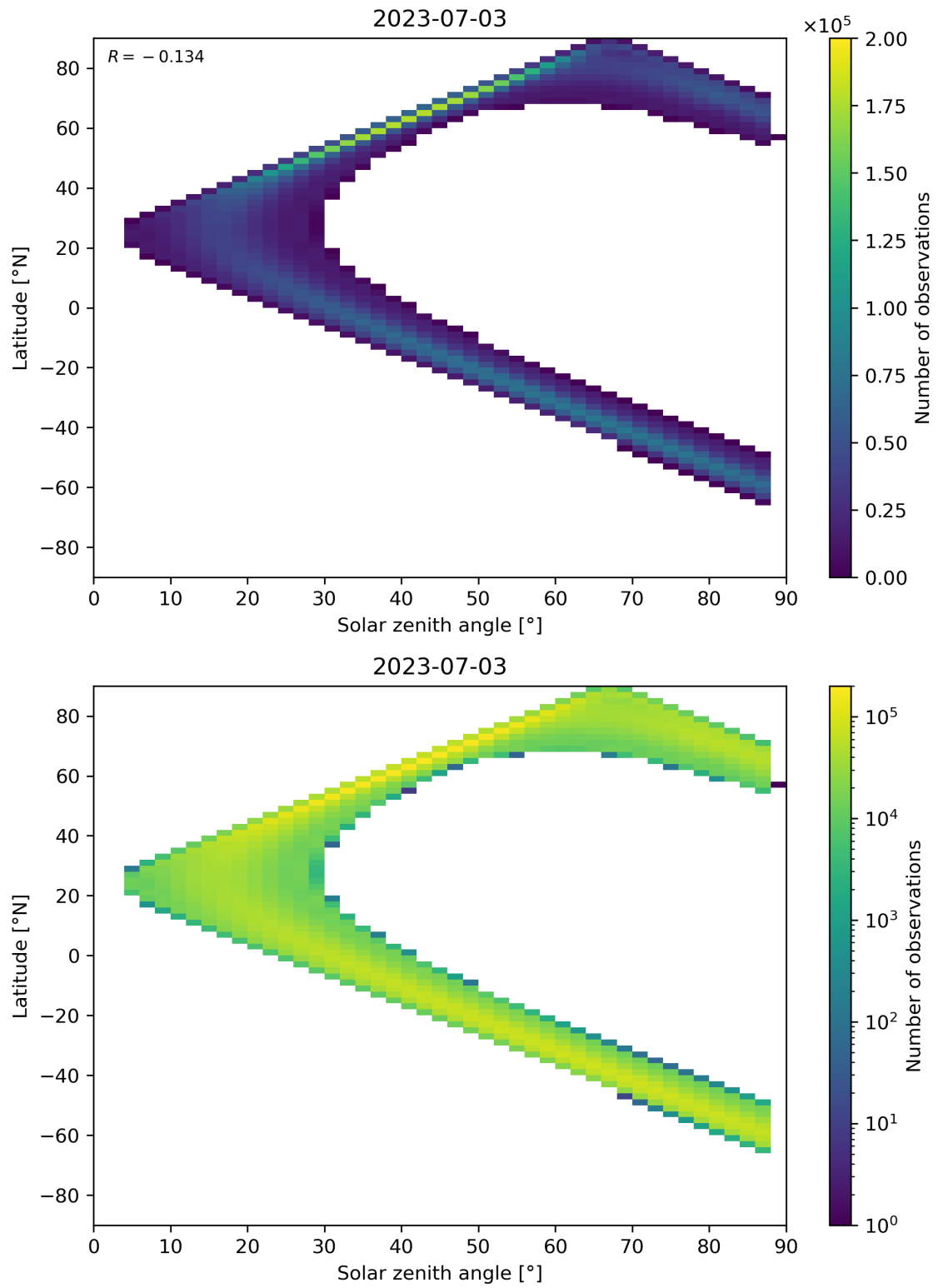
Figure 124: Scatter density plot of “Solar zenith angle” against “Latitude” for 2023-07-03 to 2023-07-04.
