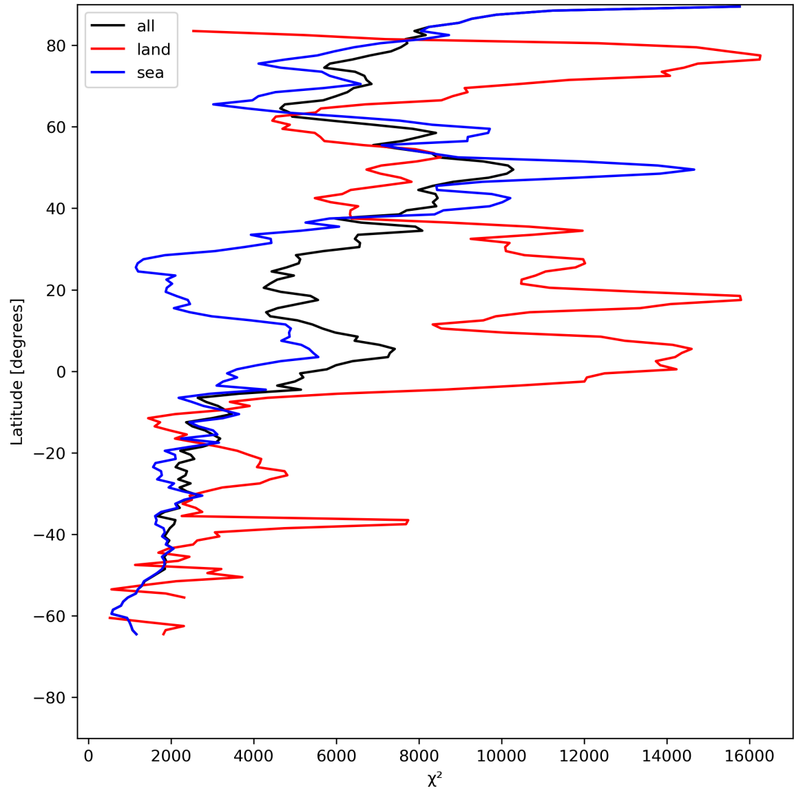
Figure 21: Zonal average of “ \chi^2 ” for 2023-07-03 to 2023-07-04.
