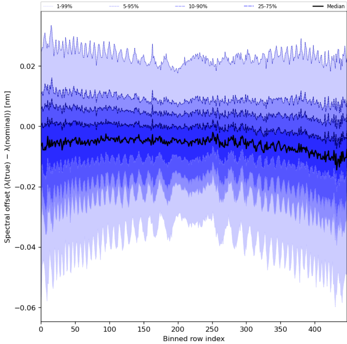
Figure 62: Along track statistics of “Spectral offset ( \lambda(\text{true}) - \lambda(\text{nominal}) )” for 2023-07-03 to 2023-07-04
