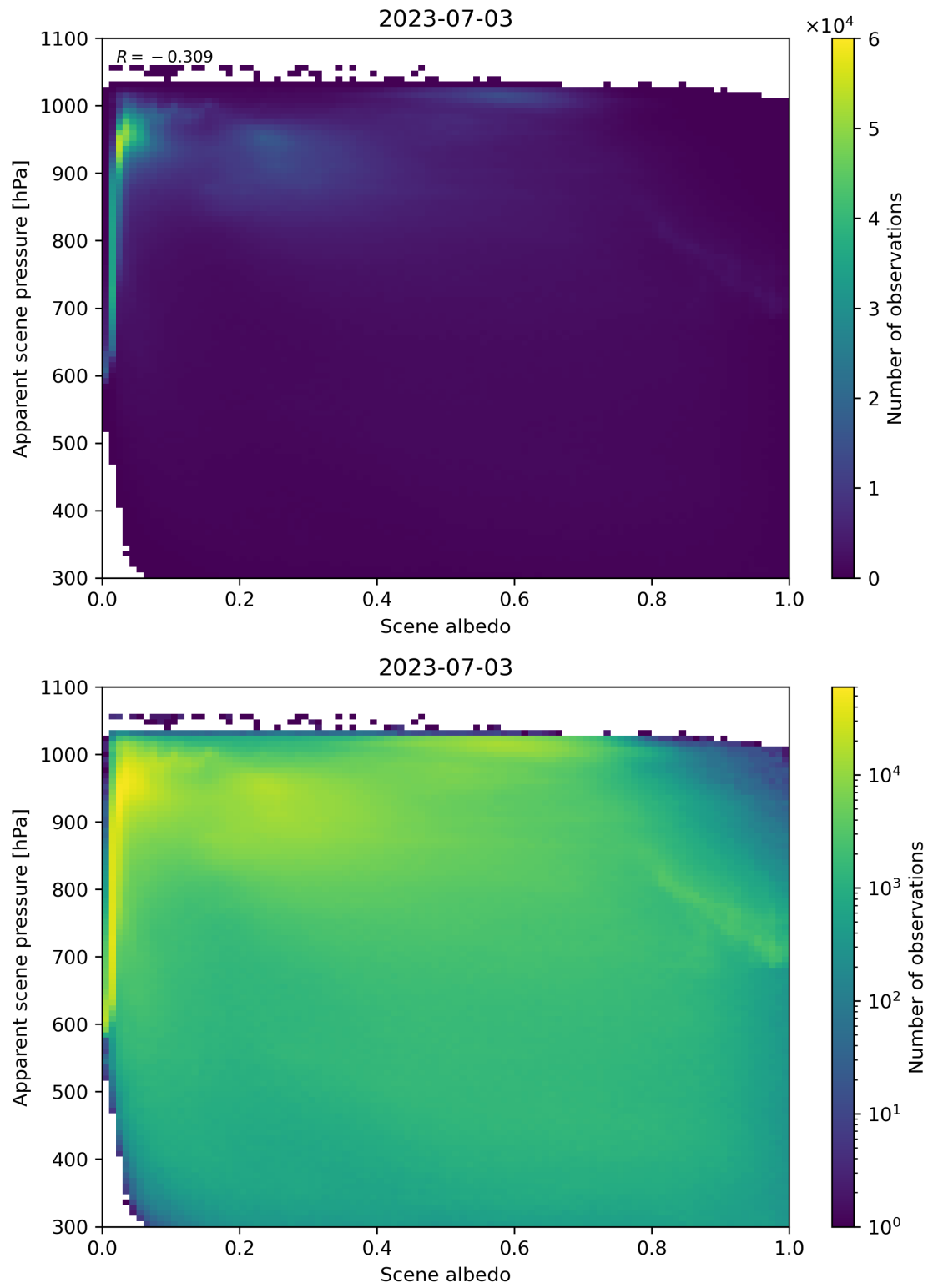
Figure 111: Scatter density plot of “Scene albedo” against “Apparent scene pressure” for 2023-07-03 to 2023-07-04.
