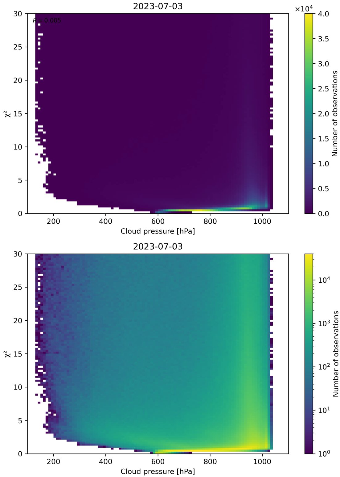
Figure 85: Scatter density plot of “Cloud pressure” against “ \chi^2 ” for 2023-07-03 to 2023-07-04.
