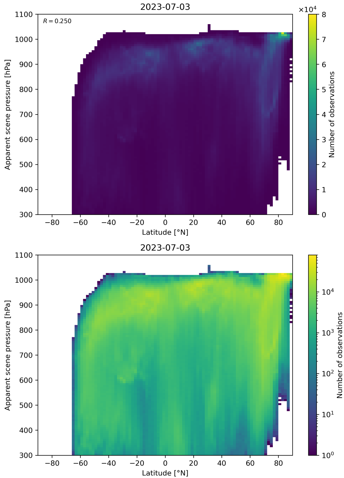
Figure 96: Scatter density plot of “Latitude” against “Apparent scene pressure” for 2023-07-03 to 2023-07-04.
