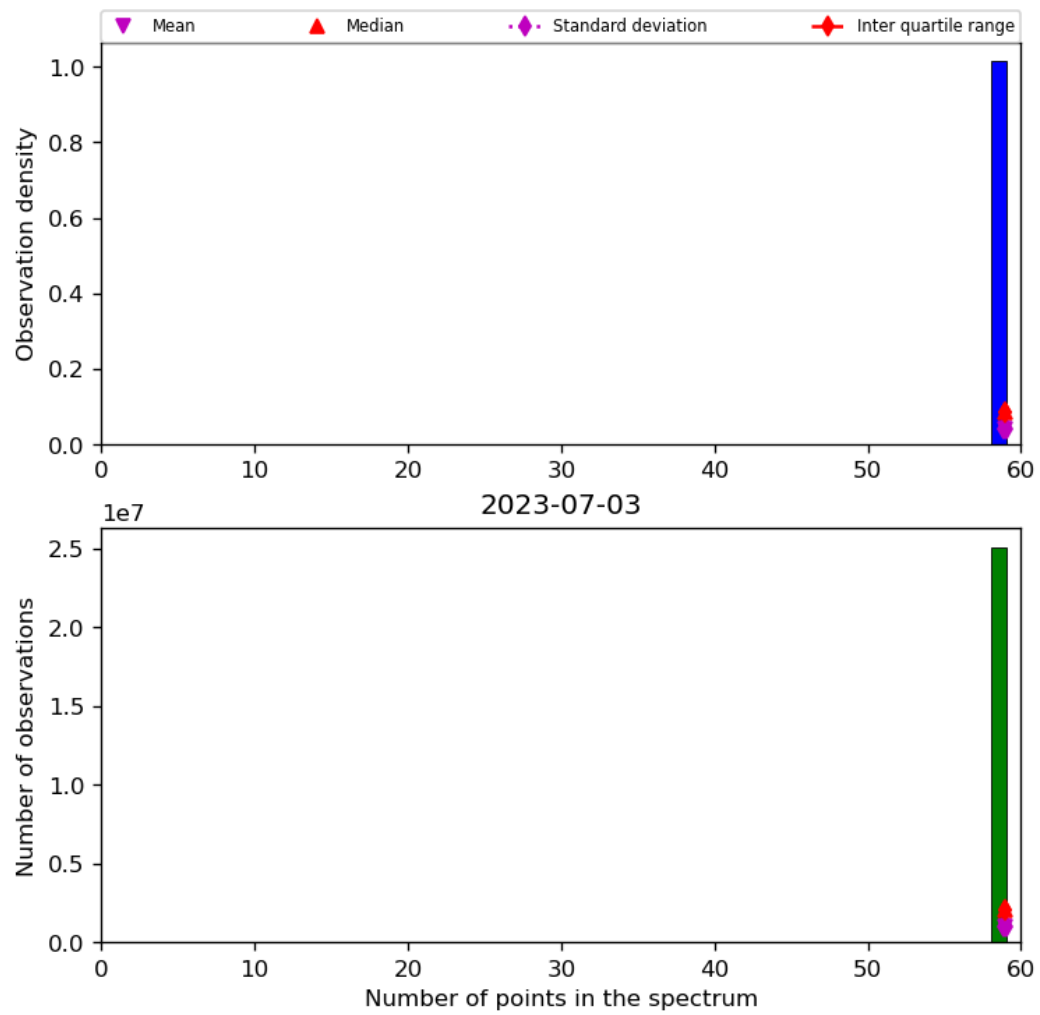
Figure 44: Histogram of “Number of points in the spectrum” for 2023-07-03 to 2023-07-04
