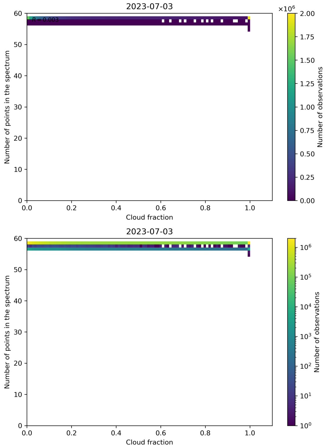
Figure 81: Scatter density plot of “Cloud fraction” against “Number of points in the spectrum” for 2023-07-03 to 2023-07-04.
