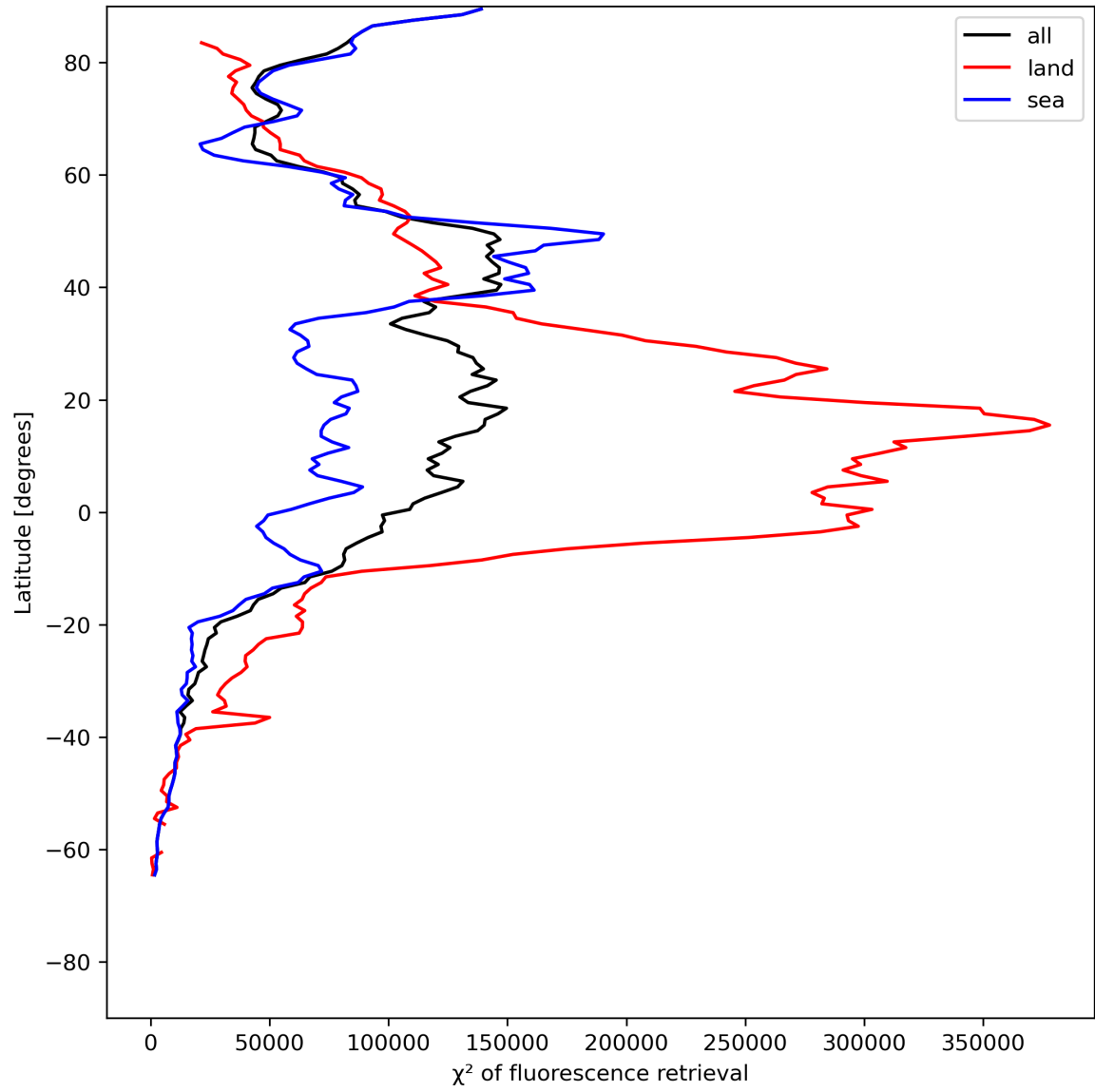
Figure 25: Zonal average of “ \chi^2 of fluorescence retrieval” for 2023-07-03 to 2023-07-04.
