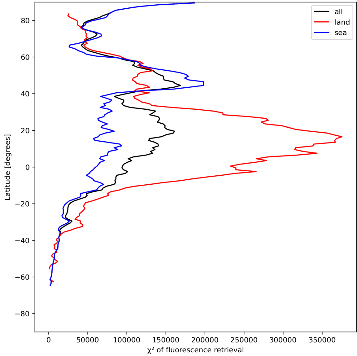
Figure 25: Zonal average of “ \chi^2 of fluorescence retrieval” for 2023-07-05 to 2023-07-07.
