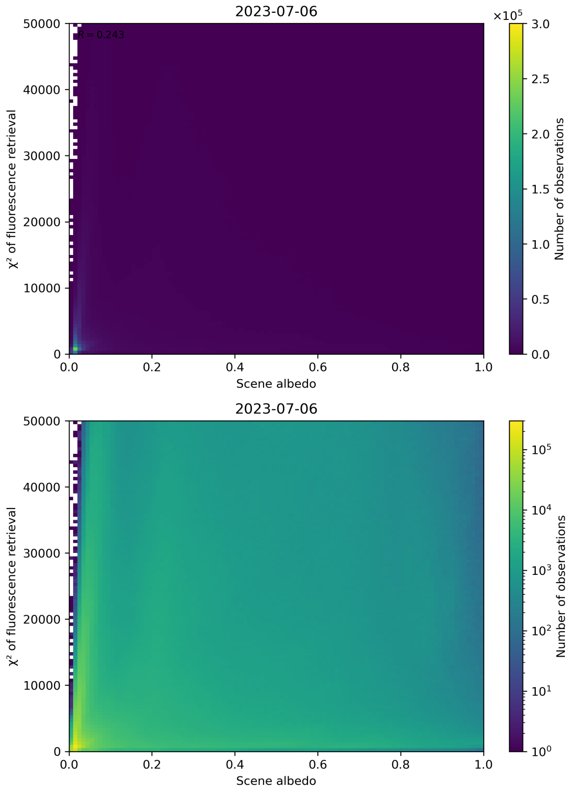
Figure 113: Scatter density plot of “Scene albedo” against “ \chi^2 of fluorescence retrieval” for 2023-07-05 to 2023-07-07.
