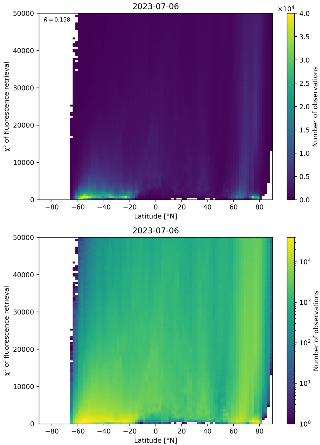
Figure 98: Scatter density plot of “Latitude” against “ \chi^2 of fluorescence retrieval” for 2023-07-05 to 2023-07-07.
