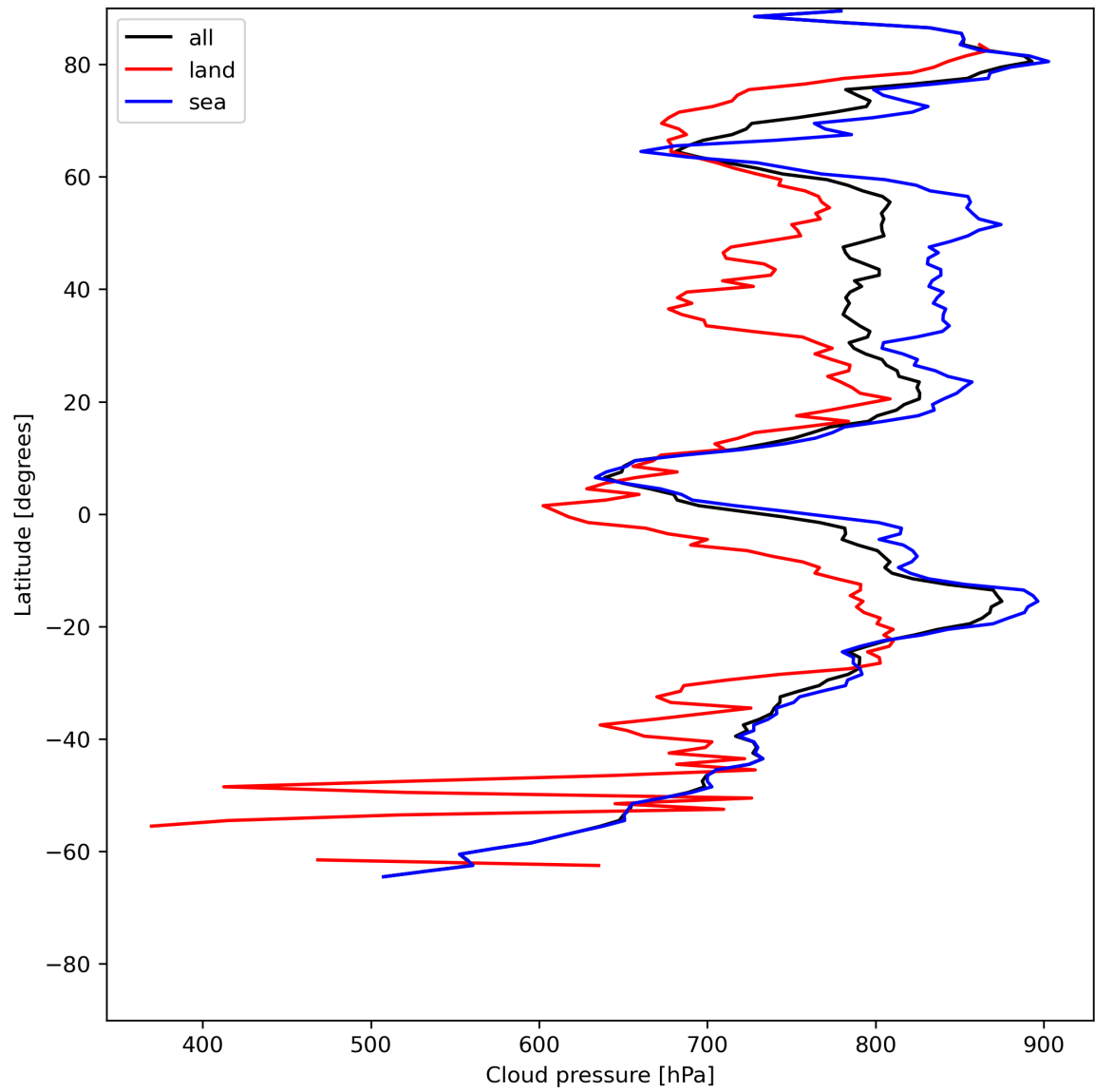
Figure 13: Zonal average of “Cloud pressure” for 2023-07-05 to 2023-07-07.
