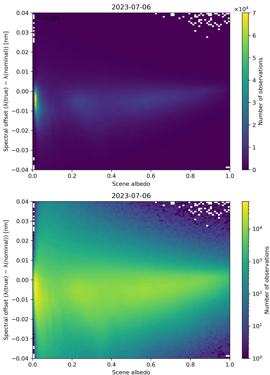
Figure 117: Scatter density plot of “Scene albedo” against “Spectral offset ( \lambda(\text{true}) - \lambda(\text{nominal}) )” for 2023-07-05 to 2023-07-07.
