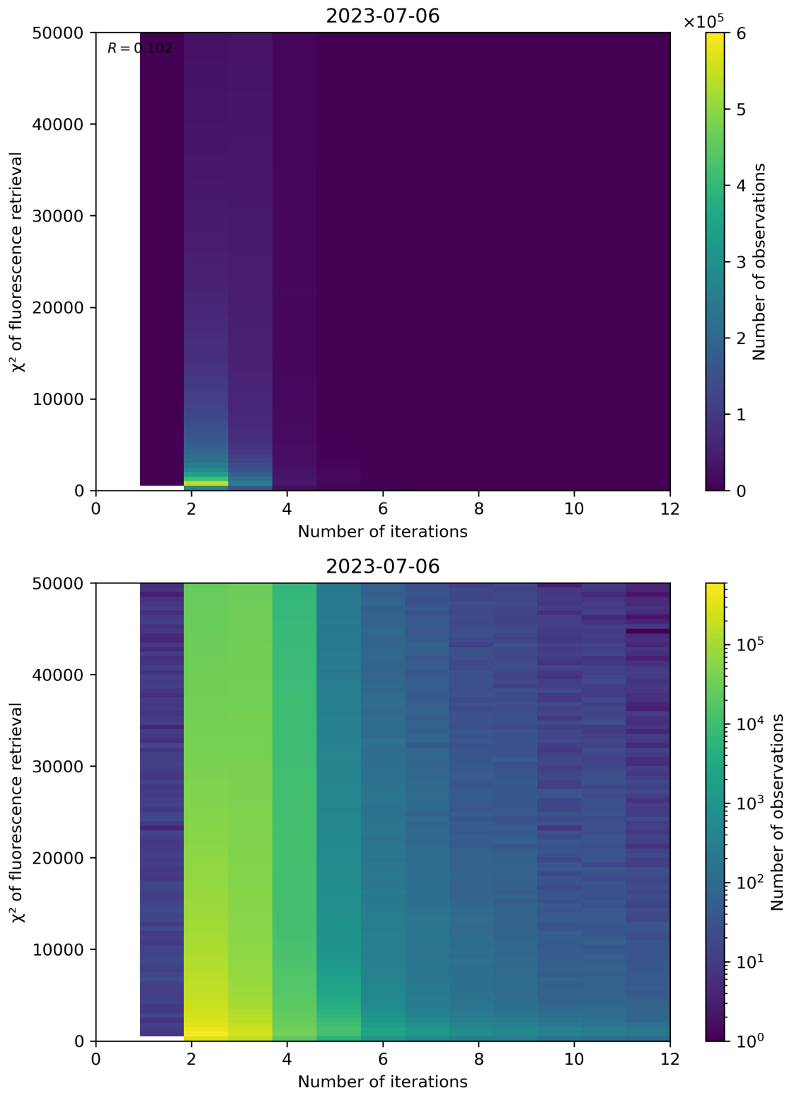
Figure 106: Scatter density plot of “Number of iterations” against “ \chi^2 of fluorescence retrieval” for 2023-07-05 to 2023-07-07.
