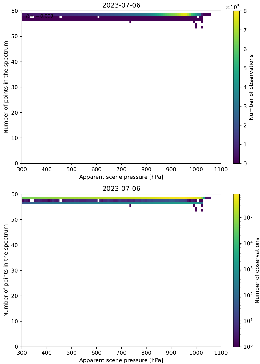
Figure 67: Scatter density plot of “Apparent scene pressure” against “Number of points in the spectrum” for 2023-07-05 to 2023-07-07.
