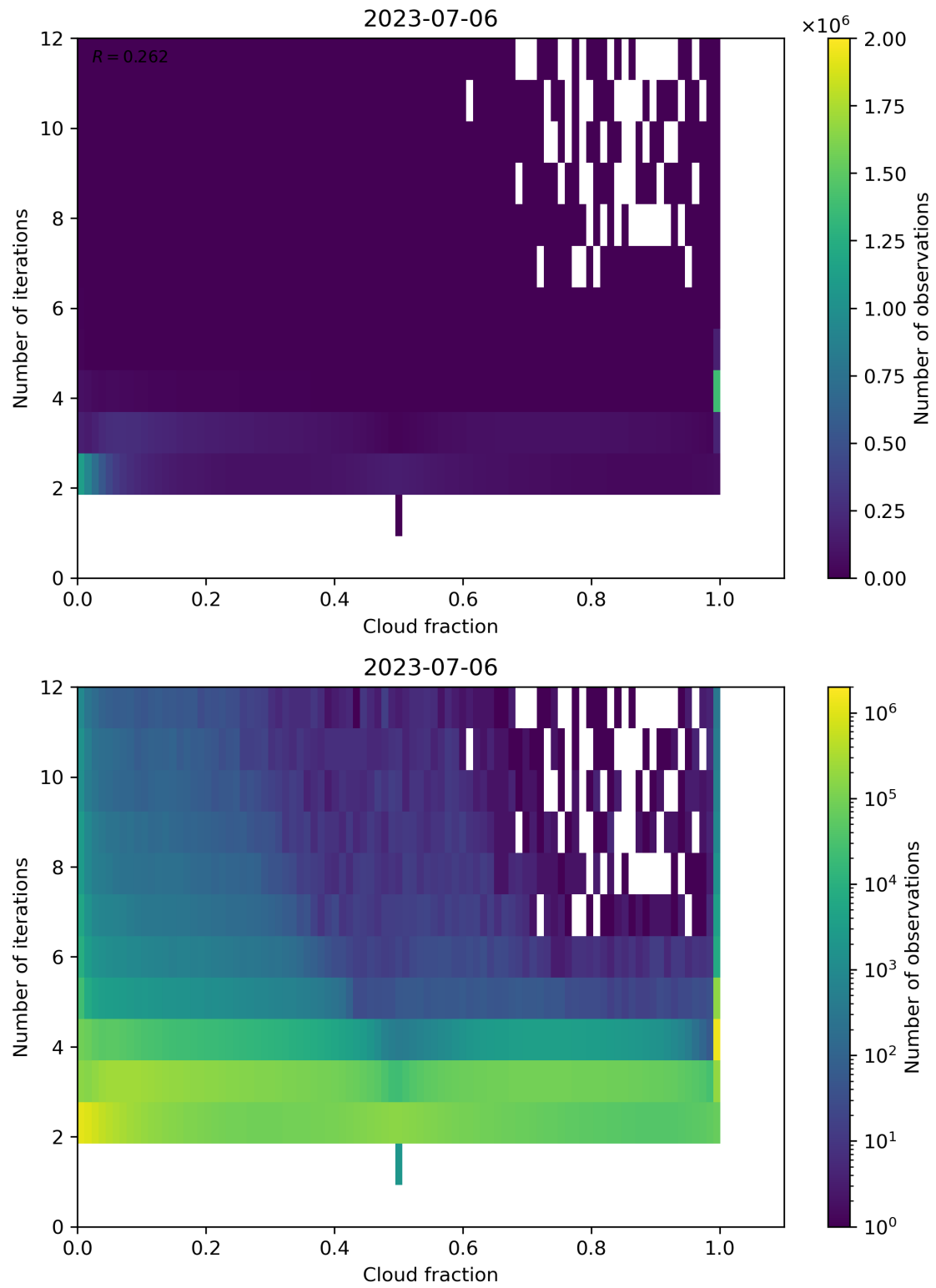
Figure 80: Scatter density plot of “Cloud fraction” against “Number of iterations” for 2023-07-05 to 2023-07-07.
