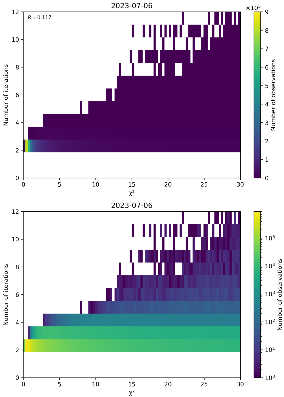
Figure 73: Scatter density plot of “ \chi^2 ” against “Number of iterations” for 2023-07-05 to 2023-07-07.
