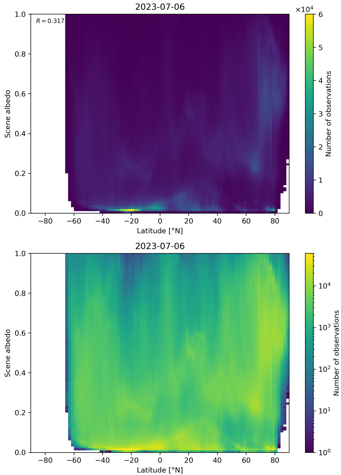
Figure 104: Scatter density plot of “Latitude” against “Scene albedo” for 2023-07-05 to 2023-07-07.
