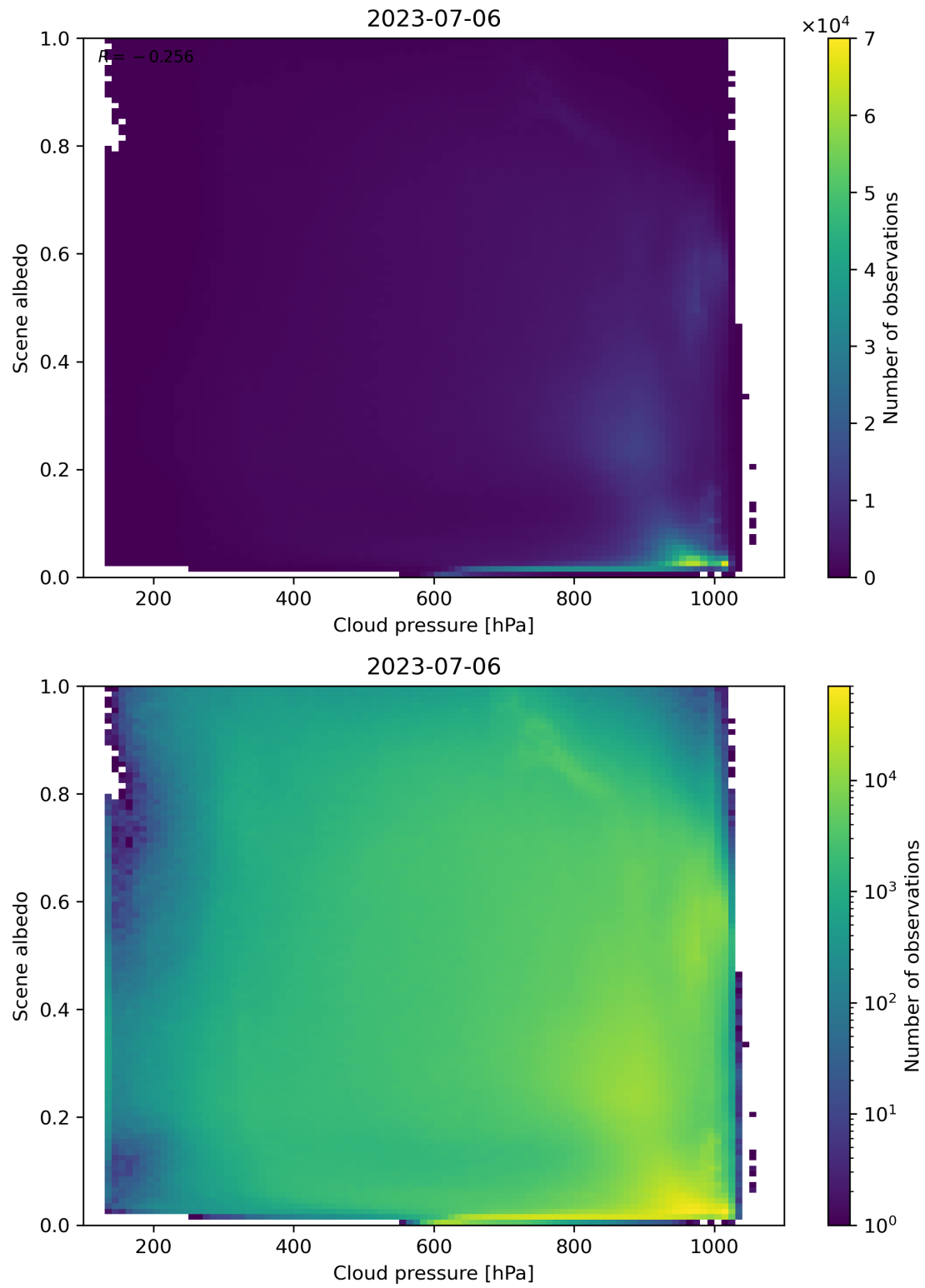
Figure 91: Scatter density plot of “Cloud pressure” against “Scene albedo” for 2023-07-05 to 2023-07-07.
