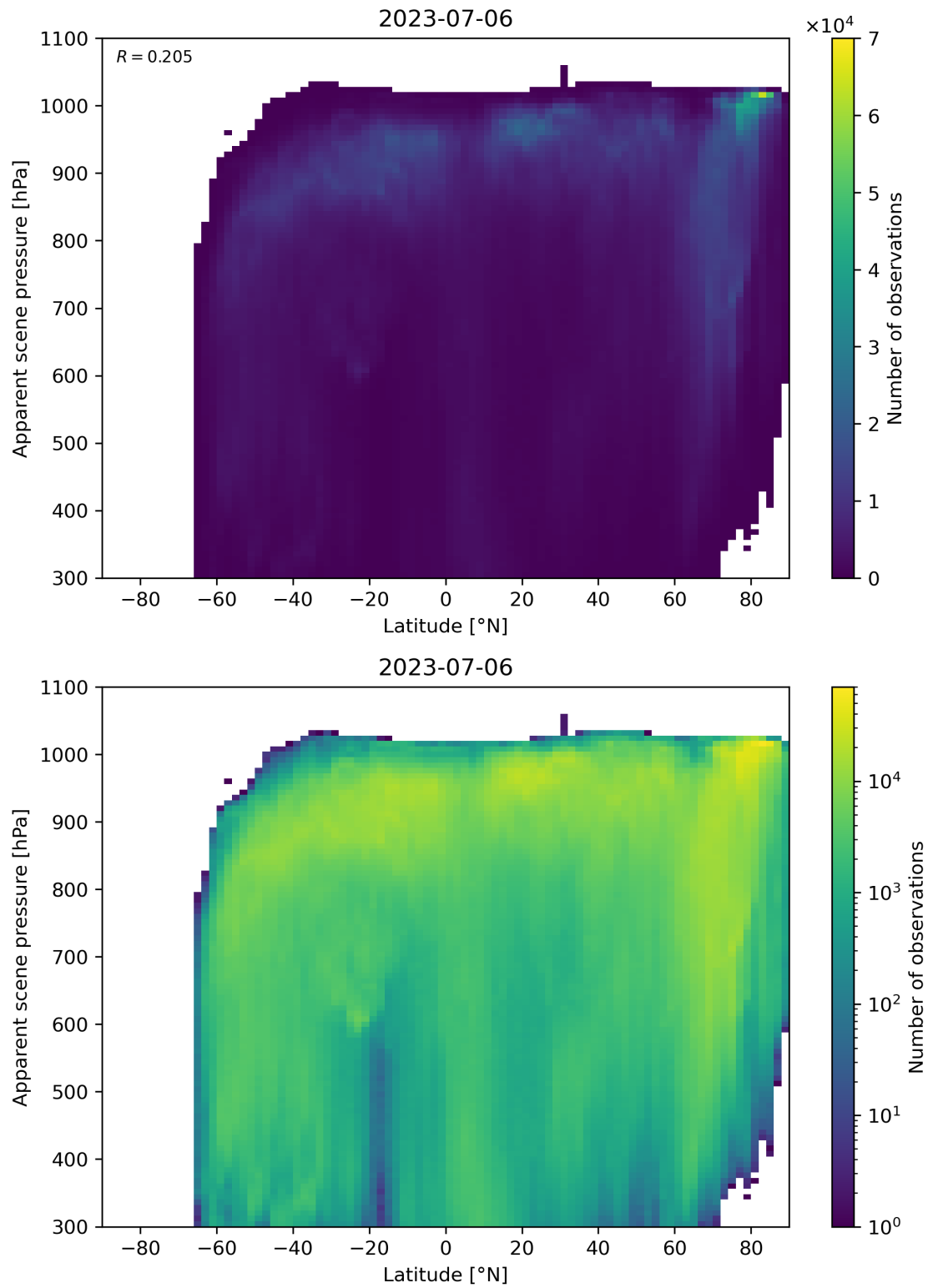
Figure 96: Scatter density plot of “Latitude” against “Apparent scene pressure” for 2023-07-05 to 2023-07-07.
