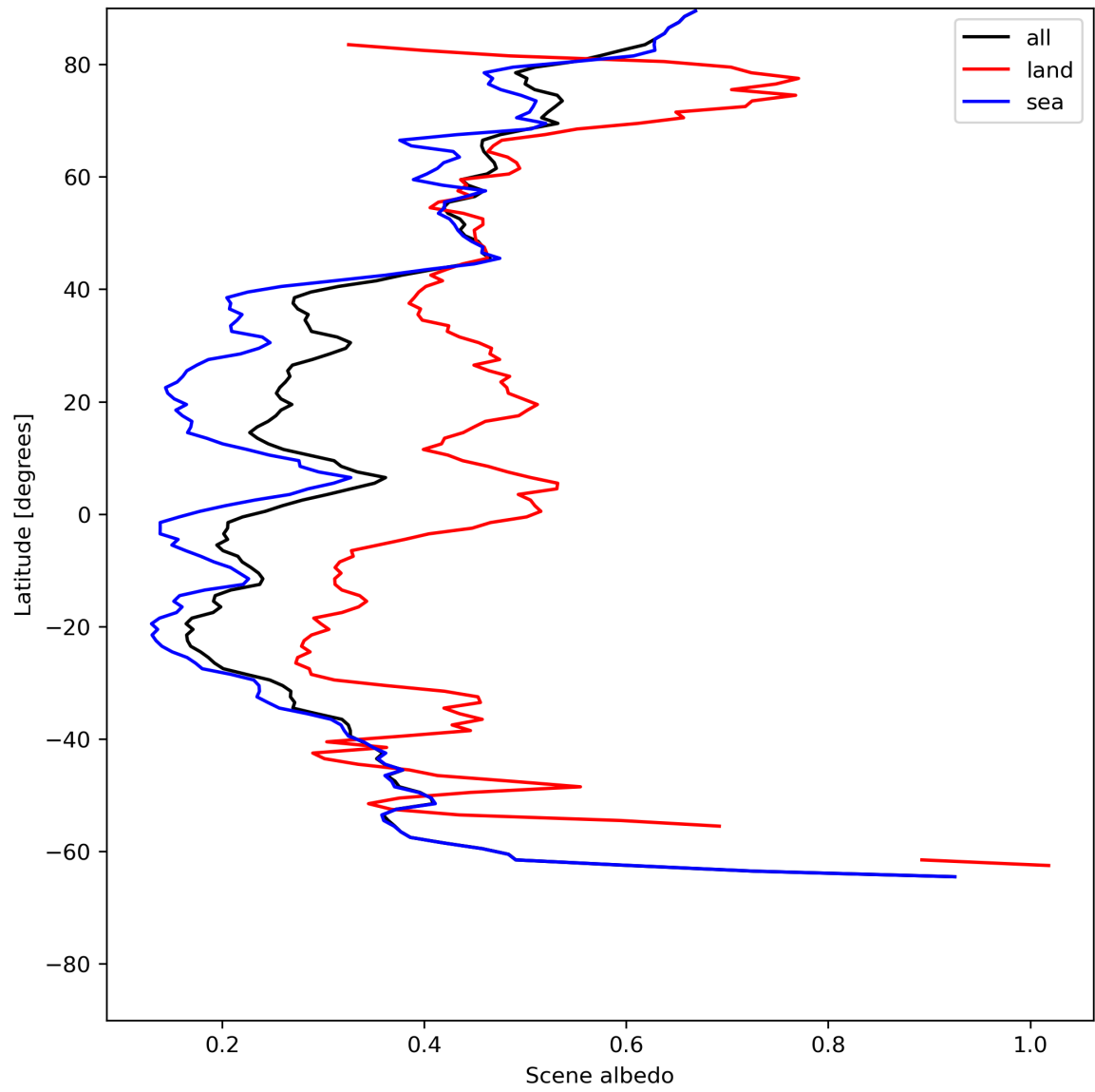
Figure 17: Zonal average of “Scene albedo” for 2023-07-05 to 2023-07-07.
