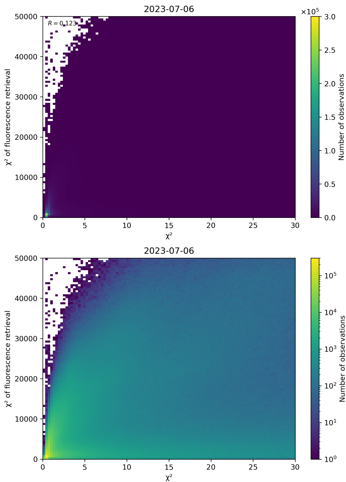
Figure 69: Scatter density plot of “ \chi^2 ” against “ \chi^2 of fluorescence retrieval” for 2023-07-05 to 2023-07-07.
