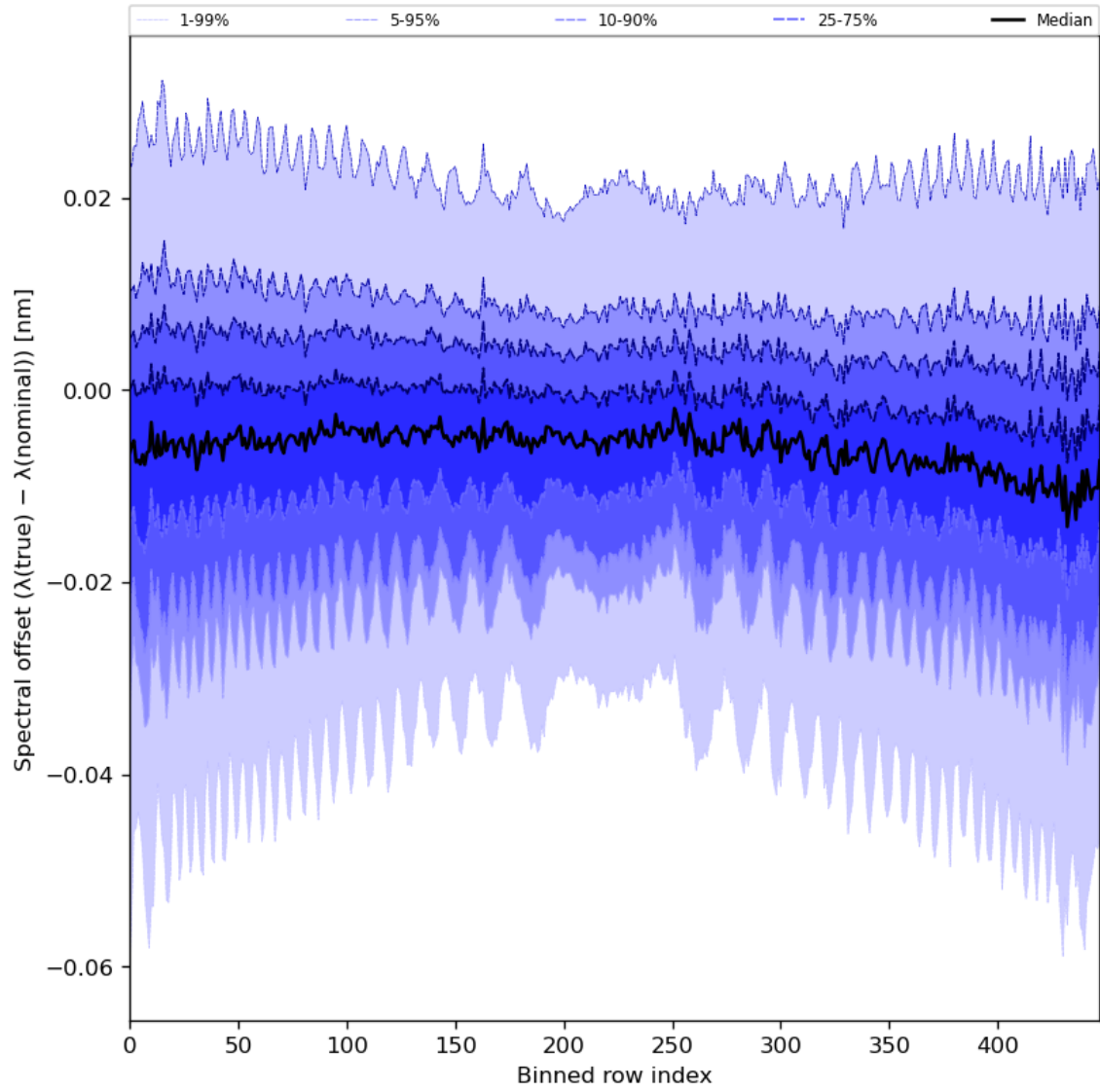
Figure 62: Along track statistics of “Spectral offset ( \lambda(\text{true}) - \lambda(\text{nominal}) )” for 2023-07-05 to 2023-07-07
