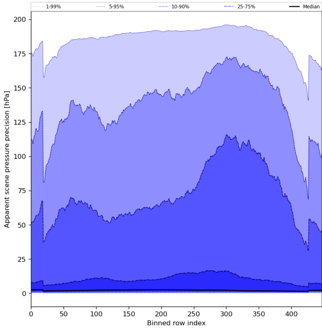
Figure 54: Along track statistics of “Apparent scene pressure precision” for 2023-07-05 to 2023-07-07
