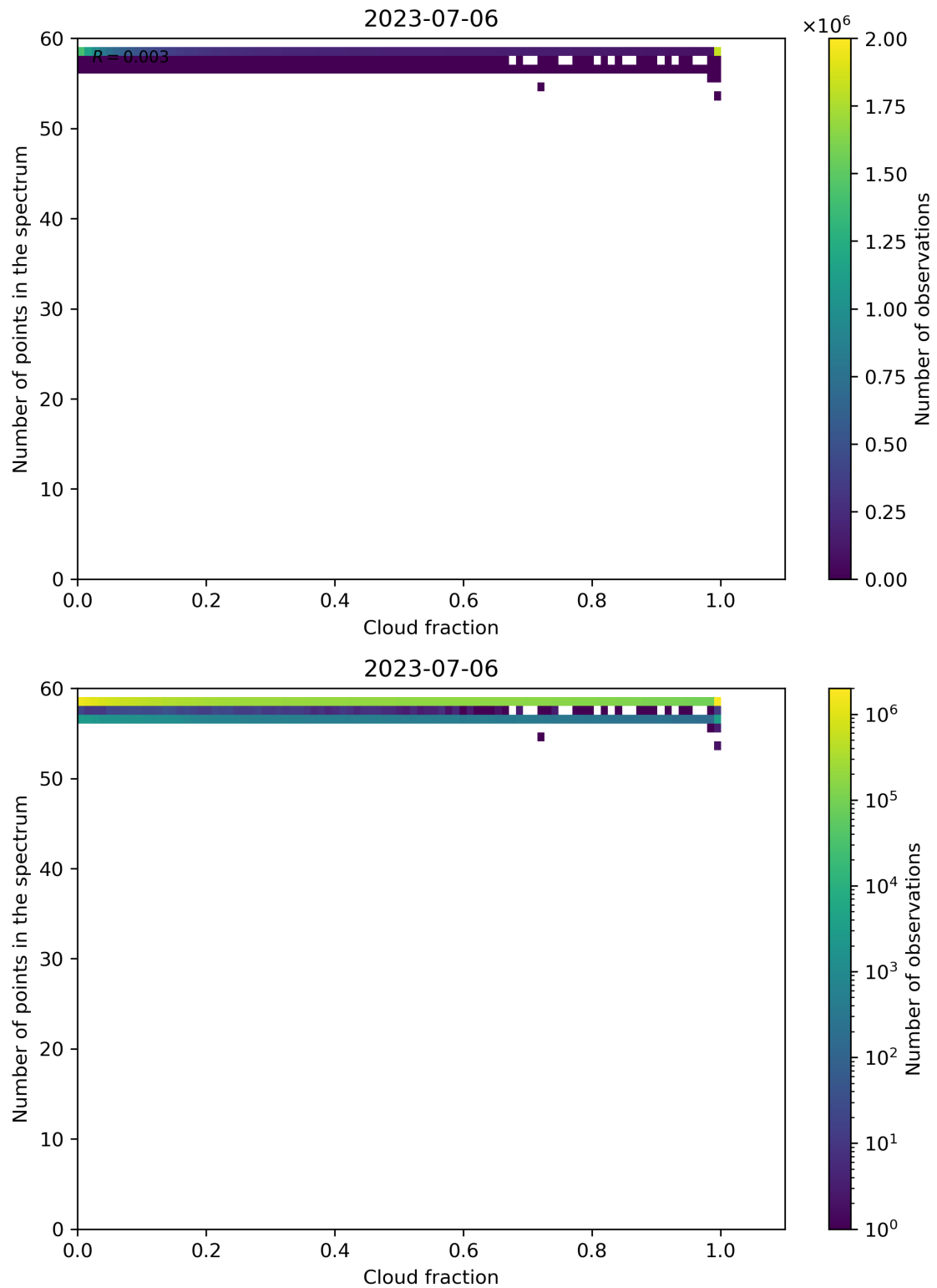
Figure 81: Scatter density plot of “Cloud fraction” against “Number of points in the spectrum” for 2023-07-05 to 2023-07-07.
