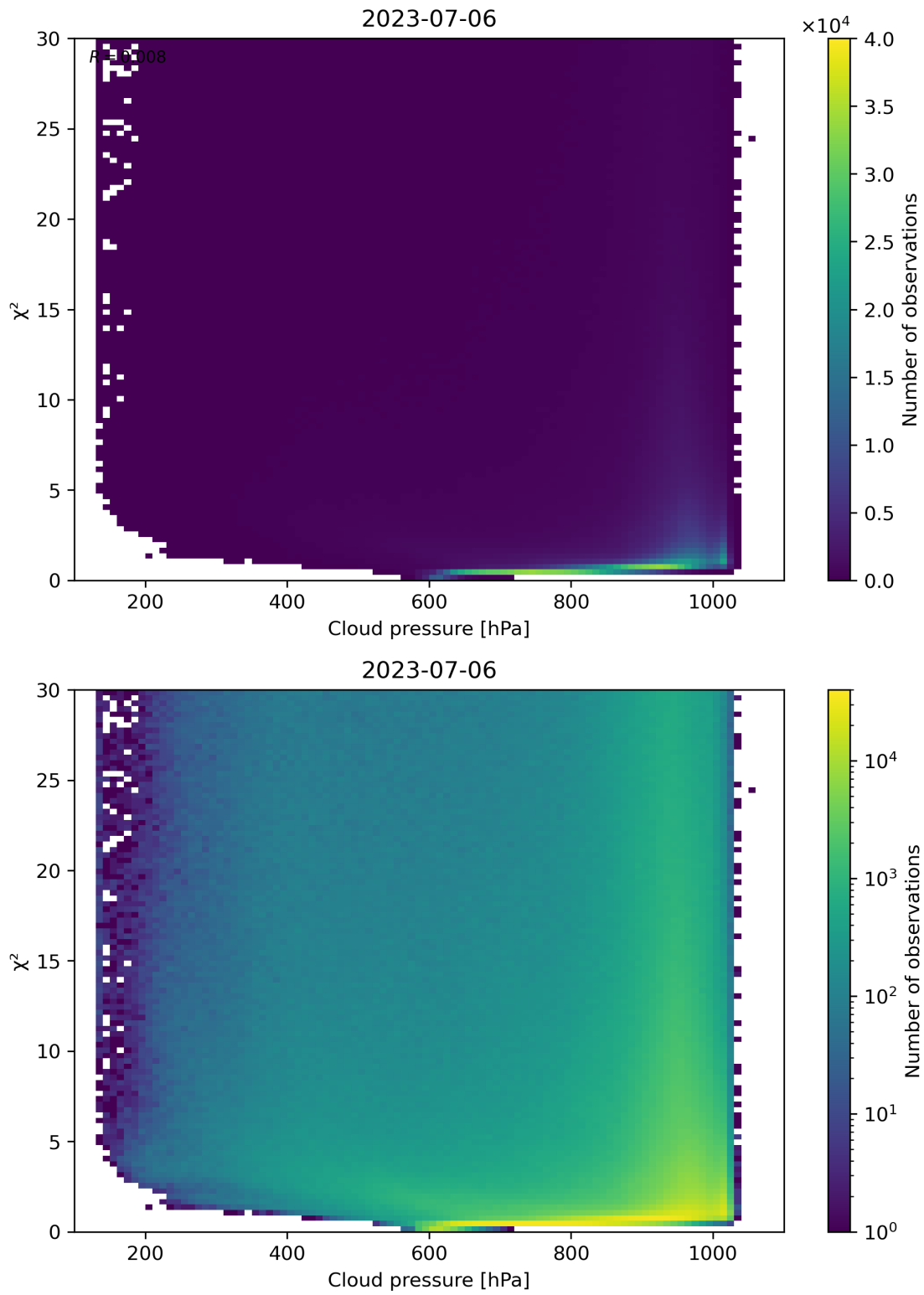
Figure 85: Scatter density plot of “Cloud pressure” against “ \chi^2 ” for 2023-07-05 to 2023-07-07.
