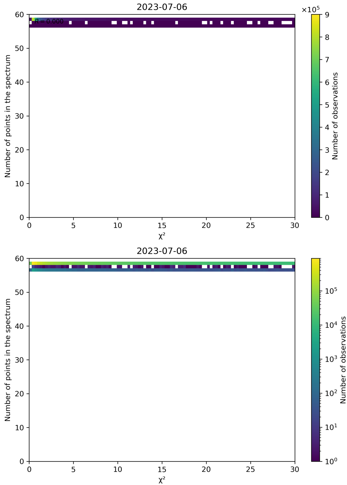
Figure 74: Scatter density plot of “ \chi^2 ” against “Number of points in the spectrum” for 2023-07-05 to 2023-07-07.
