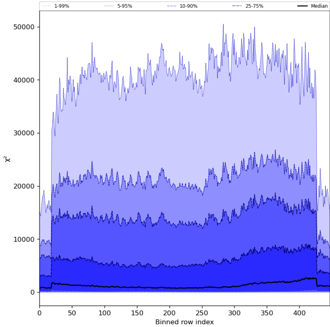
Figure 55: Along track statistics of “ \chi^2 ” for 2023-07-05 to 2023-07-07
