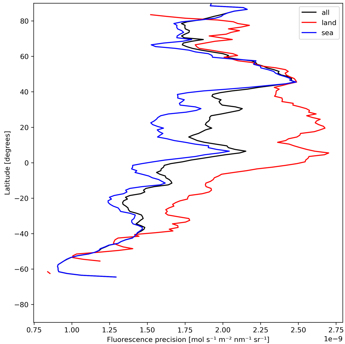
Figure 24: Zonal average of “Fluorescence precision” for 2023-07-05 to 2023-07-07.
