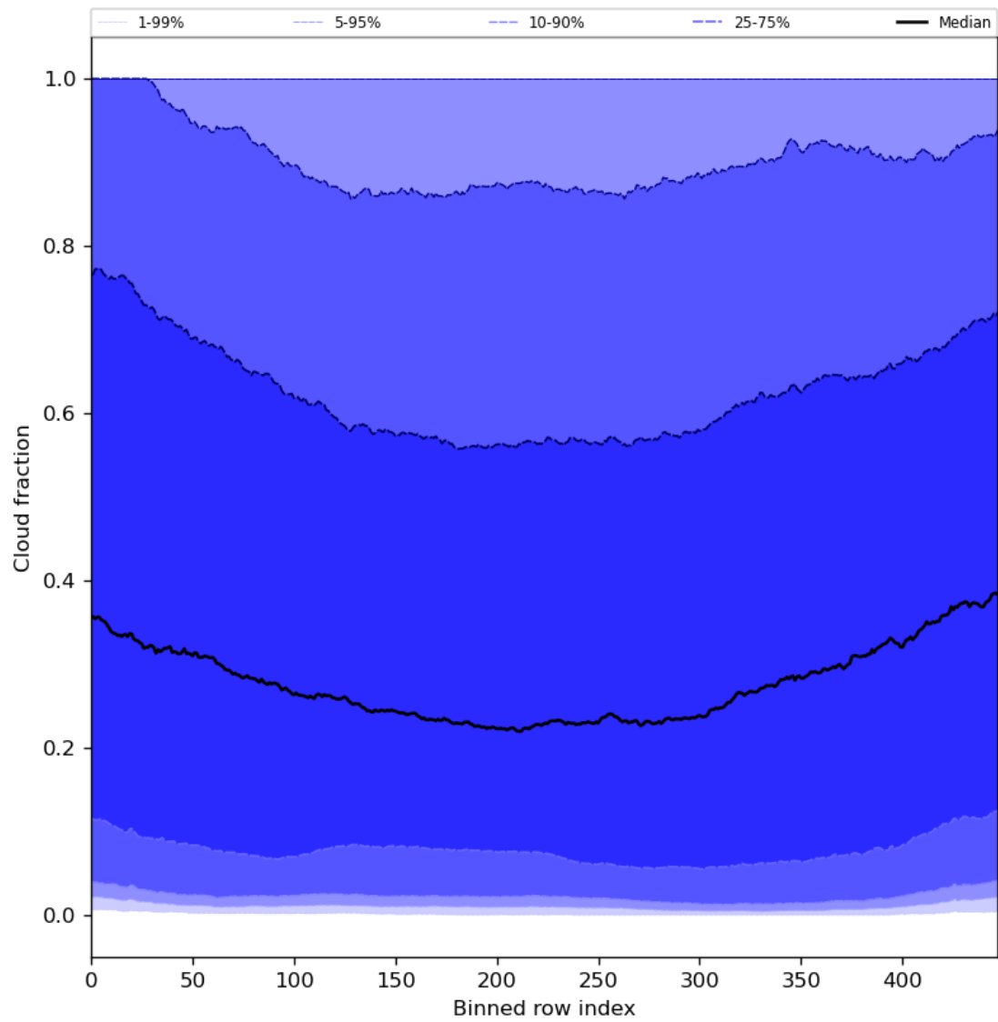
Figure 49: Along track statistics of “Cloud fraction” for 2023-07-05 to 2023-07-07
