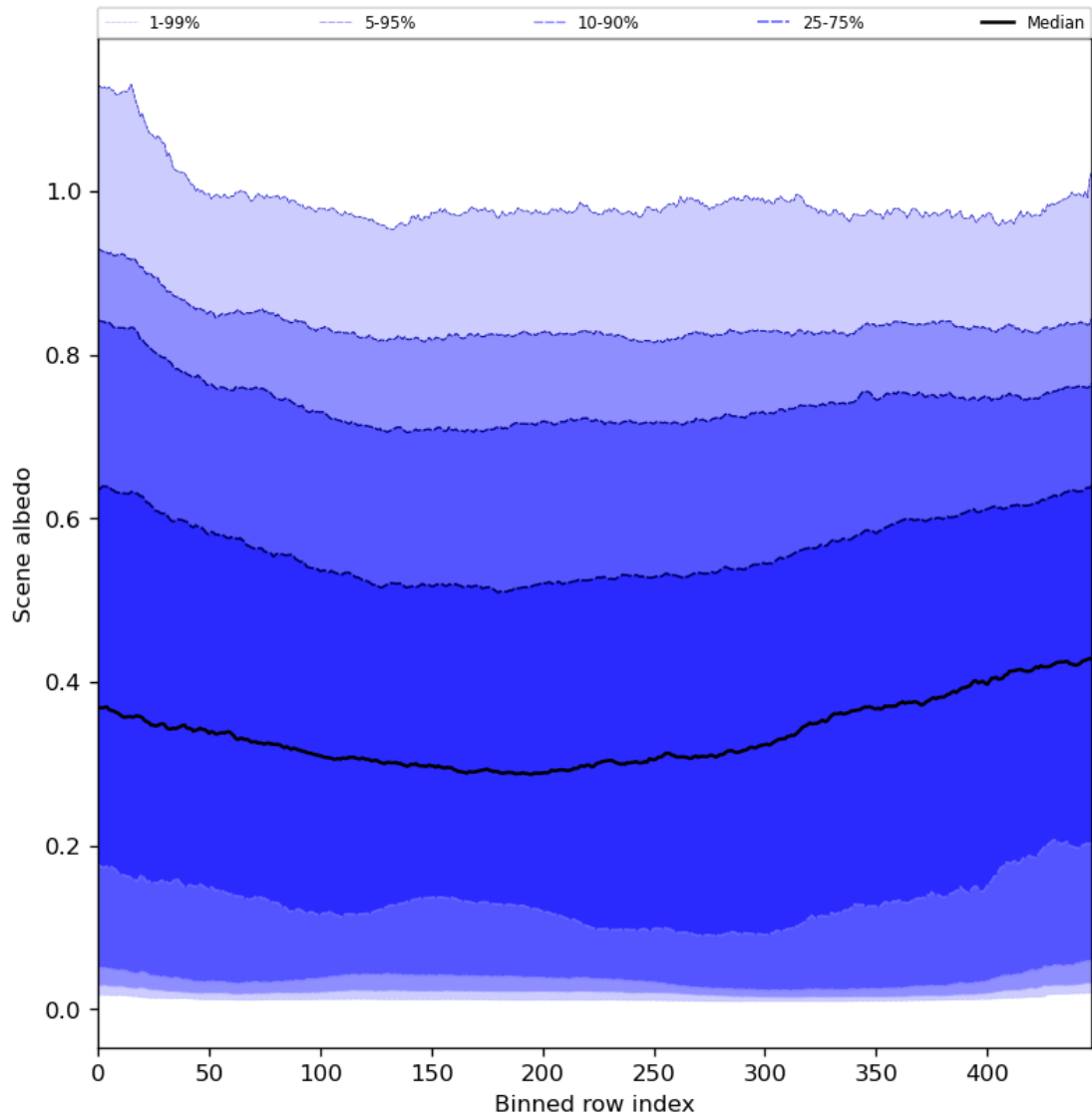
Figure 51: Along track statistics of “Scene albedo” for 2023-07-05 to 2023-07-07
