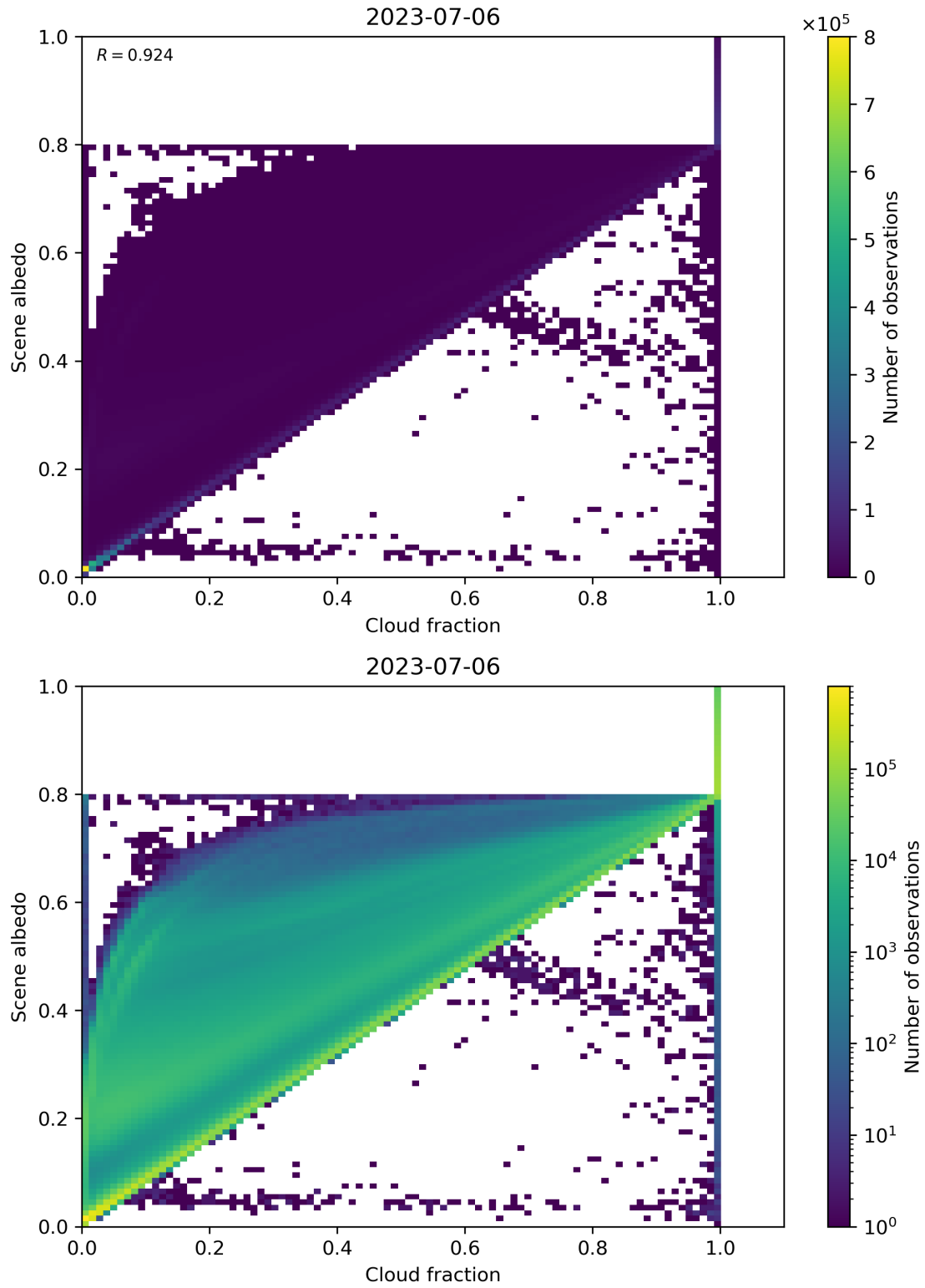
Figure 82: Scatter density plot of “Cloud fraction” against “Scene albedo” for 2023-07-05 to 2023-07-07.
