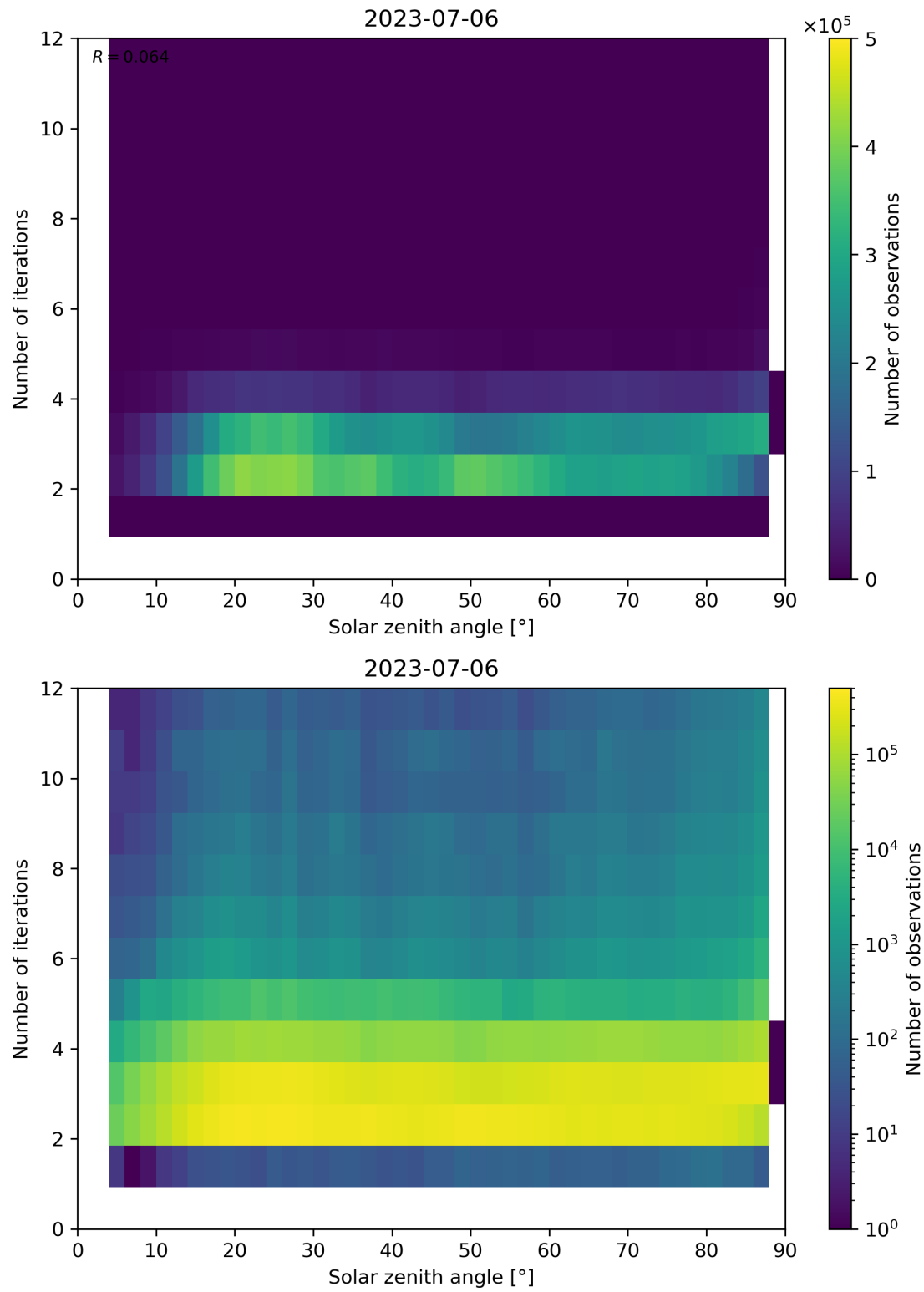
Figure 125: Scatter density plot of “Solar zenith angle” against “Number of iterations” for 2023-07-05 to 2023-07-07.
