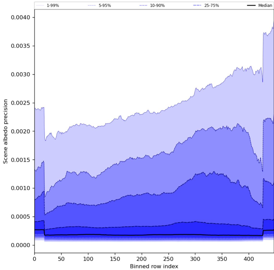
Figure 52: Along track statistics of “Scene albedo precision” for 2023-07-05 to 2023-07-07
