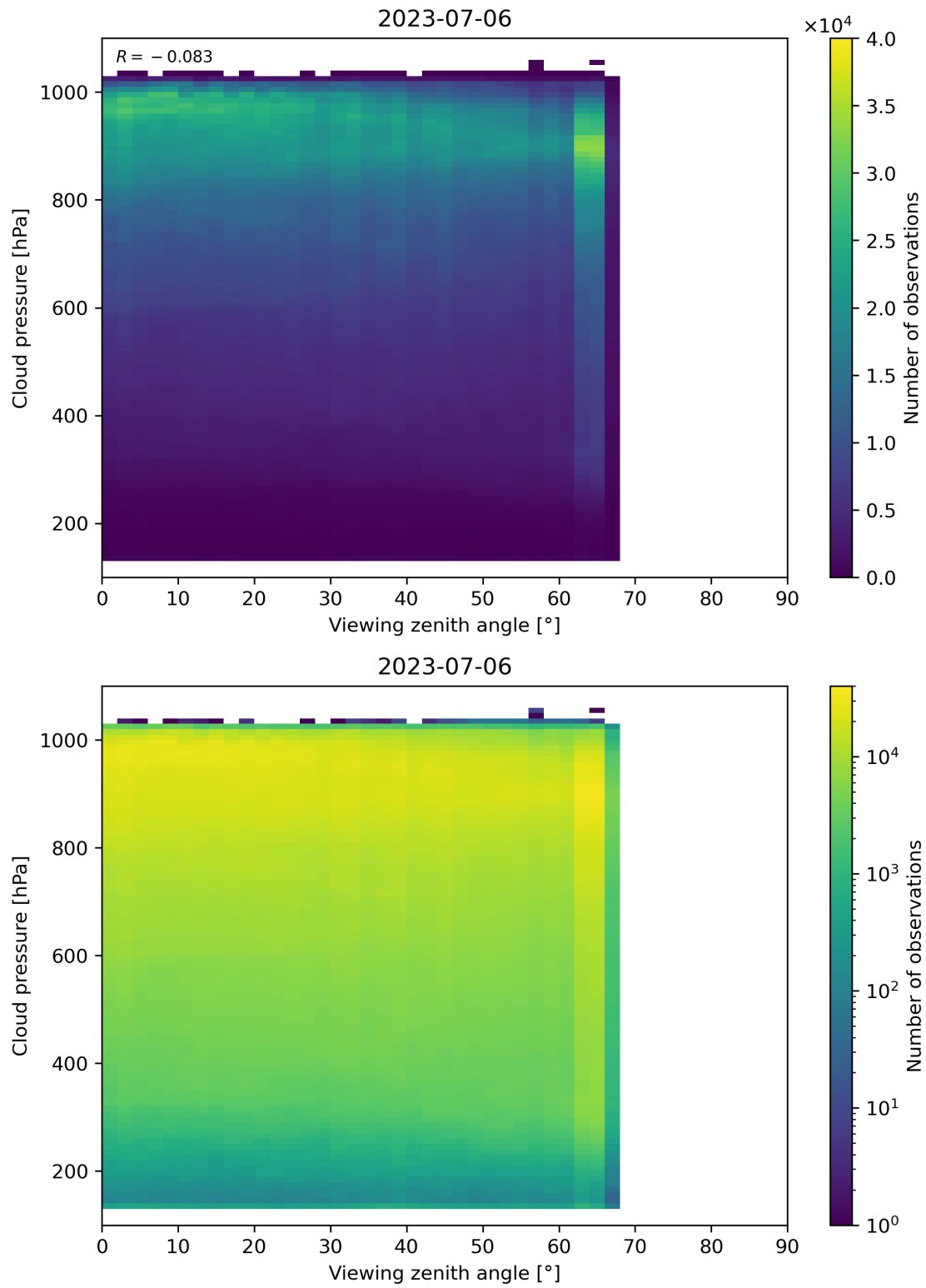
Figure 133: Scatter density plot of “Viewing zenith angle” against “Cloud pressure” for 2023-07-05 to 2023-07-07.
