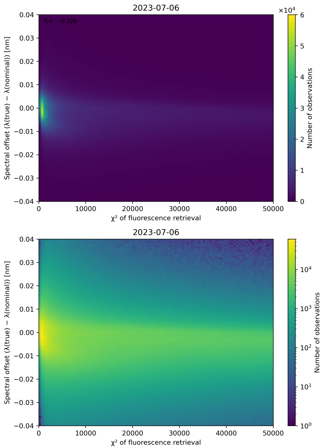
Figure 72: Scatter density plot of " \chi^2 of fluorescence retrieval" against "Spectral offset ( \lambda(\text{true}) - \lambda(\text{nominal})) " for 2023-07-05 to 2023-07-07.
