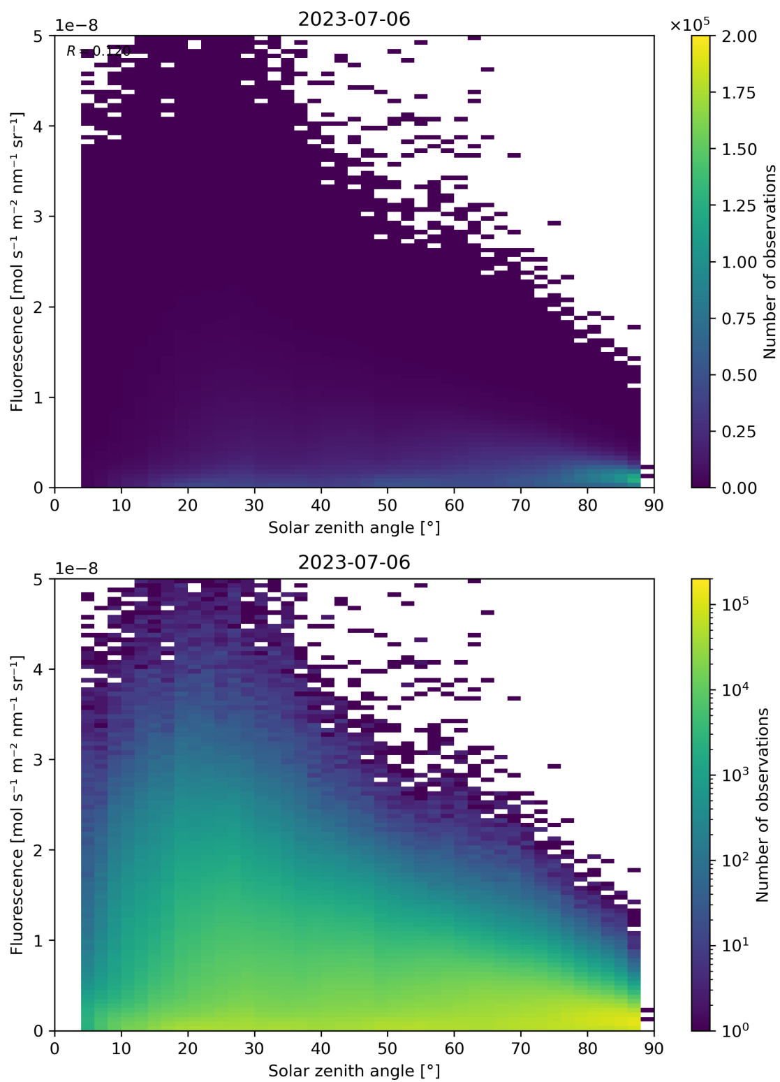
Figure 123: Scatter density plot of “Solar zenith angle” against “Fluorescence” for 2023-07-05 to 2023-07-07.
