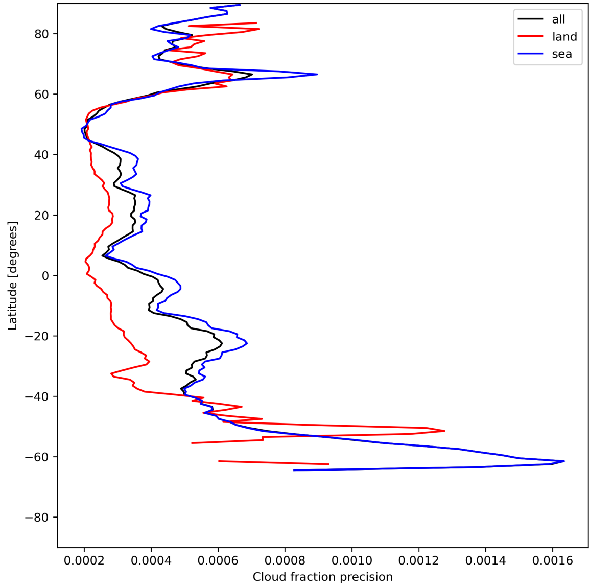
Figure 16: Zonal average of “Cloud fraction precision” for 2023-07-05 to 2023-07-07.
