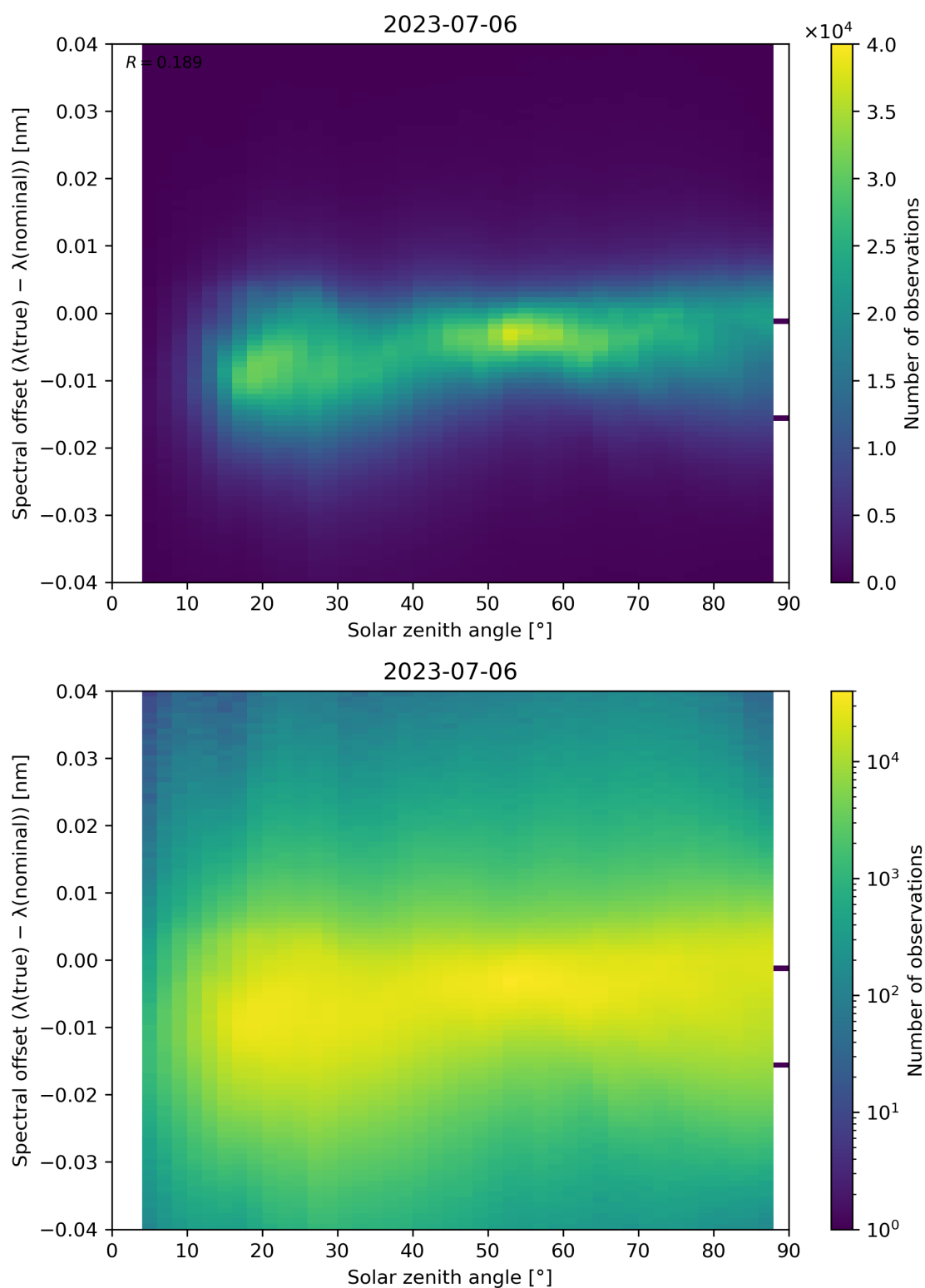
Figure 128: Scatter density plot of “Solar zenith angle” against “Spectral offset ( \lambda(\text{true}) - \lambda(\text{nominal}) )” for 2023-07-05 to 2023-07-07.
