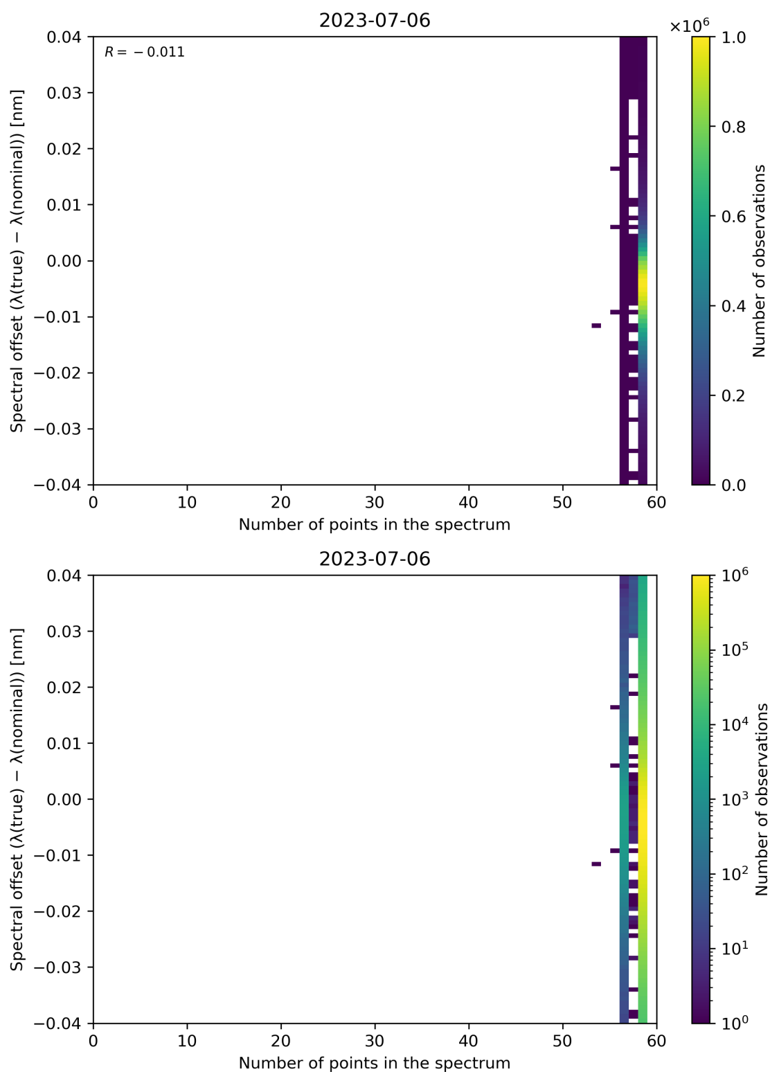
Figure 110: Scatter density plot of “Number of points in the spectrum” against “Spectral offset ( \lambda(\text{true}) - \lambda(\text{nominal}) )” for 2023-07-05 to 2023-07-07.
