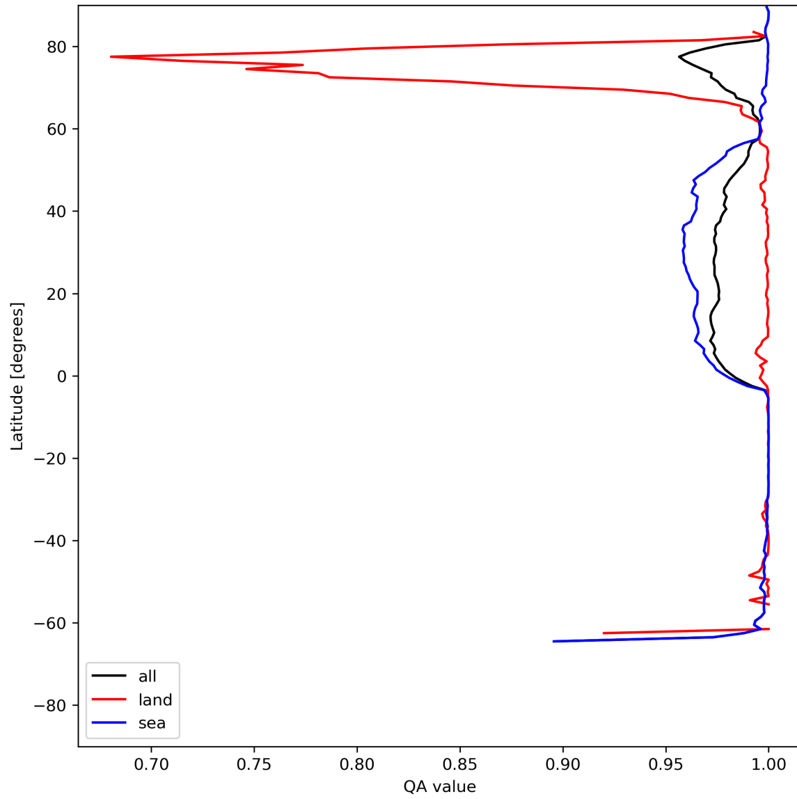
Figure 12: Zonal average of “QA value” for 2023-07-05 to 2023-07-07.
