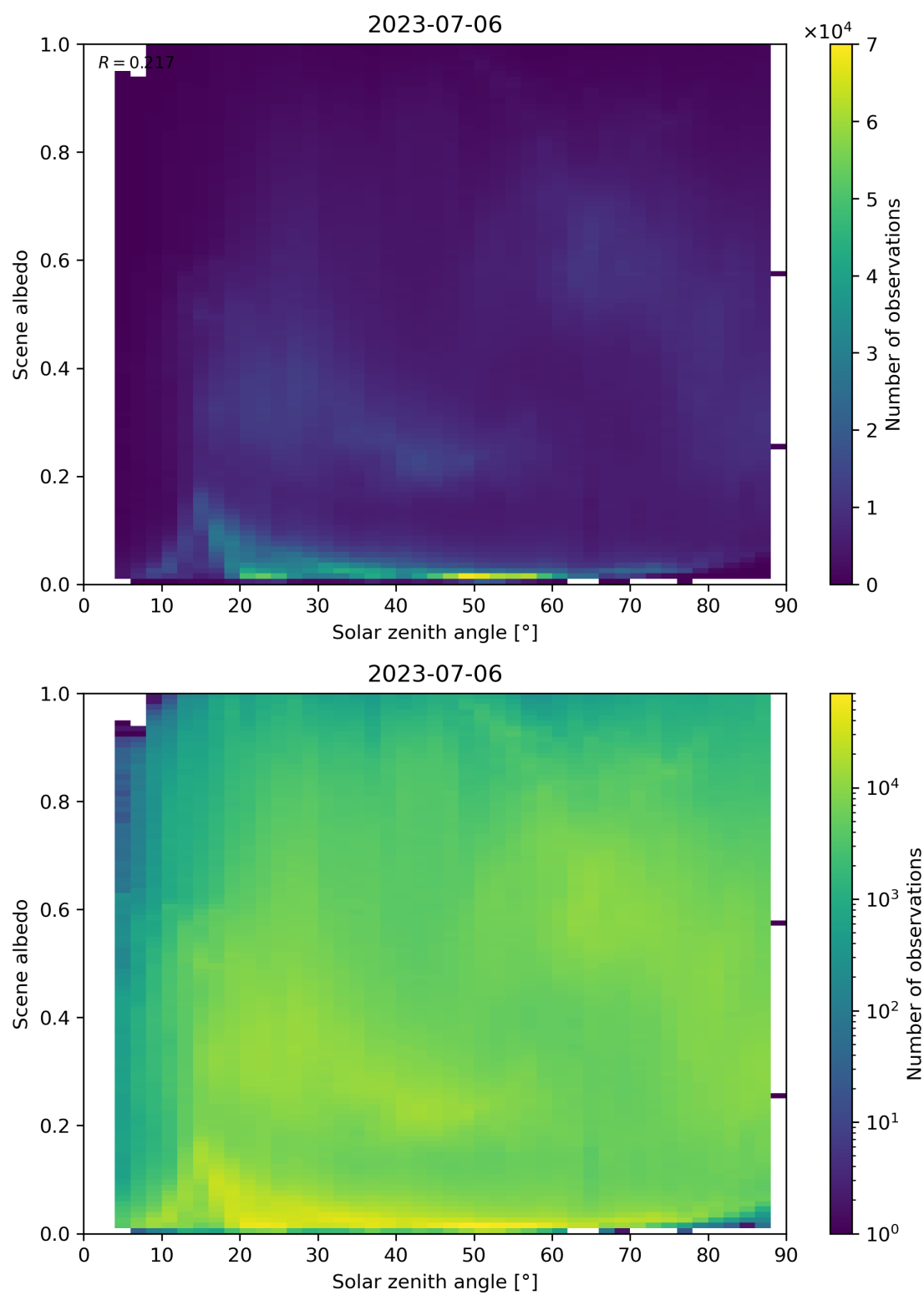
Figure 127: Scatter density plot of “Solar zenith angle” against “Scene albedo” for 2023-07-05 to 2023-07-07.
