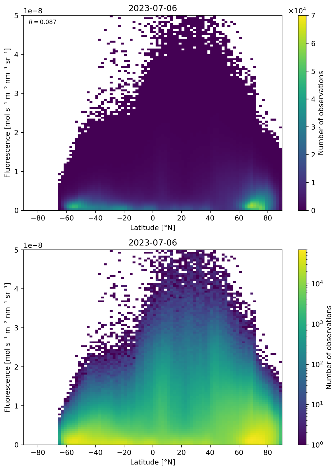
Figure 101: Scatter density plot of “Latitude” against “Fluorescence” for 2023-07-05 to 2023-07-07.
