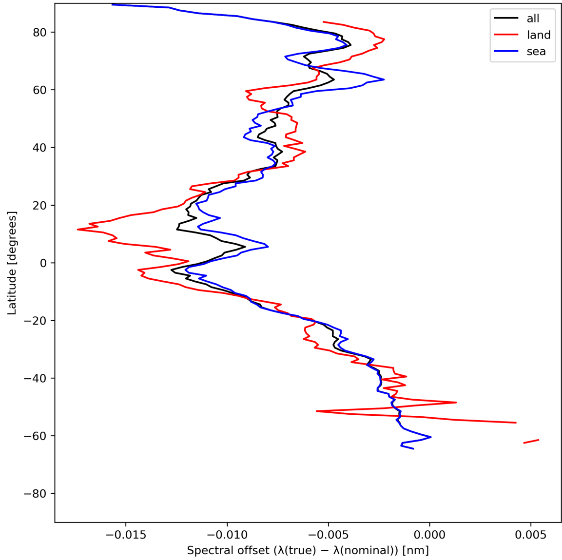
Figure 28: Zonal average of “Spectral offset ( \lambda(\text{true}) - \lambda(\text{nominal}) )” for 2023-07-05 to 2023-07-07.
