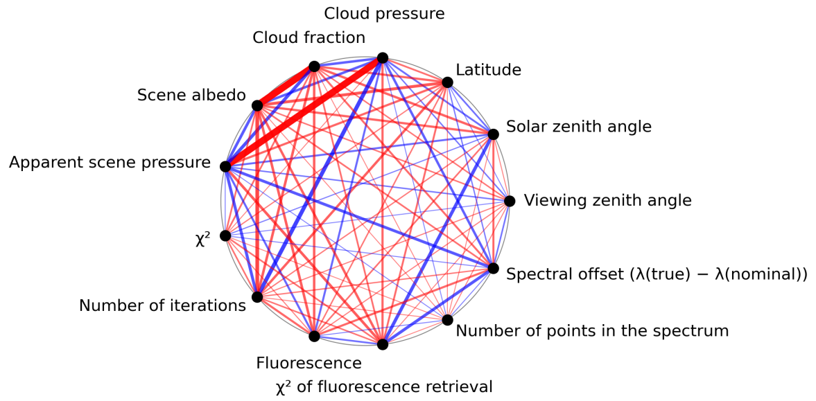
Figure 1: Map of correlation graph for 2023-07-05 to 2023-07-07.
