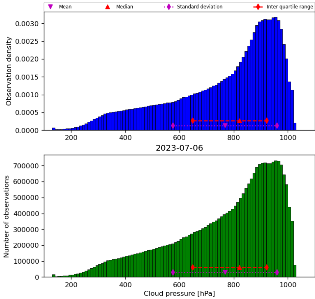
Figure 30: Histogram of “Cloud pressure” for 2023-07-05 to 2023-07-07
