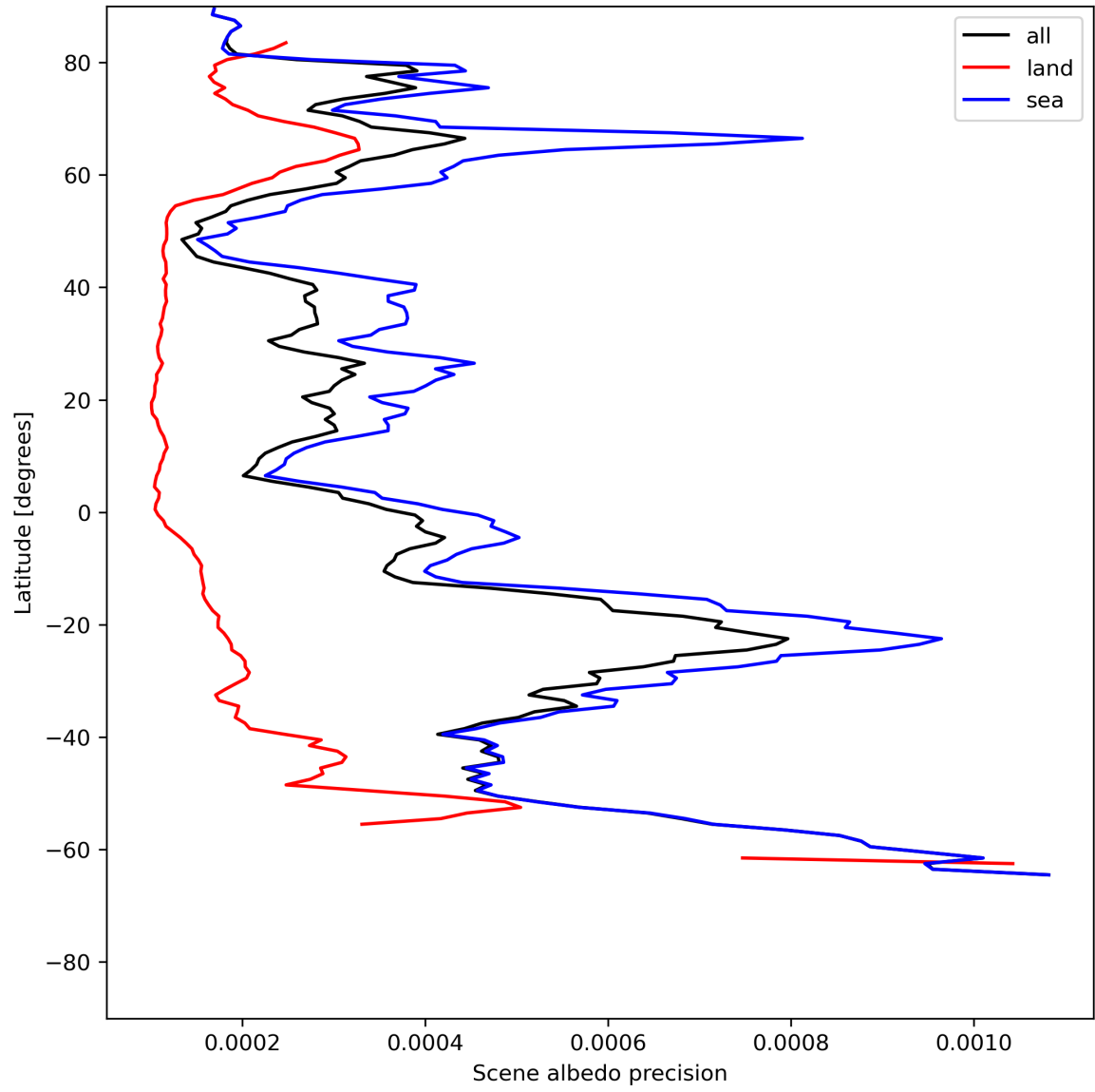
Figure 18: Zonal average of “Scene albedo precision” for 2023-07-05 to 2023-07-07.
