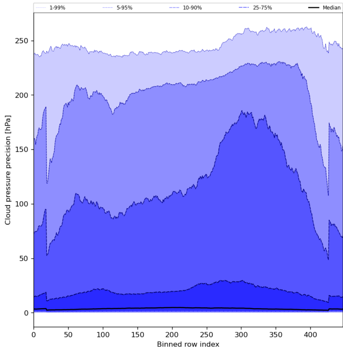
Figure 48: Along track statistics of “Cloud pressure precision” for 2023-07-05 to 2023-07-07
