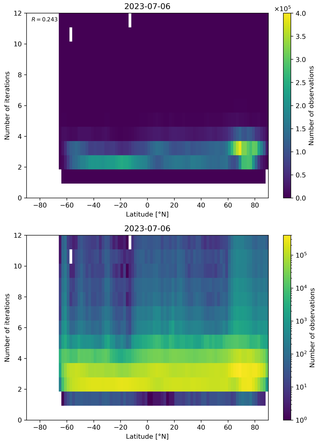
Figure 102: Scatter density plot of “Latitude” against “Number of iterations” for 2023-07-05 to 2023-07-07.
