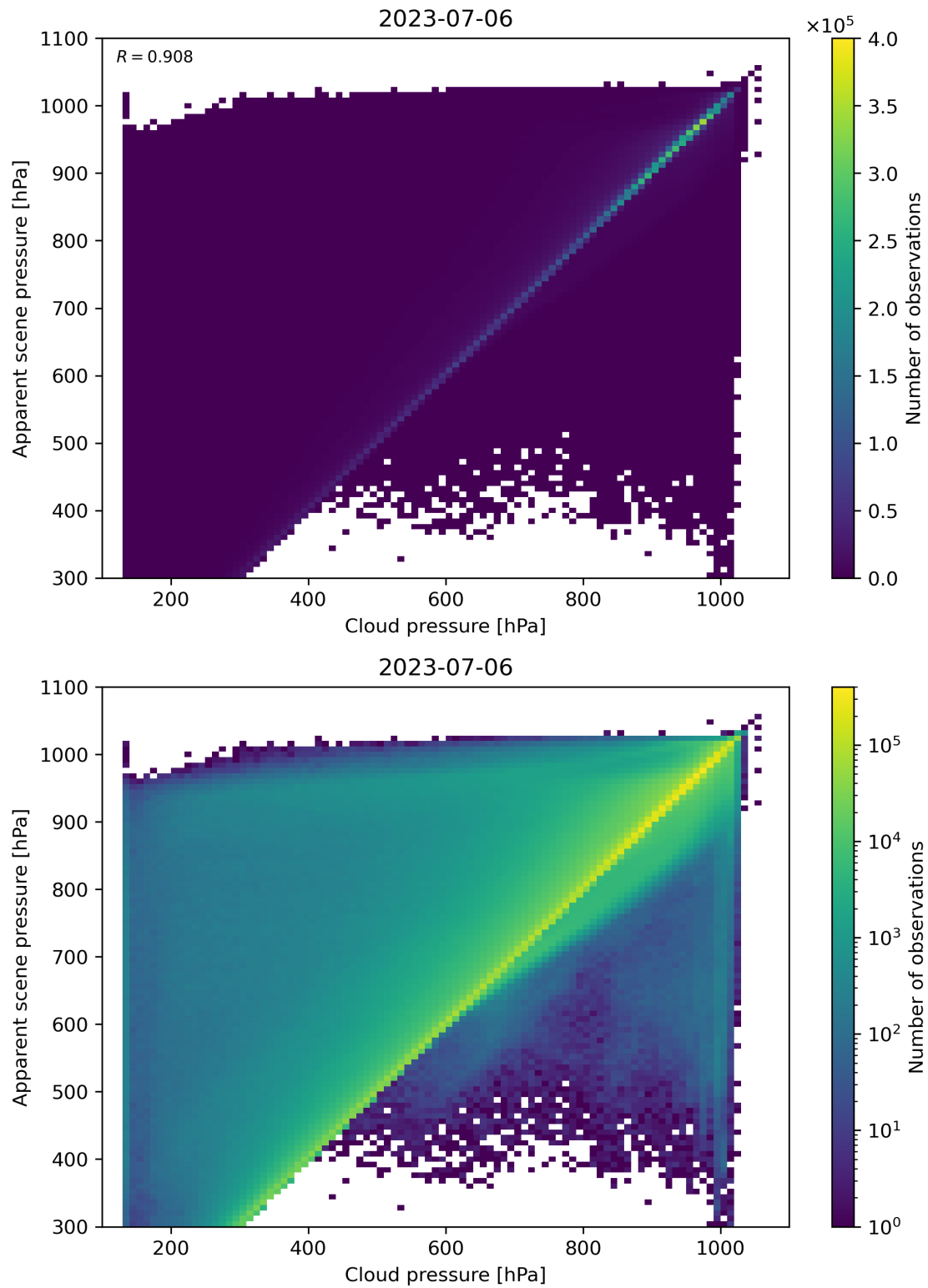
Figure 84: Scatter density plot of “Cloud pressure” against “Apparent scene pressure” for 2023-07-05 to 2023-07-07.
