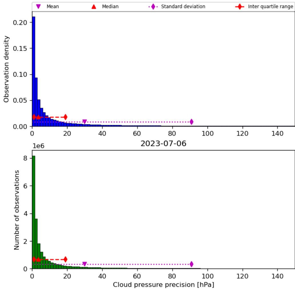
Figure 31: Histogram of “Cloud pressure precision” for 2023-07-05 to 2023-07-07
