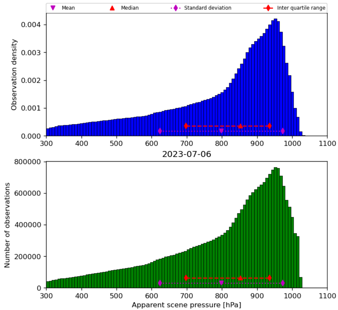
Figure 36: Histogram of “Apparent scene pressure” for 2023-07-05 to 2023-07-07
