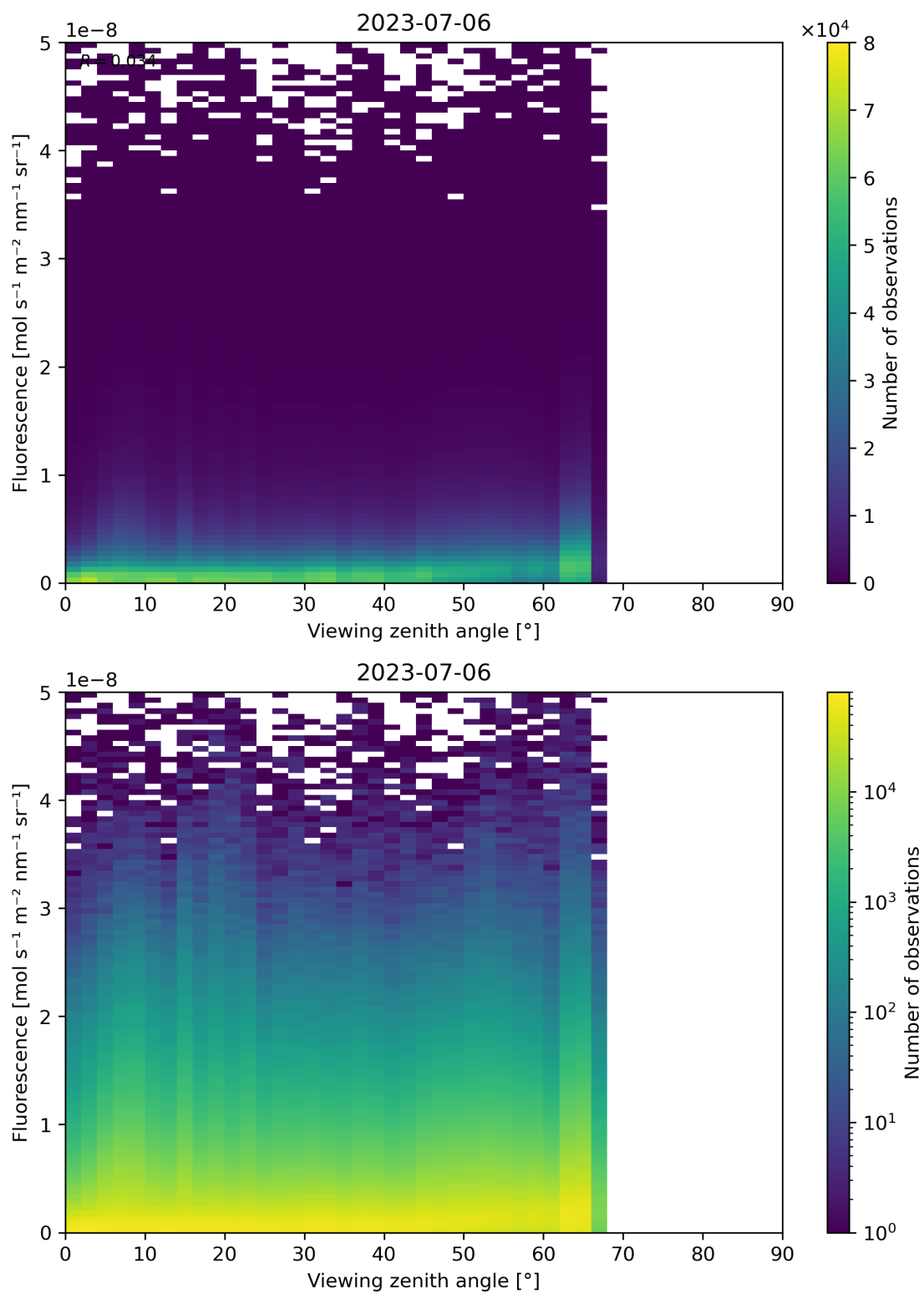
Figure 134: Scatter density plot of “Viewing zenith angle” against “Fluorescence” for 2023-07-05 to 2023-07-07.
