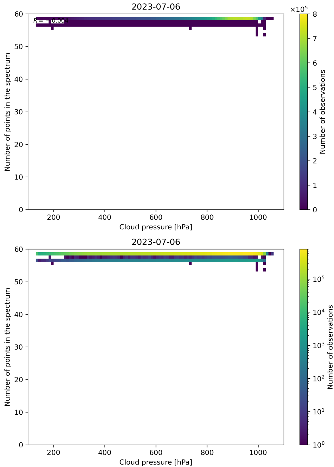
Figure 90: Scatter density plot of “Cloud pressure” against “Number of points in the spectrum” for 2023-07-05 to 2023-07-07.
