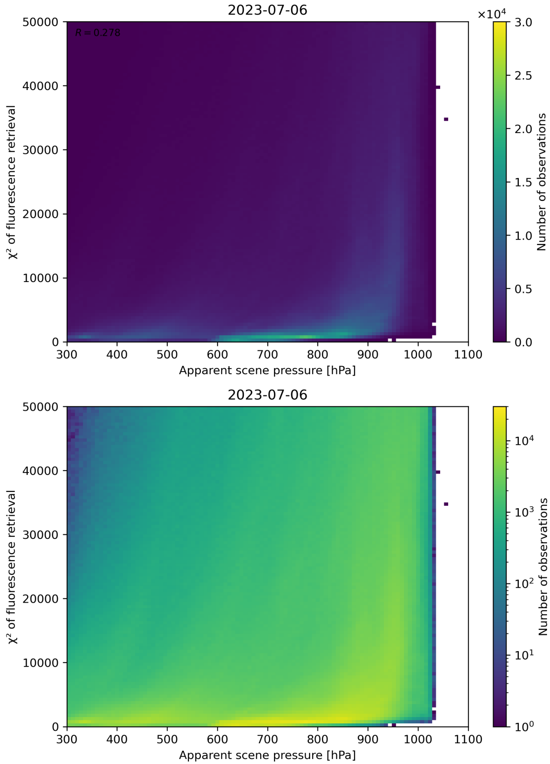
Figure 64: Scatter density plot of “Apparent scene pressure” against “ \chi^2 of fluorescence retrieval” for 2023-07-05 to 2023-07-07.
