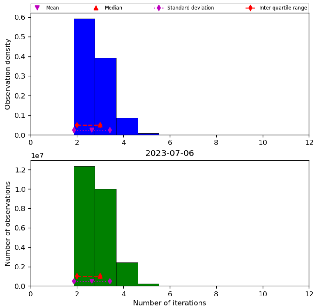
Figure 39: Histogram of “Number of iterations” for 2023-07-05 to 2023-07-07
