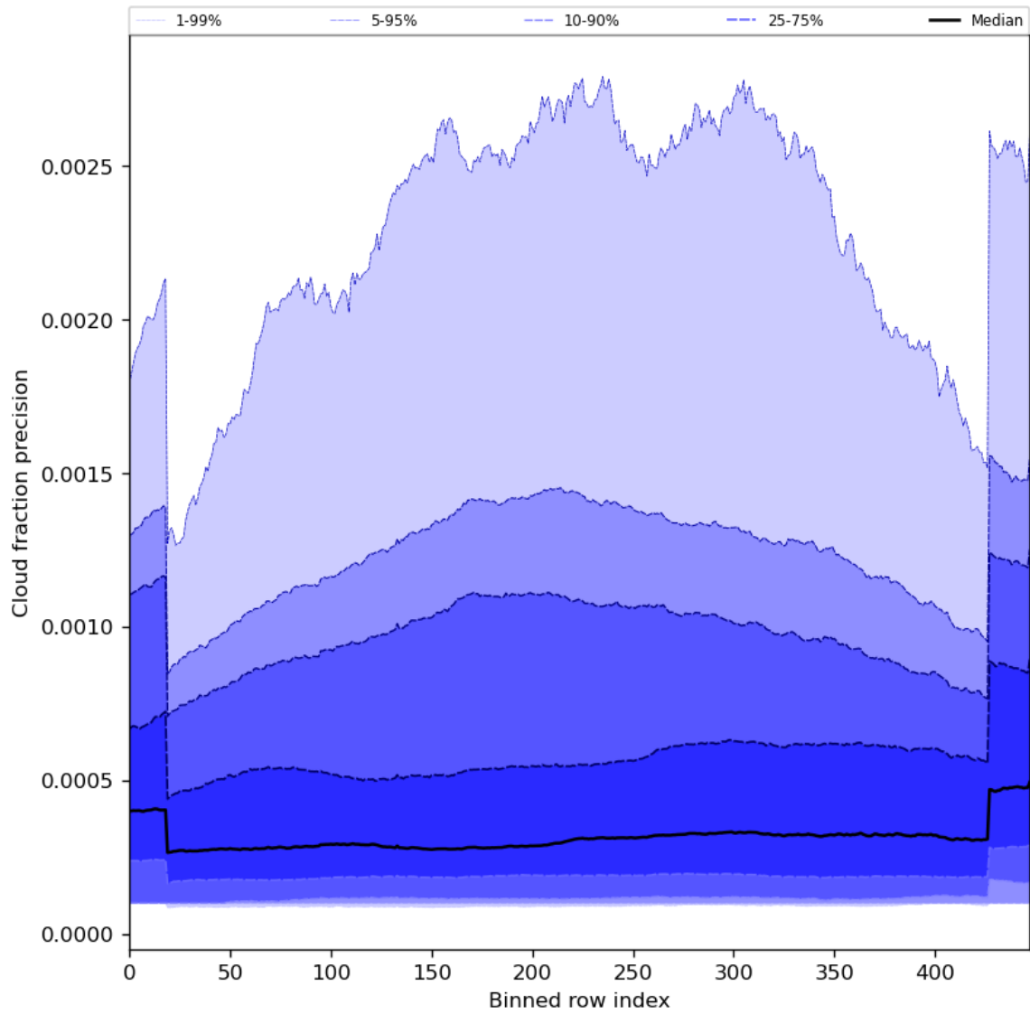
Figure 50: Along track statistics of “Cloud fraction precision” for 2023-07-05 to 2023-07-07
