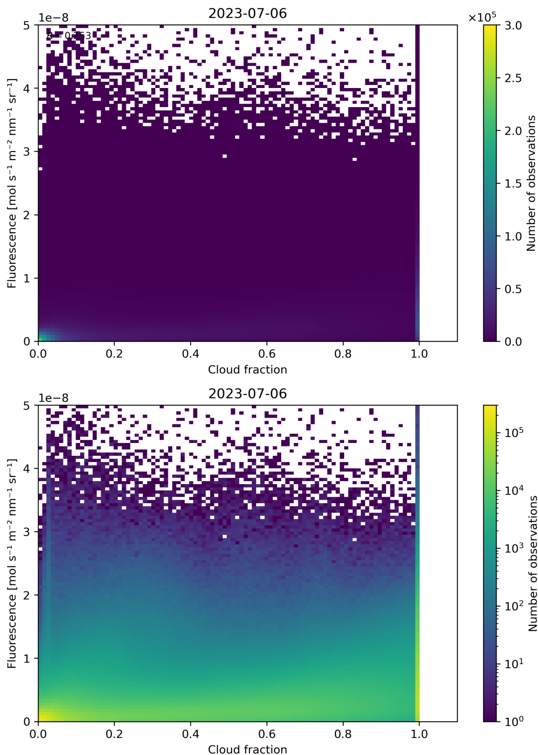
Figure 79: Scatter density plot of “Cloud fraction” against “Fluorescence” for 2023-07-05 to 2023-07-07.
