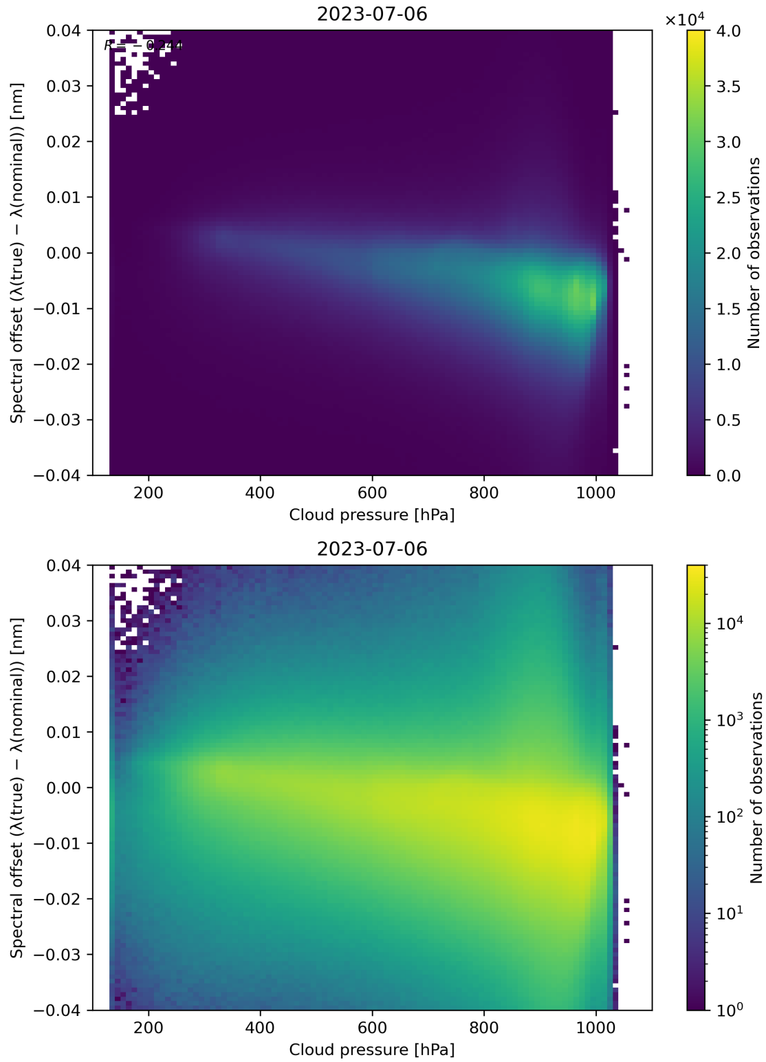
Figure 92: Scatter density plot of “Cloud pressure” against “Spectral offset ( \lambda(\text{true}) - \lambda(\text{nominal}) )” for 2023-07-05 to 2023-07-07.
