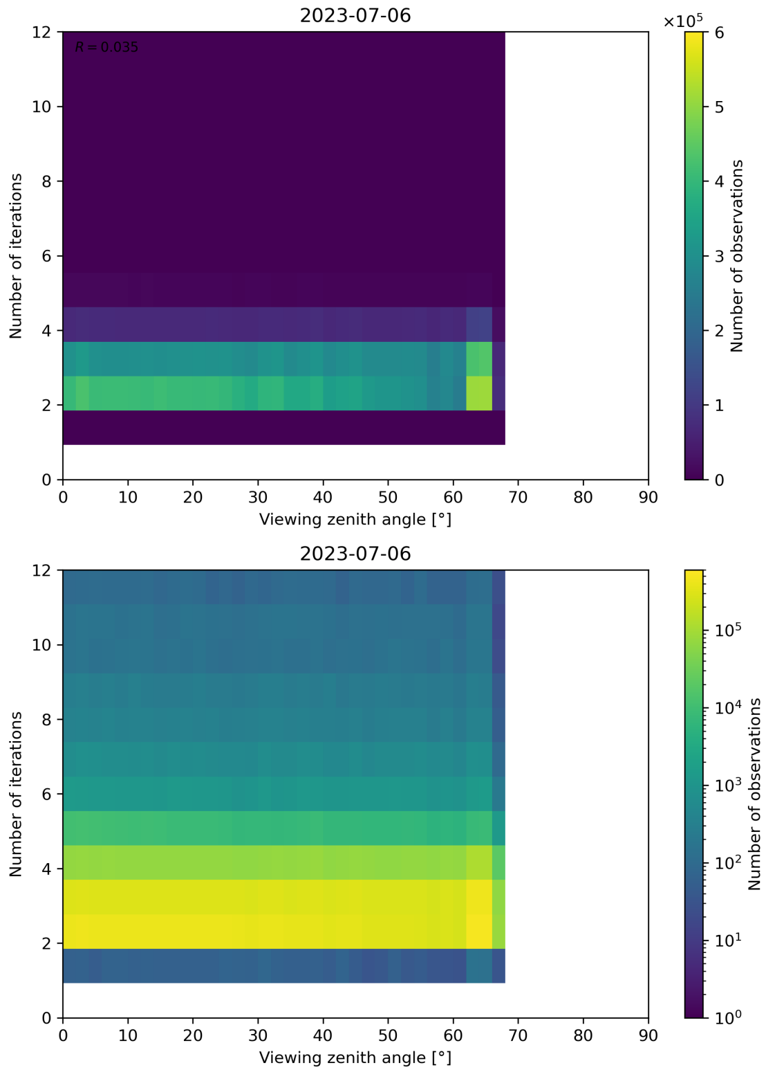
Figure 136: Scatter density plot of “Viewing zenith angle” against “Number of iterations” for 2023-07-05 to 2023-07-07.
