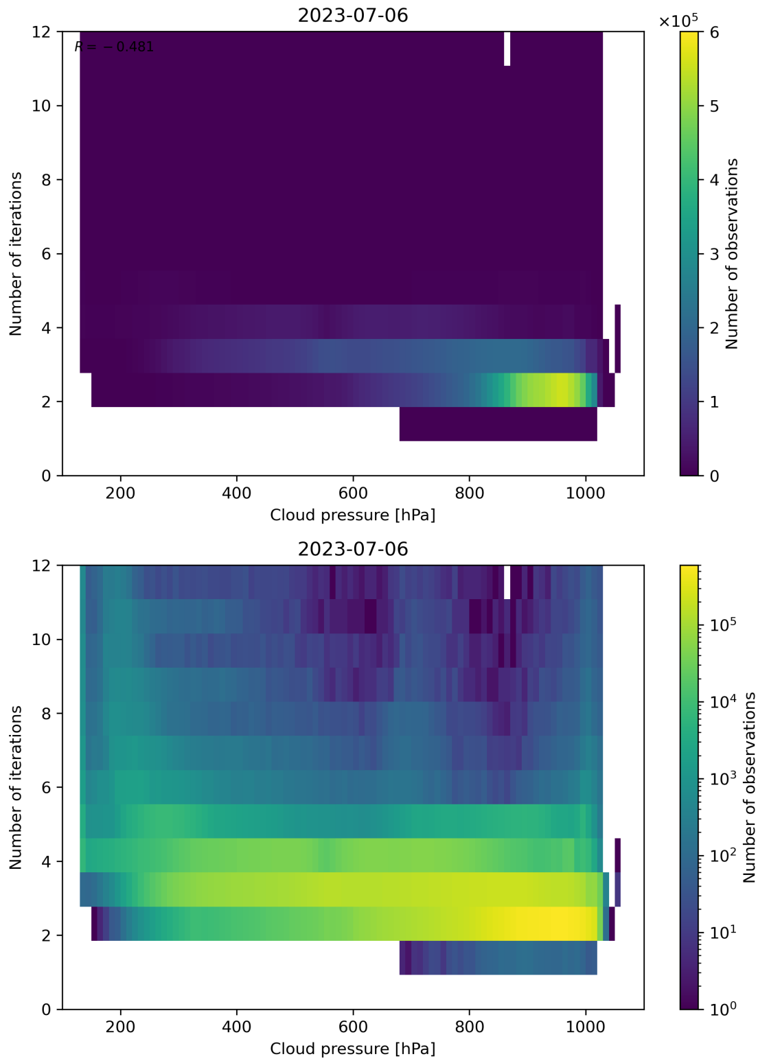
Figure 89: Scatter density plot of “Cloud pressure” against “Number of iterations” for 2023-07-05 to 2023-07-07.
