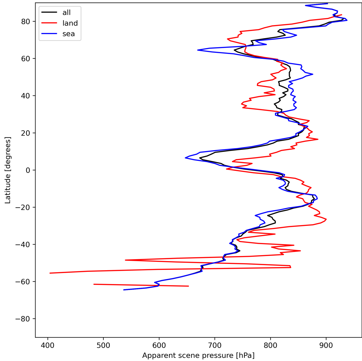
Figure 19: Zonal average of “Apparent scene pressure” for 2023-07-05 to 2023-07-07.
