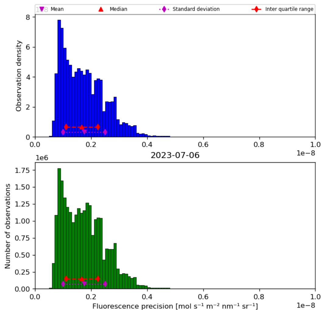
Figure 41: Histogram of “Fluorescence precision” for 2023-07-05 to 2023-07-07
