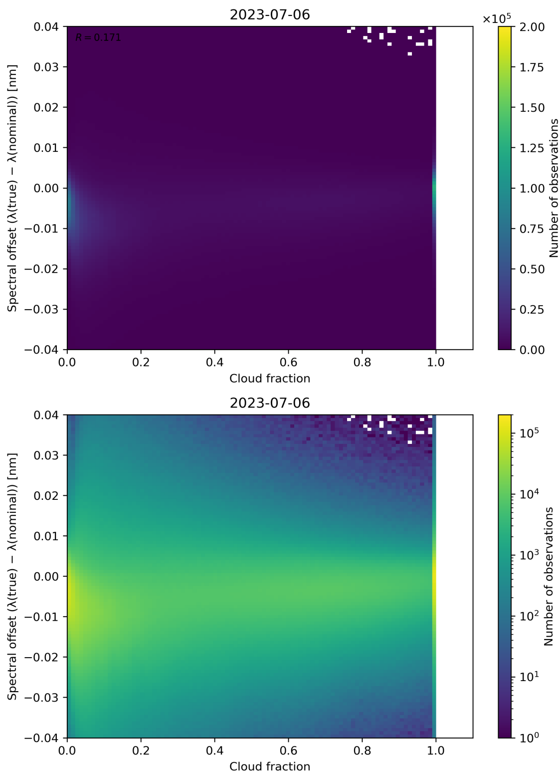
Figure 83: Scatter density plot of “Cloud fraction” against “Spectral offset ( \lambda(\text{true}) - \lambda(\text{nominal}) )” for 2023-07-05 to 2023-07-07.
