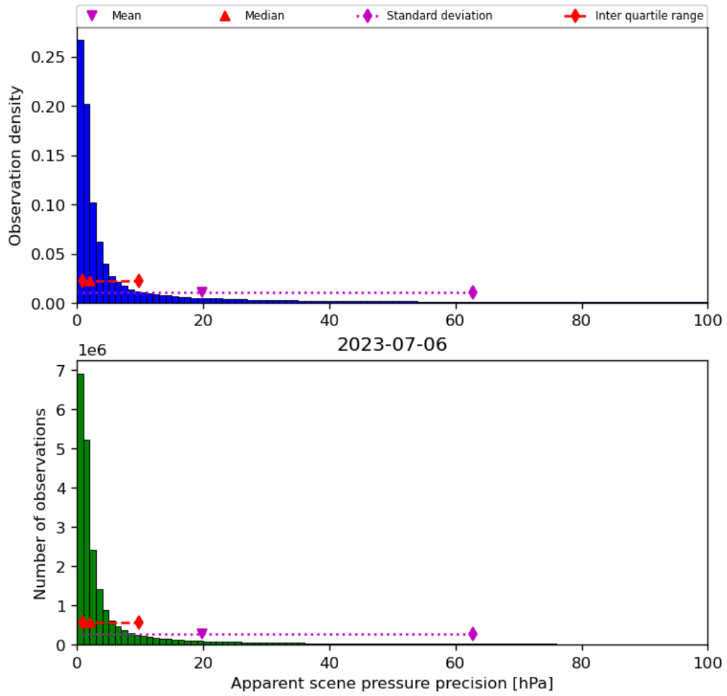
Figure 37: Histogram of “Apparent scene pressure precision” for 2023-07-05 to 2023-07-07
