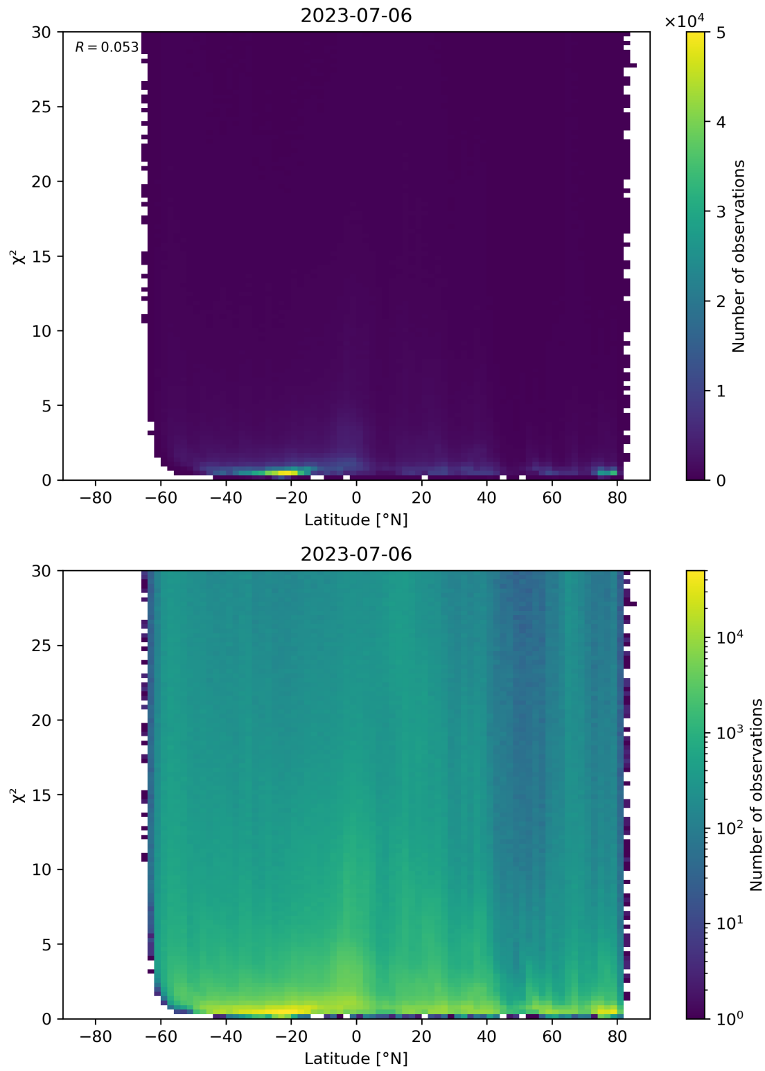
Figure 97: Scatter density plot of “Latitude” against “ \chi^2 ” for 2023-07-05 to 2023-07-07.
