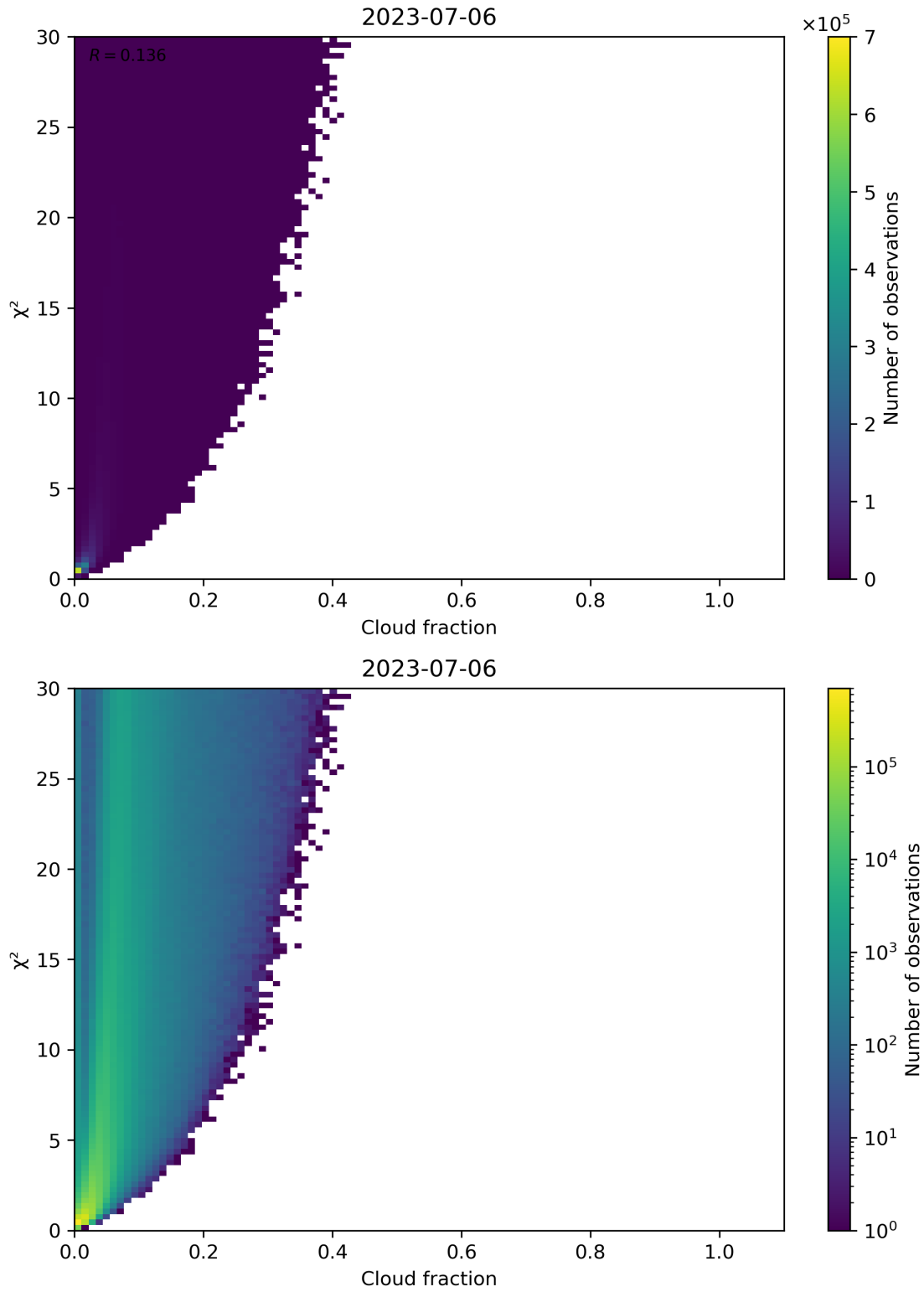
Figure 77: Scatter density plot of “Cloud fraction” against “ \chi^2 ” for 2023-07-05 to 2023-07-07.
