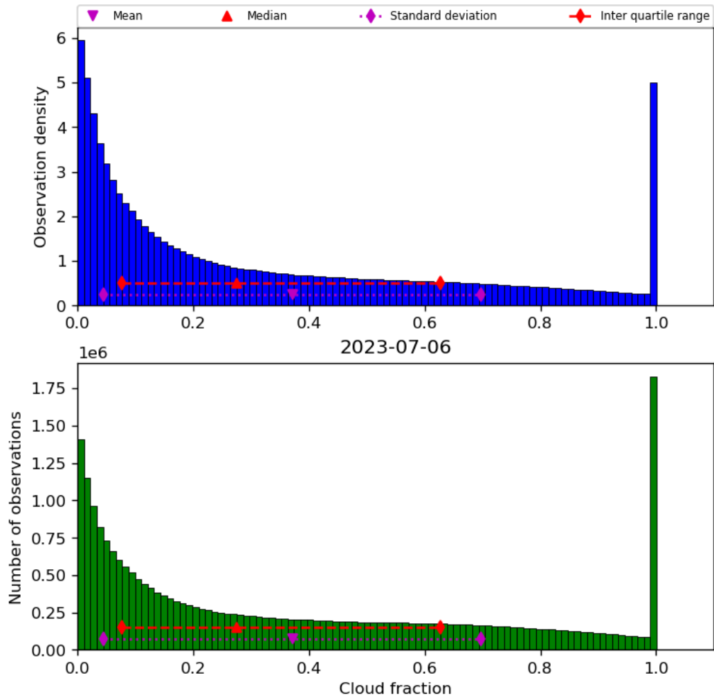
Figure 32: Histogram of “Cloud fraction” for 2023-07-05 to 2023-07-07
