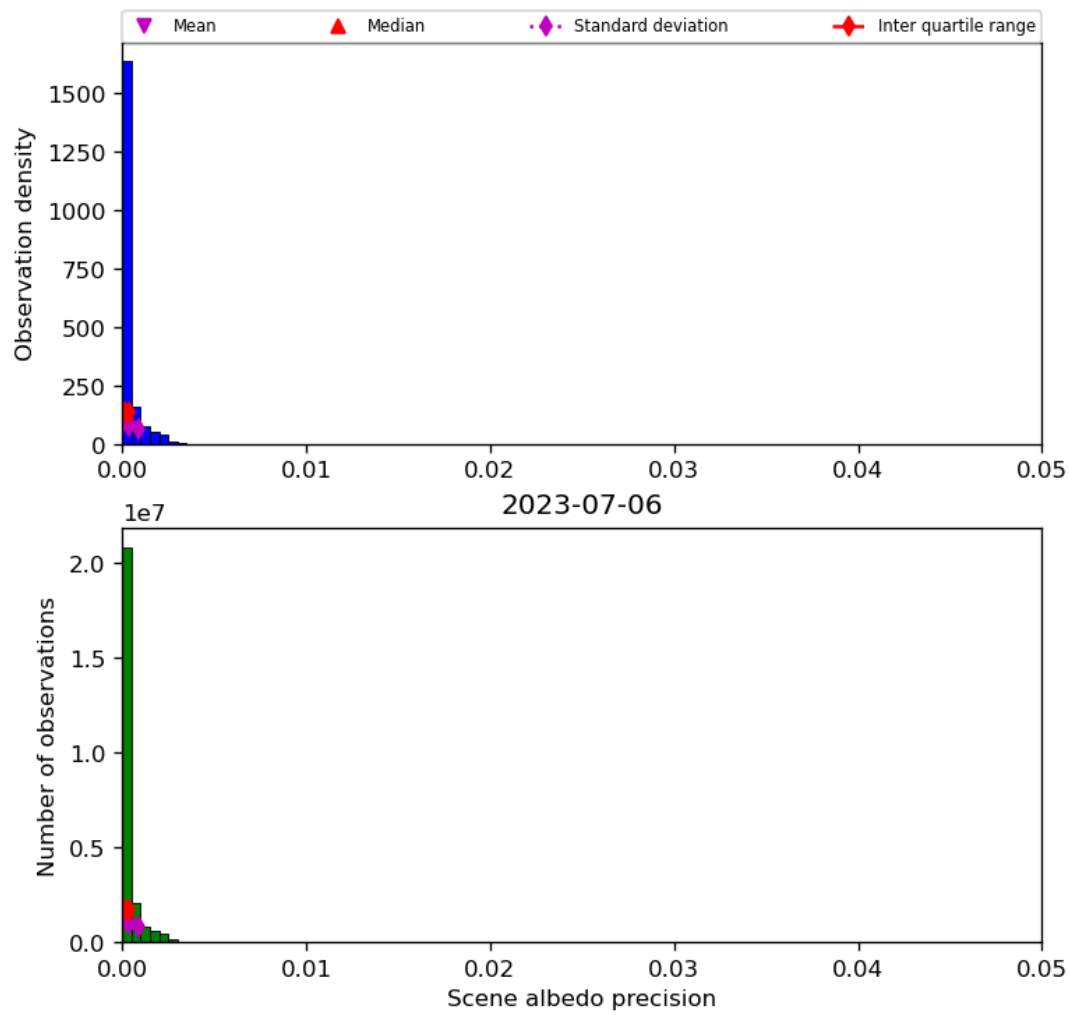
Figure 35: Histogram of “Scene albedo precision” for 2023-07-05 to 2023-07-07
