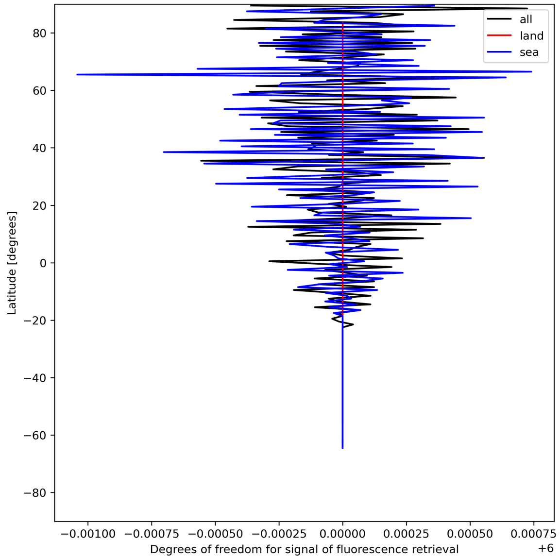
Figure 26: Zonal average of “Degrees of freedom for signal of fluorescence retrieval” for 2023-07-05 to 2023-07-07.
