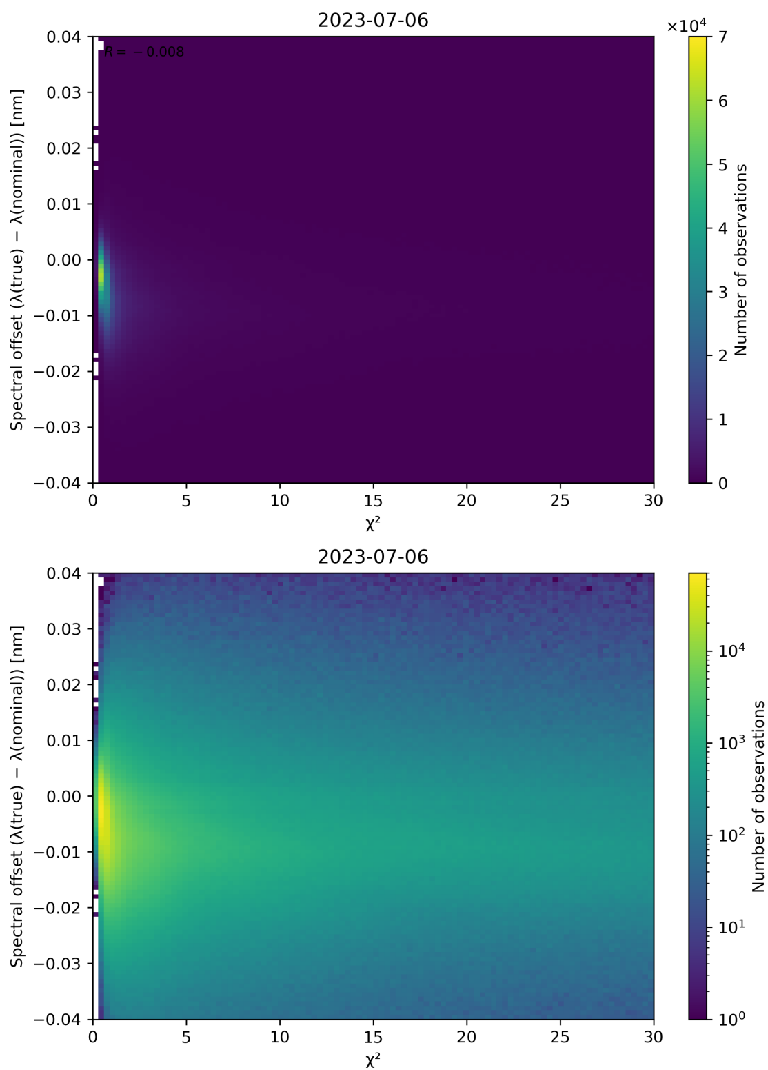
Figure 75: Scatter density plot of “ \chi^2 ” against “Spectral offset ( \lambda(\text{true}) - \lambda(\text{nominal}) )” for 2023-07-05 to 2023-07-07.
