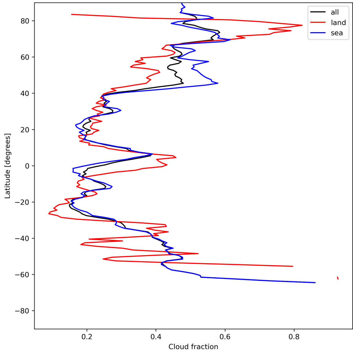
Figure 15: Zonal average of “Cloud fraction” for 2023-07-05 to 2023-07-07.
