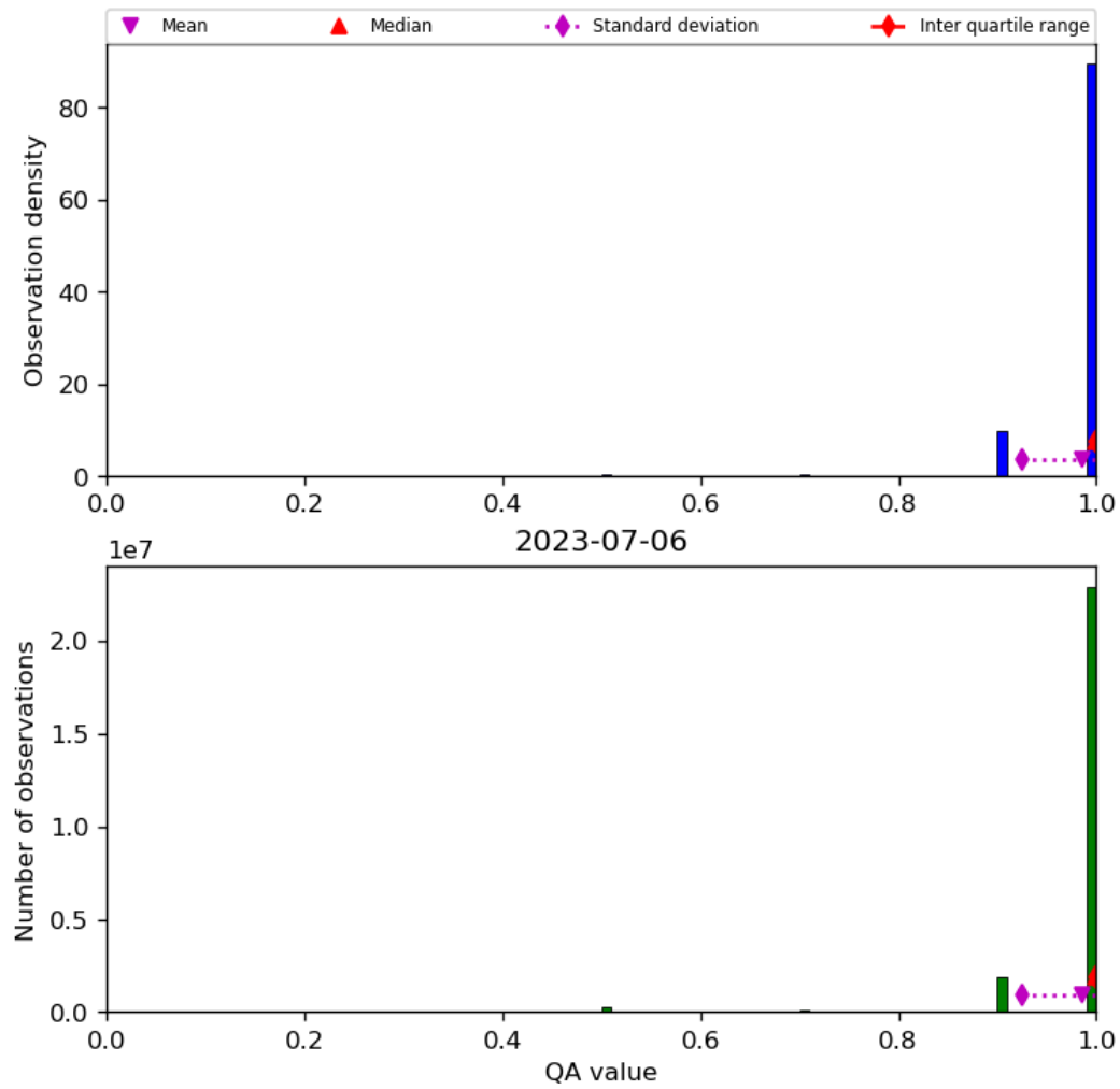
Figure 29: Histogram of “QA value” for 2023-07-05 to 2023-07-07
