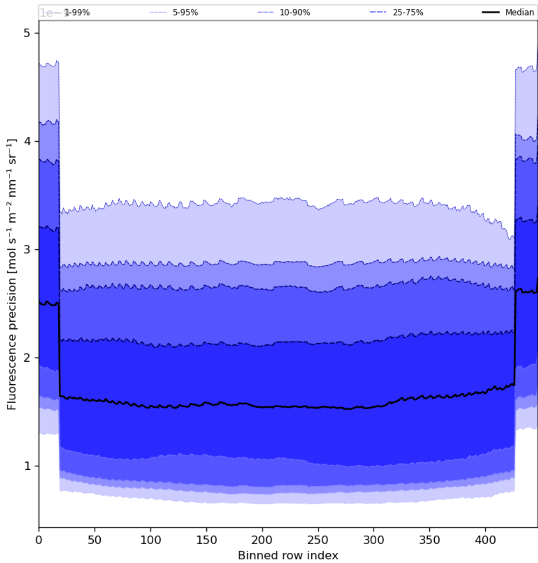
Figure 58: Along track statistics of “Fluorescence precision” for 2023-07-05 to 2023-07-07
