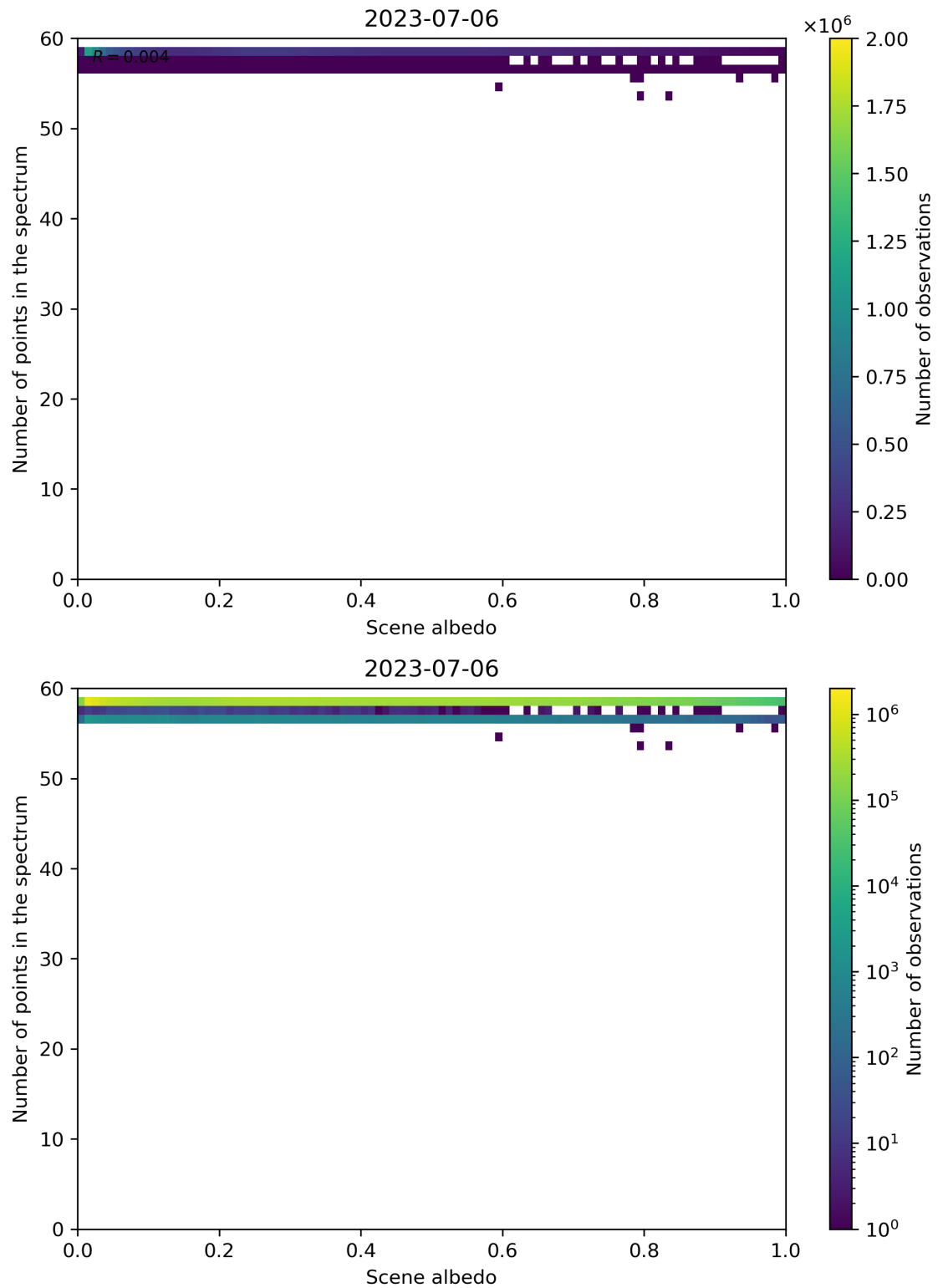
Figure 116: Scatter density plot of “Scene albedo” against “Number of points in the spectrum” for 2023-07-05 to 2023-07-07.
