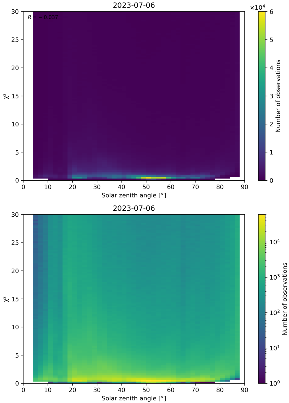
Figure 119: Scatter density plot of “Solar zenith angle” against “ \chi^2 ” for 2023-07-05 to 2023-07-07.
