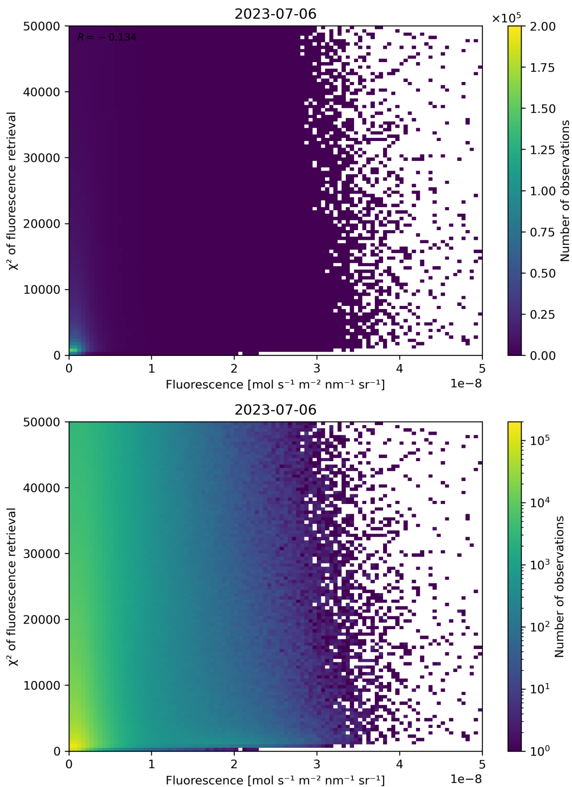
Figure 93: Scatter density plot of “Fluorescence” against “ \chi^2 of fluorescence retrieval” for 2023-07-05 to 2023-07-07.
