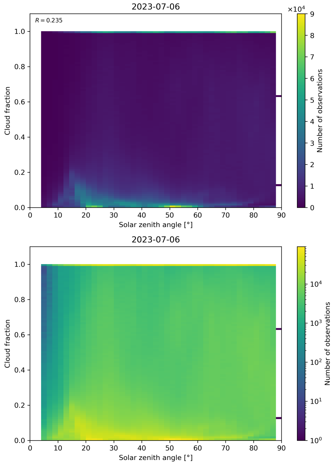
Figure 121: Scatter density plot of “Solar zenith angle” against “Cloud fraction” for 2023-07-05 to 2023-07-07.
