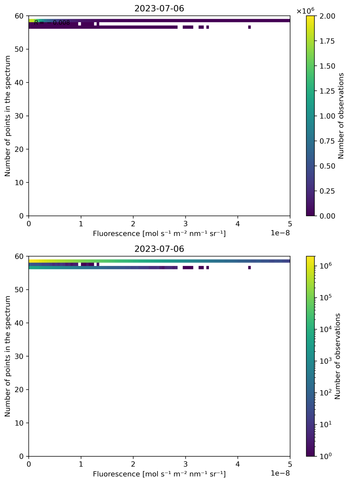
Figure 94: Scatter density plot of “Fluorescence” against “Number of points in the spectrum” for 2023-07-05 to 2023-07-07.
