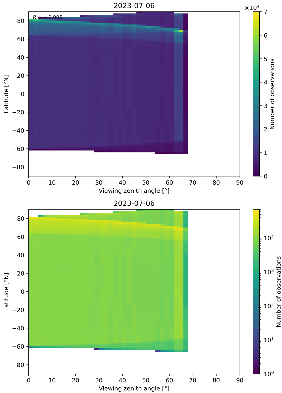
Figure 135: Scatter density plot of “Viewing zenith angle” against “Latitude” for 2023-07-05 to 2023-07-07.
