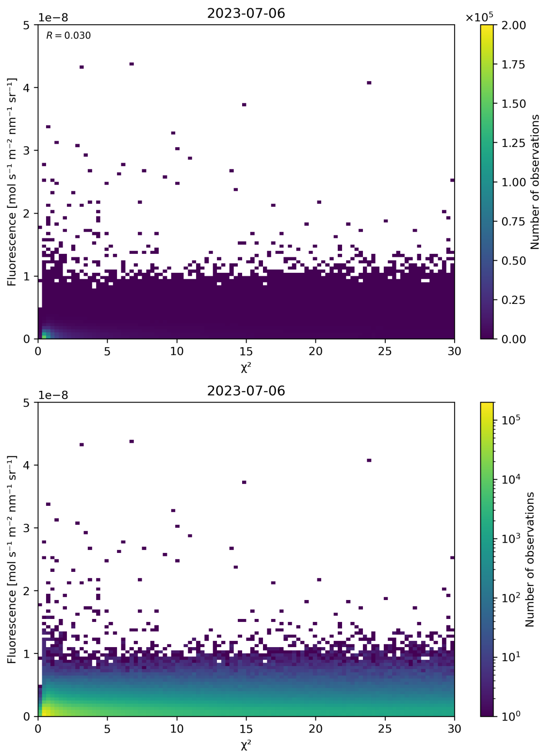
Figure 70: Scatter density plot of “ \chi^2 ” against “Fluorescence” for 2023-07-05 to 2023-07-07.
