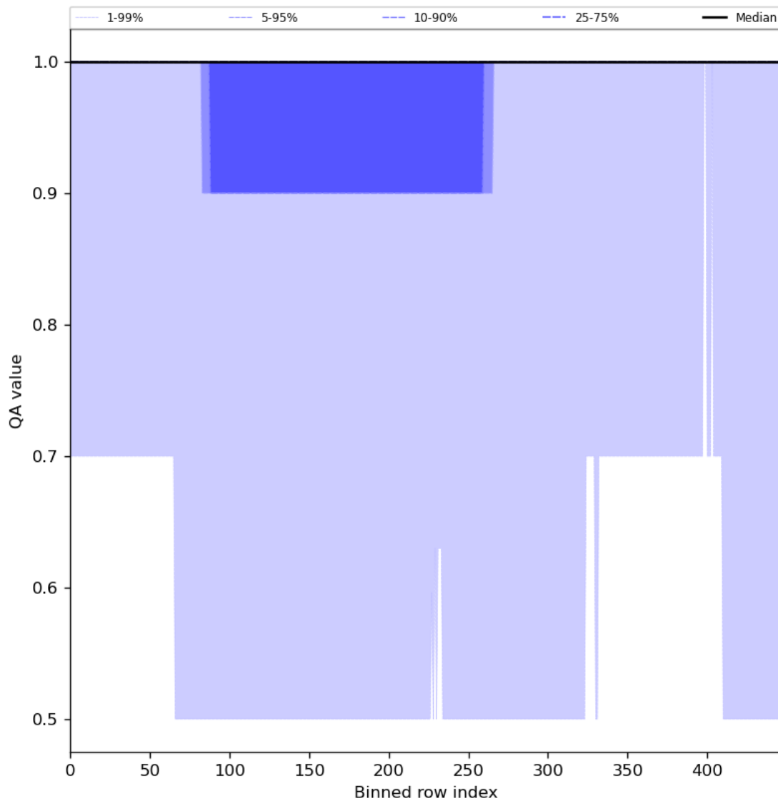
Figure 46: Along track statistics of "QA value" for 2023-07-05 to 2023-07-07
