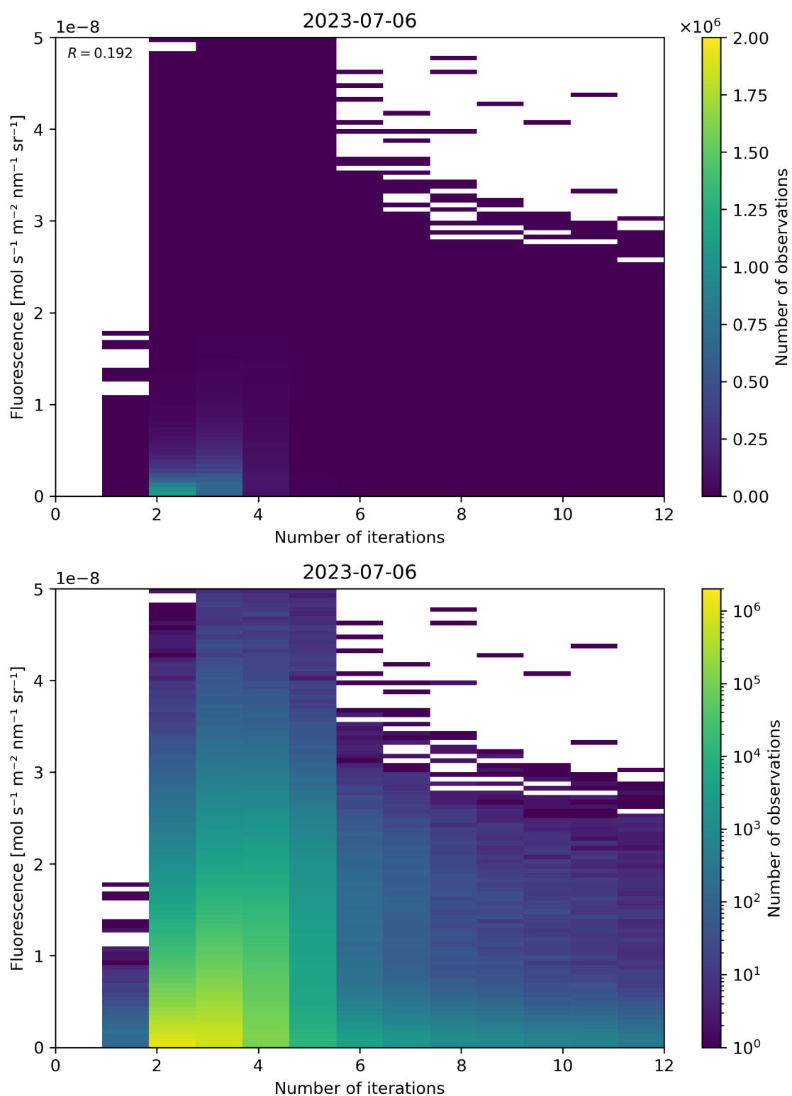
Figure 107: Scatter density plot of “Number of iterations” against “Fluorescence” for 2023-07-05 to 2023-07-07.
