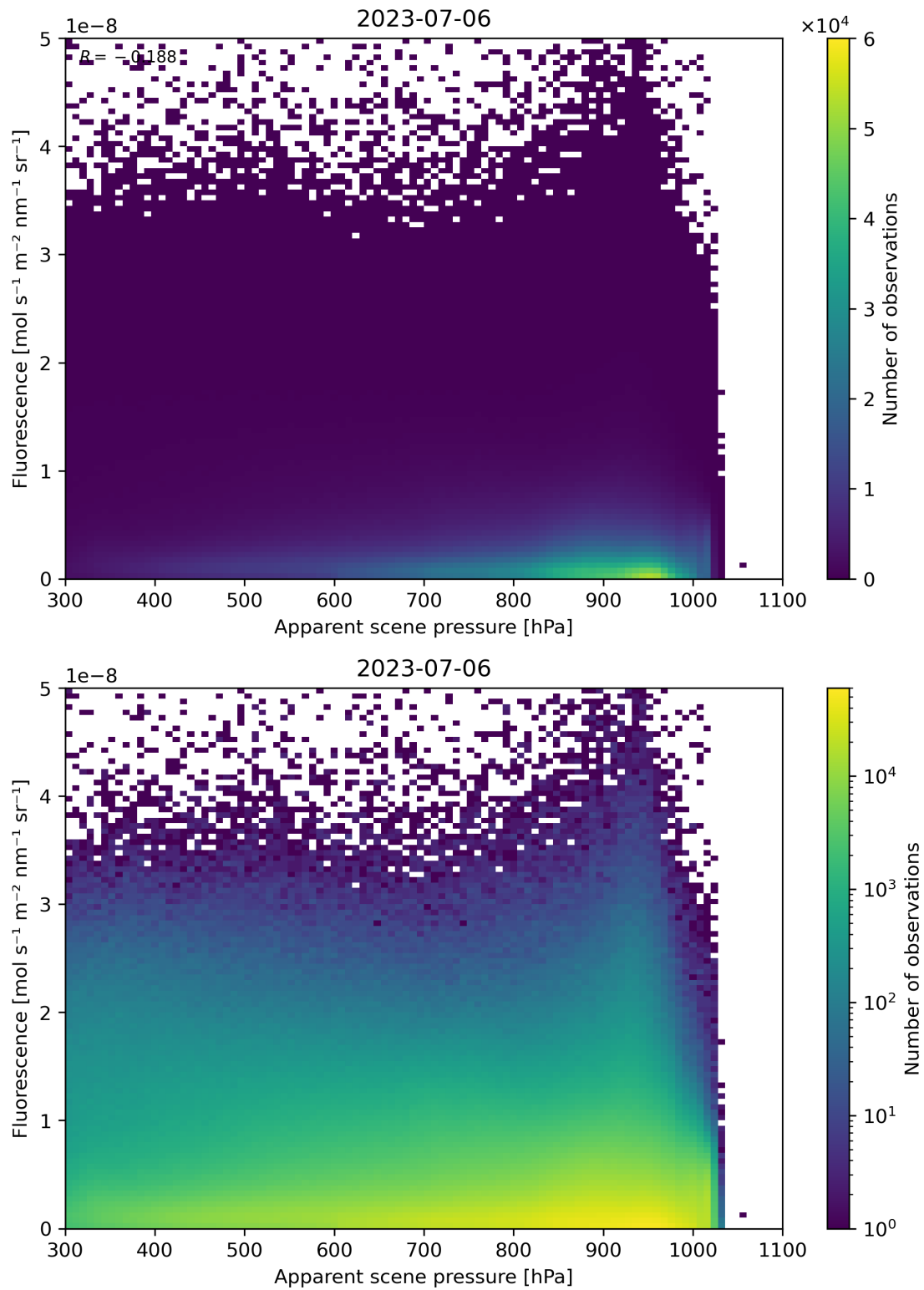
Figure 65: Scatter density plot of “Apparent scene pressure” against “Fluorescence” for 2023-07-05 to 2023-07-07.
