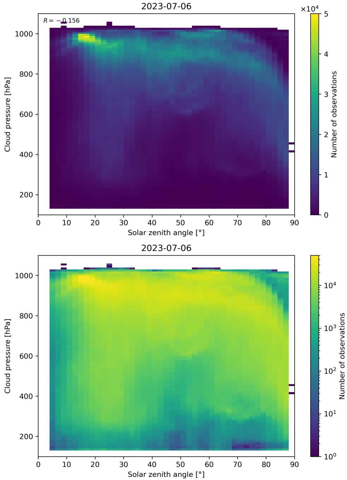
Figure 122: Scatter density plot of “Solar zenith angle” against “Cloud pressure” for 2023-07-05 to 2023-07-07.
