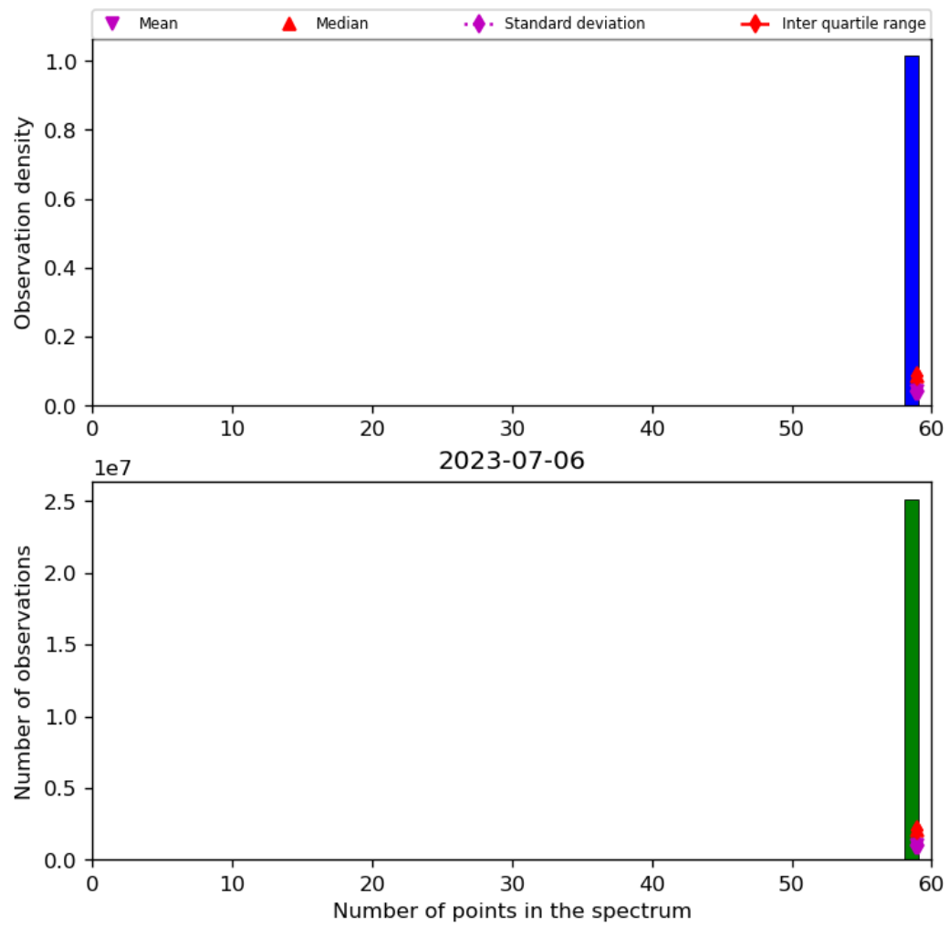
Figure 44: Histogram of “Number of points in the spectrum” for 2023-07-05 to 2023-07-07
