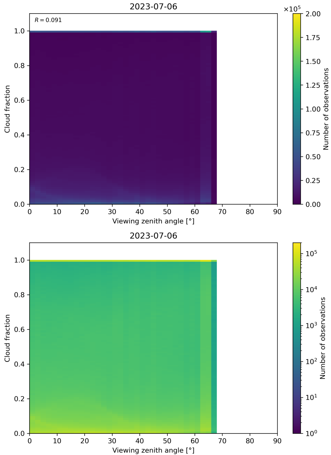
Figure 132: Scatter density plot of “Viewing zenith angle” against “Cloud fraction” for 2023-07-05 to 2023-07-07.
