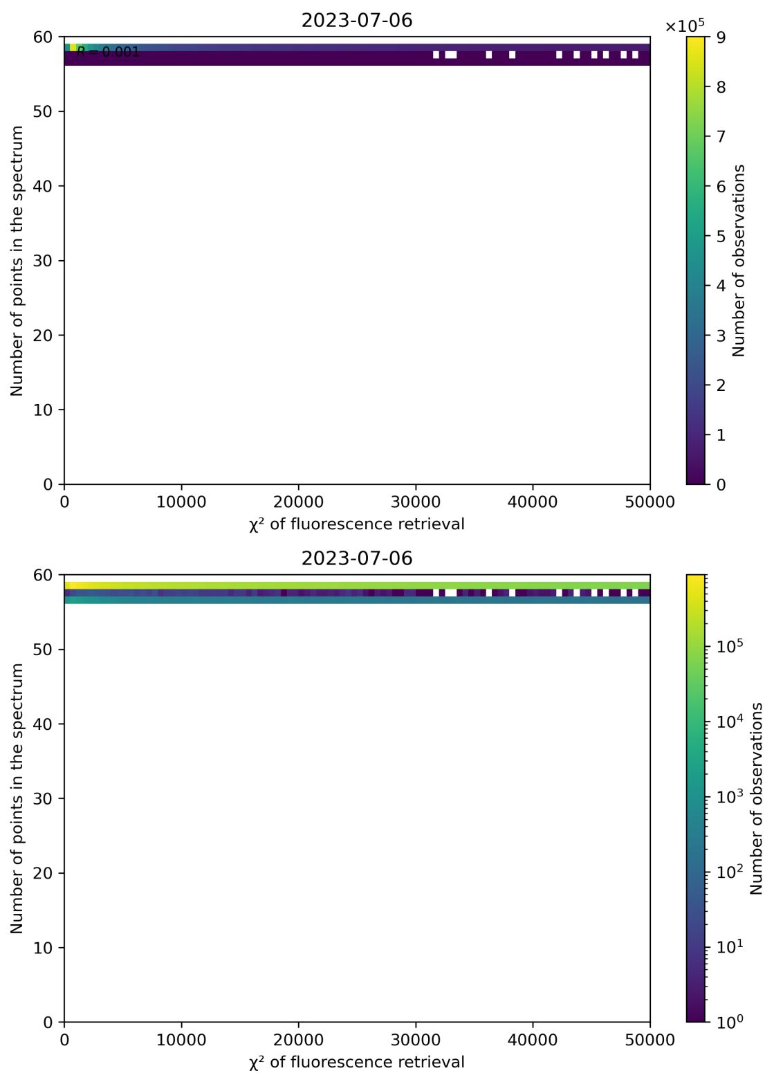
Figure 71: Scatter density plot of " \chi^2 of fluorescence retrieval" against "Number of points in the spectrum" for 2023-07-05 to 2023-07-07.
