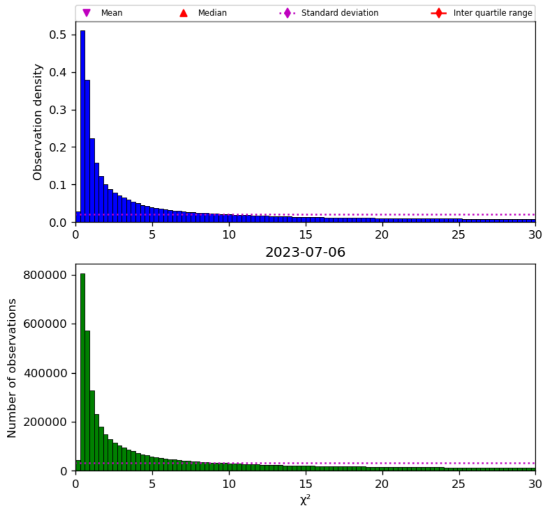
Figure 38: Histogram of " \chi^2 " for 2023-07-05 to 2023-07-07
