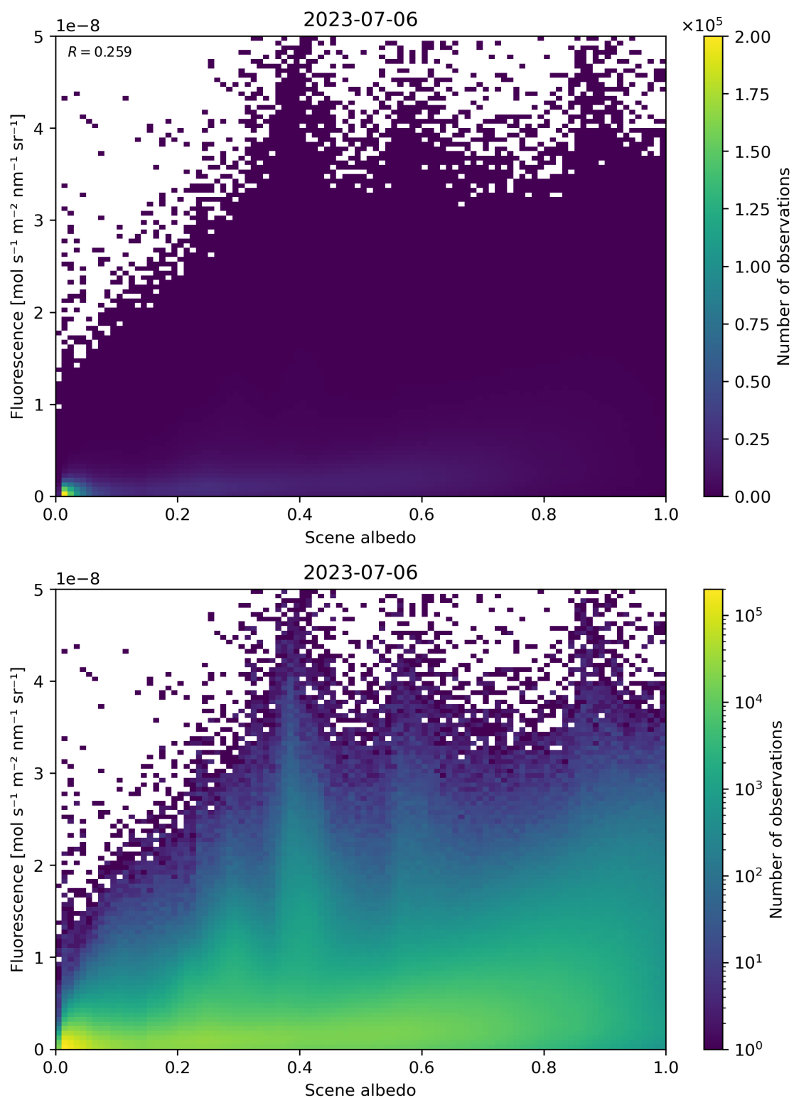
Figure 114: Scatter density plot of “Scene albedo” against “Fluorescence” for 2023-07-05 to 2023-07-07.
