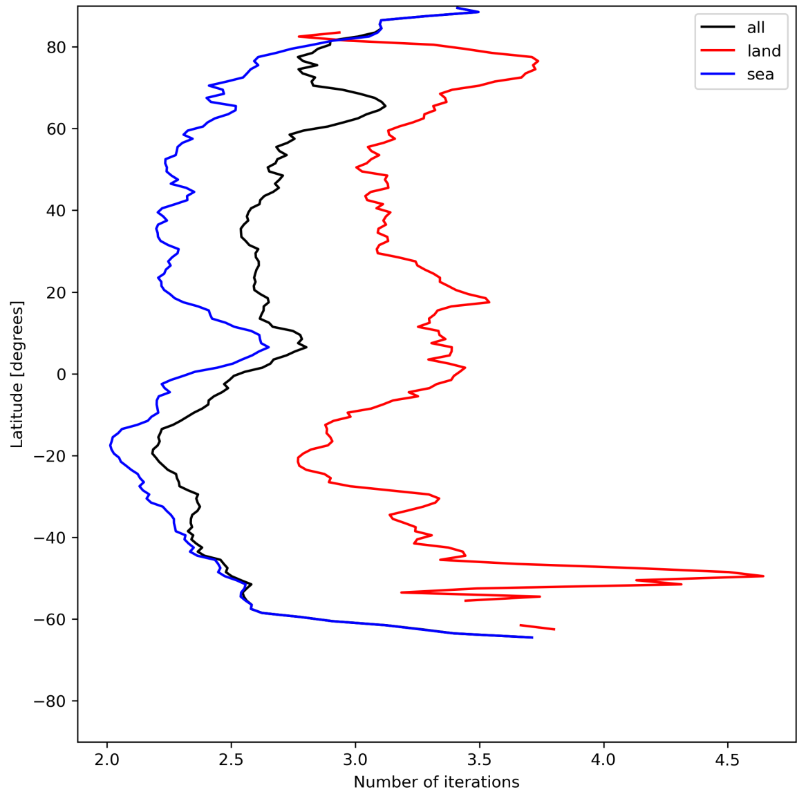
Figure 22: Zonal average of “Number of iterations” for 2023-07-05 to 2023-07-07.
