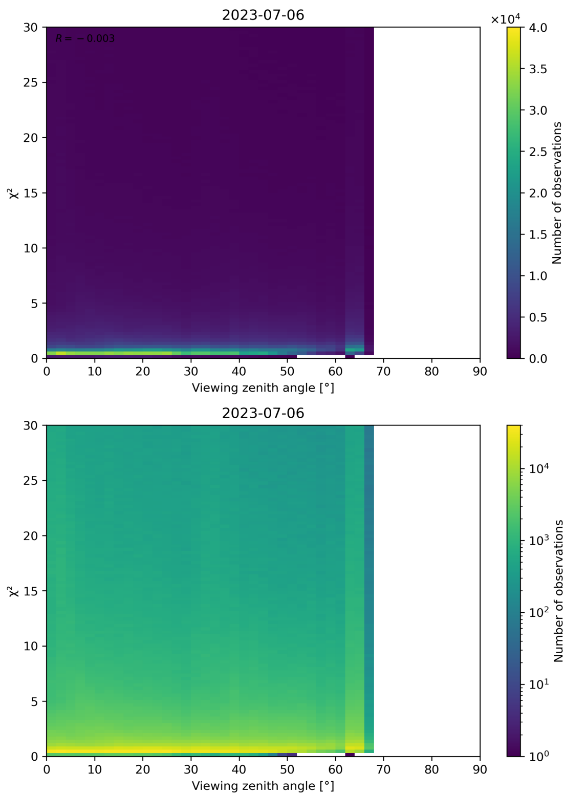
Figure 130: Scatter density plot of “Viewing zenith angle” against “ \chi^2 ” for 2023-07-05 to 2023-07-07.
