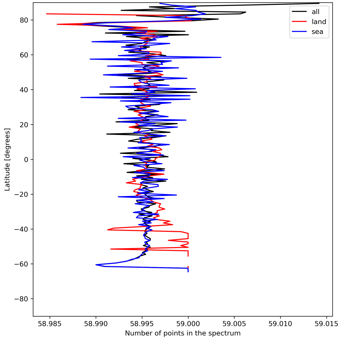
Figure 27: Zonal average of “Number of points in the spectrum” for 2023-07-05 to 2023-07-07.
