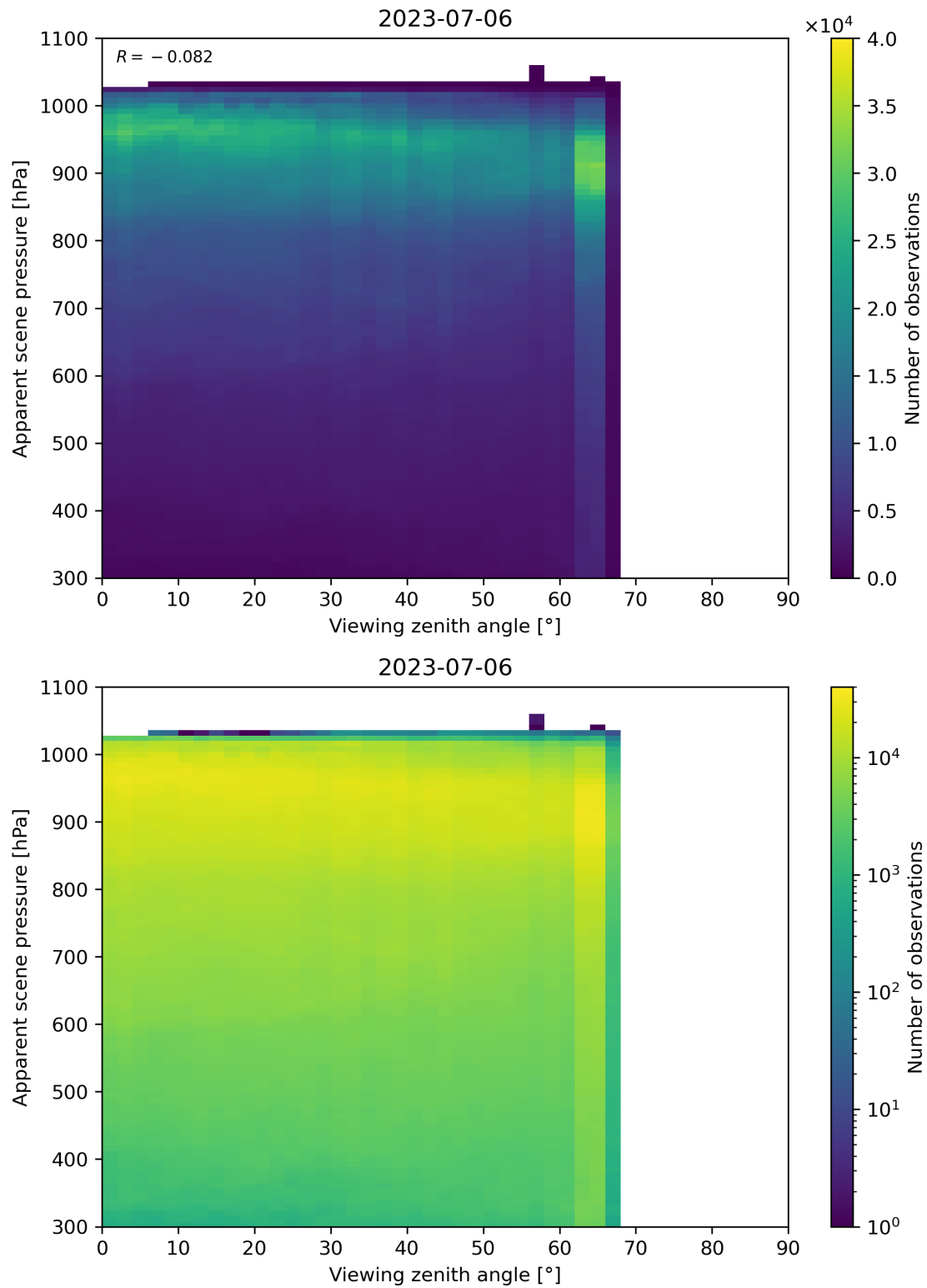
Figure 129: Scatter density plot of “Viewing zenith angle” against “Apparent scene pressure” for 2023-07-05 to 2023-07-07.
