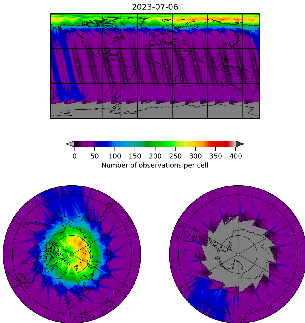
Figure 11: Map of the number of observations for 2023-07-05 to 2023-07-07
