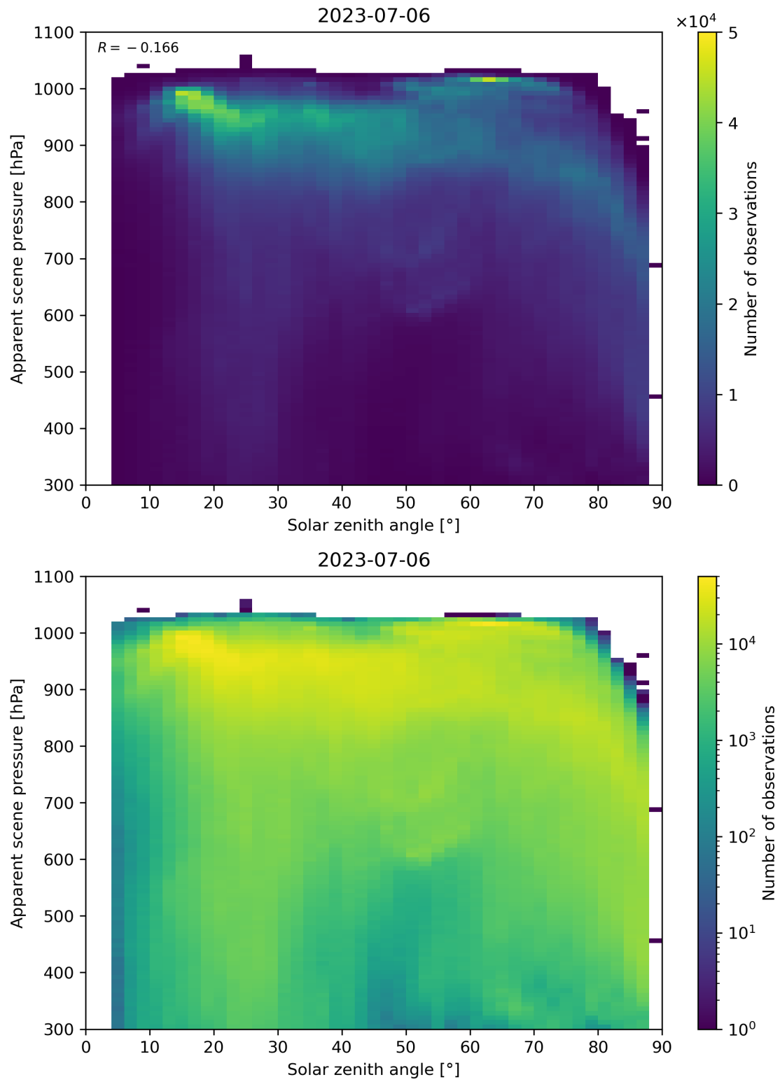
Figure 118: Scatter density plot of “Solar zenith angle” against “Apparent scene pressure” for 2023-07-05 to 2023-07-07.
