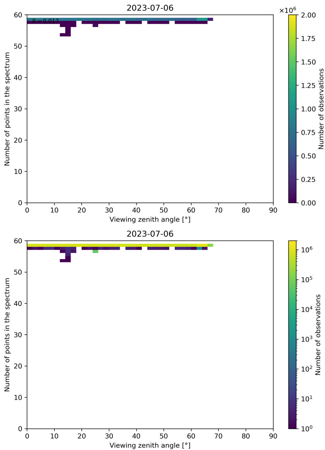
Figure 137: Scatter density plot of “Viewing zenith angle” against “Number of points in the spectrum” for 2023-07-05 to 2023-07-07.
