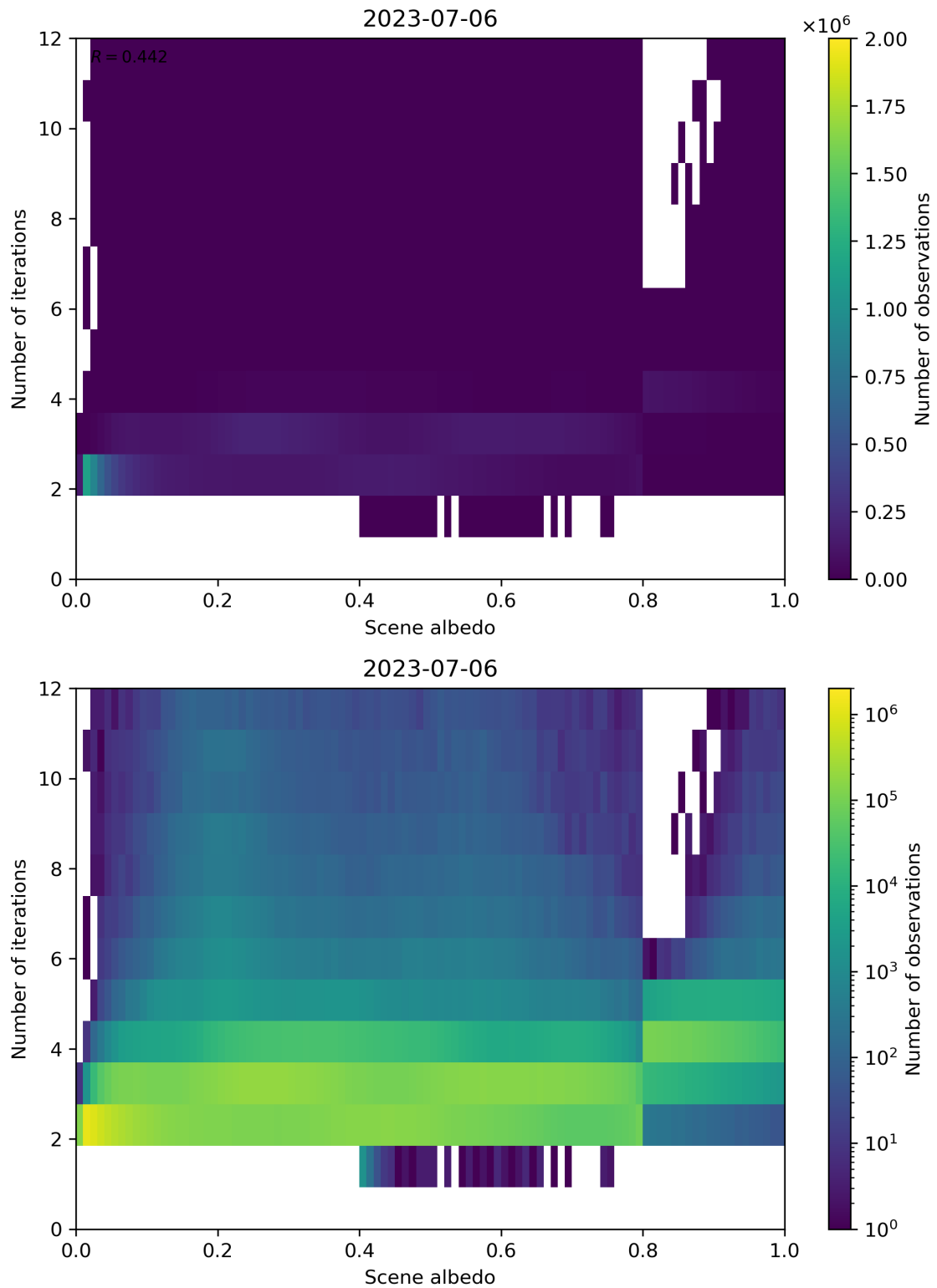
Figure 115: Scatter density plot of “Scene albedo” against “Number of iterations” for 2023-07-05 to 2023-07-07.
