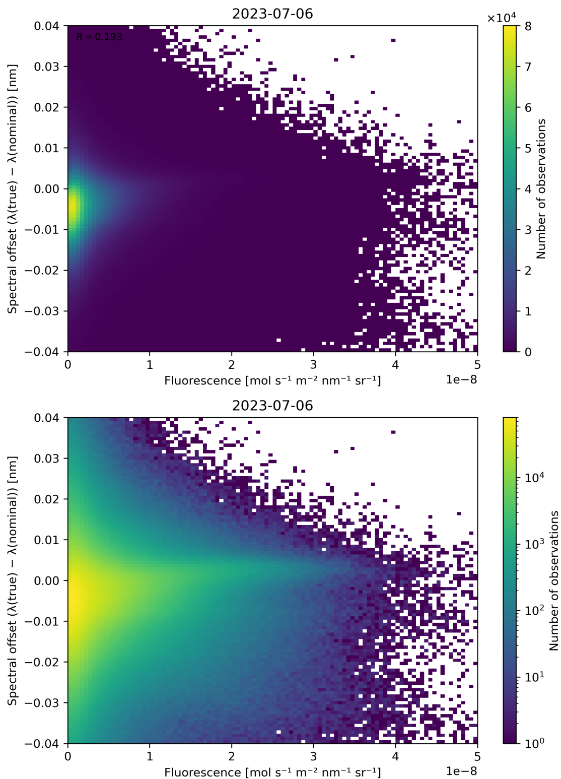
Figure 95: Scatter density plot of “Fluorescence” against “Spectral offset ( \lambda(\text{true}) - \lambda(\text{nominal}) )” for 2023-07-05 to 2023-07-07.
