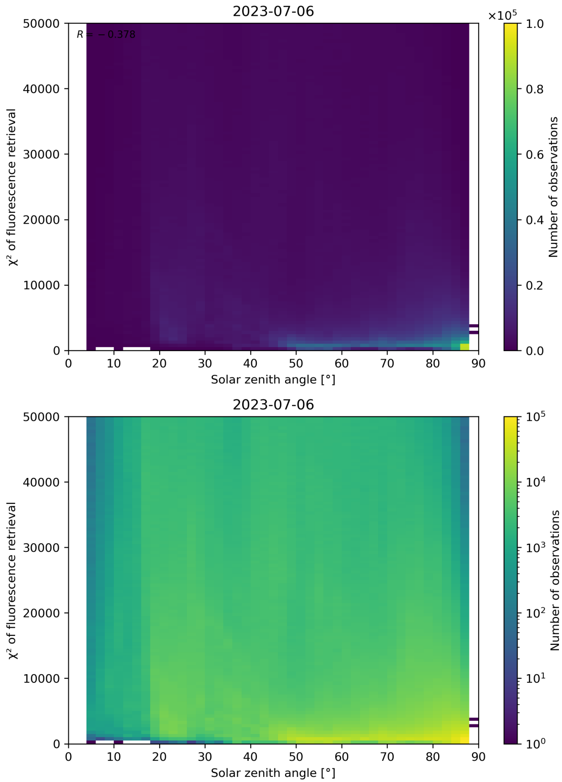
Figure 120: Scatter density plot of “Solar zenith angle” against “ \chi^2 of fluorescence retrieval” for 2023-07-05 to 2023-07-07.
