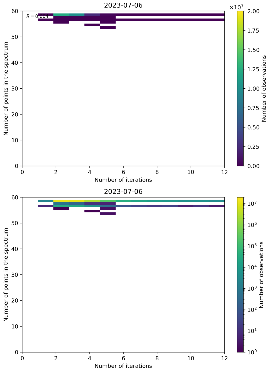
Figure 108: Scatter density plot of “Number of iterations” against “Number of points in the spectrum” for 2023-07-05 to 2023-07-07.
