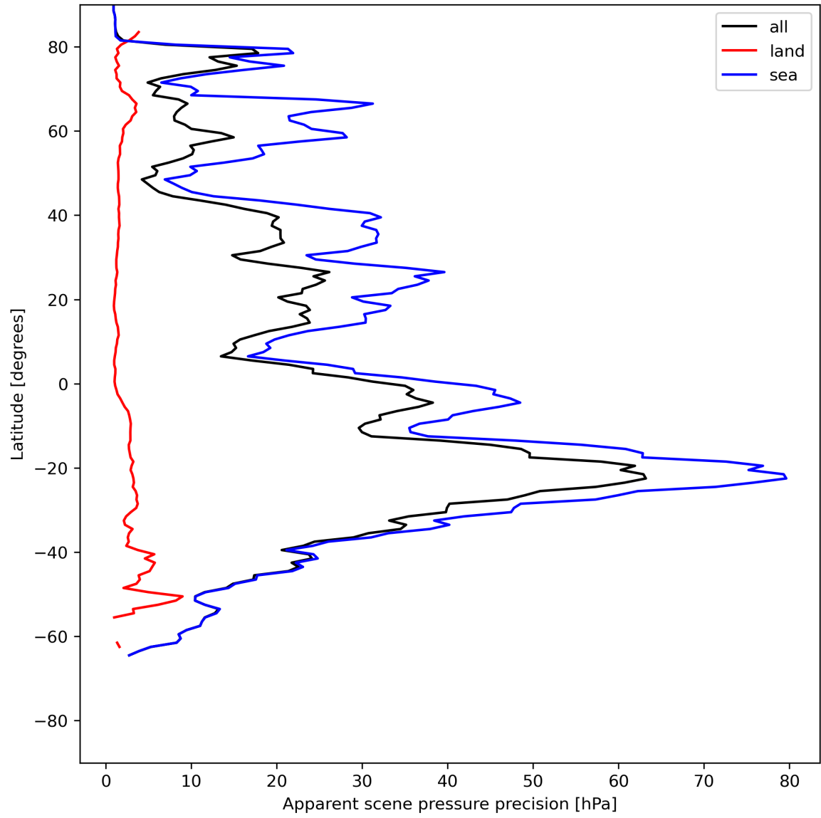
Figure 20: Zonal average of “Apparent scene pressure precision” for 2023-07-05 to 2023-07-07.
