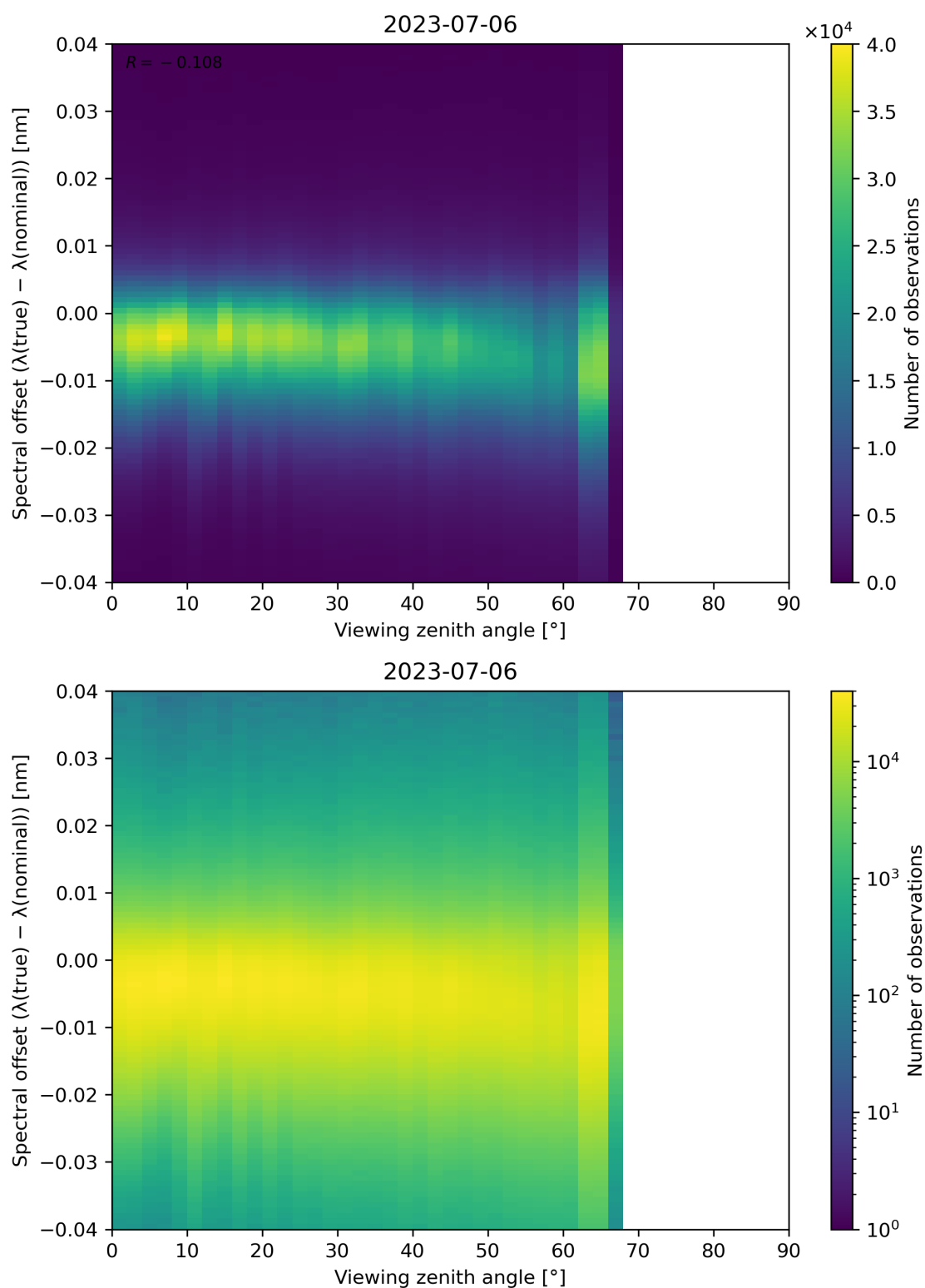
Figure 140: Scatter density plot of “Viewing zenith angle” against “Spectral offset ( \lambda(\text{true}) - \lambda(\text{nominal}) )” for 2023-07-05 to 2023-07-07.
