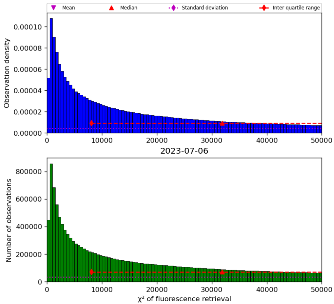
Figure 42: Histogram of “ \chi^2 of fluorescence retrieval” for 2023-07-05 to 2023-07-07
