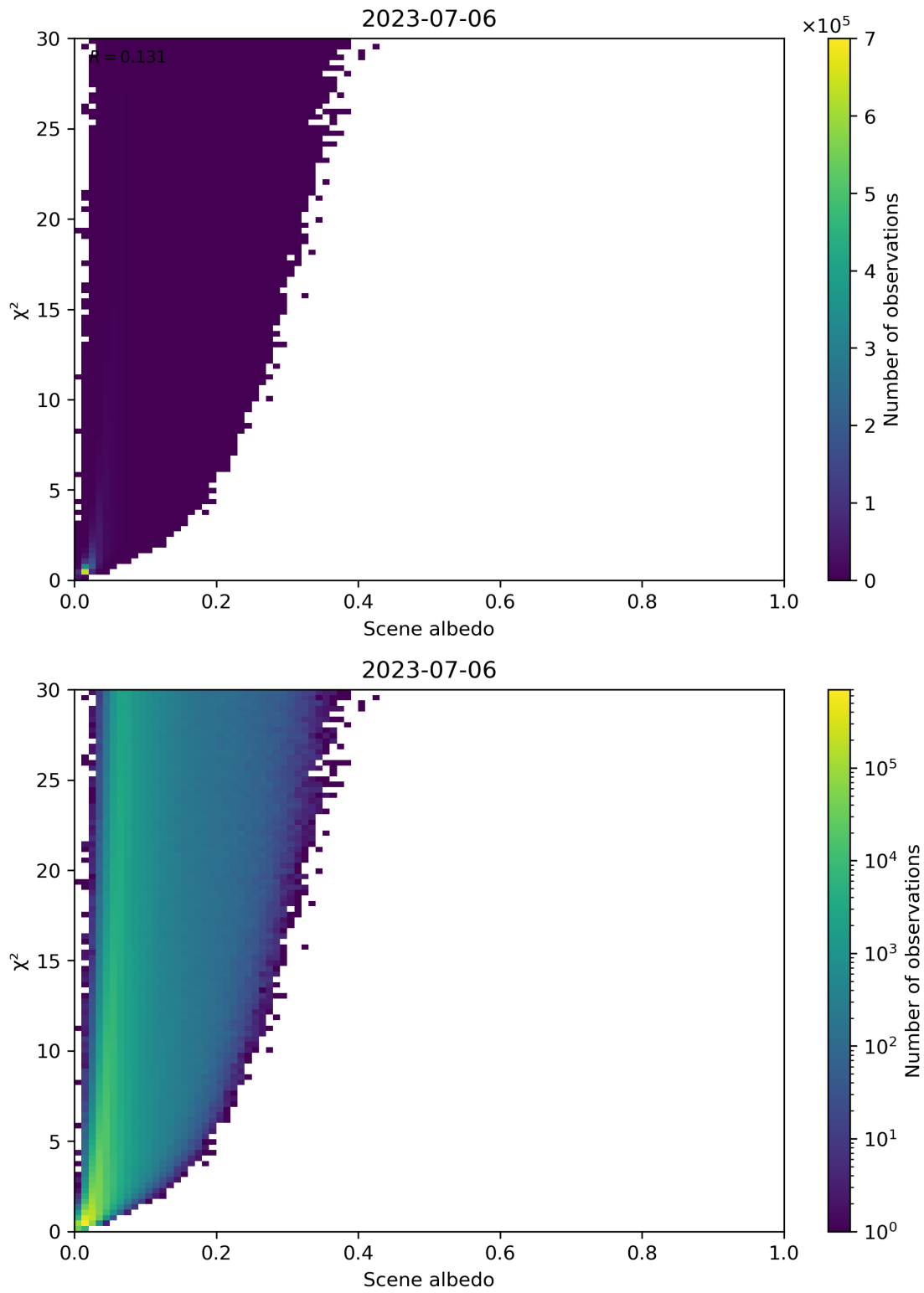
Figure 112: Scatter density plot of “Scene albedo” against “ \chi^2 ” for 2023-07-05 to 2023-07-07.
