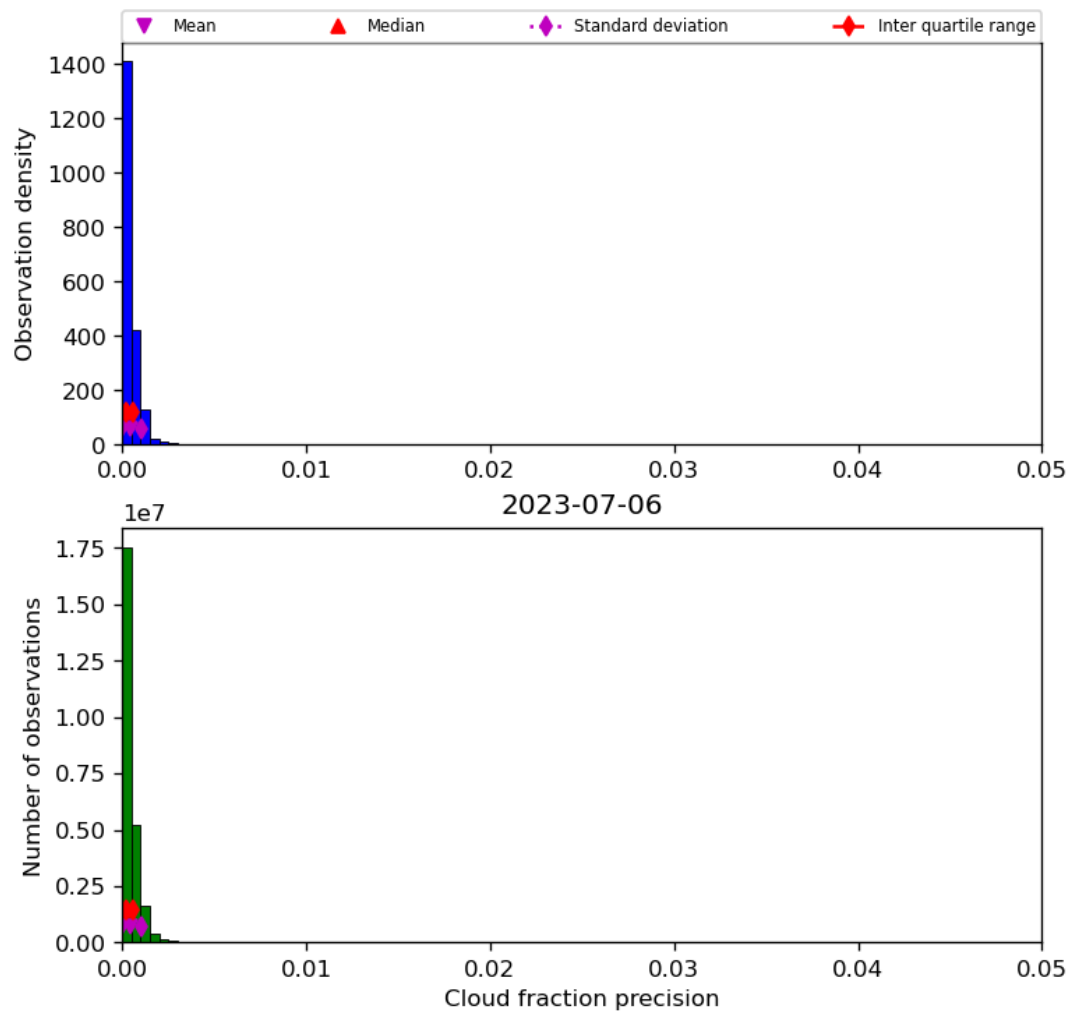
Figure 33: Histogram of “Cloud fraction precision” for 2023-07-05 to 2023-07-07
