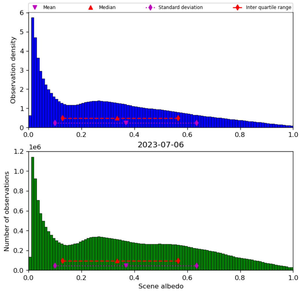
Figure 34: Histogram of “Scene albedo” for 2023-07-05 to 2023-07-07
