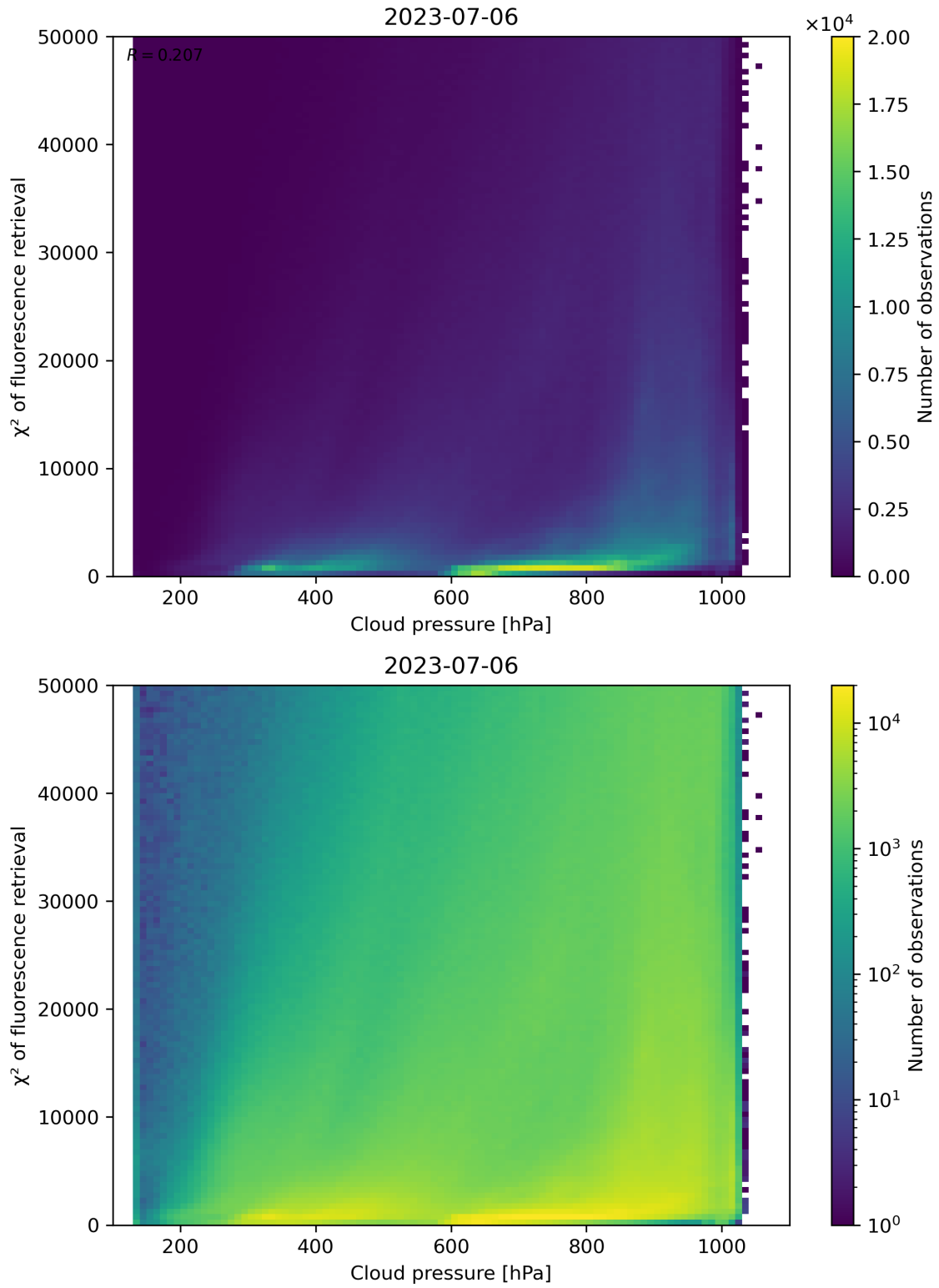
Figure 86: Scatter density plot of “Cloud pressure” against “ \chi^2 of fluorescence retrieval” for 2023-07-05 to 2023-07-07.
