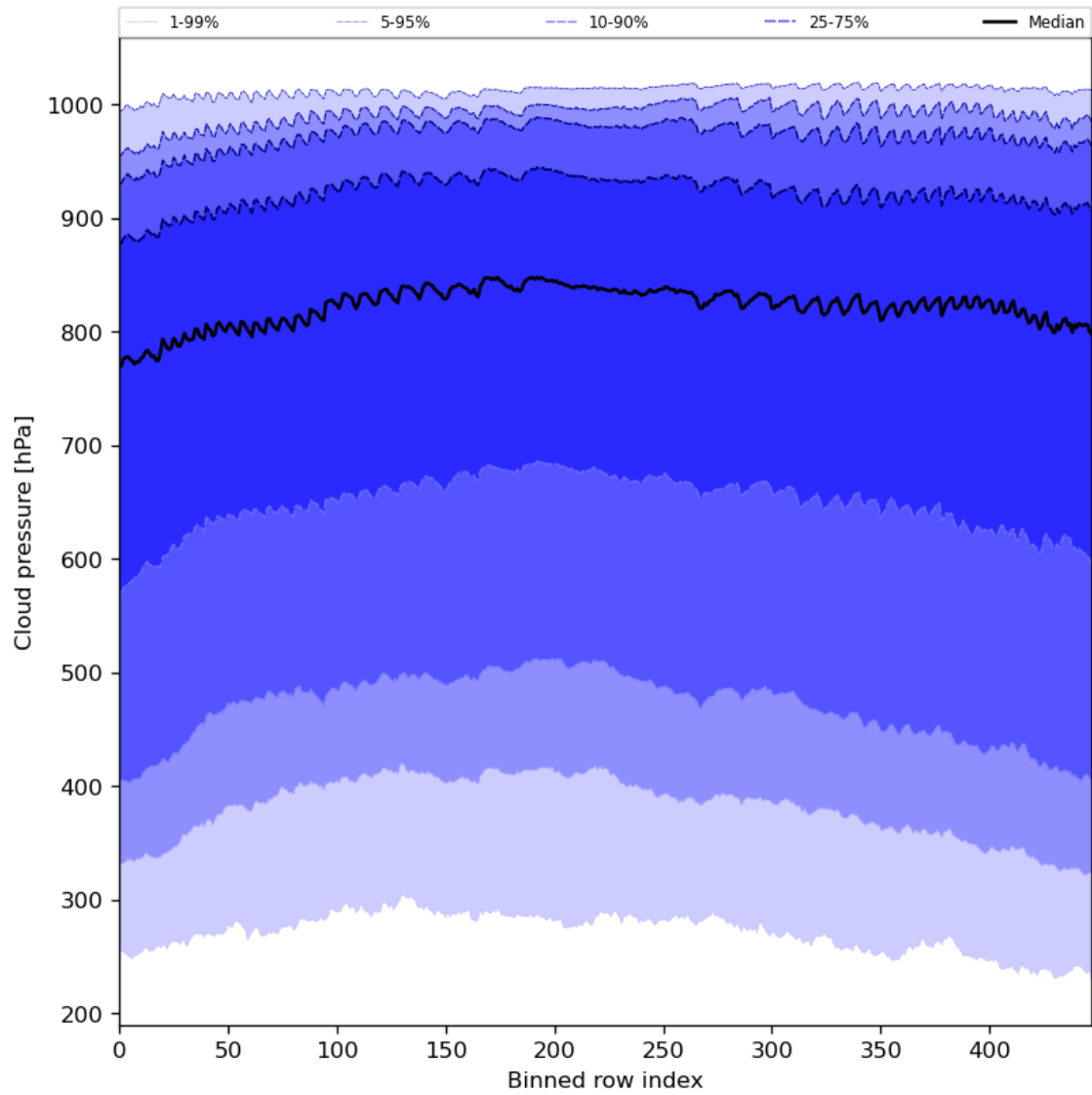
Figure 47: Along track statistics of “Cloud pressure” for 2023-07-05 to 2023-07-07
