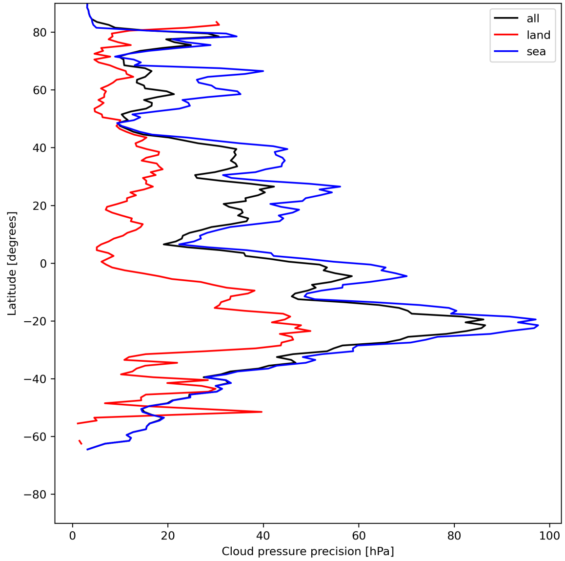
Figure 14: Zonal average of “Cloud pressure precision” for 2023-07-05 to 2023-07-07.
