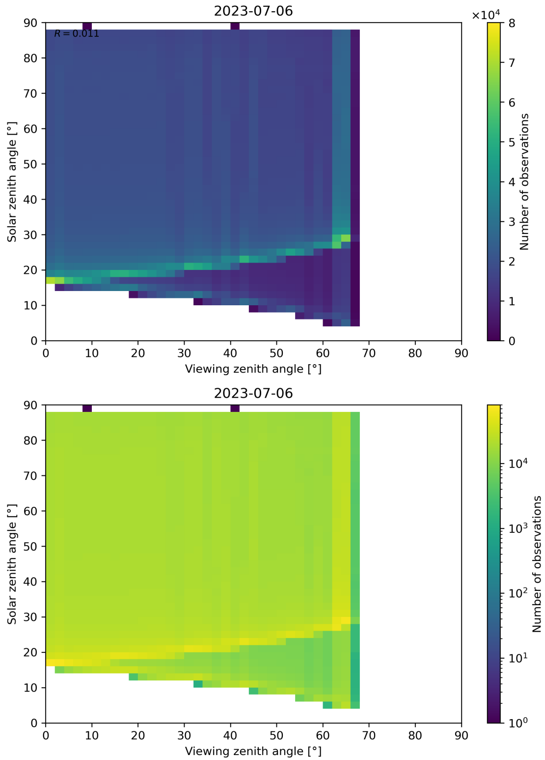
Figure 139: Scatter density plot of “Viewing zenith angle” against “Solar zenith angle” for 2023-07-05 to 2023-07-07.
