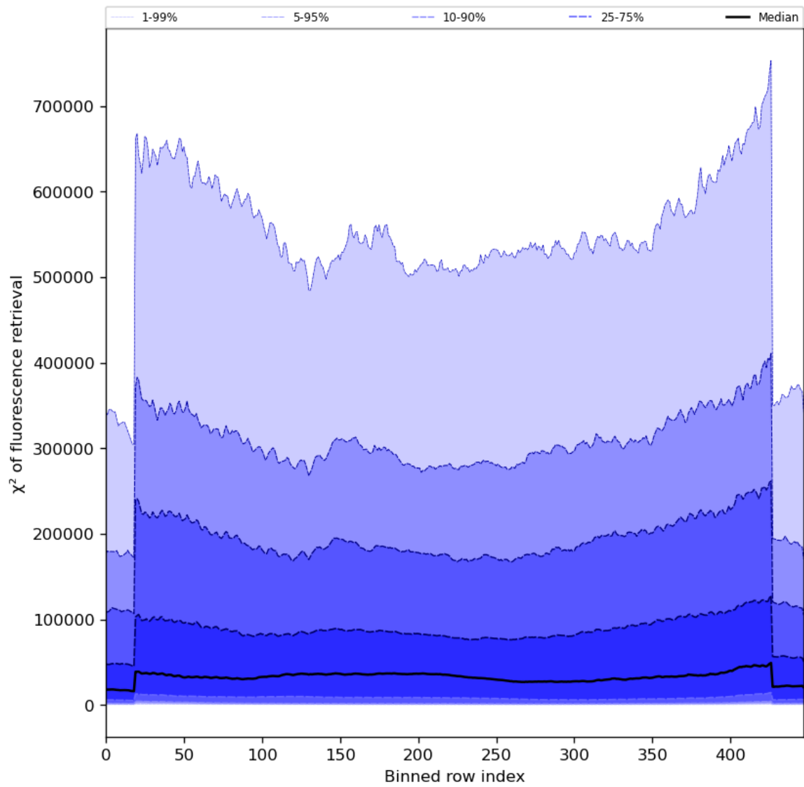
Figure 59: Along track statistics of “ \chi^2 of fluorescence retrieval” for 2023-07-05 to 2023-07-07
