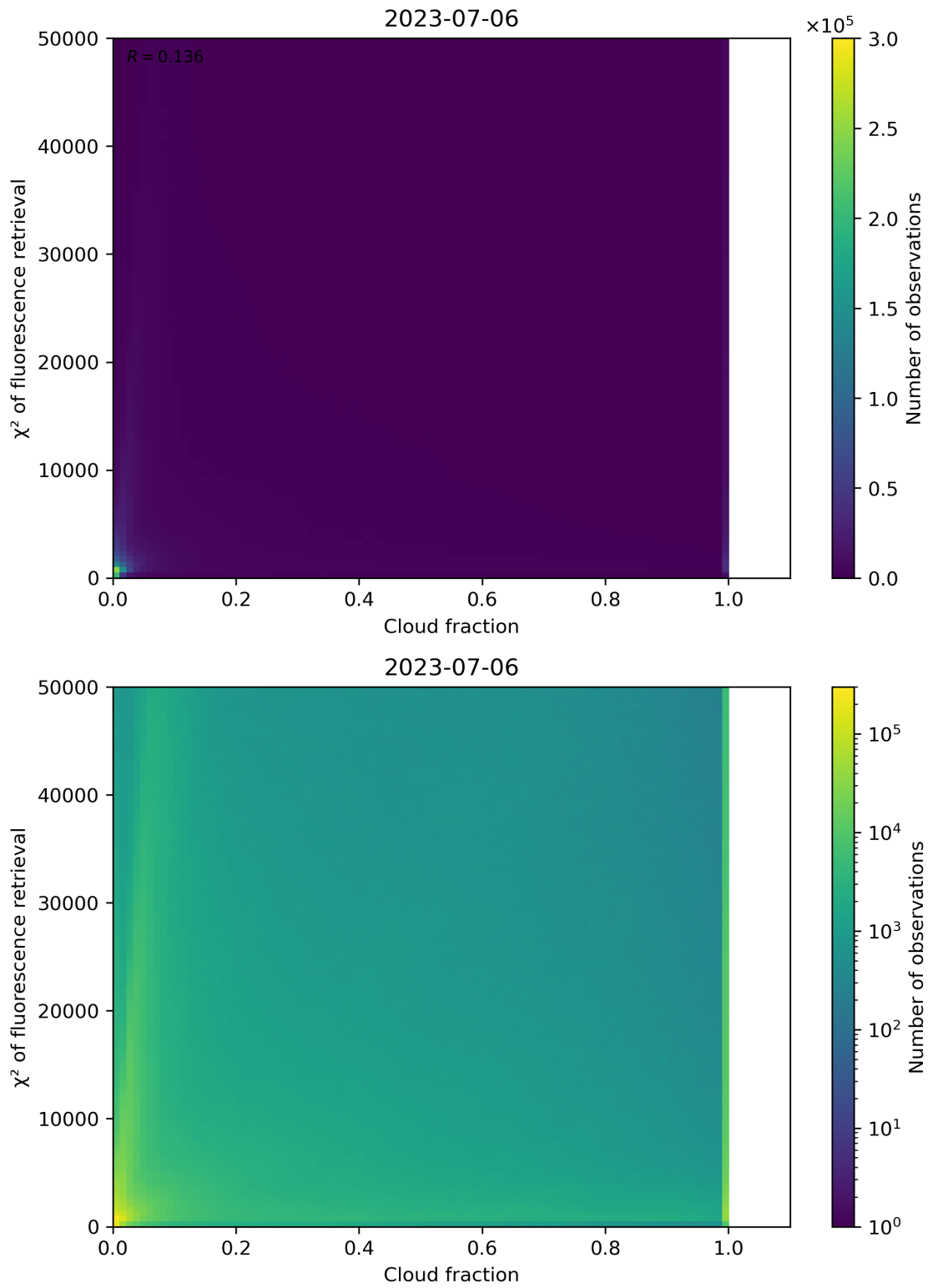
Figure 78: Scatter density plot of “Cloud fraction” against “ \chi^2 of fluorescence retrieval” for 2023-07-05 to 2023-07-07.
