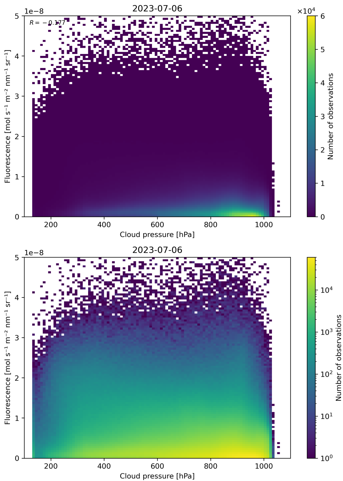
Figure 88: Scatter density plot of “Cloud pressure” against “Fluorescence” for 2023-07-05 to 2023-07-07.
