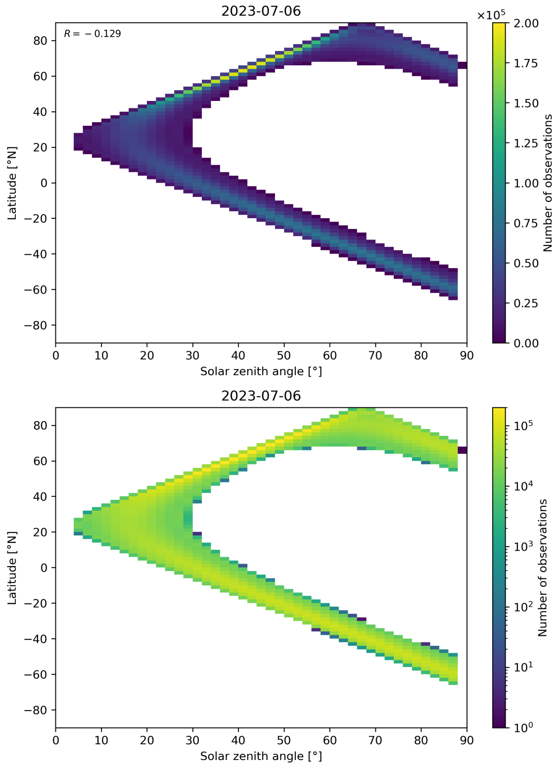
Figure 124: Scatter density plot of “Solar zenith angle” against “Latitude” for 2023-07-05 to 2023-07-07.
