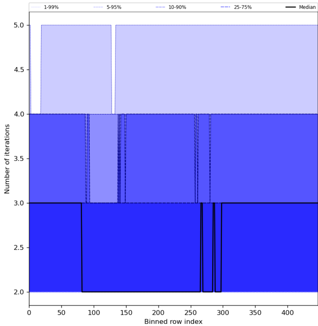
Figure 56: Along track statistics of “Number of iterations” for 2023-07-05 to 2023-07-07
