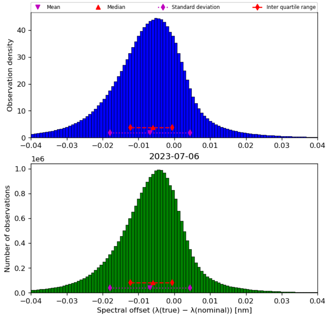
Figure 45: Histogram of “Spectral offset ( \lambda(\text{true}) - \lambda(\text{nominal}) )” for 2023-07-05 to 2023-07-07
