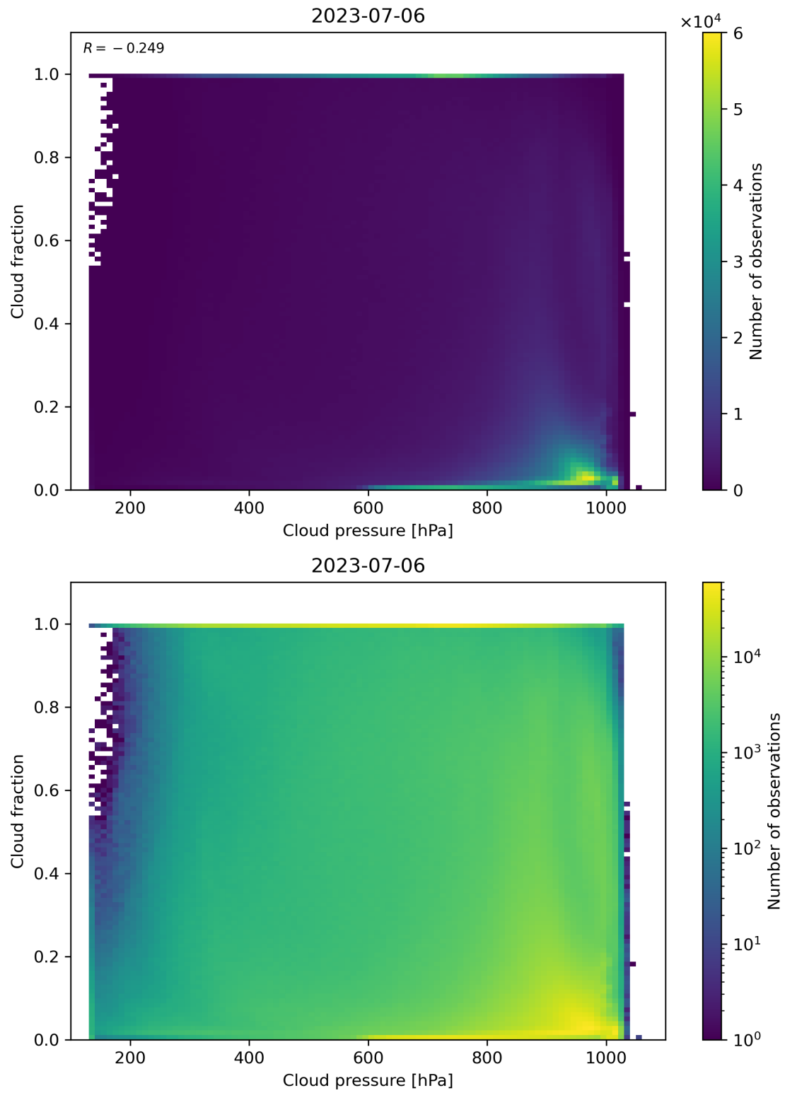
Figure 87: Scatter density plot of “Cloud pressure” against “Cloud fraction” for 2023-07-05 to 2023-07-07.
