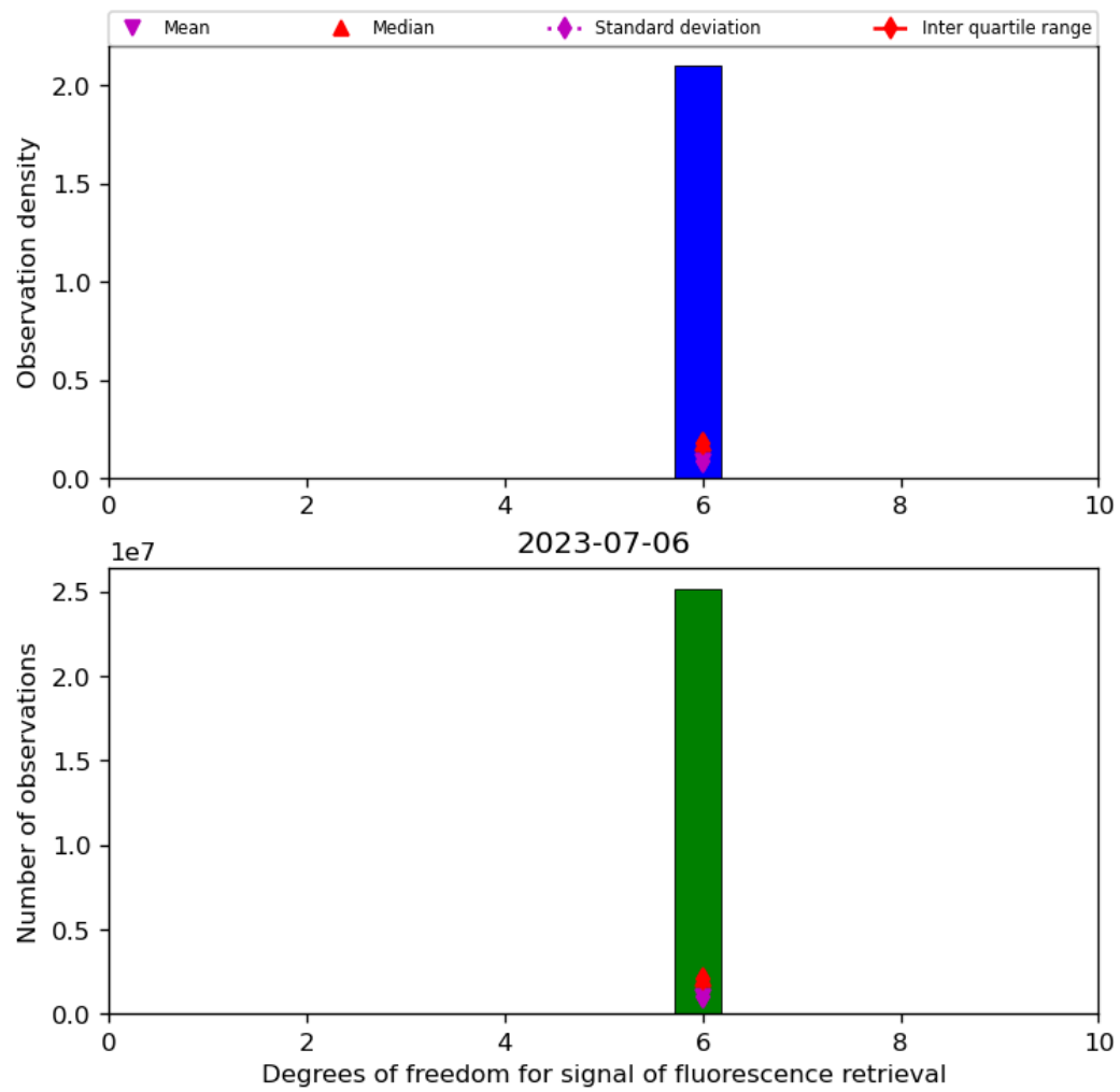
Figure 43: Histogram of “Degrees of freedom for signal of fluorescence retrieval” for 2023-07-05 to 2023-07-07
