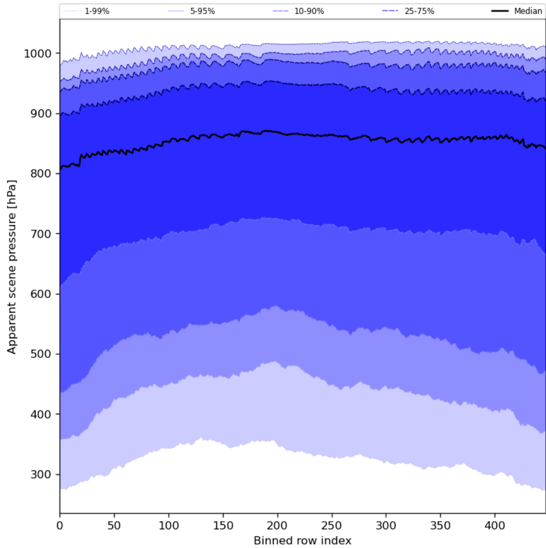
Figure 53: Along track statistics of “Apparent scene pressure” for 2023-07-05 to 2023-07-07
