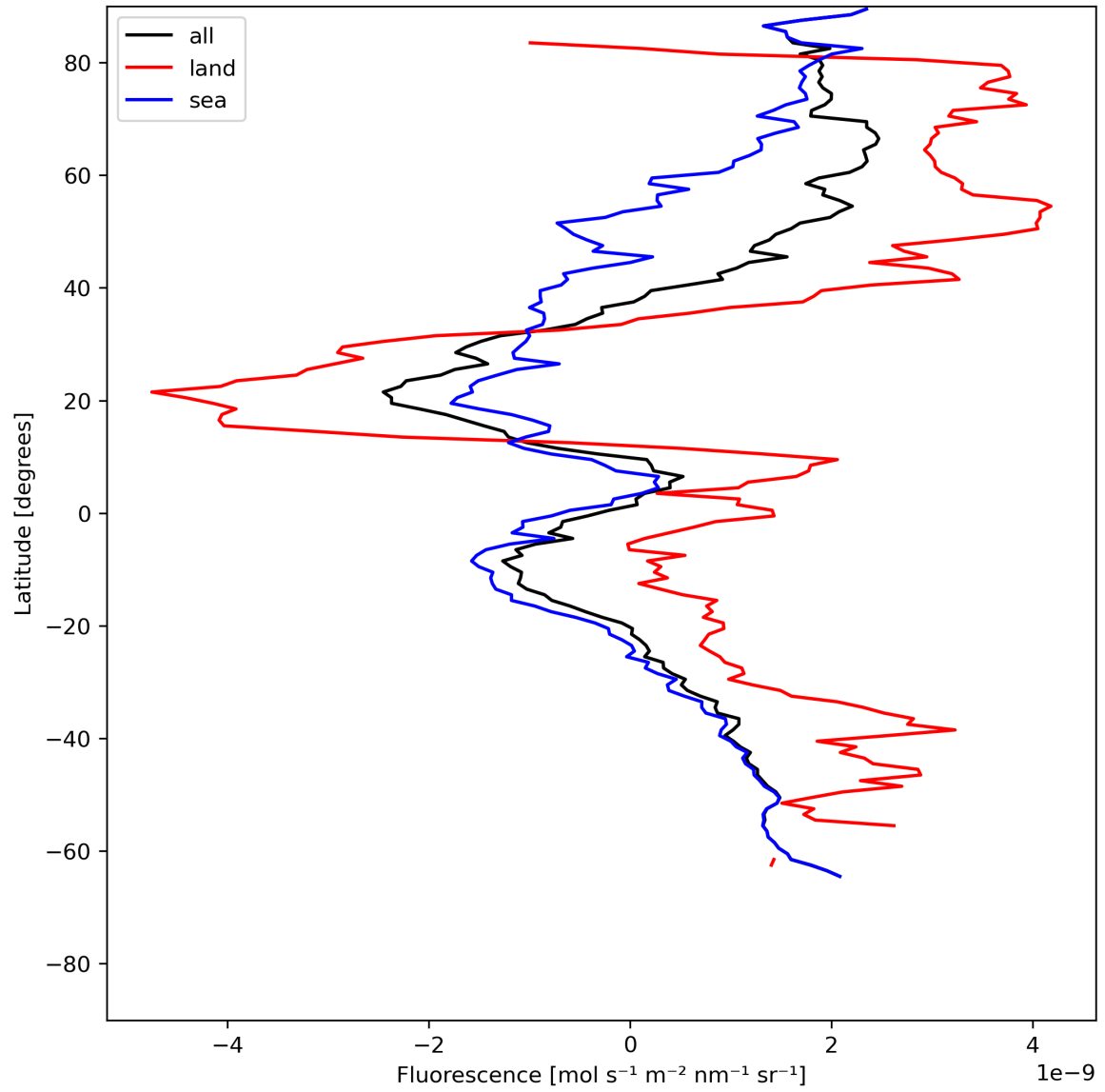
Figure 23: Zonal average of “Fluorescence” for 2023-07-05 to 2023-07-07.
