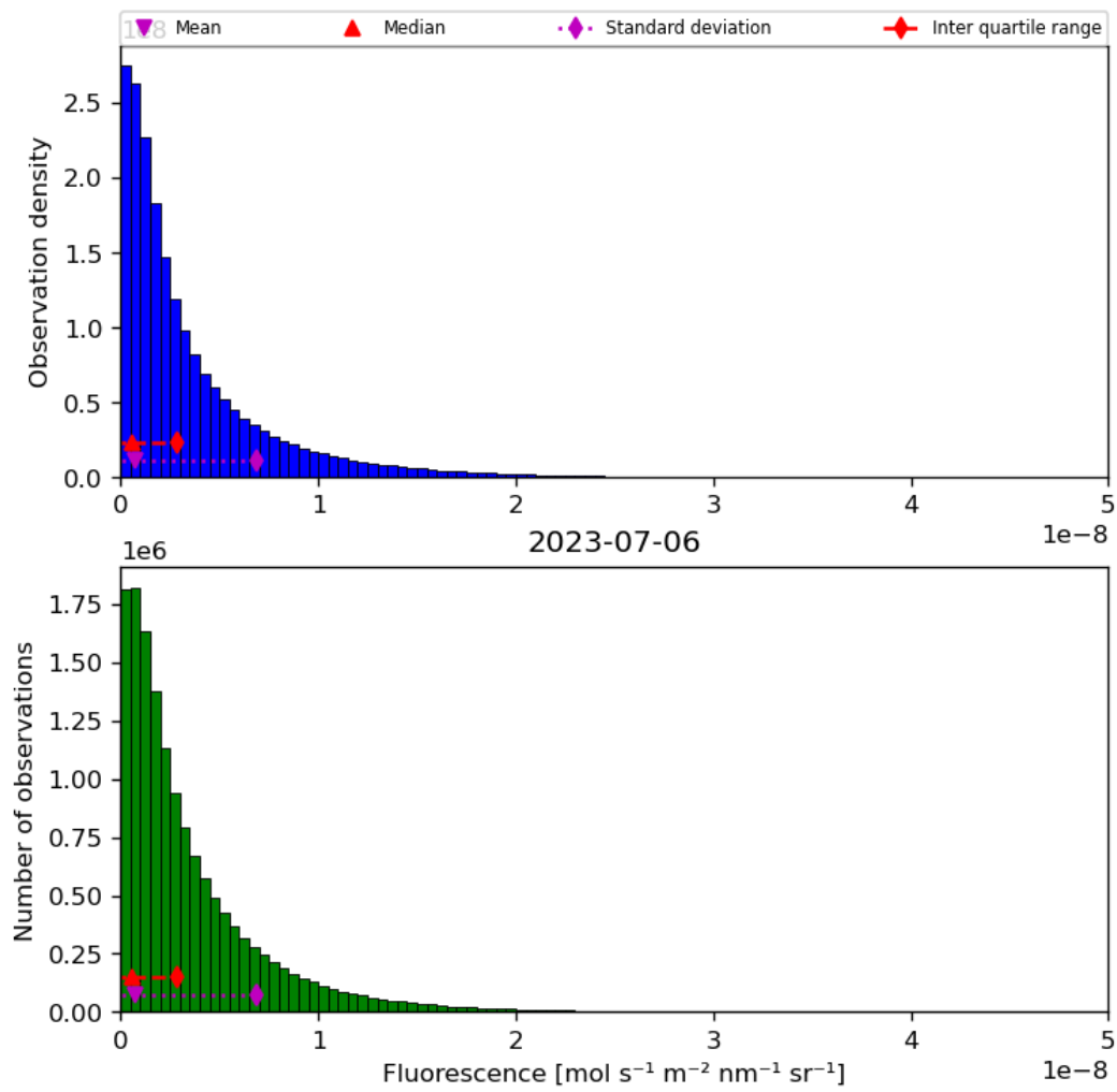
Figure 40: Histogram of “Fluorescence” for 2023-07-05 to 2023-07-07
