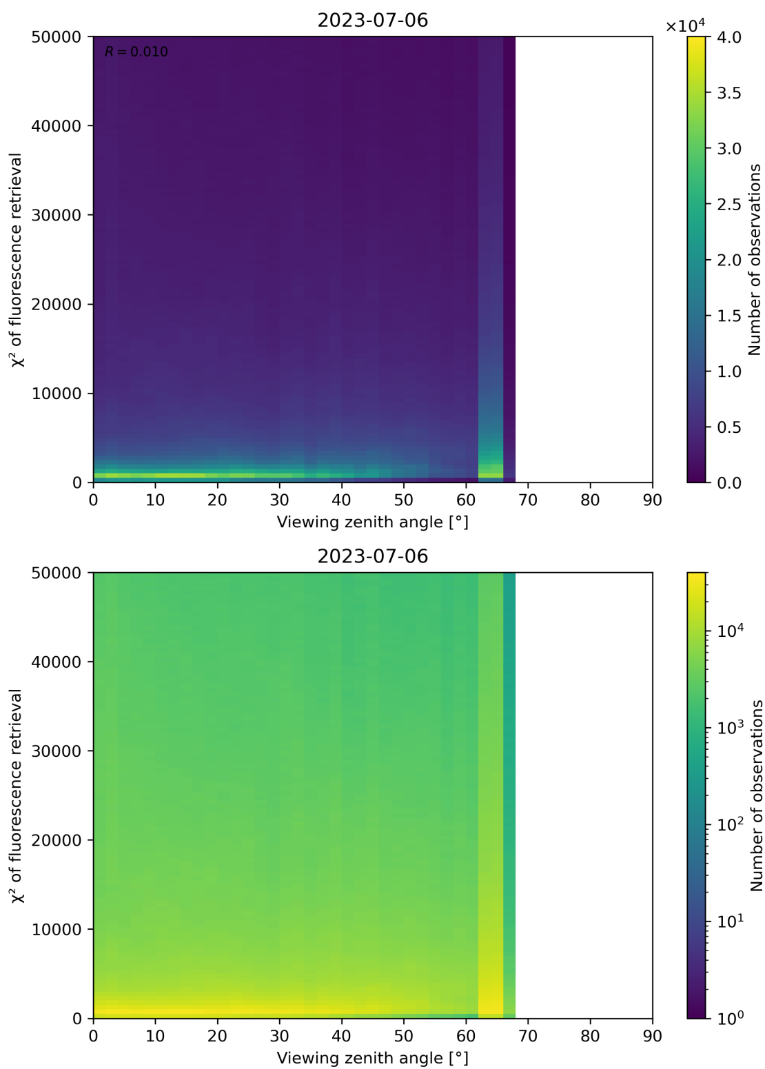
Figure 131: Scatter density plot of “Viewing zenith angle” against “ \chi^2 of fluorescence retrieval” for 2023-07-05 to 2023-07-07.
