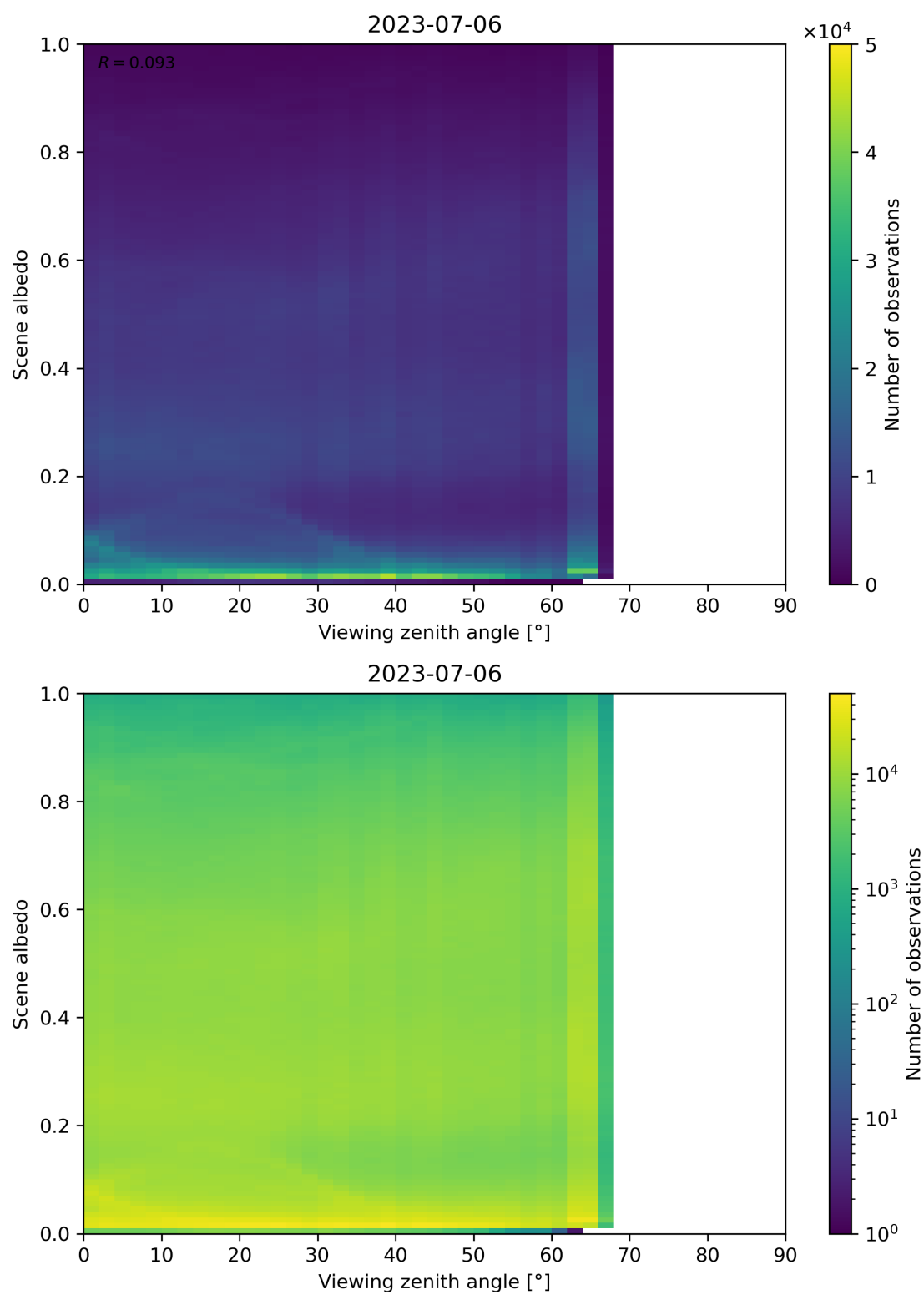
Figure 138: Scatter density plot of “Viewing zenith angle” against “Scene albedo” for 2023-07-05 to 2023-07-07.
