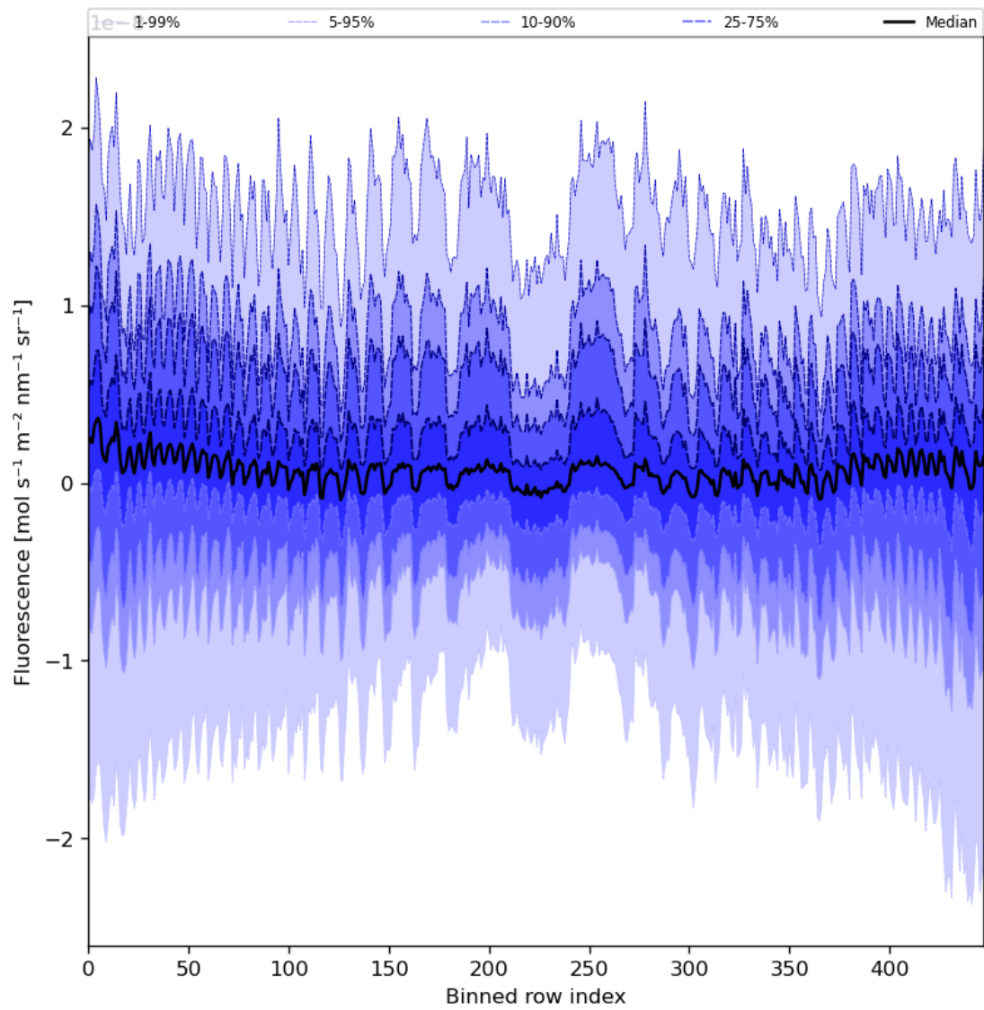
Figure 57: Along track statistics of “Fluorescence” for 2023-07-05 to 2023-07-07
