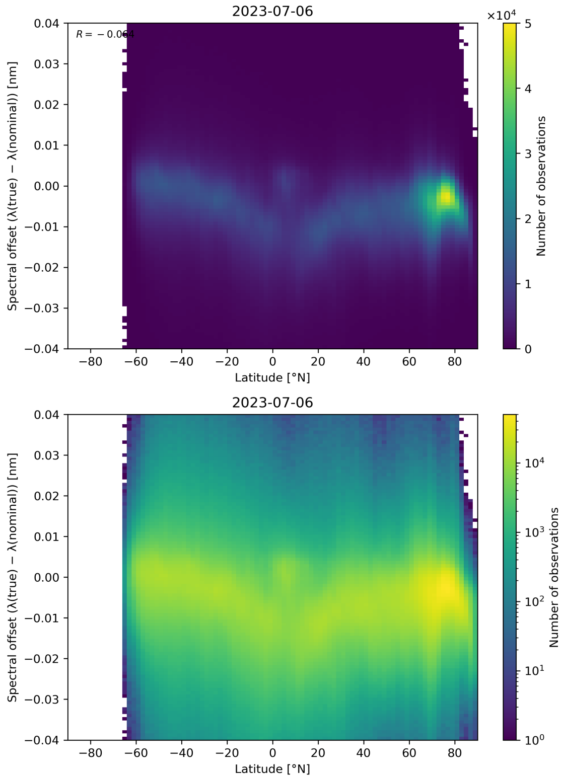
Figure 105: Scatter density plot of “Latitude” against “Spectral offset ( \lambda(\text{true}) - \lambda(\text{nominal}) )” for 2023-07-05 to 2023-07-07.
