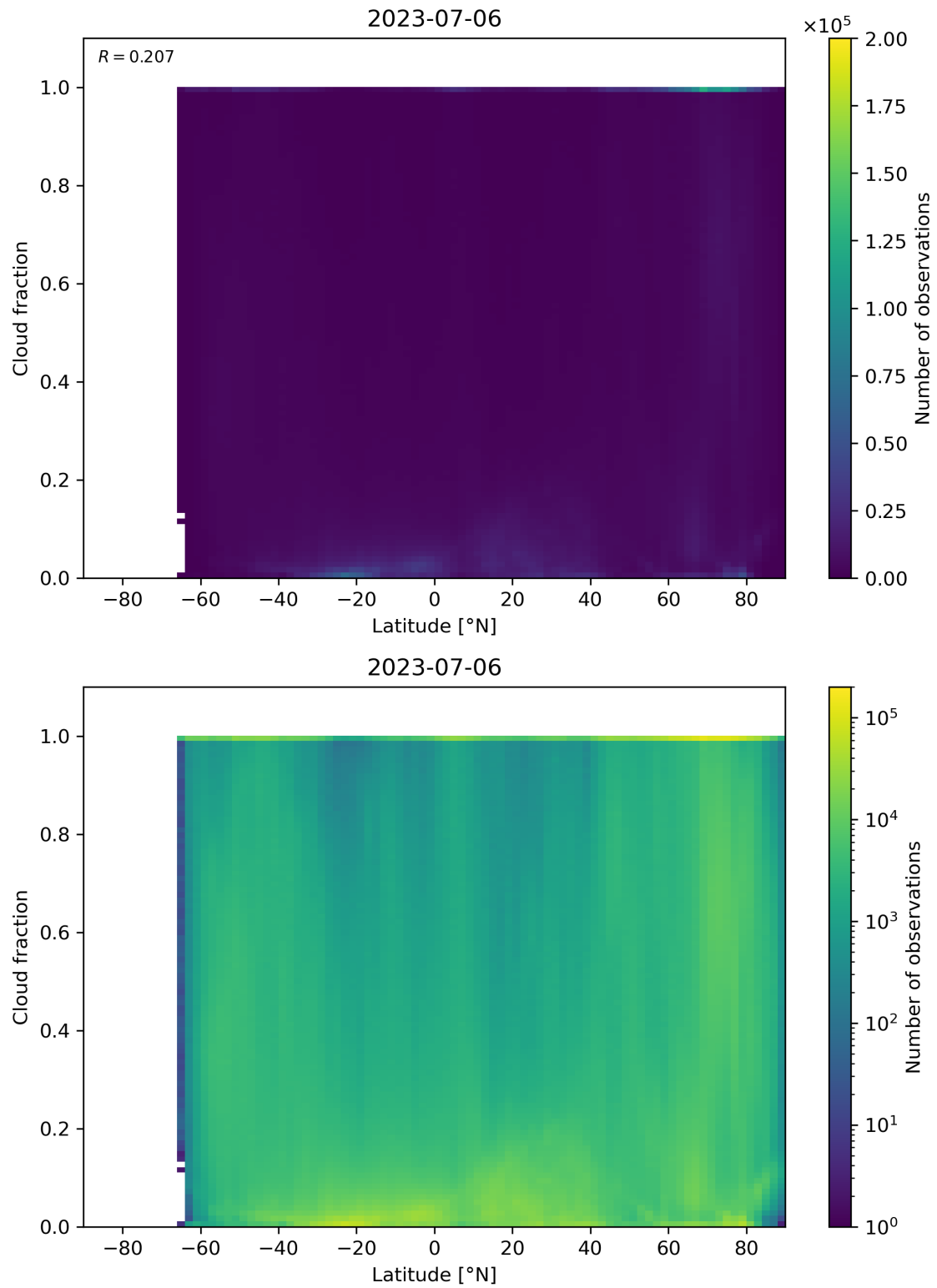
Figure 99: Scatter density plot of “Latitude” against “Cloud fraction” for 2023-07-05 to 2023-07-07.
