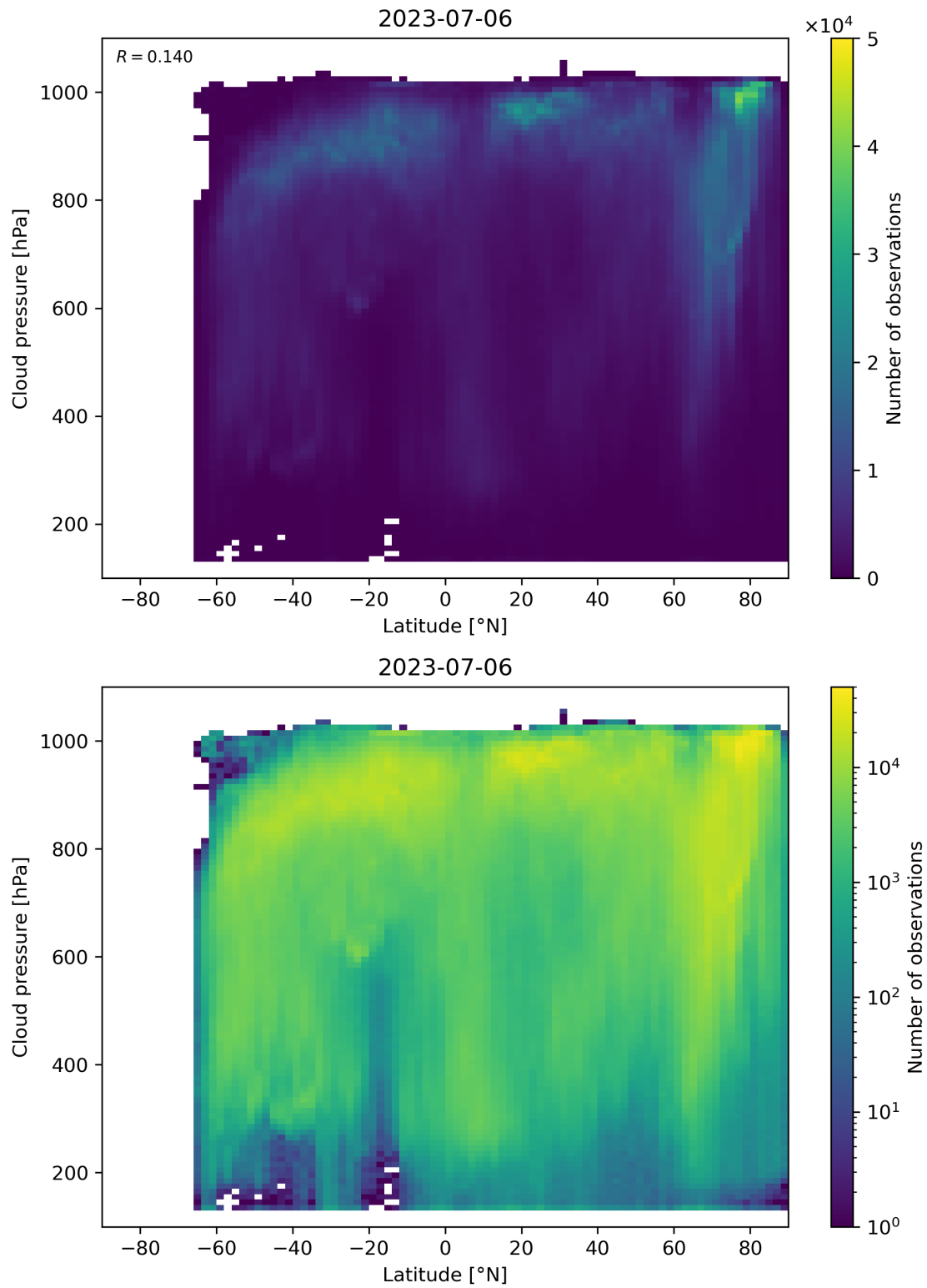
Figure 100: Scatter density plot of “Latitude” against “Cloud pressure” for 2023-07-05 to 2023-07-07.
