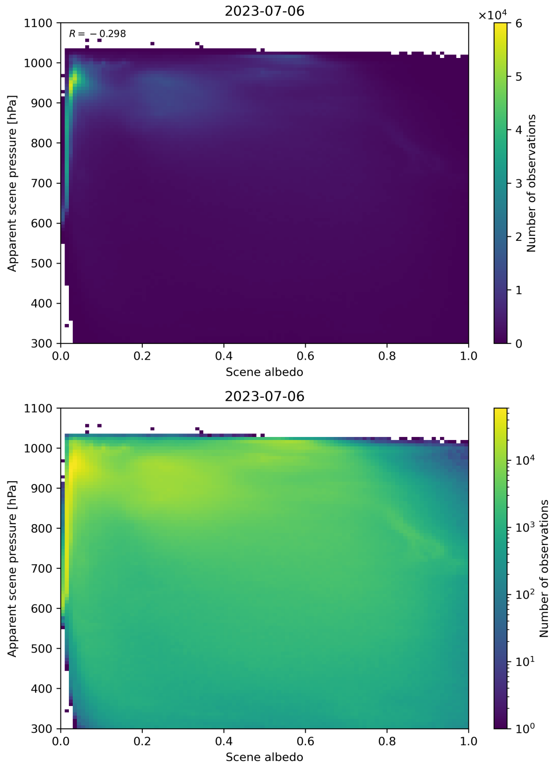
Figure 111: Scatter density plot of “Scene albedo” against “Apparent scene pressure” for 2023-07-05 to 2023-07-07.
