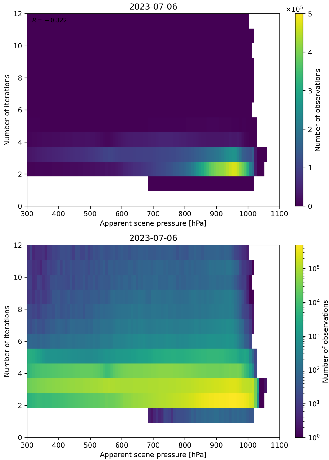
Figure 66: Scatter density plot of “Apparent scene pressure” against “Number of iterations” for 2023-07-05 to 2023-07-07.
