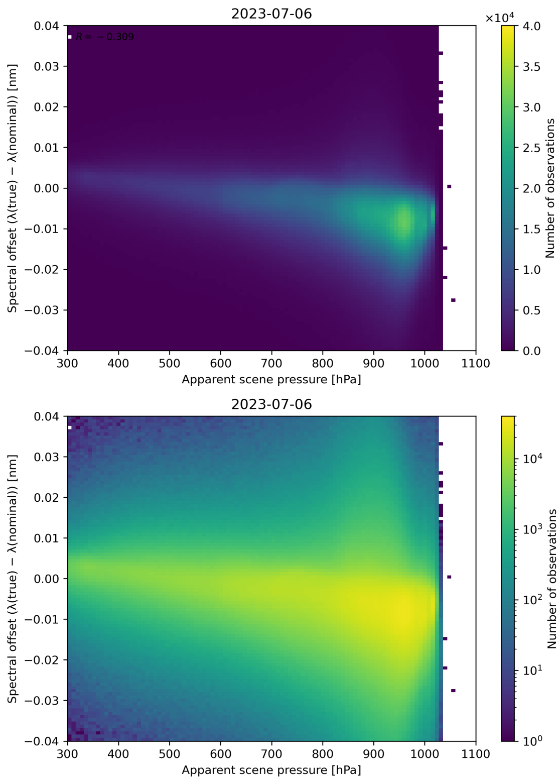
Figure 68: Scatter density plot of “Apparent scene pressure” against “Spectral offset ( \lambda(\text{true}) - \lambda(\text{nominal}) )” for 2023-07-05 to 2023-07-07.
