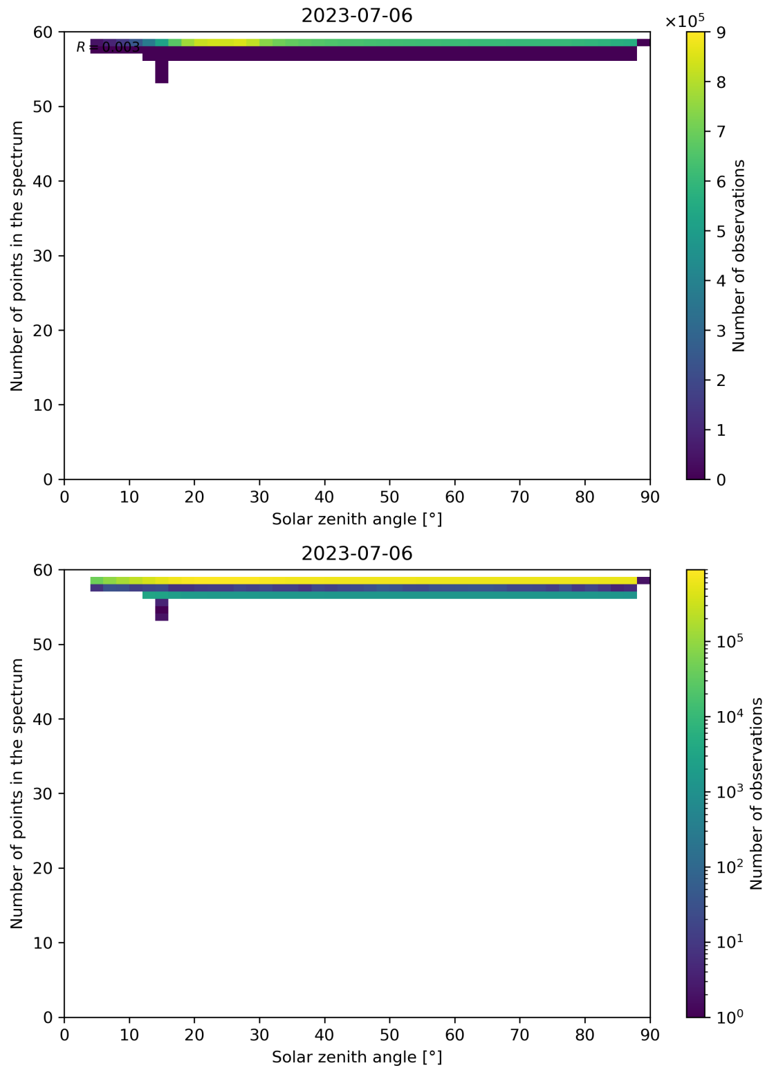
Figure 126: Scatter density plot of “Solar zenith angle” against “Number of points in the spectrum” for 2023-07-05 to 2023-07-07.
