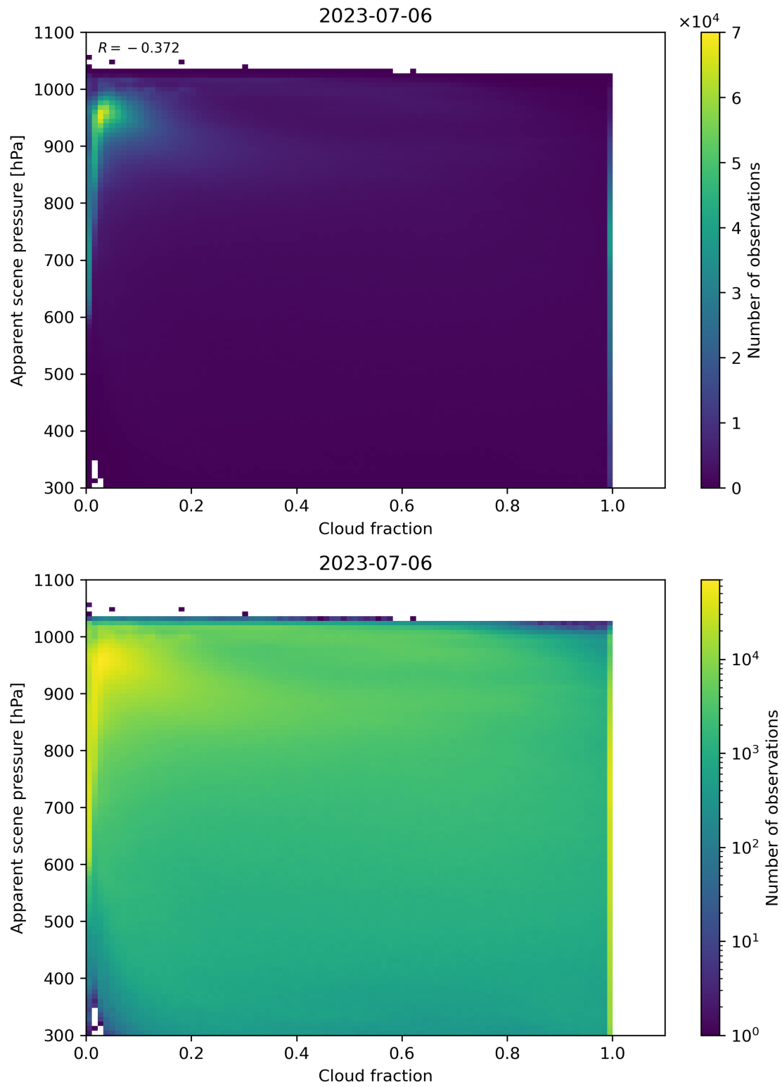
Figure 76: Scatter density plot of “Cloud fraction” against “Apparent scene pressure” for 2023-07-05 to 2023-07-07.
