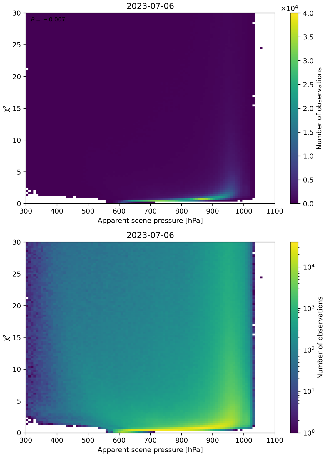
Figure 63: Scatter density plot of “Apparent scene pressure” against “ \chi^2 ” for 2023-07-05 to 2023-07-07.
