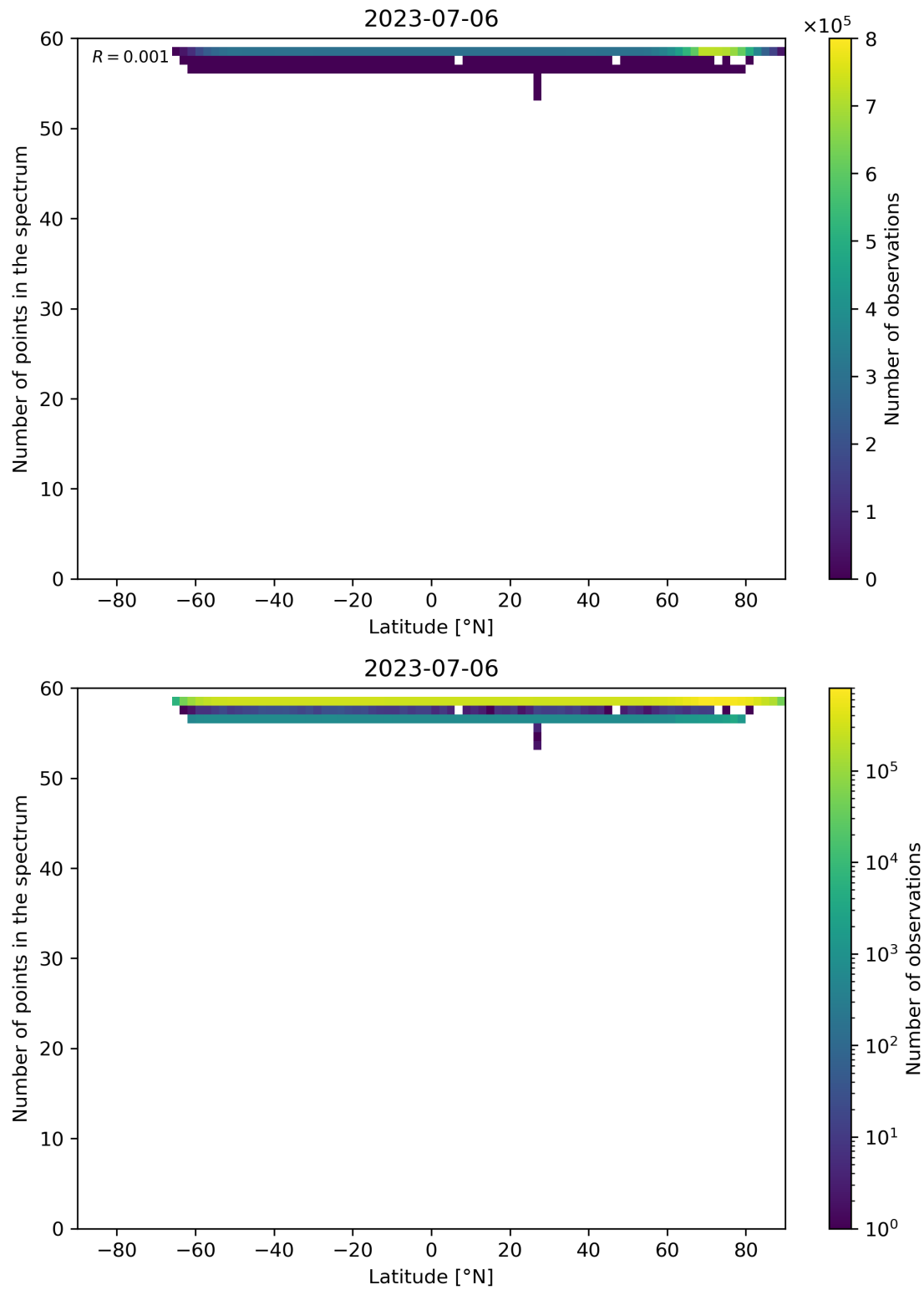
Figure 103: Scatter density plot of “Latitude” against “Number of points in the spectrum” for 2023-07-05 to 2023-07-07.
