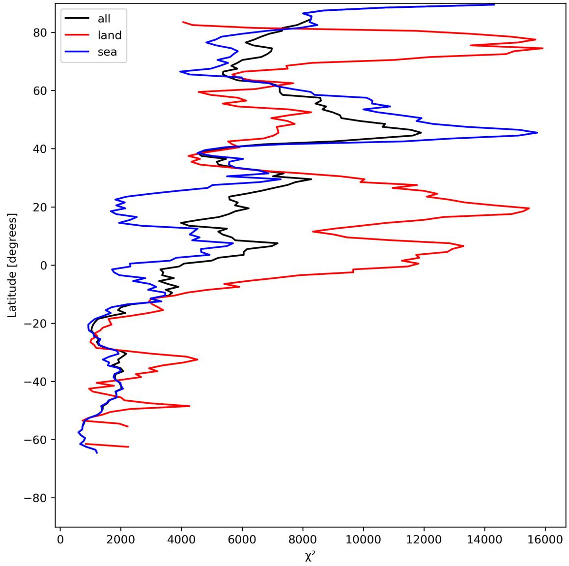
Figure 21: Zonal average of “ \chi^2 ” for 2023-07-05 to 2023-07-07.
