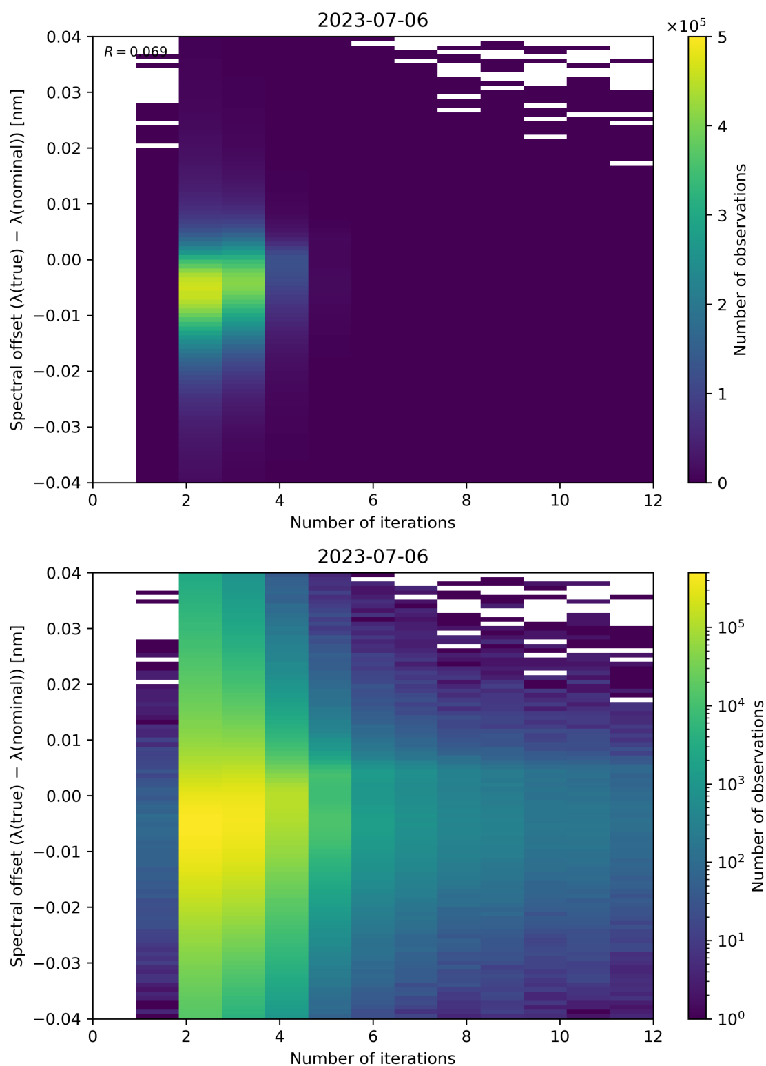
Figure 109: Scatter density plot of “Number of iterations” against “Spectral offset ( \lambda(\text{true}) - \lambda(\text{nominal}) )” for 2023-07-05 to 2023-07-07.
