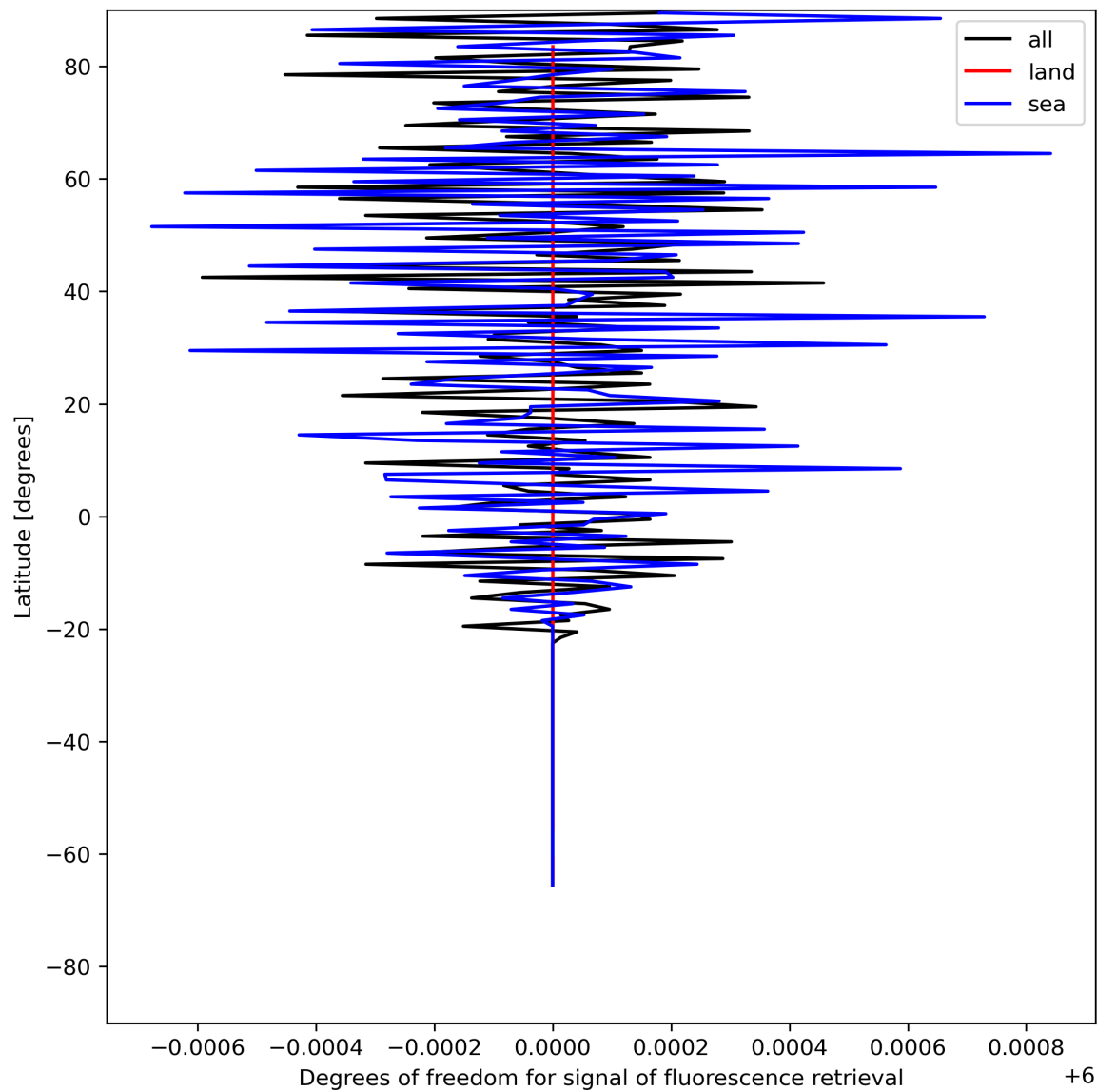
Figure 26: Zonal average of “Degrees of freedom for signal of fluorescence retrieval” for 2023-07-08 to 2023-07-09.
