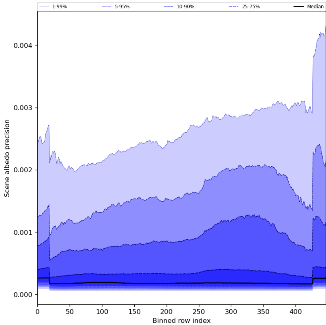
Figure 52: Along track statistics of “Scene albedo precision” for 2023-07-08 to 2023-07-09
