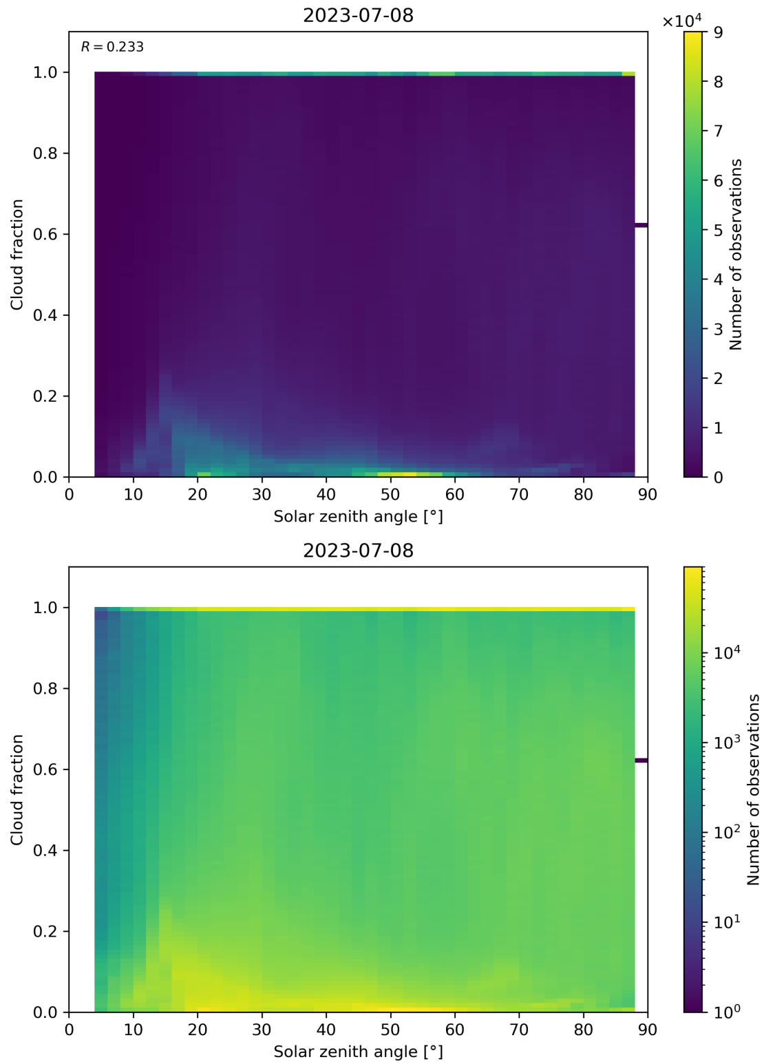
Figure 121: Scatter density plot of “Solar zenith angle” against “Cloud fraction” for 2023-07-08 to 2023-07-09.
