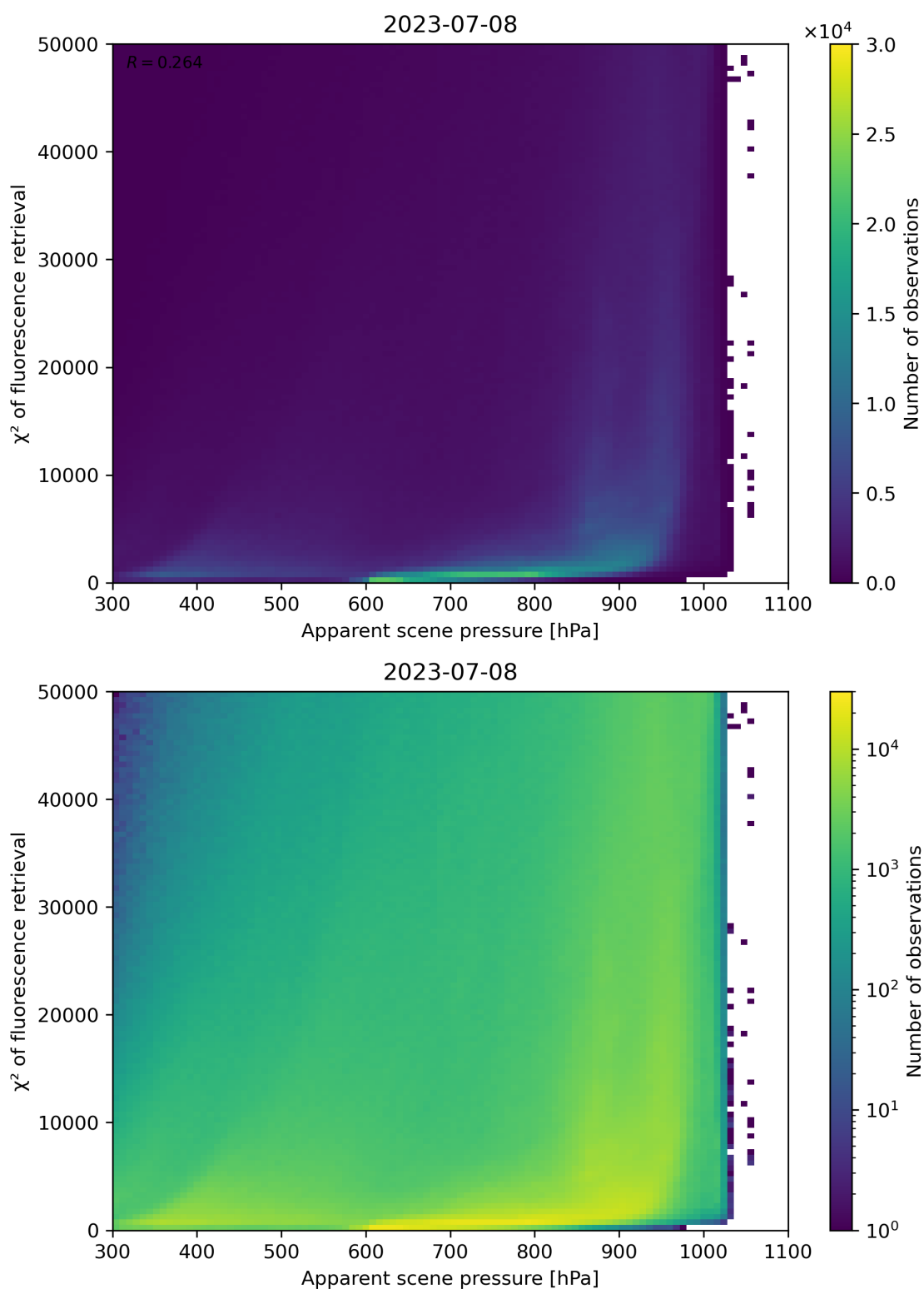
Figure 64: Scatter density plot of “Apparent scene pressure” against “ \chi^2 of fluorescence retrieval” for 2023-07-08 to 2023-07-09.
