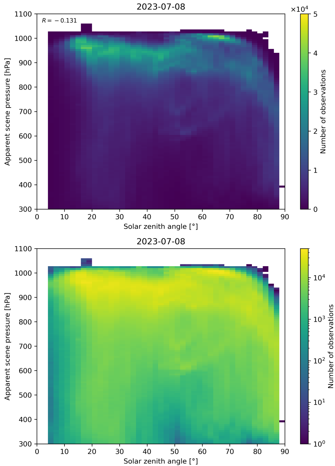
Figure 118: Scatter density plot of “Solar zenith angle” against “Apparent scene pressure” for 2023-07-08 to 2023-07-09.
