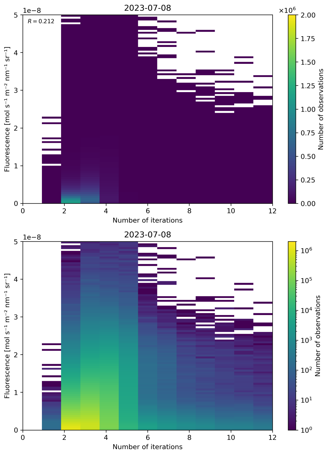
Figure 107: Scatter density plot of “Number of iterations” against “Fluorescence” for 2023-07-08 to 2023-07-09.
