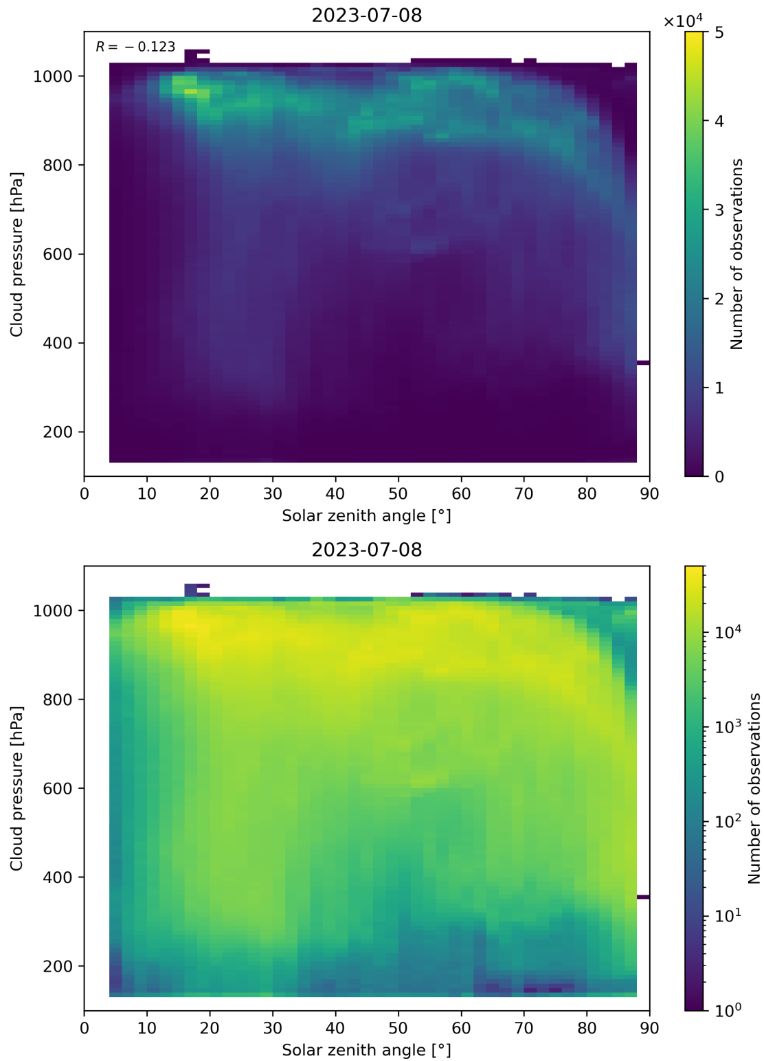
Figure 122: Scatter density plot of “Solar zenith angle” against “Cloud pressure” for 2023-07-08 to 2023-07-09.
