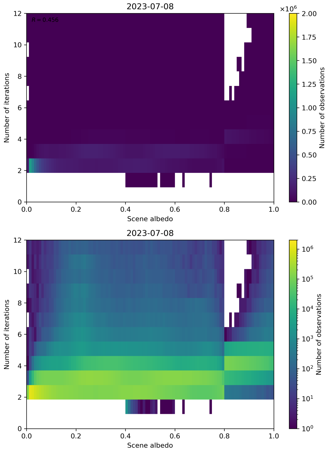
Figure 115: Scatter density plot of “Scene albedo” against “Number of iterations” for 2023-07-08 to 2023-07-09.
