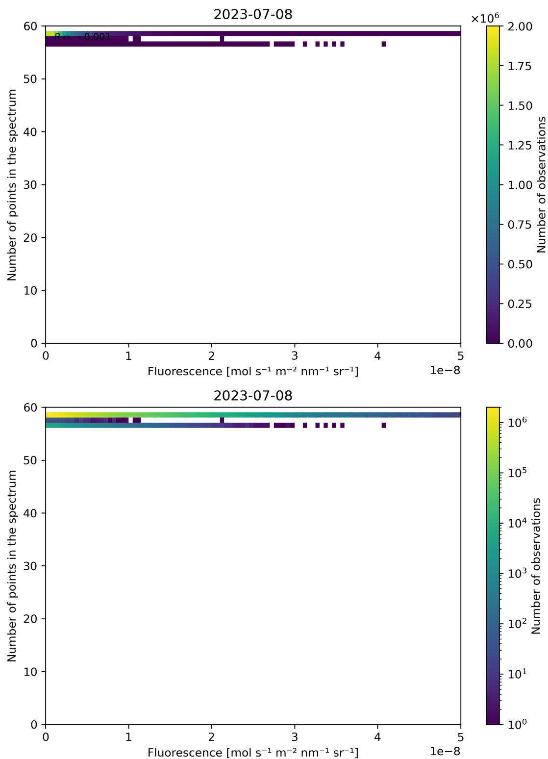
Figure 94: Scatter density plot of “Fluorescence” against “Number of points in the spectrum” for 2023-07-08 to 2023-07-09.
