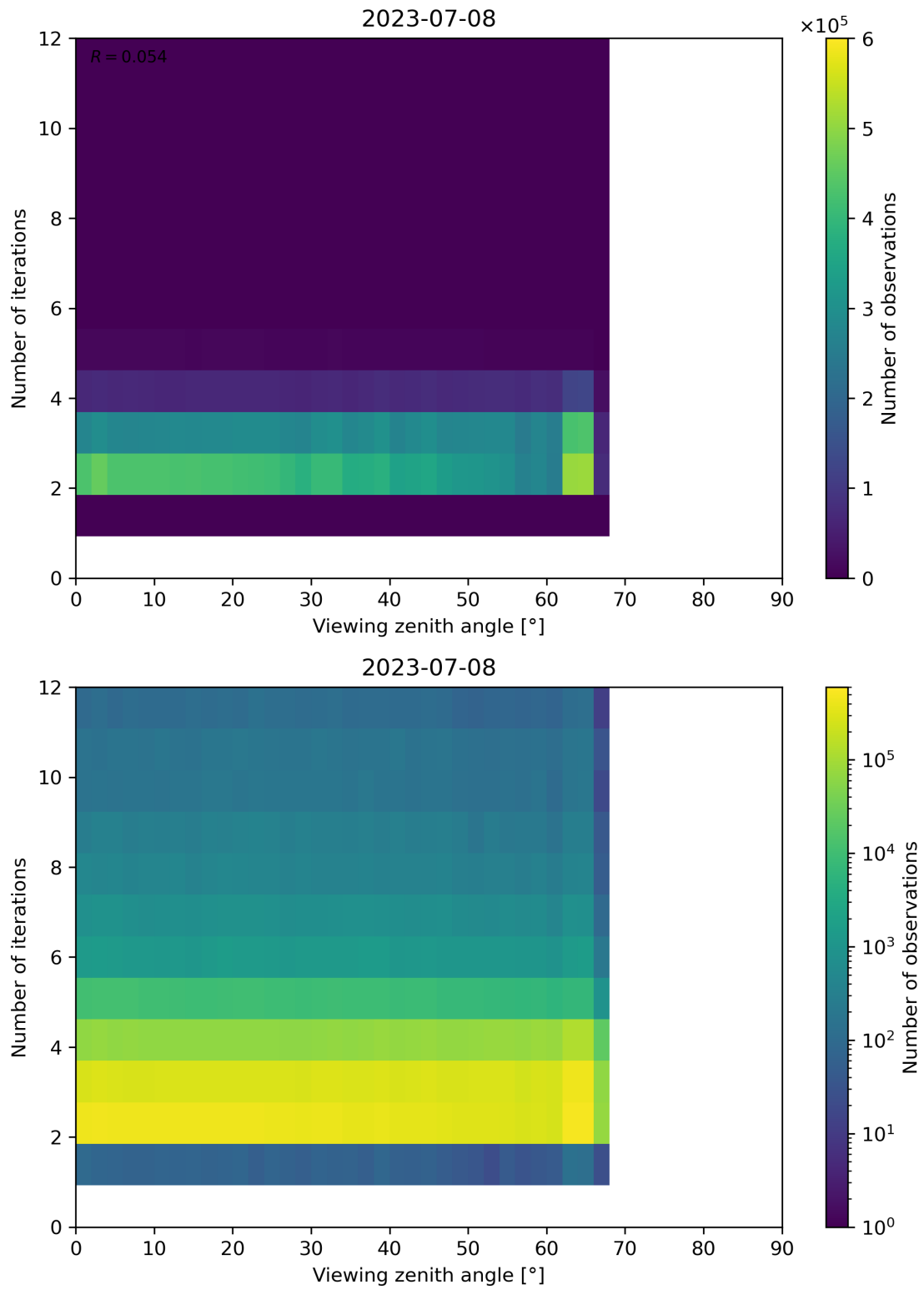
Figure 136: Scatter density plot of “Viewing zenith angle” against “Number of iterations” for 2023-07-08 to 2023-07-09.
