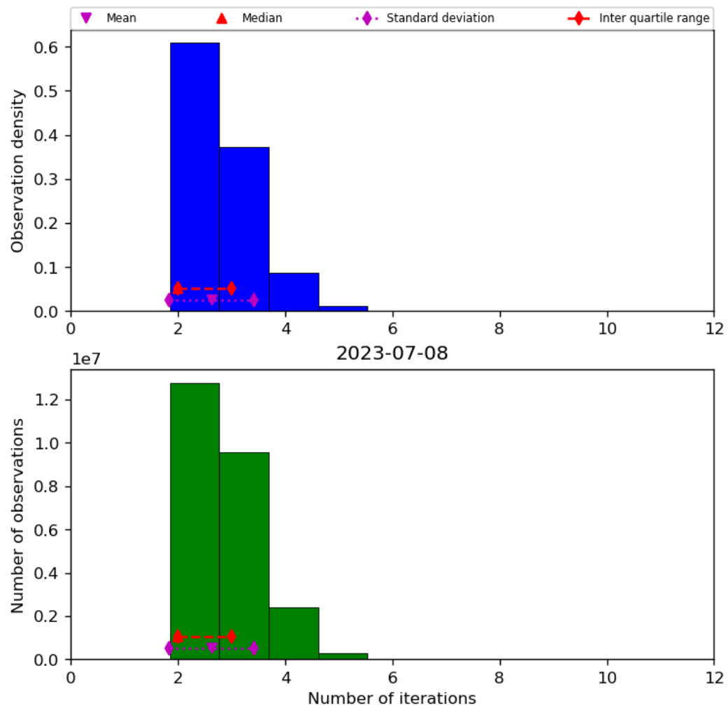
Figure 39: Histogram of “Number of iterations” for 2023-07-08 to 2023-07-09
