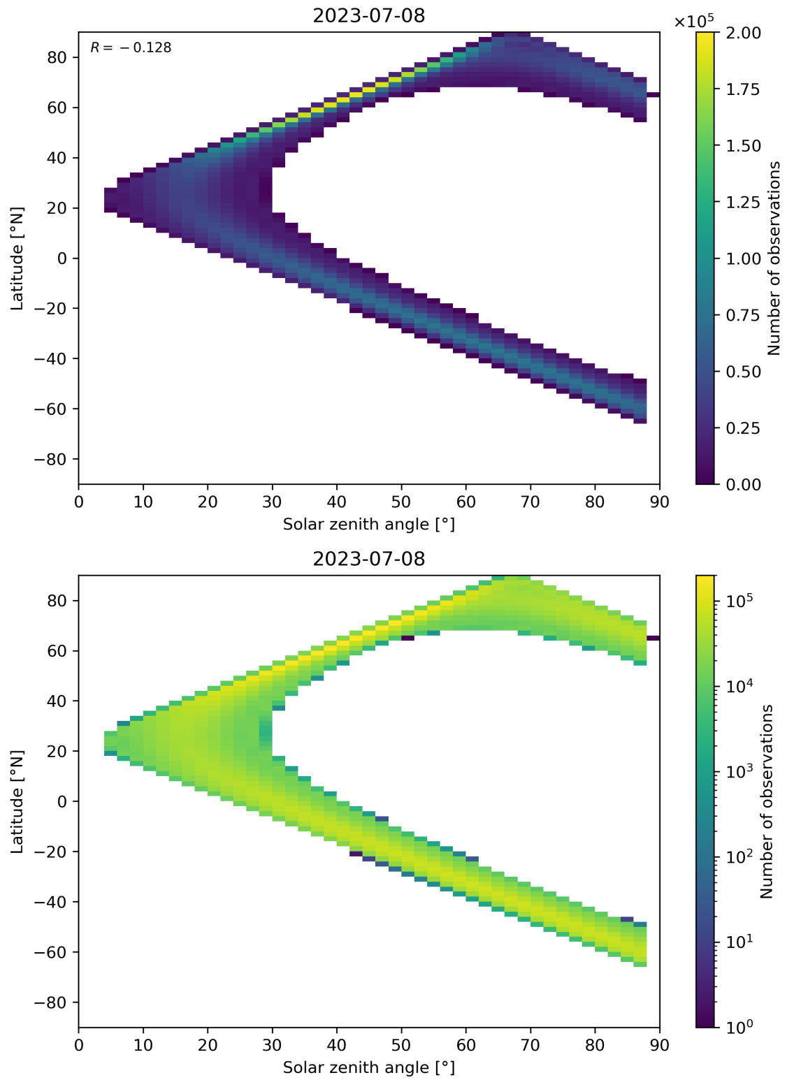
Figure 124: Scatter density plot of “Solar zenith angle” against “Latitude” for 2023-07-08 to 2023-07-09.
