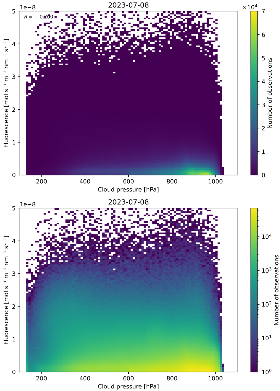
Figure 88: Scatter density plot of “Cloud pressure” against “Fluorescence” for 2023-07-08 to 2023-07-09.
