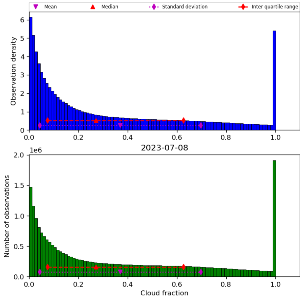
Figure 32: Histogram of “Cloud fraction” for 2023-07-08 to 2023-07-09
