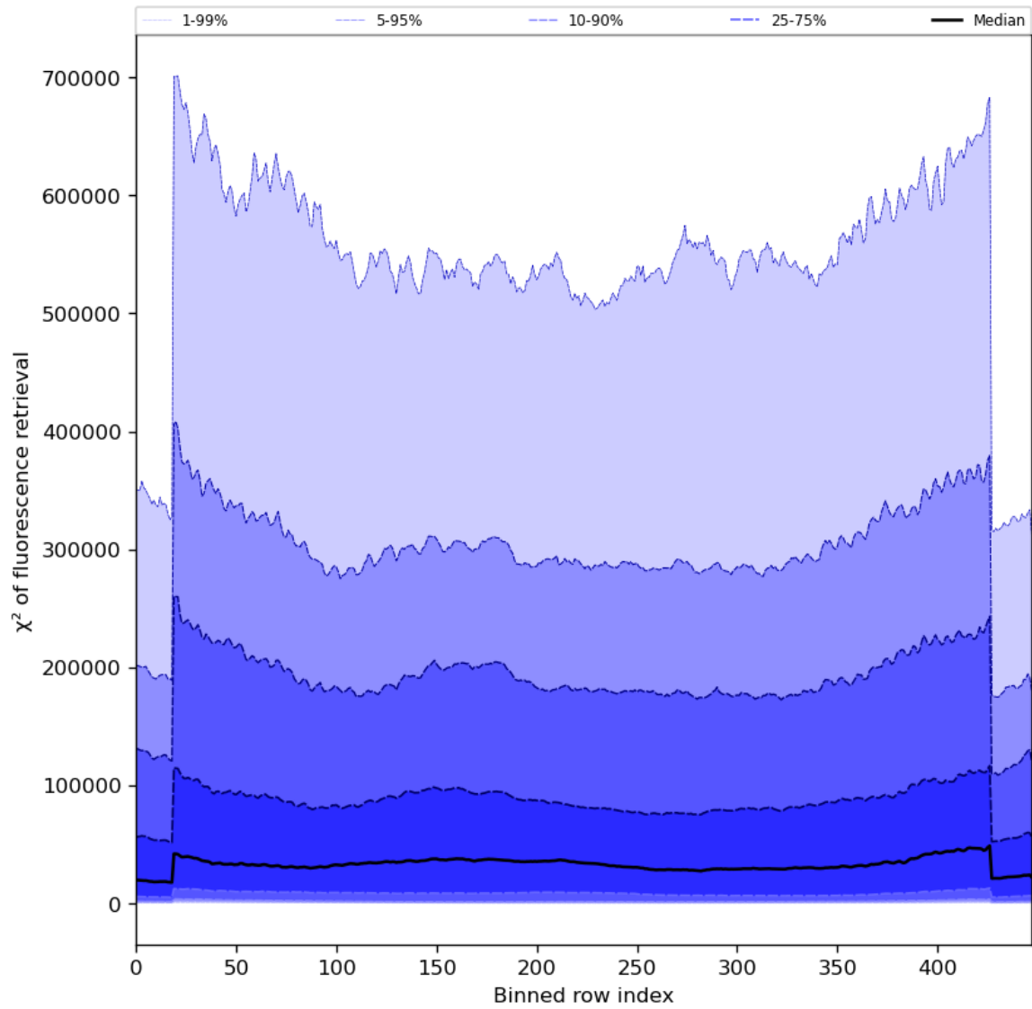
Figure 59: Along track statistics of “ \chi^2 of fluorescence retrieval” for 2023-07-08 to 2023-07-09
