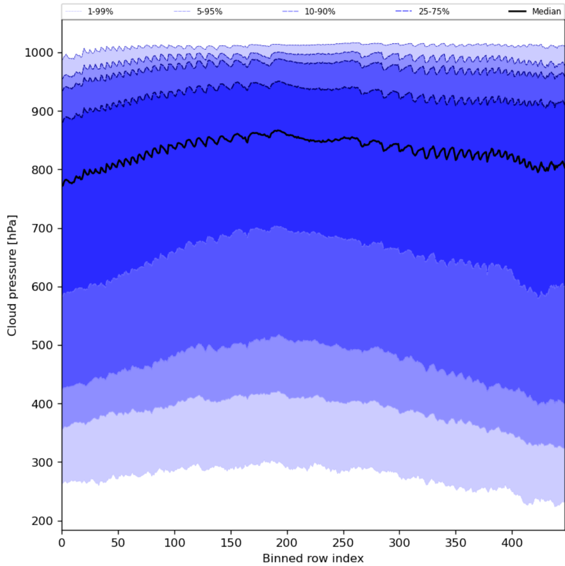
Figure 47: Along track statistics of “Cloud pressure” for 2023-07-08 to 2023-07-09
