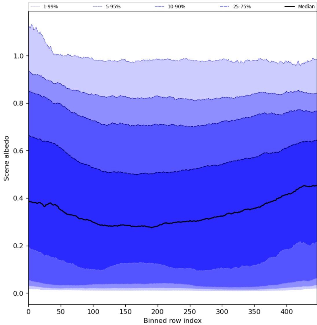
Figure 51: Along track statistics of “Scene albedo” for 2023-07-08 to 2023-07-09
