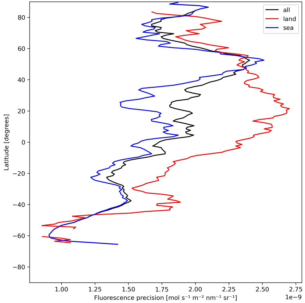
Figure 24: Zonal average of “Fluorescence precision” for 2023-07-08 to 2023-07-09.
