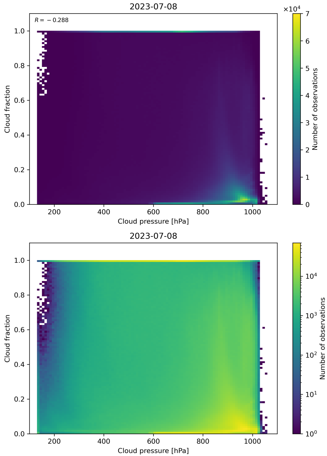
Figure 87: Scatter density plot of “Cloud pressure” against “Cloud fraction” for 2023-07-08 to 2023-07-09.
