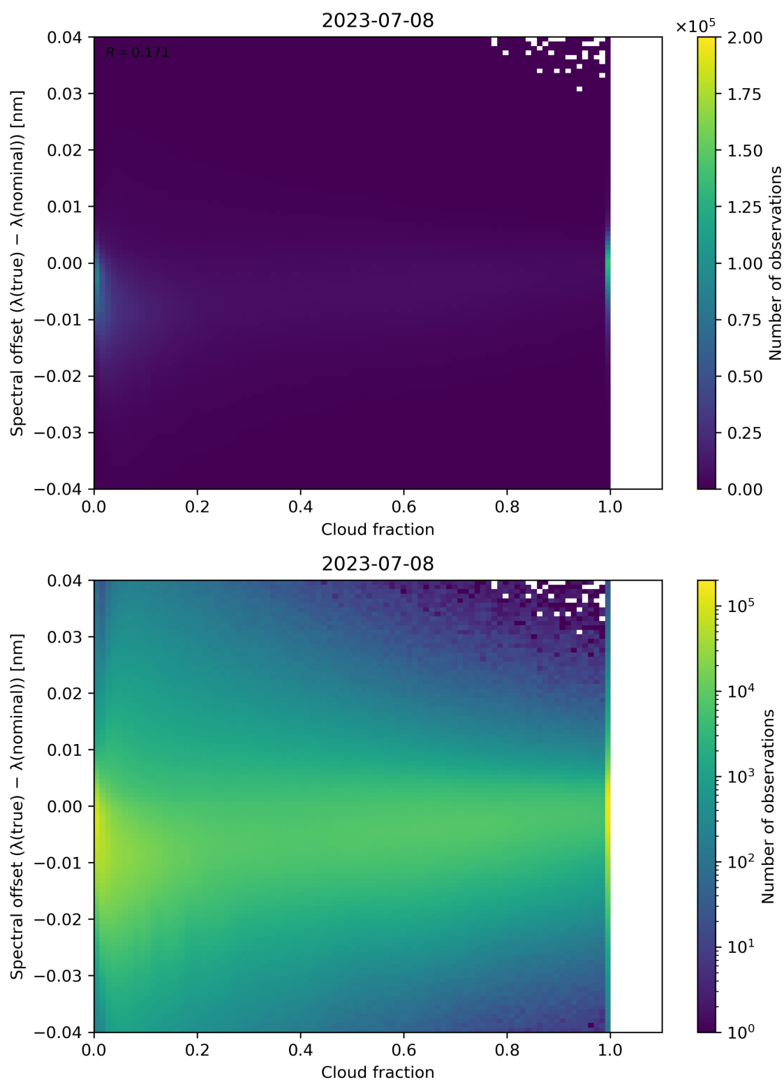
Figure 83: Scatter density plot of “Cloud fraction” against “Spectral offset ( \lambda(\text{true}) - \lambda(\text{nominal}) )” for 2023-07-08 to 2023-07-09.
