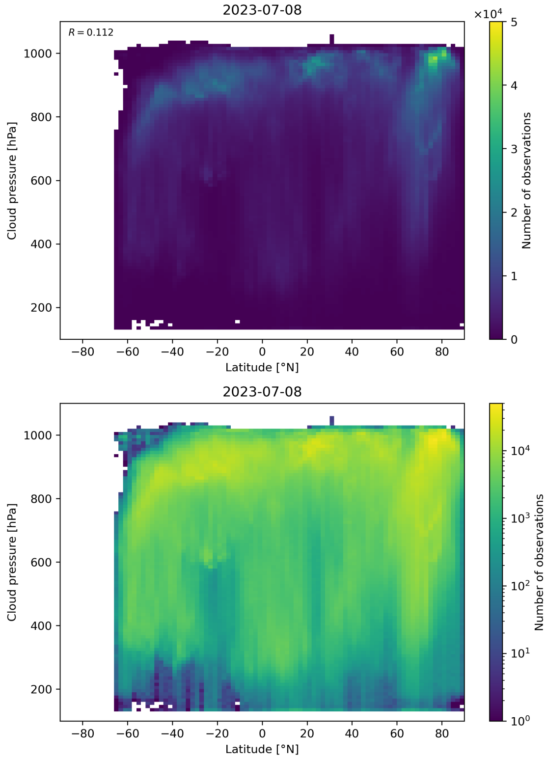
Figure 100: Scatter density plot of “Latitude” against “Cloud pressure” for 2023-07-08 to 2023-07-09.
