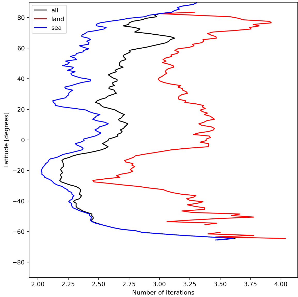
Figure 22: Zonal average of “Number of iterations” for 2023-07-08 to 2023-07-09.
