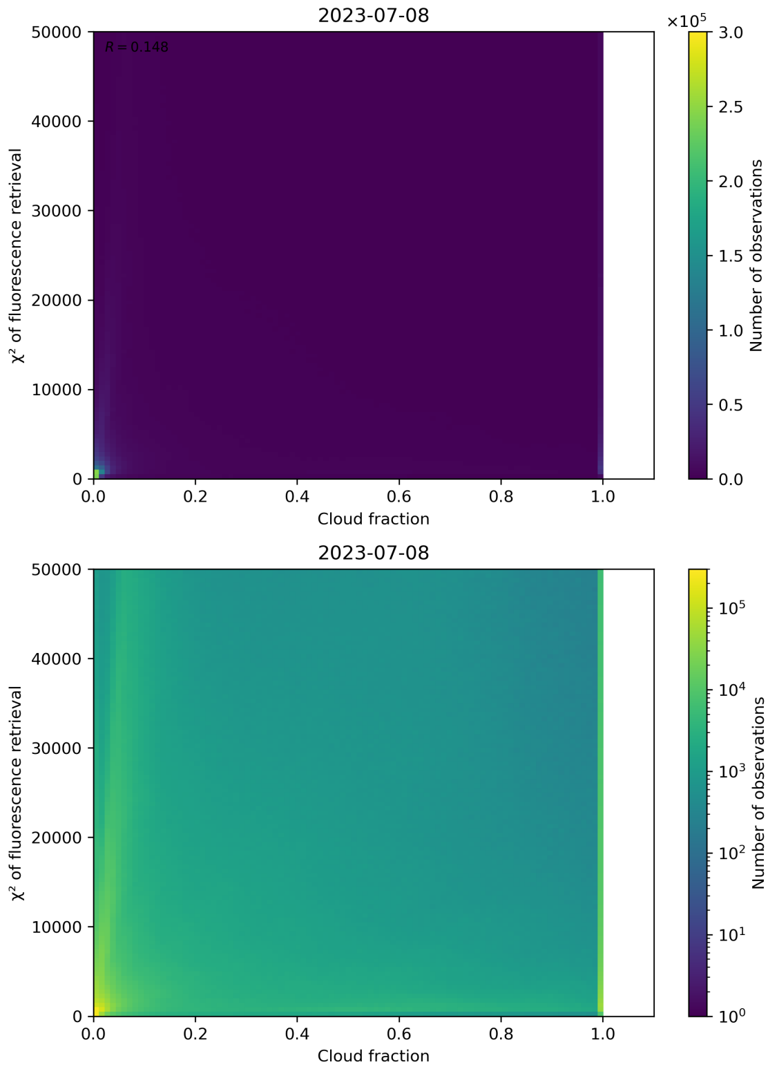
Figure 78: Scatter density plot of “Cloud fraction” against “ \chi^2 of fluorescence retrieval” for 2023-07-08 to 2023-07-09.
