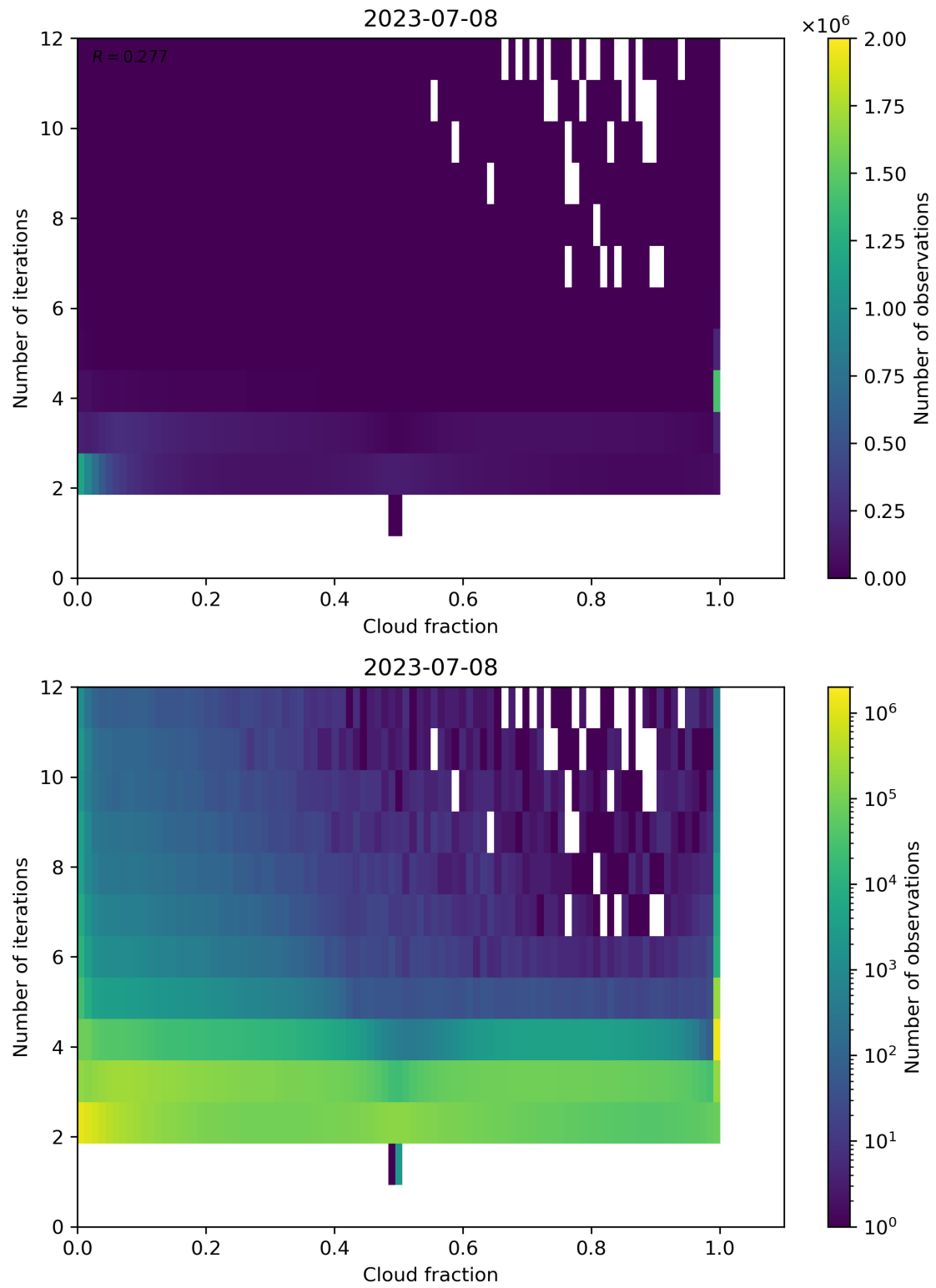
Figure 80: Scatter density plot of “Cloud fraction” against “Number of iterations” for 2023-07-08 to 2023-07-09.
