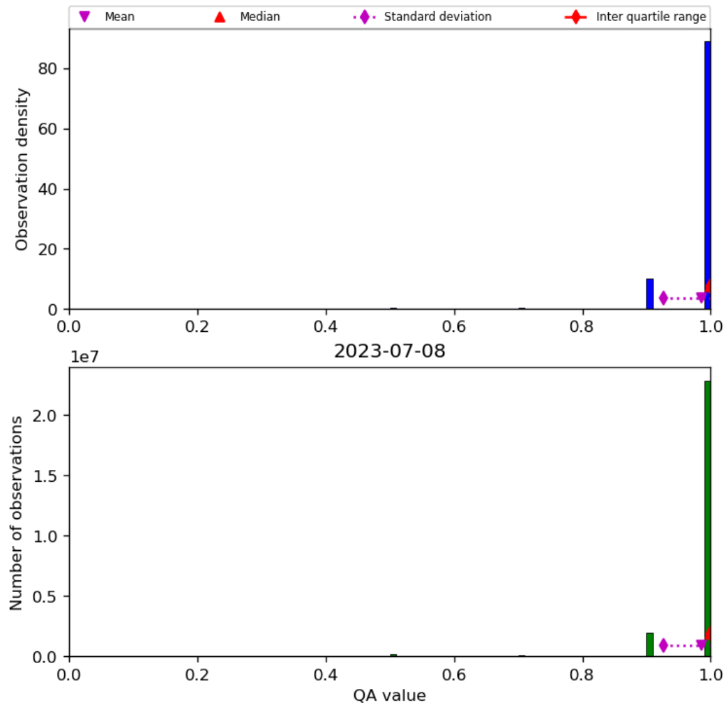
Figure 29: Histogram of “QA value” for 2023-07-08 to 2023-07-09
