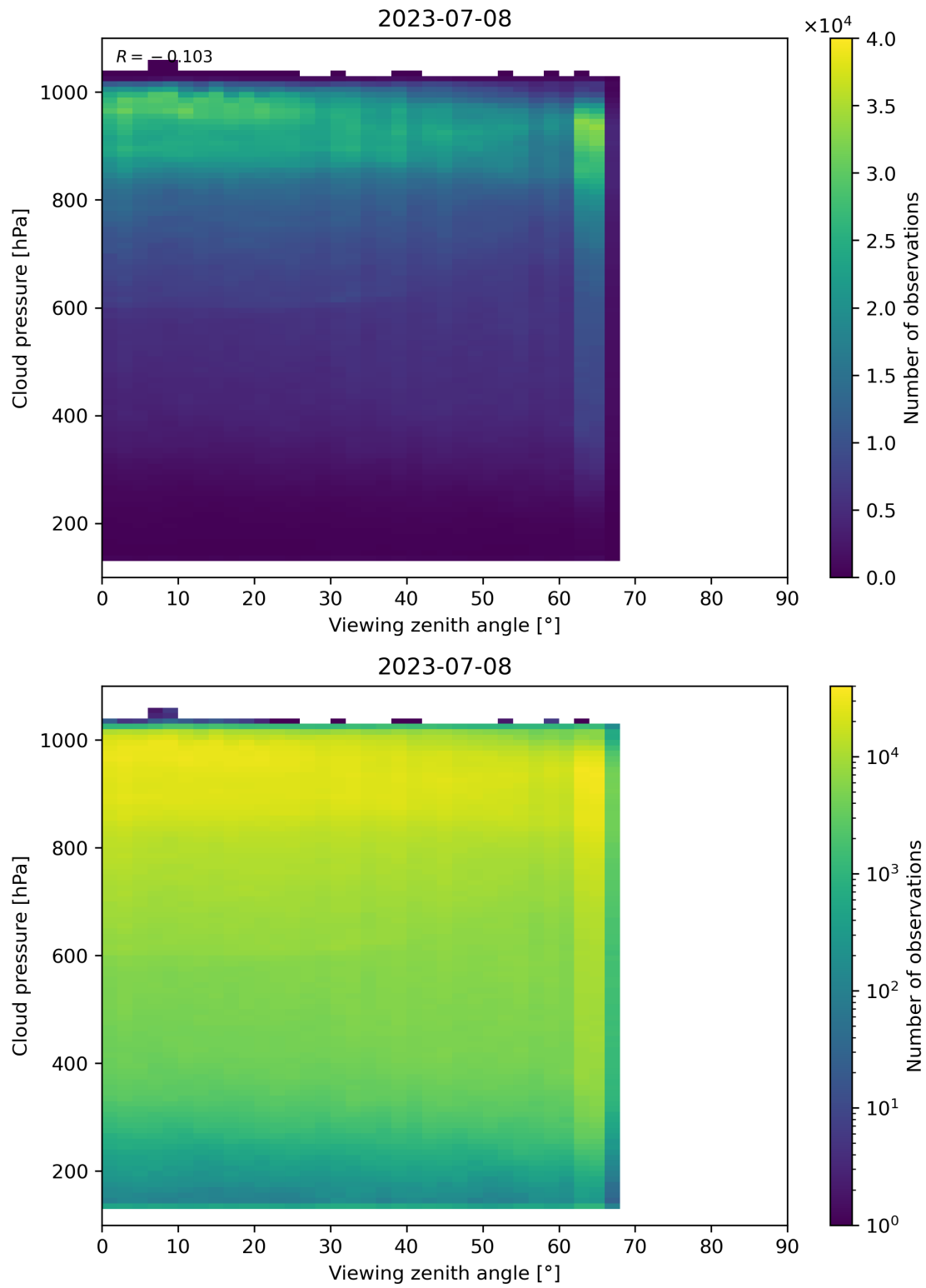
Figure 133: Scatter density plot of “Viewing zenith angle” against “Cloud pressure” for 2023-07-08 to 2023-07-09.
