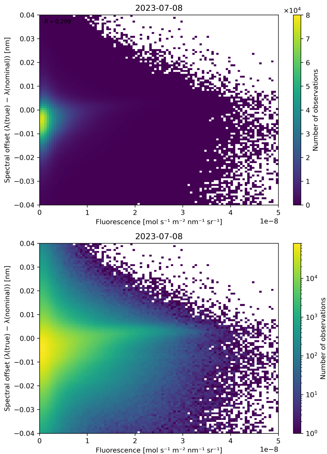
Figure 95: Scatter density plot of “Fluorescence” against “Spectral offset ( \lambda(\text{true}) - \lambda(\text{nominal}) )” for 2023-07-08 to 2023-07-09.
