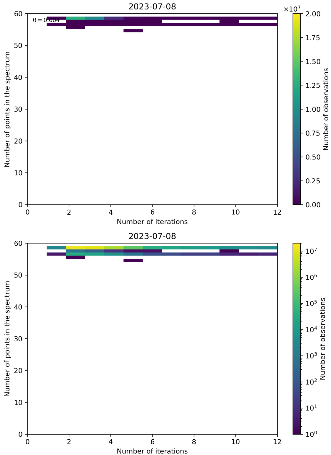
Figure 108: Scatter density plot of “Number of iterations” against “Number of points in the spectrum” for 2023-07-08 to 2023-07-09.
