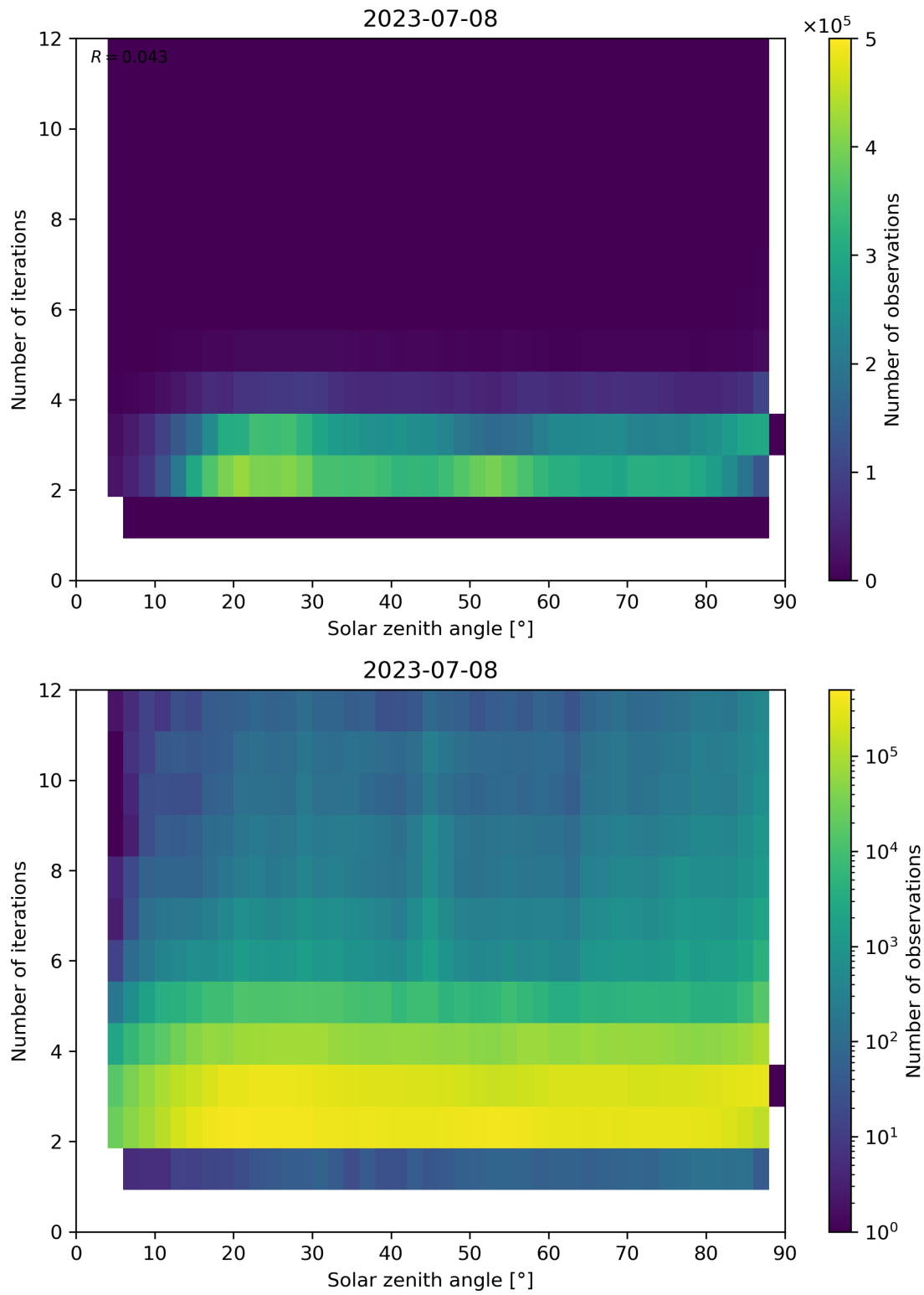
Figure 125: Scatter density plot of “Solar zenith angle” against “Number of iterations” for 2023-07-08 to 2023-07-09.
