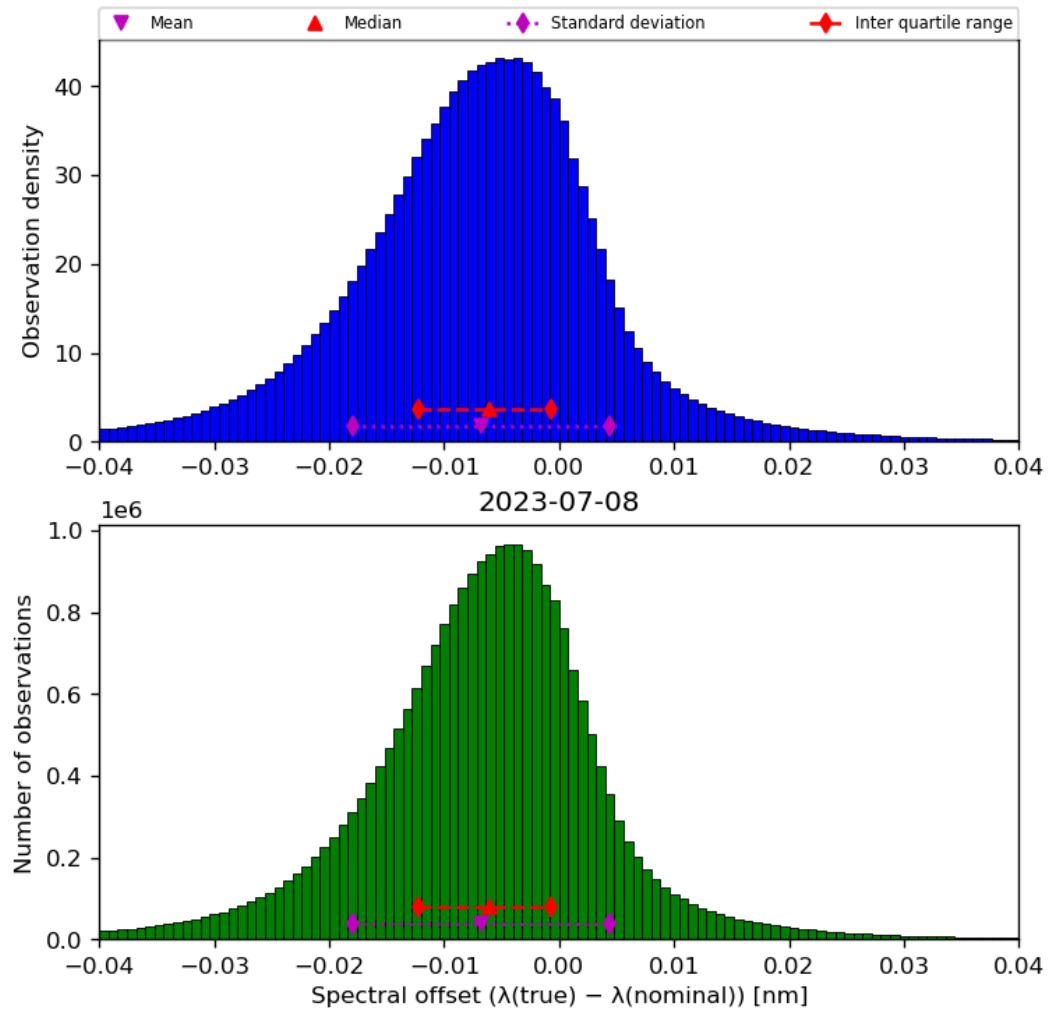
Figure 45: Histogram of “Spectral offset ( \lambda(\text{true}) - \lambda(\text{nominal}) )” for 2023-07-08 to 2023-07-09
