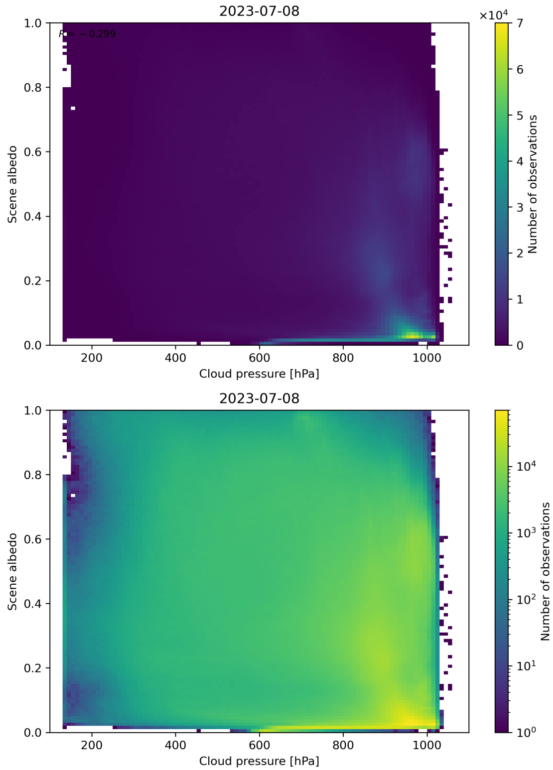
Figure 91: Scatter density plot of “Cloud pressure” against “Scene albedo” for 2023-07-08 to 2023-07-09.
