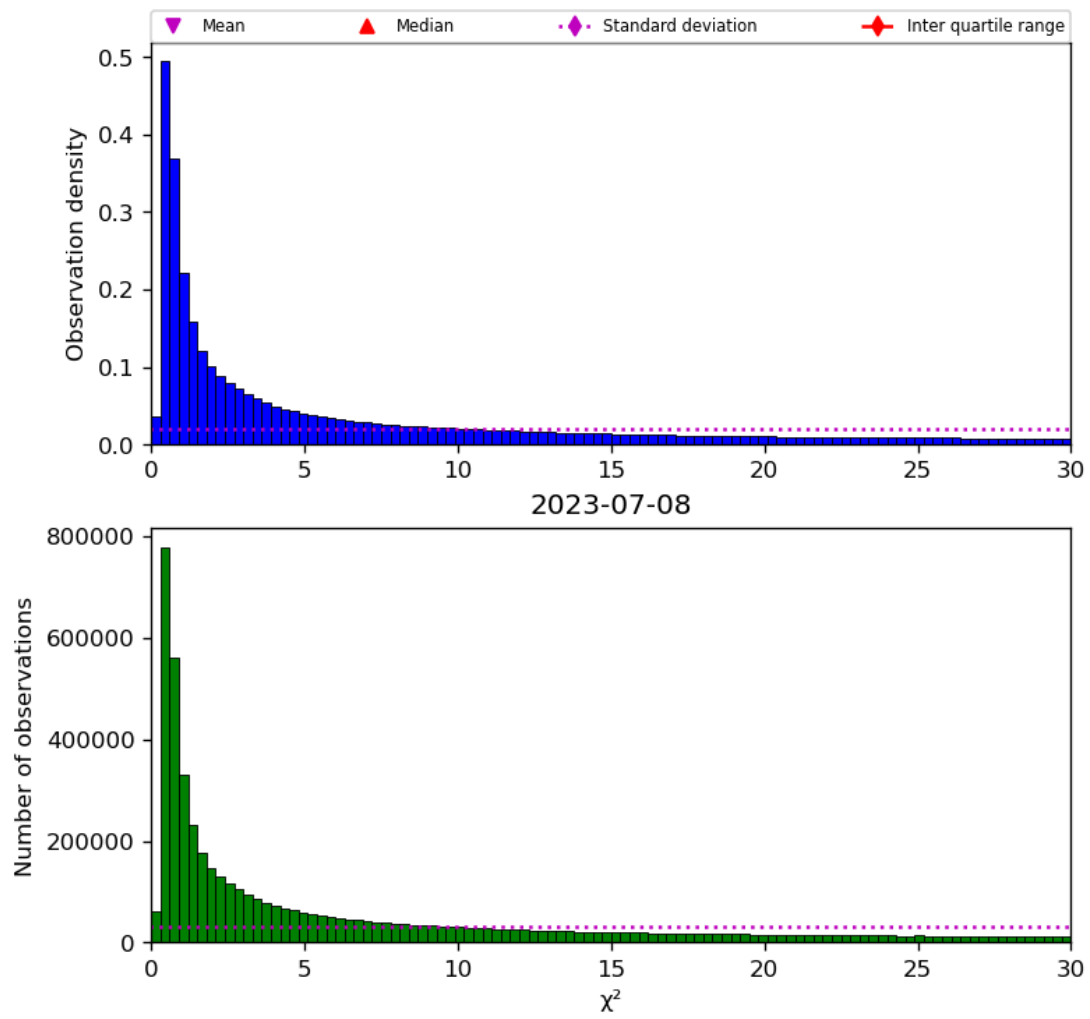
Figure 38: Histogram of " \chi^2 " for 2023-07-08 to 2023-07-09
