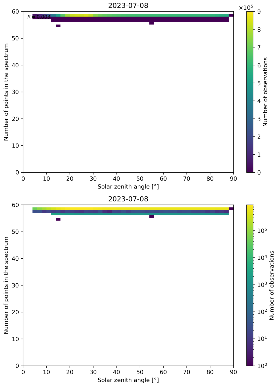
Figure 126: Scatter density plot of “Solar zenith angle” against “Number of points in the spectrum” for 2023-07-08 to 2023-07-09.
