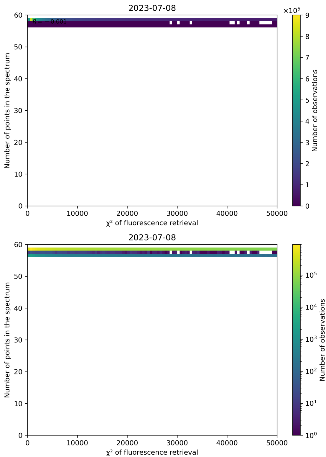
Figure 71: Scatter density plot of " \chi^2 of fluorescence retrieval" against "Number of points in the spectrum" for 2023-07-08 to 2023-07-09.
