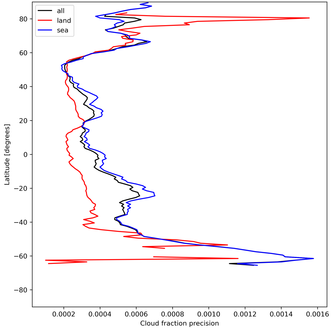
Figure 16: Zonal average of “Cloud fraction precision” for 2023-07-08 to 2023-07-09.
