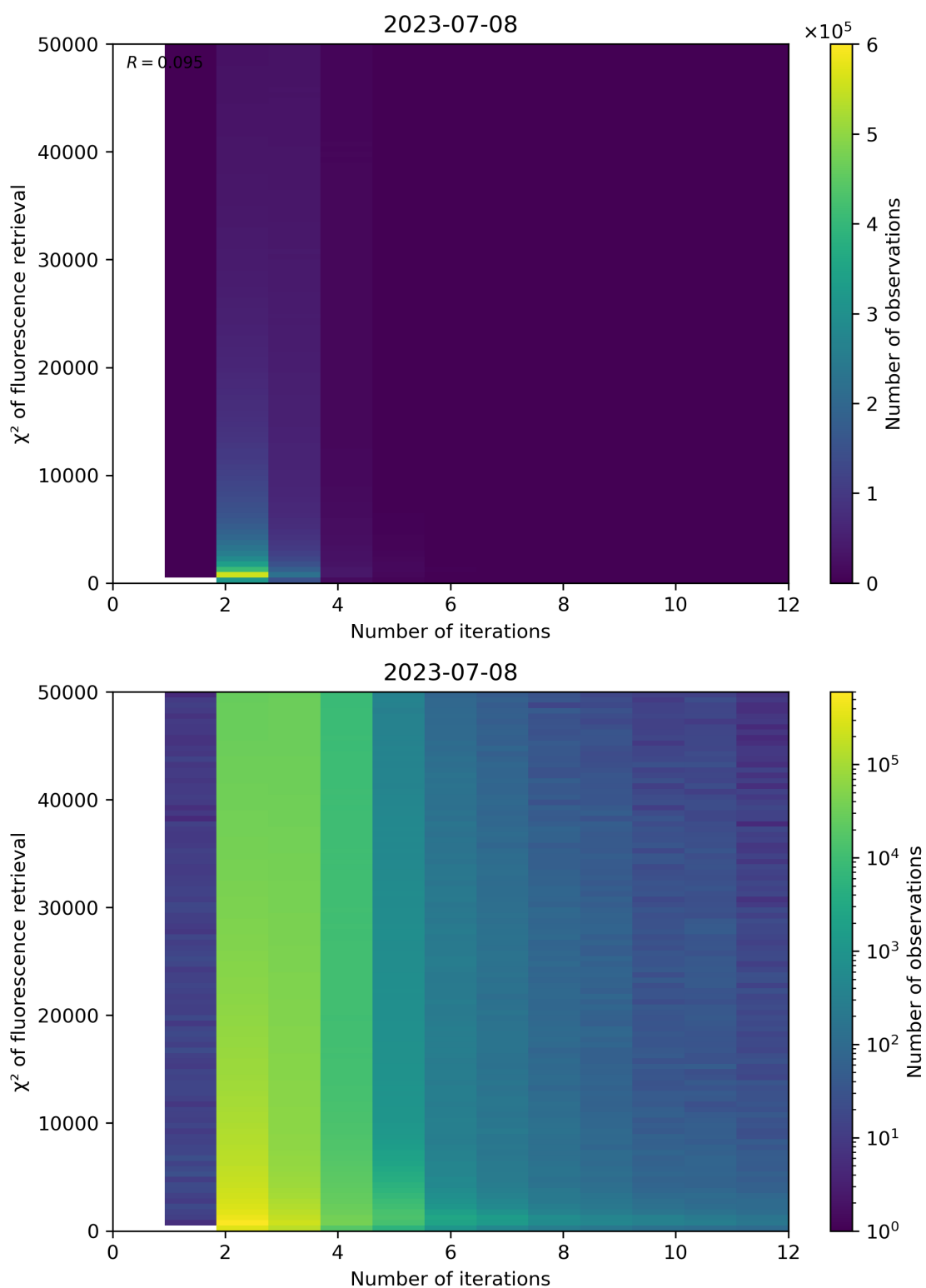
Figure 106: Scatter density plot of “Number of iterations” against “ \chi^2 of fluorescence retrieval” for 2023-07-08 to 2023-07-09.
