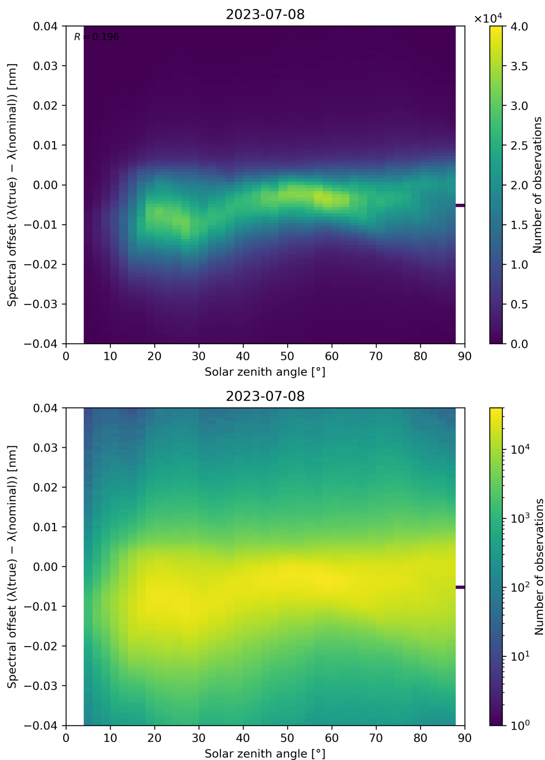
Figure 128: Scatter density plot of “Solar zenith angle” against “Spectral offset ( \lambda(\text{true}) - \lambda(\text{nominal}) )” for 2023-07-08 to 2023-07-09.
