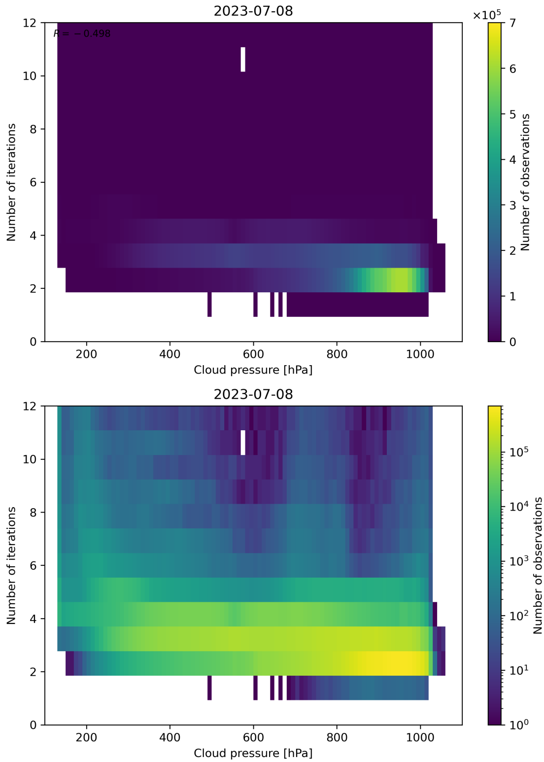
Figure 89: Scatter density plot of “Cloud pressure” against “Number of iterations” for 2023-07-08 to 2023-07-09.
