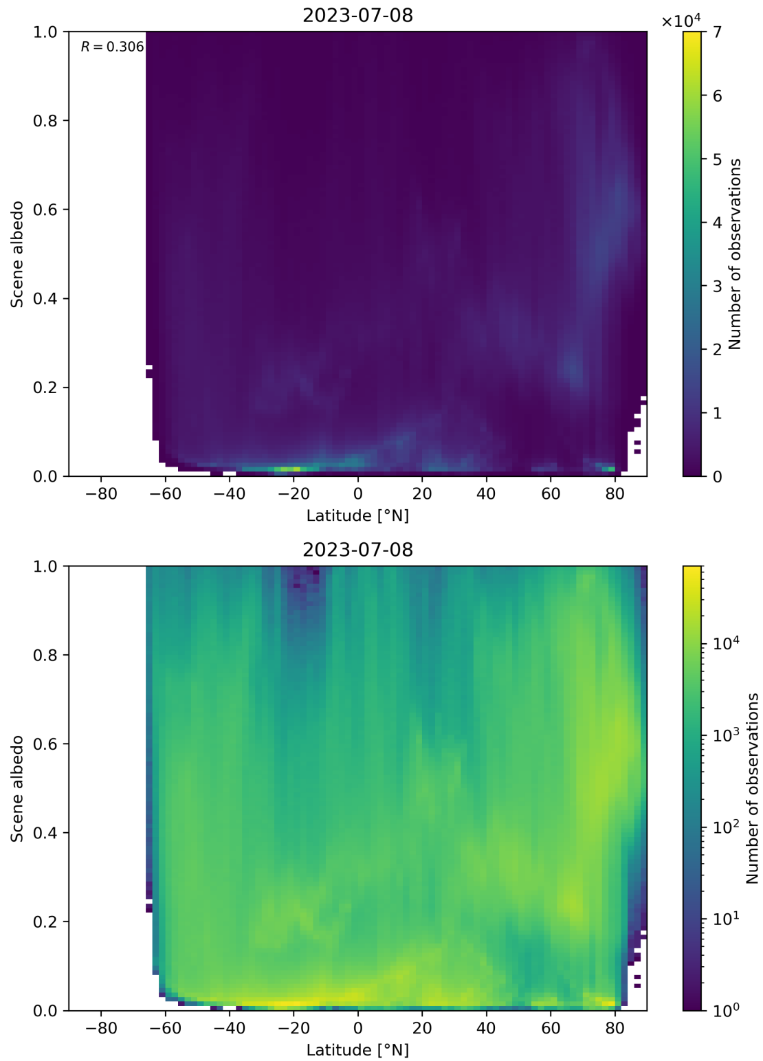
Figure 104: Scatter density plot of “Latitude” against “Scene albedo” for 2023-07-08 to 2023-07-09.
