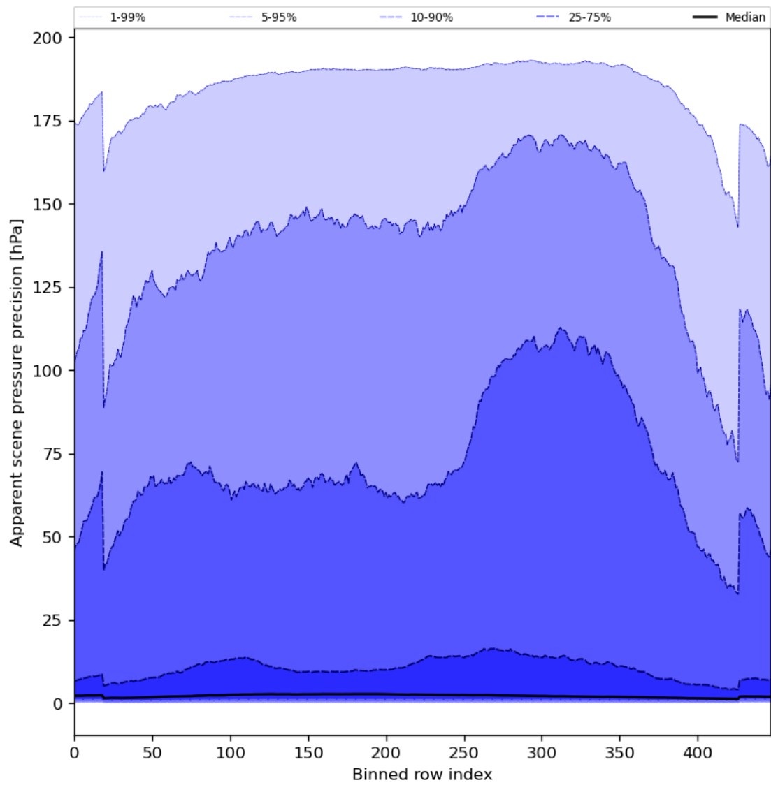
Figure 54: Along track statistics of “Apparent scene pressure precision” for 2023-07-08 to 2023-07-09
