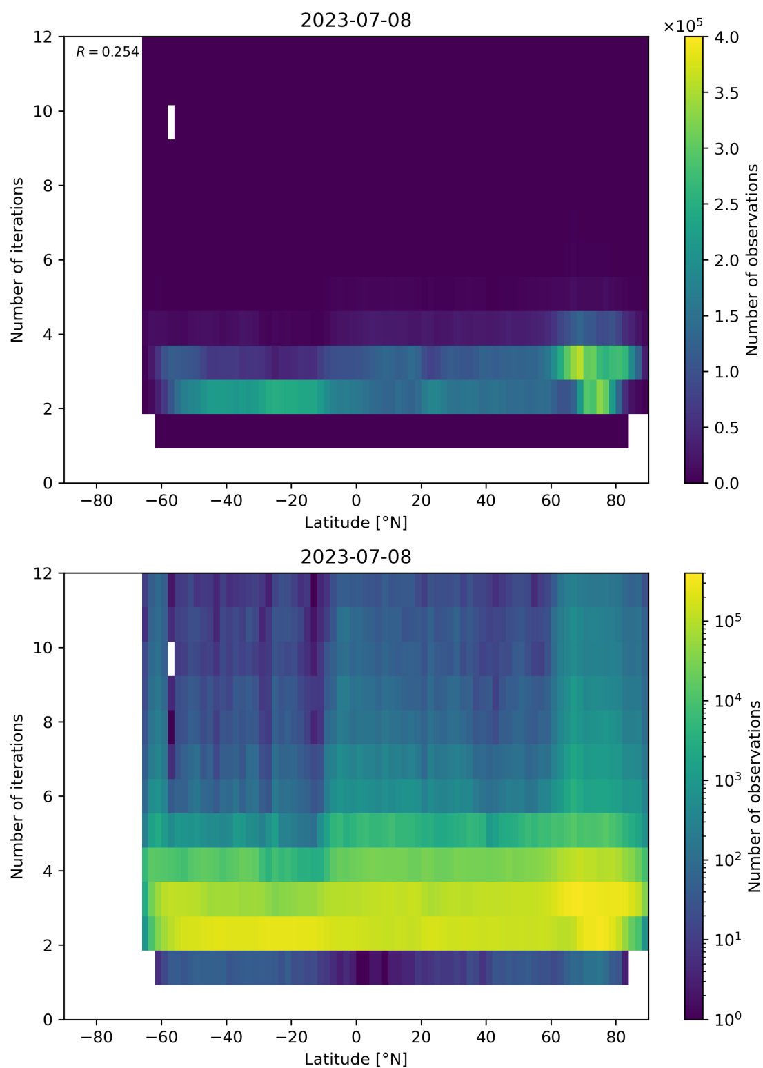
Figure 102: Scatter density plot of “Latitude” against “Number of iterations” for 2023-07-08 to 2023-07-09.
