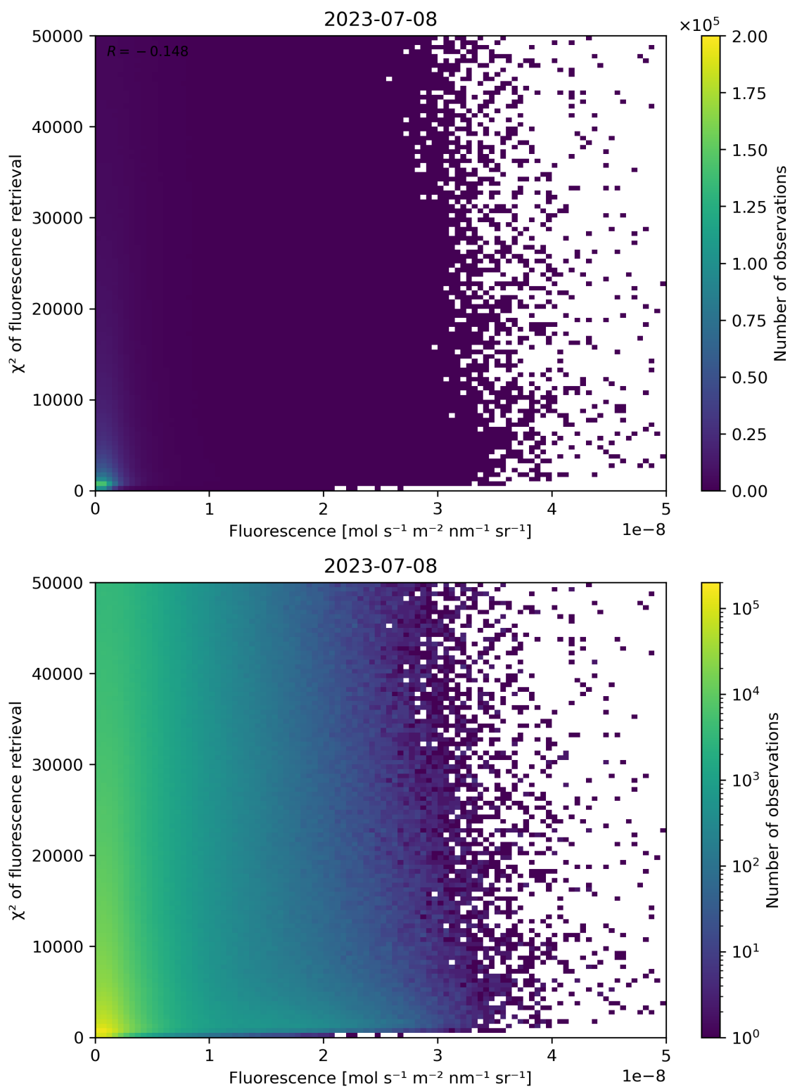
Figure 93: Scatter density plot of “Fluorescence” against “ \chi^2 of fluorescence retrieval” for 2023-07-08 to 2023-07-09.
