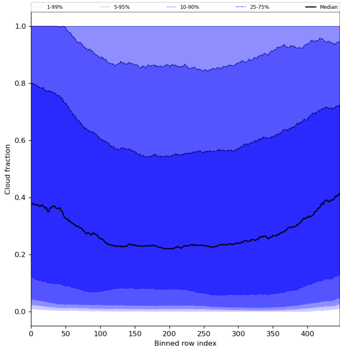
Figure 49: Along track statistics of “Cloud fraction” for 2023-07-08 to 2023-07-09
