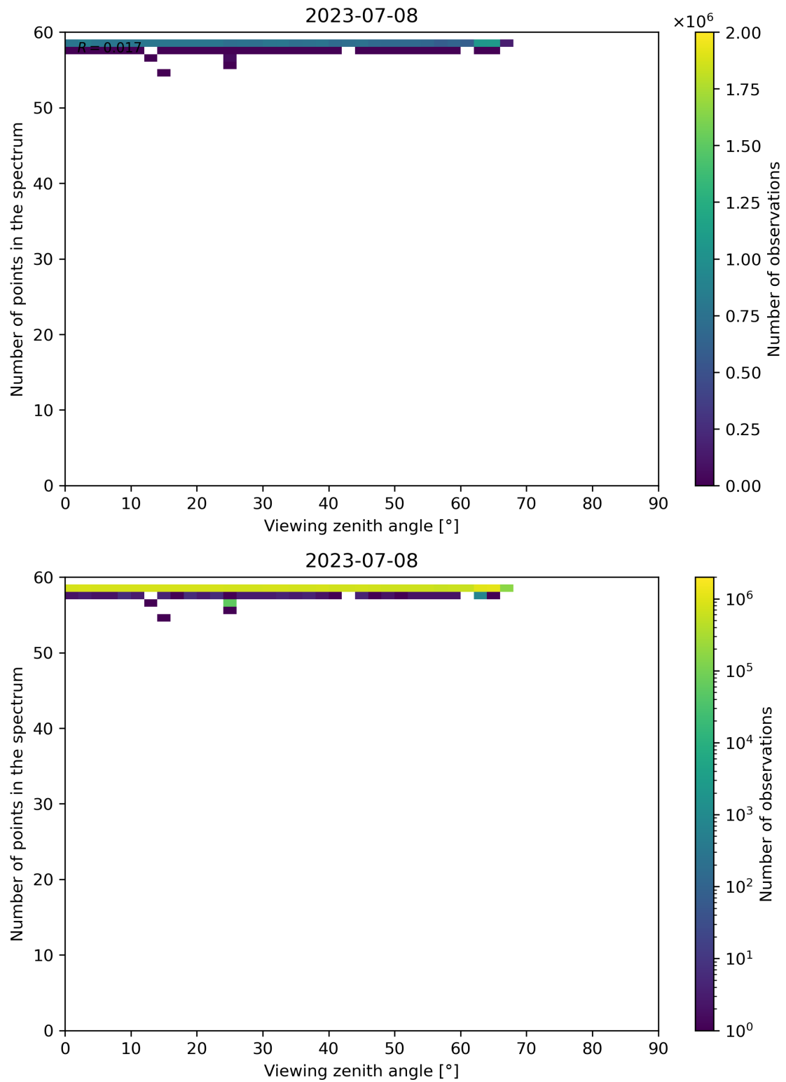
Figure 137: Scatter density plot of “Viewing zenith angle” against “Number of points in the spectrum” for 2023-07-08 to 2023-07-09.
