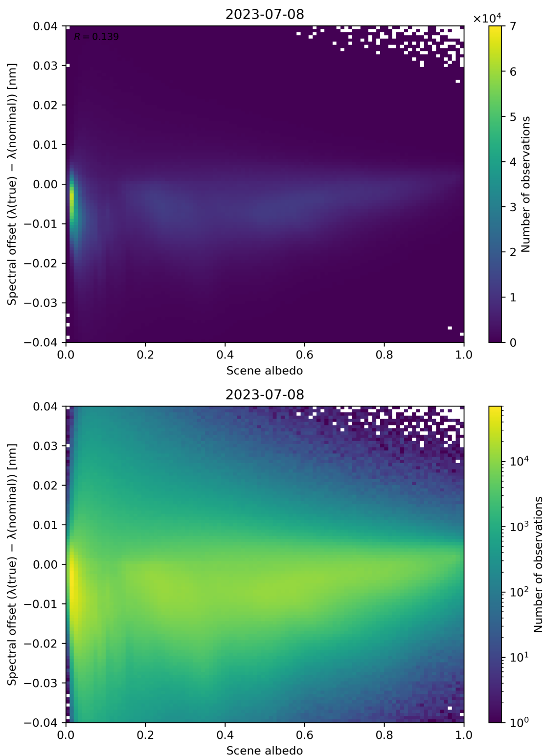
Figure 117: Scatter density plot of “Scene albedo” against “Spectral offset ( \lambda(\text{true}) - \lambda(\text{nominal}) )” for 2023-07-08 to 2023-07-09.
