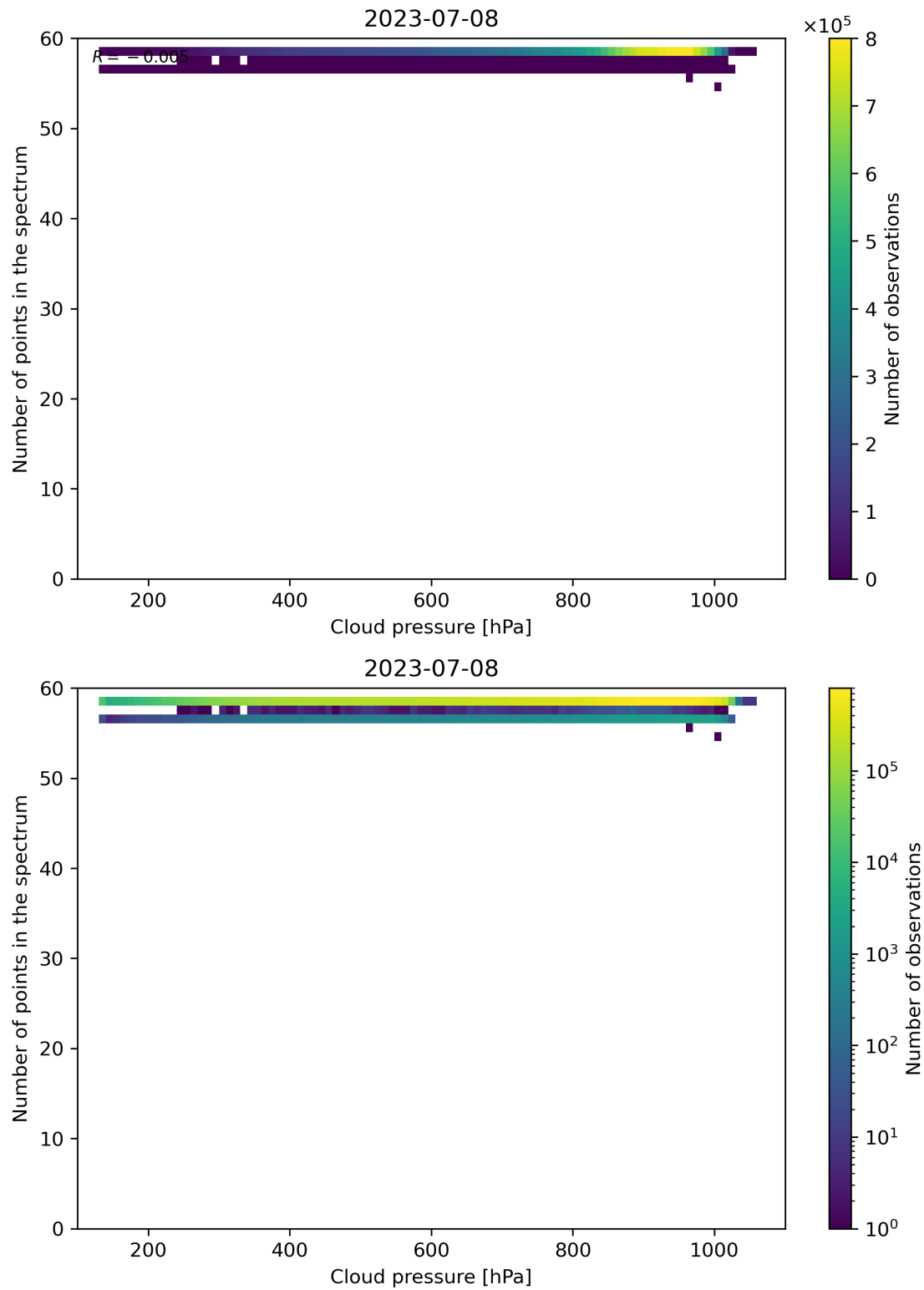
Figure 90: Scatter density plot of “Cloud pressure” against “Number of points in the spectrum” for 2023-07-08 to 2023-07-09.
