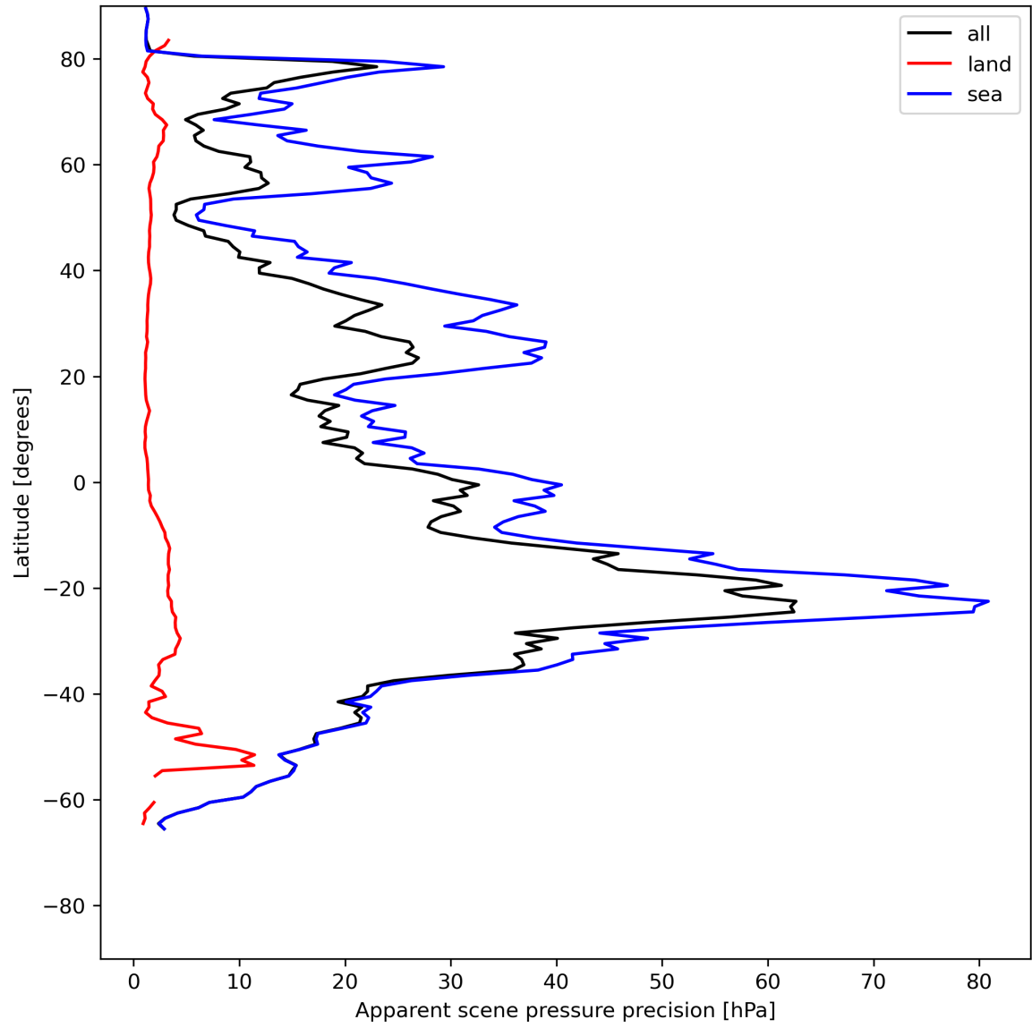
Figure 20: Zonal average of “Apparent scene pressure precision” for 2023-07-08 to 2023-07-09.
