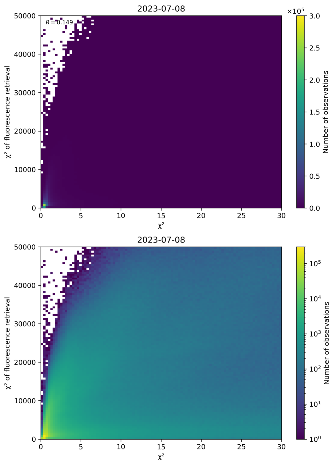
Figure 69: Scatter density plot of “ \chi^2 ” against “ \chi^2 of fluorescence retrieval” for 2023-07-08 to 2023-07-09.
