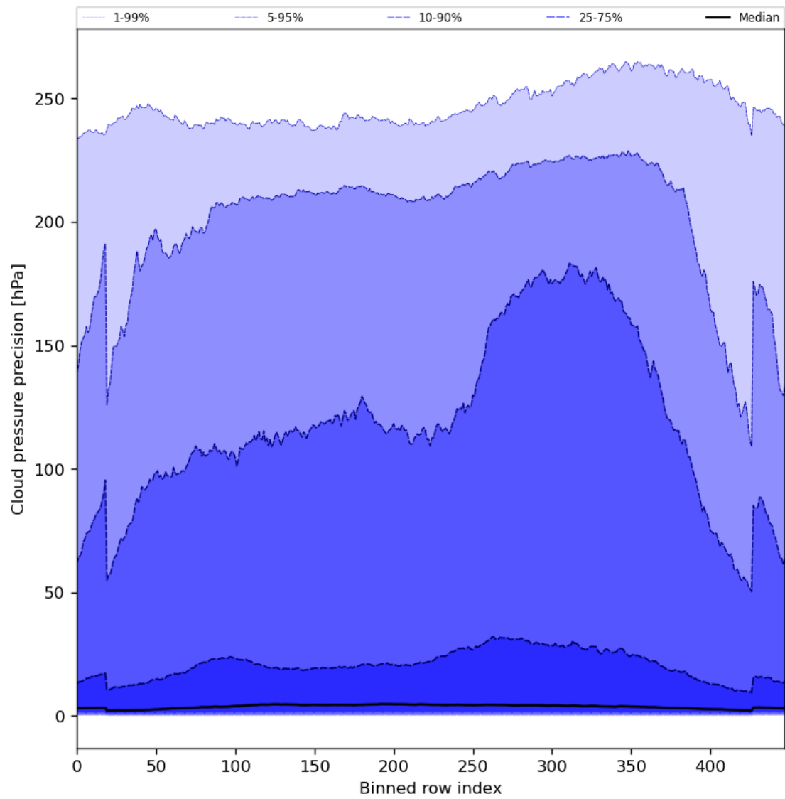
Figure 48: Along track statistics of “Cloud pressure precision” for 2023-07-08 to 2023-07-09
