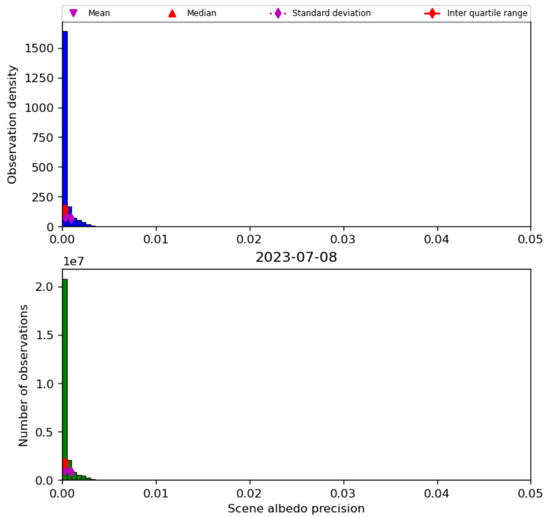
Figure 35: Histogram of “Scene albedo precision” for 2023-07-08 to 2023-07-09
