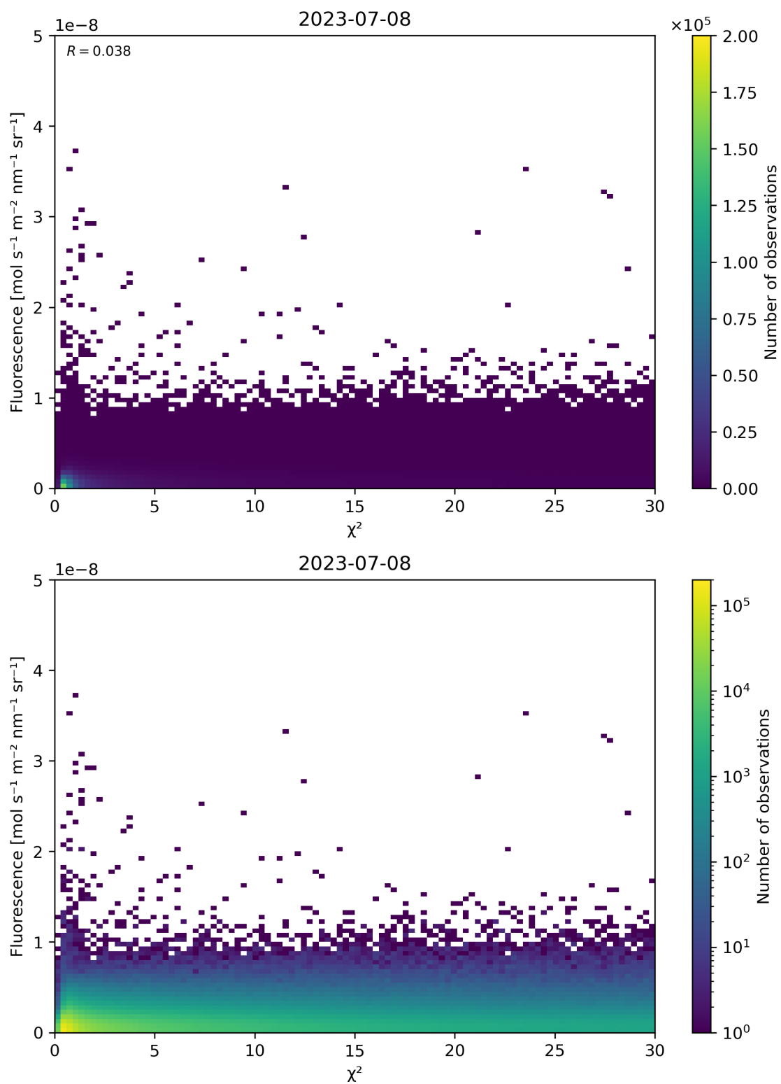
Figure 70: Scatter density plot of “ \chi^2 ” against “Fluorescence” for 2023-07-08 to 2023-07-09.
