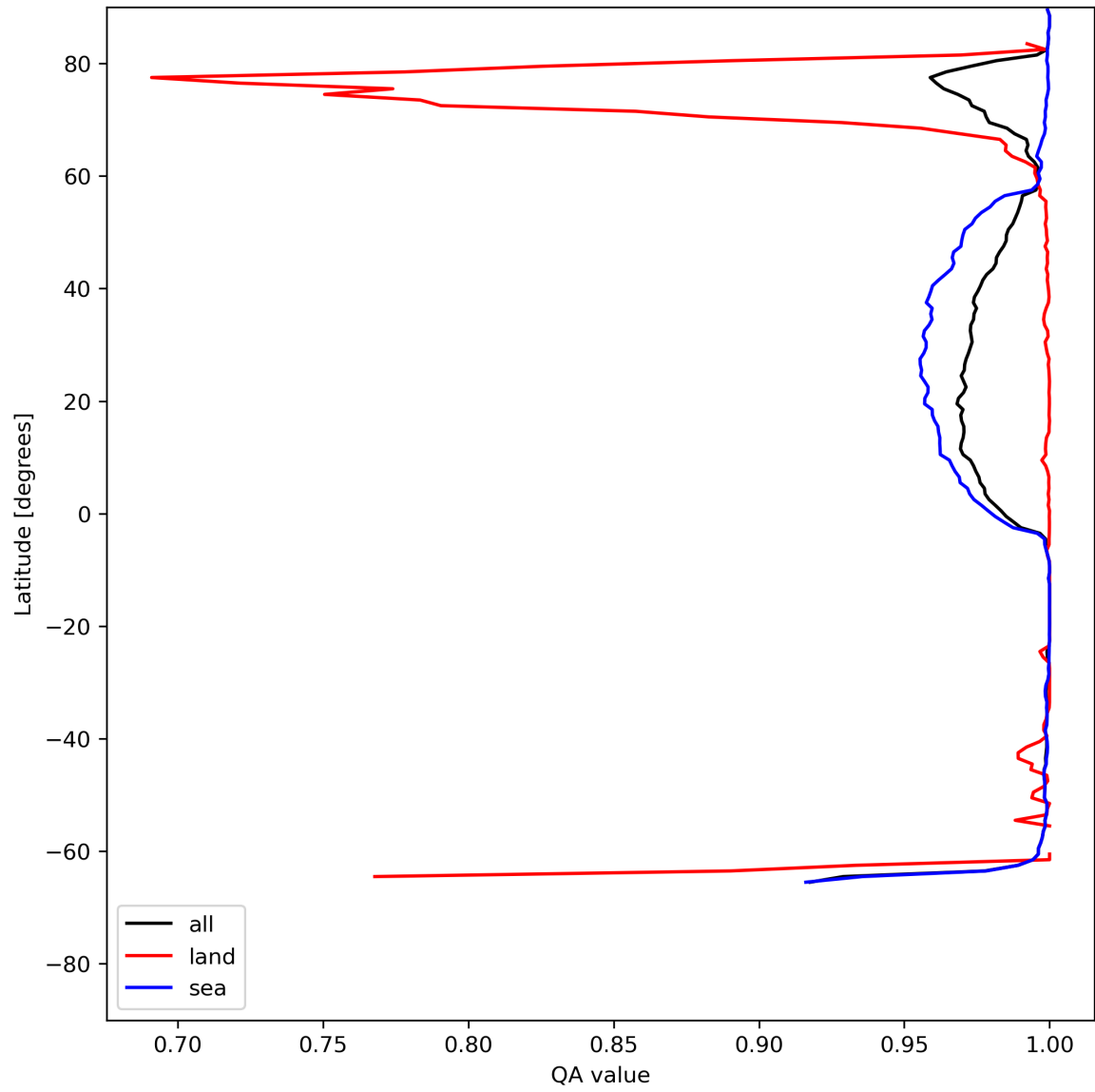
Figure 12: Zonal average of “QA value” for 2023-07-08 to 2023-07-09.
