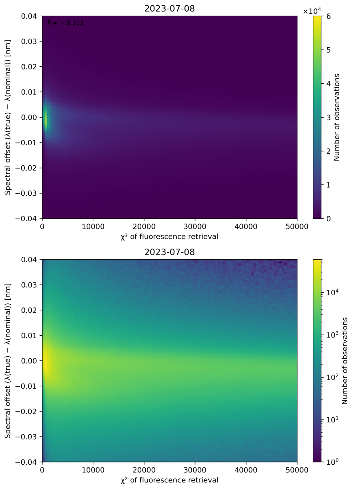
Figure 72: Scatter density plot of " \chi^2 of fluorescence retrieval" against "Spectral offset ( \lambda(\text{true}) - \lambda(\text{nominal})) " for 2023-07-08 to 2023-07-09.
