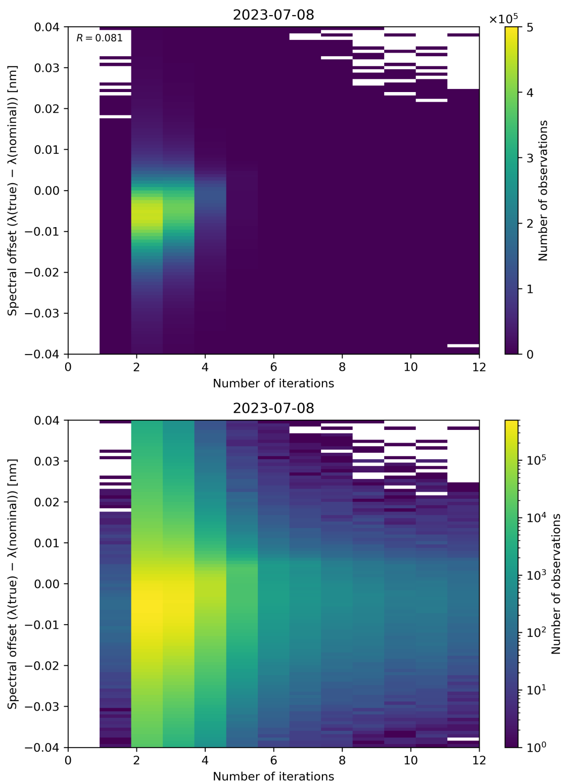
Figure 109: Scatter density plot of “Number of iterations” against “Spectral offset ( \lambda(\text{true}) - \lambda(\text{nominal}) )” for 2023-07-08 to 2023-07-09.
