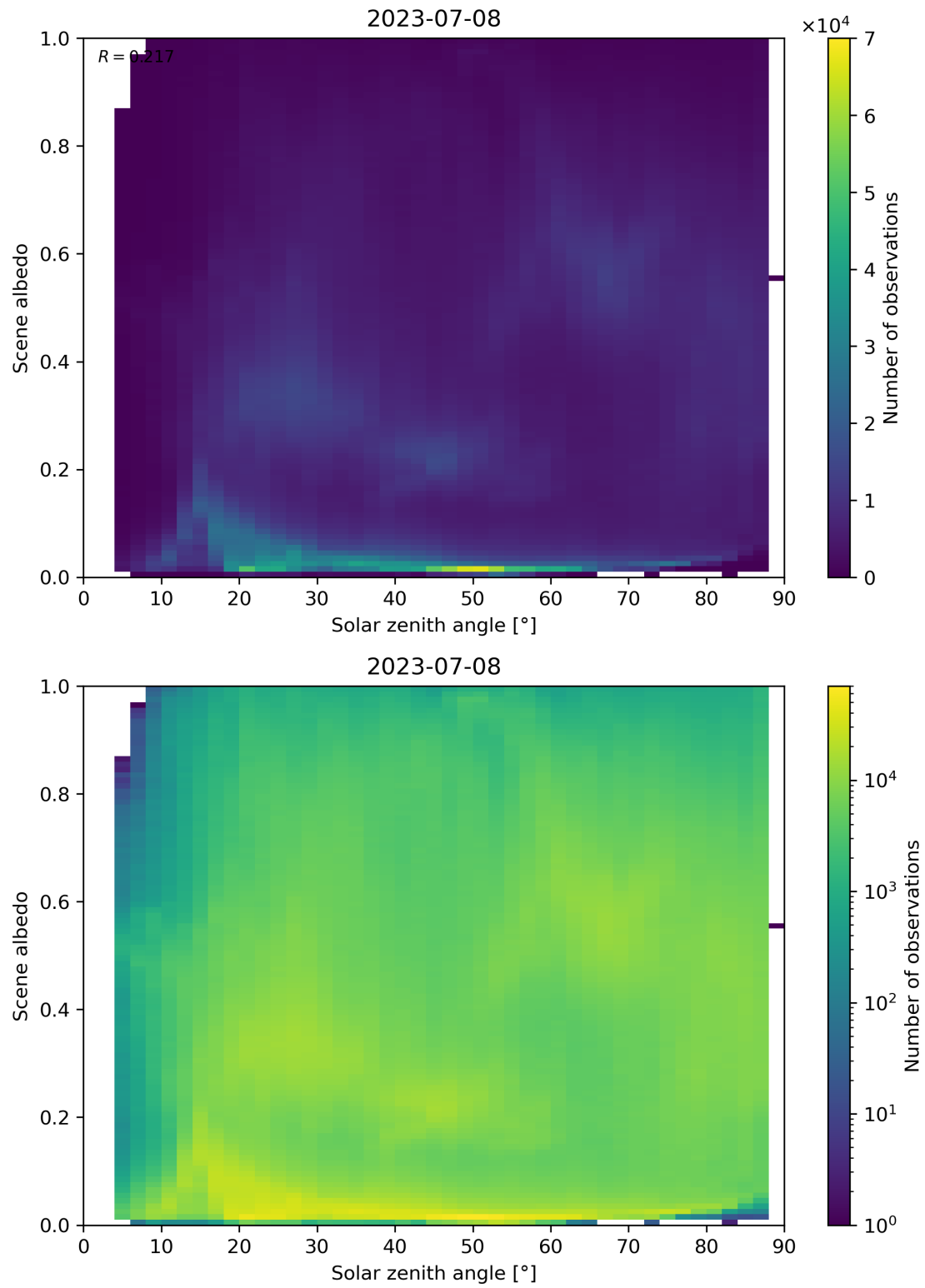
Figure 127: Scatter density plot of “Solar zenith angle” against “Scene albedo” for 2023-07-08 to 2023-07-09.
