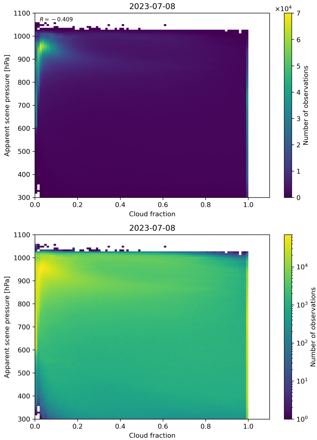
Figure 76: Scatter density plot of “Cloud fraction” against “Apparent scene pressure” for 2023-07-08 to 2023-07-09.
