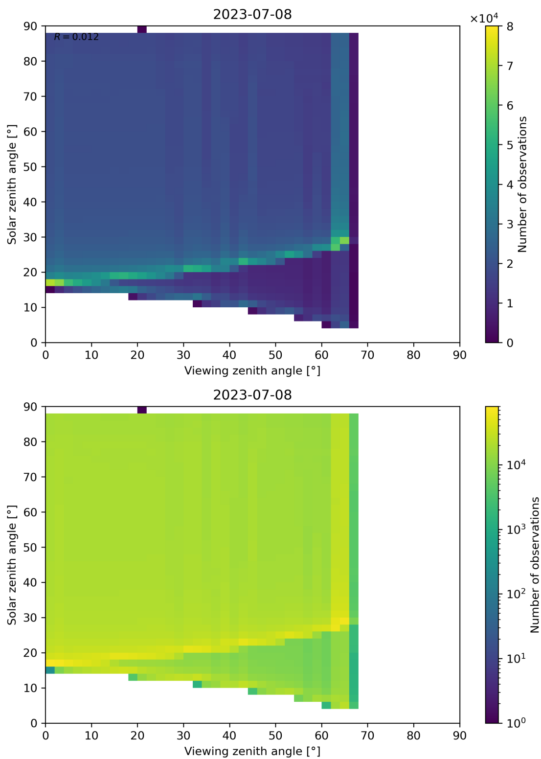
Figure 139: Scatter density plot of “Viewing zenith angle” against “Solar zenith angle” for 2023-07-08 to 2023-07-09.
