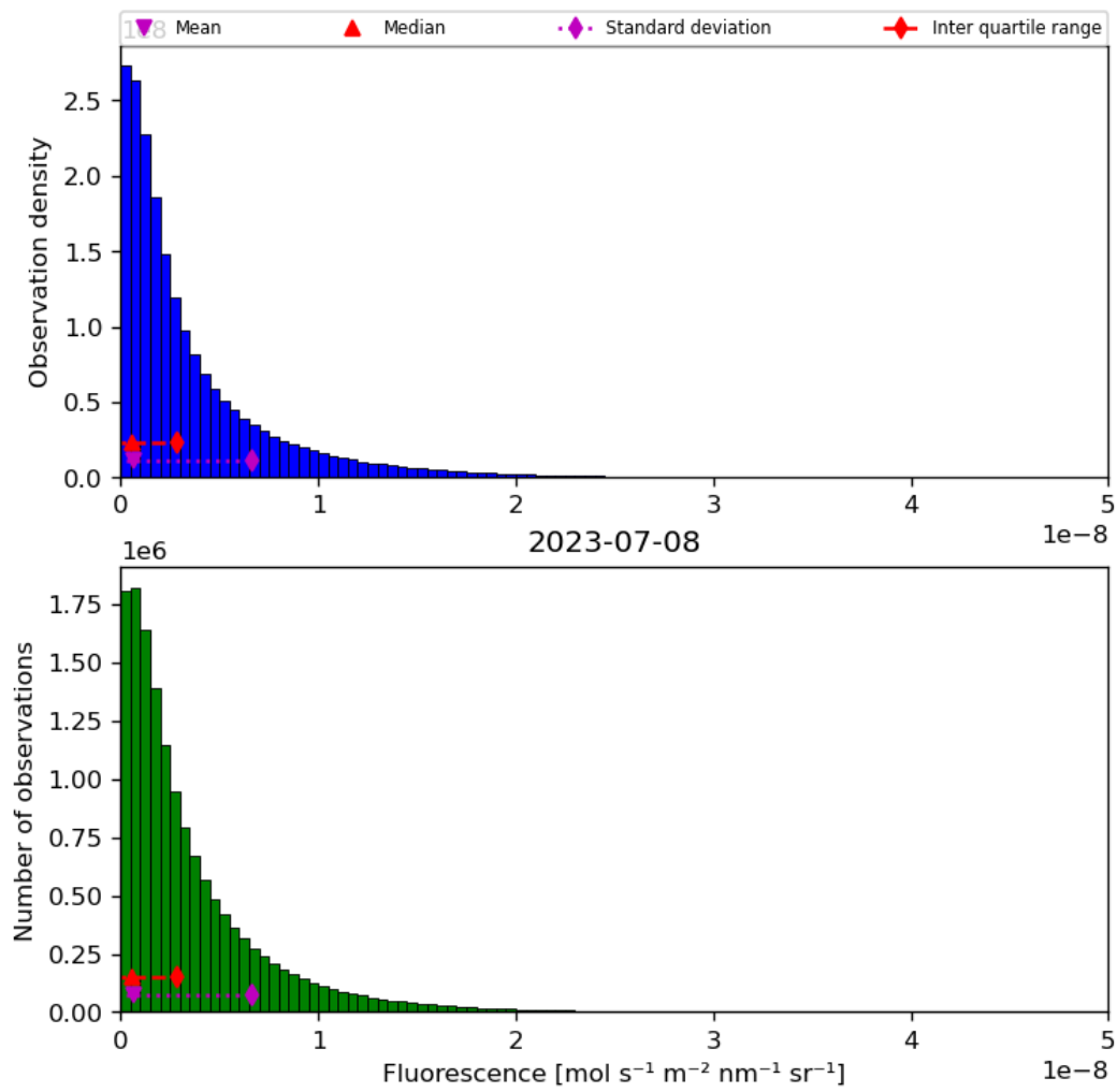
Figure 40: Histogram of “Fluorescence” for 2023-07-08 to 2023-07-09
