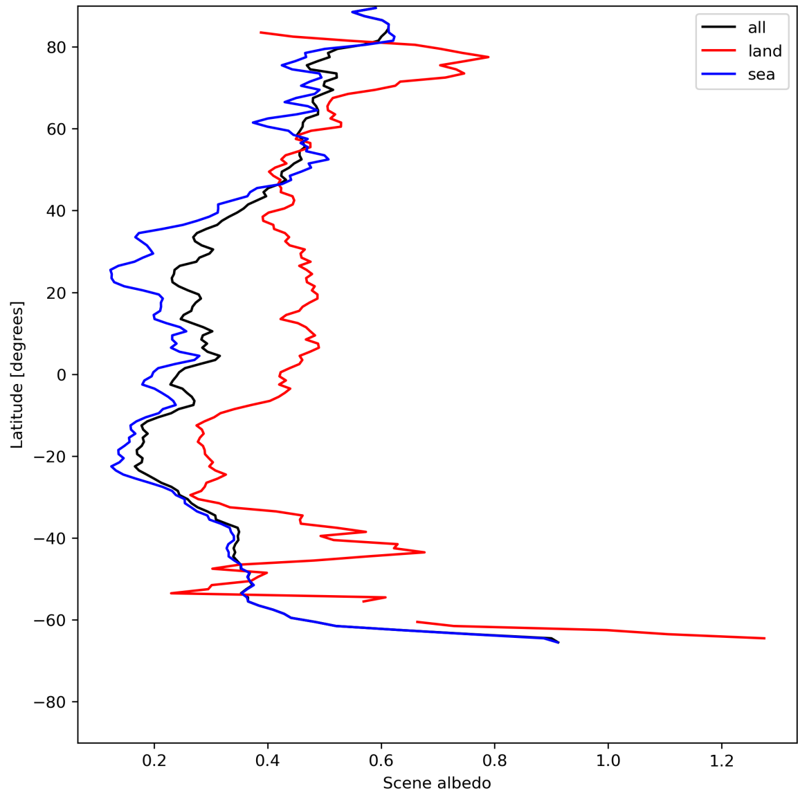
Figure 17: Zonal average of “Scene albedo” for 2023-07-08 to 2023-07-09.
