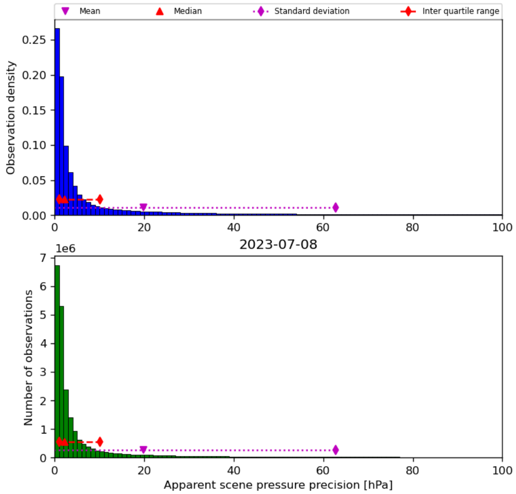
Figure 37: Histogram of “Apparent scene pressure precision” for 2023-07-08 to 2023-07-09
