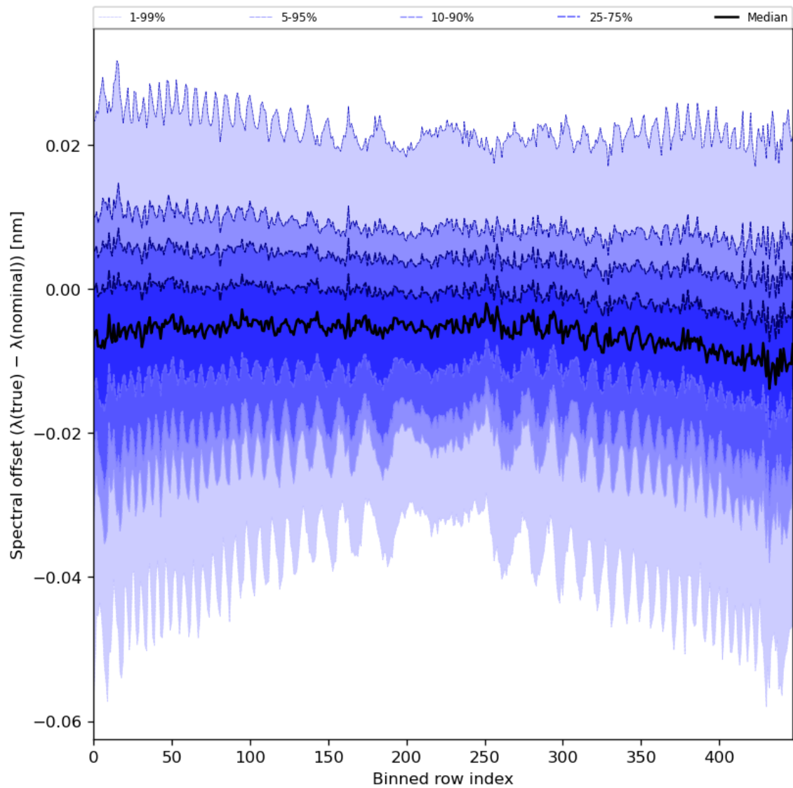
Figure 62: Along track statistics of “Spectral offset ( \lambda(\text{true}) - \lambda(\text{nominal}) )” for 2023-07-08 to 2023-07-09
