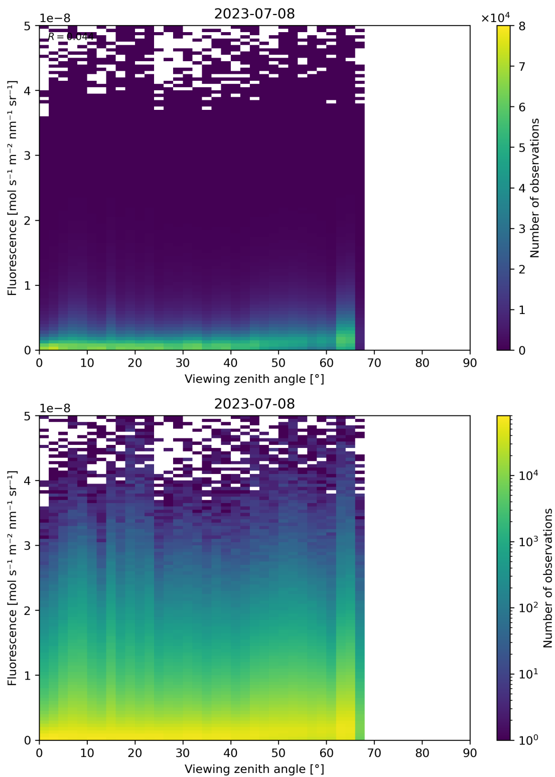
Figure 134: Scatter density plot of “Viewing zenith angle” against “Fluorescence” for 2023-07-08 to 2023-07-09.
