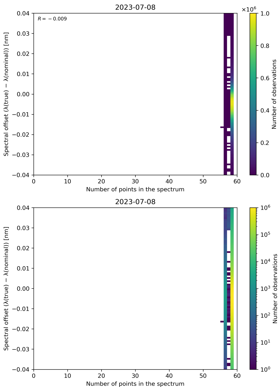
Figure 110: Scatter density plot of “Number of points in the spectrum” against “Spectral offset ( \lambda(\text{true}) - \lambda(\text{nominal}) )” for 2023-07-08 to 2023-07-09.
