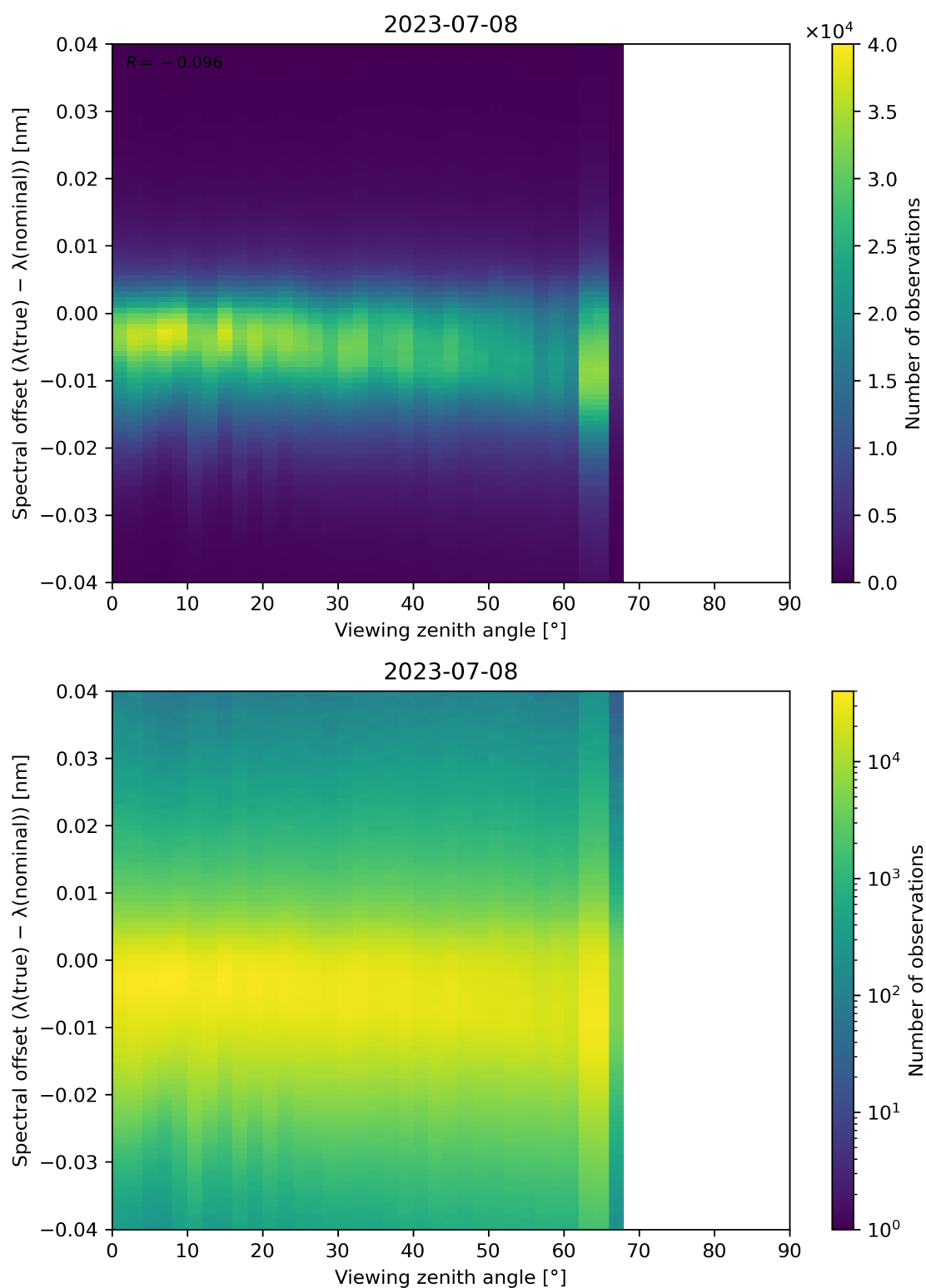
Figure 140: Scatter density plot of “Viewing zenith angle” against “Spectral offset ( \lambda(\text{true}) - \lambda(\text{nominal}) )” for 2023-07-08 to 2023-07-09.
