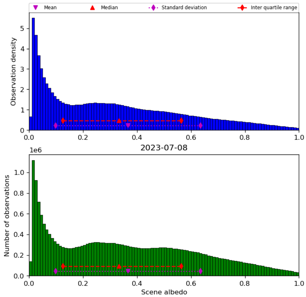
Figure 34: Histogram of “Scene albedo” for 2023-07-08 to 2023-07-09
