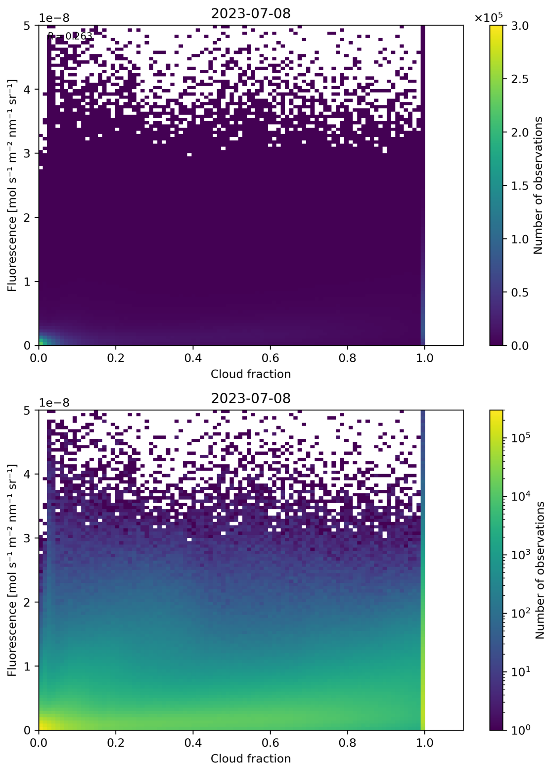
Figure 79: Scatter density plot of “Cloud fraction” against “Fluorescence” for 2023-07-08 to 2023-07-09.
