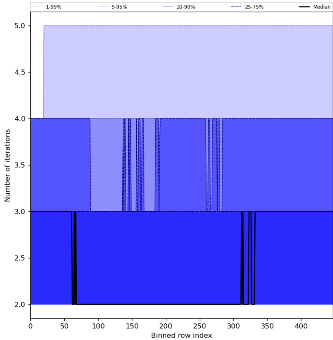
Figure 56: Along track statistics of “Number of iterations” for 2023-07-08 to 2023-07-09
