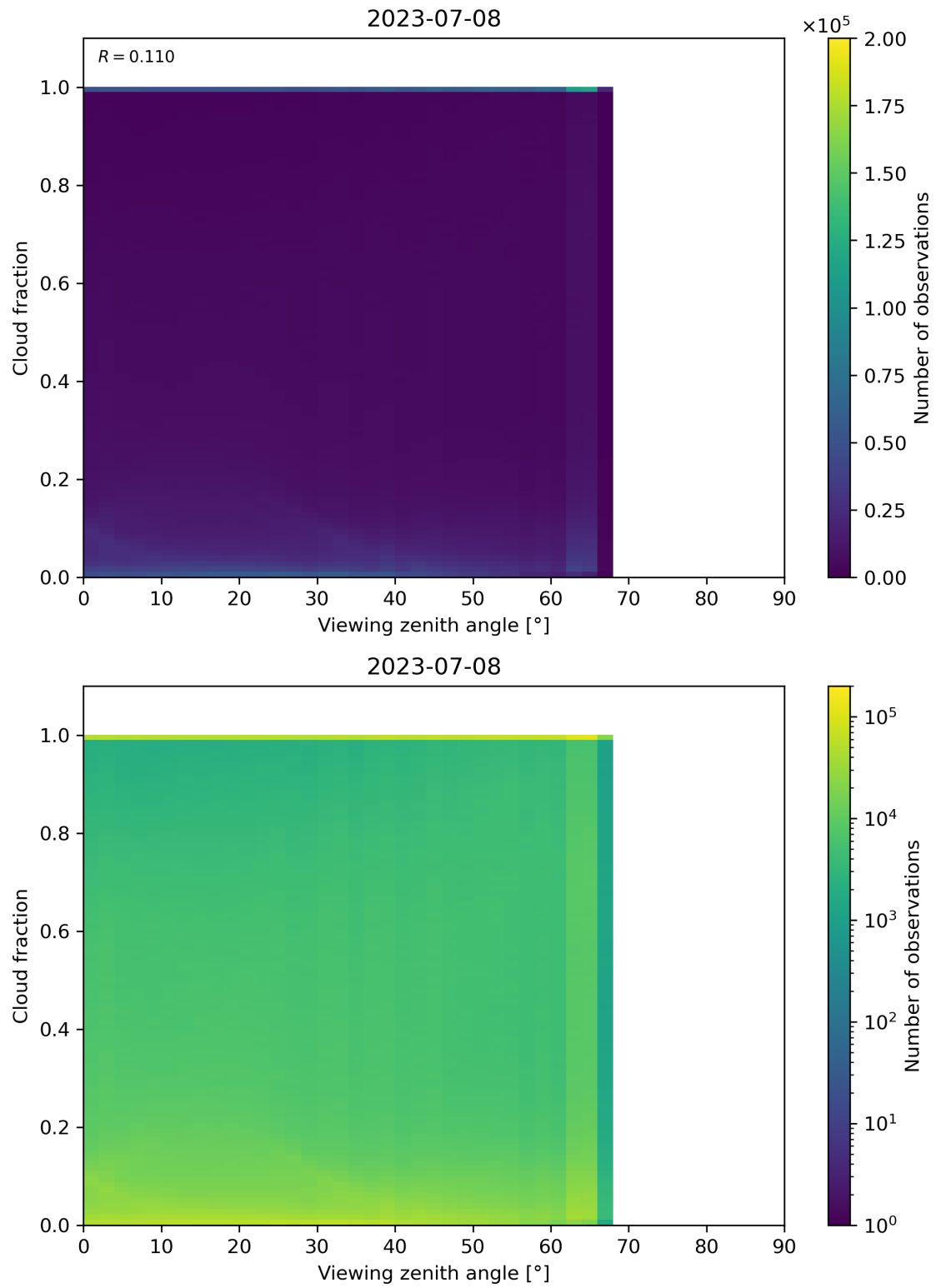
Figure 132: Scatter density plot of “Viewing zenith angle” against “Cloud fraction” for 2023-07-08 to 2023-07-09.
