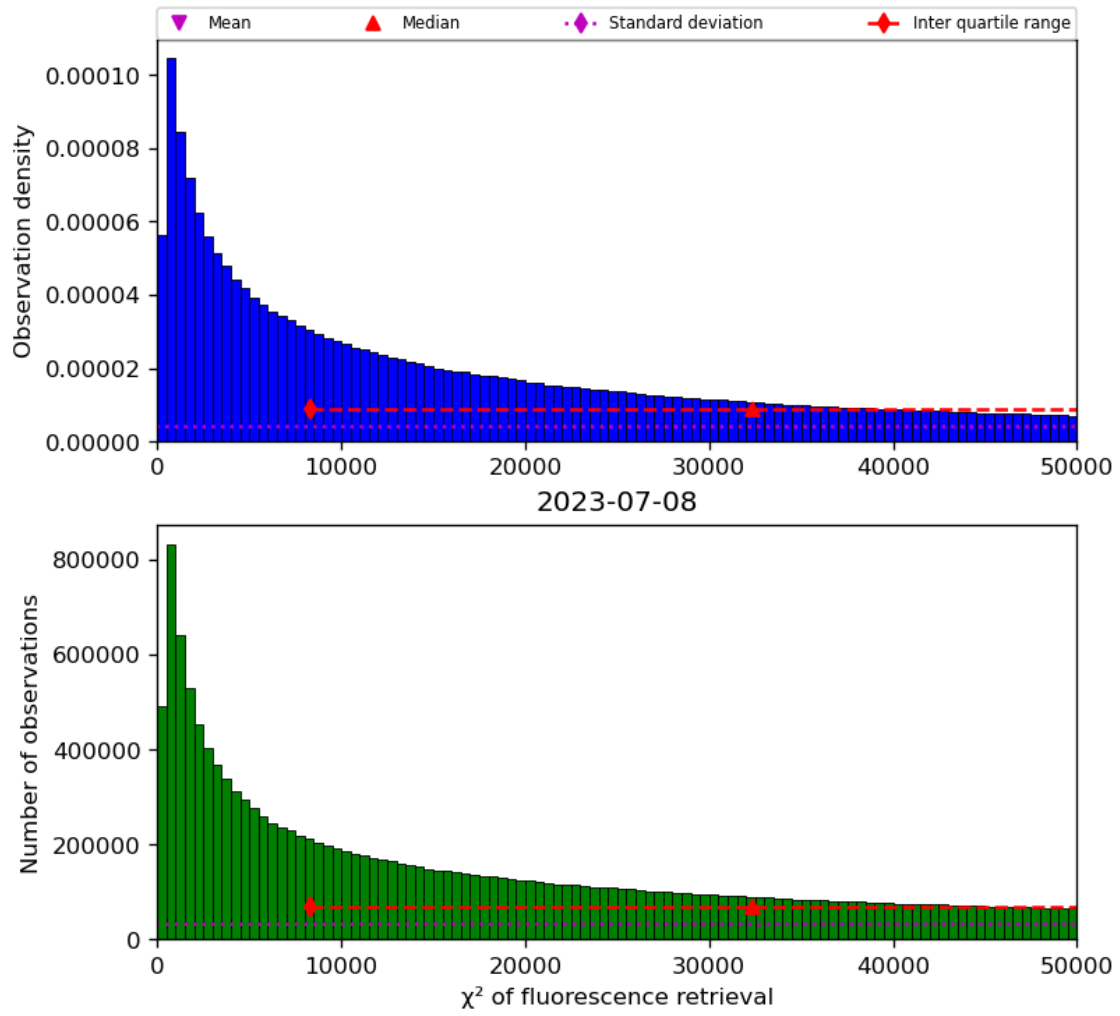
Figure 42: Histogram of “ \chi^2 of fluorescence retrieval” for 2023-07-08 to 2023-07-09
