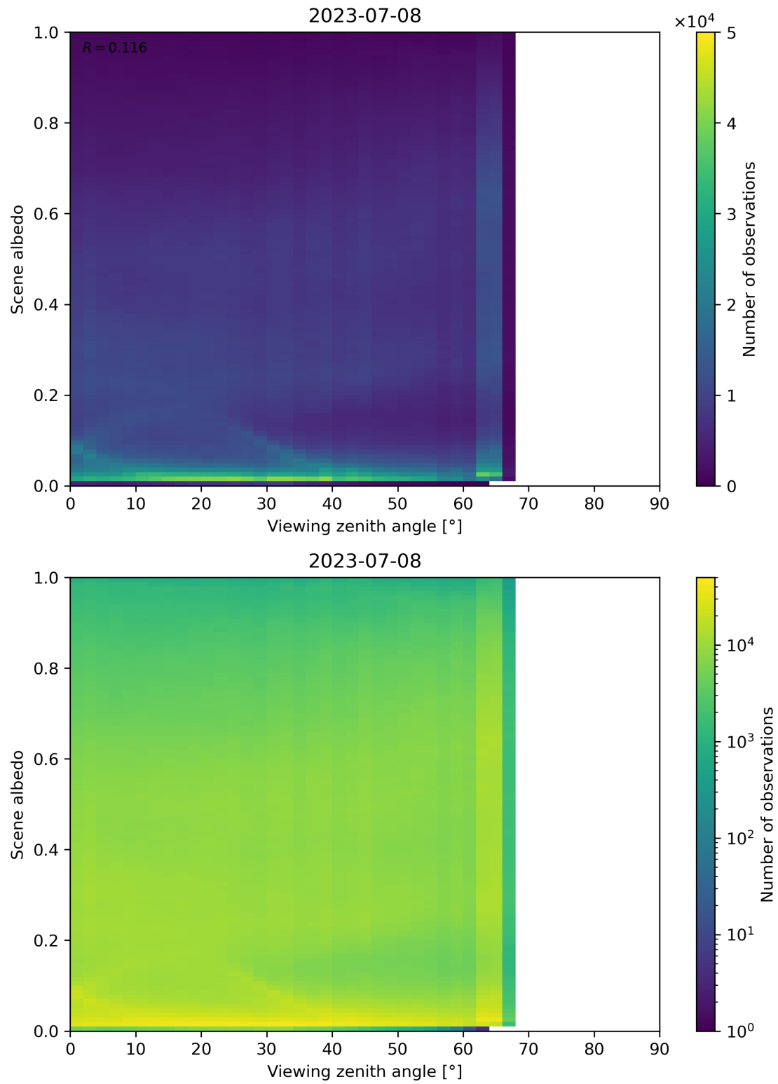
Figure 138: Scatter density plot of “Viewing zenith angle” against “Scene albedo” for 2023-07-08 to 2023-07-09.
