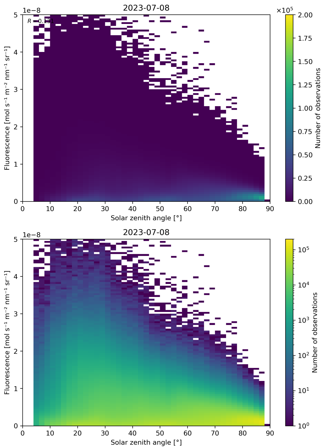
Figure 123: Scatter density plot of “Solar zenith angle” against “Fluorescence” for 2023-07-08 to 2023-07-09.
