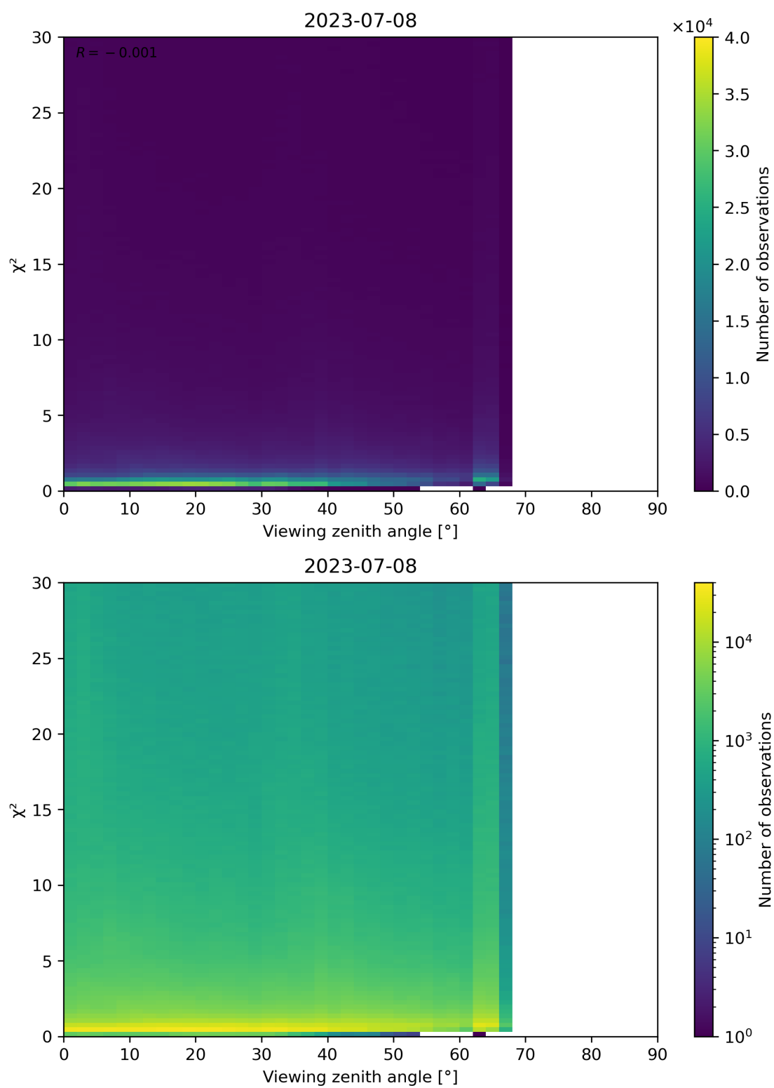
Figure 130: Scatter density plot of “Viewing zenith angle” against “ \chi^2 ” for 2023-07-08 to 2023-07-09.
