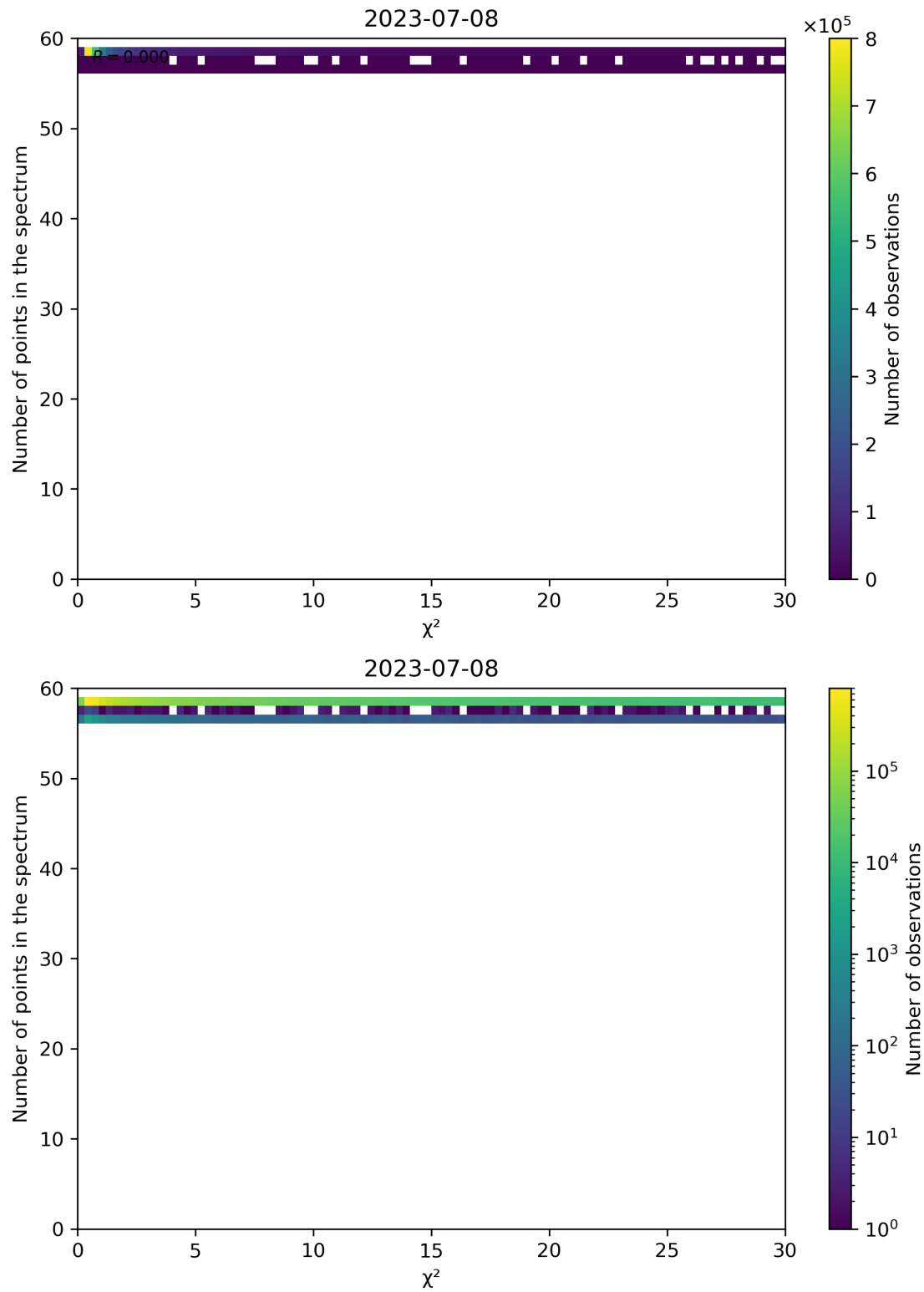
Figure 74: Scatter density plot of “ \chi^2 ” against “Number of points in the spectrum” for 2023-07-08 to 2023-07-09.
