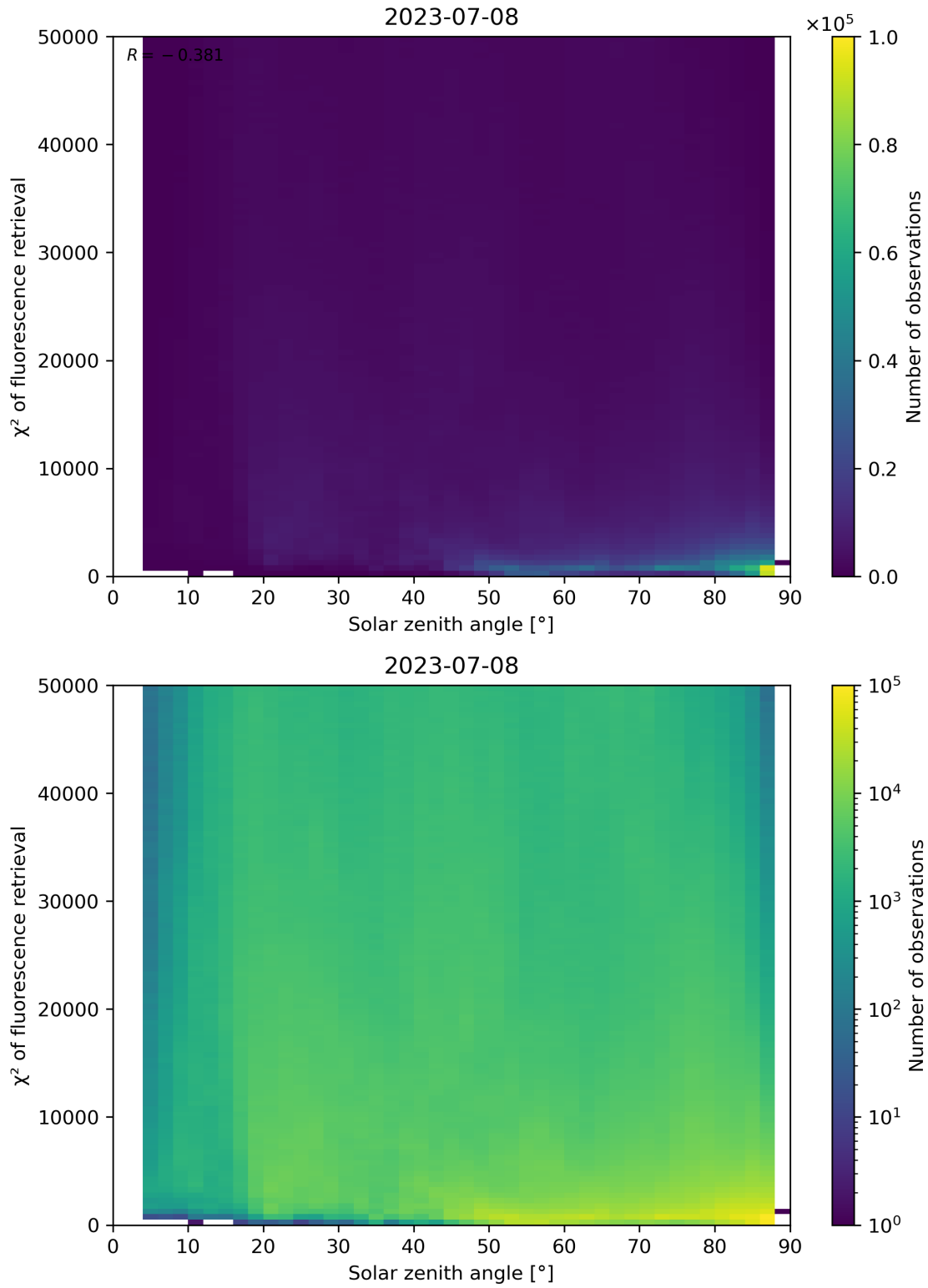
Figure 120: Scatter density plot of “Solar zenith angle” against “ \chi^2 of fluorescence retrieval” for 2023-07-08 to 2023-07-09.
