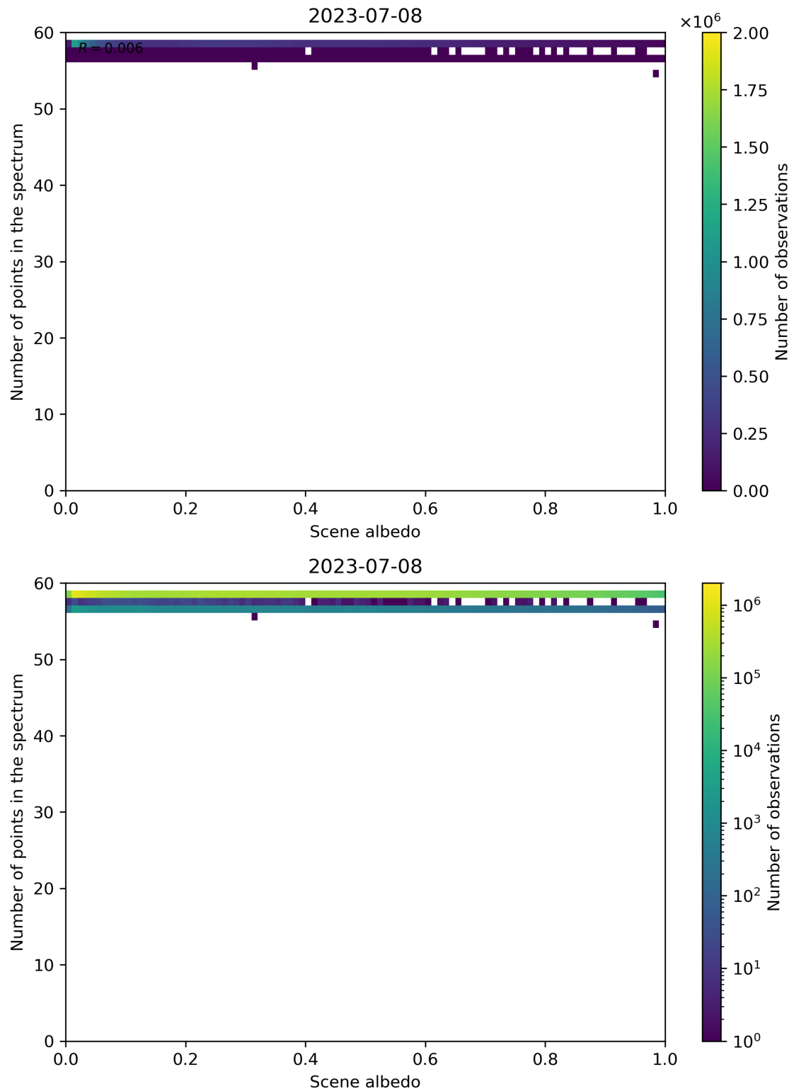
Figure 116: Scatter density plot of “Scene albedo” against “Number of points in the spectrum” for 2023-07-08 to 2023-07-09.
