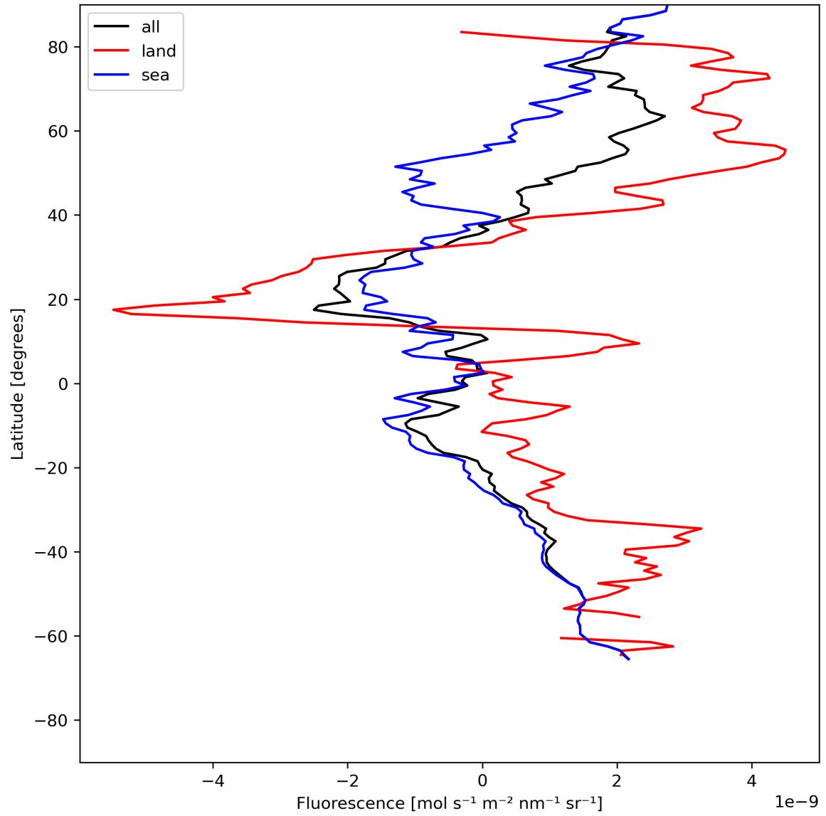
Figure 23: Zonal average of “Fluorescence” for 2023-07-08 to 2023-07-09.
