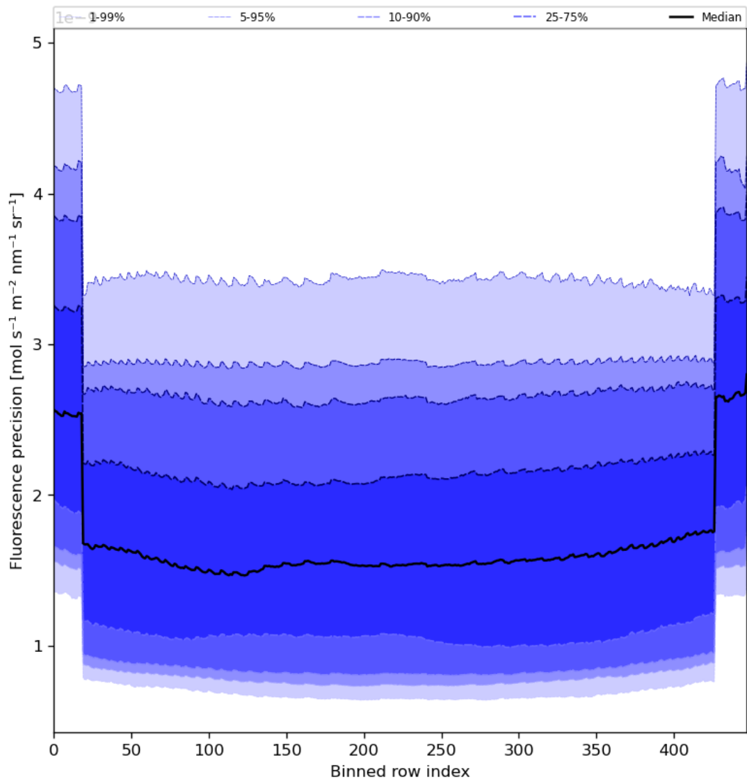
Figure 58: Along track statistics of “Fluorescence precision” for 2023-07-08 to 2023-07-09
