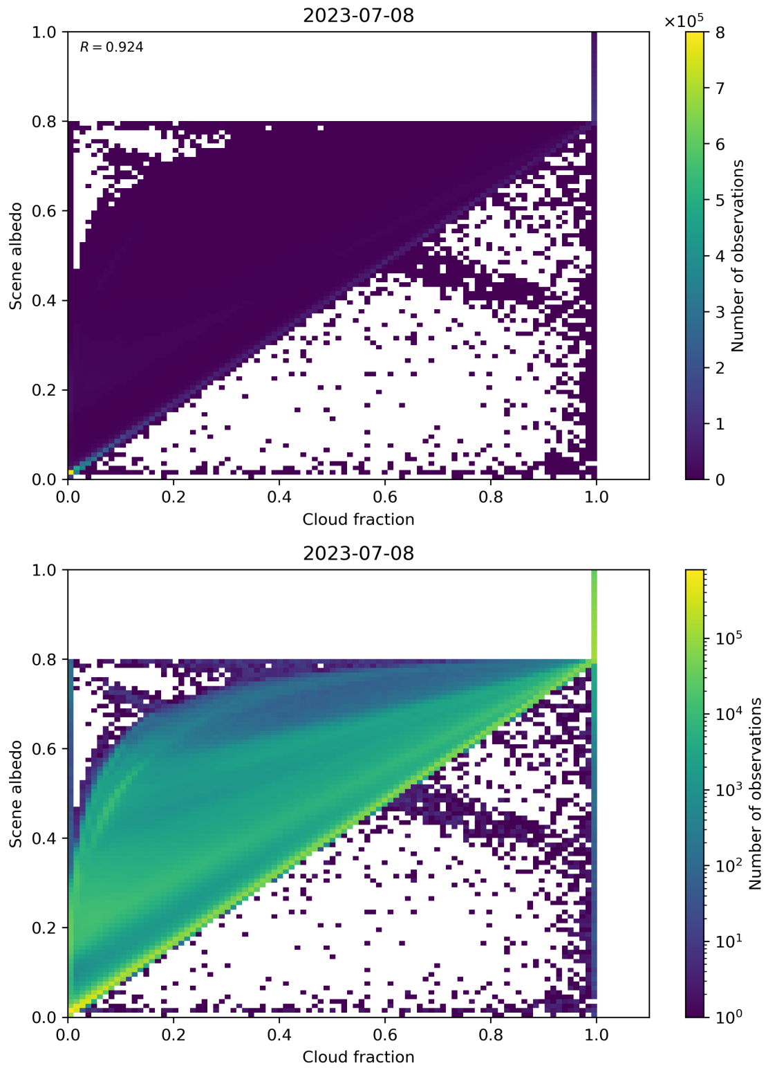
Figure 82: Scatter density plot of “Cloud fraction” against “Scene albedo” for 2023-07-08 to 2023-07-09.
