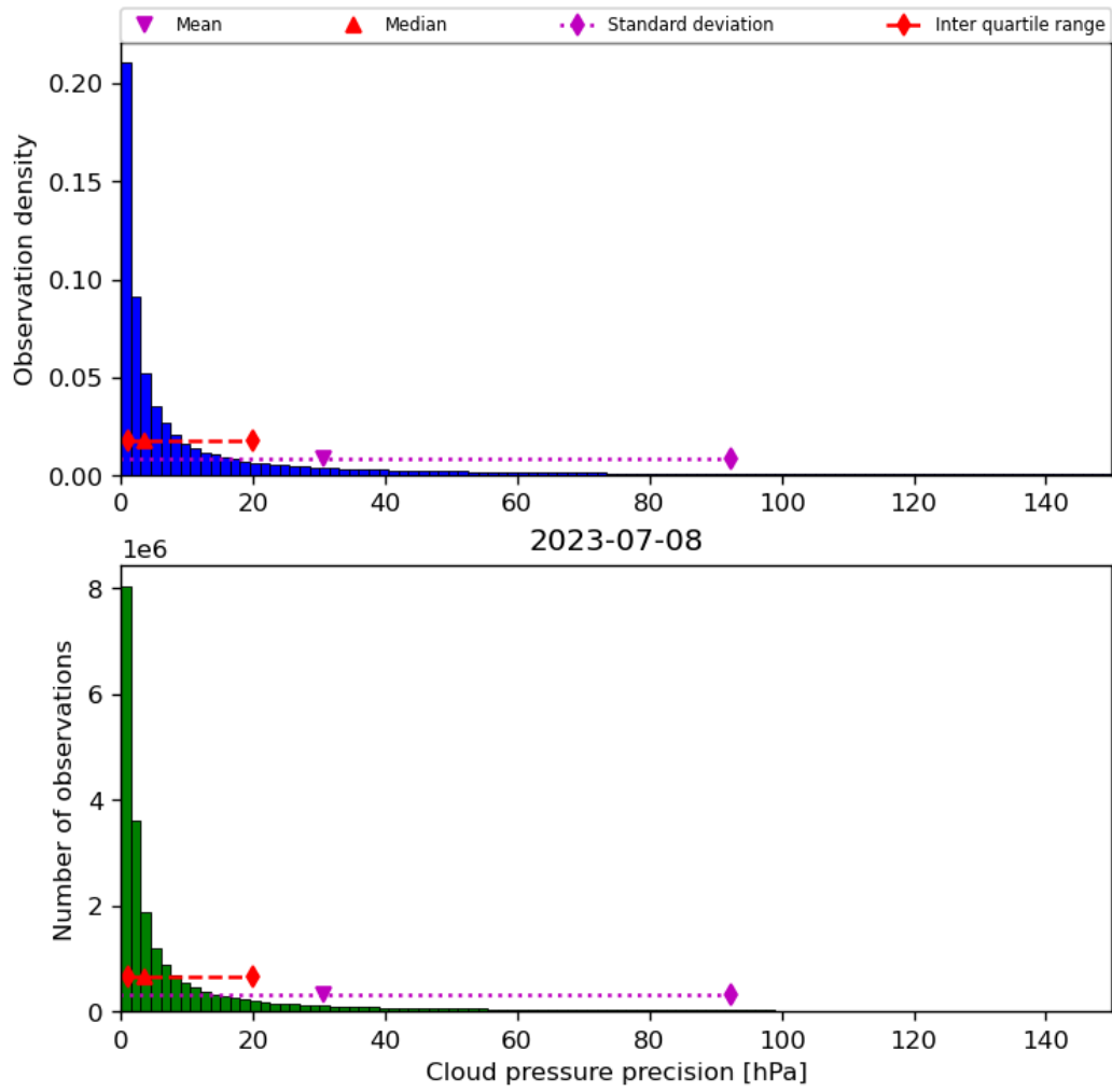
Figure 31: Histogram of “Cloud pressure precision” for 2023-07-08 to 2023-07-09
