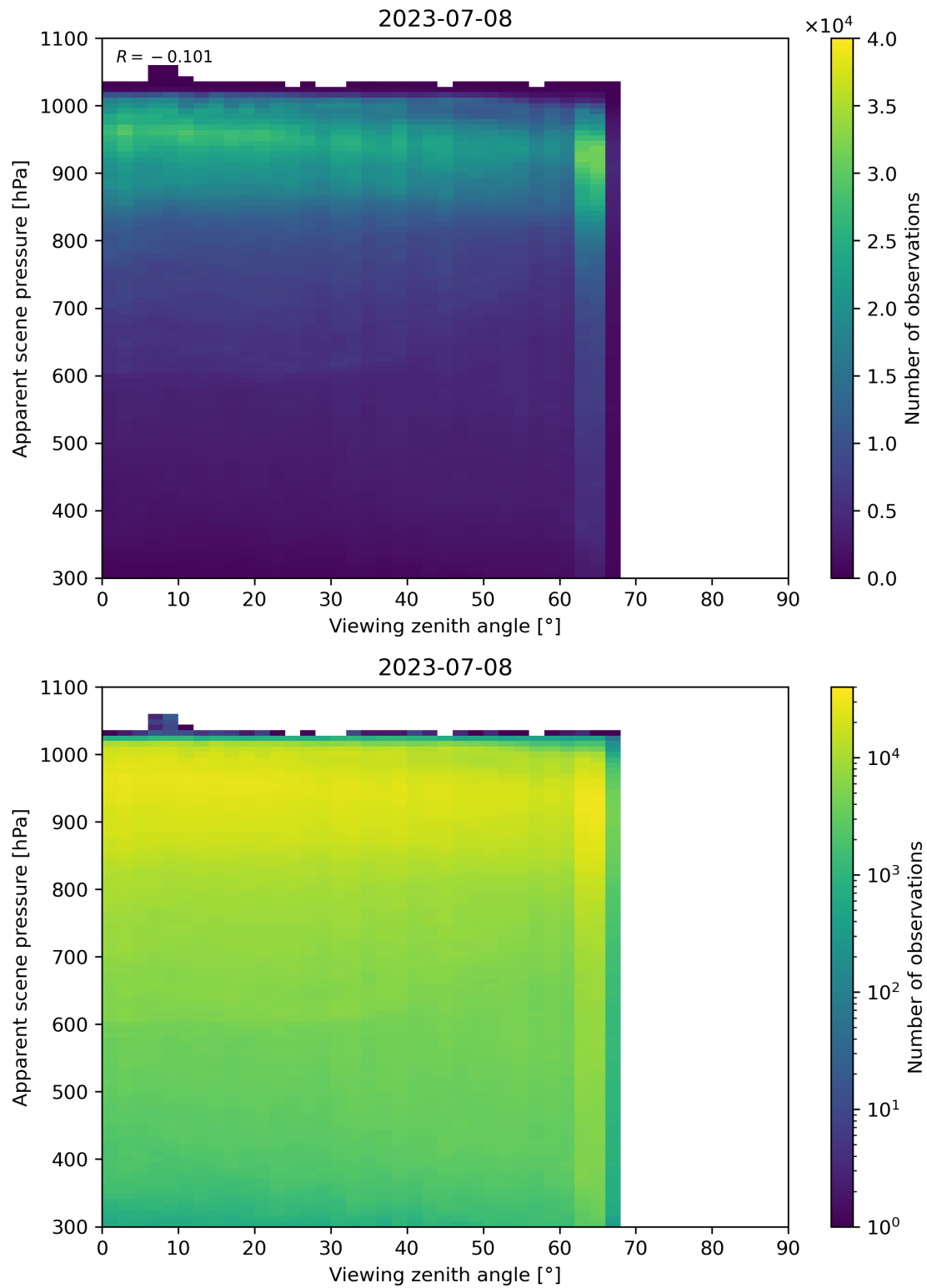
Figure 129: Scatter density plot of “Viewing zenith angle” against “Apparent scene pressure” for 2023-07-08 to 2023-07-09.
