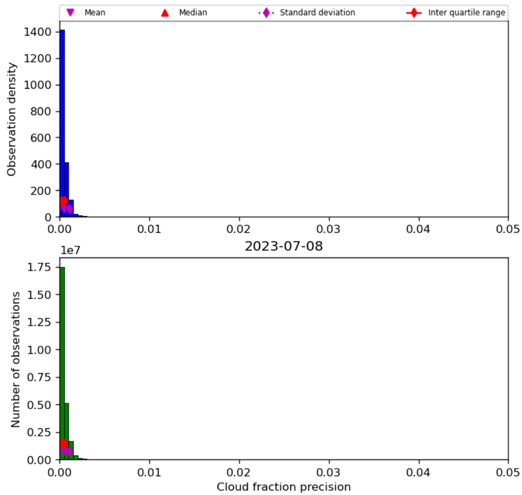
Figure 33: Histogram of “Cloud fraction precision” for 2023-07-08 to 2023-07-09
