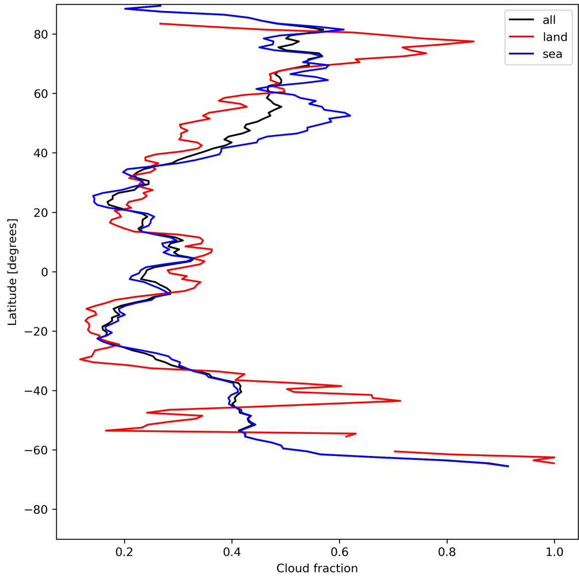
Figure 15: Zonal average of “Cloud fraction” for 2023-07-08 to 2023-07-09.
