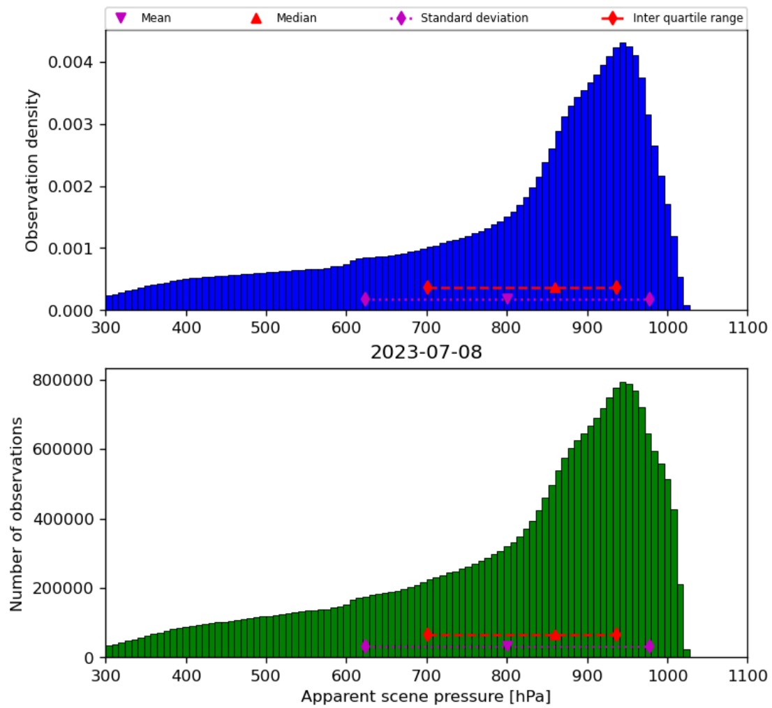
Figure 36: Histogram of “Apparent scene pressure” for 2023-07-08 to 2023-07-09
