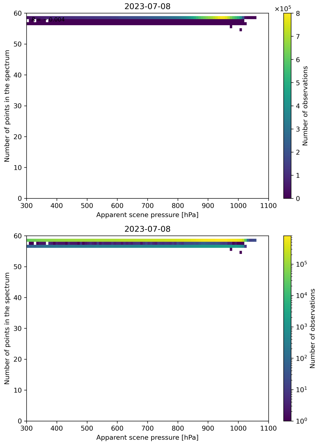
Figure 67: Scatter density plot of “Apparent scene pressure” against “Number of points in the spectrum” for 2023-07-08 to 2023-07-09.
