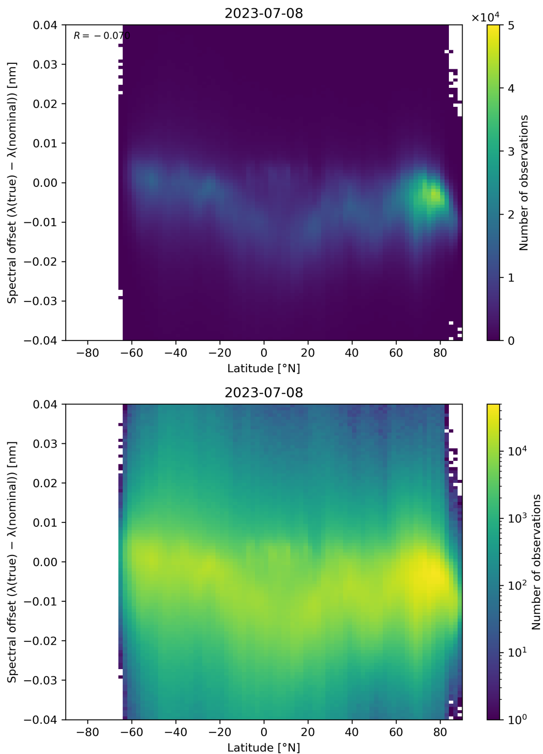
Figure 105: Scatter density plot of “Latitude” against “Spectral offset ( \lambda(\text{true}) - \lambda(\text{nominal}) )” for 2023-07-08 to 2023-07-09.
