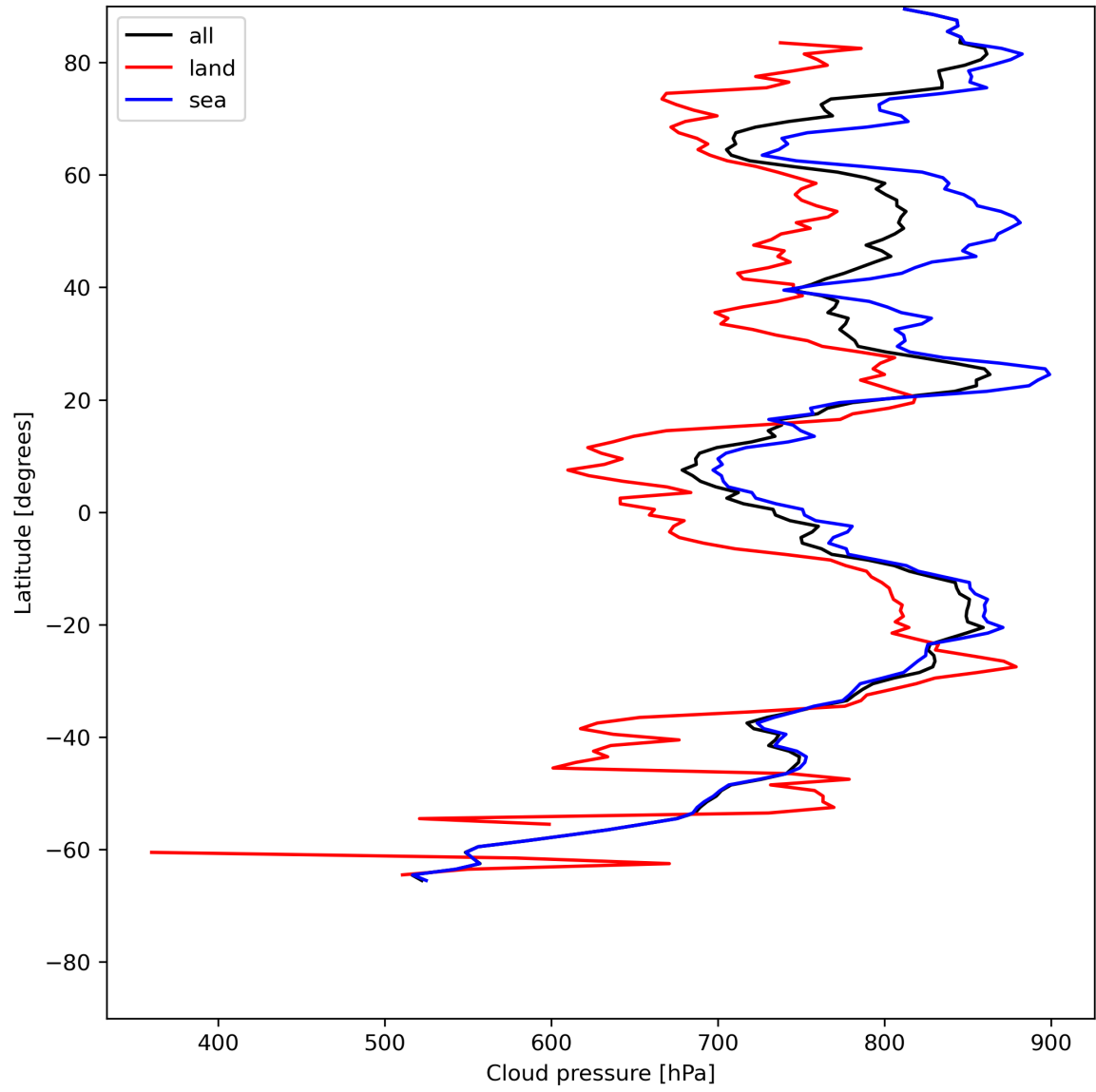
Figure 13: Zonal average of “Cloud pressure” for 2023-07-08 to 2023-07-09.
