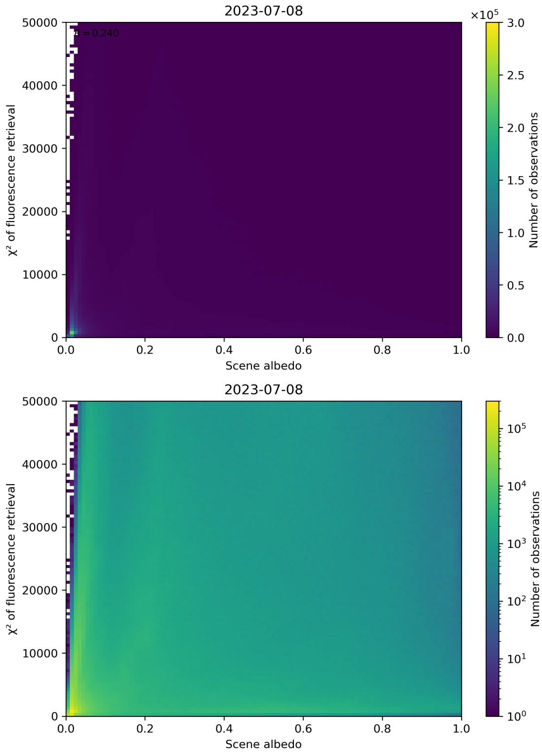
Figure 113: Scatter density plot of “Scene albedo” against “ \chi^2 of fluorescence retrieval” for 2023-07-08 to 2023-07-09.
