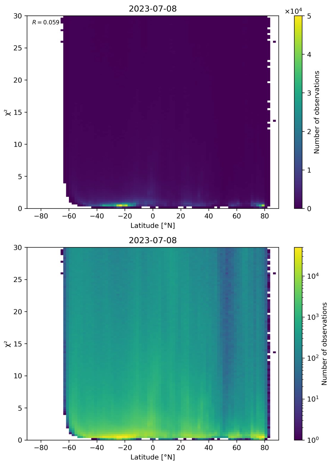
Figure 97: Scatter density plot of “Latitude” against “ \chi^2 ” for 2023-07-08 to 2023-07-09.
