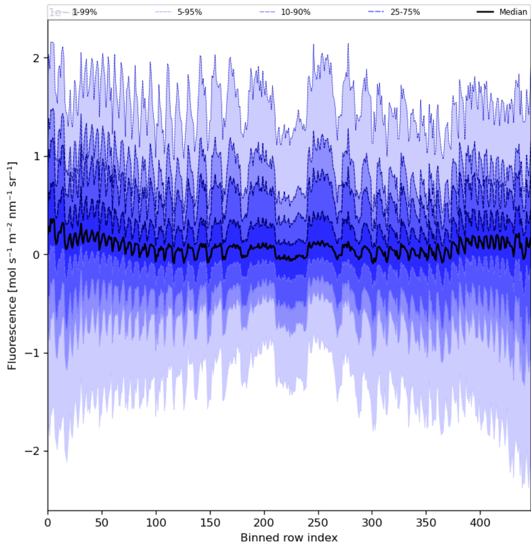
Figure 57: Along track statistics of "Fluorescence" for 2023-07-08 to 2023-07-09
