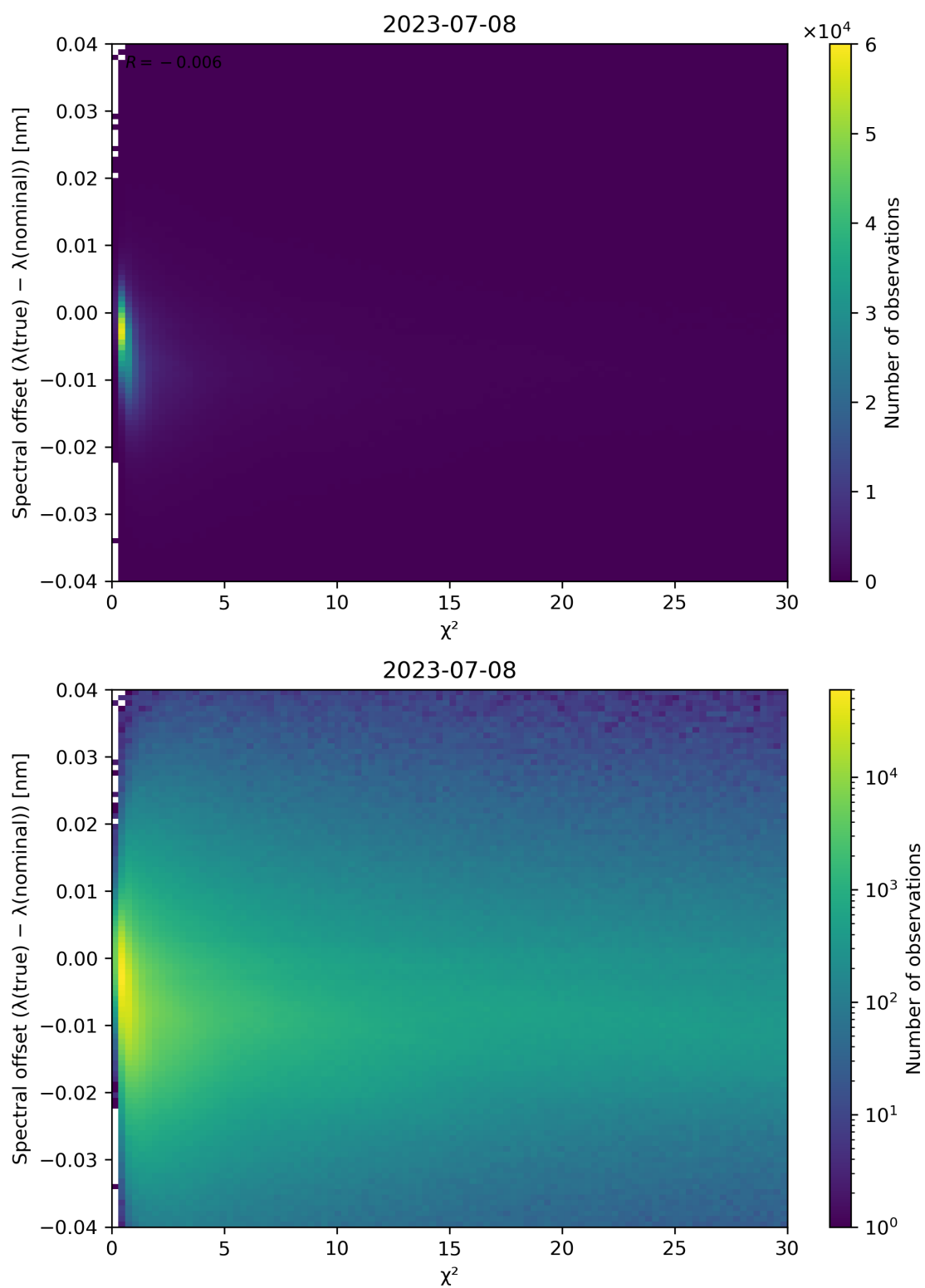
Figure 75: Scatter density plot of “ \chi^2 ” against “Spectral offset ( \lambda(\text{true}) - \lambda(\text{nominal}) )” for 2023-07-08 to 2023-07-09.
