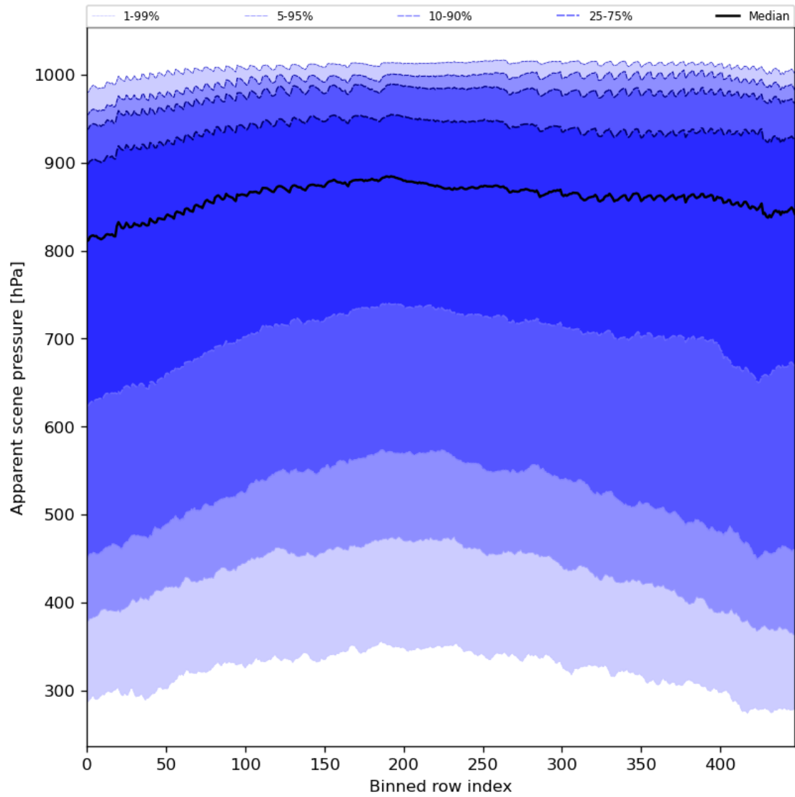
Figure 53: Along track statistics of “Apparent scene pressure” for 2023-07-08 to 2023-07-09
