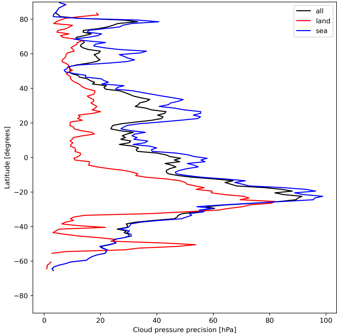
Figure 14: Zonal average of “Cloud pressure precision” for 2023-07-08 to 2023-07-09.
