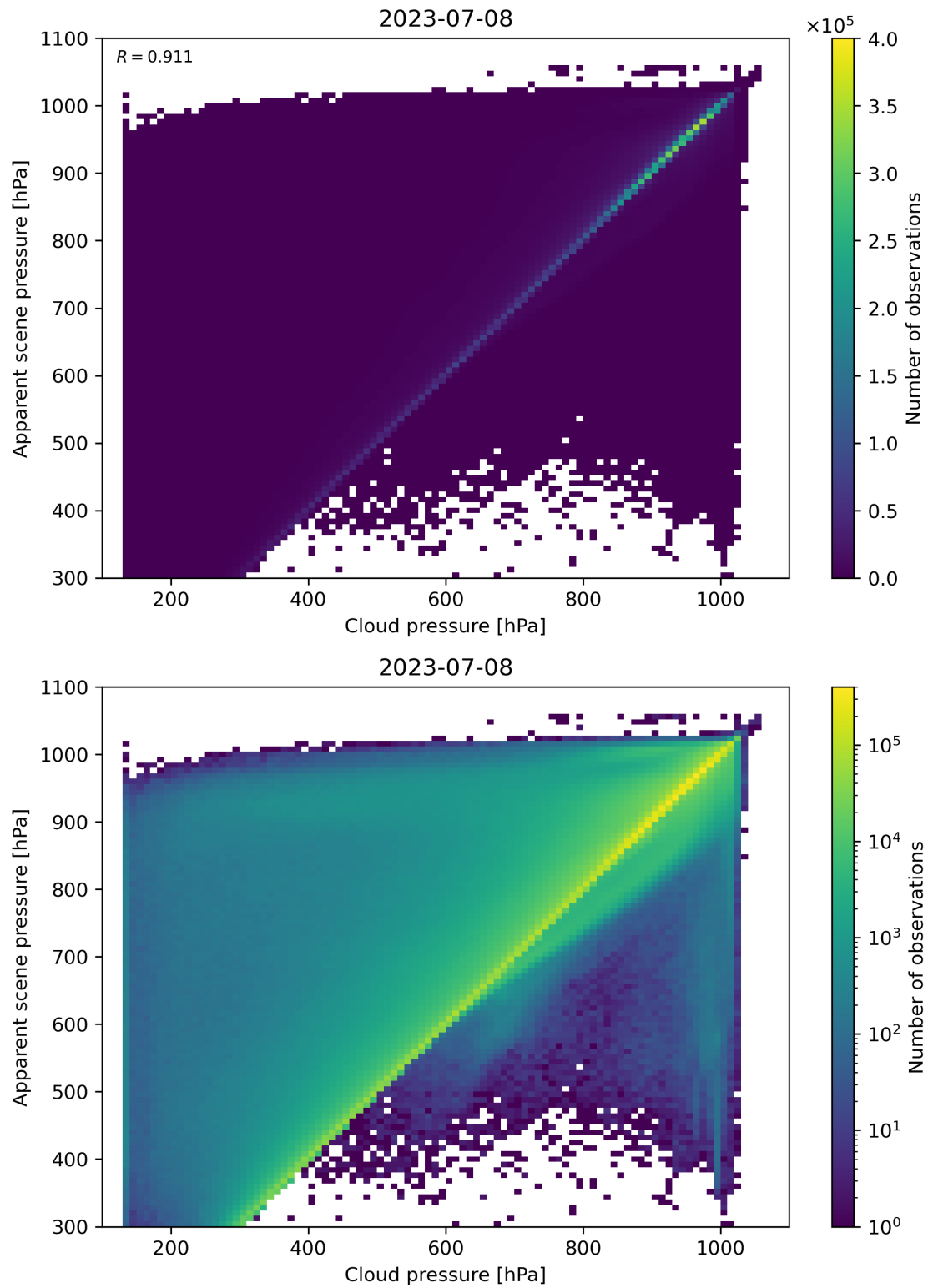
Figure 84: Scatter density plot of “Cloud pressure” against “Apparent scene pressure” for 2023-07-08 to 2023-07-09.
