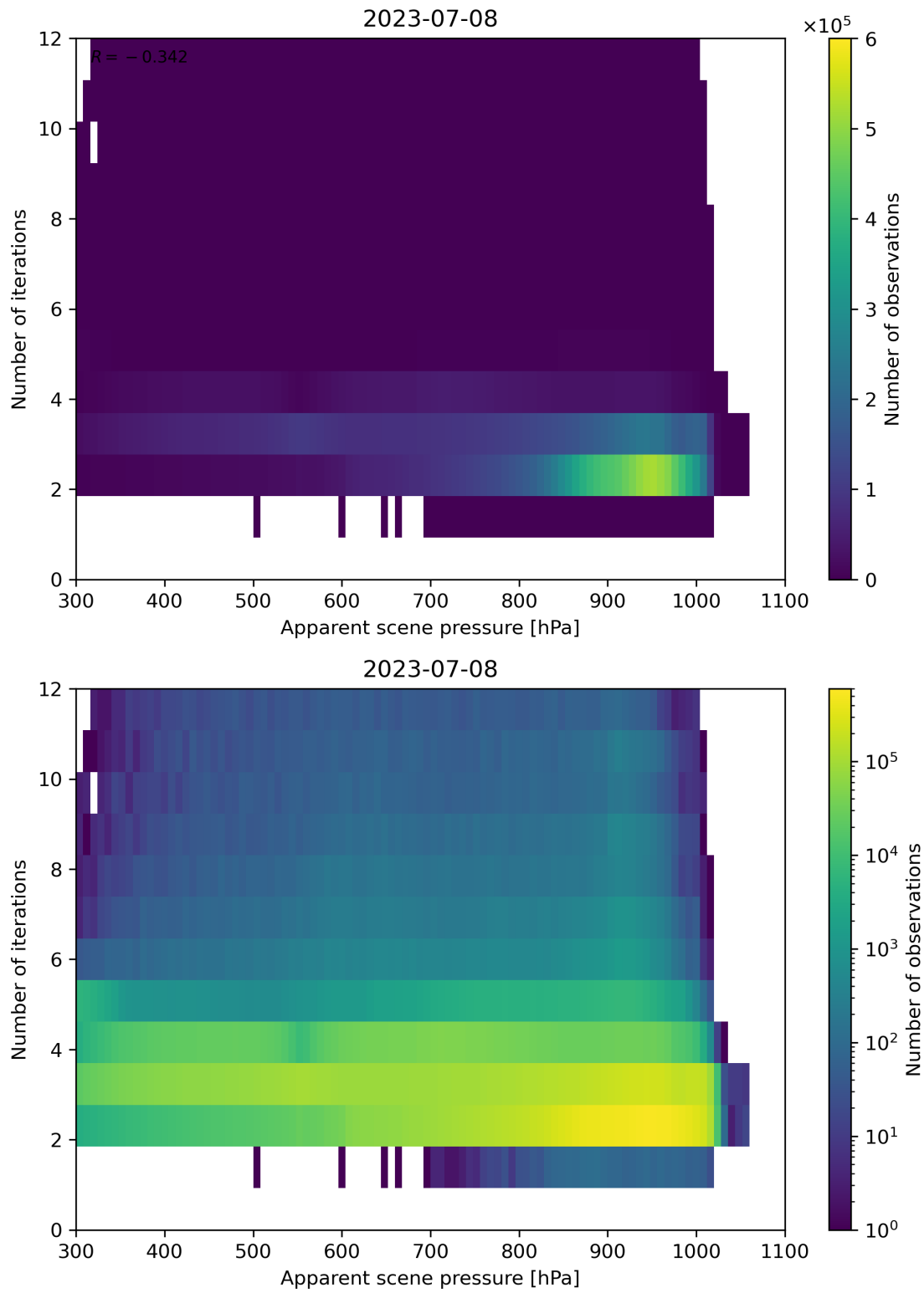
Figure 66: Scatter density plot of “Apparent scene pressure” against “Number of iterations” for 2023-07-08 to 2023-07-09.
