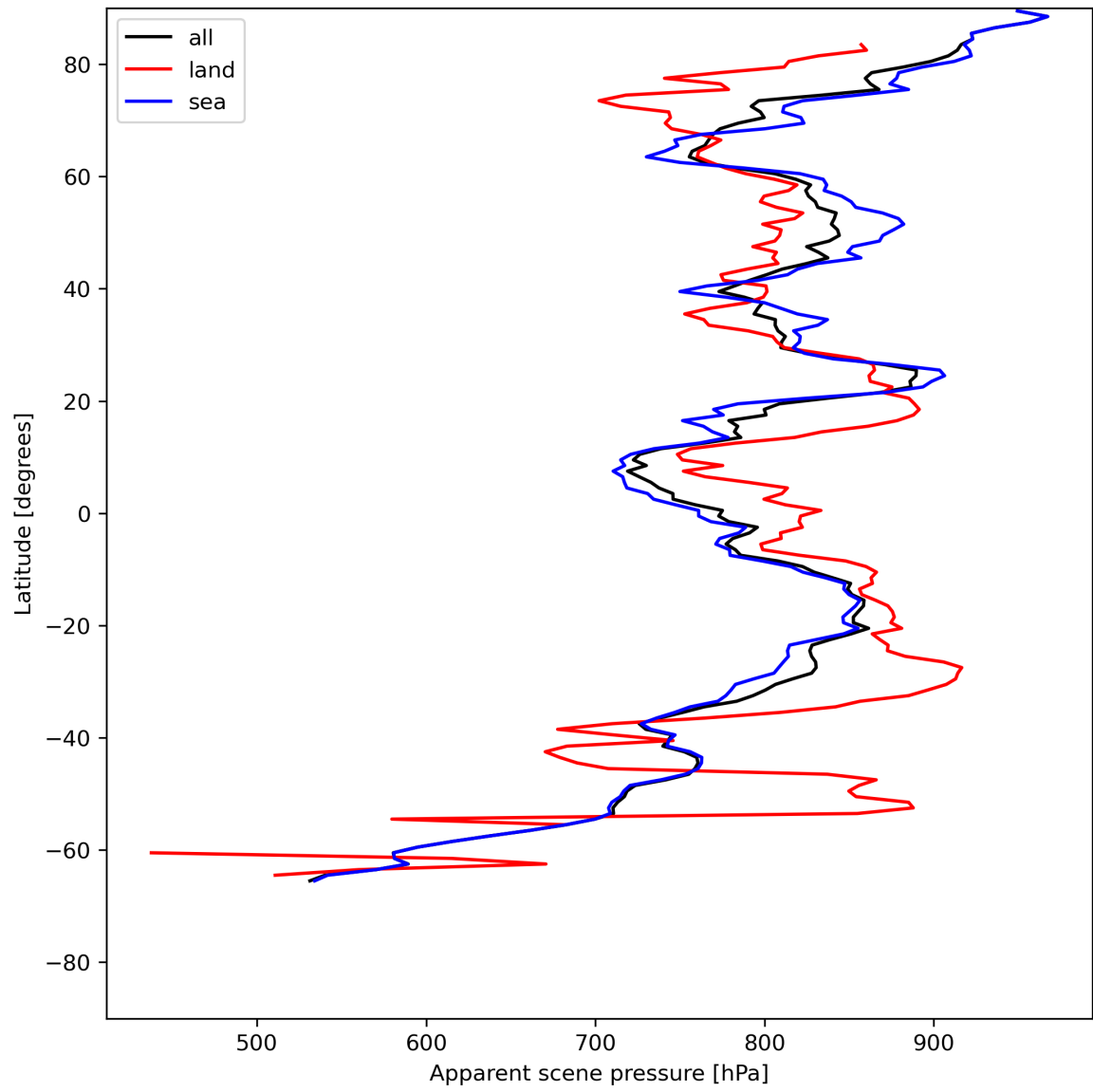
Figure 19: Zonal average of “Apparent scene pressure” for 2023-07-08 to 2023-07-09.
