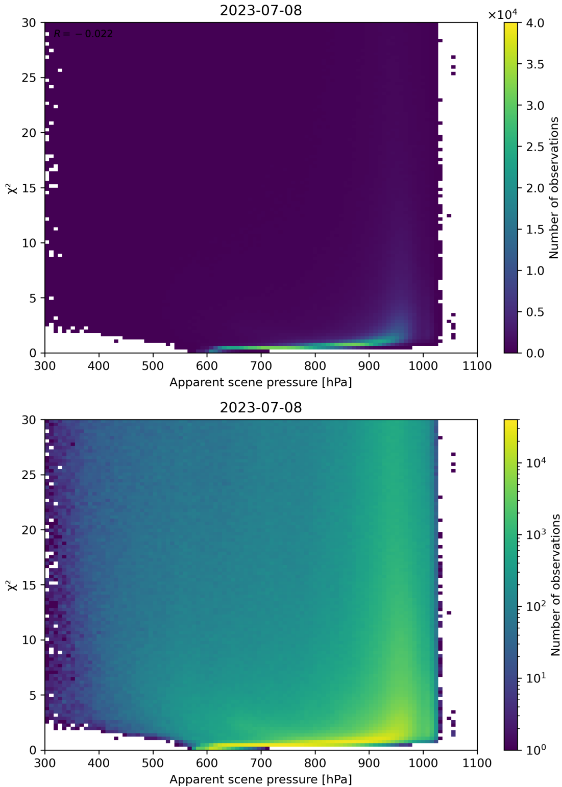
Figure 63: Scatter density plot of “Apparent scene pressure” against “ \chi^2 ” for 2023-07-08 to 2023-07-09.
