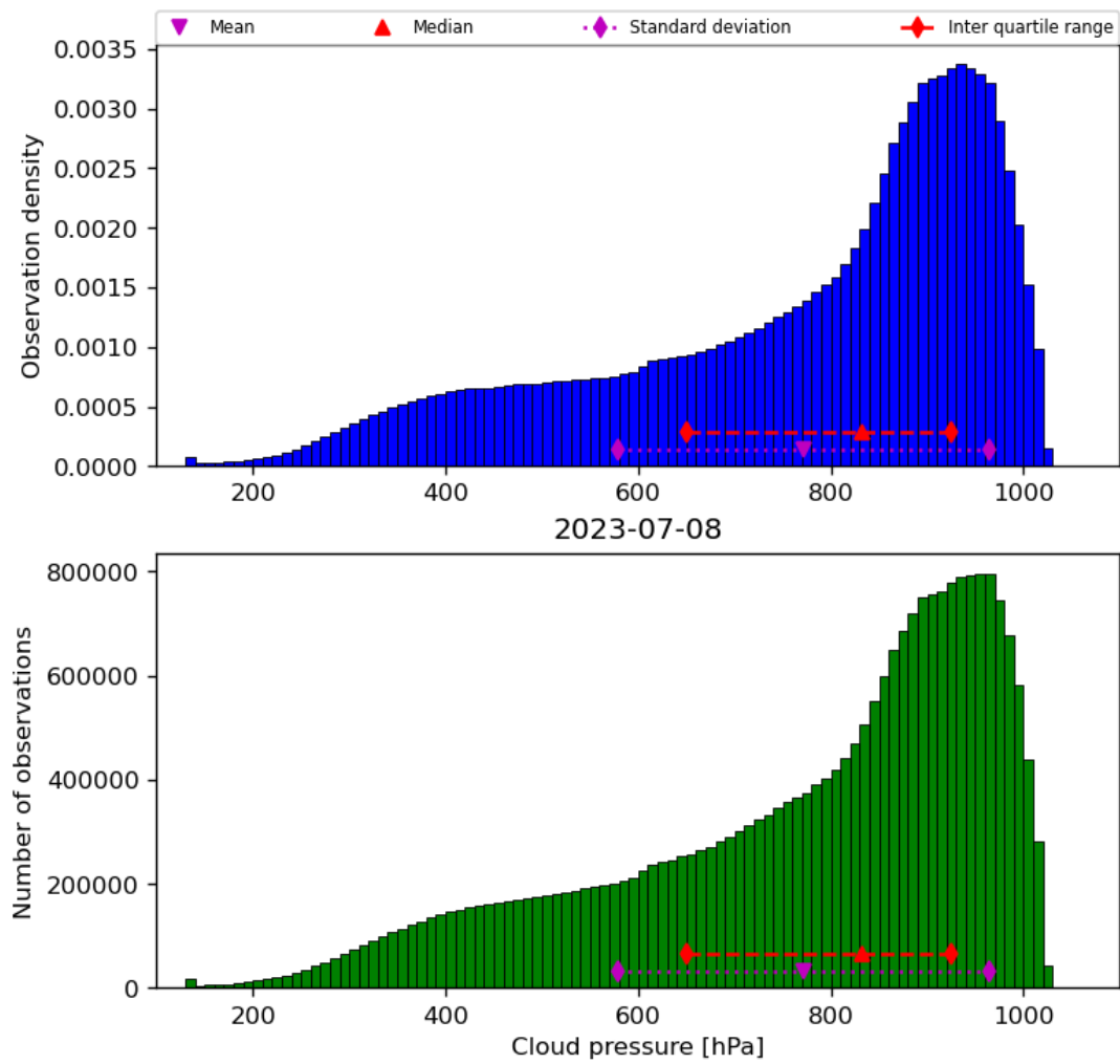
Figure 30: Histogram of “Cloud pressure” for 2023-07-08 to 2023-07-09
