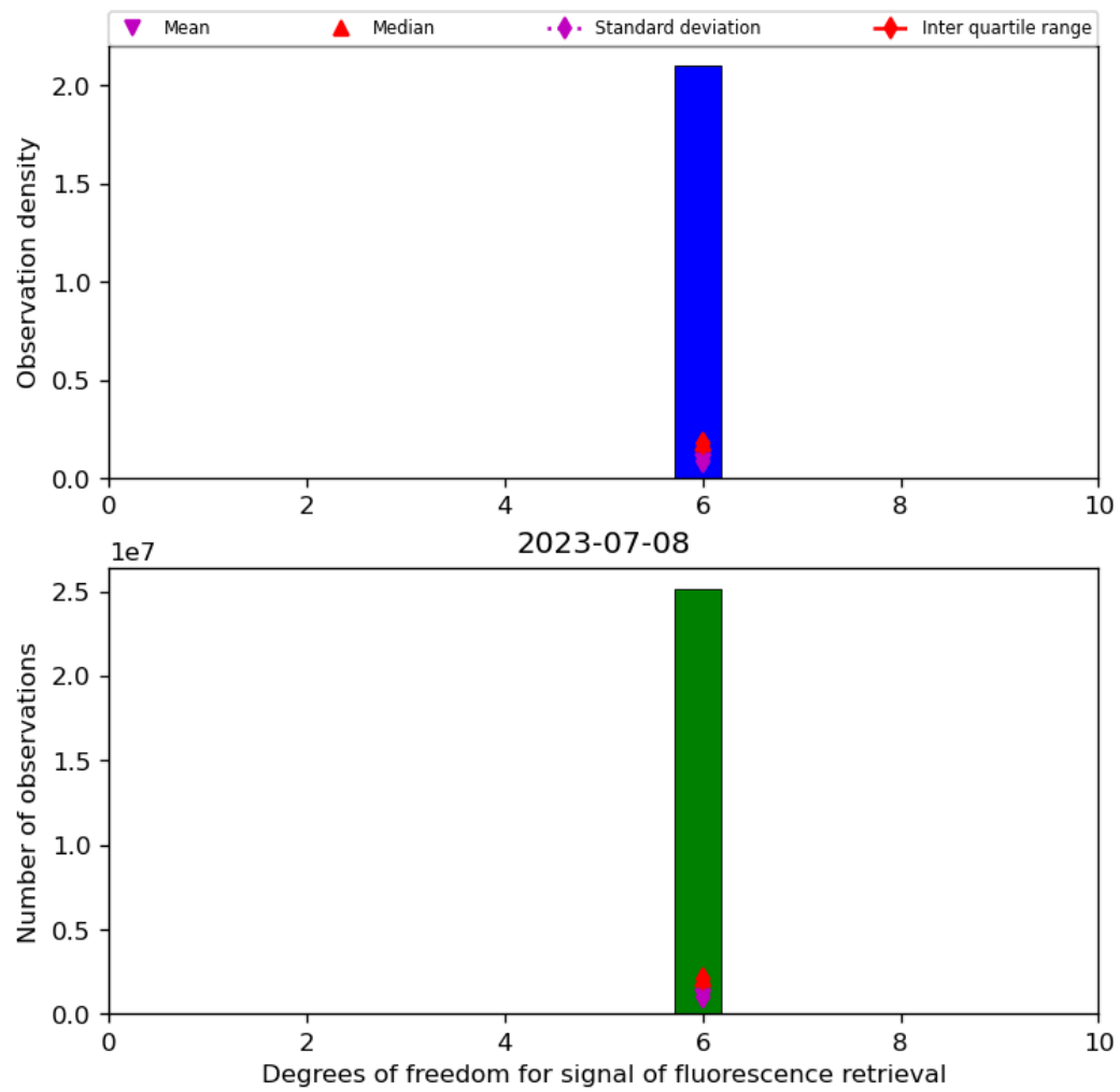
Figure 43: Histogram of “Degrees of freedom for signal of fluorescence retrieval” for 2023-07-08 to 2023-07-09
