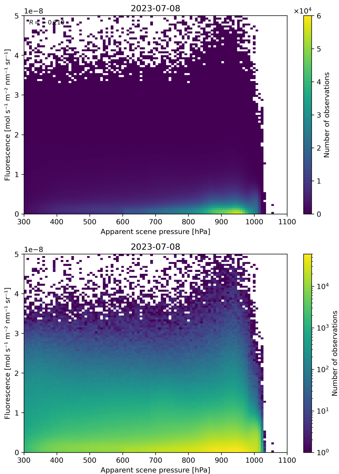
Figure 65: Scatter density plot of “Apparent scene pressure” against “Fluorescence” for 2023-07-08 to 2023-07-09.
