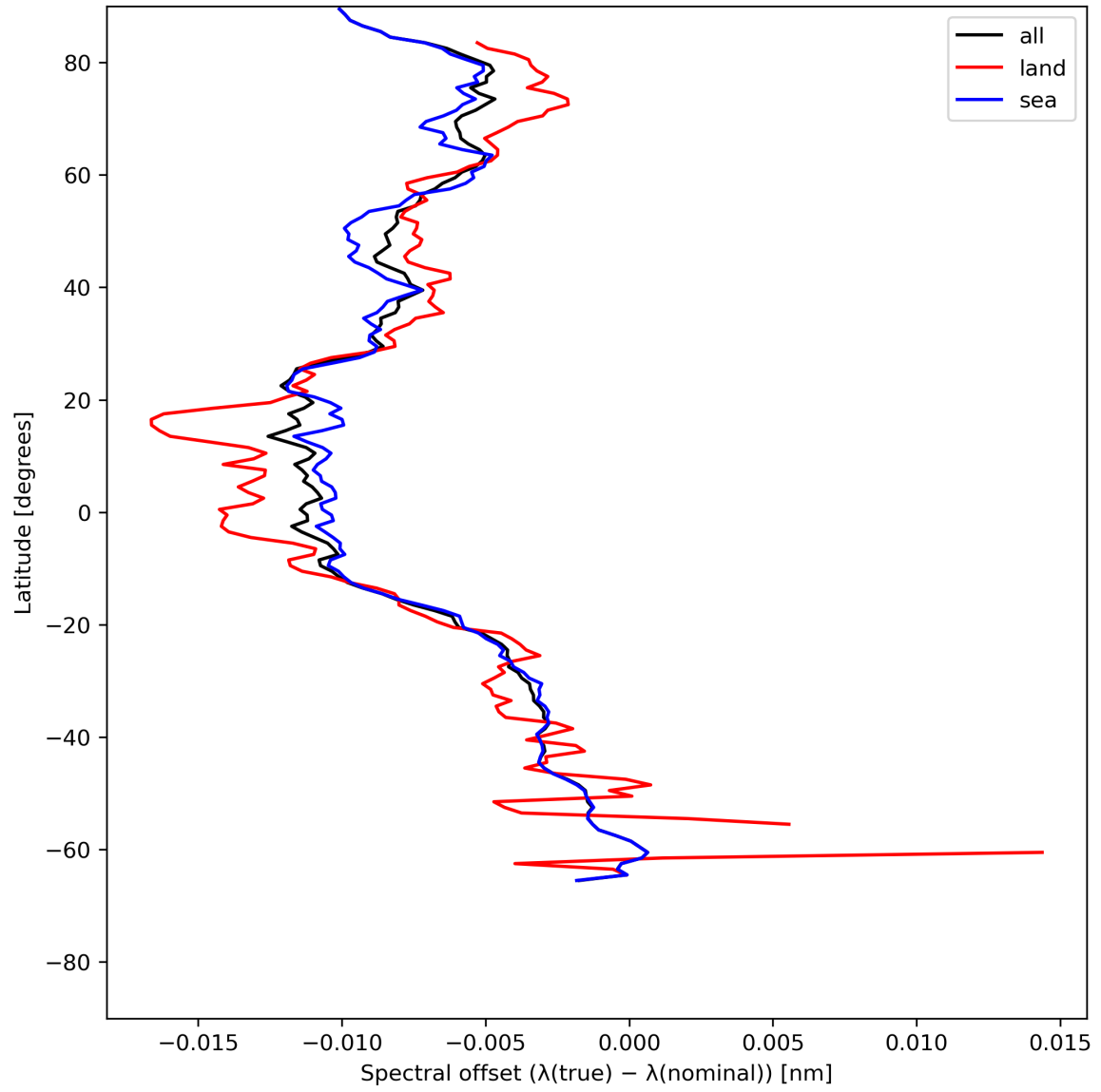
Figure 28: Zonal average of “Spectral offset ( \lambda(\text{true}) - \lambda(\text{nominal}) )” for 2023-07-08 to 2023-07-09.
