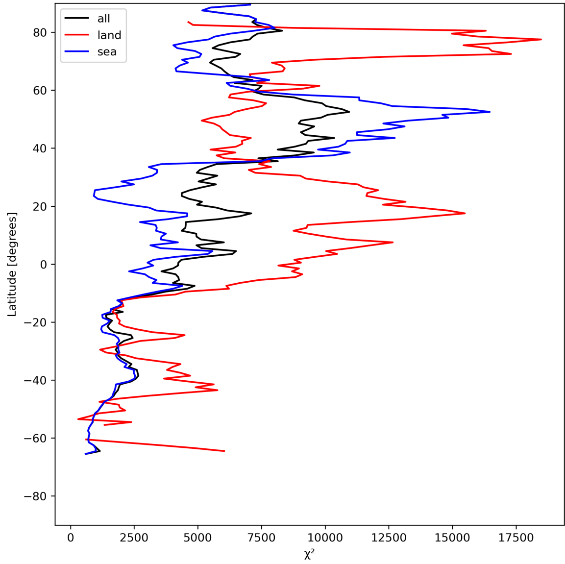
Figure 21: Zonal average of “ \chi^2 ” for 2023-07-08 to 2023-07-09.
