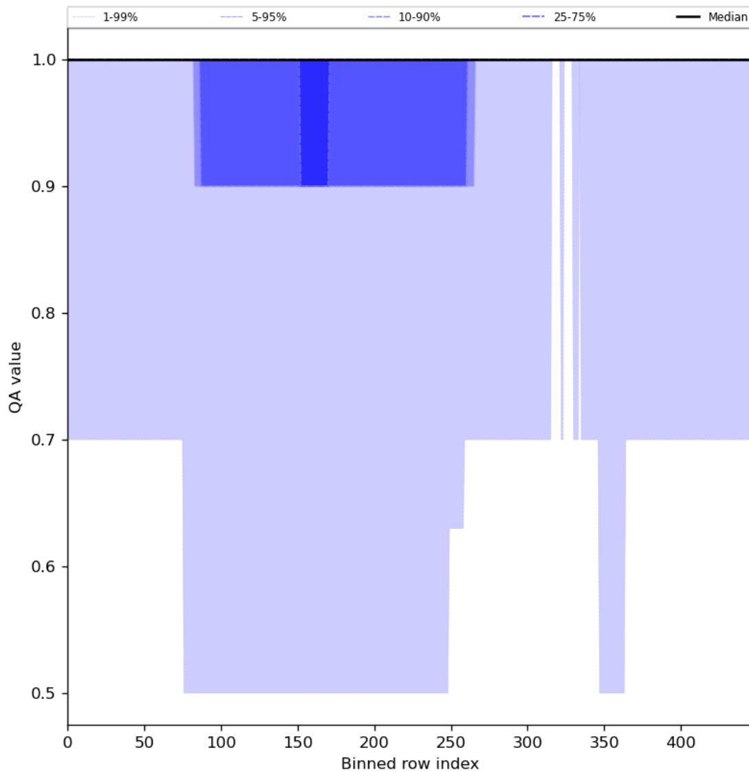
Figure 46: Along track statistics of “QA value” for 2023-07-08 to 2023-07-09
