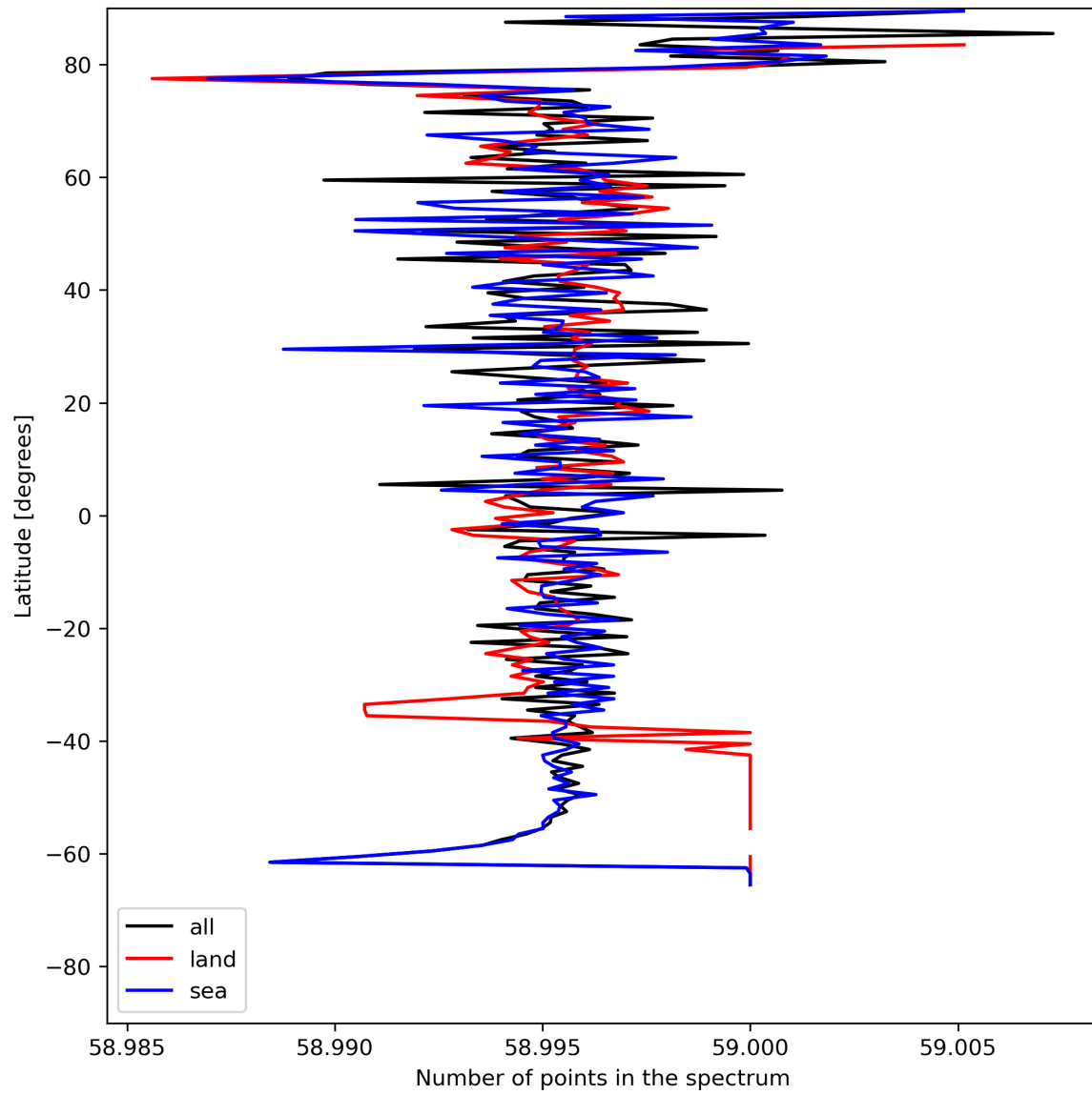
Figure 27: Zonal average of “Number of points in the spectrum” for 2023-07-08 to 2023-07-09.
