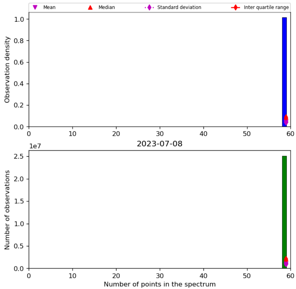
Figure 44: Histogram of "Number of points in the spectrum" for 2023-07-08 to 2023-07-09
