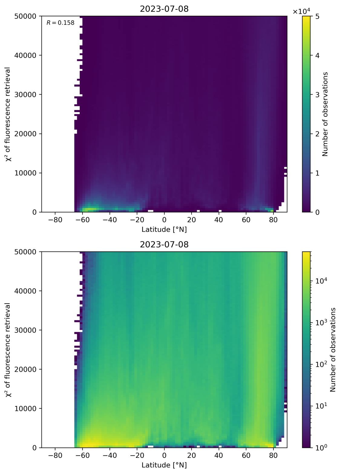
Figure 98: Scatter density plot of “Latitude” against “ \chi^2 of fluorescence retrieval” for 2023-07-08 to 2023-07-09.
