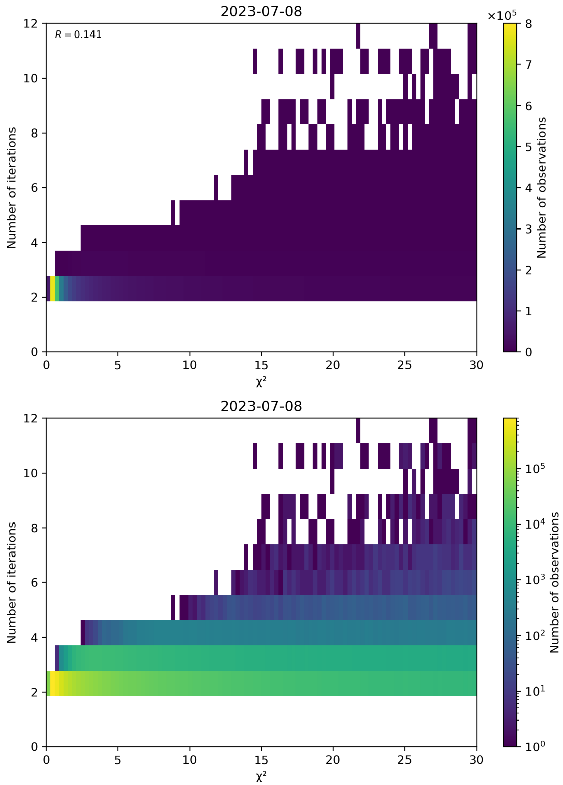
Figure 73: Scatter density plot of " \chi^2 " against "Number of iterations" for 2023-07-08 to 2023-07-09.
