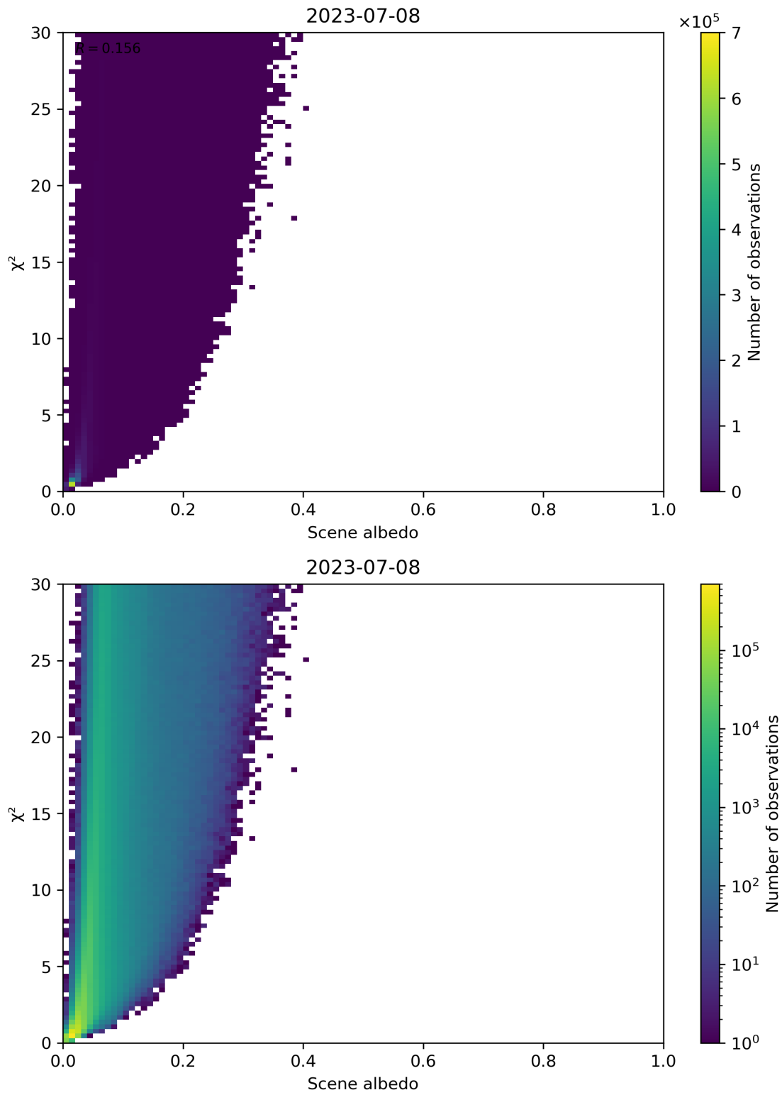
Figure 112: Scatter density plot of "Scene albedo" against " \chi^2 " for 2023-07-08 to 2023-07-09.
