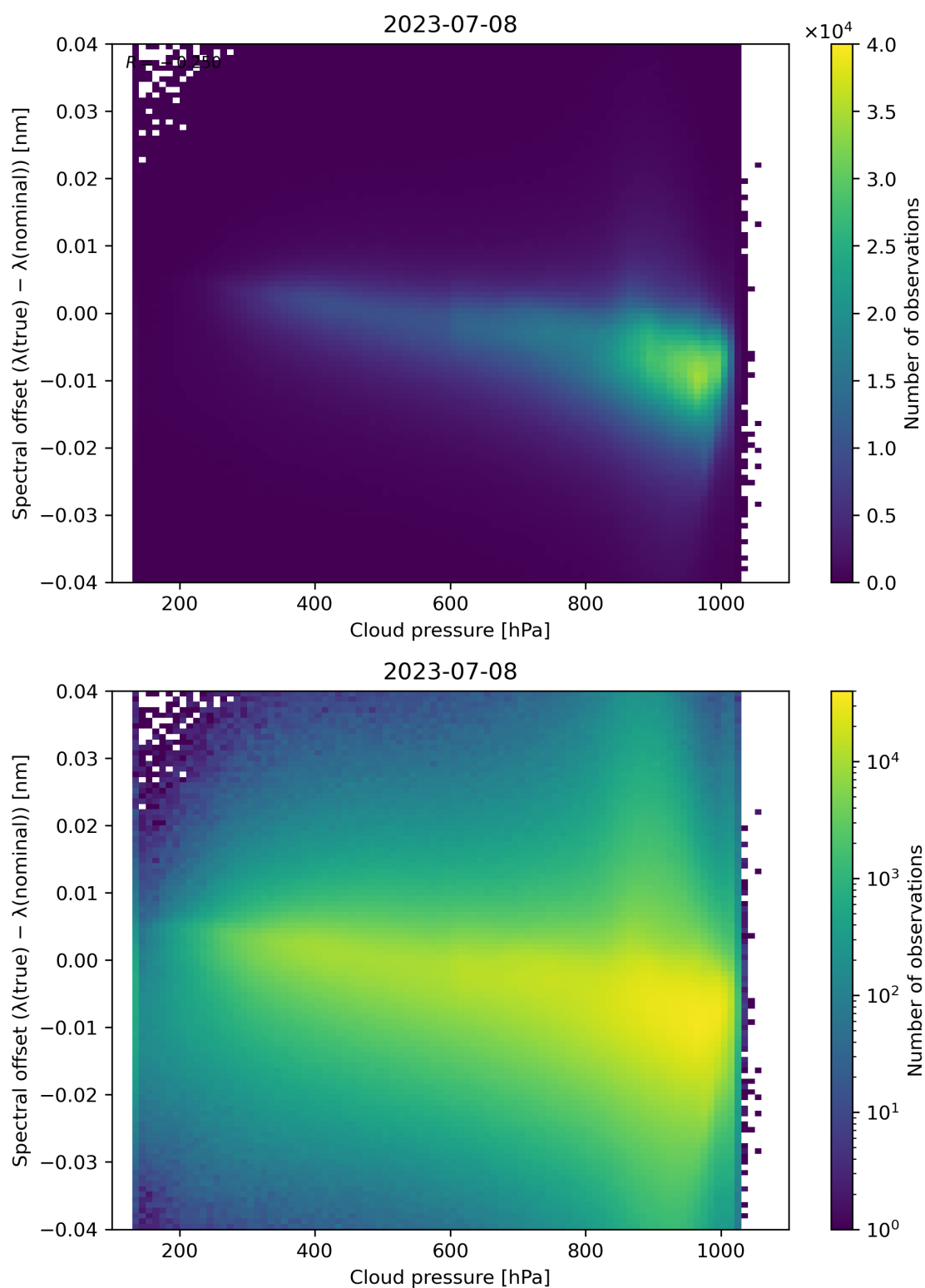
Figure 92: Scatter density plot of “Cloud pressure” against “Spectral offset ( \lambda(\text{true}) - \lambda(\text{nominal}) )” for 2023-07-08 to 2023-07-09.
