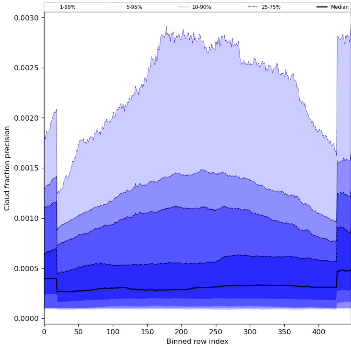
Figure 50: Along track statistics of “Cloud fraction precision” for 2023-07-08 to 2023-07-09
