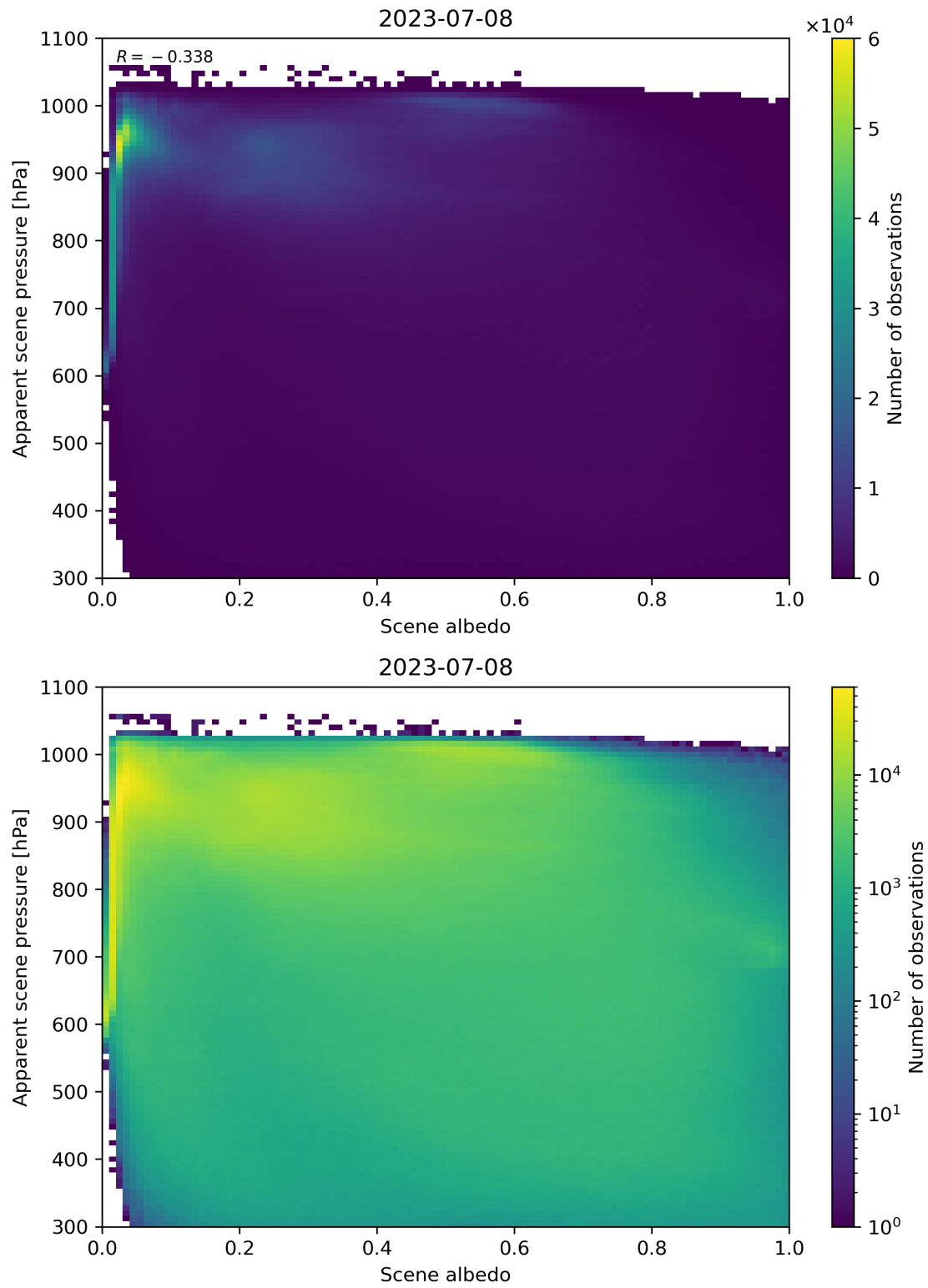
Figure 111: Scatter density plot of “Scene albedo” against “Apparent scene pressure” for 2023-07-08 to 2023-07-09.
