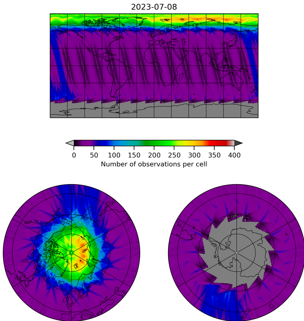
Figure 11: Map of the number of observations for 2023-07-08 to 2023-07-09
