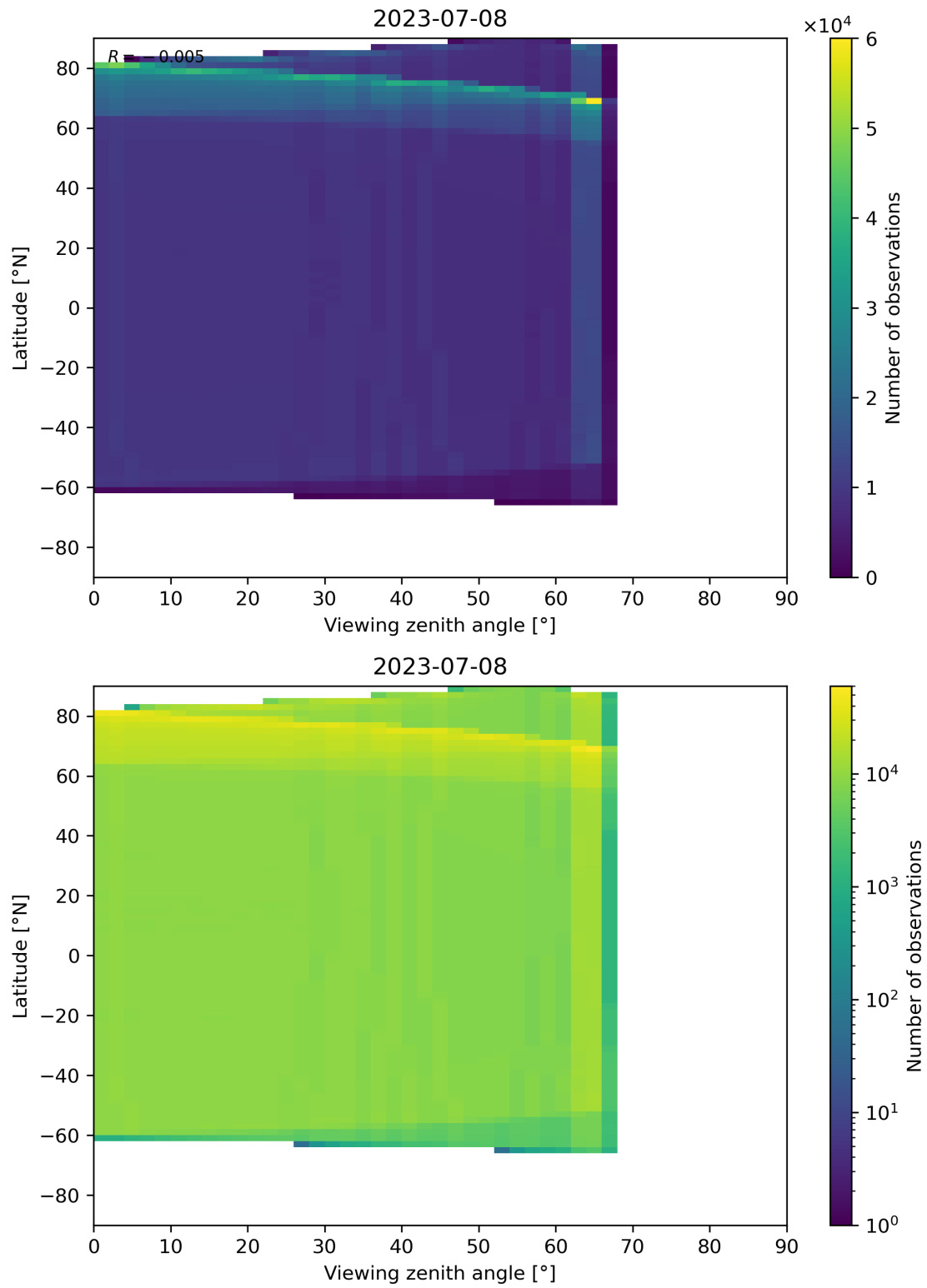
Figure 135: Scatter density plot of “Viewing zenith angle” against “Latitude” for 2023-07-08 to 2023-07-09.
