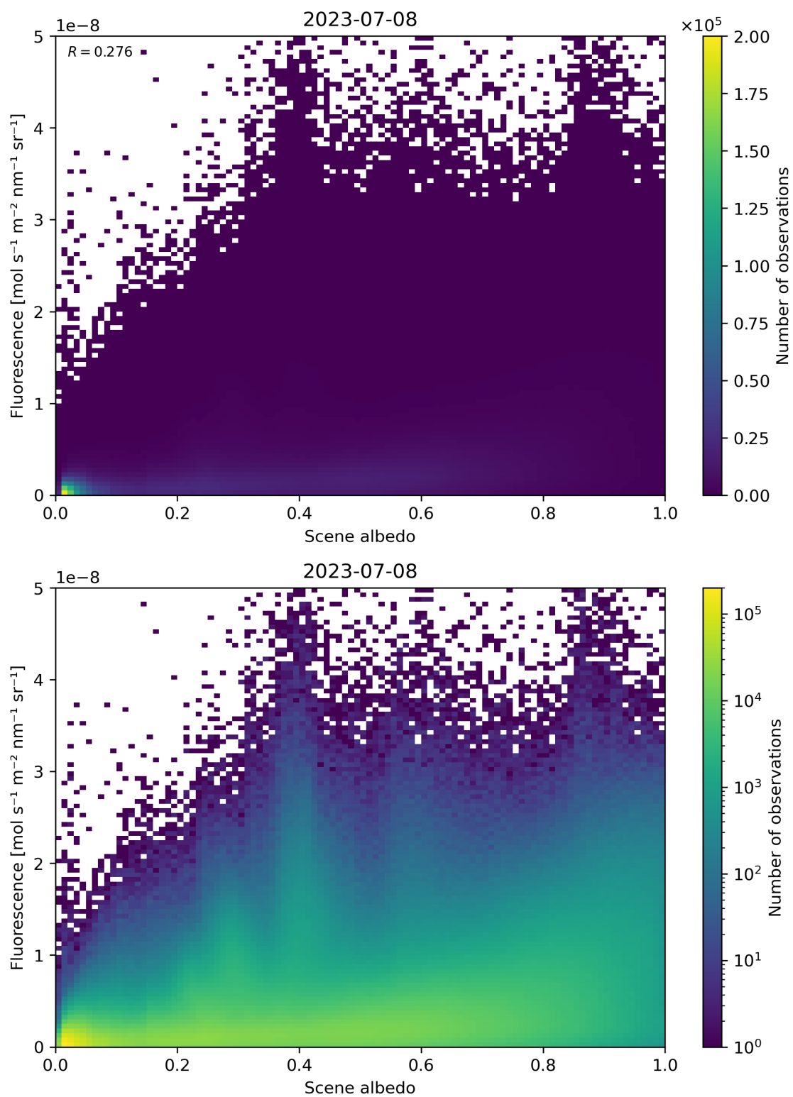
Figure 114: Scatter density plot of “Scene albedo” against “Fluorescence” for 2023-07-08 to 2023-07-09.
