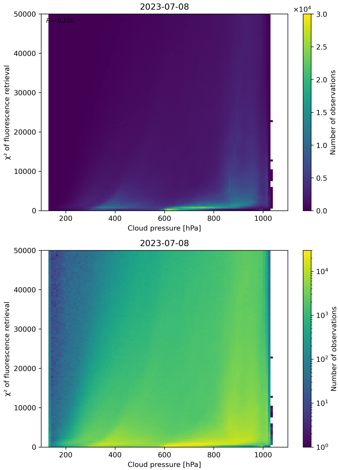
Figure 86: Scatter density plot of “Cloud pressure” against “ \chi^2 of fluorescence retrieval” for 2023-07-08 to 2023-07-09.
