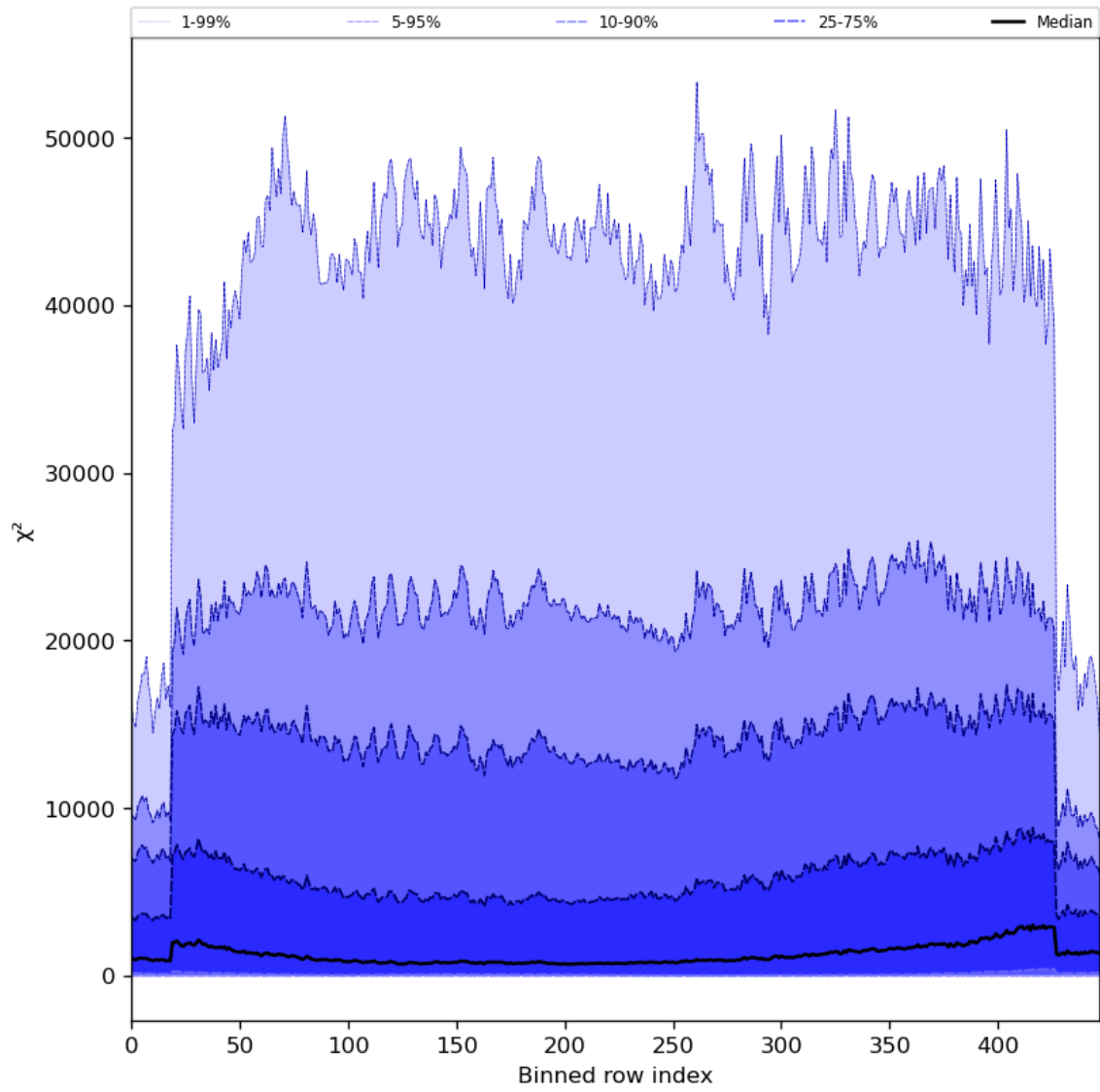
Figure 55: Along track statistics of “ \chi^2 ” for 2023-07-08 to 2023-07-09
