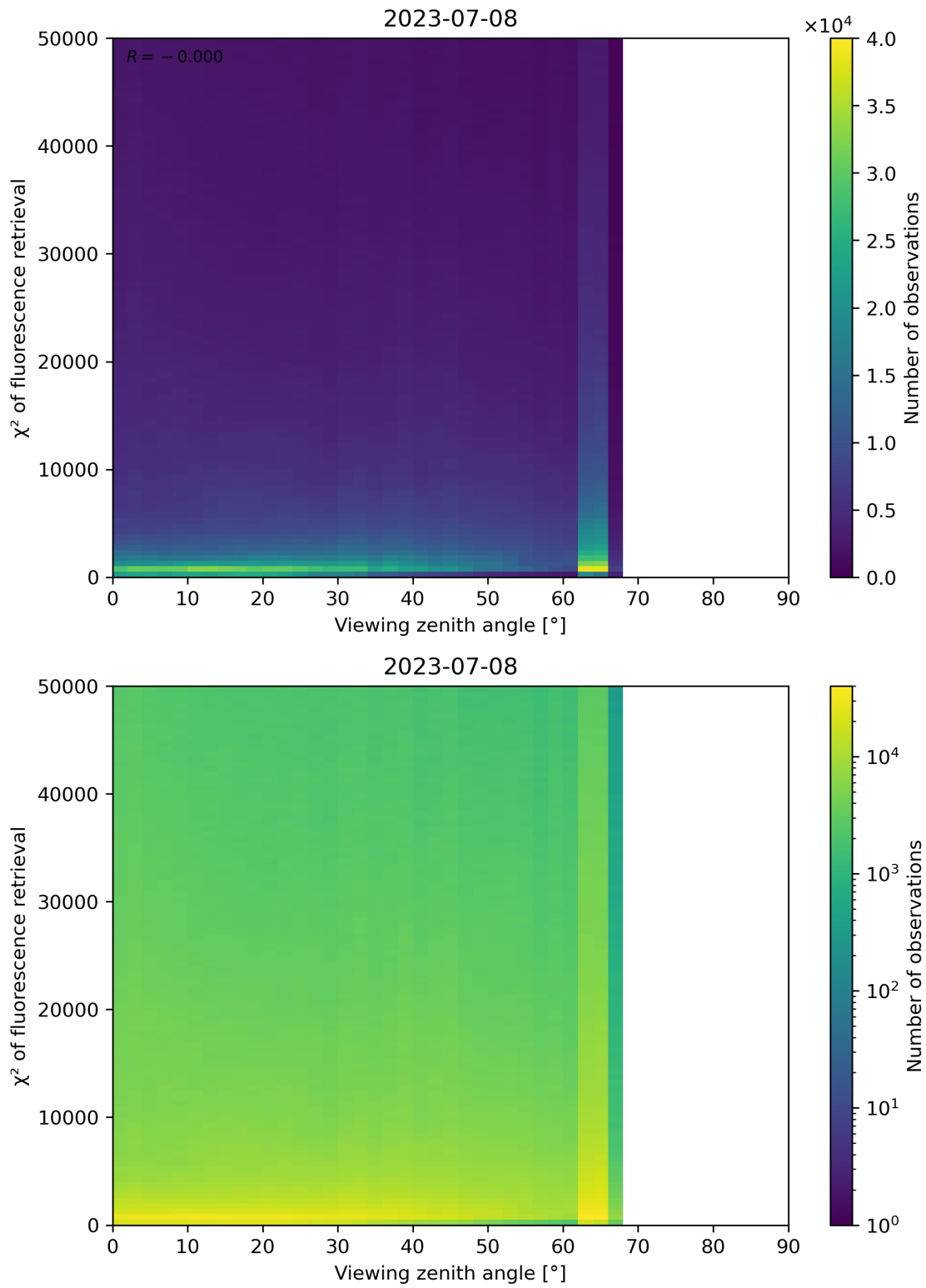
Figure 131: Scatter density plot of “Viewing zenith angle” against “ \chi^2 of fluorescence retrieval” for 2023-07-08 to 2023-07-09.
