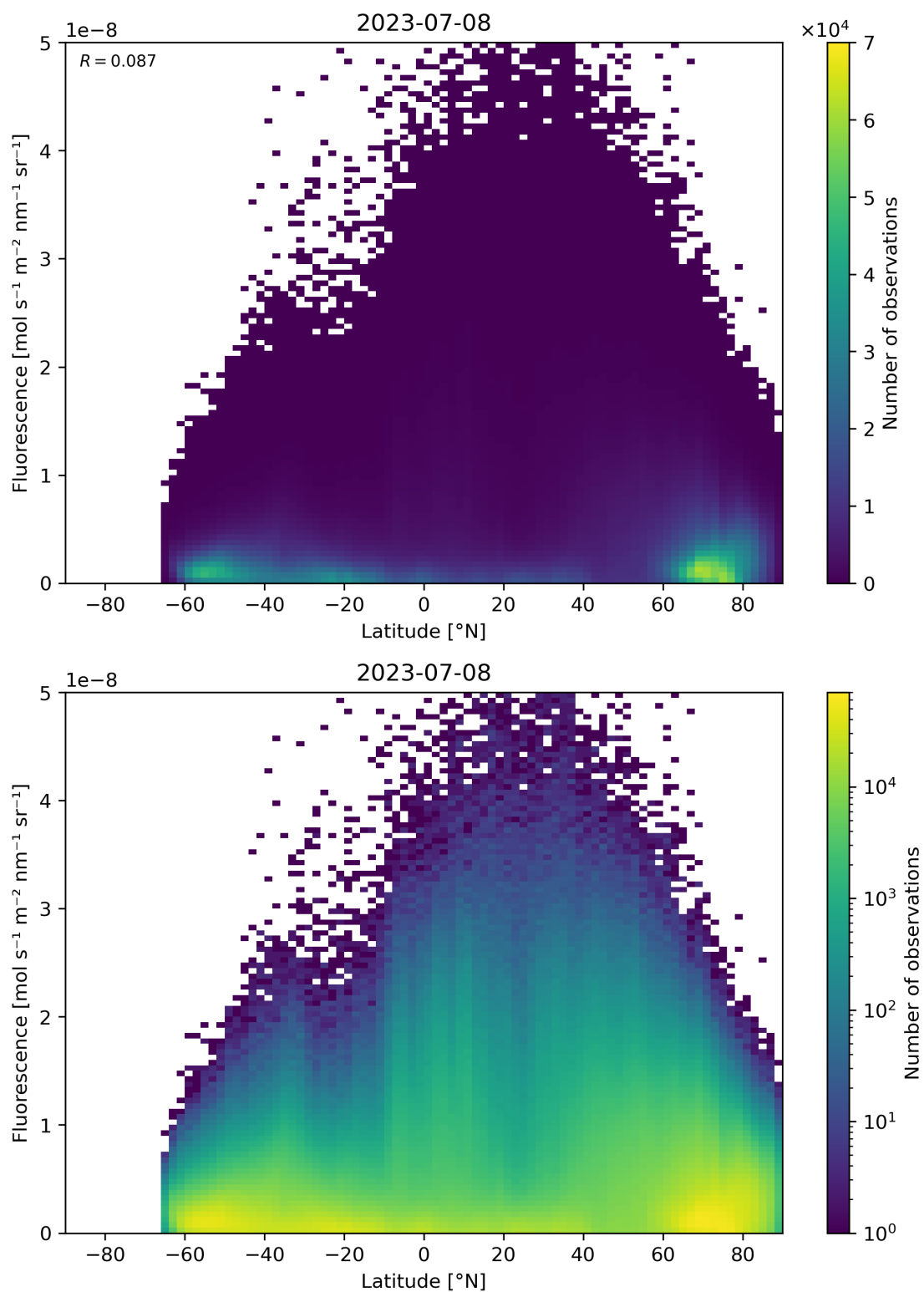
Figure 101: Scatter density plot of “Latitude” against “Fluorescence” for 2023-07-08 to 2023-07-09.
