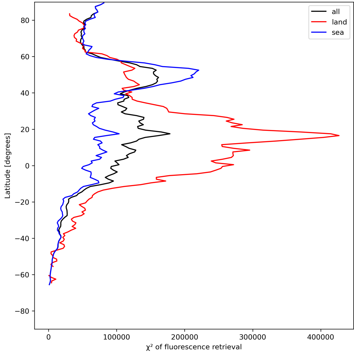
Figure 25: Zonal average of “ \chi^2 of fluorescence retrieval” for 2023-07-08 to 2023-07-09.
