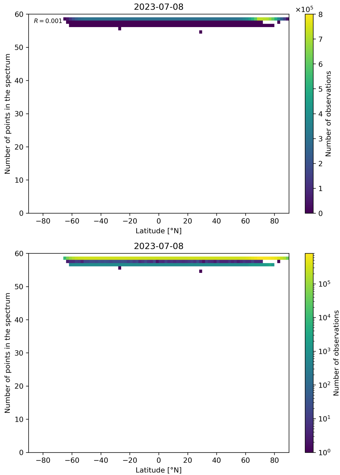
Figure 103: Scatter density plot of “Latitude” against “Number of points in the spectrum” for 2023-07-08 to 2023-07-09.
