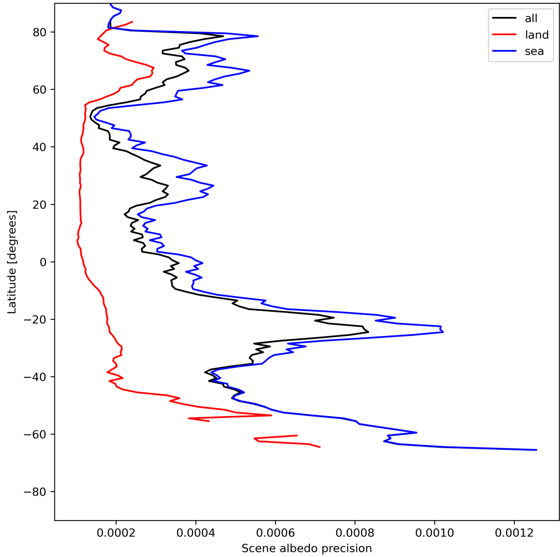
Figure 18: Zonal average of “Scene albedo precision” for 2023-07-08 to 2023-07-09.
