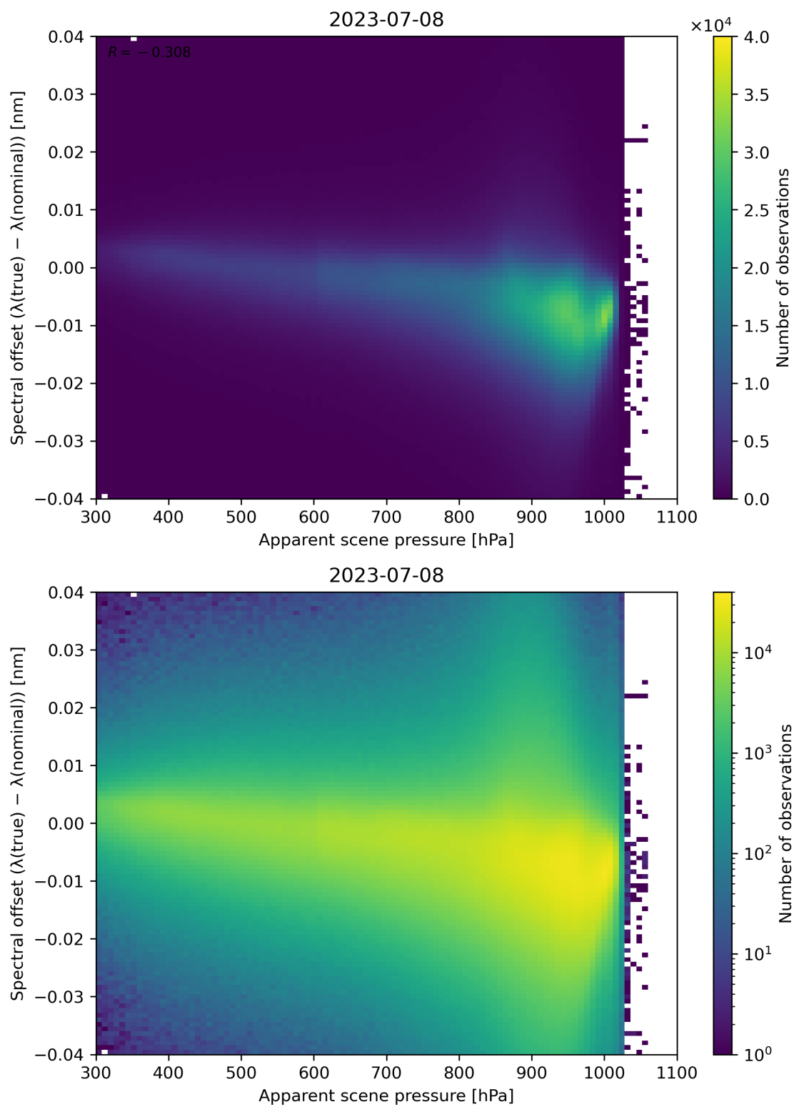
Figure 68: Scatter density plot of “Apparent scene pressure” against “Spectral offset ( \lambda(\text{true}) - \lambda(\text{nominal}) )” for 2023-07-08 to 2023-07-09.
