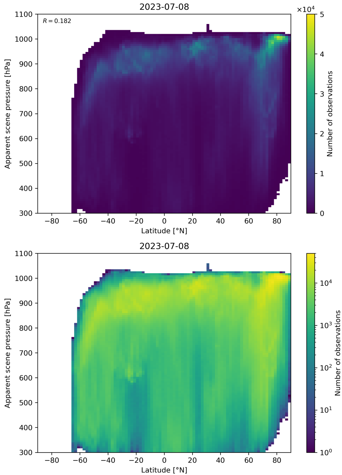
Figure 96: Scatter density plot of “Latitude” against “Apparent scene pressure” for 2023-07-08 to 2023-07-09.
