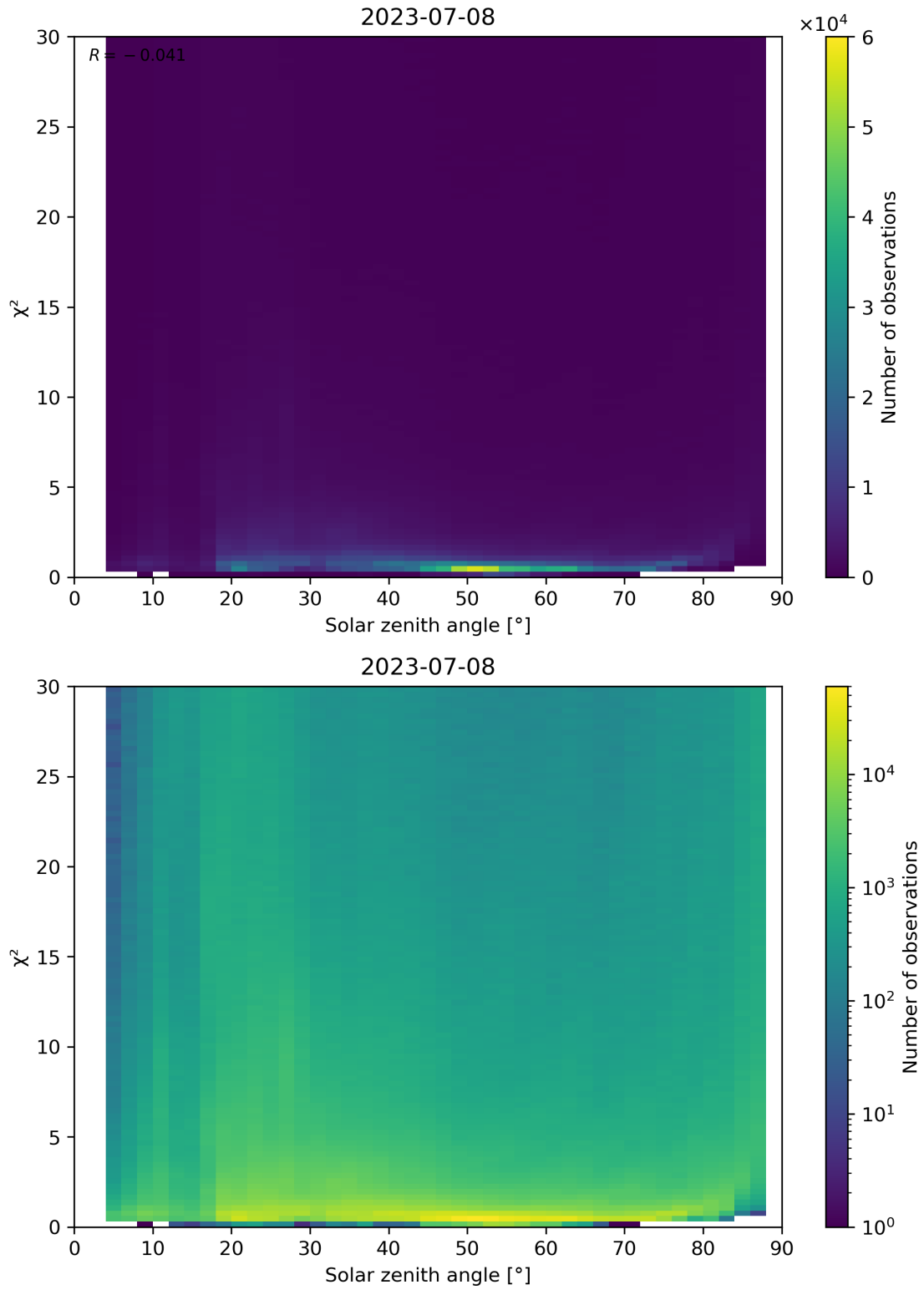
Figure 119: Scatter density plot of “Solar zenith angle” against “ \chi^2 ” for 2023-07-08 to 2023-07-09.
