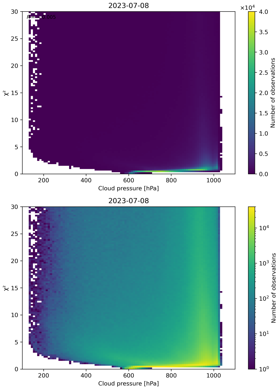
Figure 85: Scatter density plot of “Cloud pressure” against “ \chi^2 ” for 2023-07-08 to 2023-07-09.
