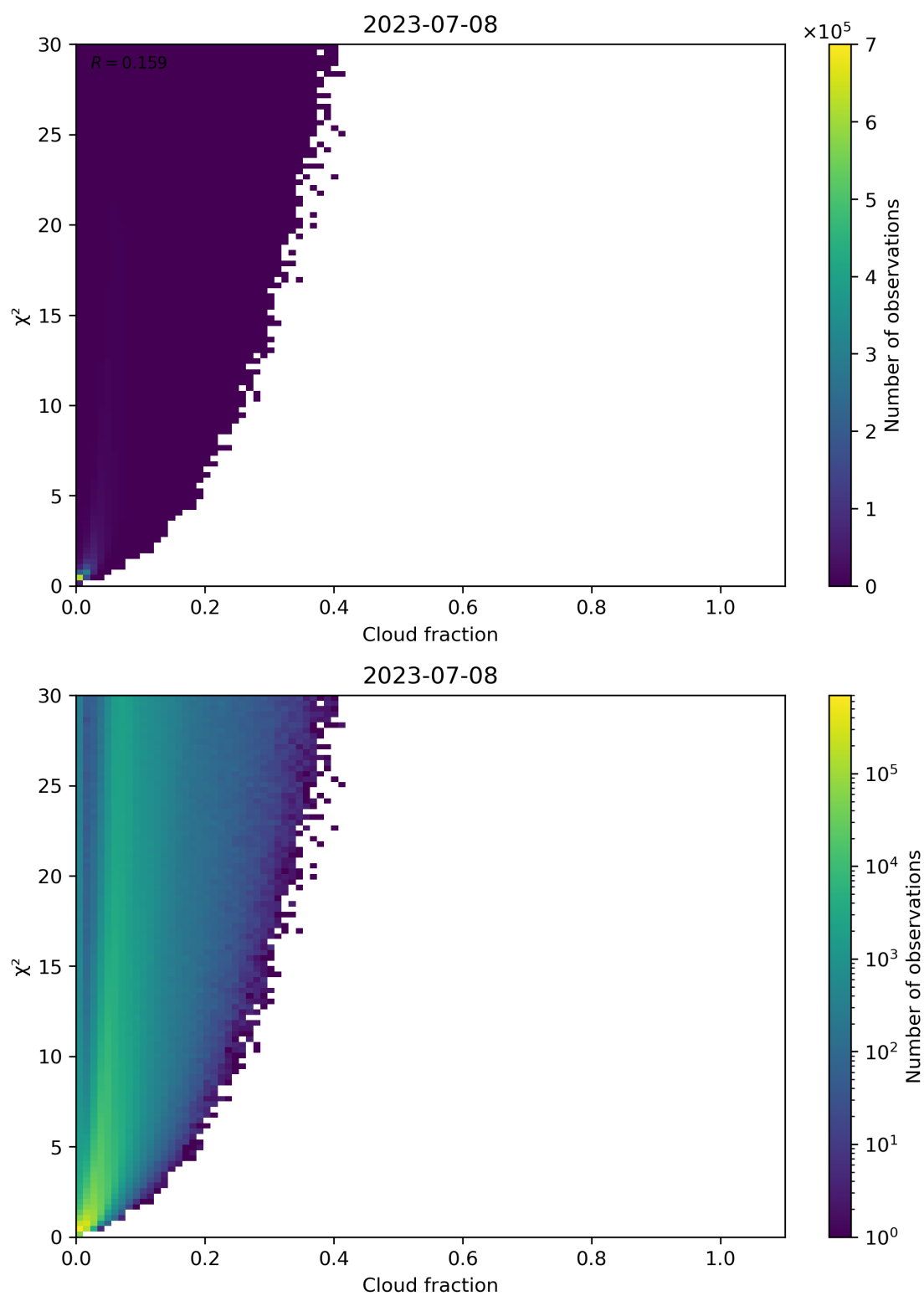
Figure 77: Scatter density plot of “Cloud fraction” against “ \chi^2 ” for 2023-07-08 to 2023-07-09.
