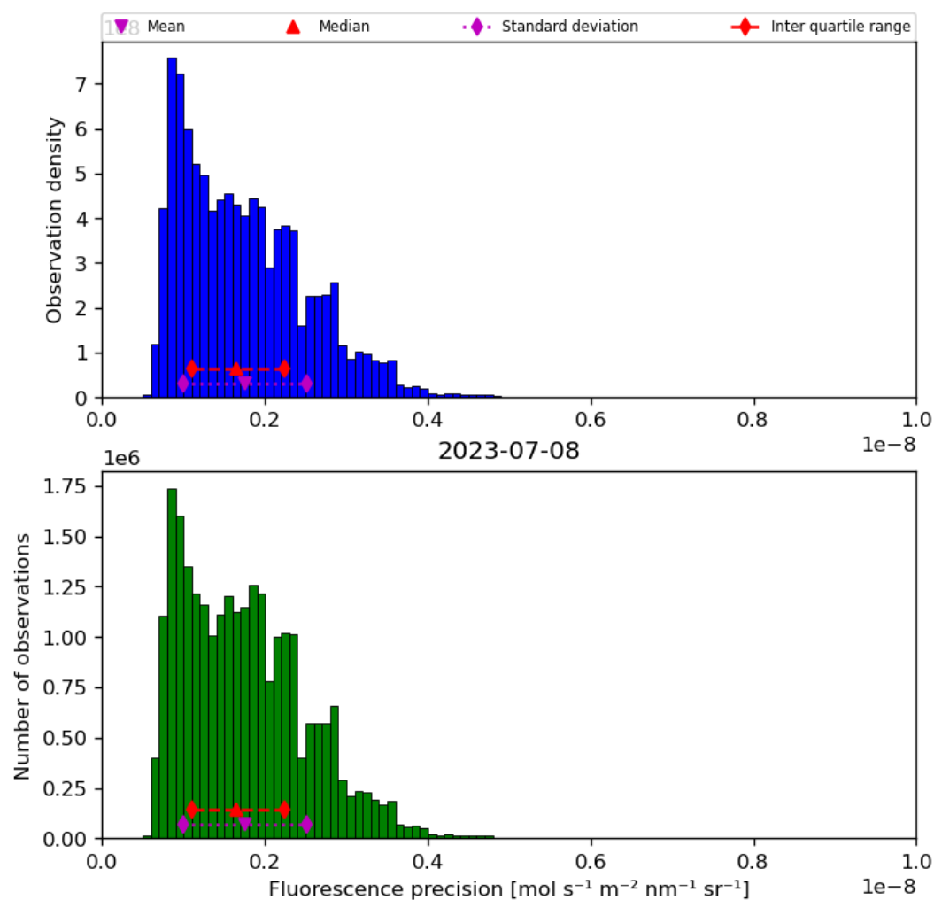
Figure 41: Histogram of “Fluorescence precision” for 2023-07-08 to 2023-07-09
