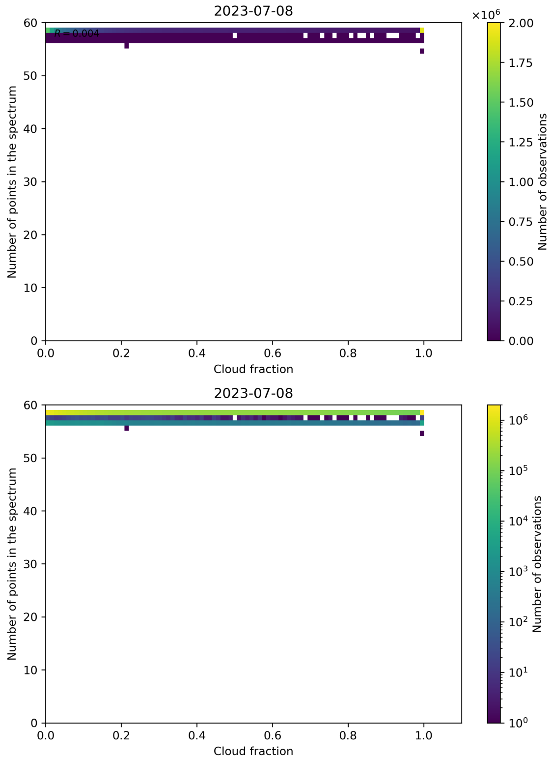
Figure 81: Scatter density plot of “Cloud fraction” against “Number of points in the spectrum” for 2023-07-08 to 2023-07-09.
