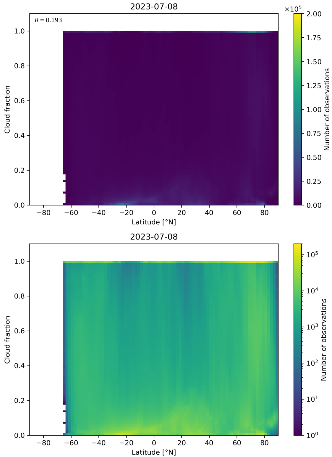
Figure 99: Scatter density plot of “Latitude” against “Cloud fraction” for 2023-07-08 to 2023-07-09.
