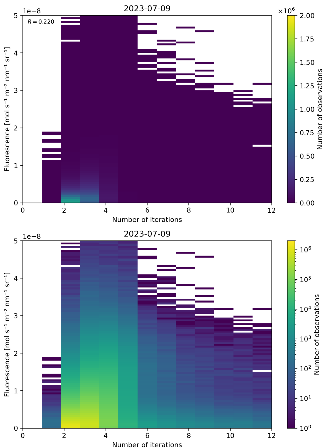
Figure 107: Scatter density plot of “Number of iterations” against “Fluorescence” for 2023-07-08 to 2023-07-10.
