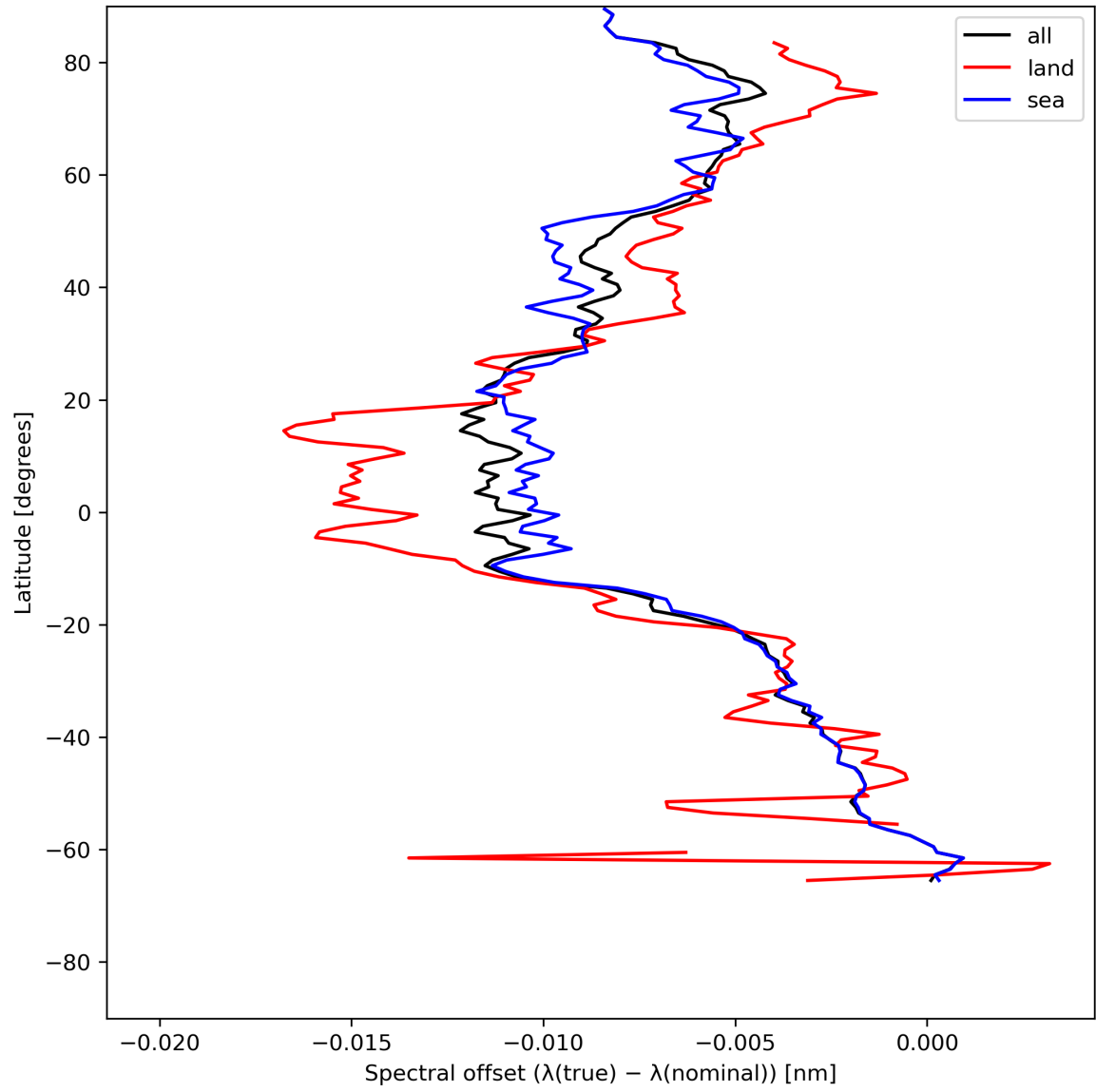
Figure 28: Zonal average of “Spectral offset ( \lambda(\text{true}) - \lambda(\text{nominal}) )” for 2023-07-08 to 2023-07-10.
