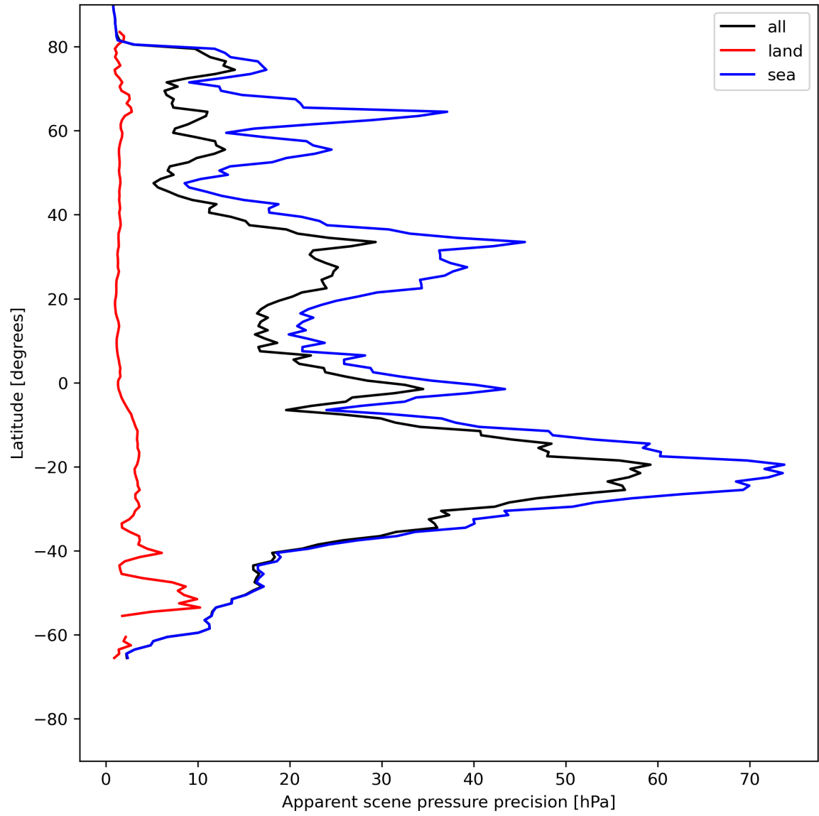
Figure 20: Zonal average of “Apparent scene pressure precision” for 2023-07-08 to 2023-07-10.
