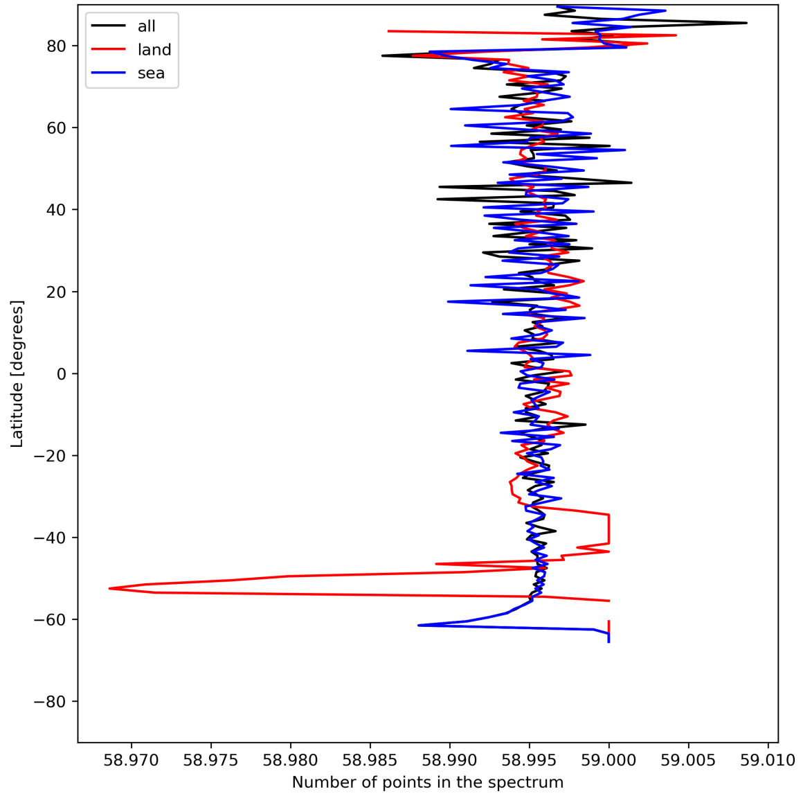
Figure 27: Zonal average of “Number of points in the spectrum” for 2023-07-08 to 2023-07-10.
