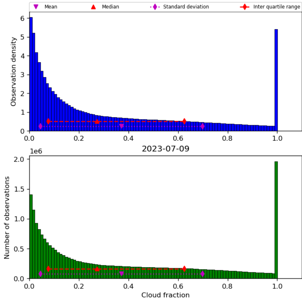
Figure 32: Histogram of “Cloud fraction” for 2023-07-08 to 2023-07-10
