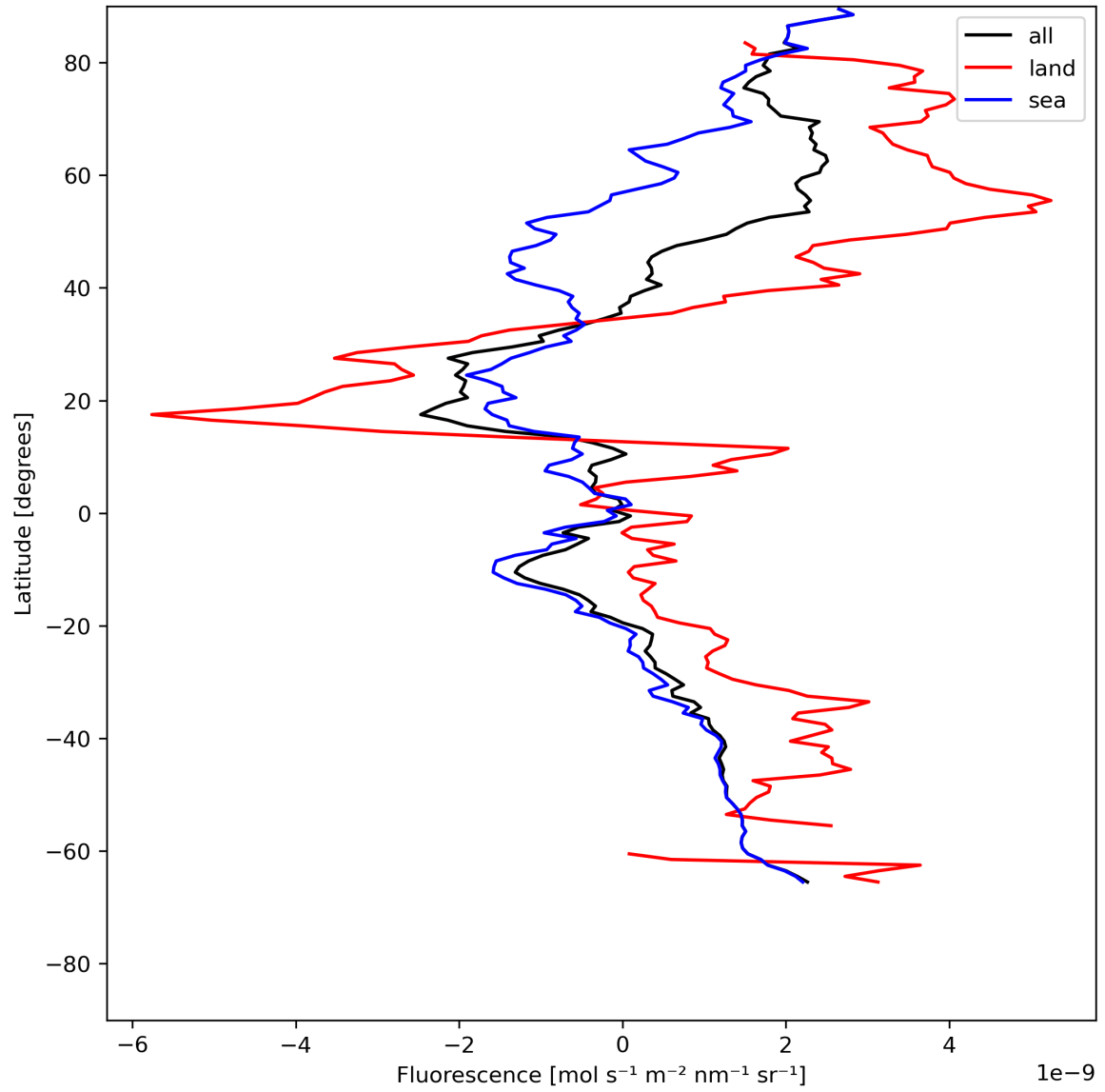
Figure 23: Zonal average of “Fluorescence” for 2023-07-08 to 2023-07-10.
