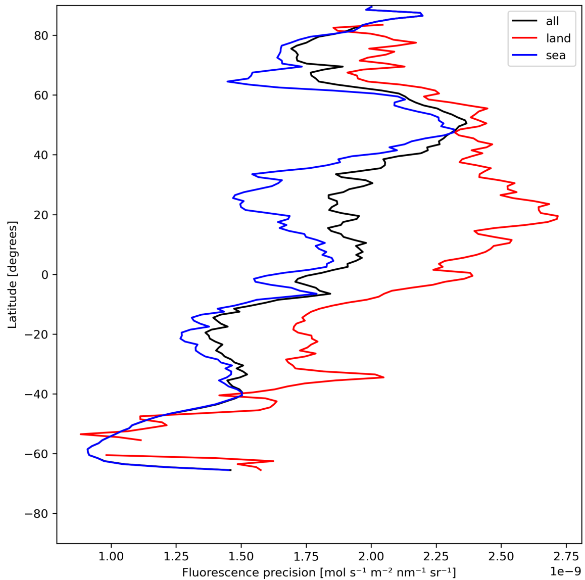
Figure 24: Zonal average of “Fluorescence precision” for 2023-07-08 to 2023-07-10.
