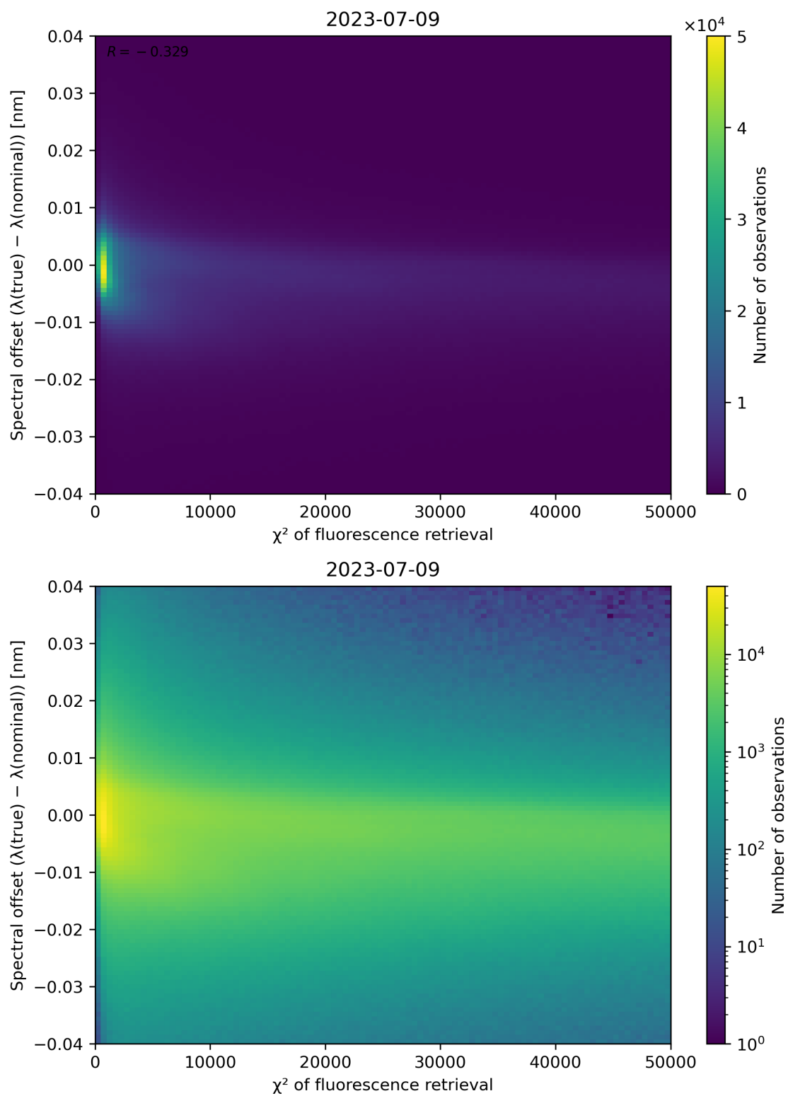
Figure 72: Scatter density plot of “ \chi^2 of fluorescence retrieval” against “Spectral offset ( \lambda(\text{true}) - \lambda(\text{nominal}) )” for 2023-07-08 to 2023-07-10.
