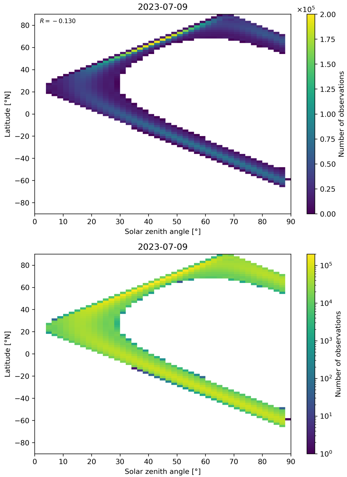
Figure 124: Scatter density plot of “Solar zenith angle” against “Latitude” for 2023-07-08 to 2023-07-10.
