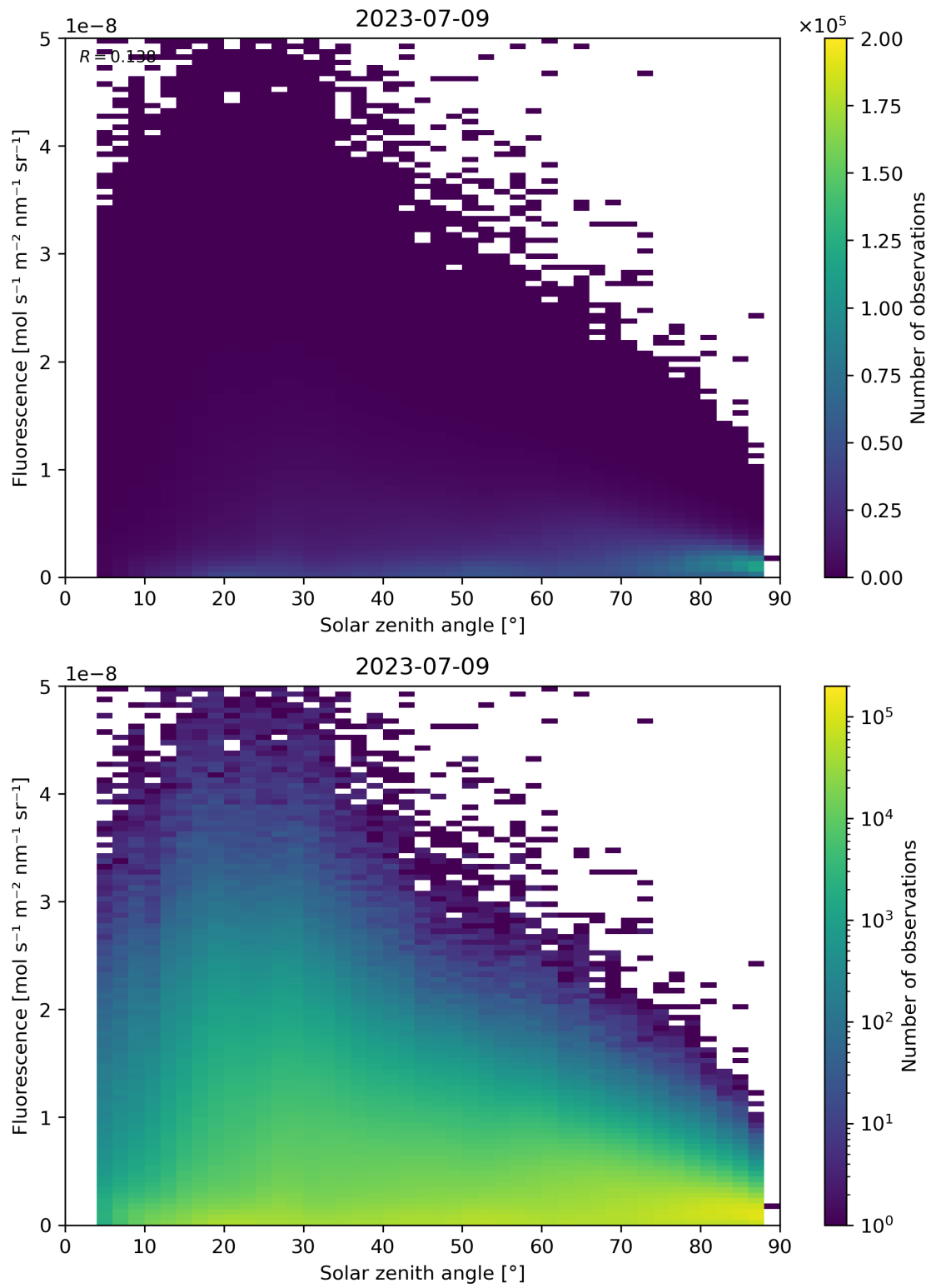
Figure 123: Scatter density plot of “Solar zenith angle” against “Fluorescence” for 2023-07-08 to 2023-07-10.
