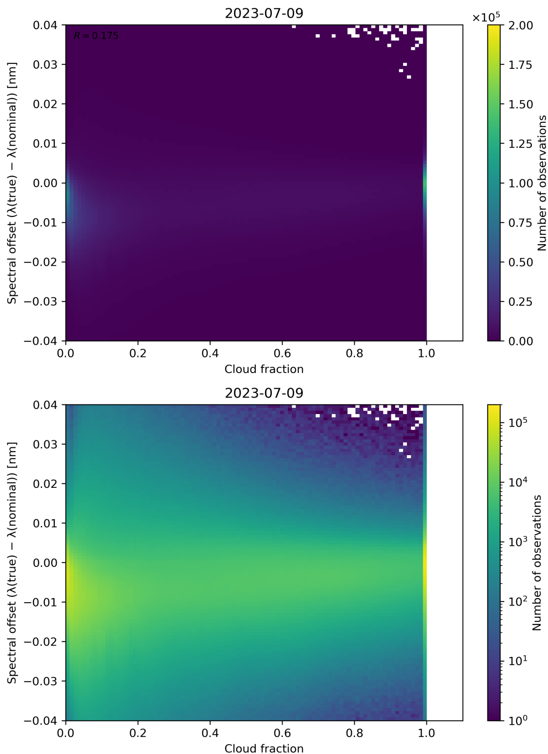
Figure 83: Scatter density plot of “Cloud fraction” against “Spectral offset ( \lambda(\text{true}) - \lambda(\text{nominal}) )” for 2023-07-08 to 2023-07-10.
