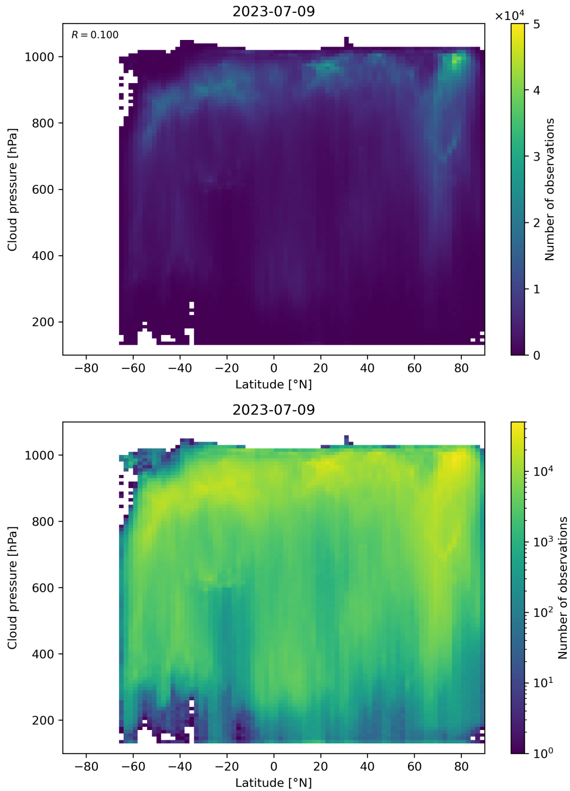
Figure 100: Scatter density plot of “Latitude” against “Cloud pressure” for 2023-07-08 to 2023-07-10.
