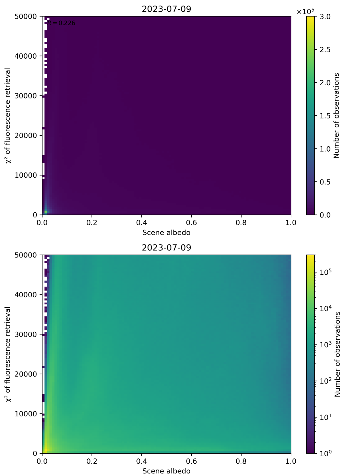
Figure 113: Scatter density plot of “Scene albedo” against “ \chi^2 of fluorescence retrieval” for 2023-07-08 to 2023-07-10.
