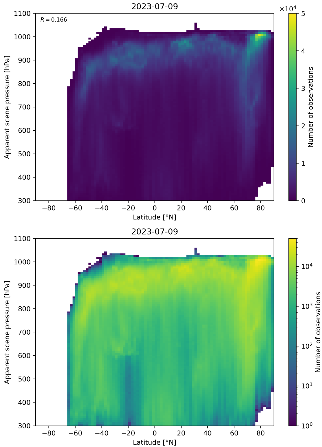
Figure 96: Scatter density plot of “Latitude” against “Apparent scene pressure” for 2023-07-08 to 2023-07-10.
