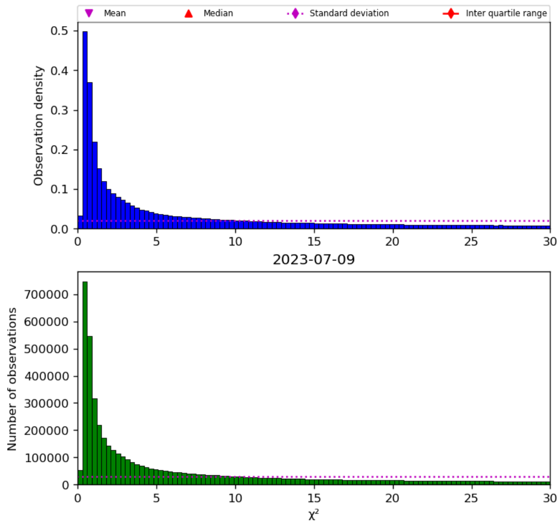
Figure 38: Histogram of “ \chi^2 ” for 2023-07-08 to 2023-07-10
