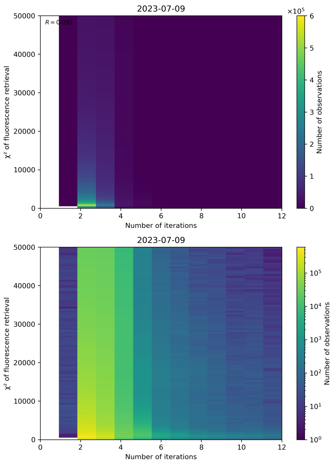
Figure 106: Scatter density plot of “Number of iterations” against “ \chi^2 of fluorescence retrieval” for 2023-07-08 to 2023-07-10.
