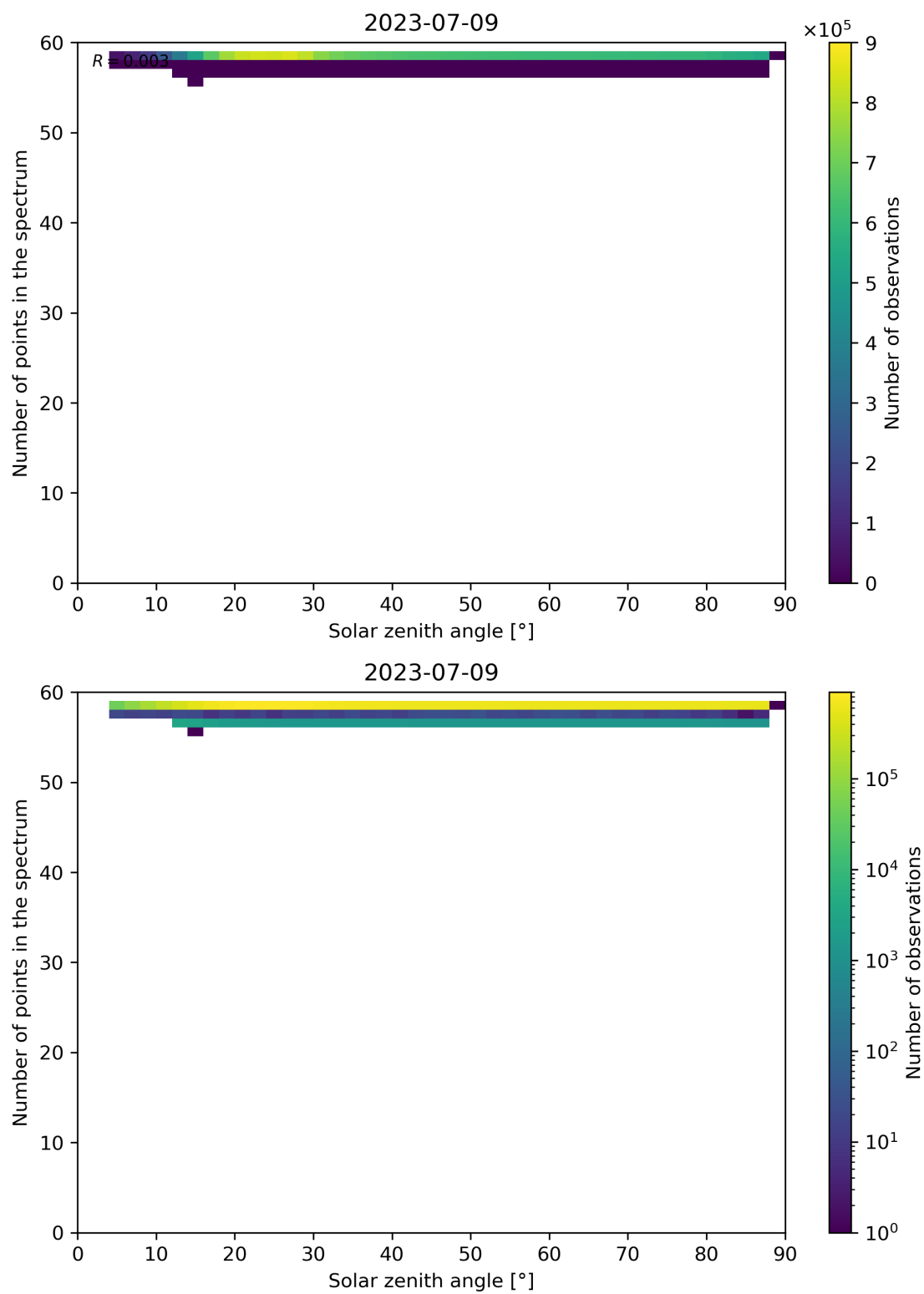
Figure 126: Scatter density plot of “Solar zenith angle” against “Number of points in the spectrum” for 2023-07-08 to 2023-07-10.
