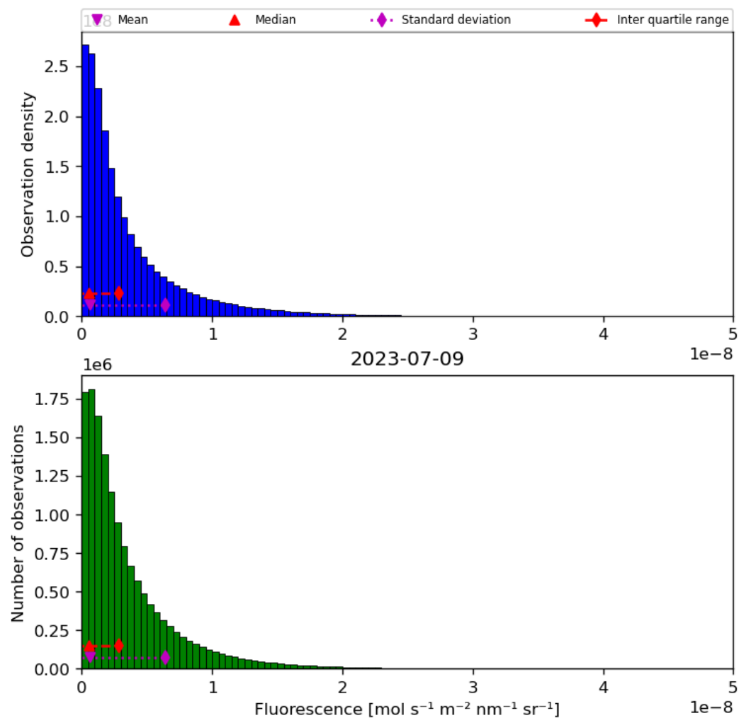
Figure 40: Histogram of “Fluorescence” for 2023-07-08 to 2023-07-10
