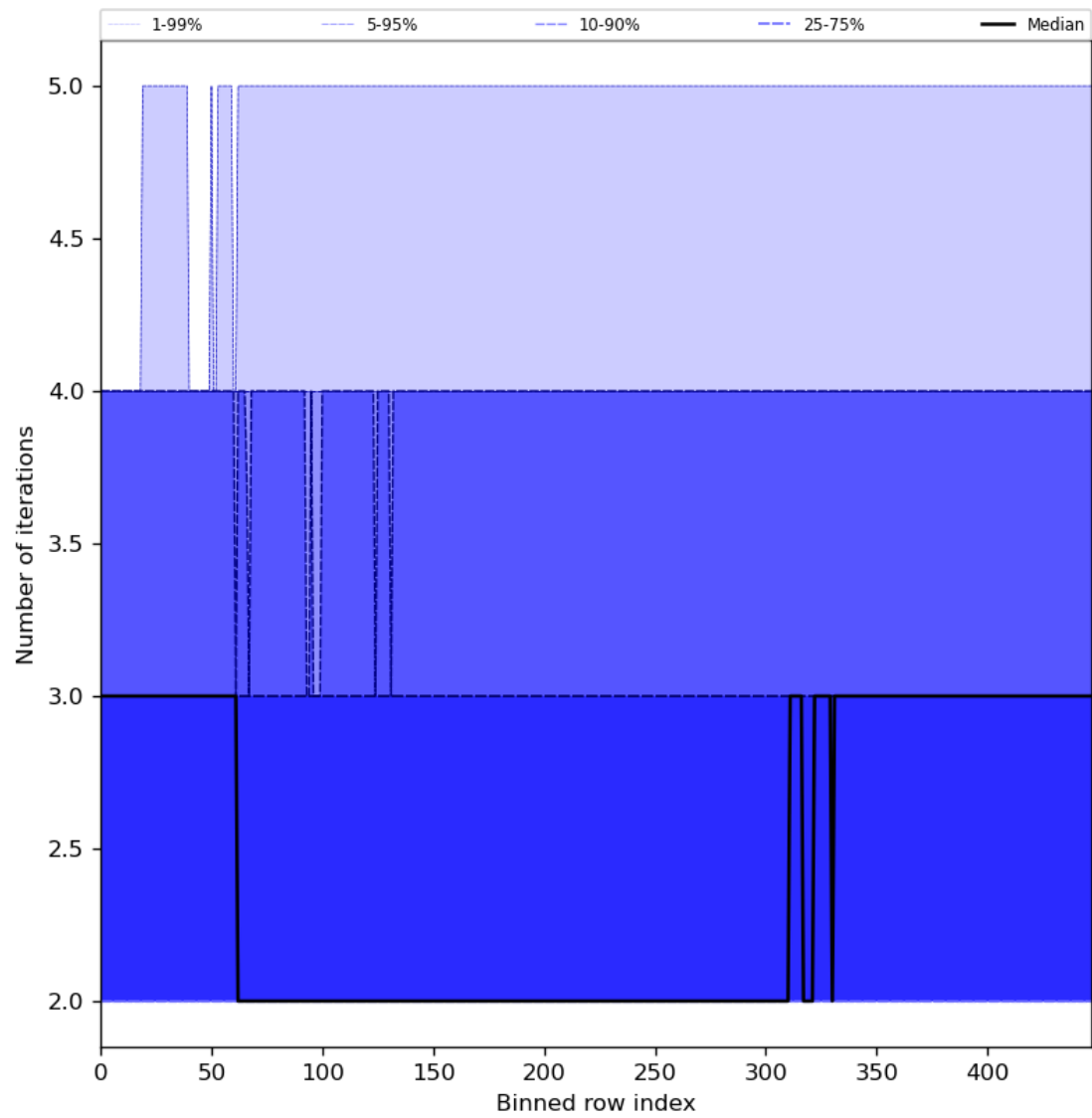
Figure 56: Along track statistics of “Number of iterations” for 2023-07-08 to 2023-07-10
