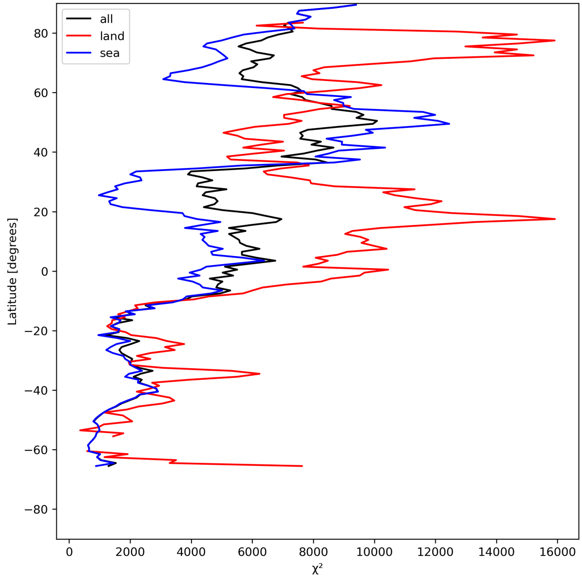
Figure 21: Zonal average of “ \chi^2 ” for 2023-07-08 to 2023-07-10.
