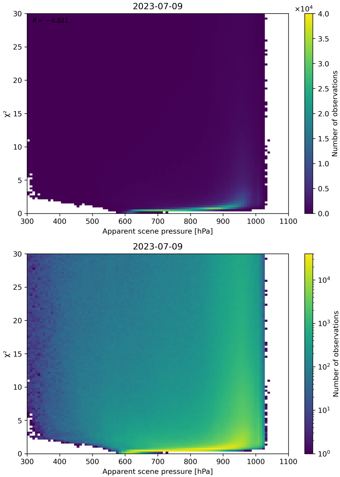
Figure 63: Scatter density plot of “Apparent scene pressure” against “ \chi^2 ” for 2023-07-08 to 2023-07-10.
