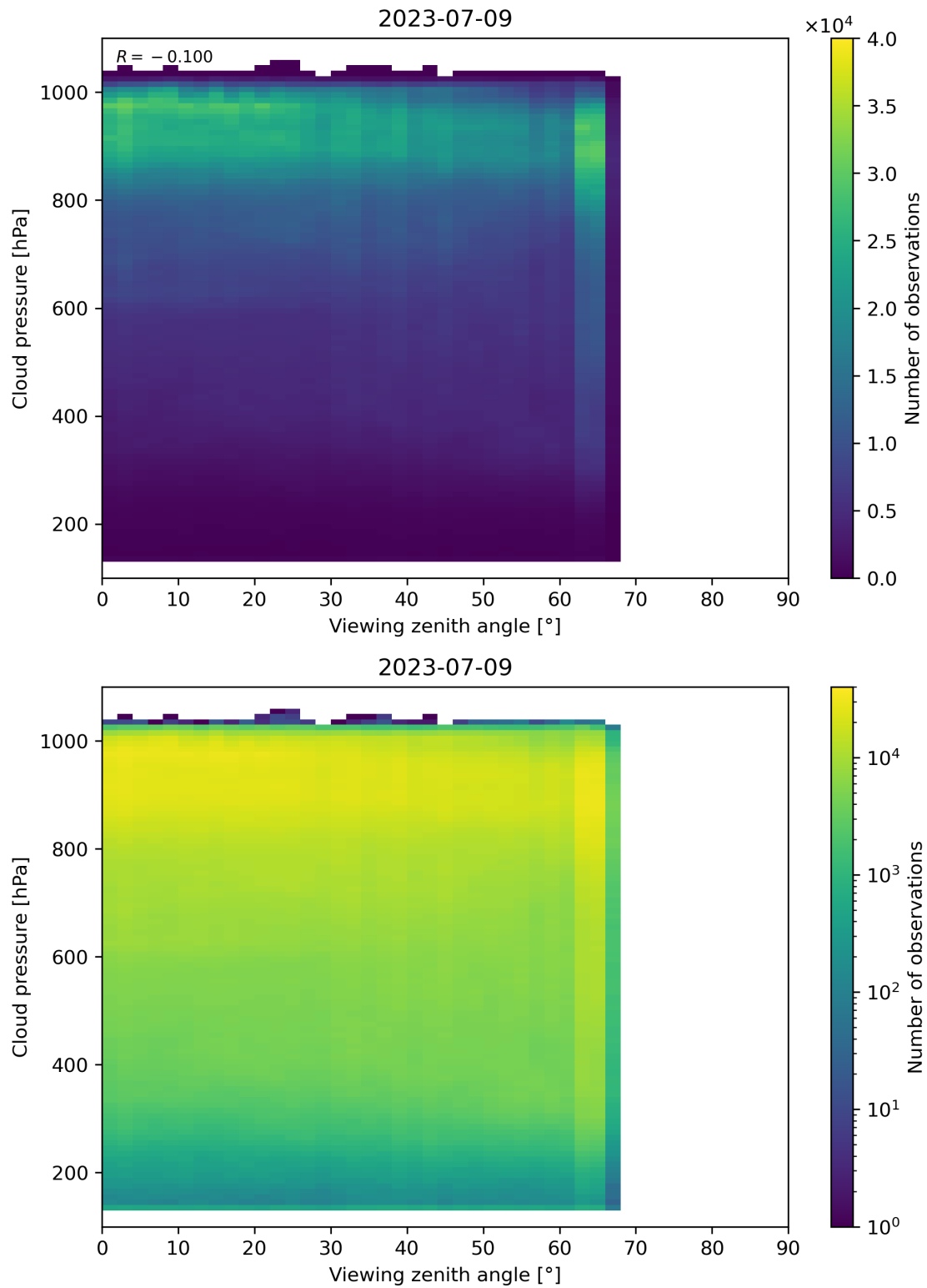
Figure 133: Scatter density plot of “Viewing zenith angle” against “Cloud pressure” for 2023-07-08 to 2023-07-10.
