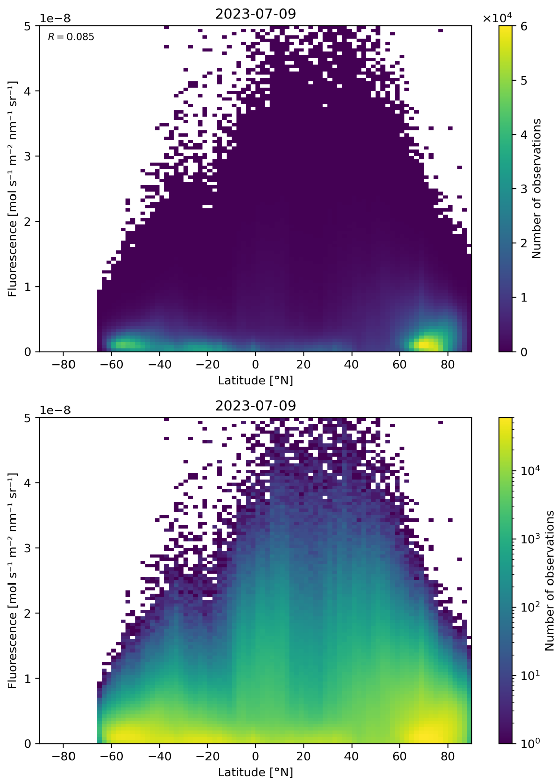
Figure 101: Scatter density plot of “Latitude” against “Fluorescence” for 2023-07-08 to 2023-07-10.
