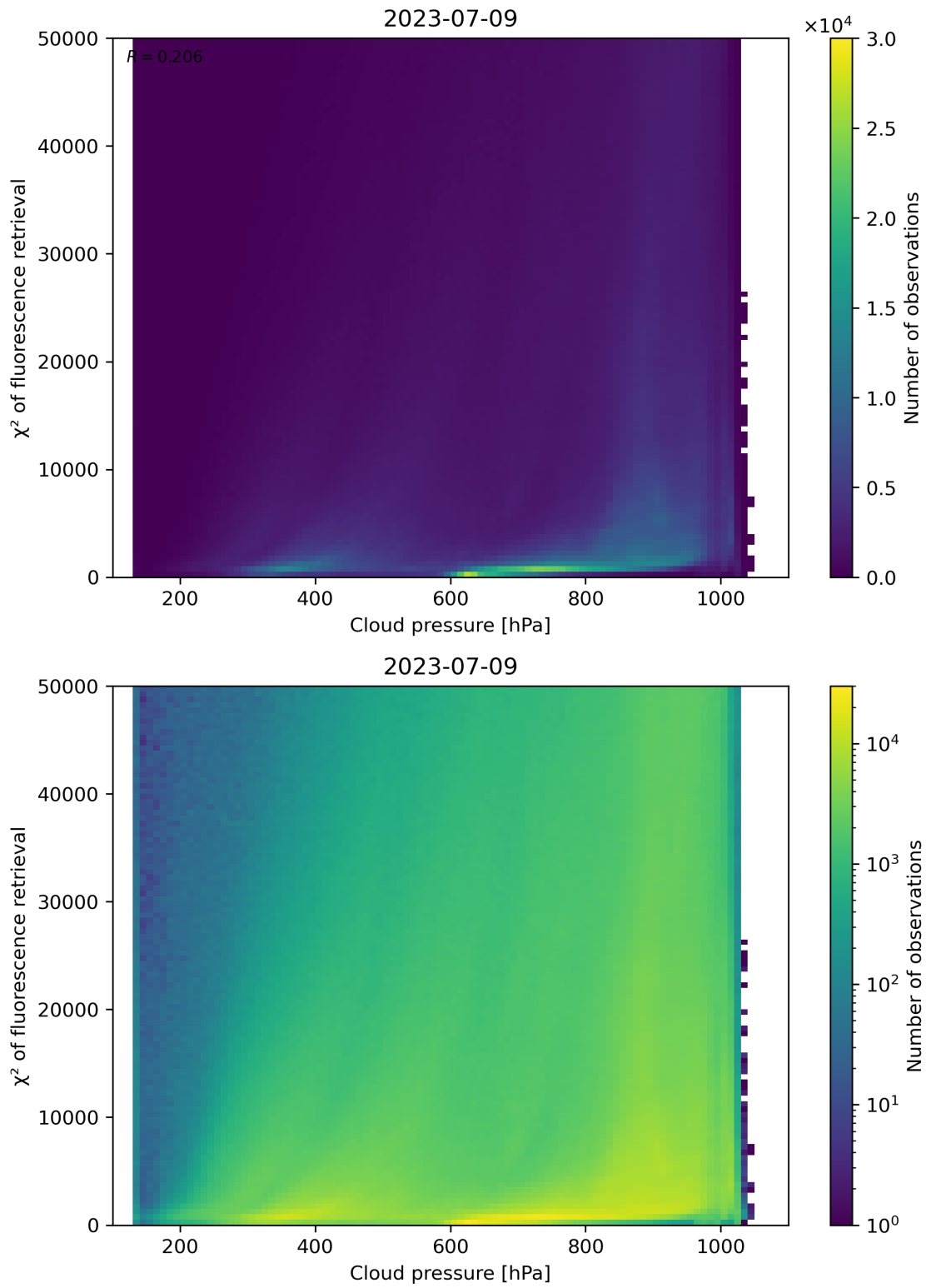
Figure 86: Scatter density plot of “Cloud pressure” against “ \chi^2 of fluorescence retrieval” for 2023-07-08 to 2023-07-10.
