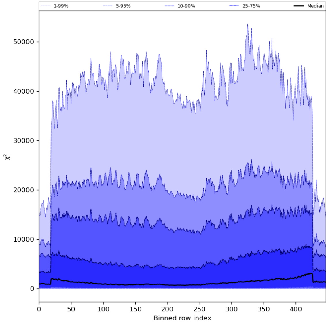
Figure 55: Along track statistics of “ \chi^2 ” for 2023-07-08 to 2023-07-10
