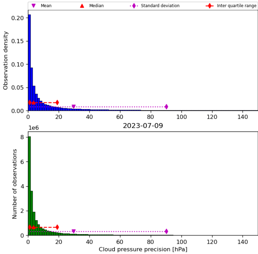
Figure 31: Histogram of “Cloud pressure precision” for 2023-07-08 to 2023-07-10
