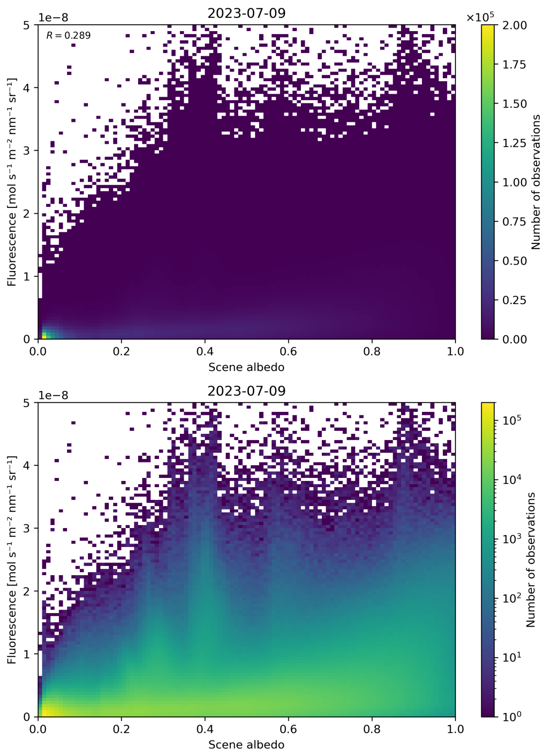
Figure 114: Scatter density plot of “Scene albedo” against “Fluorescence” for 2023-07-08 to 2023-07-10.
