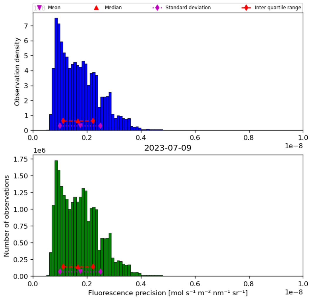
Figure 41: Histogram of “Fluorescence precision” for 2023-07-08 to 2023-07-10
