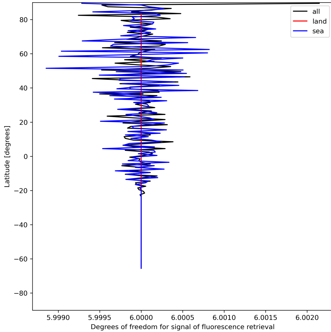
Figure 26: Zonal average of “Degrees of freedom for signal of fluorescence retrieval” for 2023-07-08 to 2023-07-10.
