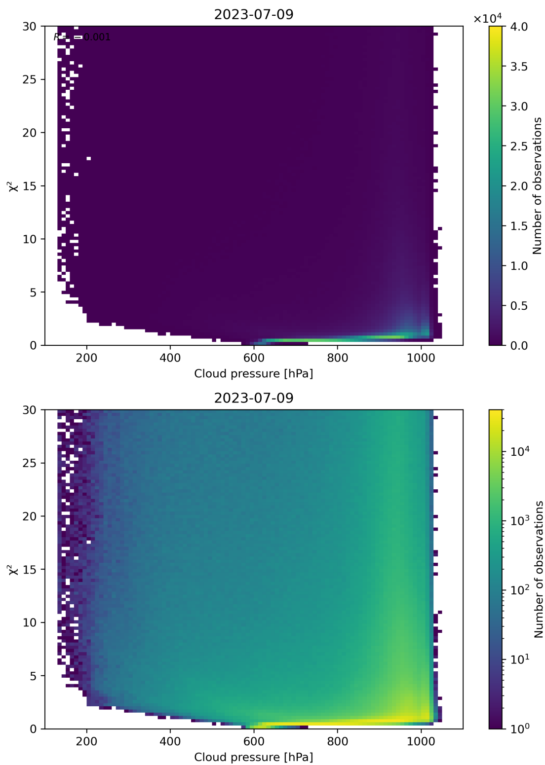
Figure 85: Scatter density plot of “Cloud pressure” against “ \chi^2 ” for 2023-07-08 to 2023-07-10.
