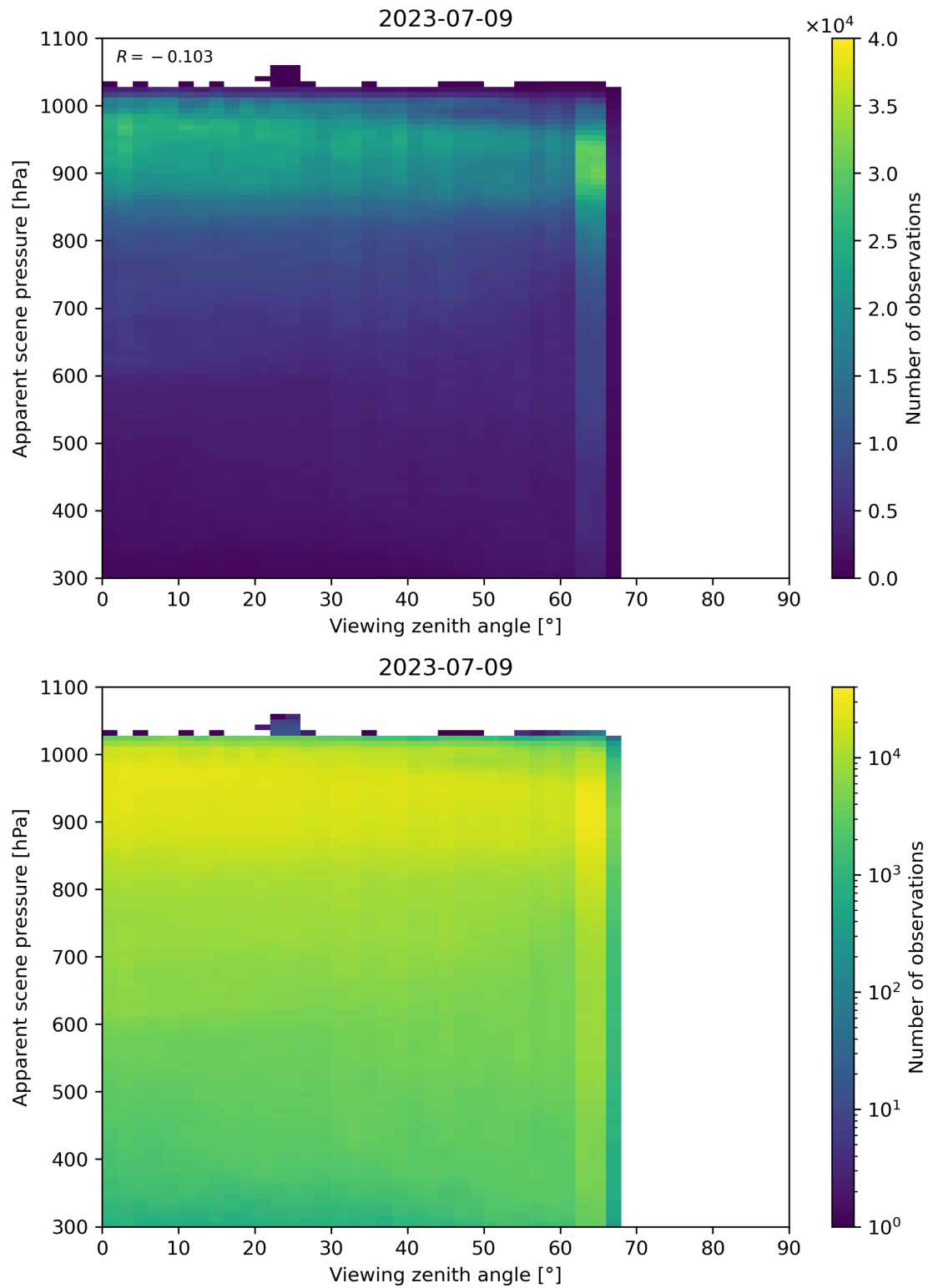
Figure 129: Scatter density plot of “Viewing zenith angle” against “Apparent scene pressure” for 2023-07-08 to 2023-07-10.
