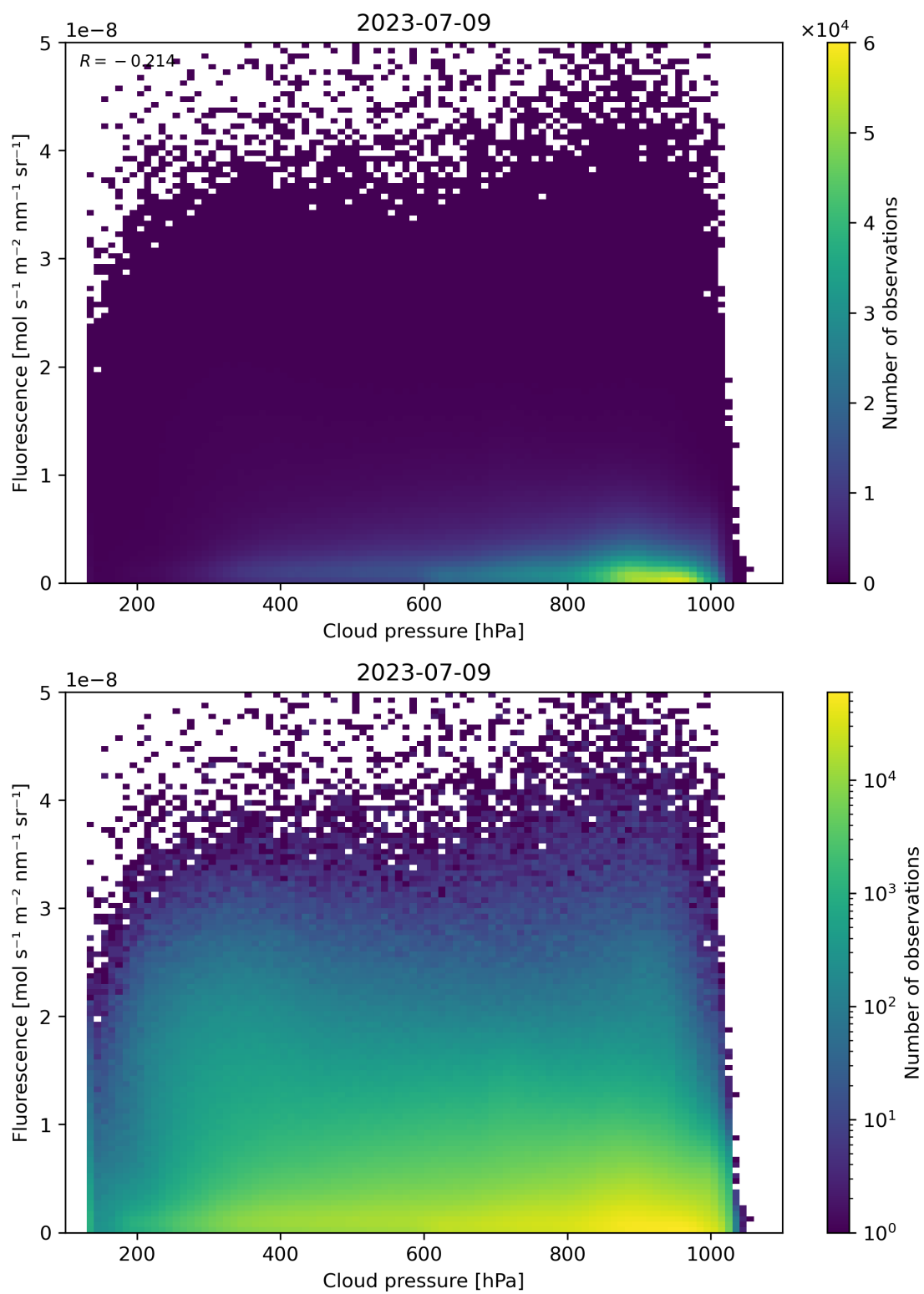
Figure 88: Scatter density plot of “Cloud pressure” against “Fluorescence” for 2023-07-08 to 2023-07-10.
