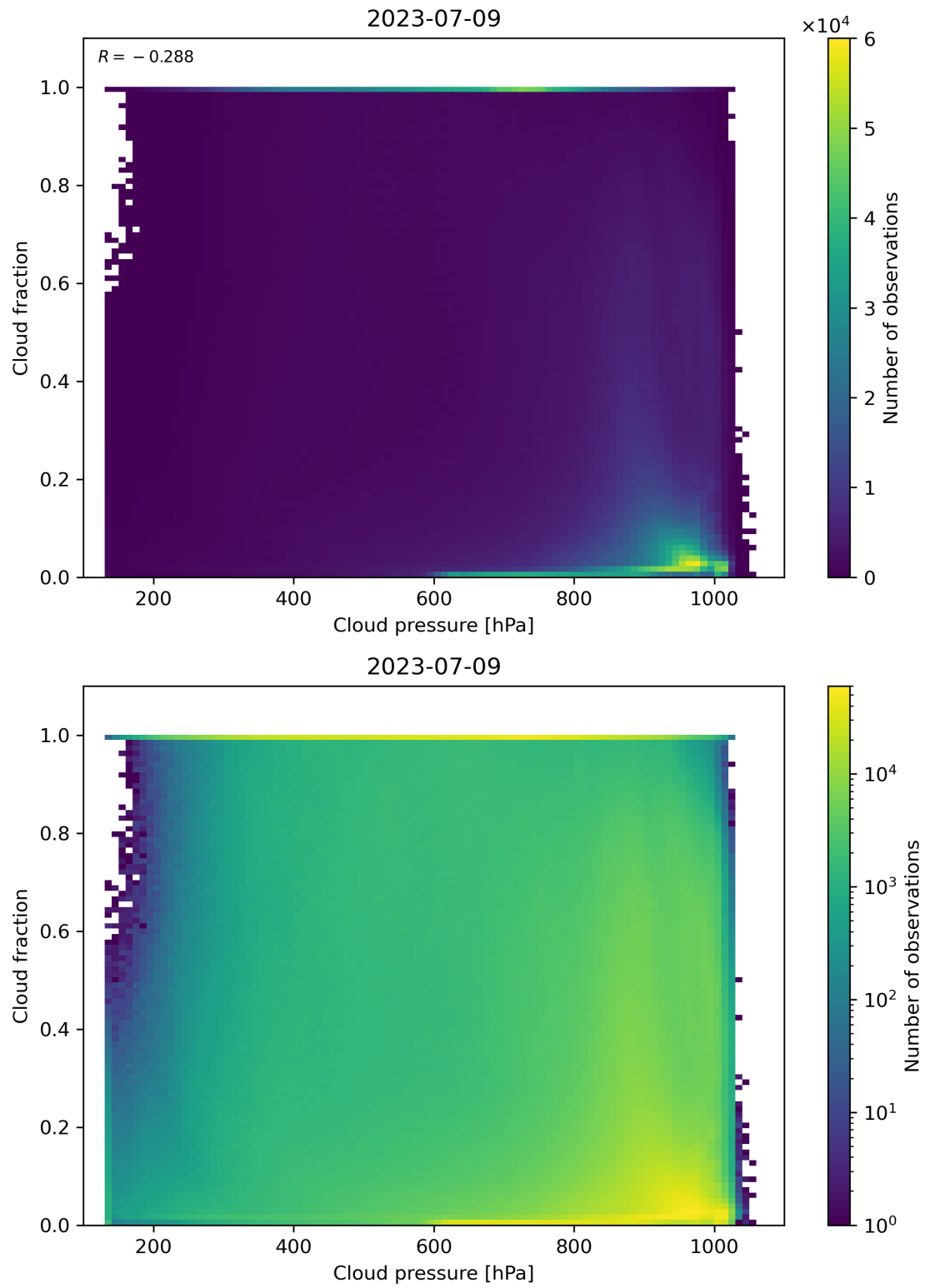
Figure 87: Scatter density plot of “Cloud pressure” against “Cloud fraction” for 2023-07-08 to 2023-07-10.
