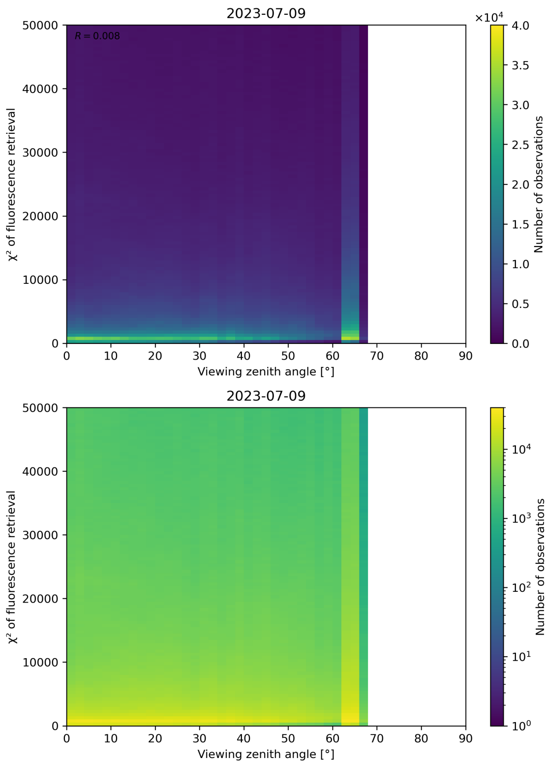
Figure 131: Scatter density plot of “Viewing zenith angle” against “ \chi^2 of fluorescence retrieval” for 2023-07-08 to 2023-07-10.
