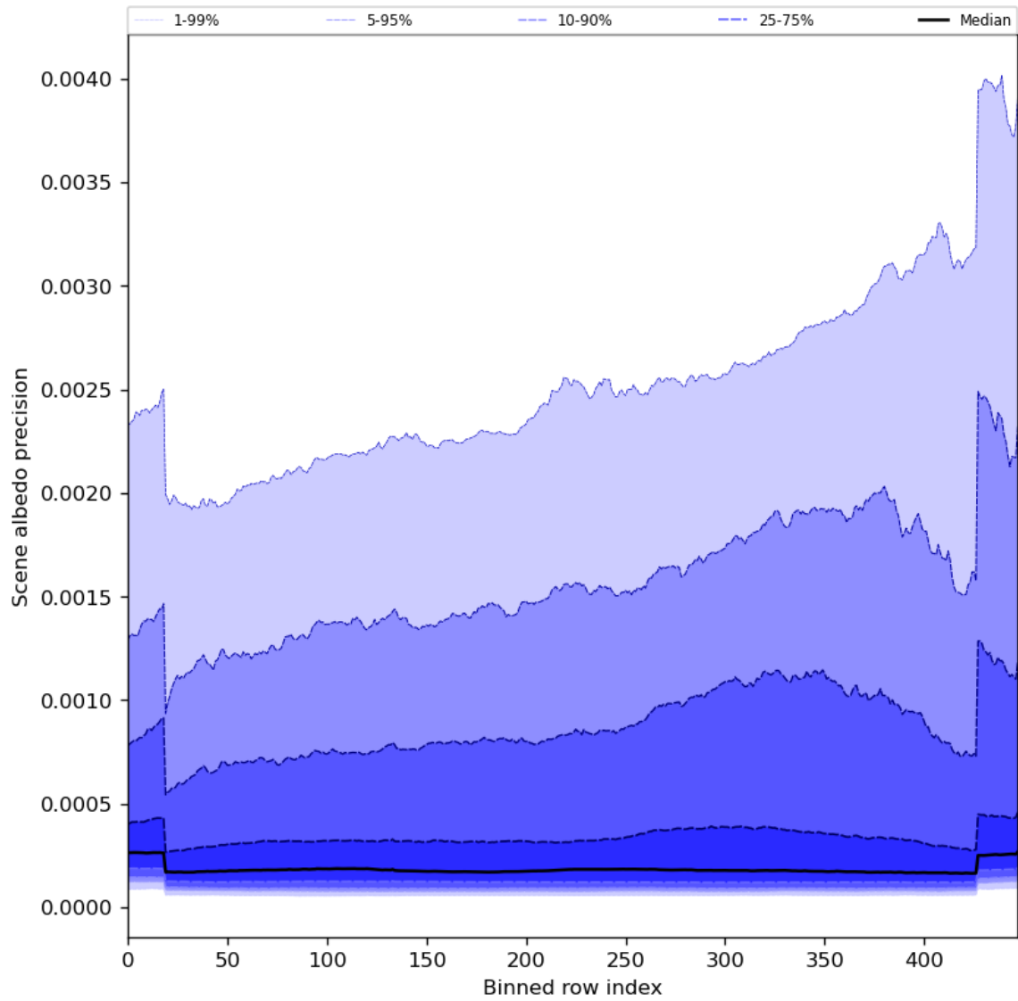
Figure 52: Along track statistics of “Scene albedo precision” for 2023-07-08 to 2023-07-10
