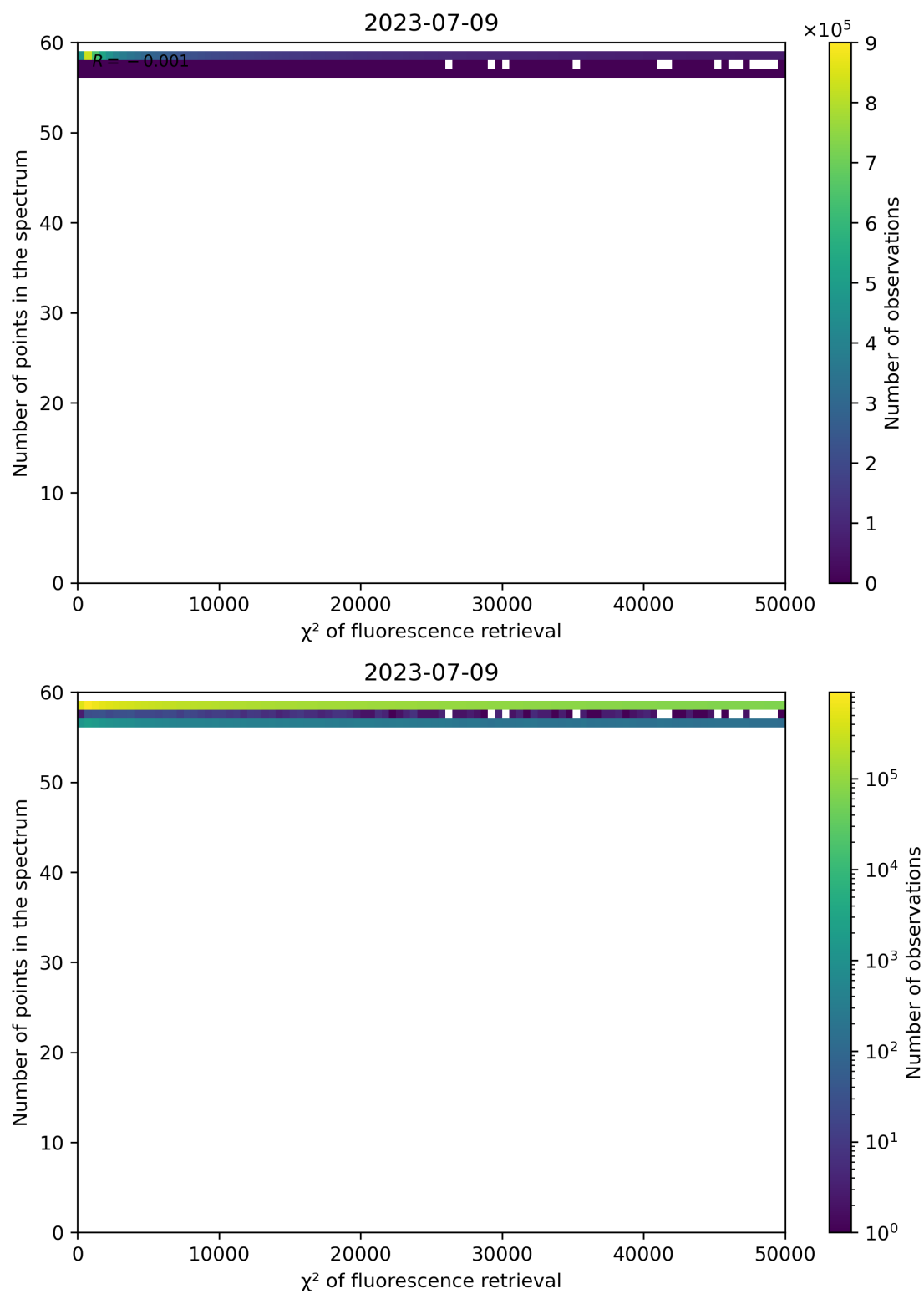
Figure 71: Scatter density plot of “ \chi^2 of fluorescence retrieval” against “Number of points in the spectrum” for 2023-07-08 to 2023-07-10.
