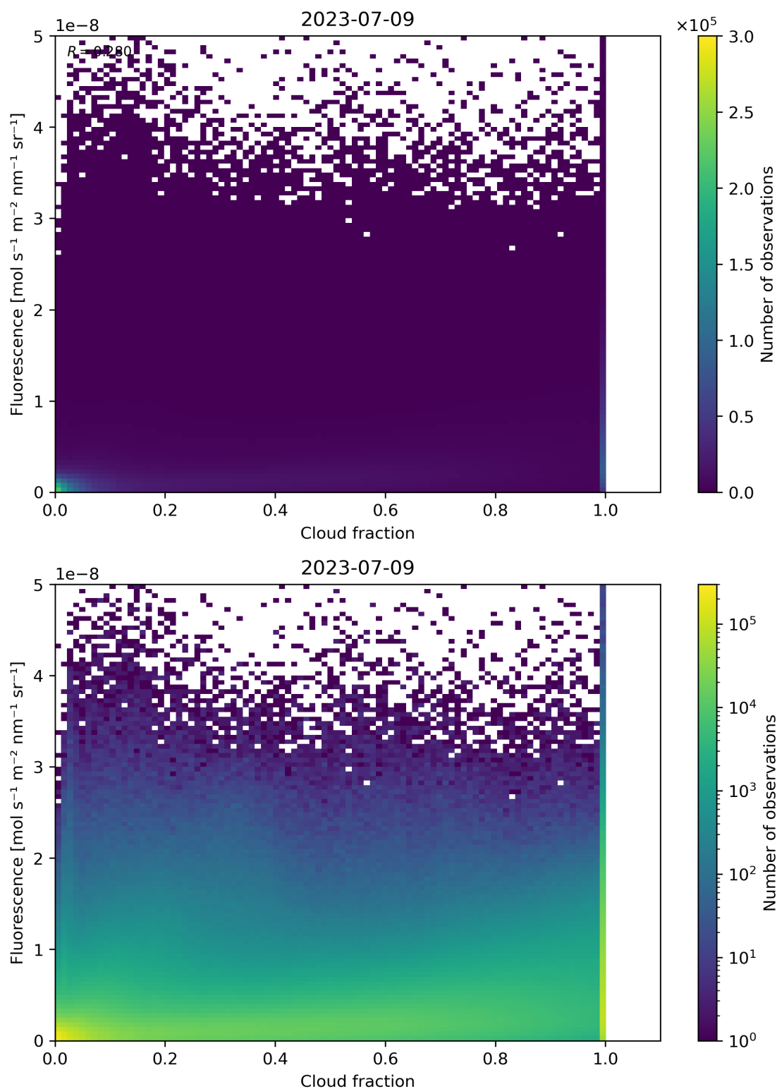
Figure 79: Scatter density plot of “Cloud fraction” against “Fluorescence” for 2023-07-08 to 2023-07-10.
