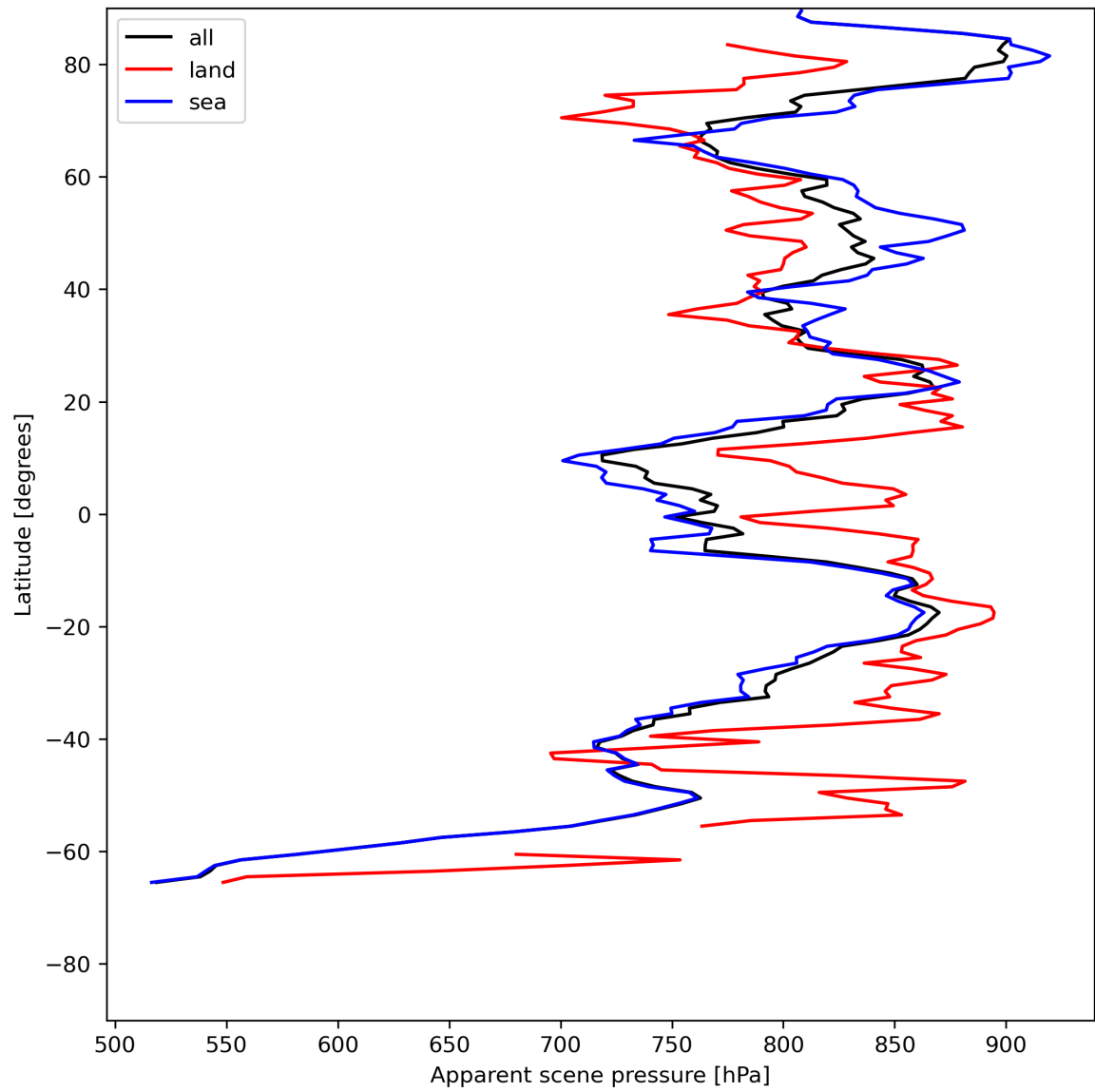
Figure 19: Zonal average of “Apparent scene pressure” for 2023-07-08 to 2023-07-10.
