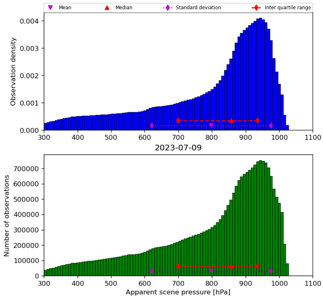
Figure 36: Histogram of “Apparent scene pressure” for 2023-07-08 to 2023-07-10
