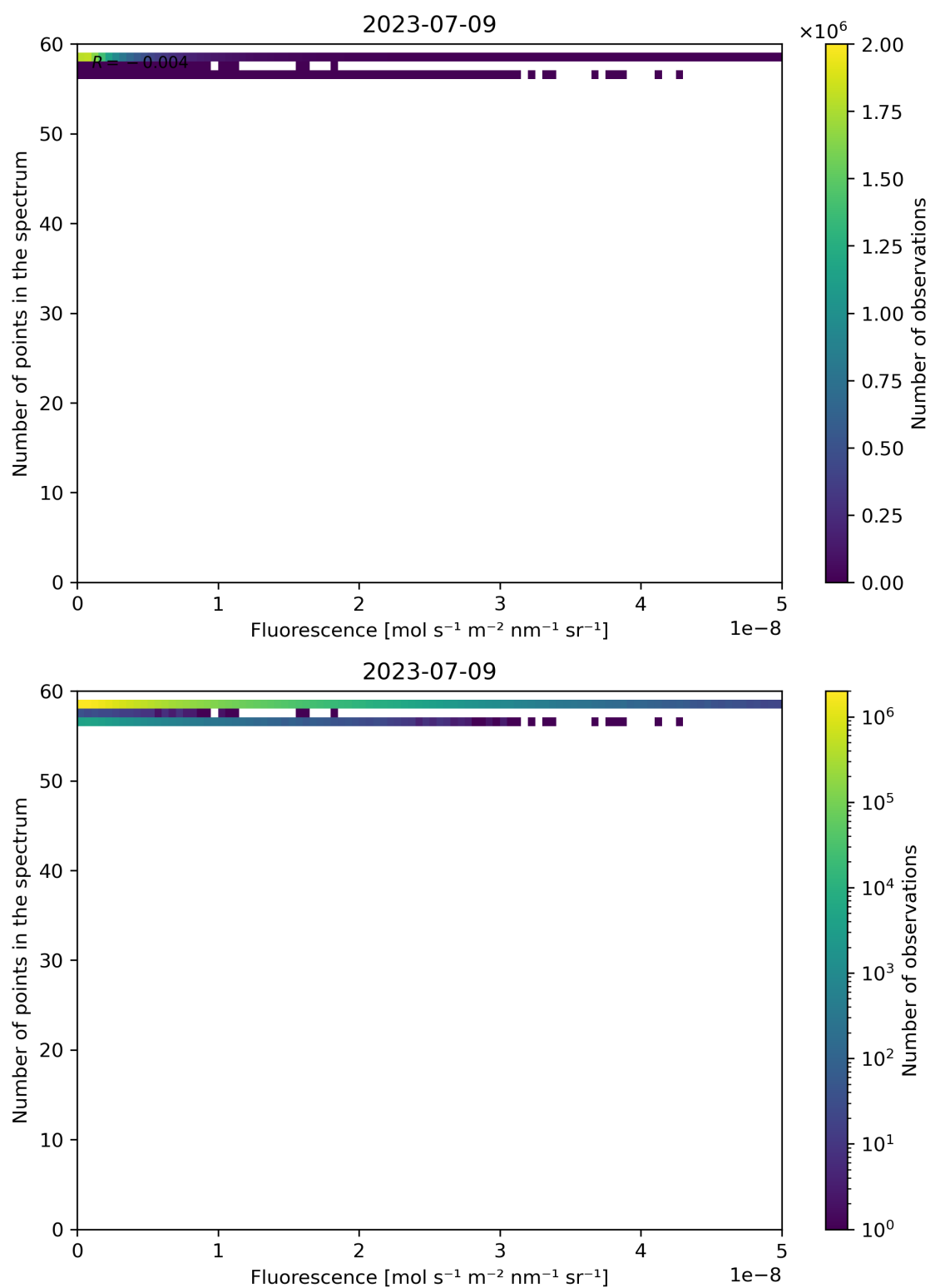
Figure 94: Scatter density plot of “Fluorescence” against “Number of points in the spectrum” for 2023-07-08 to 2023-07-10.
