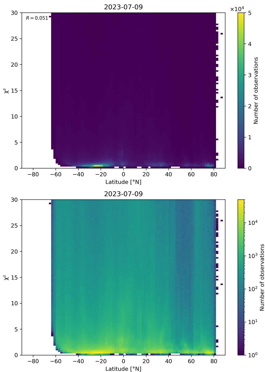
Figure 97: Scatter density plot of “Latitude” against “ \chi^2 ” for 2023-07-08 to 2023-07-10.
