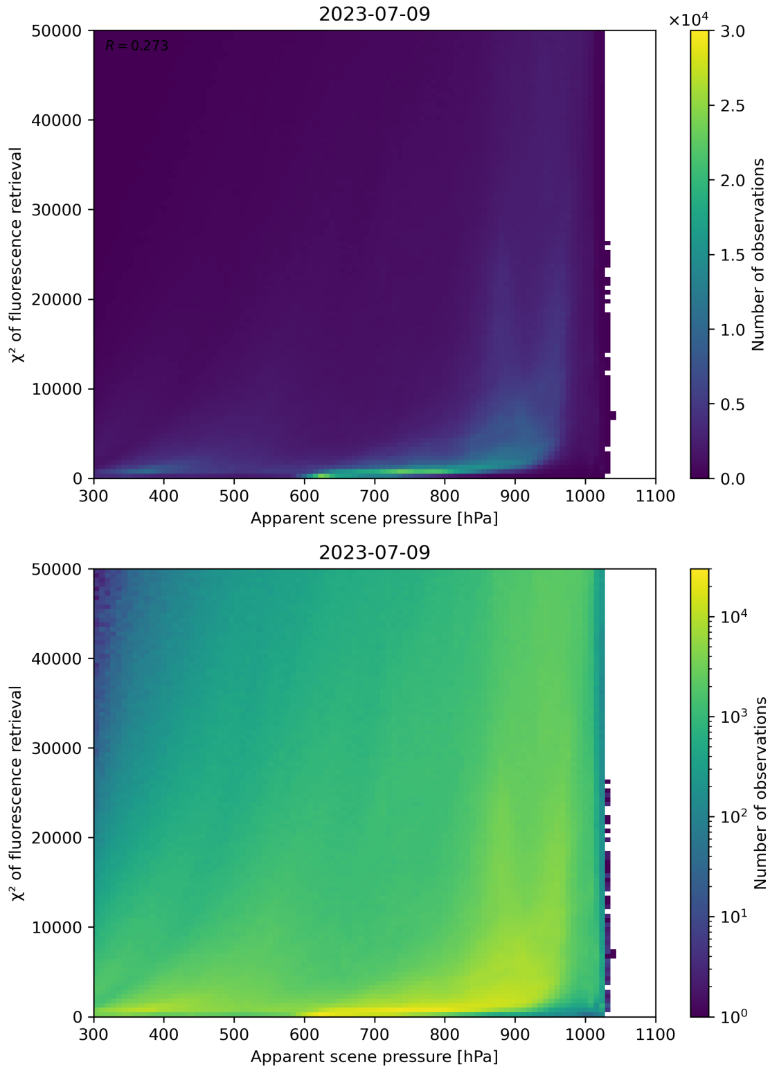
Figure 64: Scatter density plot of “Apparent scene pressure” against “ \chi^2 of fluorescence retrieval” for 2023-07-08 to 2023-07-10.
