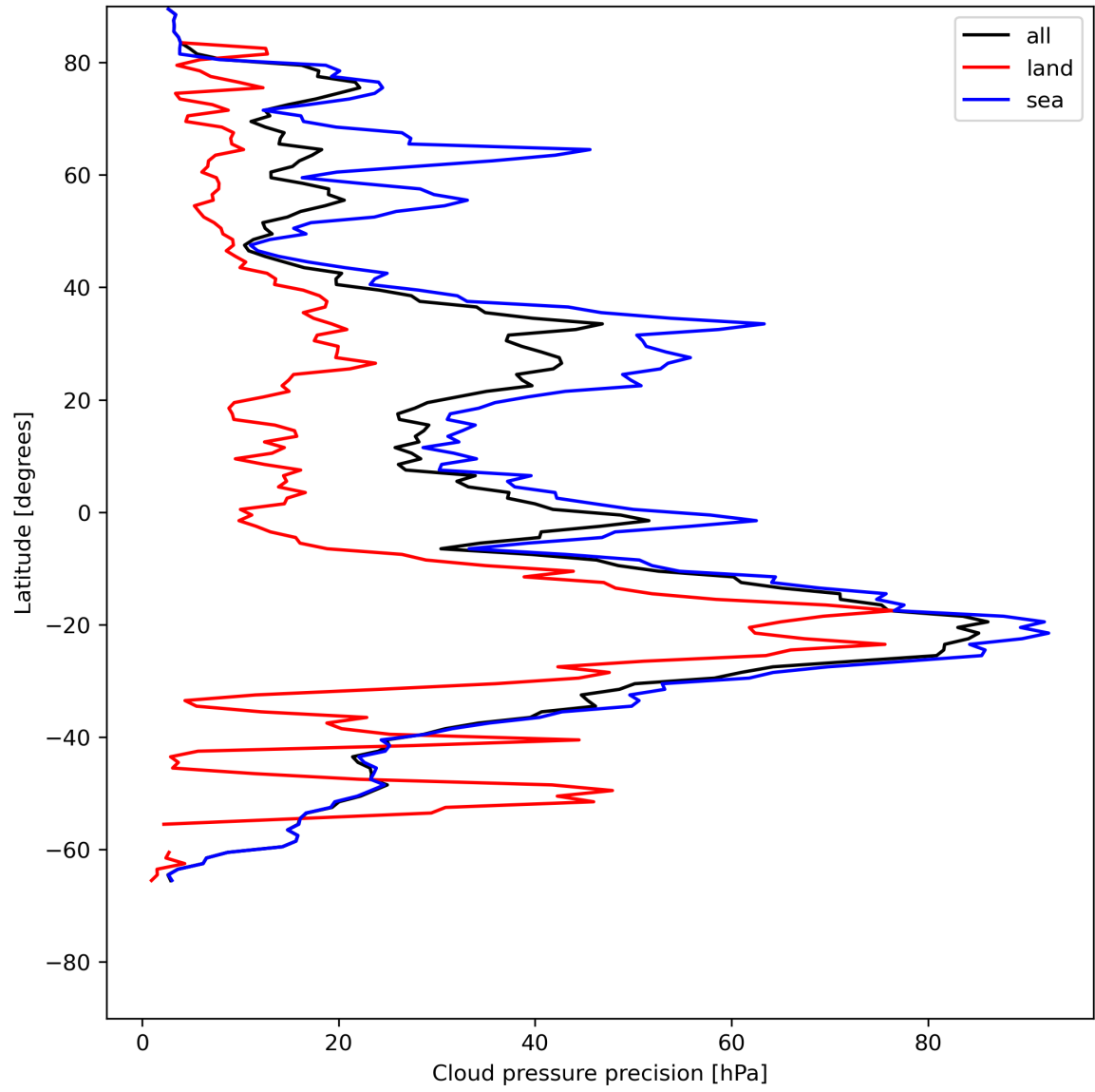
Figure 14: Zonal average of "Cloud pressure precision" for 2023-07-08 to 2023-07-10.
