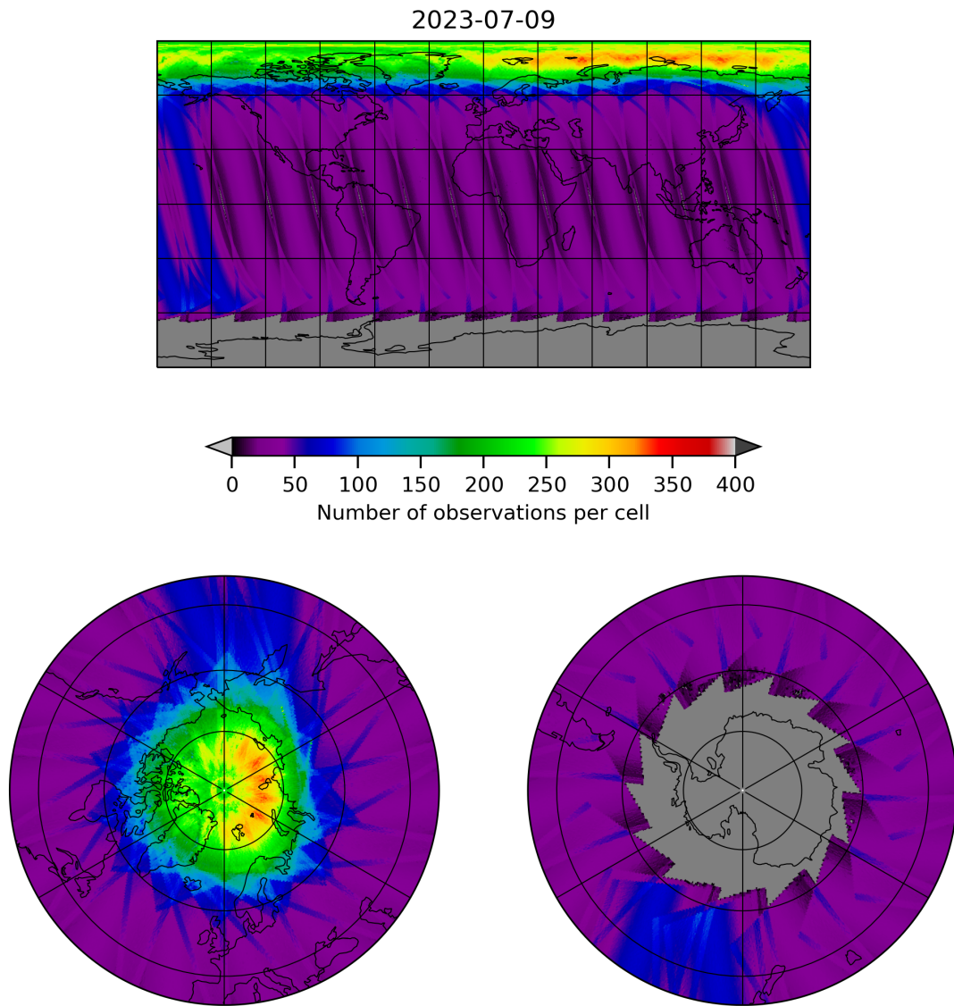
Figure 11: Map of the number of observations for 2023-07-08 to 2023-07-10
