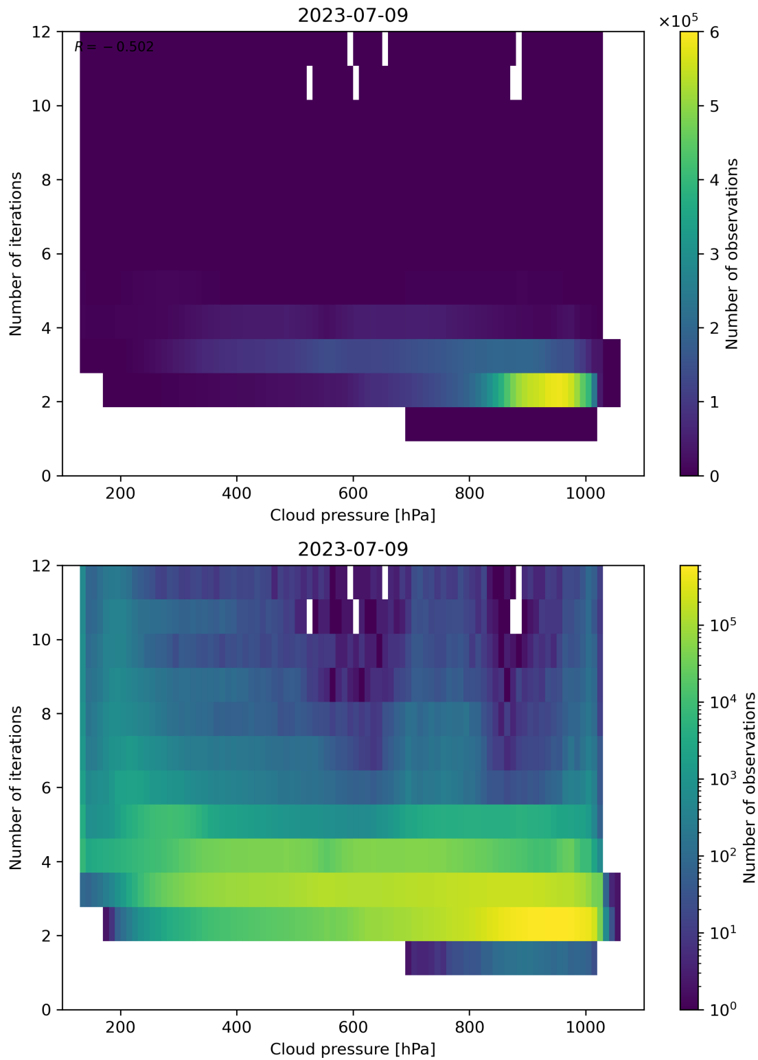
Figure 89: Scatter density plot of “Cloud pressure” against “Number of iterations” for 2023-07-08 to 2023-07-10.
