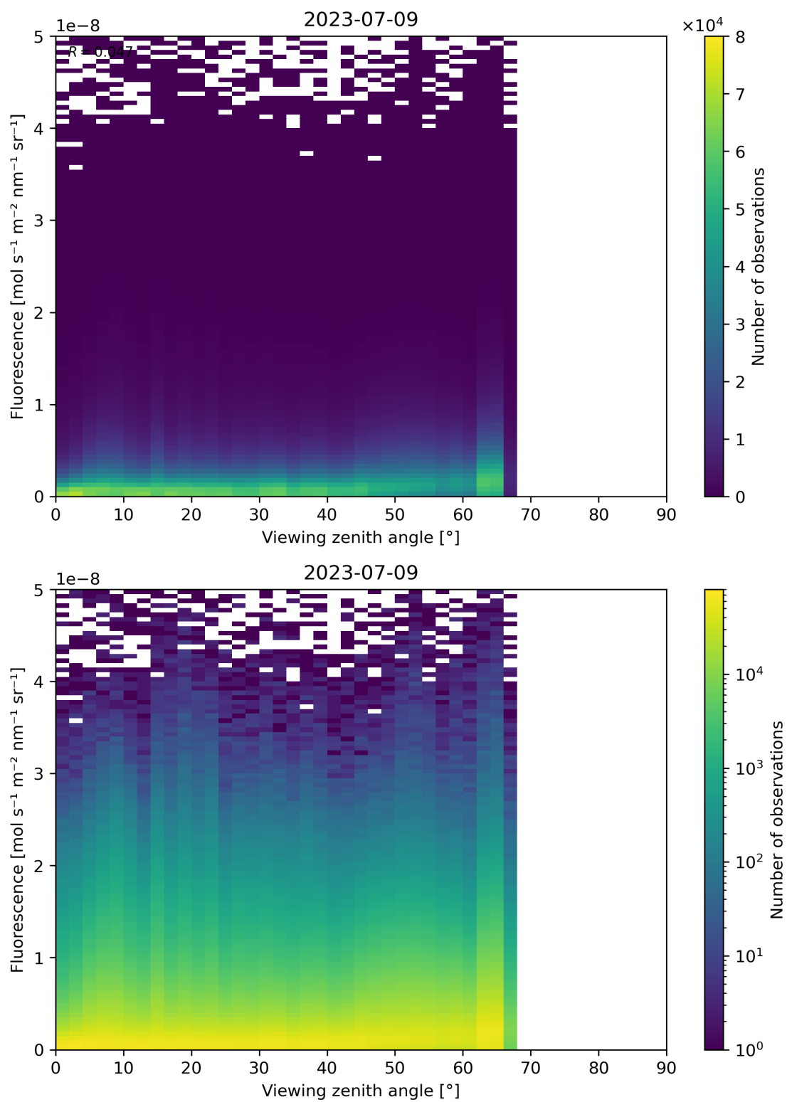
Figure 134: Scatter density plot of “Viewing zenith angle” against “Fluorescence” for 2023-07-08 to 2023-07-10.
