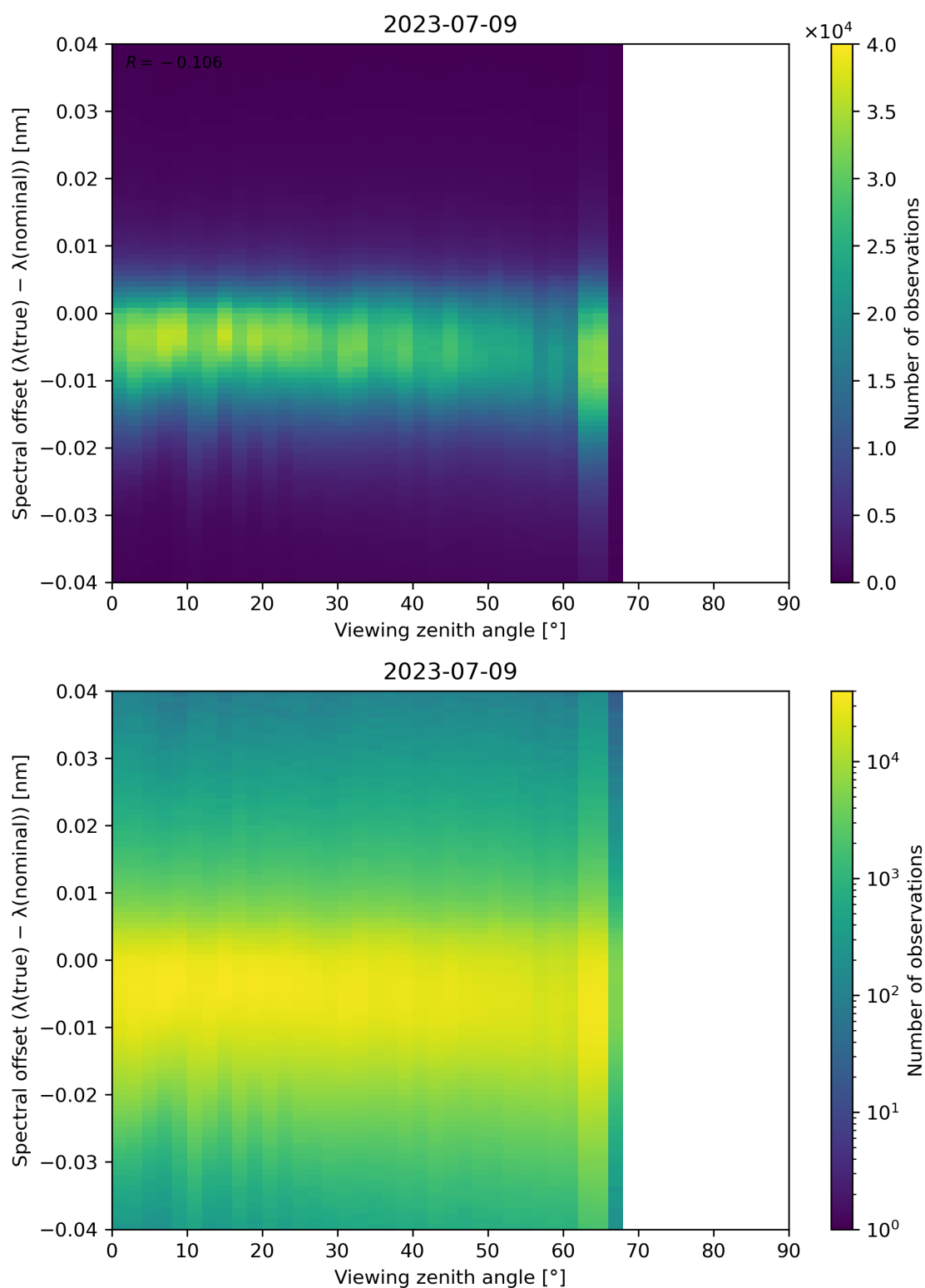
Figure 140: Scatter density plot of “Viewing zenith angle” against “Spectral offset ( \lambda(\text{true}) - \lambda(\text{nominal}) )” for 2023-07-08 to 2023-07-10.
