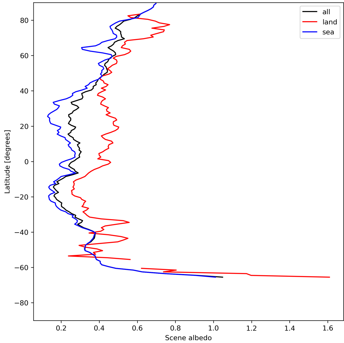
Figure 17: Zonal average of “Scene albedo” for 2023-07-08 to 2023-07-10.
