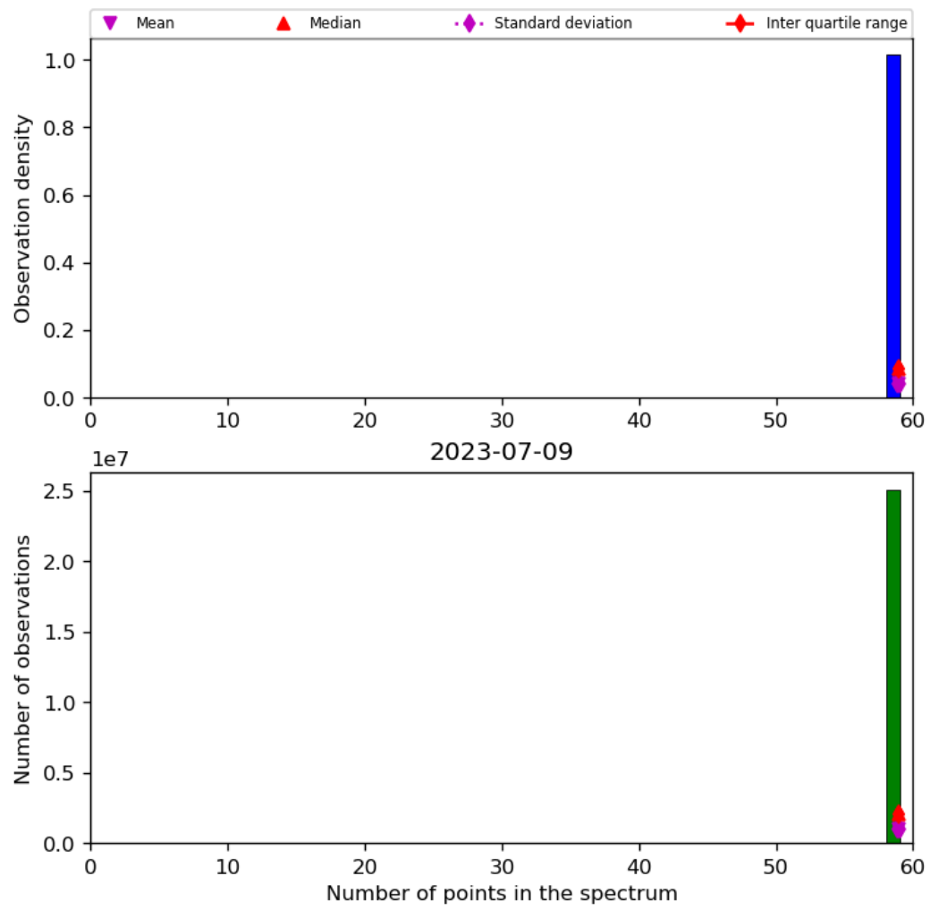
Figure 44: Histogram of “Number of points in the spectrum” for 2023-07-08 to 2023-07-10
