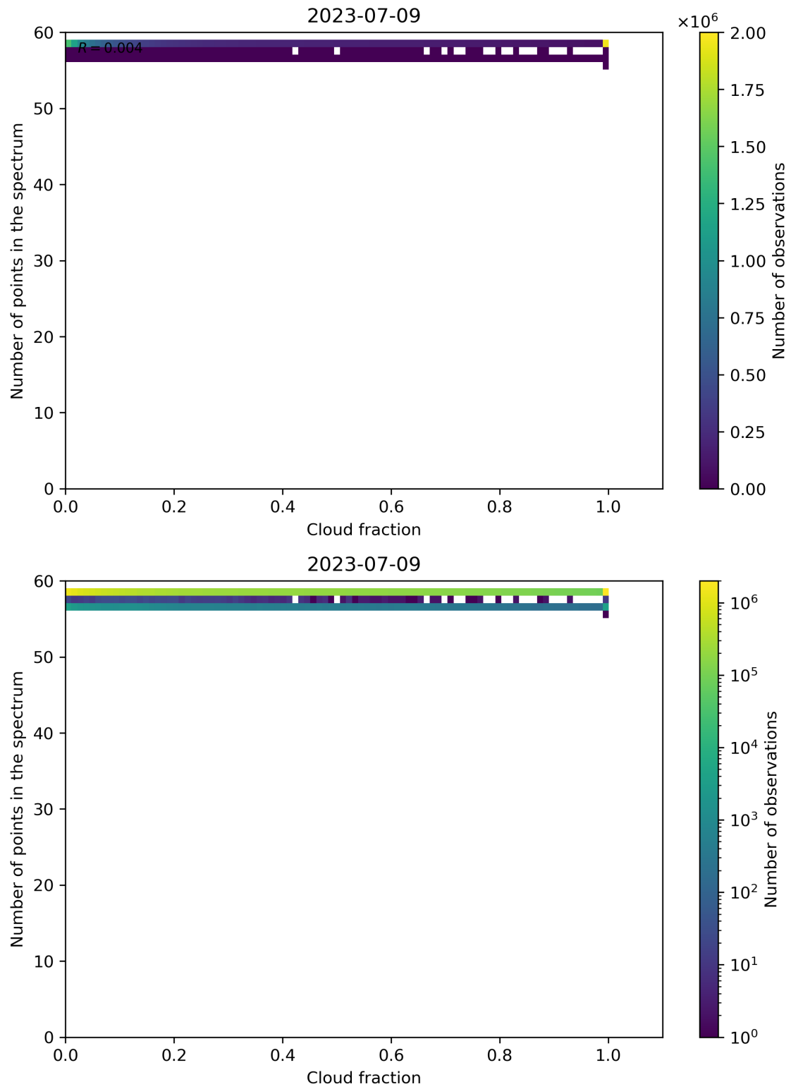
Figure 81: Scatter density plot of “Cloud fraction” against “Number of points in the spectrum” for 2023-07-08 to 2023-07-10.
