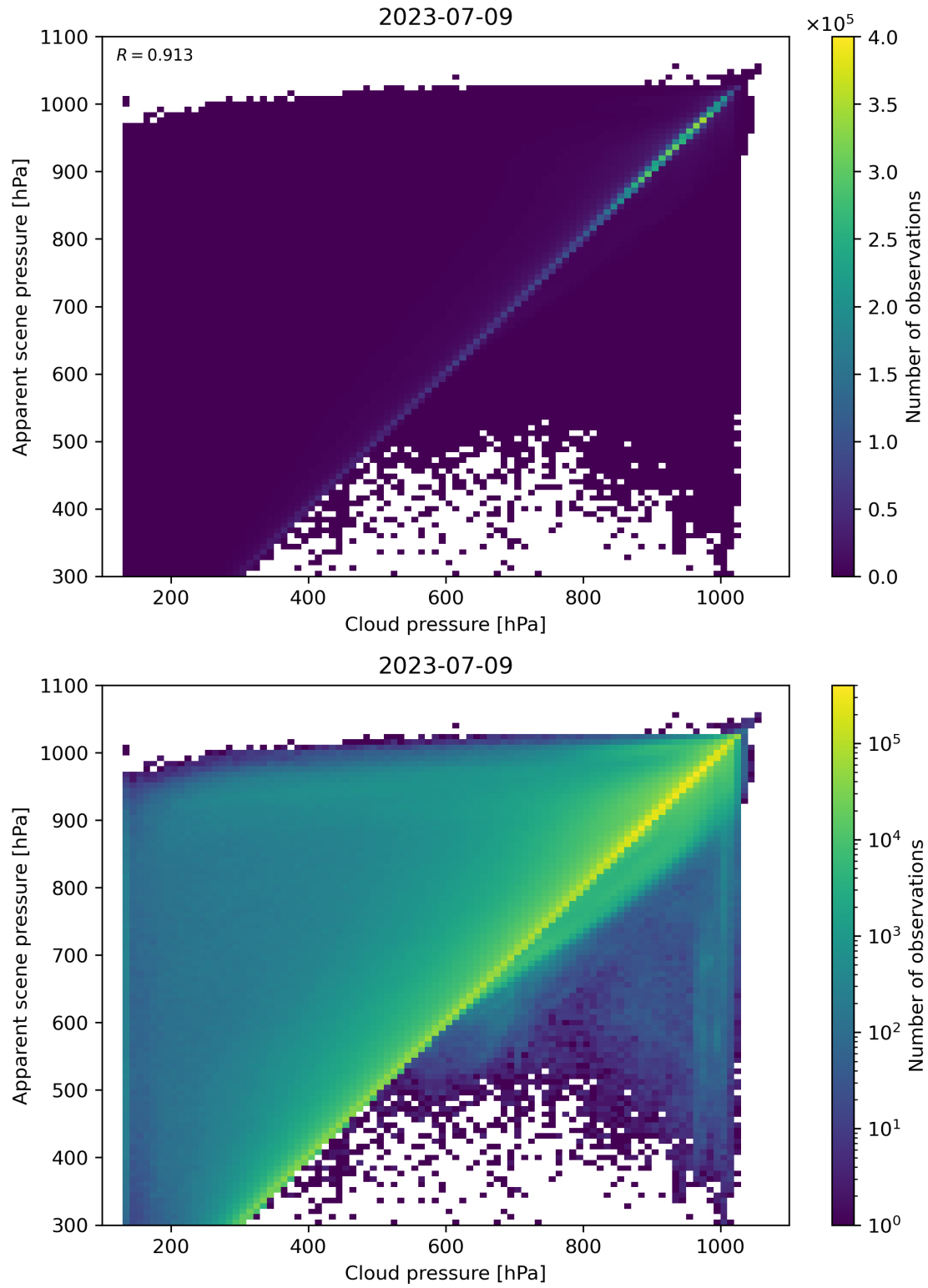
Figure 84: Scatter density plot of “Cloud pressure” against “Apparent scene pressure” for 2023-07-08 to 2023-07-10.
