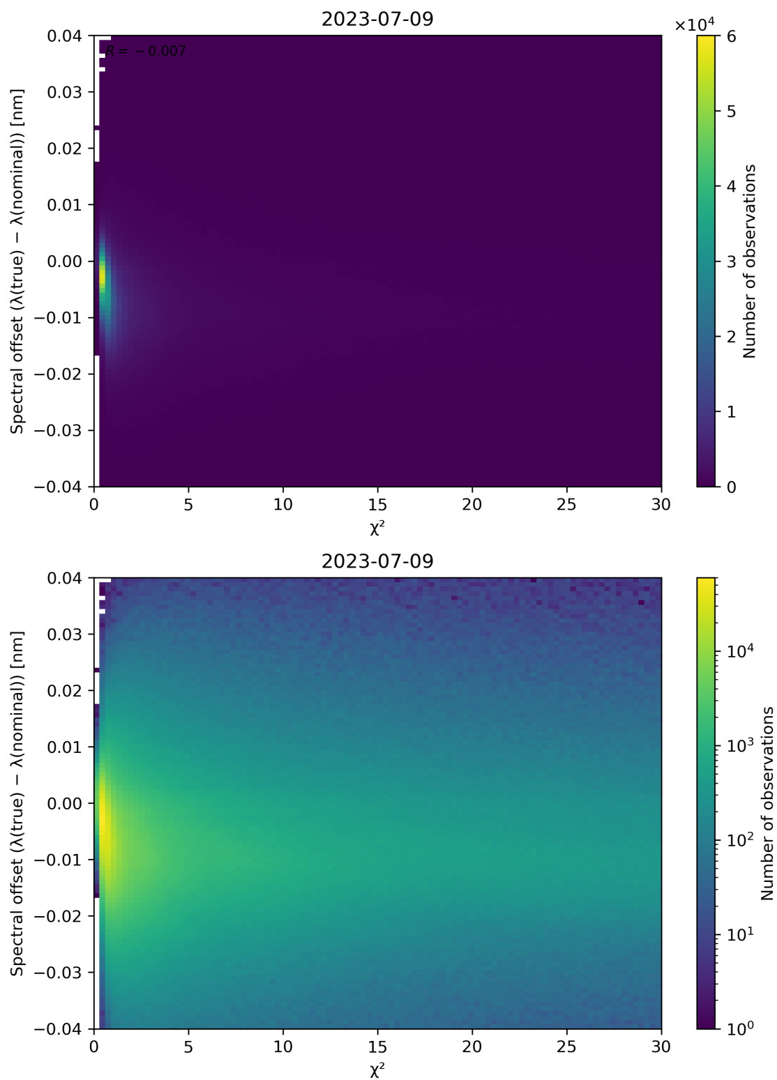
Figure 75: Scatter density plot of “ \chi^2 ” against “Spectral offset ( \lambda(\text{true}) - \lambda(\text{nominal}) )” for 2023-07-08 to 2023-07-10.
