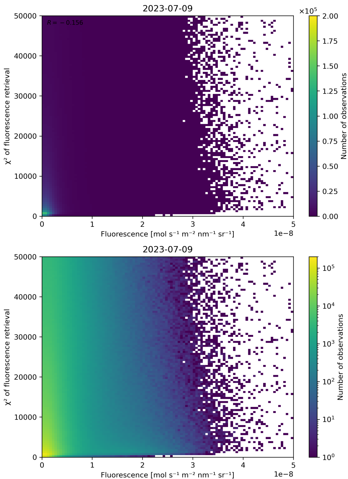
Figure 93: Scatter density plot of “Fluorescence” against “ \chi^2 of fluorescence retrieval” for 2023-07-08 to 2023-07-10.
