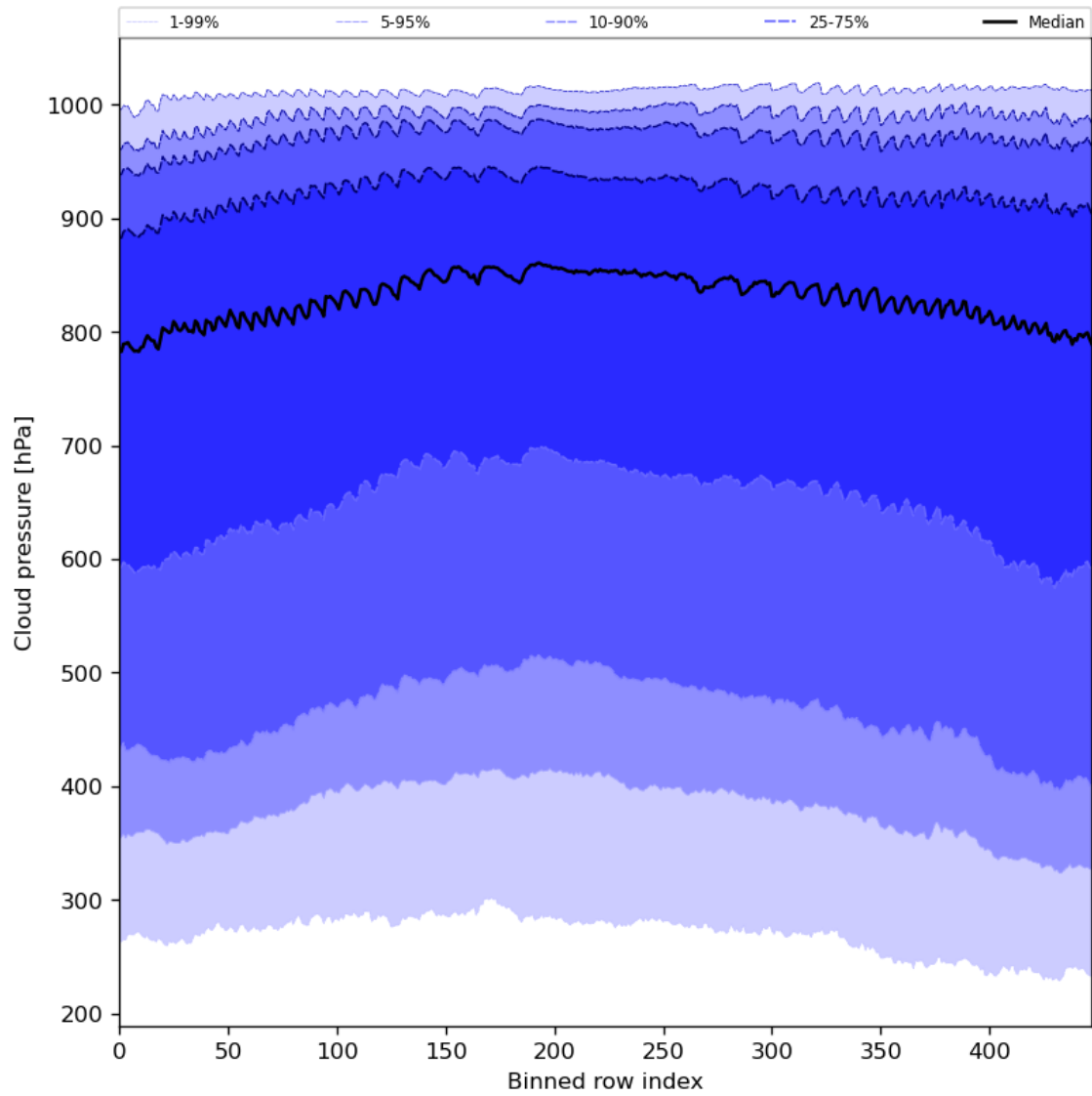
Figure 47: Along track statistics of “Cloud pressure” for 2023-07-08 to 2023-07-10
