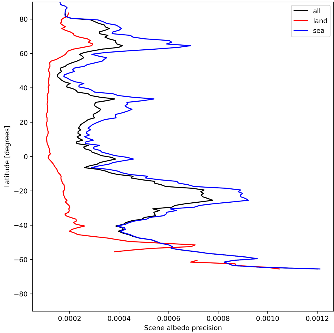
Figure 18: Zonal average of “Scene albedo precision” for 2023-07-08 to 2023-07-10.
