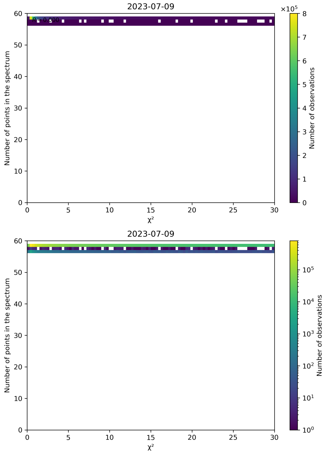
Figure 74: Scatter density plot of “ \chi^2 ” against “Number of points in the spectrum” for 2023-07-08 to 2023-07-10.
