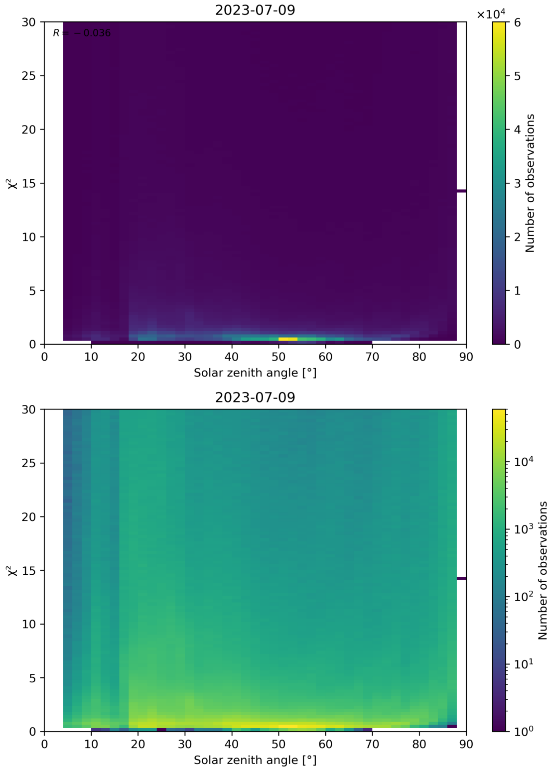
Figure 119: Scatter density plot of “Solar zenith angle” against “ \chi^2 ” for 2023-07-08 to 2023-07-10.
