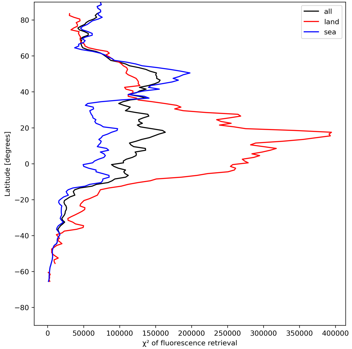
Figure 25: Zonal average of “ \chi^2 of fluorescence retrieval” for 2023-07-08 to 2023-07-10.
