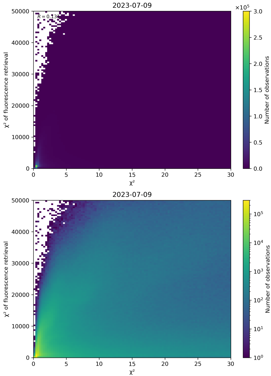
Figure 69: Scatter density plot of “ \chi^2 ” against “ \chi^2 of fluorescence retrieval” for 2023-07-08 to 2023-07-10.
