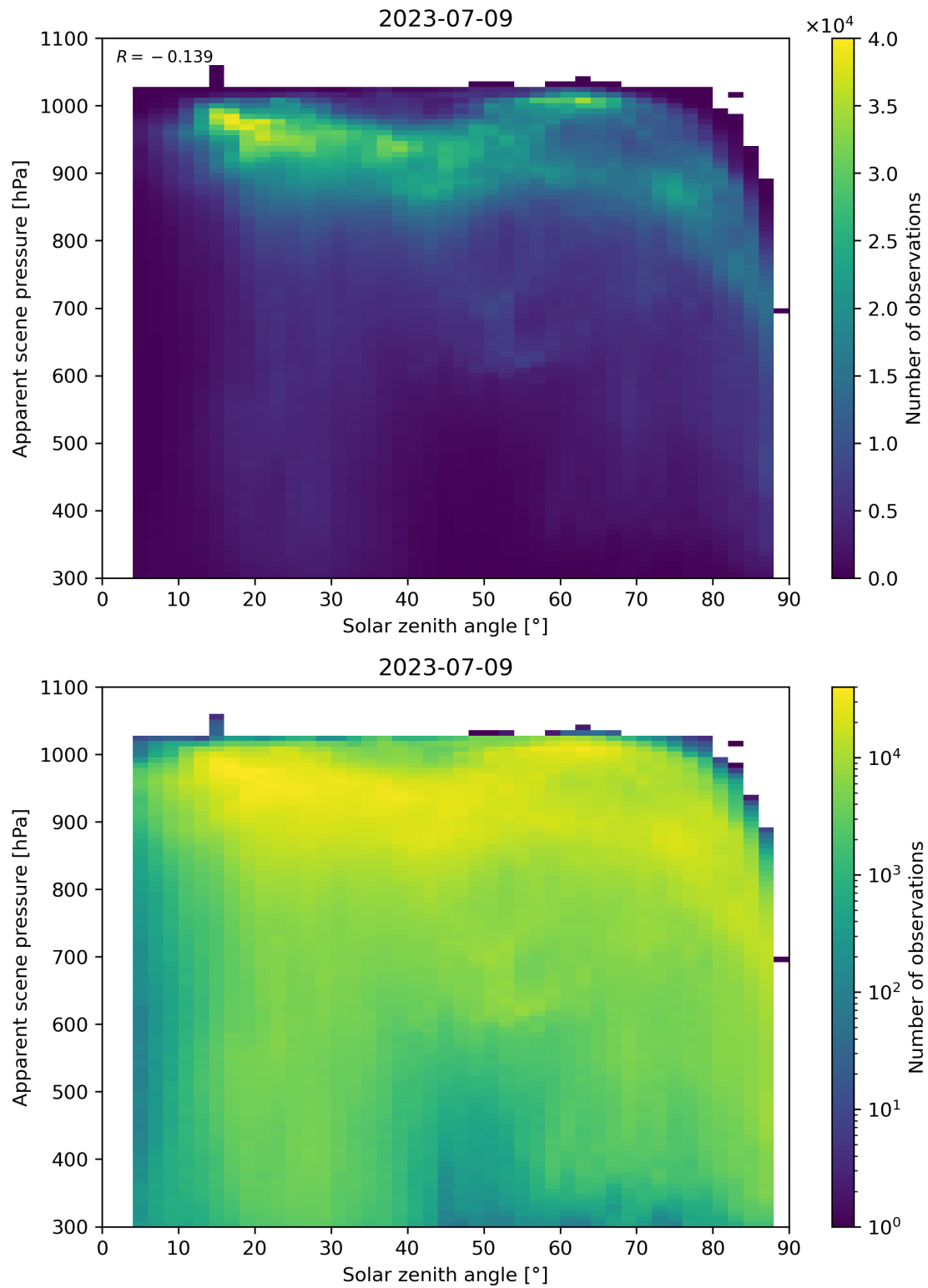
Figure 118: Scatter density plot of “Solar zenith angle” against “Apparent scene pressure” for 2023-07-08 to 2023-07-10.
