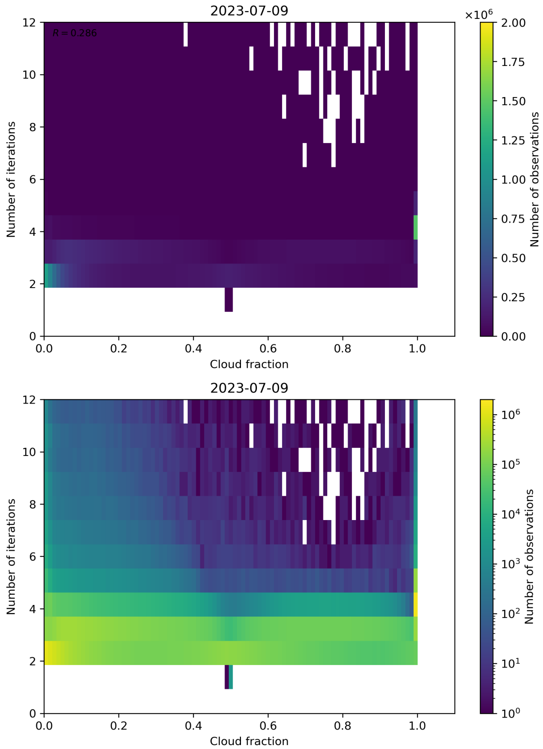
Figure 80: Scatter density plot of “Cloud fraction” against “Number of iterations” for 2023-07-08 to 2023-07-10.
