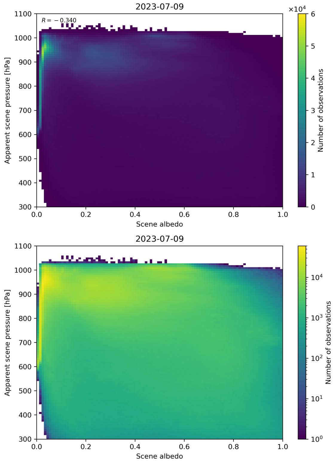
Figure 111: Scatter density plot of “Scene albedo” against “Apparent scene pressure” for 2023-07-08 to 2023-07-10.
