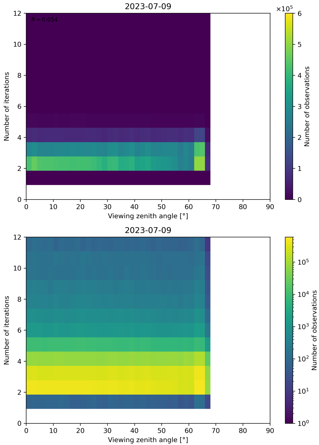
Figure 136: Scatter density plot of “Viewing zenith angle” against “Number of iterations” for 2023-07-08 to 2023-07-10.
