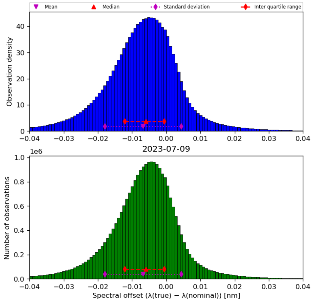
Figure 45: Histogram of “Spectral offset ( \lambda(\text{true}) - \lambda(\text{nominal}) )” for 2023-07-08 to 2023-07-10
