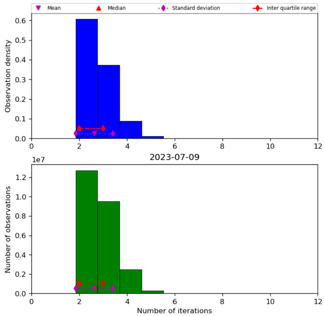
Figure 39: Histogram of “Number of iterations” for 2023-07-08 to 2023-07-10
