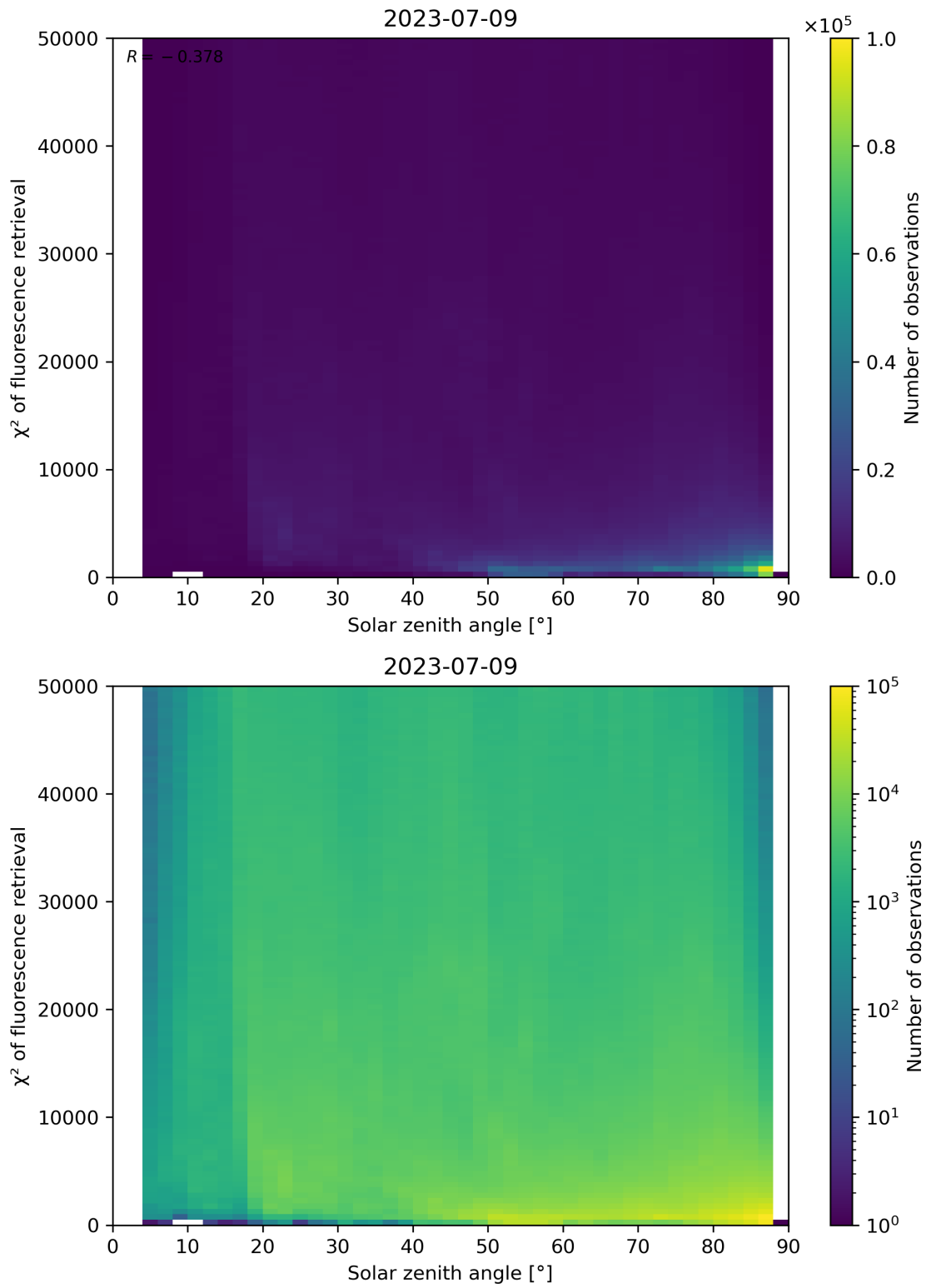
Figure 120: Scatter density plot of “Solar zenith angle” against “ \chi^2 of fluorescence retrieval” for 2023-07-08 to 2023-07-10.
