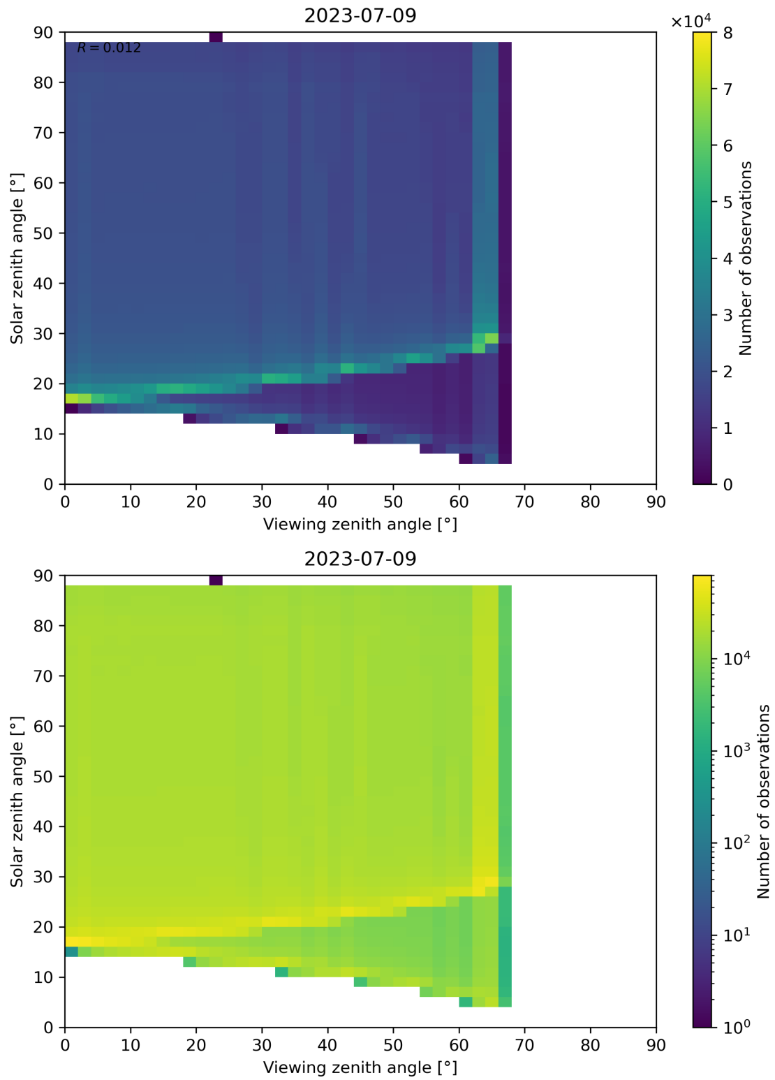
Figure 139: Scatter density plot of “Viewing zenith angle” against “Solar zenith angle” for 2023-07-08 to 2023-07-10.
