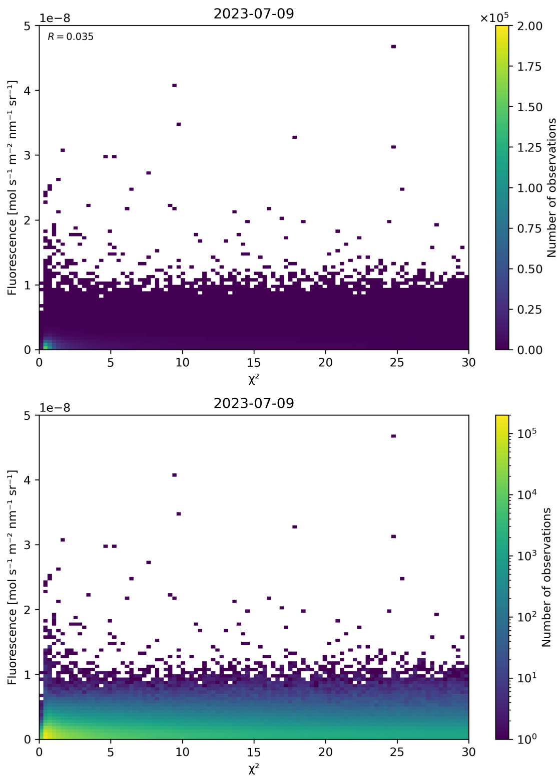
Figure 70: Scatter density plot of “ \chi^2 ” against “Fluorescence” for 2023-07-08 to 2023-07-10.
