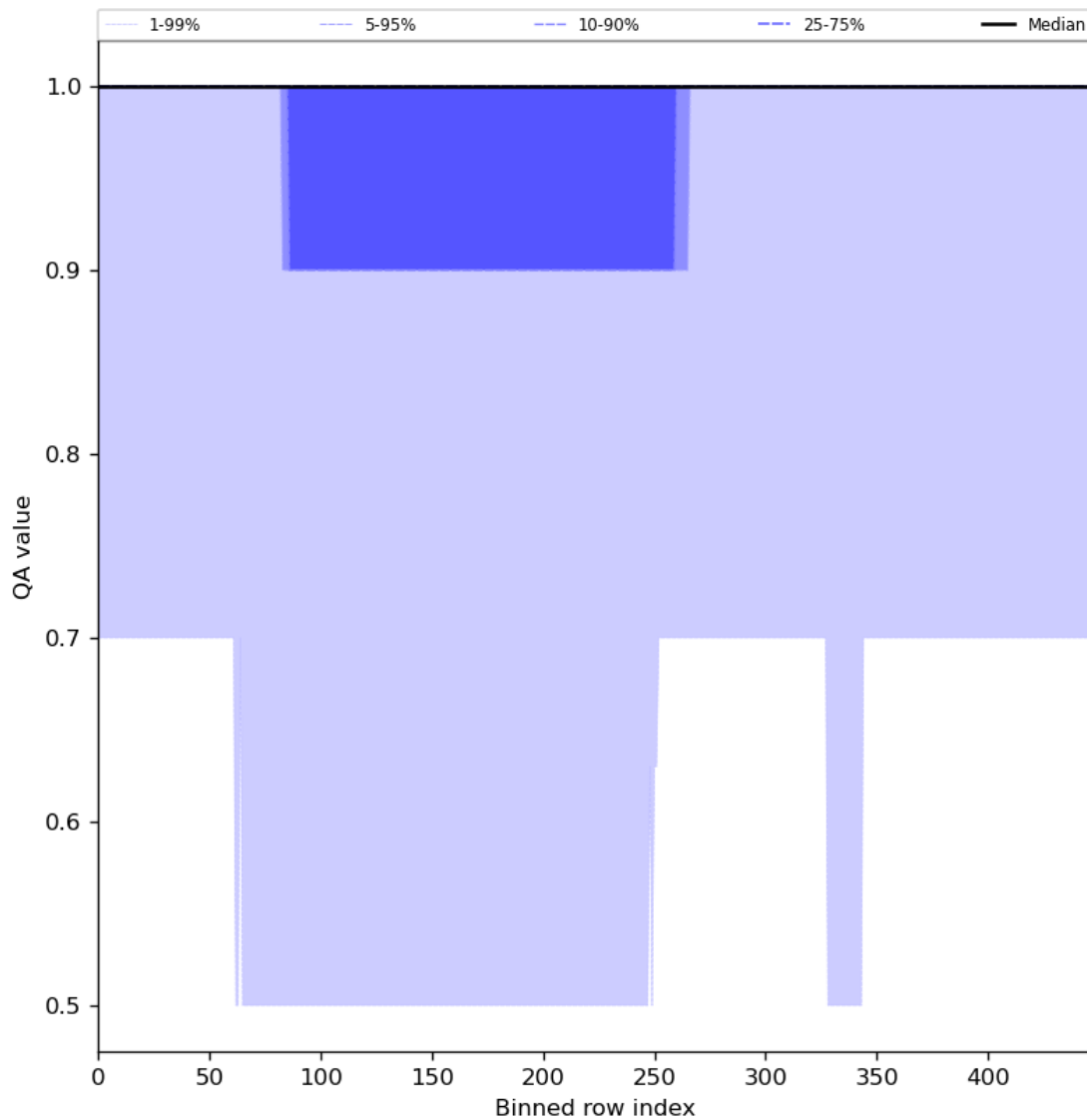
Figure 46: Along track statistics of “QA value” for 2023-07-08 to 2023-07-10
