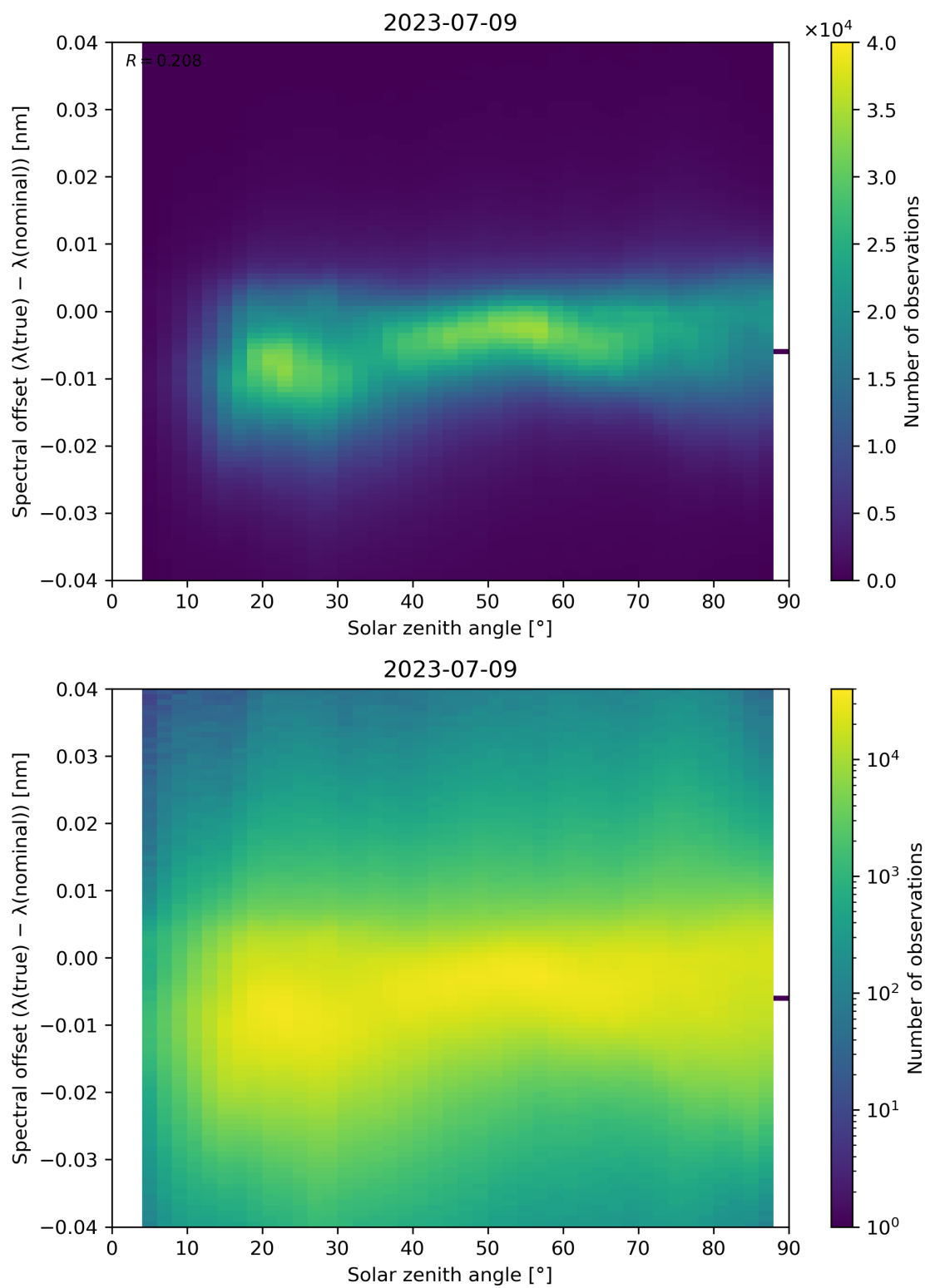
Figure 128: Scatter density plot of “Solar zenith angle” against “Spectral offset ( \lambda(\text{true}) - \lambda(\text{nominal}) )” for 2023-07-08 to 2023-07-10.
