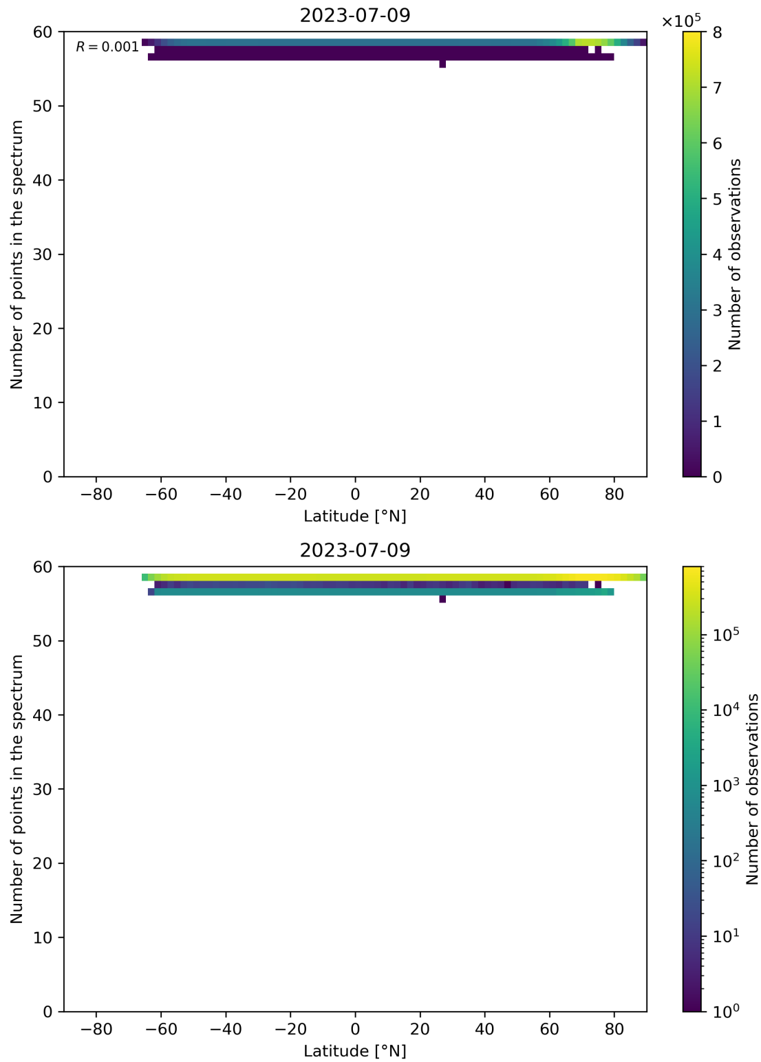
Figure 103: Scatter density plot of “Latitude” against “Number of points in the spectrum” for 2023-07-08 to 2023-07-10.
