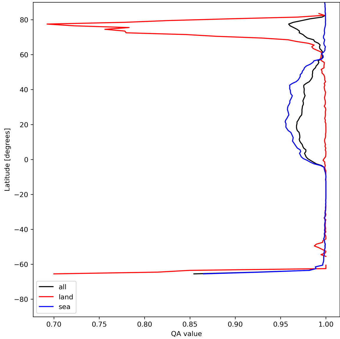
Figure 12: Zonal average of “QA value” for 2023-07-08 to 2023-07-10.
