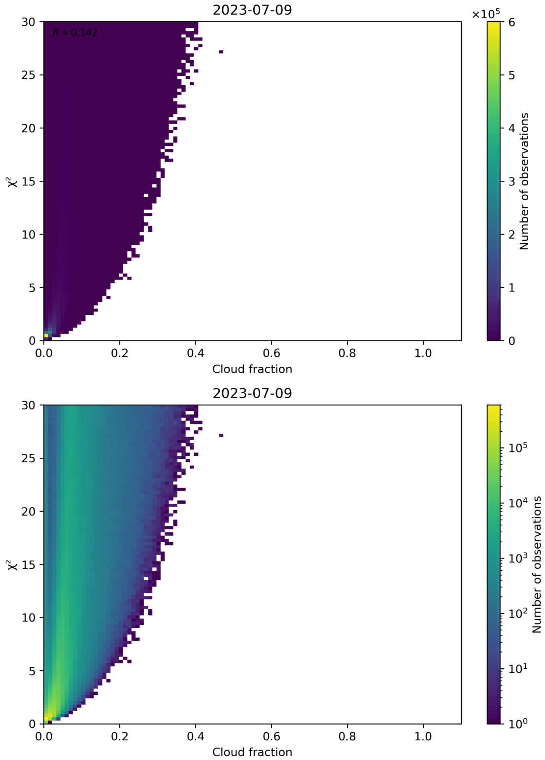
Figure 77: Scatter density plot of “Cloud fraction” against “ \chi^2 ” for 2023-07-08 to 2023-07-10.
