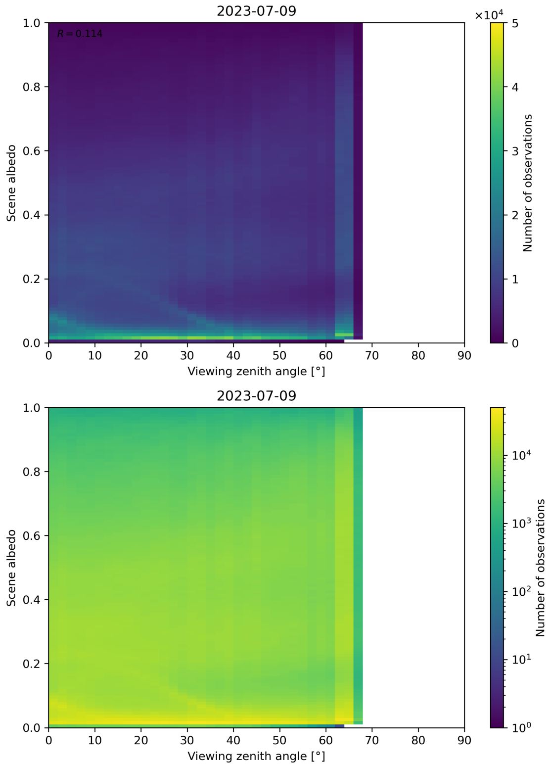
Figure 138: Scatter density plot of “Viewing zenith angle” against “Scene albedo” for 2023-07-08 to 2023-07-10.
