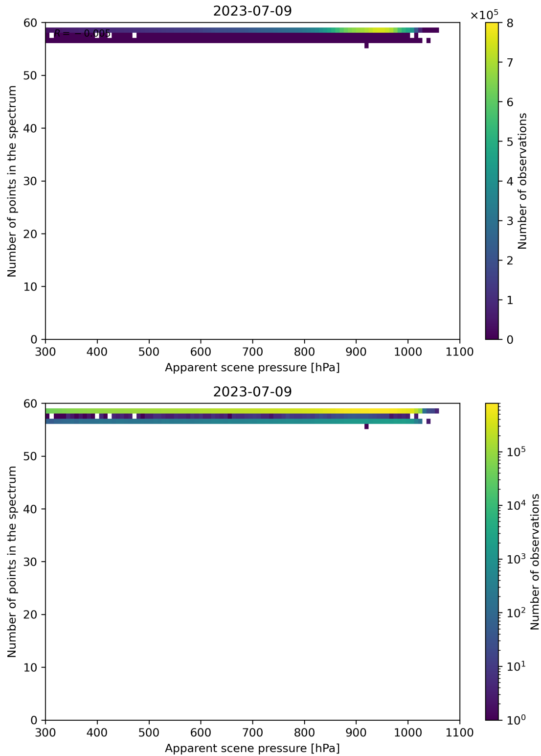
Figure 67: Scatter density plot of “Apparent scene pressure” against “Number of points in the spectrum” for 2023-07-08 to 2023-07-10.
