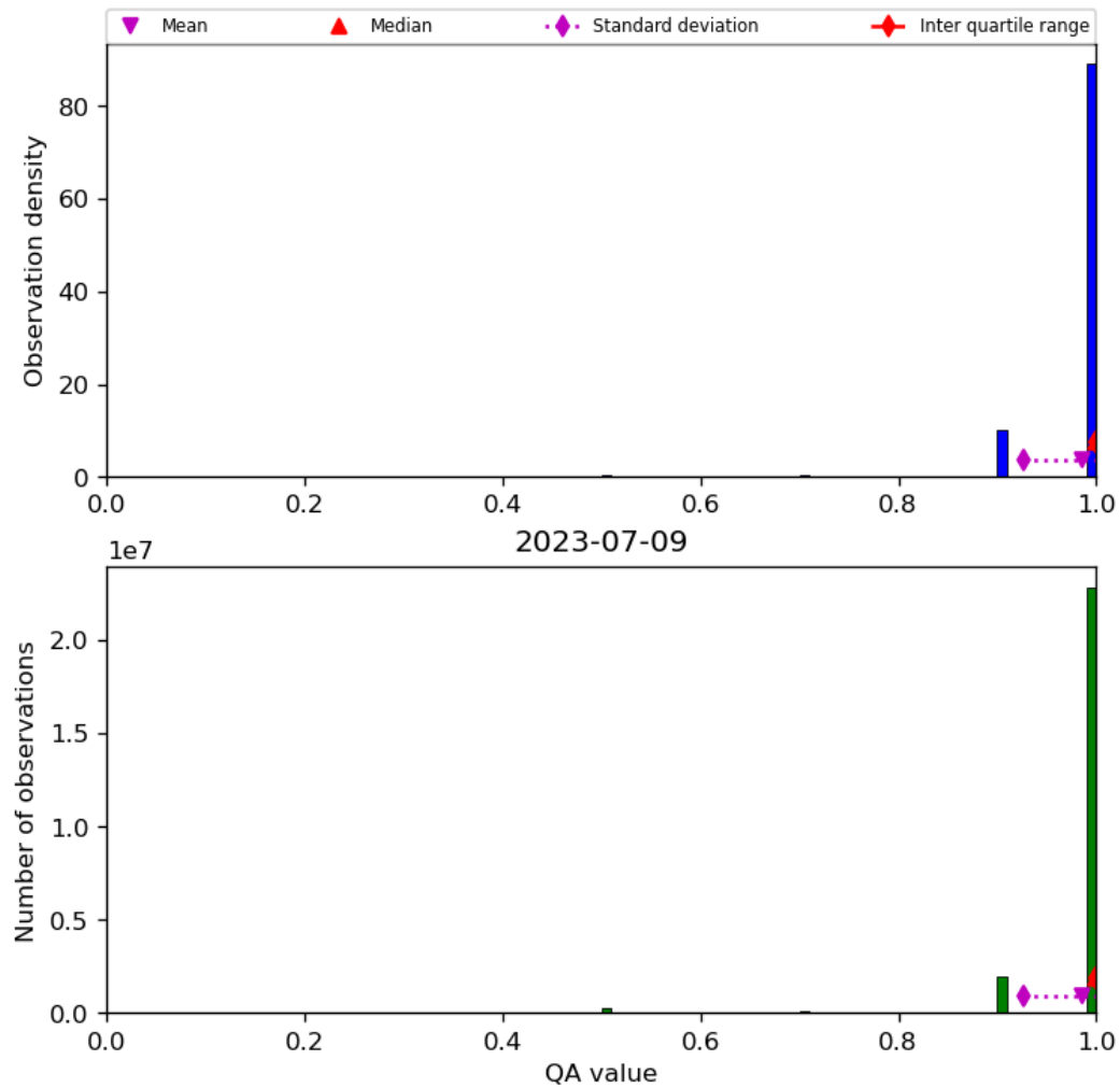
Figure 29: Histogram of “QA value” for 2023-07-08 to 2023-07-10
