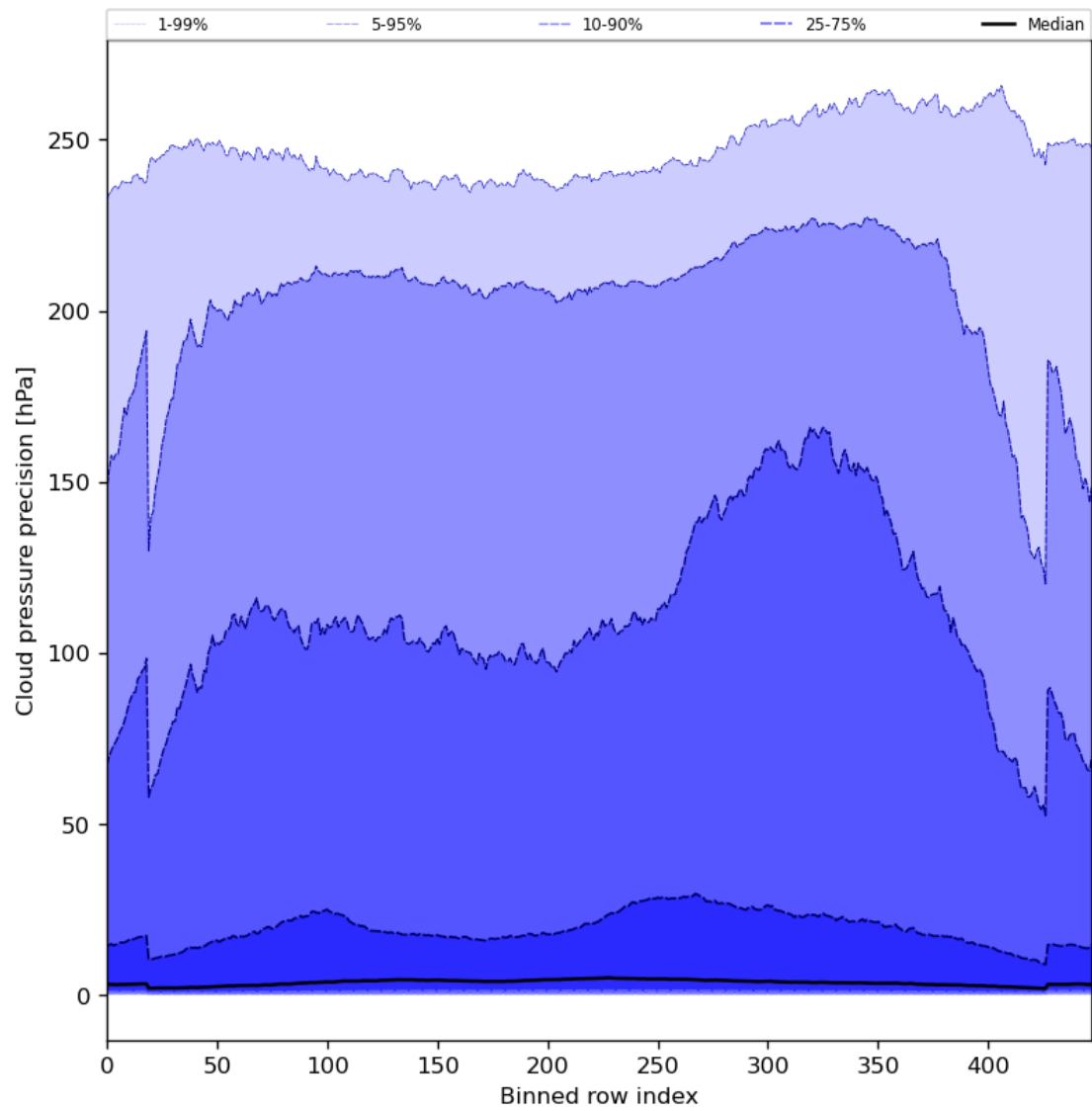
Figure 48: Along track statistics of “Cloud pressure precision” for 2023-07-08 to 2023-07-10
