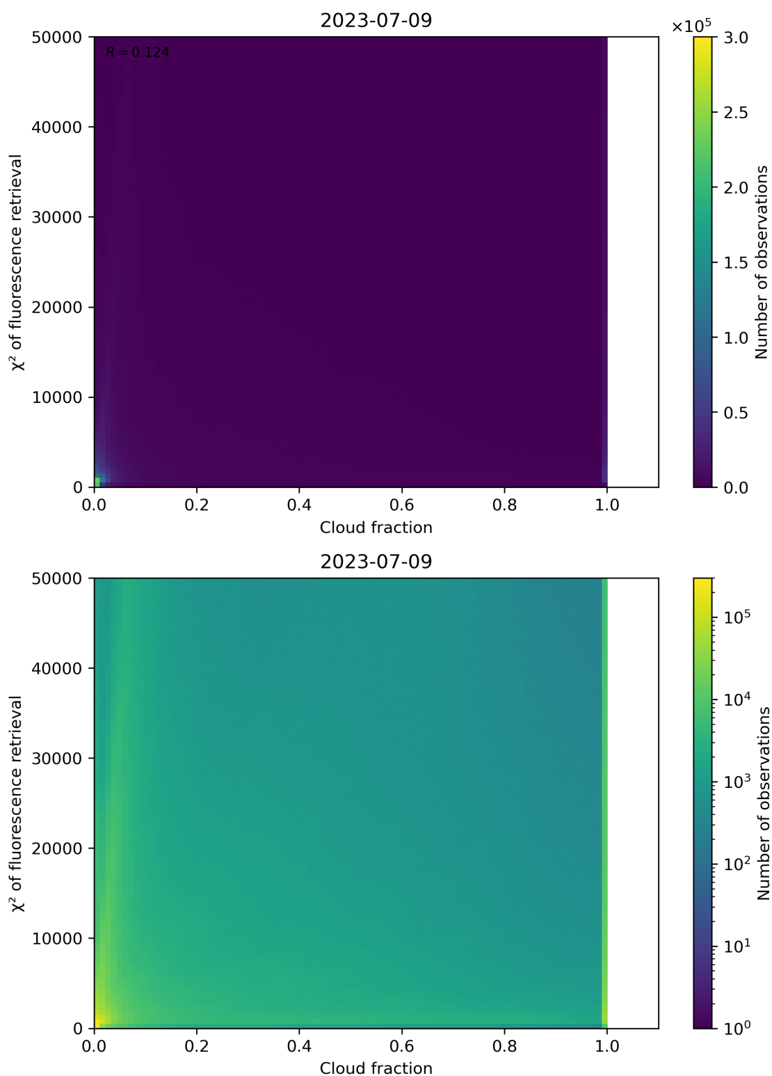
Figure 78: Scatter density plot of “Cloud fraction” against “ \chi^2 of fluorescence retrieval” for 2023-07-08 to 2023-07-10.
