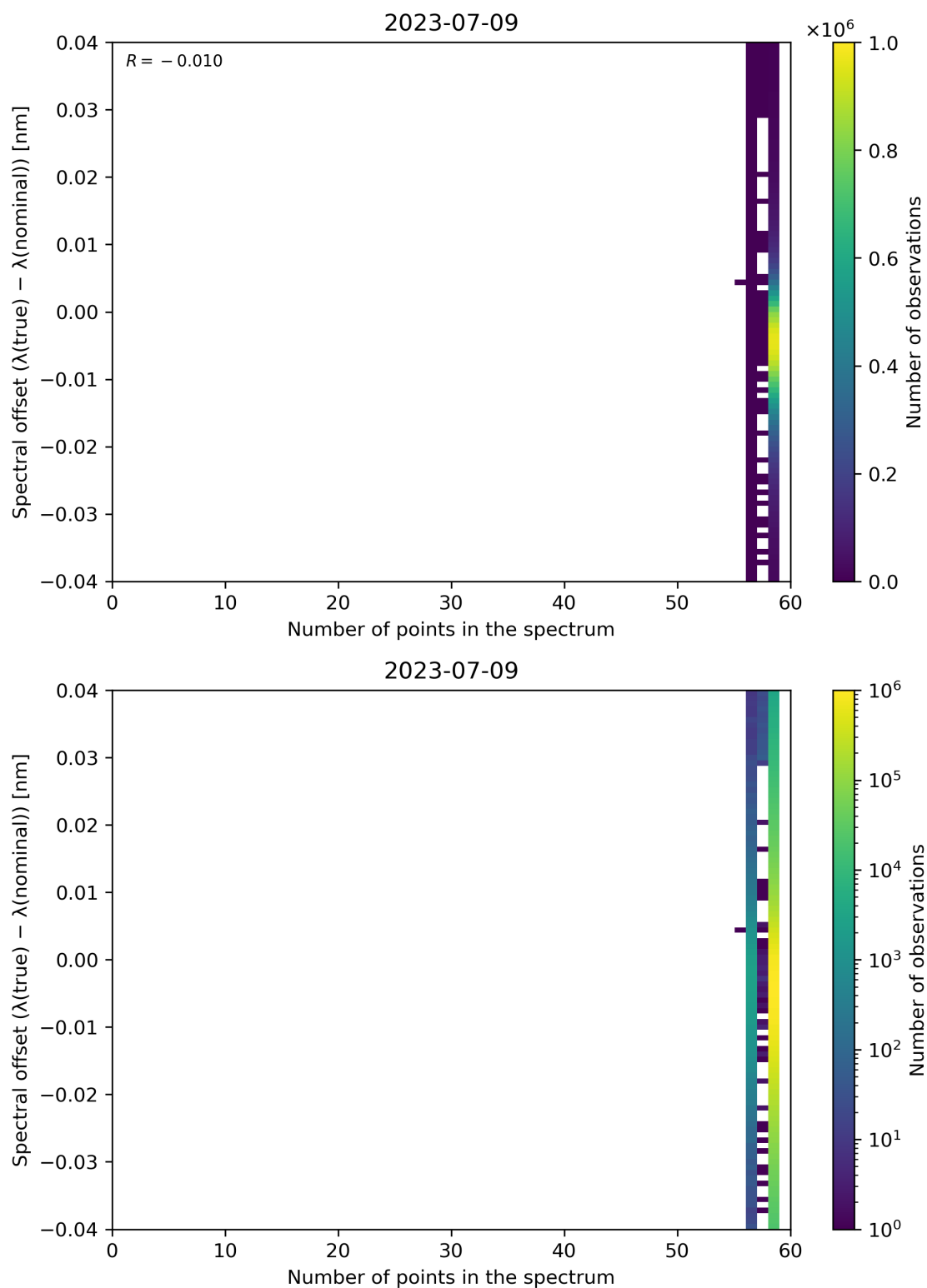
Figure 110: Scatter density plot of “Number of points in the spectrum” against “Spectral offset ( \lambda(\text{true}) - \lambda(\text{nominal}) )” for 2023-07-08 to 2023-07-10.
