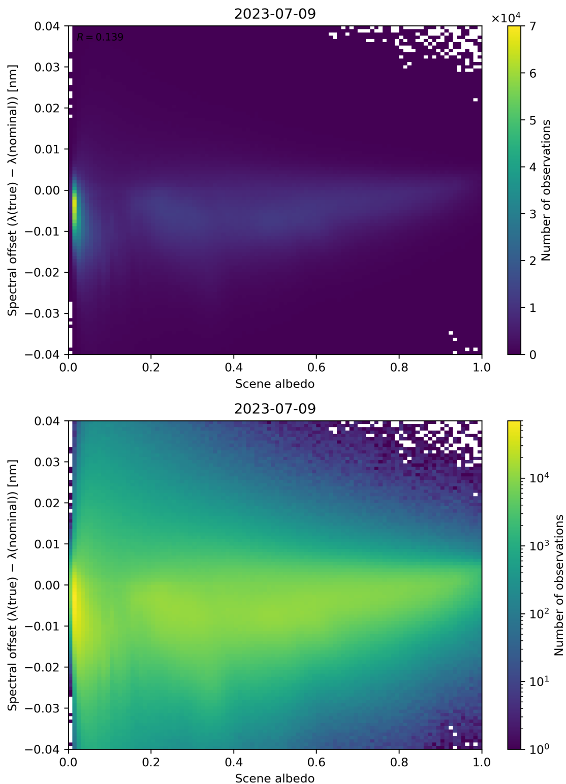
Figure 117: Scatter density plot of “Scene albedo” against “Spectral offset ( \lambda(\text{true}) - \lambda(\text{nominal}) )” for 2023-07-08 to 2023-07-10.
