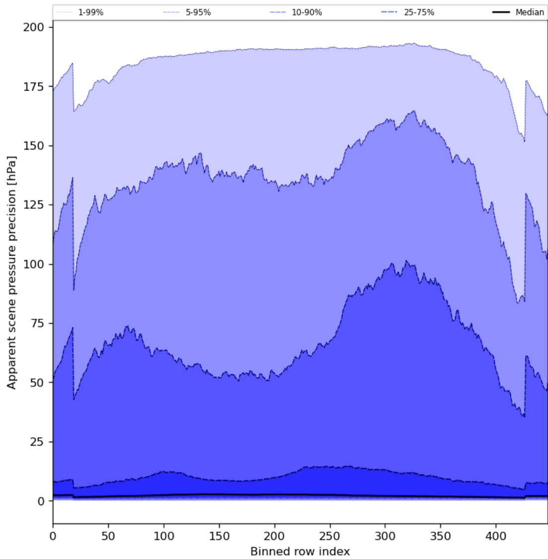
Figure 54: Along track statistics of “Apparent scene pressure precision” for 2023-07-08 to 2023-07-10
