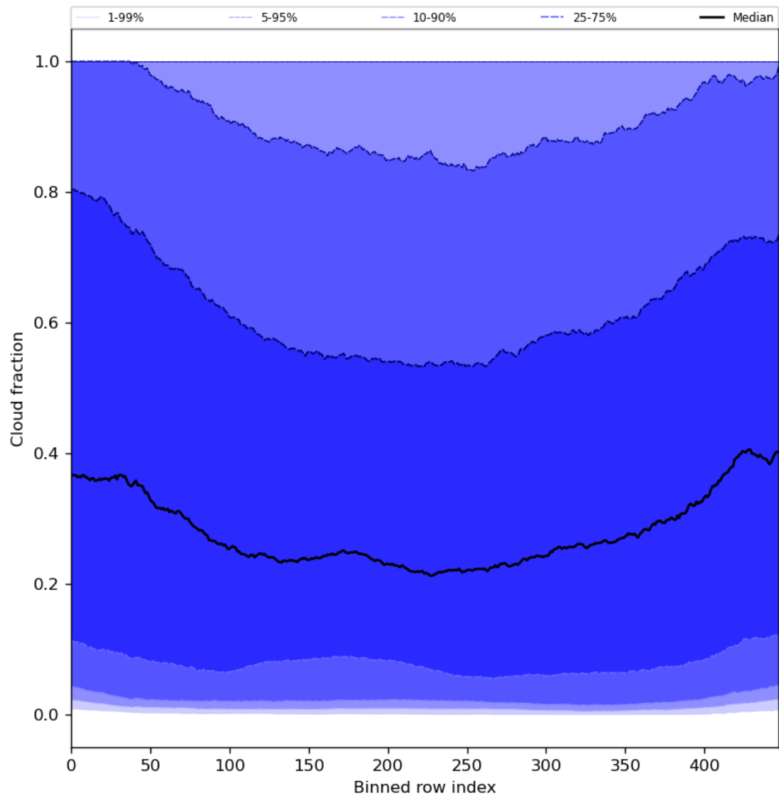
Figure 49: Along track statistics of “Cloud fraction” for 2023-07-08 to 2023-07-10
