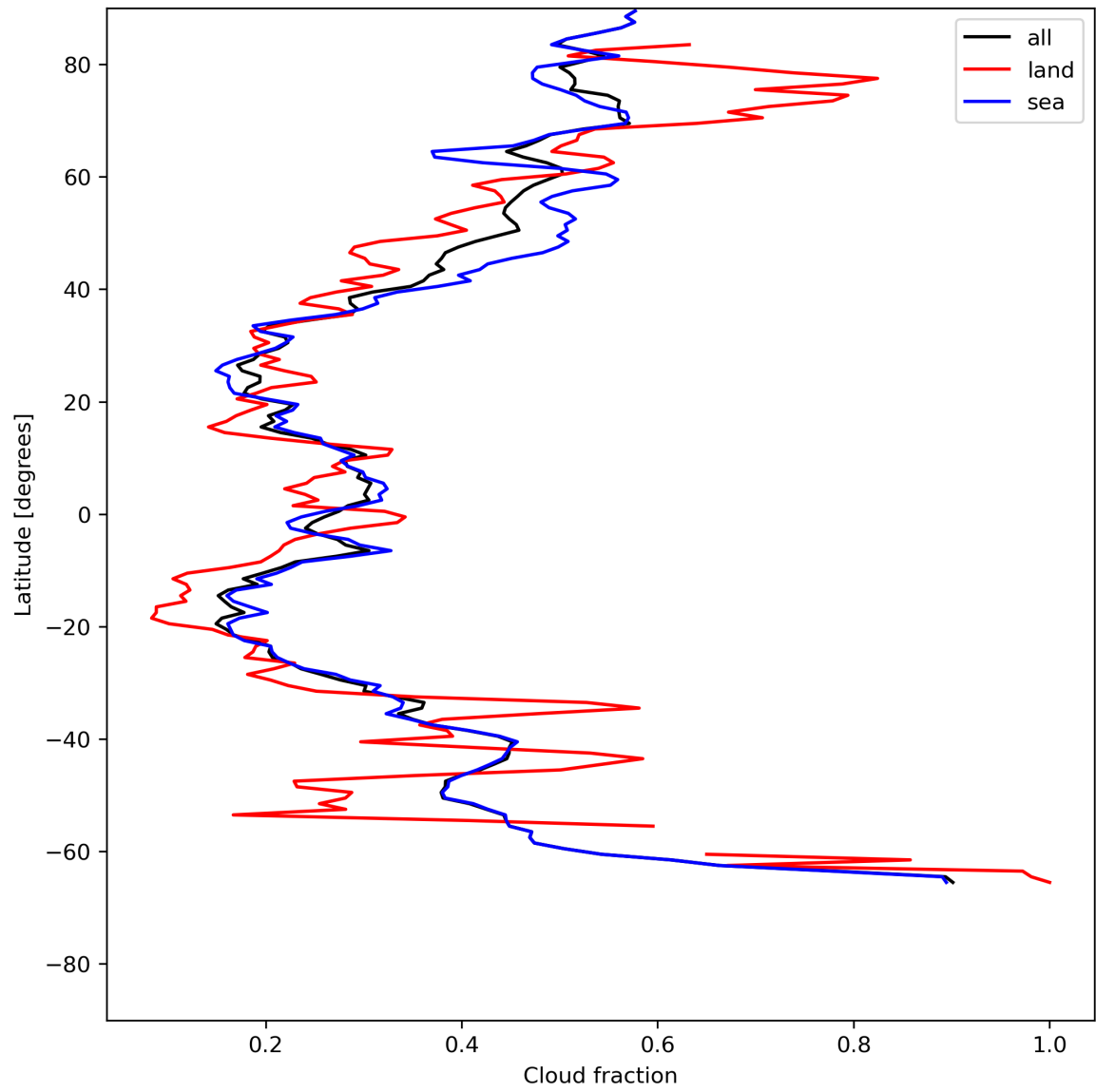
Figure 15: Zonal average of “Cloud fraction” for 2023-07-08 to 2023-07-10.
