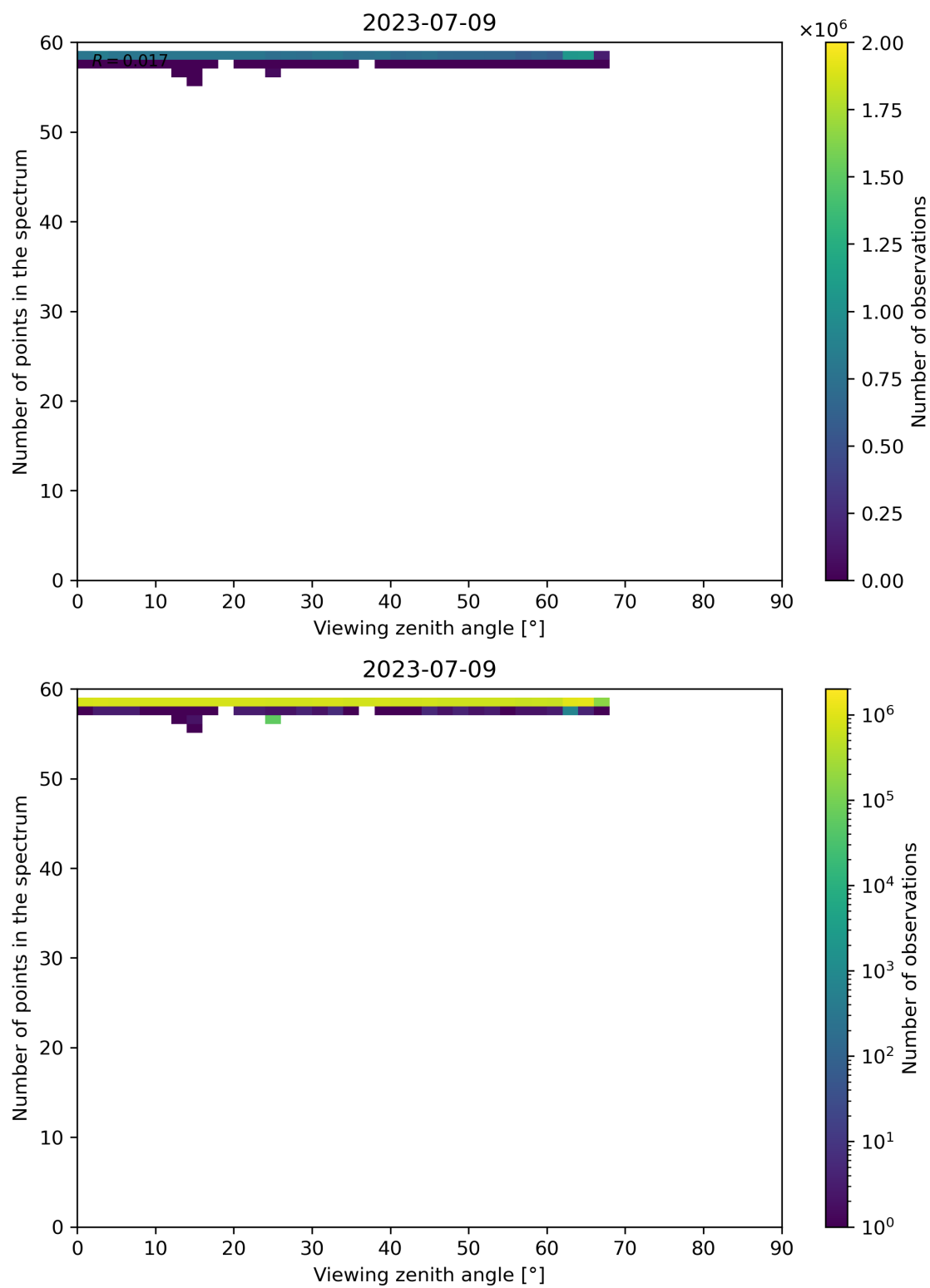
Figure 137: Scatter density plot of “Viewing zenith angle” against “Number of points in the spectrum” for 2023-07-08 to 2023-07-10.
