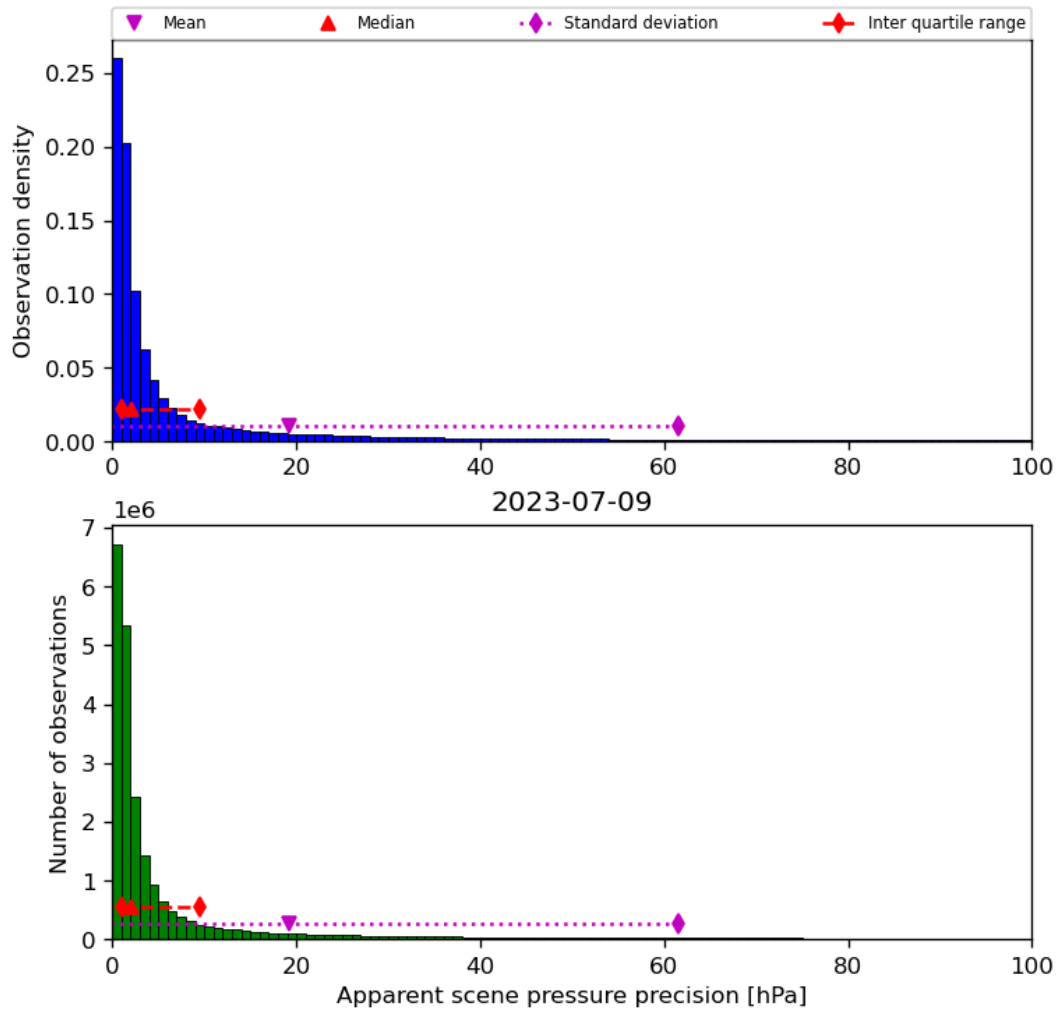
Figure 37: Histogram of “Apparent scene pressure precision” for 2023-07-08 to 2023-07-10
