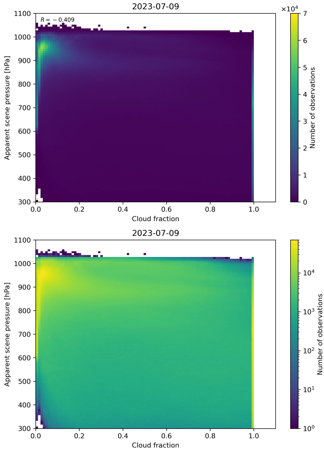
Figure 76: Scatter density plot of “Cloud fraction” against “Apparent scene pressure” for 2023-07-08 to 2023-07-10.
