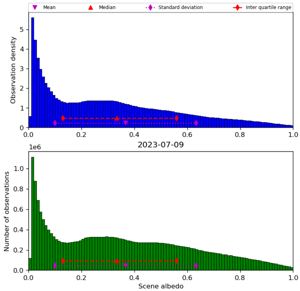
Figure 34: Histogram of “Scene albedo” for 2023-07-08 to 2023-07-10
