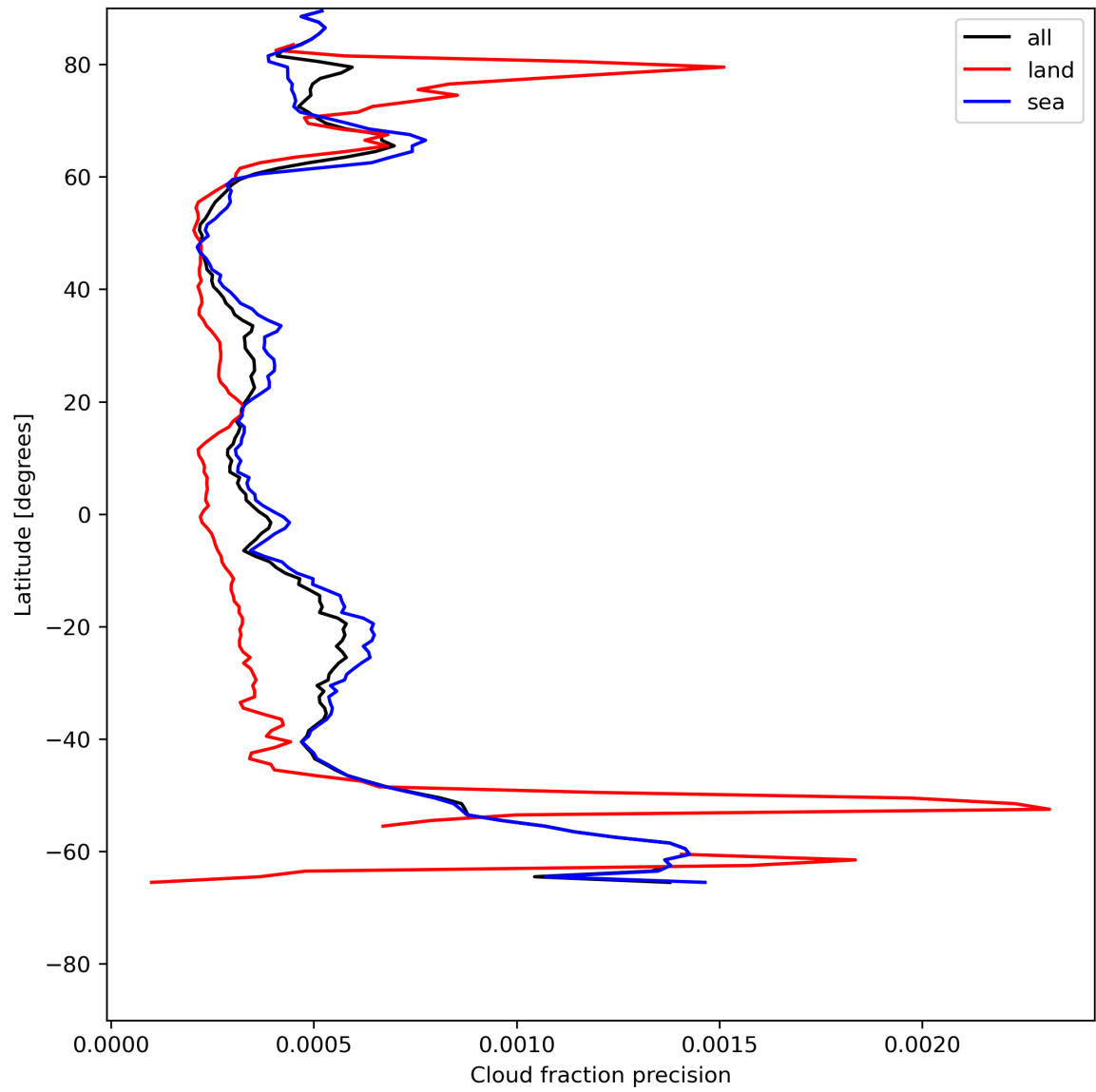
Figure 16: Zonal average of “Cloud fraction precision” for 2023-07-08 to 2023-07-10.
