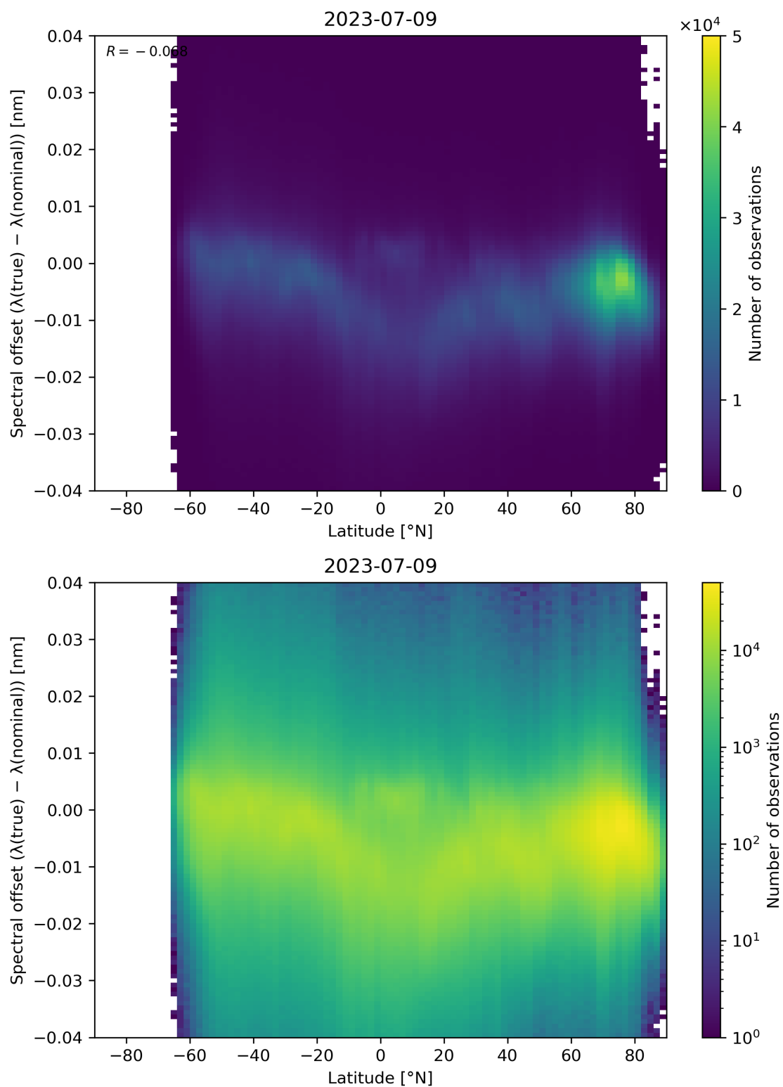
Figure 105: Scatter density plot of “Latitude” against “Spectral offset ( \lambda(\text{true}) - \lambda(\text{nominal}) )” for 2023-07-08 to 2023-07-10.
