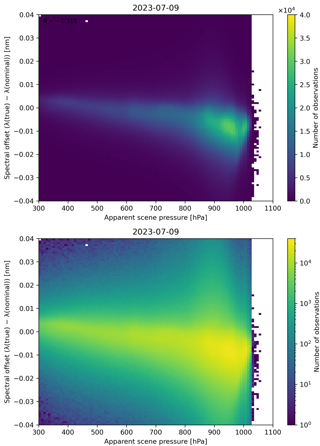
Figure 68: Scatter density plot of “Apparent scene pressure” against “Spectral offset ( \lambda(\text{true}) - \lambda(\text{nominal}) )” for 2023-07-08 to 2023-07-10.
