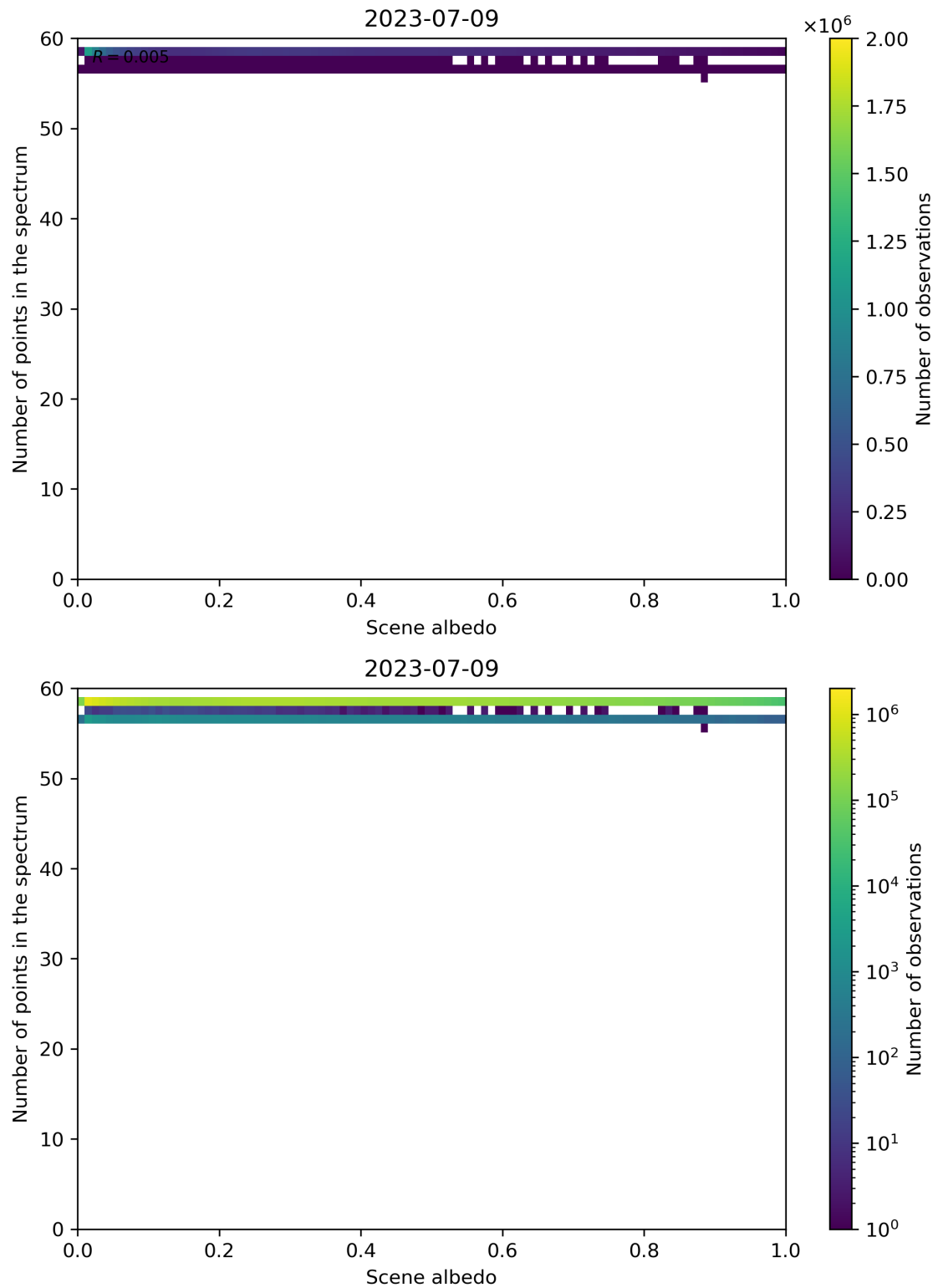
Figure 116: Scatter density plot of “Scene albedo” against “Number of points in the spectrum” for 2023-07-08 to 2023-07-10.
