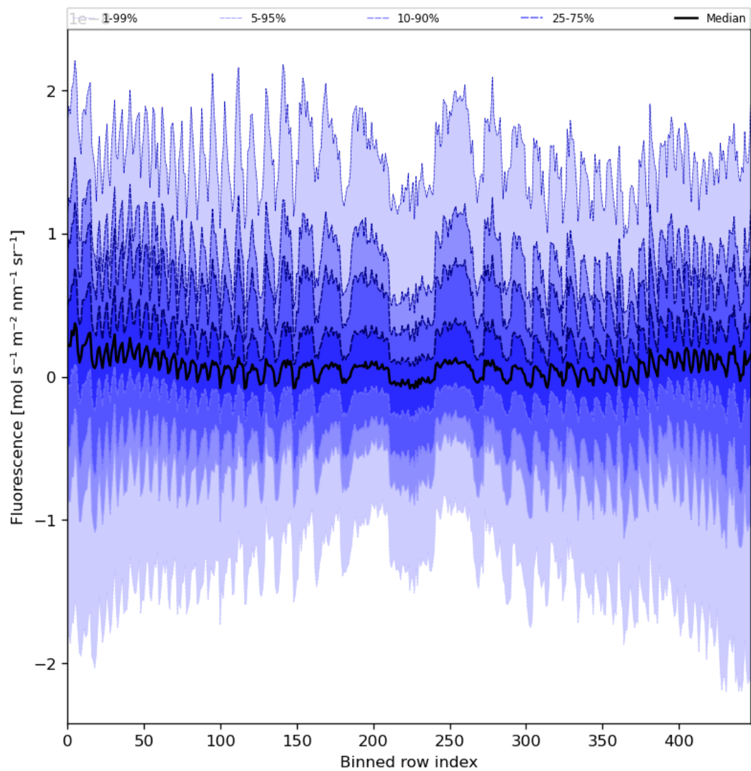
Figure 57: Along track statistics of “Fluorescence” for 2023-07-08 to 2023-07-10
