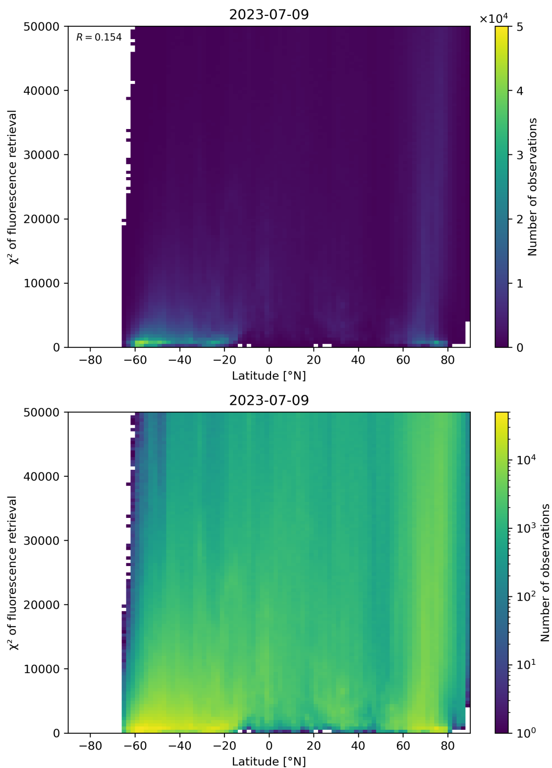
Figure 98: Scatter density plot of “Latitude” against “ \chi^2 of fluorescence retrieval” for 2023-07-08 to 2023-07-10.
