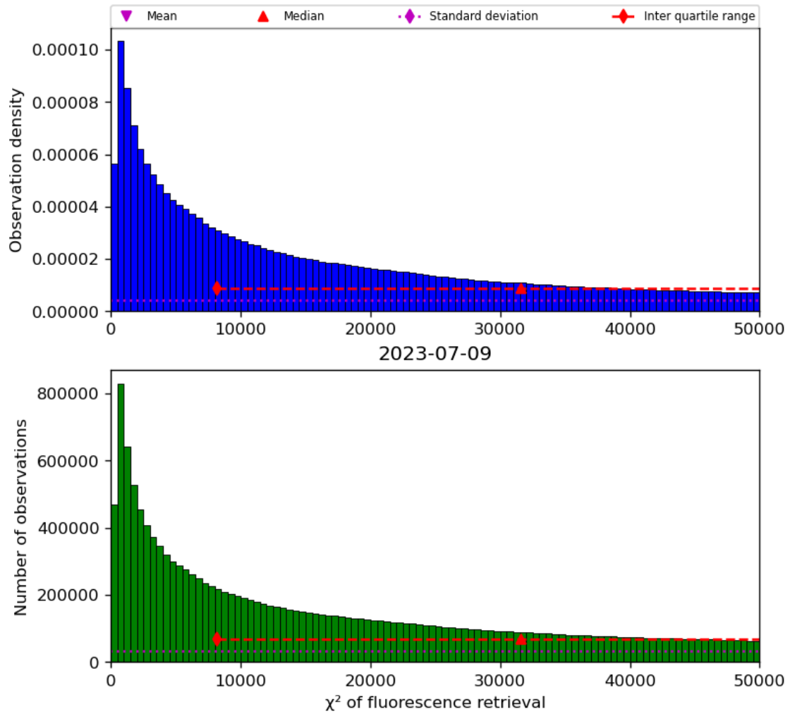
Figure 42: Histogram of “ \chi^2 of fluorescence retrieval” for 2023-07-08 to 2023-07-10
