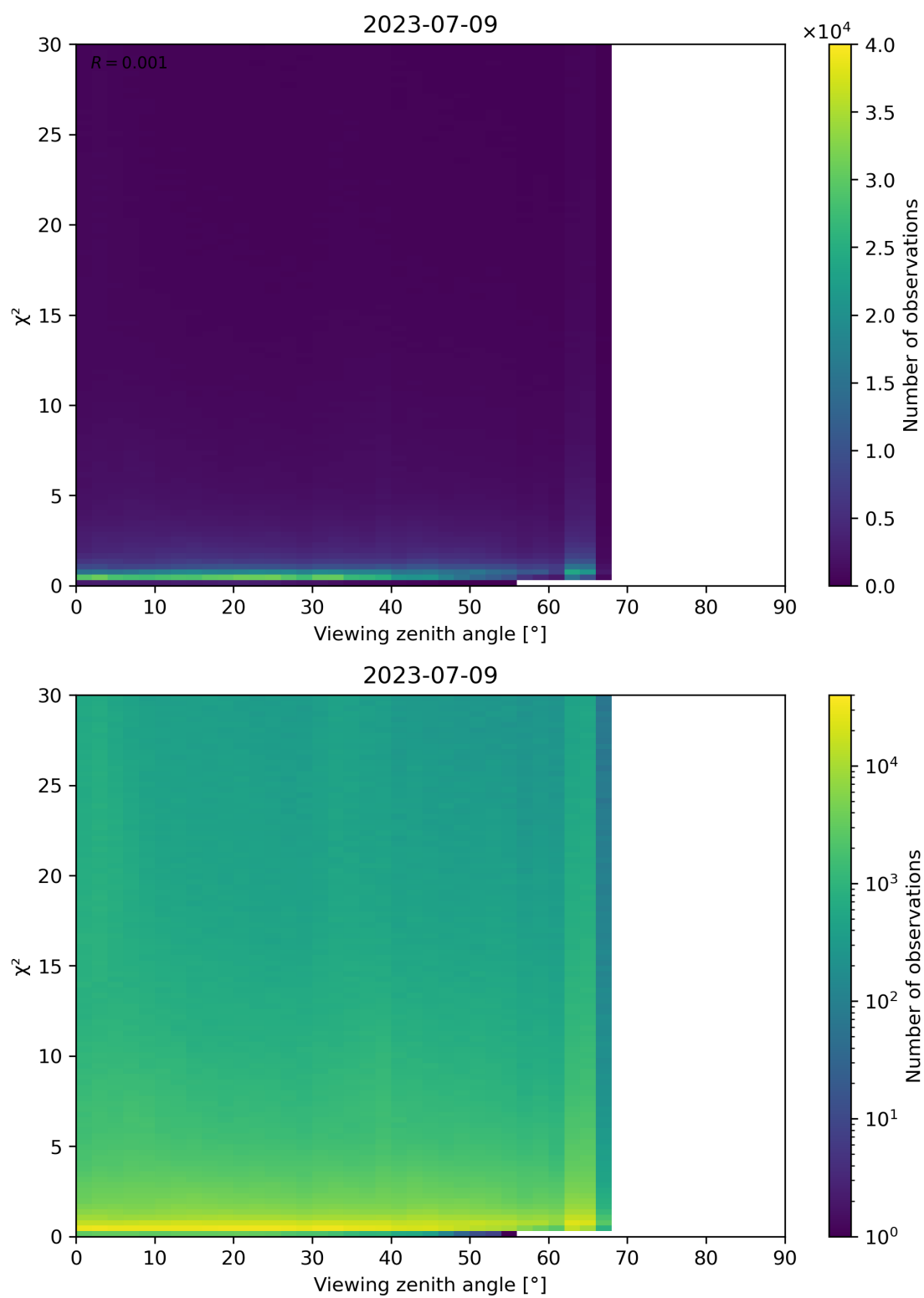
Figure 130: Scatter density plot of “Viewing zenith angle” against “ \chi^2 ” for 2023-07-08 to 2023-07-10.
