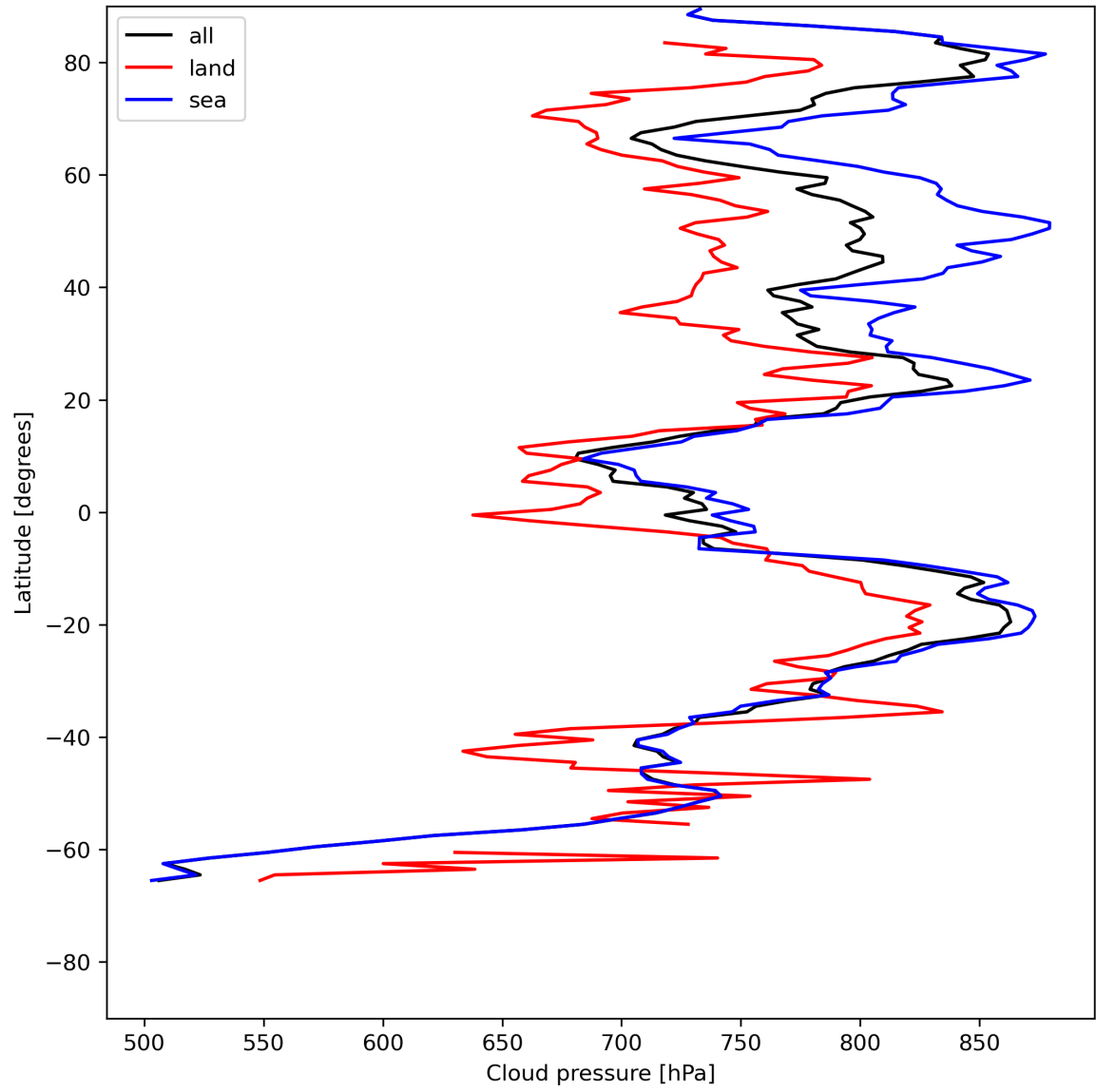
Figure 13: Zonal average of “Cloud pressure” for 2023-07-08 to 2023-07-10.
