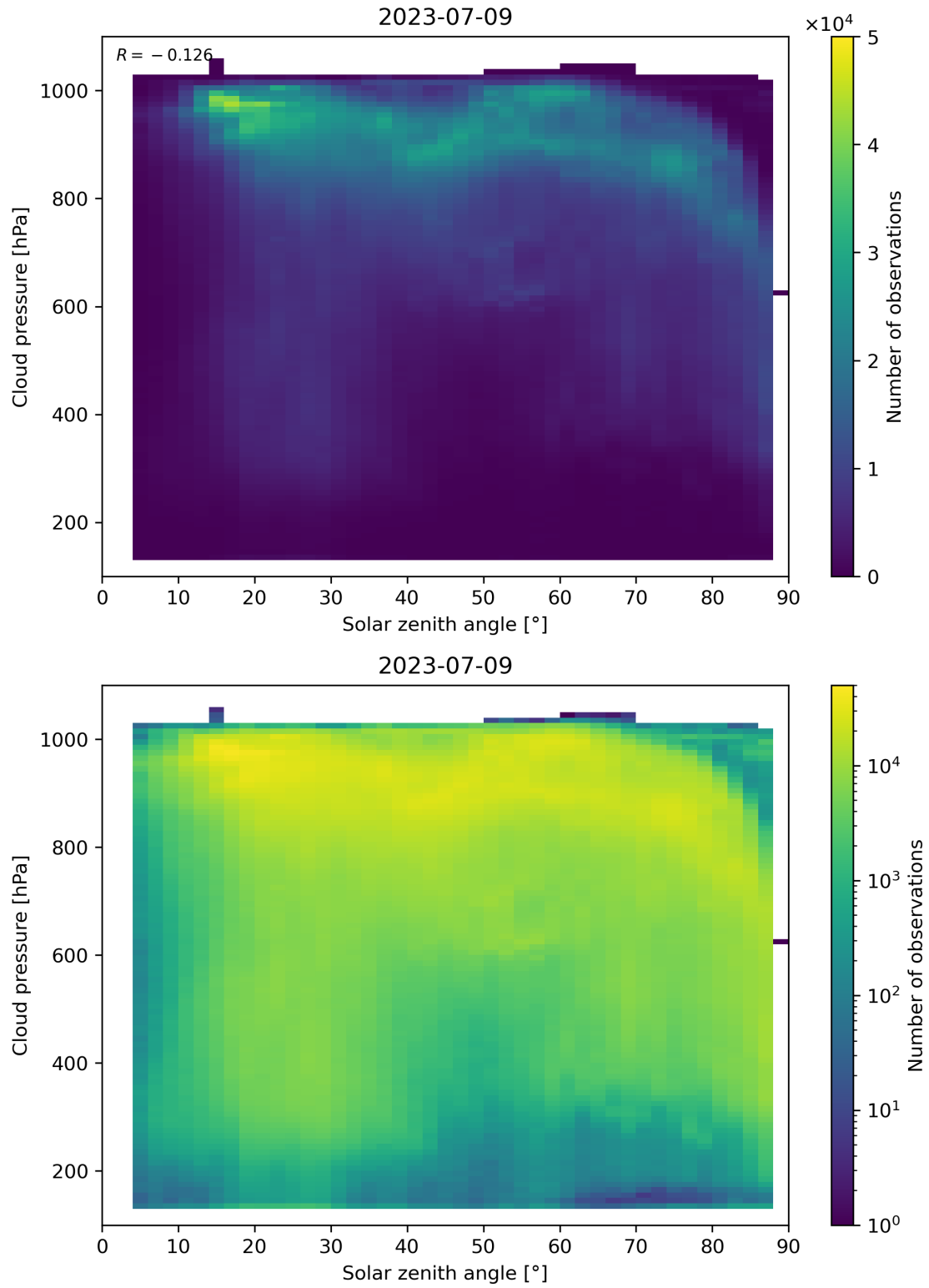
Figure 122: Scatter density plot of “Solar zenith angle” against “Cloud pressure” for 2023-07-08 to 2023-07-10.
