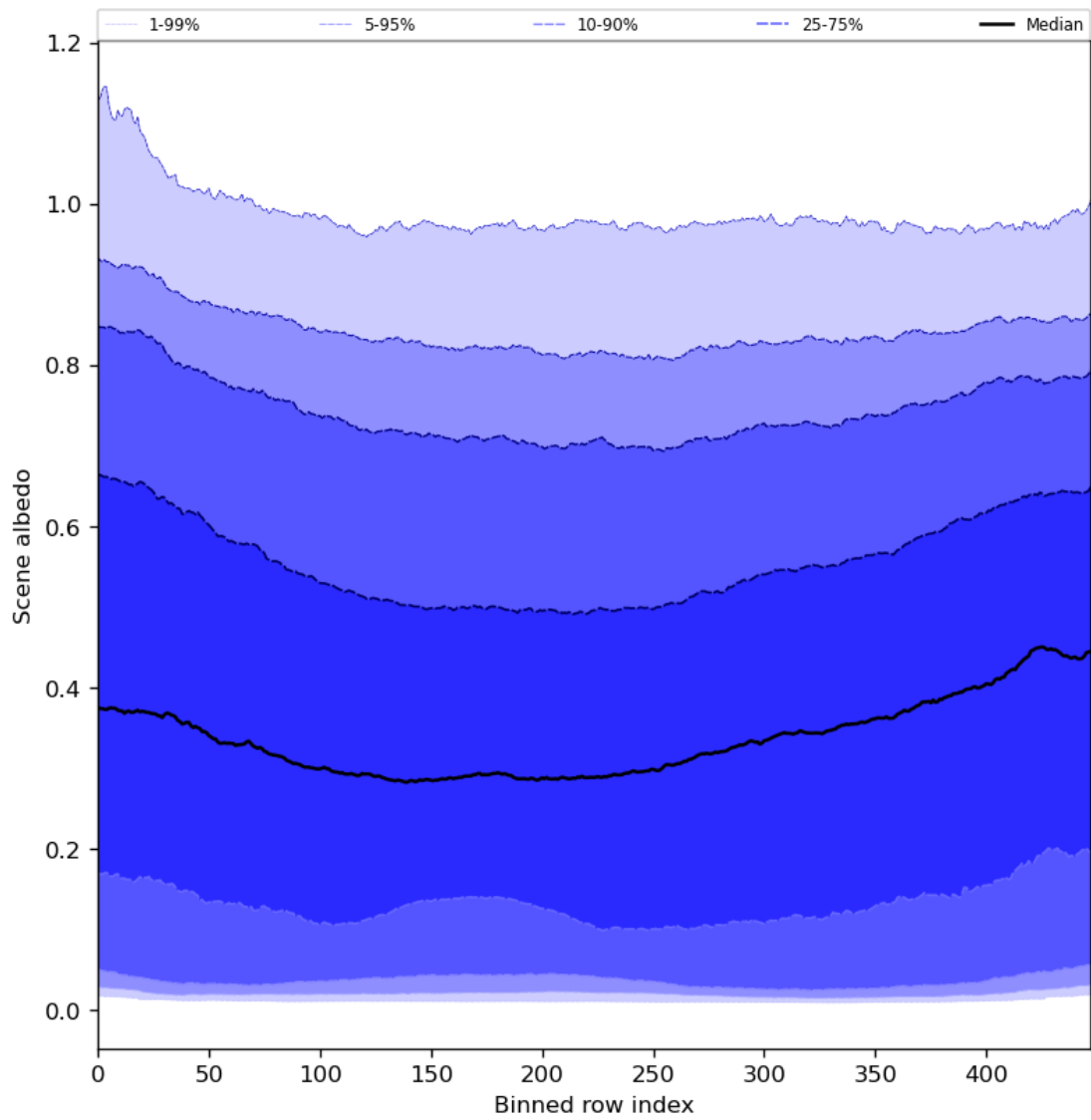
Figure 51: Along track statistics of “Scene albedo” for 2023-07-08 to 2023-07-10
