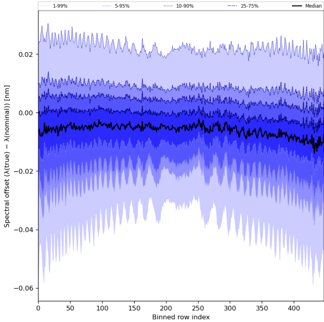
Figure 62: Along track statistics of “Spectral offset ( \lambda(\text{true}) - \lambda(\text{nominal}) )” for 2023-07-08 to 2023-07-10
