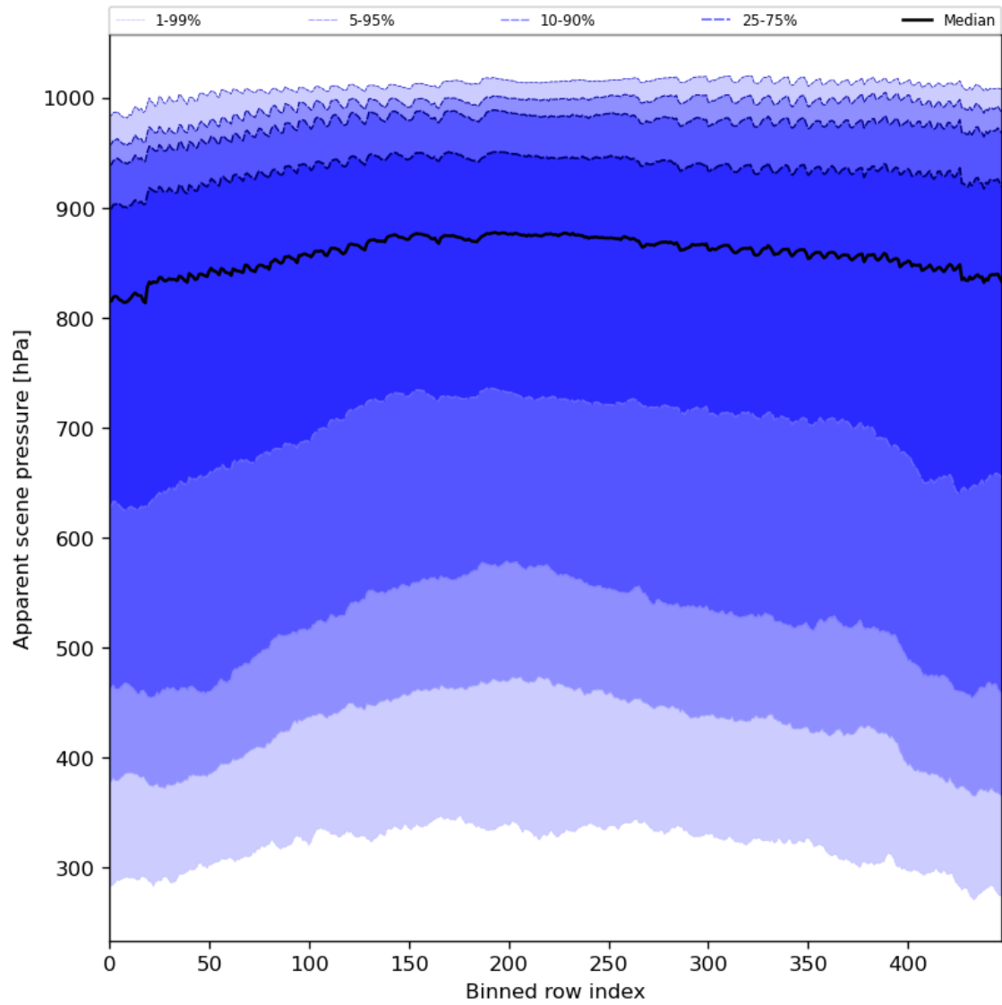
Figure 53: Along track statistics of “Apparent scene pressure” for 2023-07-08 to 2023-07-10
