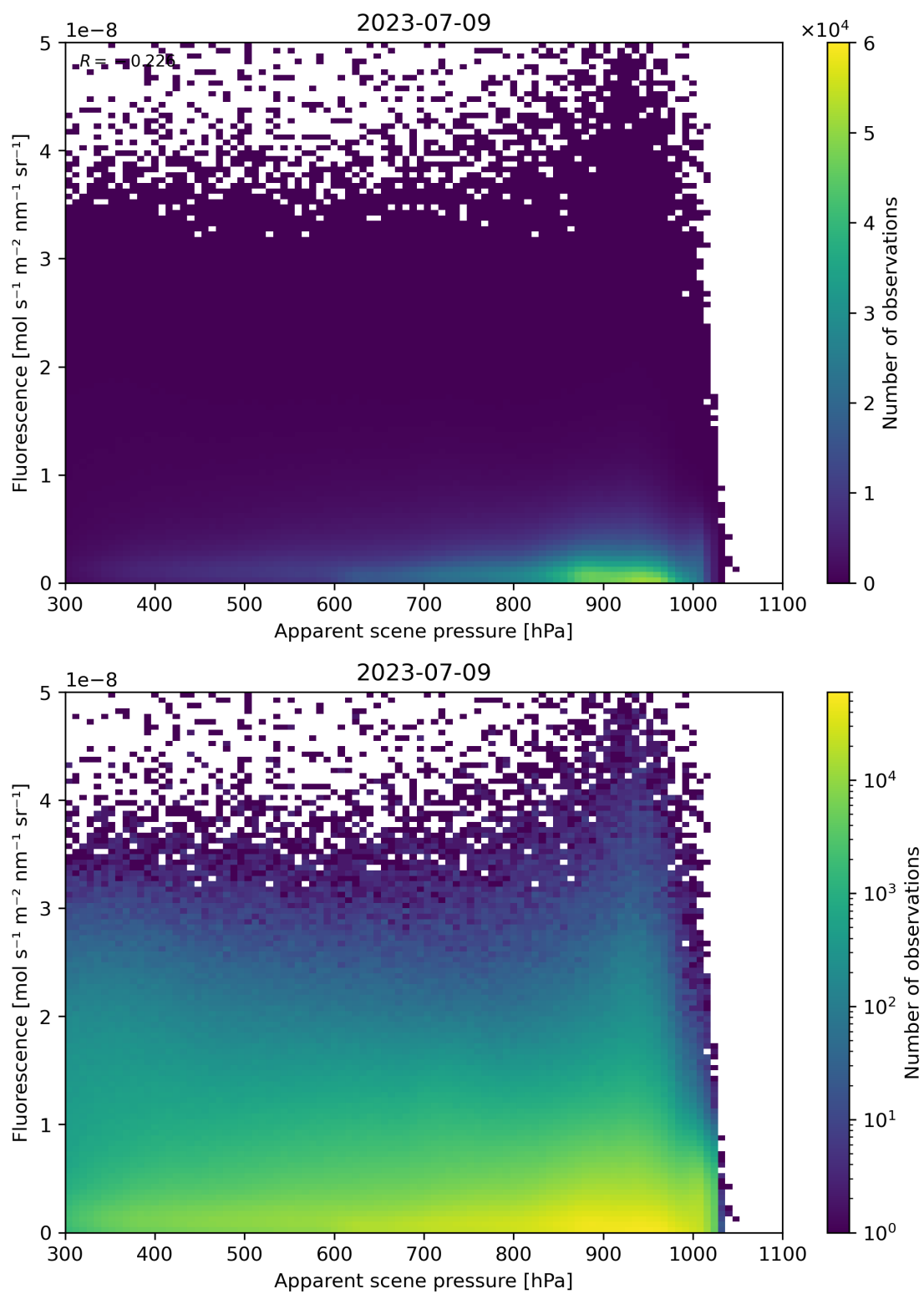
Figure 65: Scatter density plot of “Apparent scene pressure” against “Fluorescence” for 2023-07-08 to 2023-07-10.
