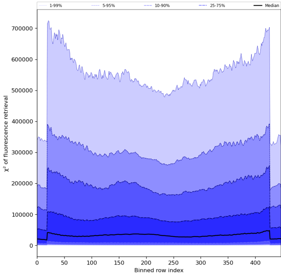
Figure 59: Along track statistics of “ \chi^2 of fluorescence retrieval” for 2023-07-08 to 2023-07-10
