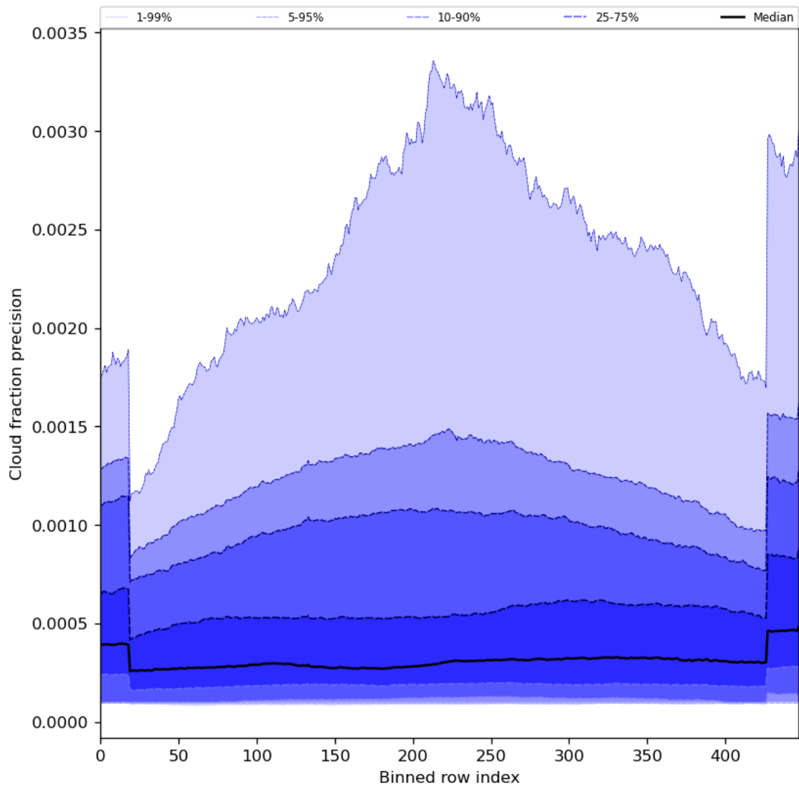
Figure 50: Along track statistics of “Cloud fraction precision” for 2023-07-08 to 2023-07-10
