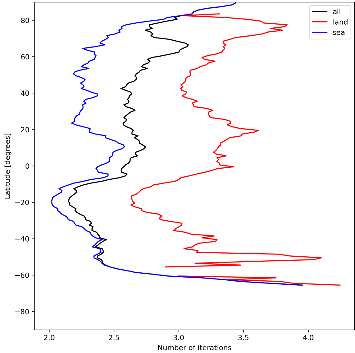
Figure 22: Zonal average of “Number of iterations” for 2023-07-08 to 2023-07-10.
