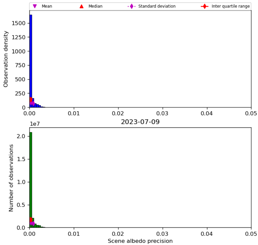
Figure 35: Histogram of “Scene albedo precision” for 2023-07-08 to 2023-07-10
