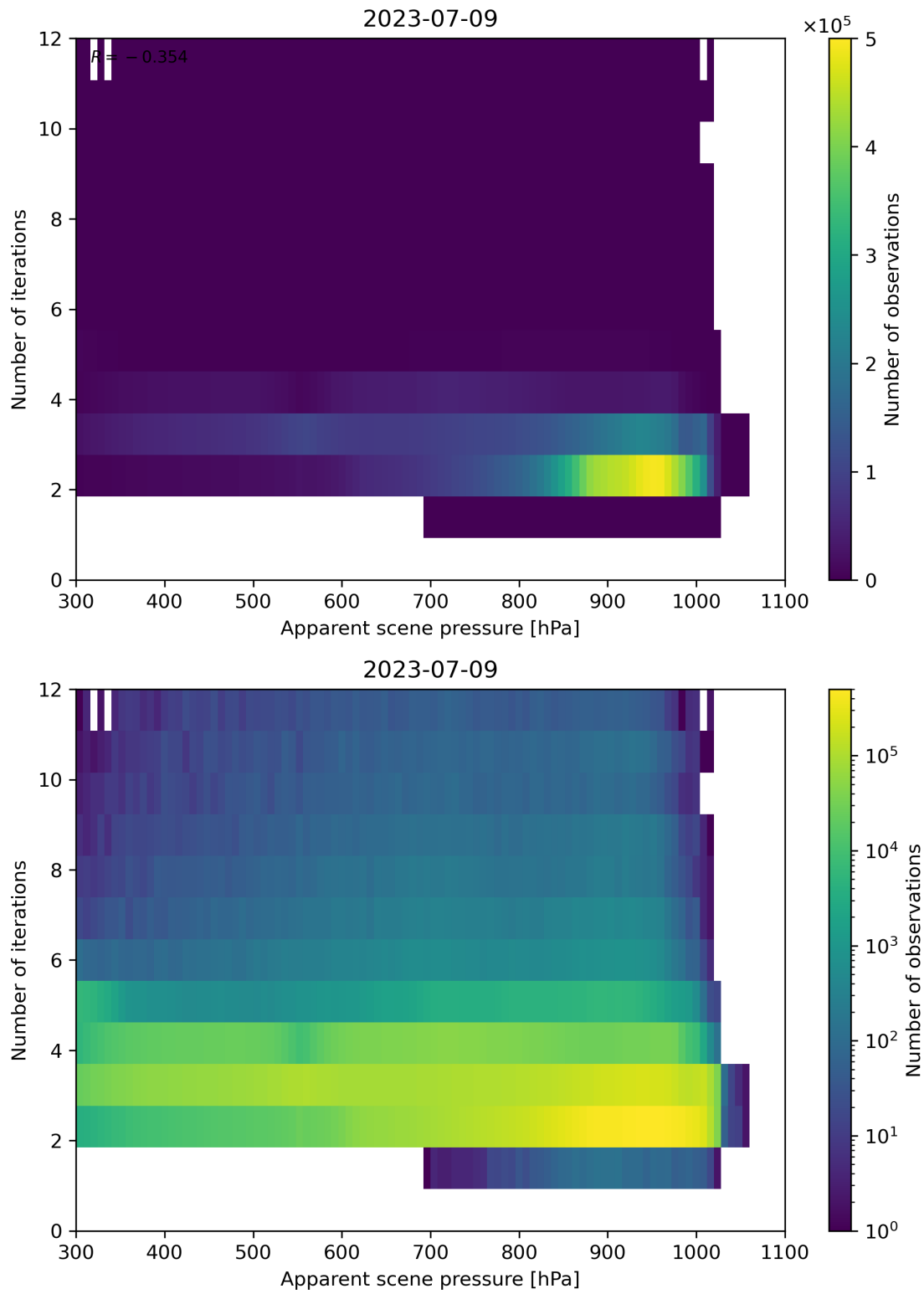
Figure 66: Scatter density plot of “Apparent scene pressure” against “Number of iterations” for 2023-07-08 to 2023-07-10.
