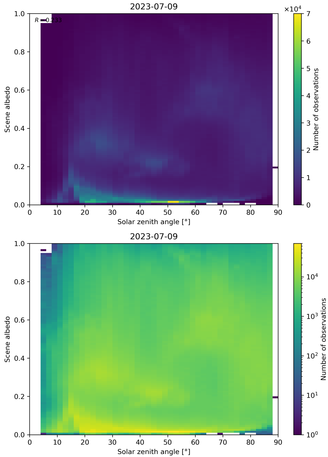
Figure 127: Scatter density plot of “Solar zenith angle” against “Scene albedo” for 2023-07-08 to 2023-07-10.
