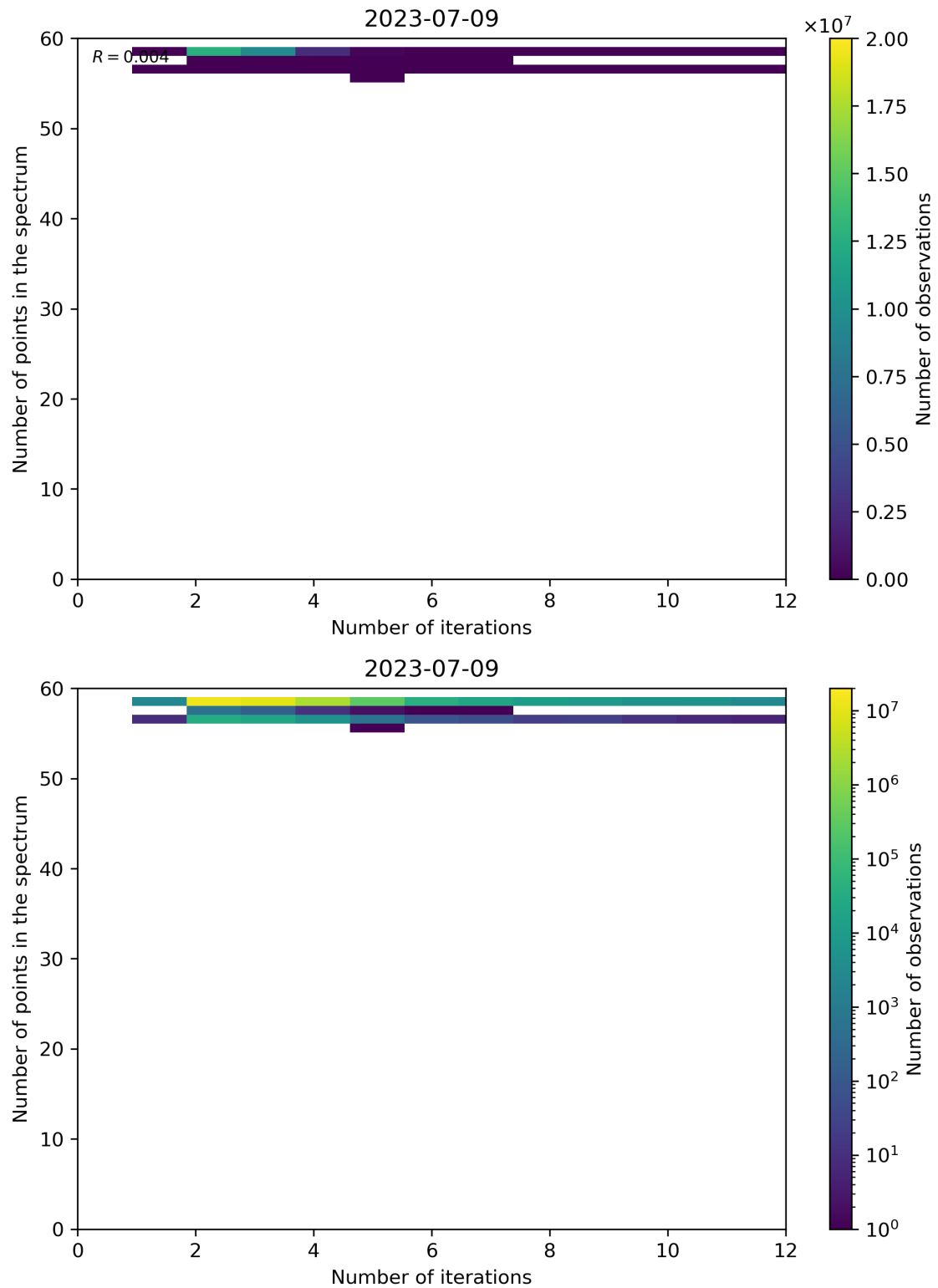
Figure 108: Scatter density plot of “Number of iterations” against “Number of points in the spectrum” for 2023-07-08 to 2023-07-10.
