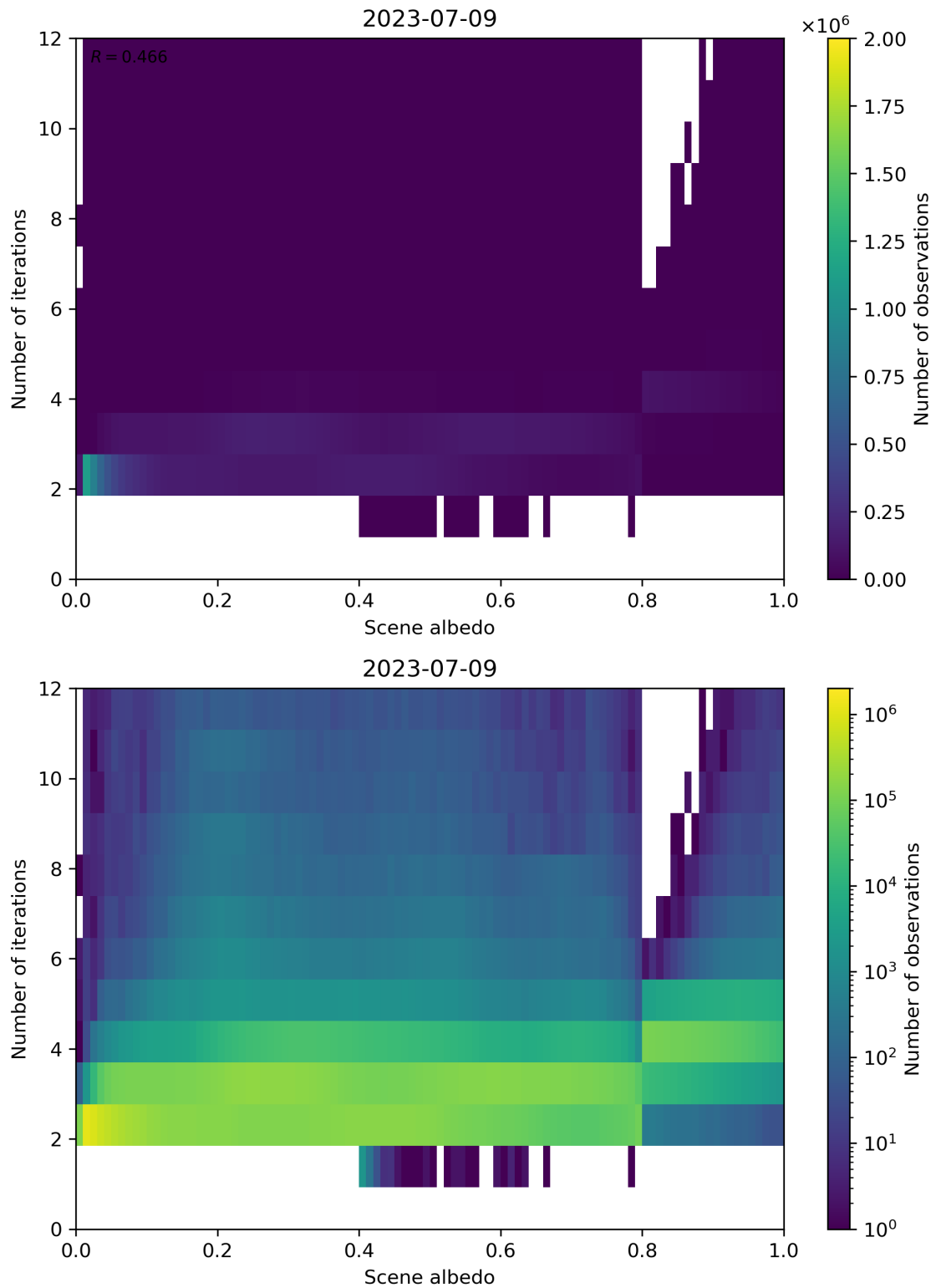
Figure 115: Scatter density plot of “Scene albedo” against “Number of iterations” for 2023-07-08 to 2023-07-10.
