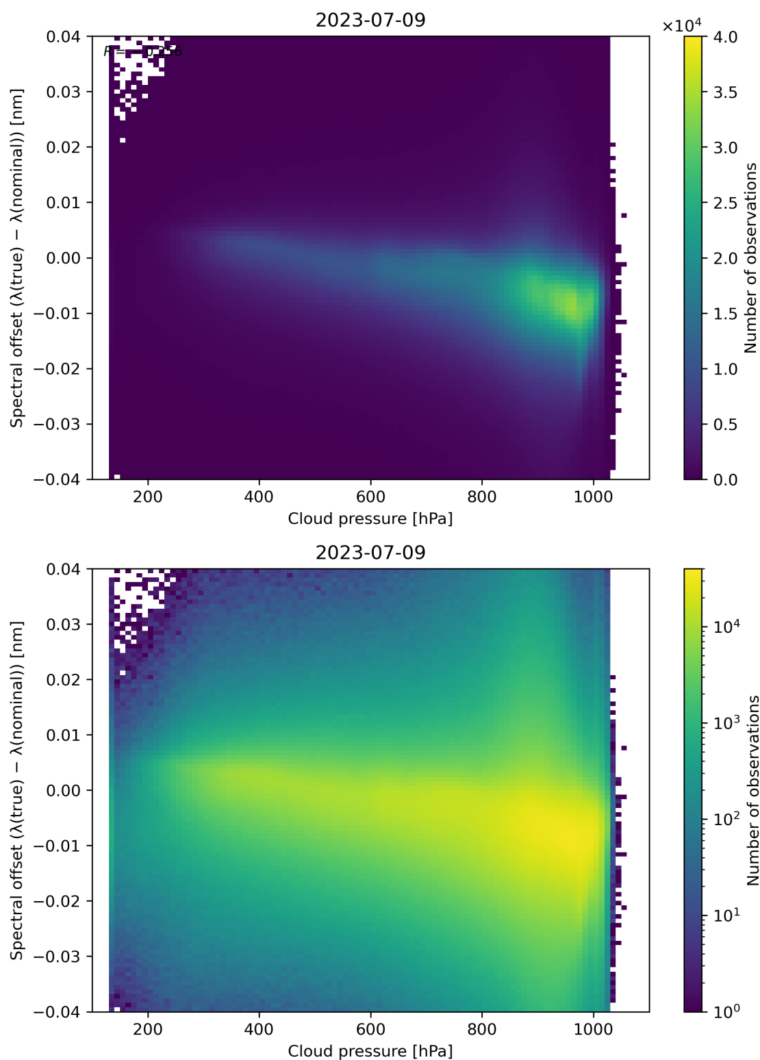
Figure 92: Scatter density plot of “Cloud pressure” against “Spectral offset ( \lambda(\text{true}) - \lambda(\text{nominal}) )” for 2023-07-08 to 2023-07-10.
