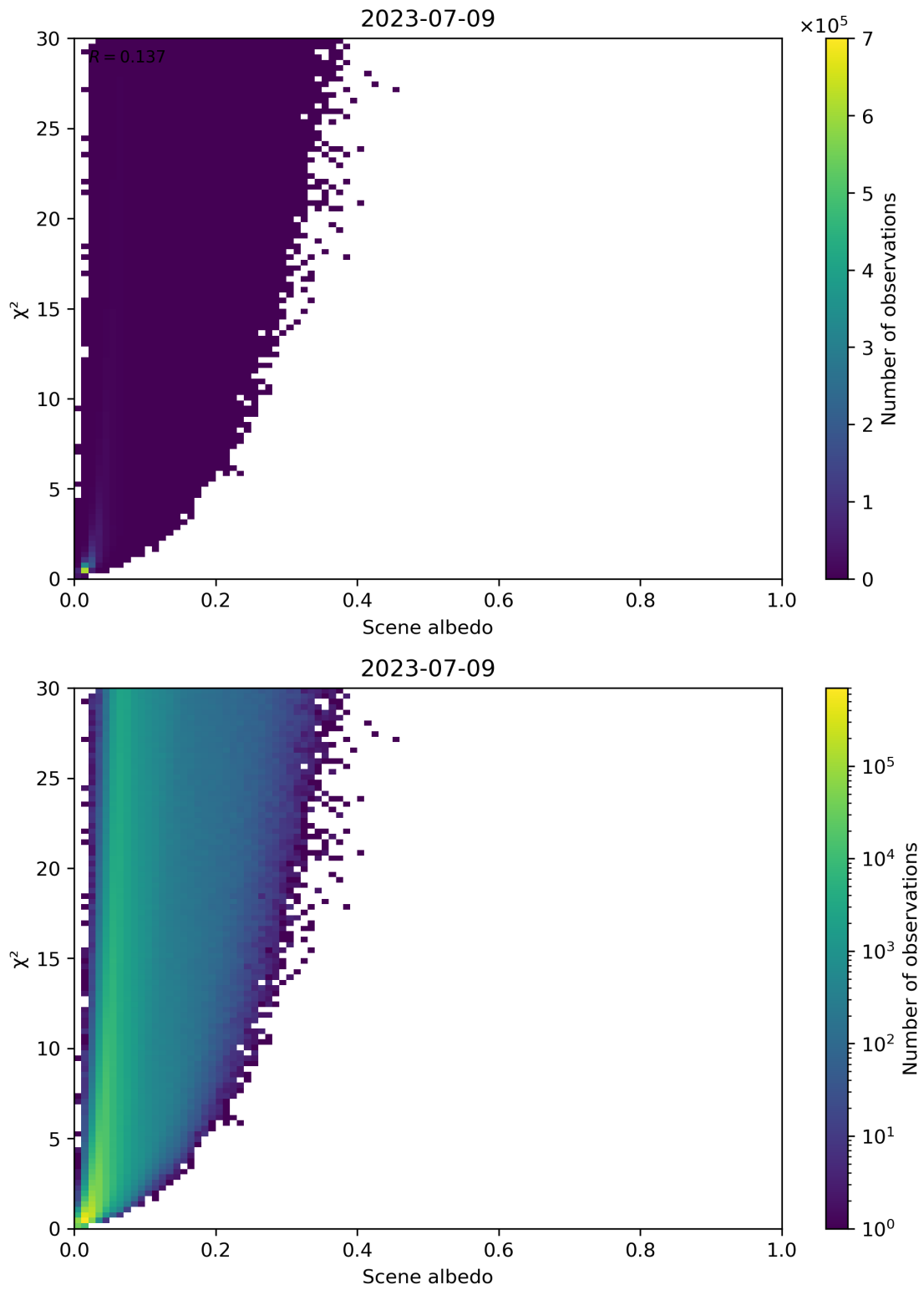
Figure 112: Scatter density plot of “Scene albedo” against “ \chi^2 ” for 2023-07-08 to 2023-07-10.
