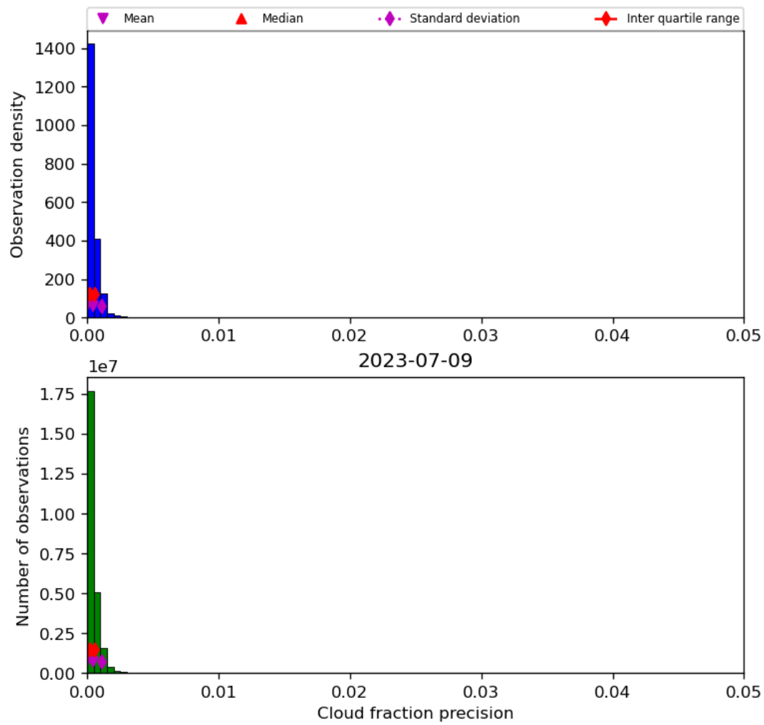
Figure 33: Histogram of “Cloud fraction precision” for 2023-07-08 to 2023-07-10
