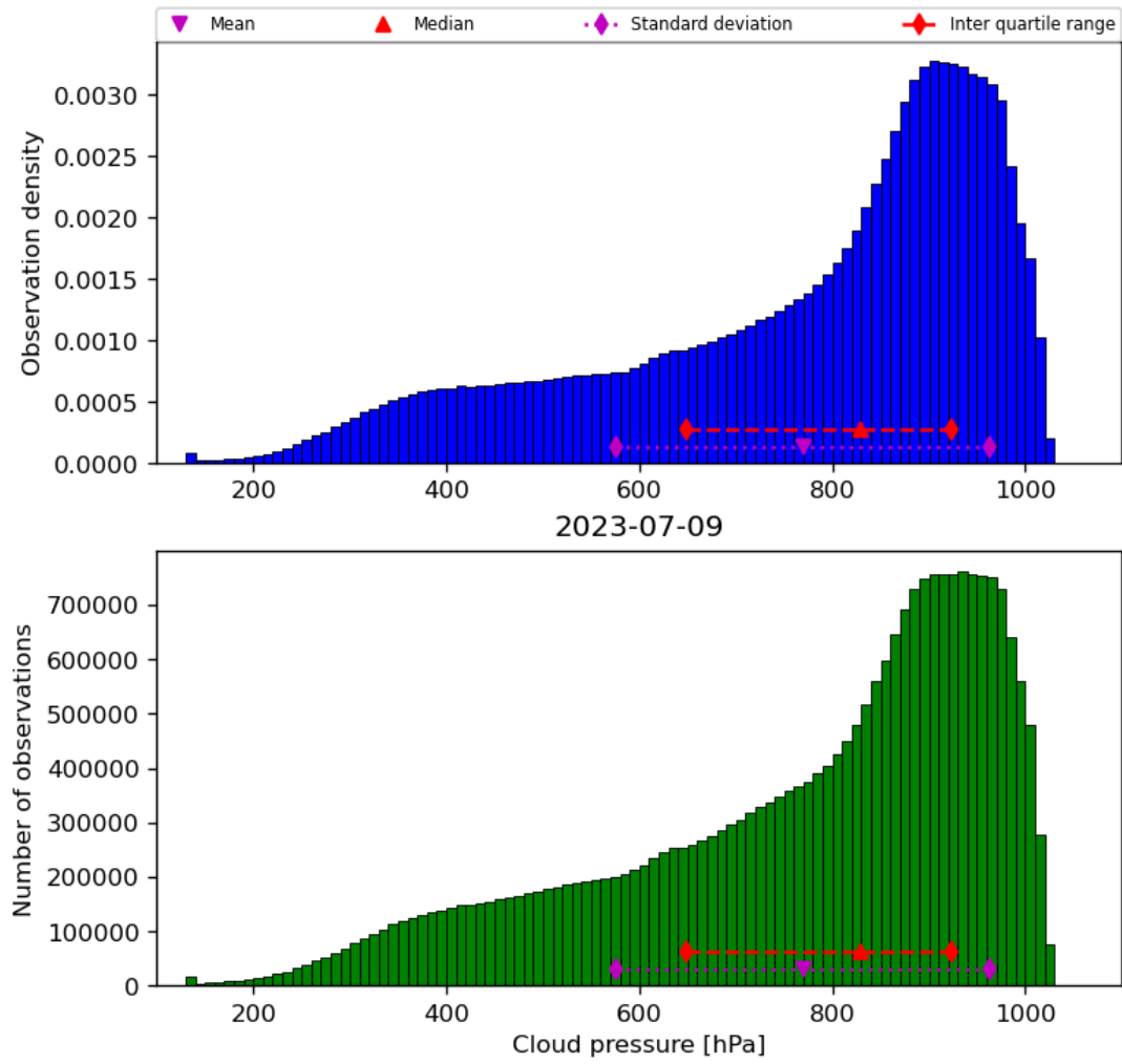
Figure 30: Histogram of “Cloud pressure” for 2023-07-08 to 2023-07-10
