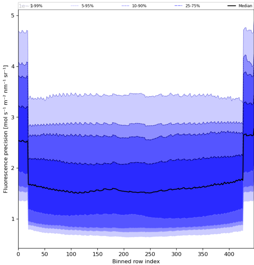
Figure 58: Along track statistics of “Fluorescence precision” for 2023-07-08 to 2023-07-10
