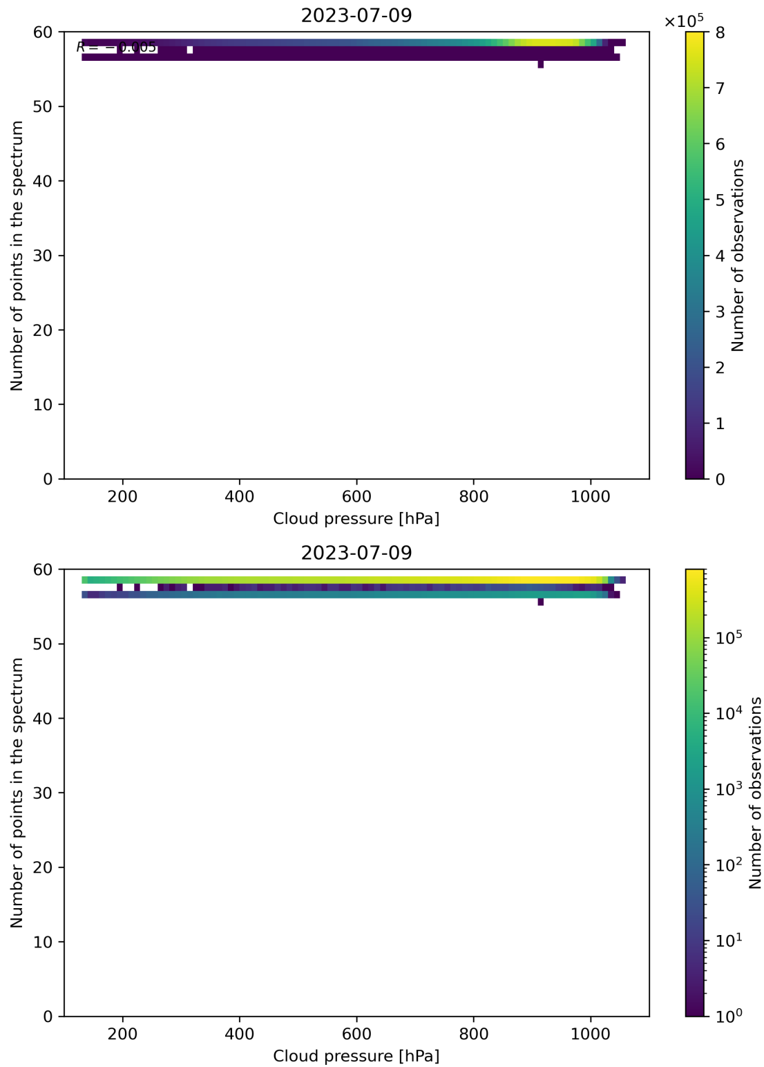
Figure 90: Scatter density plot of “Cloud pressure” against “Number of points in the spectrum” for 2023-07-08 to 2023-07-10.
