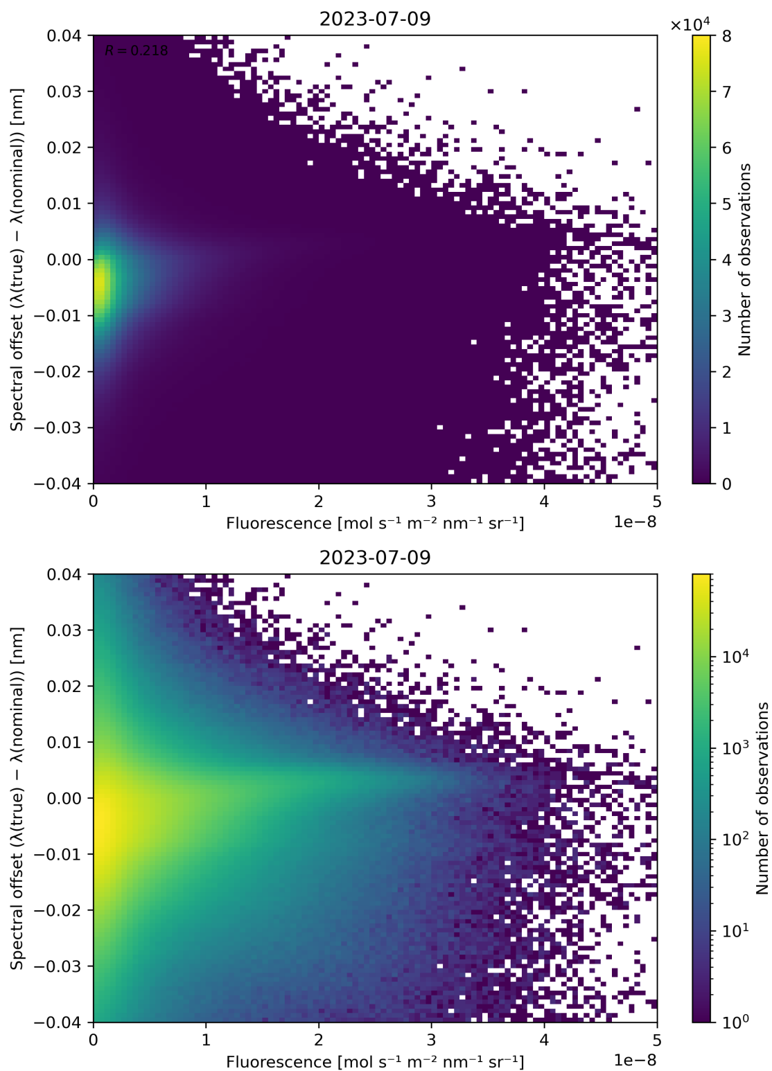
Figure 95: Scatter density plot of “Fluorescence” against “Spectral offset ( \lambda(\text{true}) - \lambda(\text{nominal}) )” for 2023-07-08 to 2023-07-10.
