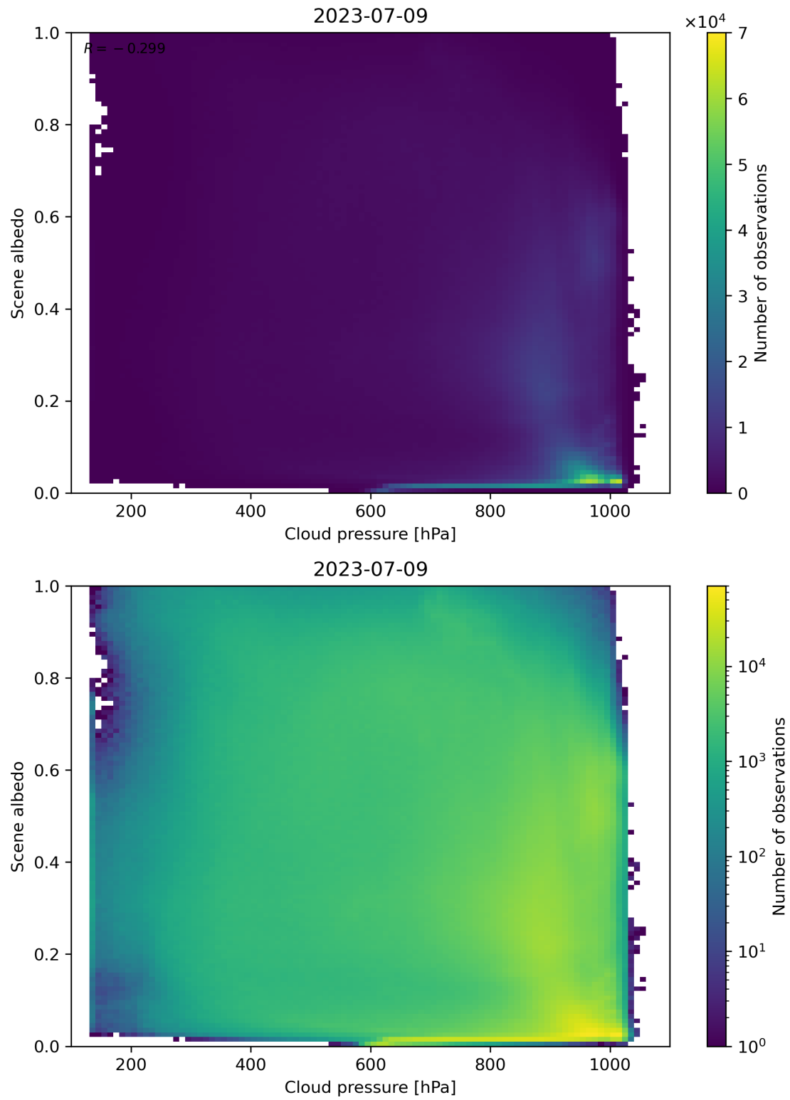
Figure 91: Scatter density plot of “Cloud pressure” against “Scene albedo” for 2023-07-08 to 2023-07-10.
