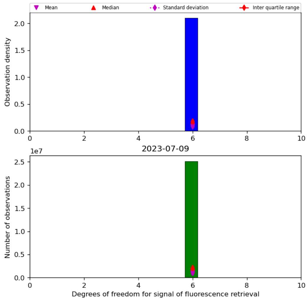
Figure 43: Histogram of “Degrees of freedom for signal of fluorescence retrieval” for 2023-07-08 to 2023-07-10
