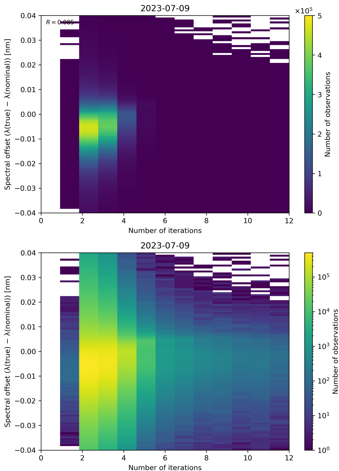
Figure 109: Scatter density plot of “Number of iterations” against “Spectral offset ( \lambda(\text{true}) - \lambda(\text{nominal}) )” for 2023-07-08 to 2023-07-10.
