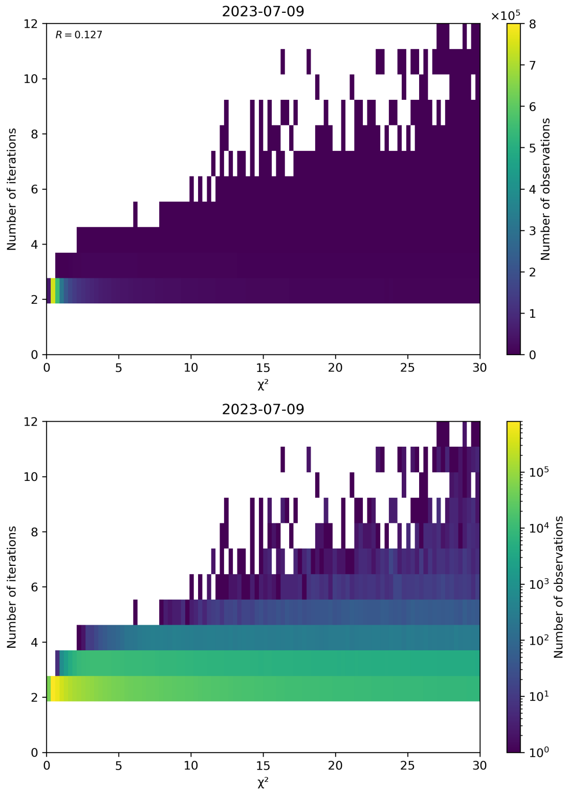
Figure 73: Scatter density plot of “ \chi^2 ” against “Number of iterations” for 2023-07-08 to 2023-07-10.
