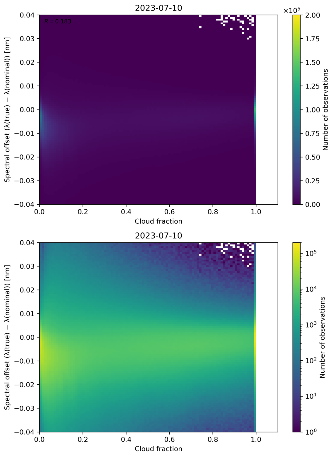
Figure 83: Scatter density plot of “Cloud fraction” against “Spectral offset ( \lambda(\text{true}) - \lambda(\text{nominal}) )” for 2023-07-09 to 2023-07-11.
