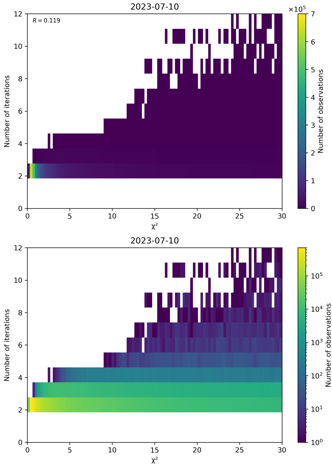
Figure 73: Scatter density plot of “ \chi^2 ” against “Number of iterations” for 2023-07-09 to 2023-07-11.
