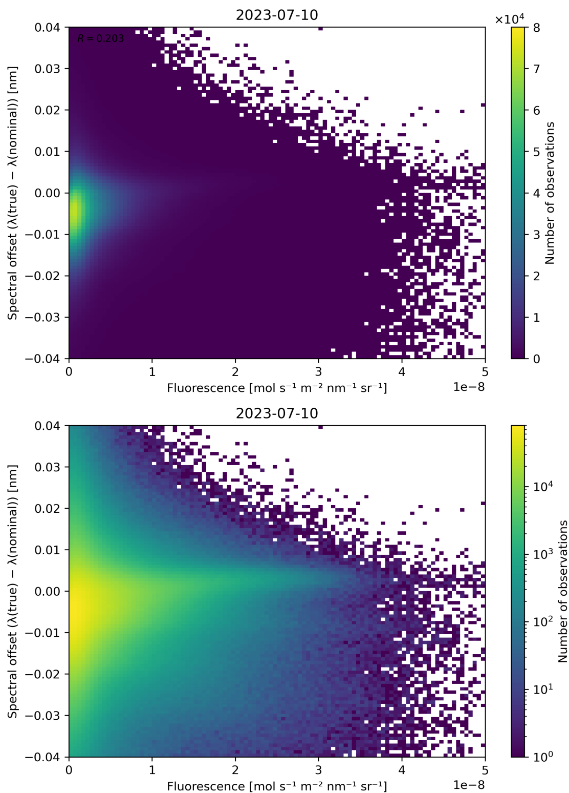
Figure 95: Scatter density plot of “Fluorescence” against “Spectral offset ( \lambda(\text{true}) - \lambda(\text{nominal}) )” for 2023-07-09 to 2023-07-11.
