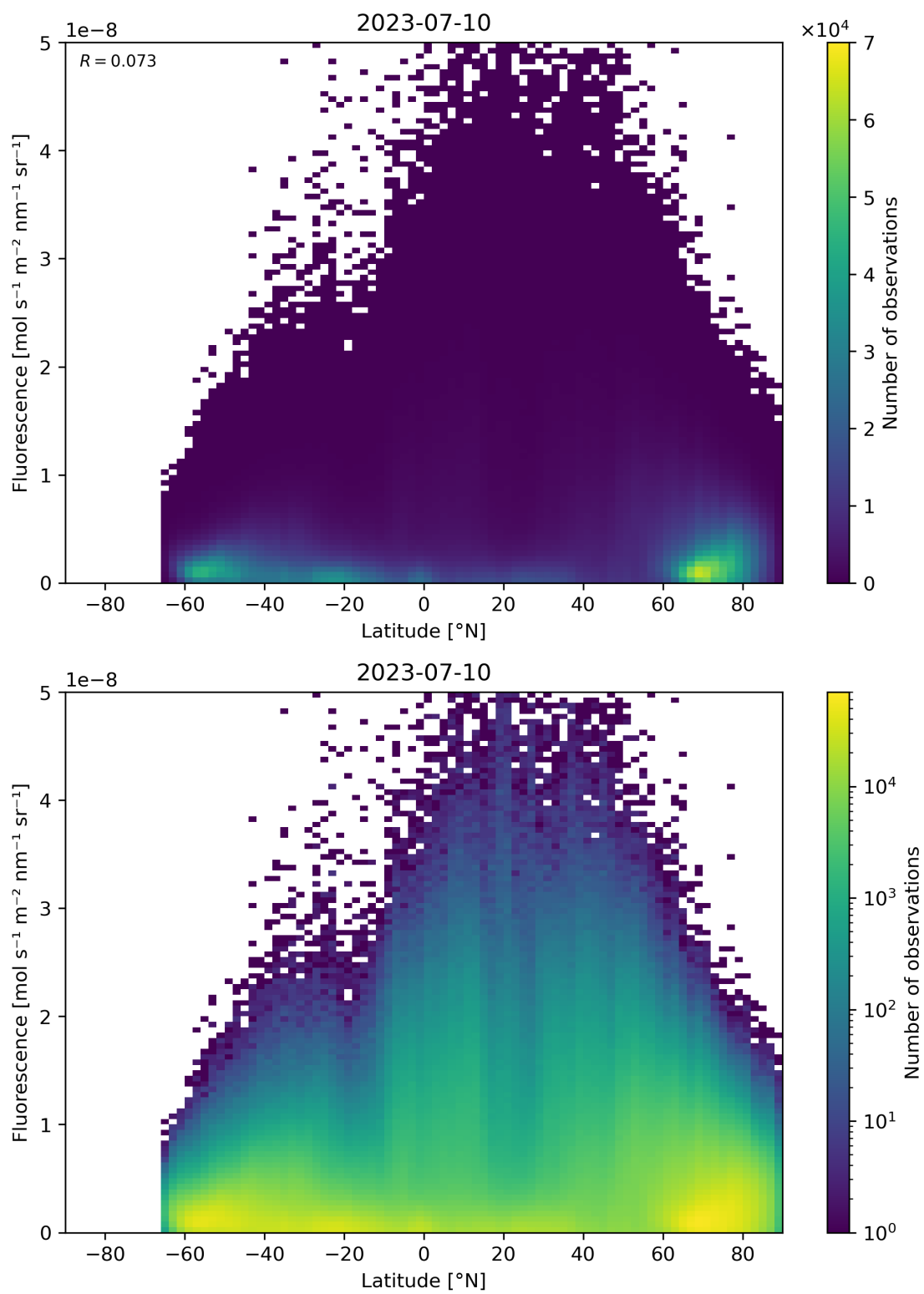
Figure 101: Scatter density plot of “Latitude” against “Fluorescence” for 2023-07-09 to 2023-07-11.
