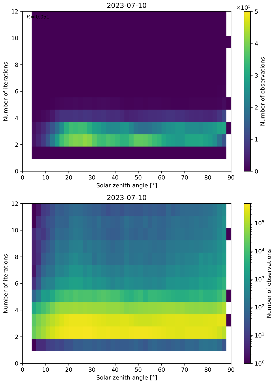
Figure 125: Scatter density plot of “Solar zenith angle” against “Number of iterations” for 2023-07-09 to 2023-07-11.
