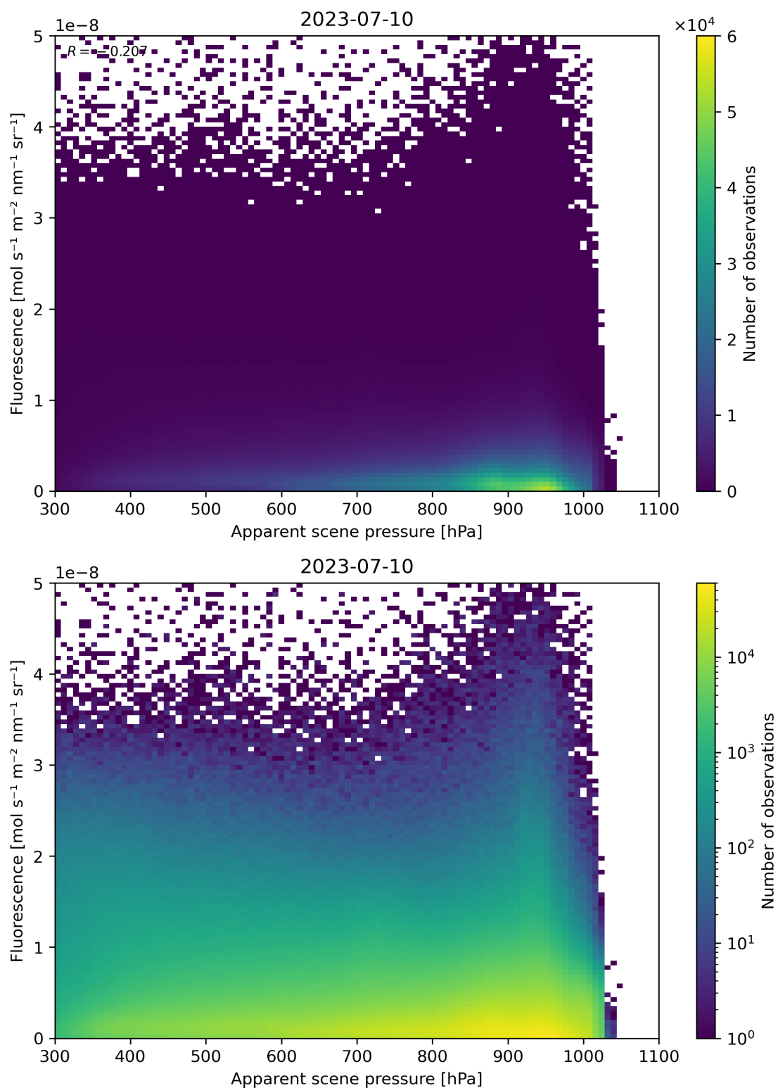
Figure 65: Scatter density plot of “Apparent scene pressure” against “Fluorescence” for 2023-07-09 to 2023-07-11.
