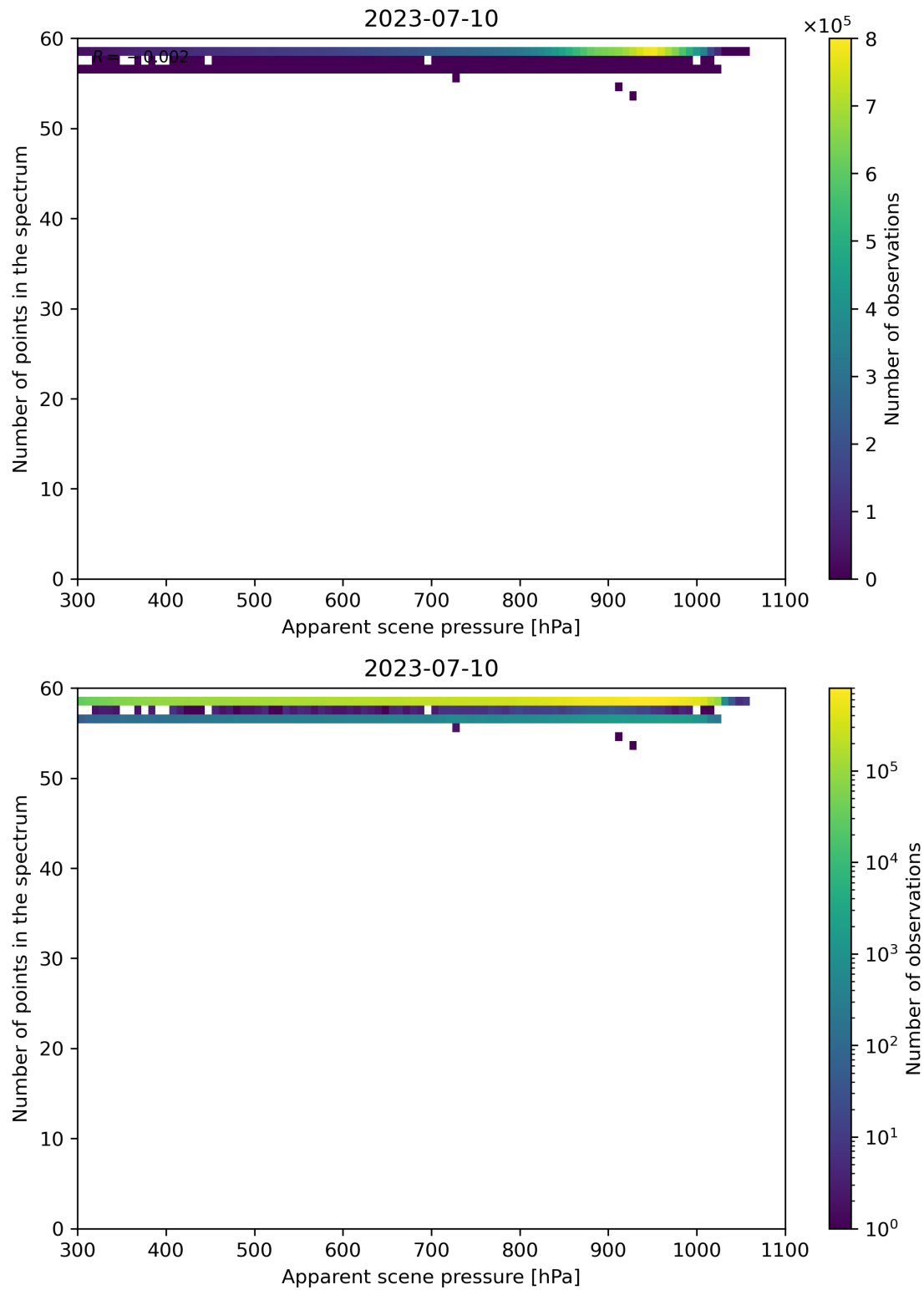
Figure 67: Scatter density plot of “Apparent scene pressure” against “Number of points in the spectrum” for 2023-07-09 to 2023-07-11.
