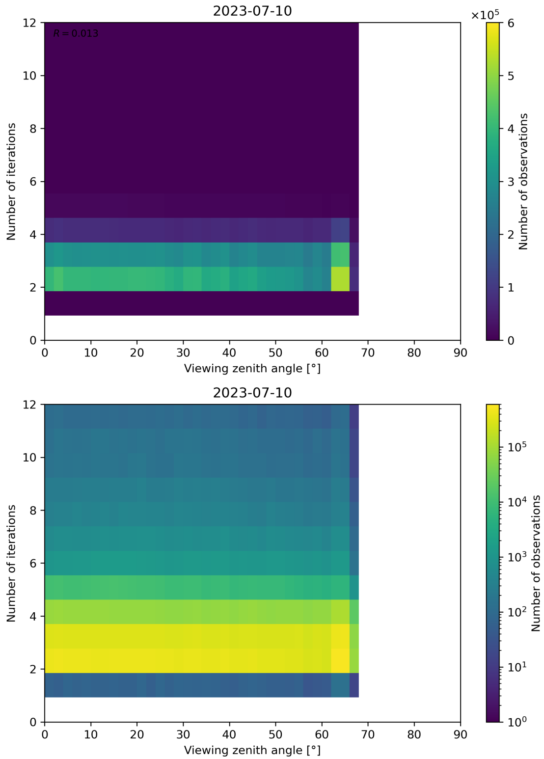
Figure 136: Scatter density plot of “Viewing zenith angle” against “Number of iterations” for 2023-07-09 to 2023-07-11.
