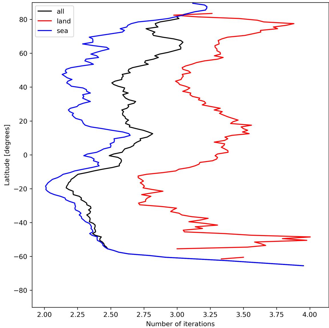
Figure 22: Zonal average of “Number of iterations” for 2023-07-09 to 2023-07-11.
