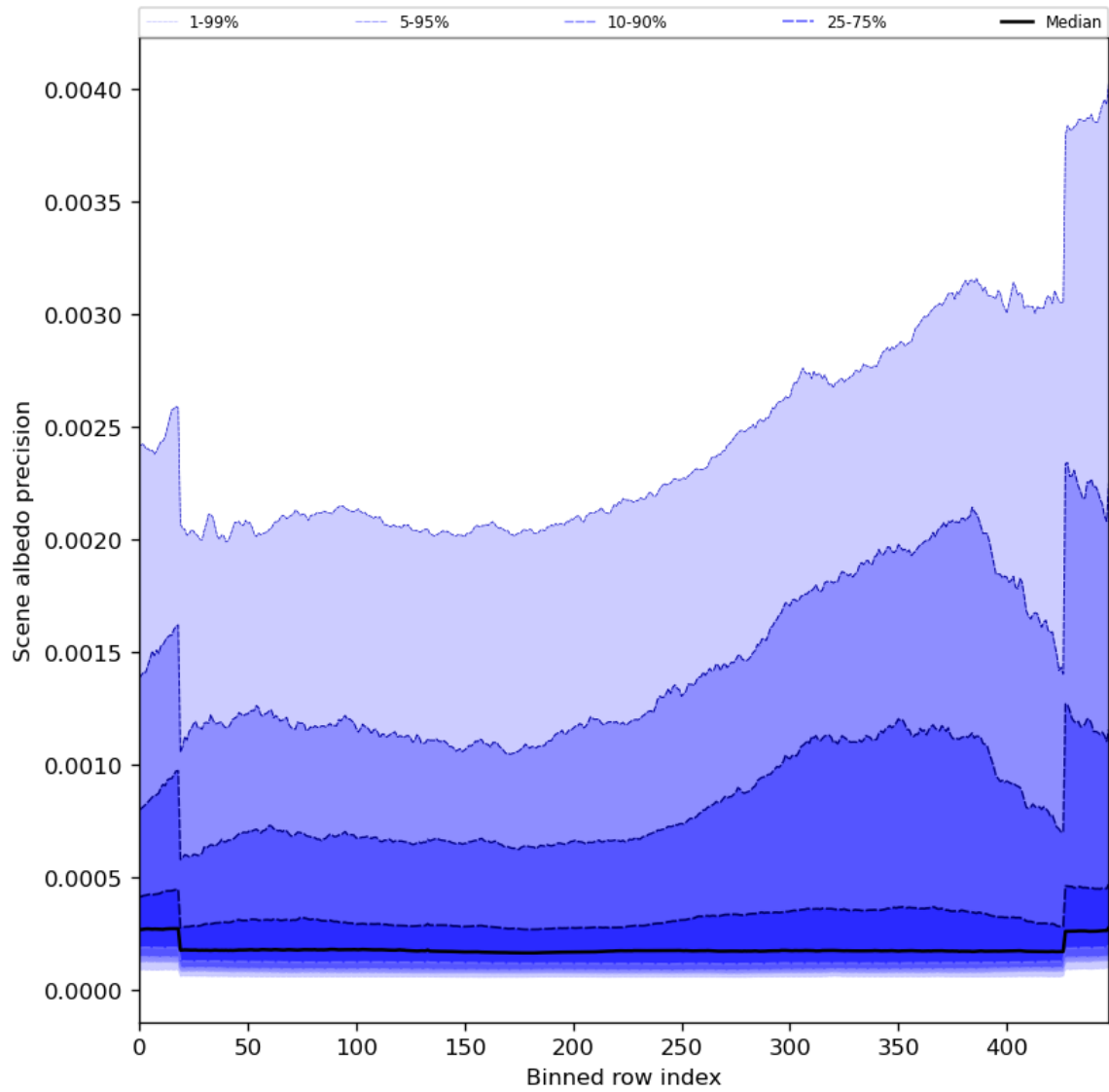
Figure 52: Along track statistics of “Scene albedo precision” for 2023-07-09 to 2023-07-11
