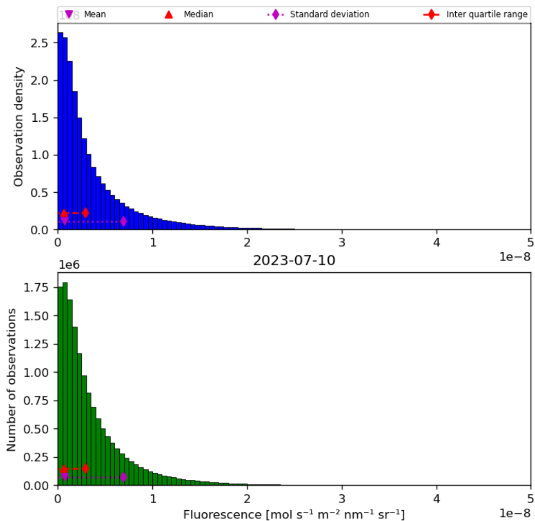
Figure 40: Histogram of “Fluorescence” for 2023-07-09 to 2023-07-11
