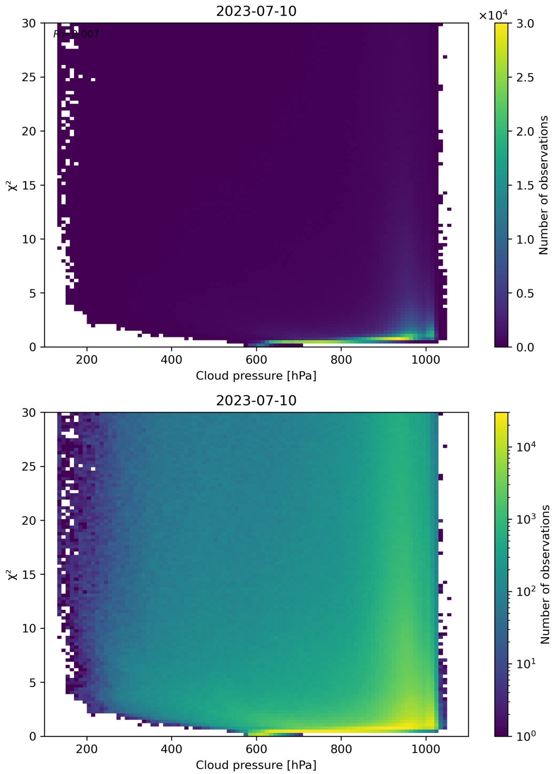
Figure 85: Scatter density plot of “Cloud pressure” against “ \chi^2 ” for 2023-07-09 to 2023-07-11.
