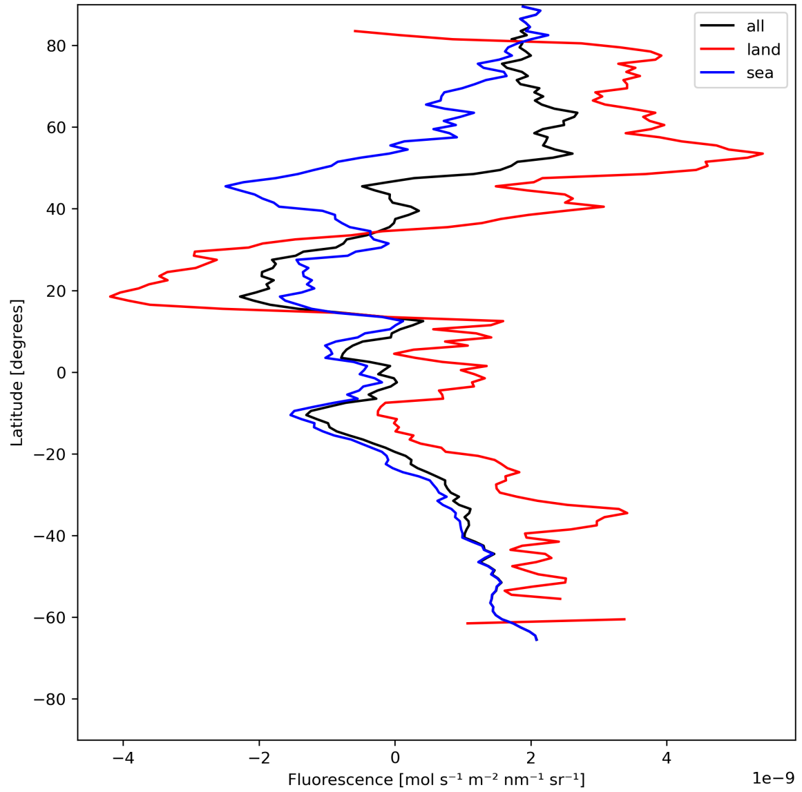
Figure 23: Zonal average of “Fluorescence” for 2023-07-09 to 2023-07-11.
