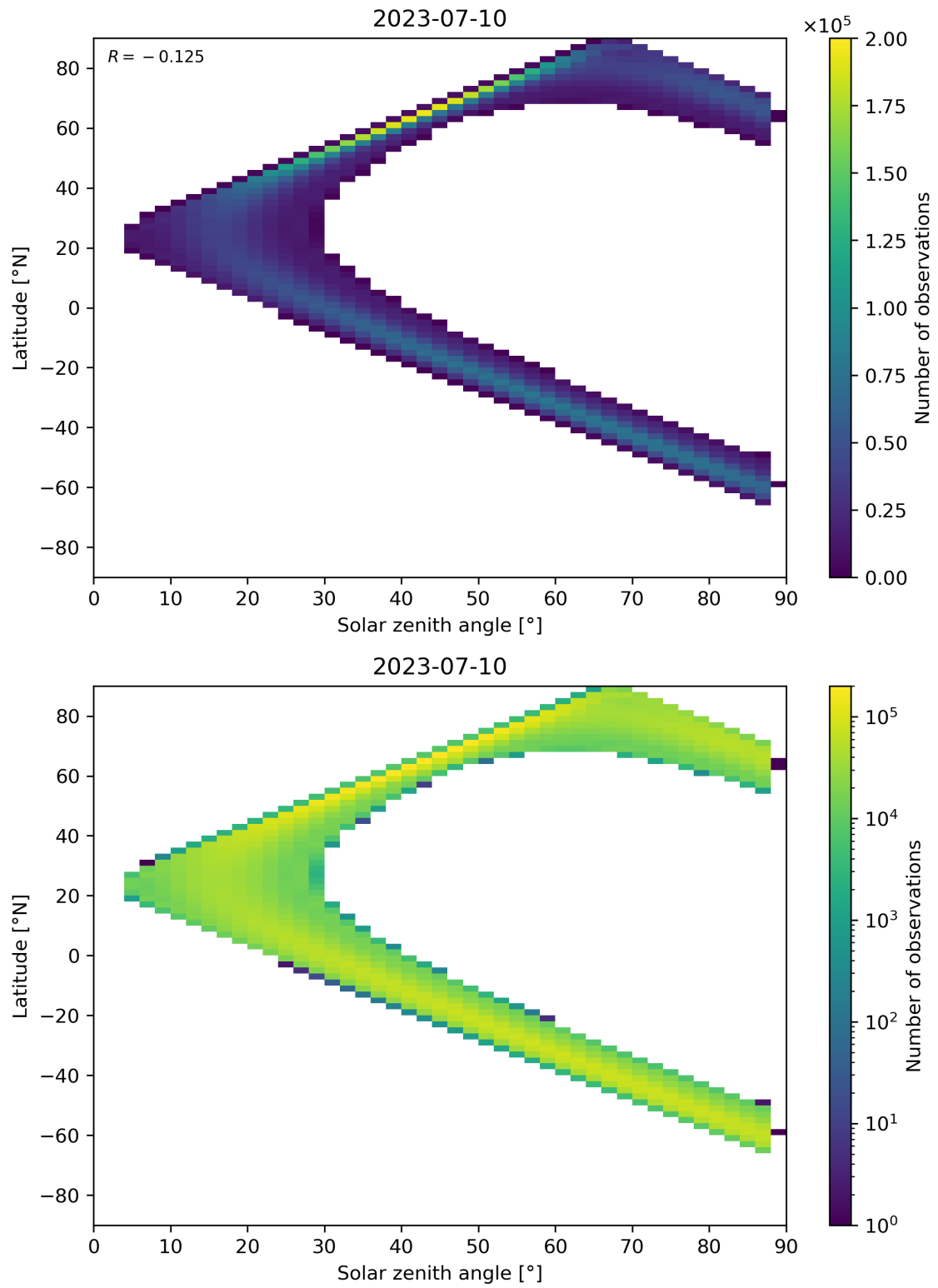
Figure 124: Scatter density plot of “Solar zenith angle” against “Latitude” for 2023-07-09 to 2023-07-11.
