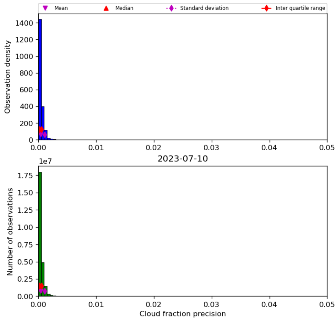
Figure 33: Histogram of “Cloud fraction precision” for 2023-07-09 to 2023-07-11
