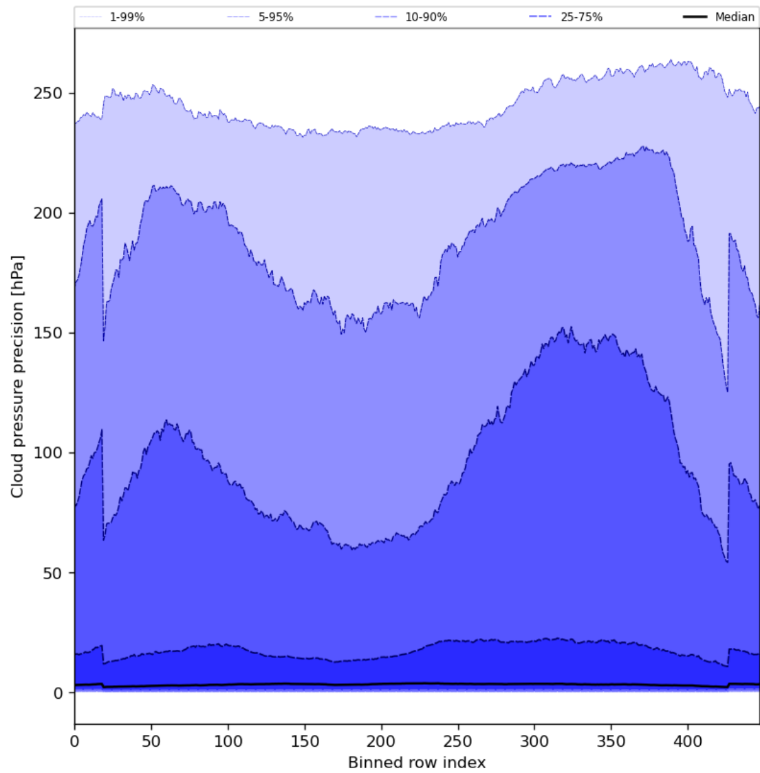
Figure 48: Along track statistics of “Cloud pressure precision” for 2023-07-09 to 2023-07-11
