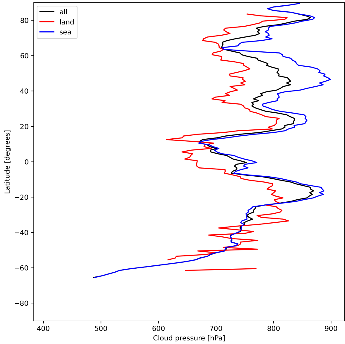
Figure 13: Zonal average of “Cloud pressure” for 2023-07-09 to 2023-07-11.
