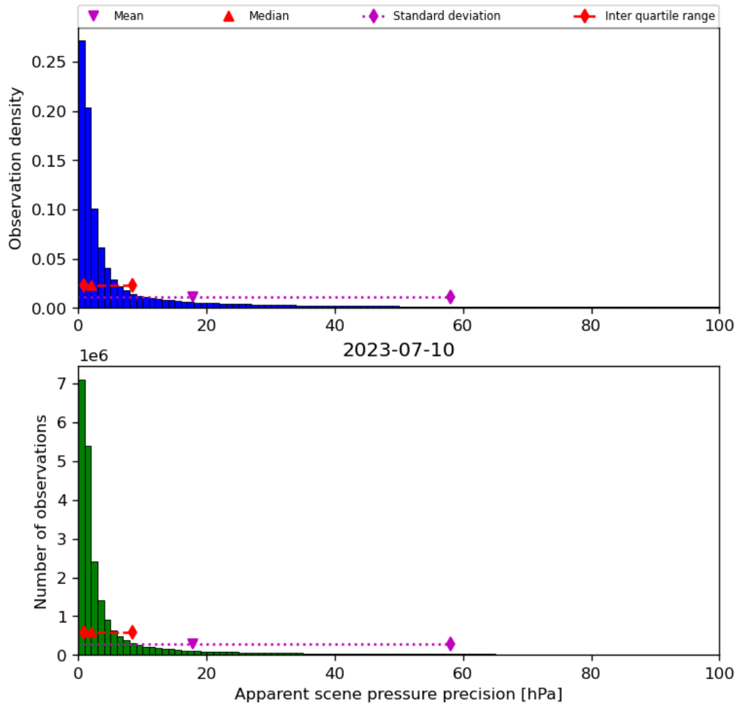
Figure 37: Histogram of “Apparent scene pressure precision” for 2023-07-09 to 2023-07-11
