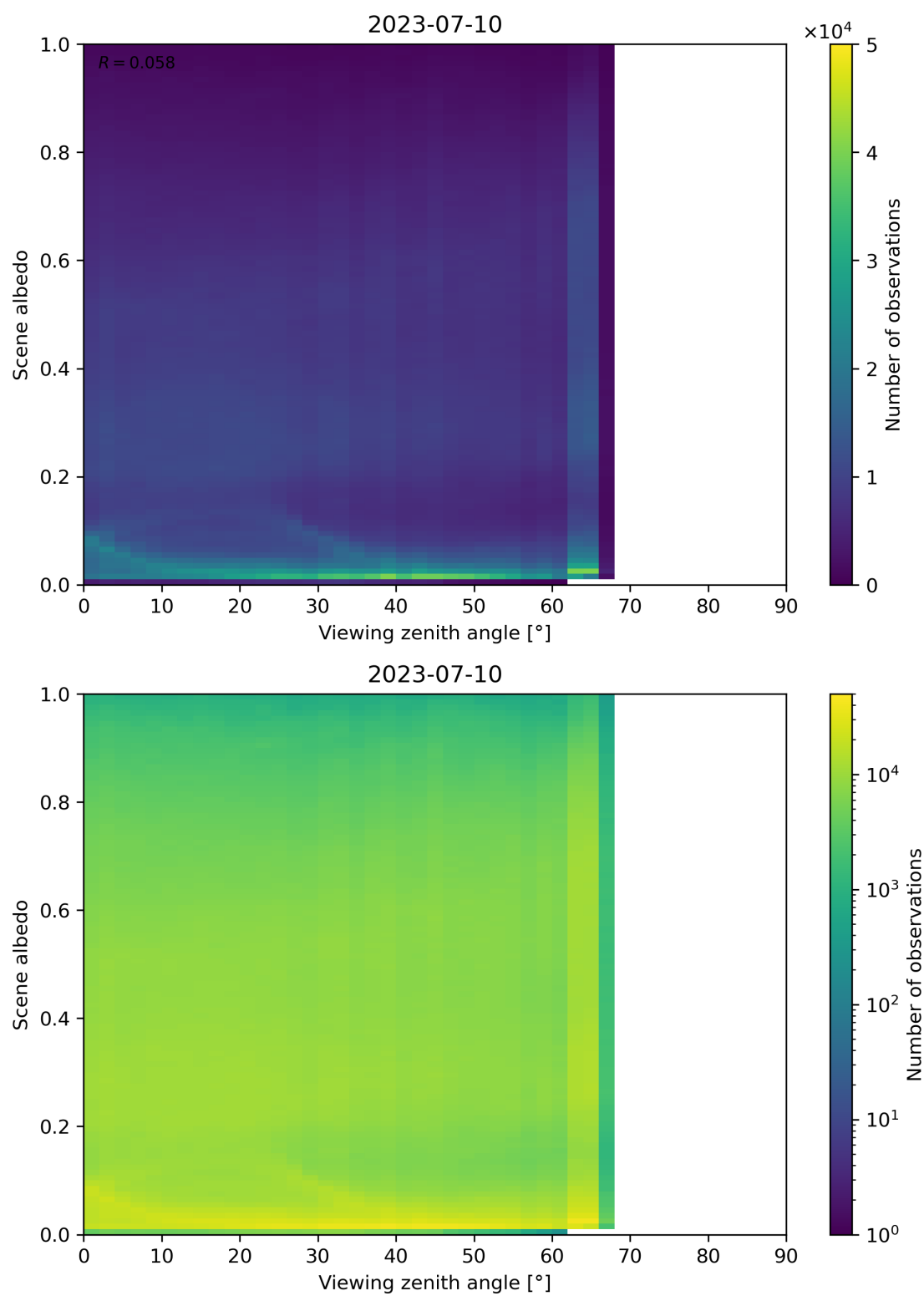
Figure 138: Scatter density plot of “Viewing zenith angle” against “Scene albedo” for 2023-07-09 to 2023-07-11.
