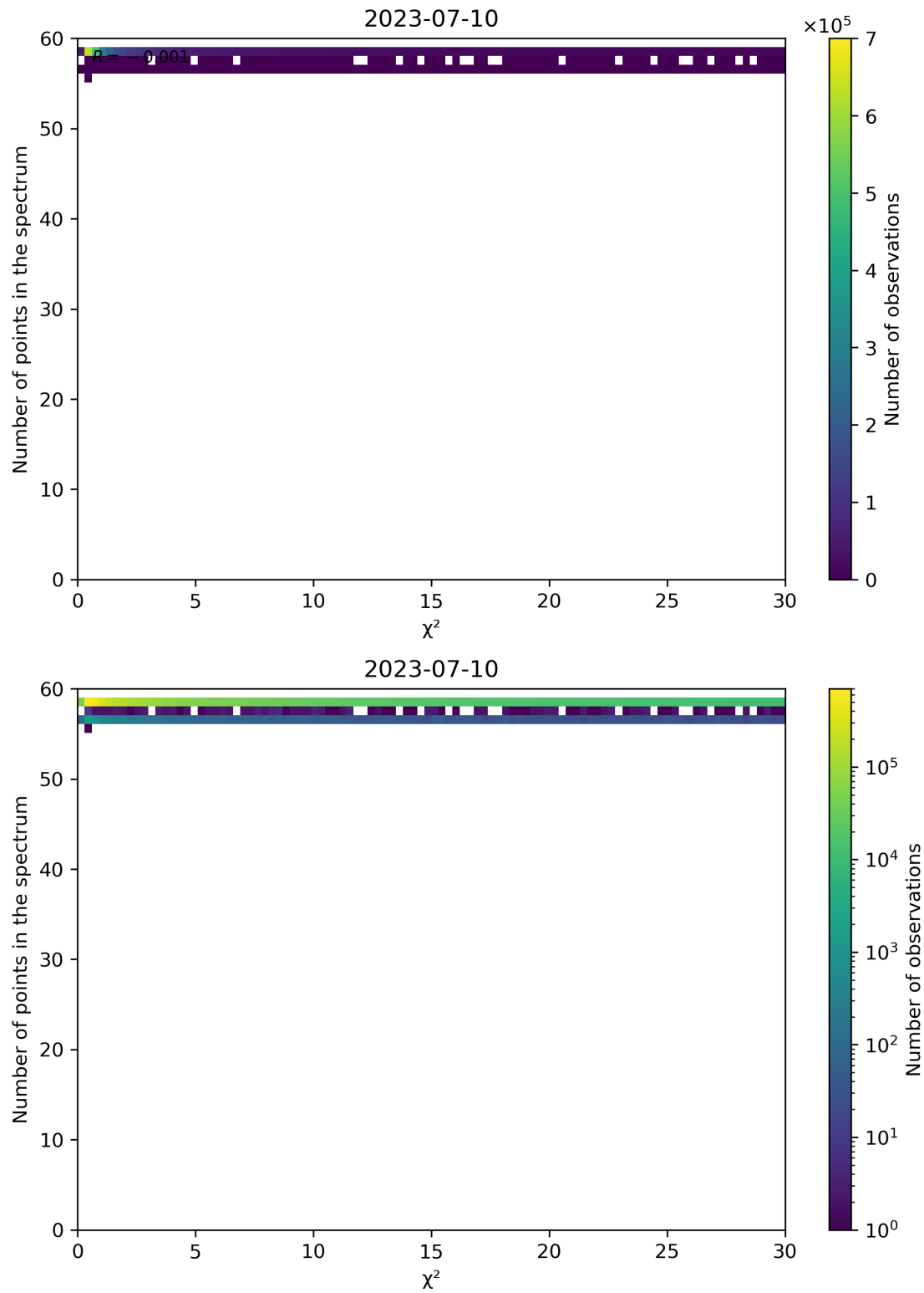
Figure 74: Scatter density plot of “ \chi^2 ” against “Number of points in the spectrum” for 2023-07-09 to 2023-07-11.
