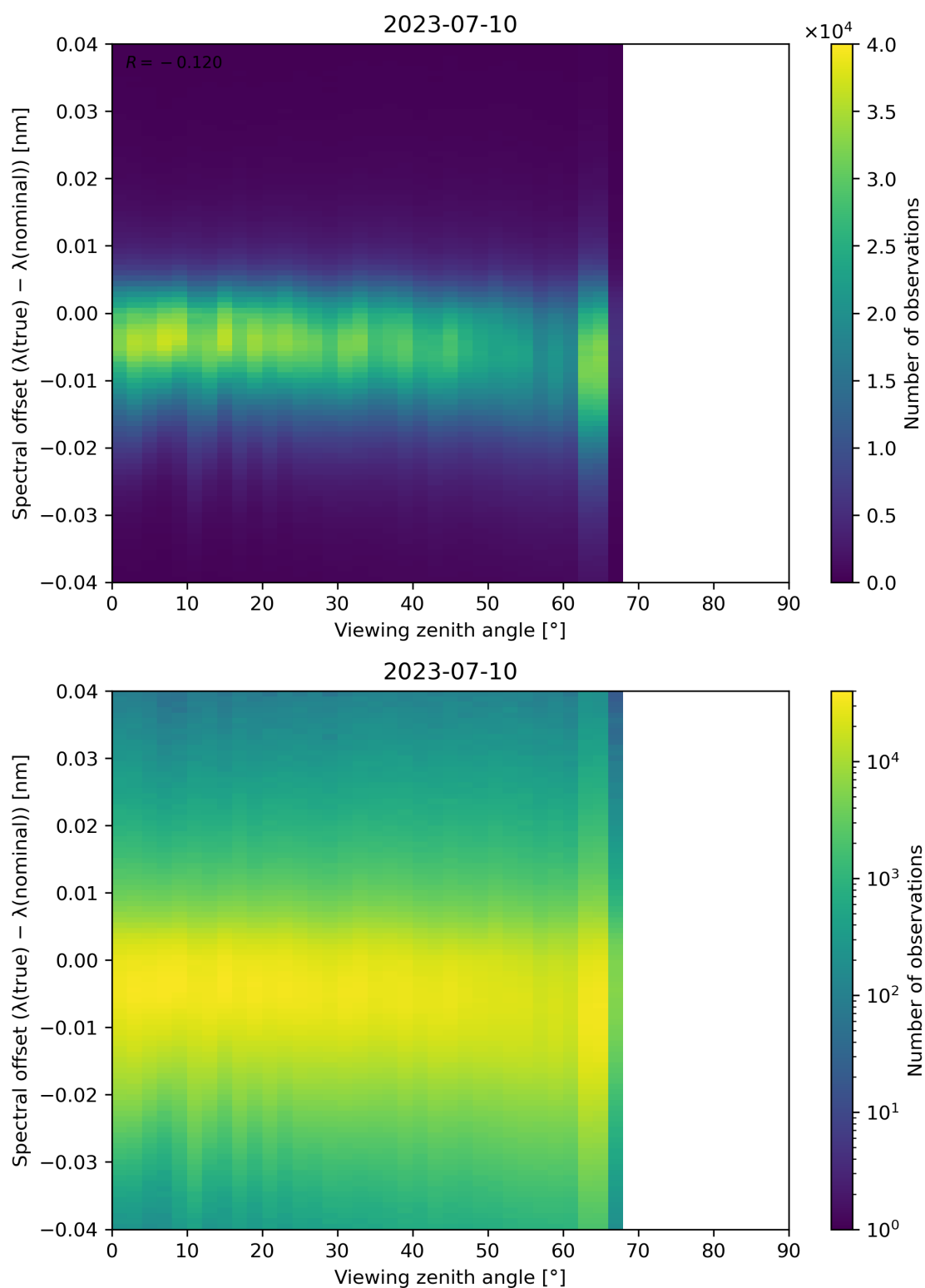
Figure 140: Scatter density plot of “Viewing zenith angle” against “Spectral offset ( \lambda(\text{true}) - \lambda(\text{nominal}) )” for 2023-07-09 to 2023-07-11.
