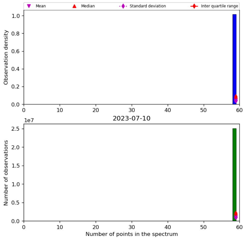
Figure 44: Histogram of "Number of points in the spectrum" for 2023-07-09 to 2023-07-11
