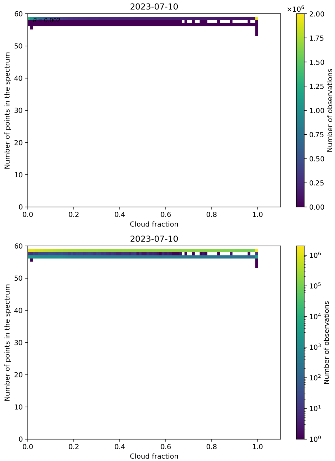
Figure 81: Scatter density plot of “Cloud fraction” against “Number of points in the spectrum” for 2023-07-09 to 2023-07-11.
