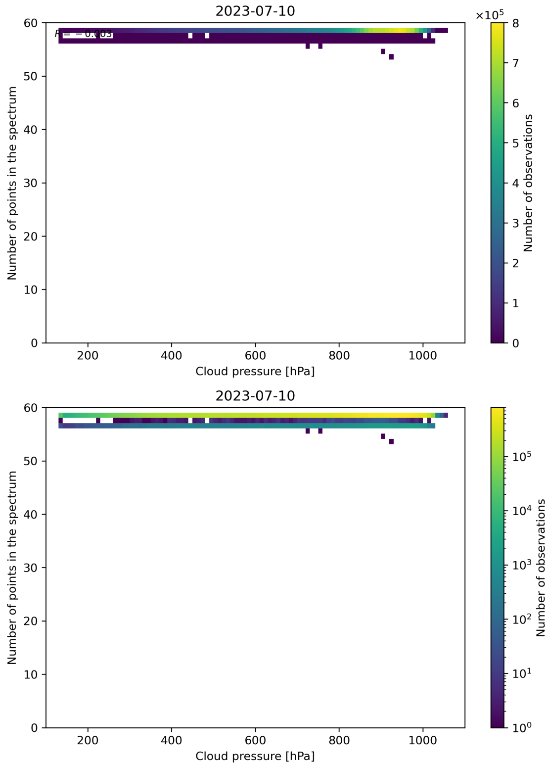
Figure 90: Scatter density plot of “Cloud pressure” against “Number of points in the spectrum” for 2023-07-09 to 2023-07-11.
