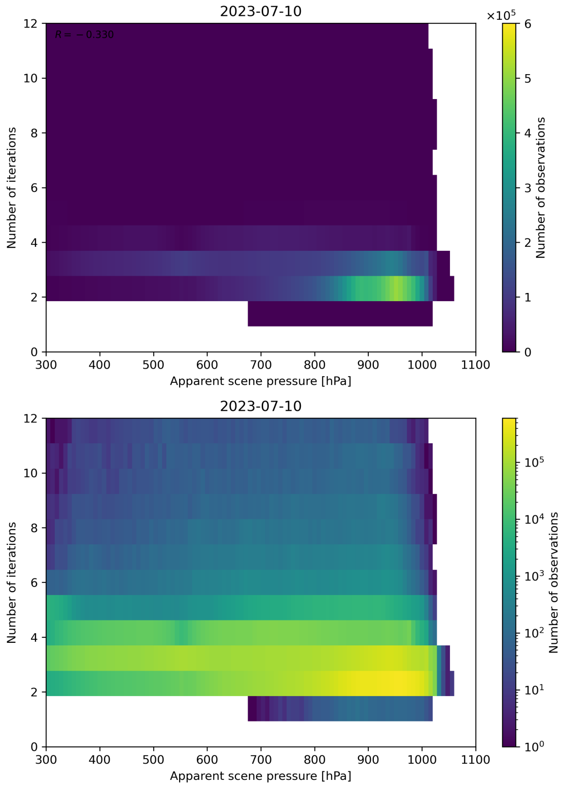
Figure 66: Scatter density plot of “Apparent scene pressure” against “Number of iterations” for 2023-07-09 to 2023-07-11.
