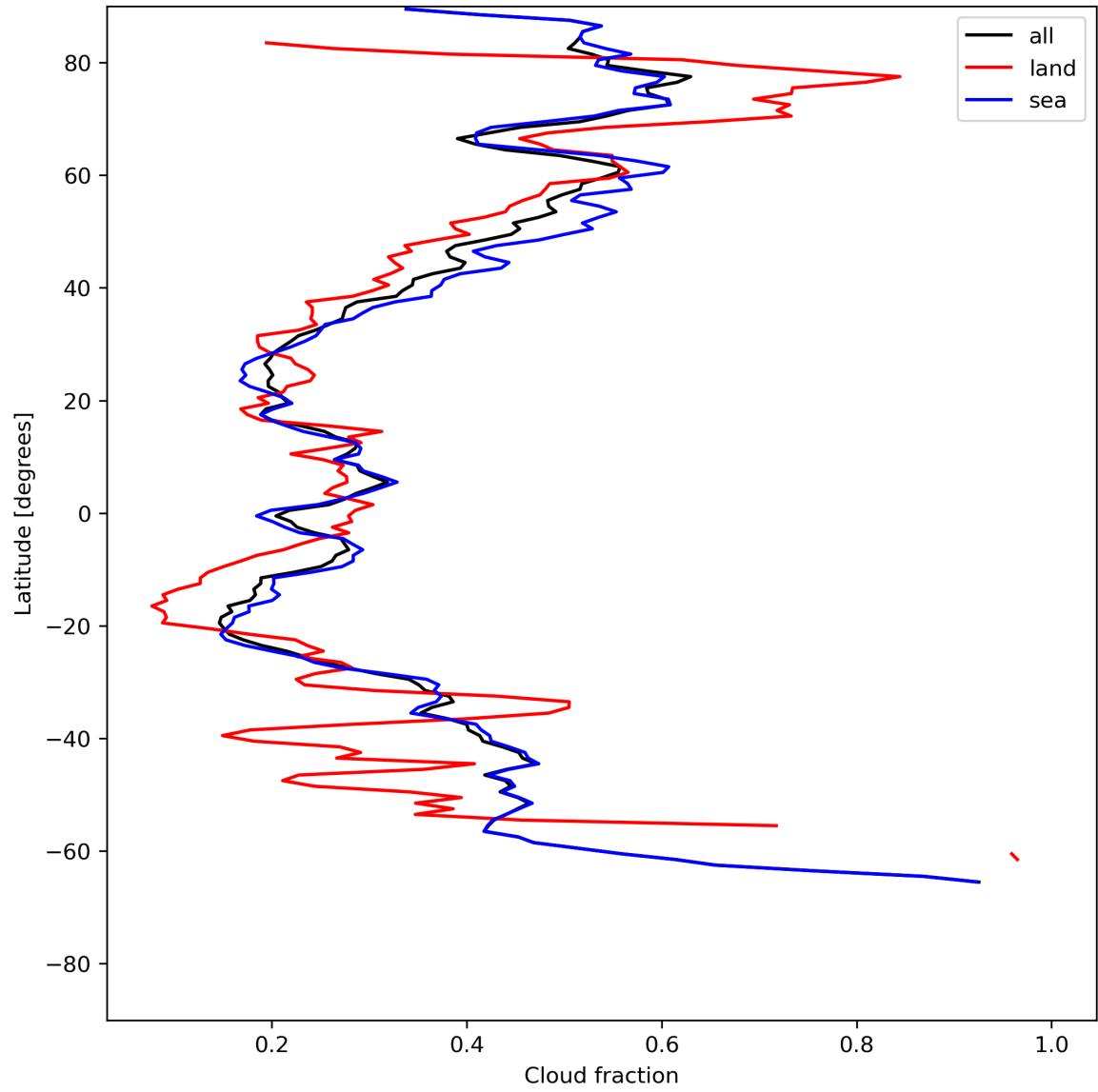
Figure 15: Zonal average of “Cloud fraction” for 2023-07-09 to 2023-07-11.
