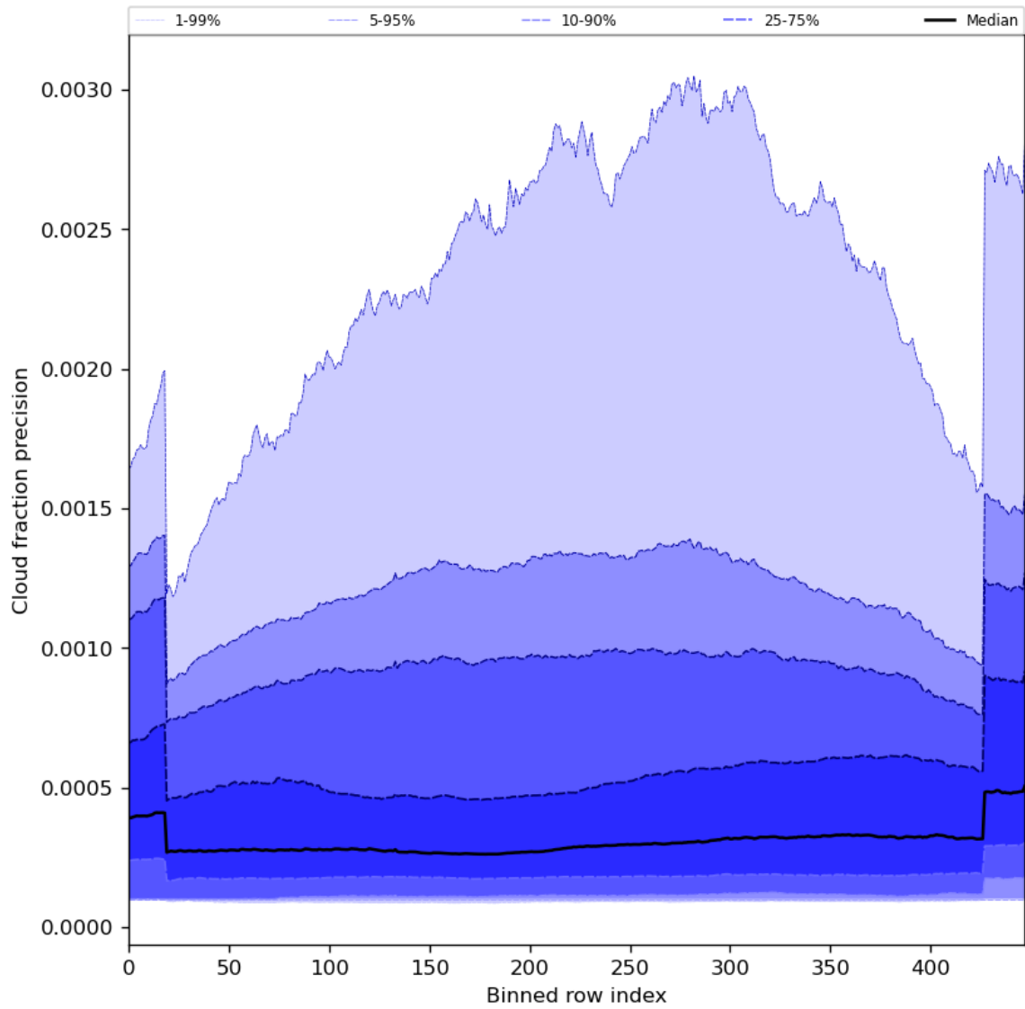
Figure 50: Along track statistics of “Cloud fraction precision” for 2023-07-09 to 2023-07-11
