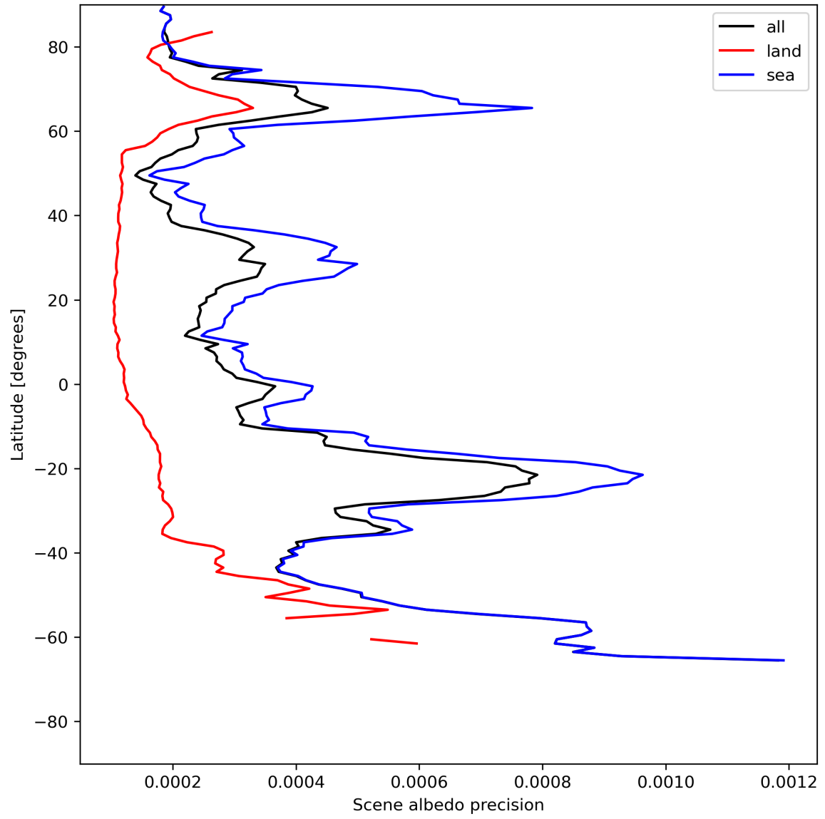
Figure 18: Zonal average of “Scene albedo precision” for 2023-07-09 to 2023-07-11.
