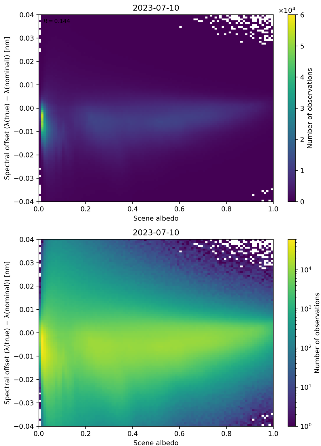
Figure 117: Scatter density plot of “Scene albedo” against “Spectral offset ( \lambda(\text{true}) - \lambda(\text{nominal}) )” for 2023-07-09 to 2023-07-11.
