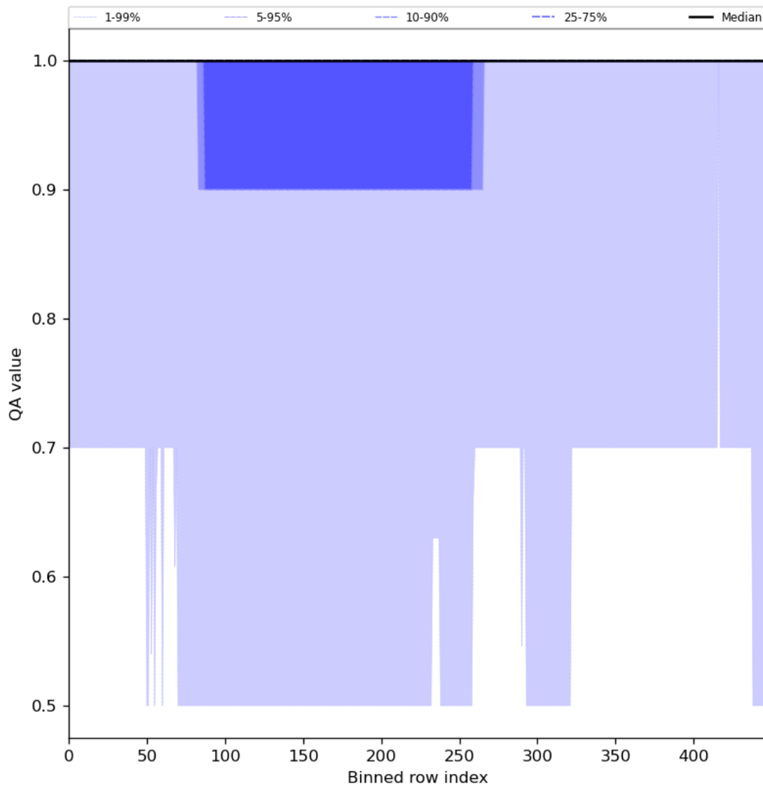
Figure 46: Along track statistics of "QA value" for 2023-07-09 to 2023-07-11
