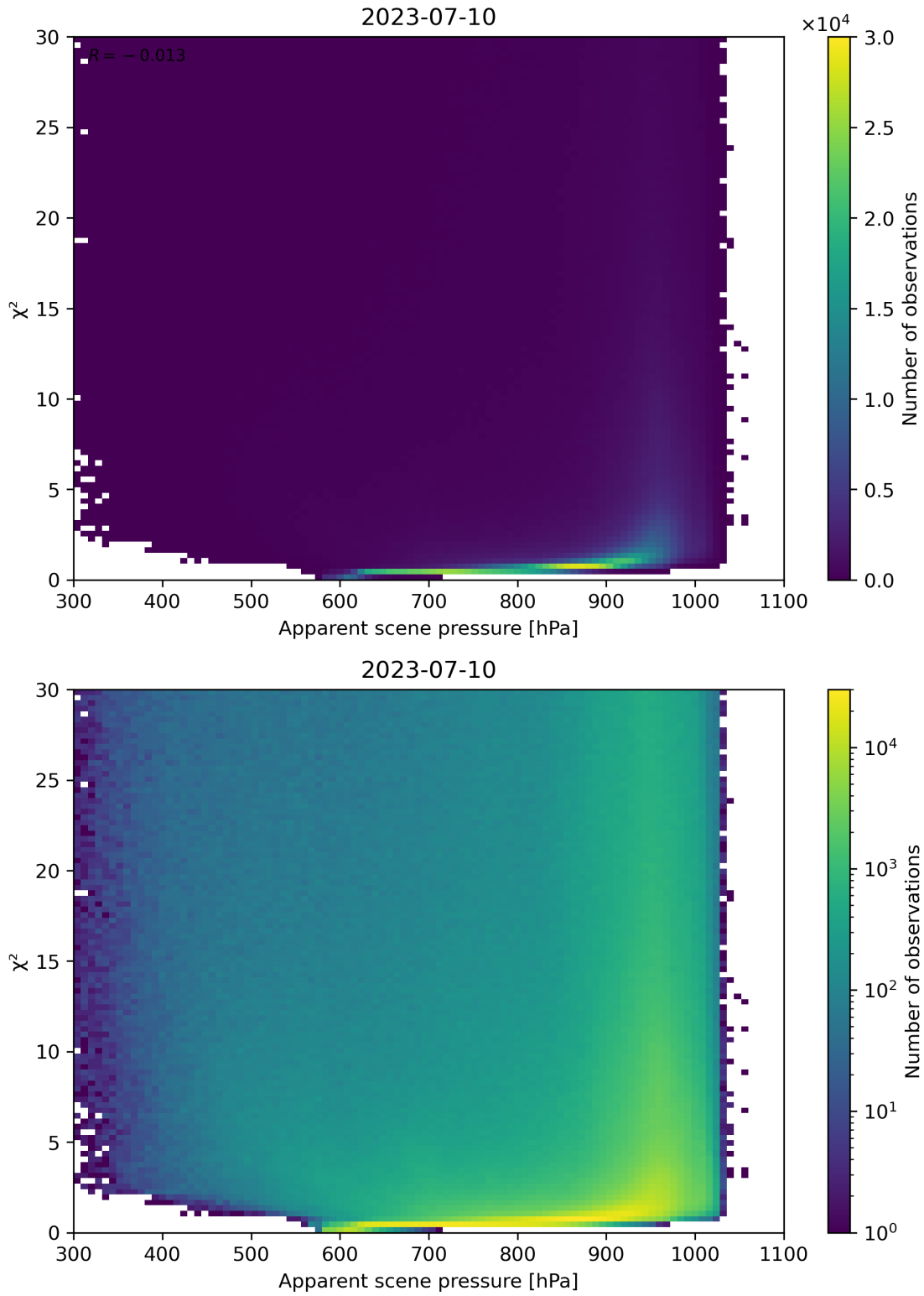
Figure 63: Scatter density plot of “Apparent scene pressure” against “ \chi^2 ” for 2023-07-09 to 2023-07-11.
