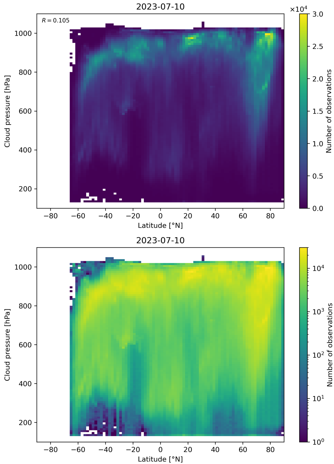
Figure 100: Scatter density plot of “Latitude” against “Cloud pressure” for 2023-07-09 to 2023-07-11.
