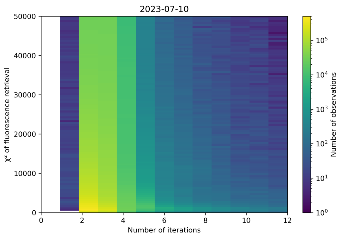
Figure 106: Scatter density plot of “Number of iterations” against “ \chi^2 of fluorescence retrieval” for 2023-07-09 to 2023-07-11.
