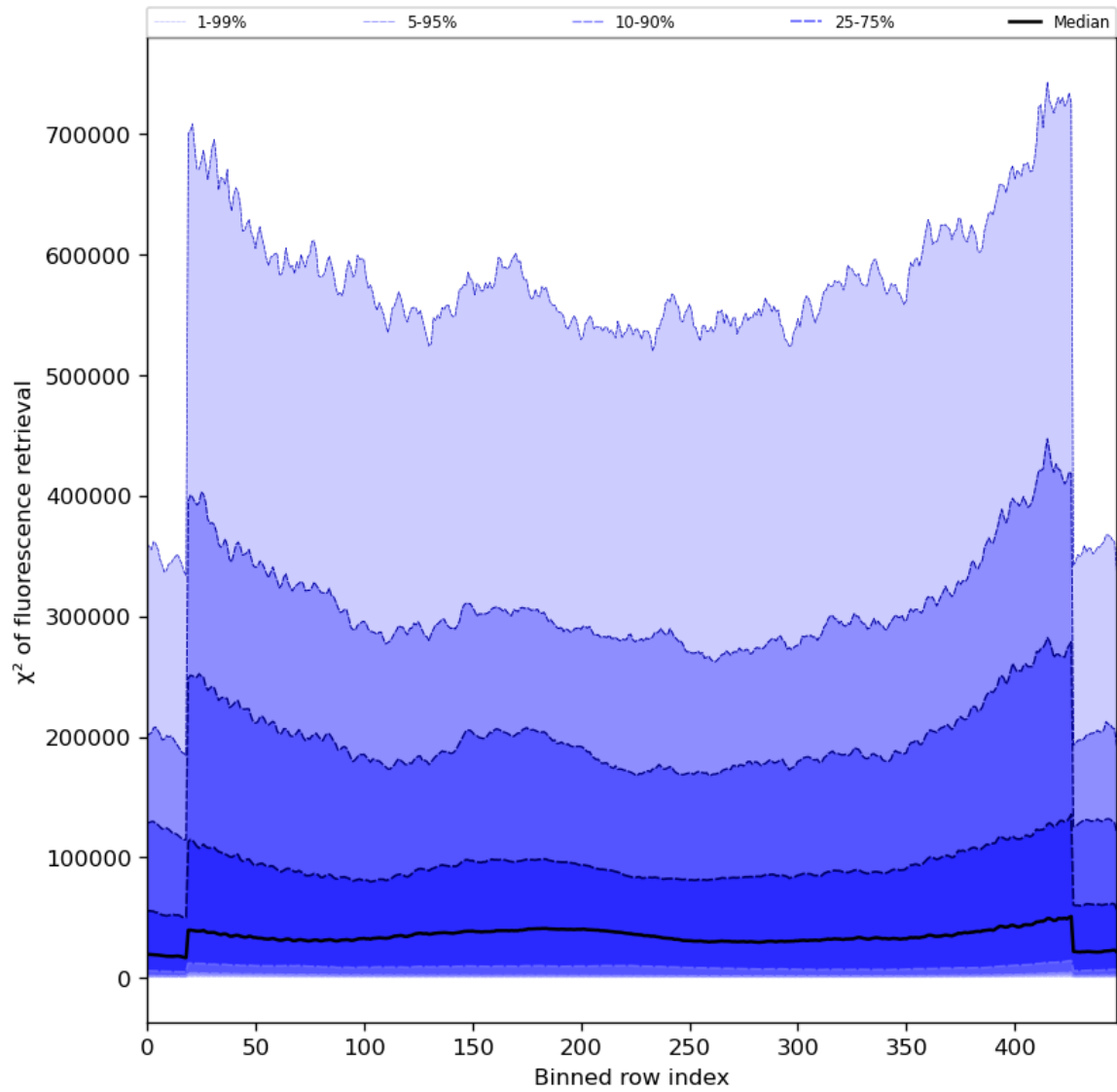
Figure 59: Along track statistics of “ \chi^2 of fluorescence retrieval” for 2023-07-09 to 2023-07-11
