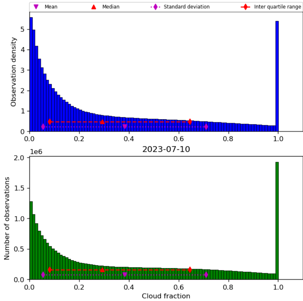
Figure 32: Histogram of “Cloud fraction” for 2023-07-09 to 2023-07-11
