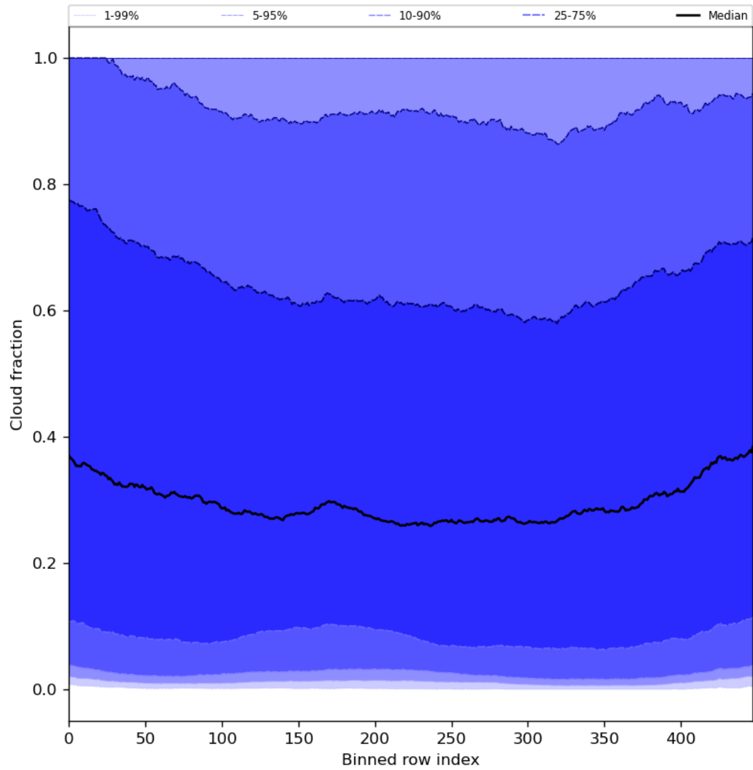
Figure 49: Along track statistics of “Cloud fraction” for 2023-07-09 to 2023-07-11
