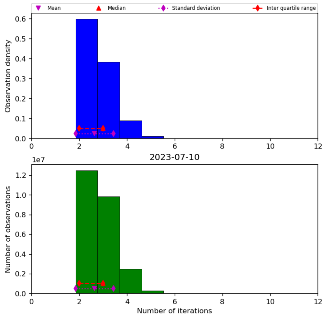
Figure 39: Histogram of “Number of iterations” for 2023-07-09 to 2023-07-11
