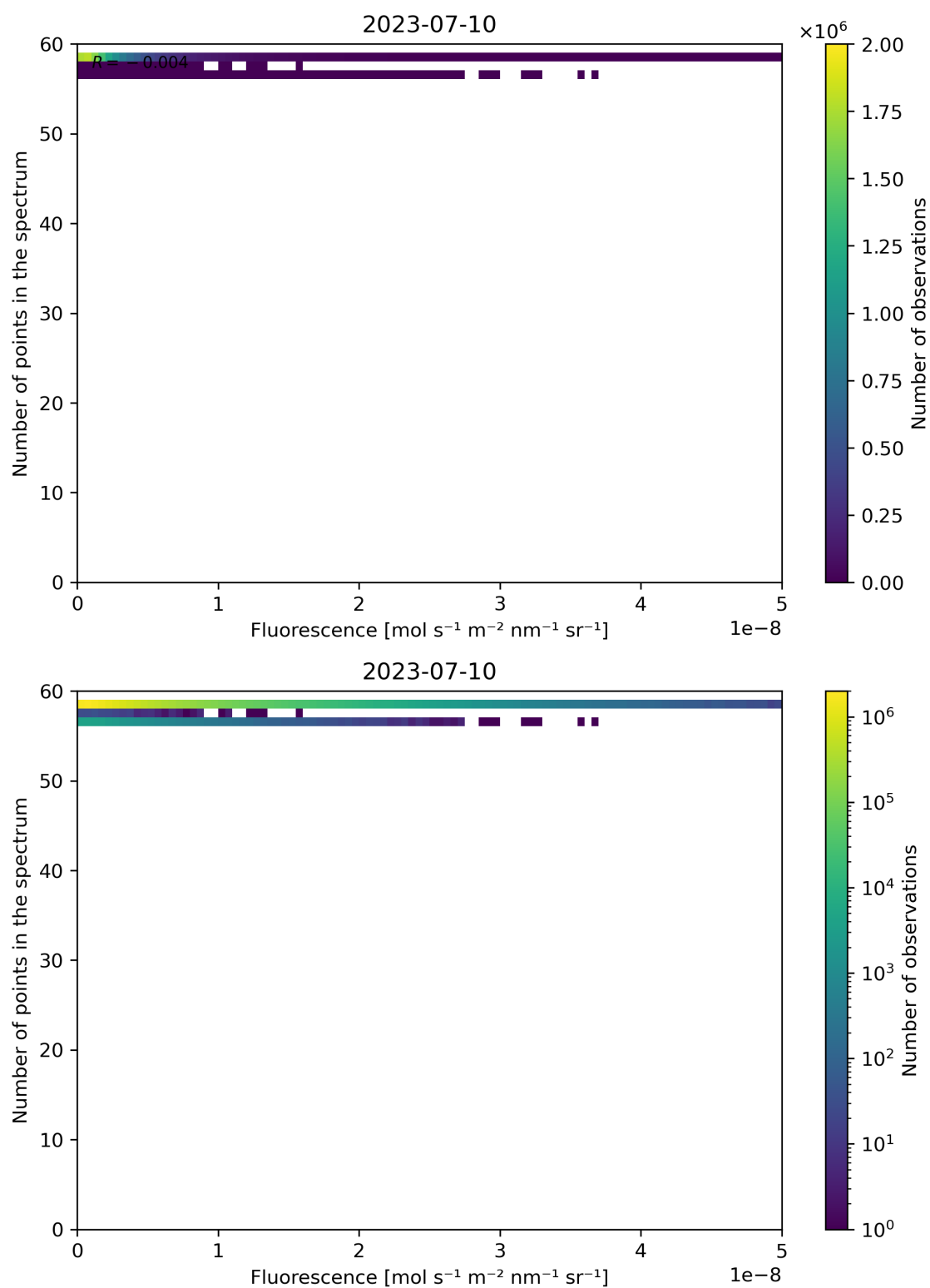
Figure 94: Scatter density plot of “Fluorescence” against “Number of points in the spectrum” for 2023-07-09 to 2023-07-11.
