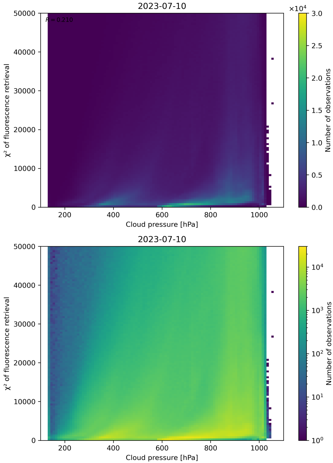
Figure 86: Scatter density plot of “Cloud pressure” against “ \chi^2 of fluorescence retrieval” for 2023-07-09 to 2023-07-11.
