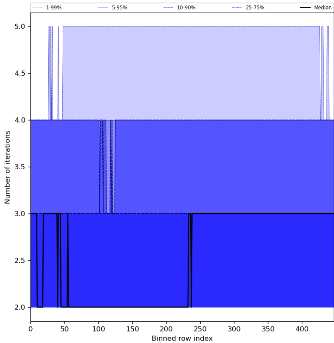
Figure 56: Along track statistics of “Number of iterations” for 2023-07-09 to 2023-07-11
