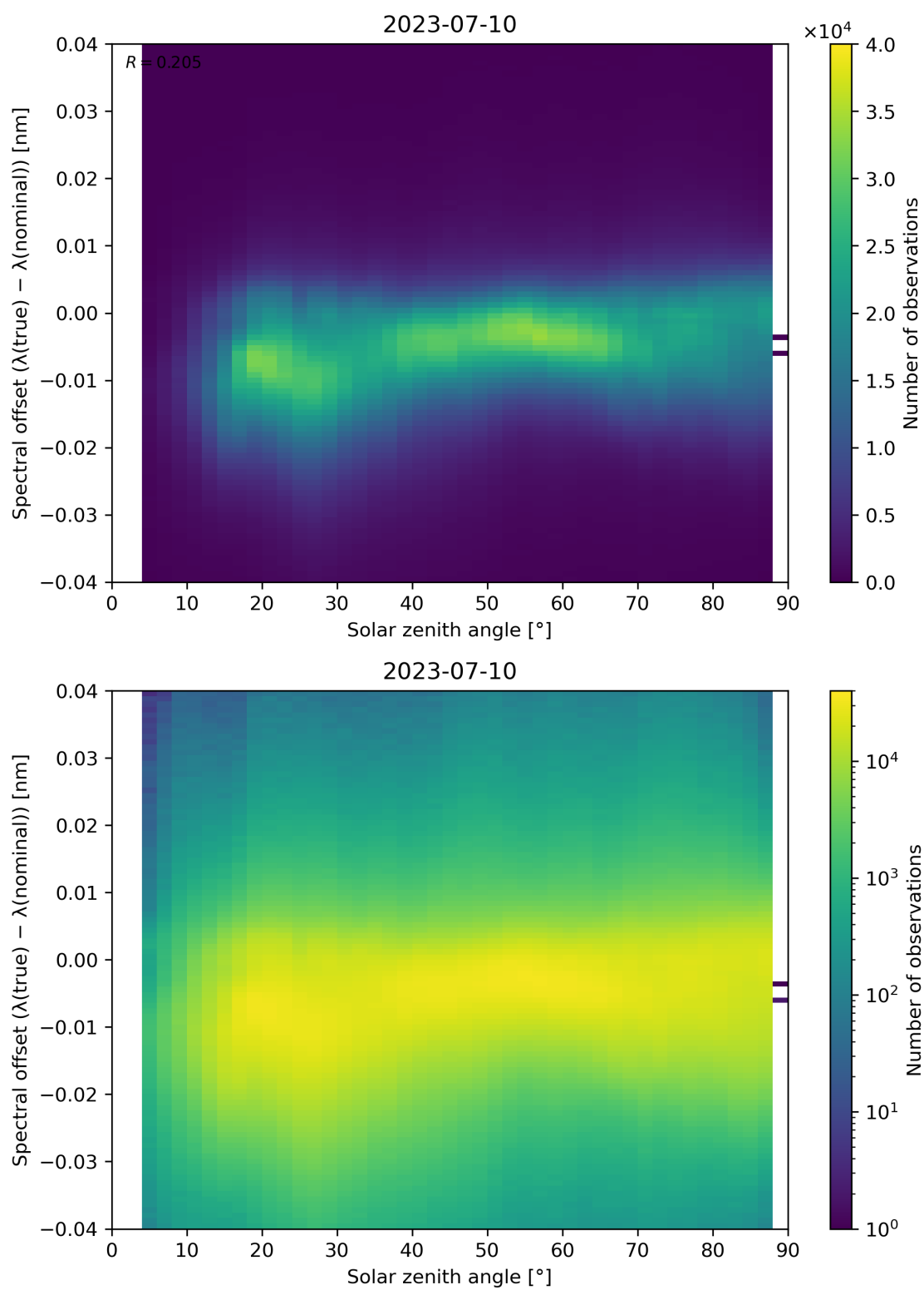
Figure 128: Scatter density plot of “Solar zenith angle” against “Spectral offset ( \lambda(\text{true}) - \lambda(\text{nominal}) )” for 2023-07-09 to 2023-07-11.
