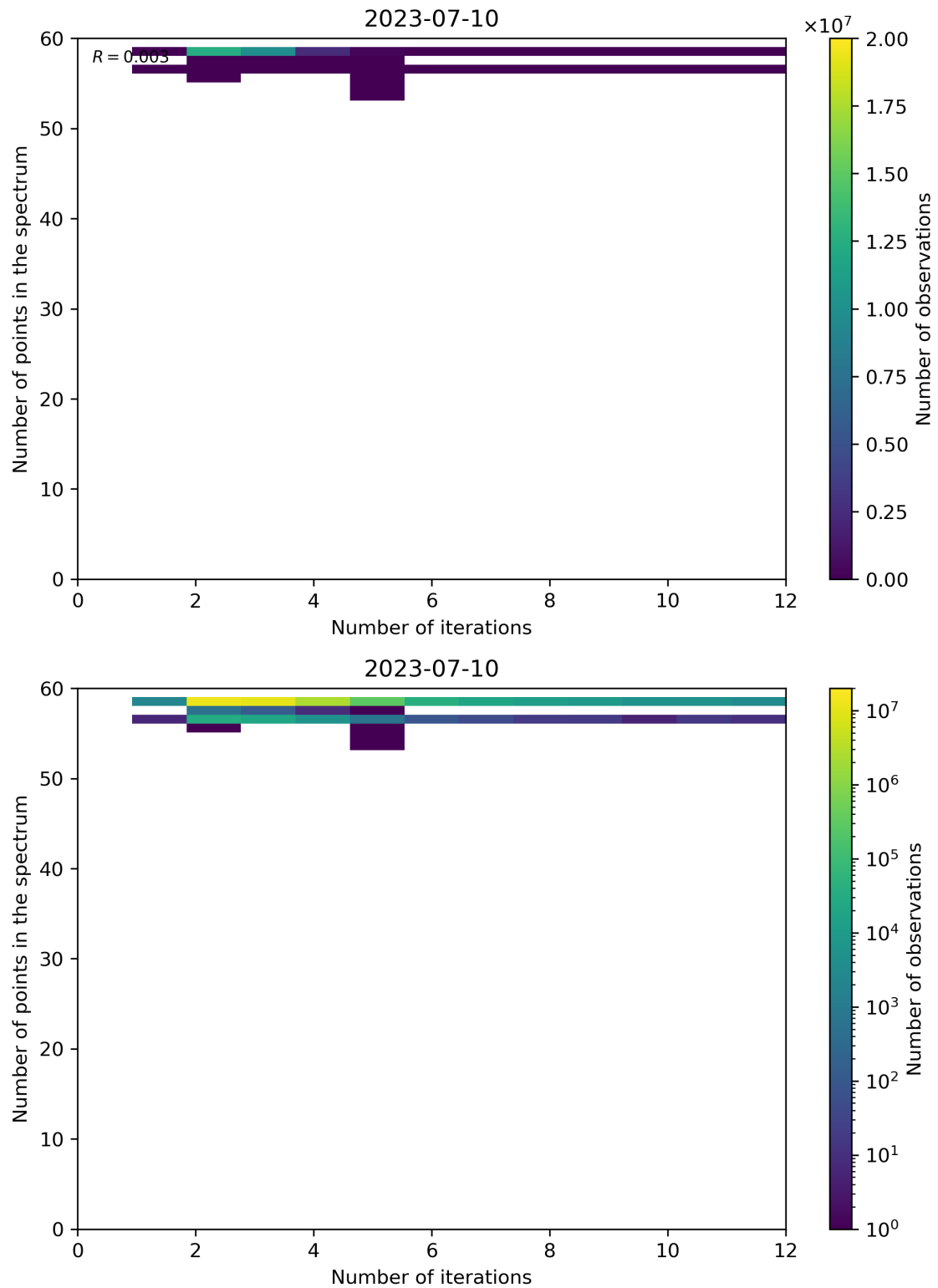
Figure 108: Scatter density plot of “Number of iterations” against “Number of points in the spectrum” for 2023-07-09 to 2023-07-11.
