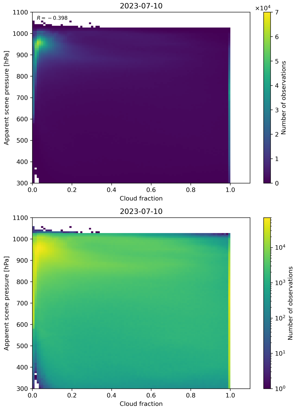
Figure 76: Scatter density plot of “Cloud fraction” against “Apparent scene pressure” for 2023-07-09 to 2023-07-11.
