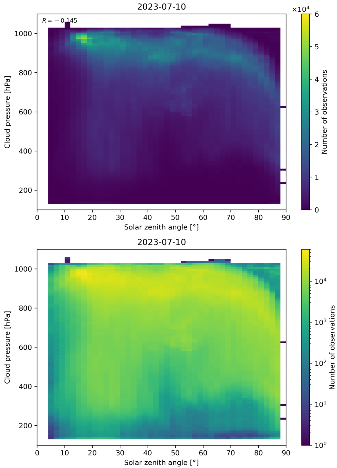
Figure 122: Scatter density plot of “Solar zenith angle” against “Cloud pressure” for 2023-07-09 to 2023-07-11.
