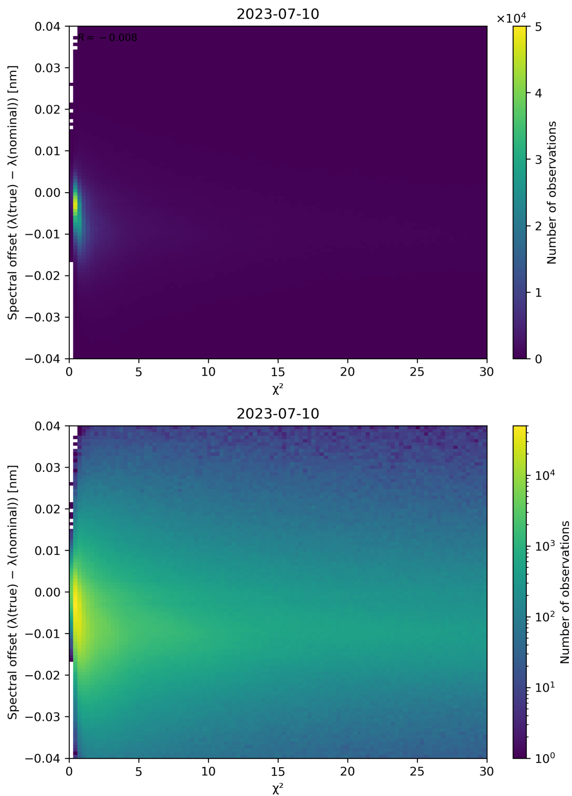
Figure 75: Scatter density plot of " \chi^2 " against "Spectral offset ( \lambda(\text{true}) - \lambda(\text{nominal}) )" for 2023-07-09 to 2023-07-11.
