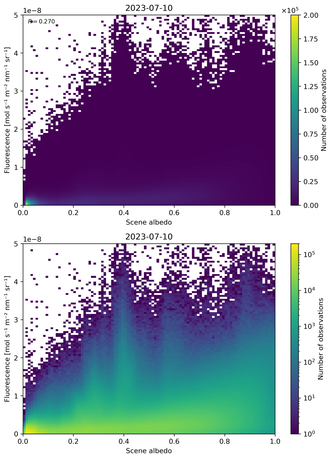
Figure 114: Scatter density plot of “Scene albedo” against “Fluorescence” for 2023-07-09 to 2023-07-11.
