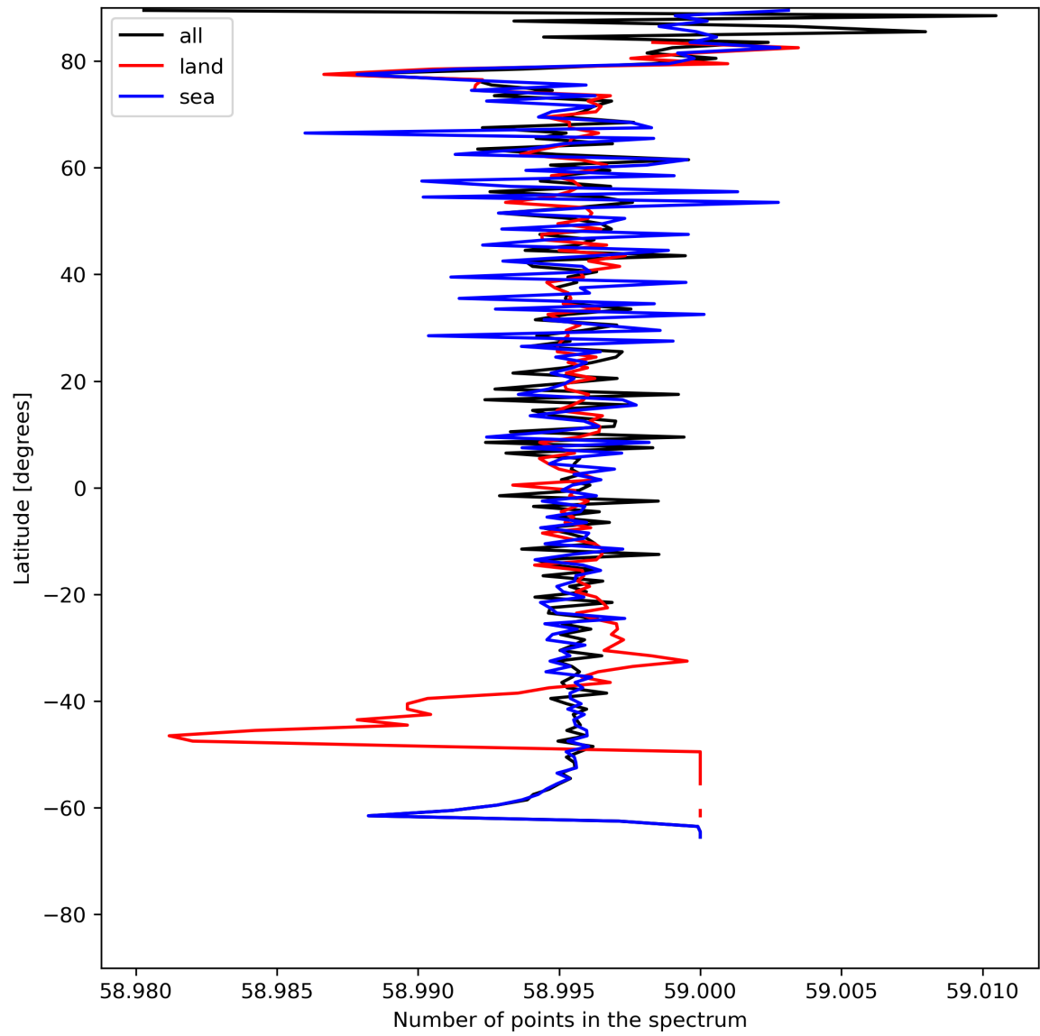
Figure 27: Zonal average of “Number of points in the spectrum” for 2023-07-09 to 2023-07-11.
