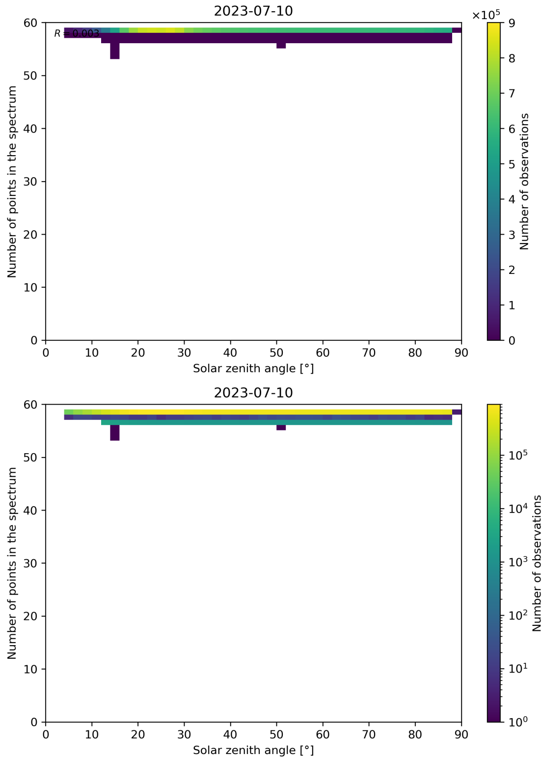
Figure 126: Scatter density plot of “Solar zenith angle” against “Number of points in the spectrum” for 2023-07-09 to 2023-07-11.
