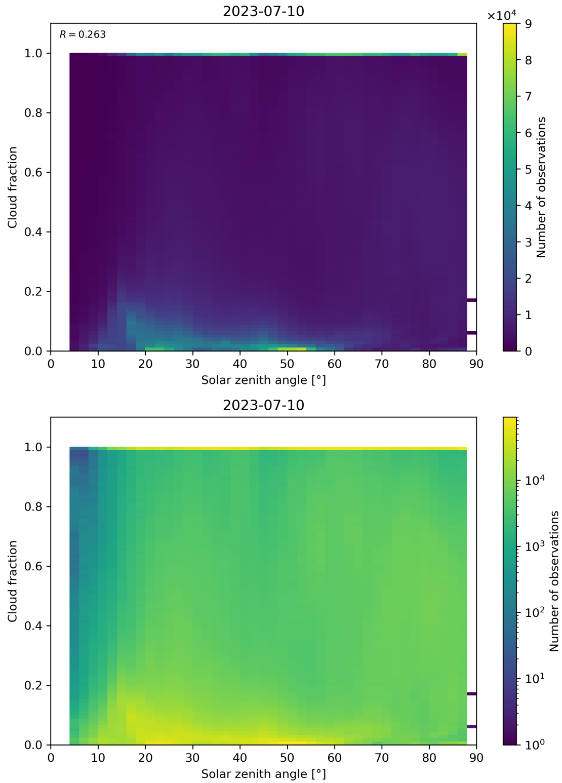
Figure 121: Scatter density plot of “Solar zenith angle” against “Cloud fraction” for 2023-07-09 to 2023-07-11.
