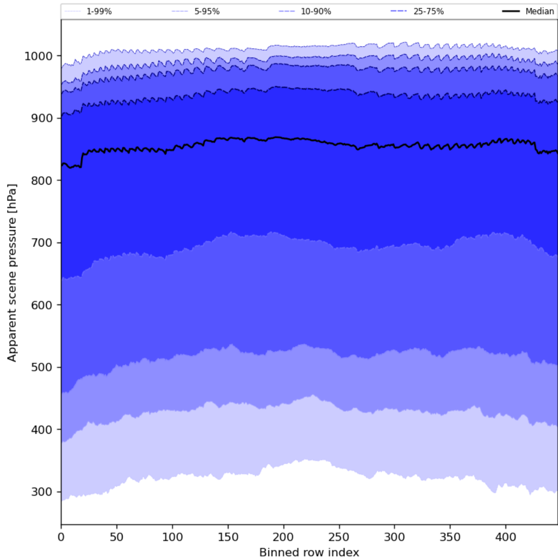
Figure 53: Along track statistics of “Apparent scene pressure” for 2023-07-09 to 2023-07-11
