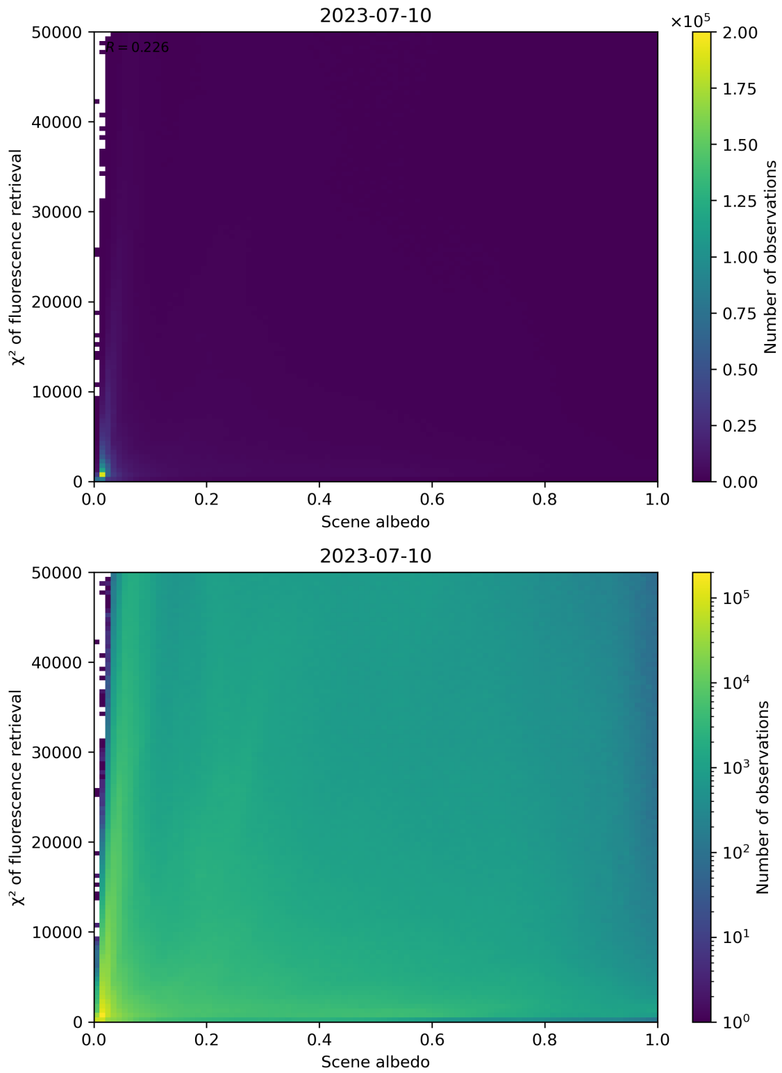
Figure 113: Scatter density plot of “Scene albedo” against “ \chi^2 of fluorescence retrieval” for 2023-07-09 to 2023-07-11.
