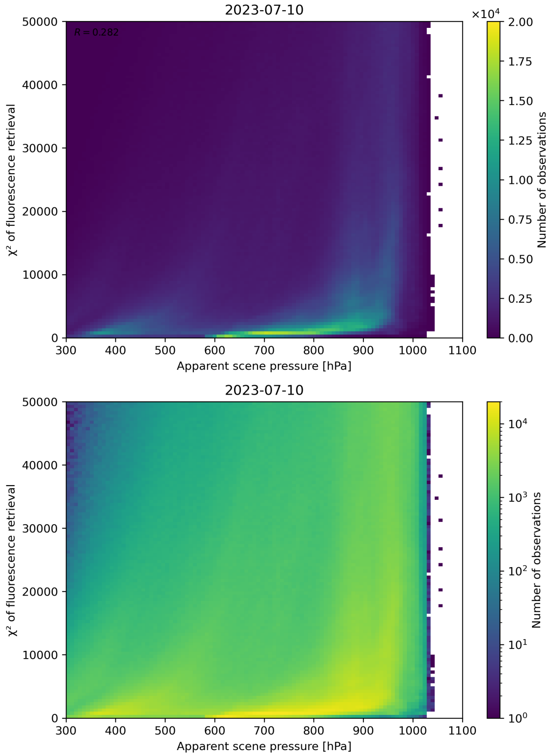
Figure 64: Scatter density plot of “Apparent scene pressure” against “ \chi^2 of fluorescence retrieval” for 2023-07-09 to 2023-07-11.
