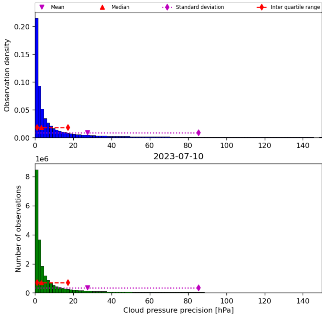
Figure 31: Histogram of “Cloud pressure precision” for 2023-07-09 to 2023-07-11
