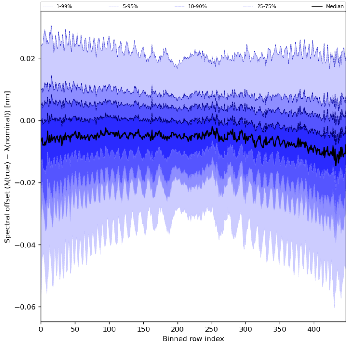
Figure 62: Along track statistics of “Spectral offset ( \lambda(\text{true}) - \lambda(\text{nominal}) )” for 2023-07-09 to 2023-07-11
