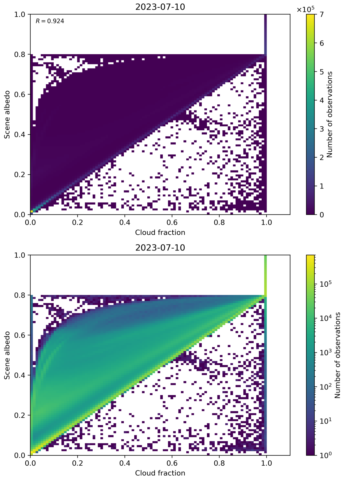
Figure 82: Scatter density plot of “Cloud fraction” against “Scene albedo” for 2023-07-09 to 2023-07-11.
