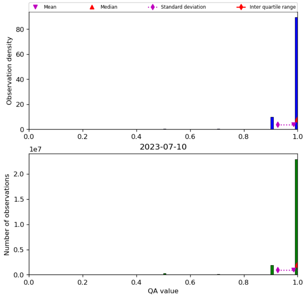
Figure 29: Histogram of “QA value” for 2023-07-09 to 2023-07-11
