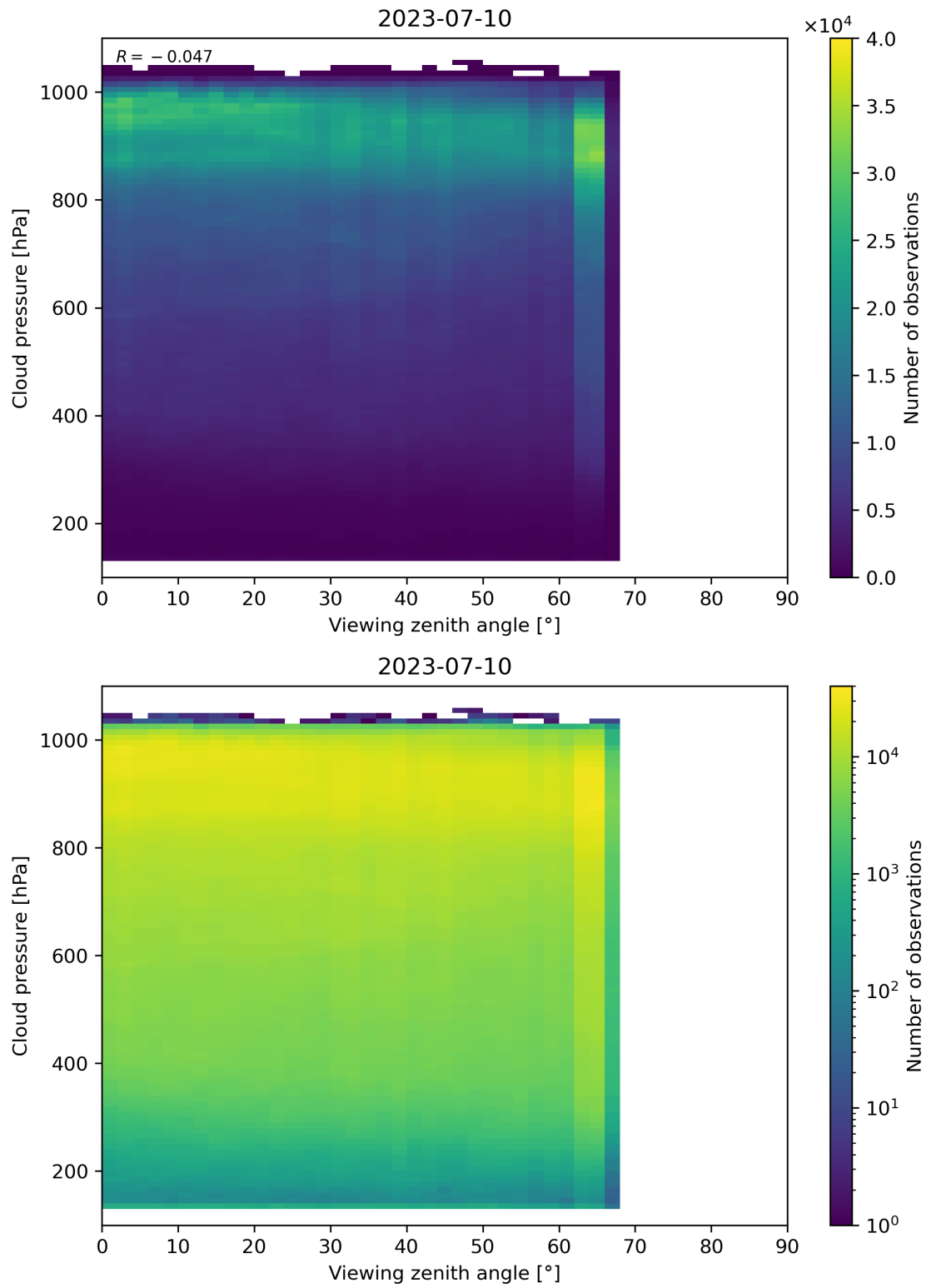
Figure 133: Scatter density plot of “Viewing zenith angle” against “Cloud pressure” for 2023-07-09 to 2023-07-11.
