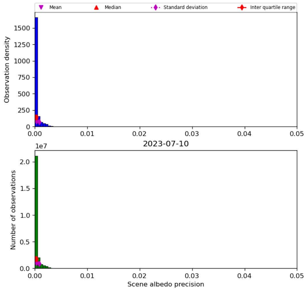
Figure 35: Histogram of “Scene albedo precision” for 2023-07-09 to 2023-07-11
