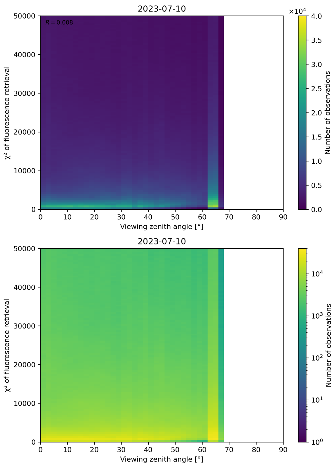
Figure 131: Scatter density plot of “Viewing zenith angle” against “ \chi^2 of fluorescence retrieval” for 2023-07-09 to 2023-07-11.
