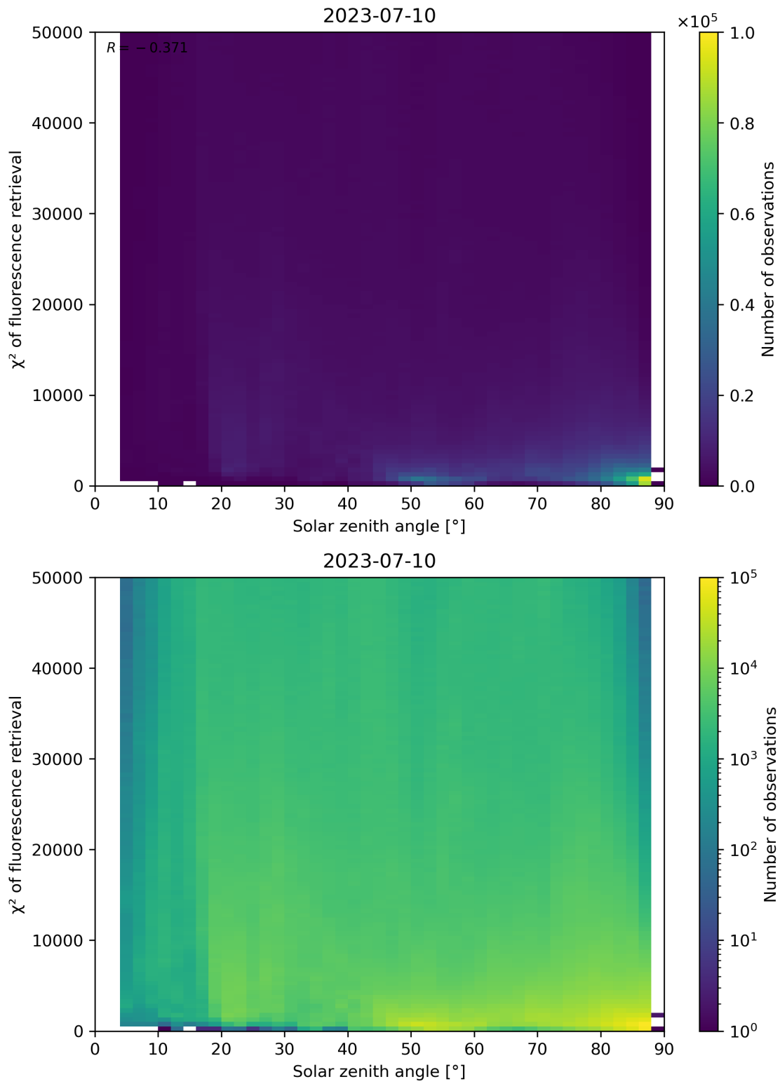
Figure 120: Scatter density plot of “Solar zenith angle” against “ \chi^2 of fluorescence retrieval” for 2023-07-09 to 2023-07-11.
