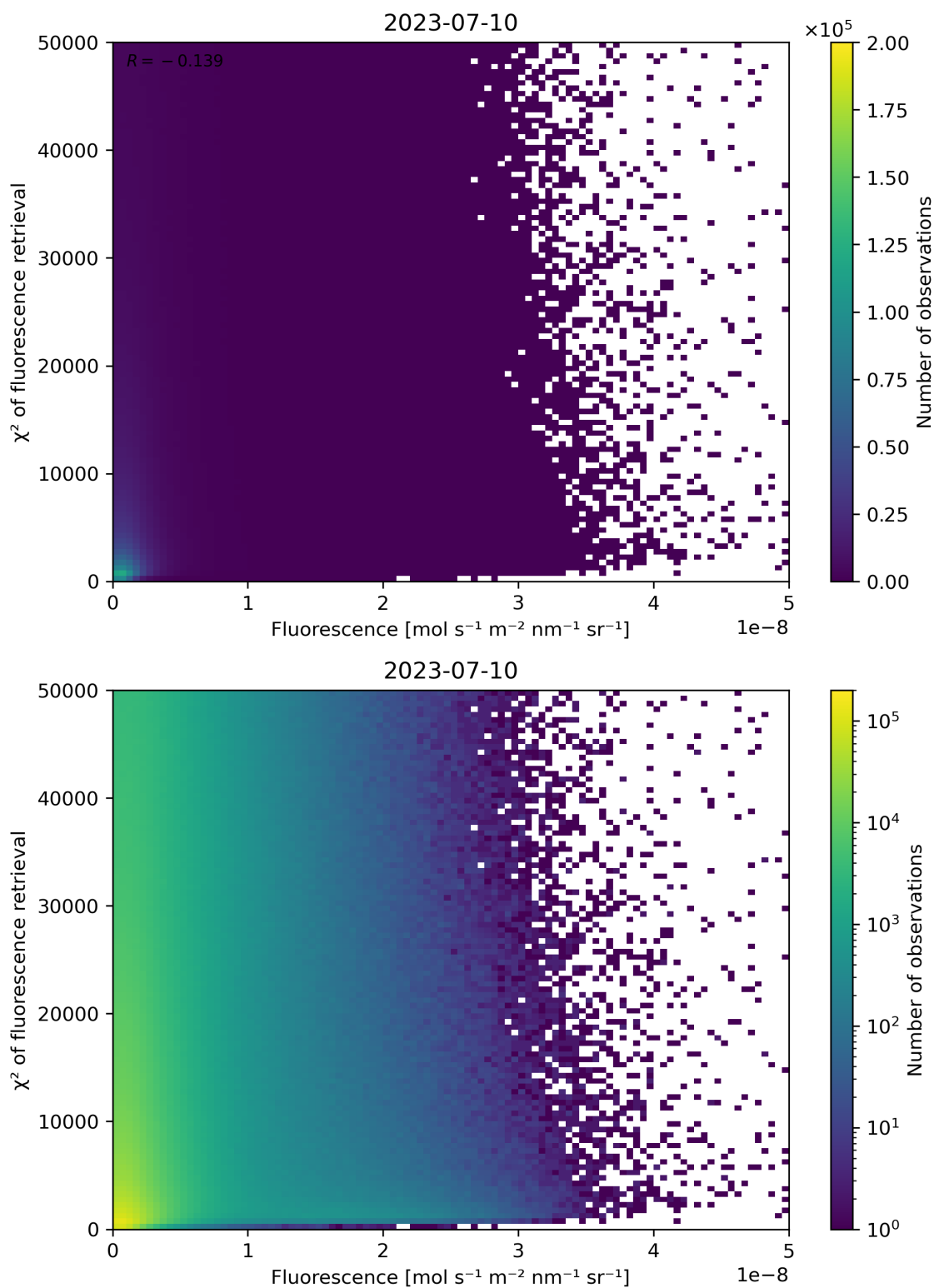
Figure 93: Scatter density plot of “Fluorescence” against “ \chi^2 of fluorescence retrieval” for 2023-07-09 to 2023-07-11.
