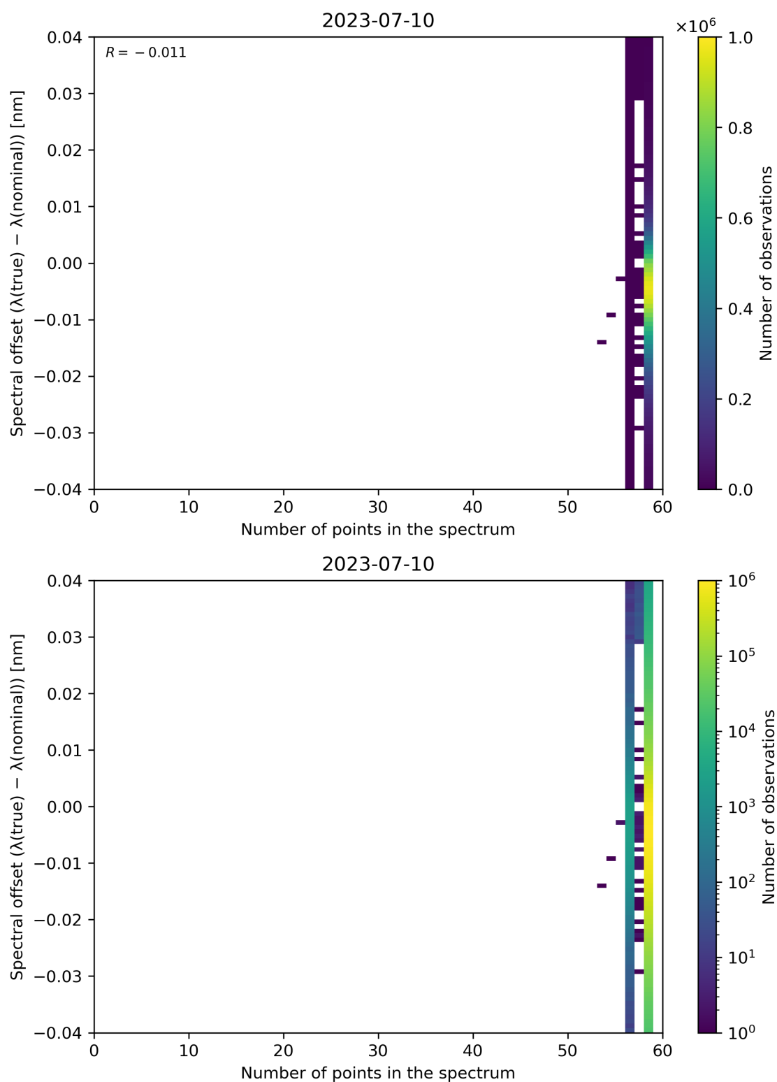
Figure 110: Scatter density plot of “Number of points in the spectrum” against “Spectral offset ( \lambda(\text{true}) - \lambda(\text{nominal}) )” for 2023-07-09 to 2023-07-11.
