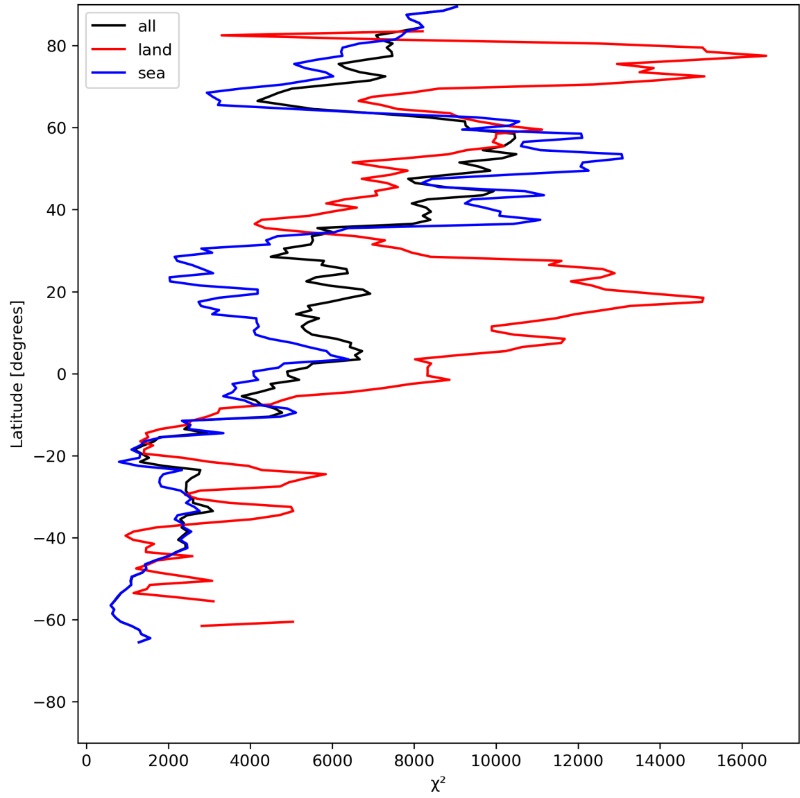
Figure 21: Zonal average of “ \chi^2 ” for 2023-07-09 to 2023-07-11.
