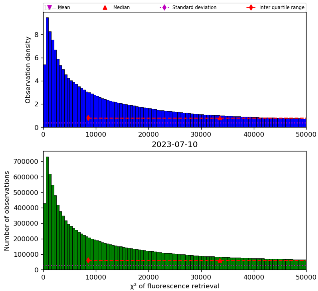
Figure 42: Histogram of “ \chi^2 of fluorescence retrieval” for 2023-07-09 to 2023-07-11
