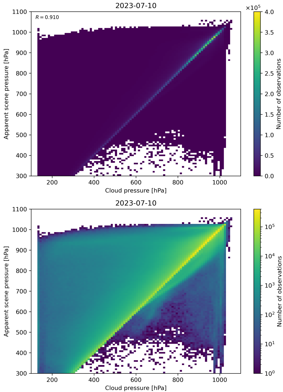
Figure 84: Scatter density plot of “Cloud pressure” against “Apparent scene pressure” for 2023-07-09 to 2023-07-11.
