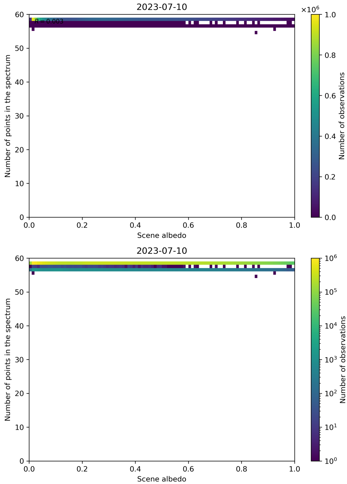
Figure 116: Scatter density plot of “Scene albedo” against “Number of points in the spectrum” for 2023-07-09 to 2023-07-11.
