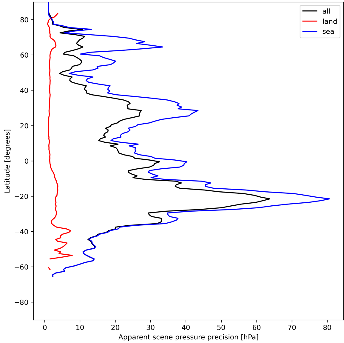
Figure 20: Zonal average of “Apparent scene pressure precision” for 2023-07-09 to 2023-07-11.
