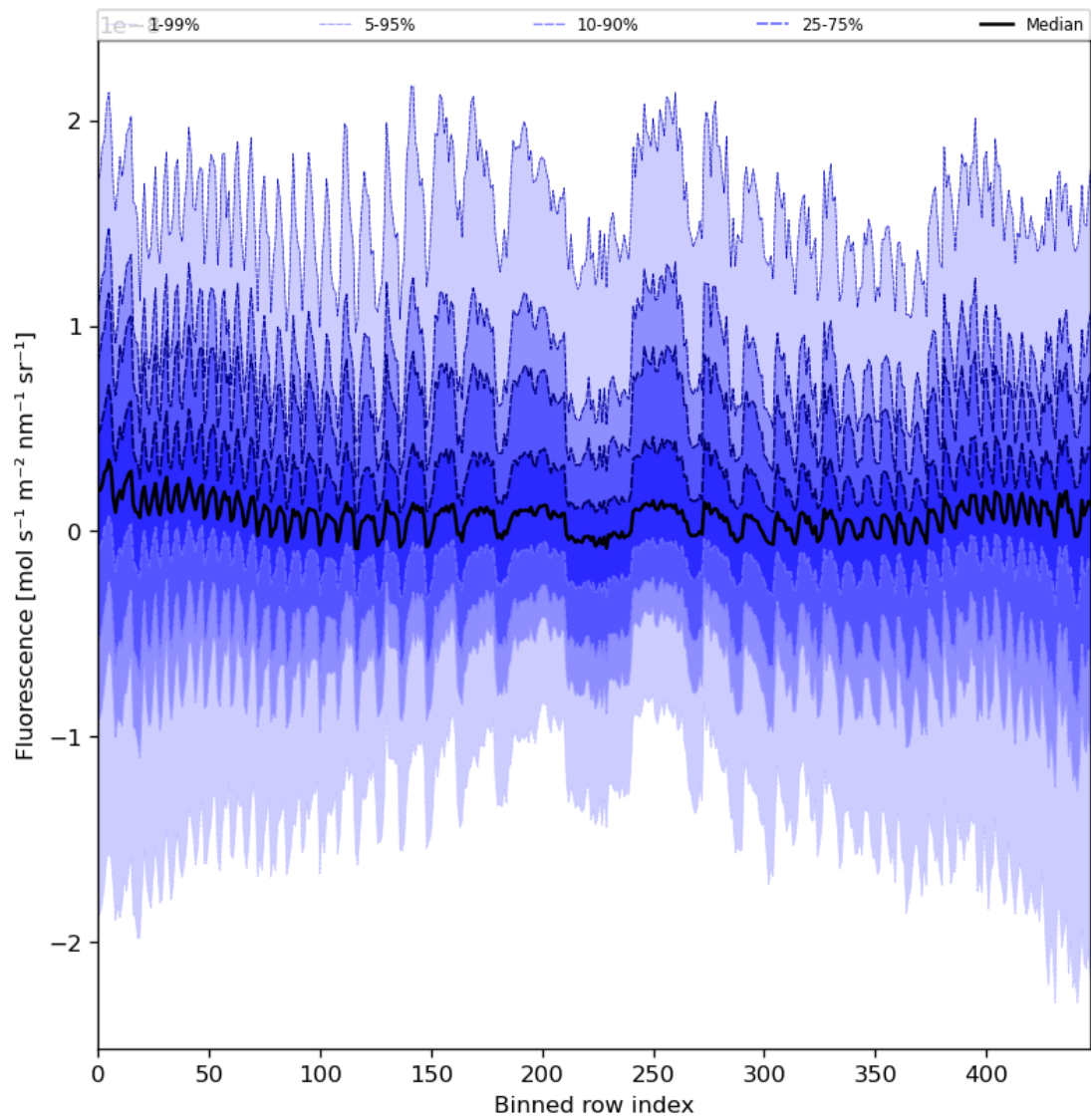
Figure 57: Along track statistics of “Fluorescence” for 2023-07-09 to 2023-07-11
