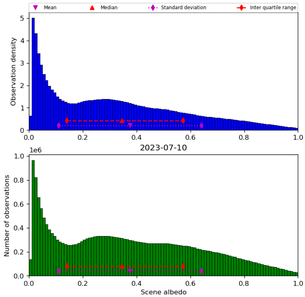
Figure 34: Histogram of “Scene albedo” for 2023-07-09 to 2023-07-11
