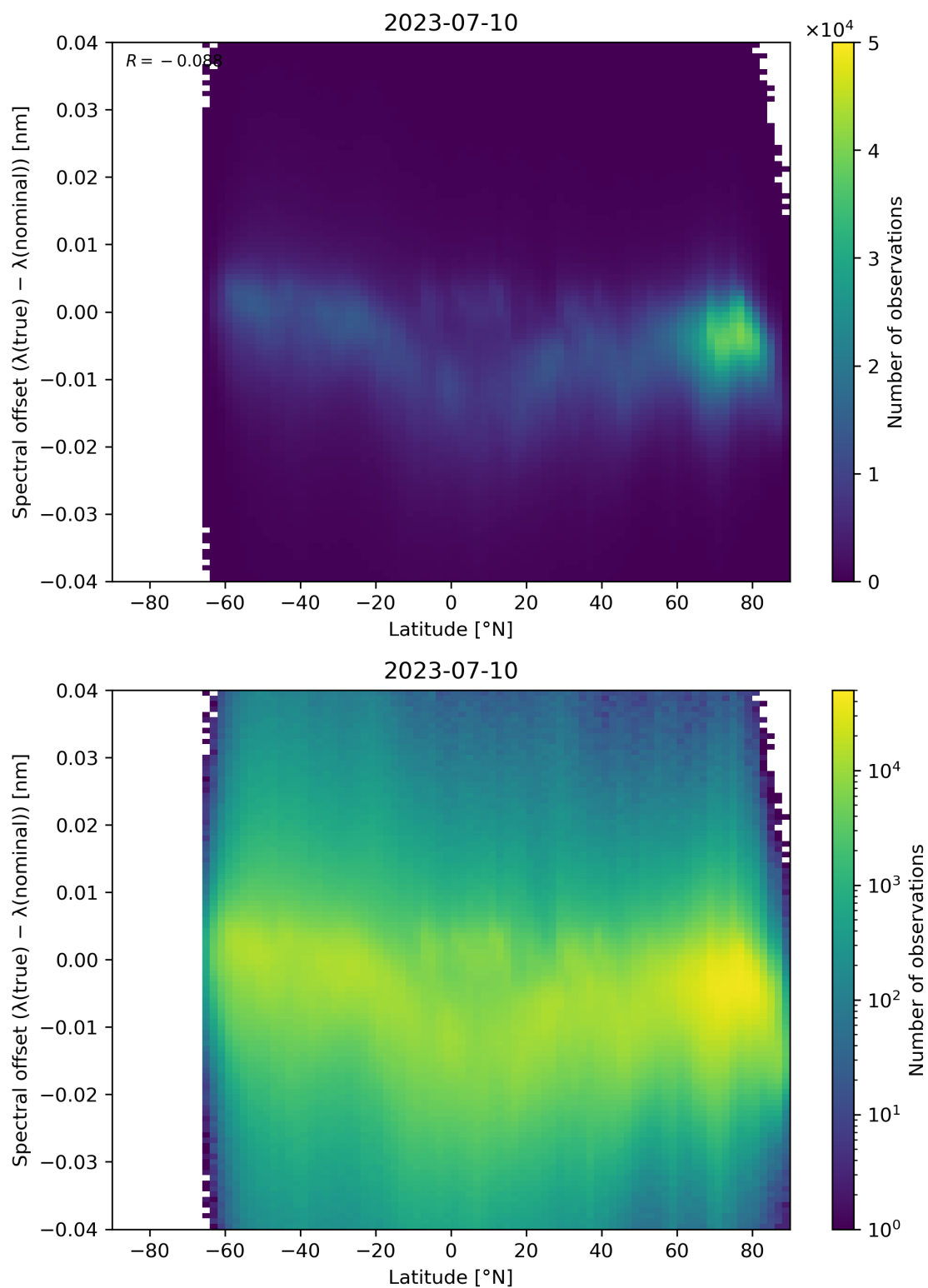
Figure 105: Scatter density plot of “Latitude” against “Spectral offset ( \lambda(\text{true}) - \lambda(\text{nominal}) )” for 2023-07-09 to 2023-07-11.
