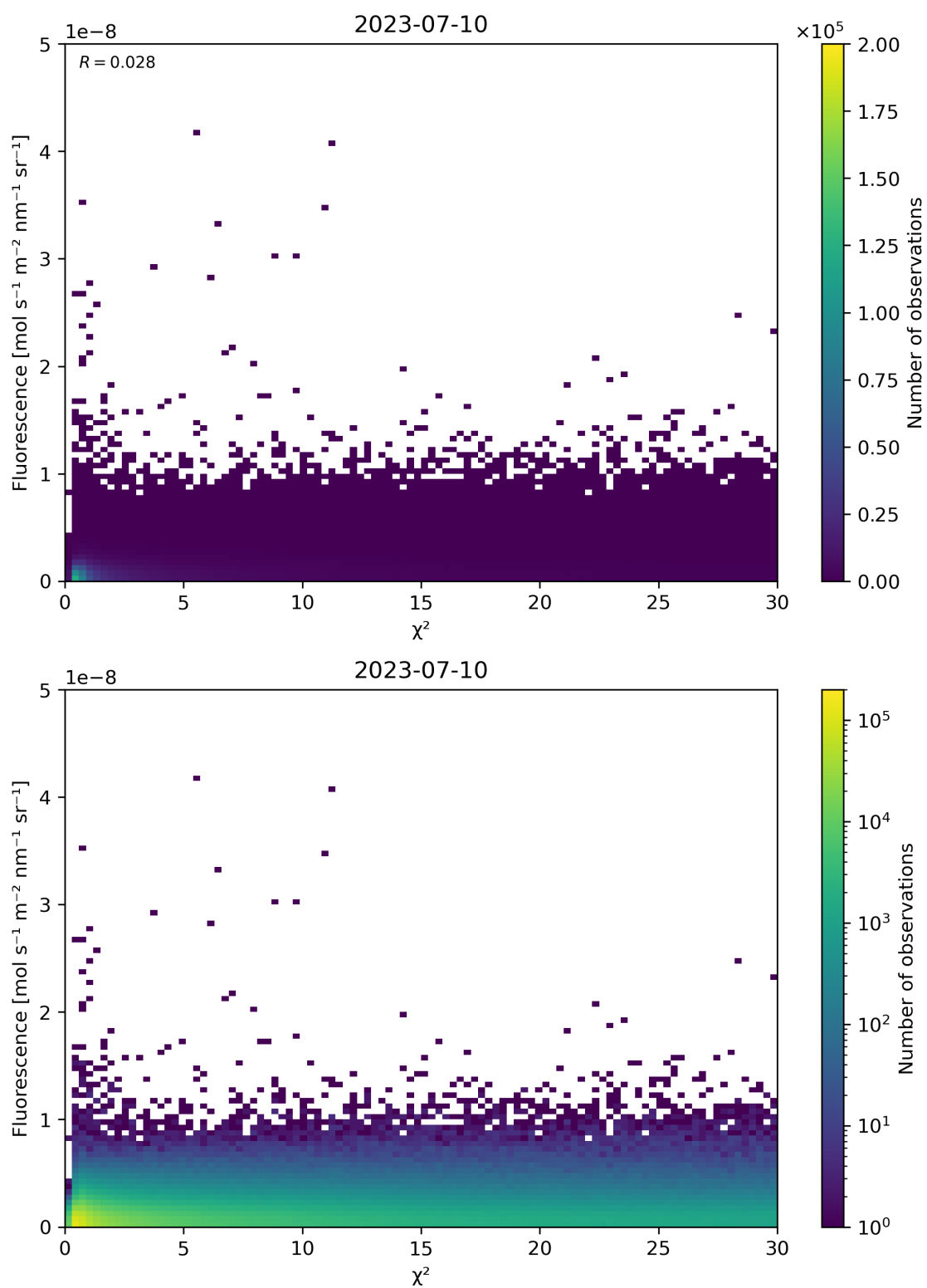
Figure 70: Scatter density plot of “ \chi^2 ” against “Fluorescence” for 2023-07-09 to 2023-07-11.
