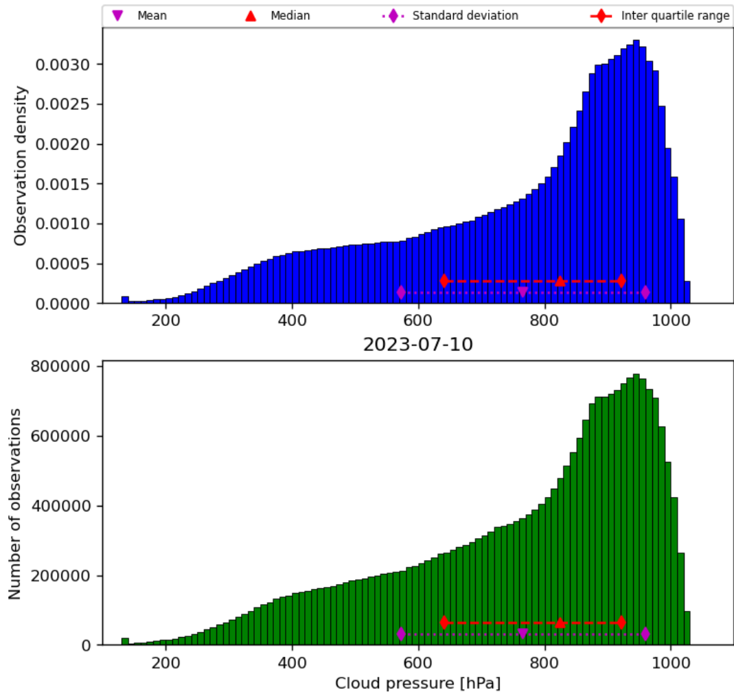
Figure 30: Histogram of “Cloud pressure” for 2023-07-09 to 2023-07-11
