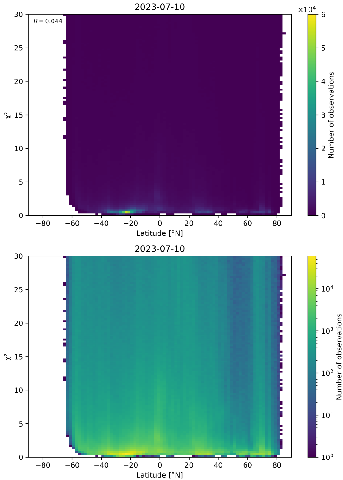
Figure 97: Scatter density plot of “Latitude” against “ \chi^2 ” for 2023-07-09 to 2023-07-11.
