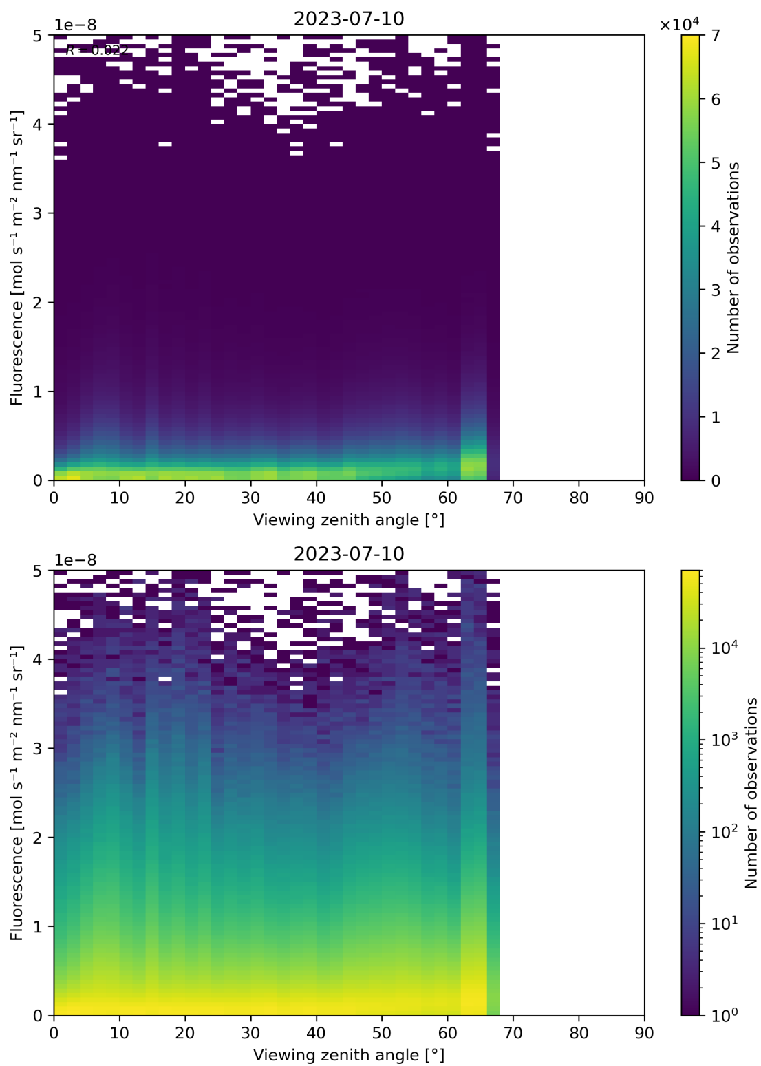
Figure 134: Scatter density plot of “Viewing zenith angle” against “Fluorescence” for 2023-07-09 to 2023-07-11.
