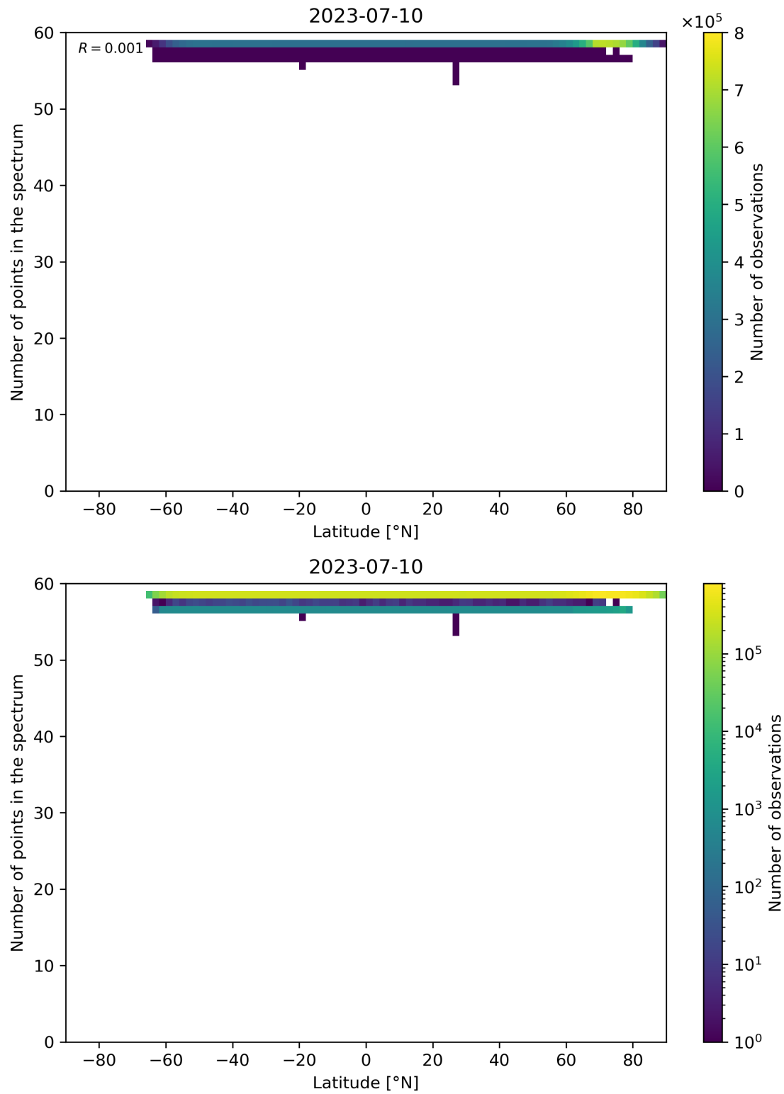
Figure 103: Scatter density plot of “Latitude” against “Number of points in the spectrum” for 2023-07-09 to 2023-07-11.
