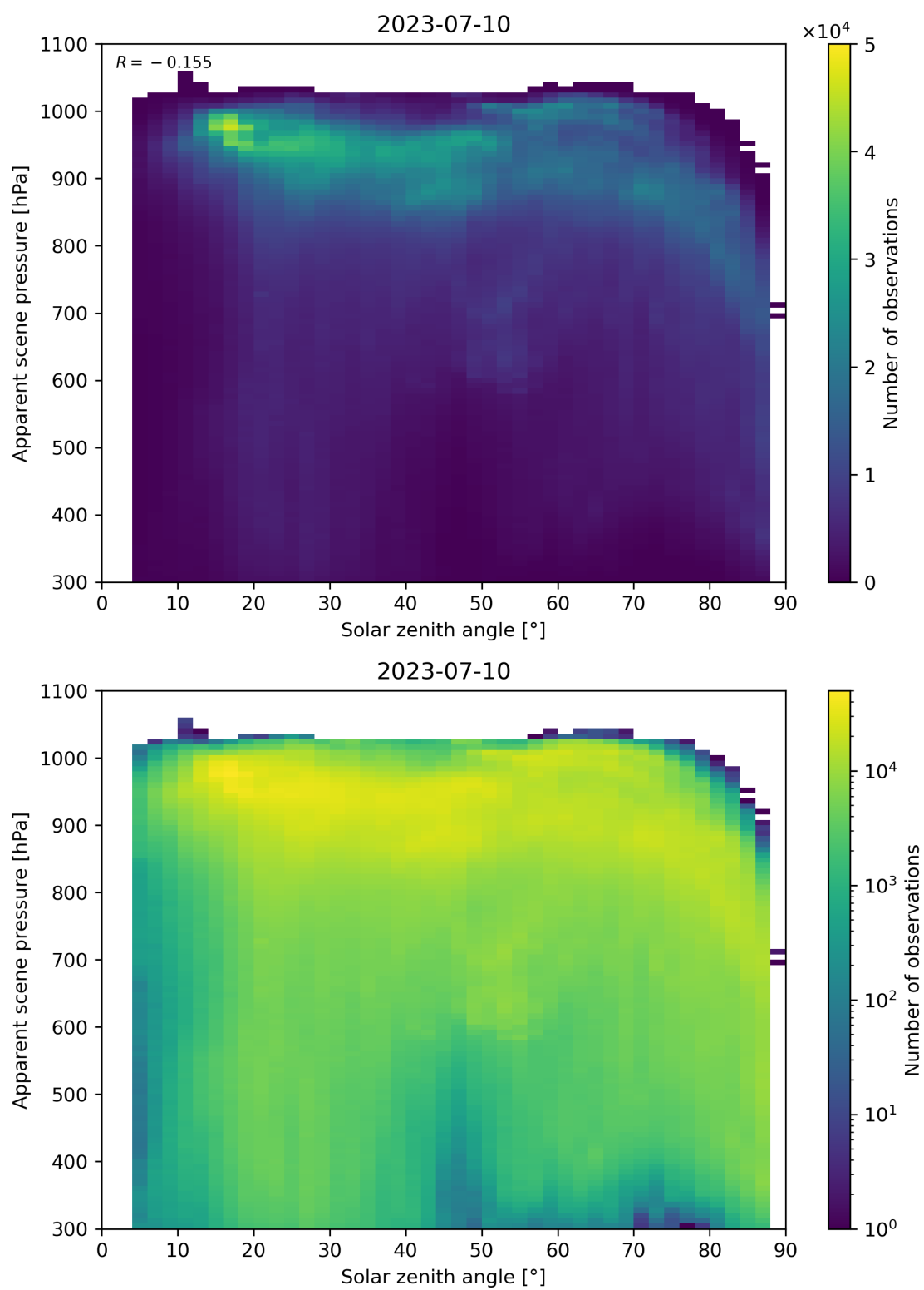
Figure 118: Scatter density plot of “Solar zenith angle” against “Apparent scene pressure” for 2023-07-09 to 2023-07-11.
