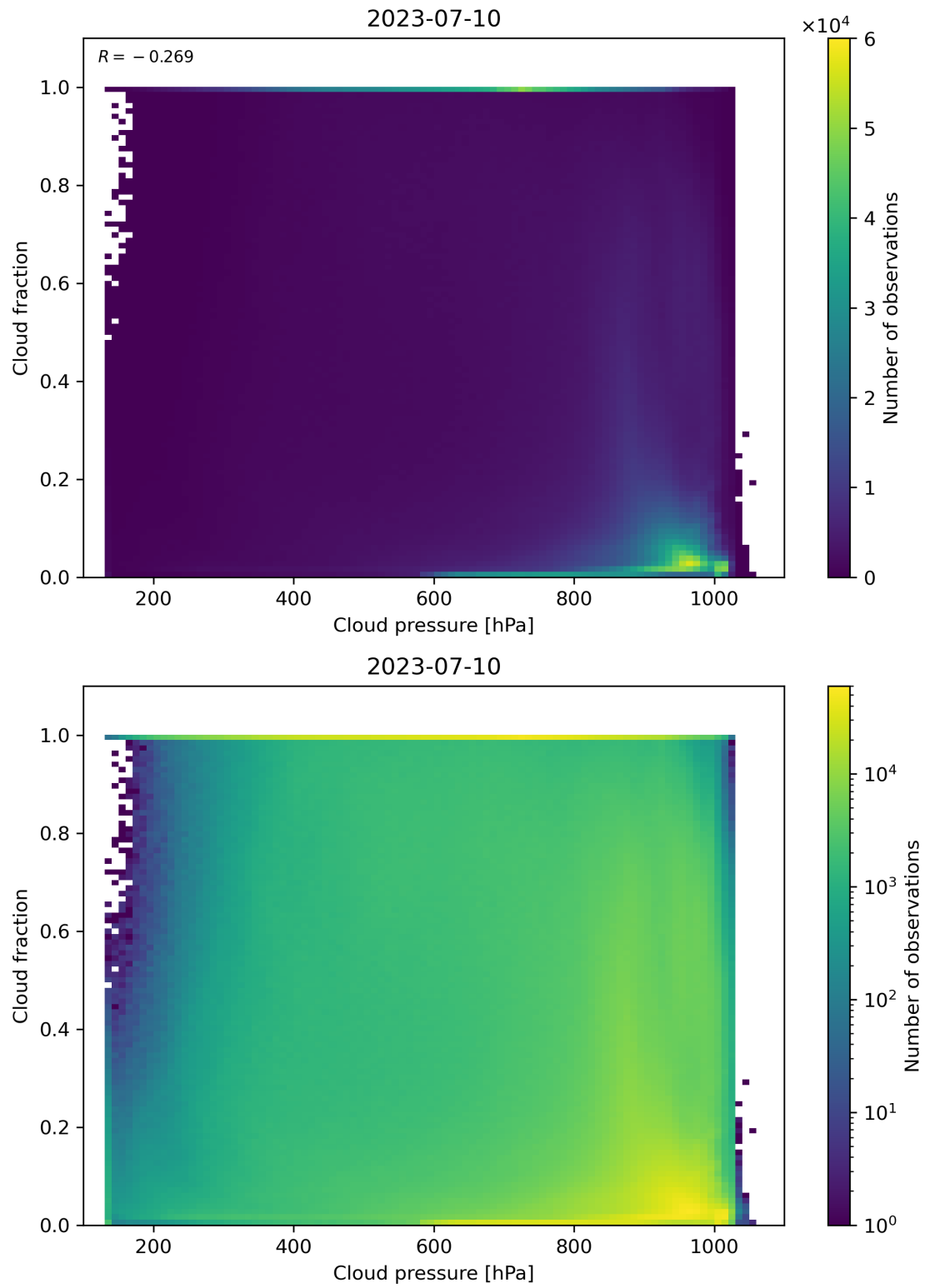
Figure 87: Scatter density plot of “Cloud pressure” against “Cloud fraction” for 2023-07-09 to 2023-07-11.
