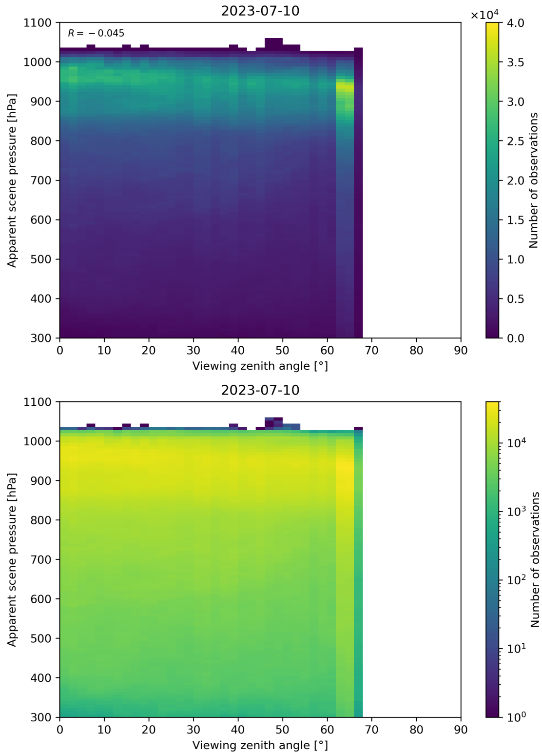
Figure 129: Scatter density plot of “Viewing zenith angle” against “Apparent scene pressure” for 2023-07-09 to 2023-07-11.
