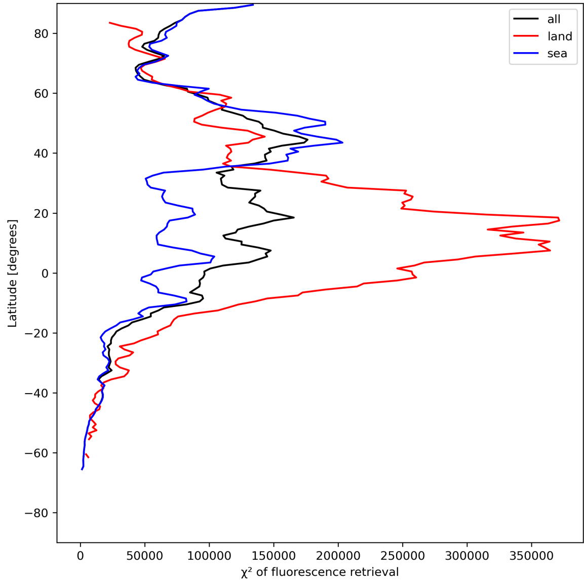
Figure 25: Zonal average of “ \chi^2 of fluorescence retrieval” for 2023-07-09 to 2023-07-11.
