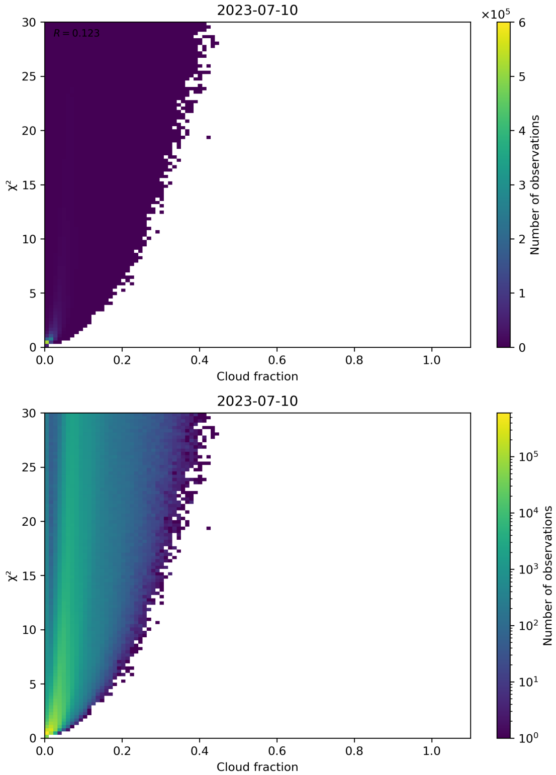
Figure 77: Scatter density plot of “Cloud fraction” against “ \chi^2 ” for 2023-07-09 to 2023-07-11.
