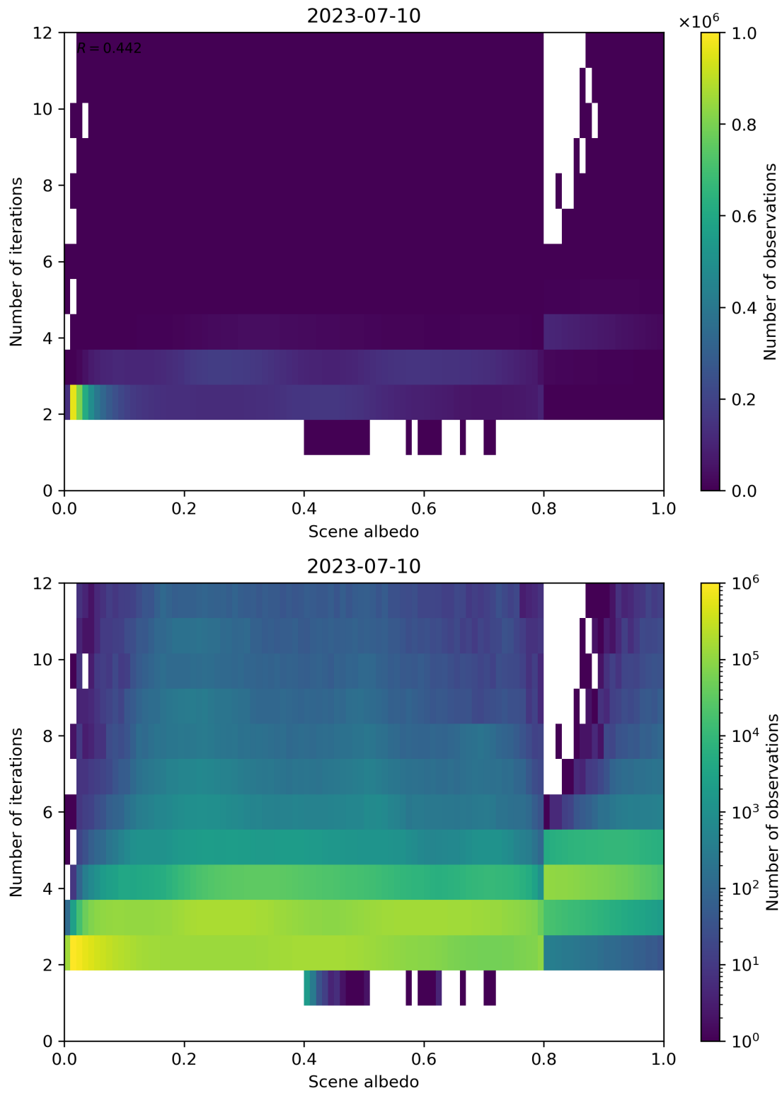
Figure 115: Scatter density plot of “Scene albedo” against “Number of iterations” for 2023-07-09 to 2023-07-11.
