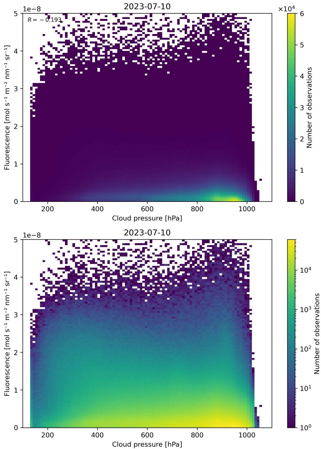
Figure 88: Scatter density plot of “Cloud pressure” against “Fluorescence” for 2023-07-09 to 2023-07-11.
