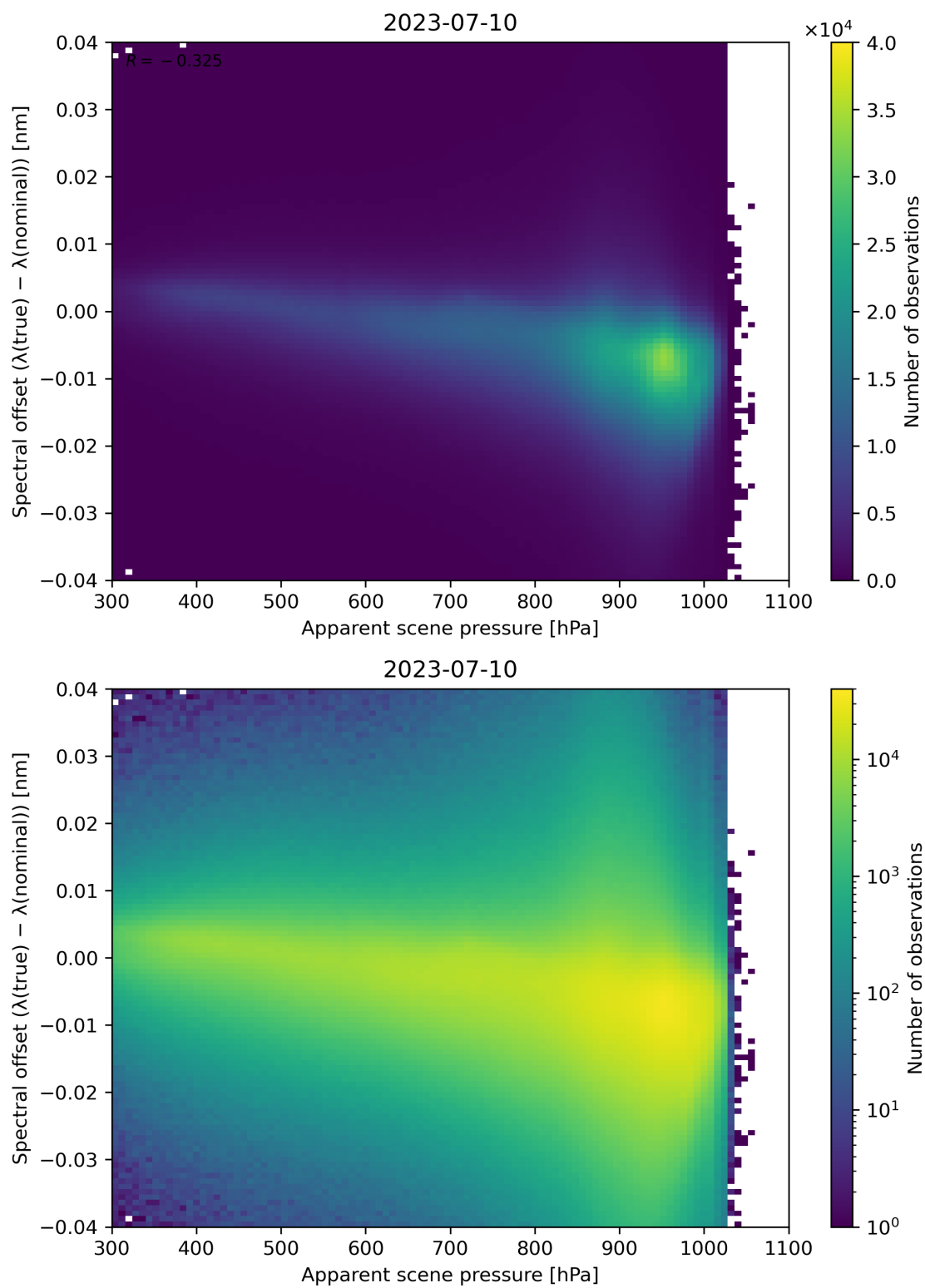
Figure 68: Scatter density plot of “Apparent scene pressure” against “Spectral offset ( \lambda(\text{true}) - \lambda(\text{nominal}) )” for 2023-07-09 to 2023-07-11.
