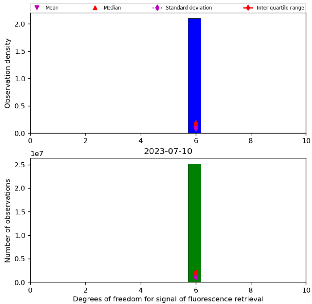
Figure 43: Histogram of “Degrees of freedom for signal of fluorescence retrieval” for 2023-07-09 to 2023-07-11
