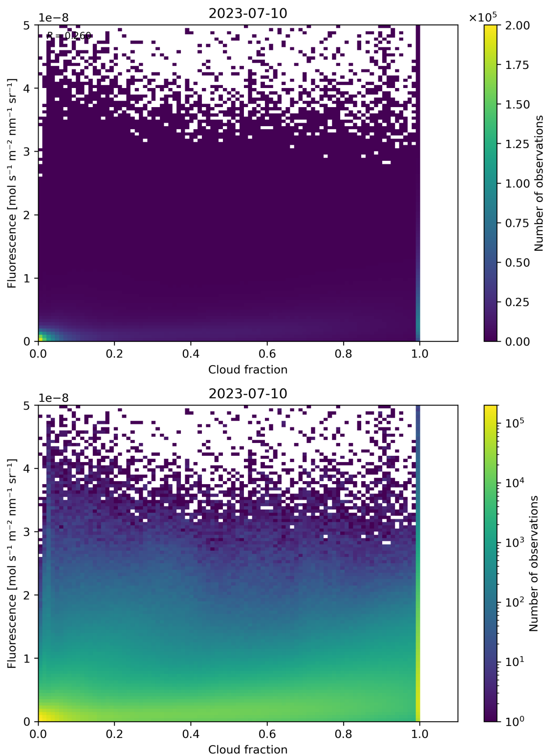
Figure 79: Scatter density plot of “Cloud fraction” against “Fluorescence” for 2023-07-09 to 2023-07-11.
