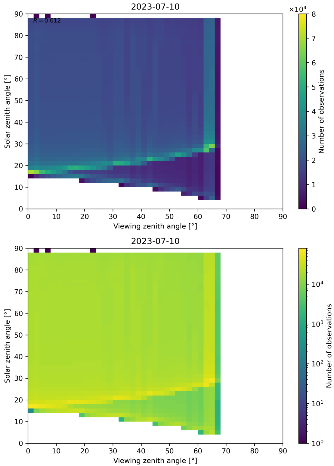
Figure 139: Scatter density plot of “Viewing zenith angle” against “Solar zenith angle” for 2023-07-09 to 2023-07-11.
