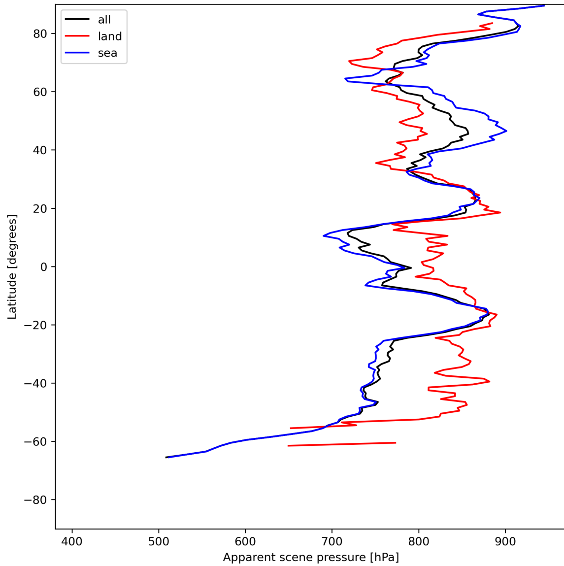
Figure 19: Zonal average of “Apparent scene pressure” for 2023-07-09 to 2023-07-11.
