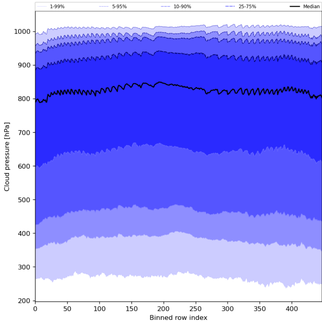
Figure 47: Along track statistics of “Cloud pressure” for 2023-07-09 to 2023-07-11
