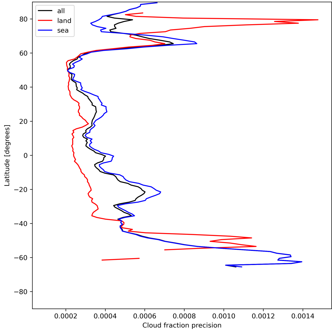
Figure 16: Zonal average of “Cloud fraction precision” for 2023-07-09 to 2023-07-11.
