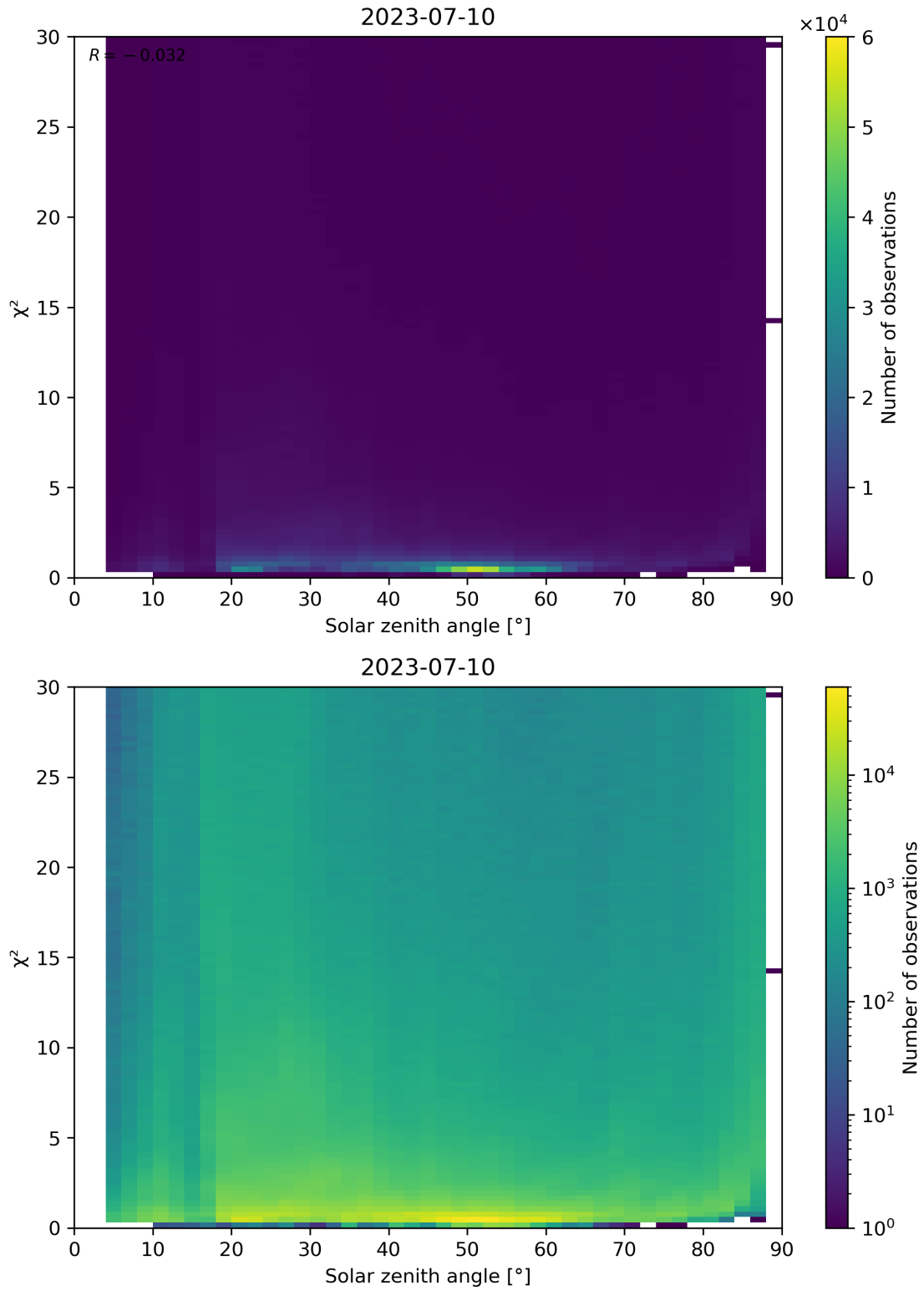
Figure 119: Scatter density plot of “Solar zenith angle” against “ \chi^2 ” for 2023-07-09 to 2023-07-11.
