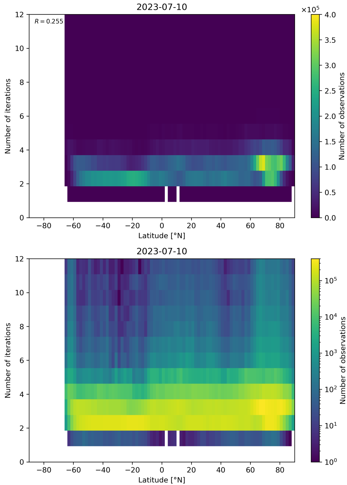
Figure 102: Scatter density plot of “Latitude” against “Number of iterations” for 2023-07-09 to 2023-07-11.
