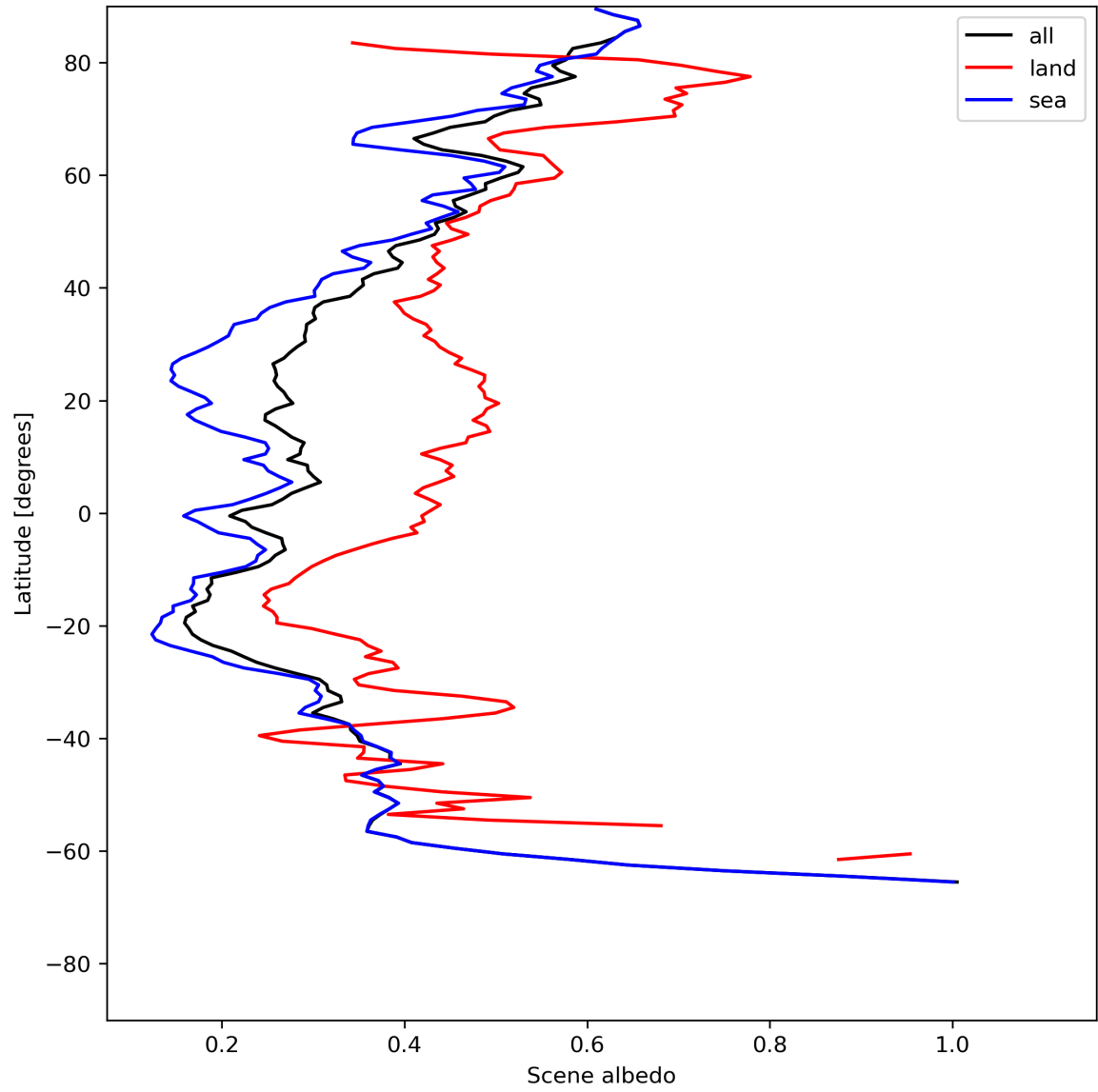
Figure 17: Zonal average of “Scene albedo” for 2023-07-09 to 2023-07-11.
