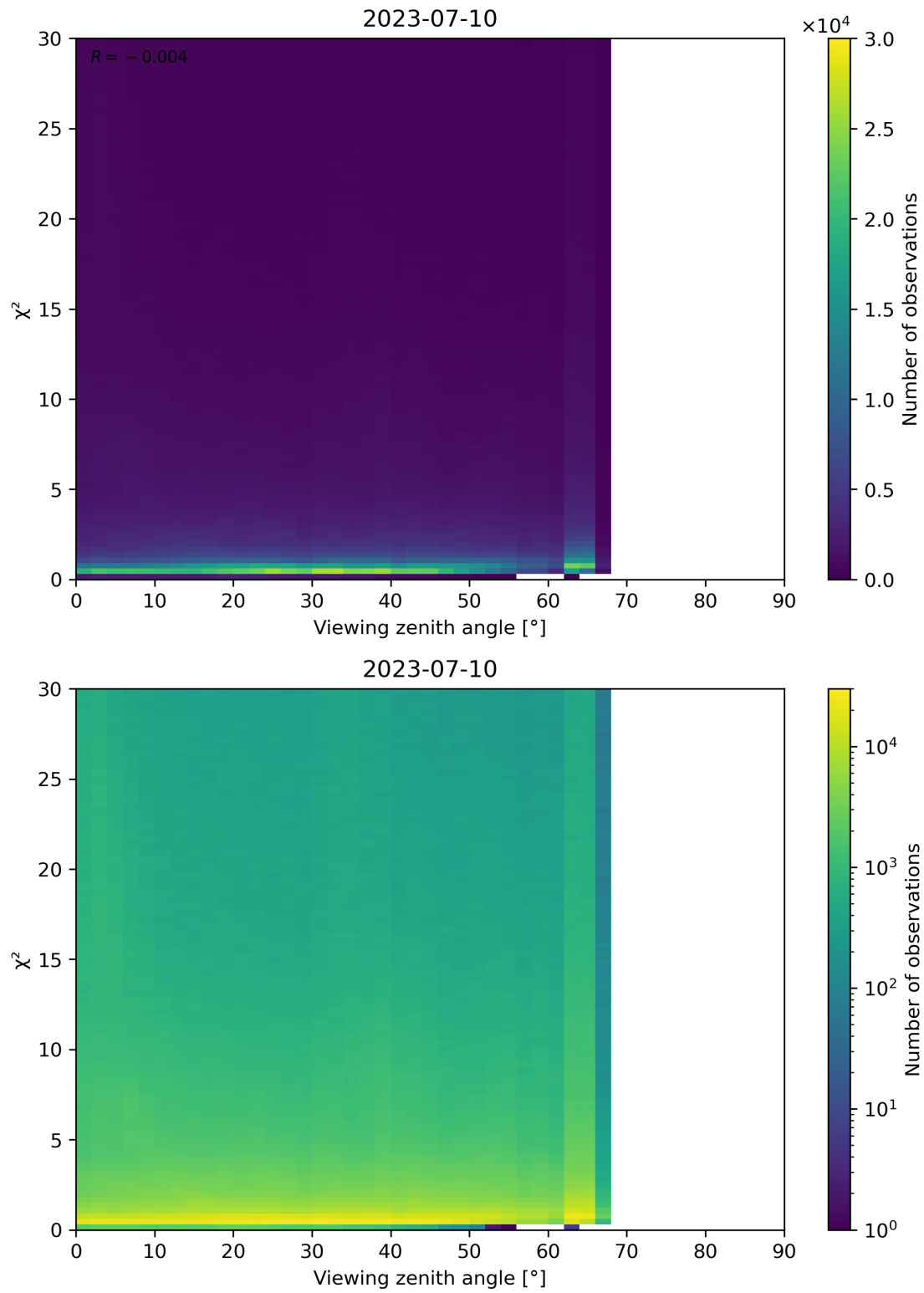
Figure 130: Scatter density plot of “Viewing zenith angle” against “ \chi^2 ” for 2023-07-09 to 2023-07-11.
