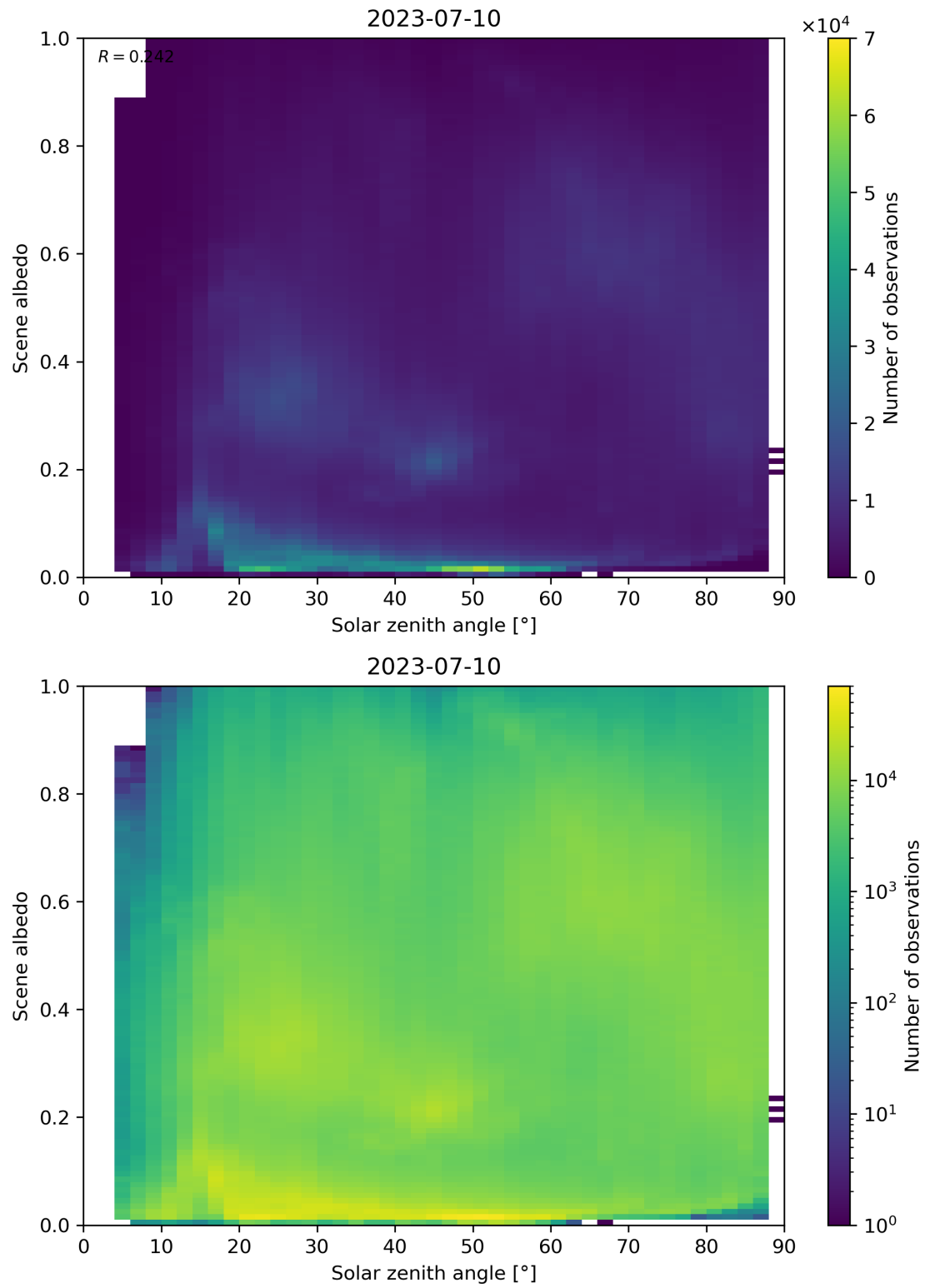
Figure 127: Scatter density plot of “Solar zenith angle” against “Scene albedo” for 2023-07-09 to 2023-07-11.
