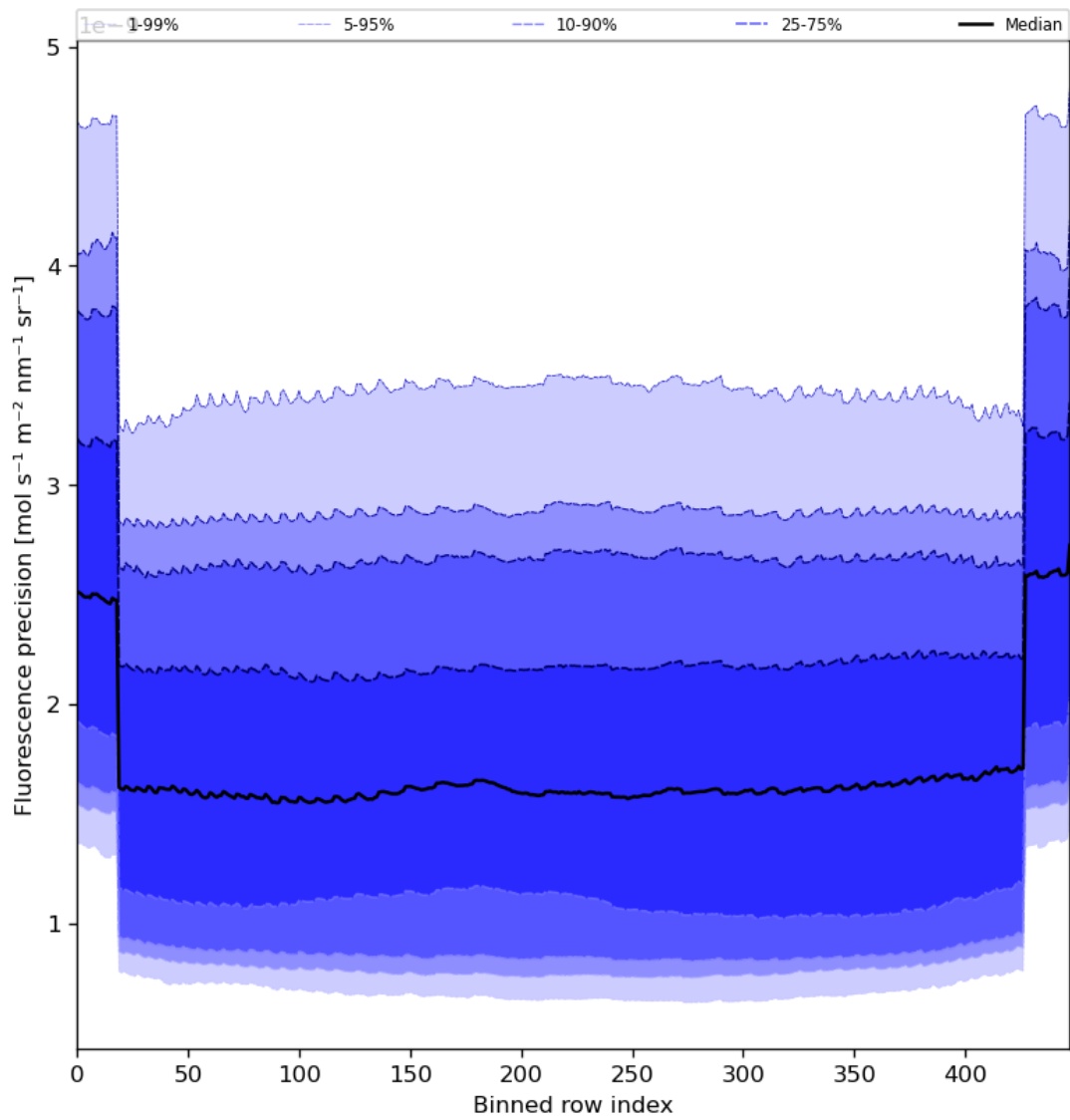
Figure 58: Along track statistics of “Fluorescence precision” for 2023-07-09 to 2023-07-11
