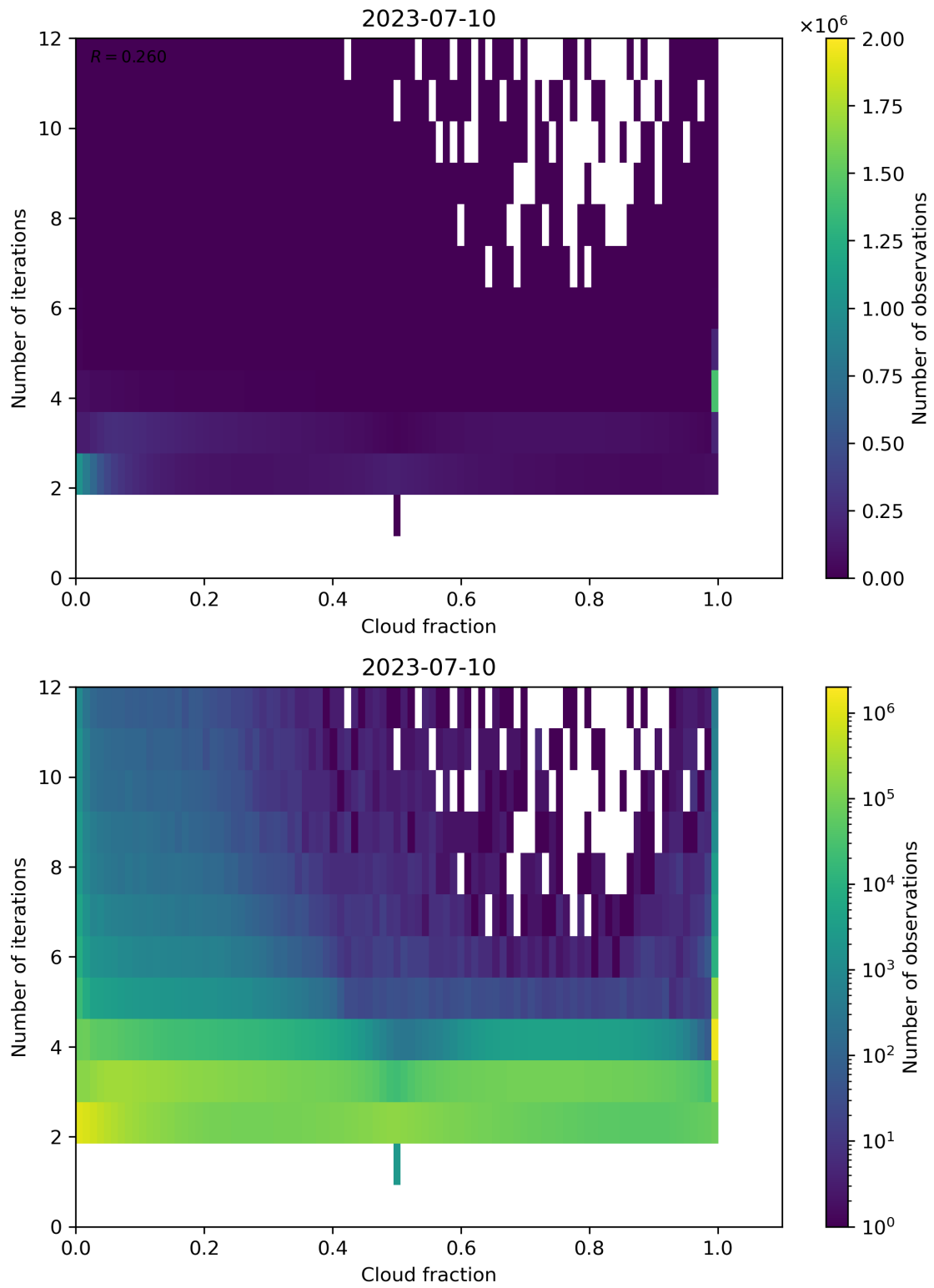
Figure 80: Scatter density plot of “Cloud fraction” against “Number of iterations” for 2023-07-09 to 2023-07-11.
