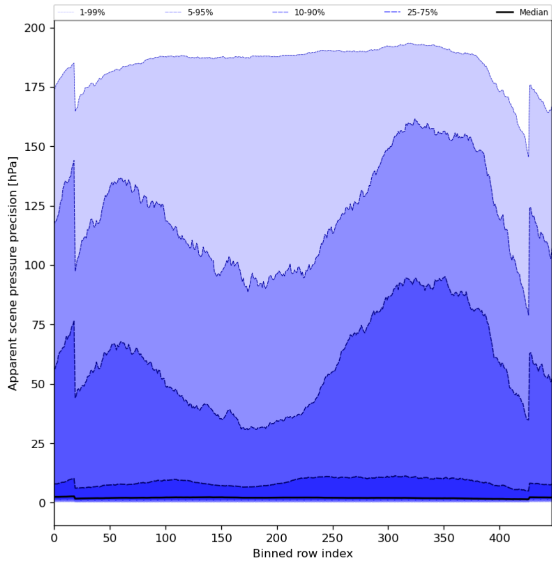
Figure 54: Along track statistics of “Apparent scene pressure precision” for 2023-07-09 to 2023-07-11
