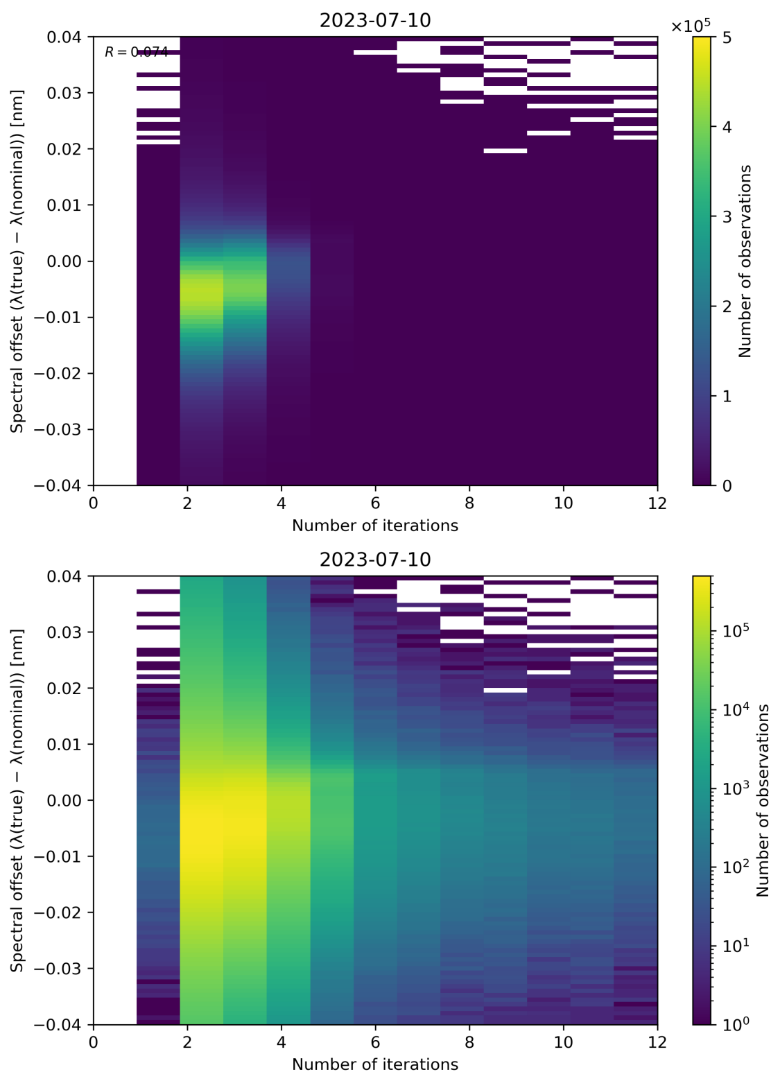
Figure 109: Scatter density plot of “Number of iterations” against “Spectral offset ( \lambda(\text{true}) - \lambda(\text{nominal}) )” for 2023-07-09 to 2023-07-11.
