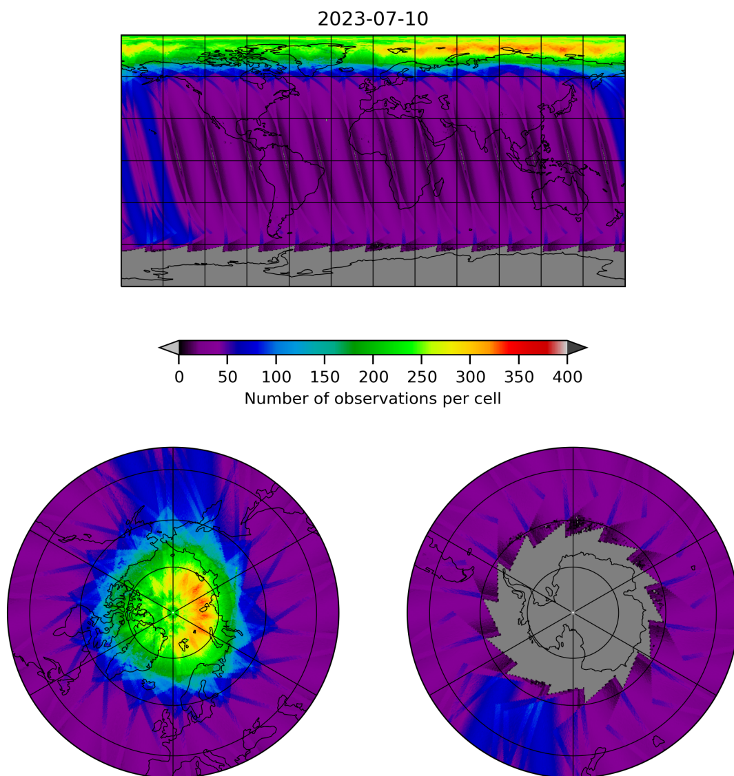
Figure 11: Map of the number of observations for 2023-07-09 to 2023-07-11
