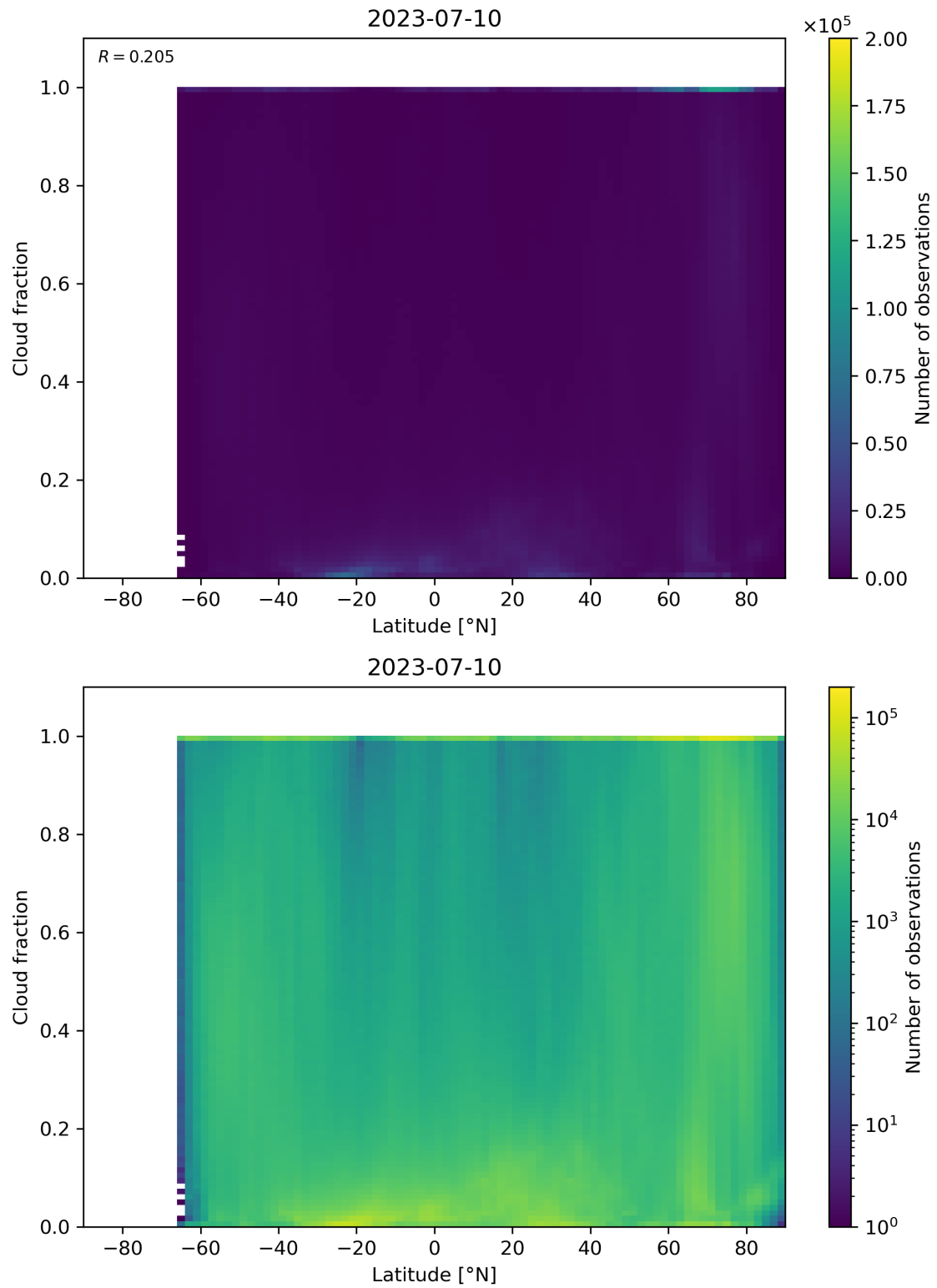
Figure 99: Scatter density plot of “Latitude” against “Cloud fraction” for 2023-07-09 to 2023-07-11.
