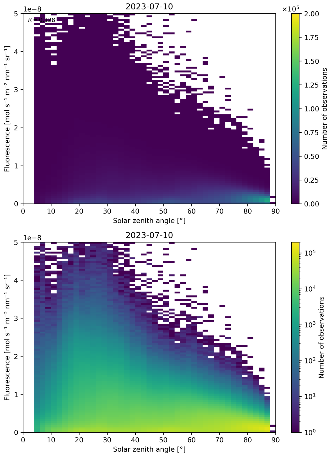
Figure 123: Scatter density plot of “Solar zenith angle” against “Fluorescence” for 2023-07-09 to 2023-07-11.
