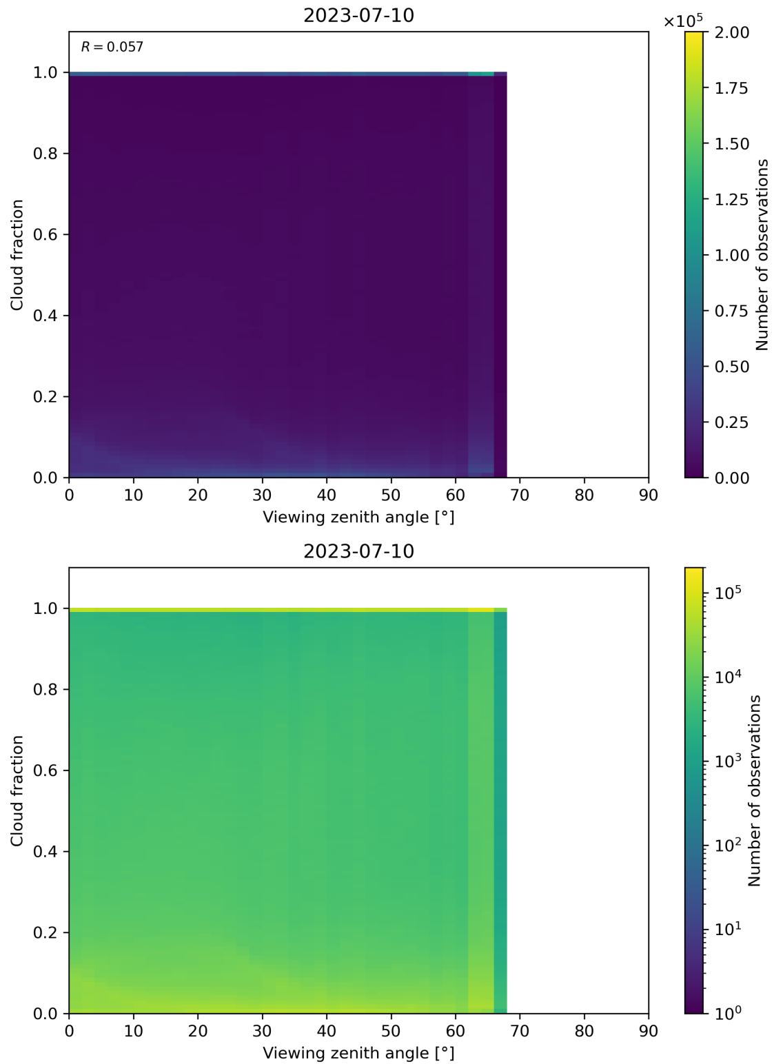
Figure 132: Scatter density plot of “Viewing zenith angle” against “Cloud fraction” for 2023-07-09 to 2023-07-11.
