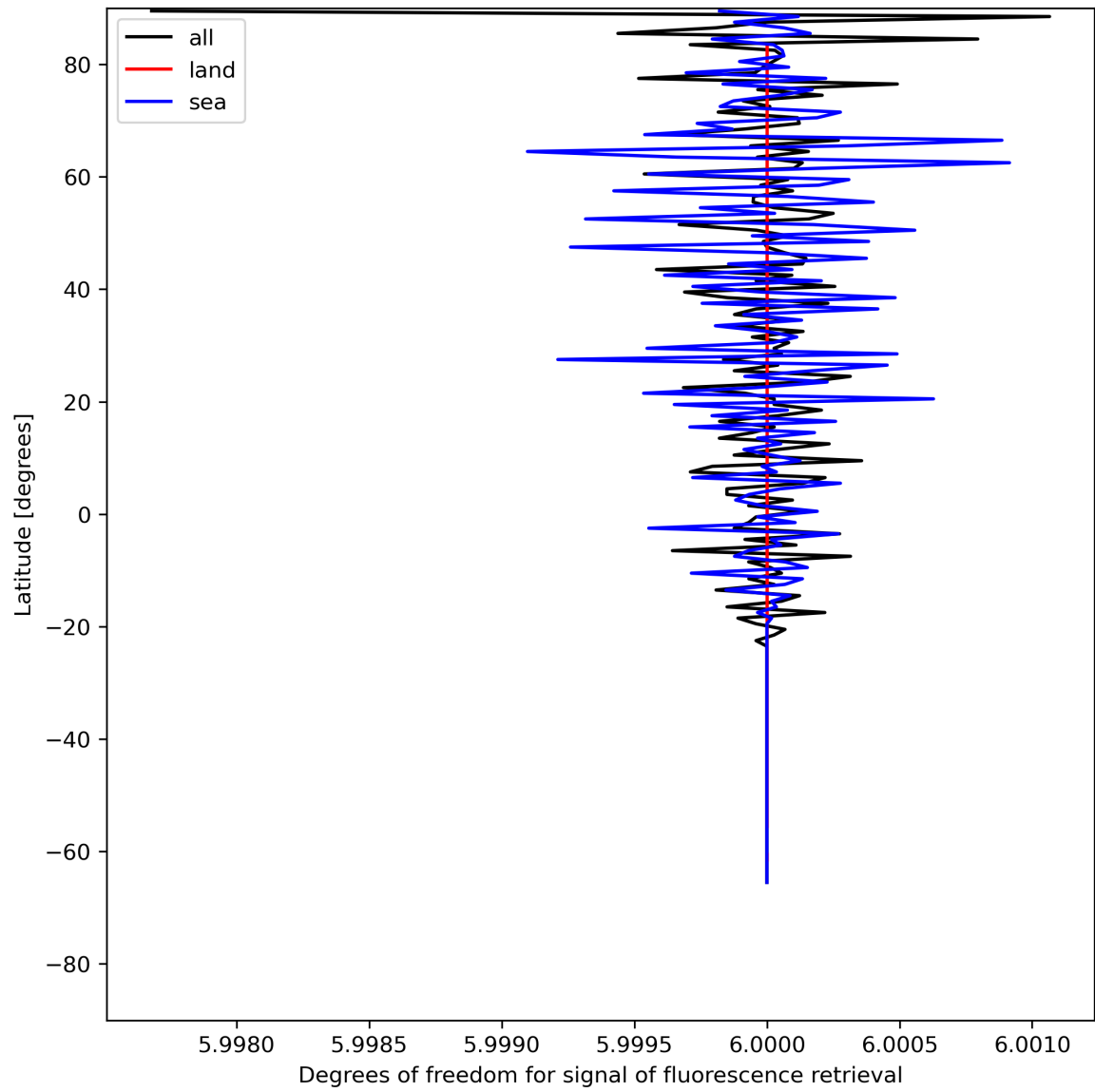
Figure 26: Zonal average of “Degrees of freedom for signal of fluorescence retrieval” for 2023-07-09 to 2023-07-11.
