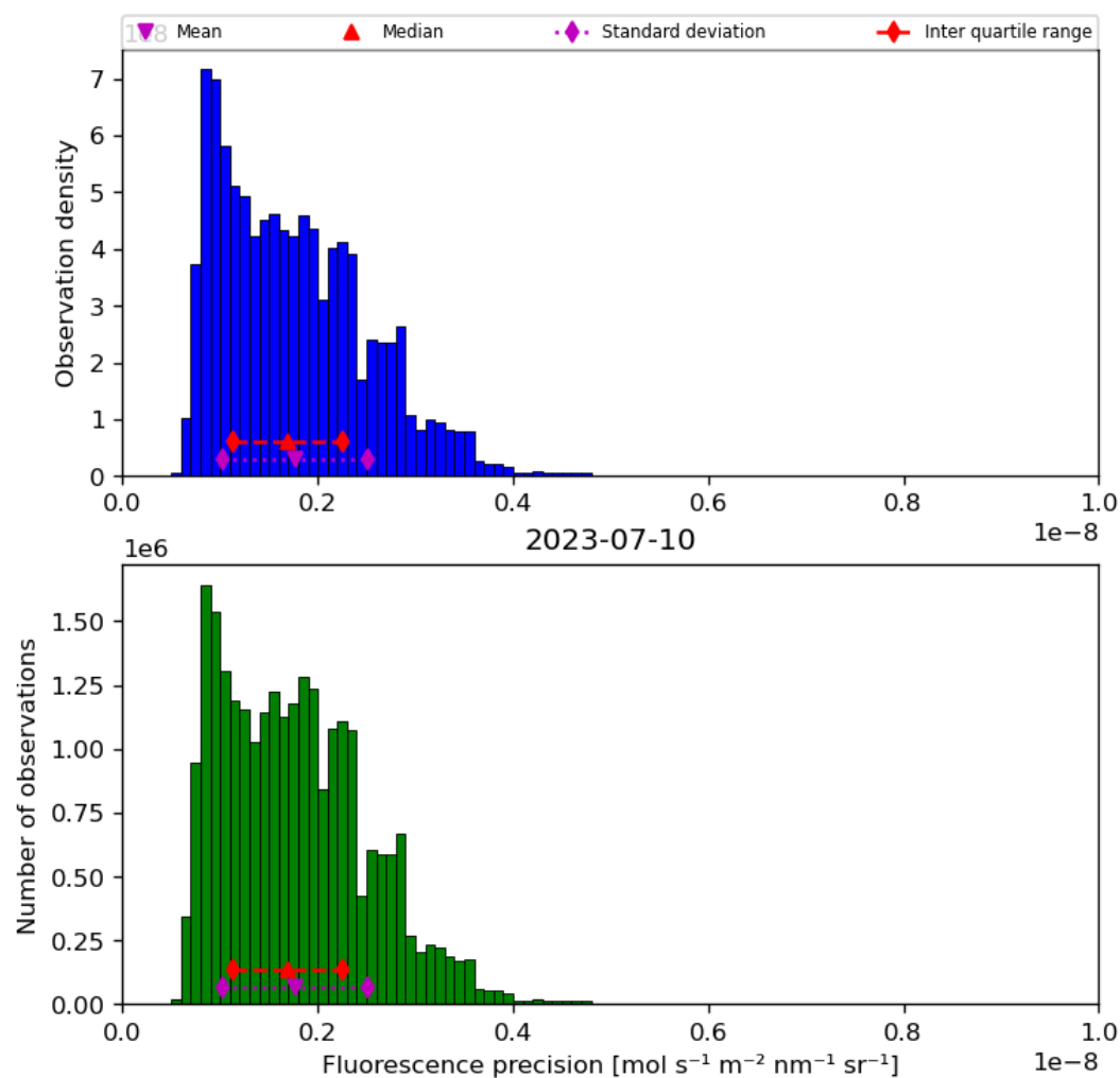
Figure 41: Histogram of “Fluorescence precision” for 2023-07-09 to 2023-07-11
