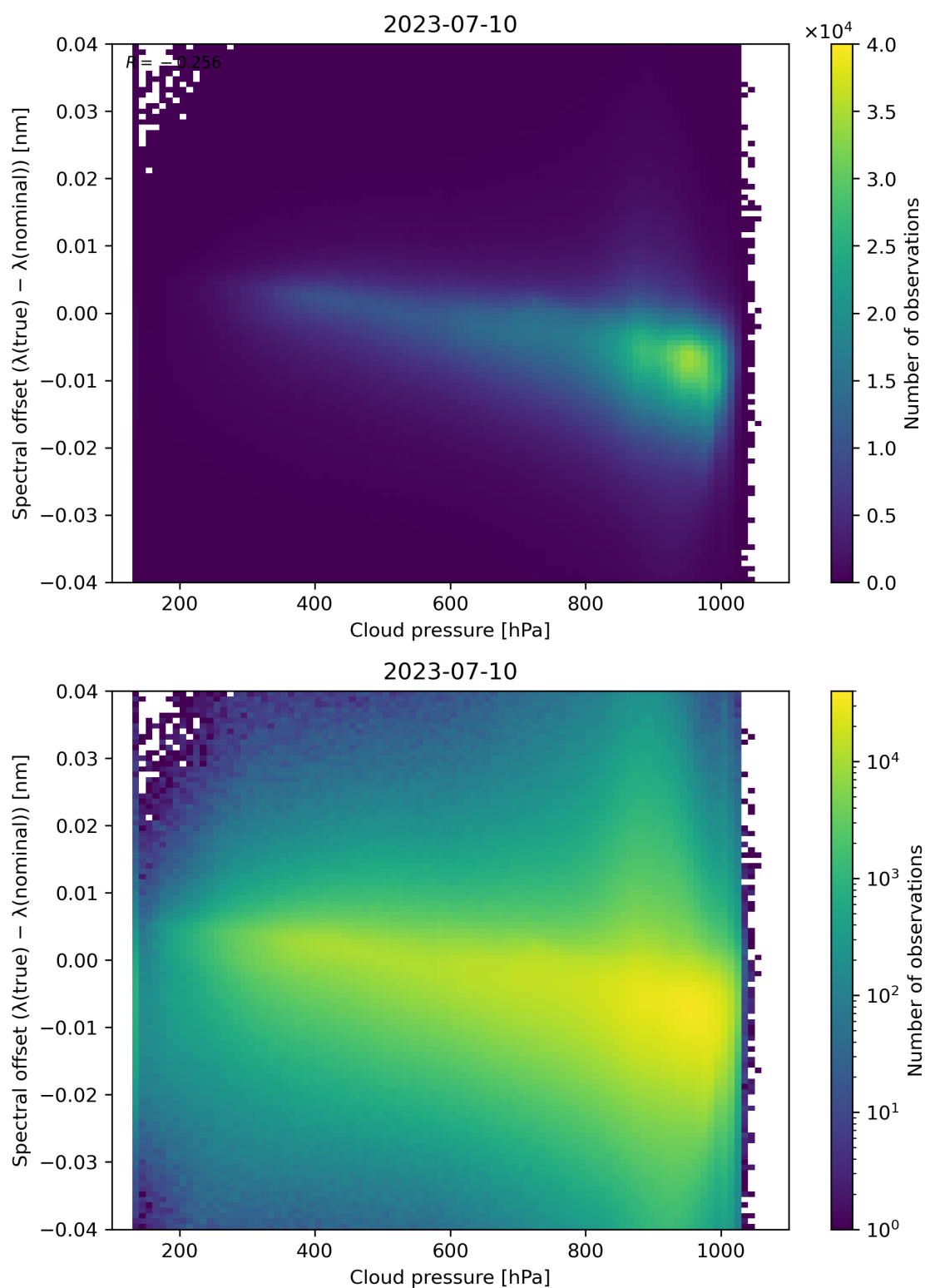
Figure 92: Scatter density plot of “Cloud pressure” against “Spectral offset ( \lambda(\text{true}) - \lambda(\text{nominal}) )” for 2023-07-09 to 2023-07-11.
