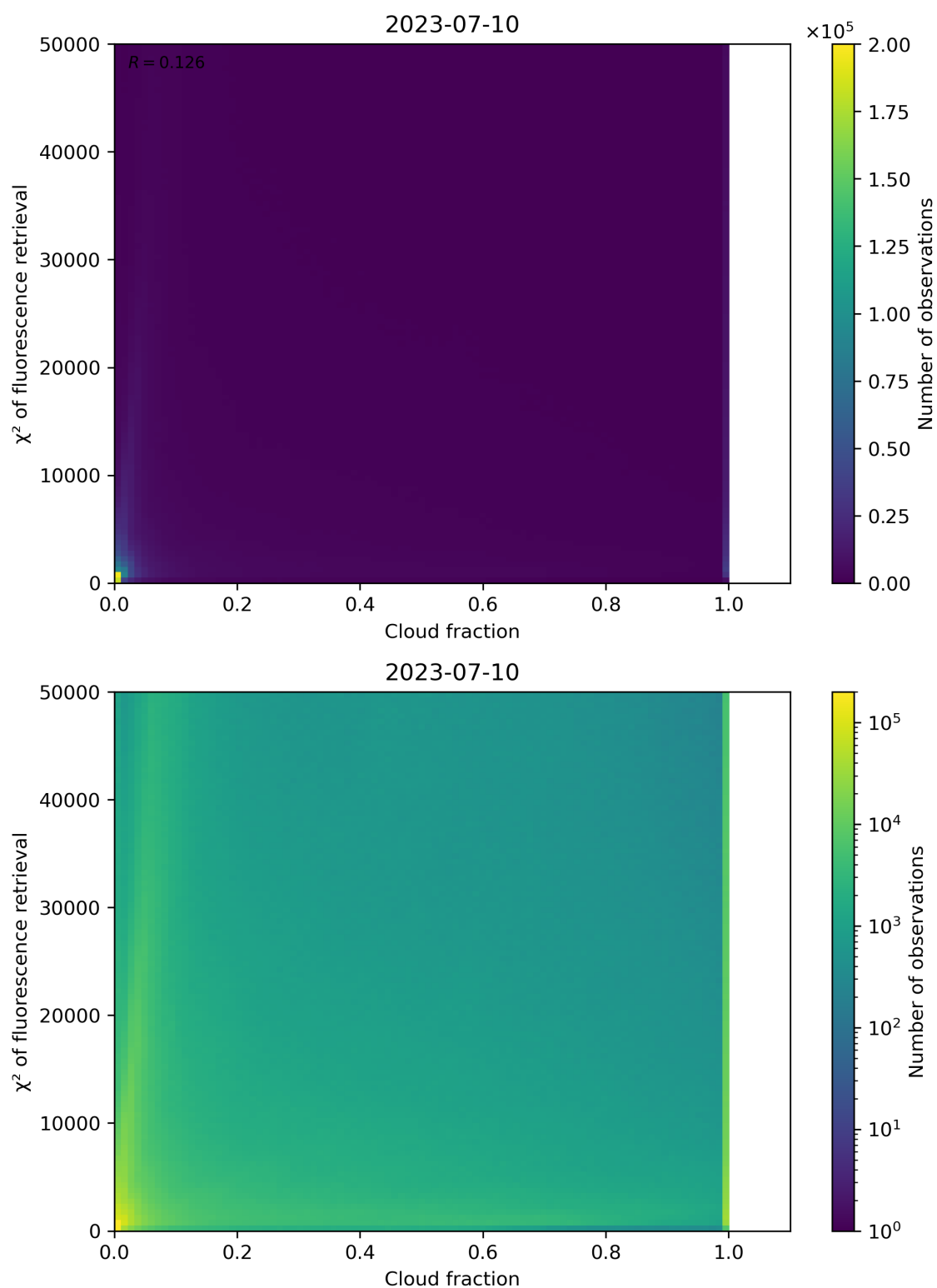
Figure 78: Scatter density plot of “Cloud fraction” against “ \chi^2 of fluorescence retrieval” for 2023-07-09 to 2023-07-11.
