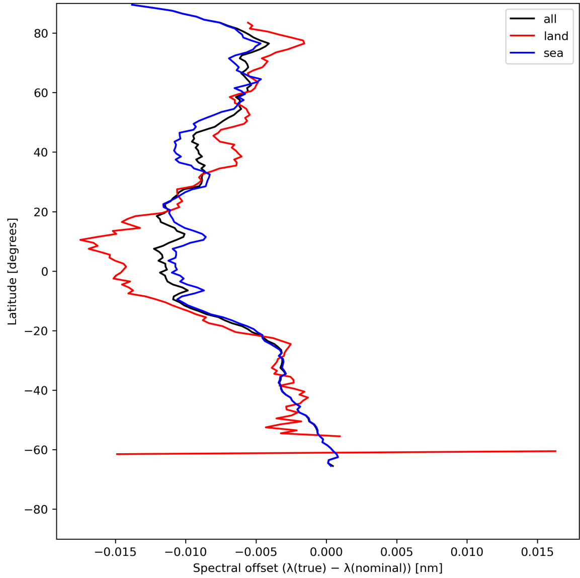
Figure 28: Zonal average of “Spectral offset ( \lambda(\text{true}) - \lambda(\text{nominal}) )” for 2023-07-09 to 2023-07-11.
