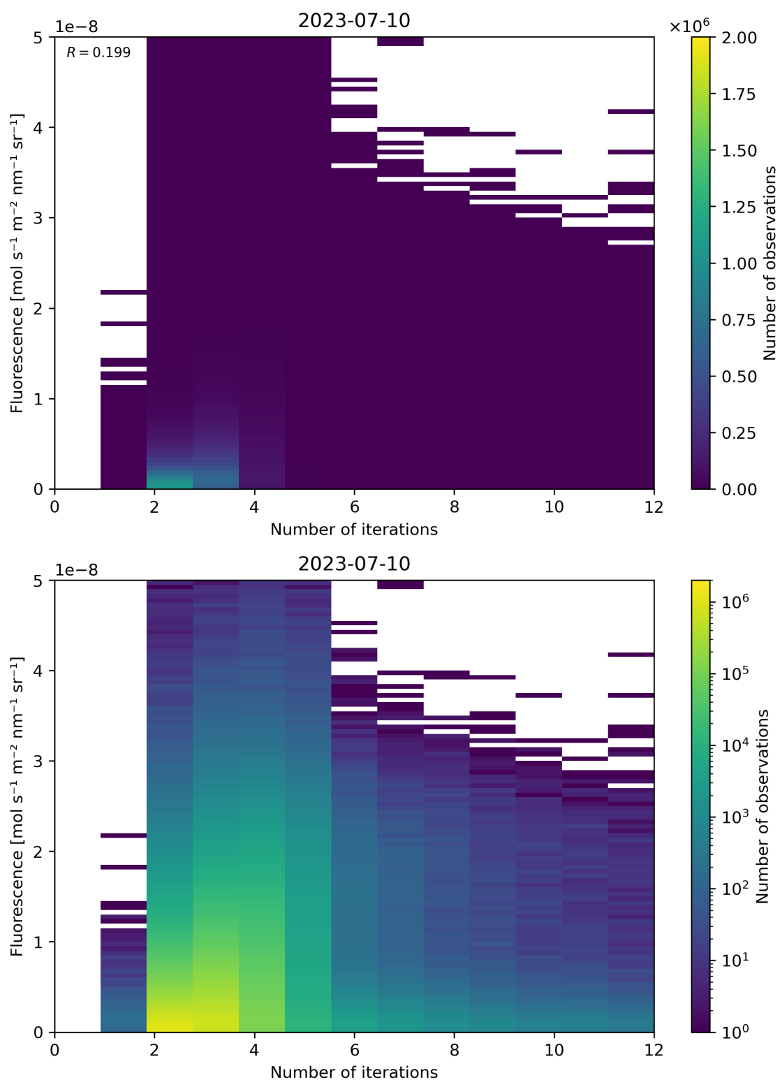
Figure 107: Scatter density plot of “Number of iterations” against “Fluorescence” for 2023-07-09 to 2023-07-11.
