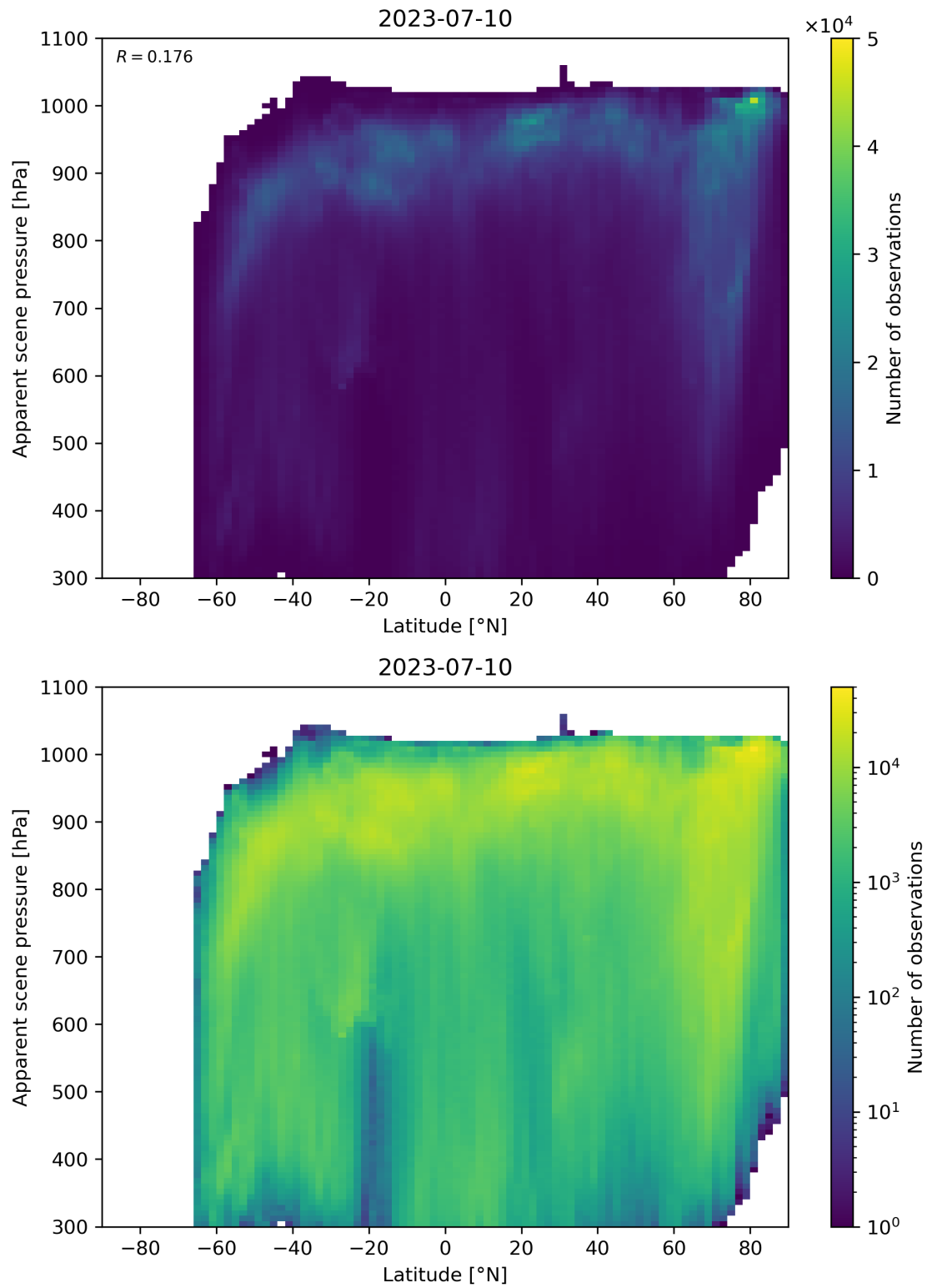
Figure 96: Scatter density plot of “Latitude” against “Apparent scene pressure” for 2023-07-09 to 2023-07-11.
