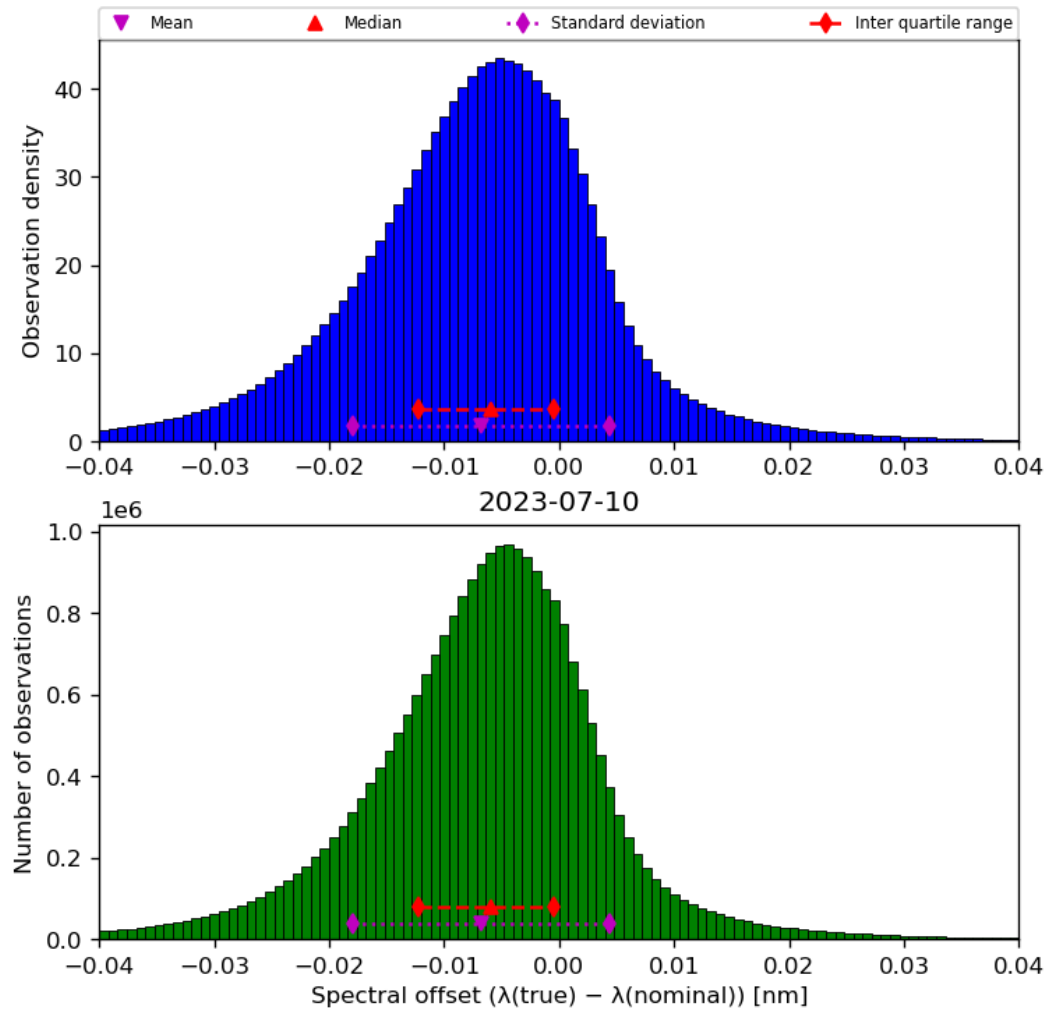
Figure 45: Histogram of “Spectral offset ( \lambda(\text{true}) - \lambda(\text{nominal}) )” for 2023-07-09 to 2023-07-11
