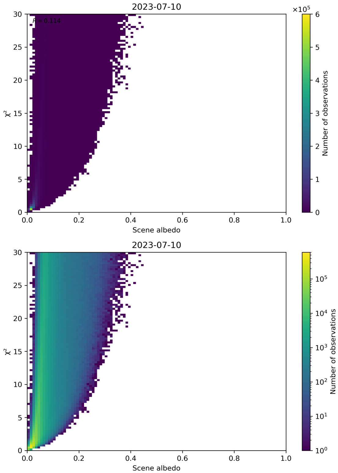
Figure 112: Scatter density plot of “Scene albedo” against “ \chi^2 ” for 2023-07-09 to 2023-07-11.
