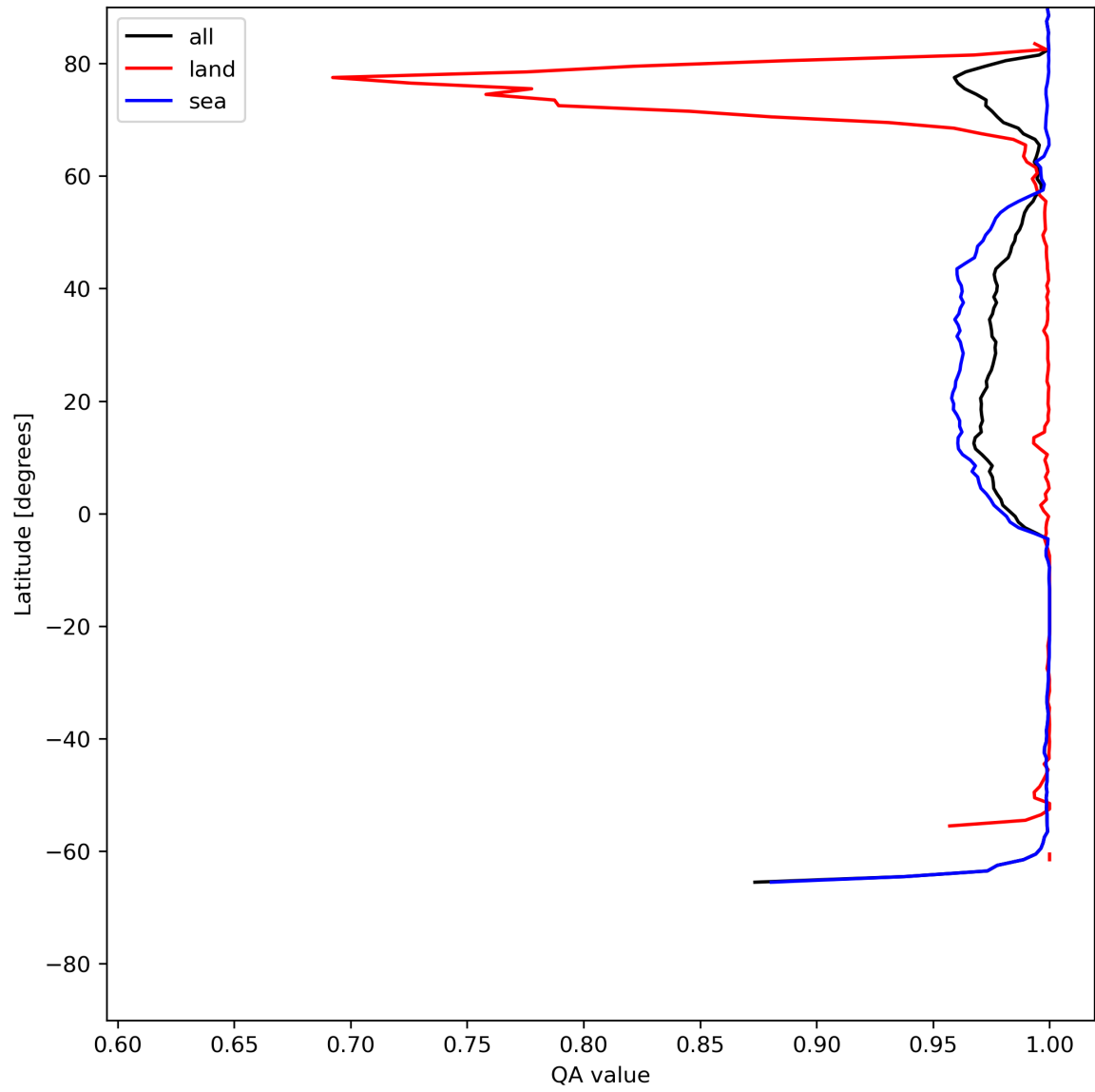
Figure 12: Zonal average of "QA value" for 2023-07-09 to 2023-07-11.
