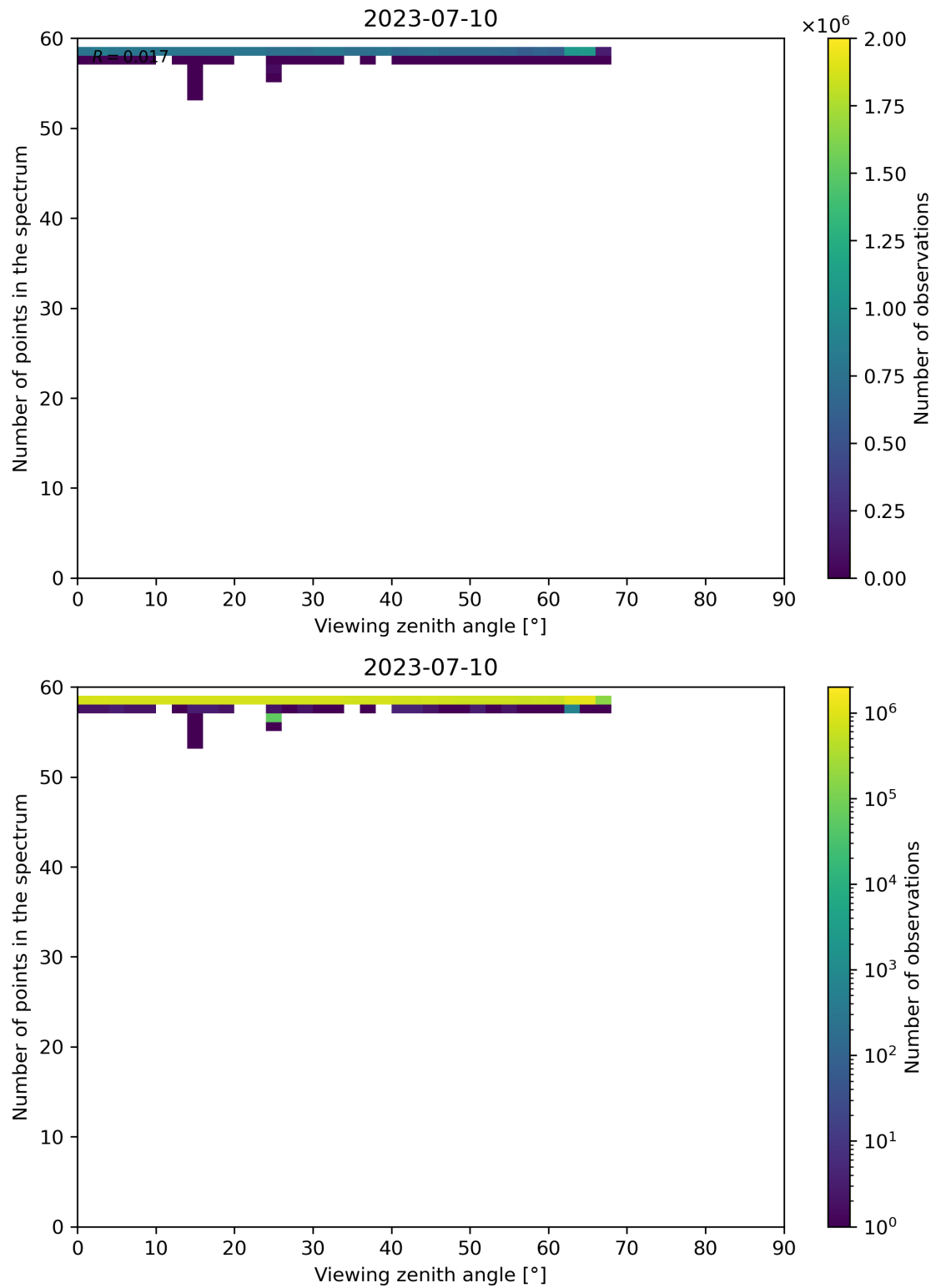
Figure 137: Scatter density plot of “Viewing zenith angle” against “Number of points in the spectrum” for 2023-07-09 to 2023-07-11.
