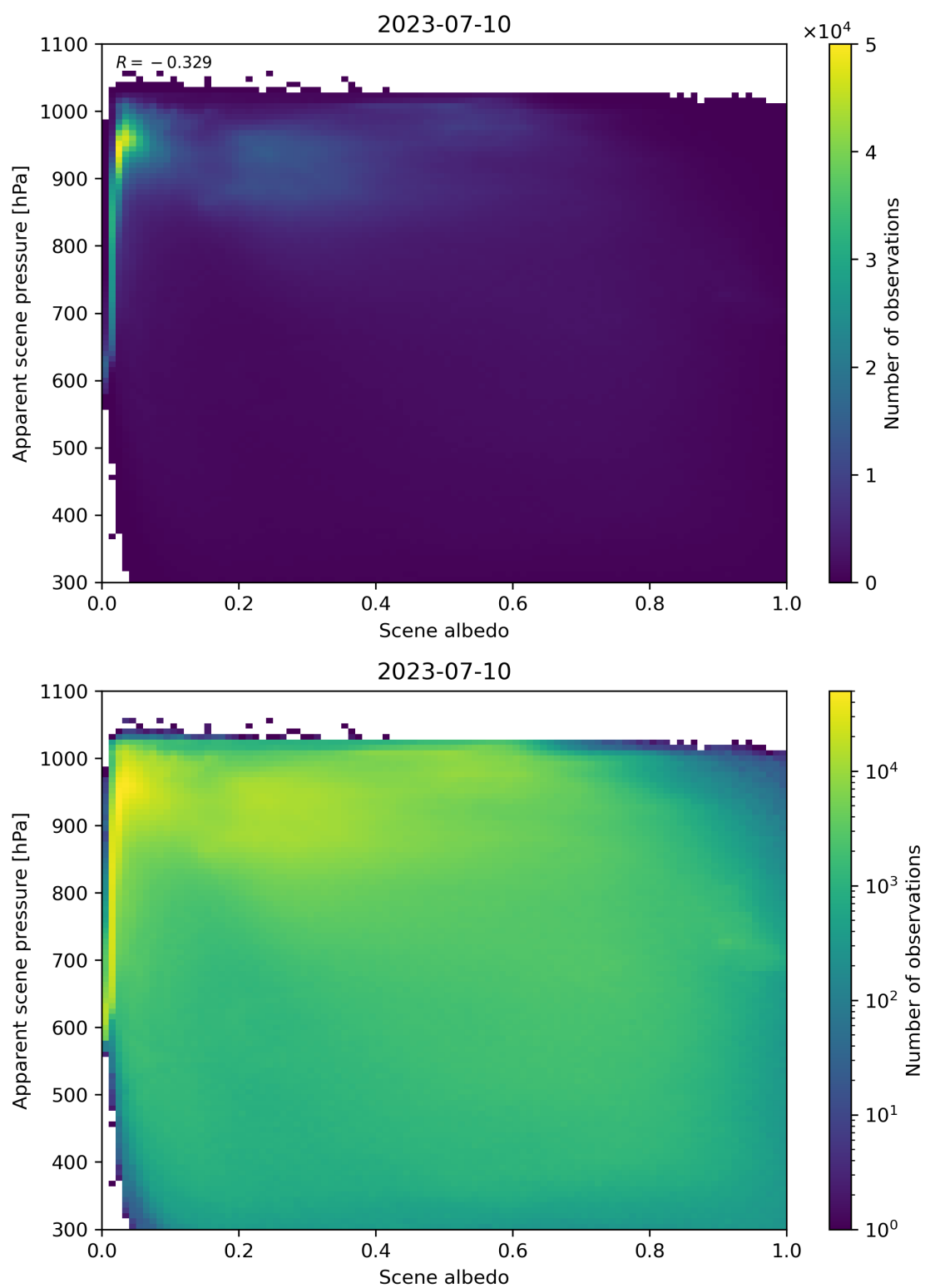
Figure 111: Scatter density plot of “Scene albedo” against “Apparent scene pressure” for 2023-07-09 to 2023-07-11.
