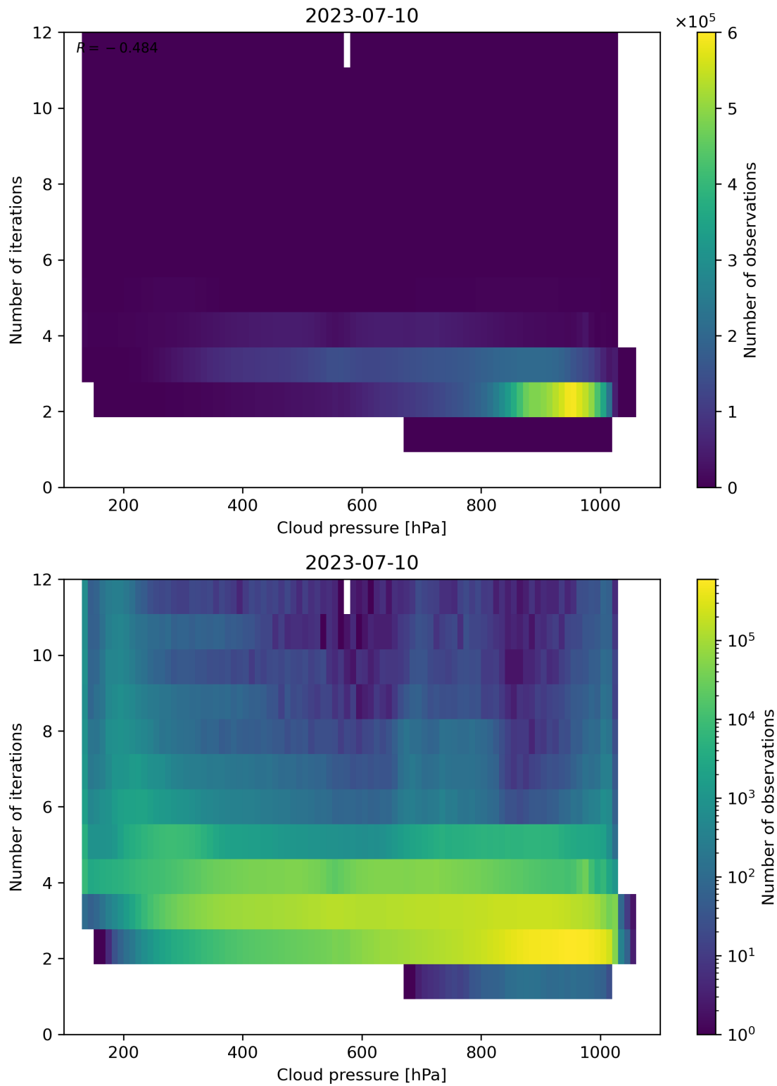
Figure 89: Scatter density plot of “Cloud pressure” against “Number of iterations” for 2023-07-09 to 2023-07-11.
