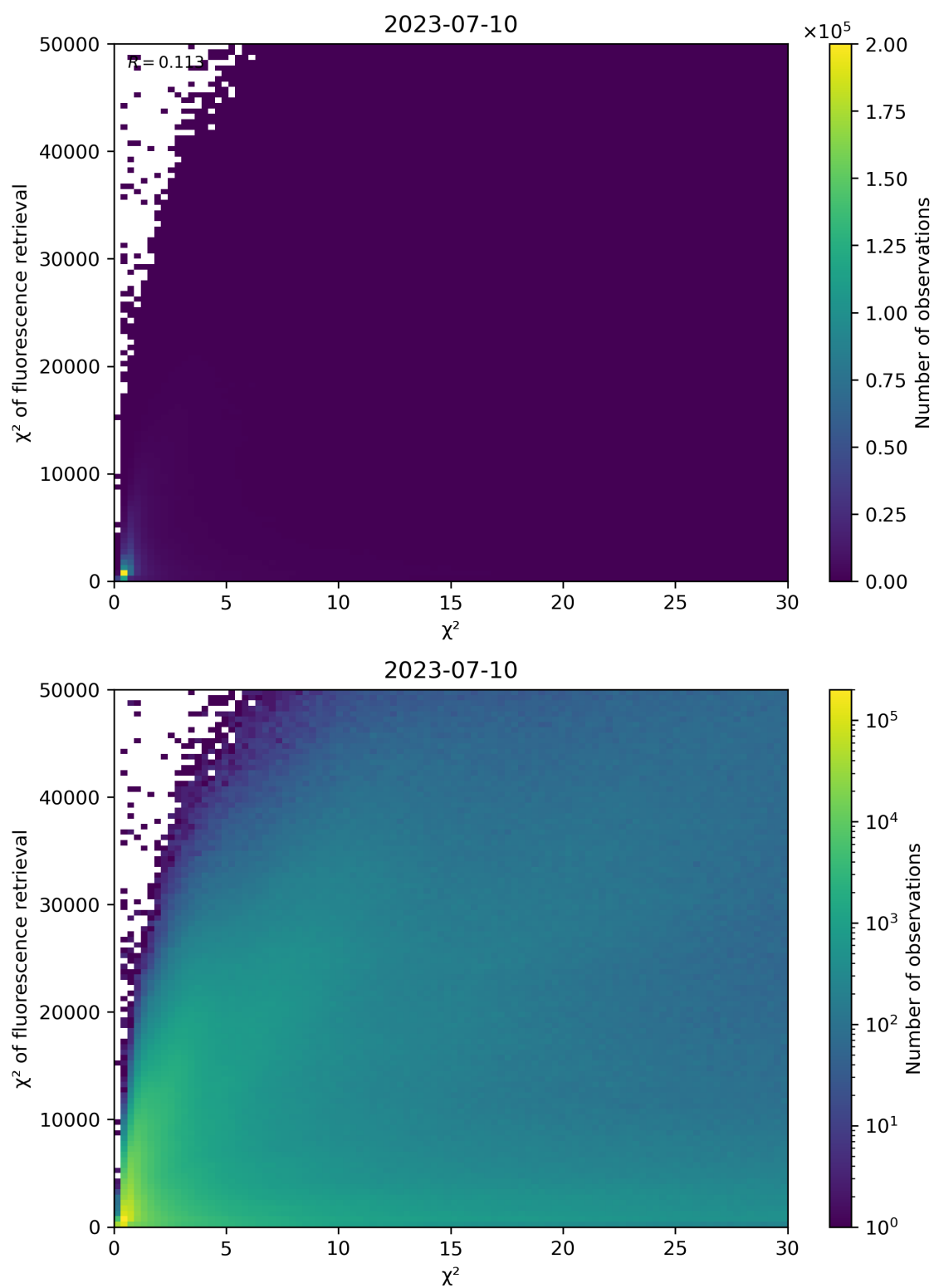
Figure 69: Scatter density plot of “ \chi^2 ” against “ \chi^2 of fluorescence retrieval” for 2023-07-09 to 2023-07-11.
