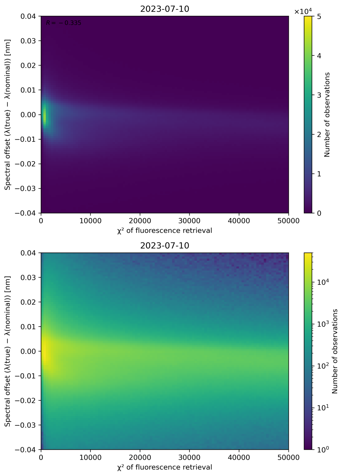
Figure 72: Scatter density plot of " \chi^2 of fluorescence retrieval" against "Spectral offset ( \lambda(\text{true}) - \lambda(\text{nominal}) )" for 2023-07-09 to 2023-07-11.
