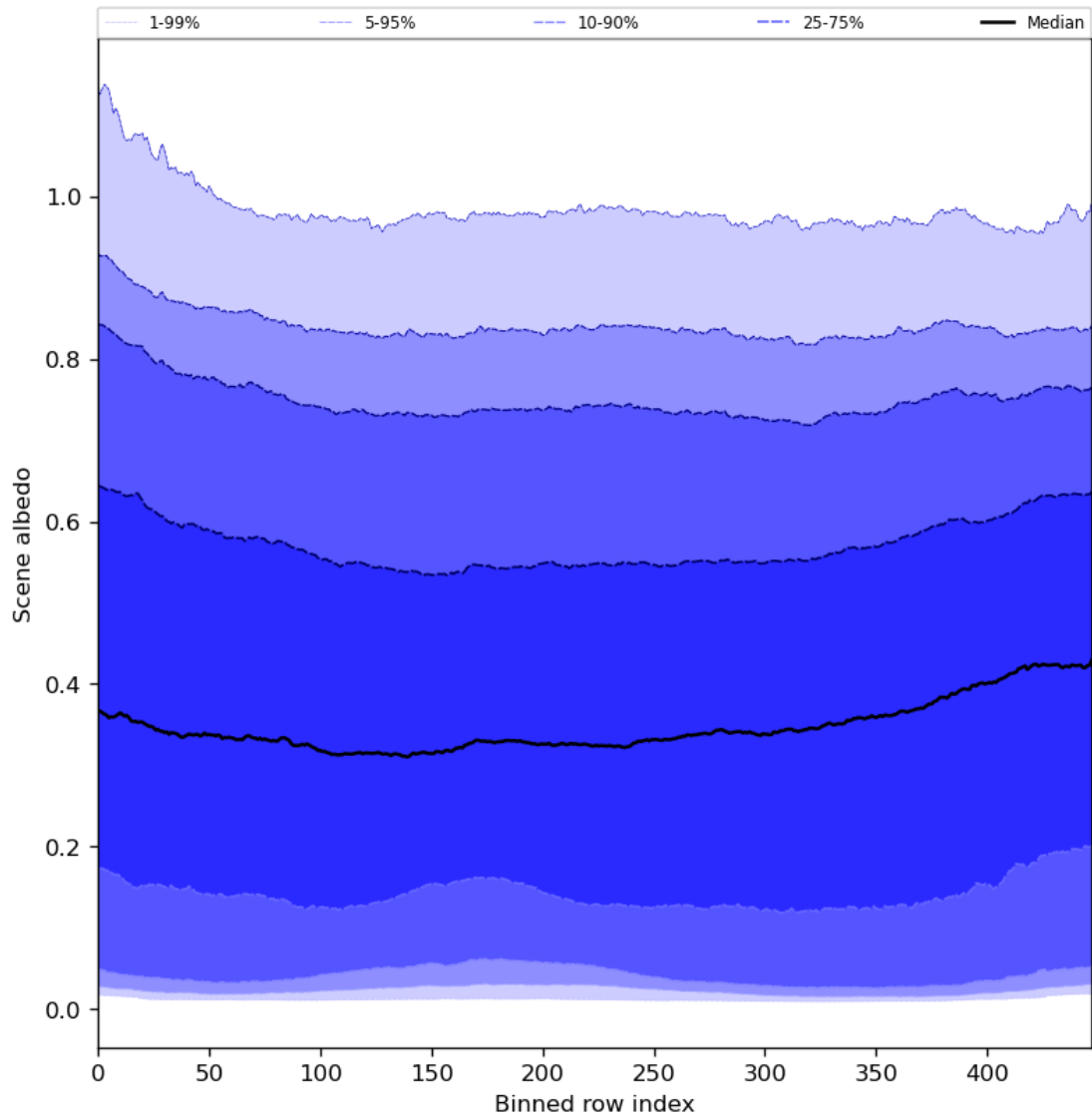
Figure 51: Along track statistics of “Scene albedo” for 2023-07-09 to 2023-07-11
