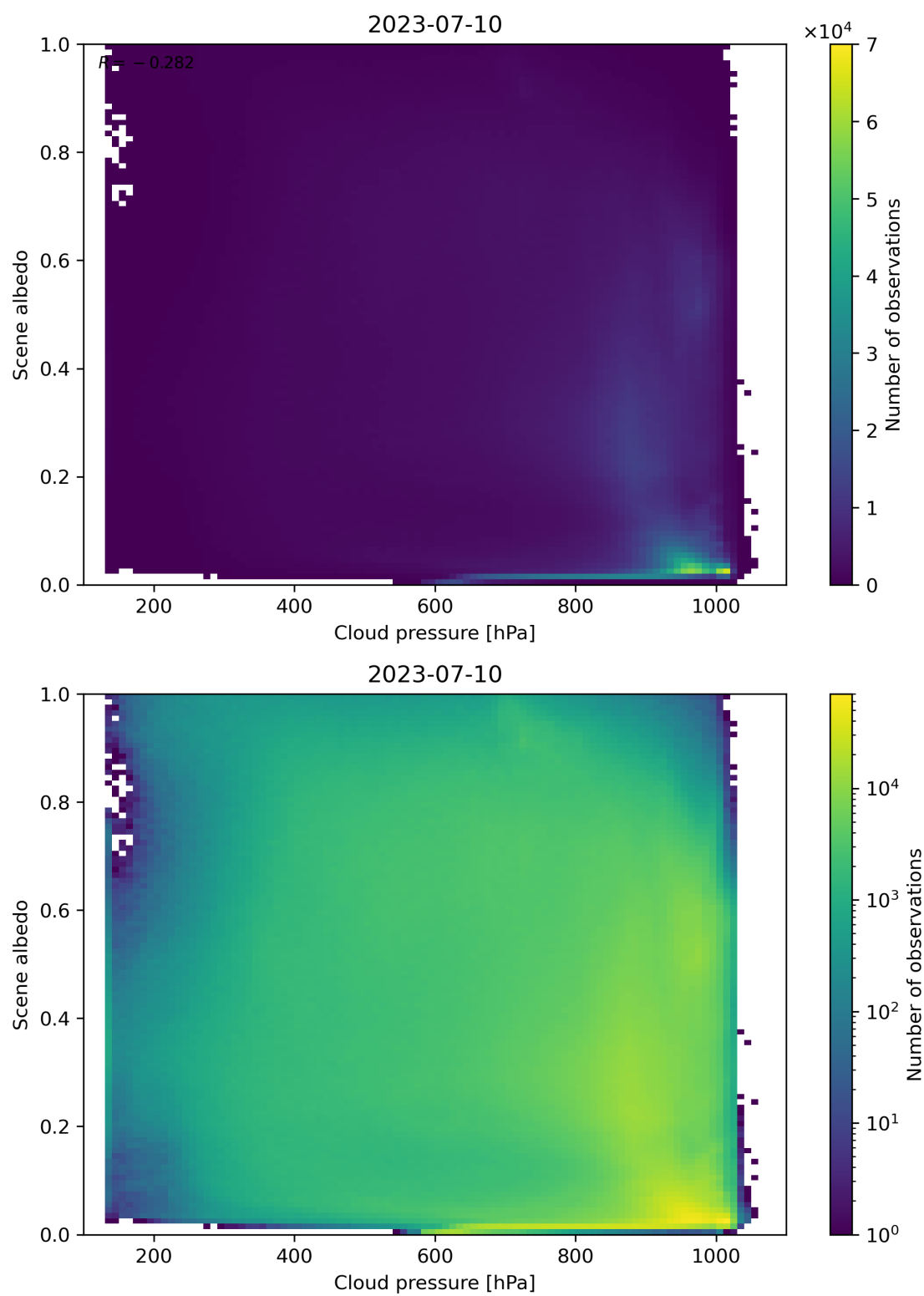
Figure 91: Scatter density plot of “Cloud pressure” against “Scene albedo” for 2023-07-09 to 2023-07-11.
