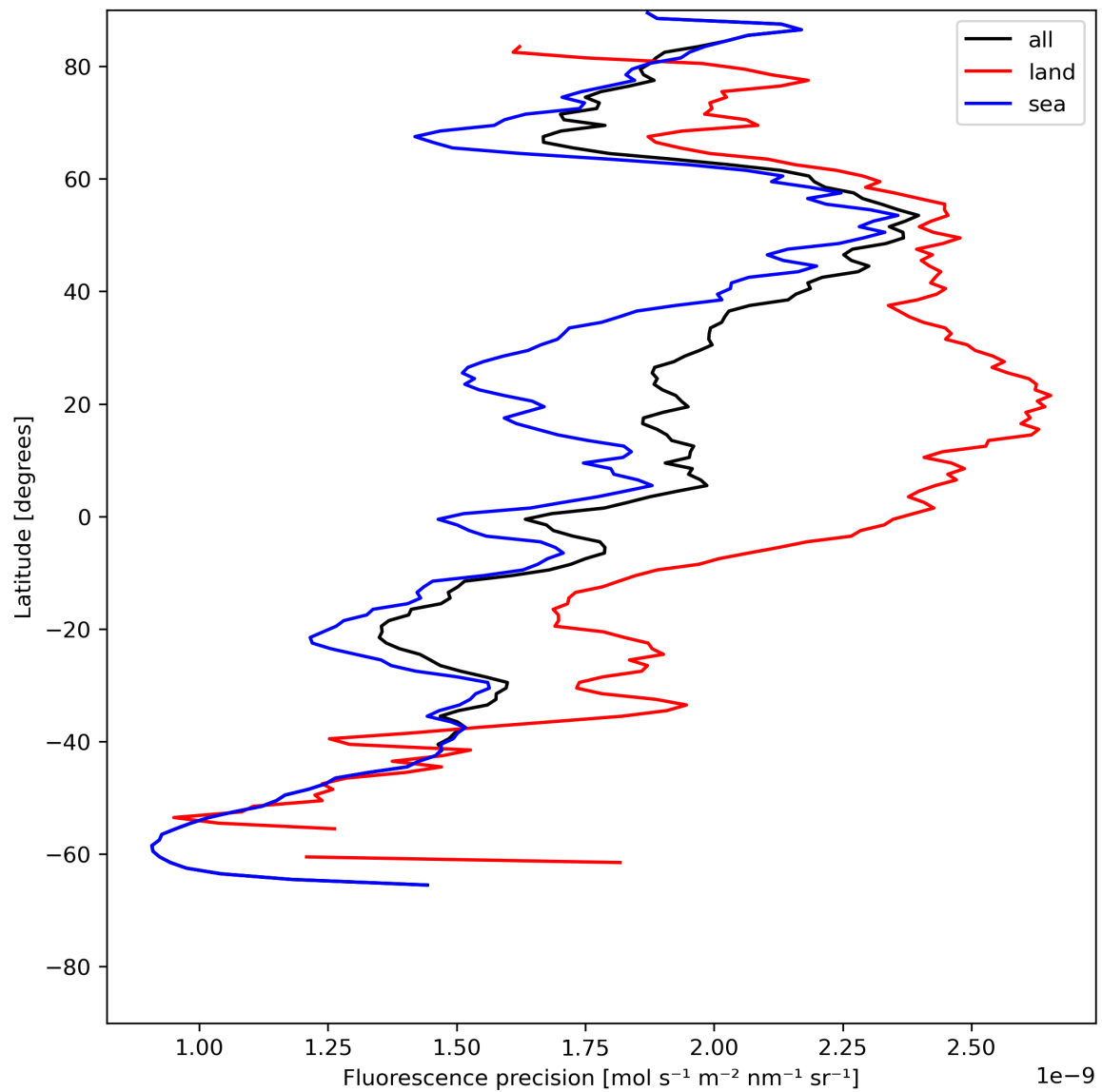
Figure 24: Zonal average of “Fluorescence precision” for 2023-07-09 to 2023-07-11.
