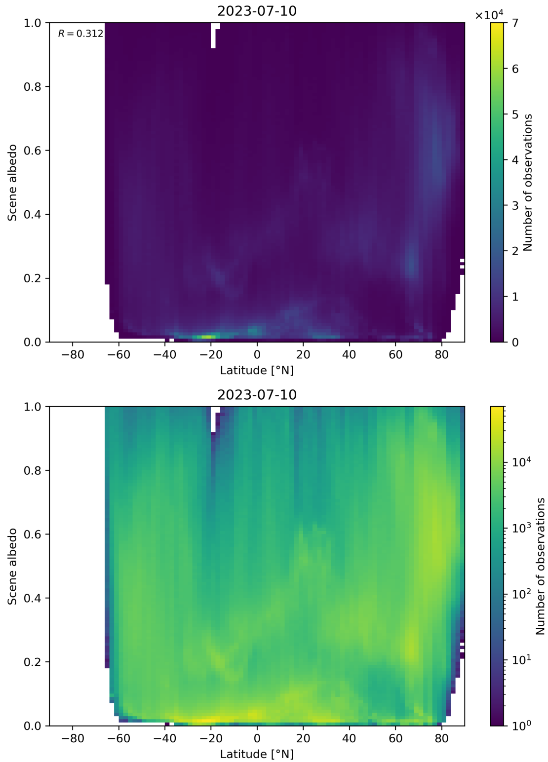
Figure 104: Scatter density plot of “Latitude” against “Scene albedo” for 2023-07-09 to 2023-07-11.
