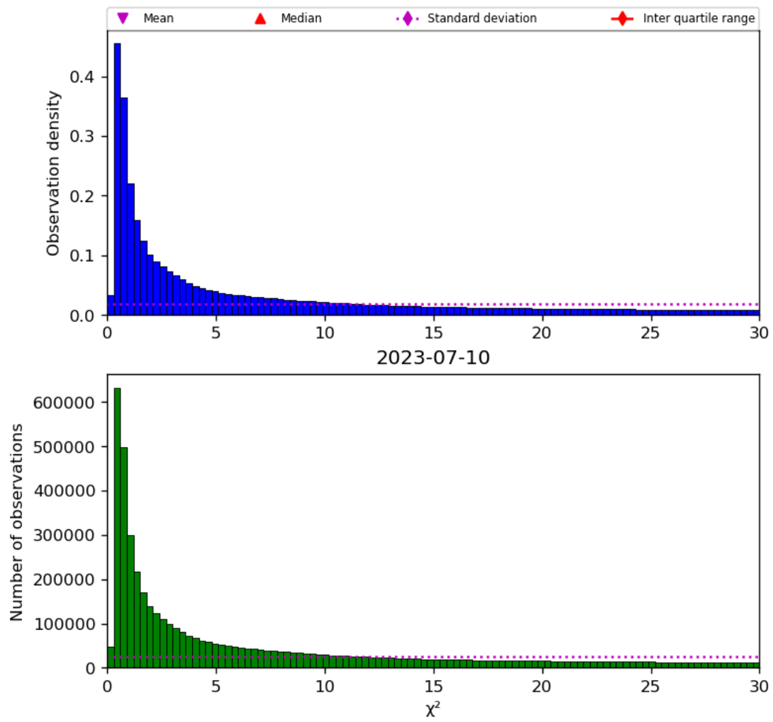
Figure 38: Histogram of “ \chi^2 ” for 2023-07-09 to 2023-07-11
