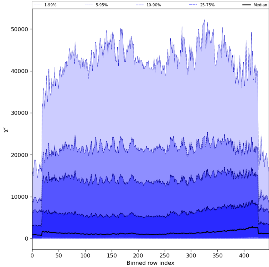
Figure 55: Along track statistics of “ \chi^2 ” for 2023-07-09 to 2023-07-11
