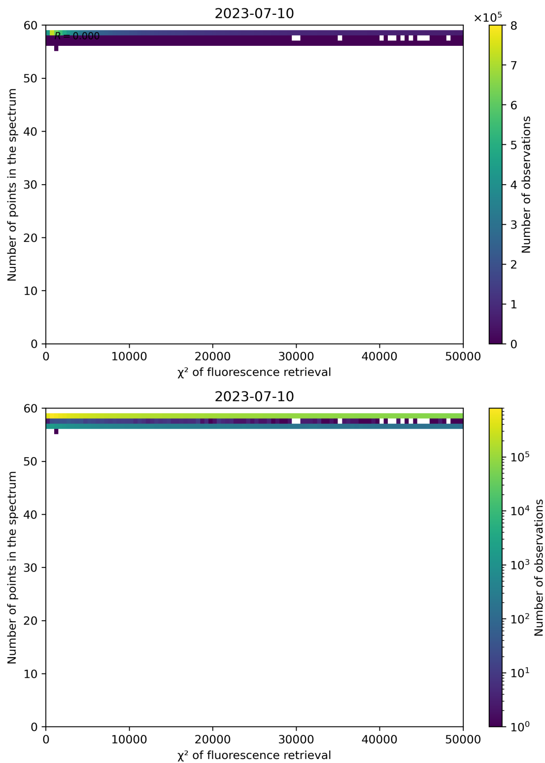
Figure 71: Scatter density plot of " \chi^2 of fluorescence retrieval" against "Number of points in the spectrum" for 2023-07-09 to 2023-07-11.
