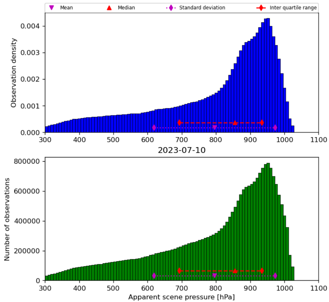
Figure 36: Histogram of “Apparent scene pressure” for 2023-07-09 to 2023-07-11
