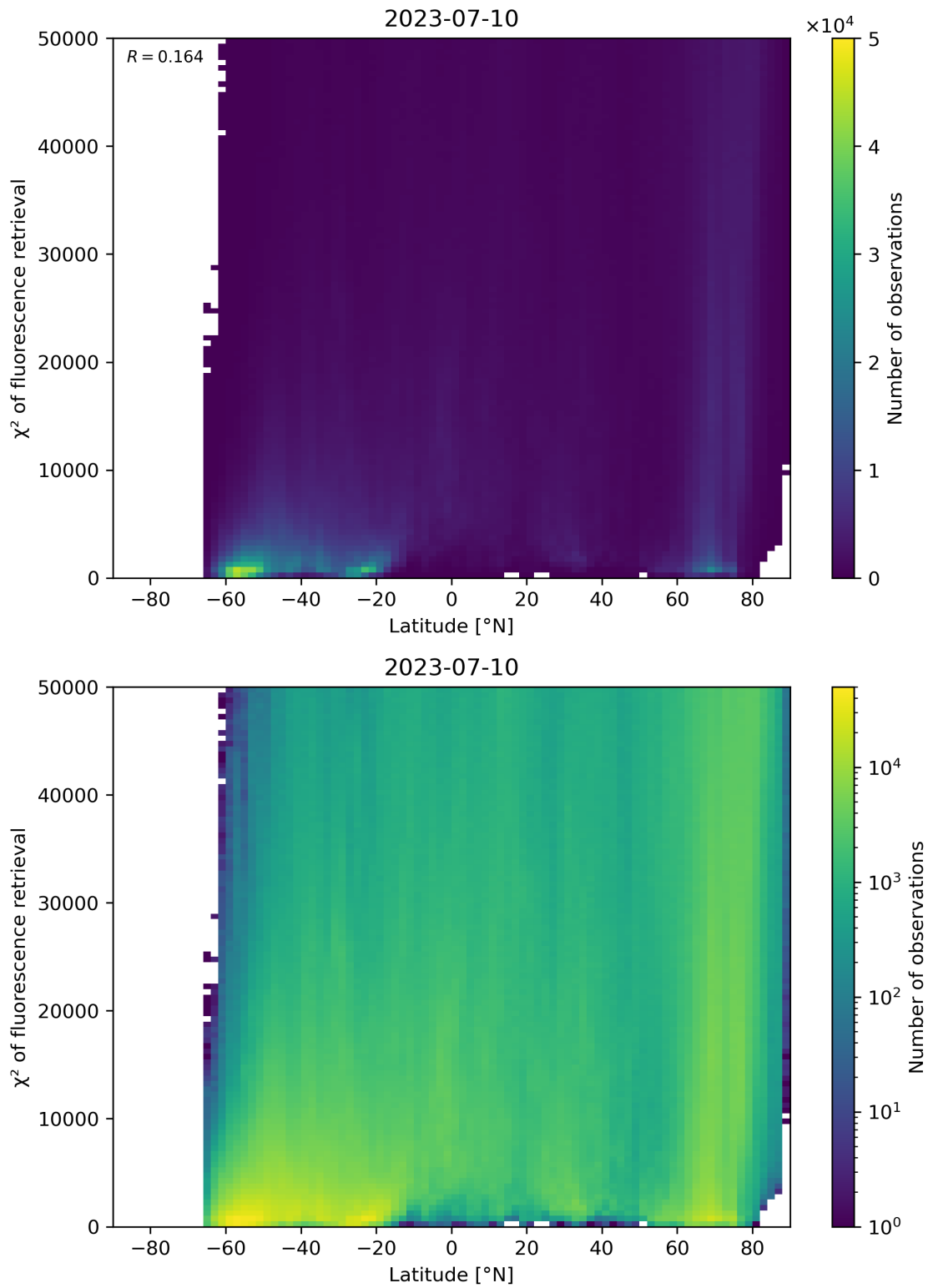
Figure 98: Scatter density plot of “Latitude” against “ \chi^2 of fluorescence retrieval” for 2023-07-09 to 2023-07-11.
