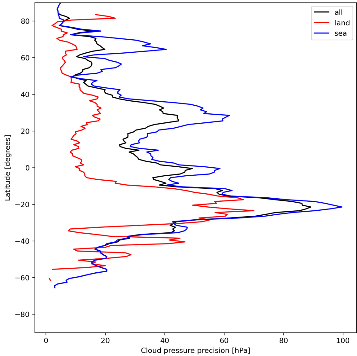
Figure 14: Zonal average of “Cloud pressure precision” for 2023-07-09 to 2023-07-11.
