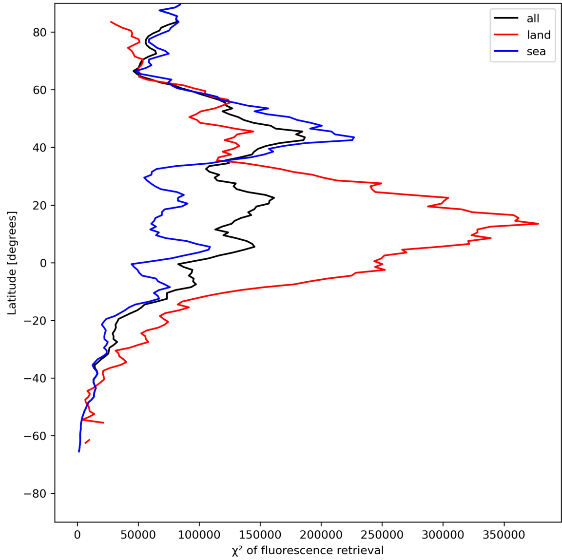
Figure 25: Zonal average of “ \chi^2 of fluorescence retrieval” for 2023-07-10 to 2023-07-12.
