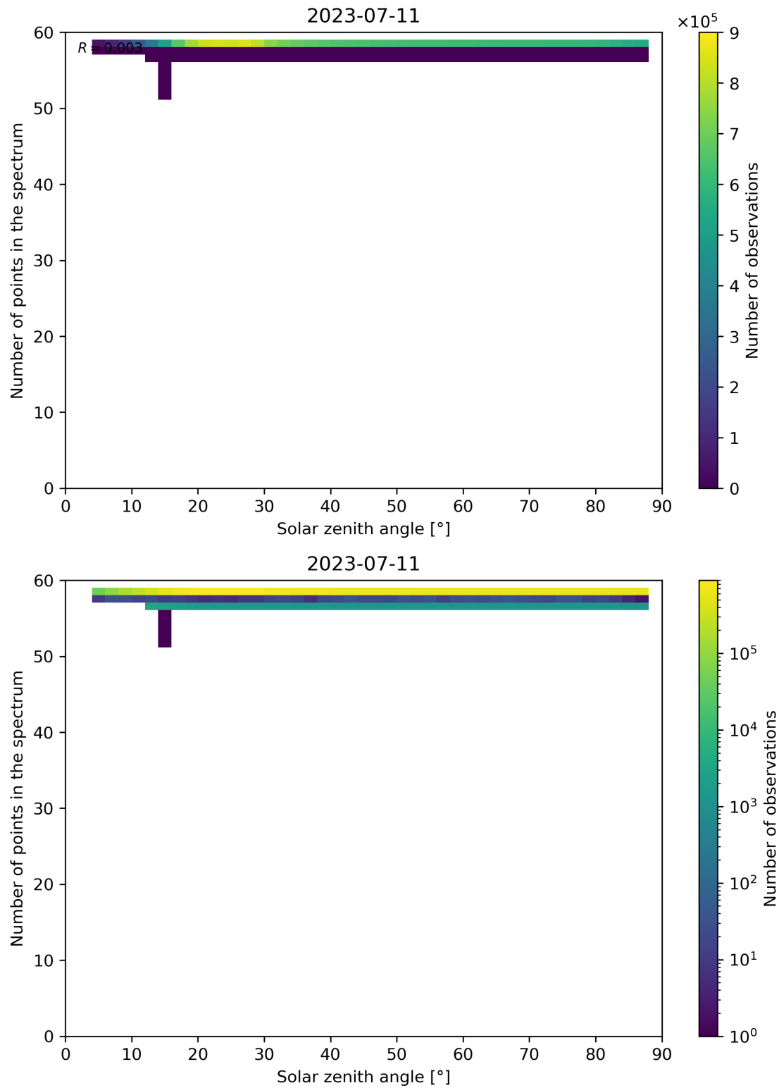
Figure 126: Scatter density plot of “Solar zenith angle” against “Number of points in the spectrum” for 2023-07-10 to 2023-07-12.
