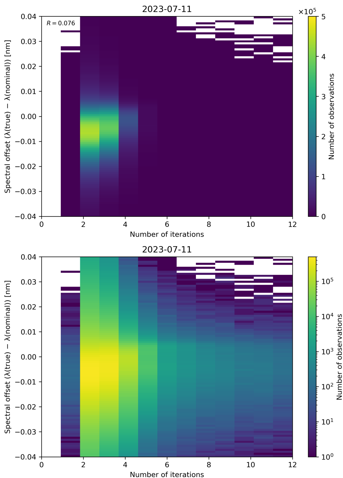
Figure 109: Scatter density plot of “Number of iterations” against “Spectral offset ( \lambda(\text{true}) - \lambda(\text{nominal}) )” for 2023-07-10 to 2023-07-12.
