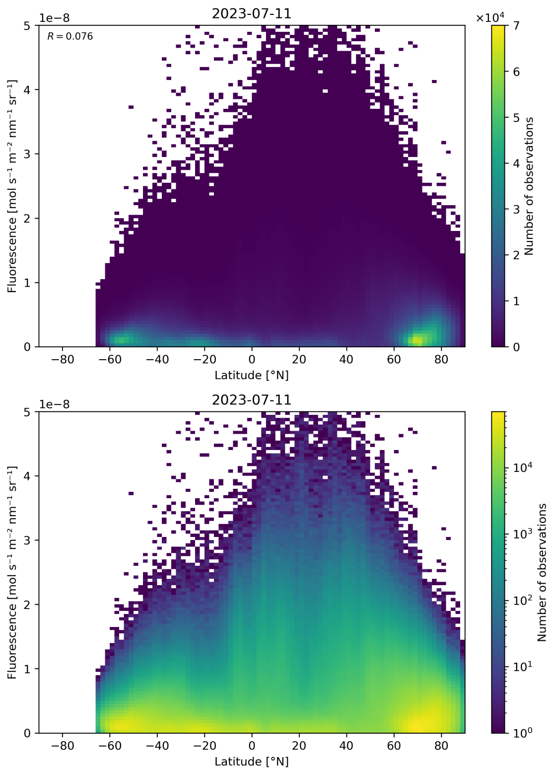
Figure 101: Scatter density plot of “Latitude” against “Fluorescence” for 2023-07-10 to 2023-07-12.
