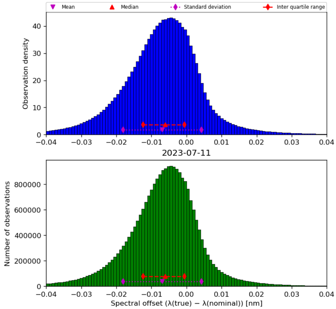
Figure 45: Histogram of “Spectral offset ( \lambda(\text{true}) - \lambda(\text{nominal}) )” for 2023-07-10 to 2023-07-12
