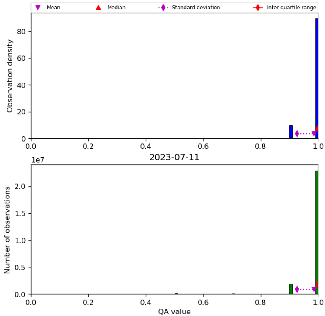
Figure 29: Histogram of “QA value” for 2023-07-10 to 2023-07-12
