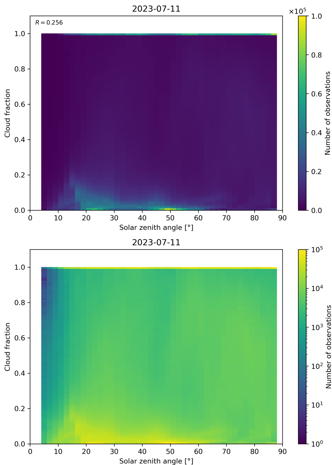
Figure 121: Scatter density plot of “Solar zenith angle” against “Cloud fraction” for 2023-07-10 to 2023-07-12.
