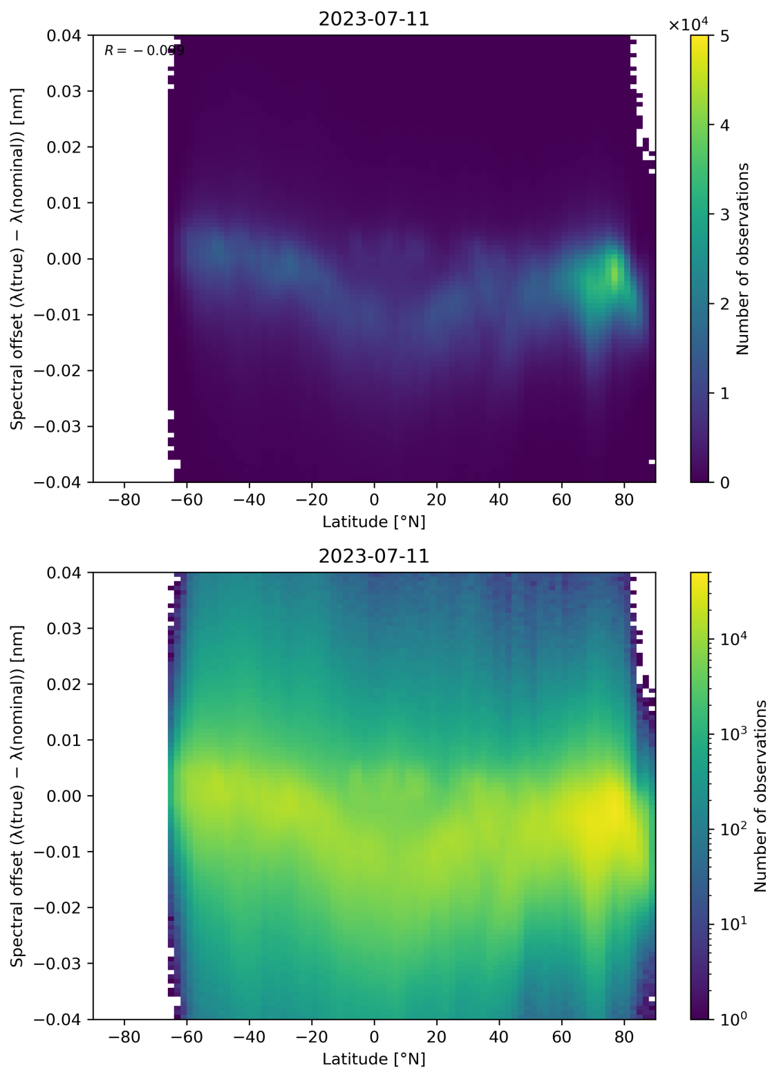
Figure 105: Scatter density plot of “Latitude” against “Spectral offset ( \lambda(\text{true}) - \lambda(\text{nominal}) )” for 2023-07-10 to 2023-07-12.
