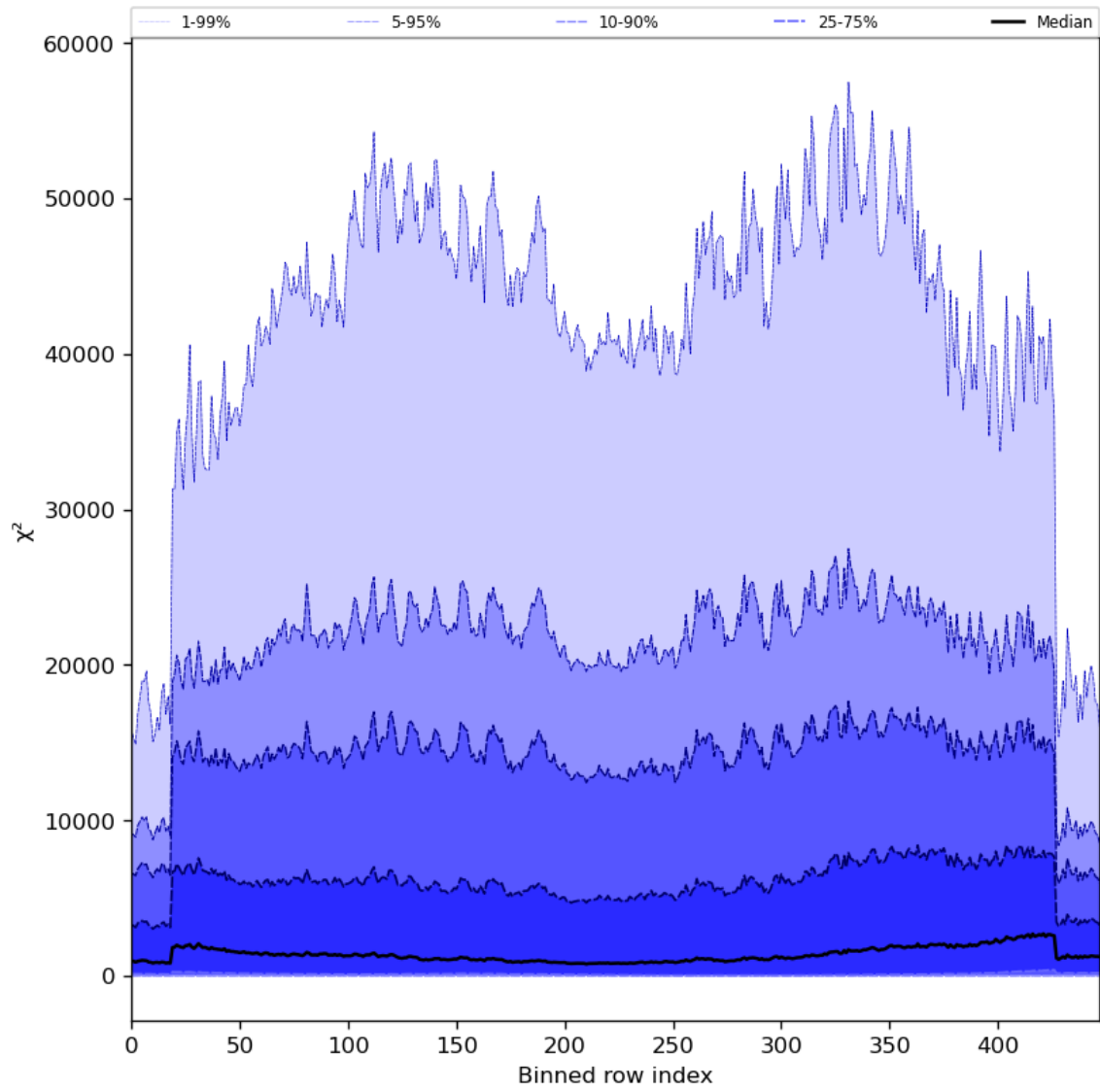
Figure 55: Along track statistics of “ \chi^2 ” for 2023-07-10 to 2023-07-12
