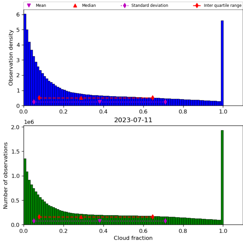
Figure 32: Histogram of “Cloud fraction” for 2023-07-10 to 2023-07-12
