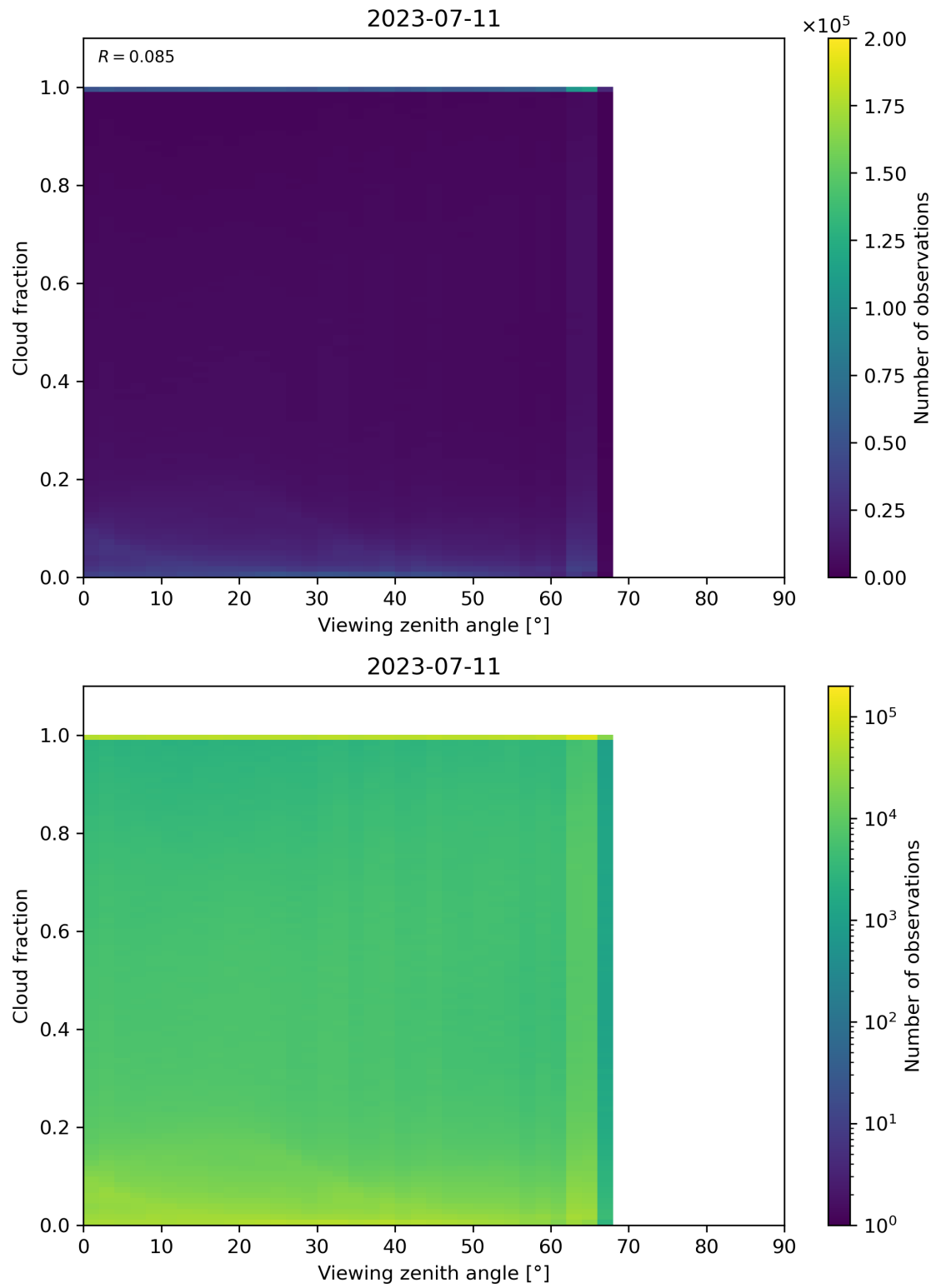
Figure 132: Scatter density plot of “Viewing zenith angle” against “Cloud fraction” for 2023-07-10 to 2023-07-12.
