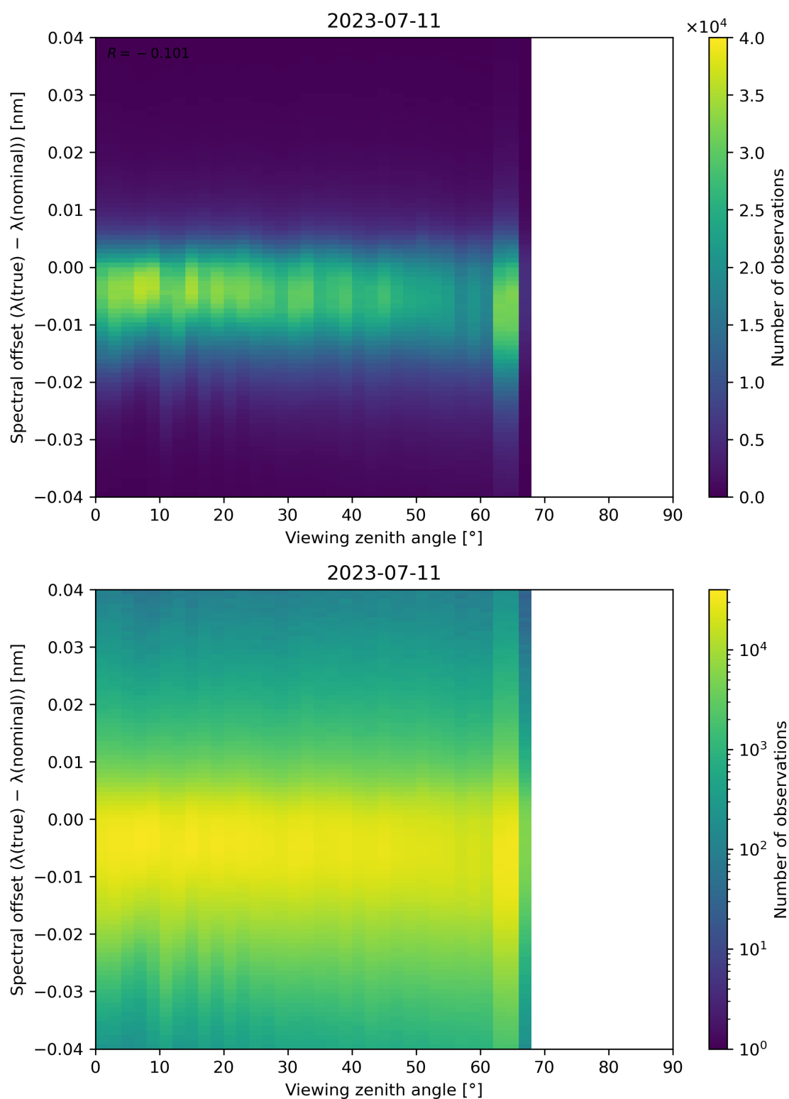
Figure 140: Scatter density plot of “Viewing zenith angle” against “Spectral offset ( \lambda(\text{true}) - \lambda(\text{nominal}) )” for 2023-07-10 to 2023-07-12.
