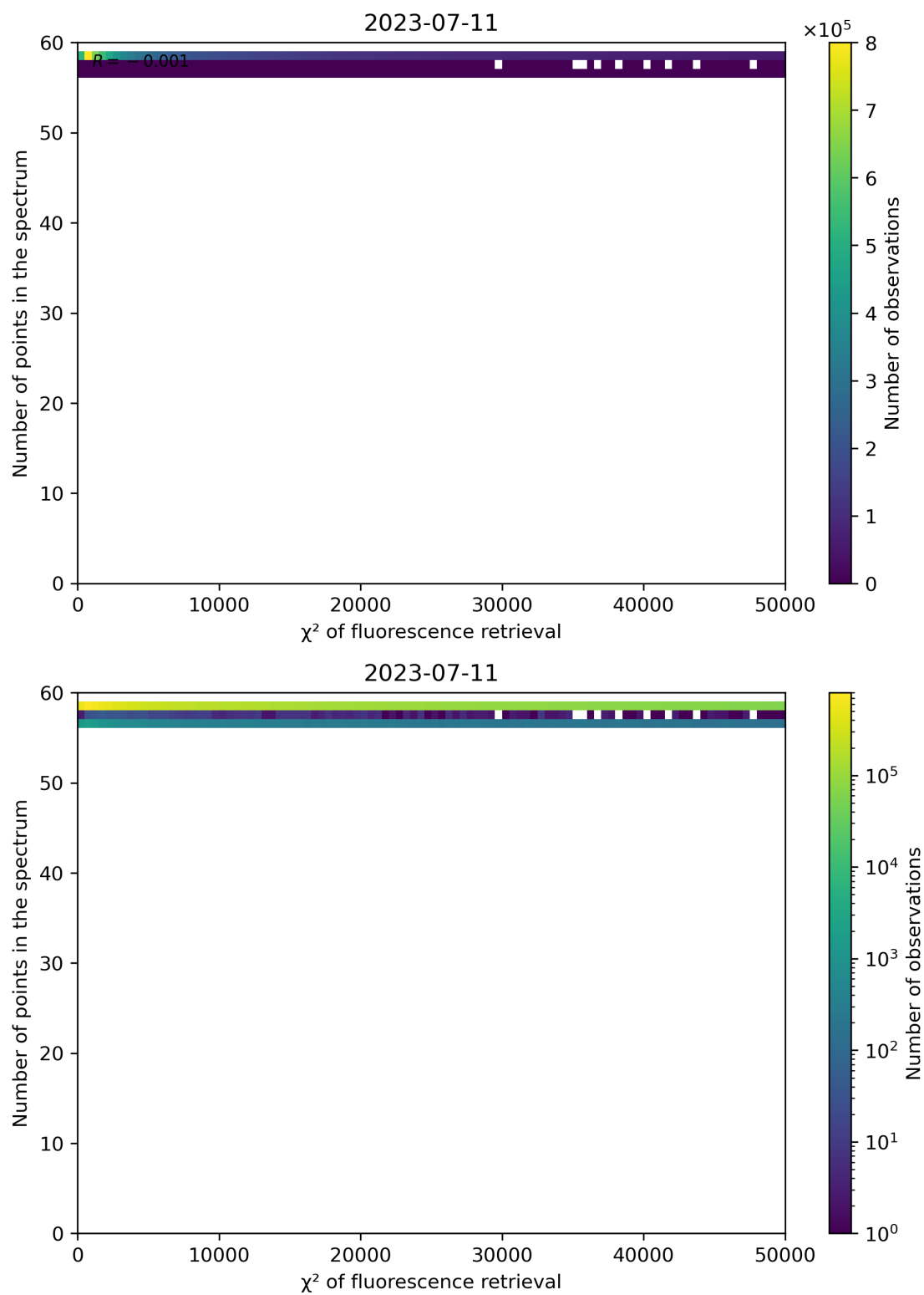
Figure 71: Scatter density plot of " \chi^2 of fluorescence retrieval" against "Number of points in the spectrum" for 2023-07-10 to 2023-07-12.
