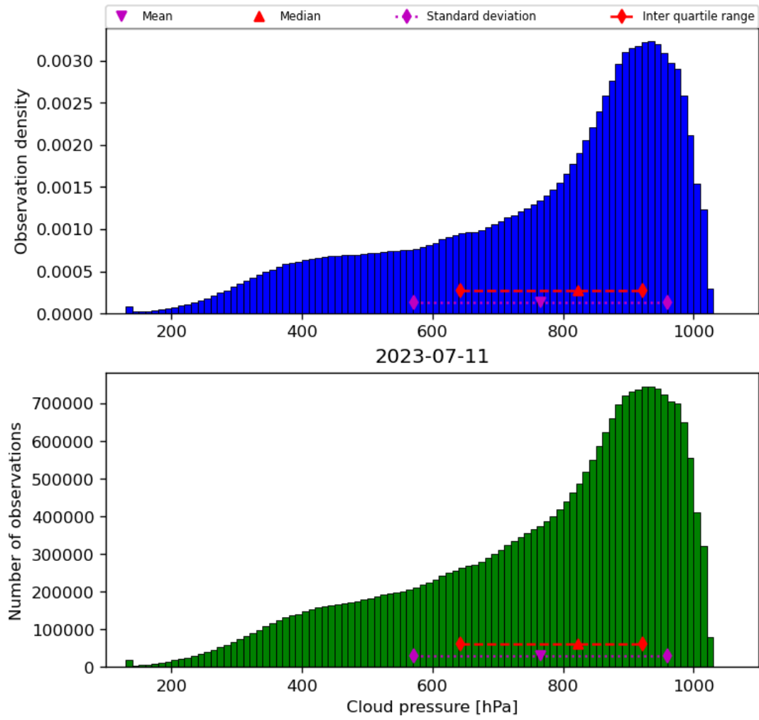
Figure 30: Histogram of “Cloud pressure” for 2023-07-10 to 2023-07-12
