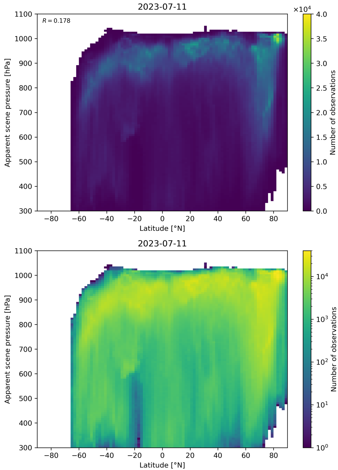
Figure 96: Scatter density plot of “Latitude” against “Apparent scene pressure” for 2023-07-10 to 2023-07-12.
