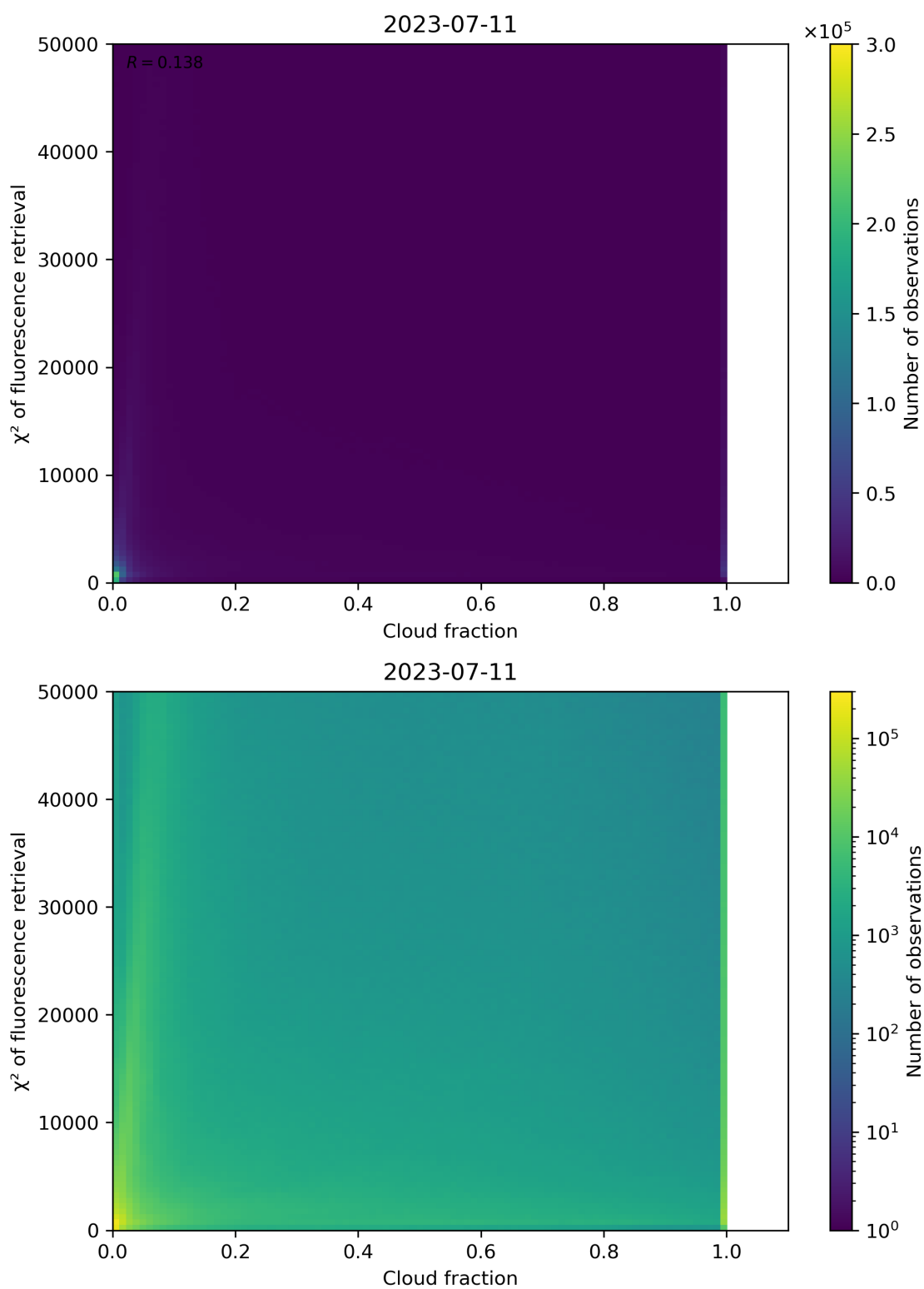
Figure 78: Scatter density plot of “Cloud fraction” against “ \chi^2 of fluorescence retrieval” for 2023-07-10 to 2023-07-12.
