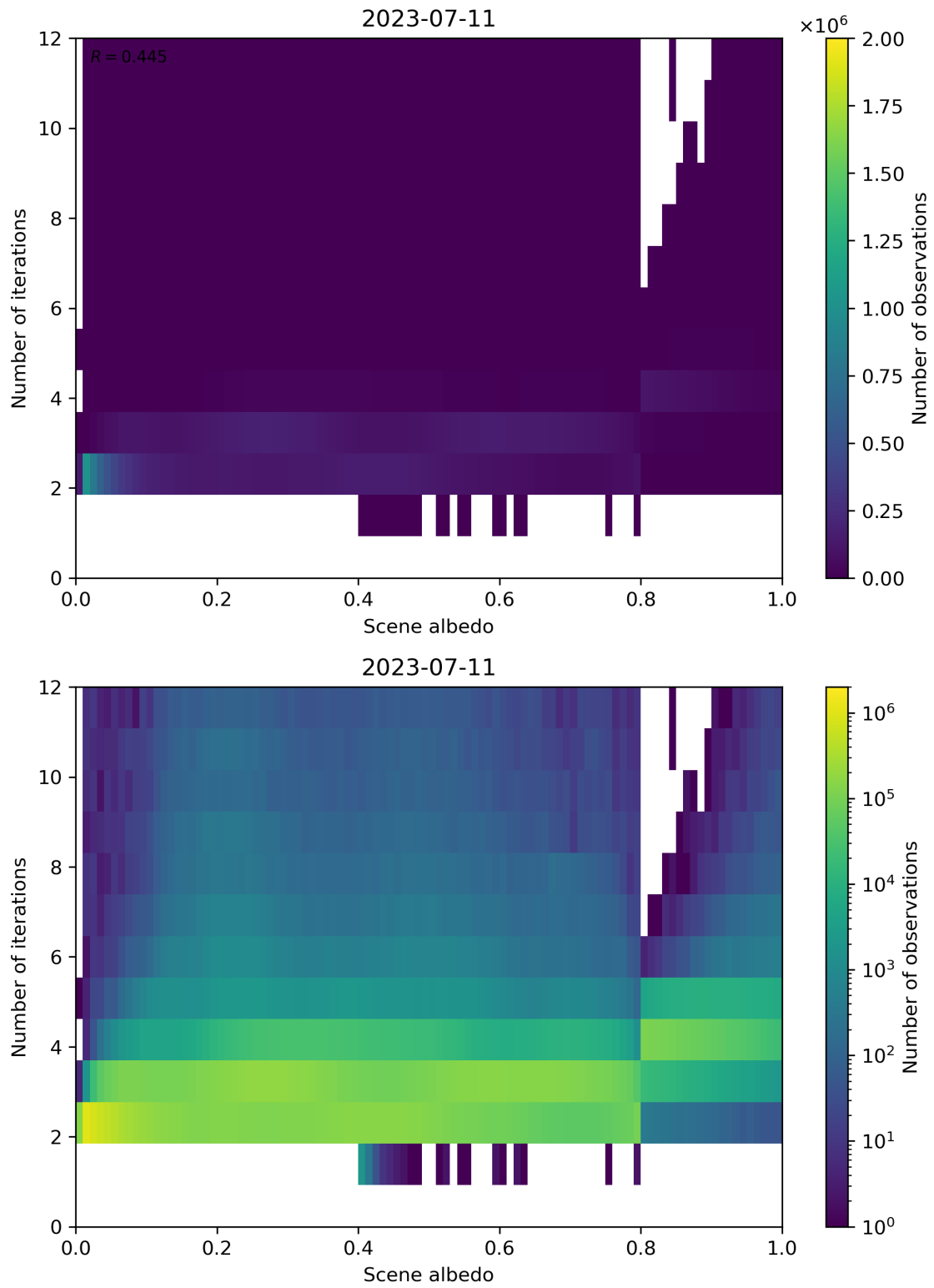
Figure 115: Scatter density plot of “Scene albedo” against “Number of iterations” for 2023-07-10 to 2023-07-12.
