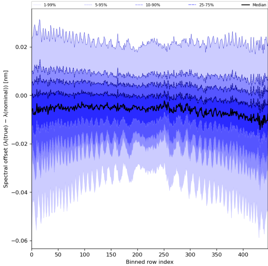
Figure 62: Along track statistics of “Spectral offset ( \lambda(\text{true}) - \lambda(\text{nominal}) )” for 2023-07-10 to 2023-07-12
