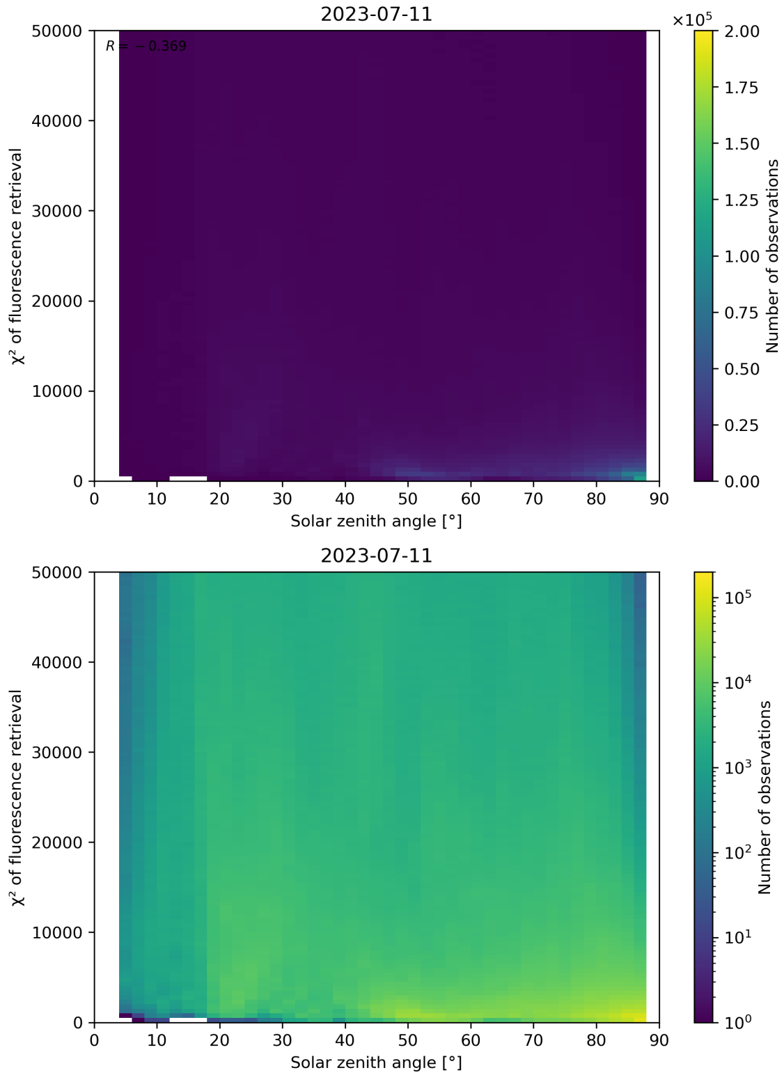
Figure 120: Scatter density plot of “Solar zenith angle” against “ \chi^2 of fluorescence retrieval” for 2023-07-10 to 2023-07-12.
