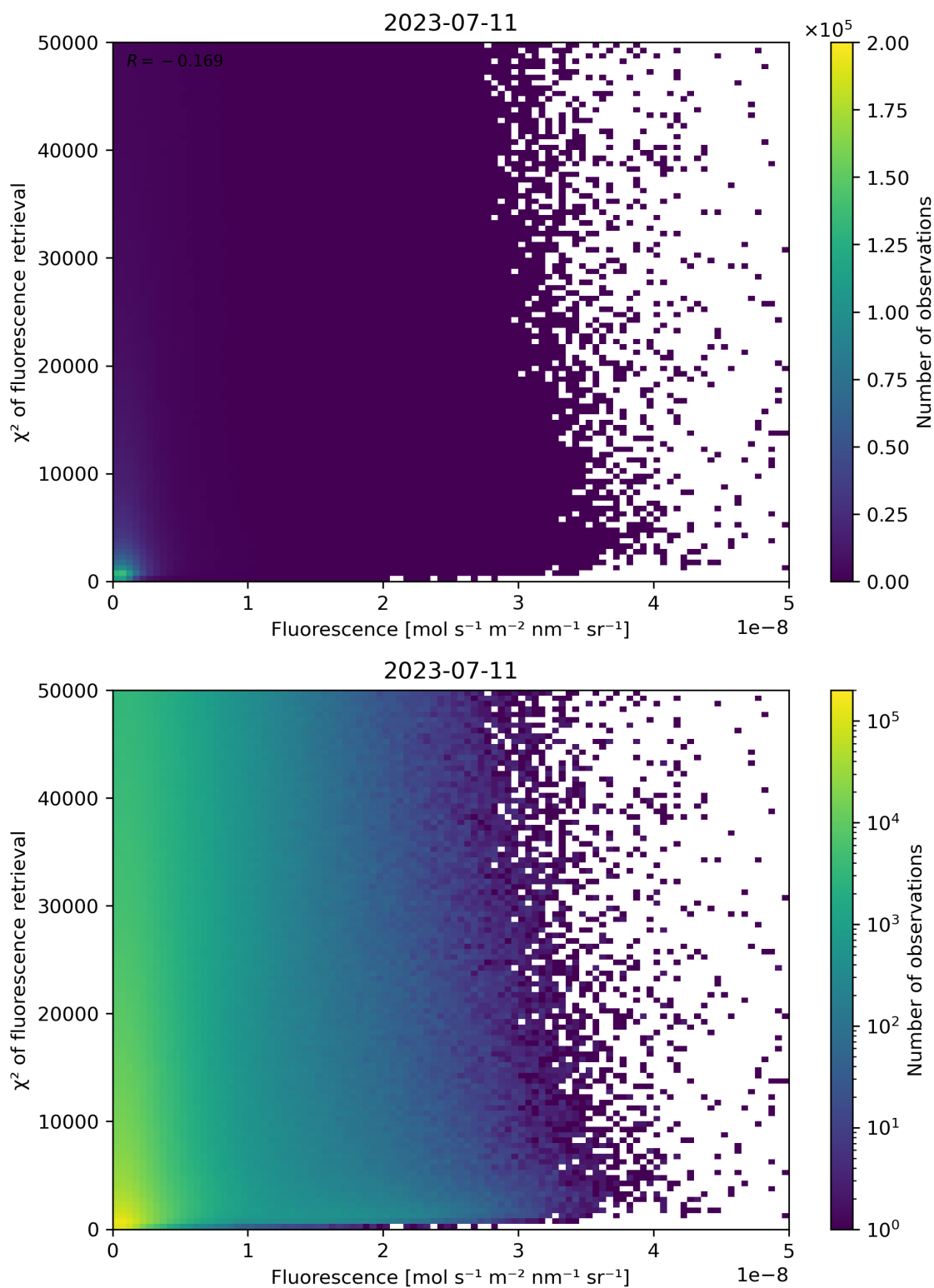
Figure 93: Scatter density plot of “Fluorescence” against “ \chi^2 of fluorescence retrieval” for 2023-07-10 to 2023-07-12.
