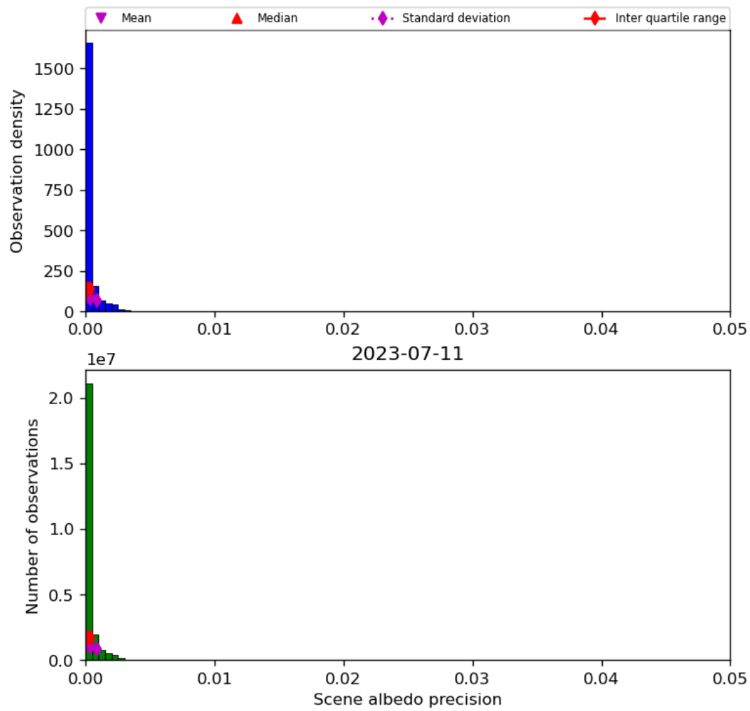
Figure 35: Histogram of “Scene albedo precision” for 2023-07-10 to 2023-07-12
