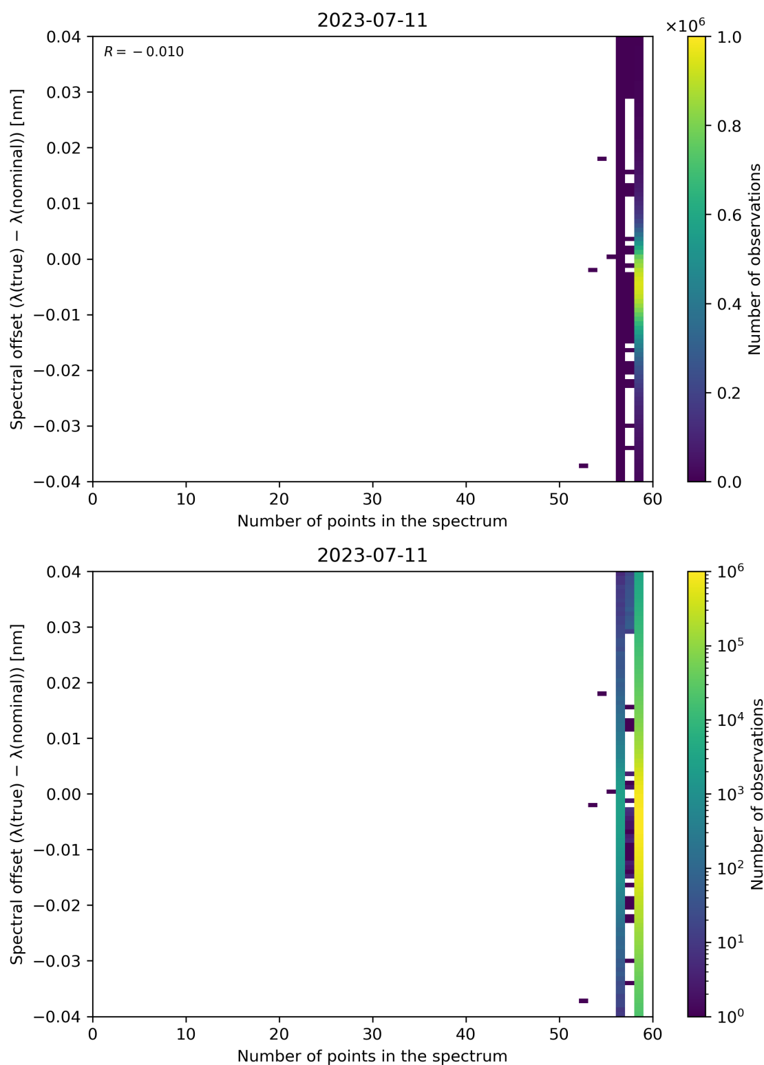
Figure 110: Scatter density plot of “Number of points in the spectrum” against “Spectral offset ( \lambda(\text{true}) - \lambda(\text{nominal}) )” for 2023-07-10 to 2023-07-12.
