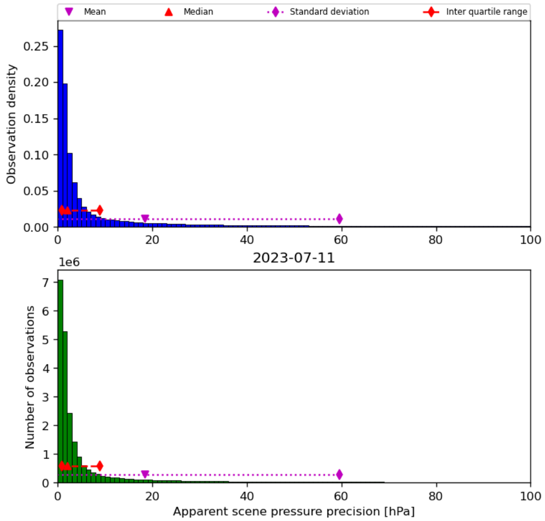
Figure 37: Histogram of “Apparent scene pressure precision” for 2023-07-10 to 2023-07-12
