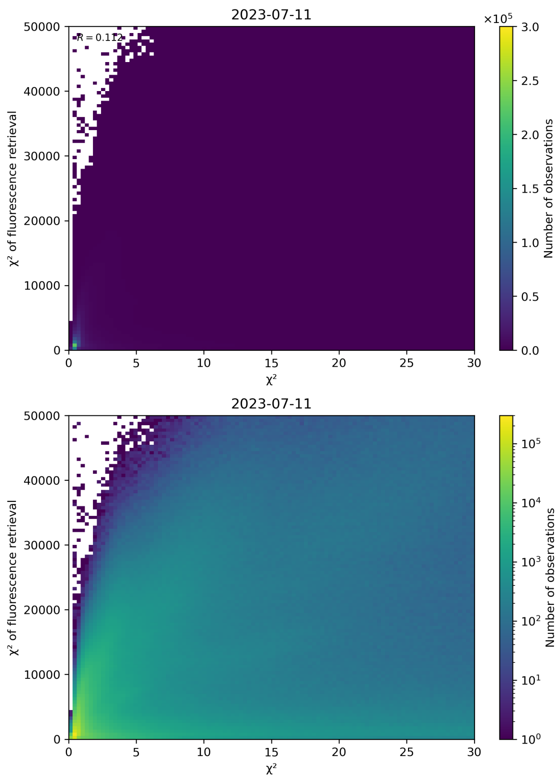
Figure 69: Scatter density plot of “ \chi^2 ” against “ \chi^2 of fluorescence retrieval” for 2023-07-10 to 2023-07-12.
