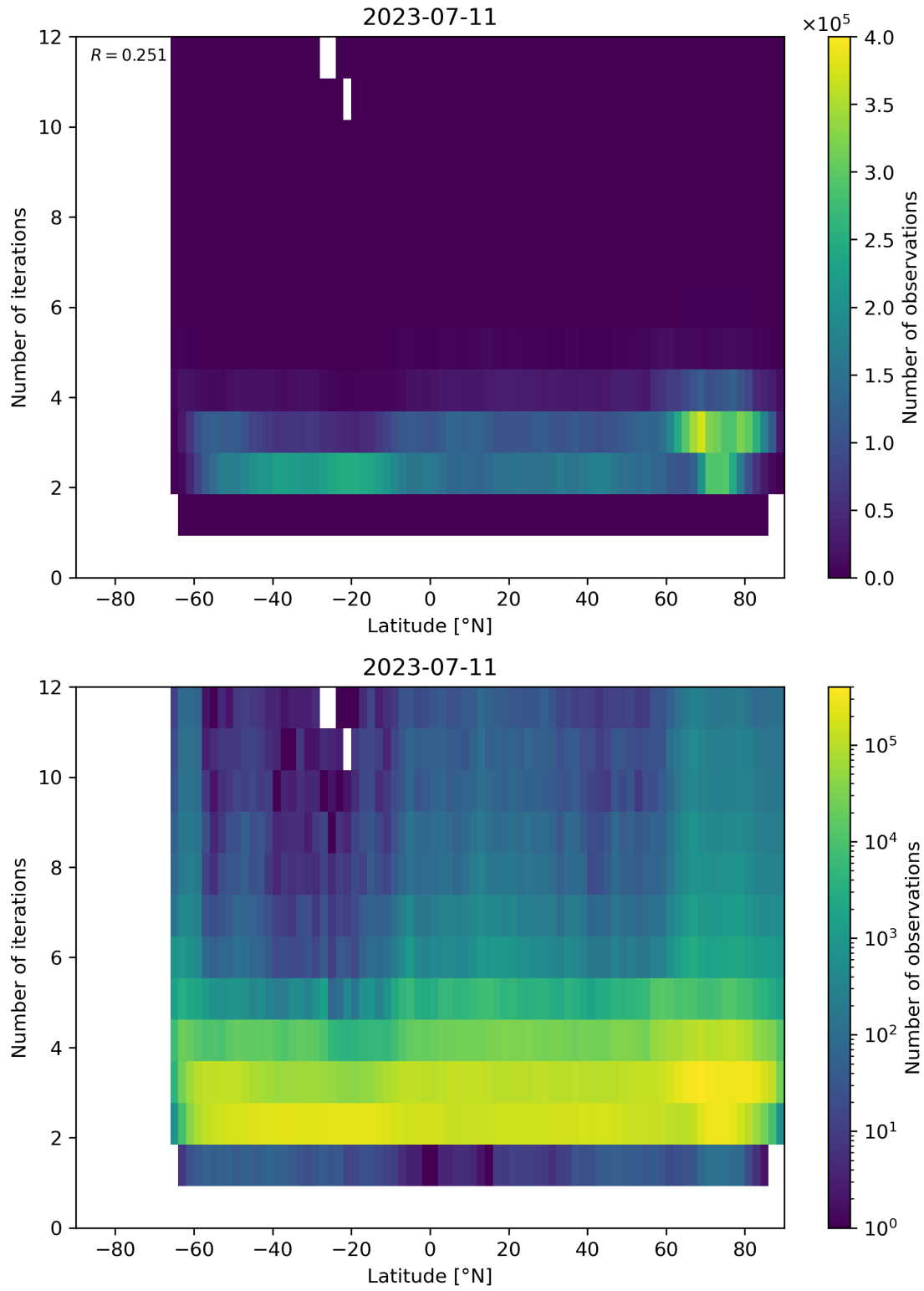
Figure 102: Scatter density plot of “Latitude” against “Number of iterations” for 2023-07-10 to 2023-07-12.
