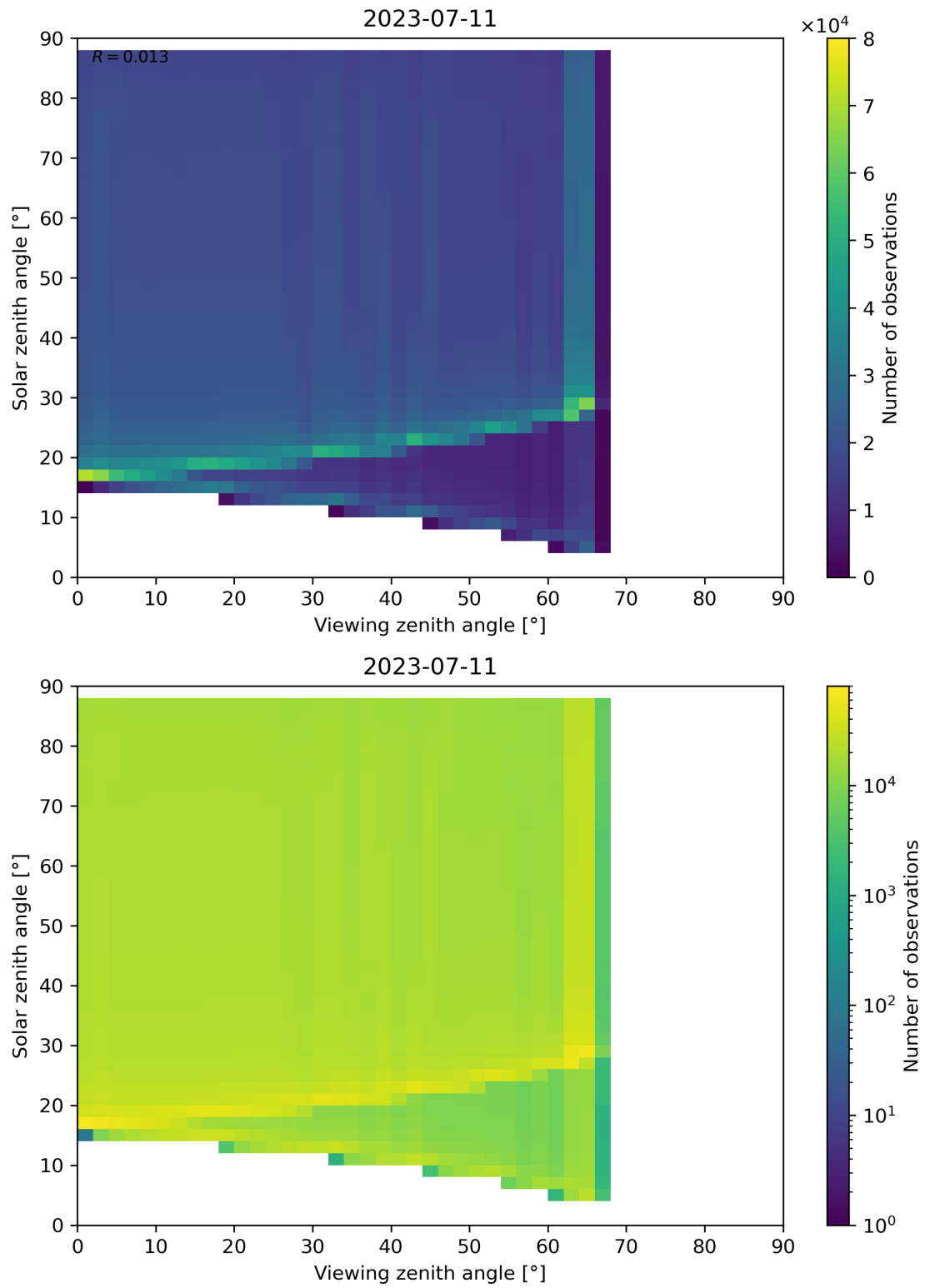
Figure 139: Scatter density plot of “Viewing zenith angle” against “Solar zenith angle” for 2023-07-10 to 2023-07-12.
