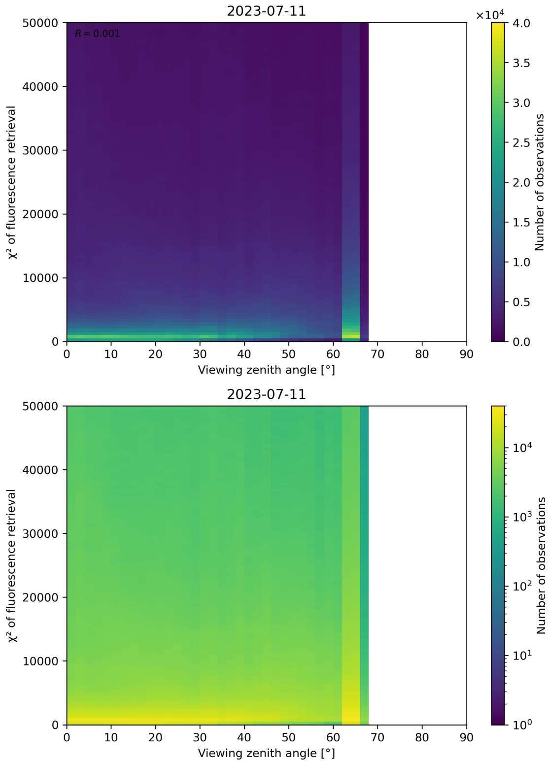
Figure 131: Scatter density plot of “Viewing zenith angle” against “ \chi^2 of fluorescence retrieval” for 2023-07-10 to 2023-07-12.
