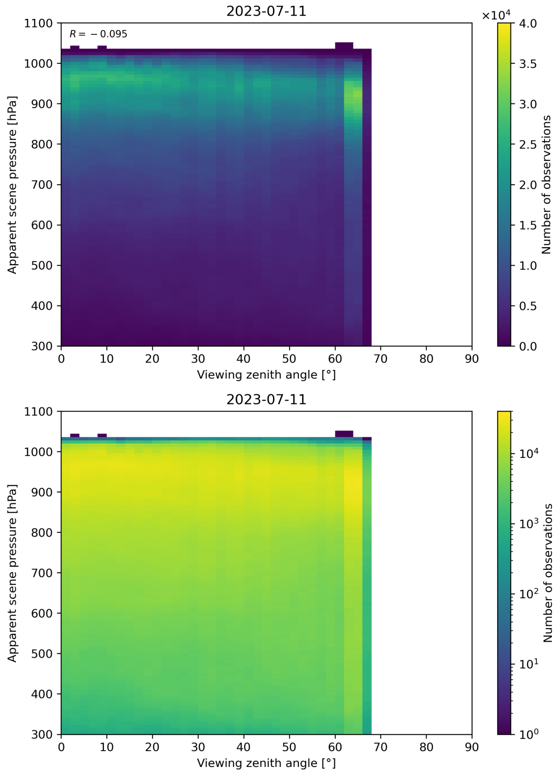
Figure 129: Scatter density plot of “Viewing zenith angle” against “Apparent scene pressure” for 2023-07-10 to 2023-07-12.
