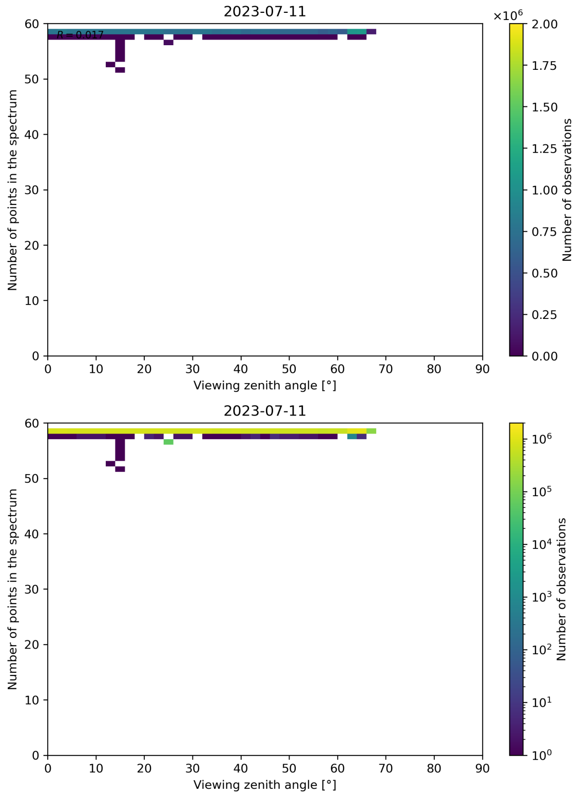
Figure 137: Scatter density plot of “Viewing zenith angle” against “Number of points in the spectrum” for 2023-07-10 to 2023-07-12.
