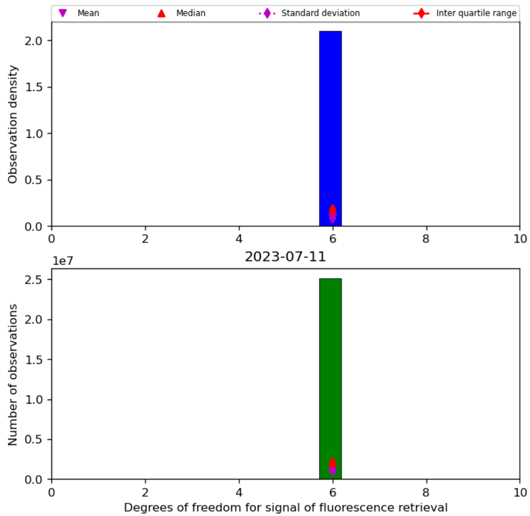
Figure 43: Histogram of “Degrees of freedom for signal of fluorescence retrieval” for 2023-07-10 to 2023-07-12
