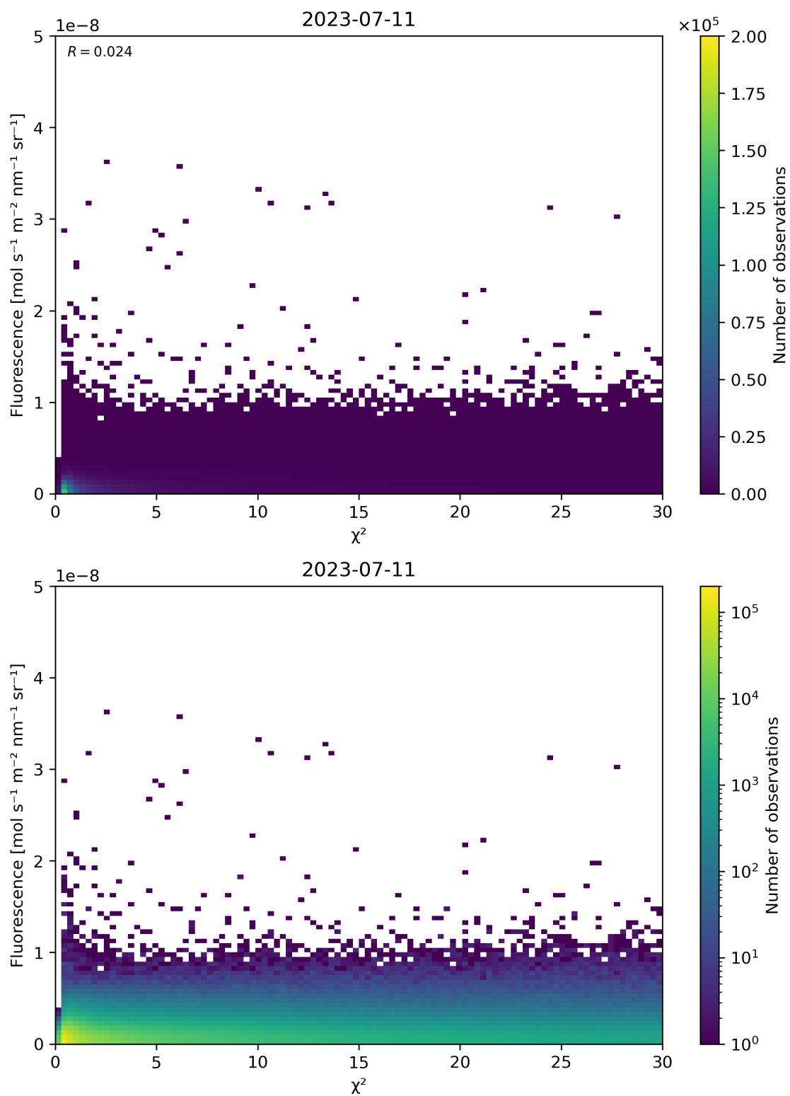
Figure 70: Scatter density plot of “ \chi^2 ” against “Fluorescence” for 2023-07-10 to 2023-07-12.
