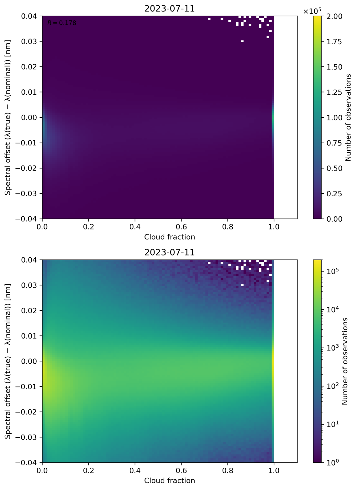
Figure 83: Scatter density plot of “Cloud fraction” against “Spectral offset ( \lambda(\text{true}) - \lambda(\text{nominal}) )” for 2023-07-10 to 2023-07-12.
