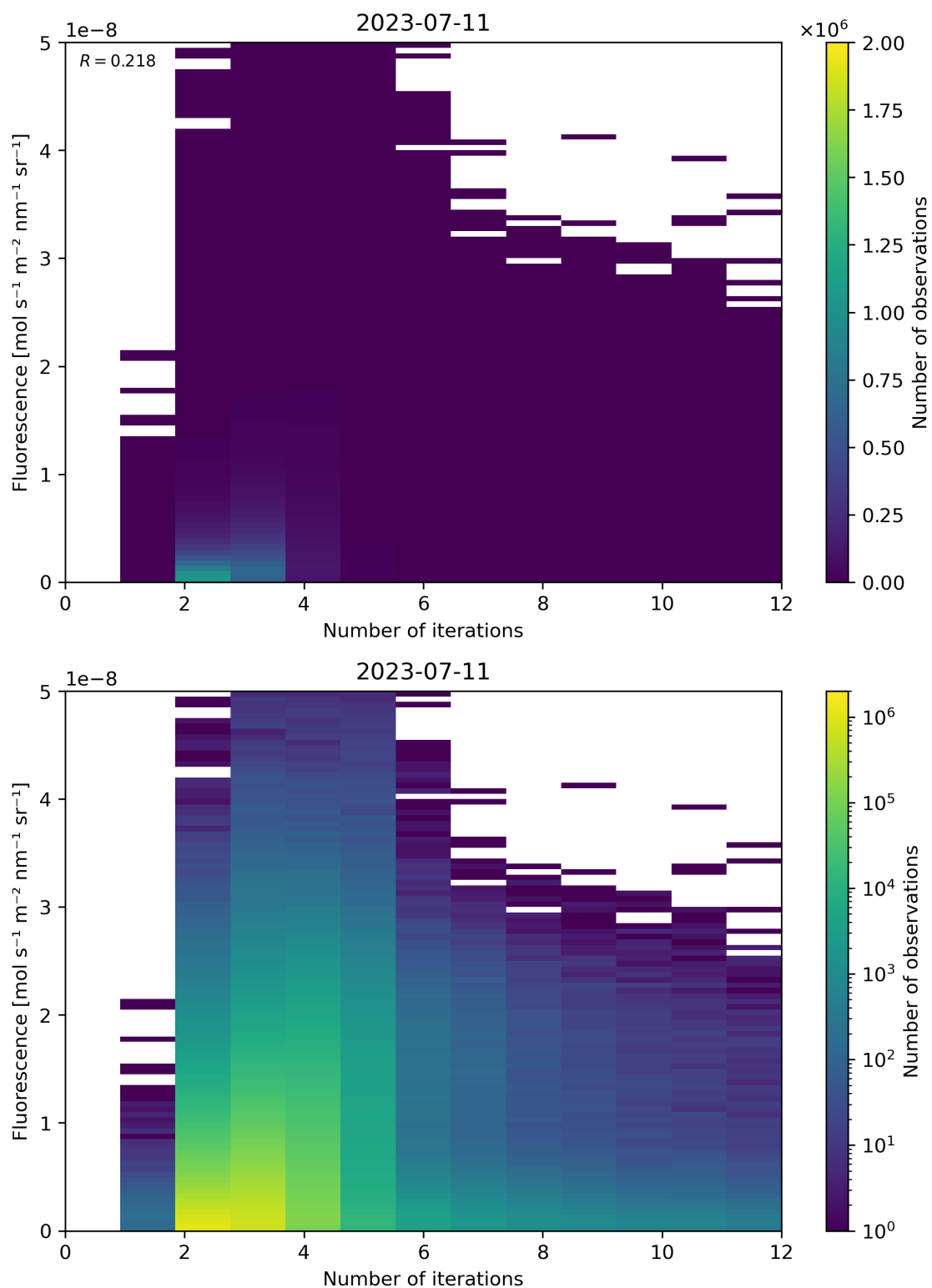
Figure 107: Scatter density plot of “Number of iterations” against “Fluorescence” for 2023-07-10 to 2023-07-12.
