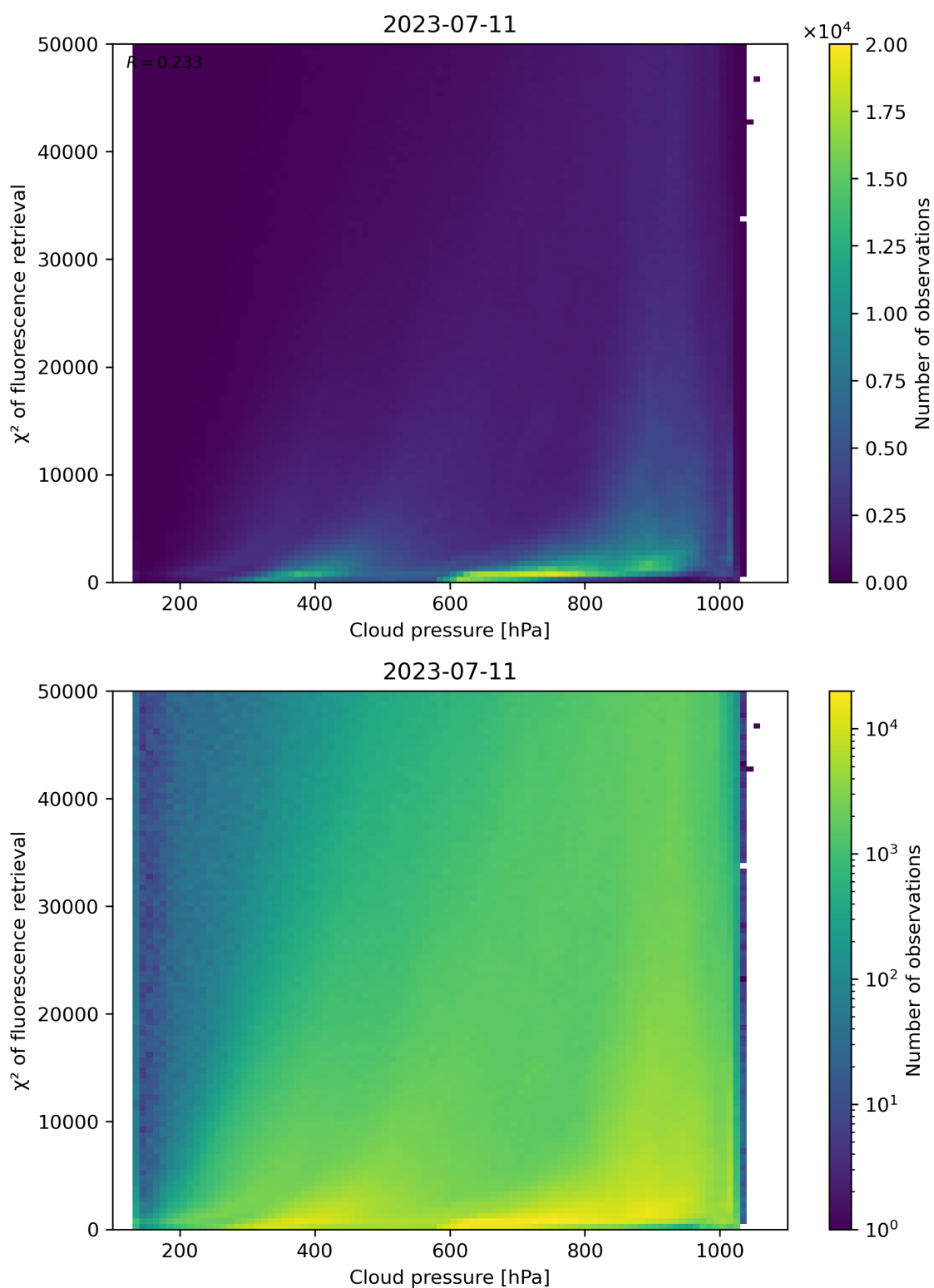
Figure 86: Scatter density plot of “Cloud pressure” against “ \chi^2 of fluorescence retrieval” for 2023-07-10 to 2023-07-12.
