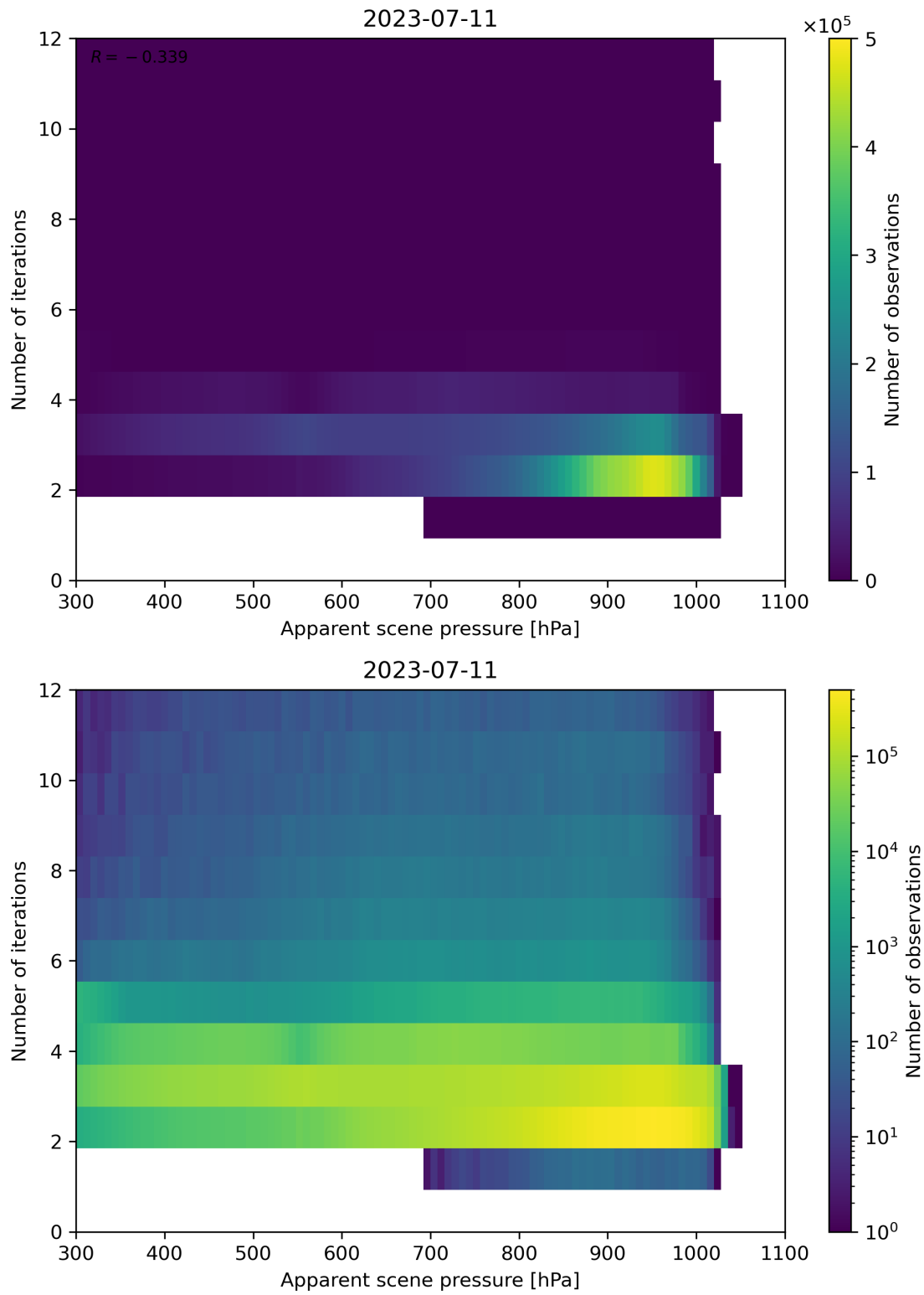
Figure 66: Scatter density plot of “Apparent scene pressure” against “Number of iterations” for 2023-07-10 to 2023-07-12.
