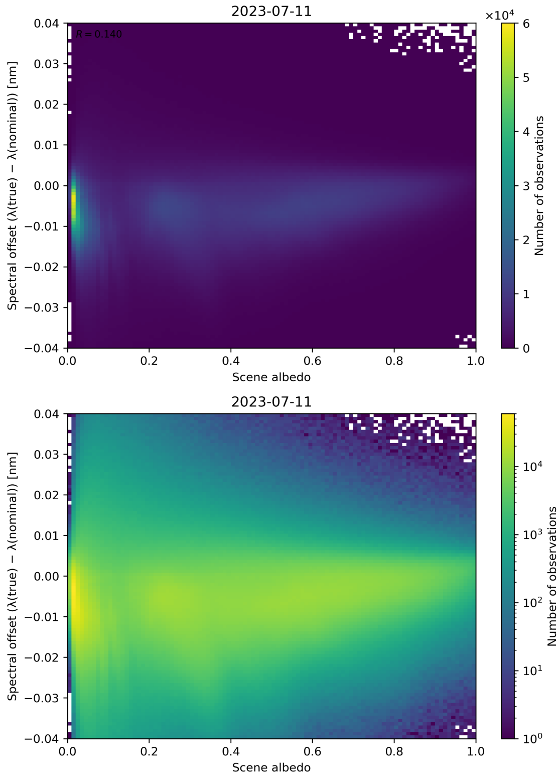
Figure 117: Scatter density plot of “Scene albedo” against “Spectral offset ( \lambda(\text{true}) - \lambda(\text{nominal}) )” for 2023-07-10 to 2023-07-12.
