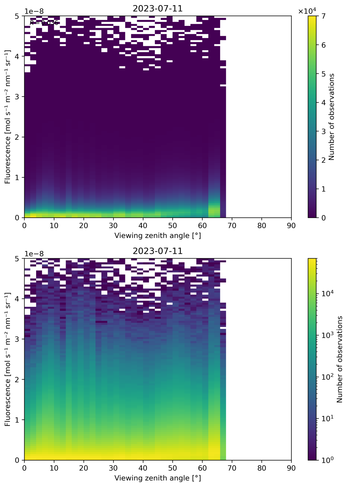
Figure 134: Scatter density plot of “Viewing zenith angle” against “Fluorescence” for 2023-07-10 to 2023-07-12.
