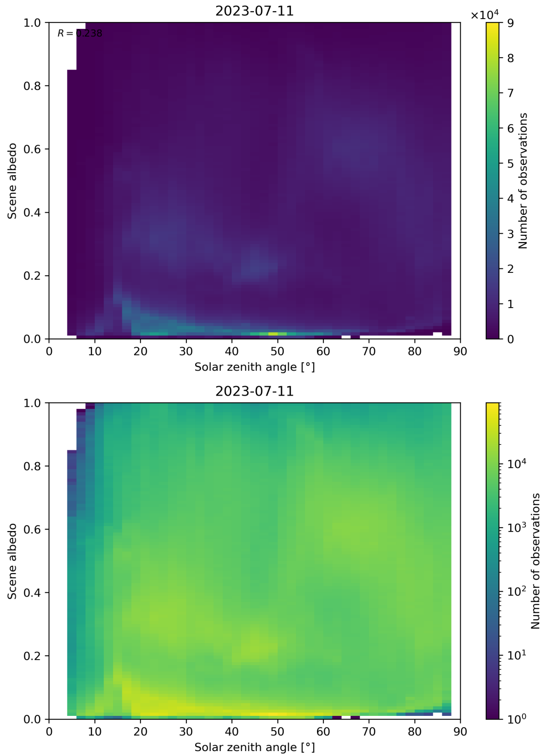
Figure 127: Scatter density plot of “Solar zenith angle” against “Scene albedo” for 2023-07-10 to 2023-07-12.
