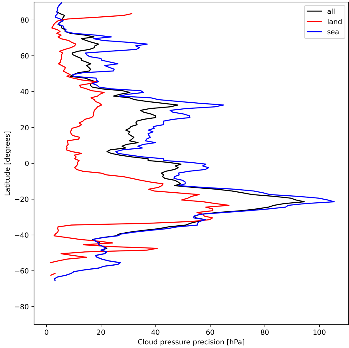
Figure 14: Zonal average of "Cloud pressure precision" for 2023-07-10 to 2023-07-12.
