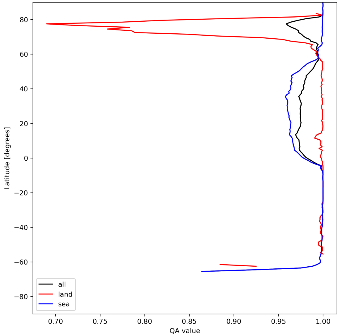
Figure 12: Zonal average of “QA value” for 2023-07-10 to 2023-07-12.
