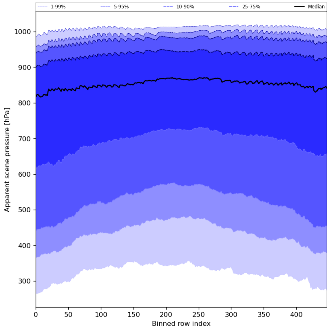
Figure 53: Along track statistics of “Apparent scene pressure” for 2023-07-10 to 2023-07-12
