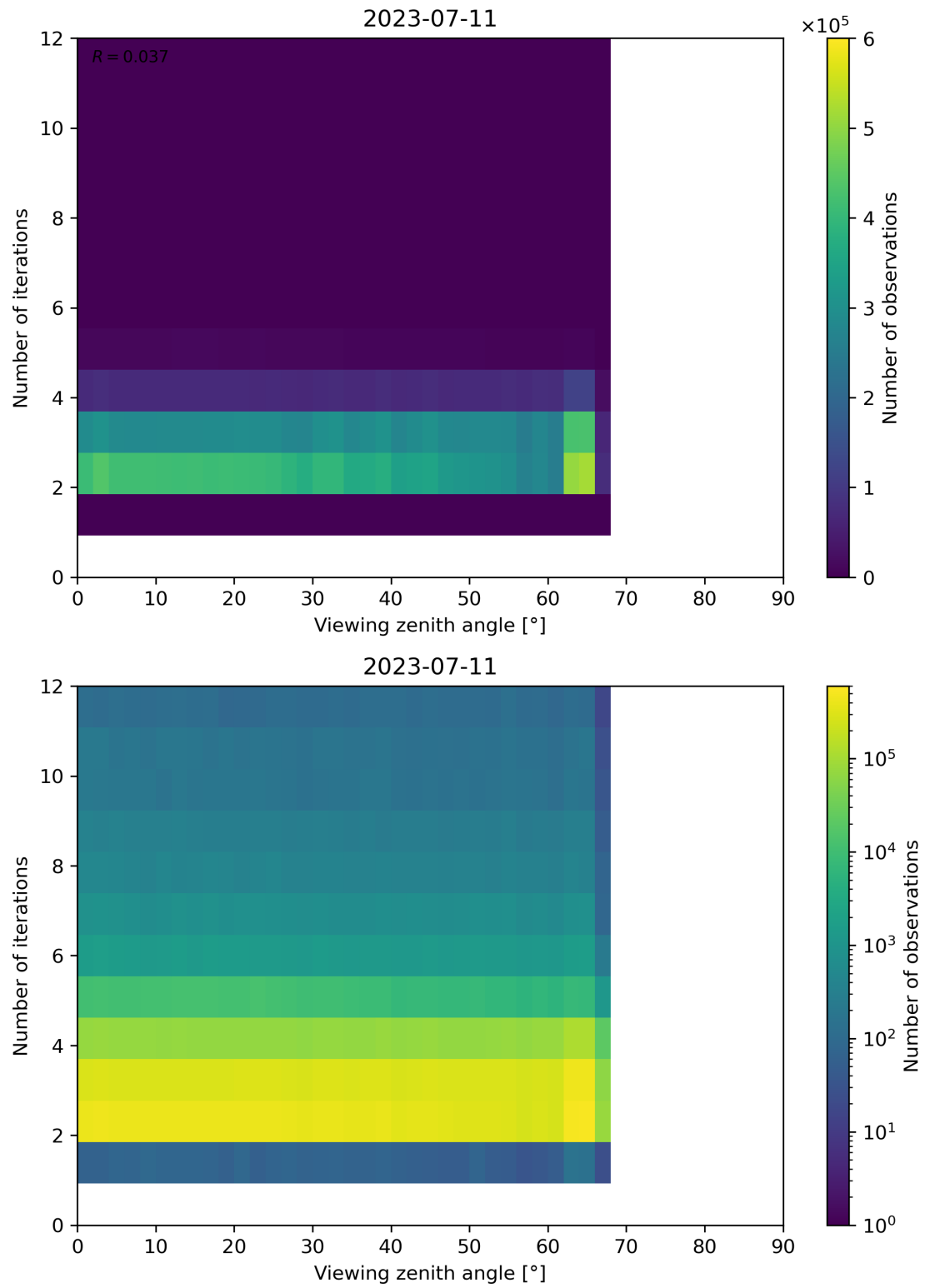
Figure 136: Scatter density plot of “Viewing zenith angle” against “Number of iterations” for 2023-07-10 to 2023-07-12.
