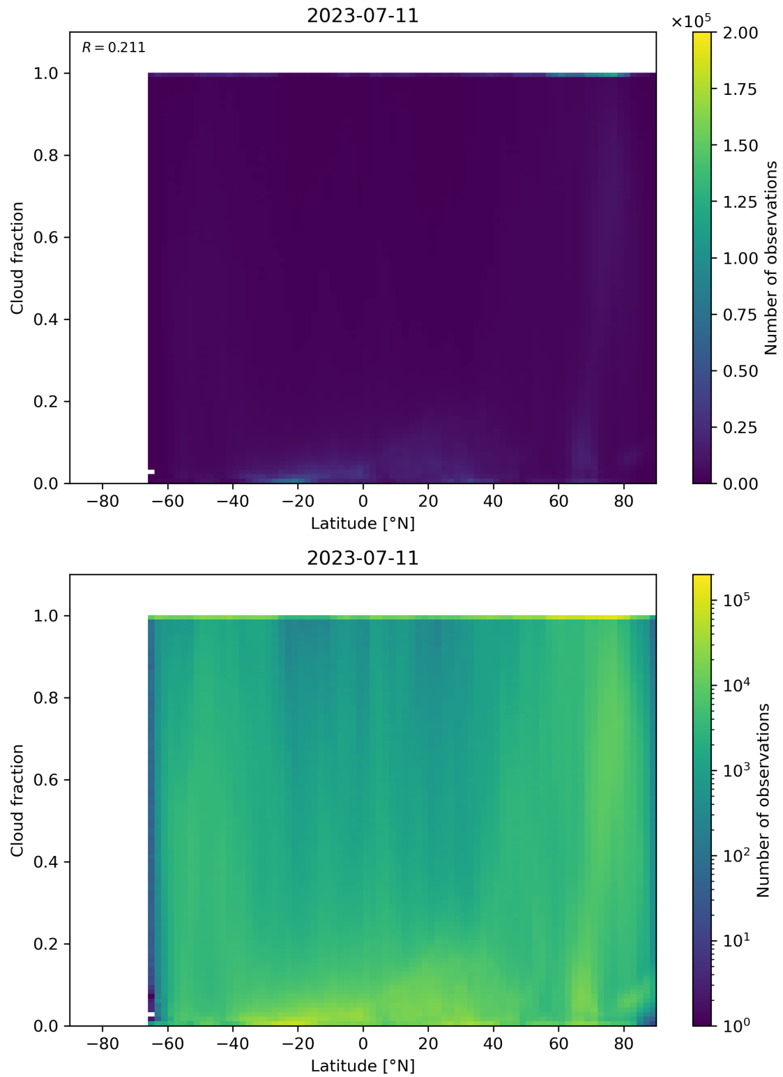
Figure 99: Scatter density plot of “Latitude” against “Cloud fraction” for 2023-07-10 to 2023-07-12.
