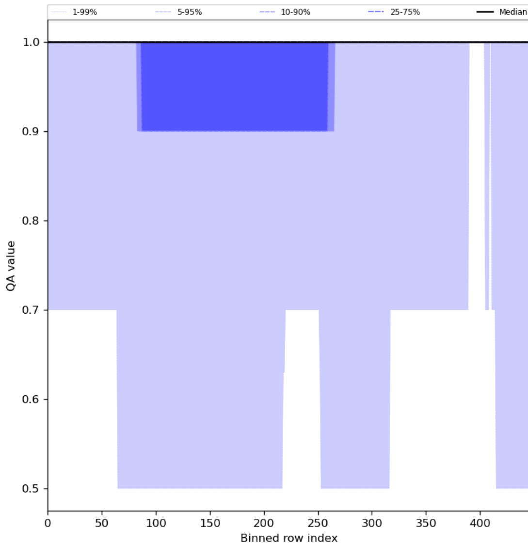
Figure 46: Along track statistics of “QA value” for 2023-07-10 to 2023-07-12
