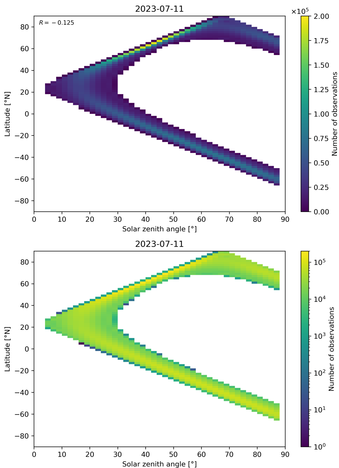
Figure 124: Scatter density plot of “Solar zenith angle” against “Latitude” for 2023-07-10 to 2023-07-12.
