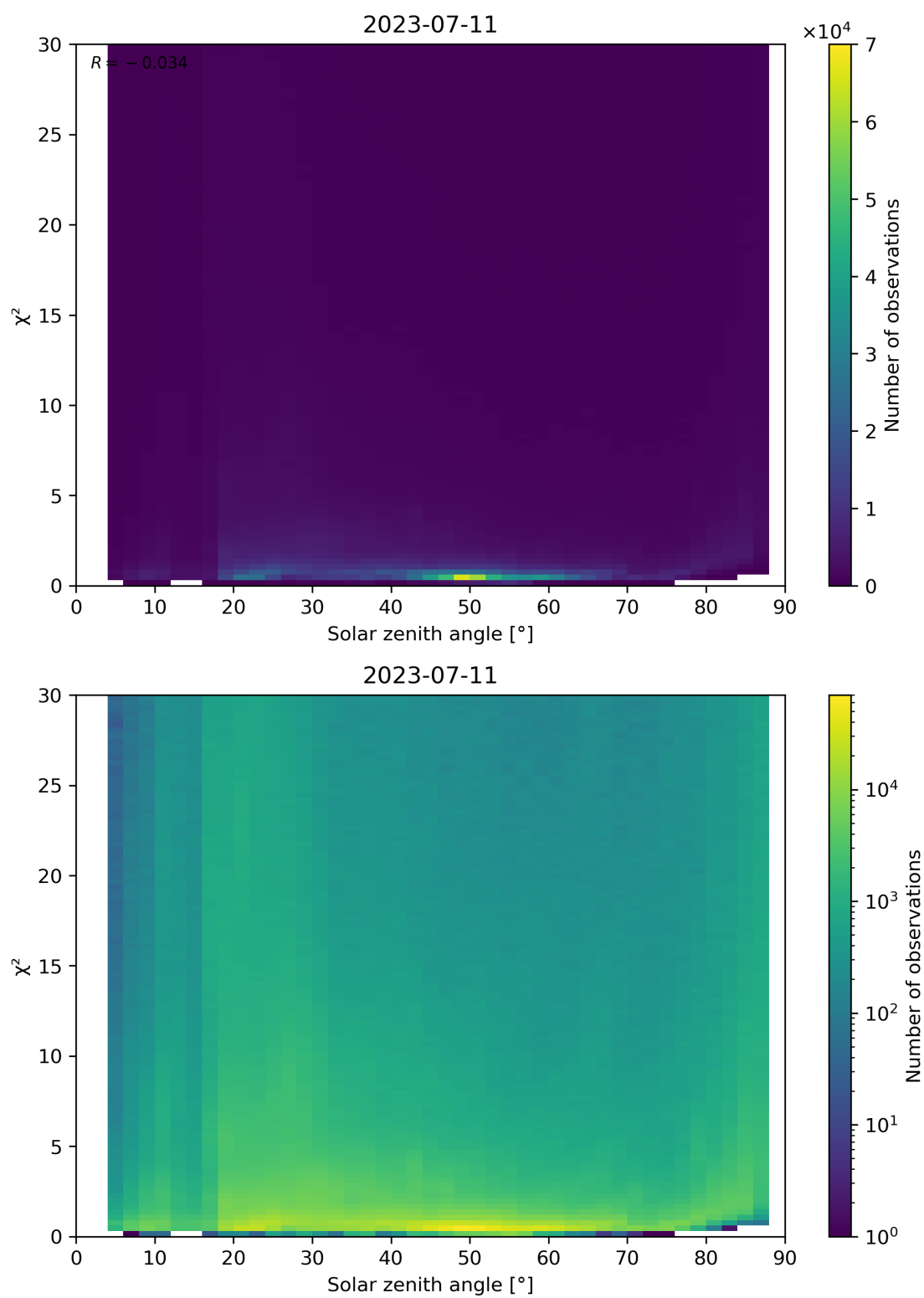
Figure 119: Scatter density plot of “Solar zenith angle” against “ \chi^2 ” for 2023-07-10 to 2023-07-12.
