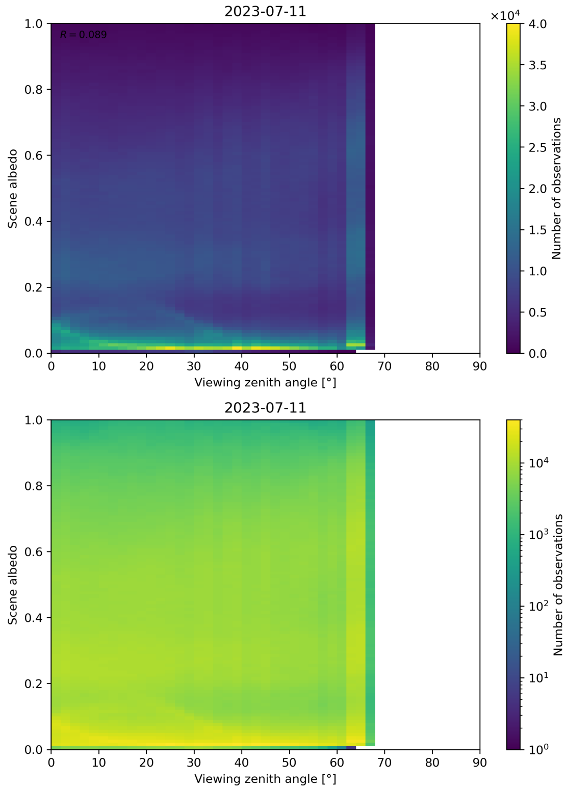
Figure 138: Scatter density plot of “Viewing zenith angle” against “Scene albedo” for 2023-07-10 to 2023-07-12.
