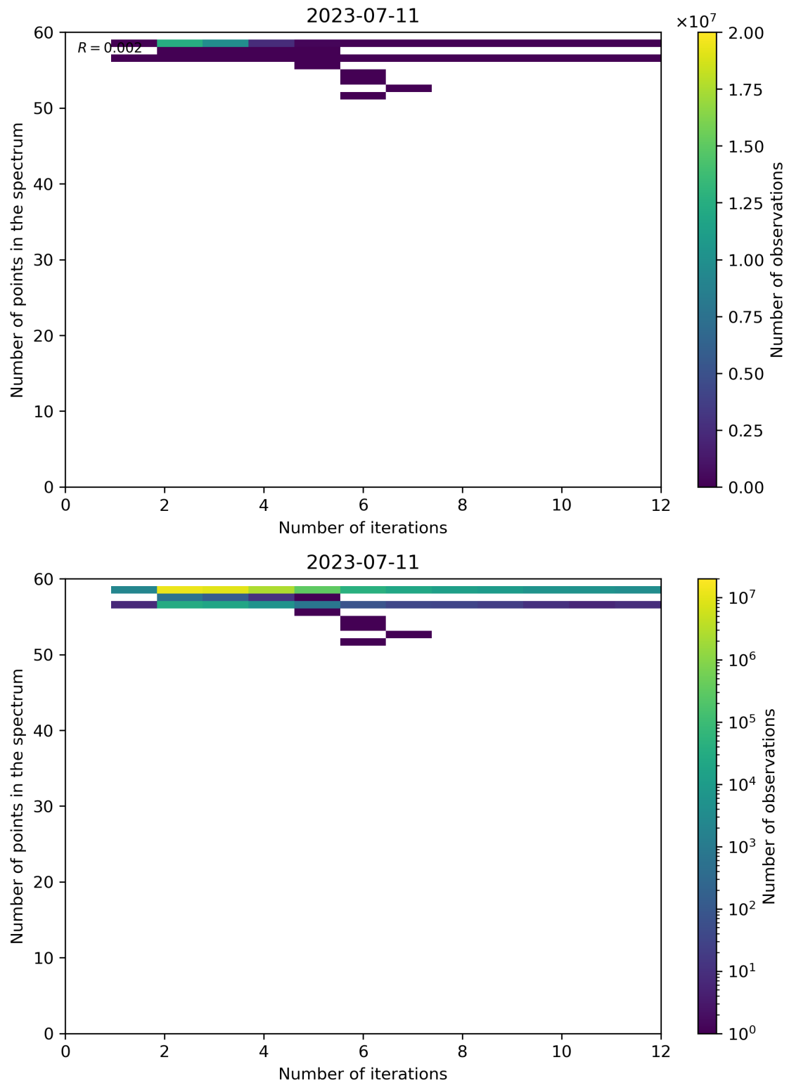
Figure 108: Scatter density plot of “Number of iterations” against “Number of points in the spectrum” for 2023-07-10 to 2023-07-12.
