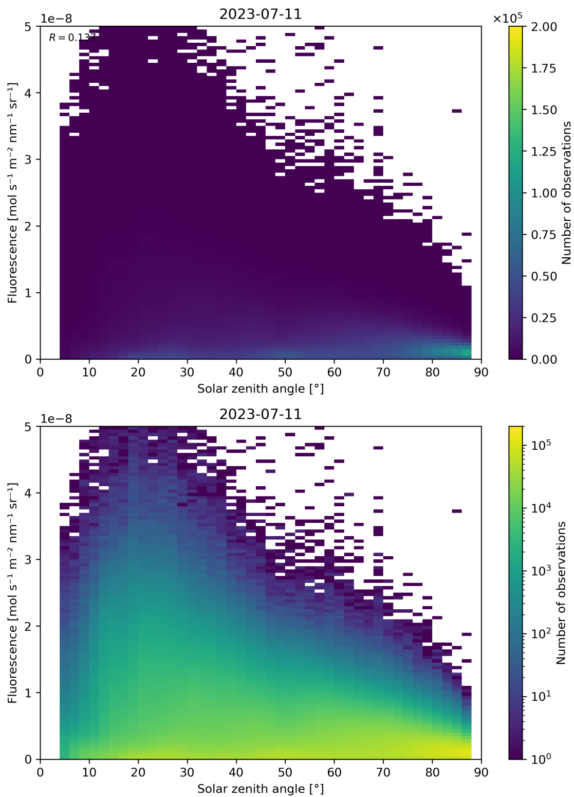
Figure 123: Scatter density plot of “Solar zenith angle” against “Fluorescence” for 2023-07-10 to 2023-07-12.
