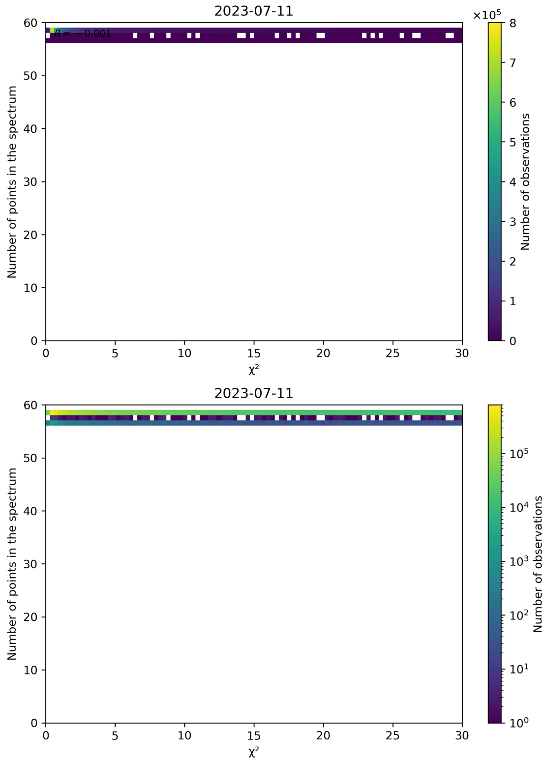
Figure 74: Scatter density plot of “ \chi^2 ” against “Number of points in the spectrum” for 2023-07-10 to 2023-07-12.
