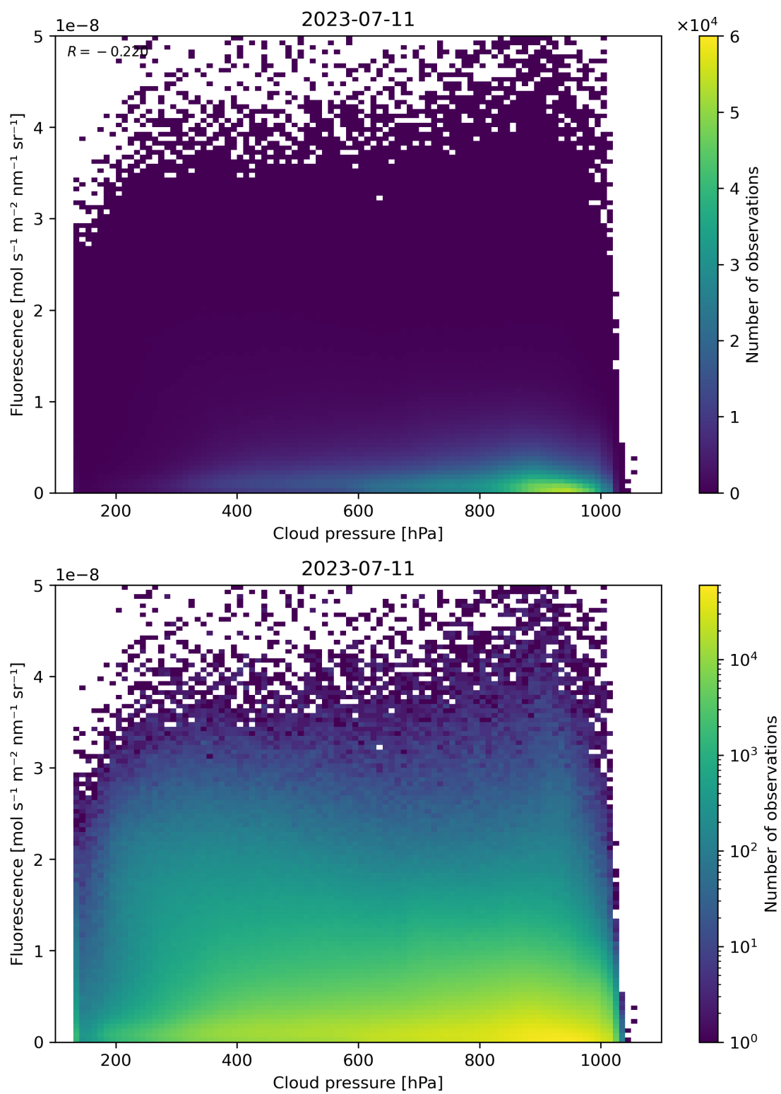
Figure 88: Scatter density plot of “Cloud pressure” against “Fluorescence” for 2023-07-10 to 2023-07-12.
