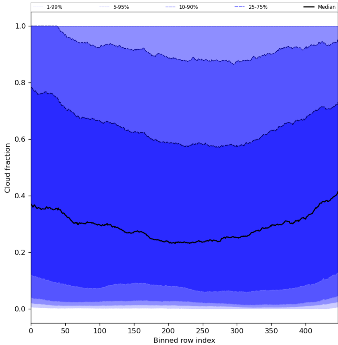
Figure 49: Along track statistics of “Cloud fraction” for 2023-07-10 to 2023-07-12
