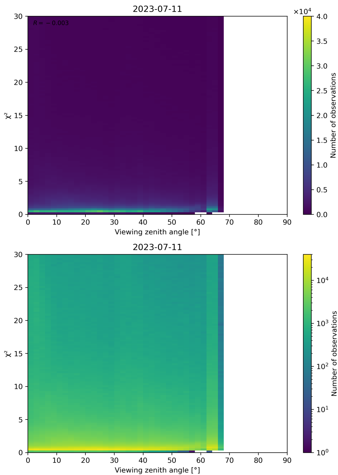
Figure 130: Scatter density plot of “Viewing zenith angle” against “ \chi^2 ” for 2023-07-10 to 2023-07-12.
