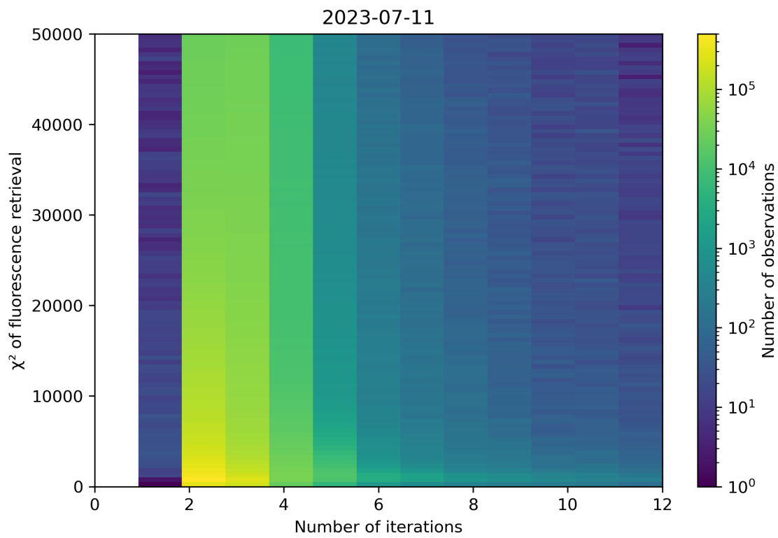
Figure 106: Scatter density plot of “Number of iterations” against “ \chi^2 of fluorescence retrieval” for 2023-07-10 to 2023-07-12.
