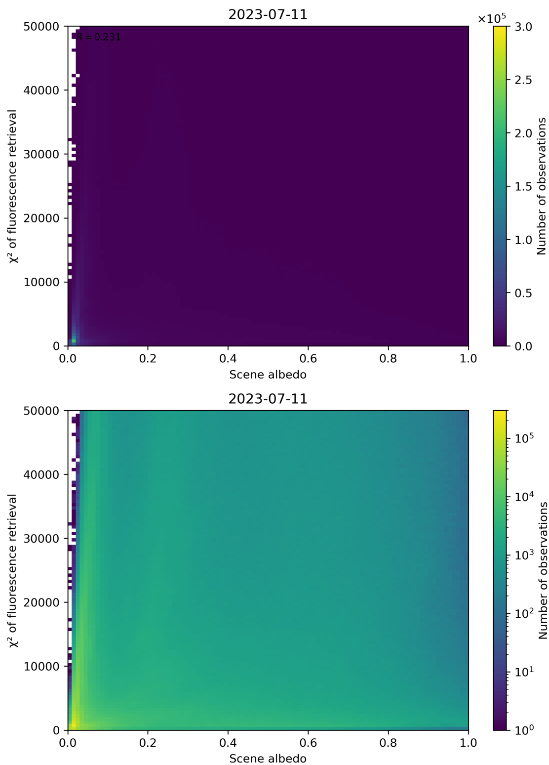
Figure 113: Scatter density plot of “Scene albedo” against “ \chi^2 of fluorescence retrieval” for 2023-07-10 to 2023-07-12.
