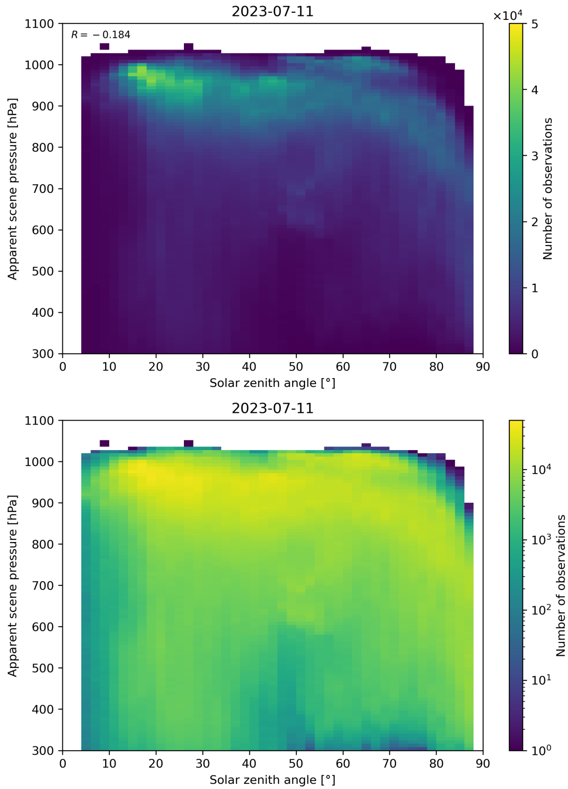
Figure 118: Scatter density plot of “Solar zenith angle” against “Apparent scene pressure” for 2023-07-10 to 2023-07-12.
