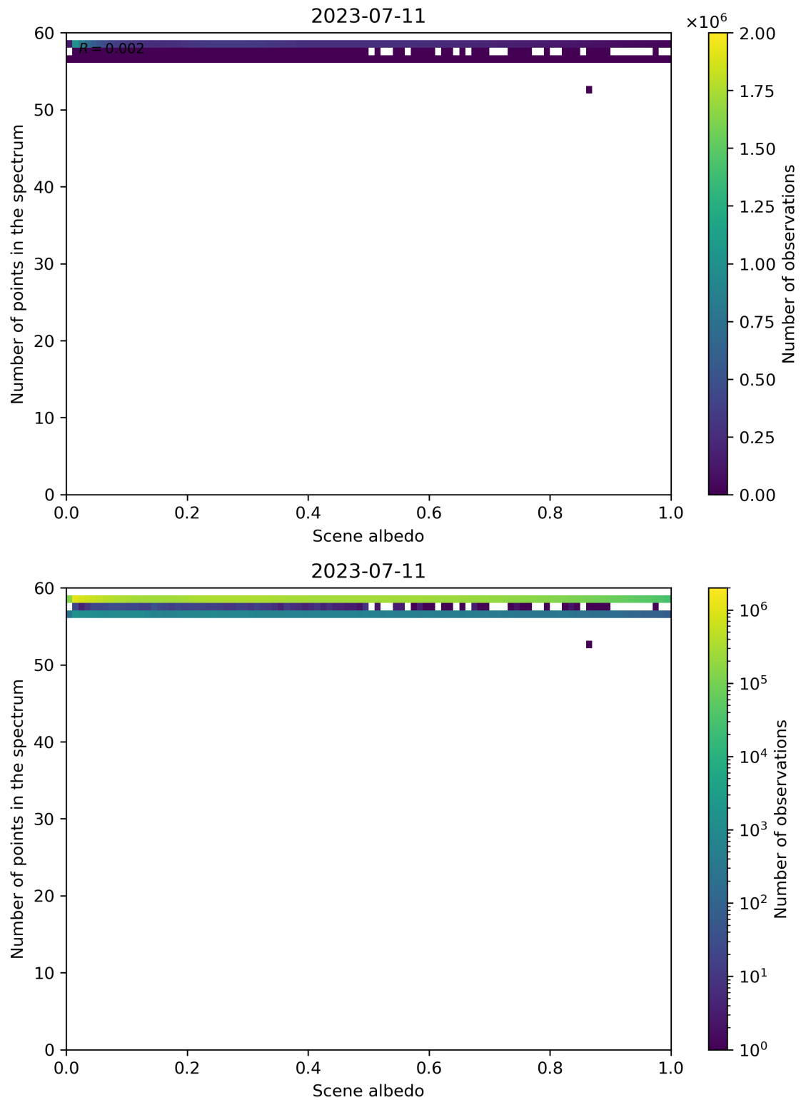
Figure 116: Scatter density plot of “Scene albedo” against “Number of points in the spectrum” for 2023-07-10 to 2023-07-12.
