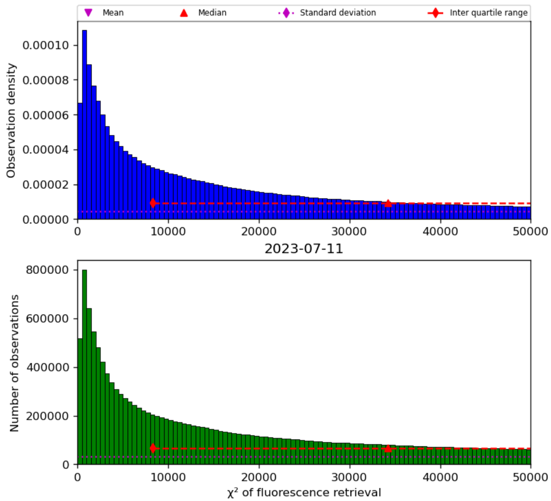
Figure 42: Histogram of “ \chi^2 of fluorescence retrieval” for 2023-07-10 to 2023-07-12
