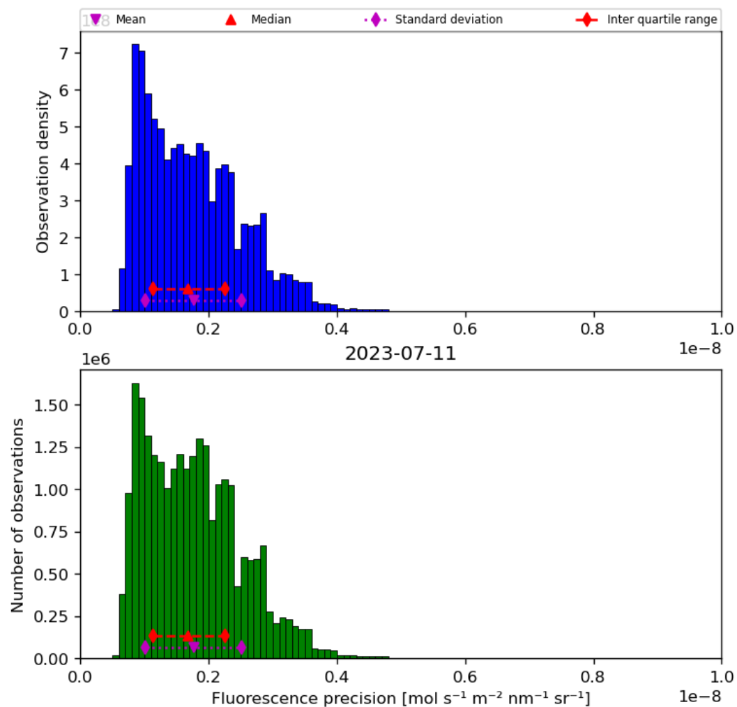
Figure 41: Histogram of “Fluorescence precision” for 2023-07-10 to 2023-07-12
