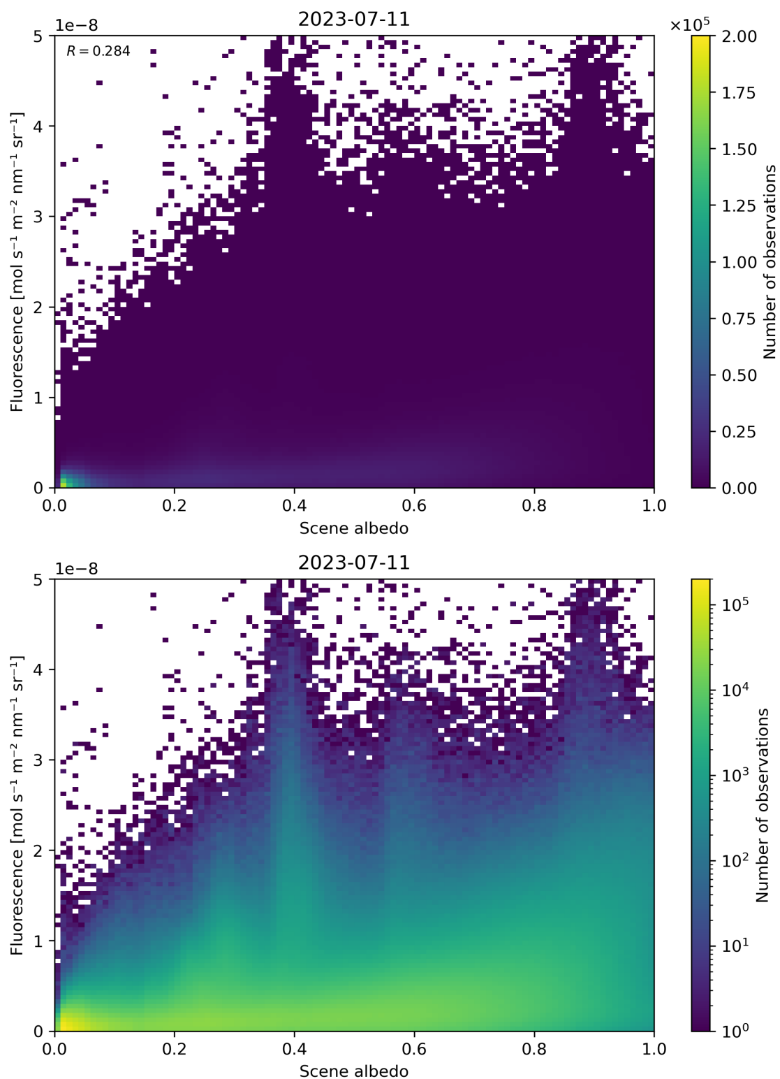
Figure 114: Scatter density plot of “Scene albedo” against “Fluorescence” for 2023-07-10 to 2023-07-12.
