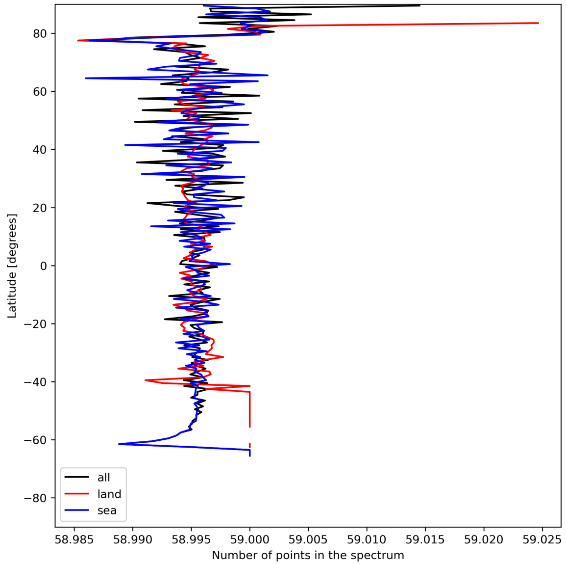
Figure 27: Zonal average of “Number of points in the spectrum” for 2023-07-10 to 2023-07-12.
