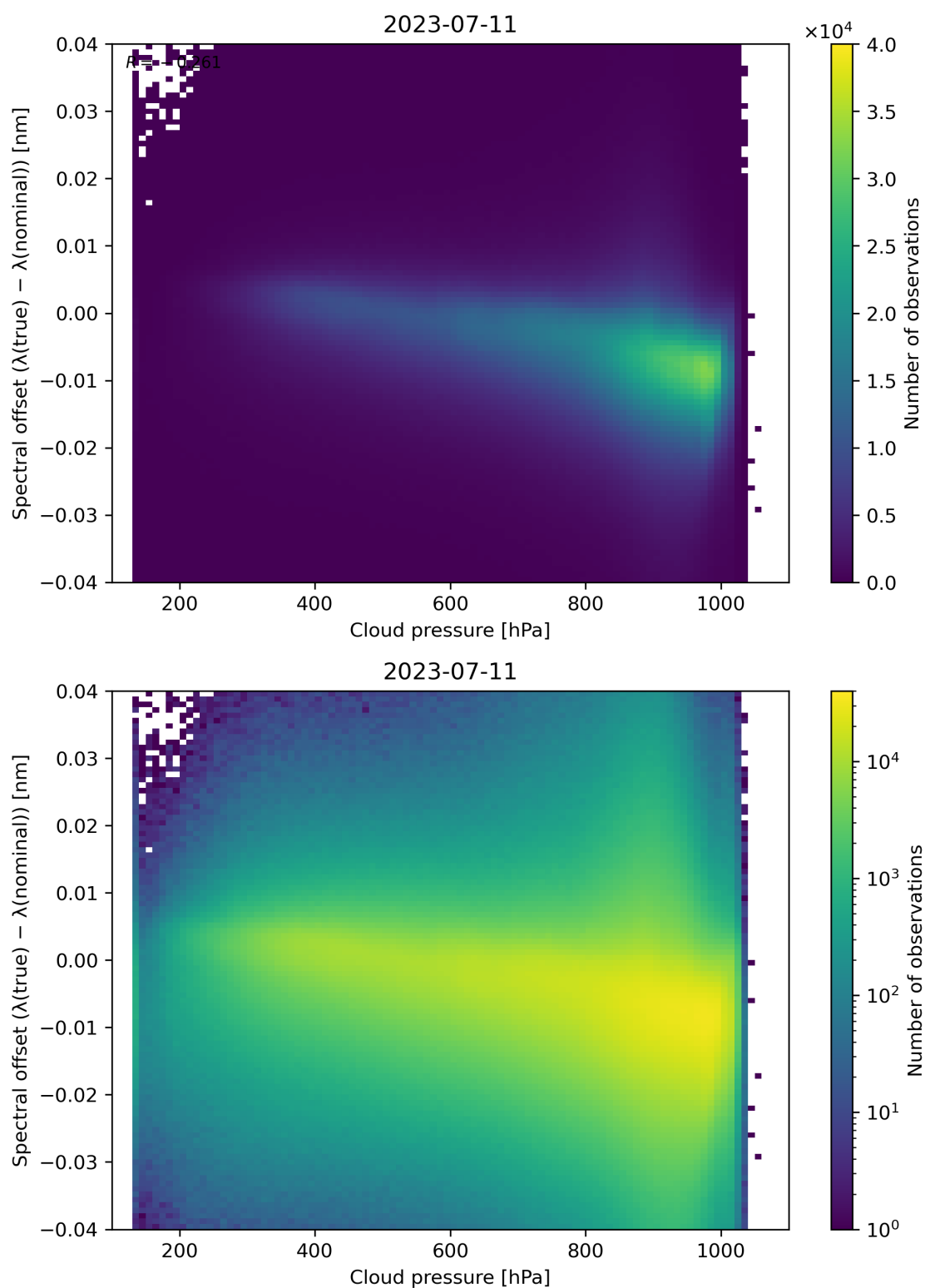
Figure 92: Scatter density plot of “Cloud pressure” against “Spectral offset ( \lambda(\text{true}) - \lambda(\text{nominal}) )” for 2023-07-10 to 2023-07-12.
