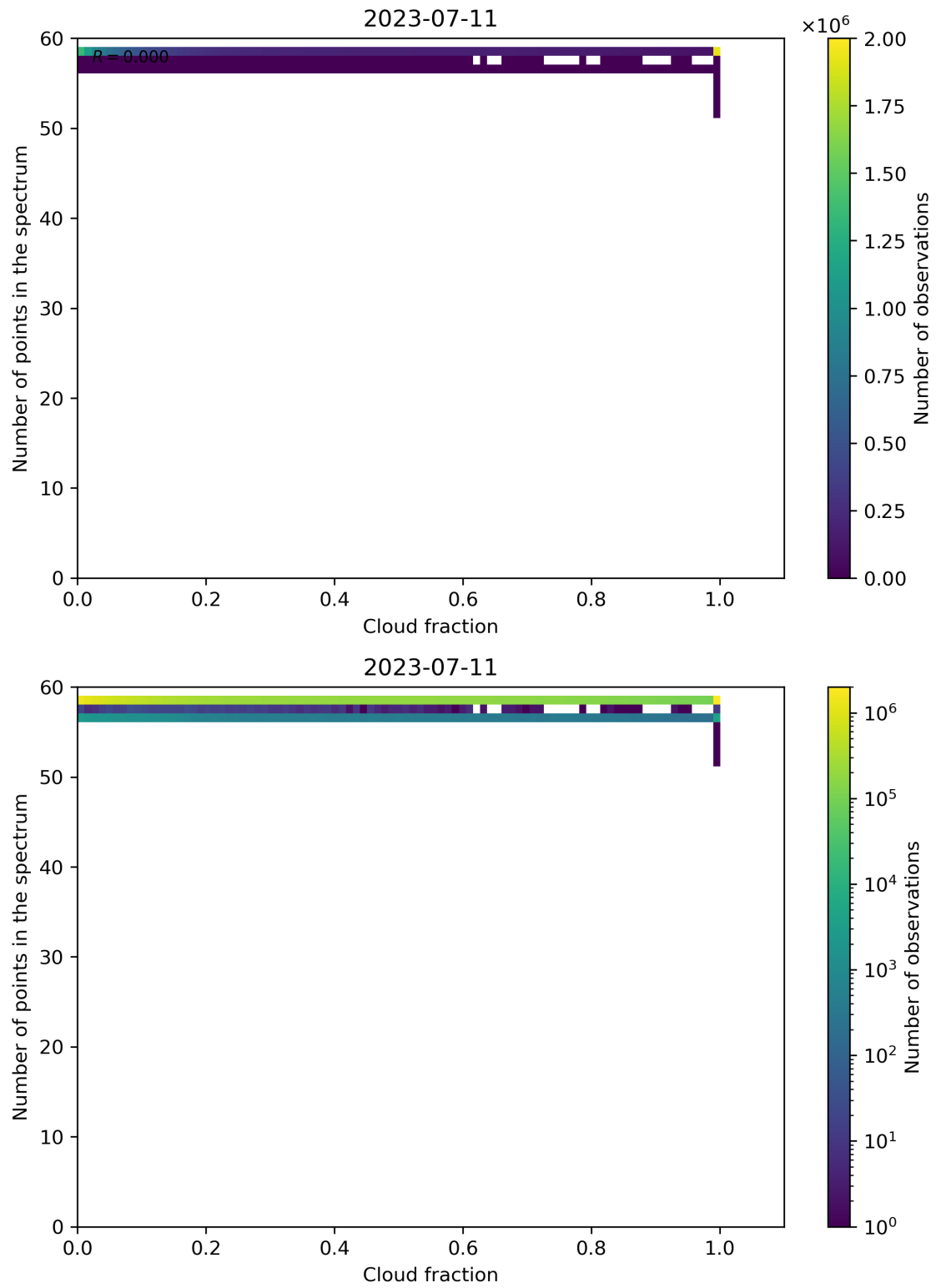
Figure 81: Scatter density plot of “Cloud fraction” against “Number of points in the spectrum” for 2023-07-10 to 2023-07-12.
