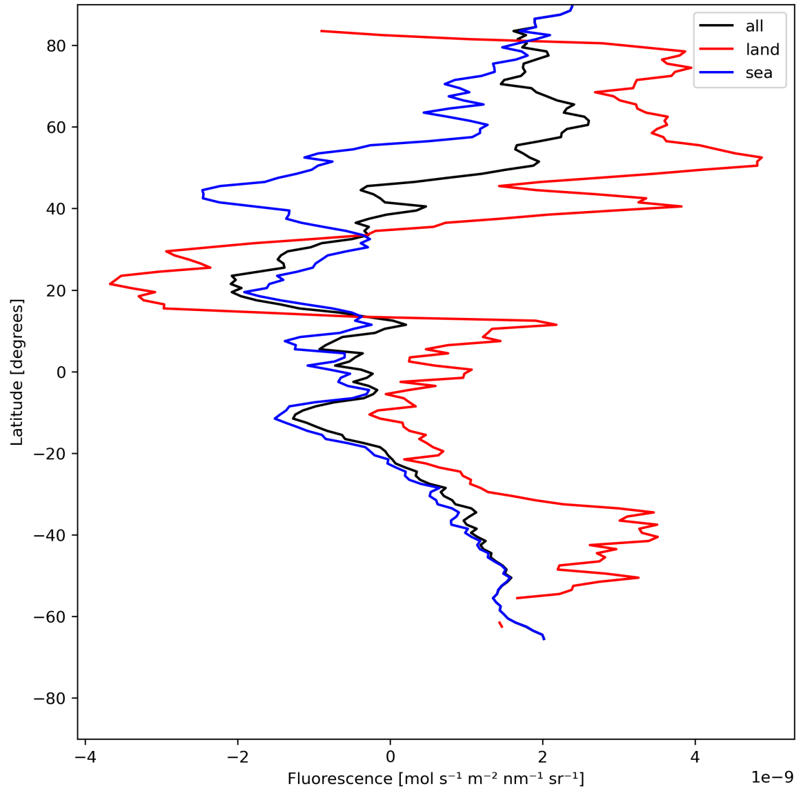
Figure 23: Zonal average of “Fluorescence” for 2023-07-10 to 2023-07-12.
