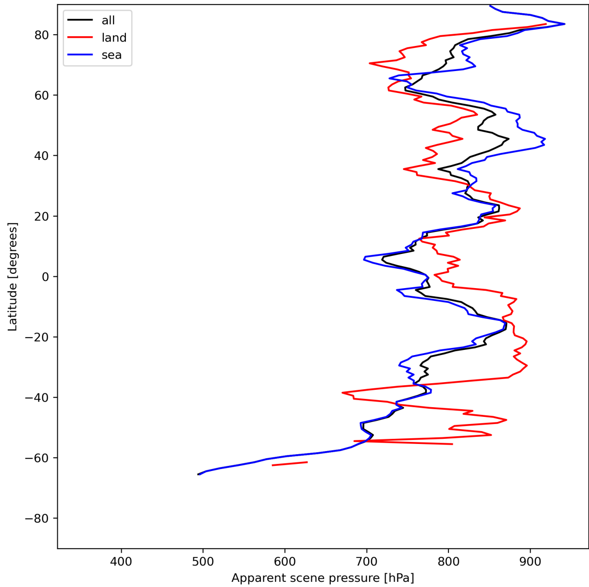
Figure 19: Zonal average of “Apparent scene pressure” for 2023-07-10 to 2023-07-12.
