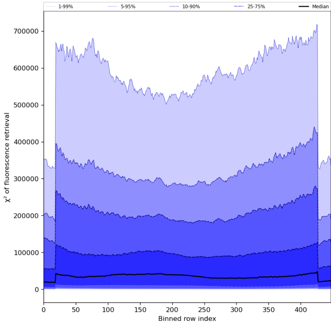
Figure 59: Along track statistics of “ \chi^2 of fluorescence retrieval” for 2023-07-10 to 2023-07-12
