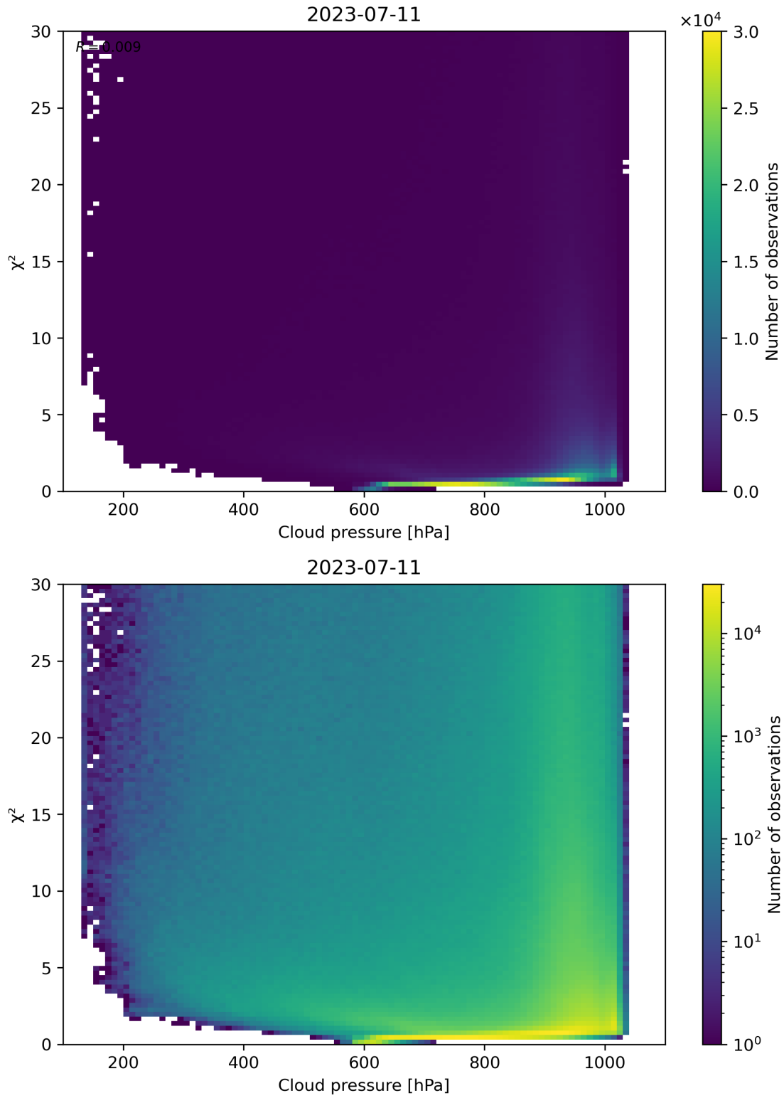
Figure 85: Scatter density plot of “Cloud pressure” against “ \chi^2 ” for 2023-07-10 to 2023-07-12.
