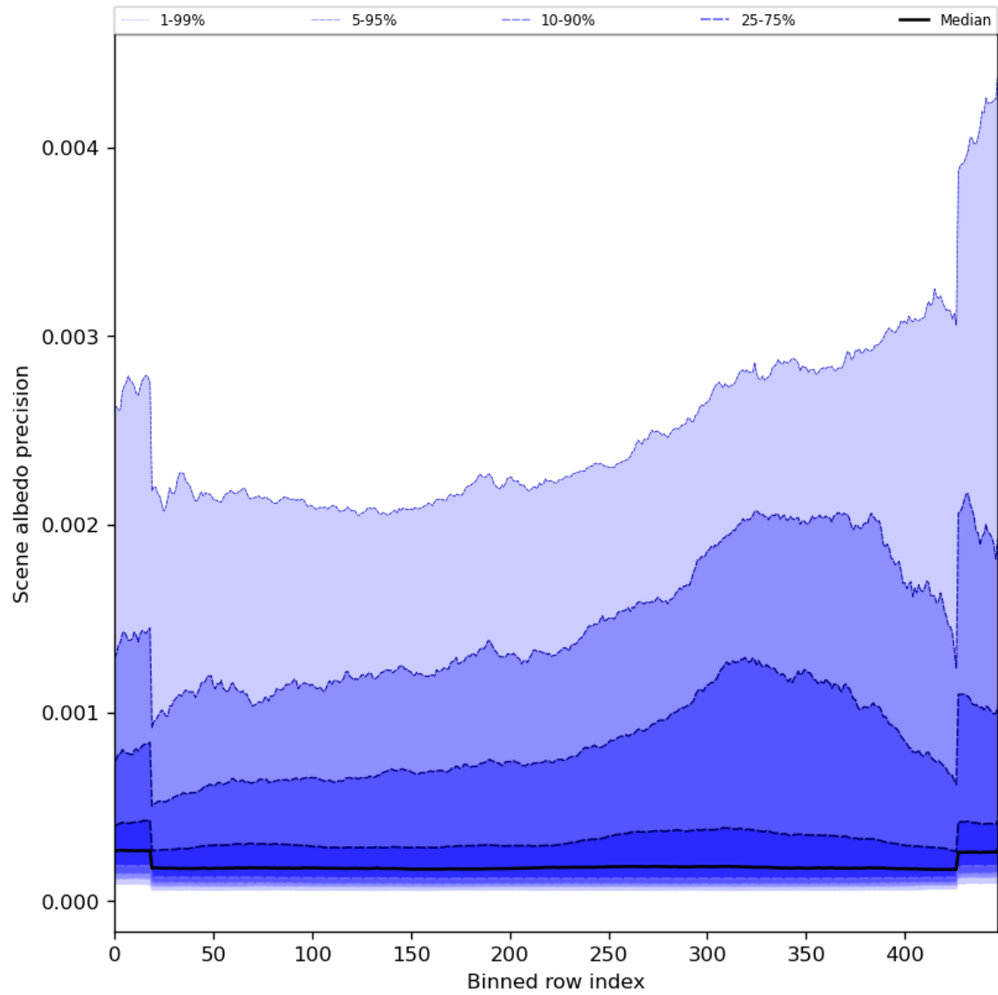
Figure 52: Along track statistics of “Scene albedo precision” for 2023-07-10 to 2023-07-12
