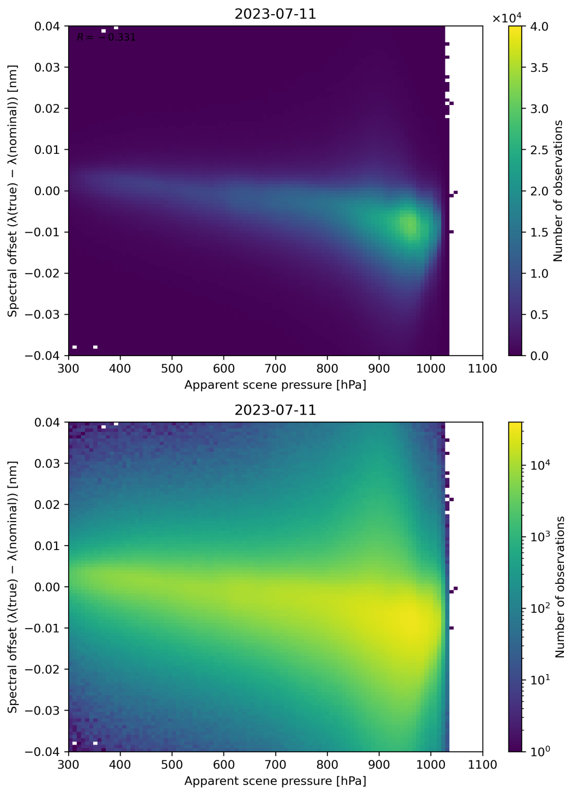
Figure 68: Scatter density plot of “Apparent scene pressure” against “Spectral offset ( \lambda(\text{true}) - \lambda(\text{nominal}) )” for 2023-07-10 to 2023-07-12.
