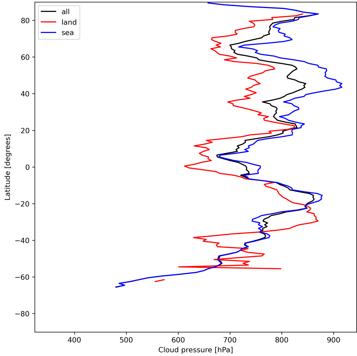
Figure 13: Zonal average of “Cloud pressure” for 2023-07-10 to 2023-07-12.
