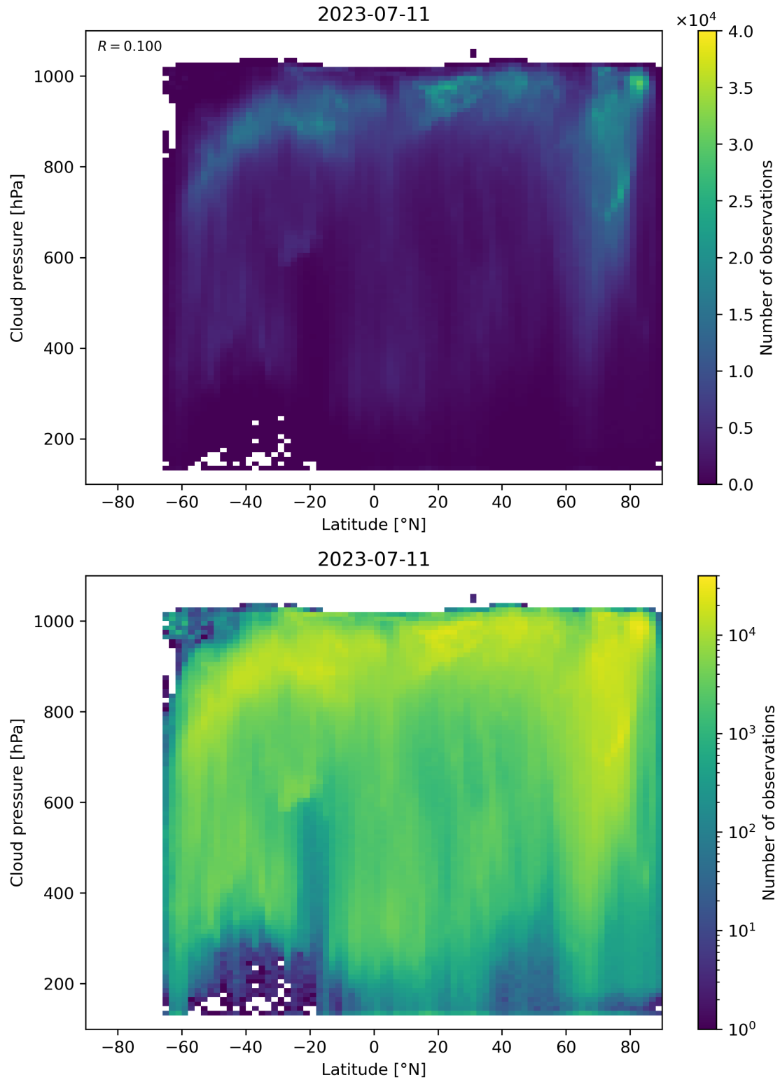
Figure 100: Scatter density plot of “Latitude” against “Cloud pressure” for 2023-07-10 to 2023-07-12.
