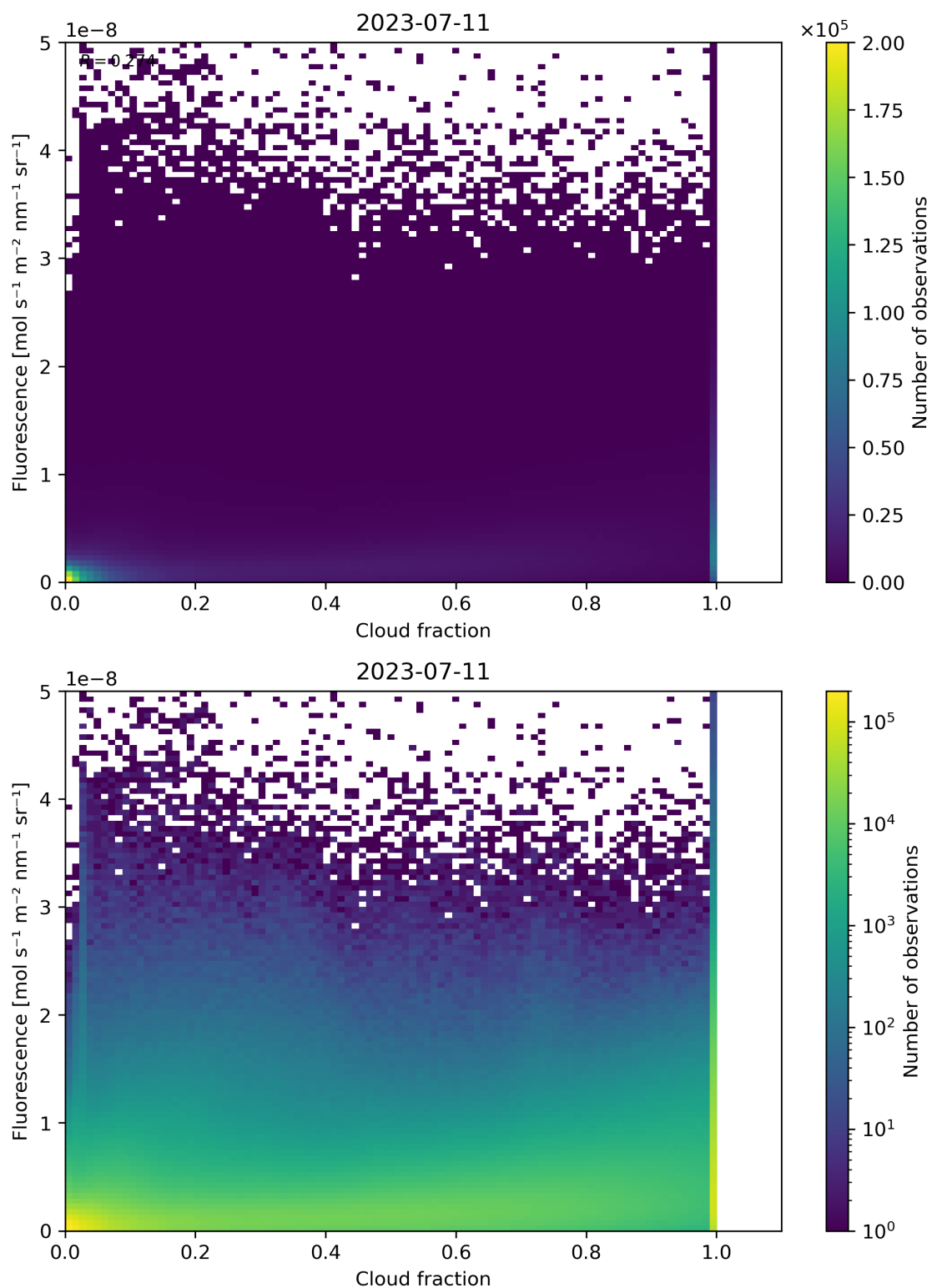
Figure 79: Scatter density plot of “Cloud fraction” against “Fluorescence” for 2023-07-10 to 2023-07-12.
