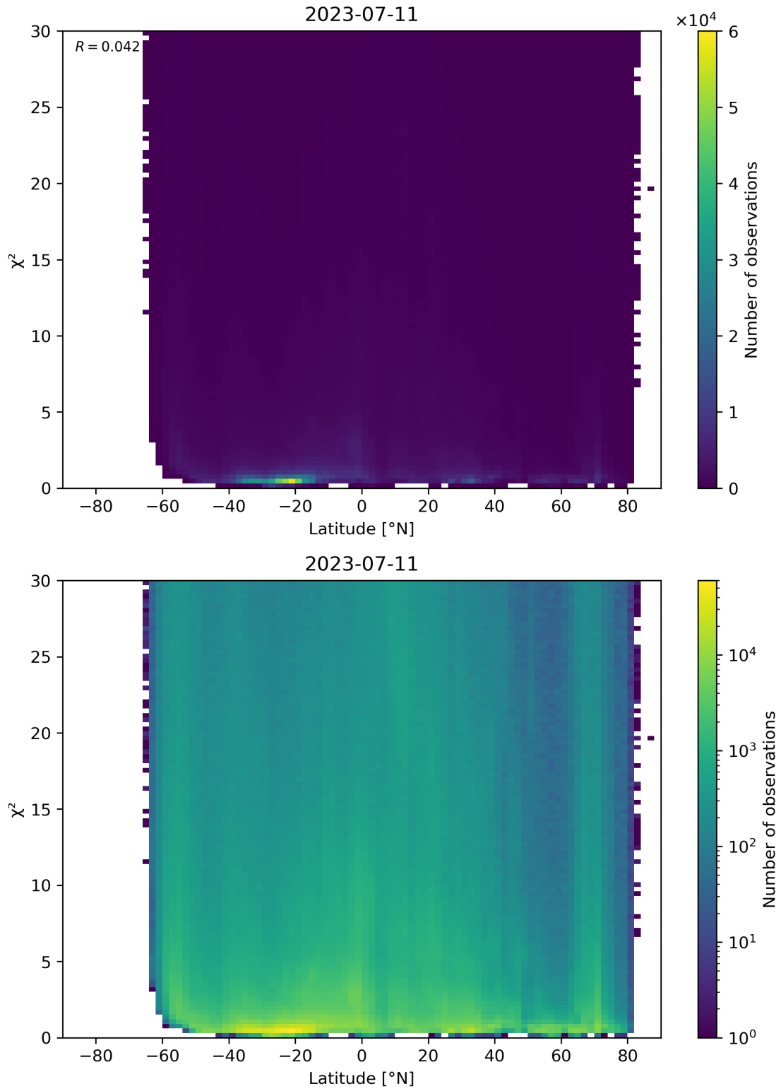
Figure 97: Scatter density plot of “Latitude” against “ \chi^2 ” for 2023-07-10 to 2023-07-12.
