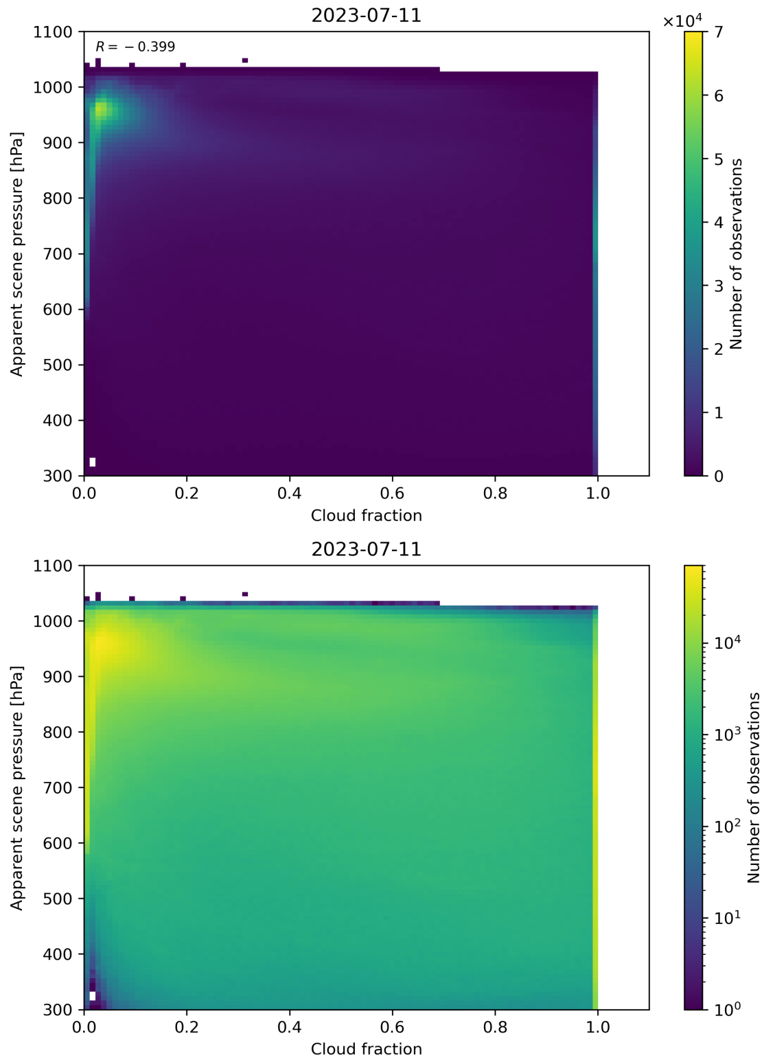
Figure 76: Scatter density plot of “Cloud fraction” against “Apparent scene pressure” for 2023-07-10 to 2023-07-12.
