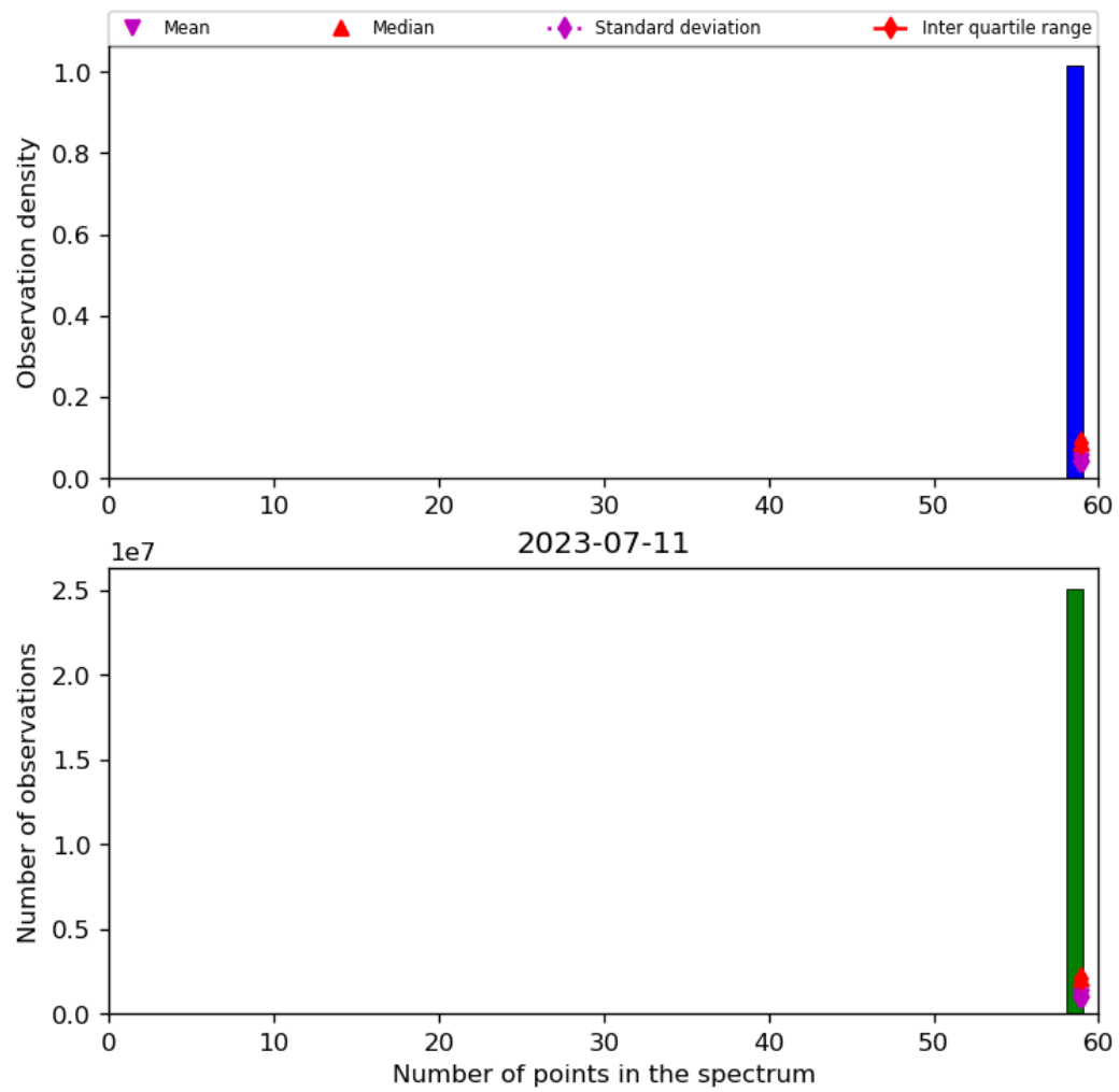
Figure 44: Histogram of “Number of points in the spectrum” for 2023-07-10 to 2023-07-12
