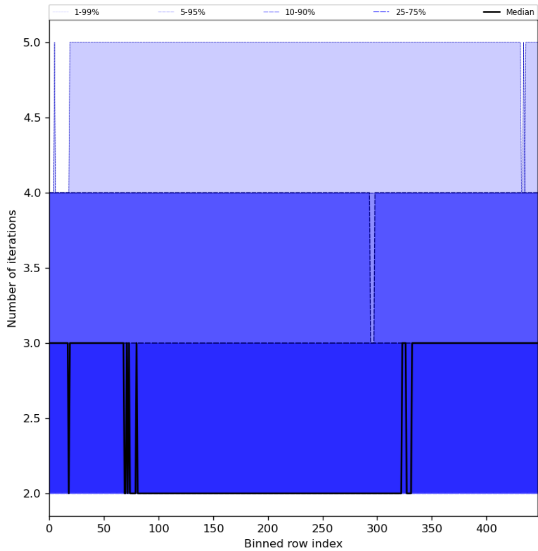
Figure 56: Along track statistics of “Number of iterations” for 2023-07-10 to 2023-07-12
