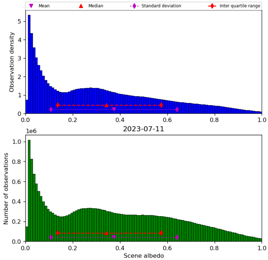
Figure 34: Histogram of “Scene albedo” for 2023-07-10 to 2023-07-12
