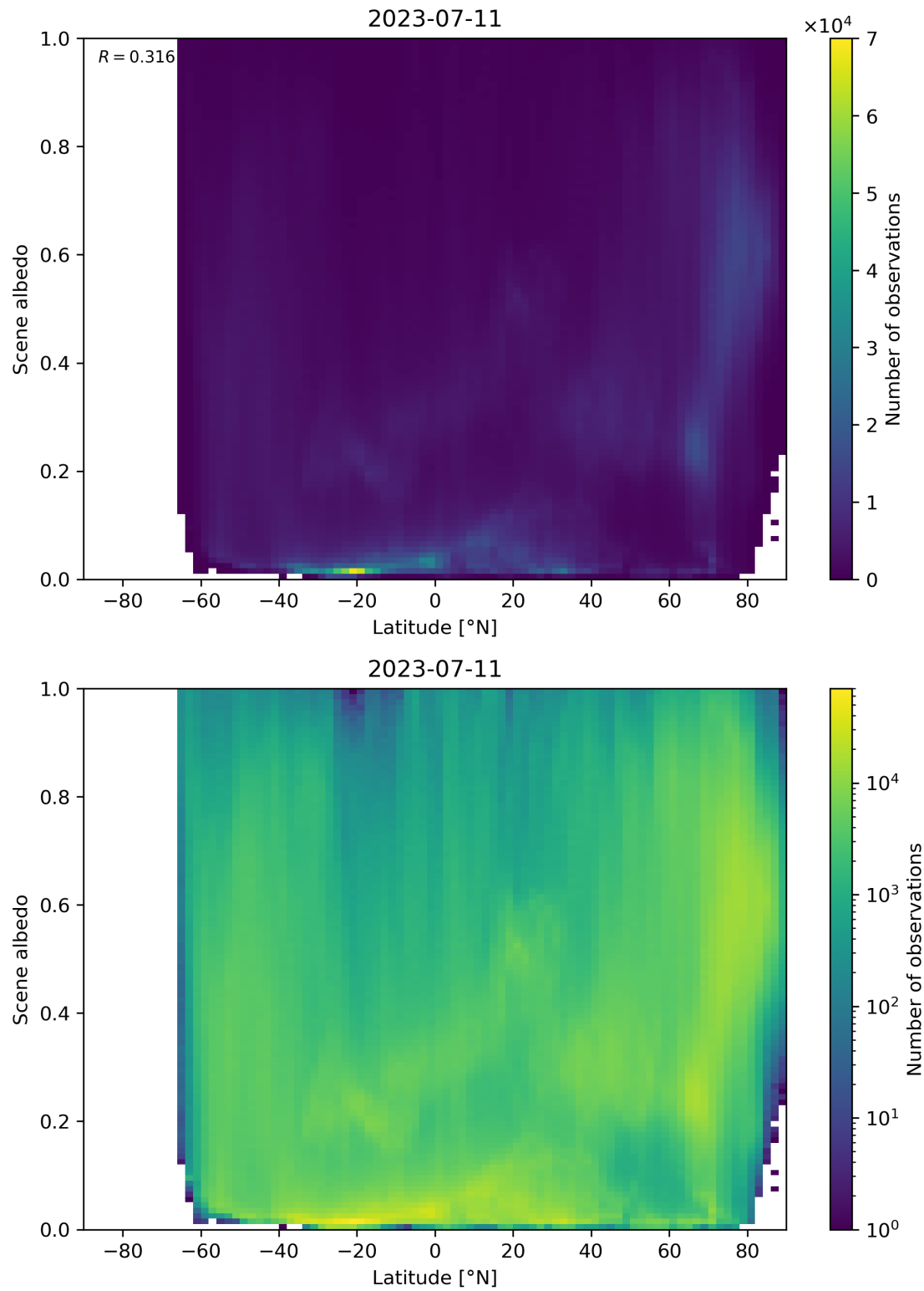
Figure 104: Scatter density plot of “Latitude” against “Scene albedo” for 2023-07-10 to 2023-07-12.
