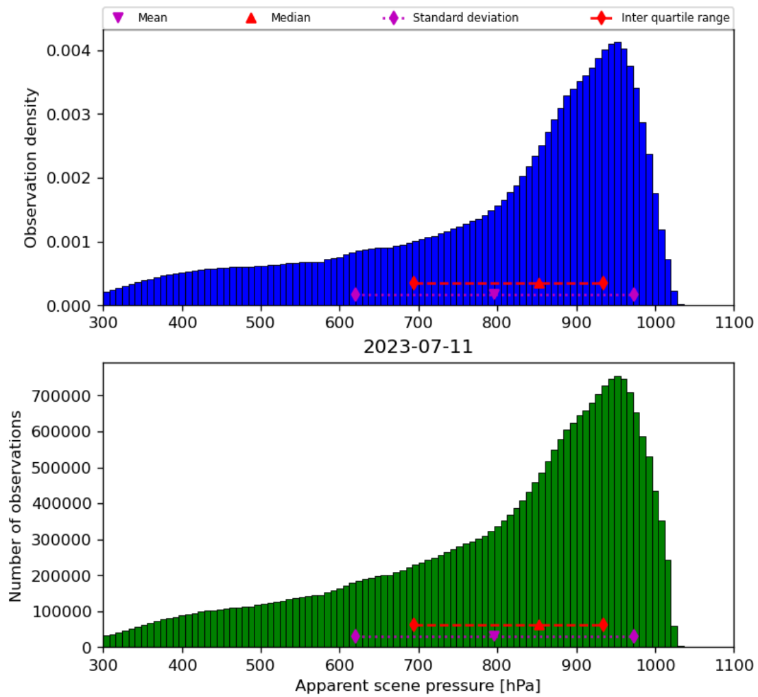
Figure 36: Histogram of “Apparent scene pressure” for 2023-07-10 to 2023-07-12
