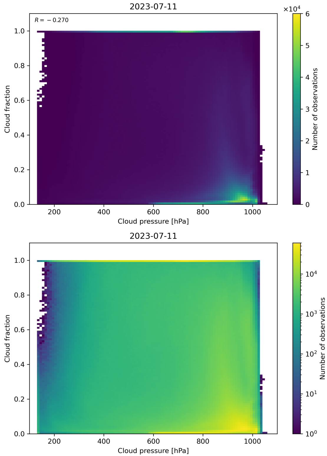
Figure 87: Scatter density plot of “Cloud pressure” against “Cloud fraction” for 2023-07-10 to 2023-07-12.
