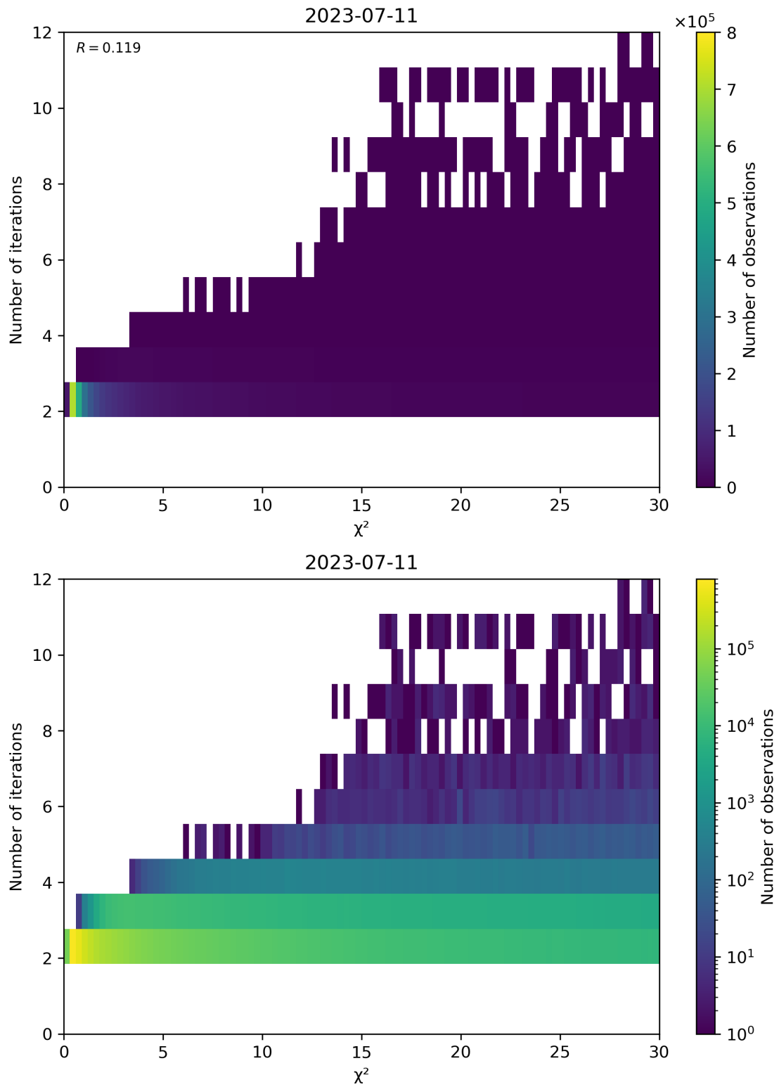
Figure 73: Scatter density plot of “ \chi^2 ” against “Number of iterations” for 2023-07-10 to 2023-07-12.
