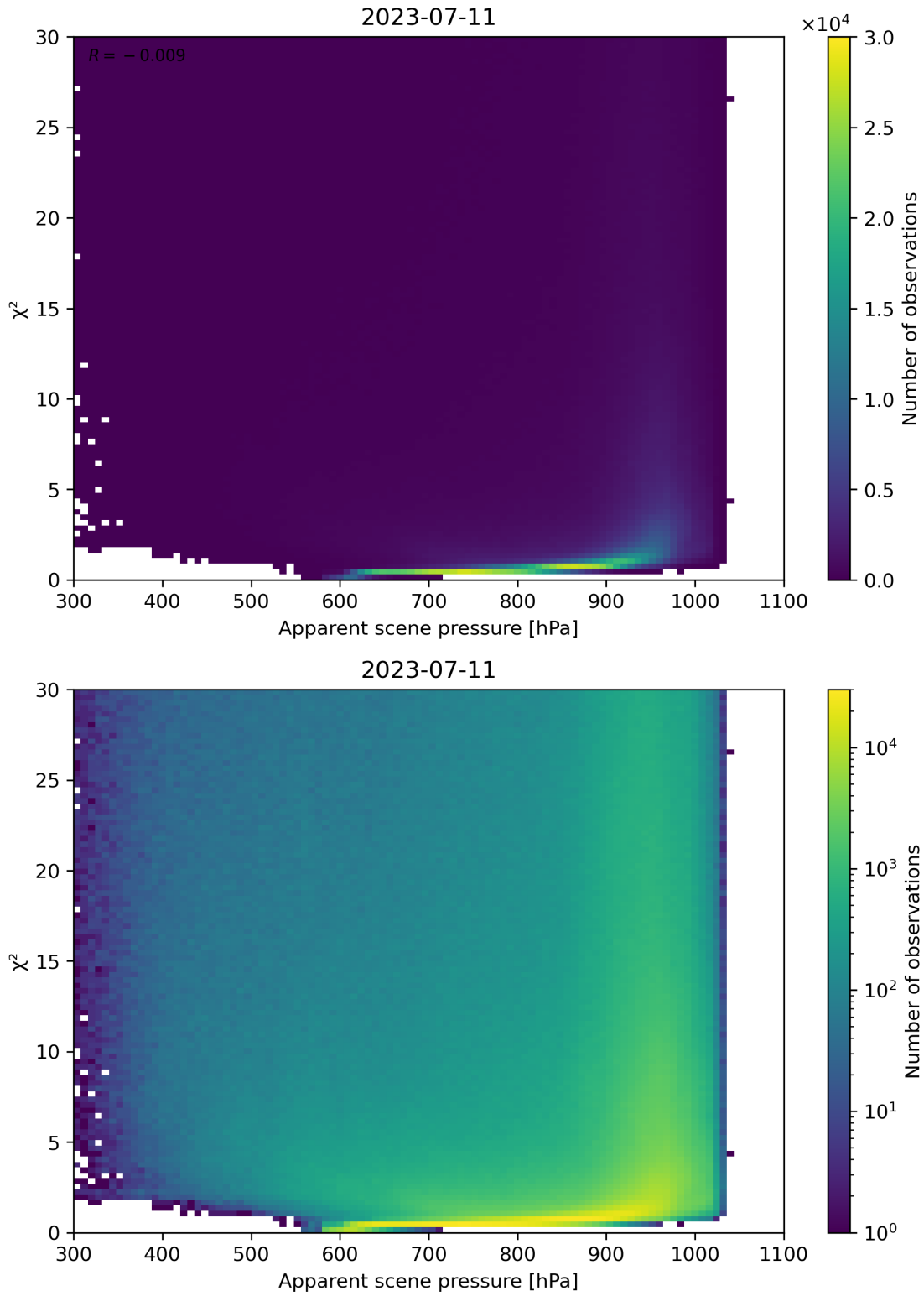
Figure 63: Scatter density plot of “Apparent scene pressure” against “ \chi^2 ” for 2023-07-10 to 2023-07-12.
