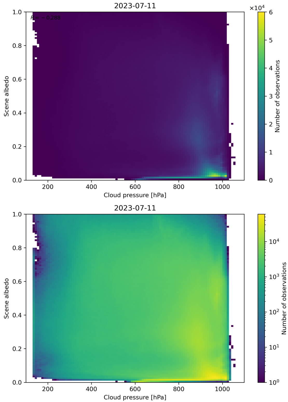
Figure 91: Scatter density plot of “Cloud pressure” against “Scene albedo” for 2023-07-10 to 2023-07-12.
