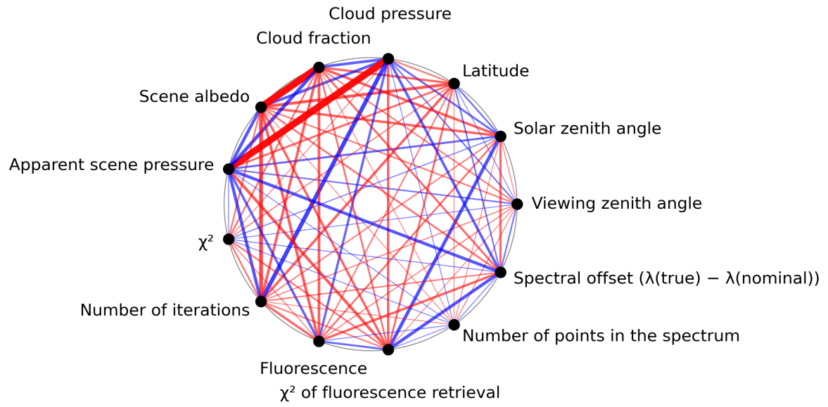
Figure 1: Map of correlation graph for 2023-07-10 to 2023-07-12.
