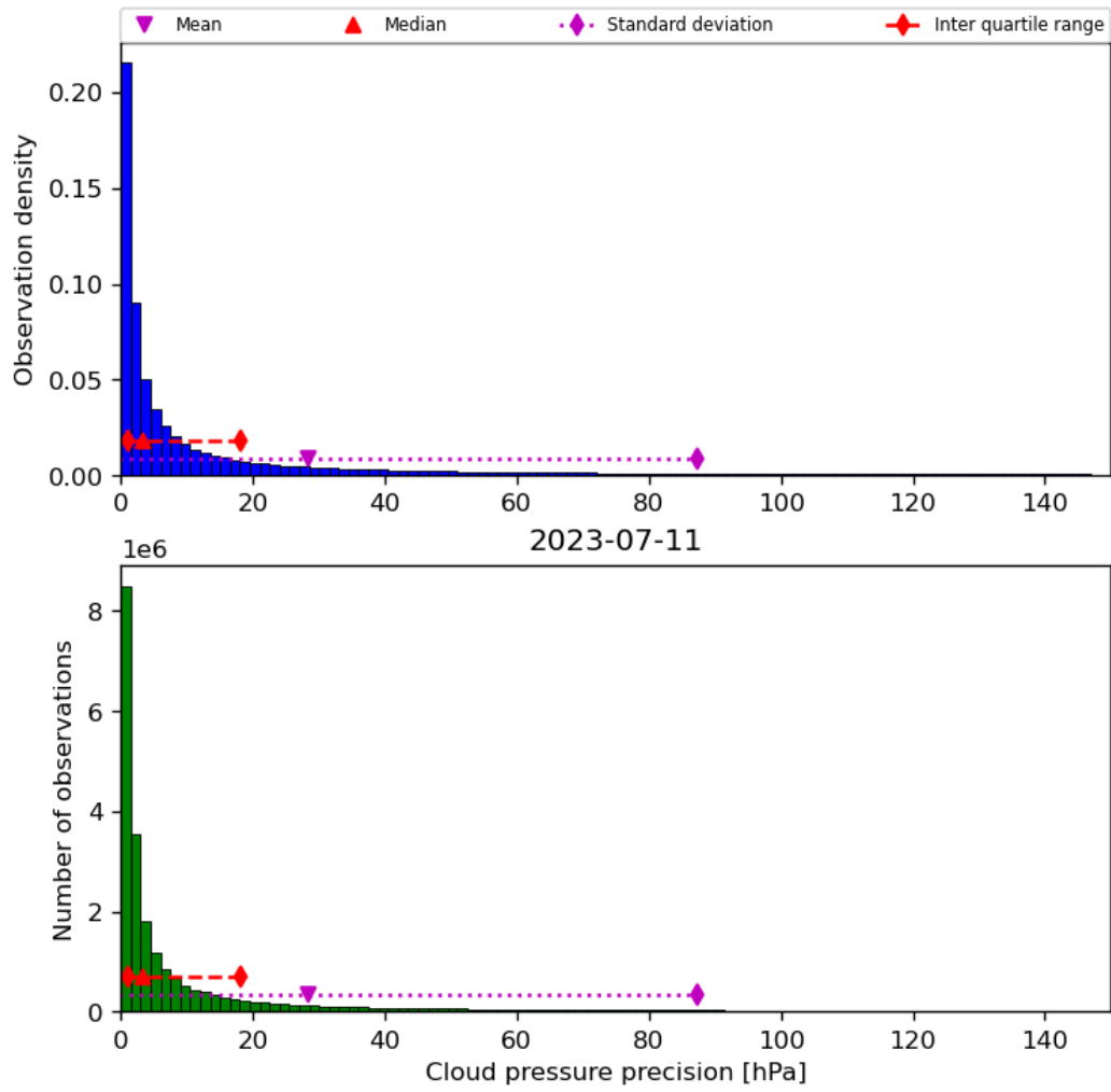
Figure 31: Histogram of “Cloud pressure precision” for 2023-07-10 to 2023-07-12
