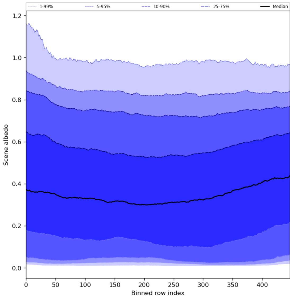
Figure 51: Along track statistics of “Scene albedo” for 2023-07-10 to 2023-07-12
