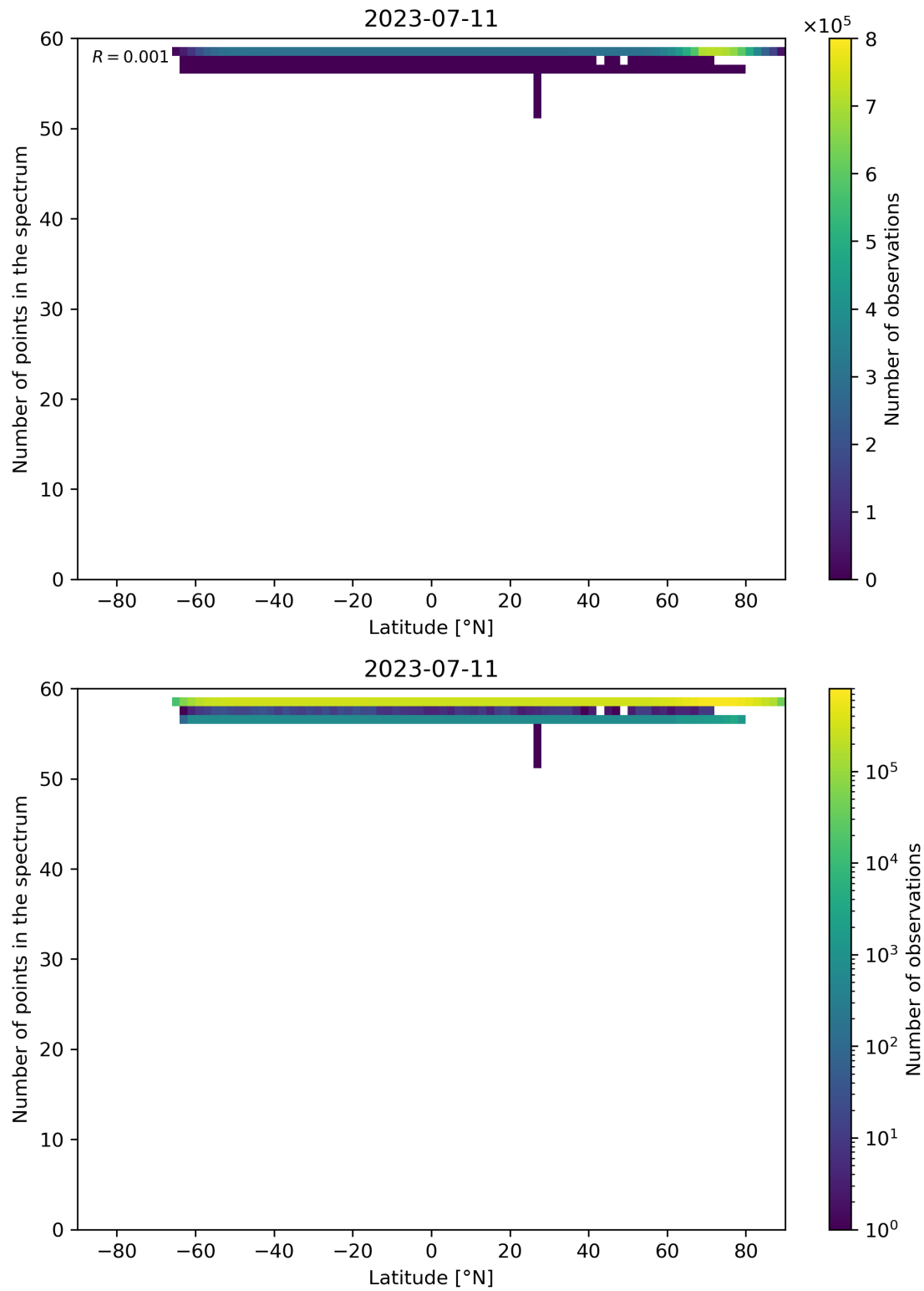
Figure 103: Scatter density plot of “Latitude” against “Number of points in the spectrum” for 2023-07-10 to 2023-07-12.
