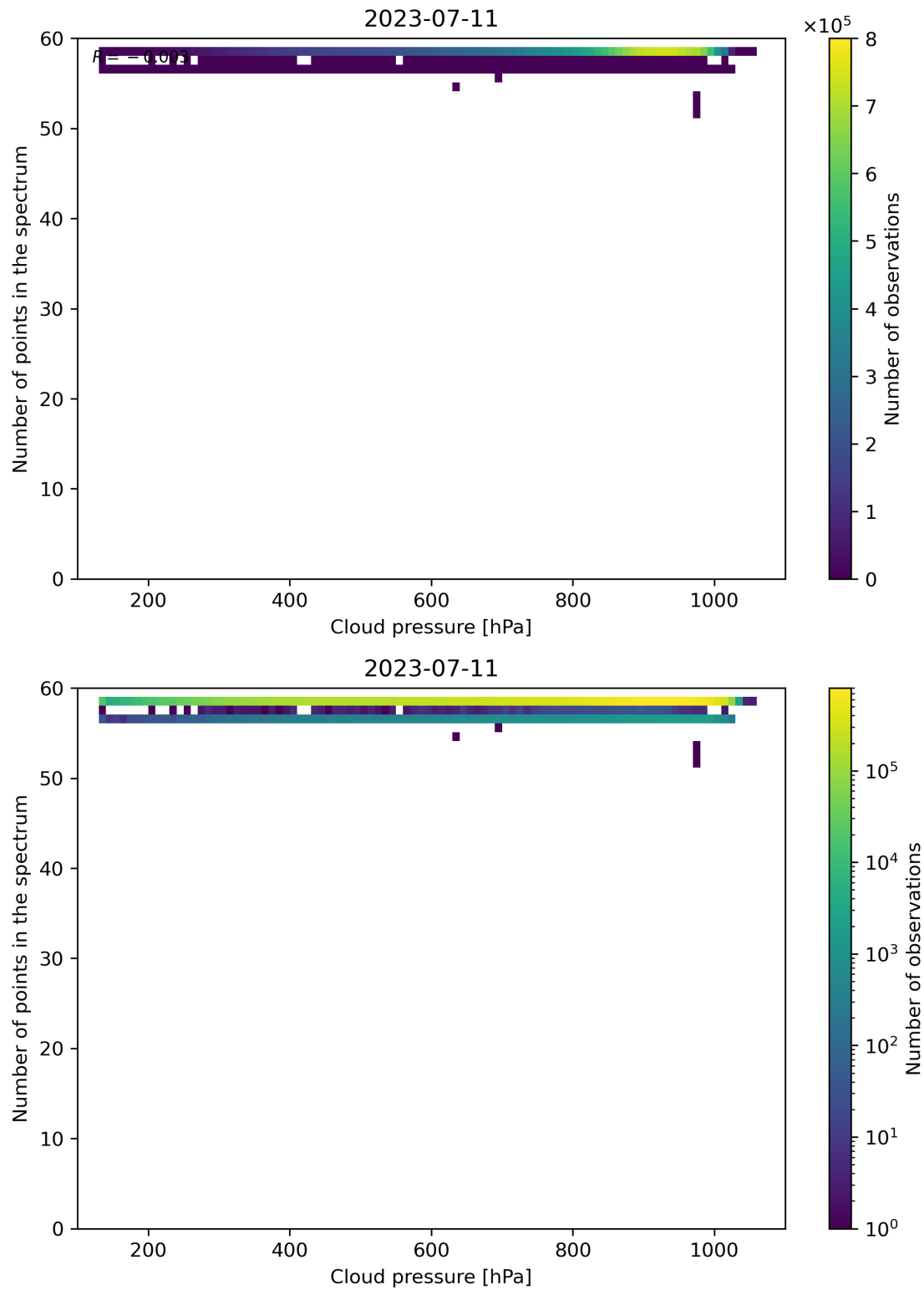
Figure 90: Scatter density plot of “Cloud pressure” against “Number of points in the spectrum” for 2023-07-10 to 2023-07-12.
