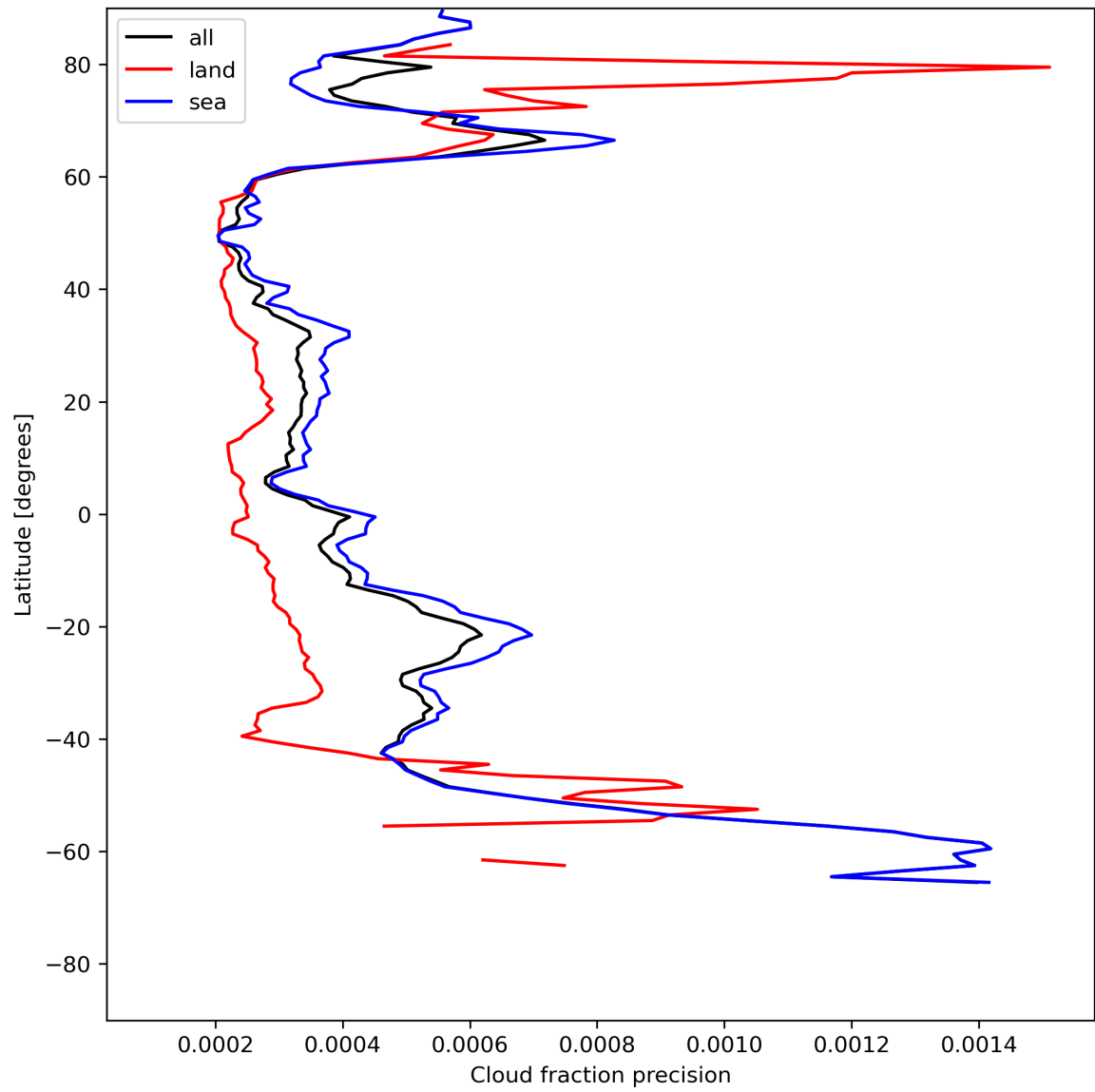
Figure 16: Zonal average of “Cloud fraction precision” for 2023-07-10 to 2023-07-12.
