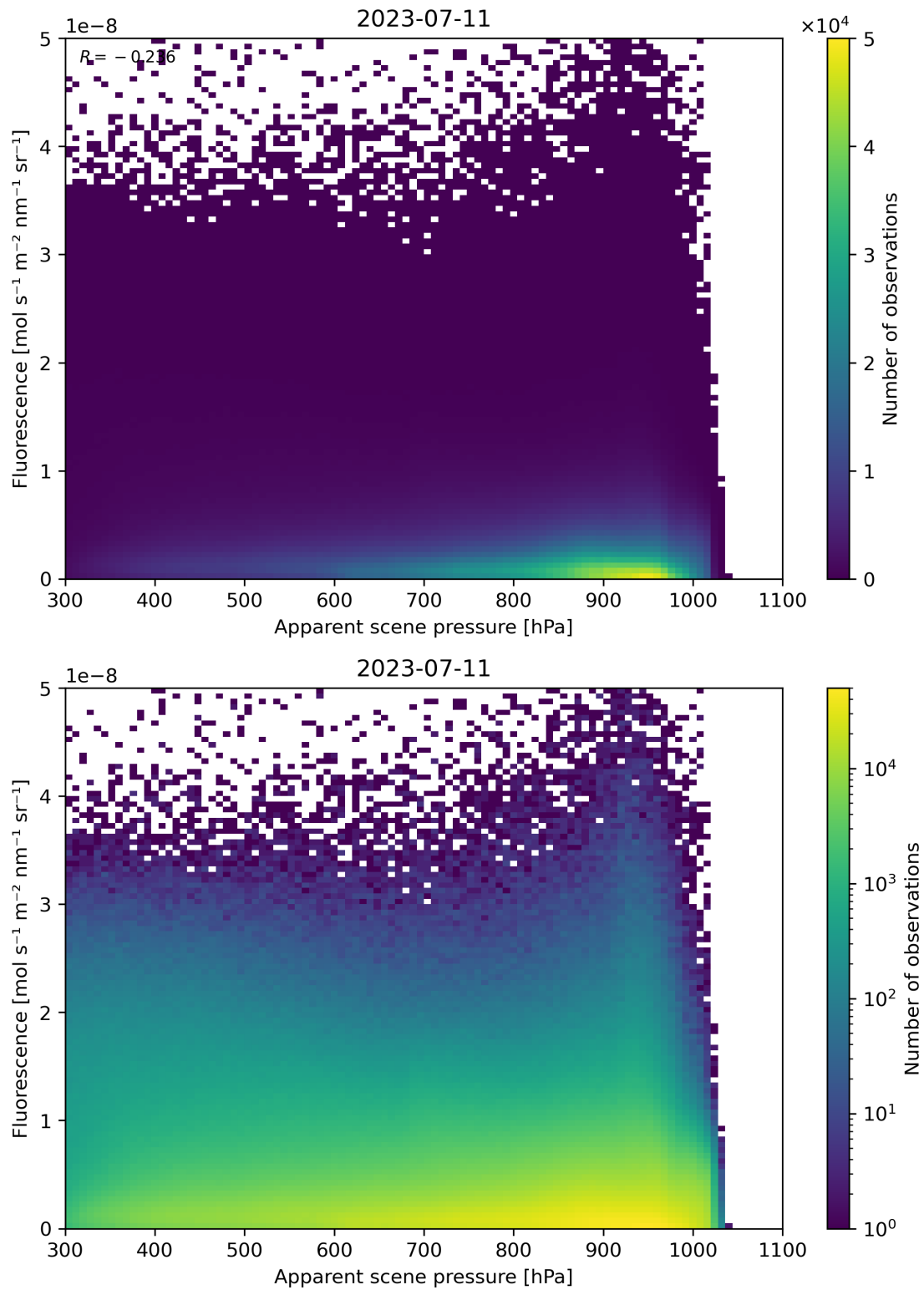
Figure 65: Scatter density plot of “Apparent scene pressure” against “Fluorescence” for 2023-07-10 to 2023-07-12.
