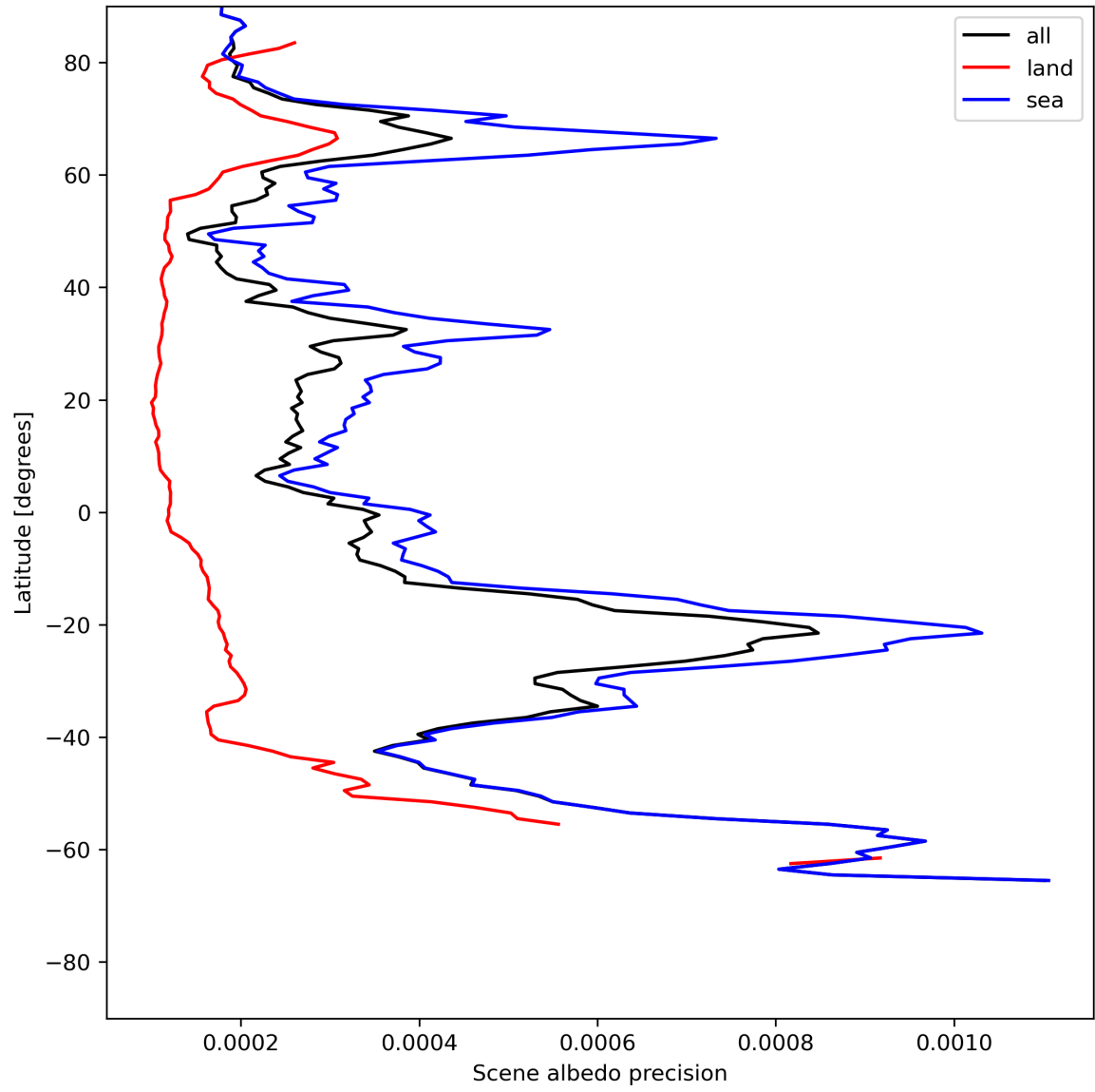
Figure 18: Zonal average of “Scene albedo precision” for 2023-07-10 to 2023-07-12.
