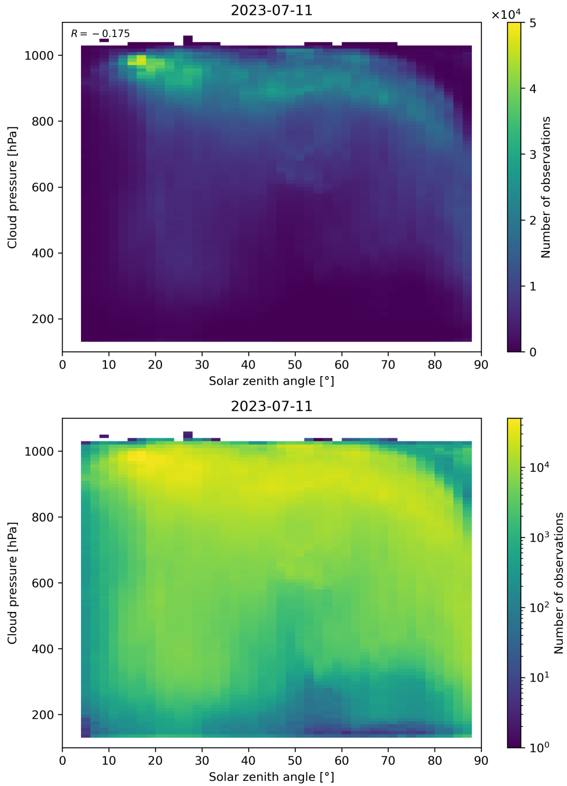
Figure 122: Scatter density plot of “Solar zenith angle” against “Cloud pressure” for 2023-07-10 to 2023-07-12.
