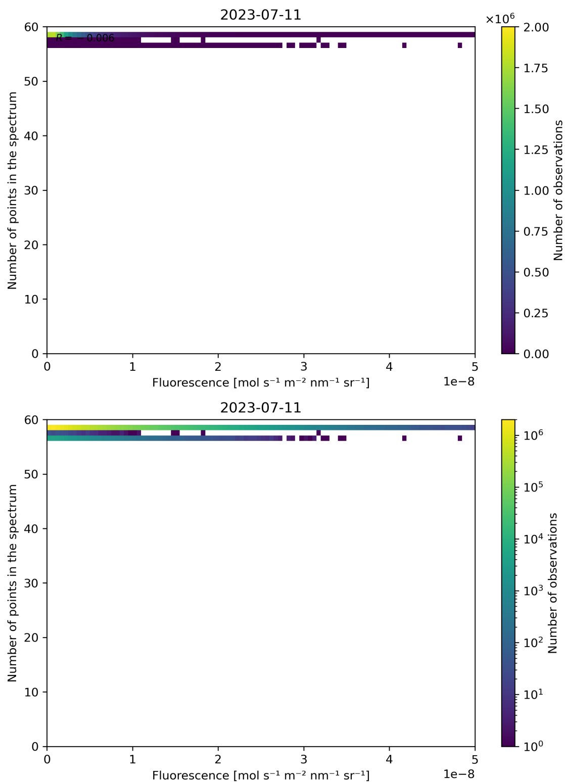
Figure 94: Scatter density plot of “Fluorescence” against “Number of points in the spectrum” for 2023-07-10 to 2023-07-12.
