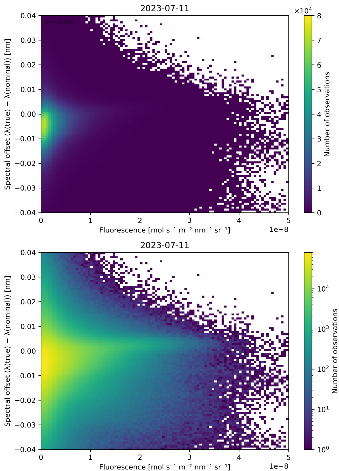
Figure 95: Scatter density plot of “Fluorescence” against “Spectral offset ( \lambda(\text{true}) - \lambda(\text{nominal}) )” for 2023-07-10 to 2023-07-12.
