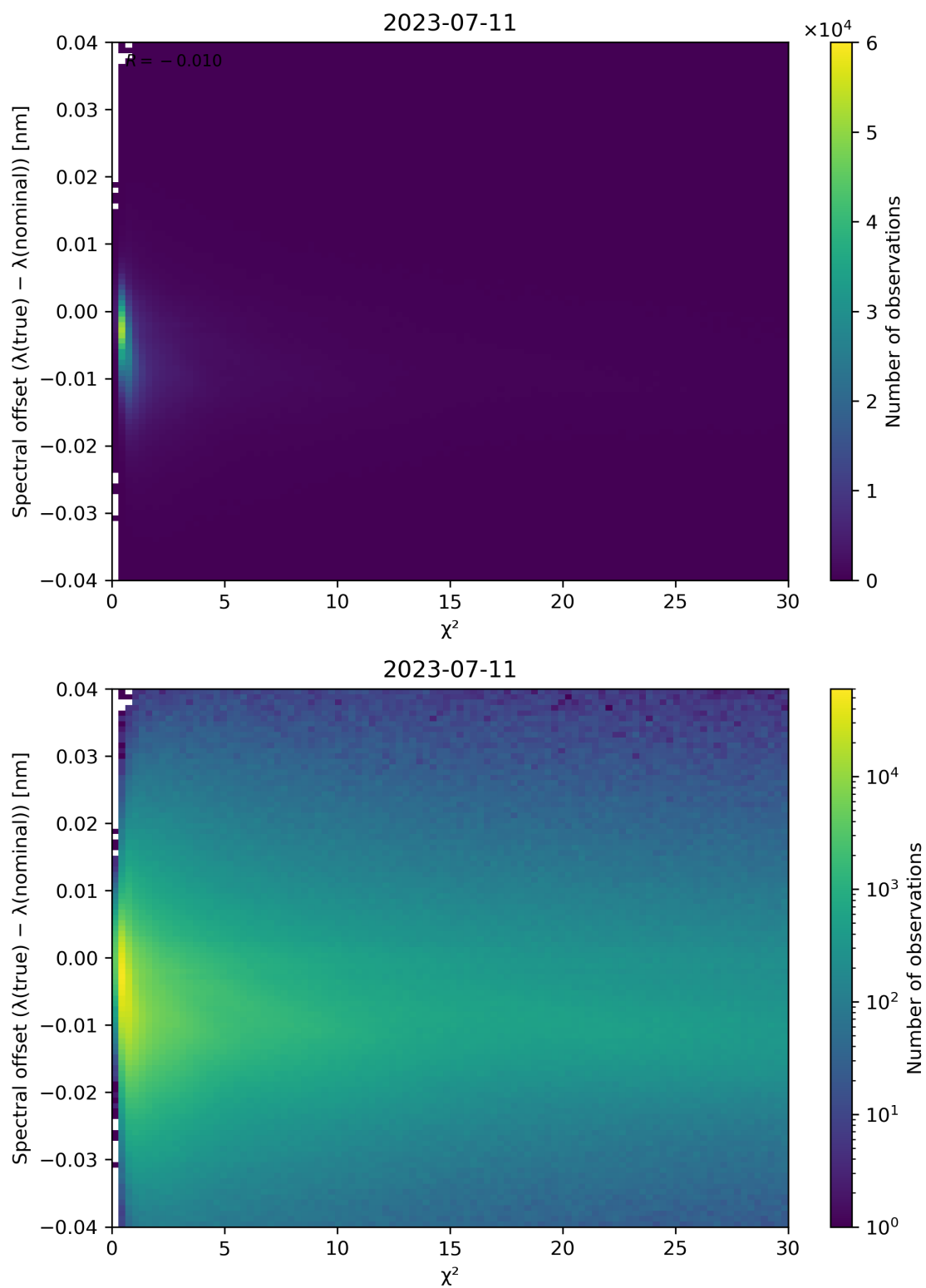
Figure 75: Scatter density plot of “ \chi^2 ” against “Spectral offset ( \lambda(\text{true}) - \lambda(\text{nominal}) )” for 2023-07-10 to 2023-07-12.
