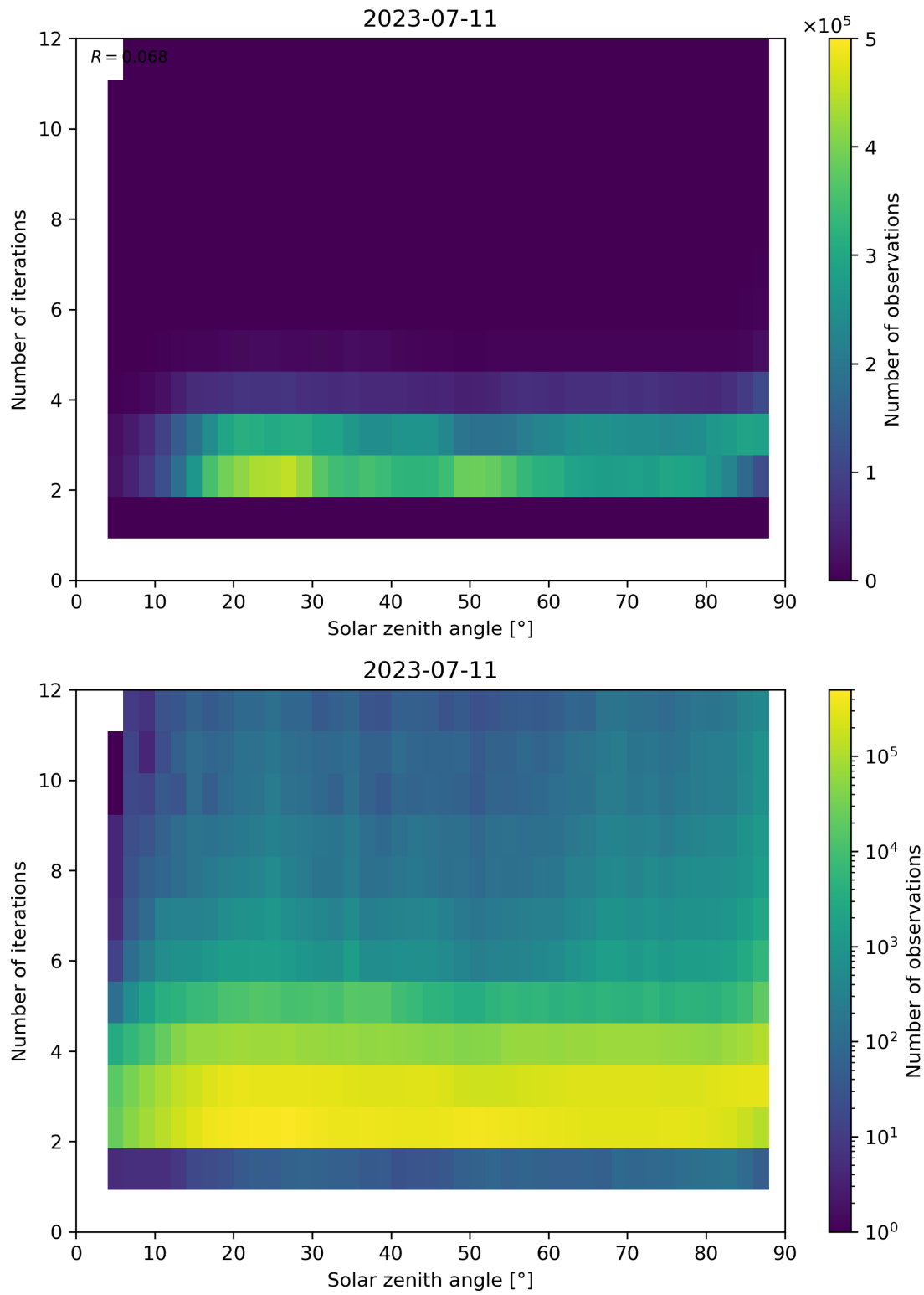
Figure 125: Scatter density plot of “Solar zenith angle” against “Number of iterations” for 2023-07-10 to 2023-07-12.
