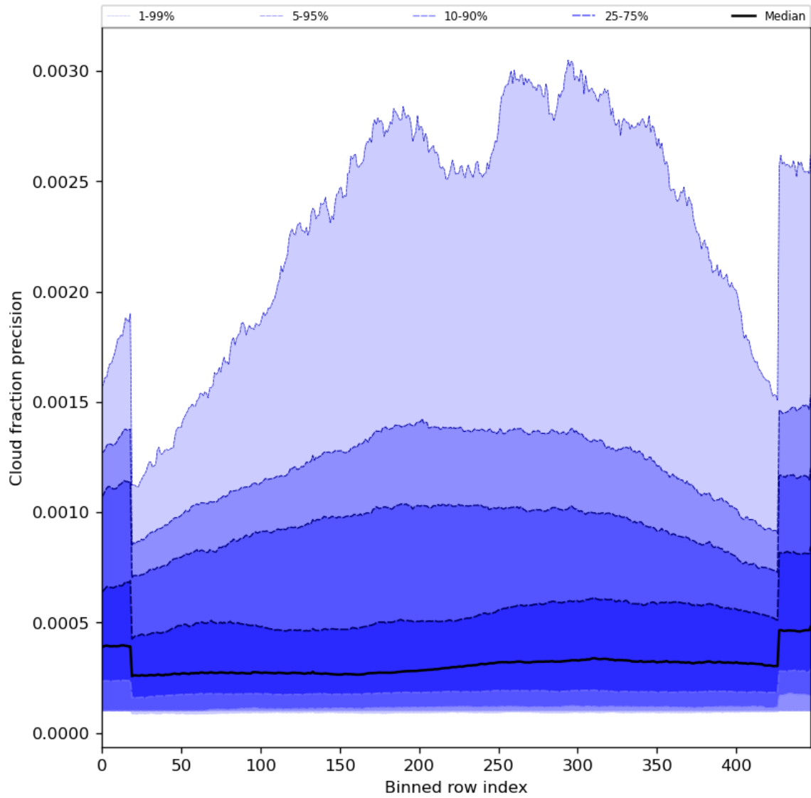
Figure 50: Along track statistics of “Cloud fraction precision” for 2023-07-10 to 2023-07-12
