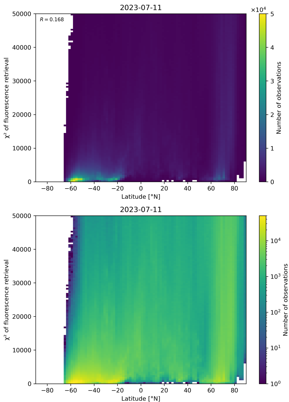
Figure 98: Scatter density plot of “Latitude” against “ \chi^2 of fluorescence retrieval” for 2023-07-10 to 2023-07-12.
