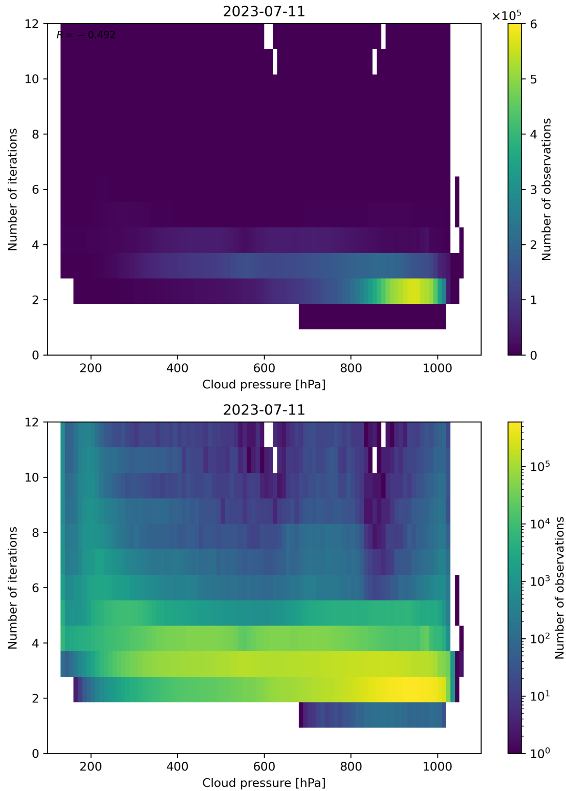
Figure 89: Scatter density plot of “Cloud pressure” against “Number of iterations” for 2023-07-10 to 2023-07-12.
