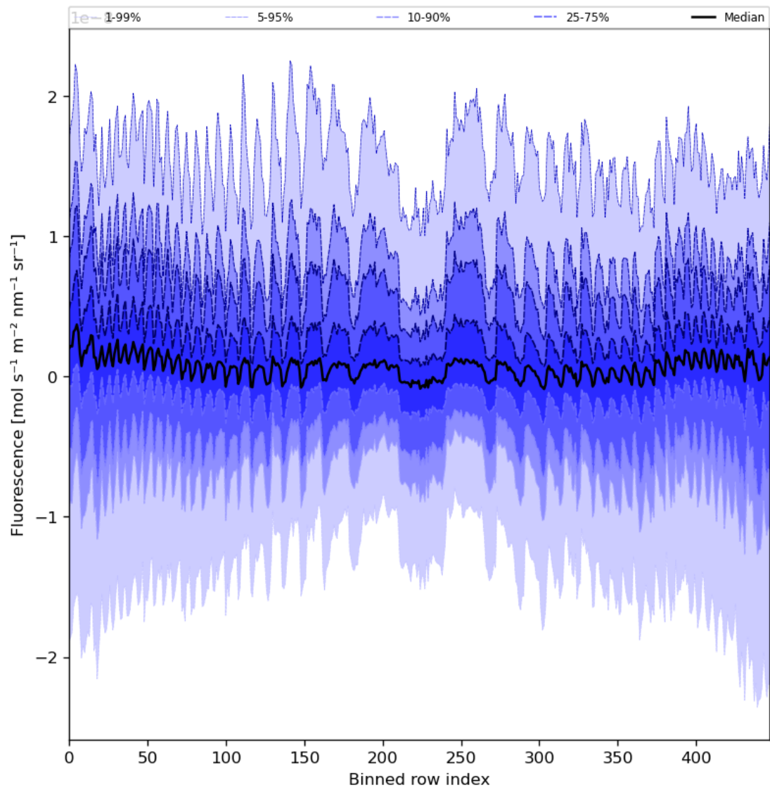
Figure 57: Along track statistics of “Fluorescence” for 2023-07-10 to 2023-07-12
