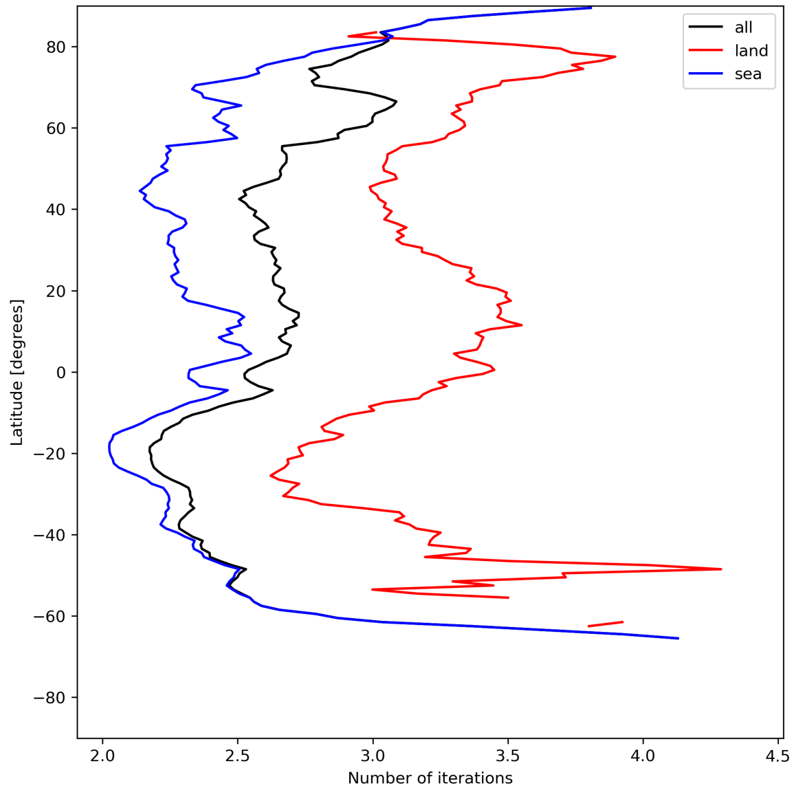
Figure 22: Zonal average of “Number of iterations” for 2023-07-10 to 2023-07-12.
