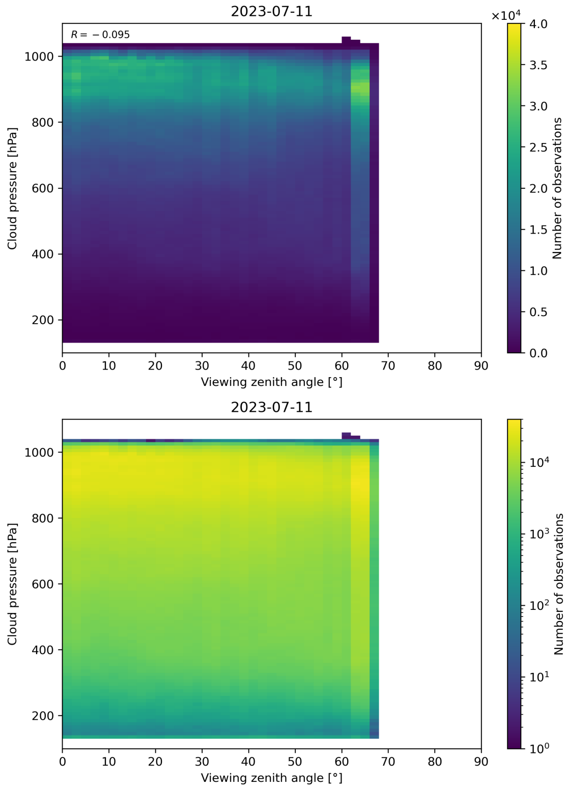
Figure 133: Scatter density plot of “Viewing zenith angle” against “Cloud pressure” for 2023-07-10 to 2023-07-12.
