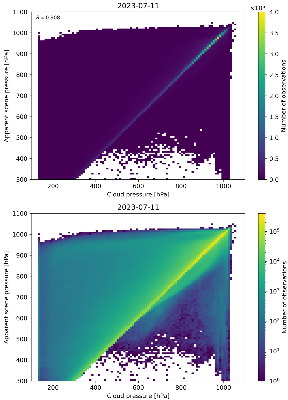
Figure 84: Scatter density plot of “Cloud pressure” against “Apparent scene pressure” for 2023-07-10 to 2023-07-12.
