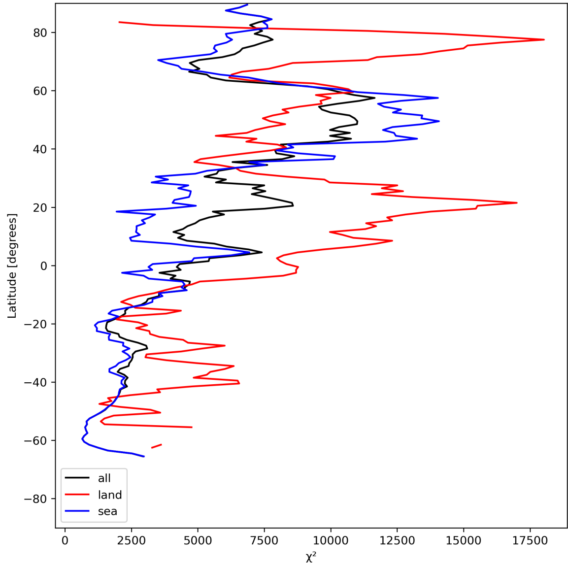
Figure 21: Zonal average of “ \chi^2 ” for 2023-07-10 to 2023-07-12.
