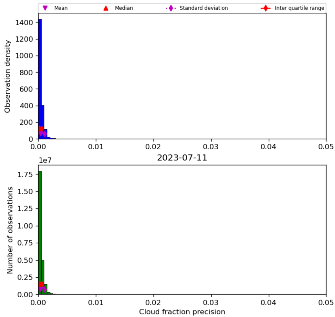
Figure 33: Histogram of “Cloud fraction precision” for 2023-07-10 to 2023-07-12
