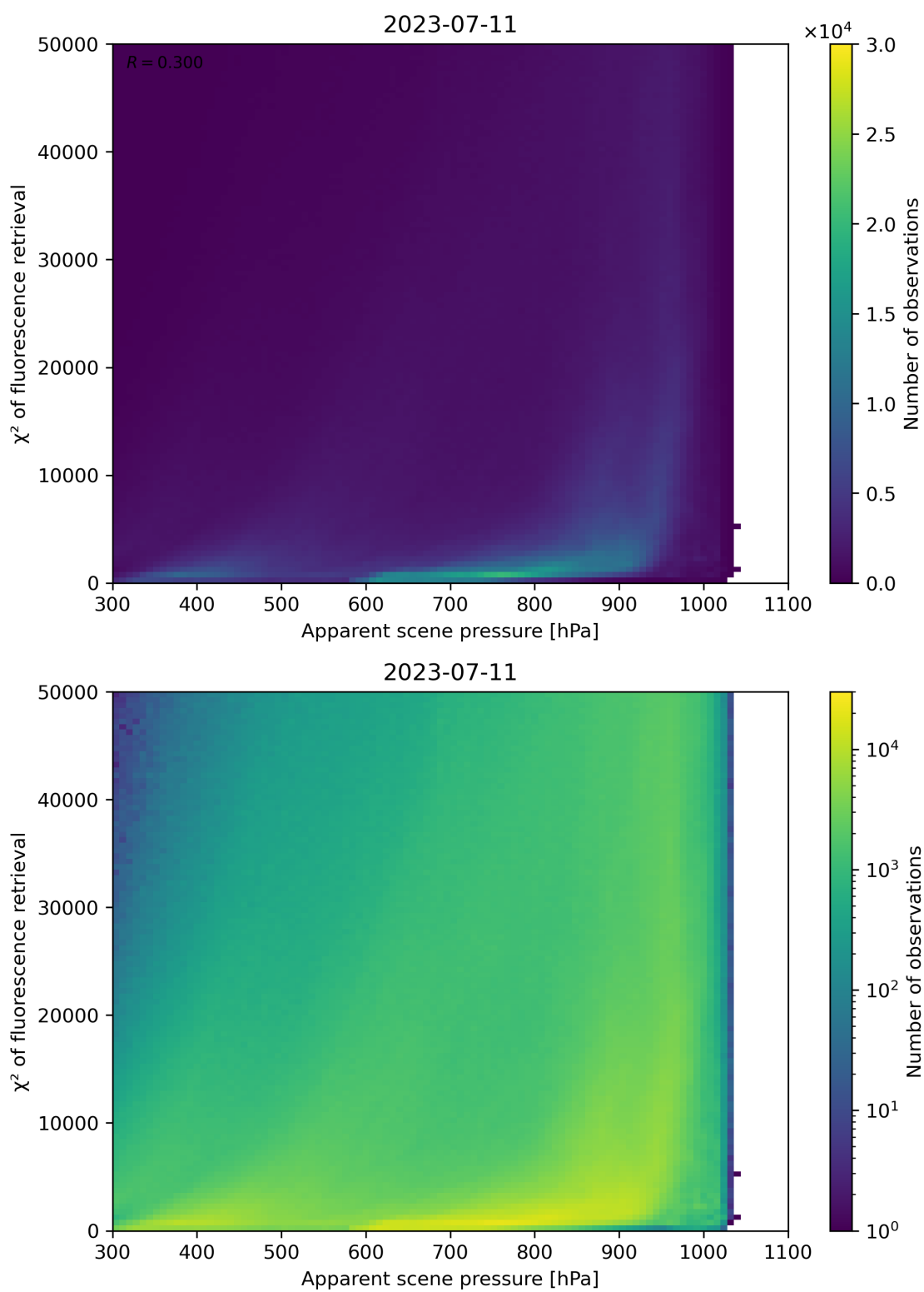
Figure 64: Scatter density plot of “Apparent scene pressure” against “ \chi^2 of fluorescence retrieval” for 2023-07-10 to 2023-07-12.
