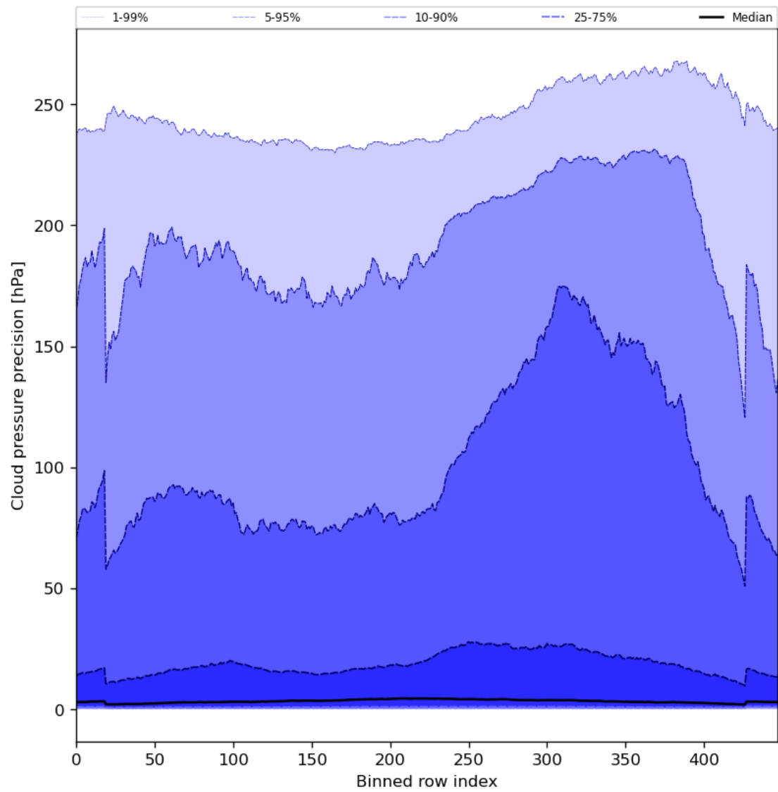
Figure 48: Along track statistics of “Cloud pressure precision” for 2023-07-10 to 2023-07-12
