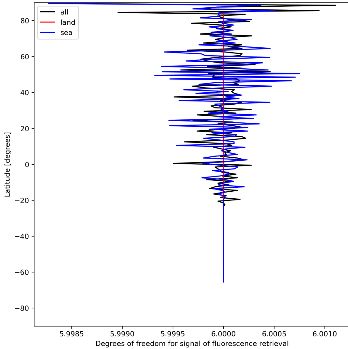
Figure 26: Zonal average of “Degrees of freedom for signal of fluorescence retrieval” for 2023-07-10 to 2023-07-12.
