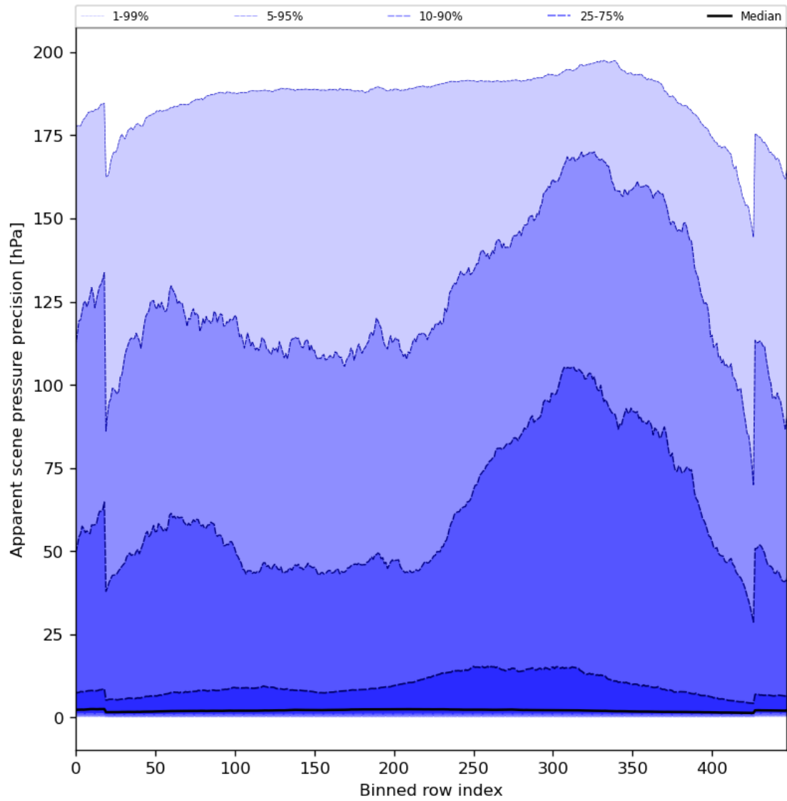
Figure 54: Along track statistics of “Apparent scene pressure precision” for 2023-07-10 to 2023-07-12
