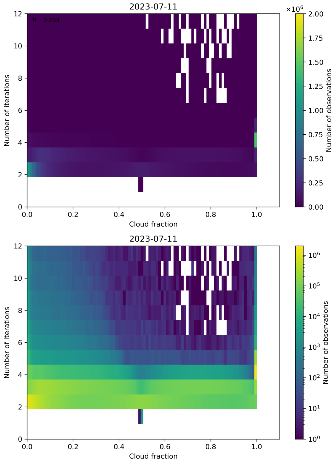
Figure 80: Scatter density plot of “Cloud fraction” against “Number of iterations” for 2023-07-10 to 2023-07-12.
