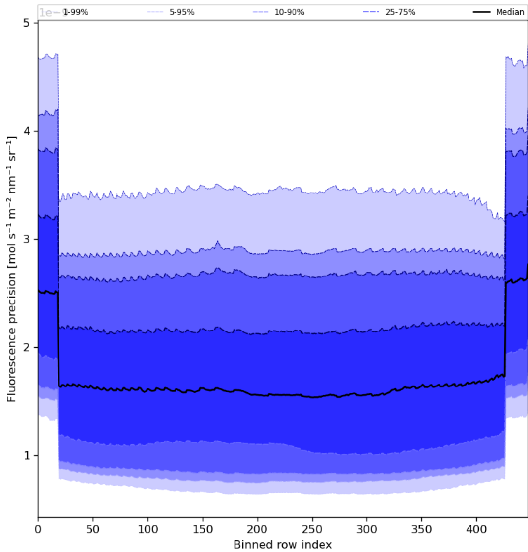
Figure 58: Along track statistics of “Fluorescence precision” for 2023-07-10 to 2023-07-12
