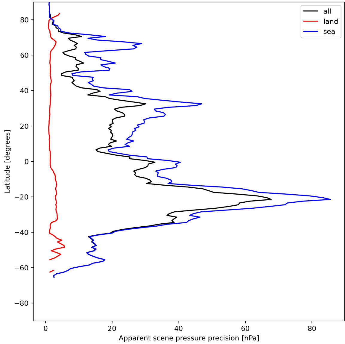
Figure 20: Zonal average of “Apparent scene pressure precision” for 2023-07-10 to 2023-07-12.
