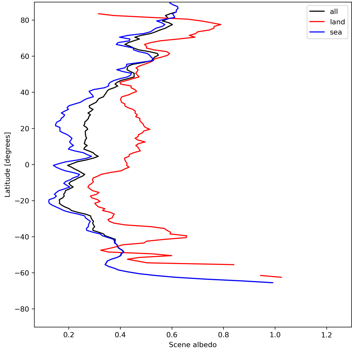
Figure 17: Zonal average of “Scene albedo” for 2023-07-10 to 2023-07-12.
