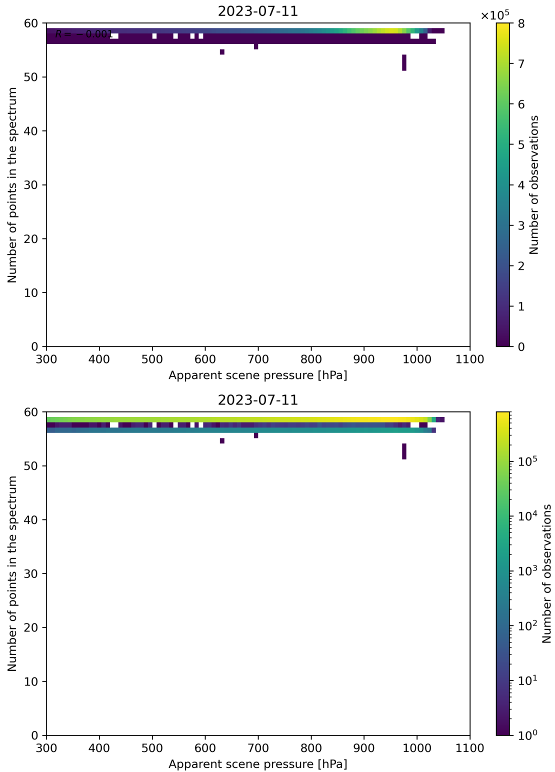
Figure 67: Scatter density plot of “Apparent scene pressure” against “Number of points in the spectrum” for 2023-07-10 to 2023-07-12.
