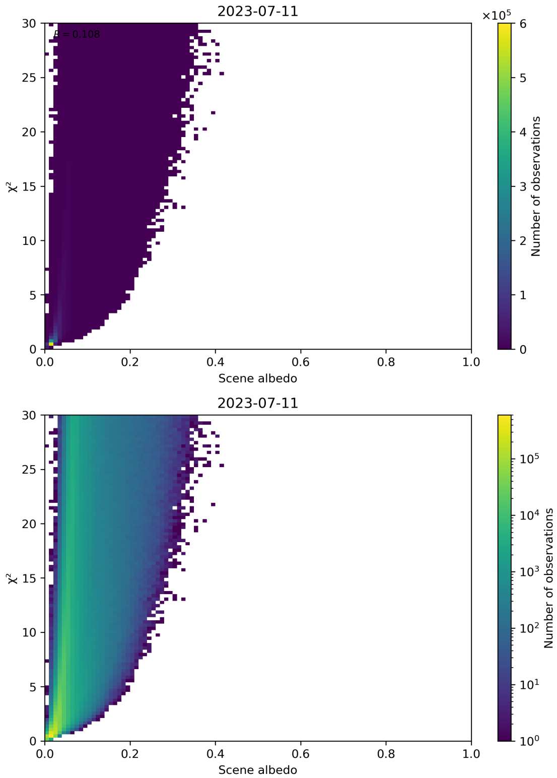
Figure 112: Scatter density plot of “Scene albedo” against “ \chi^2 ” for 2023-07-10 to 2023-07-12.
