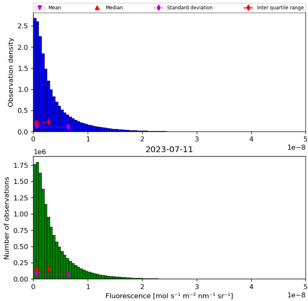
Figure 40: Histogram of “Fluorescence” for 2023-07-10 to 2023-07-12
