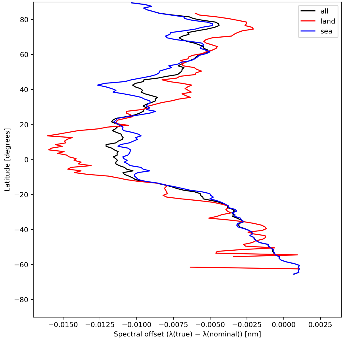
Figure 28: Zonal average of “Spectral offset ( \lambda(\text{true}) - \lambda(\text{nominal}) )” for 2023-07-10 to 2023-07-12.
