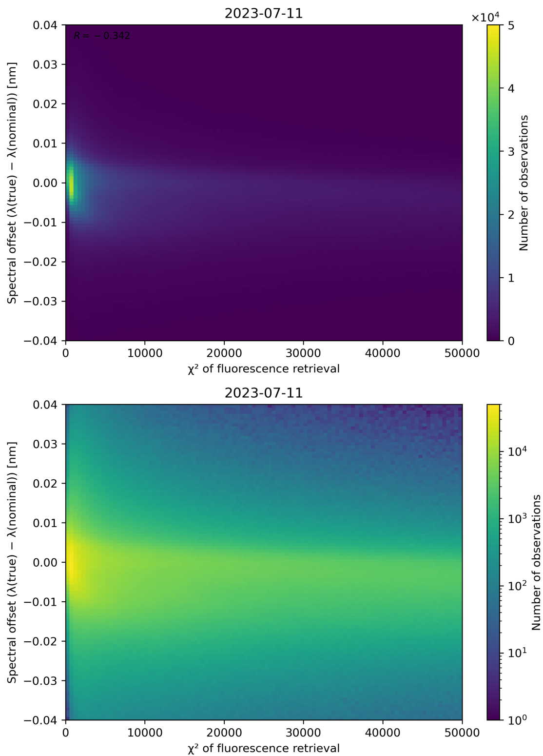
Figure 72: Scatter density plot of " \chi^2 of fluorescence retrieval" against "Spectral offset ( \lambda(\text{true}) - \lambda(\text{nominal}) )" for 2023-07-10 to 2023-07-12.
