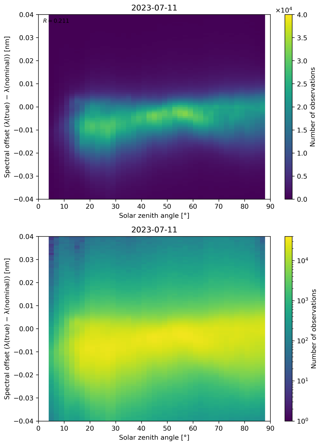
Figure 128: Scatter density plot of “Solar zenith angle” against “Spectral offset ( \lambda(\text{true}) - \lambda(\text{nominal}) )” for 2023-07-10 to 2023-07-12.
