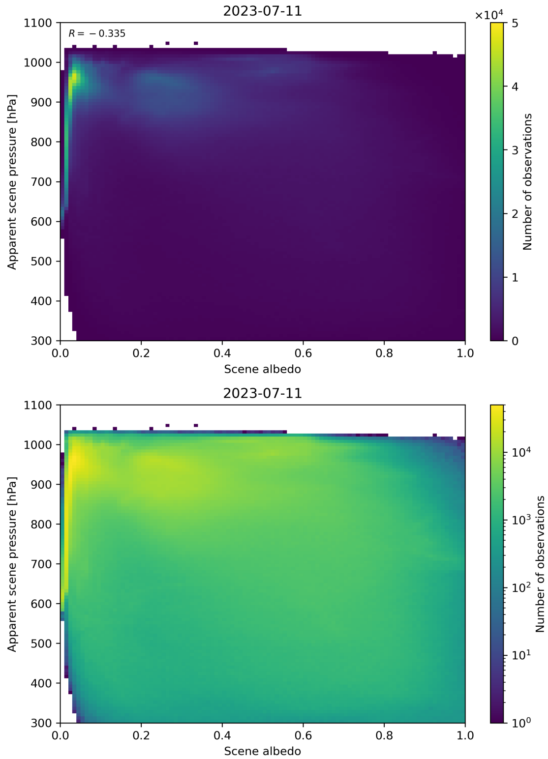
Figure 111: Scatter density plot of “Scene albedo” against “Apparent scene pressure” for 2023-07-10 to 2023-07-12.
