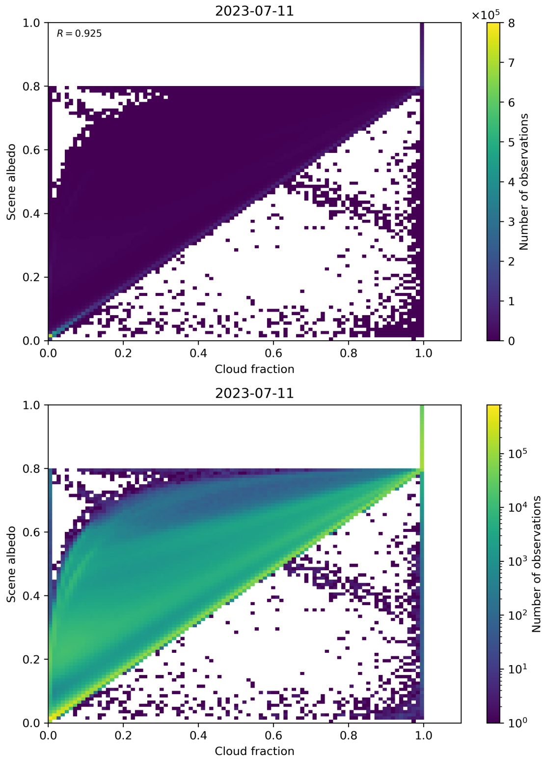
Figure 82: Scatter density plot of “Cloud fraction” against “Scene albedo” for 2023-07-10 to 2023-07-12.
