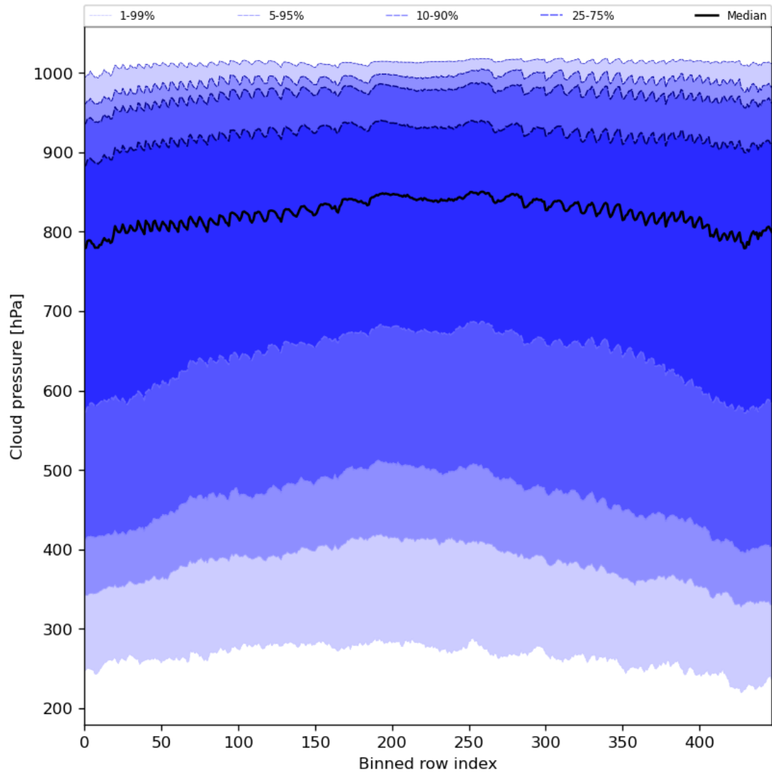
Figure 47: Along track statistics of “Cloud pressure” for 2023-07-10 to 2023-07-12
