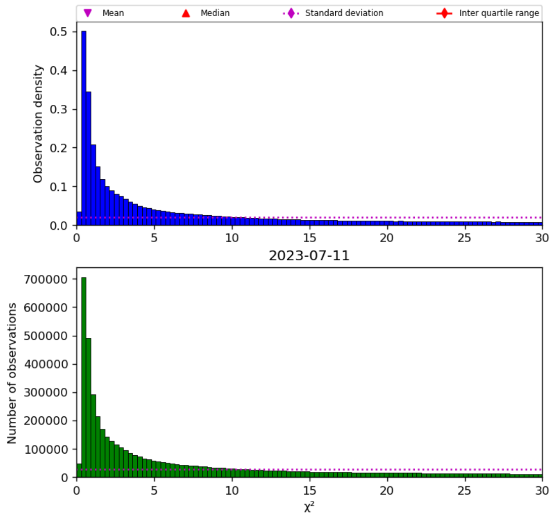
Figure 38: Histogram of “ \chi^2 ” for 2023-07-10 to 2023-07-12
