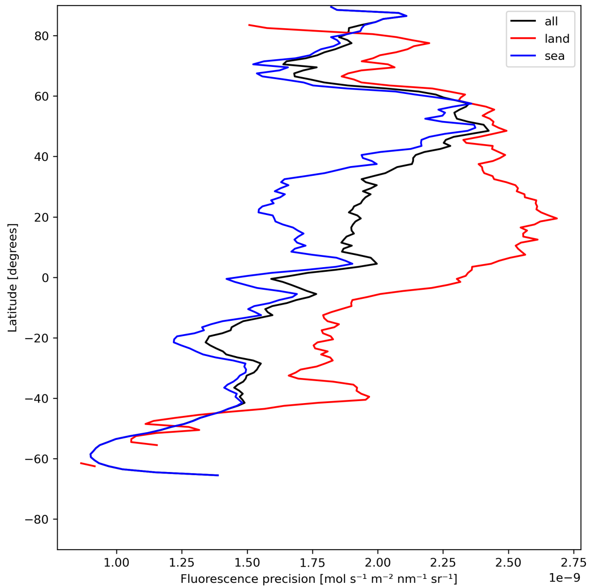
Figure 24: Zonal average of “Fluorescence precision” for 2023-07-10 to 2023-07-12.
