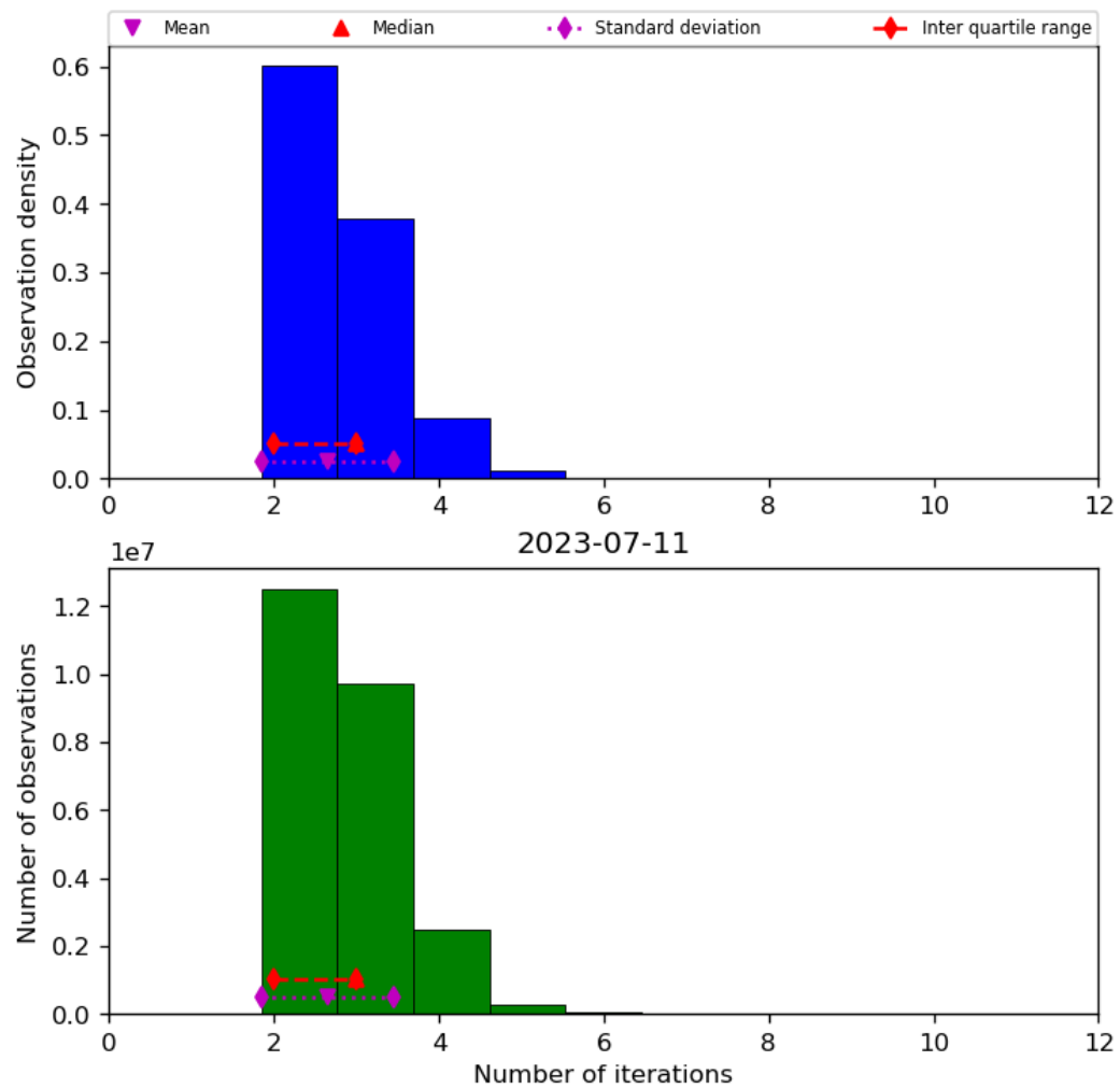
Figure 39: Histogram of “Number of iterations” for 2023-07-10 to 2023-07-12
