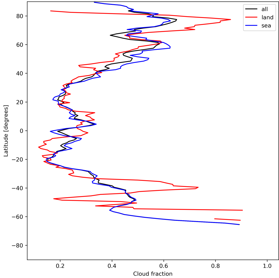
Figure 15: Zonal average of “Cloud fraction” for 2023-07-10 to 2023-07-12.
