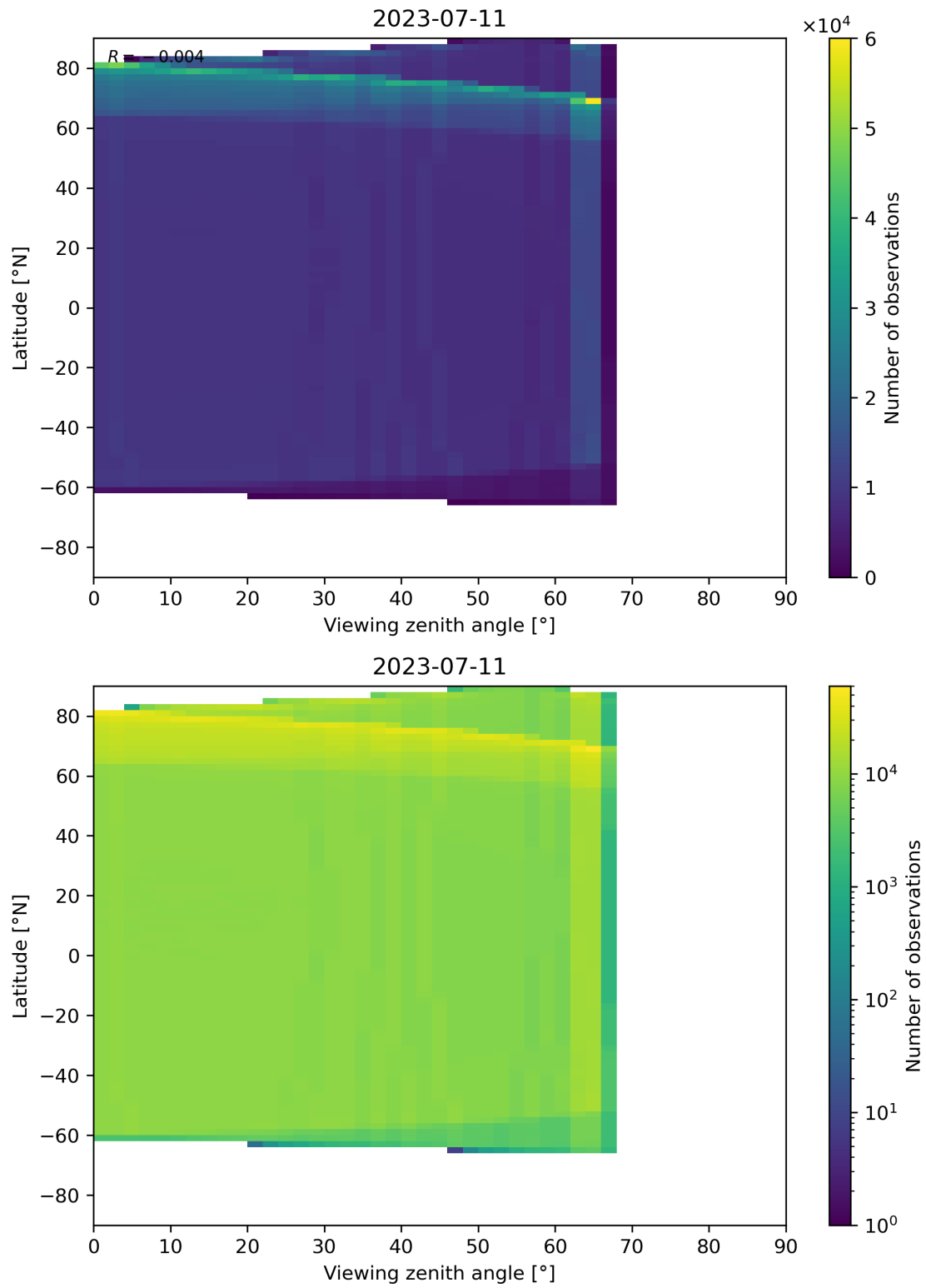
Figure 135: Scatter density plot of “Viewing zenith angle” against “Latitude” for 2023-07-10 to 2023-07-12.
