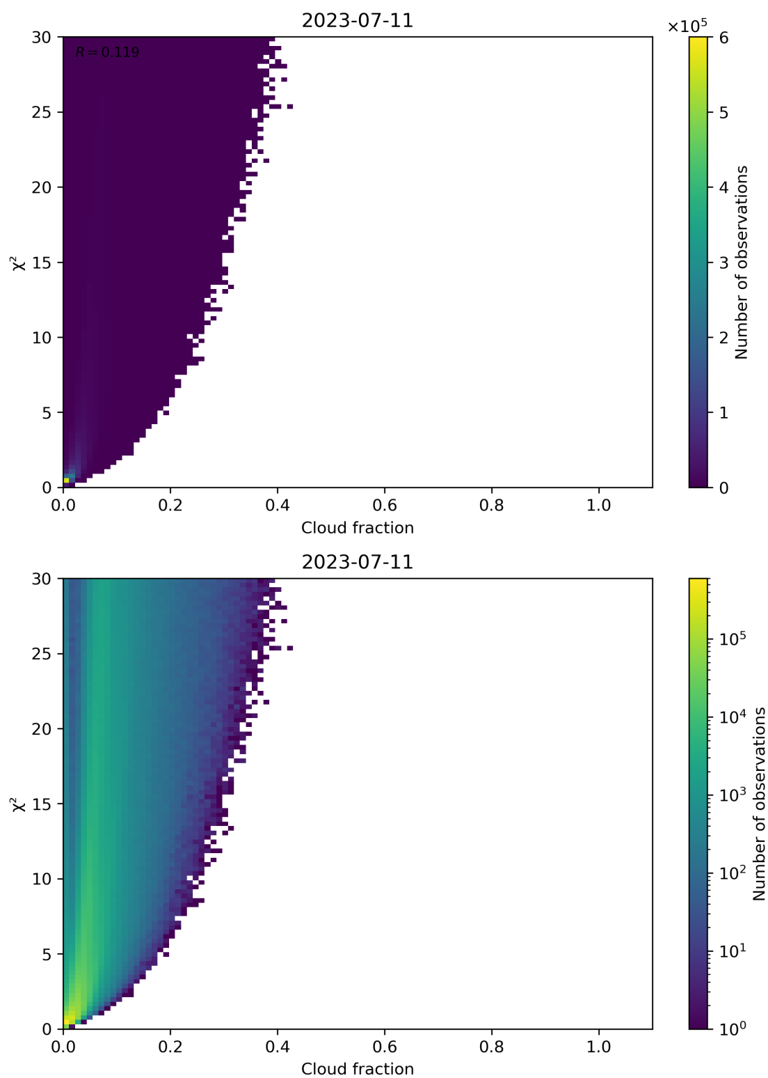
Figure 77: Scatter density plot of “Cloud fraction” against “ \chi^2 ” for 2023-07-10 to 2023-07-12.
