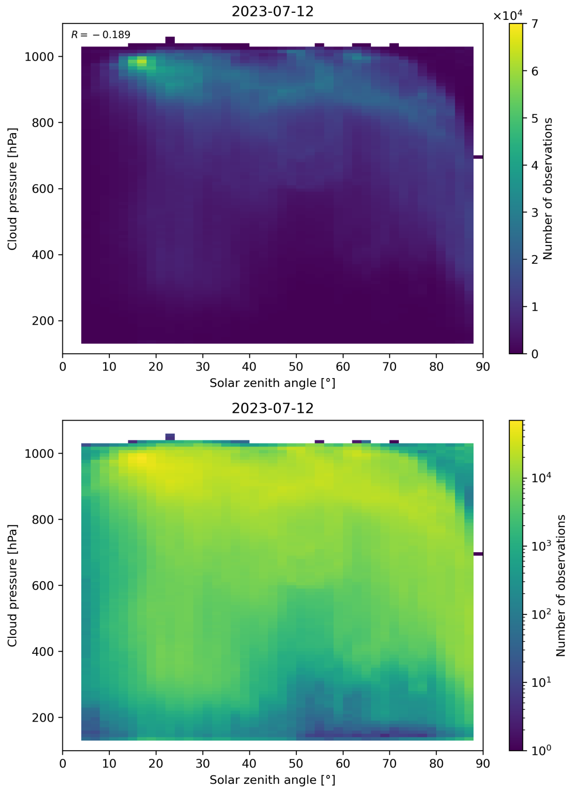
Figure 122: Scatter density plot of “Solar zenith angle” against “Cloud pressure” for 2023-07-11 to 2023-07-13.
