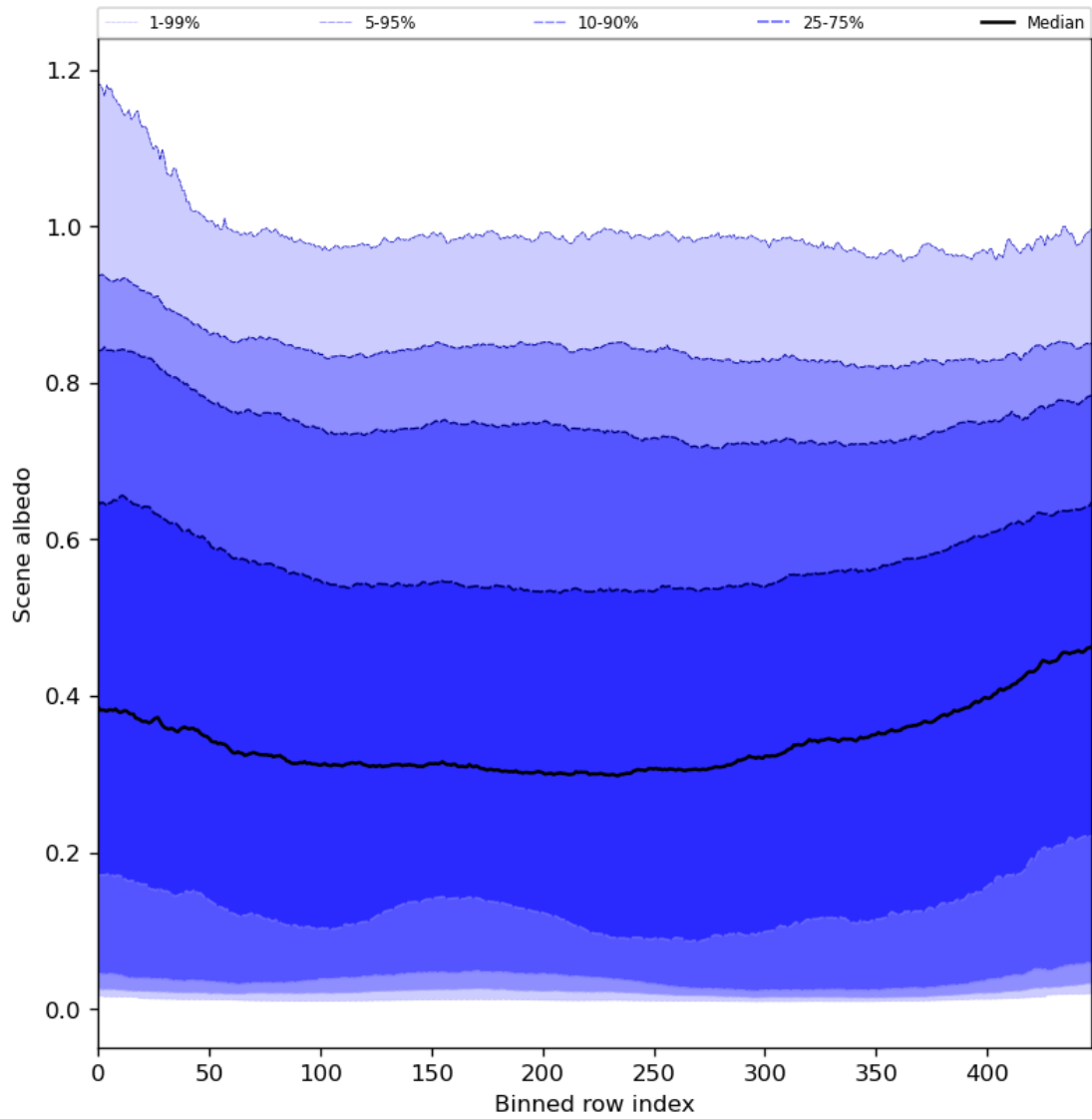
Figure 51: Along track statistics of “Scene albedo” for 2023-07-11 to 2023-07-13
