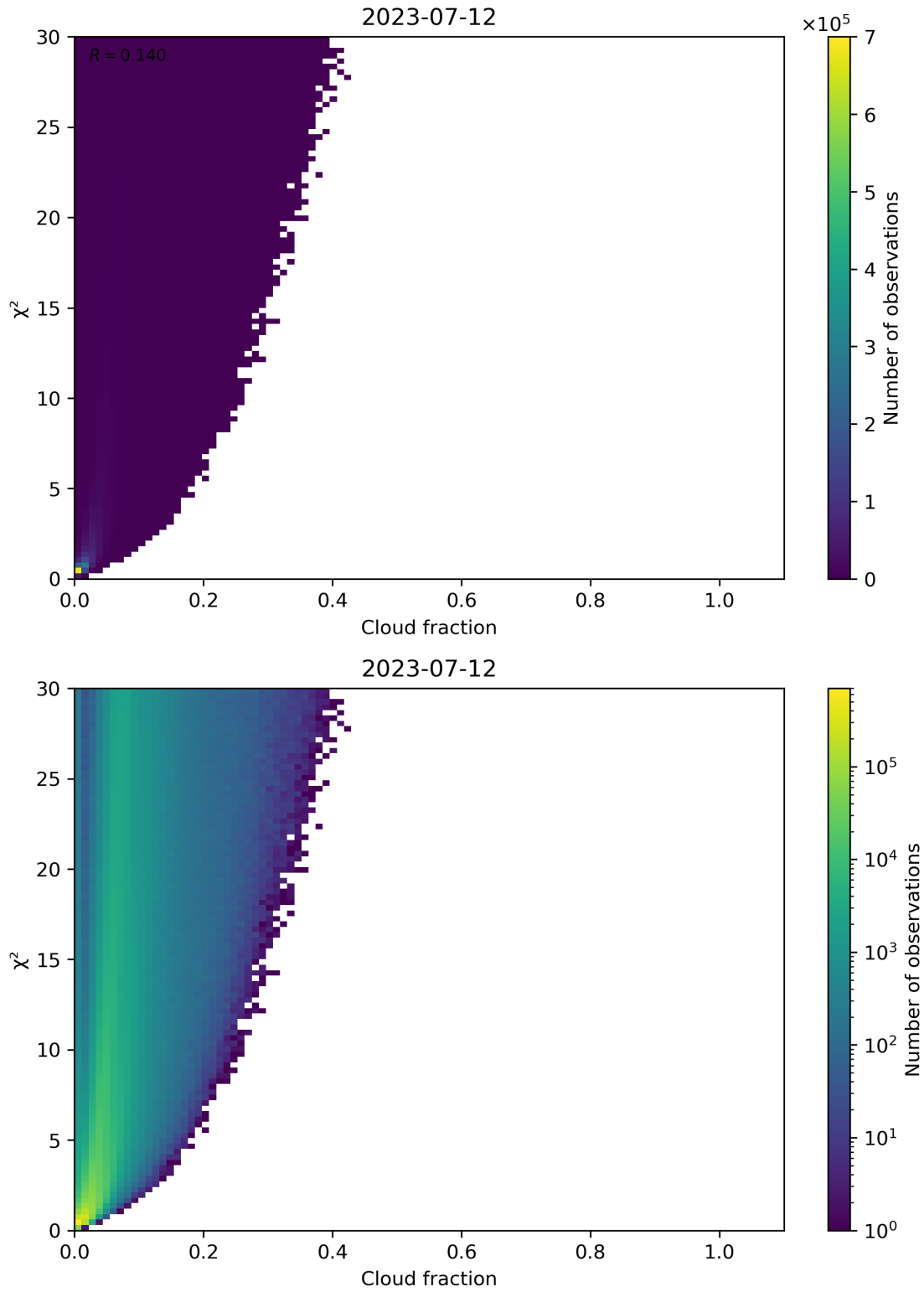
Figure 77: Scatter density plot of “Cloud fraction” against “ \chi^2 ” for 2023-07-11 to 2023-07-13.
