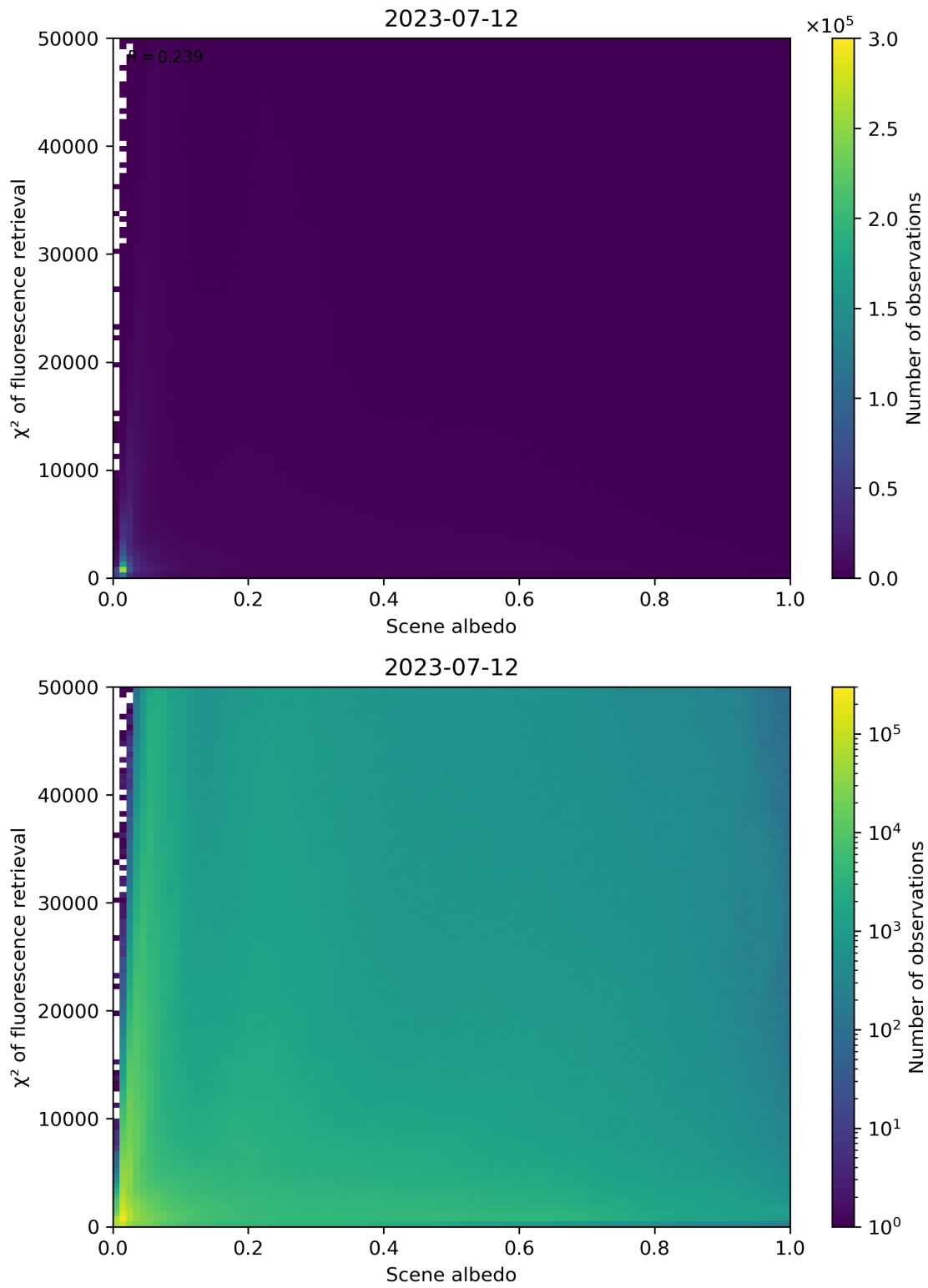
Figure 113: Scatter density plot of “Scene albedo” against “ \chi^2 of fluorescence retrieval” for 2023-07-11 to 2023-07-13.
