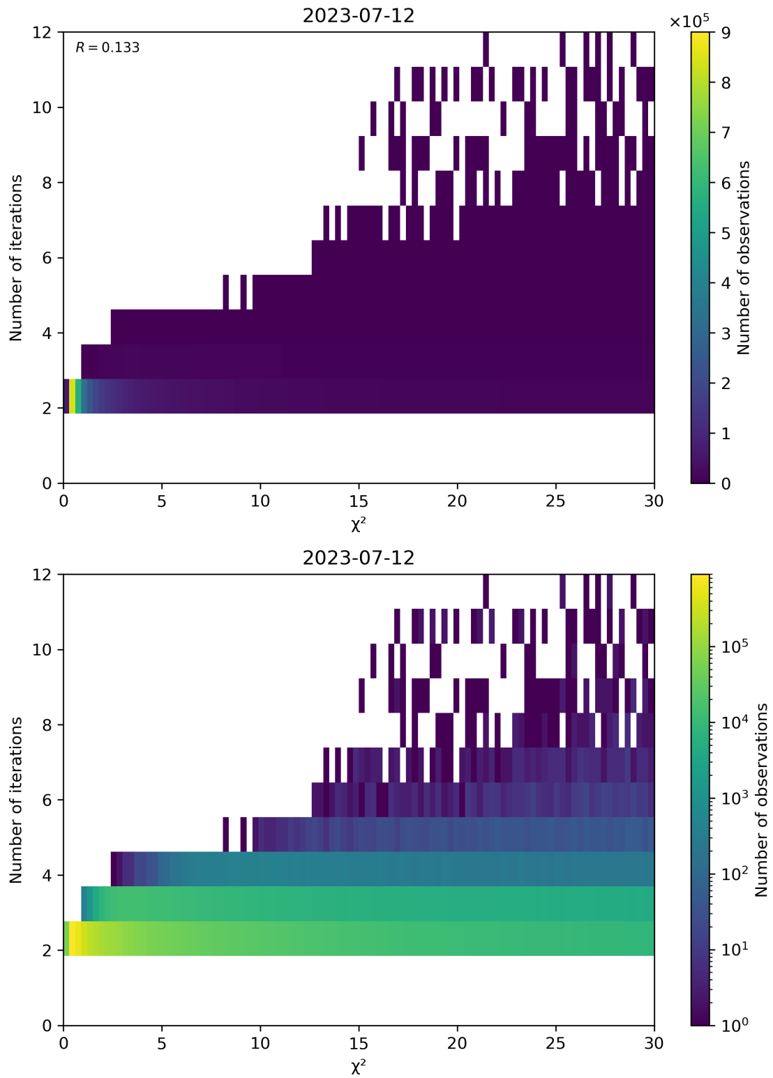
Figure 73: Scatter density plot of “ \chi^2 ” against “Number of iterations” for 2023-07-11 to 2023-07-13.
