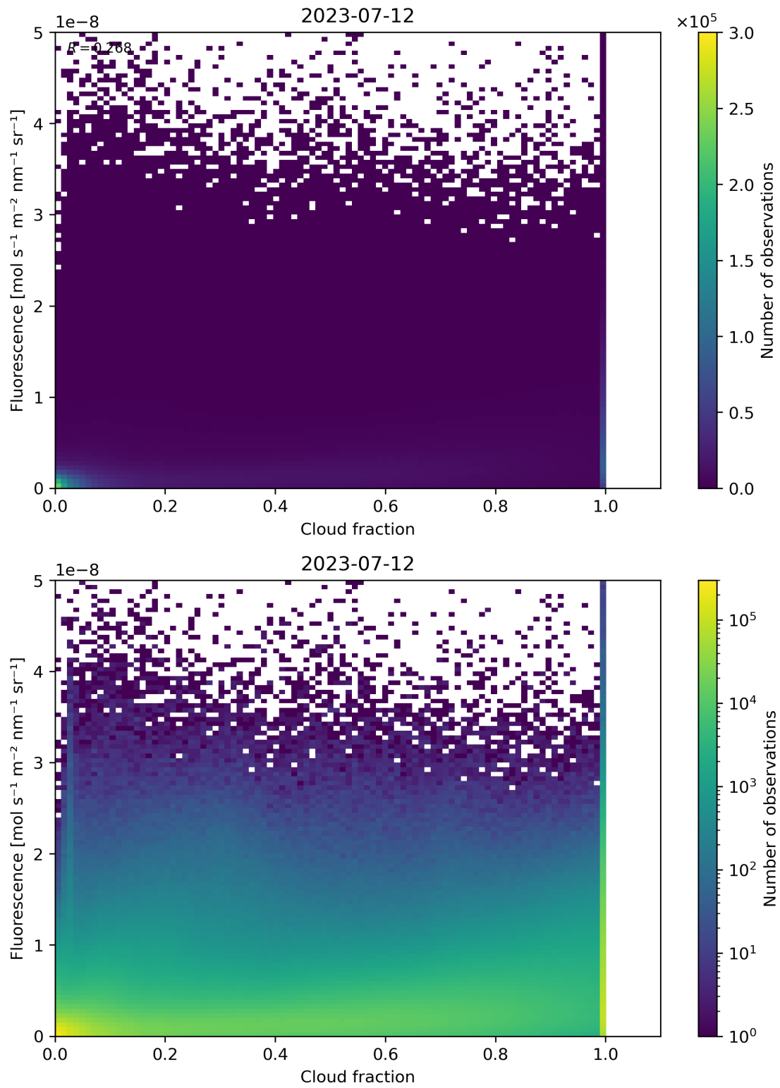
Figure 79: Scatter density plot of “Cloud fraction” against “Fluorescence” for 2023-07-11 to 2023-07-13.
