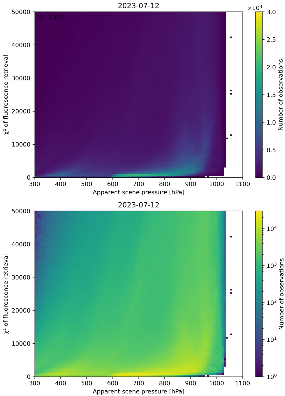
Figure 64: Scatter density plot of “Apparent scene pressure” against “ \chi^2 of fluorescence retrieval” for 2023-07-11 to 2023-07-13.
