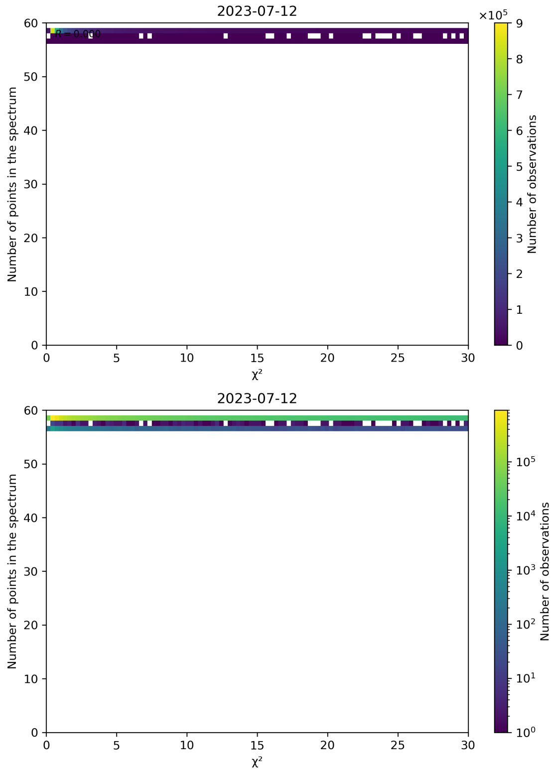
Figure 74: Scatter density plot of " \chi^2 " against "Number of points in the spectrum" for 2023-07-11 to 2023-07-13.
