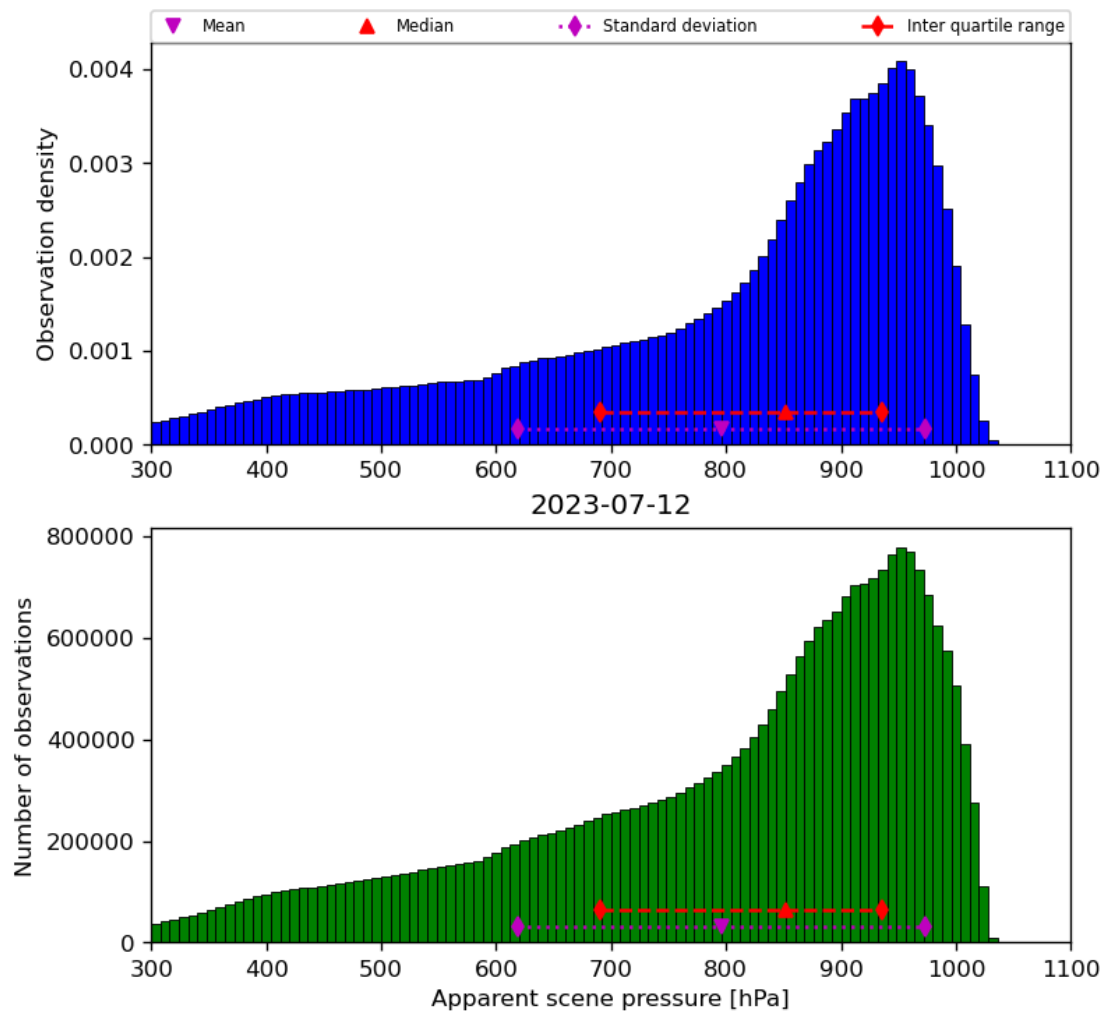
Figure 36: Histogram of “Apparent scene pressure” for 2023-07-11 to 2023-07-13
