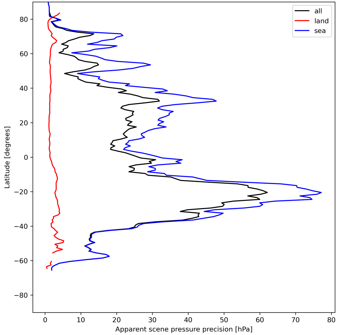
Figure 20: Zonal average of “Apparent scene pressure precision” for 2023-07-11 to 2023-07-13.
