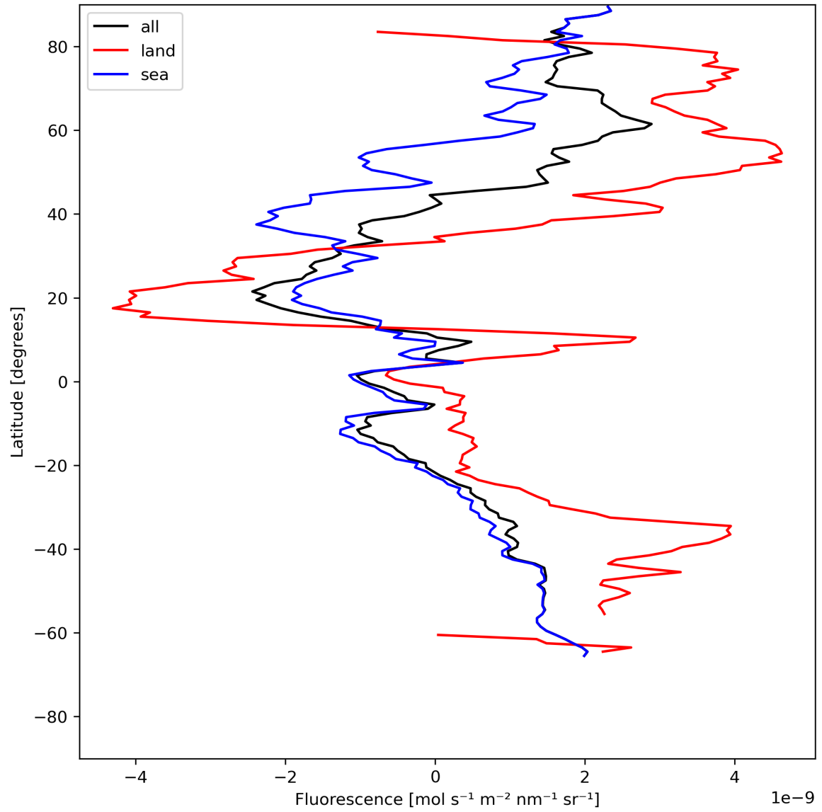
Figure 23: Zonal average of “Fluorescence” for 2023-07-11 to 2023-07-13.
