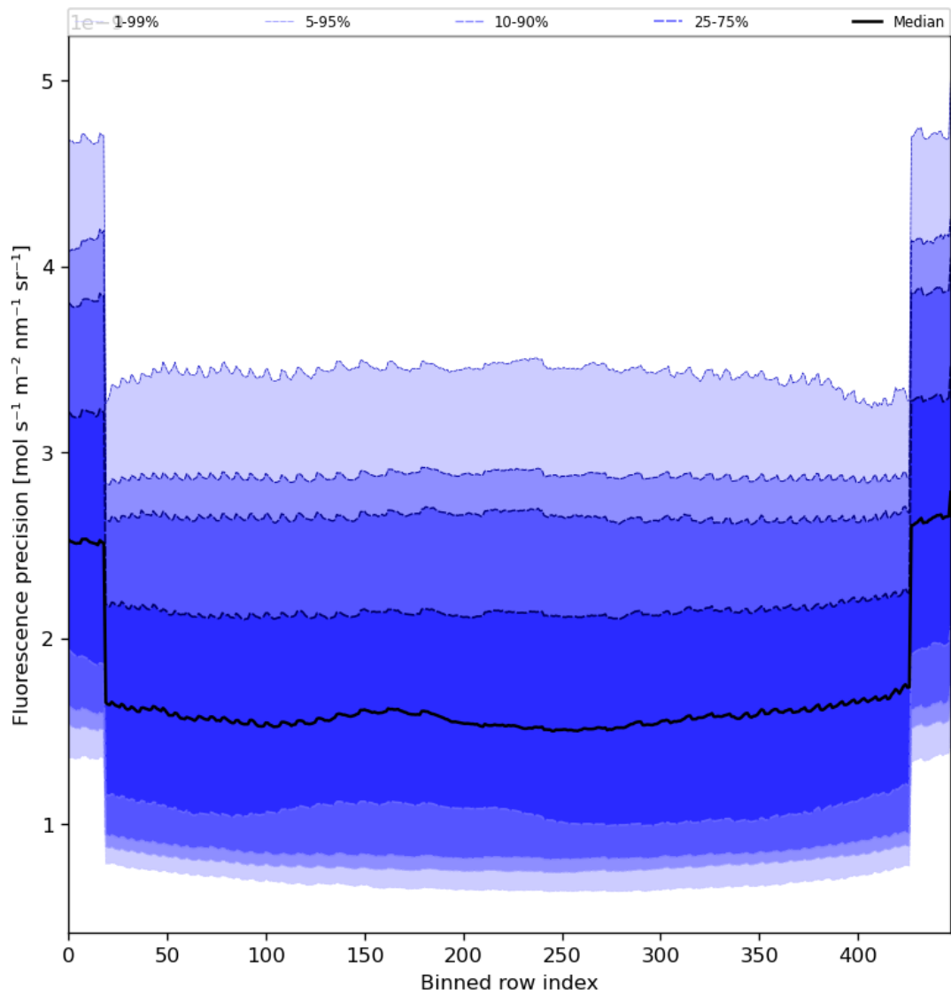
Figure 58: Along track statistics of “Fluorescence precision” for 2023-07-11 to 2023-07-13
