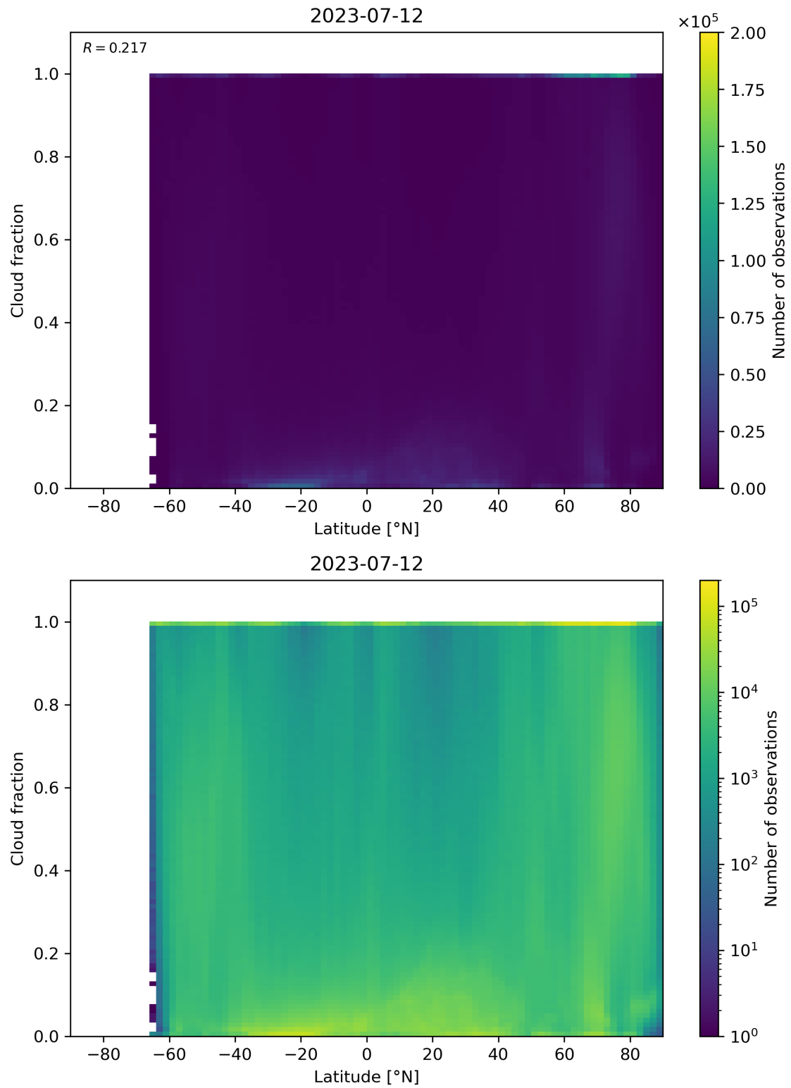
Figure 99: Scatter density plot of “Latitude” against “Cloud fraction” for 2023-07-11 to 2023-07-13.
