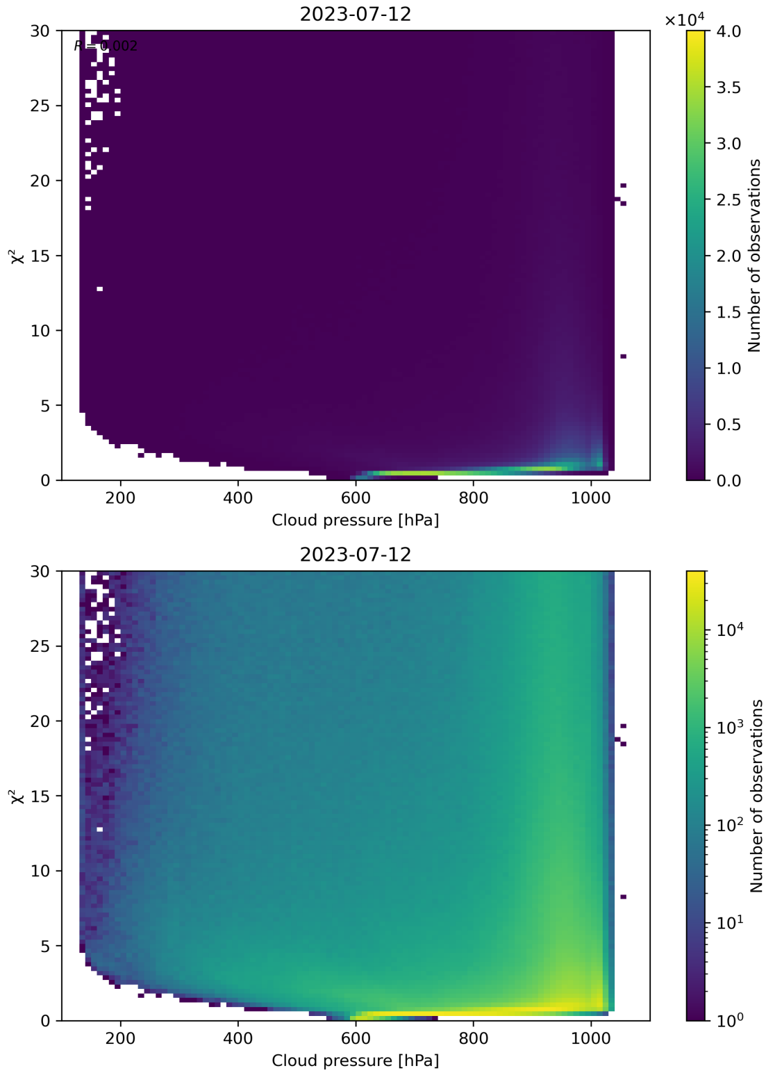
Figure 85: Scatter density plot of “Cloud pressure” against “ \chi^2 ” for 2023-07-11 to 2023-07-13.
