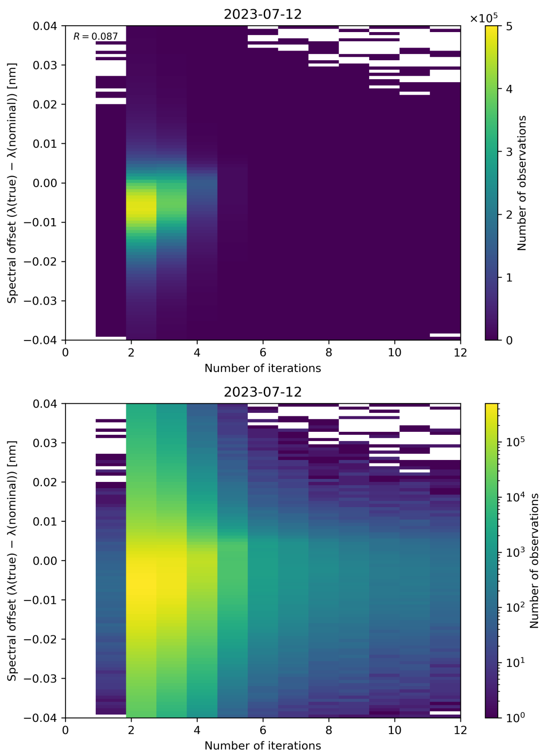
Figure 109: Scatter density plot of “Number of iterations” against “Spectral offset ( \lambda(\text{true}) - \lambda(\text{nominal}) )” for 2023-07-11 to 2023-07-13.
