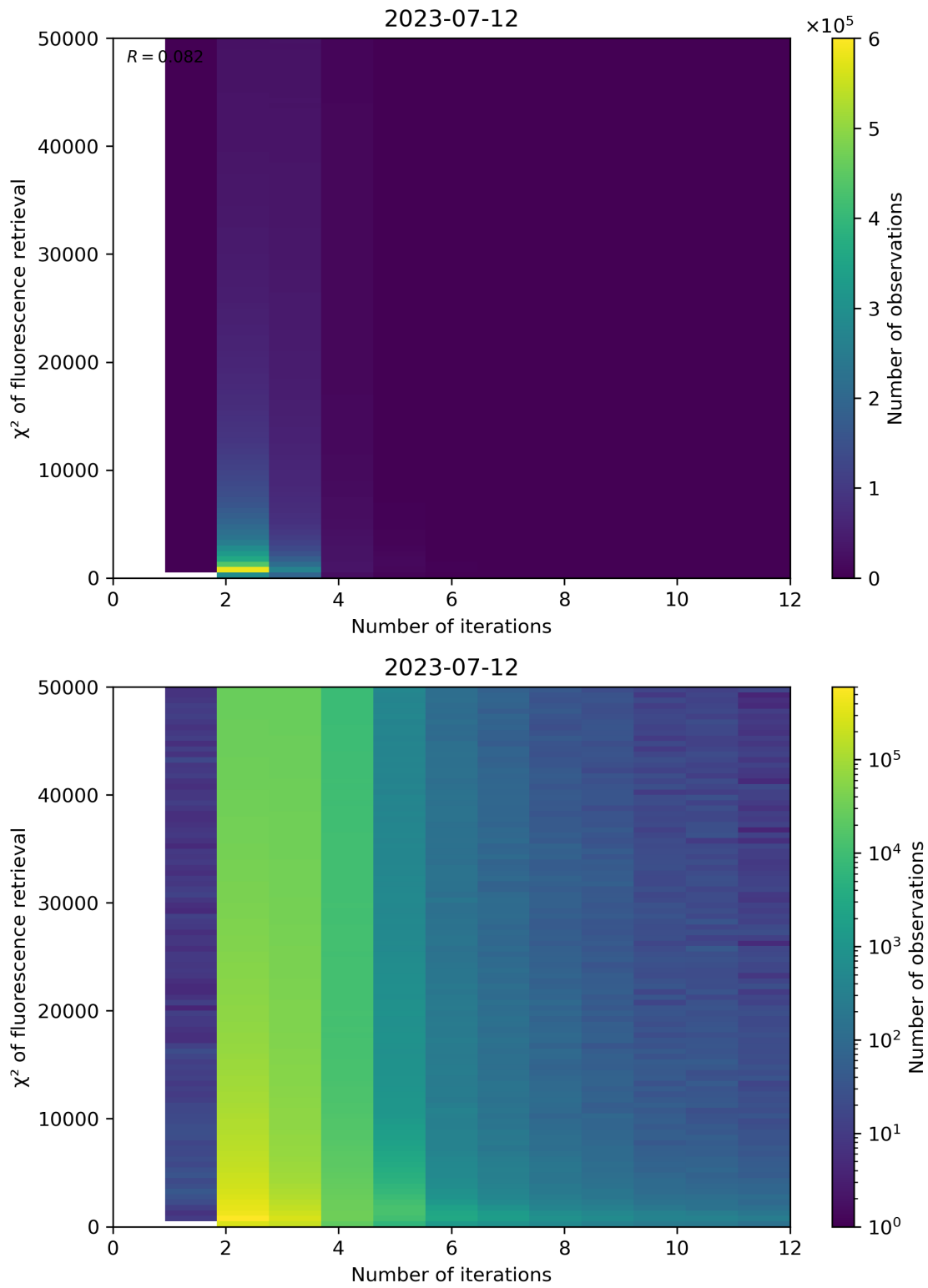
Figure 106: Scatter density plot of “Number of iterations” against “ \chi^2 of fluorescence retrieval” for 2023-07-11 to 2023-07-13.
