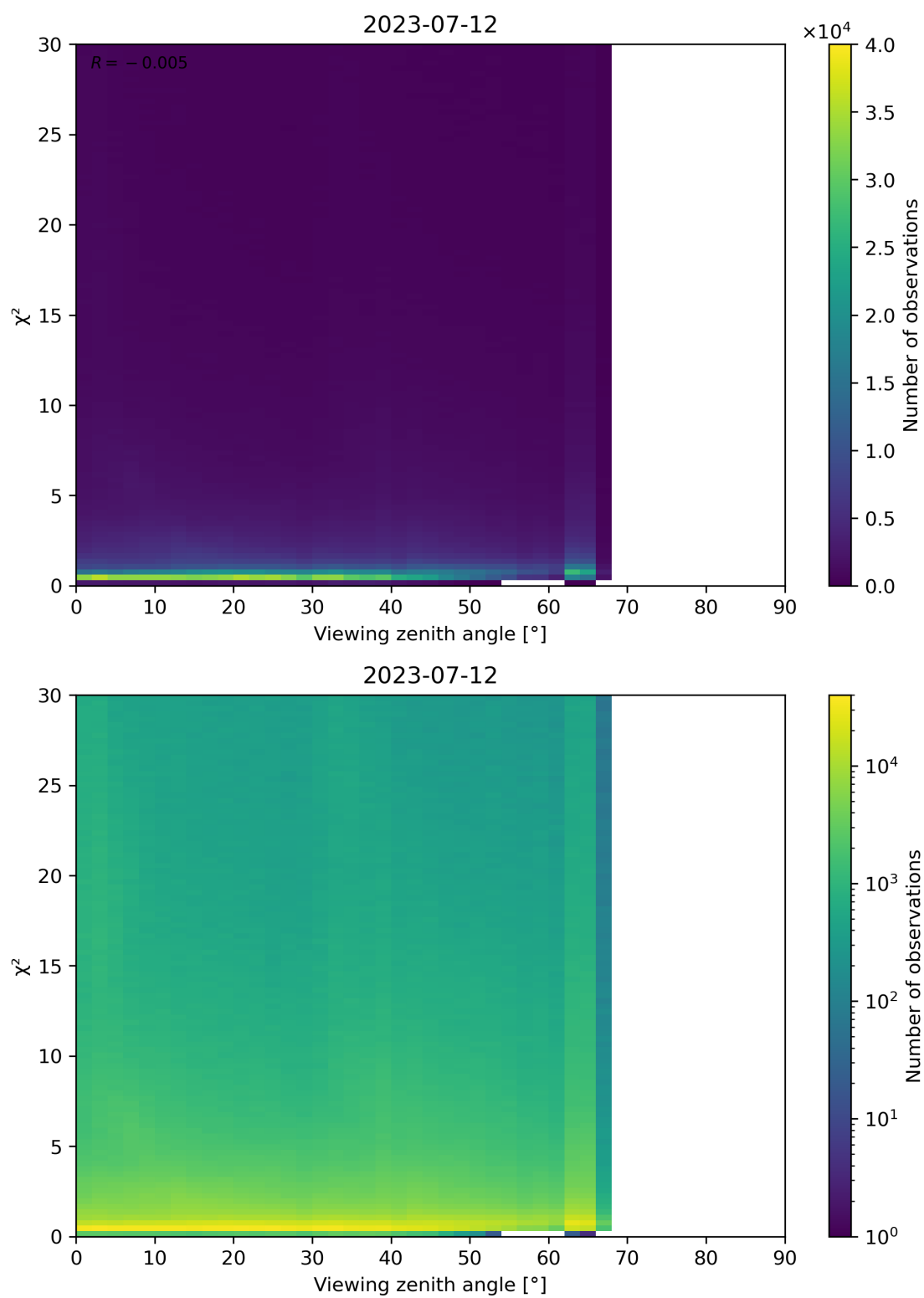
Figure 130: Scatter density plot of “Viewing zenith angle” against “ \chi^2 ” for 2023-07-11 to 2023-07-13.
