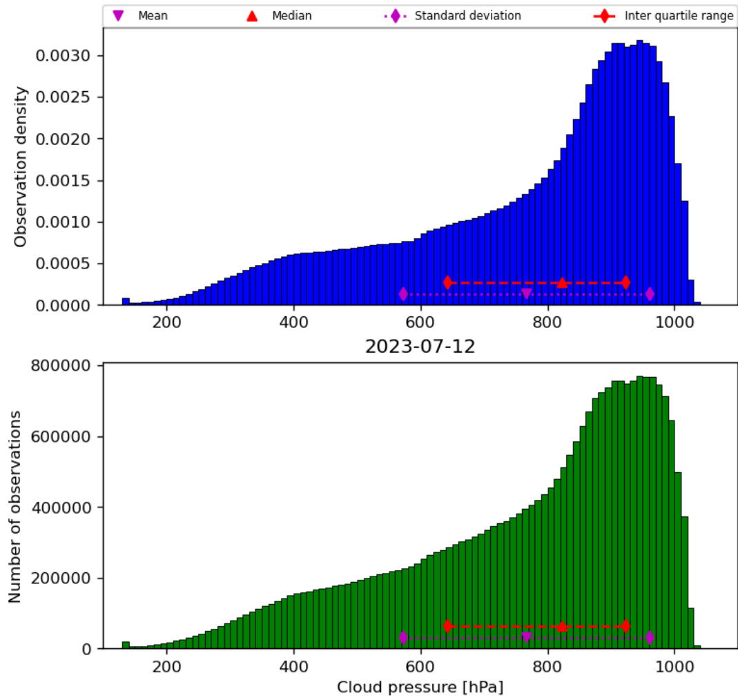
Figure 30: Histogram of “Cloud pressure” for 2023-07-11 to 2023-07-13
