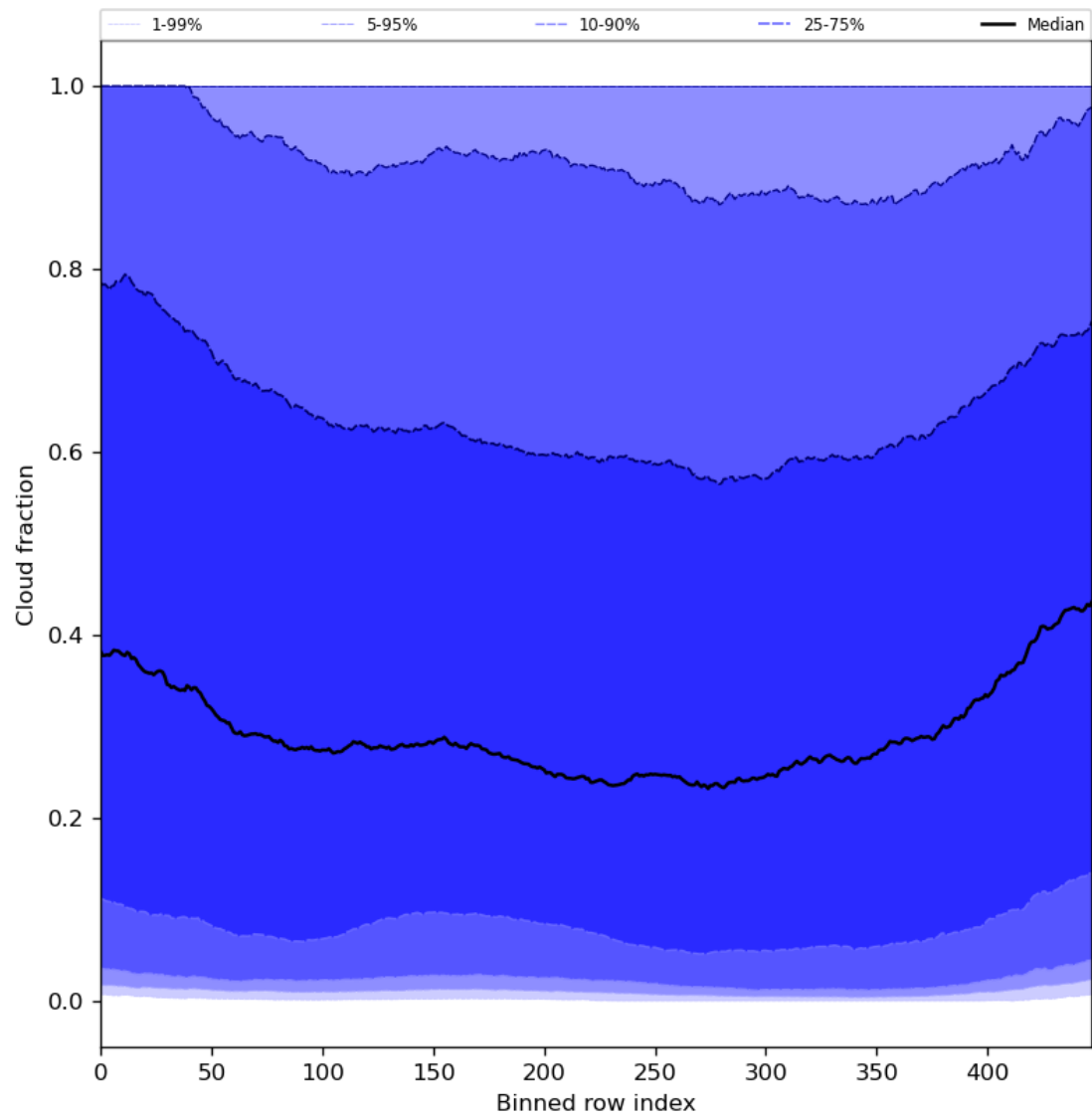
Figure 49: Along track statistics of “Cloud fraction” for 2023-07-11 to 2023-07-13
