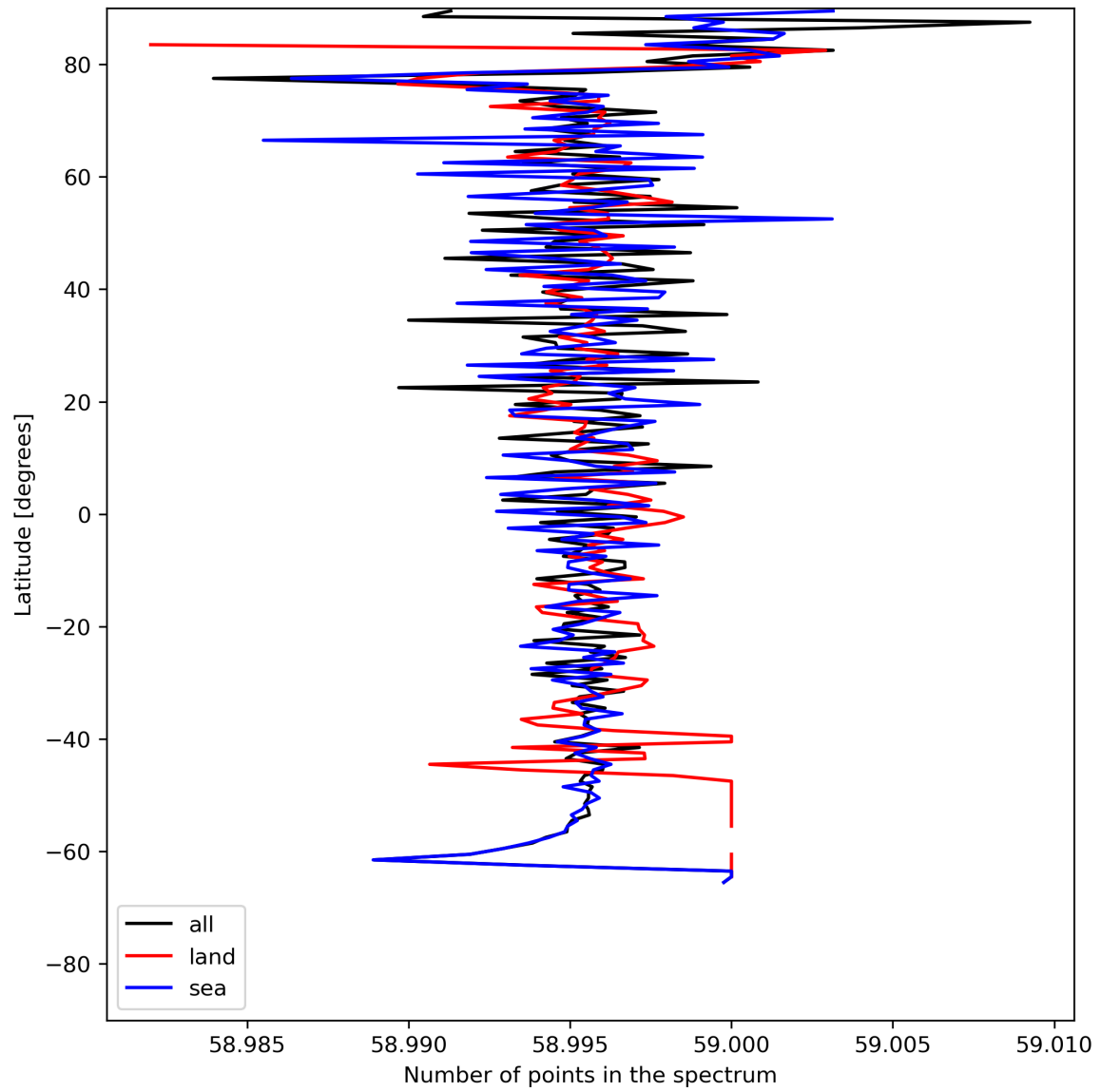
Figure 27: Zonal average of “Number of points in the spectrum” for 2023-07-11 to 2023-07-13.
