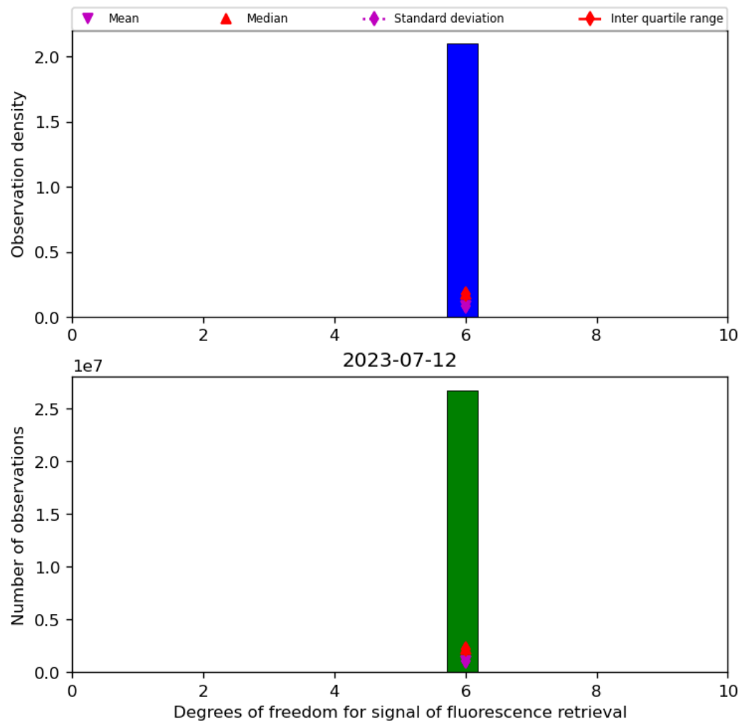
Figure 43: Histogram of “Degrees of freedom for signal of fluorescence retrieval” for 2023-07-11 to 2023-07-13
