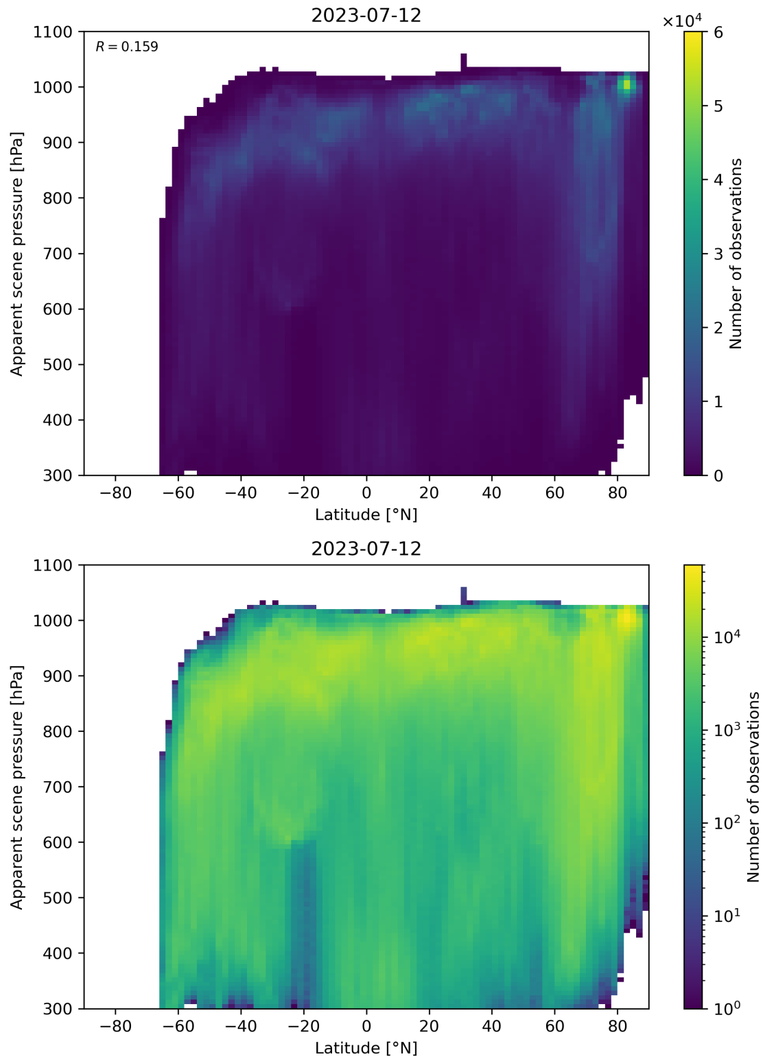
Figure 96: Scatter density plot of “Latitude” against “Apparent scene pressure” for 2023-07-11 to 2023-07-13.
