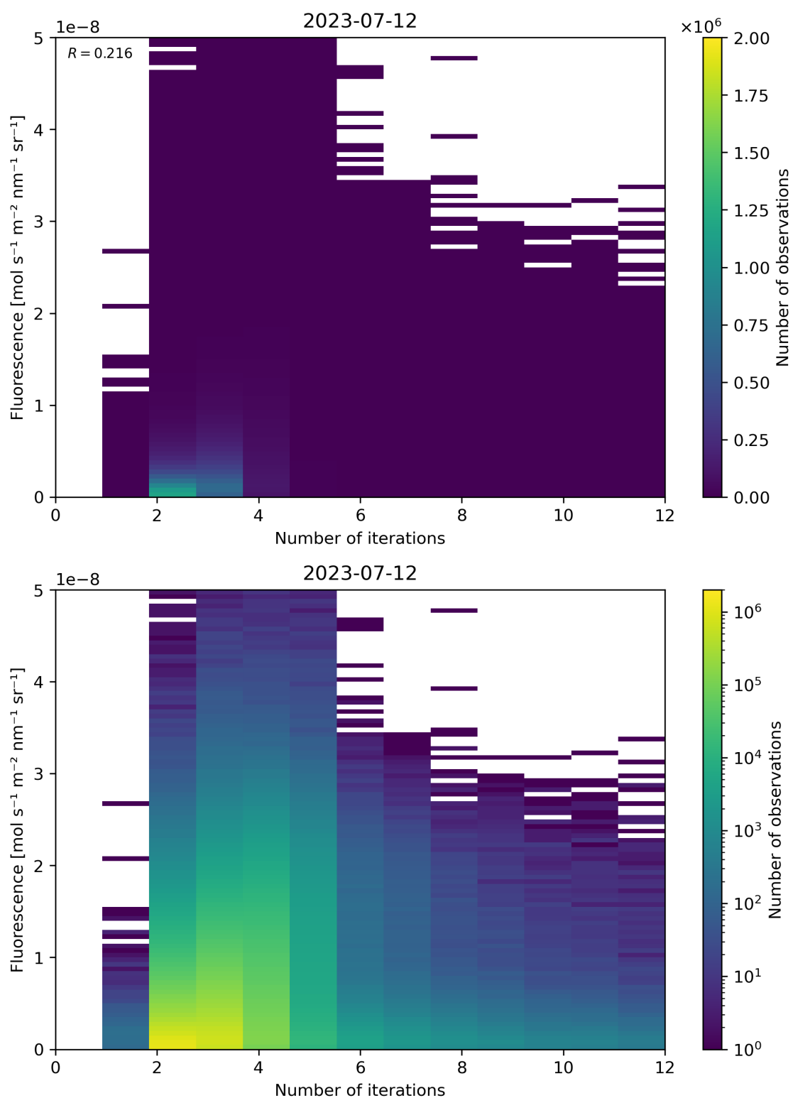
Figure 107: Scatter density plot of “Number of iterations” against “Fluorescence” for 2023-07-11 to 2023-07-13.
