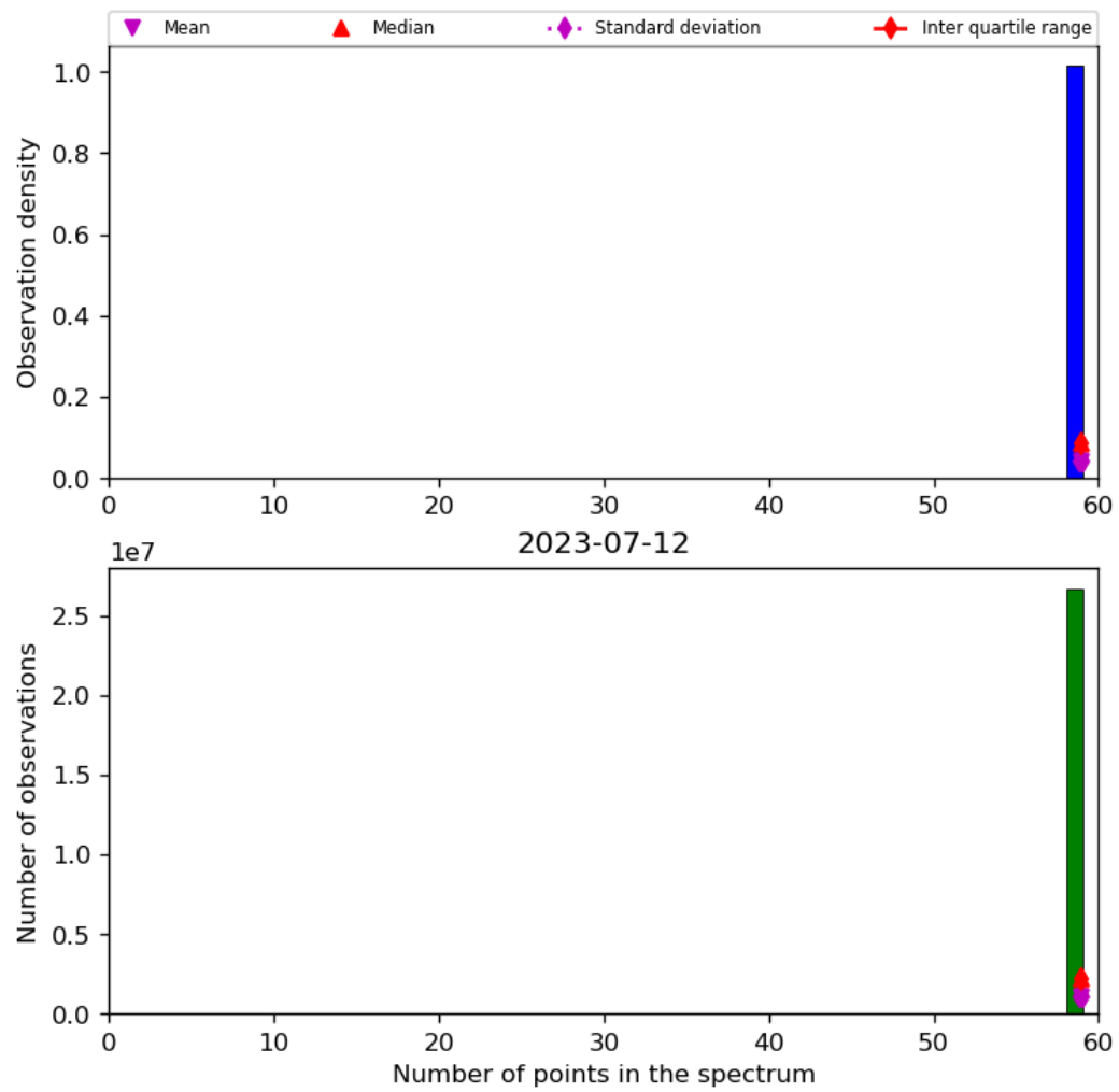
Figure 44: Histogram of “Number of points in the spectrum” for 2023-07-11 to 2023-07-13
