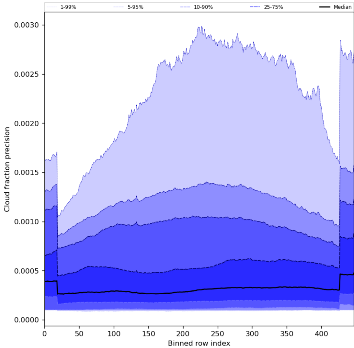
Figure 50: Along track statistics of “Cloud fraction precision” for 2023-07-11 to 2023-07-13
