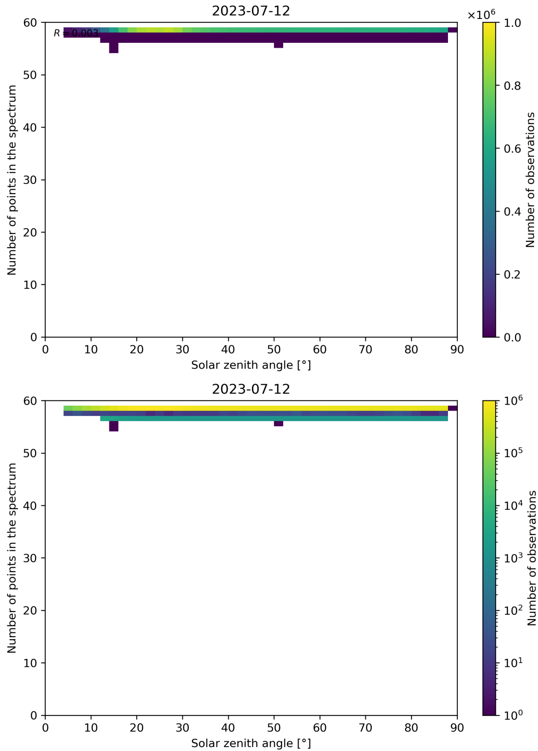
Figure 126: Scatter density plot of “Solar zenith angle” against “Number of points in the spectrum” for 2023-07-11 to 2023-07-13.
