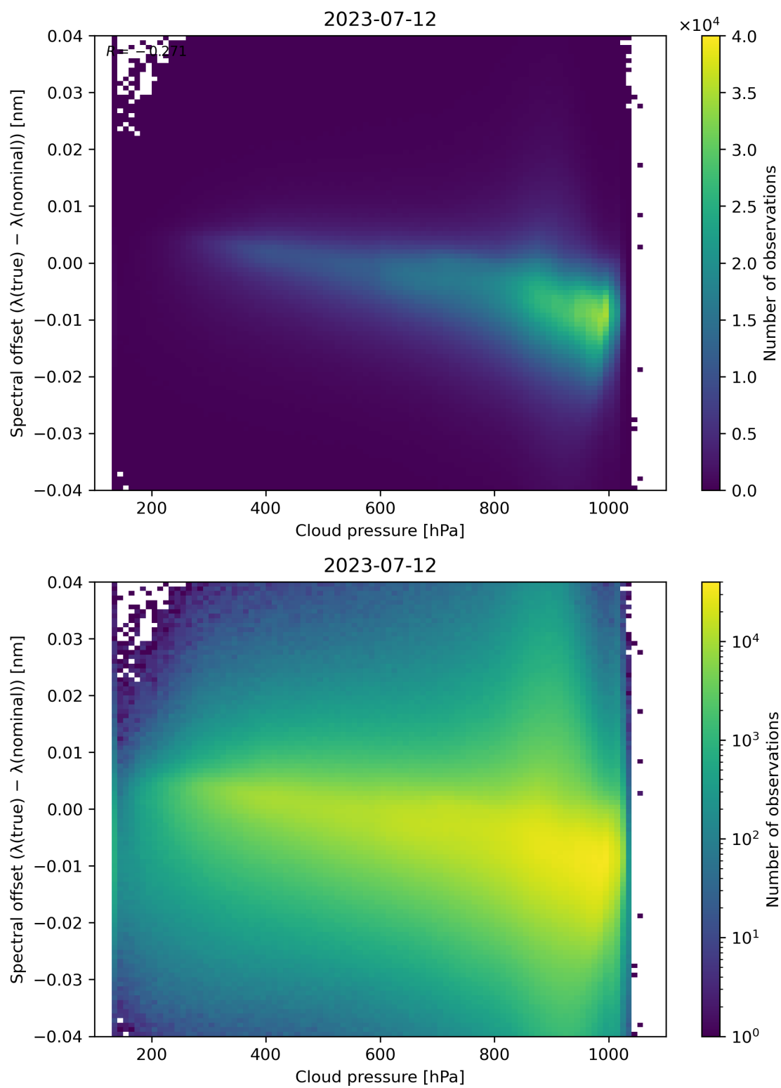
Figure 92: Scatter density plot of “Cloud pressure” against “Spectral offset ( \lambda(\text{true}) - \lambda(\text{nominal}) )” for 2023-07-11 to 2023-07-13.
