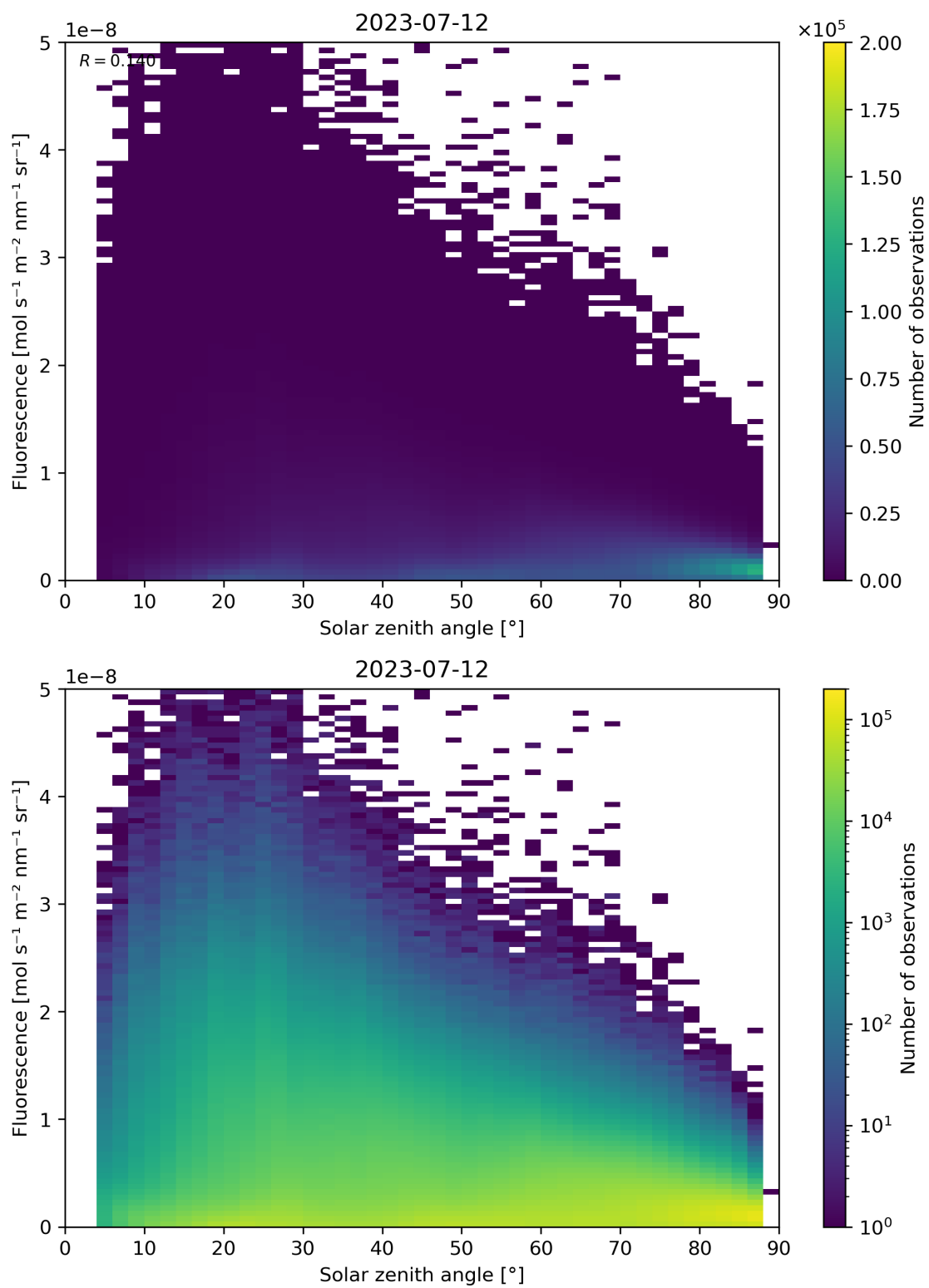
Figure 123: Scatter density plot of “Solar zenith angle” against “Fluorescence” for 2023-07-11 to 2023-07-13.
