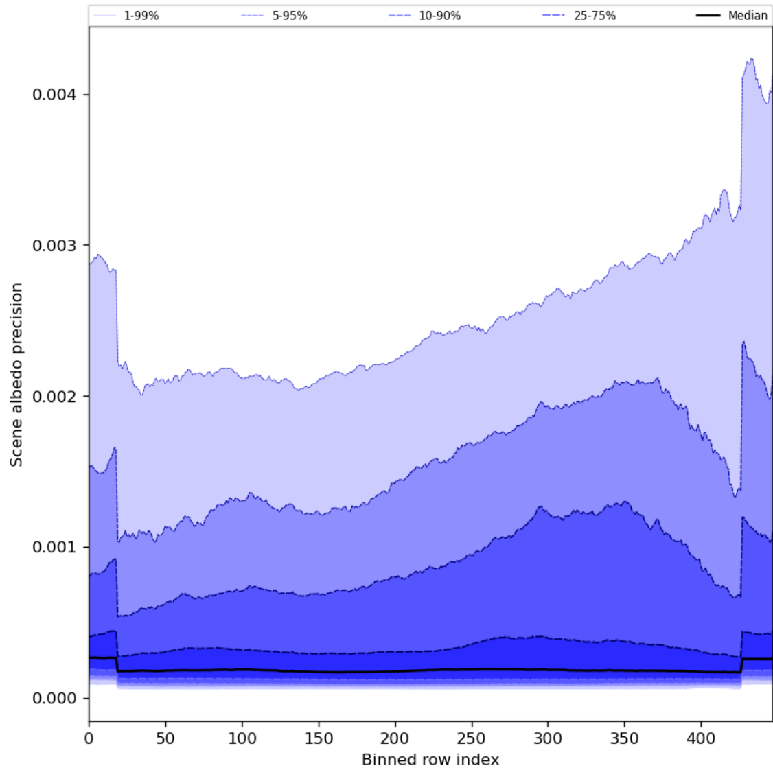
Figure 52: Along track statistics of “Scene albedo precision” for 2023-07-11 to 2023-07-13
