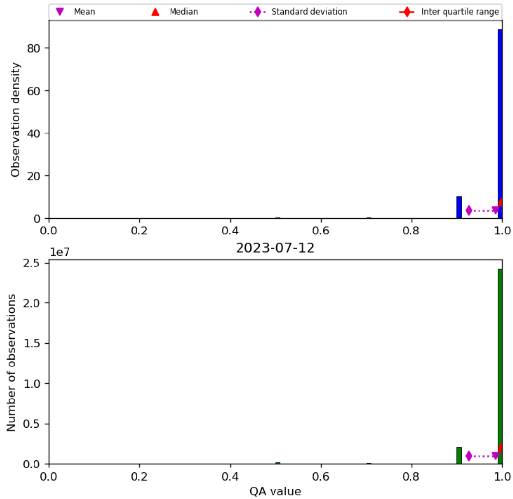
Figure 29: Histogram of “QA value” for 2023-07-11 to 2023-07-13
