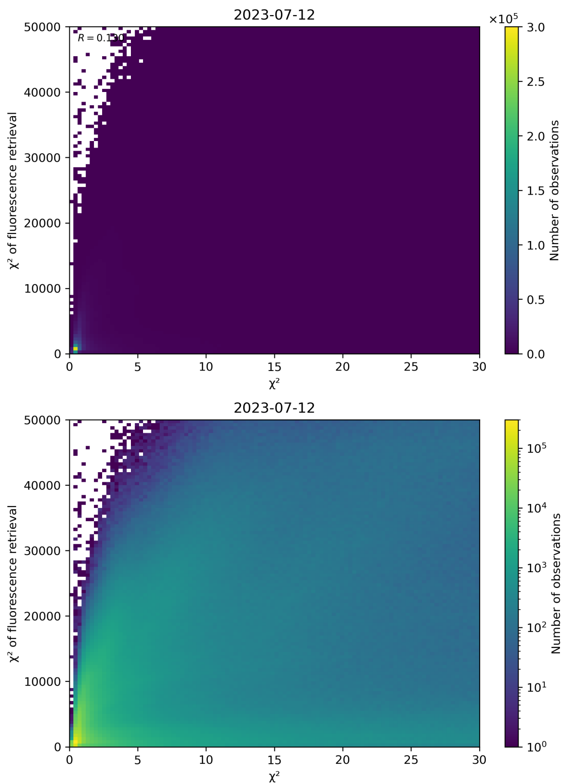
Figure 69: Scatter density plot of “ \chi^2 ” against “ \chi^2 of fluorescence retrieval” for 2023-07-11 to 2023-07-13.
