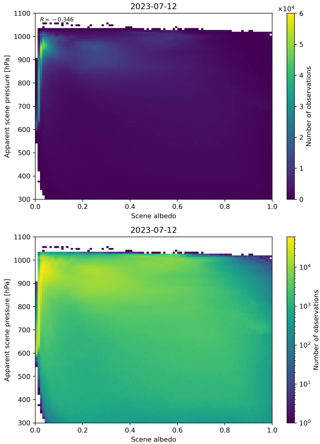
Figure 111: Scatter density plot of “Scene albedo” against “Apparent scene pressure” for 2023-07-11 to 2023-07-13.
