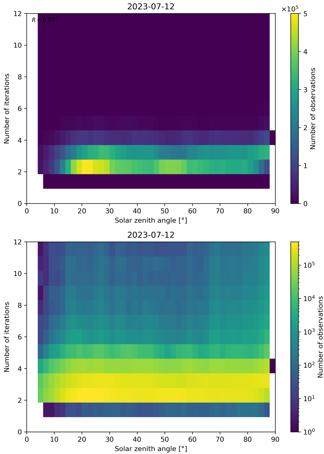
Figure 125: Scatter density plot of “Solar zenith angle” against “Number of iterations” for 2023-07-11 to 2023-07-13.
