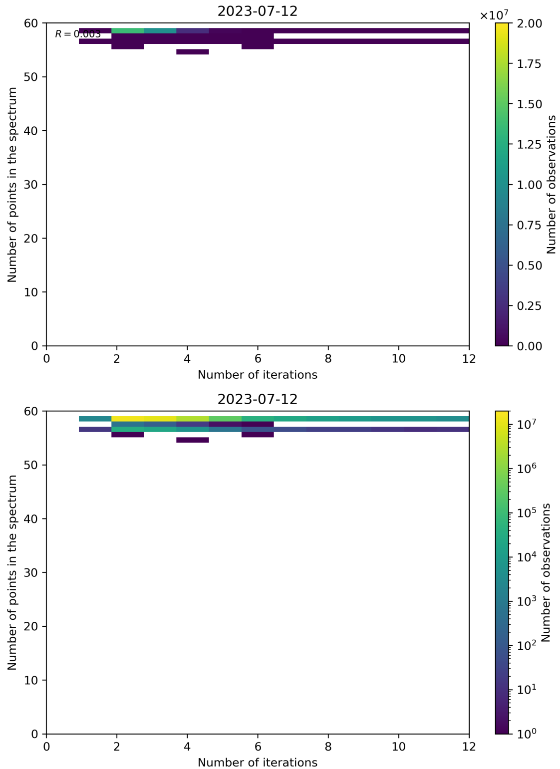
Figure 108: Scatter density plot of “Number of iterations” against “Number of points in the spectrum” for 2023-07-11 to 2023-07-13.
