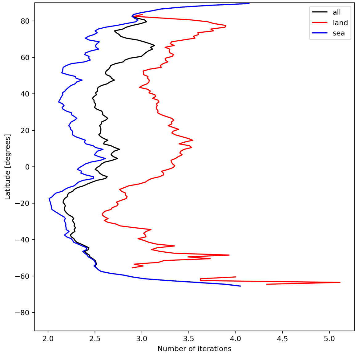
Figure 22: Zonal average of “Number of iterations” for 2023-07-11 to 2023-07-13.
