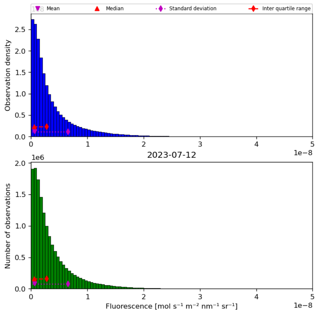
Figure 40: Histogram of “Fluorescence” for 2023-07-11 to 2023-07-13
