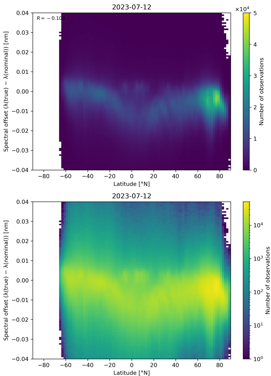
Figure 105: Scatter density plot of “Latitude” against “Spectral offset ( \lambda(\text{true}) - \lambda(\text{nominal}) )” for 2023-07-11 to 2023-07-13.
