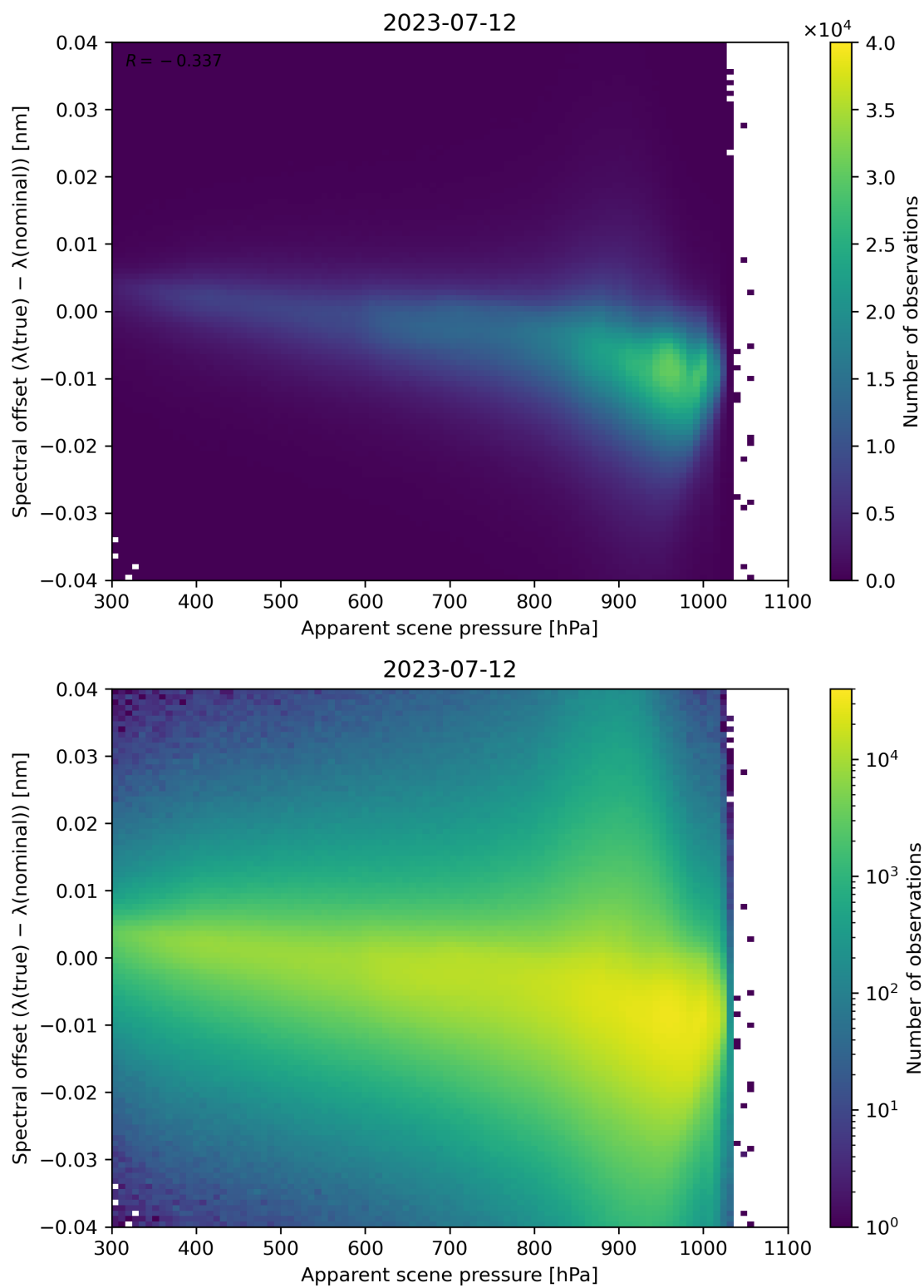
Figure 68: Scatter density plot of “Apparent scene pressure” against “Spectral offset ( \lambda(\text{true}) - \lambda(\text{nominal}) )” for 2023-07-11 to 2023-07-13.
