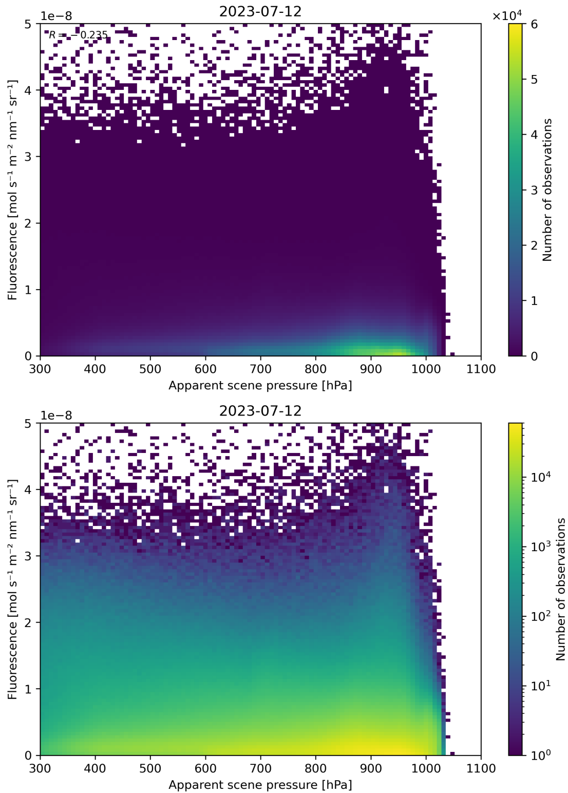
Figure 65: Scatter density plot of “Apparent scene pressure” against “Fluorescence” for 2023-07-11 to 2023-07-13.
