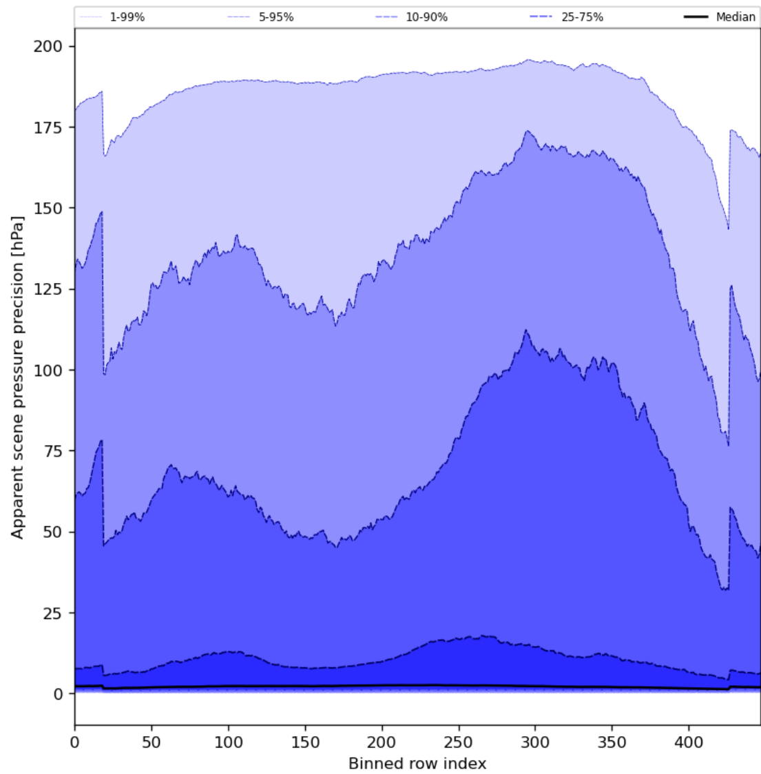
Figure 54: Along track statistics of “Apparent scene pressure precision” for 2023-07-11 to 2023-07-13
