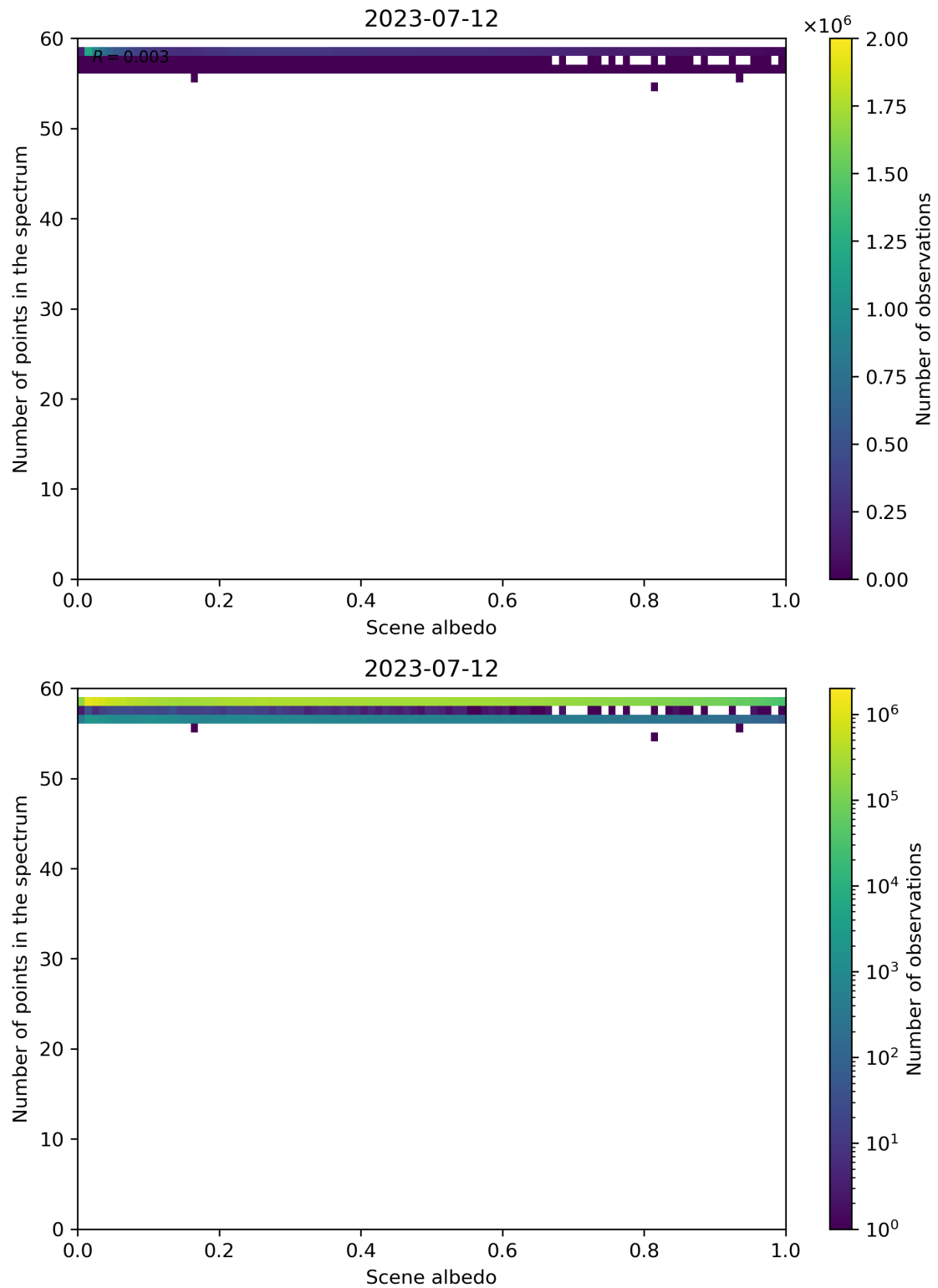
Figure 116: Scatter density plot of “Scene albedo” against “Number of points in the spectrum” for 2023-07-11 to 2023-07-13.
