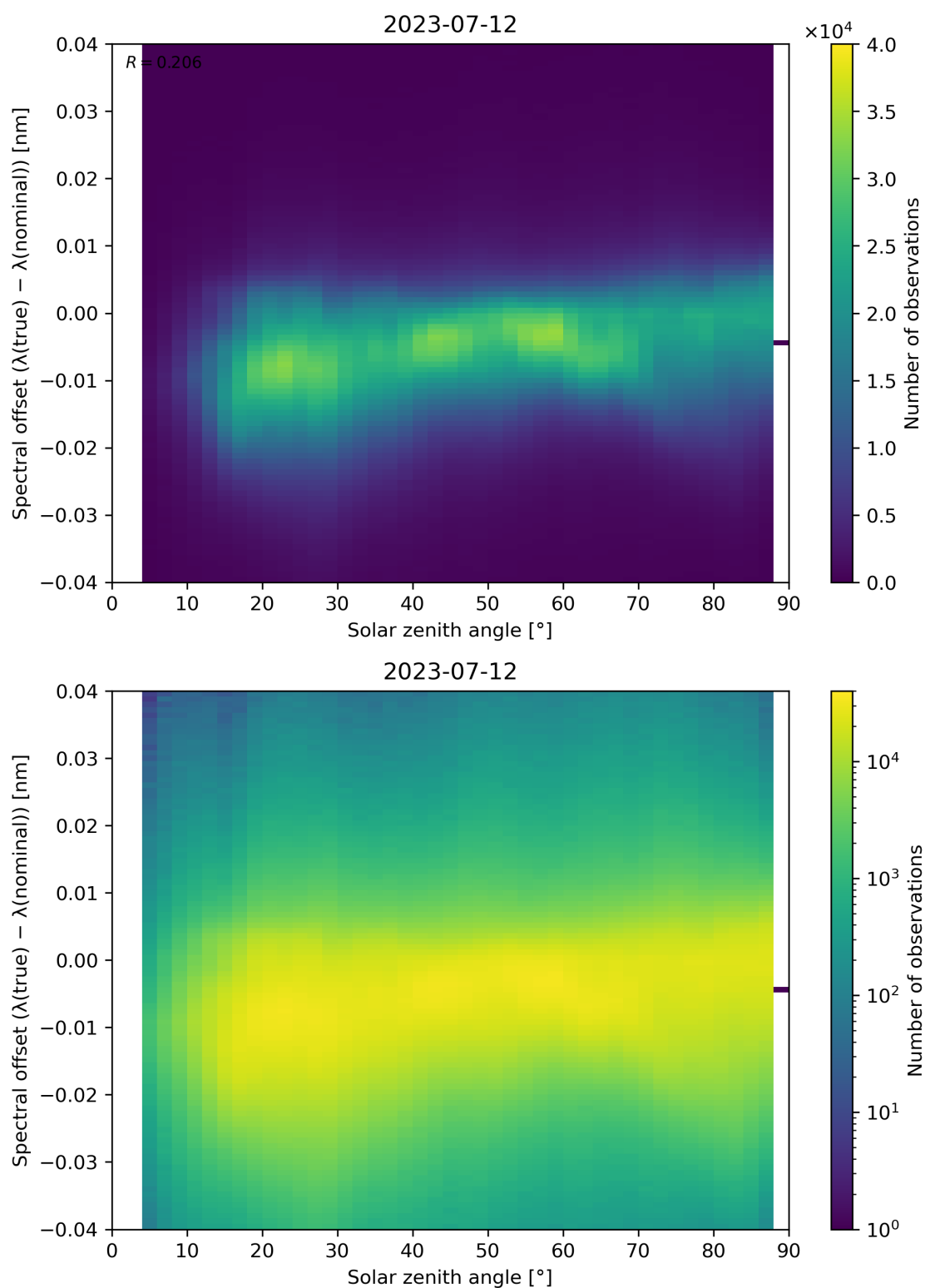
Figure 128: Scatter density plot of “Solar zenith angle” against “Spectral offset ( \lambda(\text{true}) - \lambda(\text{nominal}) )” for 2023-07-11 to 2023-07-13.
