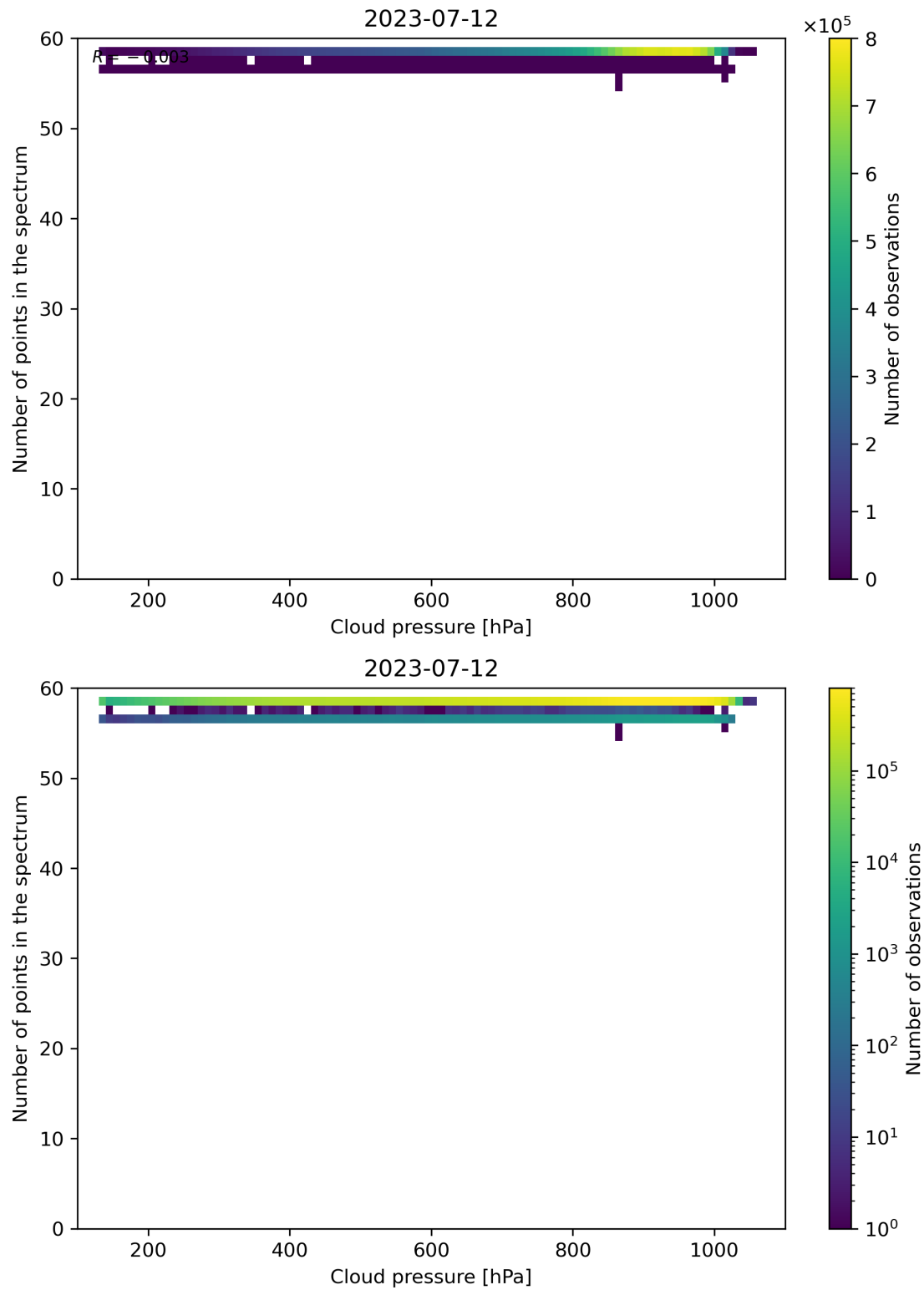
Figure 90: Scatter density plot of “Cloud pressure” against “Number of points in the spectrum” for 2023-07-11 to 2023-07-13.
