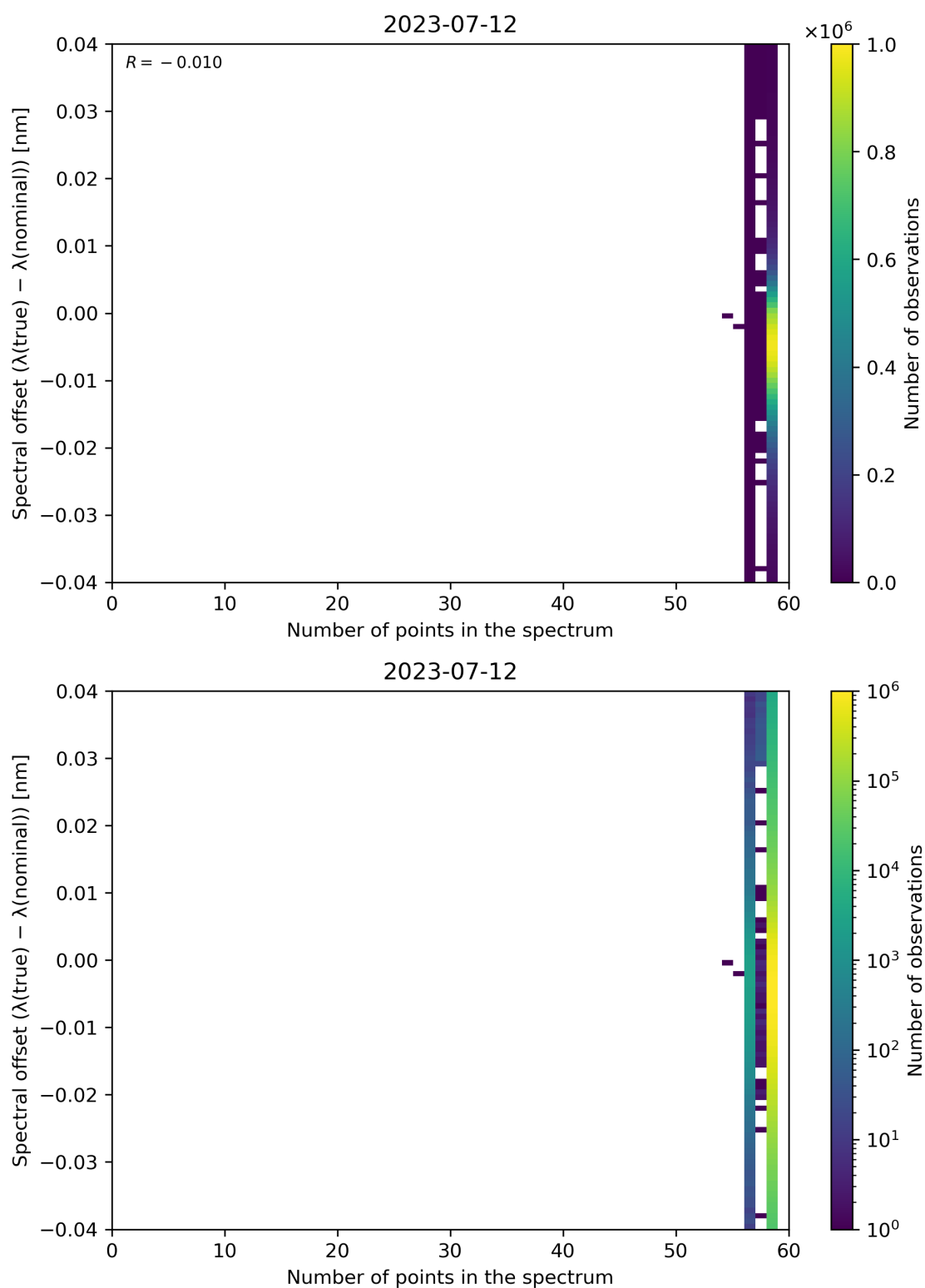
Figure 110: Scatter density plot of “Number of points in the spectrum” against “Spectral offset ( \lambda(\text{true}) - \lambda(\text{nominal}) )” for 2023-07-11 to 2023-07-13.
