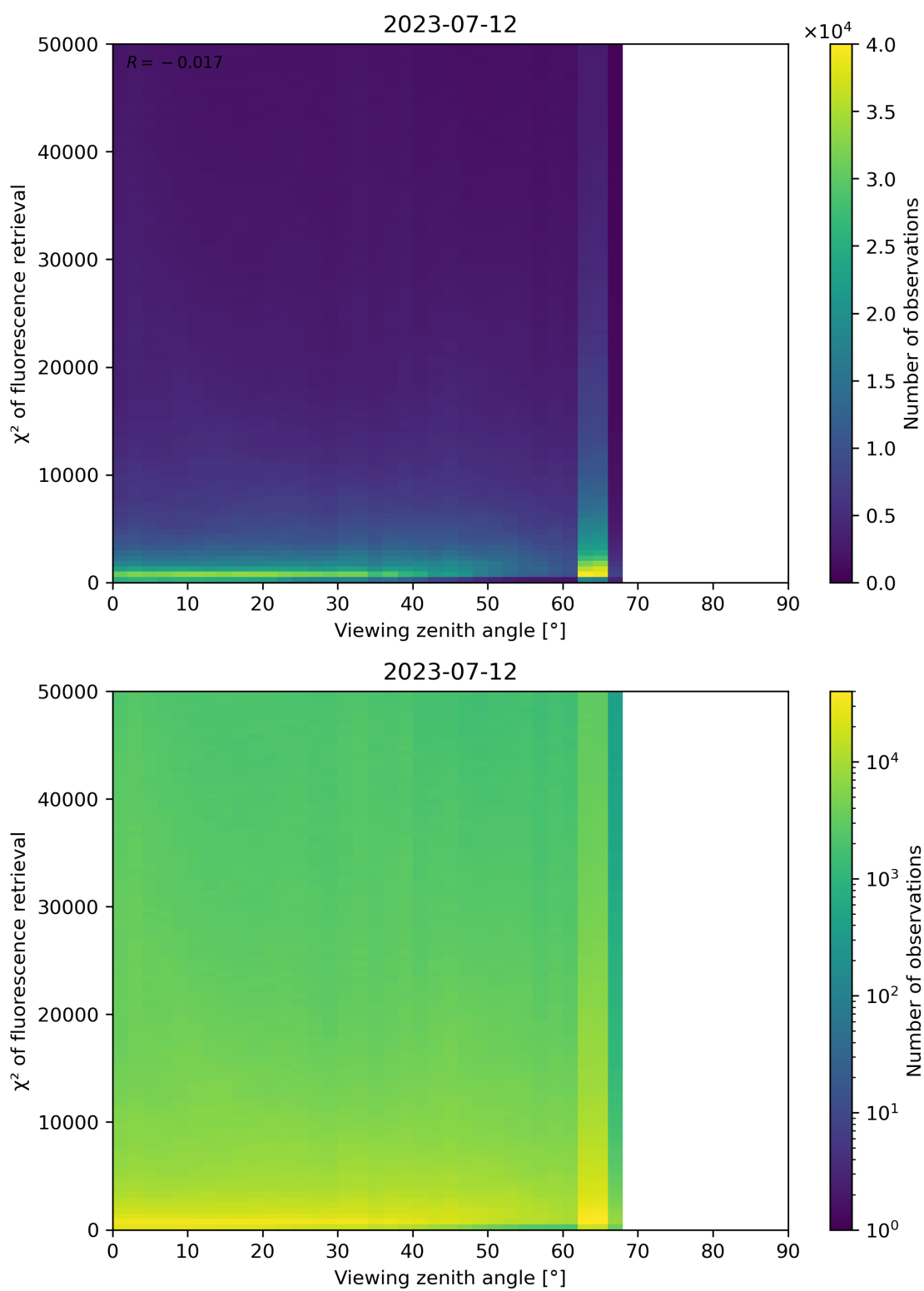
Figure 131: Scatter density plot of “Viewing zenith angle” against “ \chi^2 of fluorescence retrieval” for 2023-07-11 to 2023-07-13.
