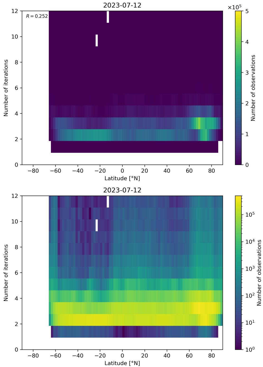
Figure 102: Scatter density plot of “Latitude” against “Number of iterations” for 2023-07-11 to 2023-07-13.
