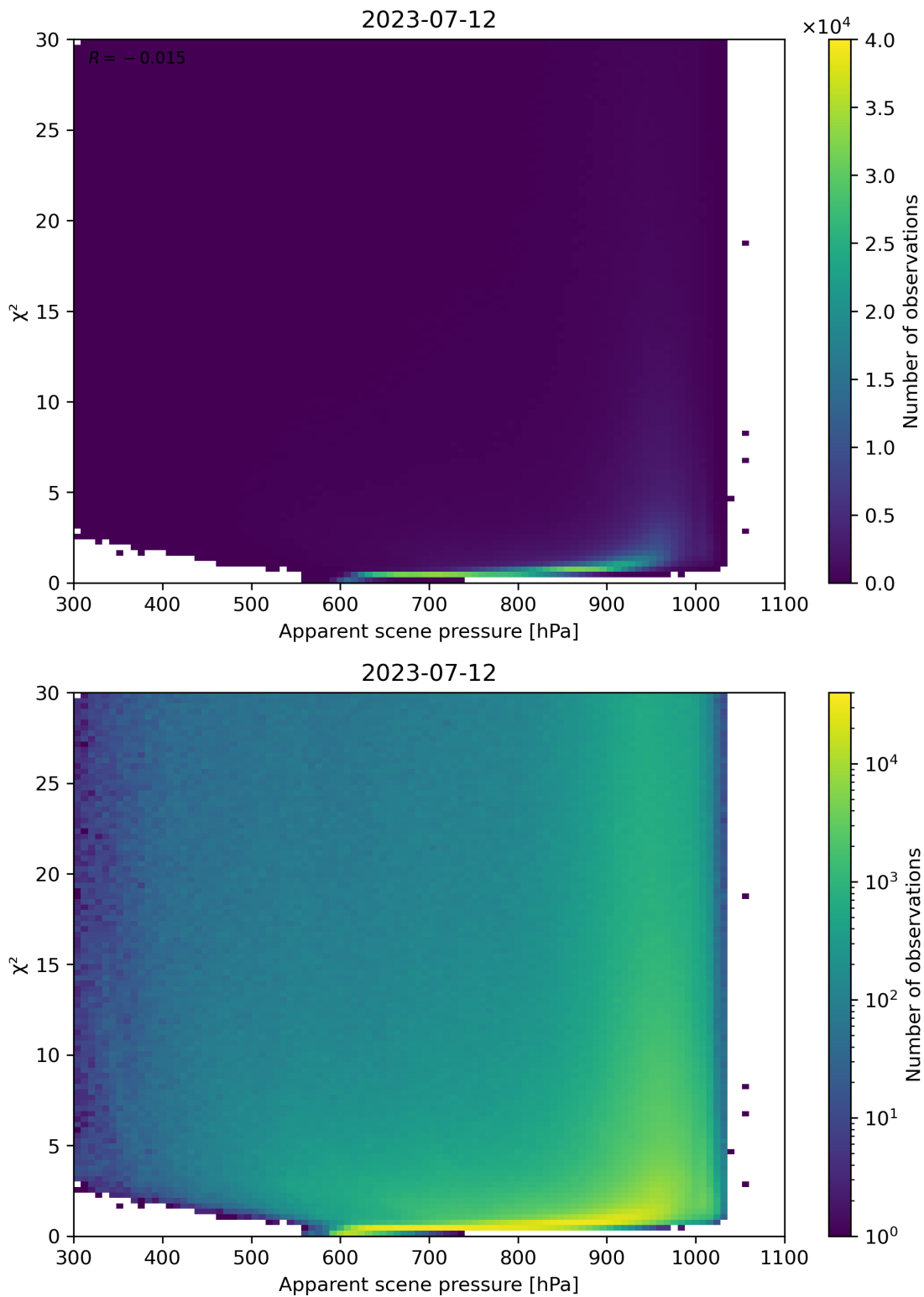
Figure 63: Scatter density plot of “Apparent scene pressure” against “ \chi^2 ” for 2023-07-11 to 2023-07-13.
