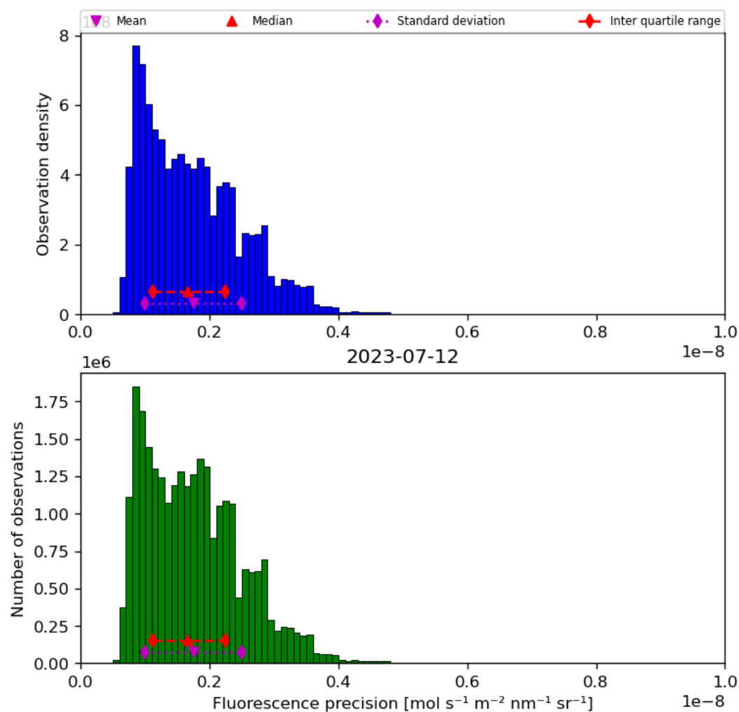
Figure 41: Histogram of “Fluorescence precision” for 2023-07-11 to 2023-07-13
