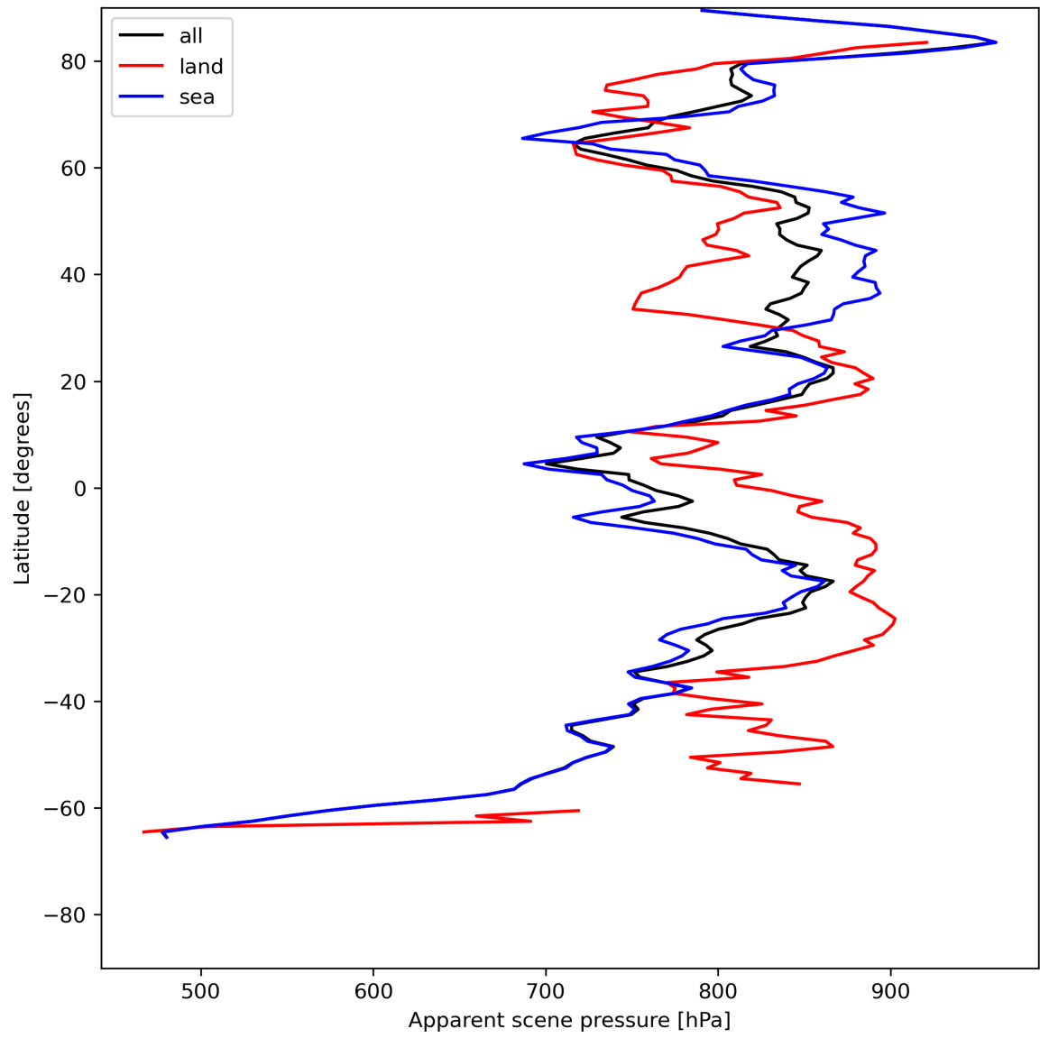
Figure 19: Zonal average of “Apparent scene pressure” for 2023-07-11 to 2023-07-13.
