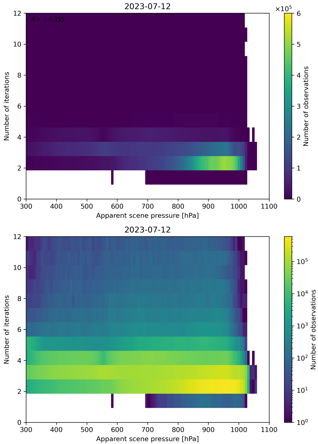
Figure 66: Scatter density plot of “Apparent scene pressure” against “Number of iterations” for 2023-07-11 to 2023-07-13.
