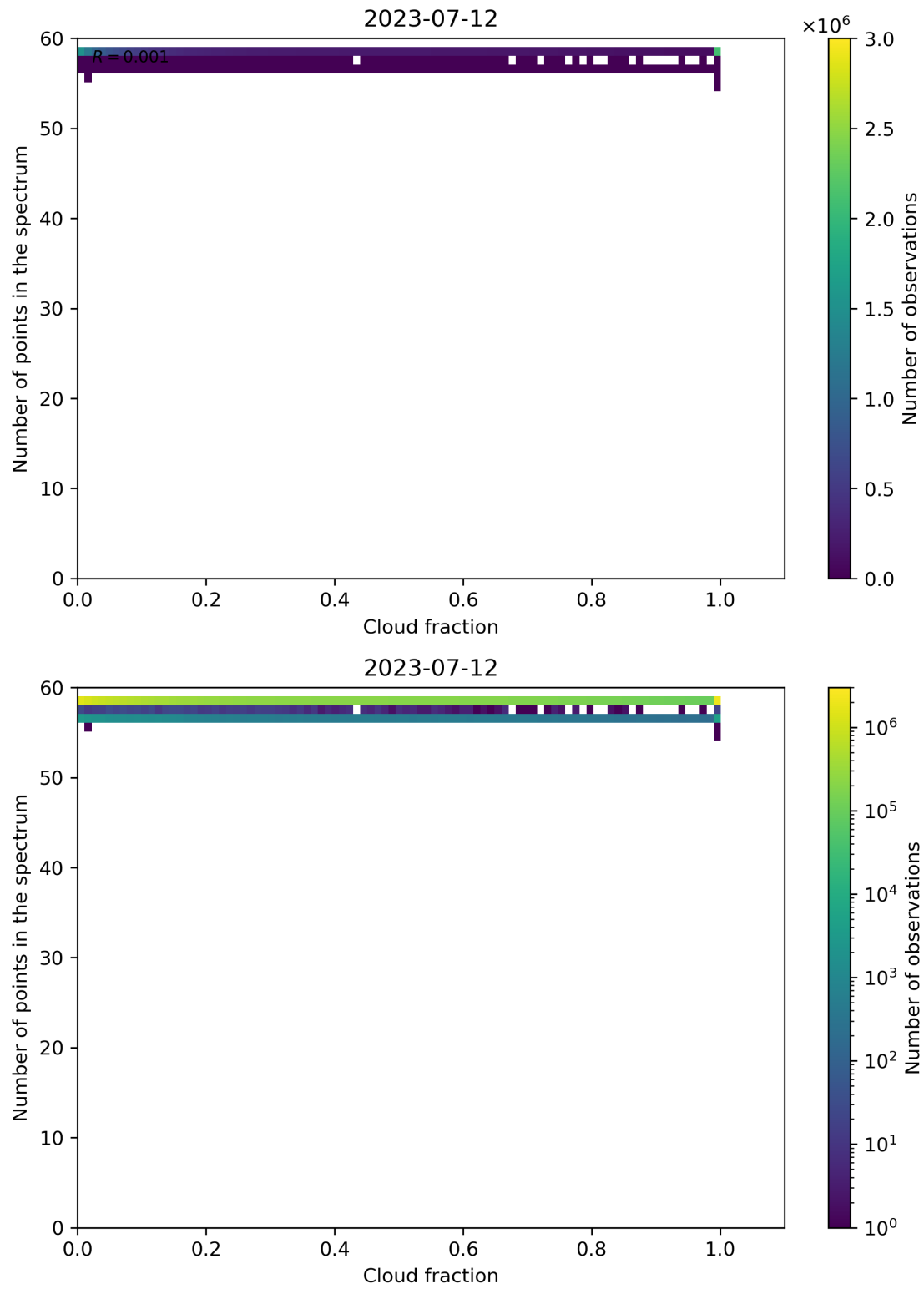
Figure 81: Scatter density plot of “Cloud fraction” against “Number of points in the spectrum” for 2023-07-11 to 2023-07-13.
