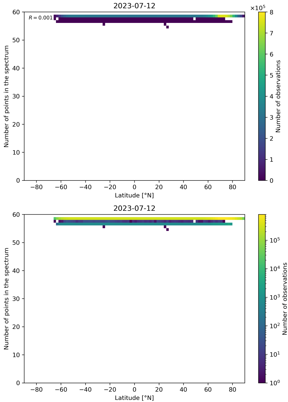
Figure 103: Scatter density plot of “Latitude” against “Number of points in the spectrum” for 2023-07-11 to 2023-07-13.
