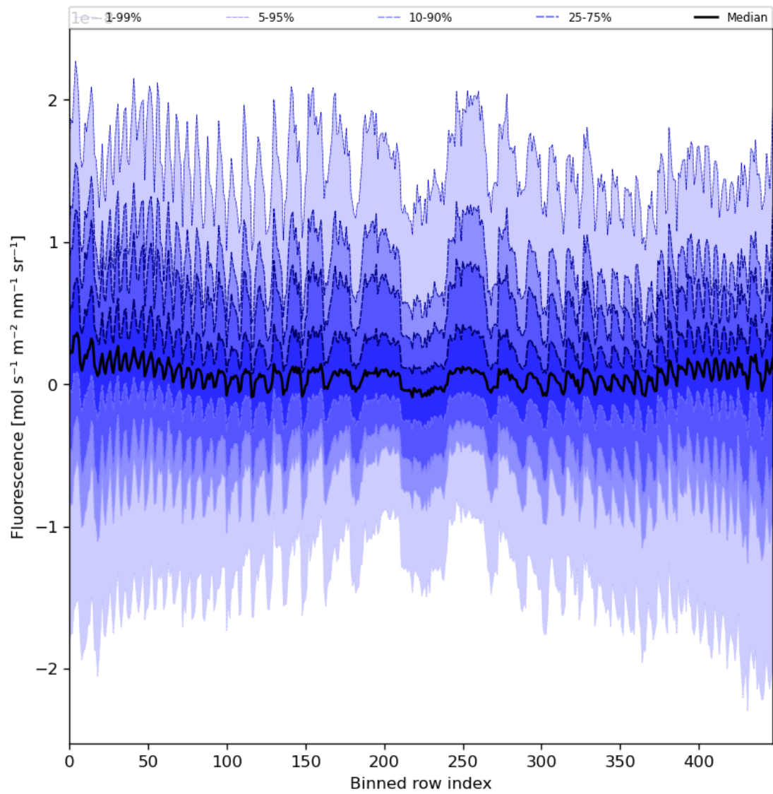
Figure 57: Along track statistics of “Fluorescence” for 2023-07-11 to 2023-07-13
