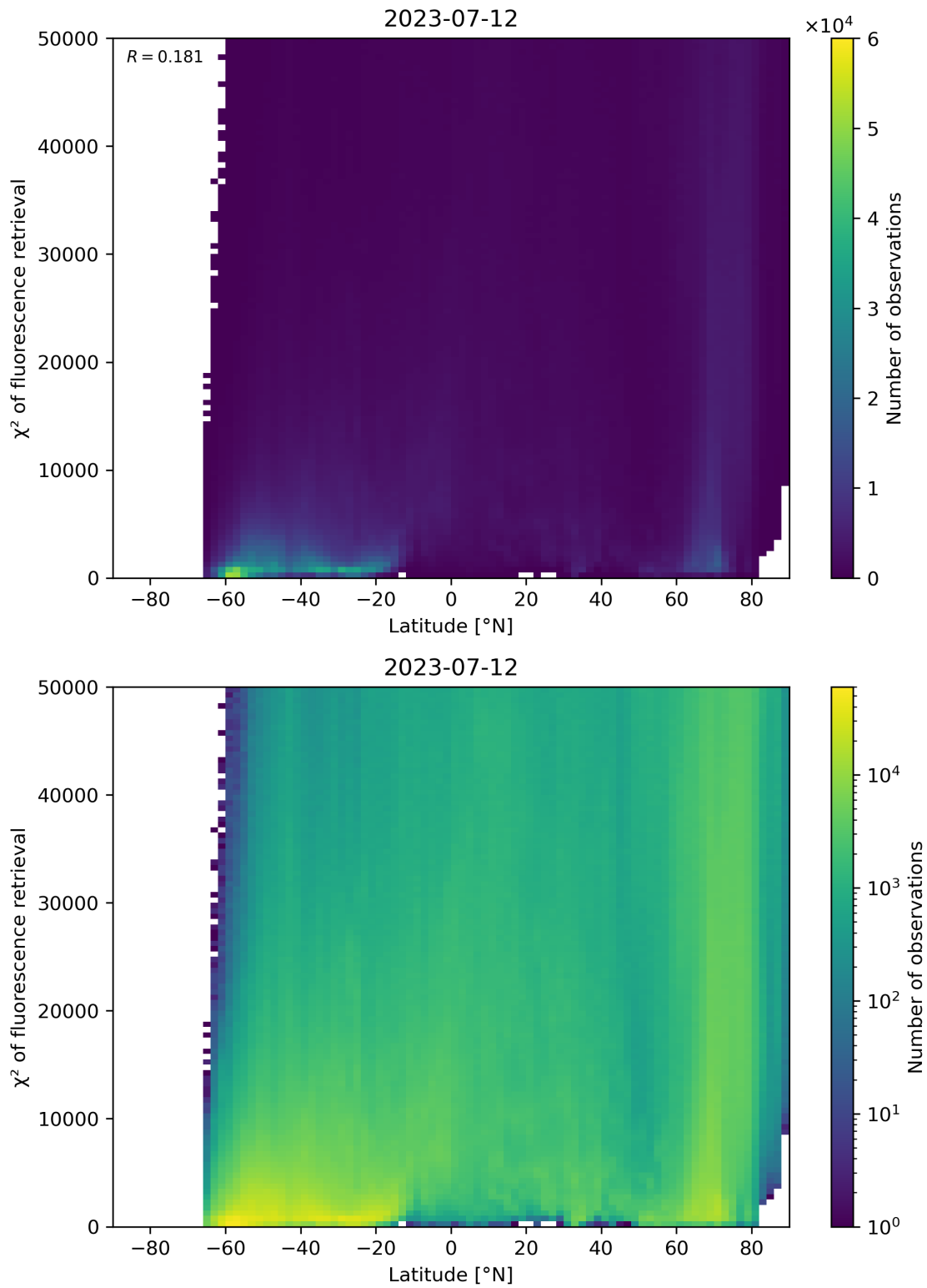
Figure 98: Scatter density plot of “Latitude” against “ \chi^2 of fluorescence retrieval” for 2023-07-11 to 2023-07-13.
