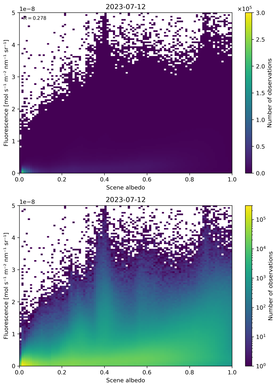
Figure 114: Scatter density plot of “Scene albedo” against “Fluorescence” for 2023-07-11 to 2023-07-13.
