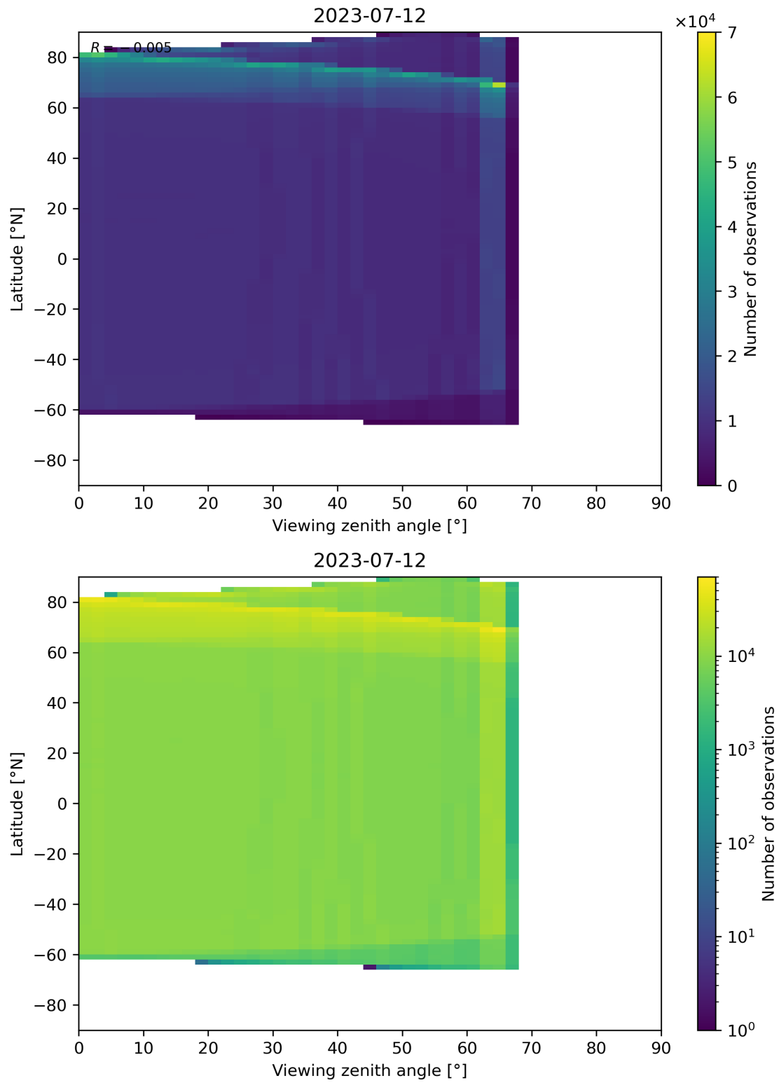
Figure 135: Scatter density plot of “Viewing zenith angle” against “Latitude” for 2023-07-11 to 2023-07-13.
