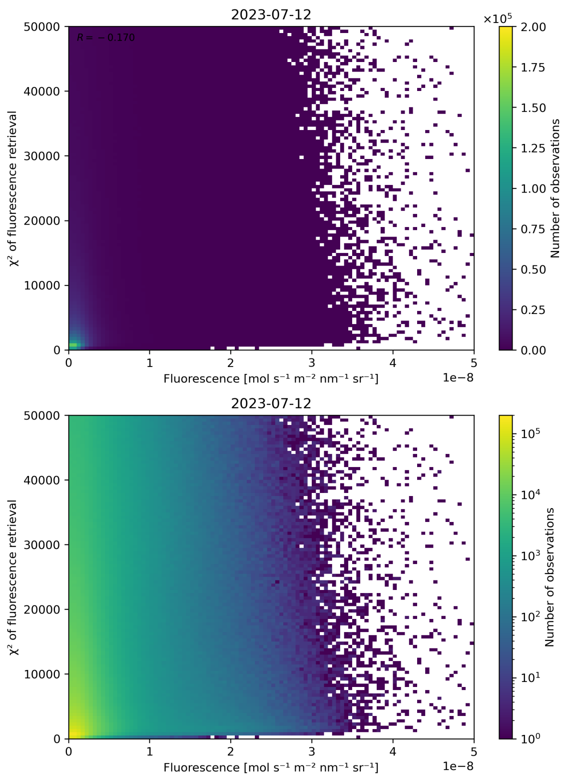
Figure 93: Scatter density plot of “Fluorescence” against “ \chi^2 of fluorescence retrieval” for 2023-07-11 to 2023-07-13.
