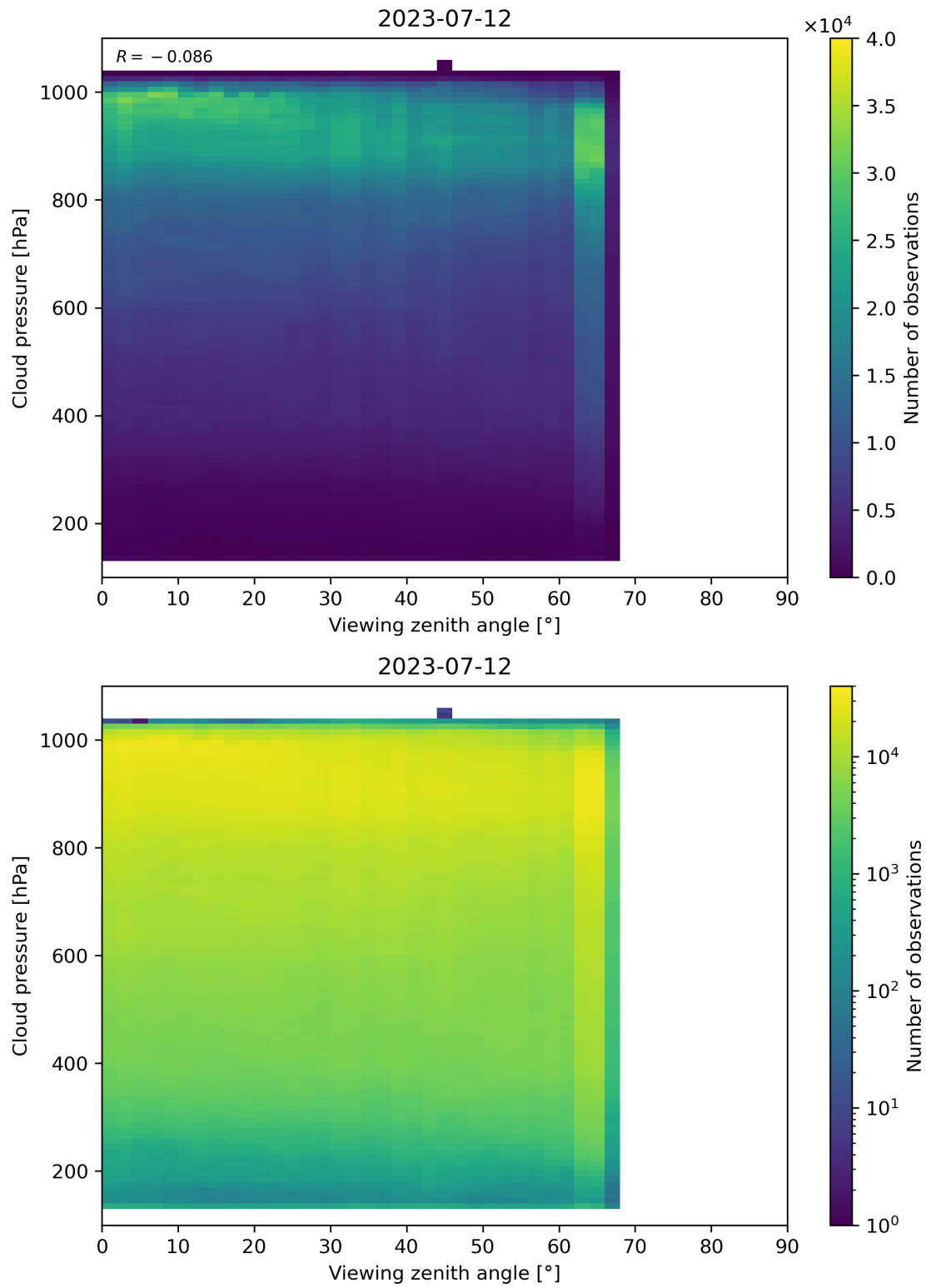
Figure 133: Scatter density plot of “Viewing zenith angle” against “Cloud pressure” for 2023-07-11 to 2023-07-13.
