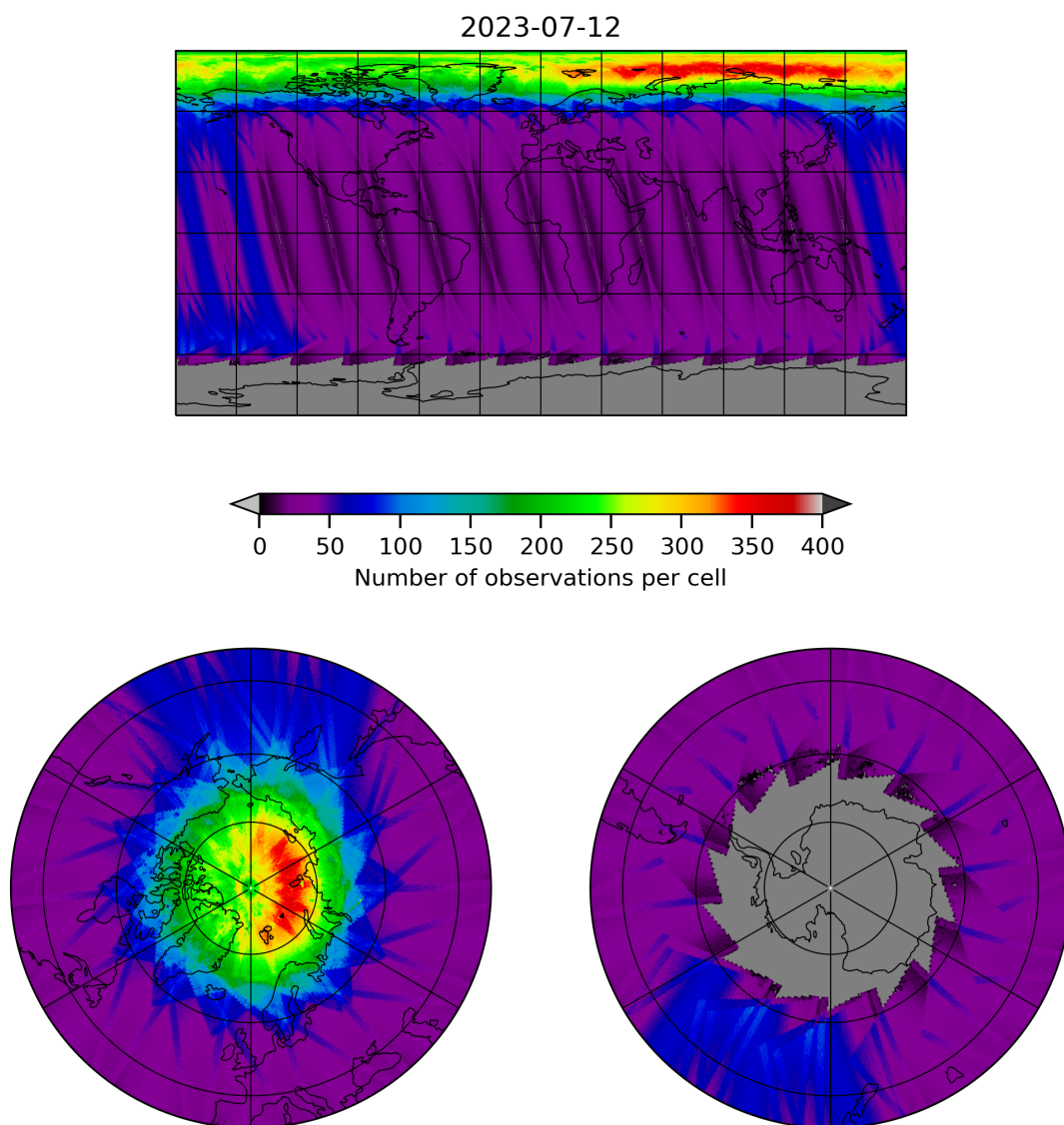
Figure 11: Map of the number of observations for 2023-07-11 to 2023-07-13
