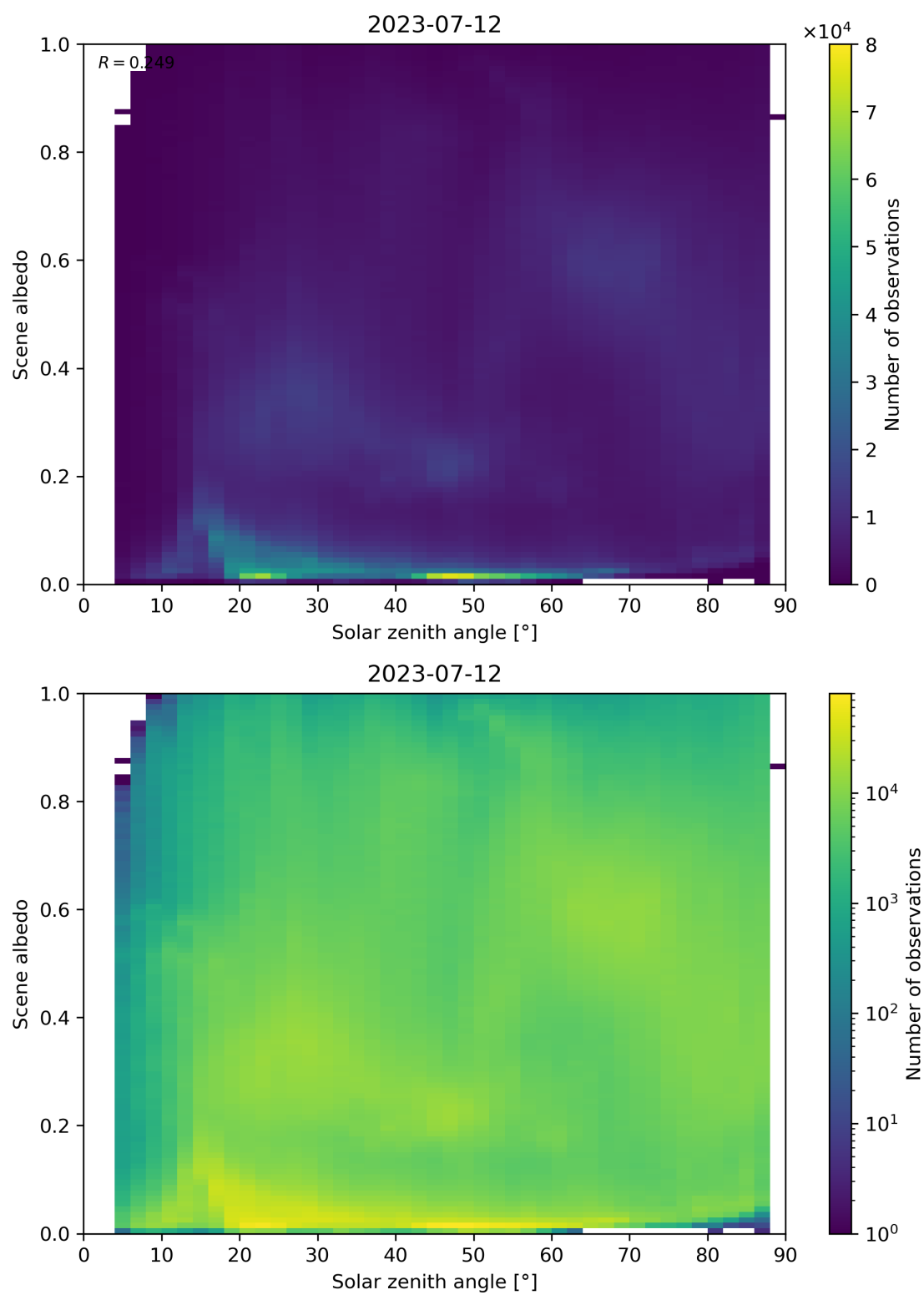
Figure 127: Scatter density plot of “Solar zenith angle” against “Scene albedo” for 2023-07-11 to 2023-07-13.
