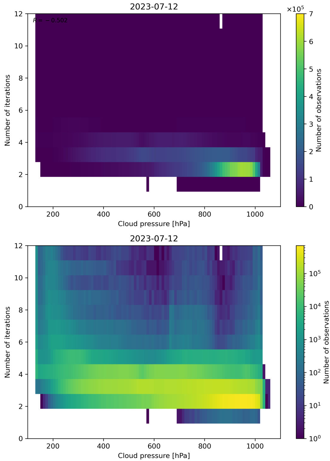
Figure 89: Scatter density plot of “Cloud pressure” against “Number of iterations” for 2023-07-11 to 2023-07-13.
