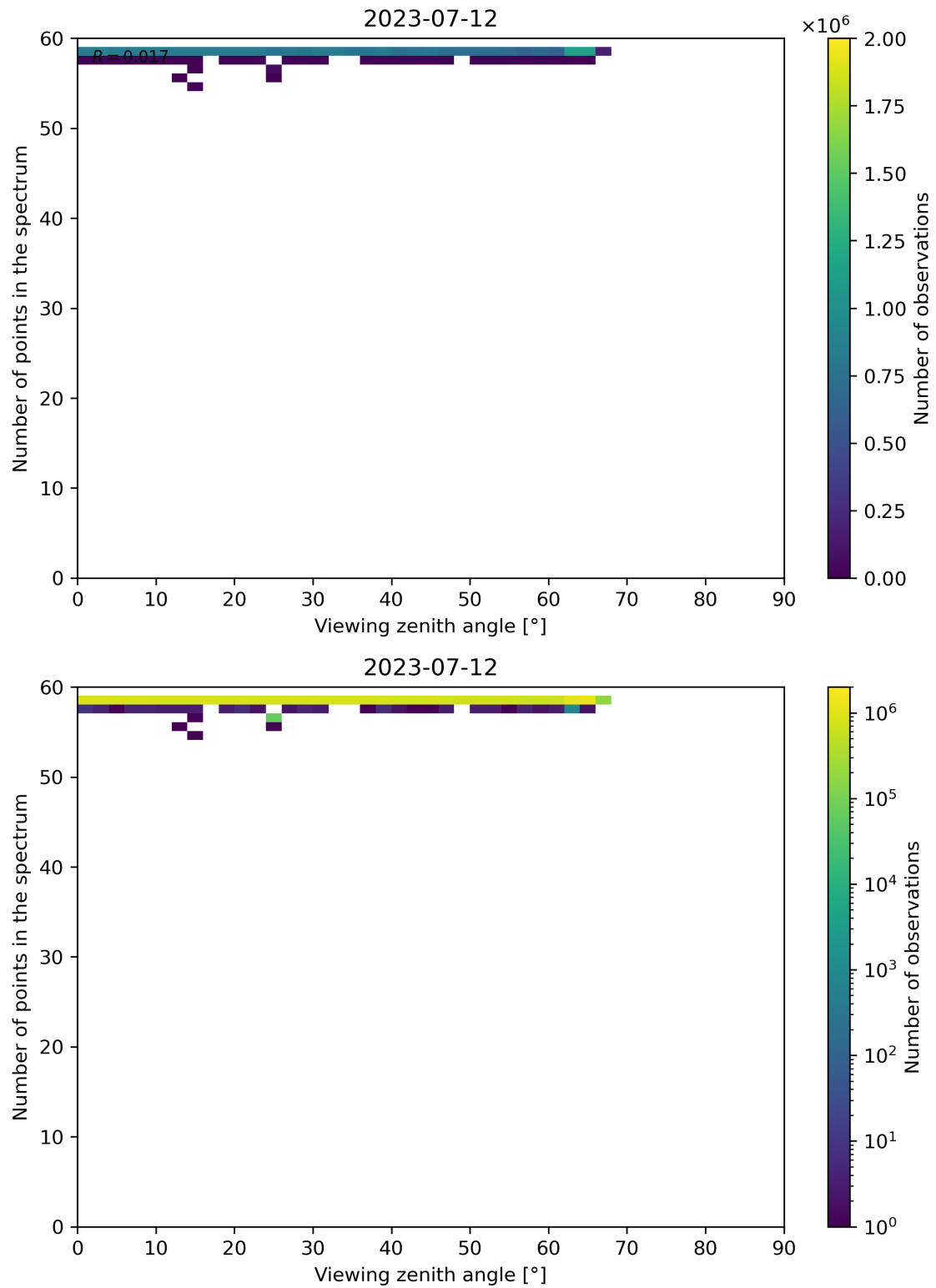
Figure 137: Scatter density plot of “Viewing zenith angle” against “Number of points in the spectrum” for 2023-07-11 to 2023-07-13.
