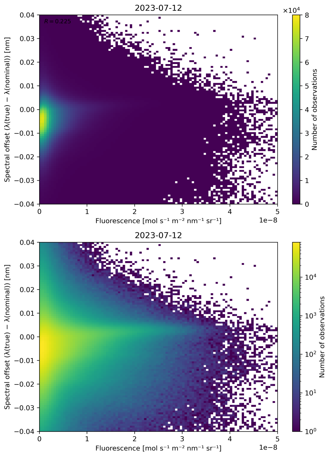
Figure 95: Scatter density plot of “Fluorescence” against “Spectral offset ( \lambda(\text{true}) - \lambda(\text{nominal}) )” for 2023-07-11 to 2023-07-13.
