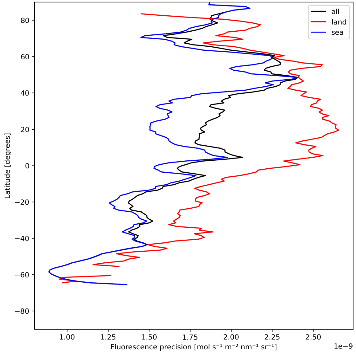
Figure 24: Zonal average of “Fluorescence precision” for 2023-07-11 to 2023-07-13.
