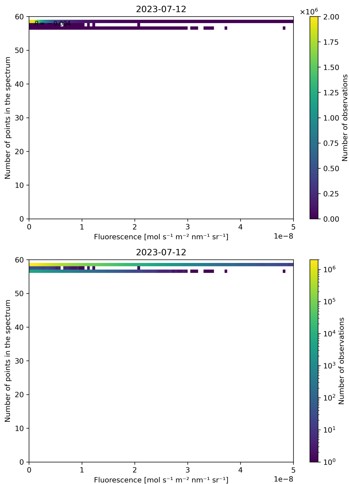
Figure 94: Scatter density plot of “Fluorescence” against “Number of points in the spectrum” for 2023-07-11 to 2023-07-13.
