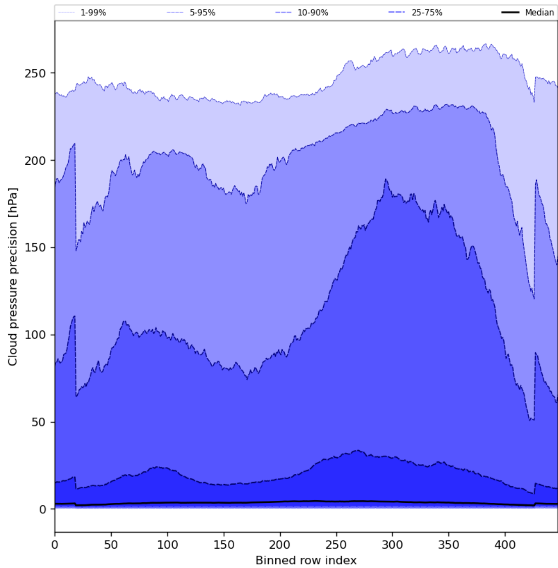
Figure 48: Along track statistics of “Cloud pressure precision” for 2023-07-11 to 2023-07-13
