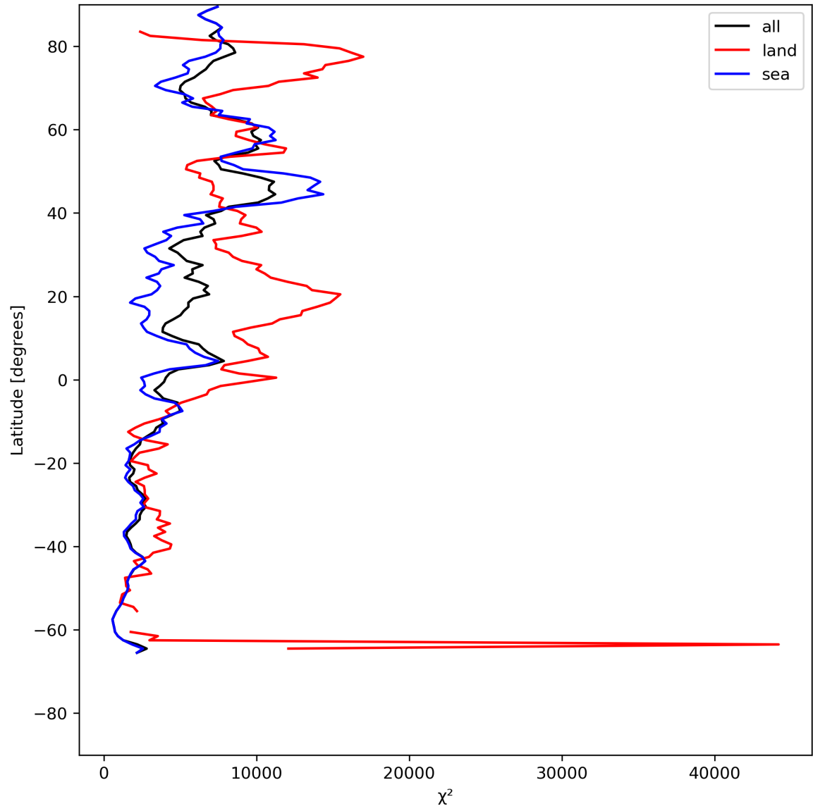
Figure 21: Zonal average of “ \chi^2 ” for 2023-07-11 to 2023-07-13.
