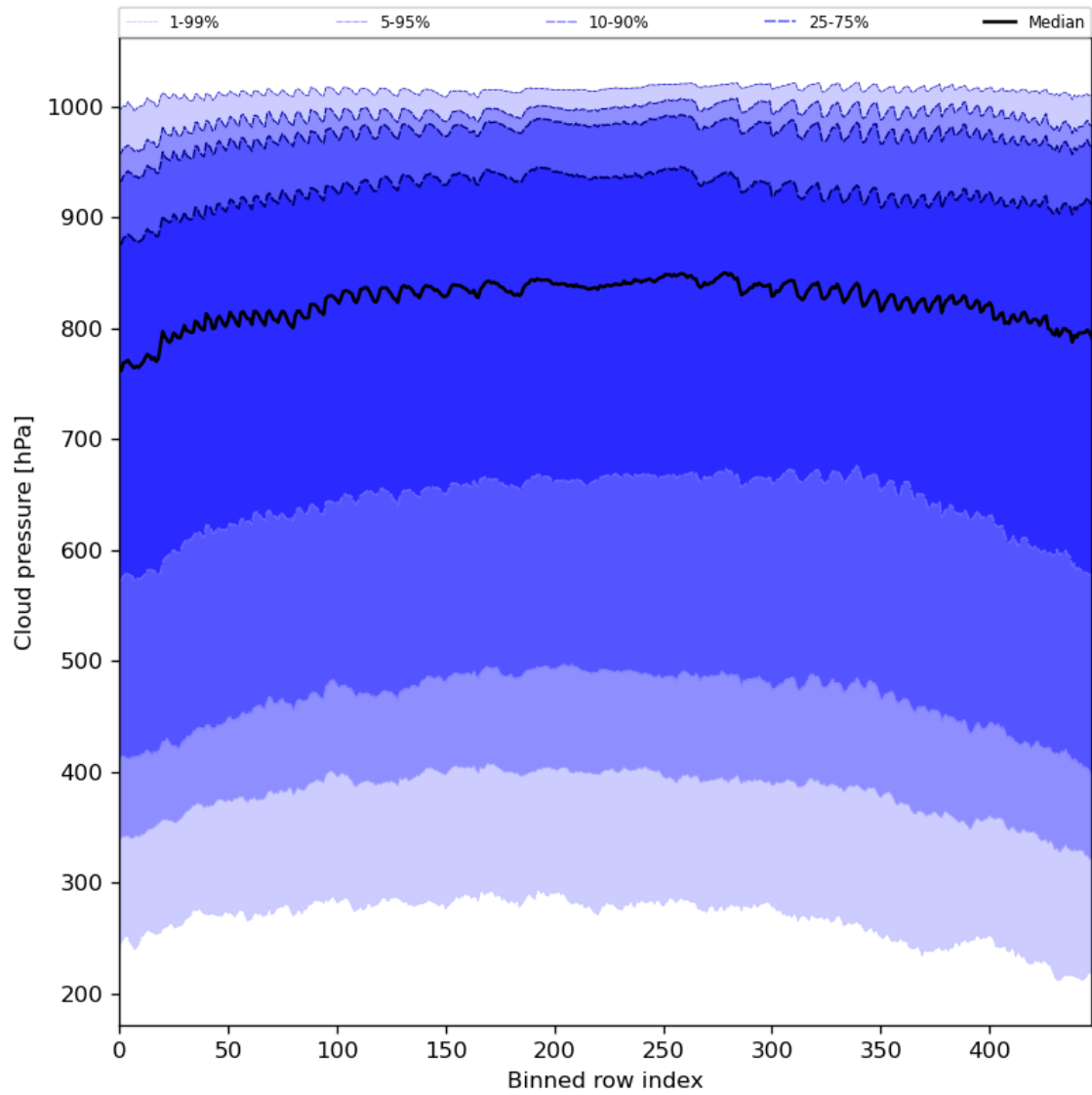
Figure 47: Along track statistics of “Cloud pressure” for 2023-07-11 to 2023-07-13
