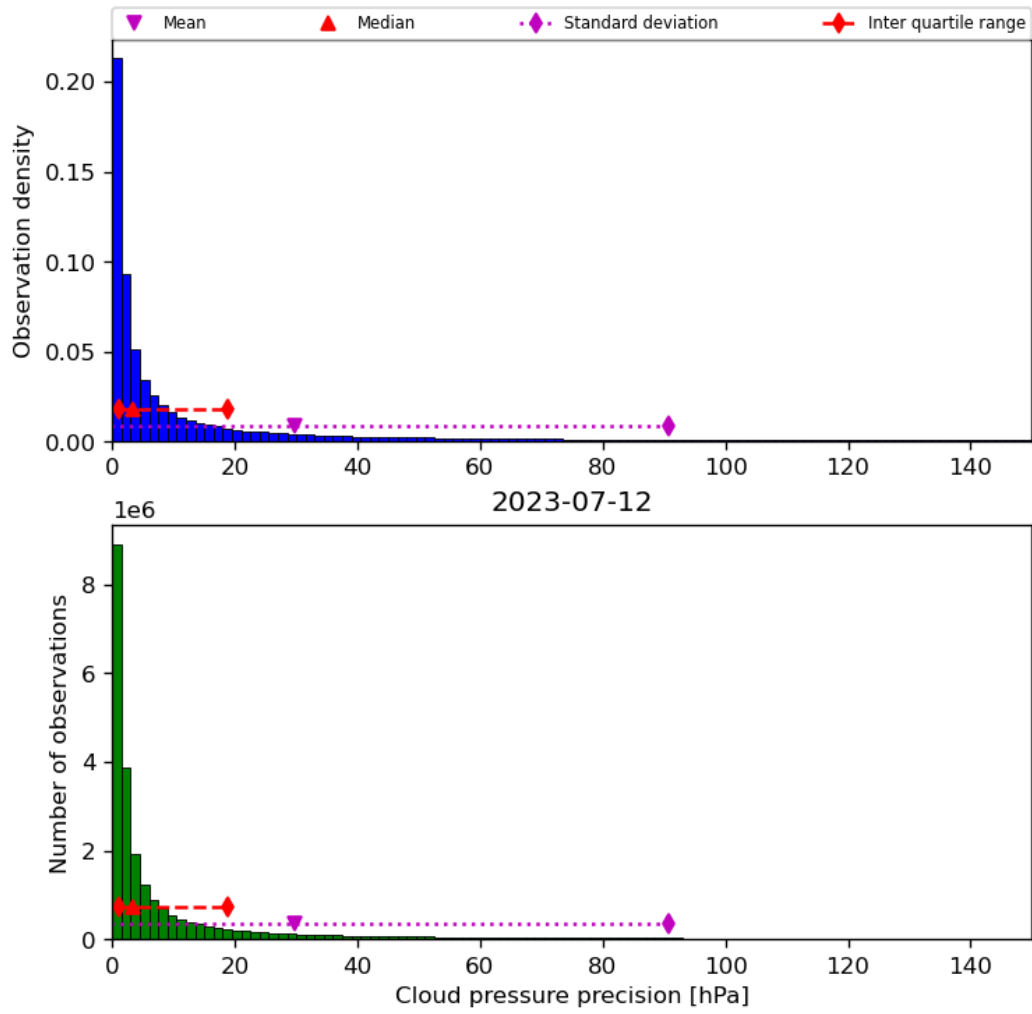
Figure 31: Histogram of “Cloud pressure precision” for 2023-07-11 to 2023-07-13
