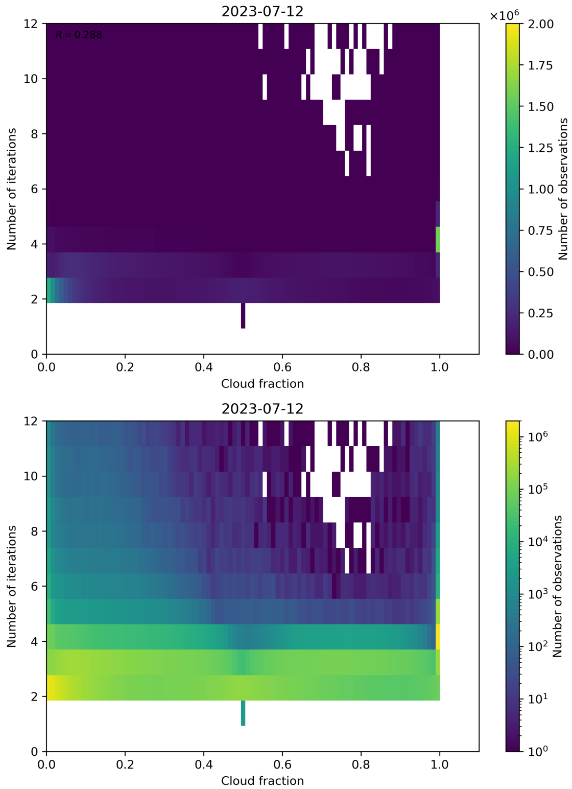
Figure 80: Scatter density plot of “Cloud fraction” against “Number of iterations” for 2023-07-11 to 2023-07-13.
