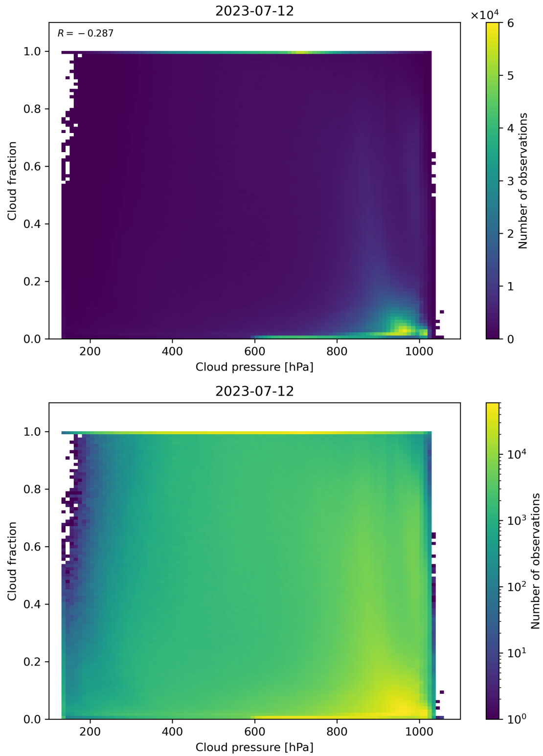
Figure 87: Scatter density plot of “Cloud pressure” against “Cloud fraction” for 2023-07-11 to 2023-07-13.
