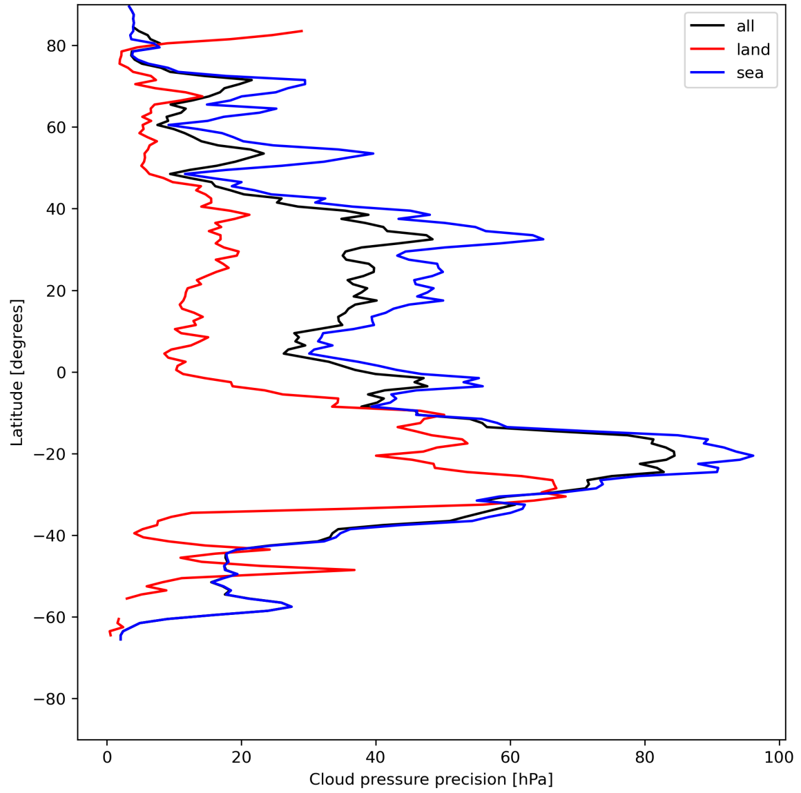
Figure 14: Zonal average of “Cloud pressure precision” for 2023-07-11 to 2023-07-13.
