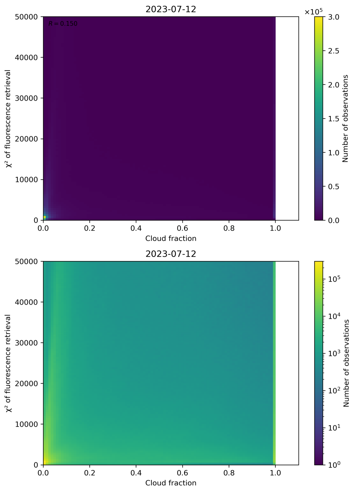
Figure 78: Scatter density plot of “Cloud fraction” against “ \chi^2 of fluorescence retrieval” for 2023-07-11 to 2023-07-13.
