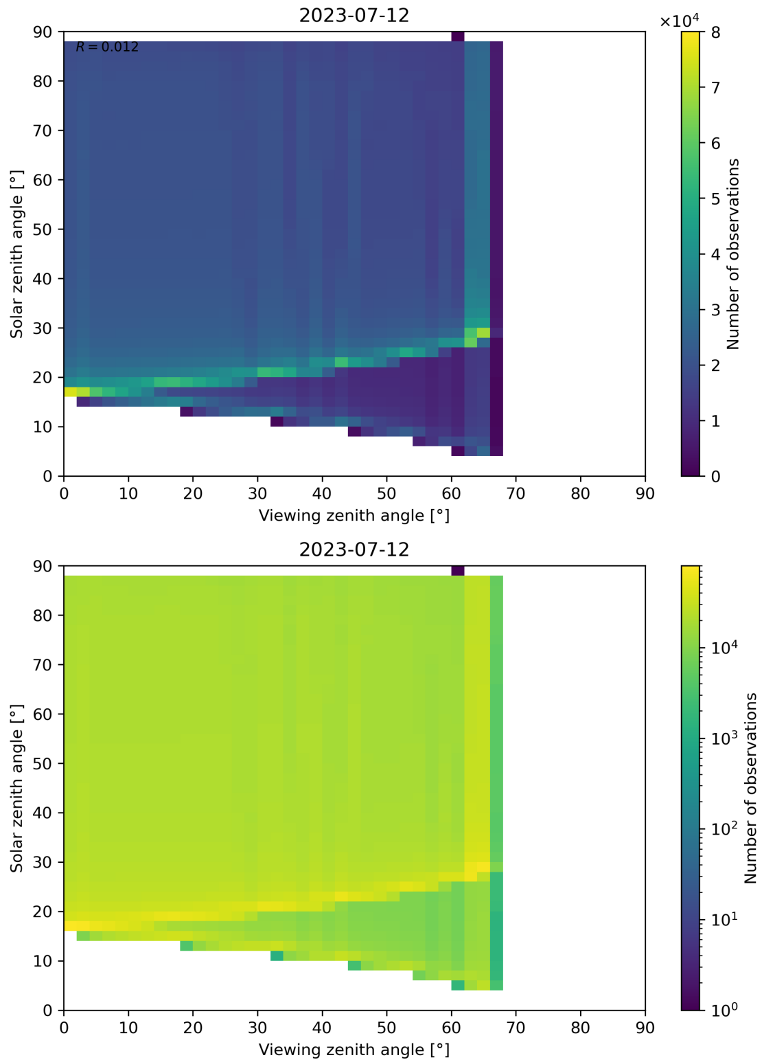
Figure 139: Scatter density plot of “Viewing zenith angle” against “Solar zenith angle” for 2023-07-11 to 2023-07-13.
