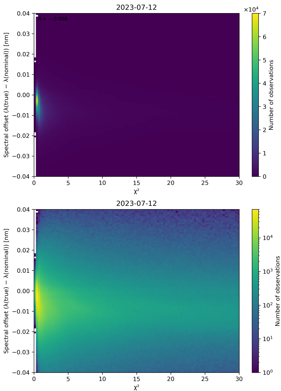
Figure 75: Scatter density plot of “ \chi^2 ” against “Spectral offset ( \lambda(\text{true}) - \lambda(\text{nominal}) )” for 2023-07-11 to 2023-07-13.
