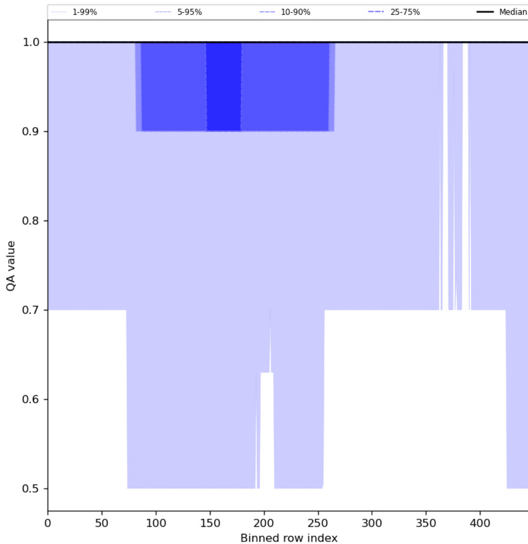
Figure 46: Along track statistics of “QA value” for 2023-07-11 to 2023-07-13
