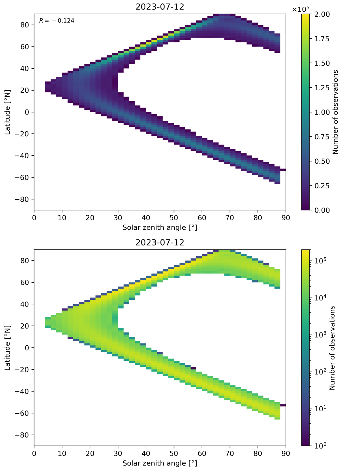
Figure 124: Scatter density plot of “Solar zenith angle” against “Latitude” for 2023-07-11 to 2023-07-13.
