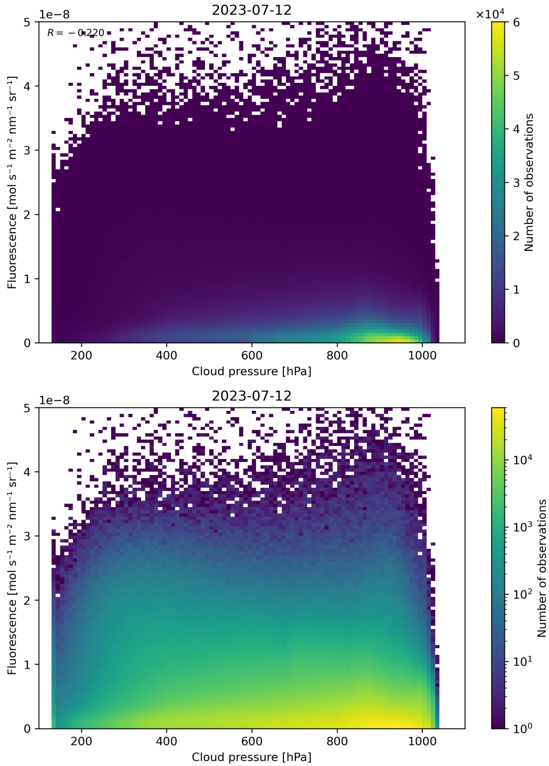
Figure 88: Scatter density plot of “Cloud pressure” against “Fluorescence” for 2023-07-11 to 2023-07-13.
