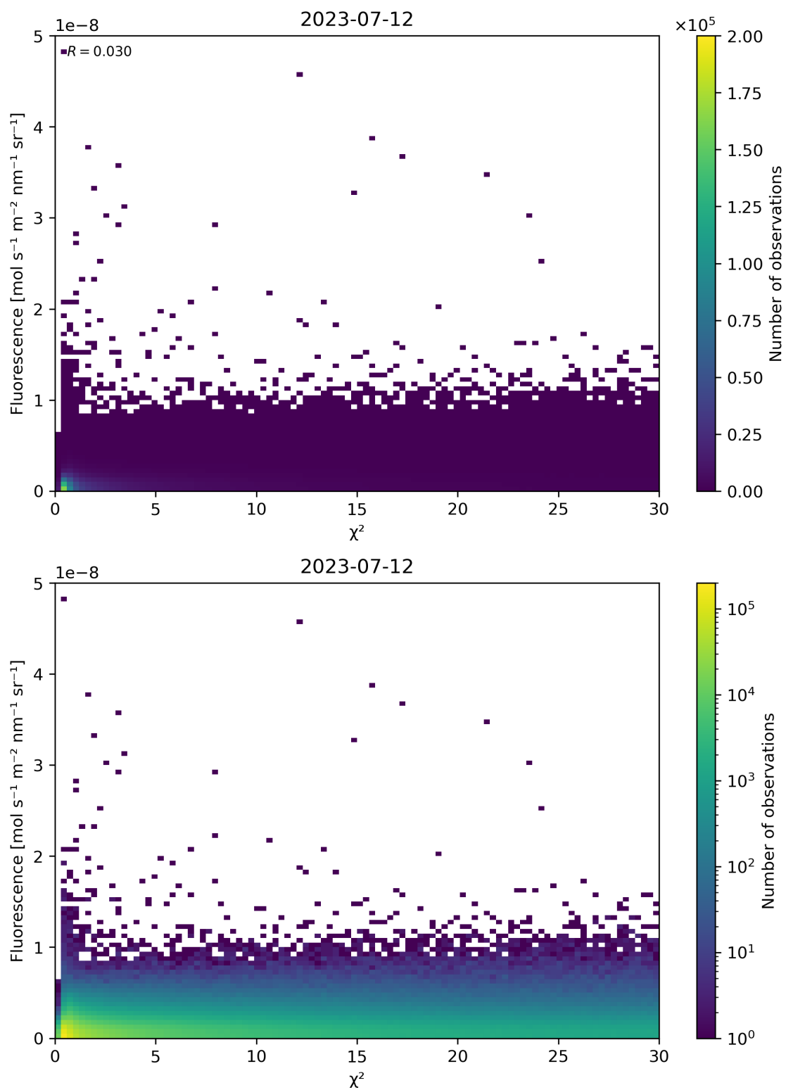
Figure 70: Scatter density plot of “ \chi^2 ” against “Fluorescence” for 2023-07-11 to 2023-07-13.
