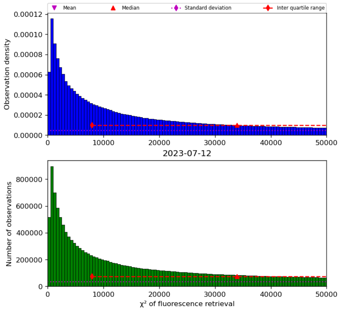
Figure 42: Histogram of “ \chi^2 of fluorescence retrieval” for 2023-07-11 to 2023-07-13
