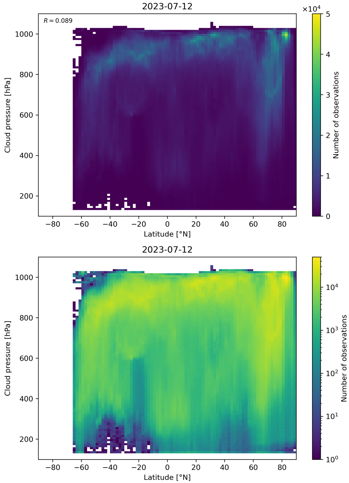
Figure 100: Scatter density plot of “Latitude” against “Cloud pressure” for 2023-07-11 to 2023-07-13.
