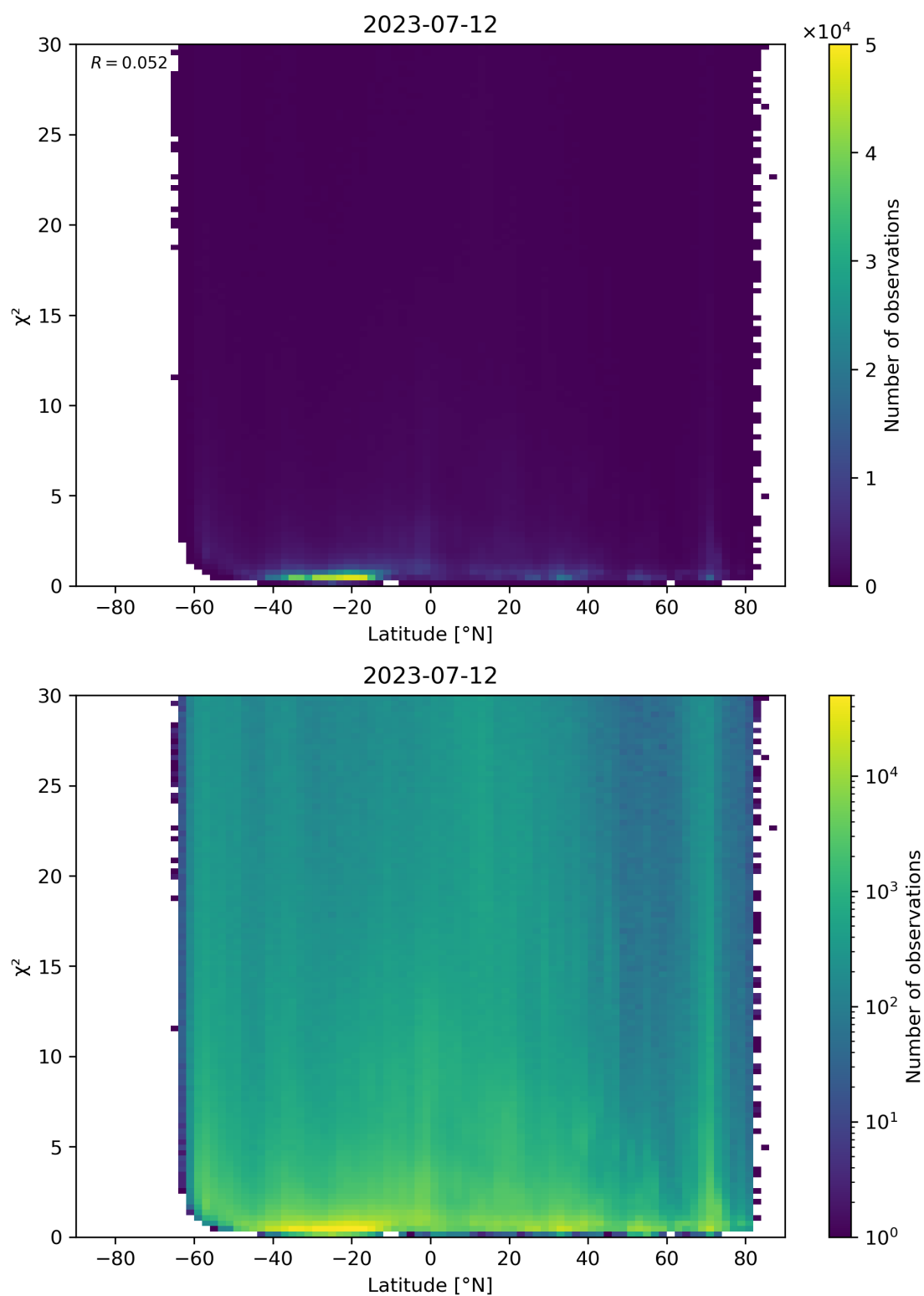
Figure 97: Scatter density plot of “Latitude” against “ \chi^2 ” for 2023-07-11 to 2023-07-13.
