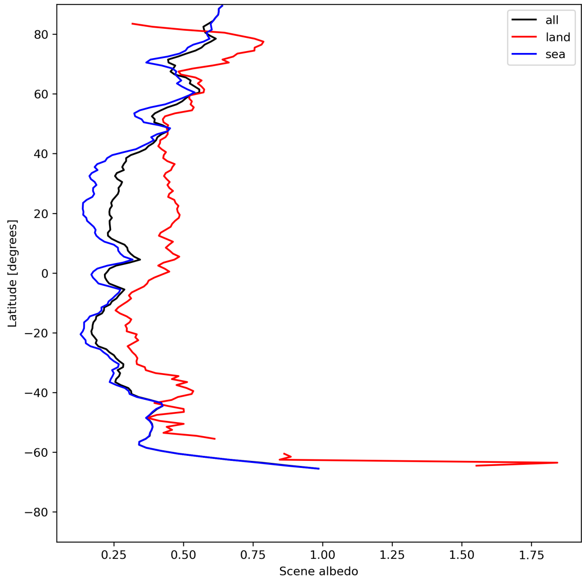
Figure 17: Zonal average of “Scene albedo” for 2023-07-11 to 2023-07-13.
