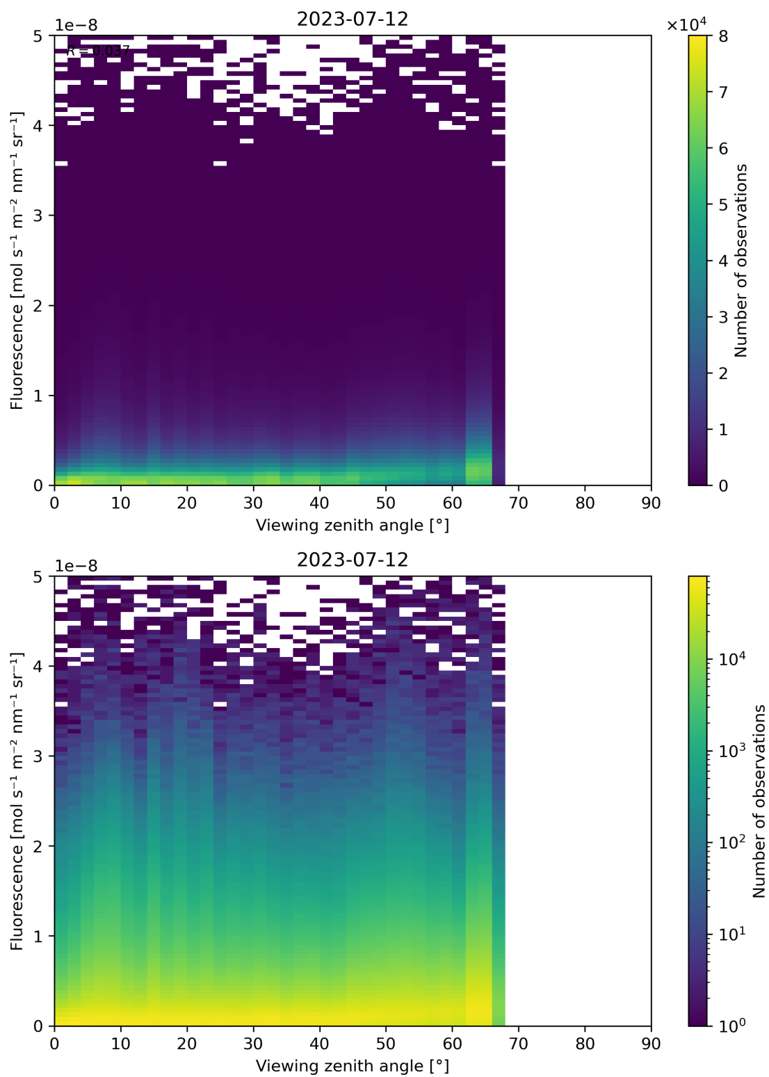
Figure 134: Scatter density plot of “Viewing zenith angle” against “Fluorescence” for 2023-07-11 to 2023-07-13.
