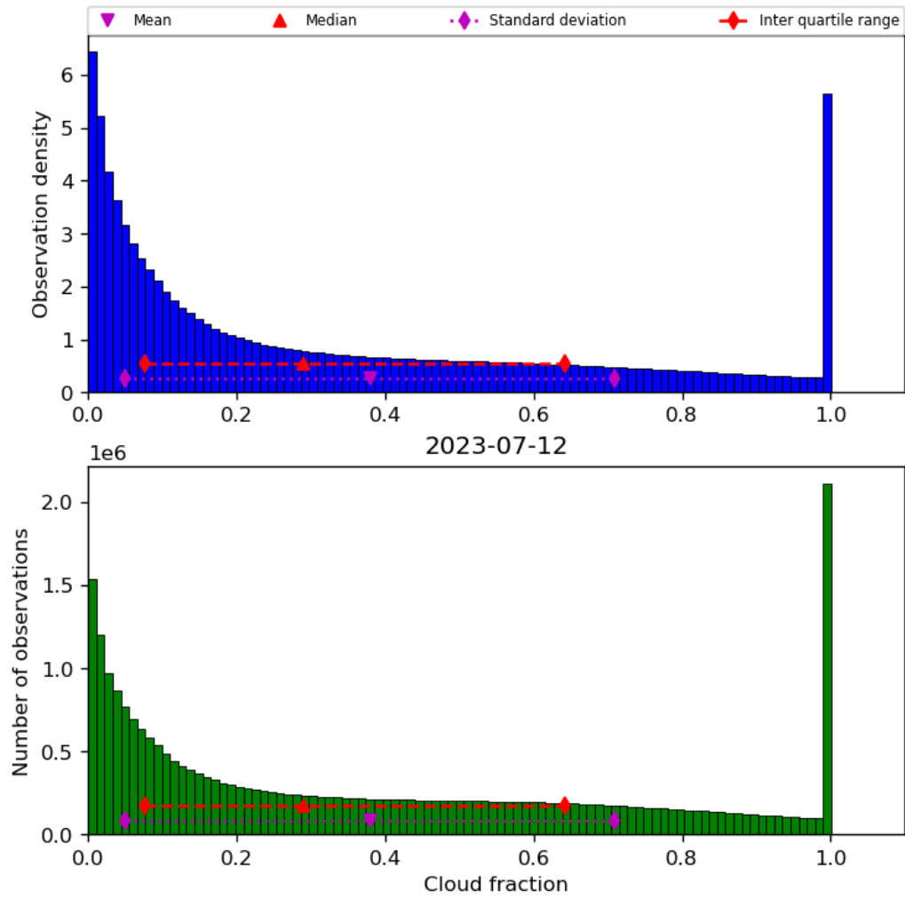
Figure 32: Histogram of “Cloud fraction” for 2023-07-11 to 2023-07-13
