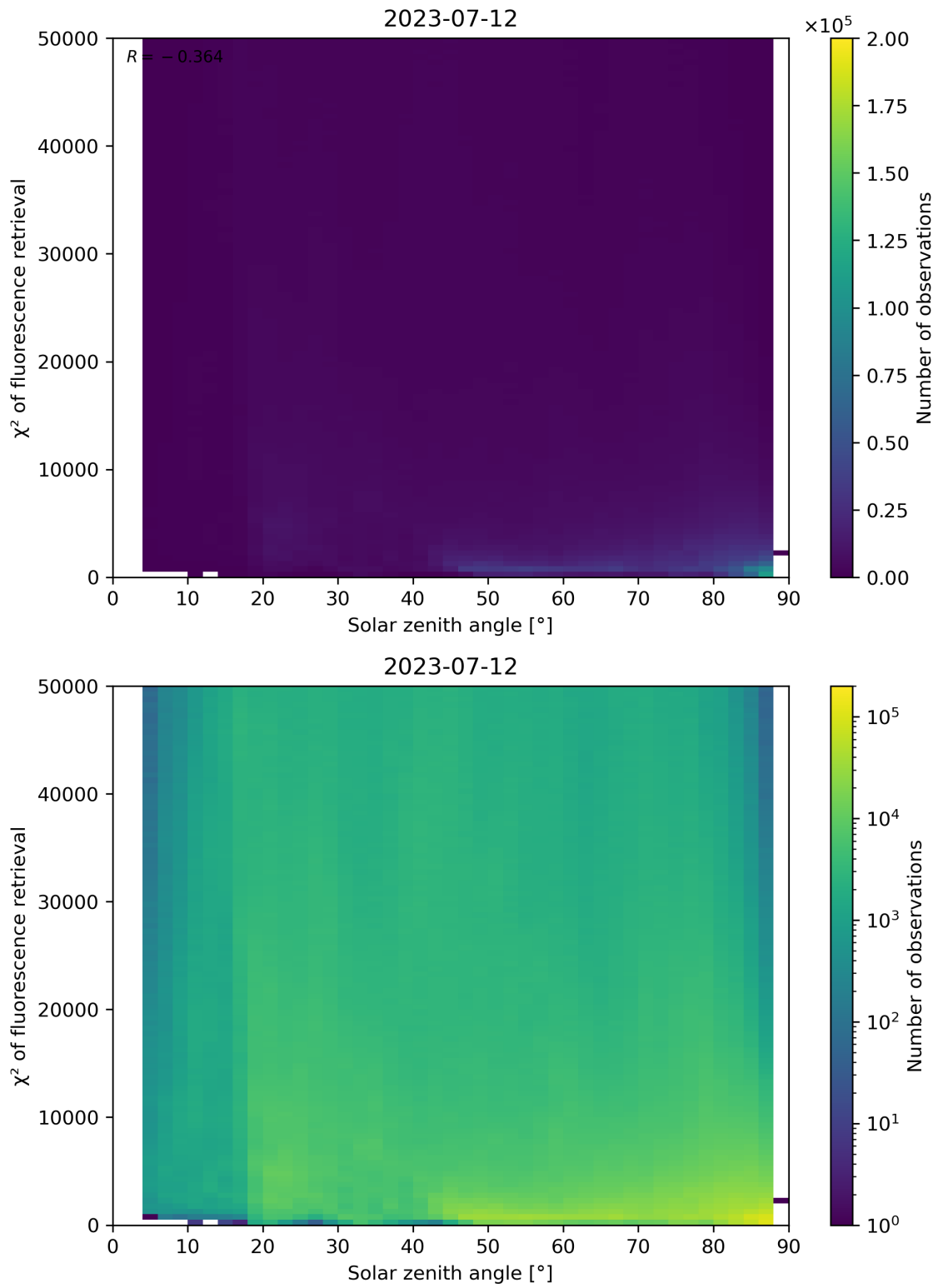
Figure 120: Scatter density plot of “Solar zenith angle” against “ \chi^2 of fluorescence retrieval” for 2023-07-11 to 2023-07-13.
