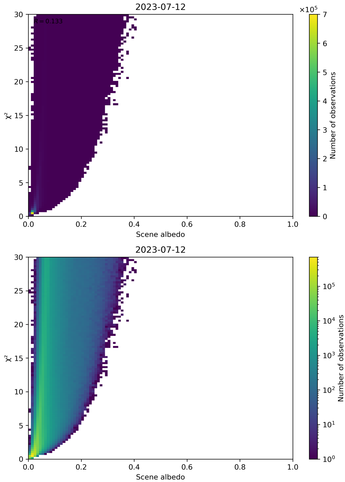
Figure 112: Scatter density plot of “Scene albedo” against “ \chi^2 ” for 2023-07-11 to 2023-07-13.
