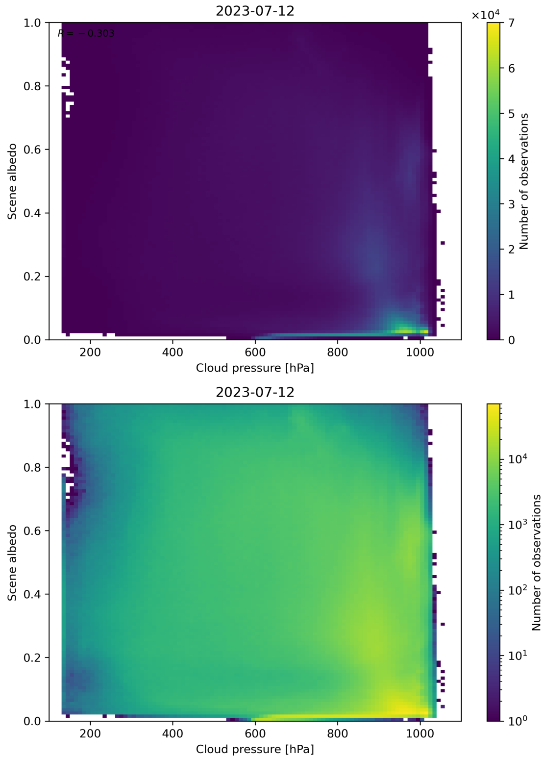
Figure 91: Scatter density plot of “Cloud pressure” against “Scene albedo” for 2023-07-11 to 2023-07-13.
