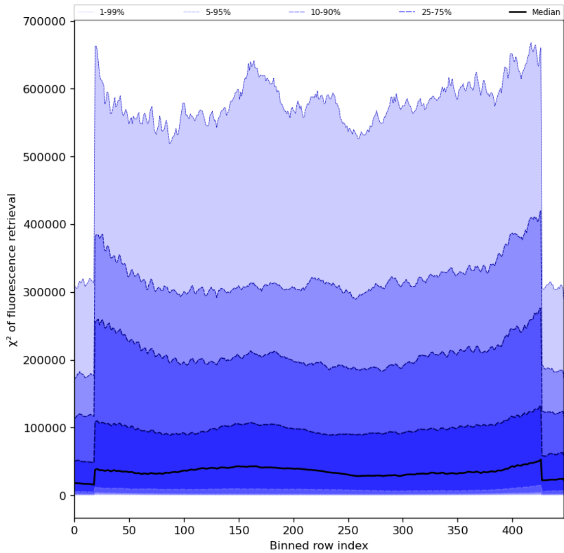
Figure 59: Along track statistics of “ \chi^2 of fluorescence retrieval” for 2023-07-11 to 2023-07-13
