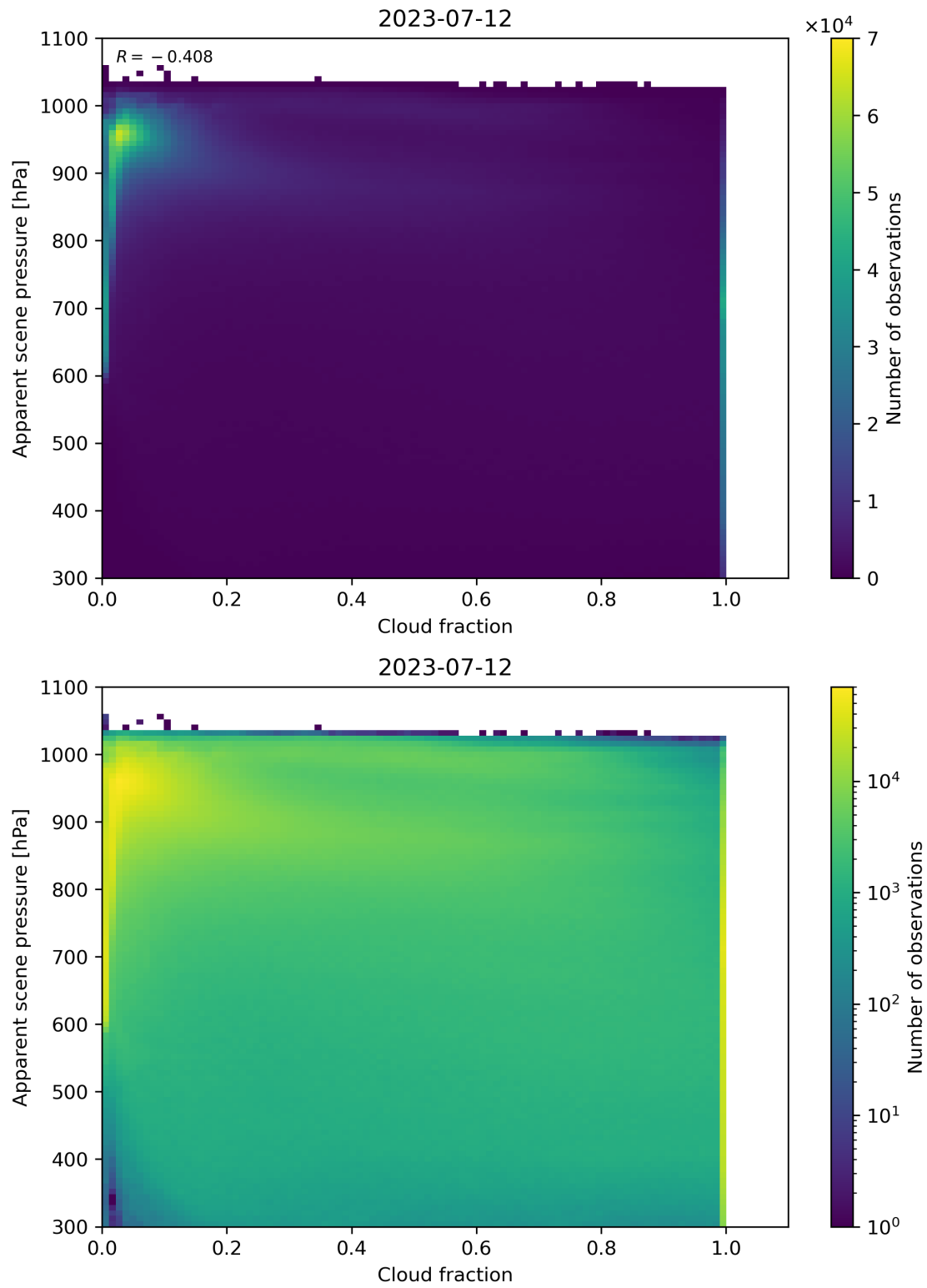
Figure 76: Scatter density plot of “Cloud fraction” against “Apparent scene pressure” for 2023-07-11 to 2023-07-13.
