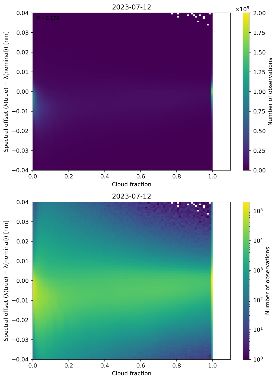
Figure 83: Scatter density plot of “Cloud fraction” against “Spectral offset ( \lambda(\text{true}) - \lambda(\text{nominal}) )” for 2023-07-11 to 2023-07-13.
