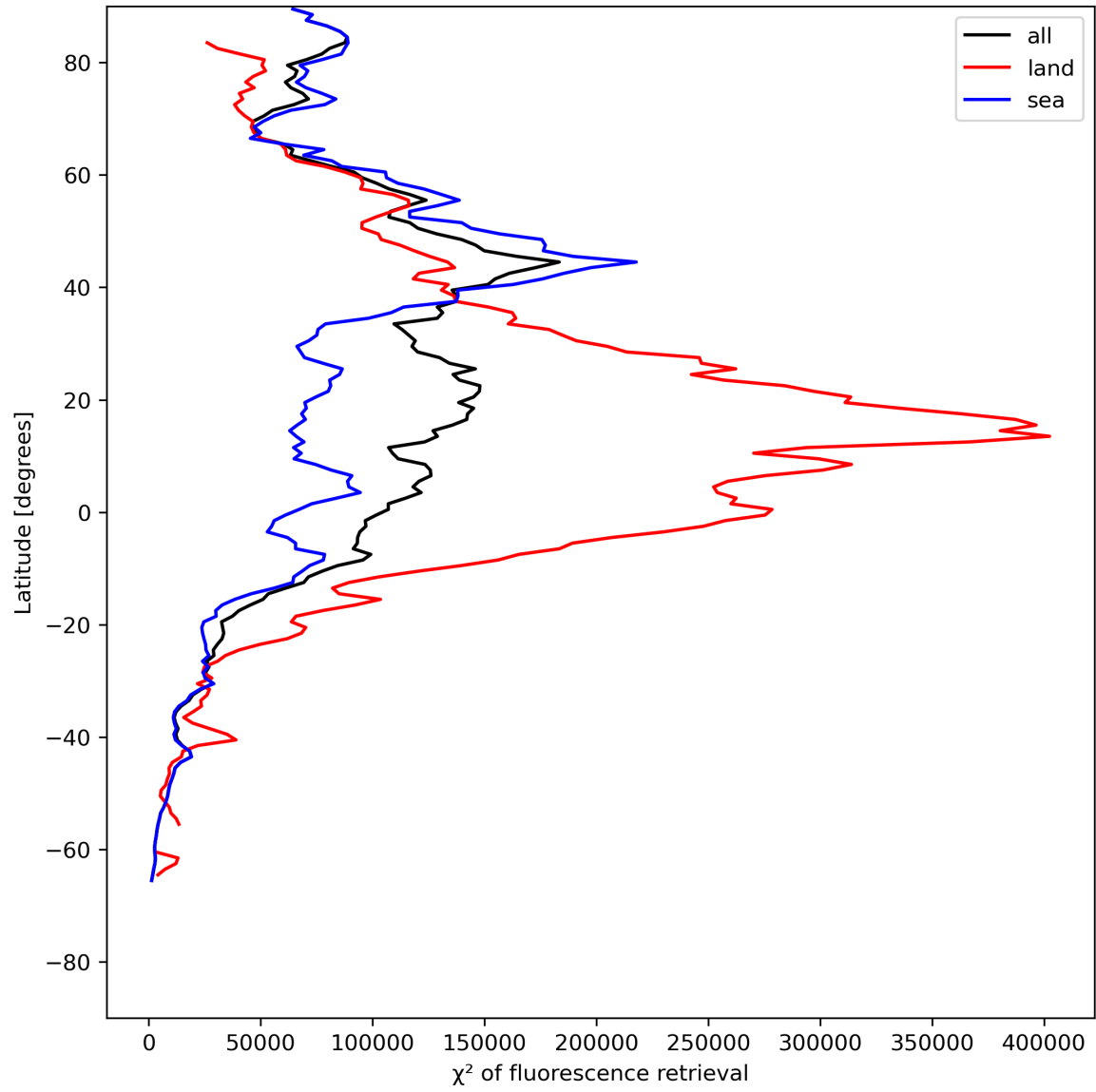
Figure 25: Zonal average of “ \chi^2 of fluorescence retrieval” for 2023-07-11 to 2023-07-13.
