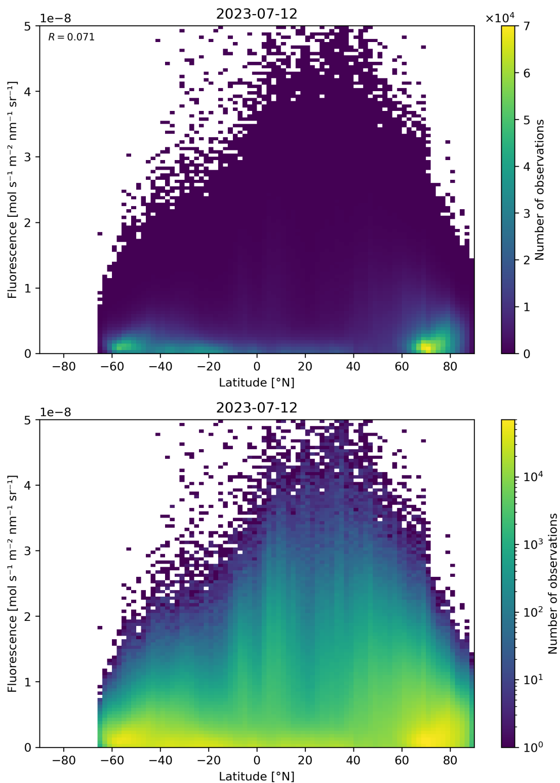
Figure 101: Scatter density plot of “Latitude” against “Fluorescence” for 2023-07-11 to 2023-07-13.
