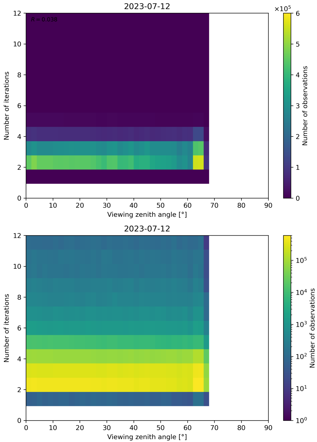
Figure 136: Scatter density plot of “Viewing zenith angle” against “Number of iterations” for 2023-07-11 to 2023-07-13.
