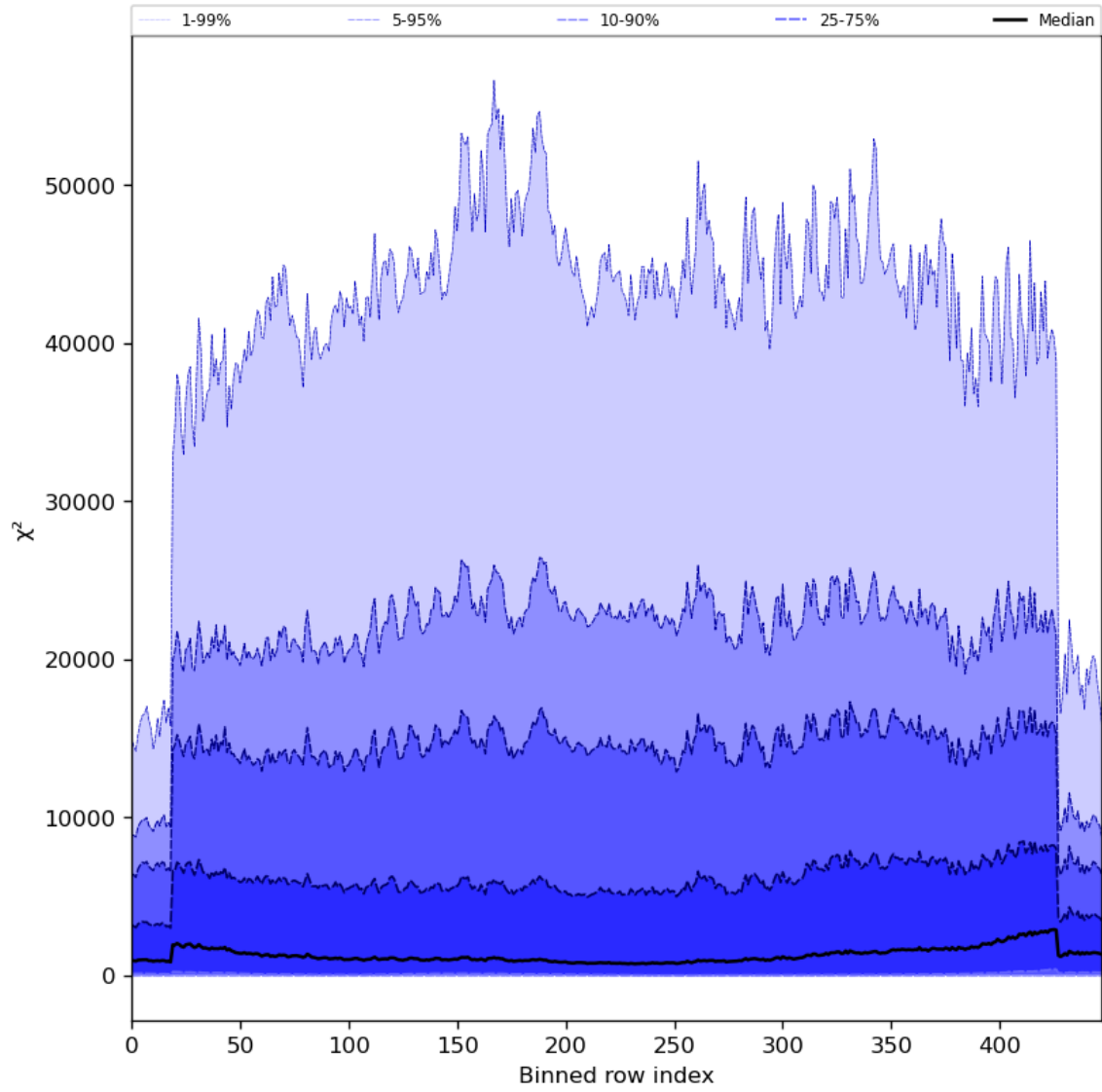
Figure 55: Along track statistics of “ \chi^2 ” for 2023-07-11 to 2023-07-13
