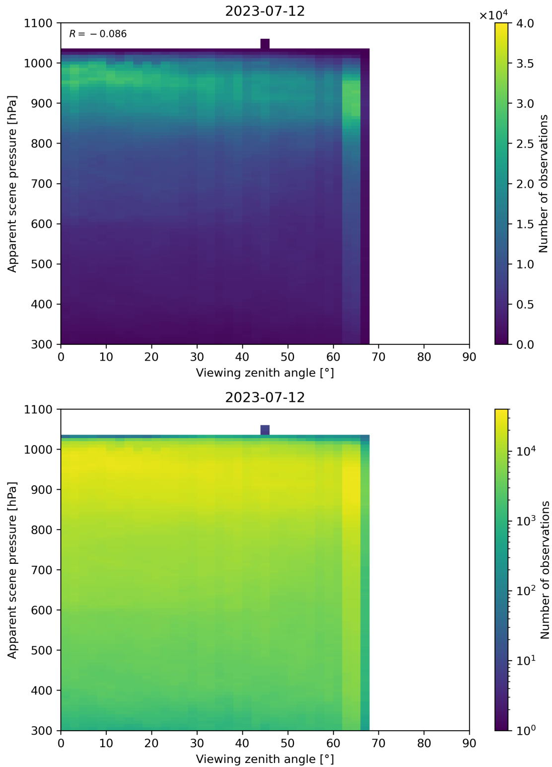
Figure 129: Scatter density plot of “Viewing zenith angle” against “Apparent scene pressure” for 2023-07-11 to 2023-07-13.
