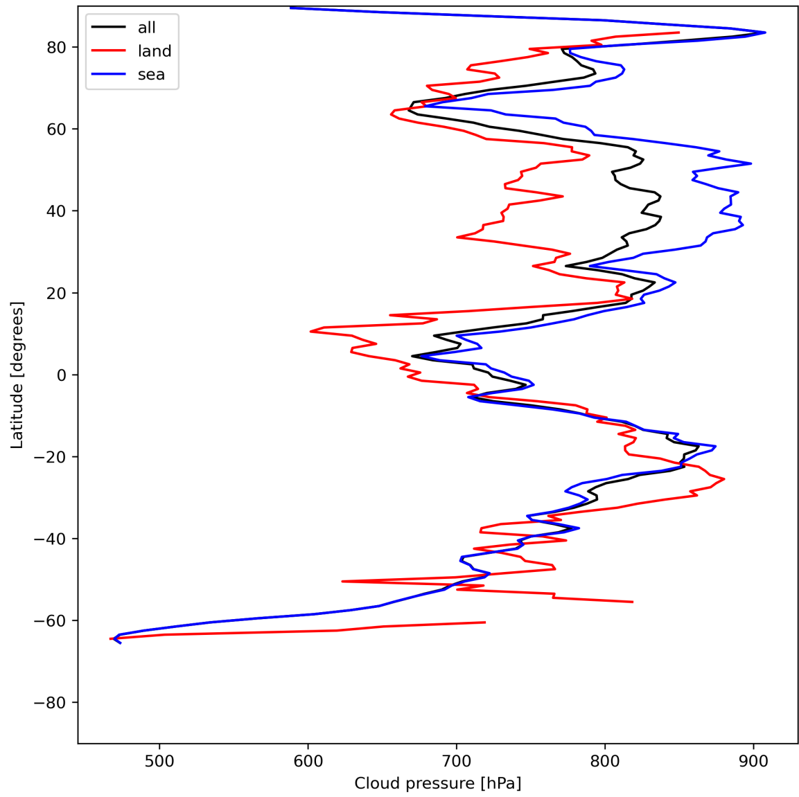
Figure 13: Zonal average of “Cloud pressure” for 2023-07-11 to 2023-07-13.
