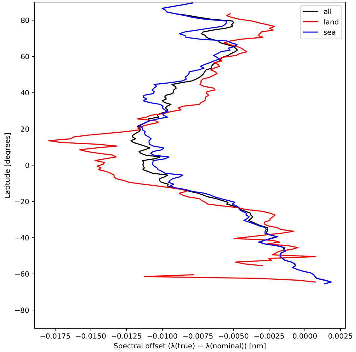
Figure 28: Zonal average of “Spectral offset ( \lambda(\text{true}) - \lambda(\text{nominal}) )” for 2023-07-11 to 2023-07-13.
