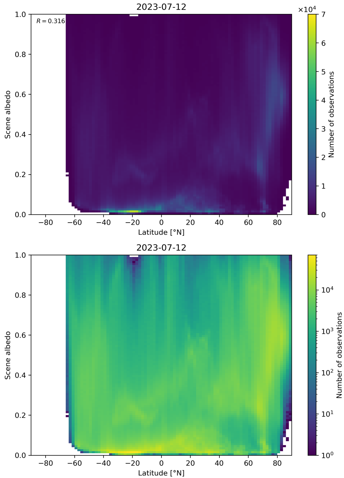
Figure 104: Scatter density plot of “Latitude” against “Scene albedo” for 2023-07-11 to 2023-07-13.
