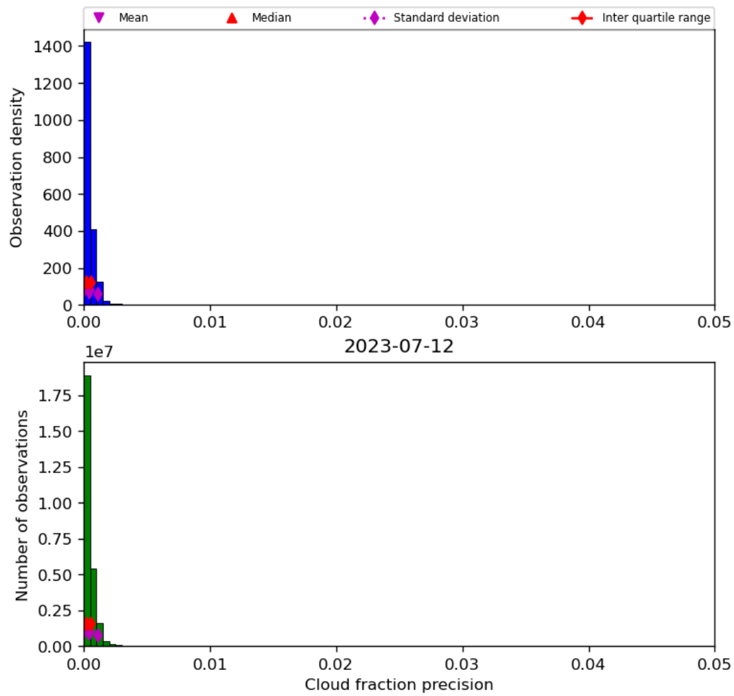
Figure 33: Histogram of “Cloud fraction precision” for 2023-07-11 to 2023-07-13
