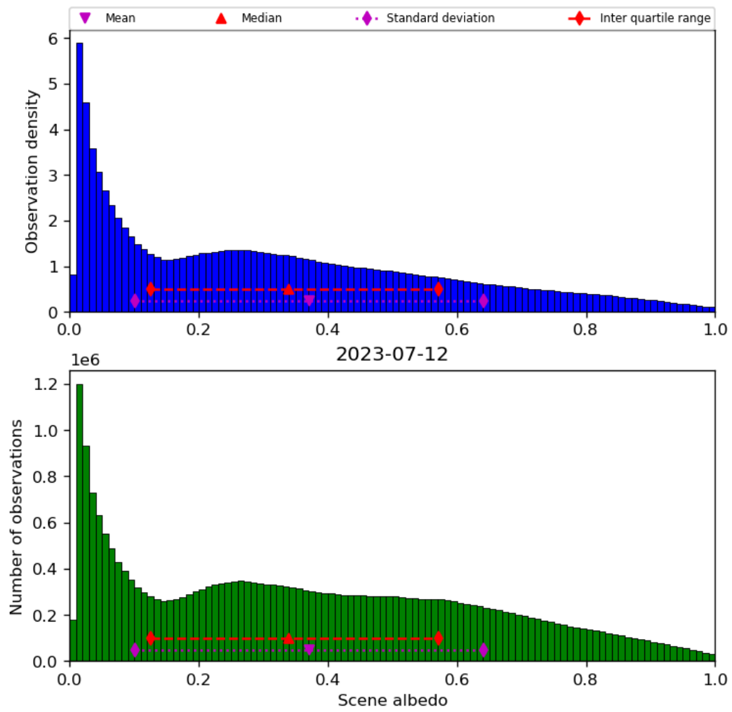
Figure 34: Histogram of “Scene albedo” for 2023-07-11 to 2023-07-13
