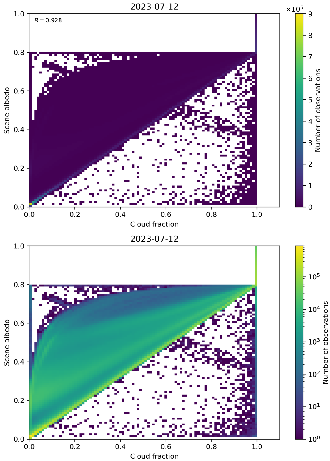
Figure 82: Scatter density plot of “Cloud fraction” against “Scene albedo” for 2023-07-11 to 2023-07-13.
