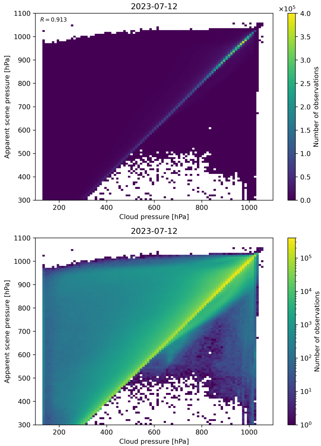
Figure 84: Scatter density plot of “Cloud pressure” against “Apparent scene pressure” for 2023-07-11 to 2023-07-13.
