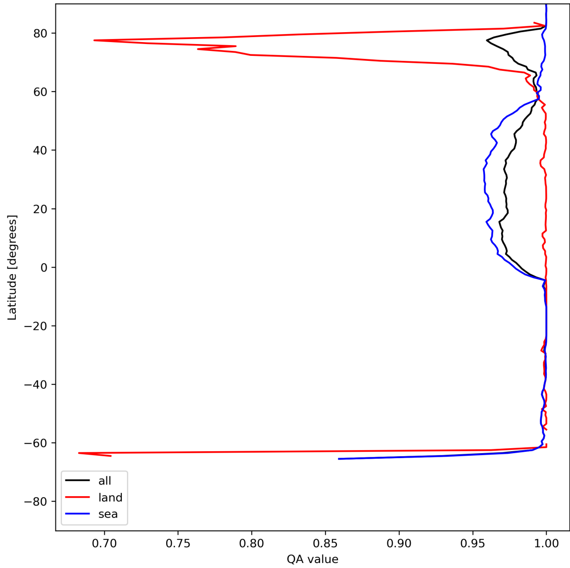
Figure 12: Zonal average of “QA value” for 2023-07-11 to 2023-07-13.
