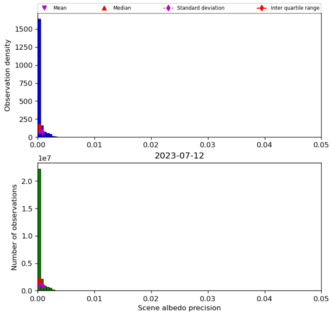
Figure 35: Histogram of “Scene albedo precision” for 2023-07-11 to 2023-07-13
