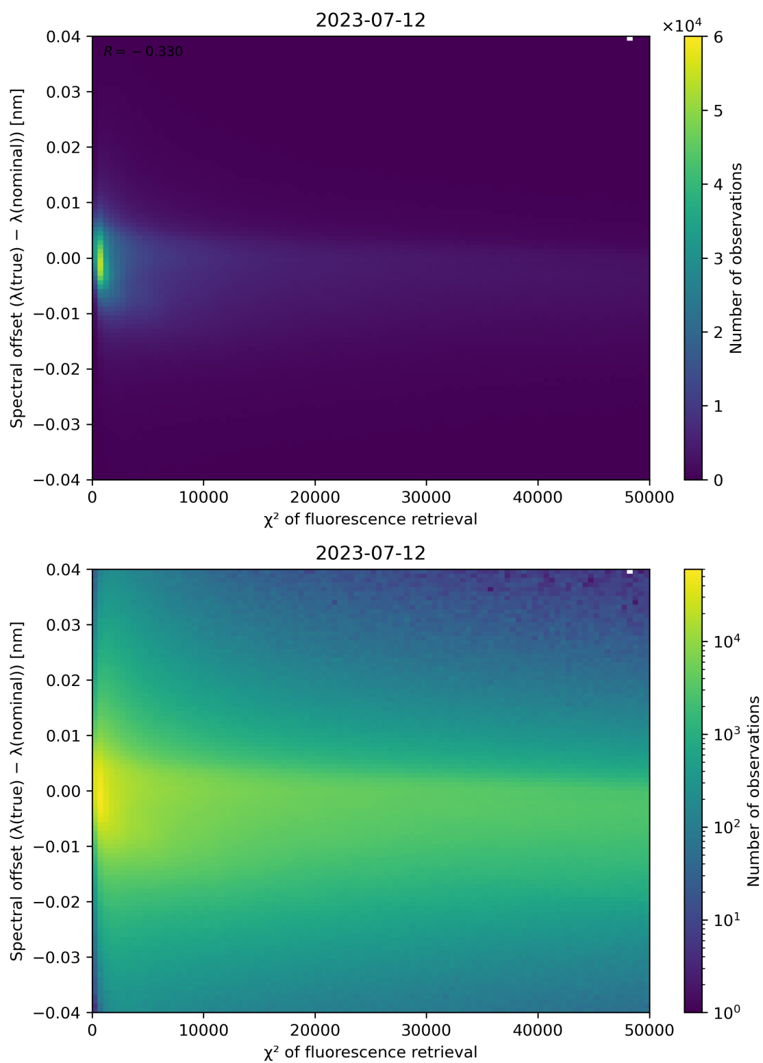
Figure 72: Scatter density plot of “ \chi^2 of fluorescence retrieval” against “Spectral offset ( \lambda(\text{true}) - \lambda(\text{nominal}) )” for 2023-07-11 to 2023-07-13.
