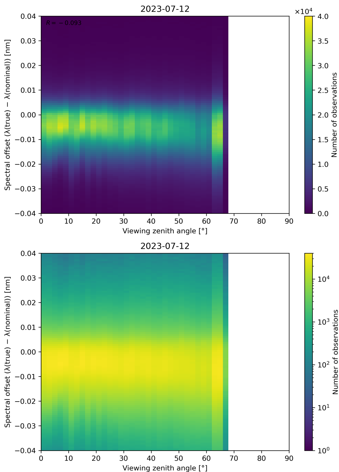
Figure 140: Scatter density plot of “Viewing zenith angle” against “Spectral offset ( \lambda(\text{true}) - \lambda(\text{nominal}) )” for 2023-07-11 to 2023-07-13.
