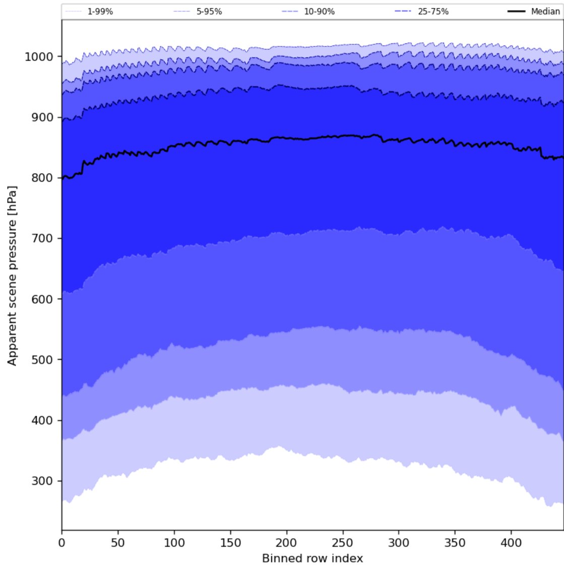
Figure 53: Along track statistics of “Apparent scene pressure” for 2023-07-11 to 2023-07-13
