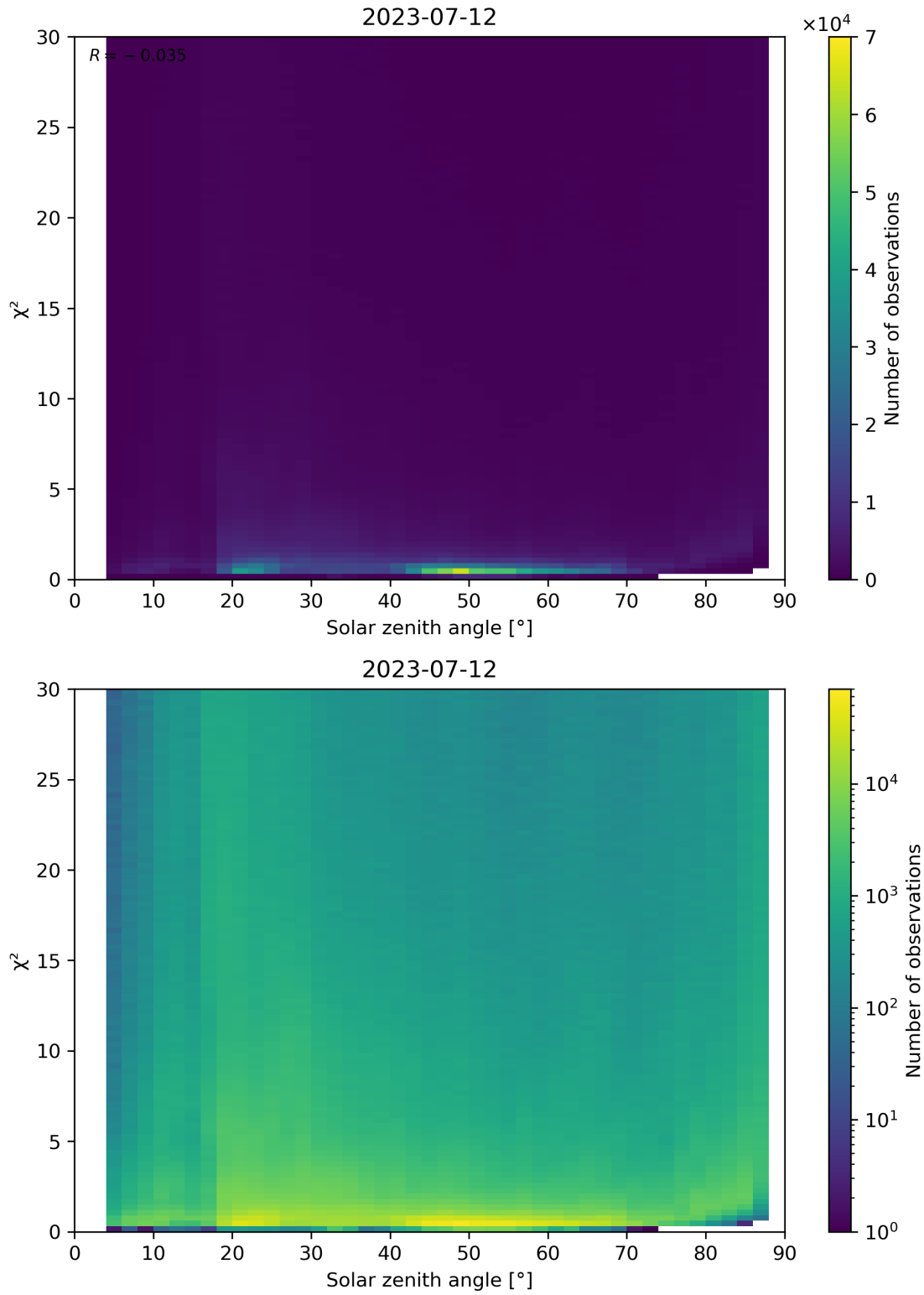
Figure 119: Scatter density plot of “Solar zenith angle” against “ \chi^2 ” for 2023-07-11 to 2023-07-13.
