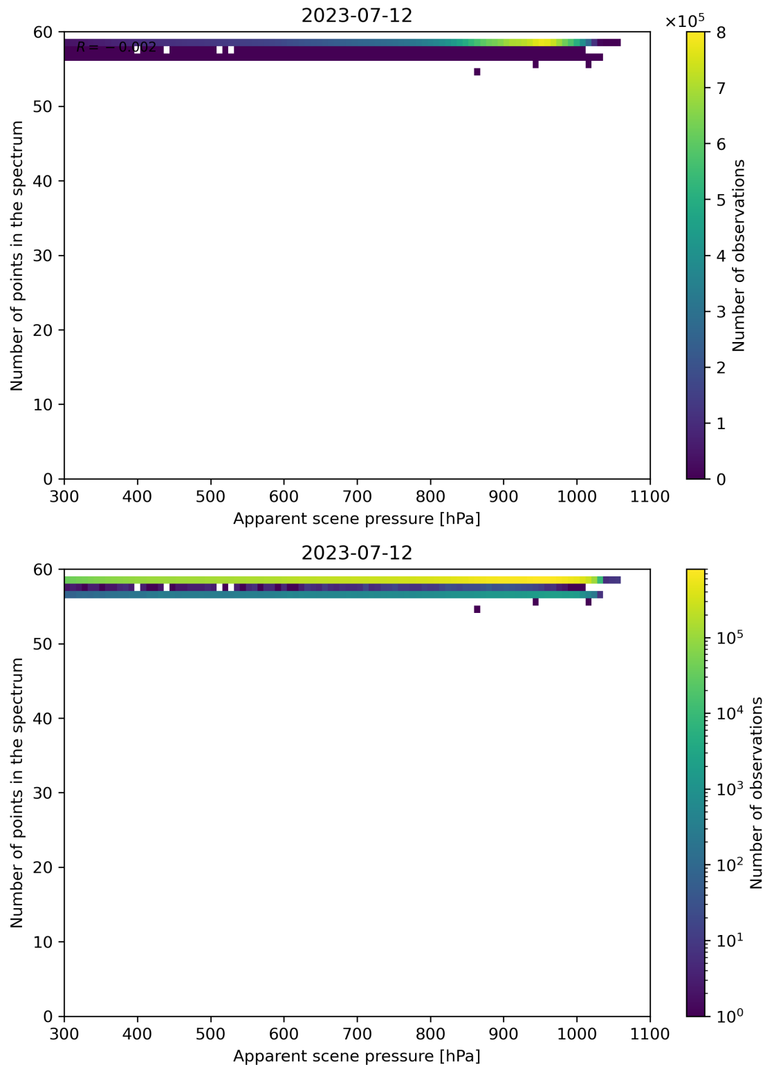
Figure 67: Scatter density plot of “Apparent scene pressure” against “Number of points in the spectrum” for 2023-07-11 to 2023-07-13.
