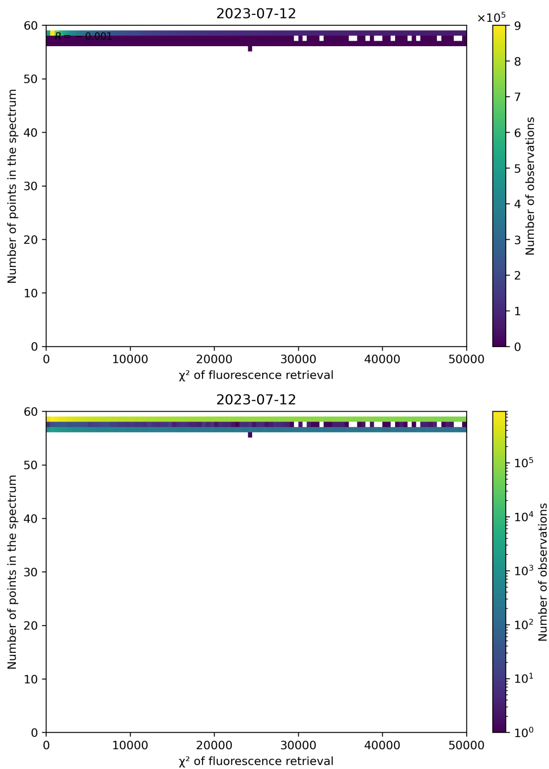
Figure 71: Scatter density plot of " \chi^2 of fluorescence retrieval" against "Number of points in the spectrum" for 2023-07-11 to 2023-07-13.
