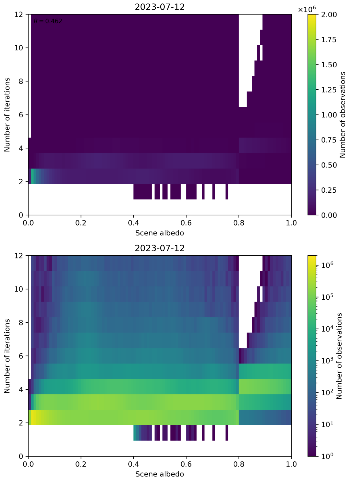
Figure 115: Scatter density plot of “Scene albedo” against “Number of iterations” for 2023-07-11 to 2023-07-13.
