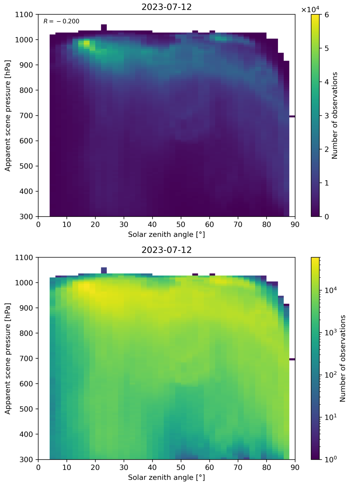
Figure 118: Scatter density plot of “Solar zenith angle” against “Apparent scene pressure” for 2023-07-11 to 2023-07-13.
