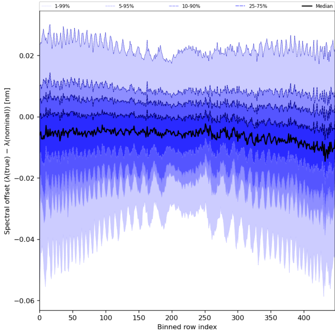
Figure 62: Along track statistics of “Spectral offset ( \lambda(\text{true}) - \lambda(\text{nominal}) )” for 2023-07-11 to 2023-07-13
