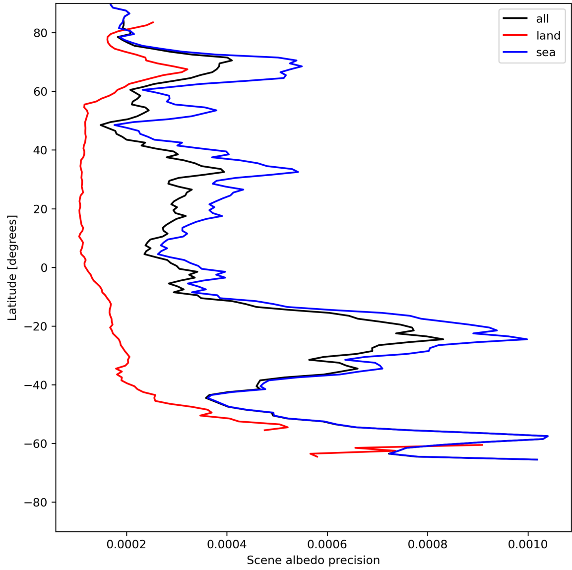
Figure 18: Zonal average of “Scene albedo precision” for 2023-07-11 to 2023-07-13.
