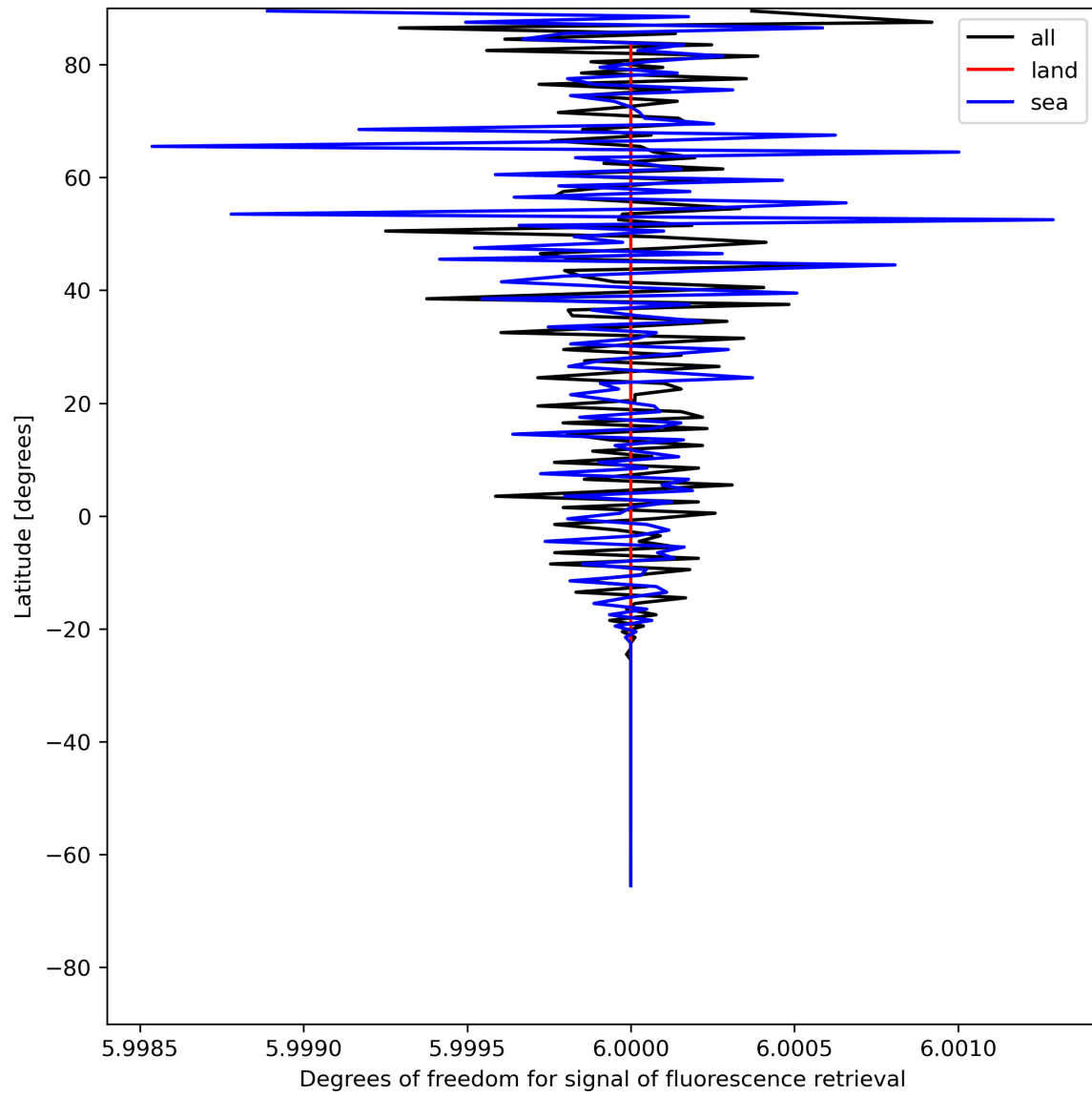
Figure 26: Zonal average of “Degrees of freedom for signal of fluorescence retrieval” for 2023-07-11 to 2023-07-13.
