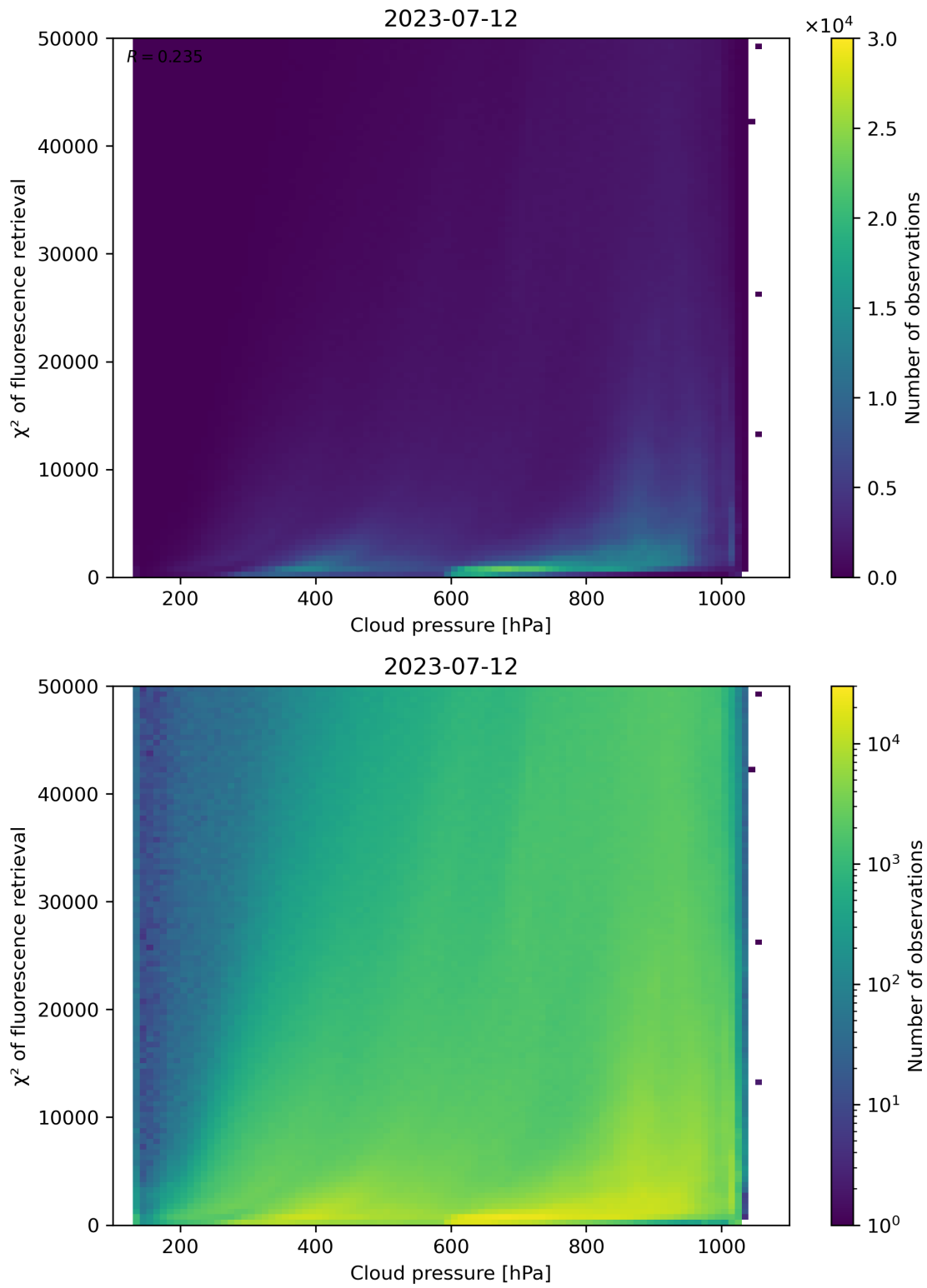
Figure 86: Scatter density plot of “Cloud pressure” against “ \chi^2 of fluorescence retrieval” for 2023-07-11 to 2023-07-13.
