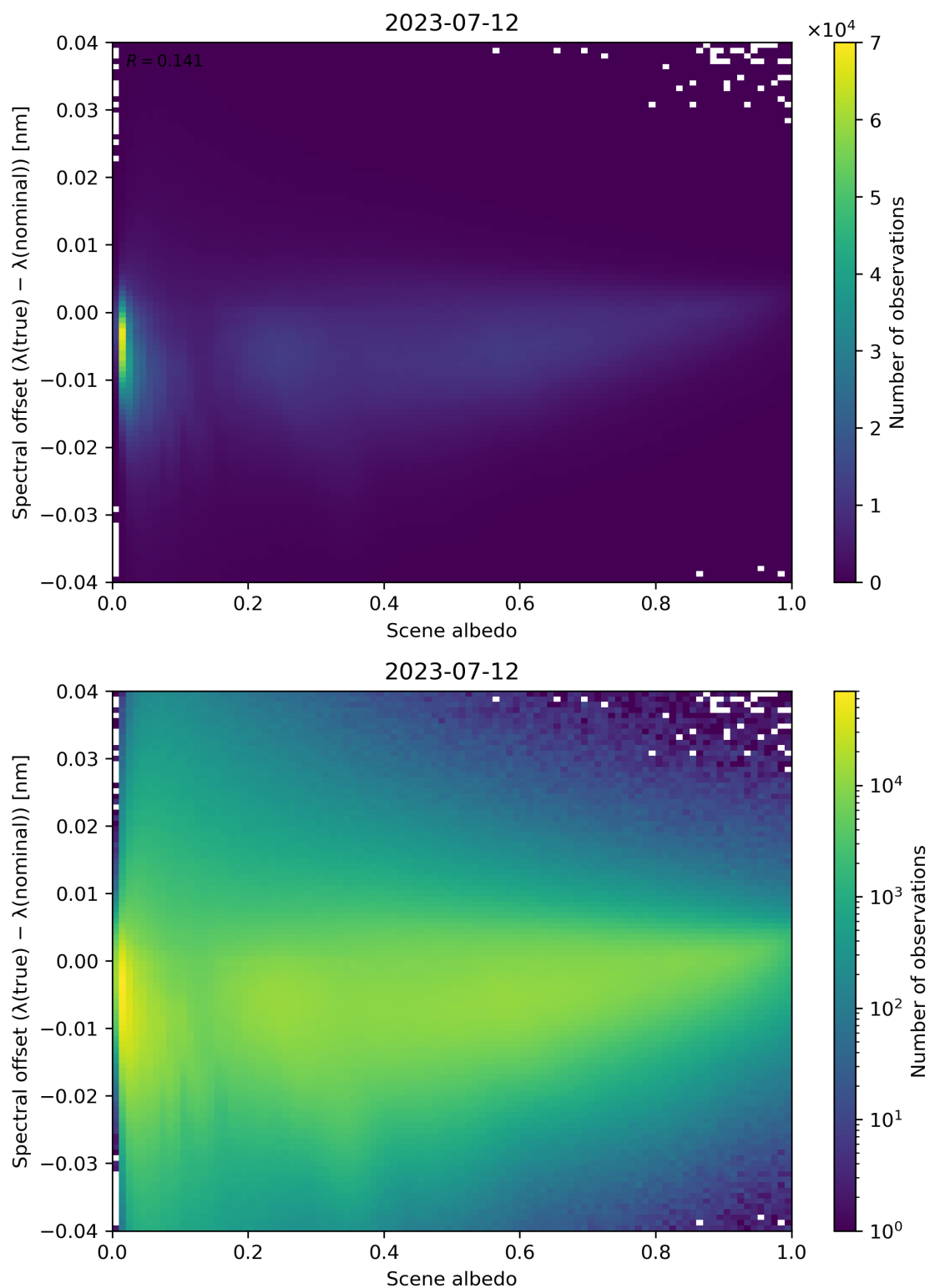
Figure 117: Scatter density plot of “Scene albedo” against “Spectral offset ( \lambda(\text{true}) - \lambda(\text{nominal}) )” for 2023-07-11 to 2023-07-13.
