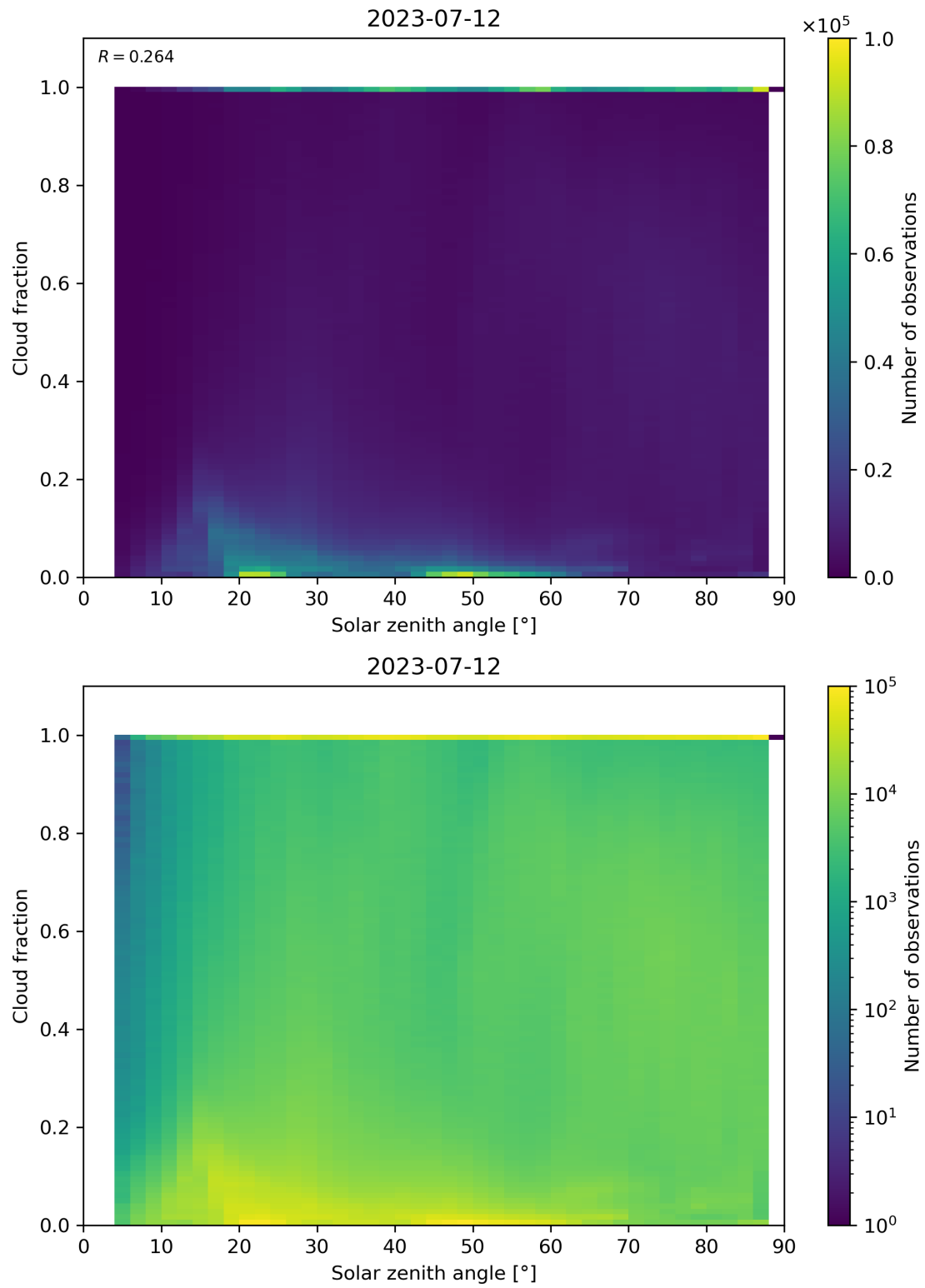
Figure 121: Scatter density plot of “Solar zenith angle” against “Cloud fraction” for 2023-07-11 to 2023-07-13.
