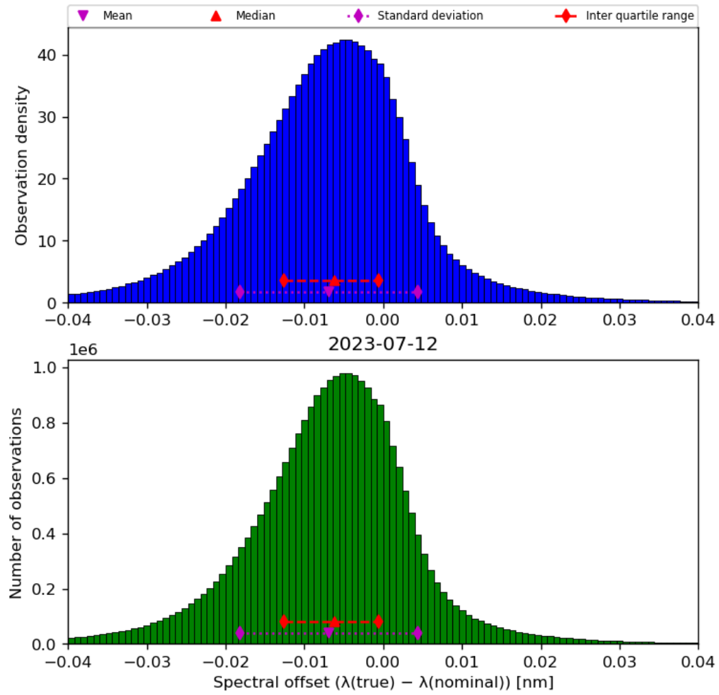
Figure 45: Histogram of “Spectral offset ( \lambda(\text{true}) - \lambda(\text{nominal}) )” for 2023-07-11 to 2023-07-13
