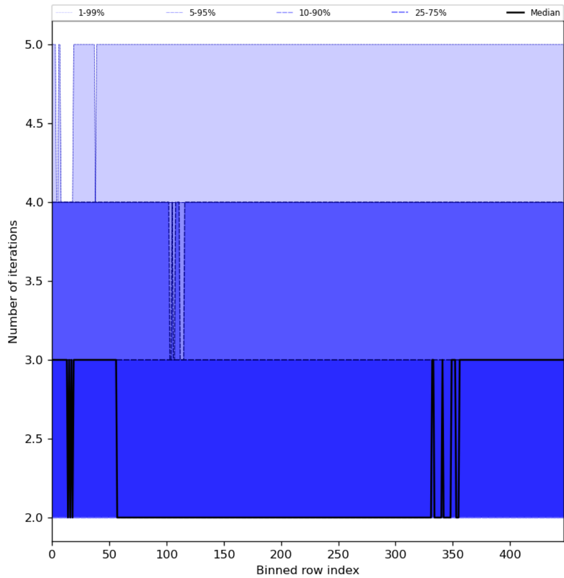
Figure 56: Along track statistics of “Number of iterations” for 2023-07-11 to 2023-07-13
