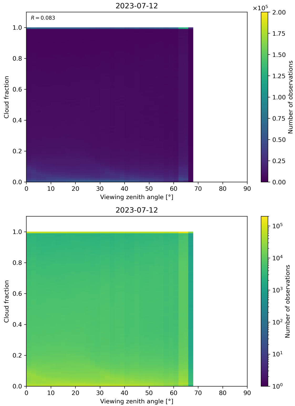
Figure 132: Scatter density plot of “Viewing zenith angle” against “Cloud fraction” for 2023-07-11 to 2023-07-13.
