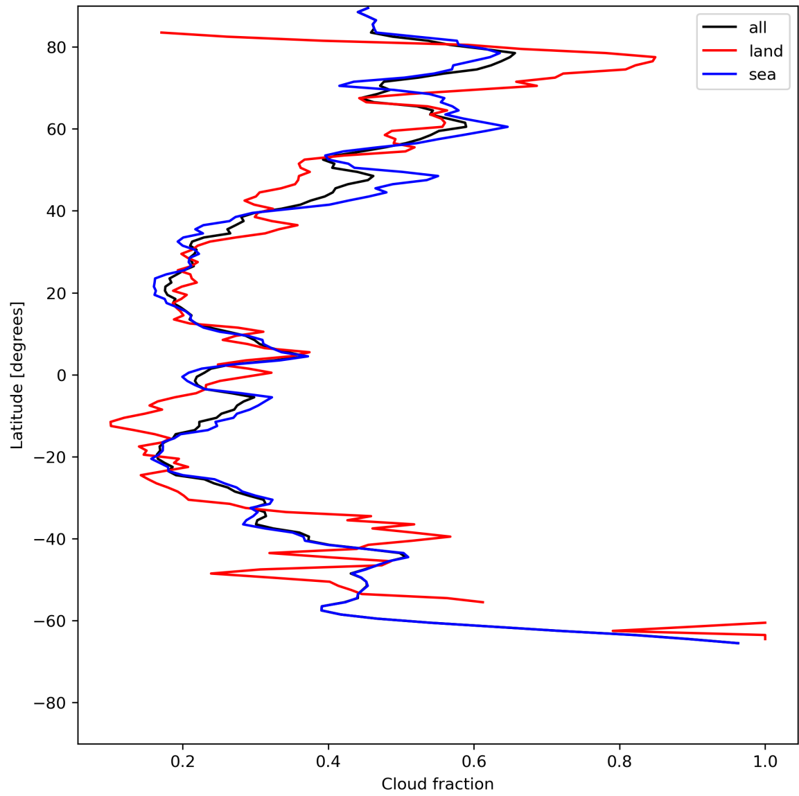
Figure 15: Zonal average of “Cloud fraction” for 2023-07-11 to 2023-07-13.
