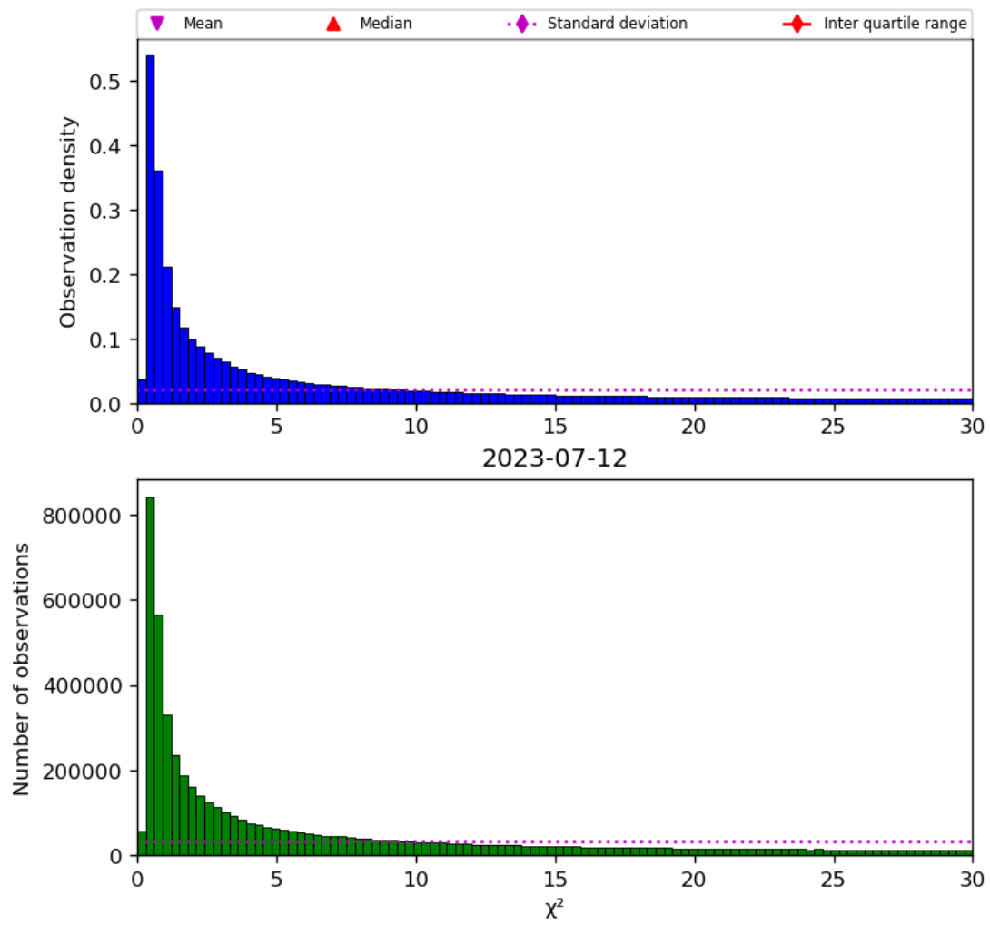
Figure 38: Histogram of “ \chi^2 ” for 2023-07-11 to 2023-07-13
