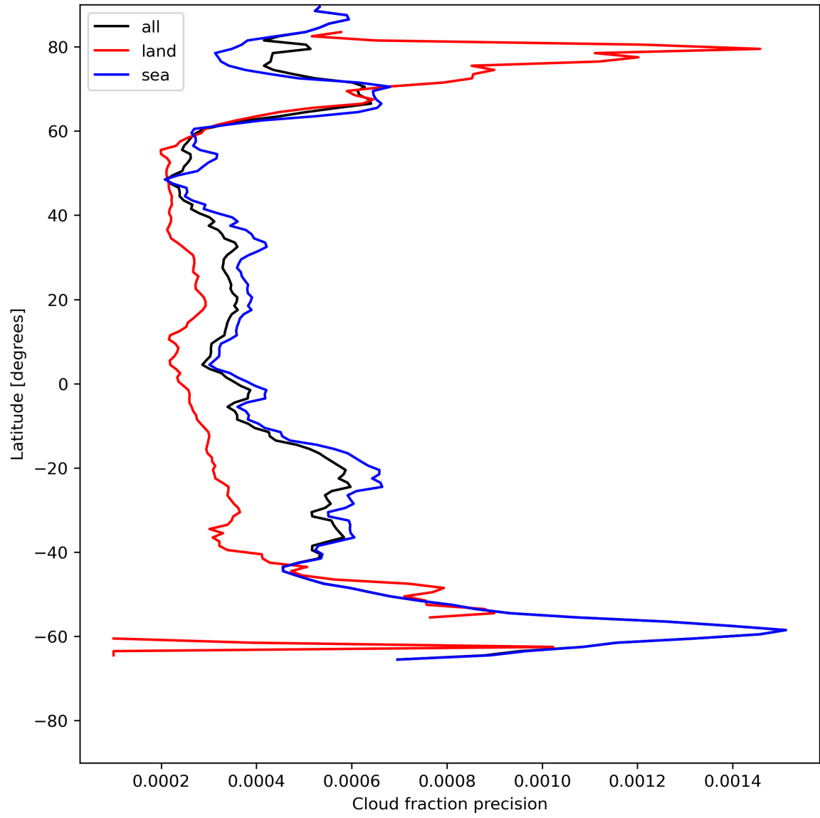
Figure 16: Zonal average of “Cloud fraction precision” for 2023-07-11 to 2023-07-13.
