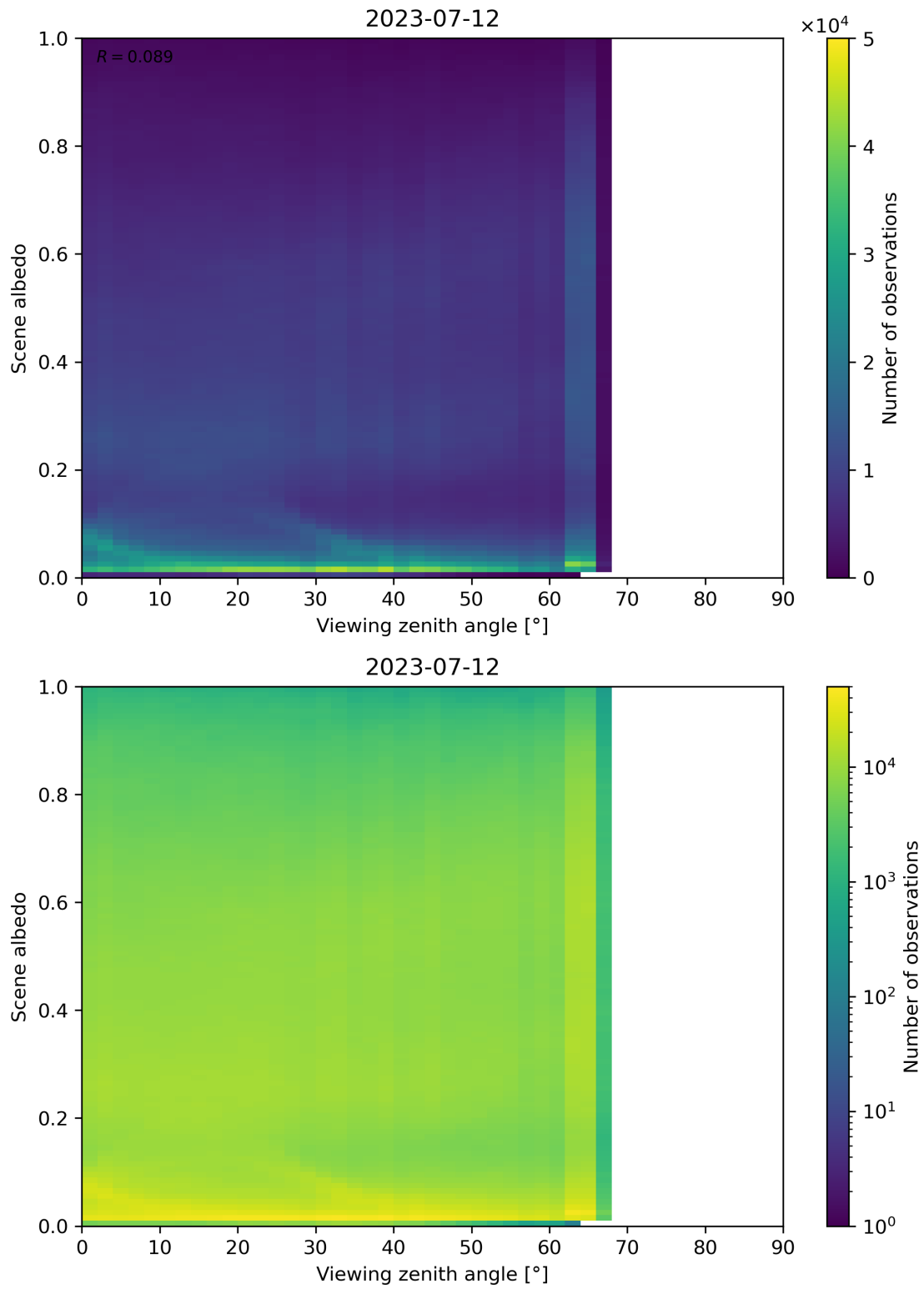
Figure 138: Scatter density plot of “Viewing zenith angle” against “Scene albedo” for 2023-07-11 to 2023-07-13.
