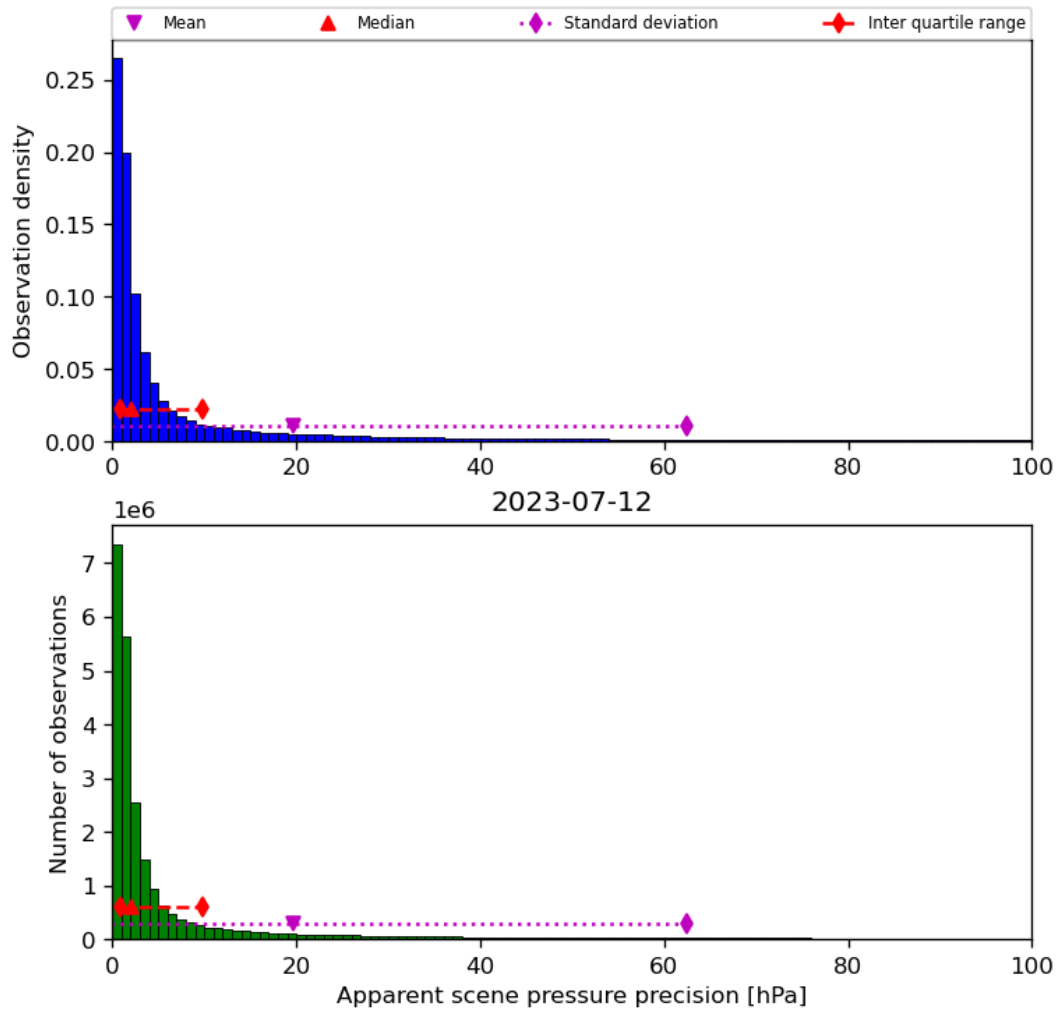
Figure 37: Histogram of “Apparent scene pressure precision” for 2023-07-11 to 2023-07-13
