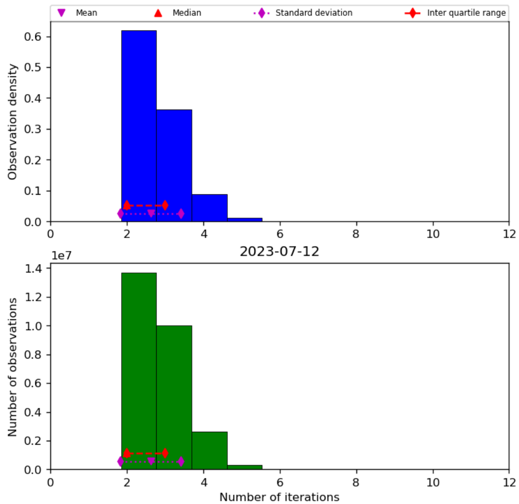
Figure 39: Histogram of “Number of iterations” for 2023-07-11 to 2023-07-13
