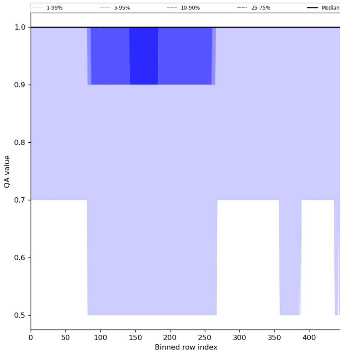
Figure 46: Along track statistics of “QA value” for 2023-07-13 to 2023-07-14
