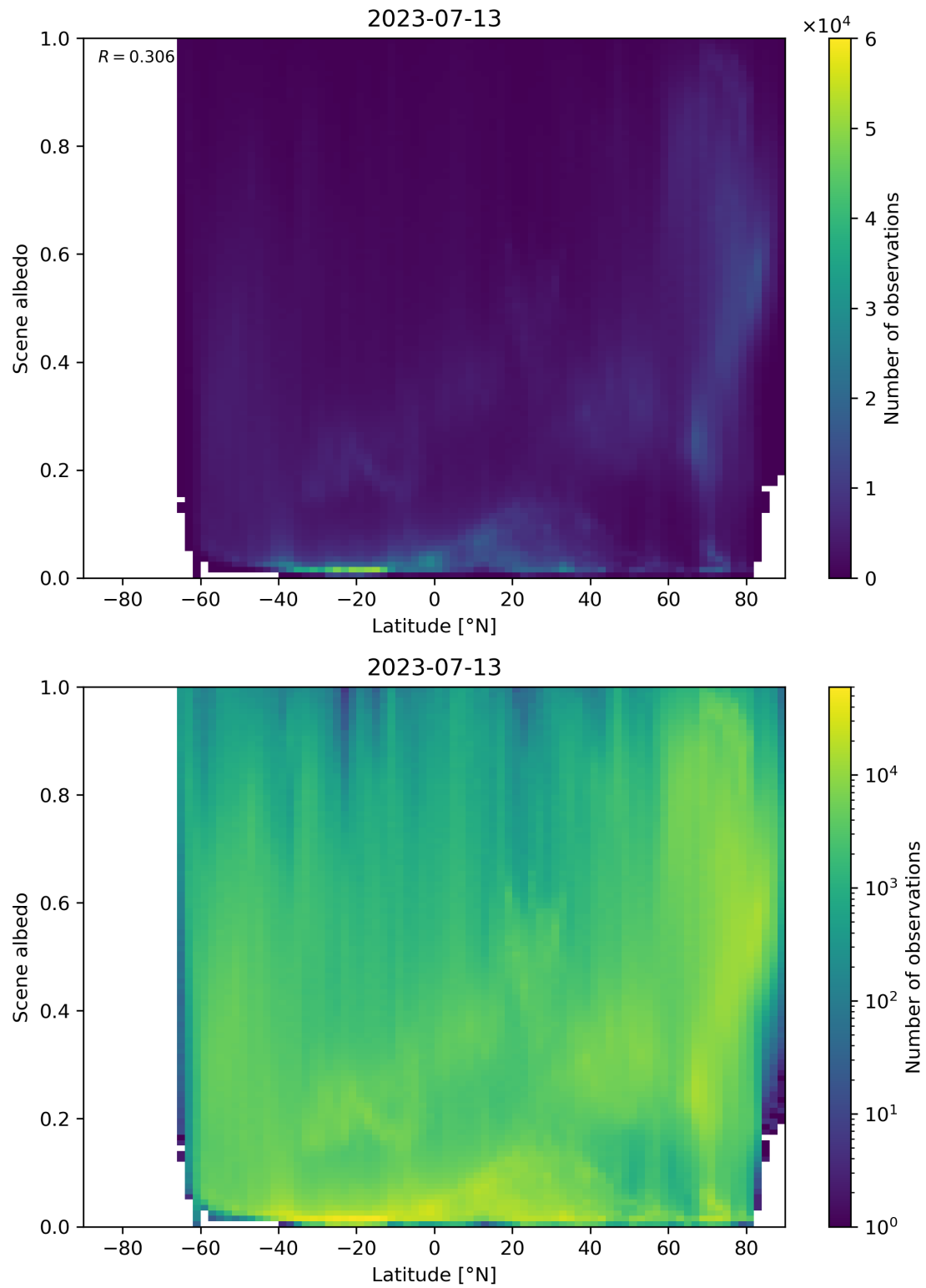
Figure 104: Scatter density plot of “Latitude” against “Scene albedo” for 2023-07-13 to 2023-07-14.
