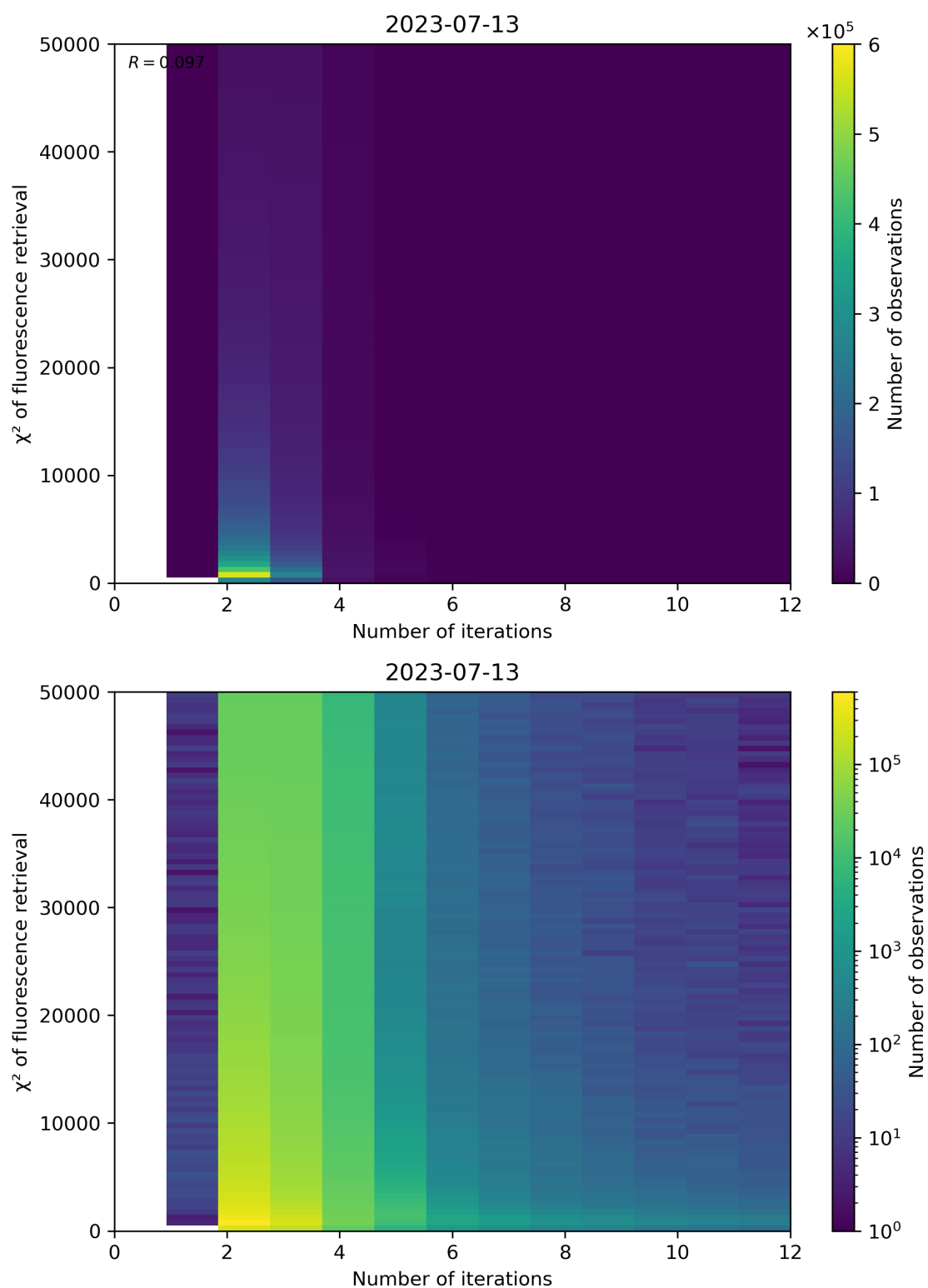
Figure 106: Scatter density plot of “Number of iterations” against “ \chi^2 of fluorescence retrieval” for 2023-07-13 to 2023-07-14.
