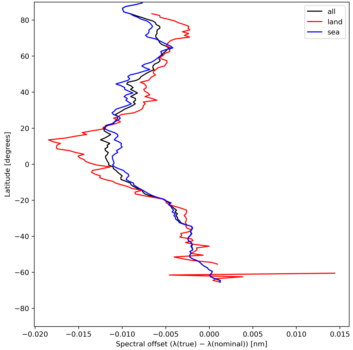
Figure 28: Zonal average of “Spectral offset ( \lambda(\text{true}) - \lambda(\text{nominal}) )” for 2023-07-13 to 2023-07-14.
