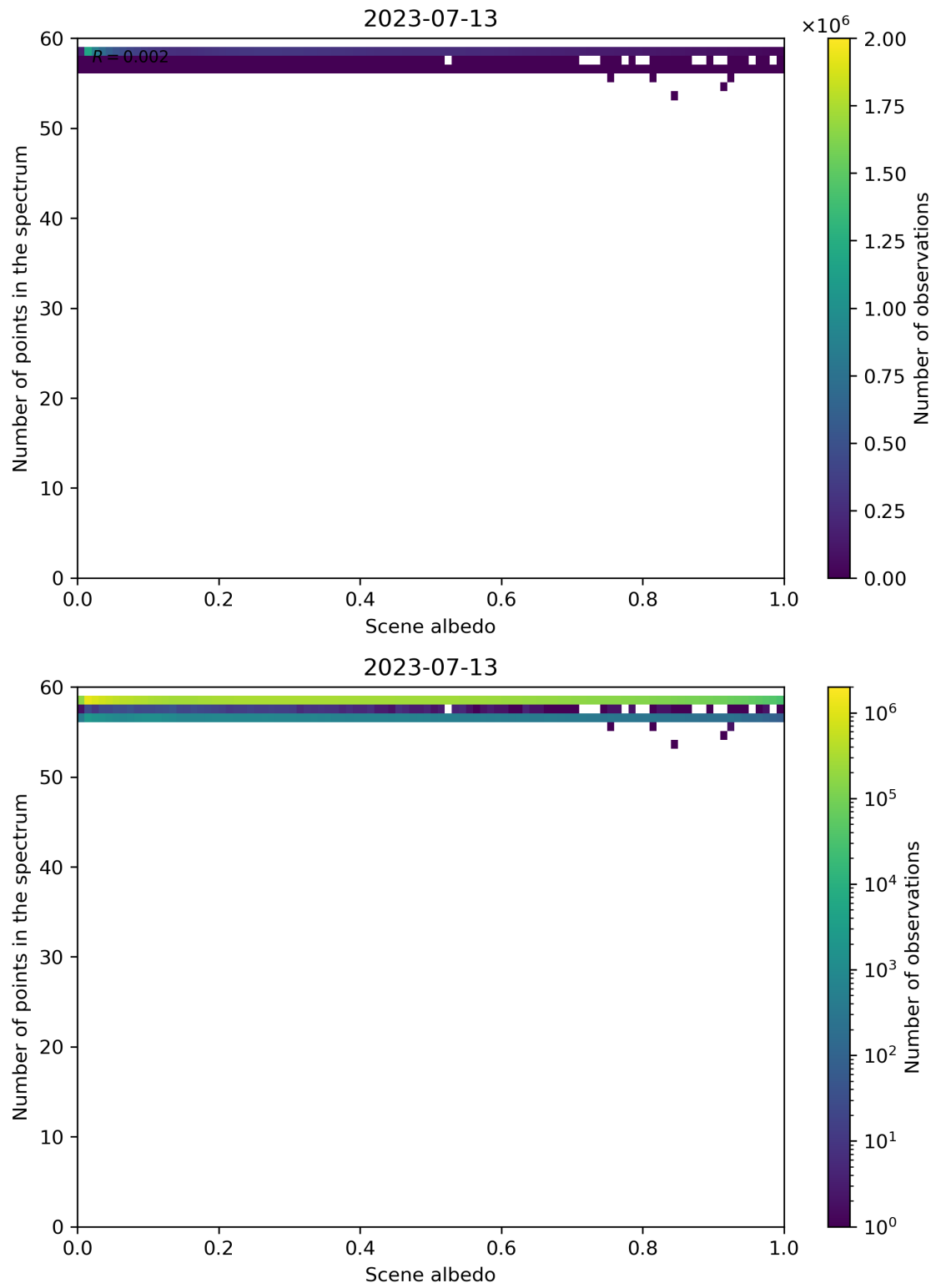
Figure 116: Scatter density plot of “Scene albedo” against “Number of points in the spectrum” for 2023-07-13 to 2023-07-14.
