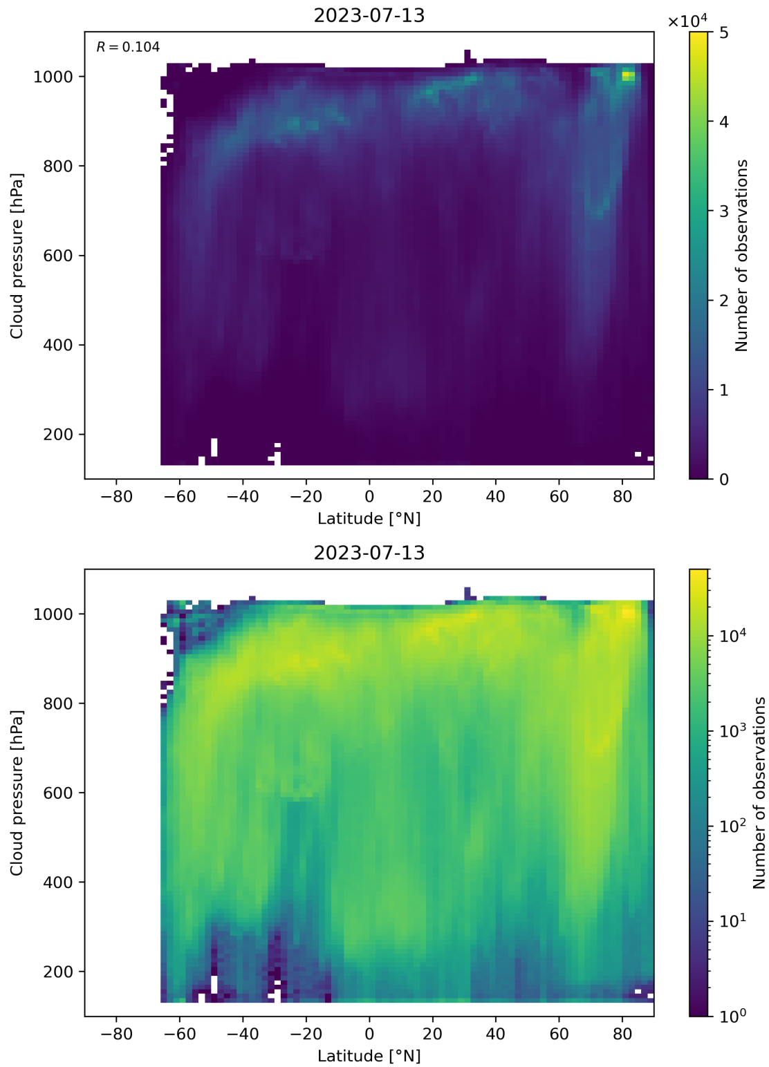
Figure 100: Scatter density plot of “Latitude” against “Cloud pressure” for 2023-07-13 to 2023-07-14.
