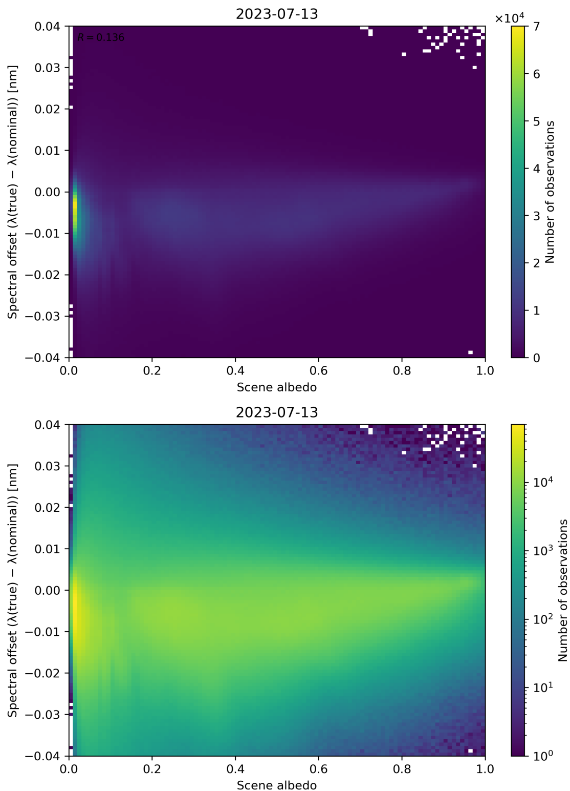
Figure 117: Scatter density plot of “Scene albedo” against “Spectral offset ( \lambda(\text{true}) - \lambda(\text{nominal}) )” for 2023-07-13 to 2023-07-14.
