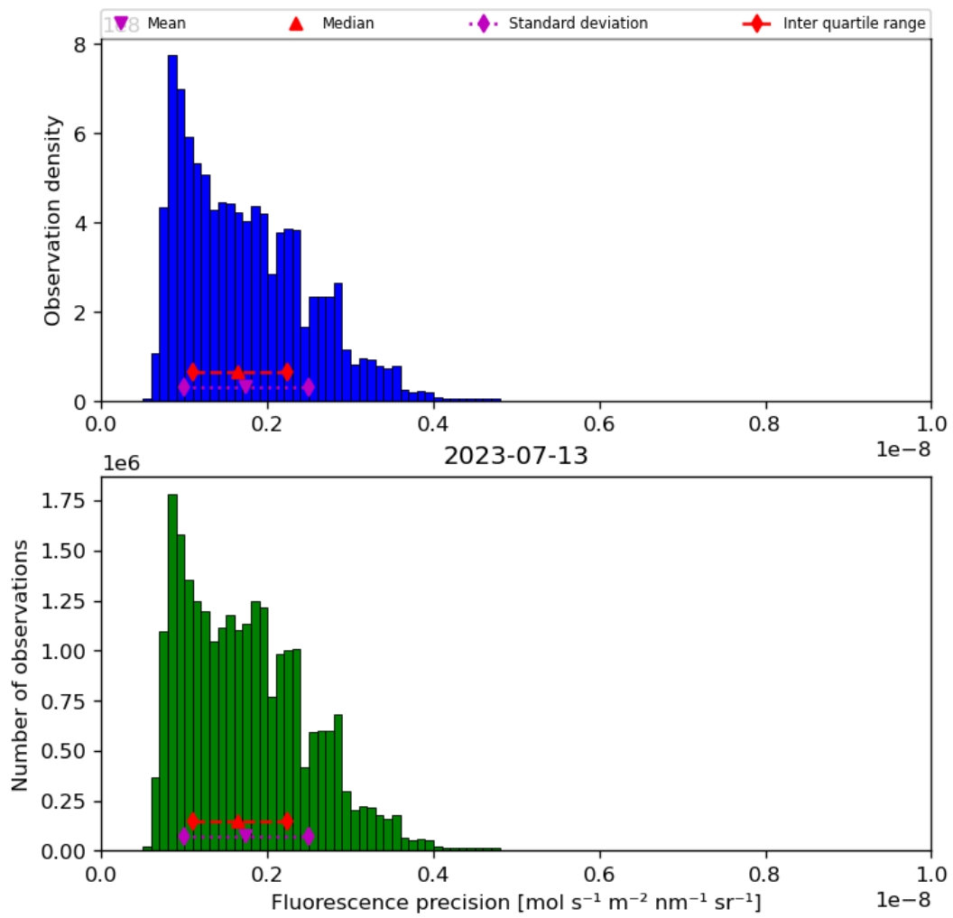
Figure 41: Histogram of “Fluorescence precision” for 2023-07-13 to 2023-07-14
