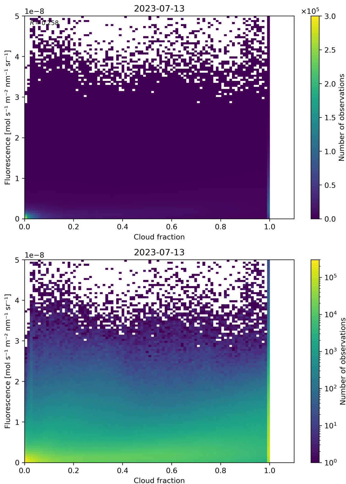
Figure 79: Scatter density plot of “Cloud fraction” against “Fluorescence” for 2023-07-13 to 2023-07-14.
