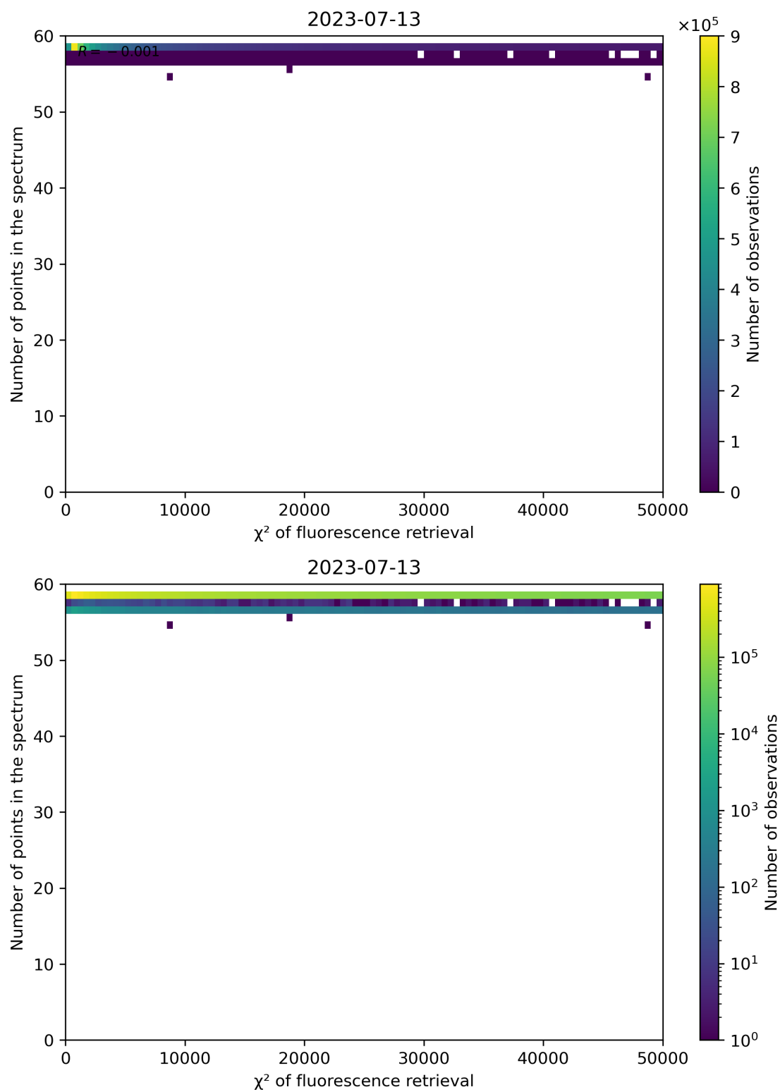
Figure 71: Scatter density plot of " \chi^2 of fluorescence retrieval" against "Number of points in the spectrum" for 2023-07-13 to 2023-07-14.
