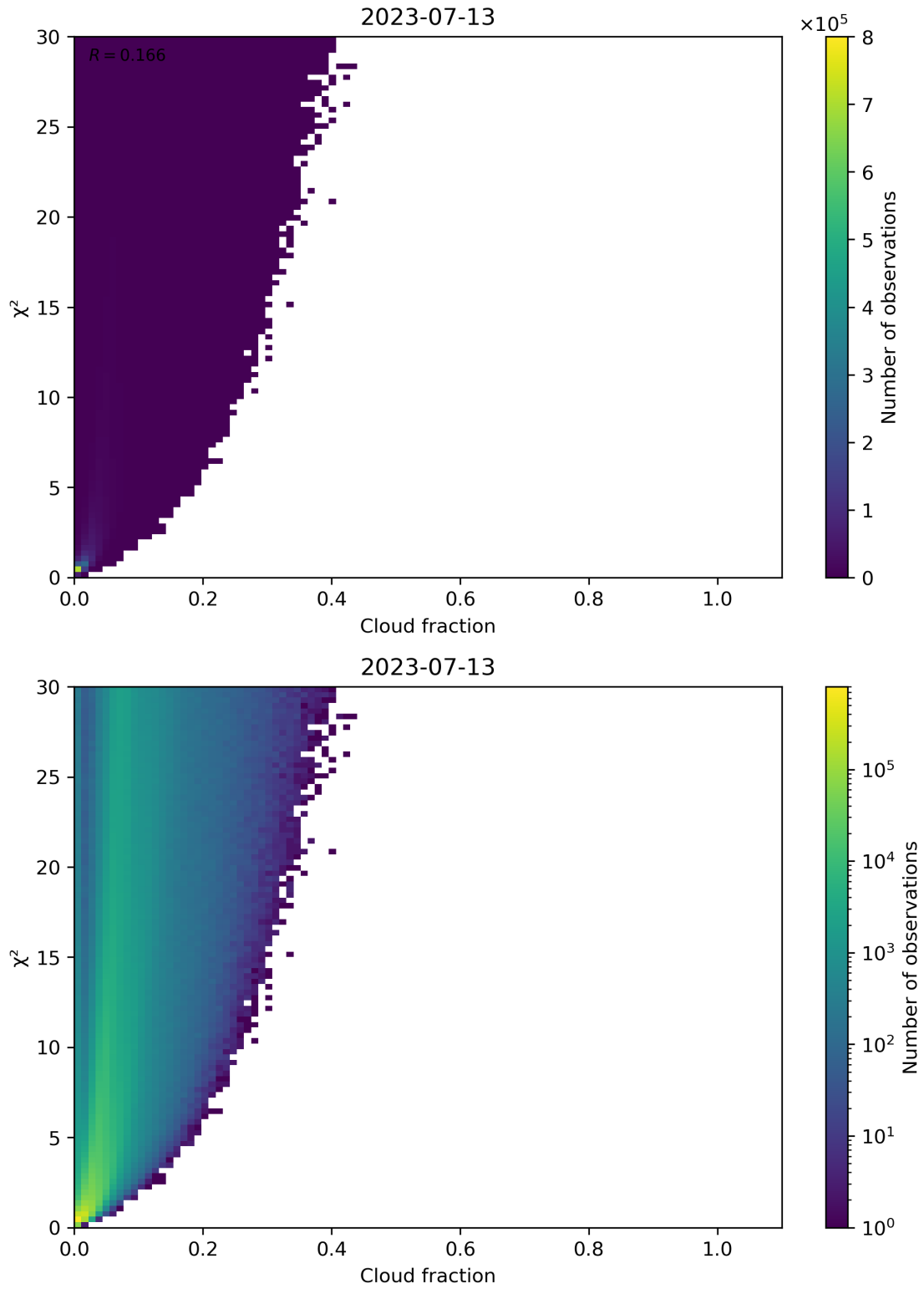
Figure 77: Scatter density plot of “Cloud fraction” against “ \chi^2 ” for 2023-07-13 to 2023-07-14.
