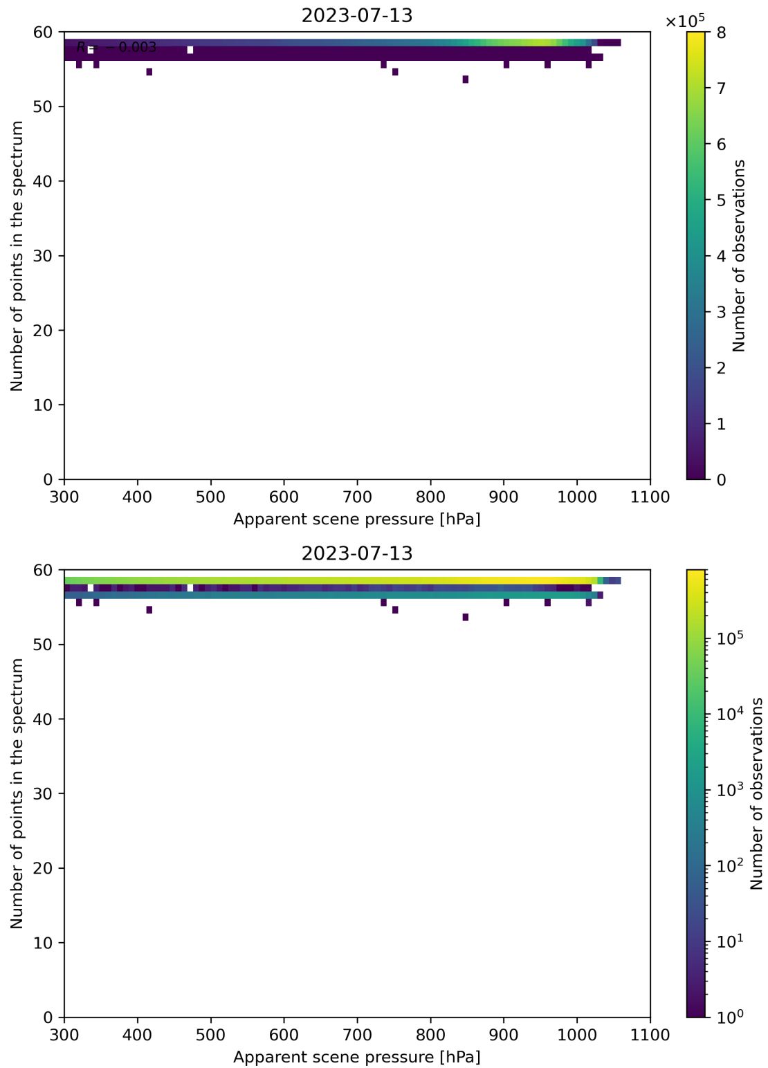
Figure 67: Scatter density plot of “Apparent scene pressure” against “Number of points in the spectrum” for 2023-07-13 to 2023-07-14.
