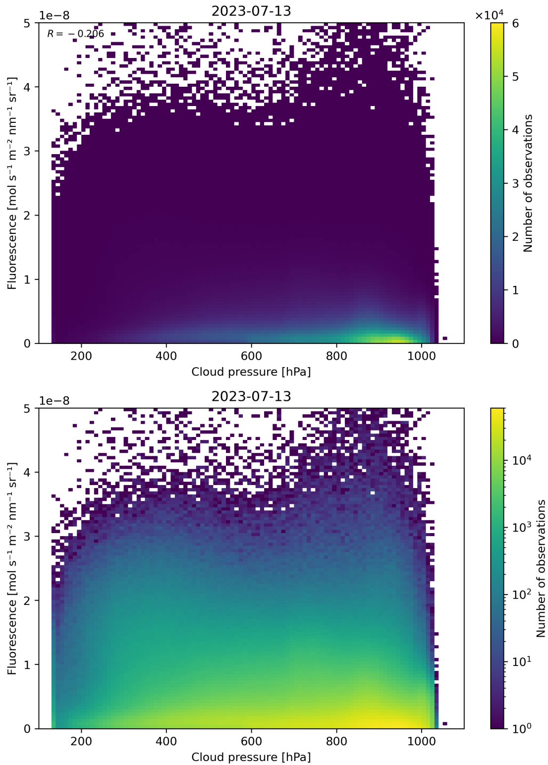
Figure 88: Scatter density plot of “Cloud pressure” against “Fluorescence” for 2023-07-13 to 2023-07-14.
