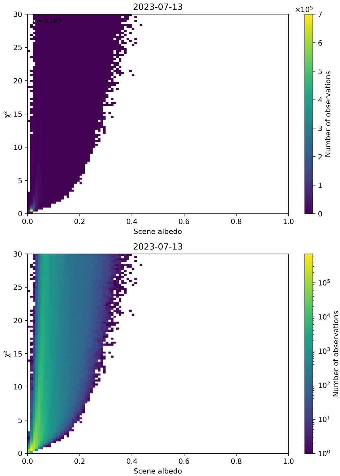
Figure 112: Scatter density plot of “Scene albedo” against “ \chi^2 ” for 2023-07-13 to 2023-07-14.
