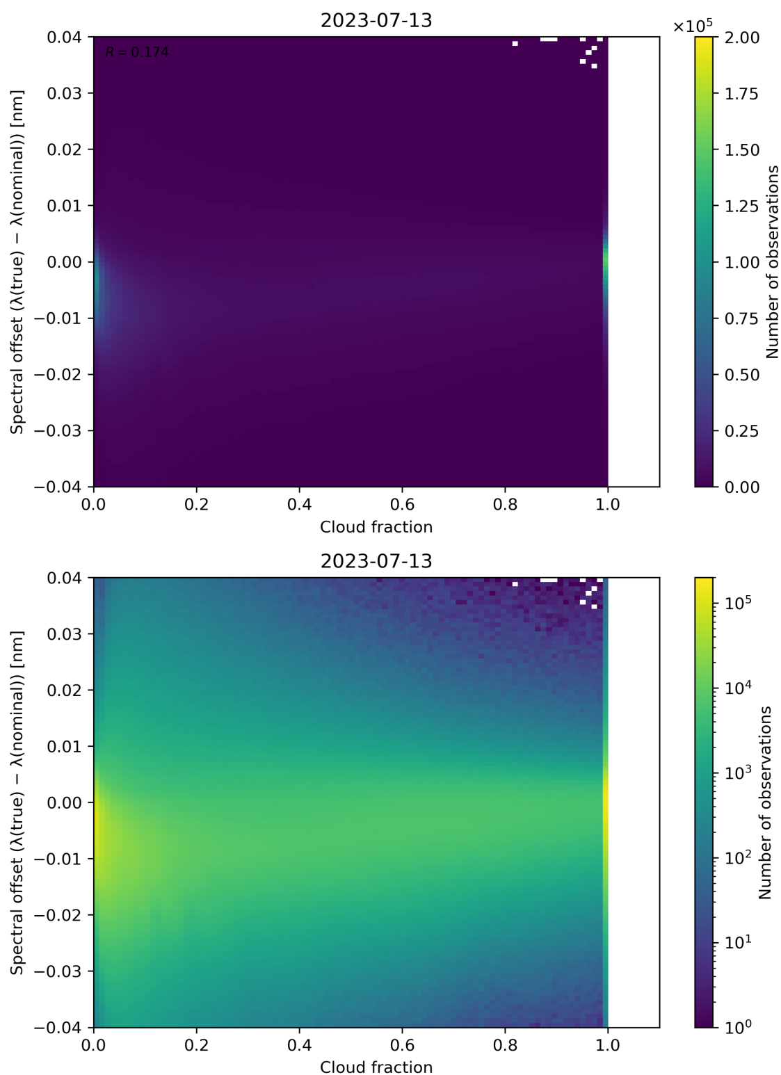
Figure 83: Scatter density plot of “Cloud fraction” against “Spectral offset ( \lambda(\text{true}) - \lambda(\text{nominal}) )” for 2023-07-13 to 2023-07-14.
