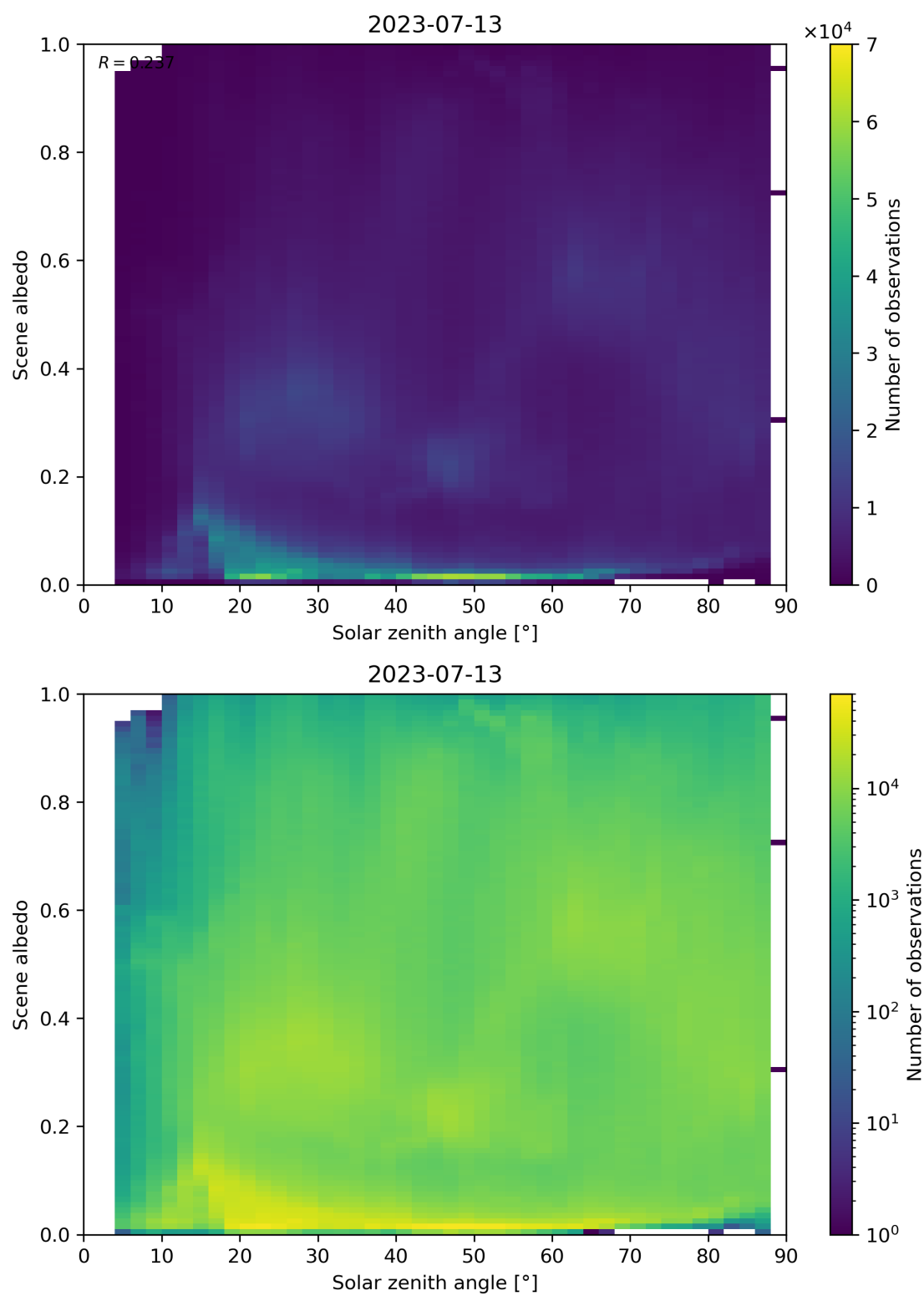
Figure 127: Scatter density plot of “Solar zenith angle” against “Scene albedo” for 2023-07-13 to 2023-07-14.
