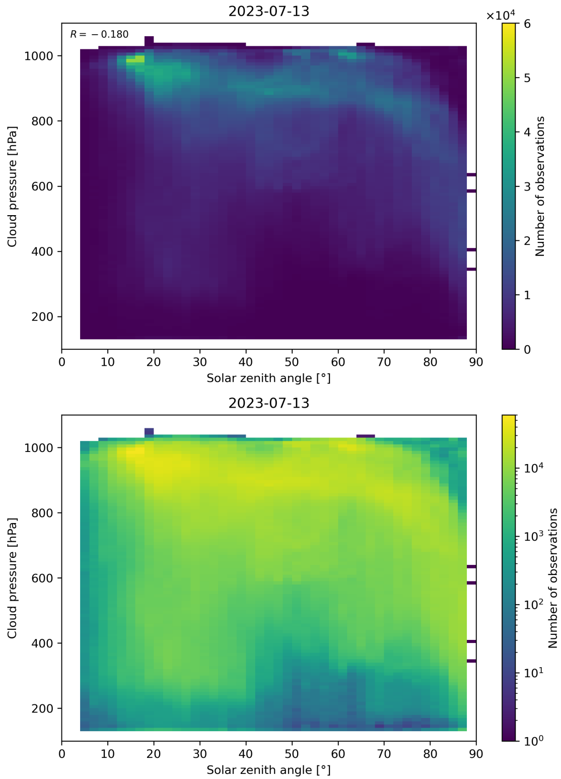
Figure 122: Scatter density plot of “Solar zenith angle” against “Cloud pressure” for 2023-07-13 to 2023-07-14.
