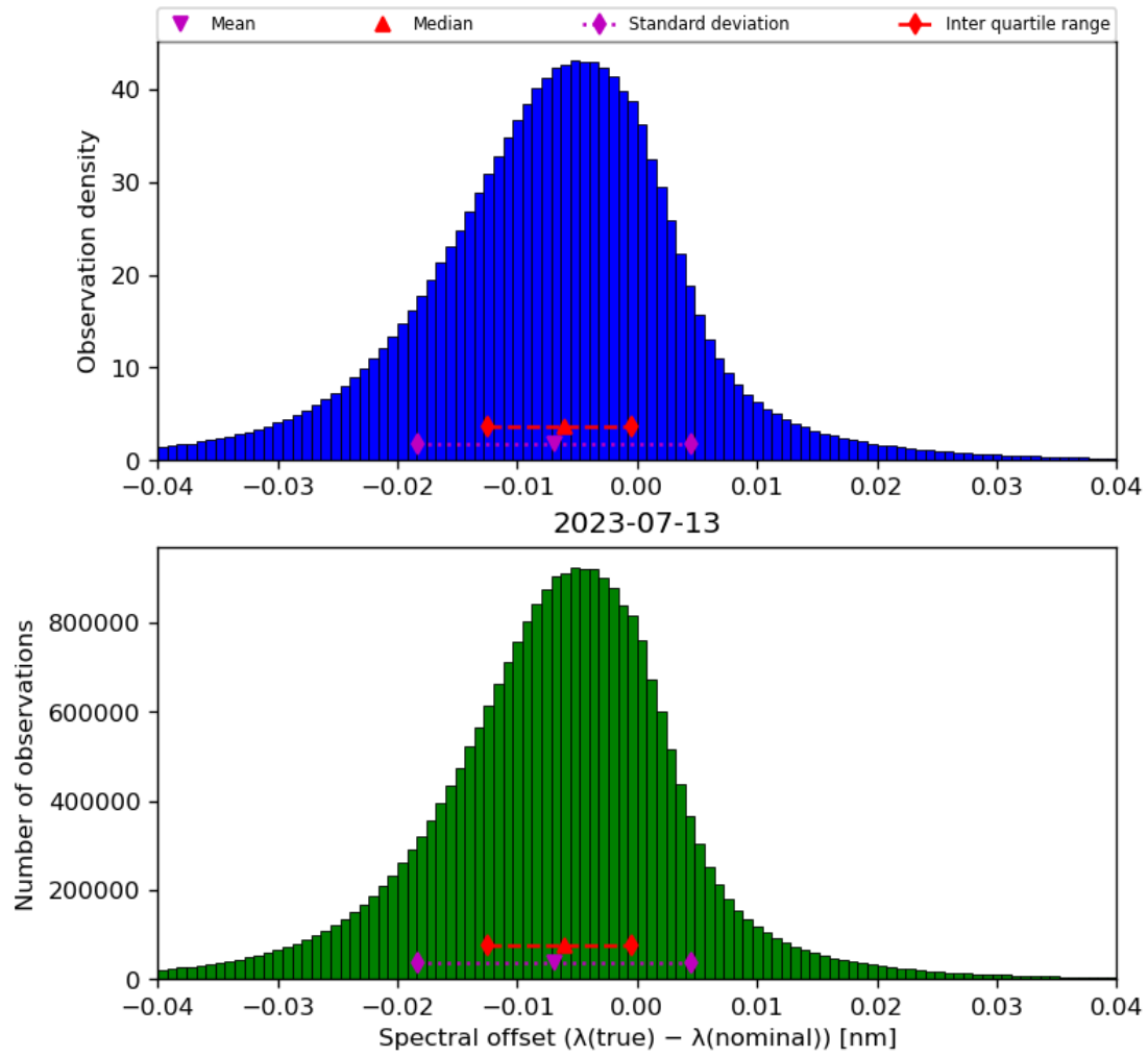
Figure 45: Histogram of “Spectral offset ( \lambda(\text{true}) - \lambda(\text{nominal}) )” for 2023-07-13 to 2023-07-14
