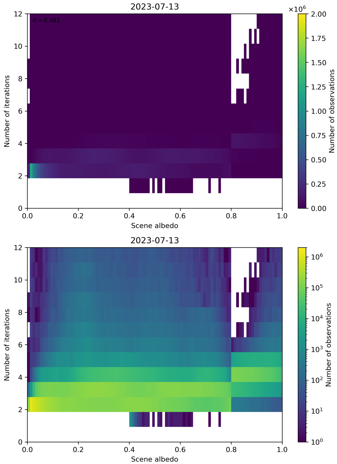
Figure 115: Scatter density plot of “Scene albedo” against “Number of iterations” for 2023-07-13 to 2023-07-14.
