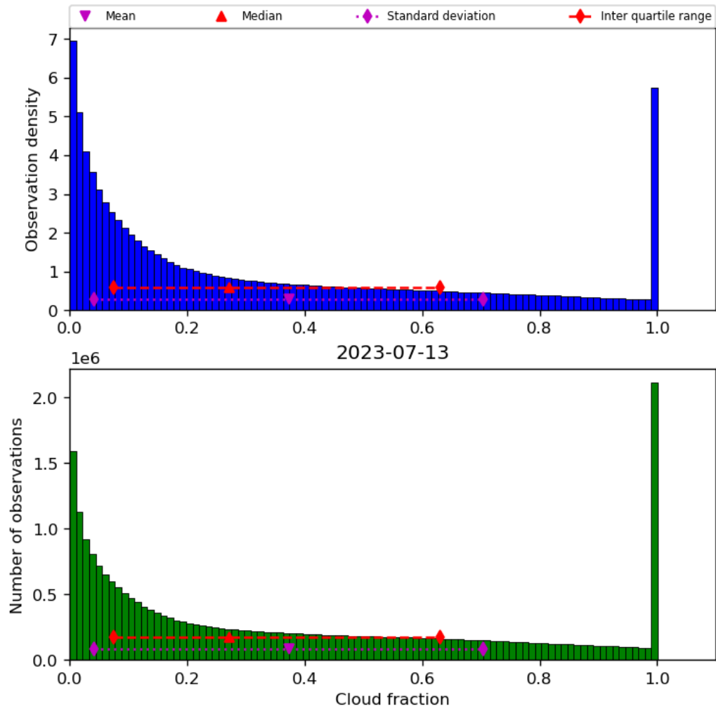
Figure 32: Histogram of “Cloud fraction” for 2023-07-13 to 2023-07-14
