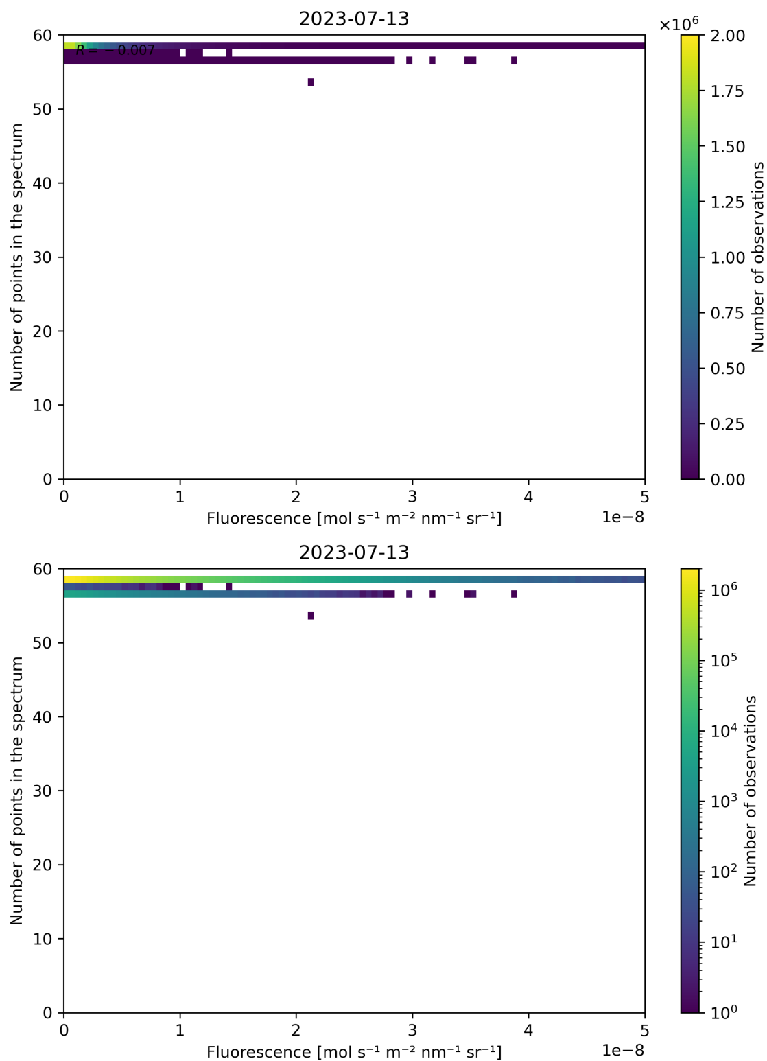
Figure 94: Scatter density plot of “Fluorescence” against “Number of points in the spectrum” for 2023-07-13 to 2023-07-14.
