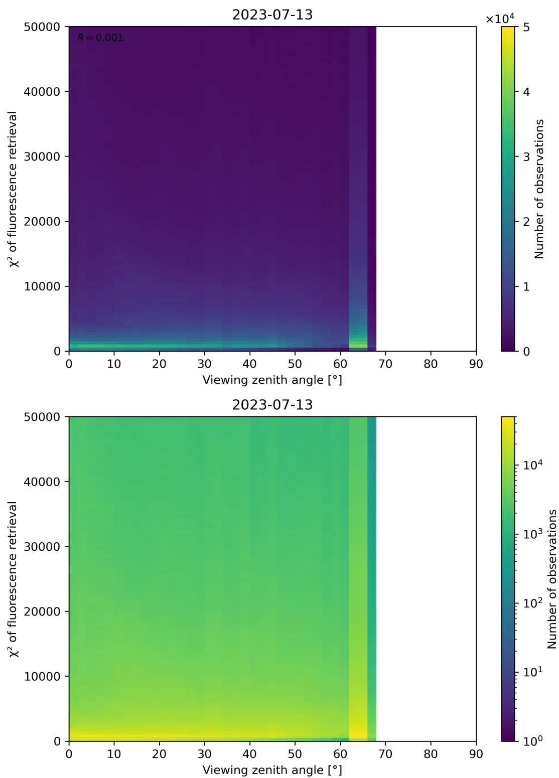
Figure 131: Scatter density plot of “Viewing zenith angle” against “ \chi^2 of fluorescence retrieval” for 2023-07-13 to 2023-07-14.
