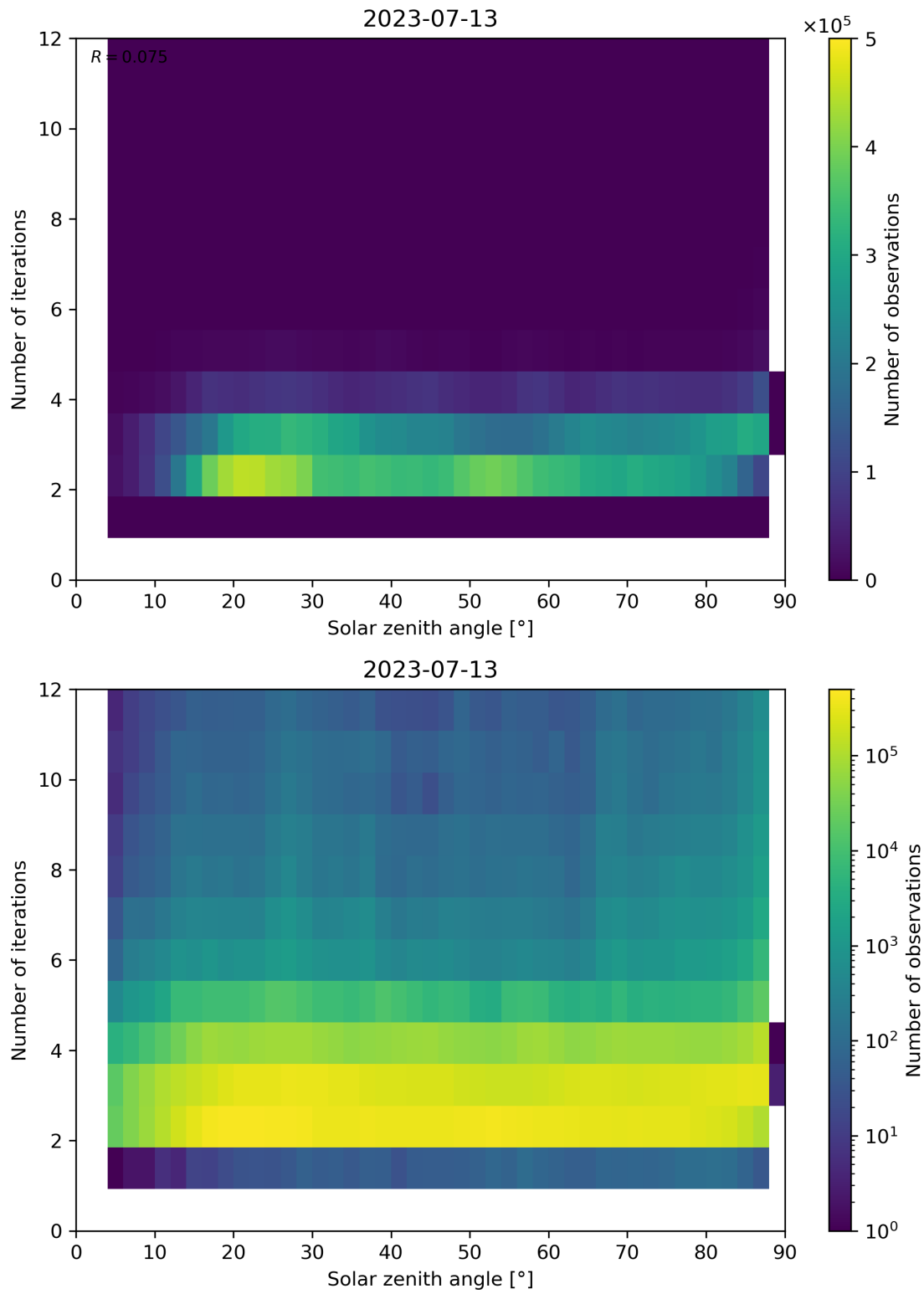
Figure 125: Scatter density plot of “Solar zenith angle” against “Number of iterations” for 2023-07-13 to 2023-07-14.
