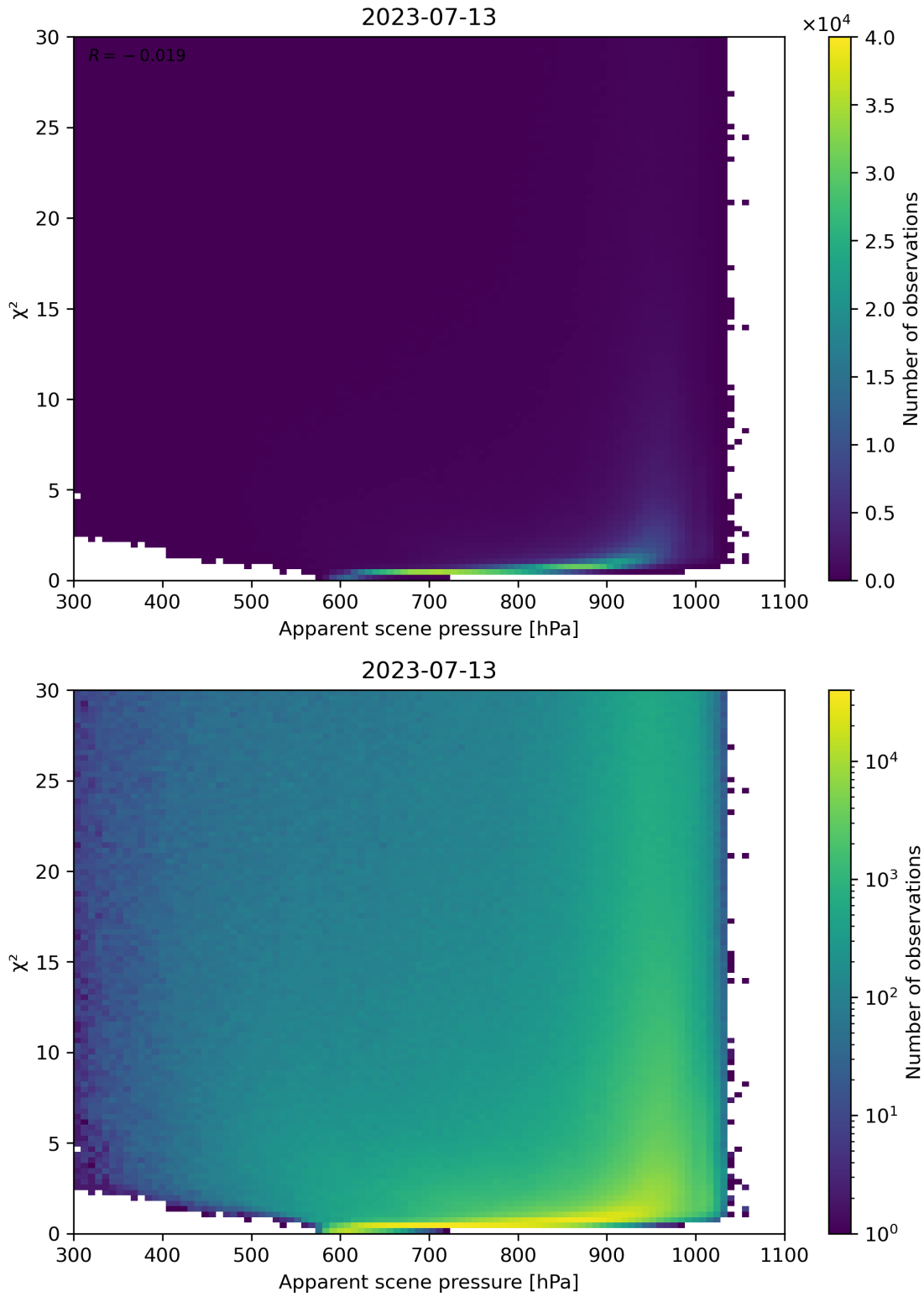
Figure 63: Scatter density plot of “Apparent scene pressure” against “ \chi^2 ” for 2023-07-13 to 2023-07-14.
