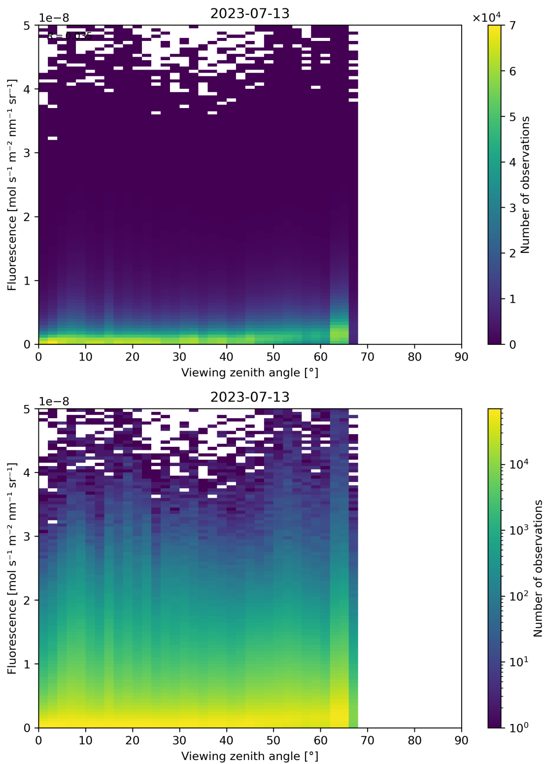
Figure 134: Scatter density plot of “Viewing zenith angle” against “Fluorescence” for 2023-07-13 to 2023-07-14.
