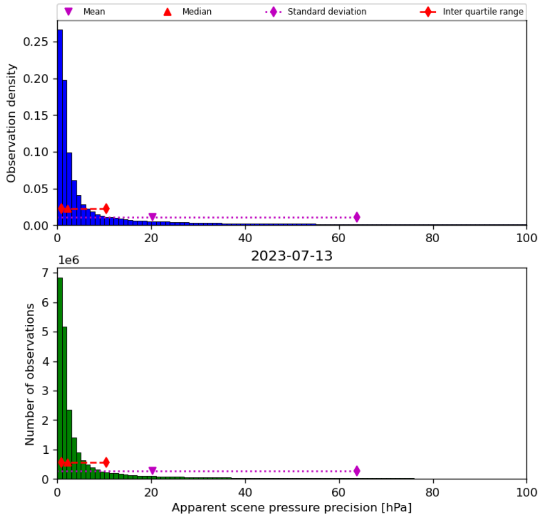
Figure 37: Histogram of “Apparent scene pressure precision” for 2023-07-13 to 2023-07-14
