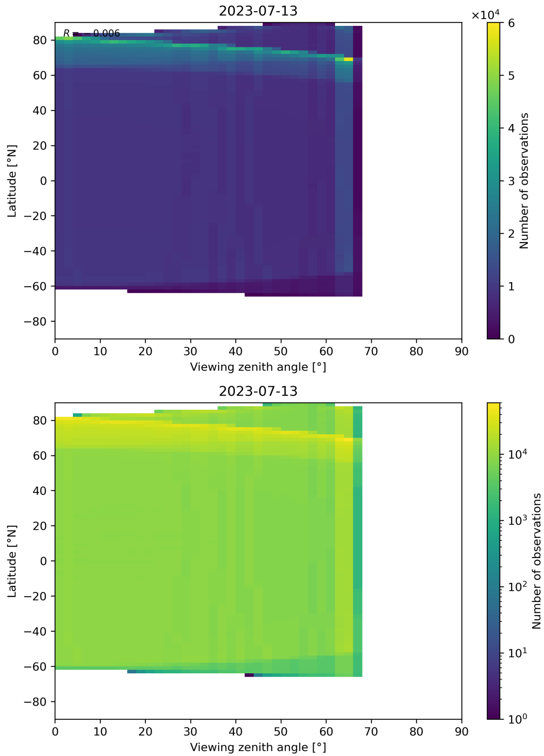
Figure 135: Scatter density plot of “Viewing zenith angle” against “Latitude” for 2023-07-13 to 2023-07-14.
