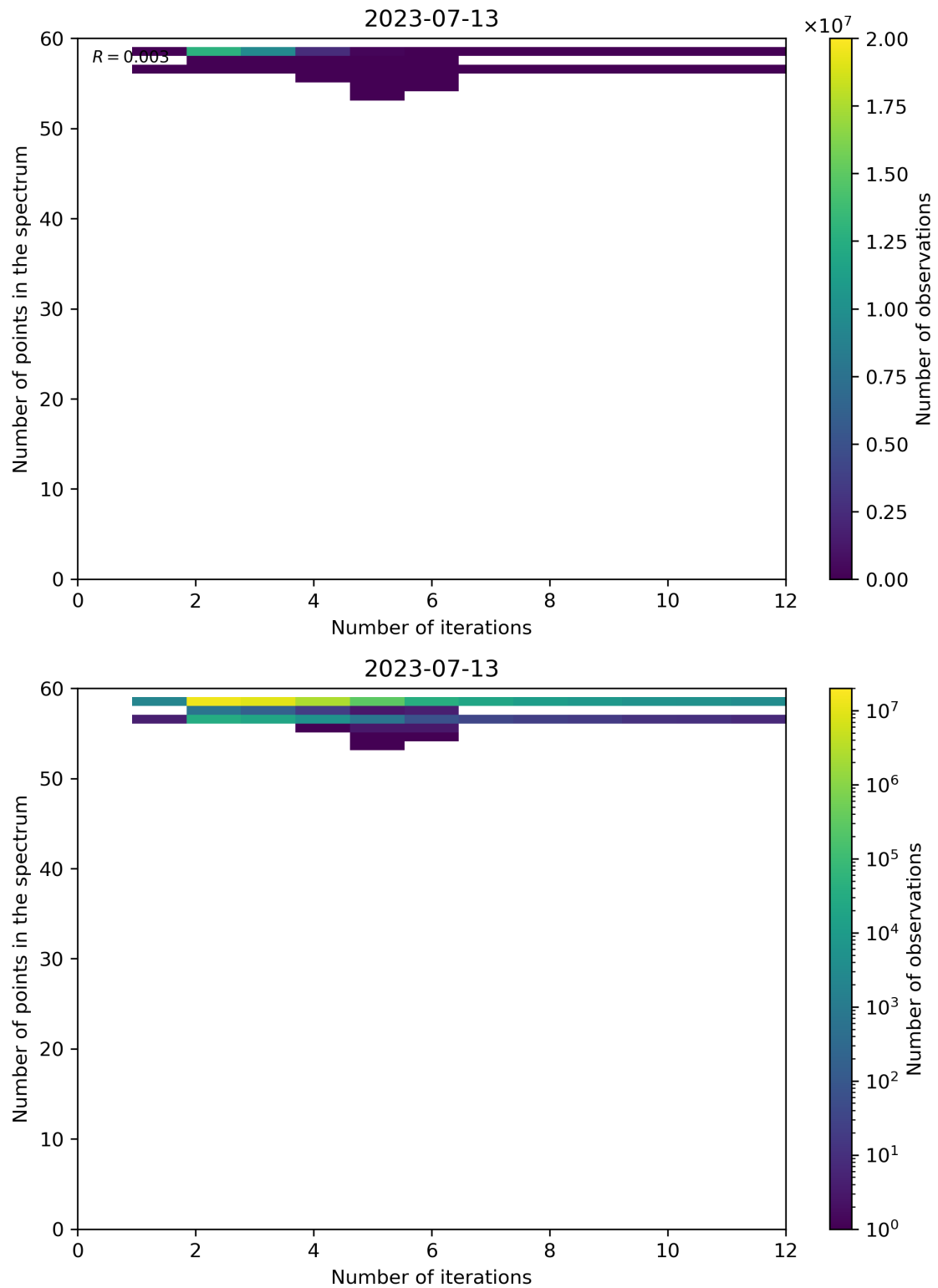
Figure 108: Scatter density plot of “Number of iterations” against “Number of points in the spectrum” for 2023-07-13 to 2023-07-14.
