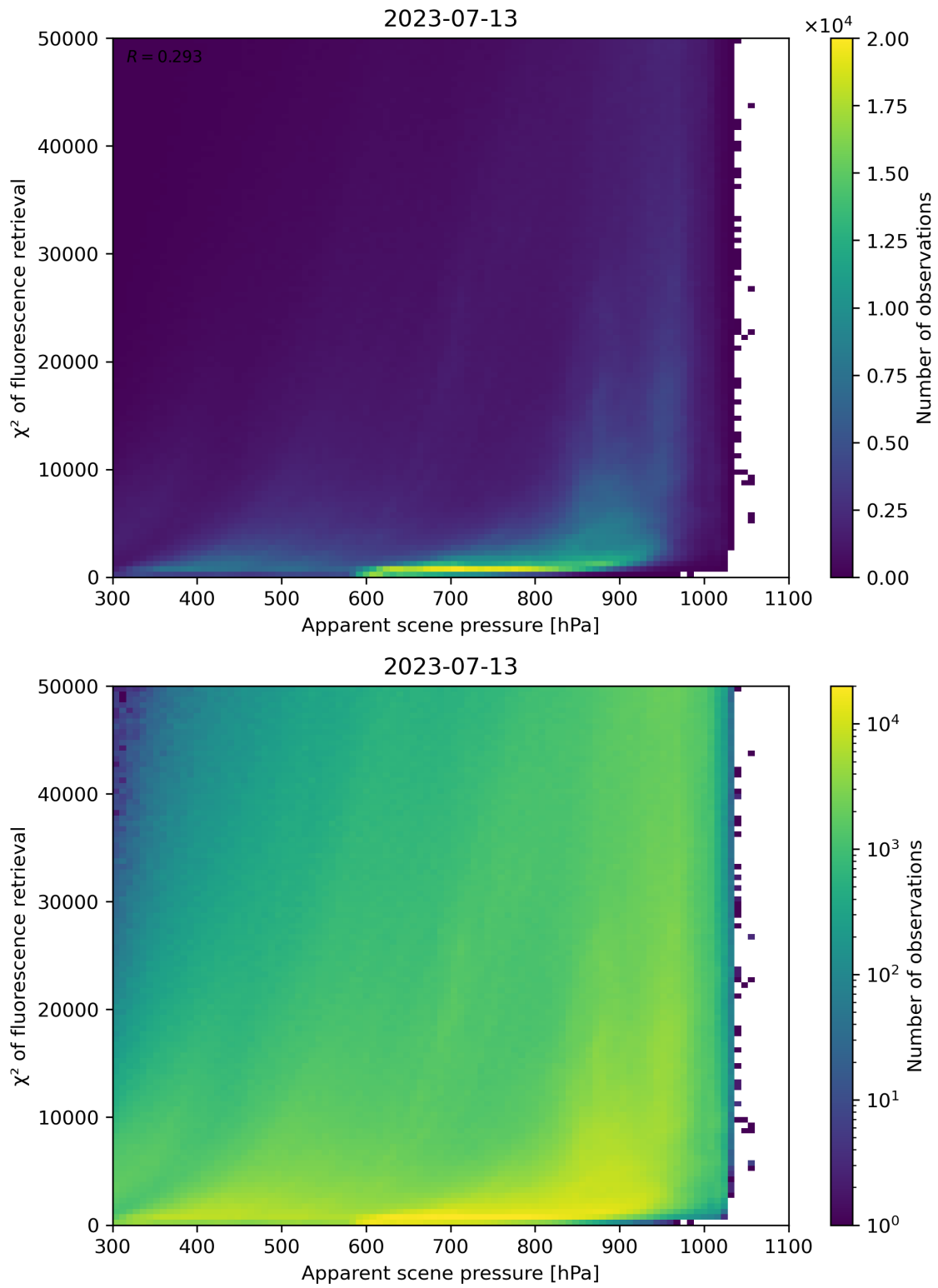
Figure 64: Scatter density plot of “Apparent scene pressure” against “ \chi^2 of fluorescence retrieval” for 2023-07-13 to 2023-07-14.
