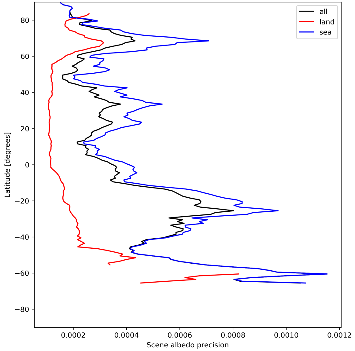
Figure 18: Zonal average of “Scene albedo precision” for 2023-07-13 to 2023-07-14.
