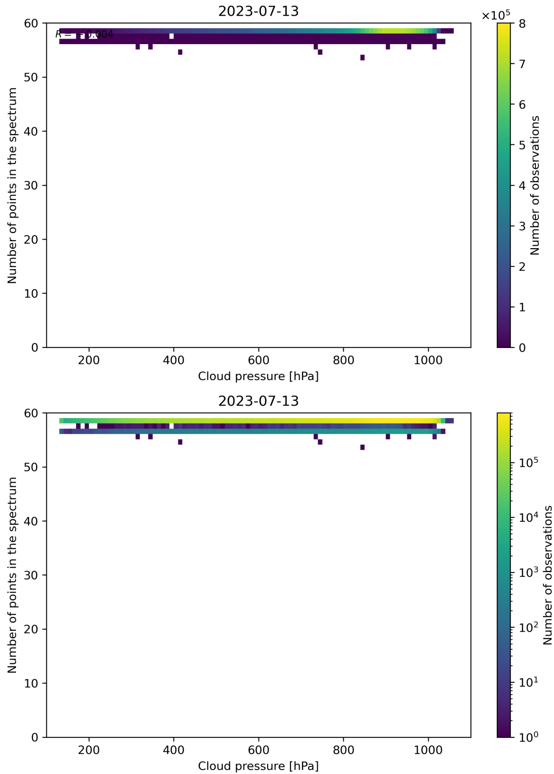
Figure 90: Scatter density plot of “Cloud pressure” against “Number of points in the spectrum” for 2023-07-13 to 2023-07-14.
