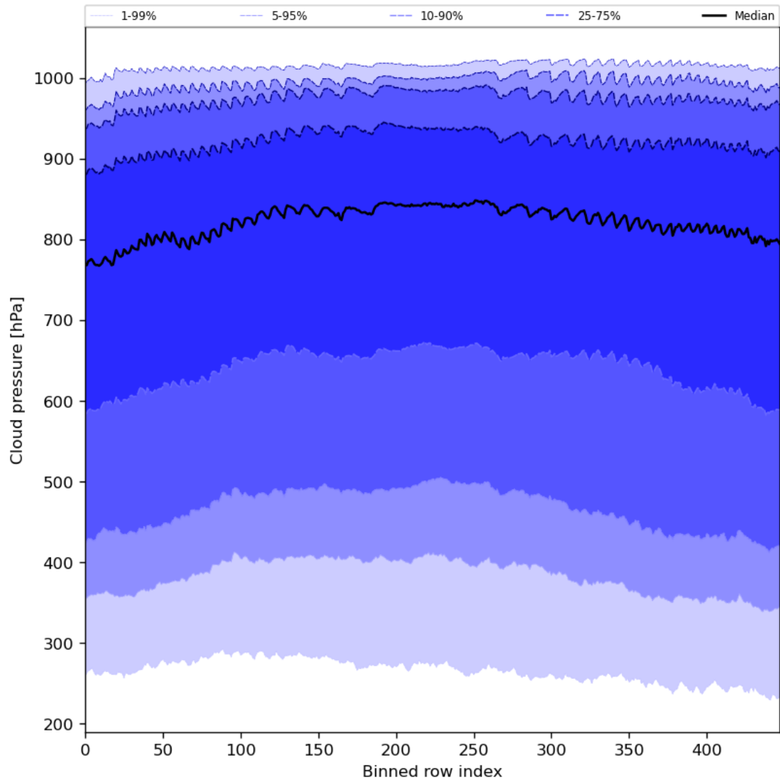
Figure 47: Along track statistics of “Cloud pressure” for 2023-07-13 to 2023-07-14
