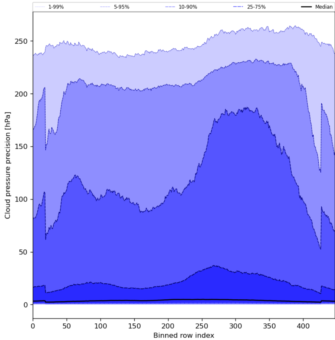
Figure 48: Along track statistics of “Cloud pressure precision” for 2023-07-13 to 2023-07-14
