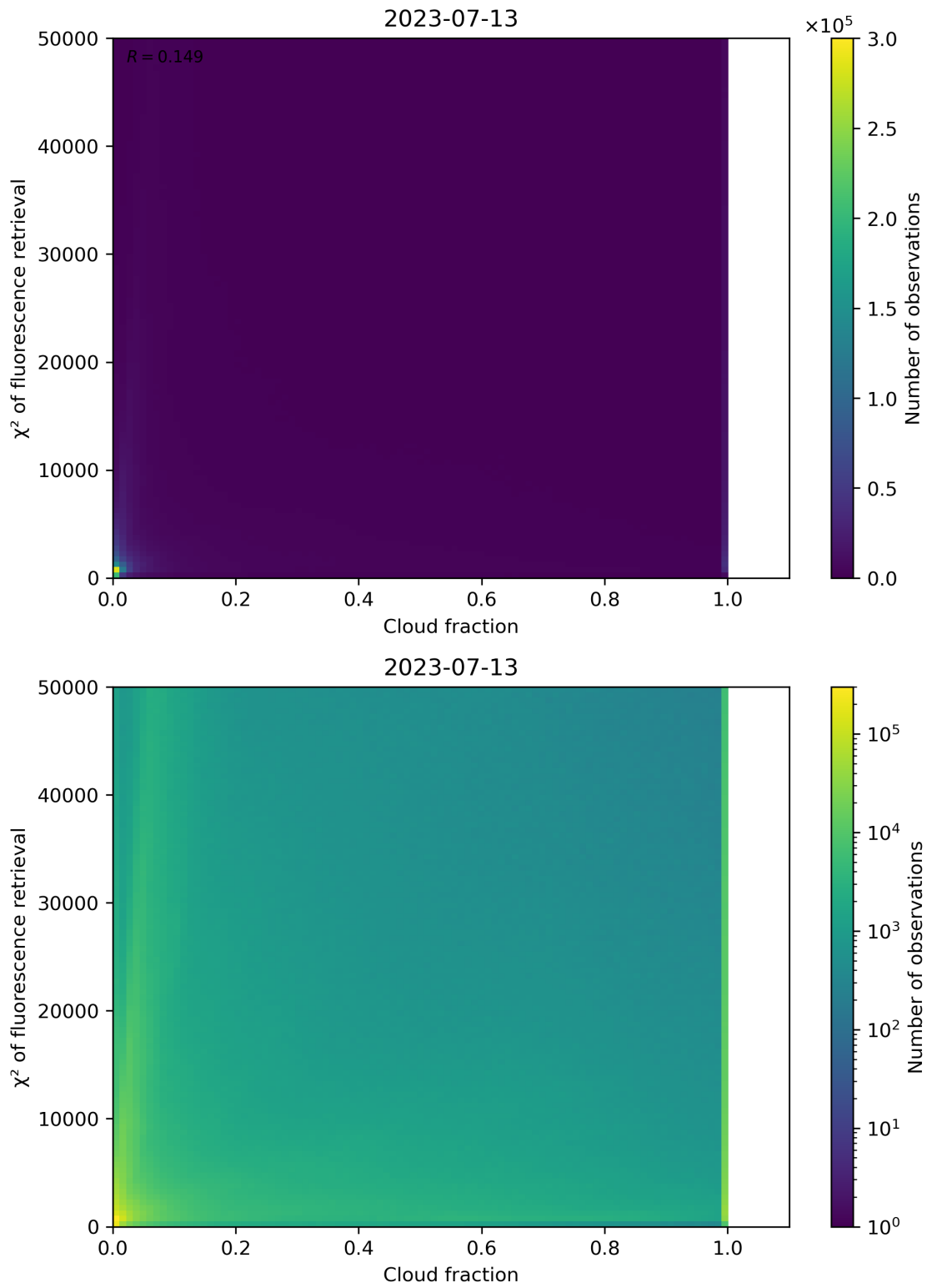
Figure 78: Scatter density plot of “Cloud fraction” against “ \chi^2 of fluorescence retrieval” for 2023-07-13 to 2023-07-14.
