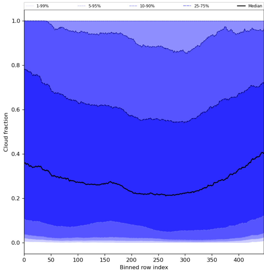
Figure 49: Along track statistics of “Cloud fraction” for 2023-07-13 to 2023-07-14
