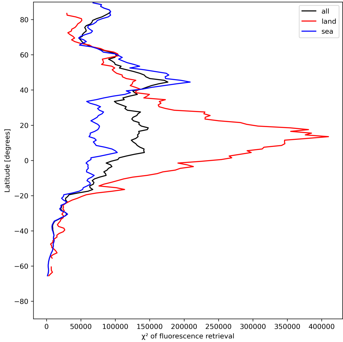
Figure 25: Zonal average of “ \chi^2 of fluorescence retrieval” for 2023-07-13 to 2023-07-14.
