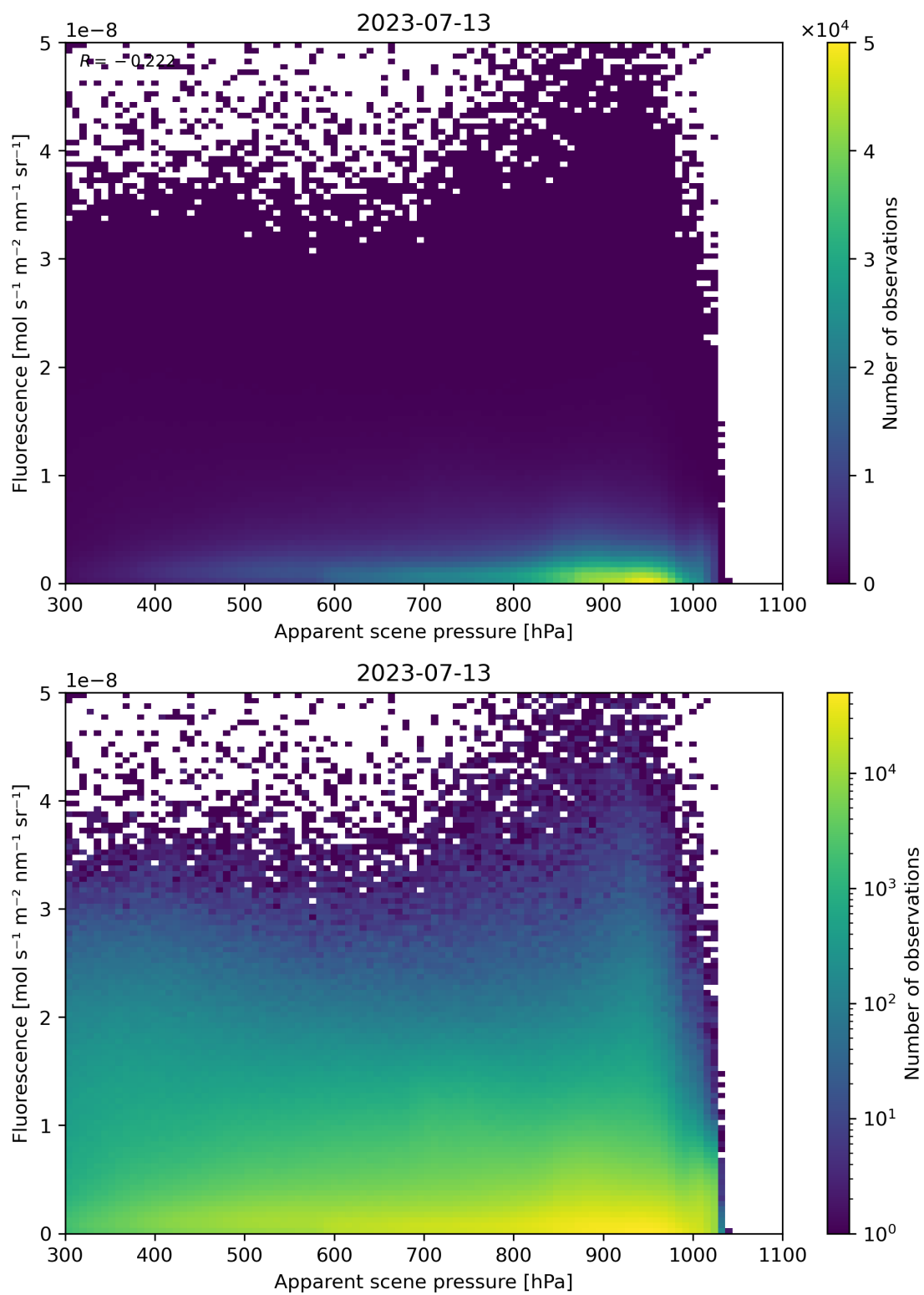
Figure 65: Scatter density plot of “Apparent scene pressure” against “Fluorescence” for 2023-07-13 to 2023-07-14.
