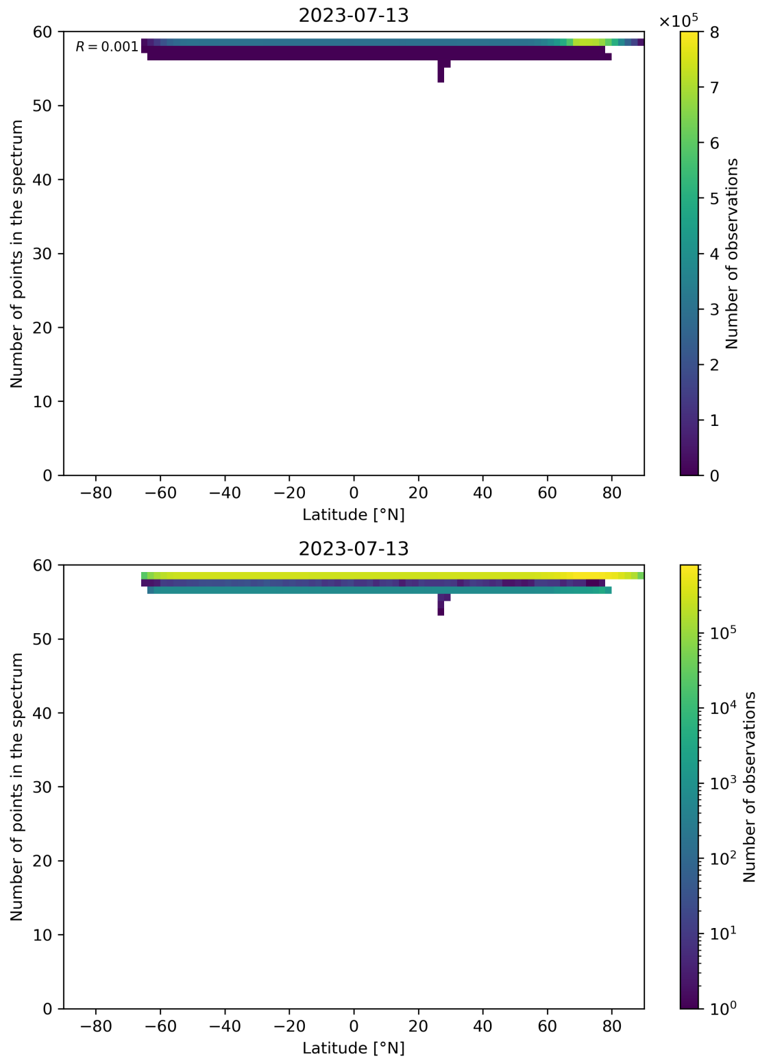
Figure 103: Scatter density plot of “Latitude” against “Number of points in the spectrum” for 2023-07-13 to 2023-07-14.
