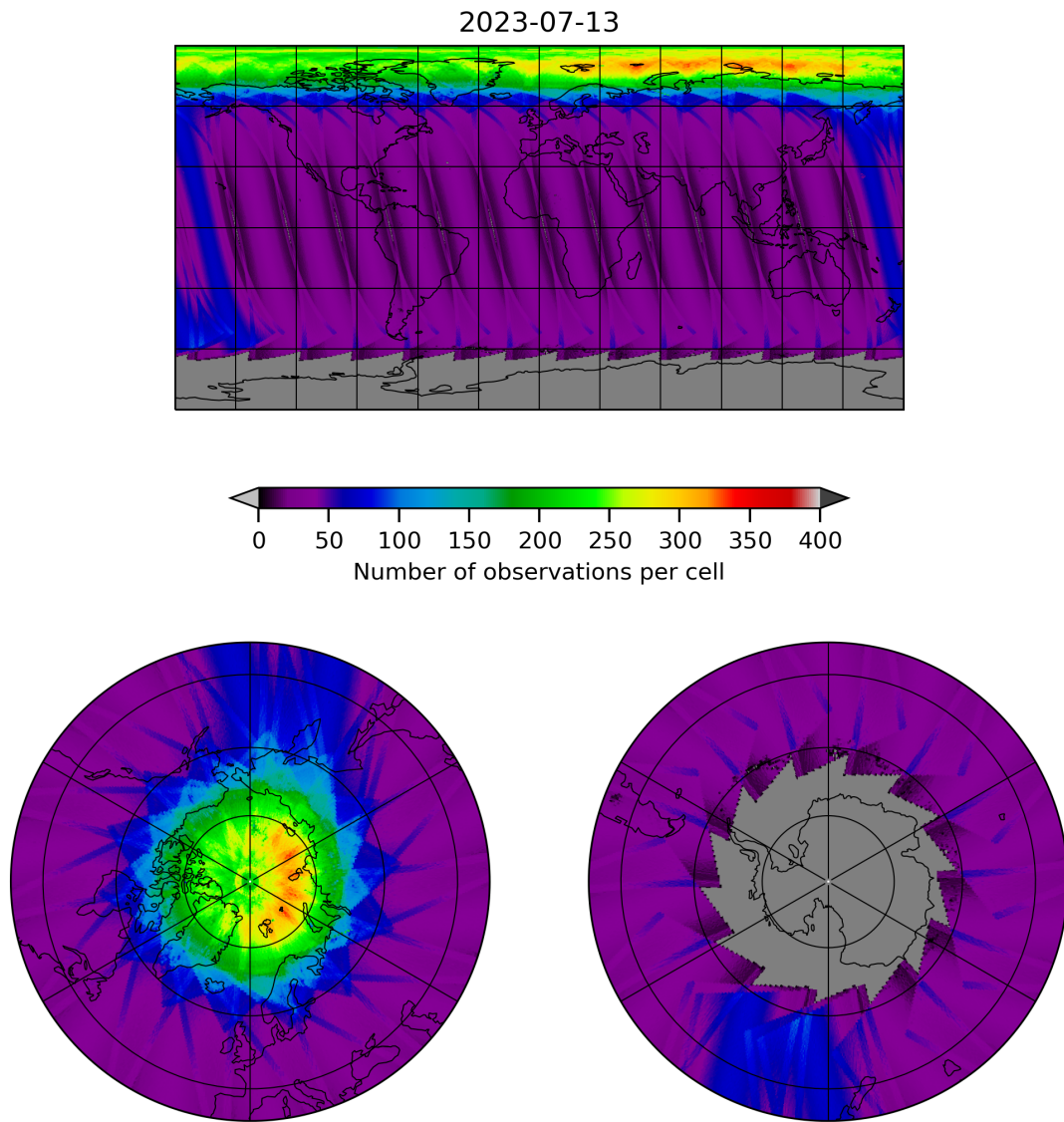
Figure 11: Map of the number of observations for 2023-07-13 to 2023-07-14
