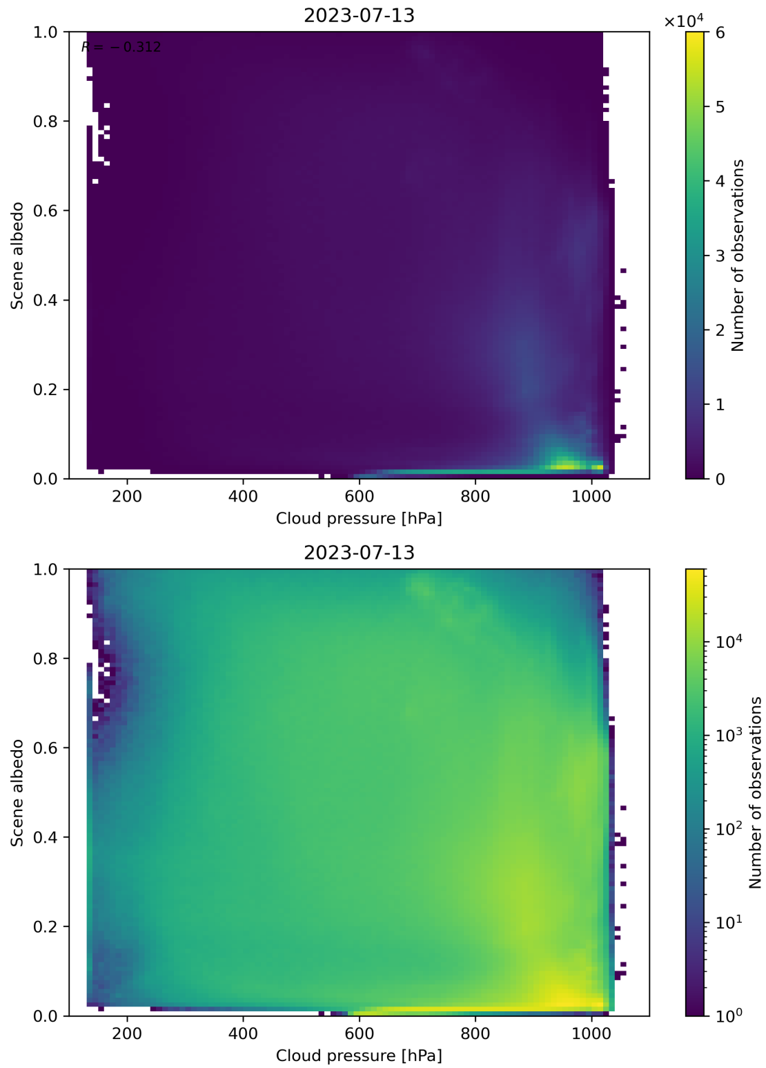
Figure 91: Scatter density plot of “Cloud pressure” against “Scene albedo” for 2023-07-13 to 2023-07-14.
