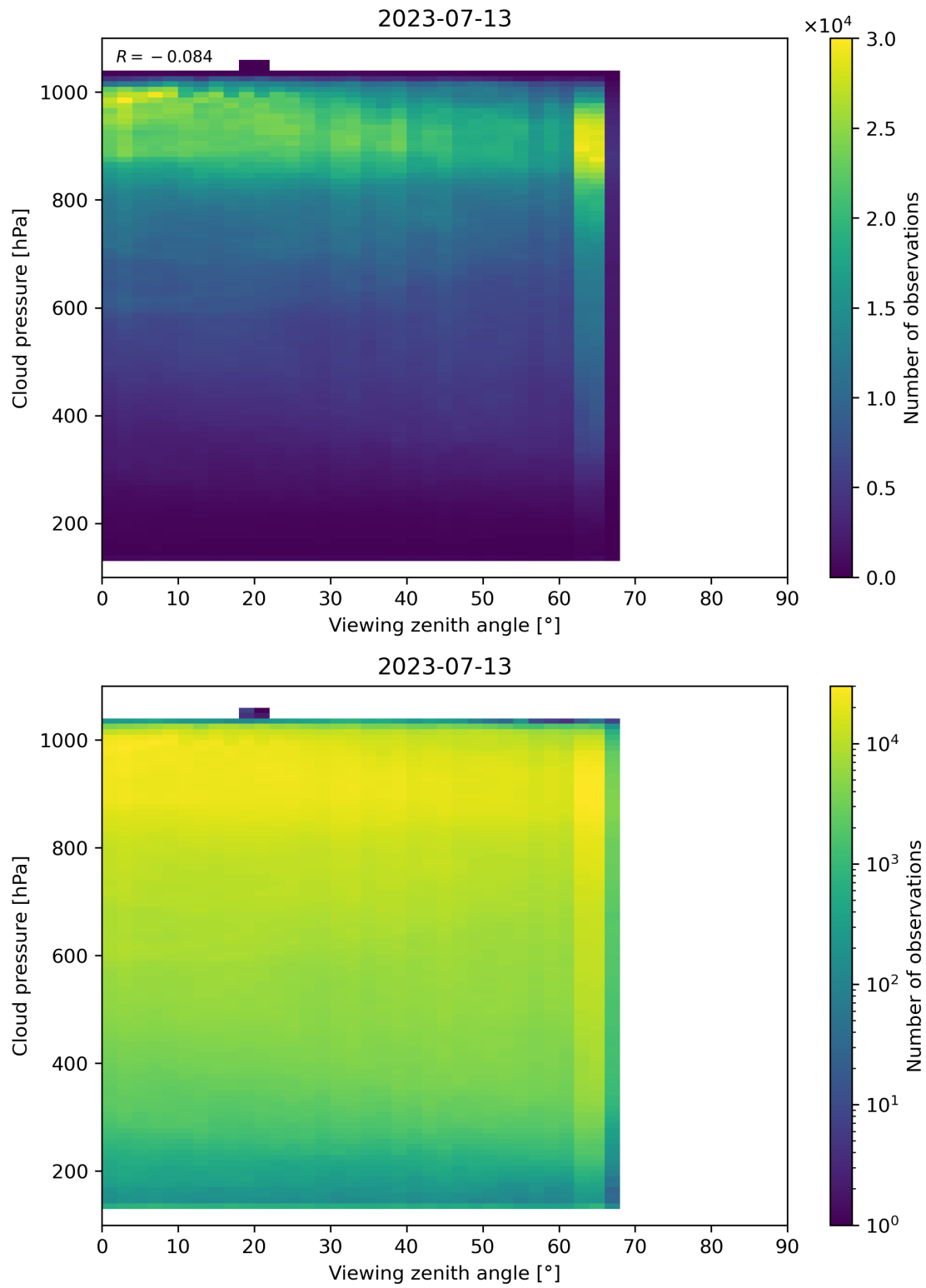
Figure 133: Scatter density plot of “Viewing zenith angle” against “Cloud pressure” for 2023-07-13 to 2023-07-14.
