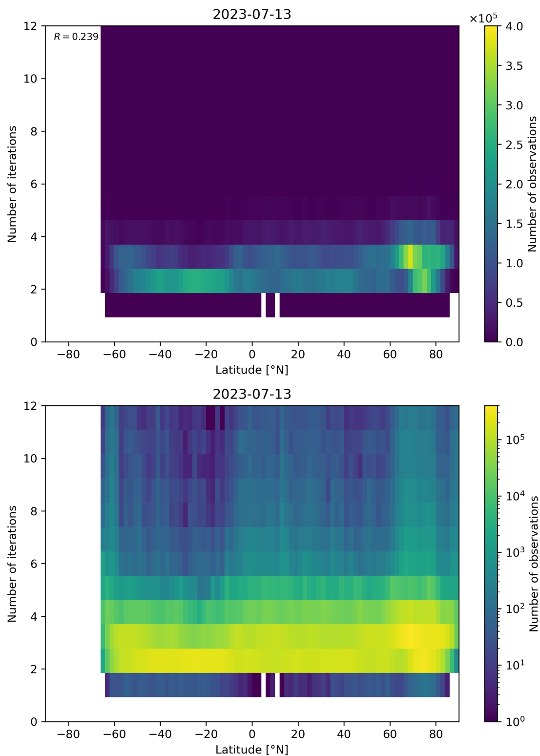
Figure 102: Scatter density plot of “Latitude” against “Number of iterations” for 2023-07-13 to 2023-07-14.
