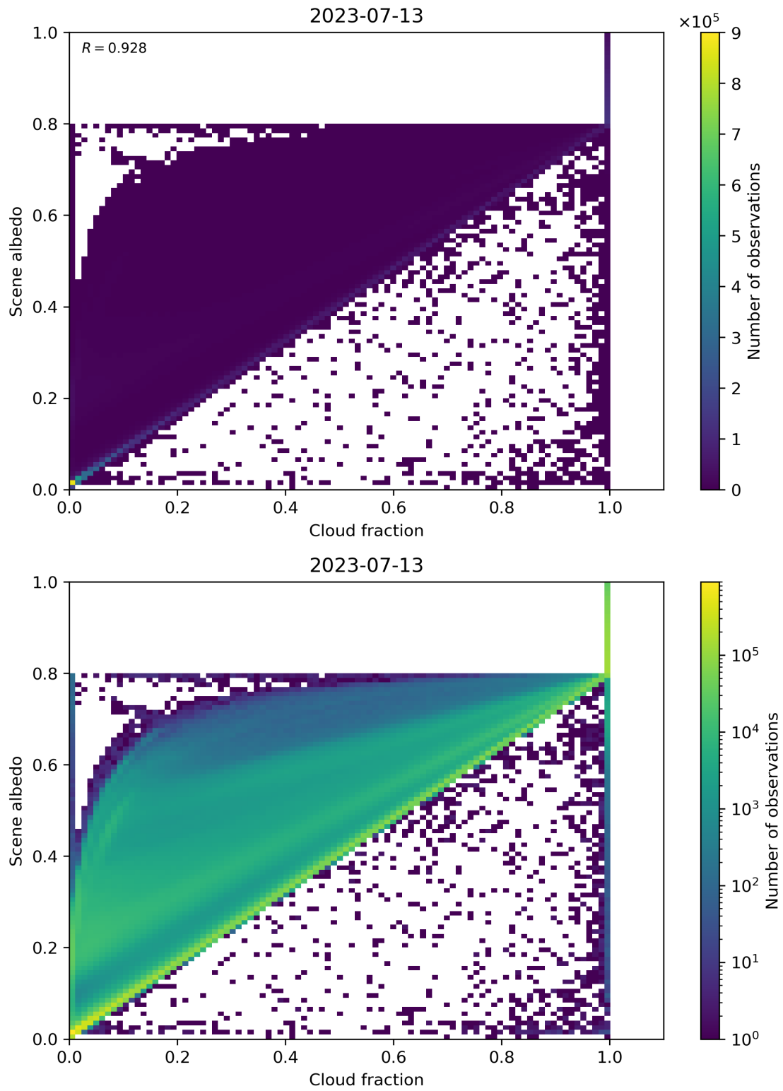
Figure 82: Scatter density plot of “Cloud fraction” against “Scene albedo” for 2023-07-13 to 2023-07-14.
