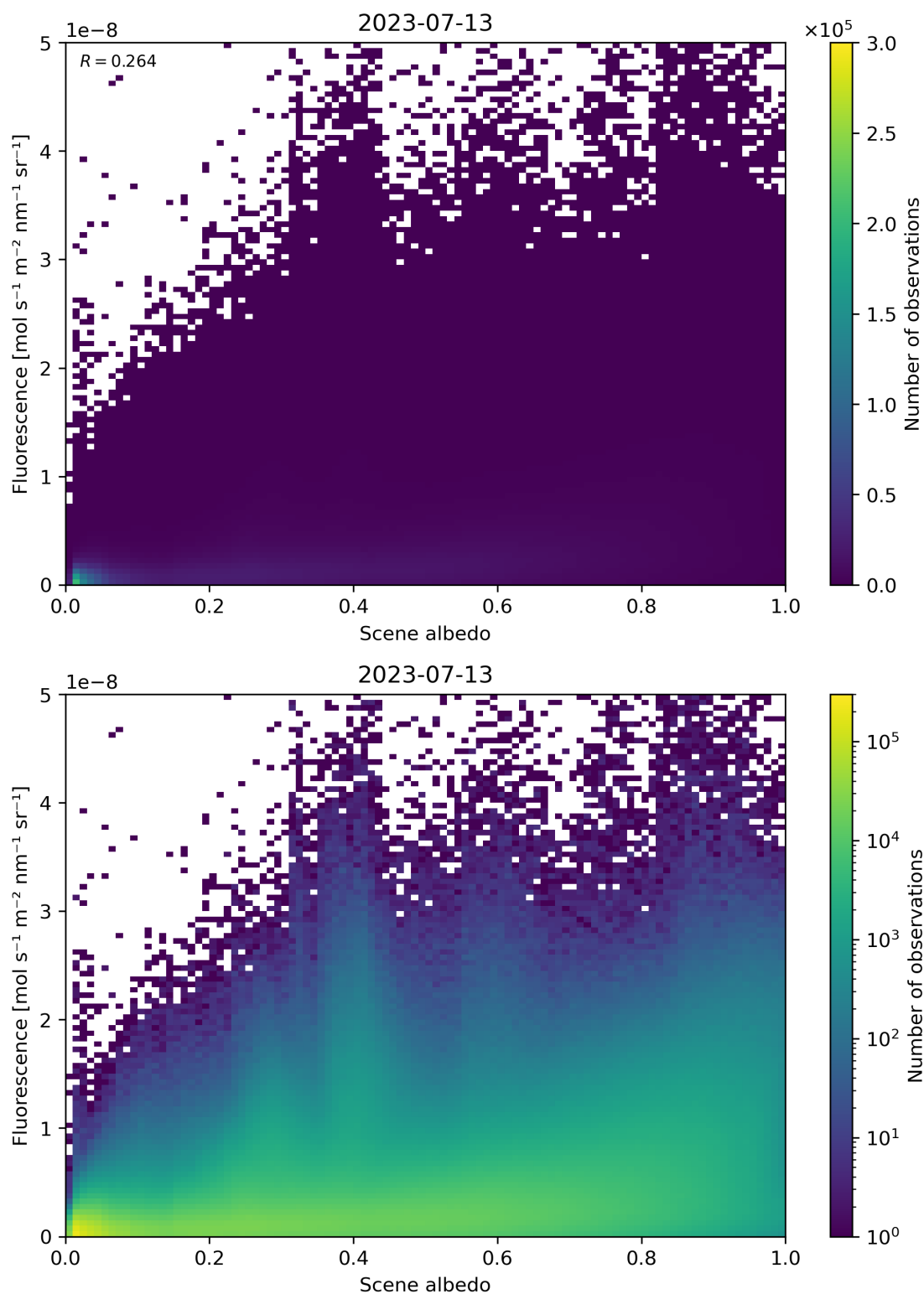
Figure 114: Scatter density plot of “Scene albedo” against “Fluorescence” for 2023-07-13 to 2023-07-14.
