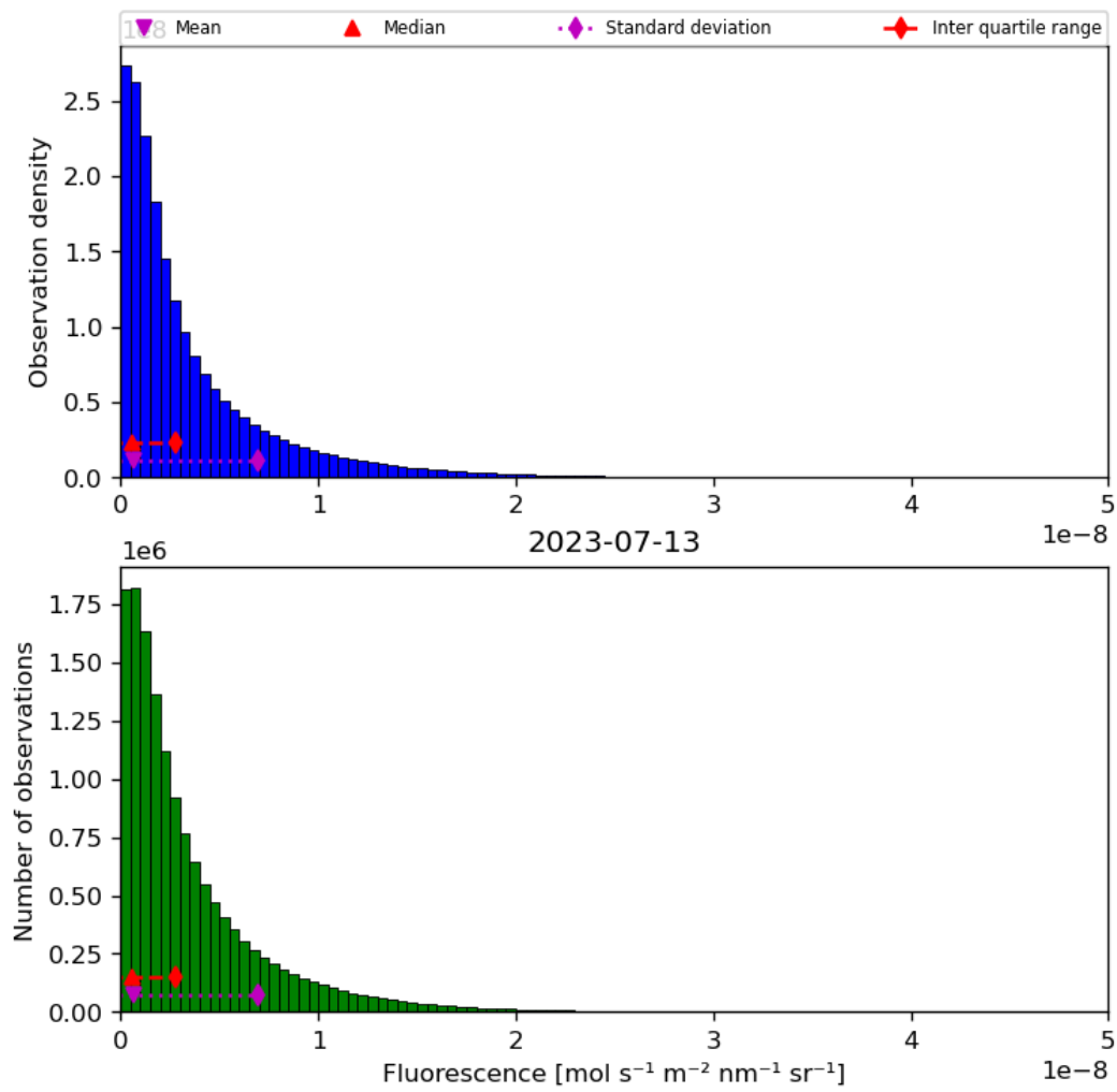
Figure 40: Histogram of “Fluorescence” for 2023-07-13 to 2023-07-14
