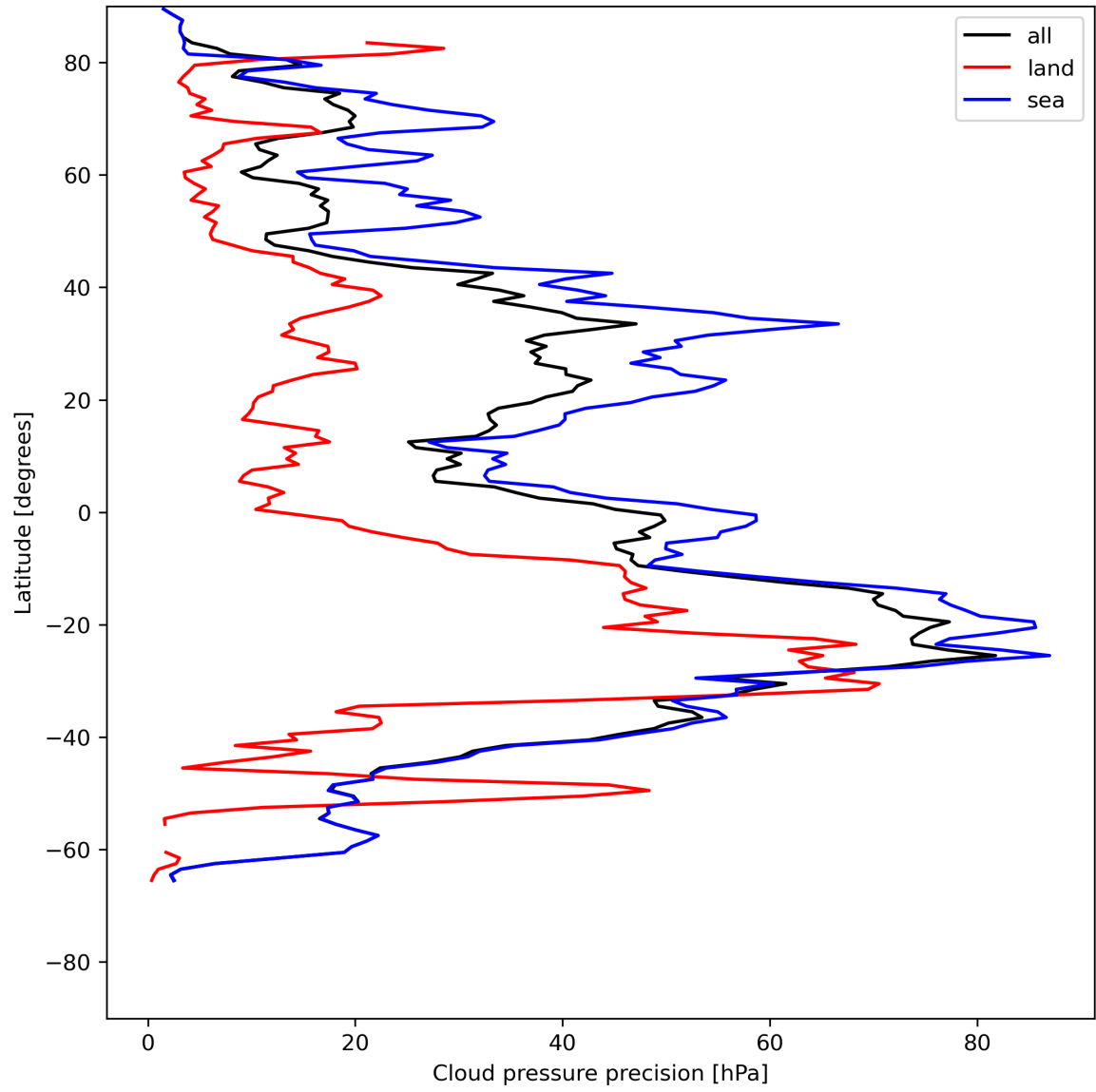
Figure 14: Zonal average of “Cloud pressure precision” for 2023-07-13 to 2023-07-14.
