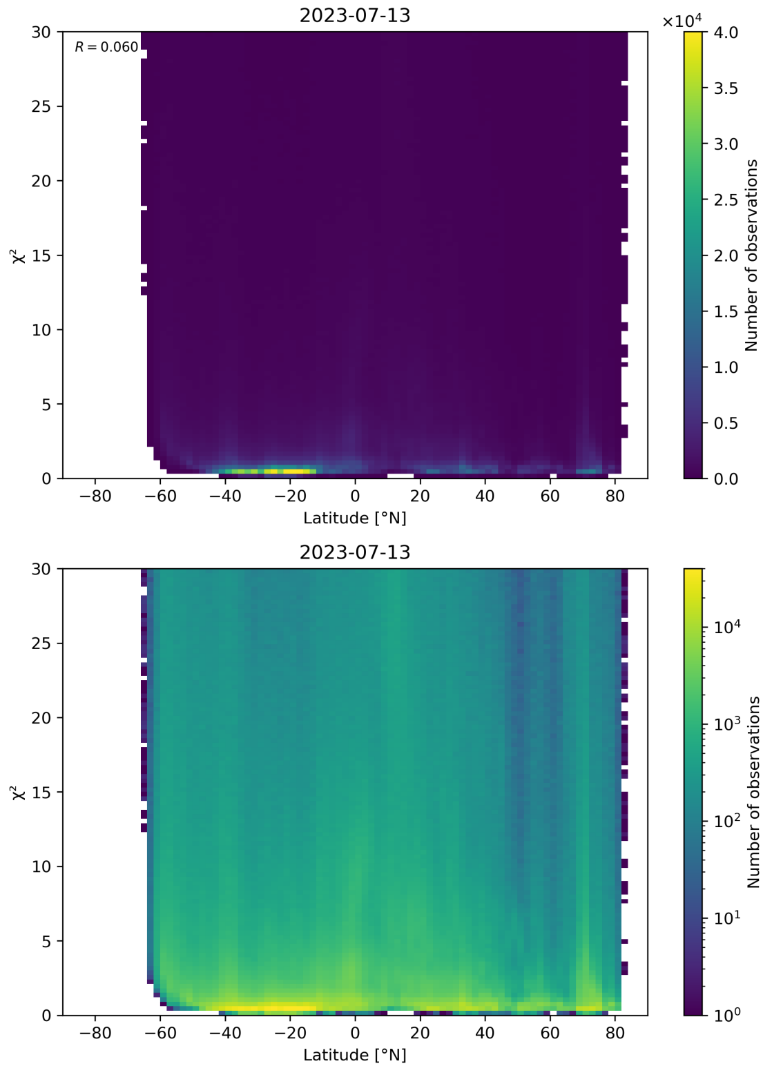
Figure 97: Scatter density plot of “Latitude” against “ \chi^2 ” for 2023-07-13 to 2023-07-14.
