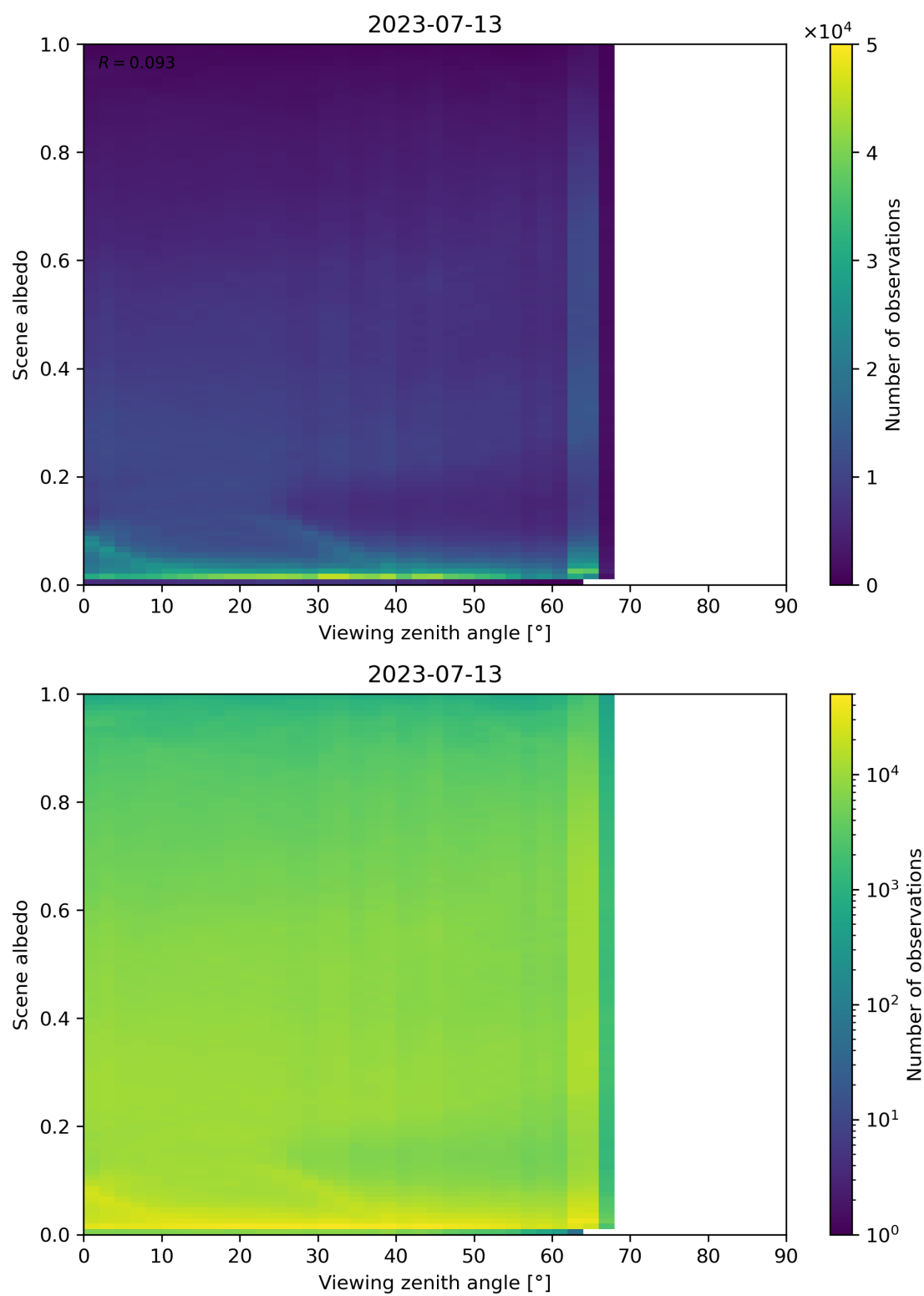
Figure 138: Scatter density plot of “Viewing zenith angle” against “Scene albedo” for 2023-07-13 to 2023-07-14.
