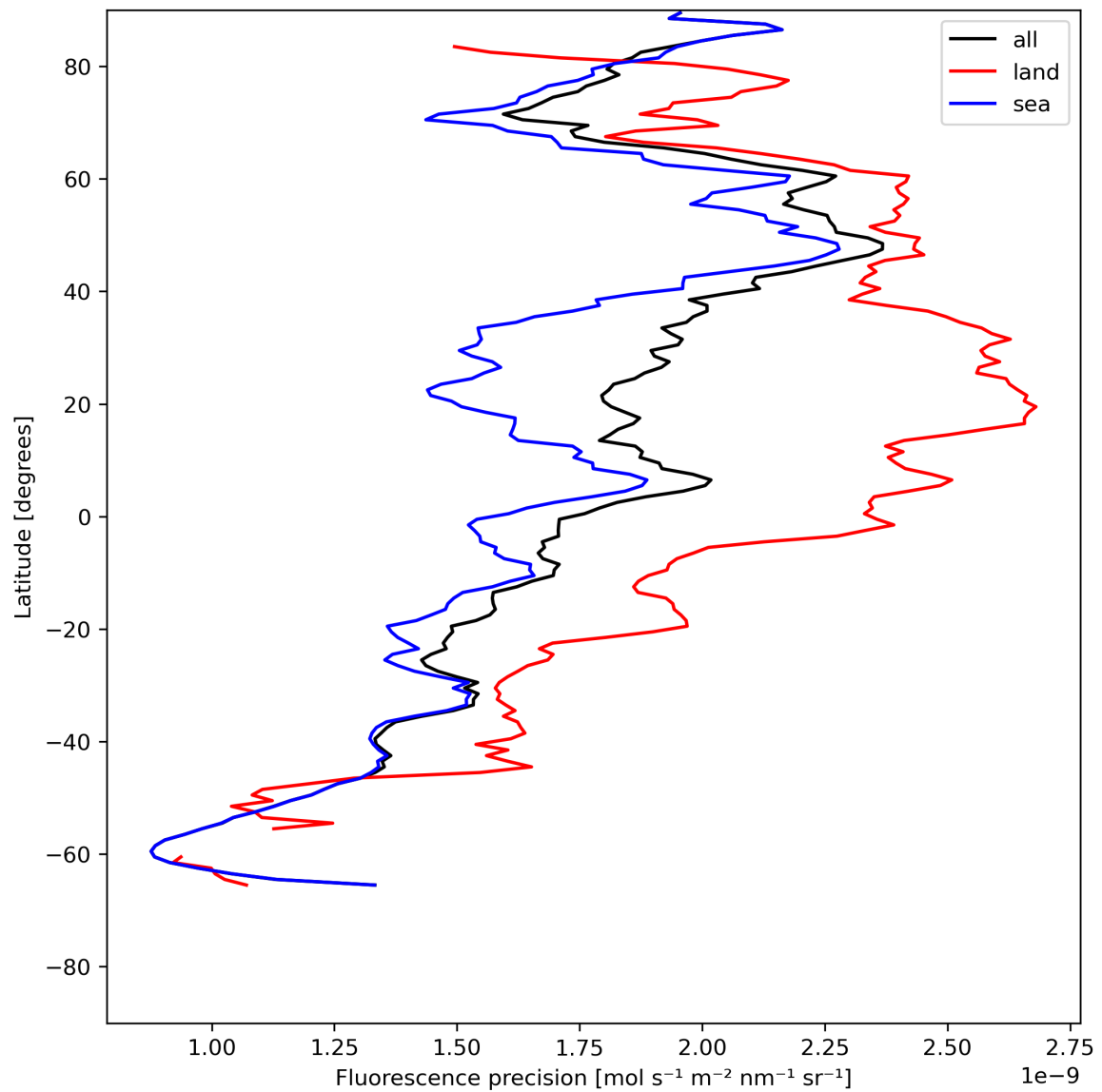
Figure 24: Zonal average of “Fluorescence precision” for 2023-07-13 to 2023-07-14.
