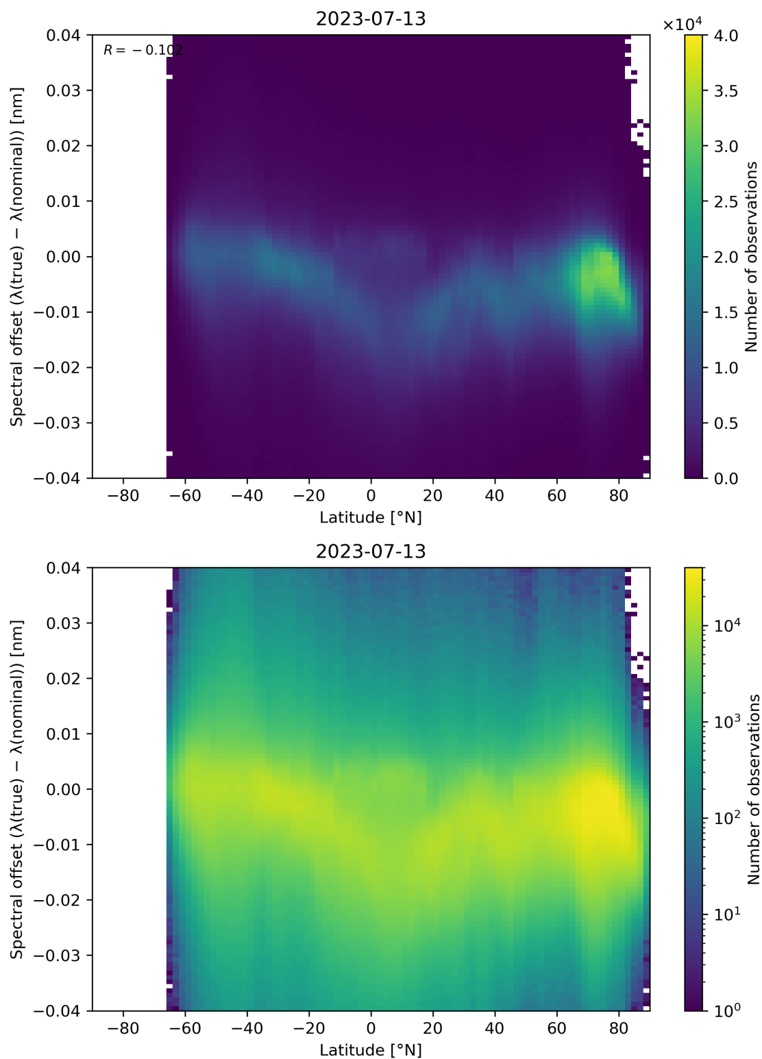
Figure 105: Scatter density plot of “Latitude” against “Spectral offset ( \lambda(\text{true}) - \lambda(\text{nominal}) )” for 2023-07-13 to 2023-07-14.
