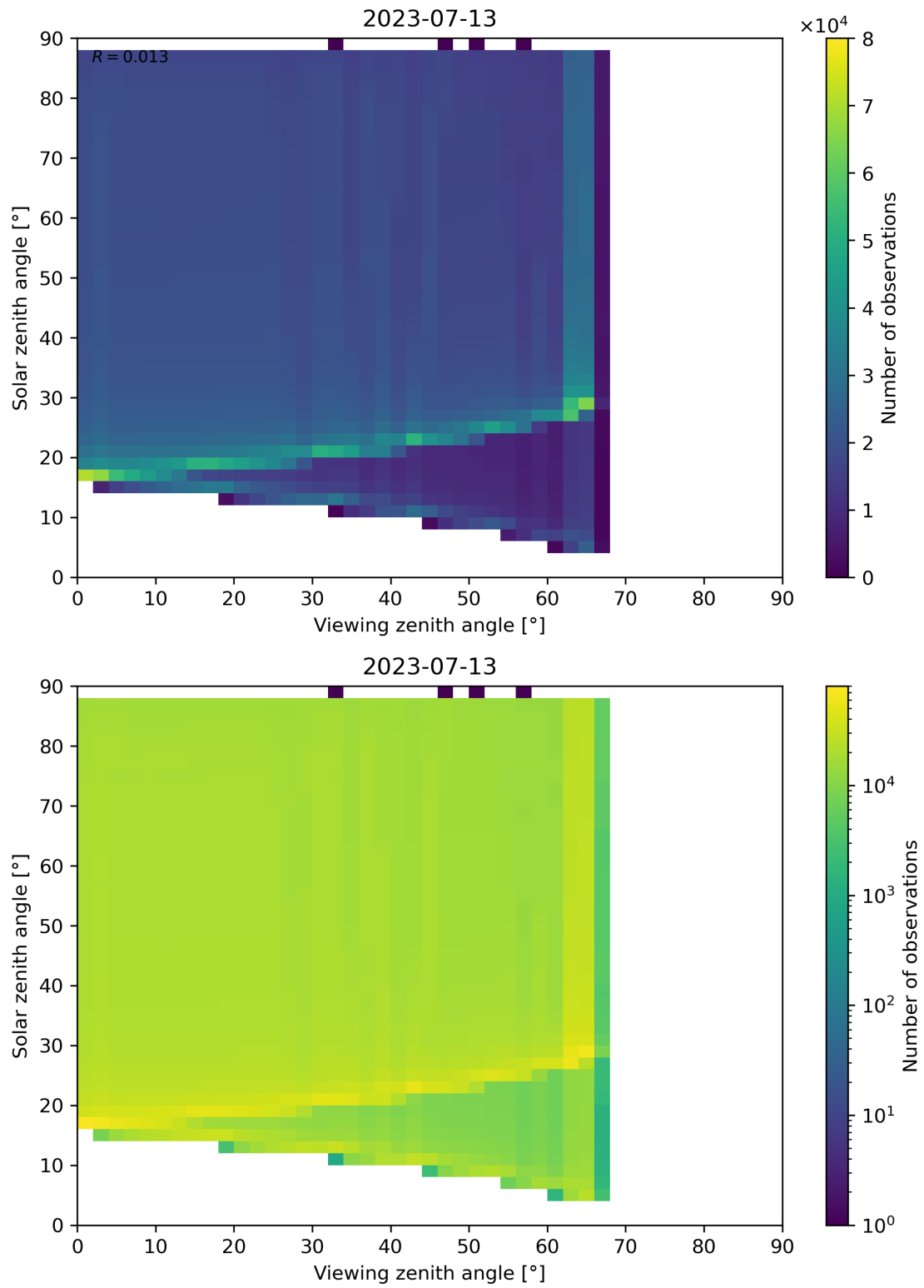
Figure 139: Scatter density plot of “Viewing zenith angle” against “Solar zenith angle” for 2023-07-13 to 2023-07-14.
