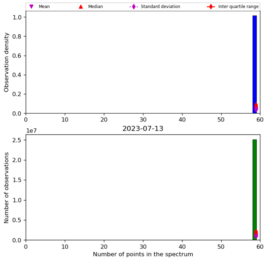
Figure 44: Histogram of “Number of points in the spectrum” for 2023-07-13 to 2023-07-14
