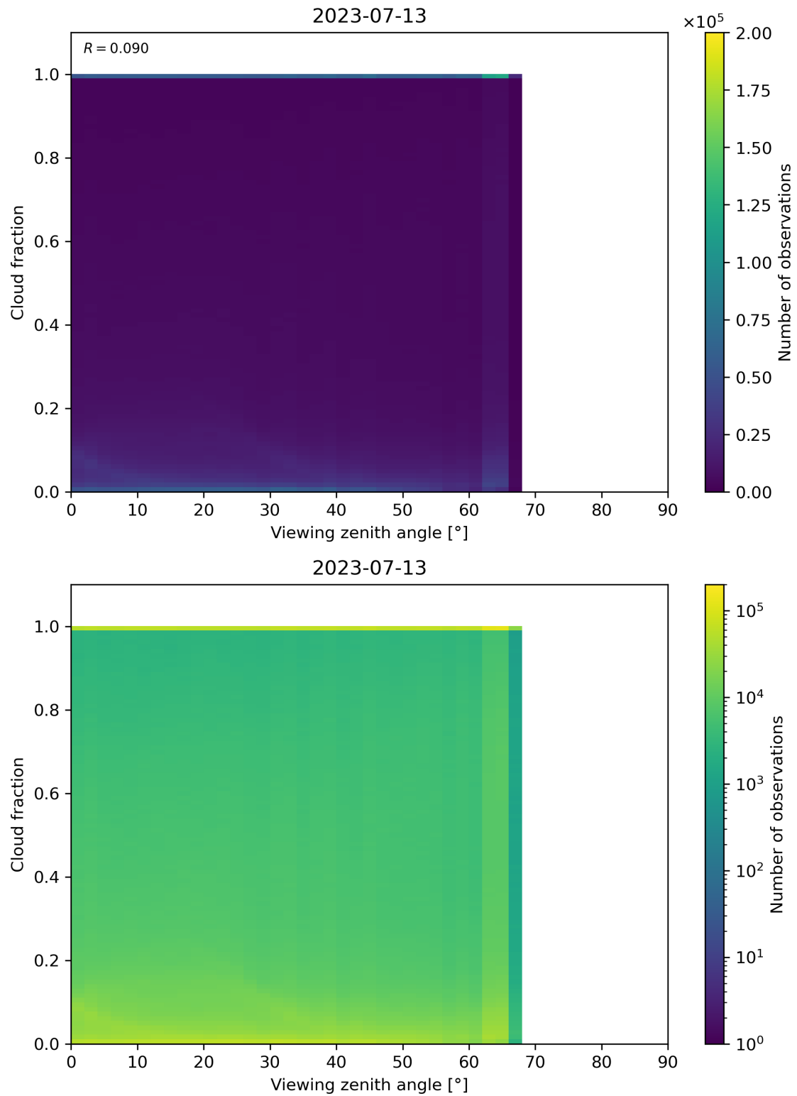
Figure 132: Scatter density plot of “Viewing zenith angle” against “Cloud fraction” for 2023-07-13 to 2023-07-14.
