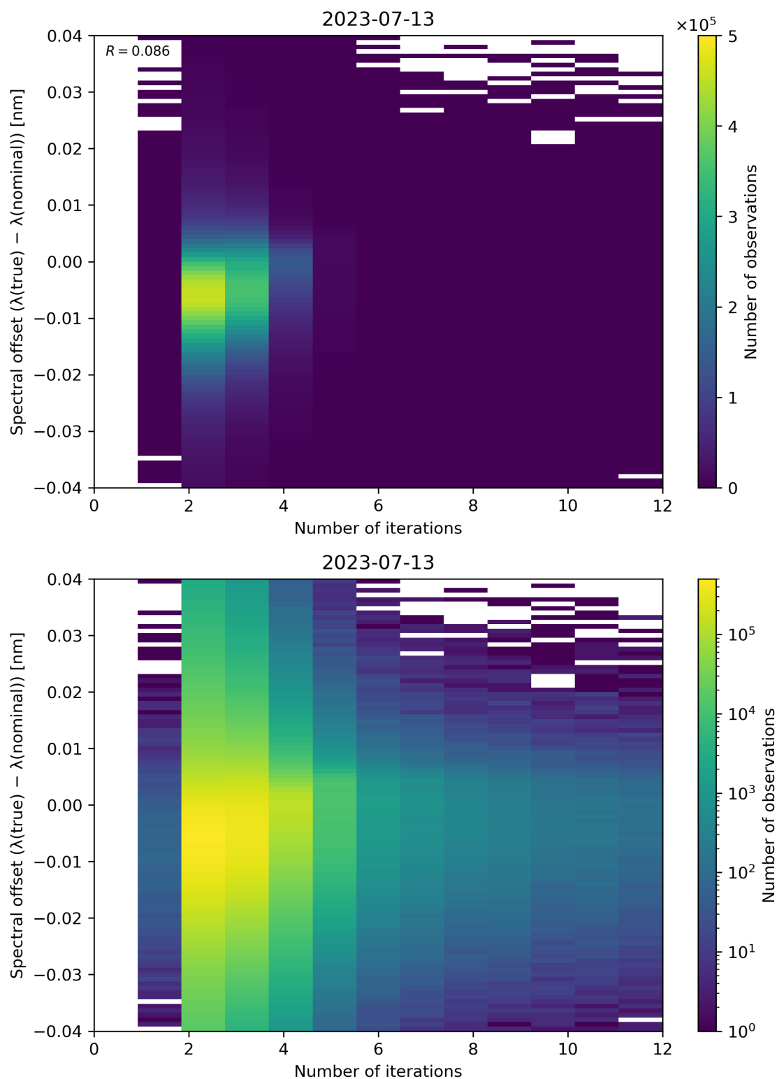
Figure 109: Scatter density plot of “Number of iterations” against “Spectral offset ( \lambda(\text{true}) - \lambda(\text{nominal}) )” for 2023-07-13 to 2023-07-14.
