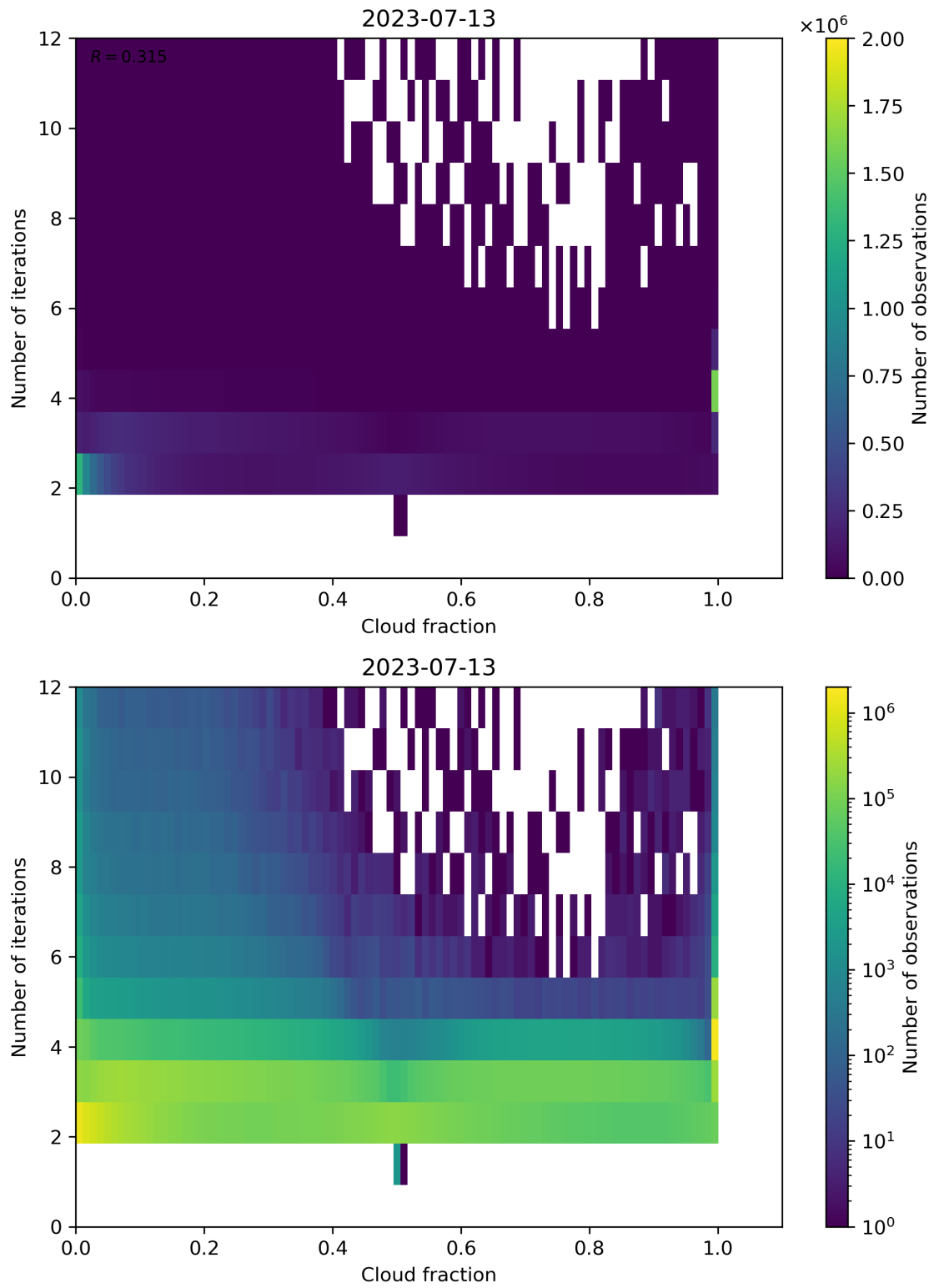
Figure 80: Scatter density plot of “Cloud fraction” against “Number of iterations” for 2023-07-13 to 2023-07-14.
