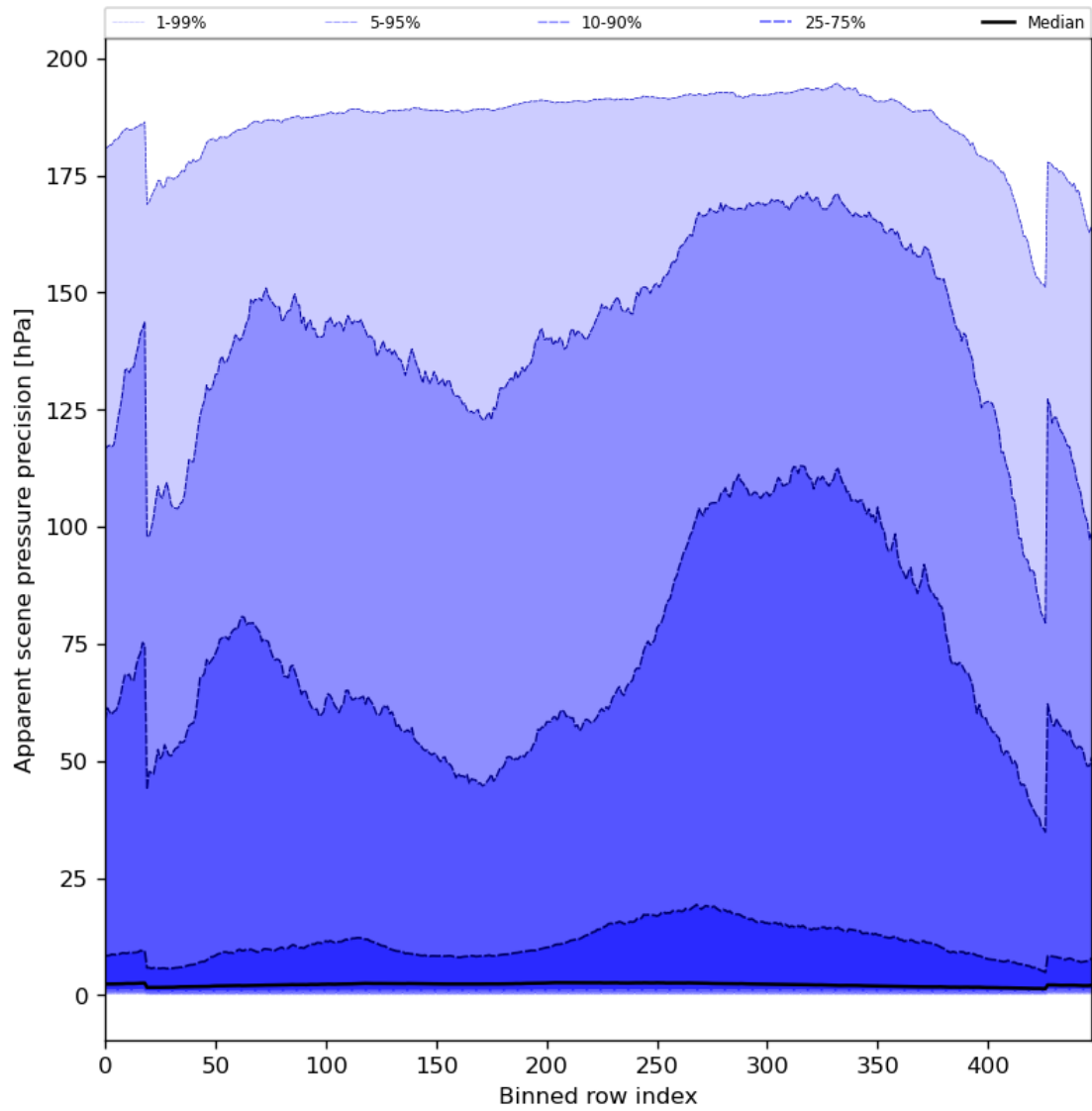
Figure 54: Along track statistics of “Apparent scene pressure precision” for 2023-07-13 to 2023-07-14
