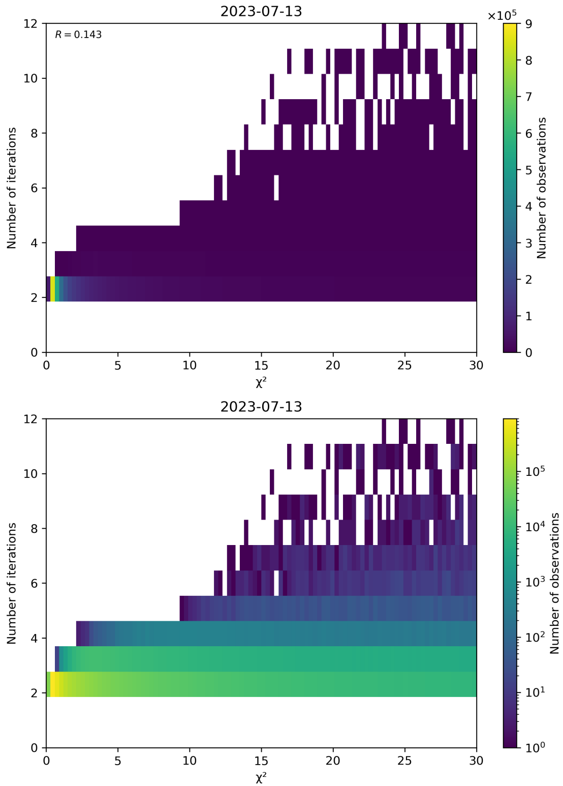
Figure 73: Scatter density plot of “ \chi^2 ” against “Number of iterations” for 2023-07-13 to 2023-07-14.
