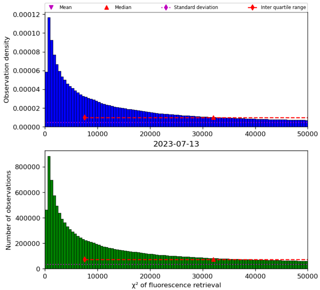
Figure 42: Histogram of “ \chi^2 of fluorescence retrieval” for 2023-07-13 to 2023-07-14
