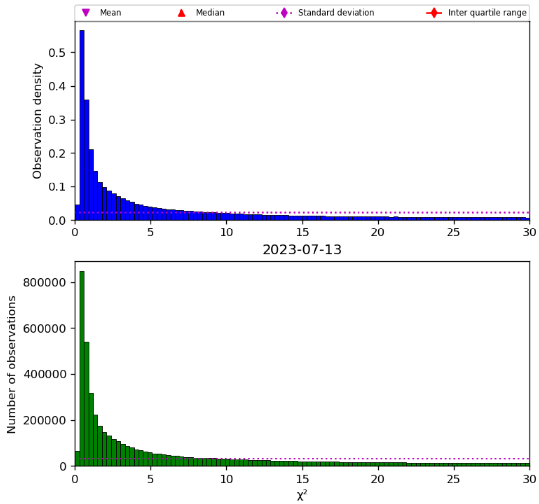
Figure 38: Histogram of “ \chi^2 ” for 2023-07-13 to 2023-07-14
