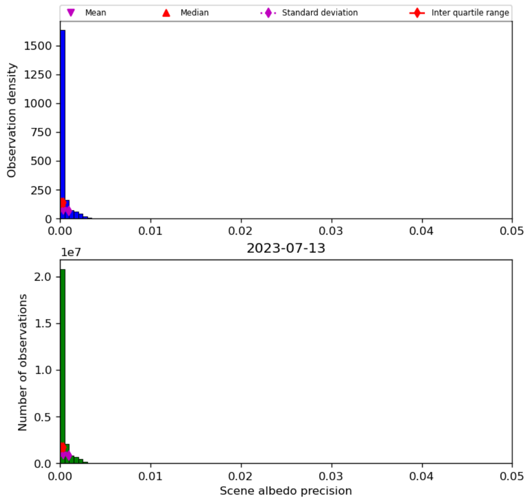
Figure 35: Histogram of “Scene albedo precision” for 2023-07-13 to 2023-07-14
