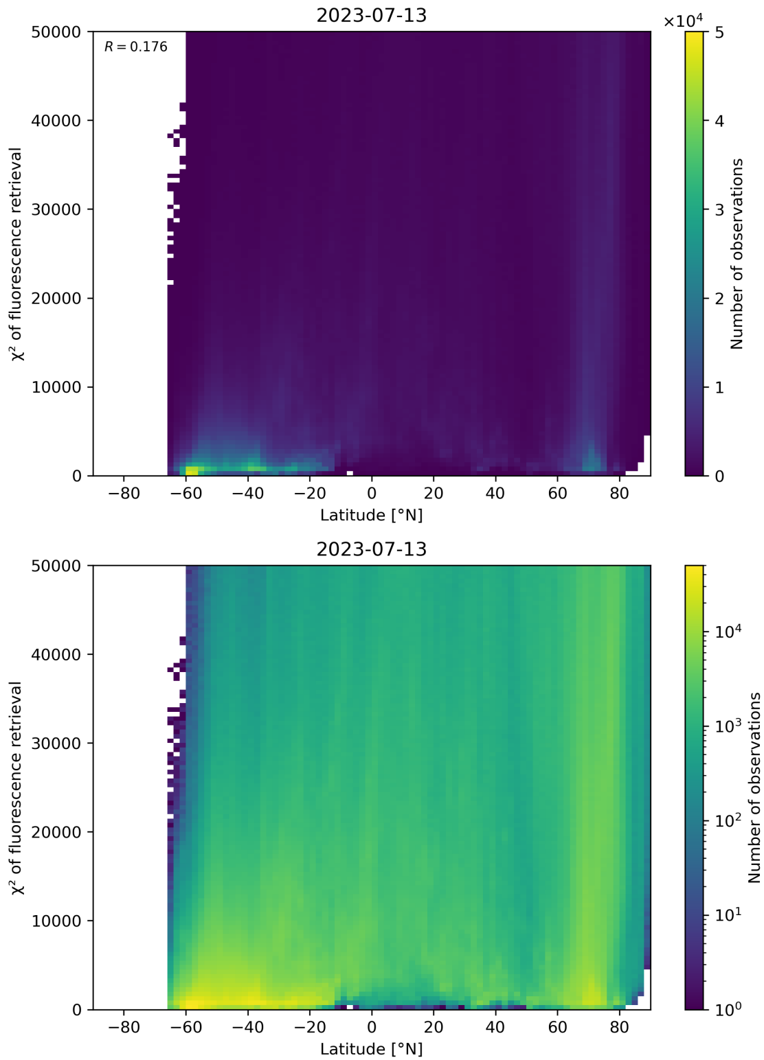
Figure 98: Scatter density plot of “Latitude” against “ \chi^2 of fluorescence retrieval” for 2023-07-13 to 2023-07-14.
