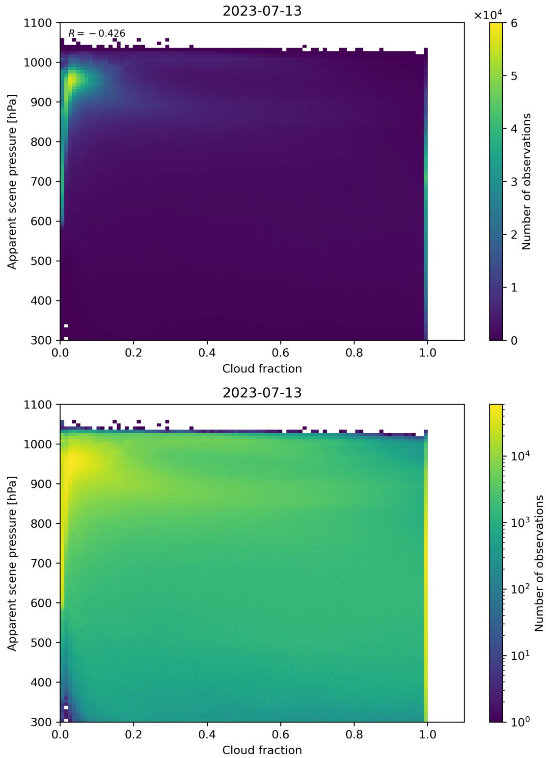
Figure 76: Scatter density plot of “Cloud fraction” against “Apparent scene pressure” for 2023-07-13 to 2023-07-14.
