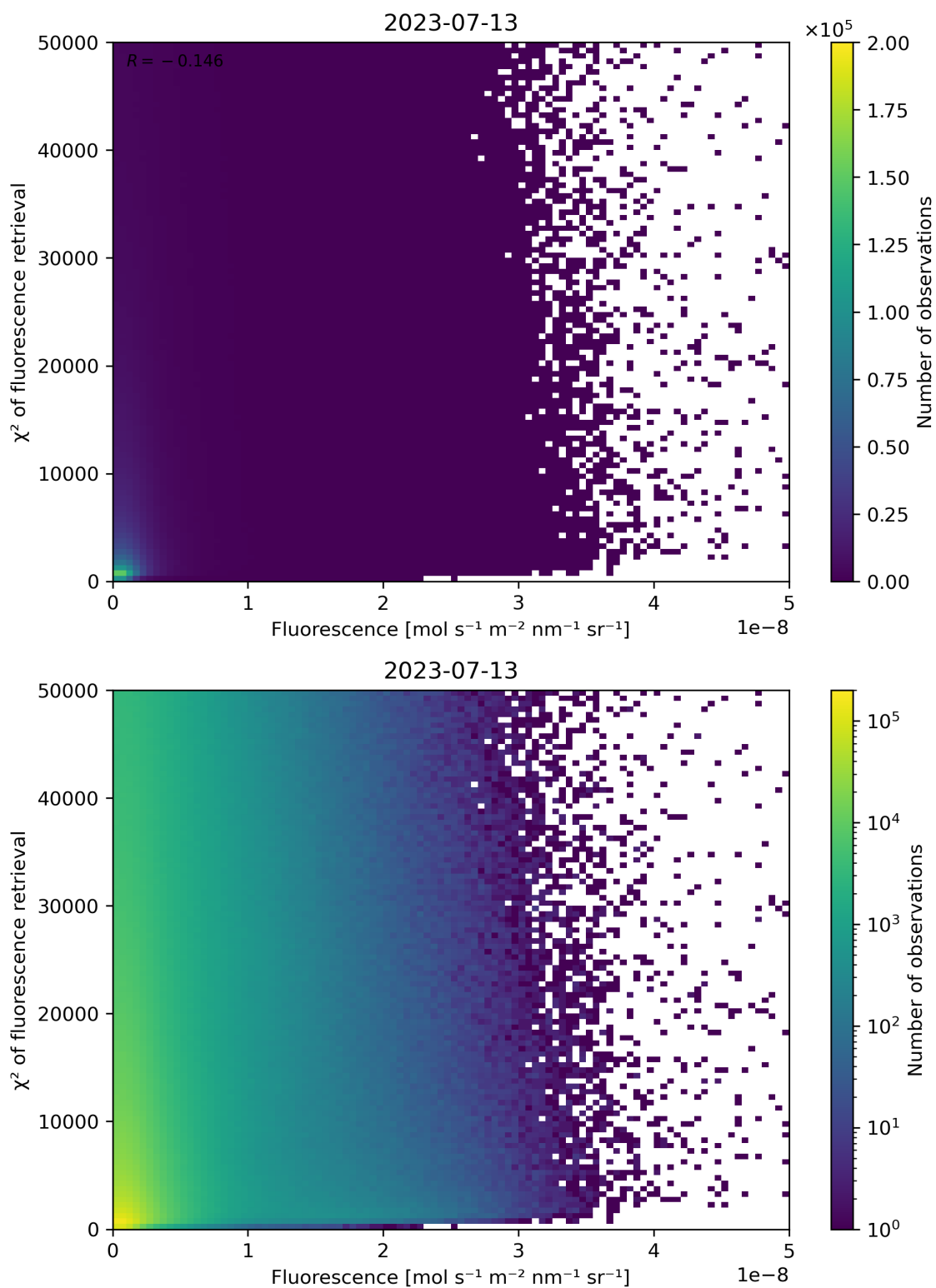
Figure 93: Scatter density plot of “Fluorescence” against “ \chi^2 of fluorescence retrieval” for 2023-07-13 to 2023-07-14.
