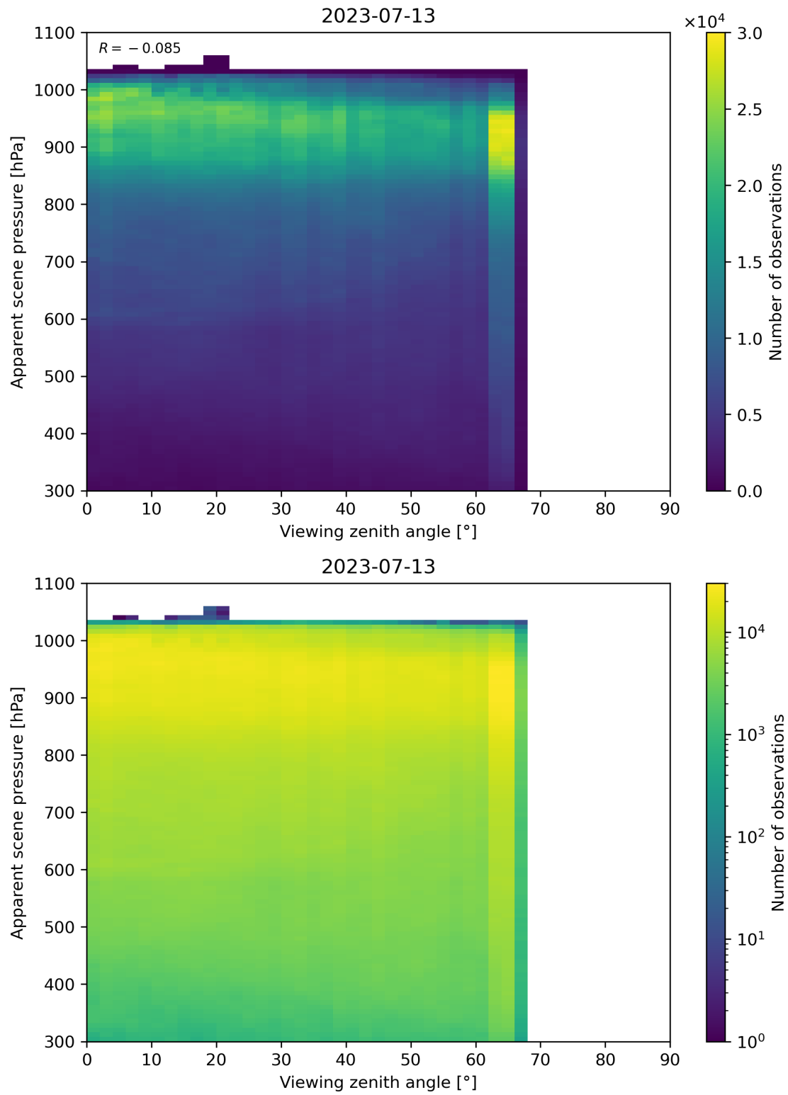
Figure 129: Scatter density plot of “Viewing zenith angle” against “Apparent scene pressure” for 2023-07-13 to 2023-07-14.
