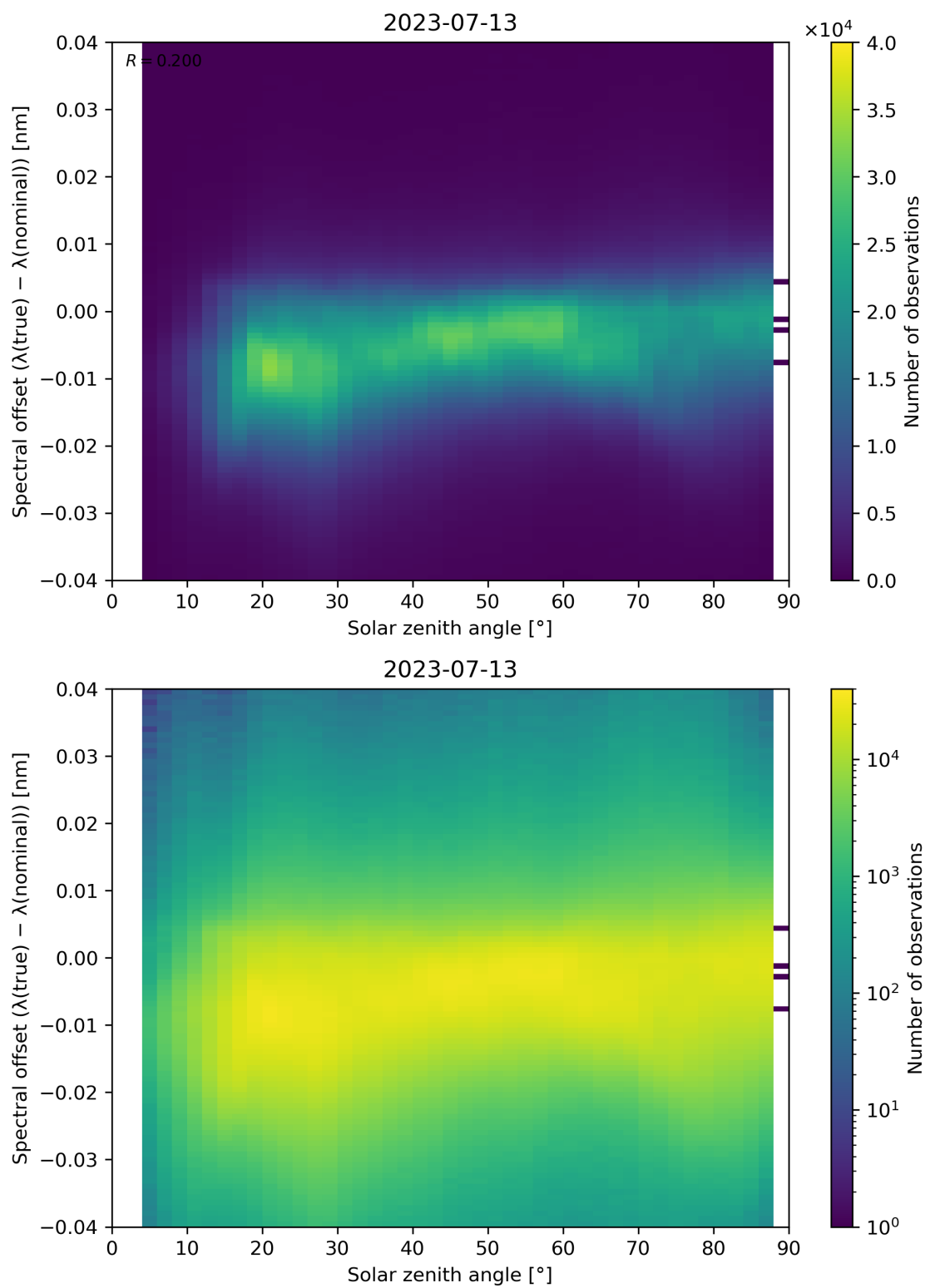
Figure 128: Scatter density plot of “Solar zenith angle” against “Spectral offset ( \lambda(\text{true}) - \lambda(\text{nominal}) )” for 2023-07-13 to 2023-07-14.
