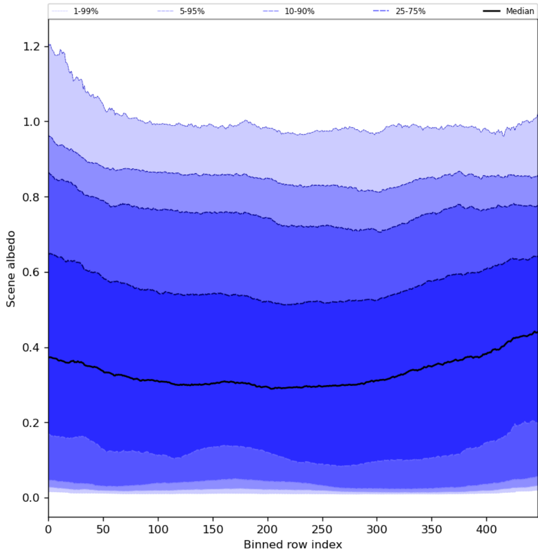
Figure 51: Along track statistics of “Scene albedo” for 2023-07-13 to 2023-07-14
