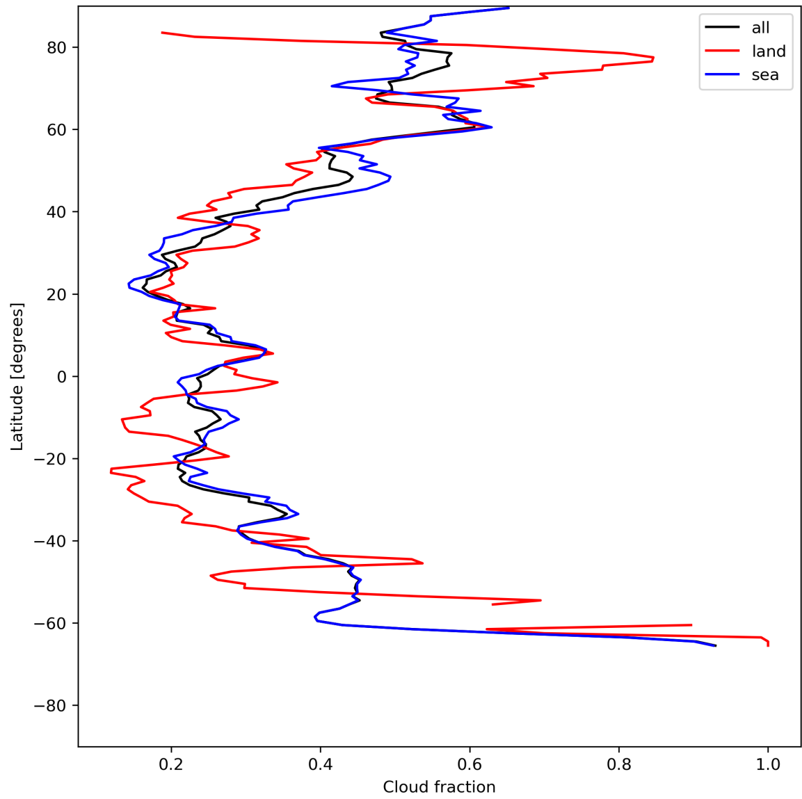
Figure 15: Zonal average of “Cloud fraction” for 2023-07-13 to 2023-07-14.
