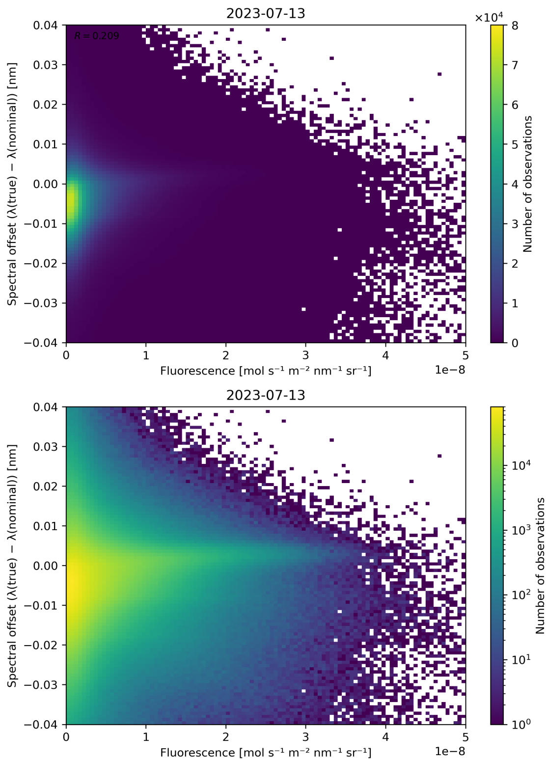
Figure 95: Scatter density plot of “Fluorescence” against “Spectral offset ( \lambda(\text{true}) - \lambda(\text{nominal}) )” for 2023-07-13 to 2023-07-14.
