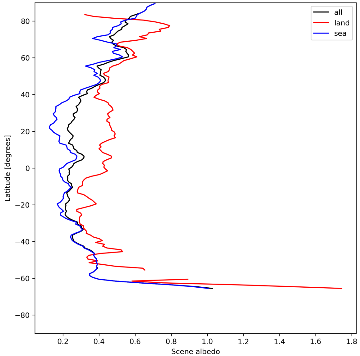
Figure 17: Zonal average of “Scene albedo” for 2023-07-13 to 2023-07-14.
