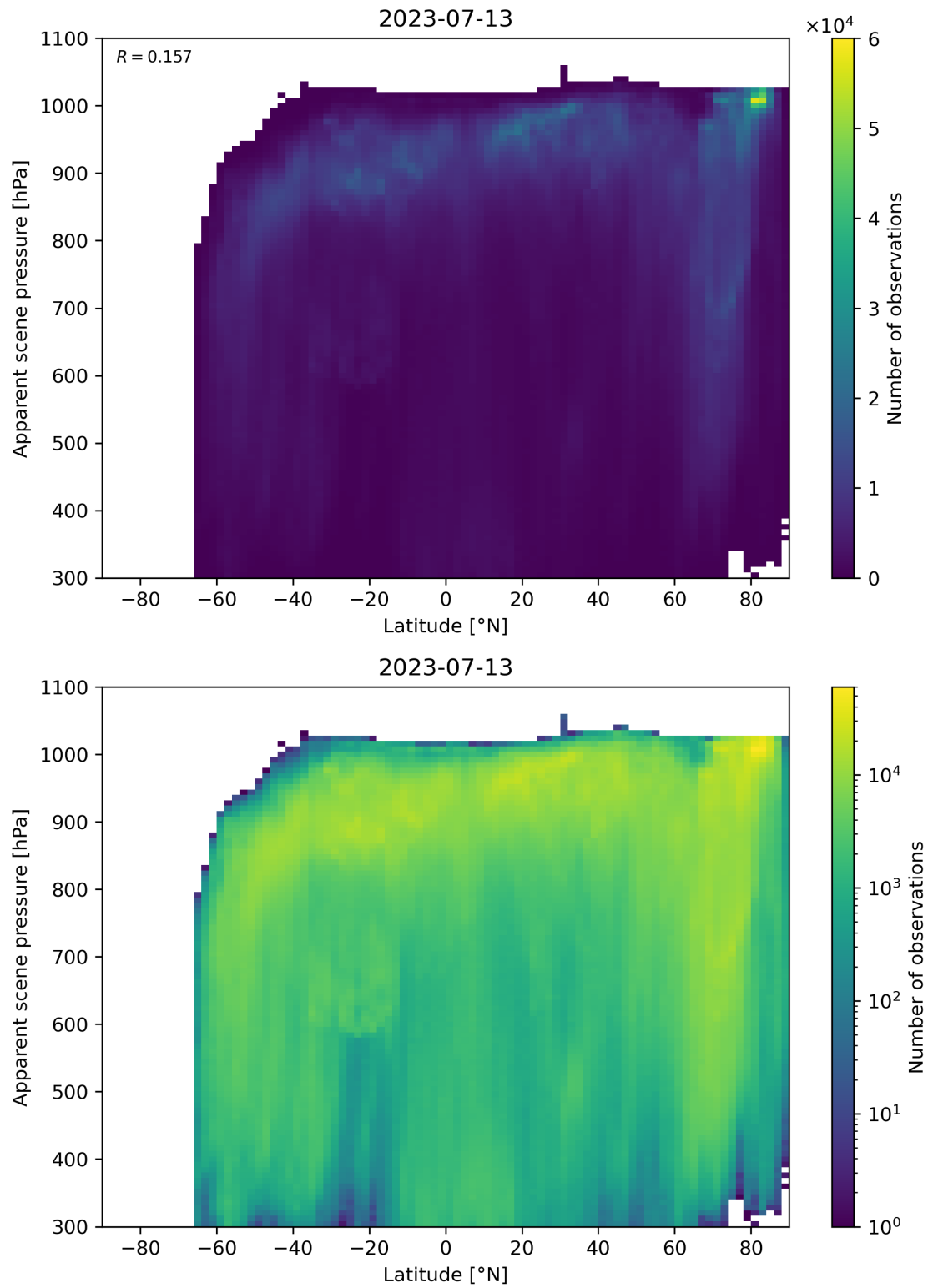
Figure 96: Scatter density plot of “Latitude” against “Apparent scene pressure” for 2023-07-13 to 2023-07-14.
