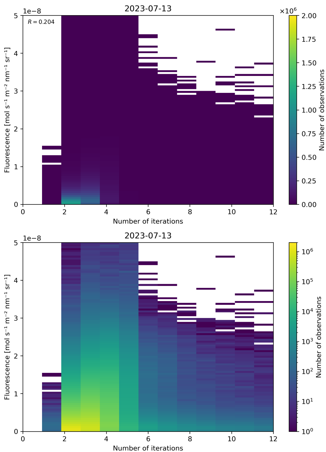
Figure 107: Scatter density plot of “Number of iterations” against “Fluorescence” for 2023-07-13 to 2023-07-14.
