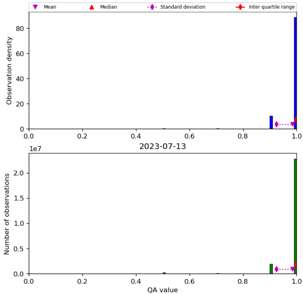
Figure 29: Histogram of “QA value” for 2023-07-13 to 2023-07-14
