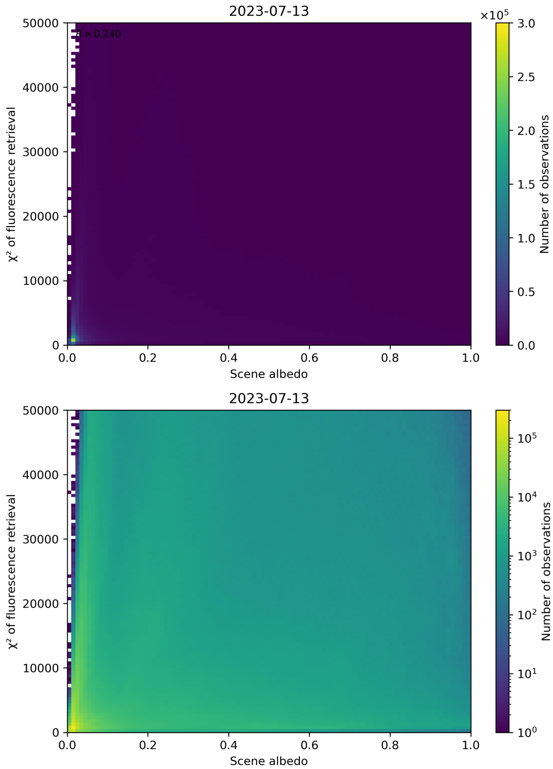
Figure 113: Scatter density plot of “Scene albedo” against “ \chi^2 of fluorescence retrieval” for 2023-07-13 to 2023-07-14.
