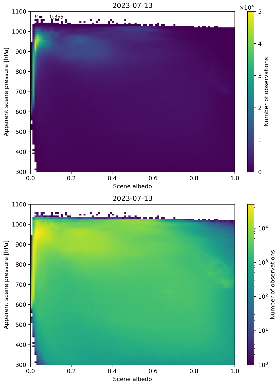
Figure 111: Scatter density plot of “Scene albedo” against “Apparent scene pressure” for 2023-07-13 to 2023-07-14.
