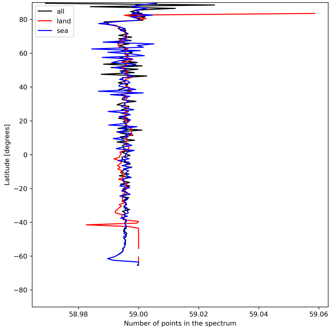
Figure 27: Zonal average of “Number of points in the spectrum” for 2023-07-13 to 2023-07-14.
