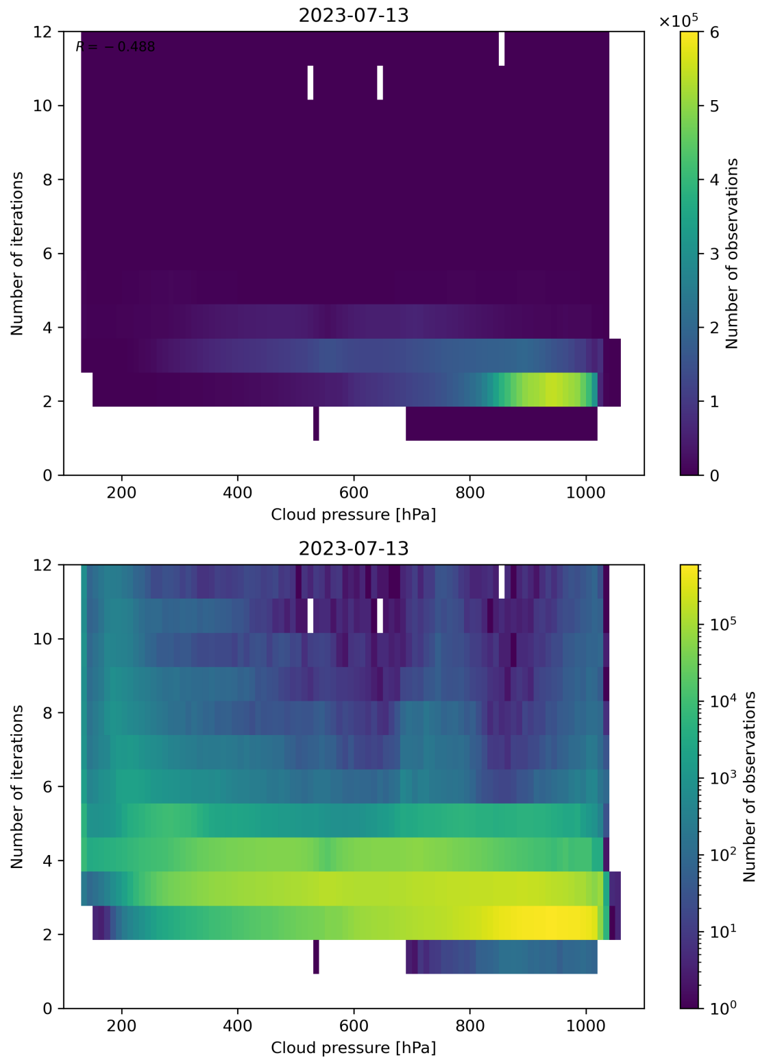
Figure 89: Scatter density plot of “Cloud pressure” against “Number of iterations” for 2023-07-13 to 2023-07-14.
