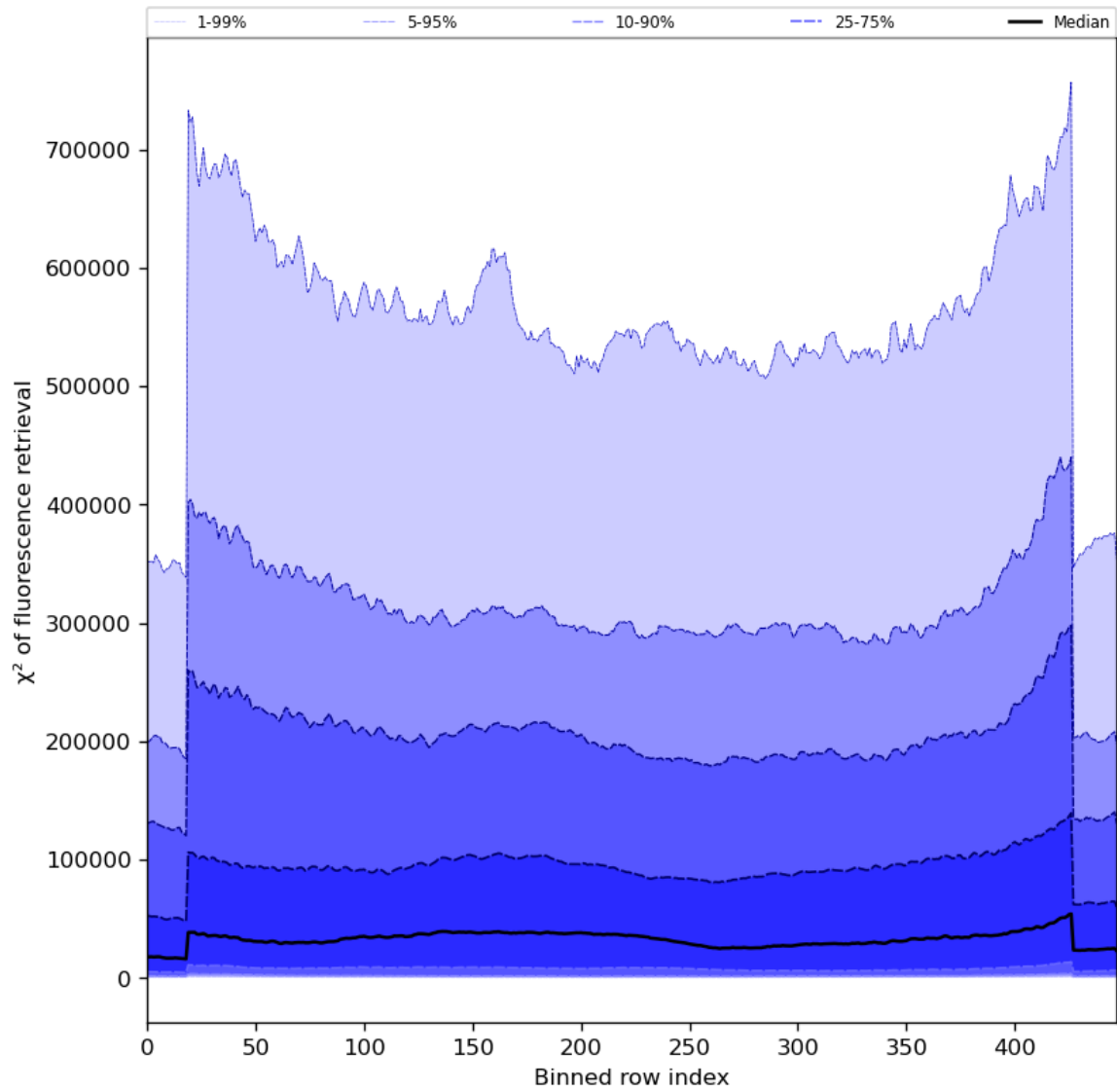
Figure 59: Along track statistics of “ \chi^2 of fluorescence retrieval” for 2023-07-13 to 2023-07-14
