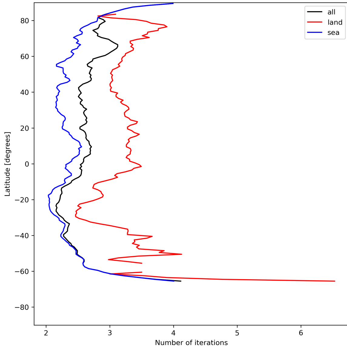
Figure 22: Zonal average of “Number of iterations” for 2023-07-13 to 2023-07-14.
