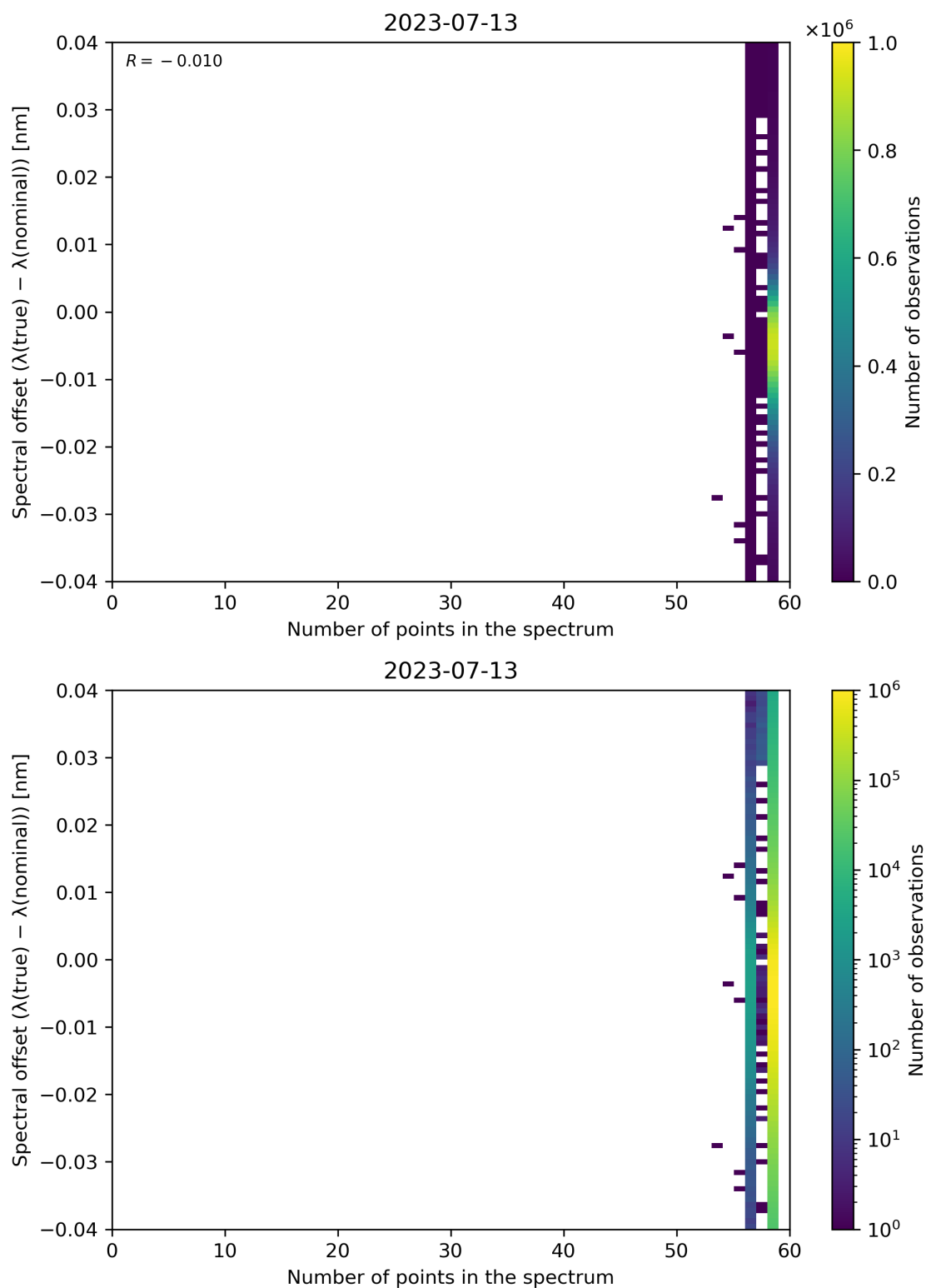
Figure 110: Scatter density plot of “Number of points in the spectrum” against “Spectral offset ( \lambda(\text{true}) - \lambda(\text{nominal}) )” for 2023-07-13 to 2023-07-14.
