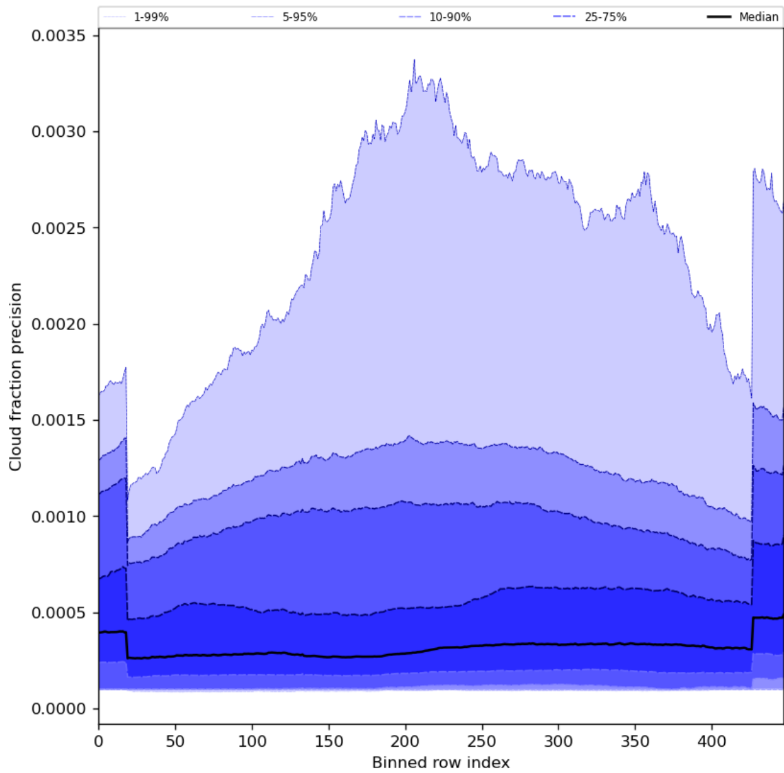
Figure 50: Along track statistics of “Cloud fraction precision” for 2023-07-13 to 2023-07-14
