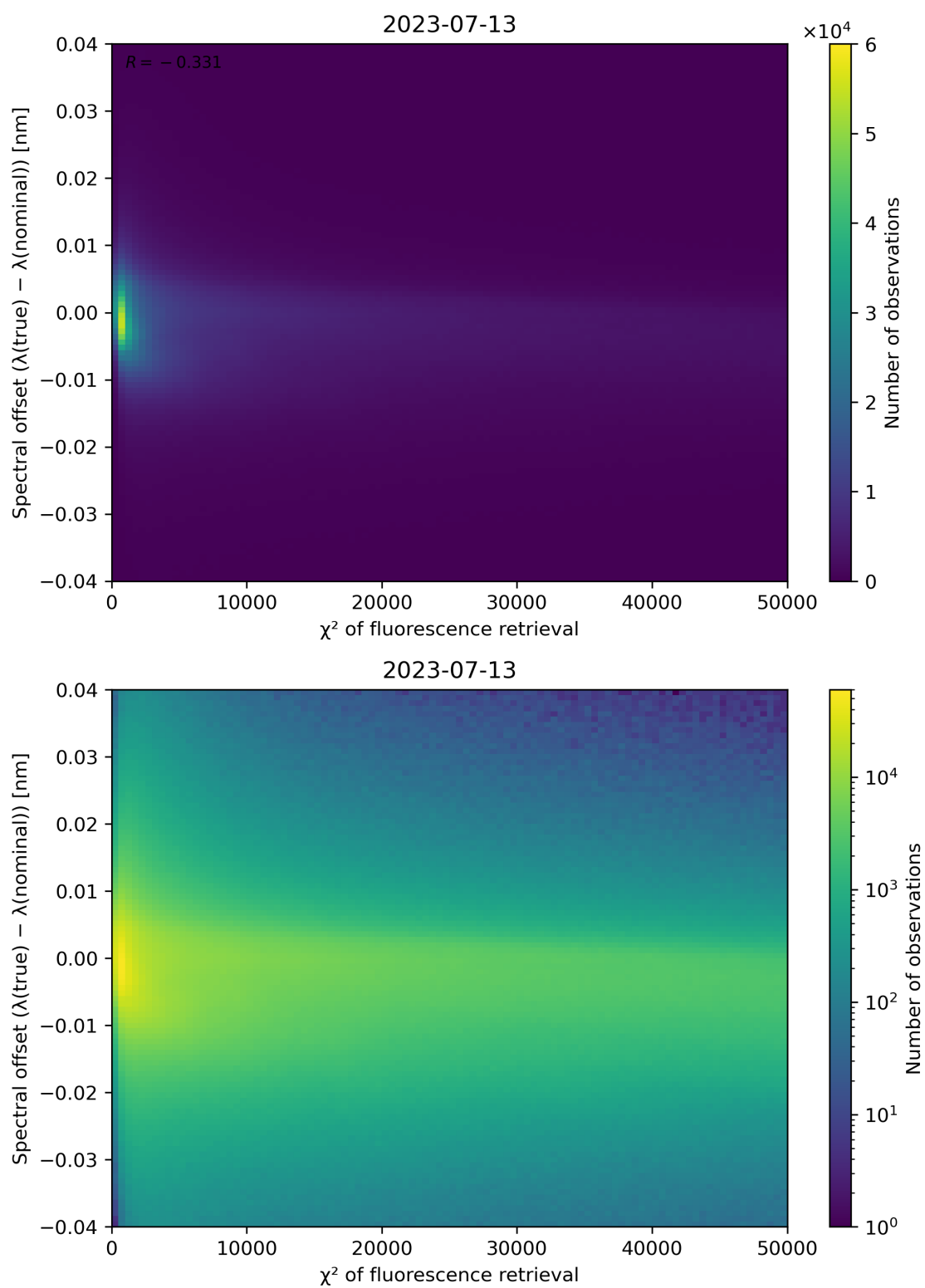
Figure 72: Scatter density plot of " \chi^2 of fluorescence retrieval" against "Spectral offset ( \lambda(\text{true}) - \lambda(\text{nominal})) " for 2023-07-13 to 2023-07-14.
