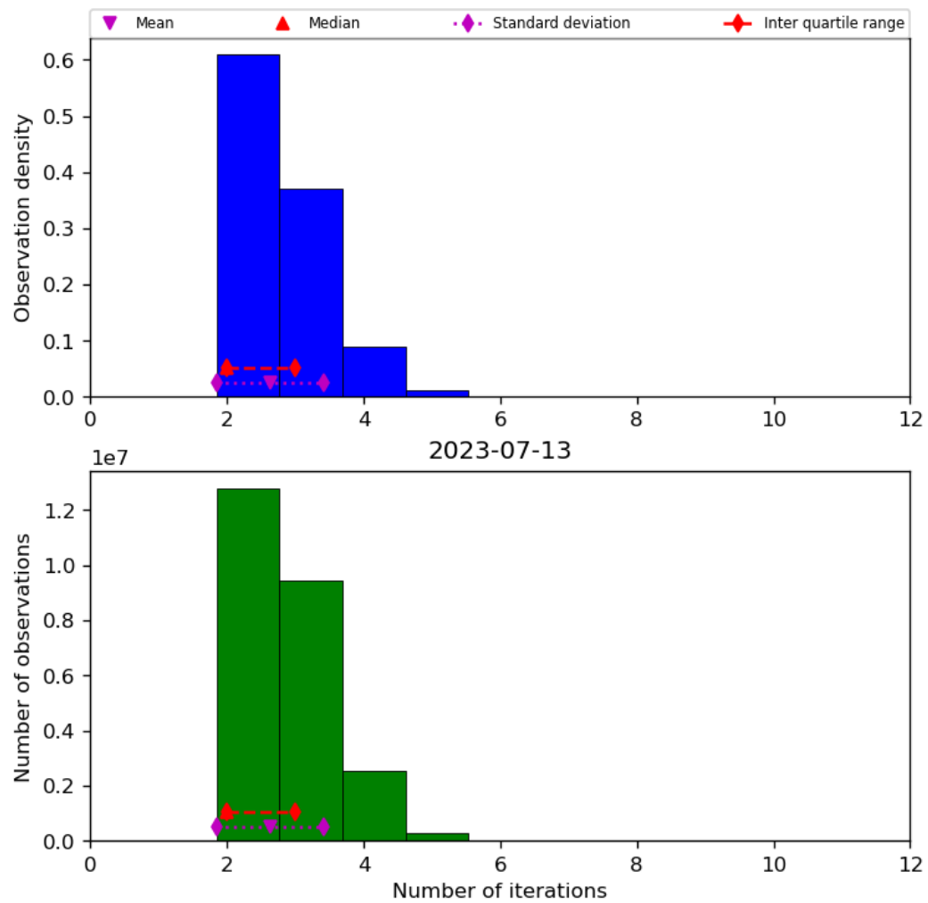
Figure 39: Histogram of “Number of iterations” for 2023-07-13 to 2023-07-14
