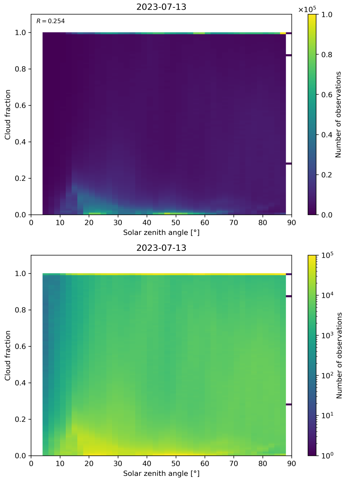
Figure 121: Scatter density plot of “Solar zenith angle” against “Cloud fraction” for 2023-07-13 to 2023-07-14.
