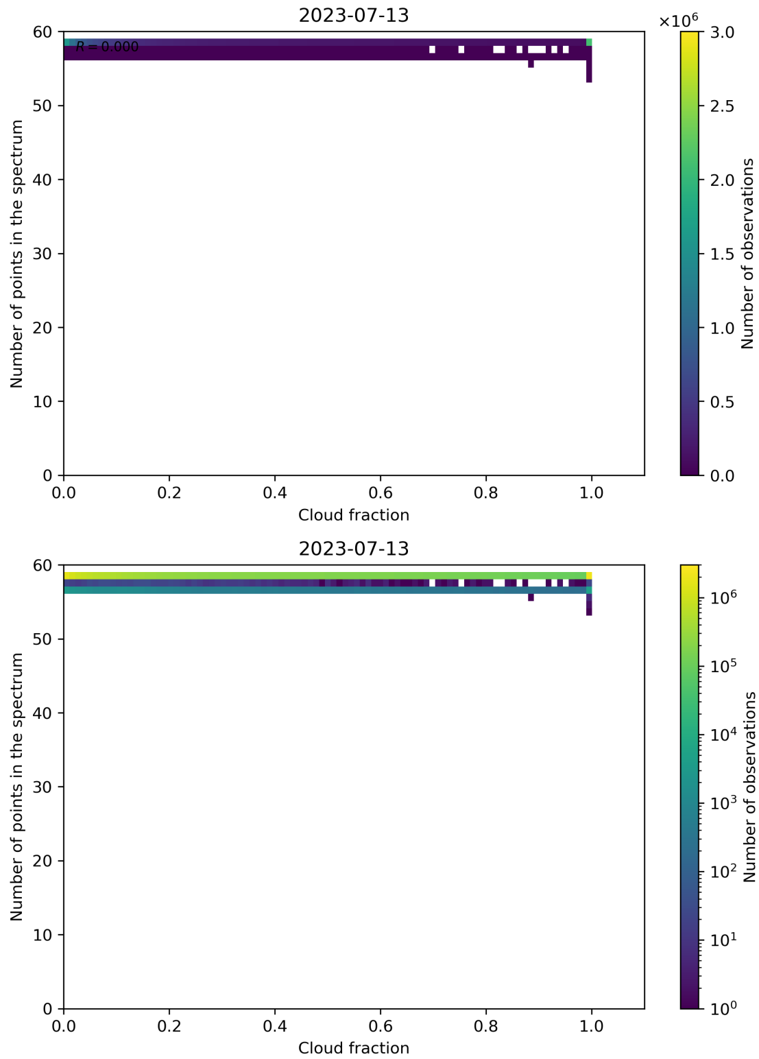
Figure 81: Scatter density plot of “Cloud fraction” against “Number of points in the spectrum” for 2023-07-13 to 2023-07-14.
