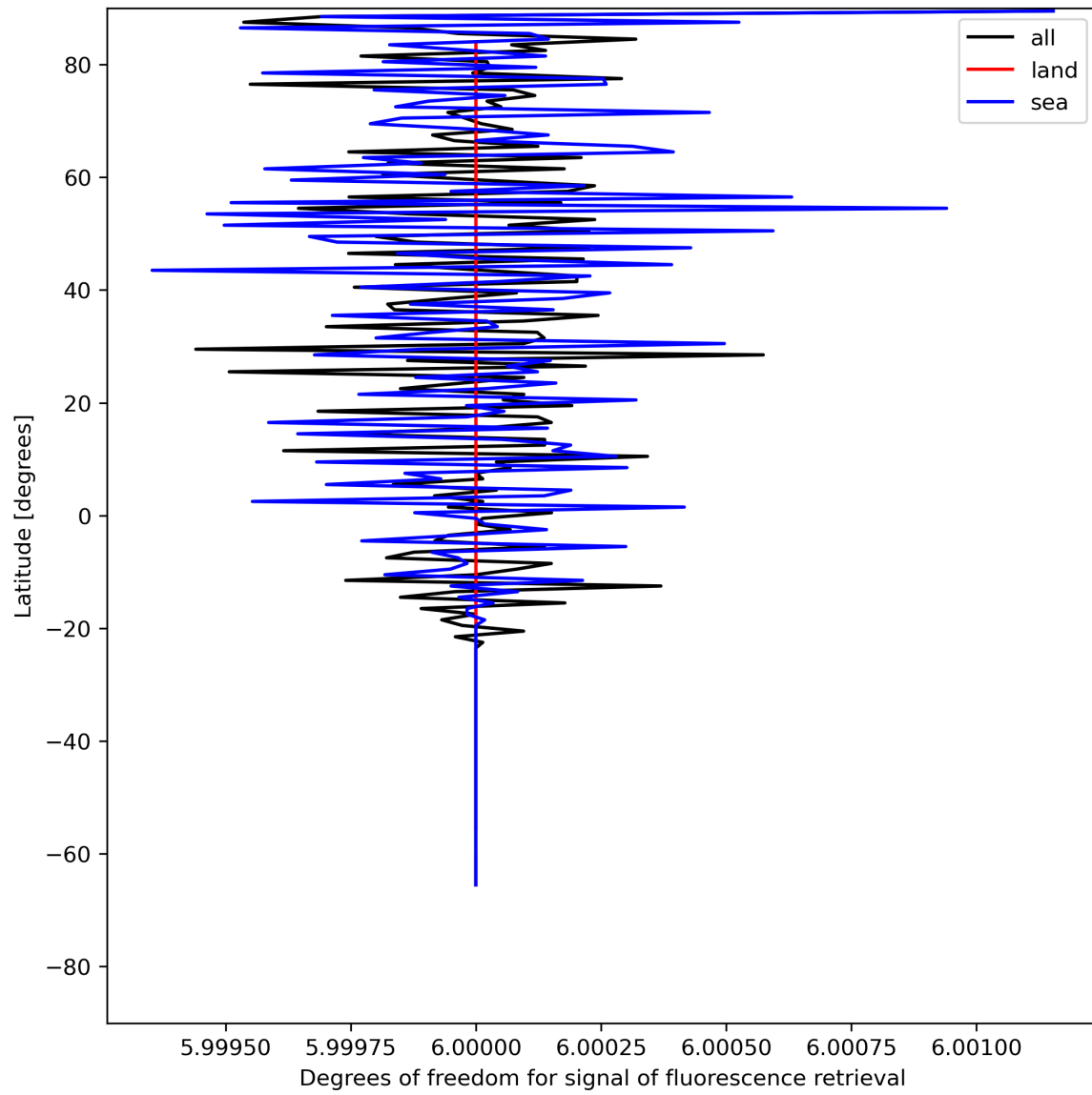
Figure 26: Zonal average of “Degrees of freedom for signal of fluorescence retrieval” for 2023-07-13 to 2023-07-14.
