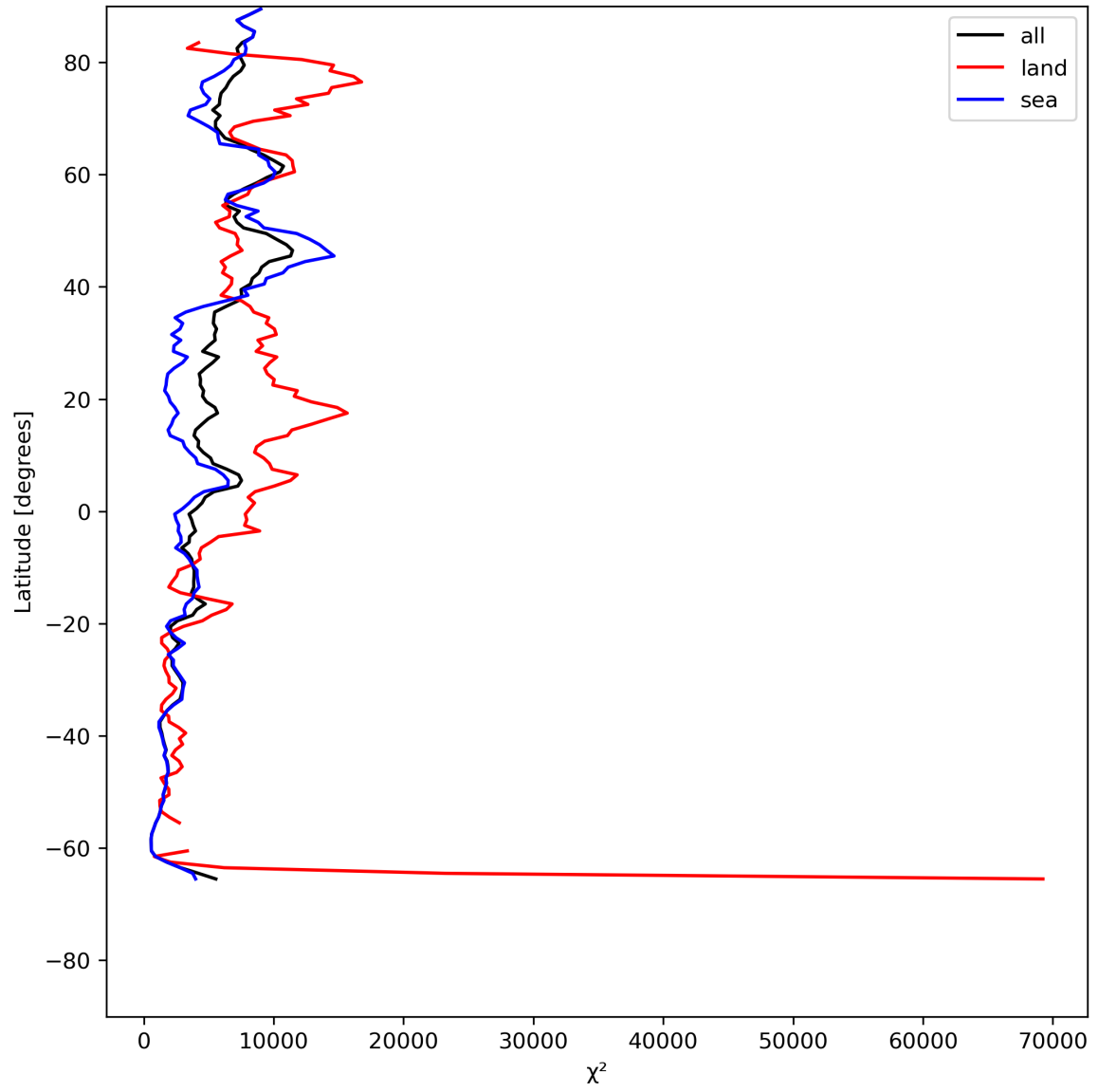
Figure 21: Zonal average of “ \chi^2 ” for 2023-07-13 to 2023-07-14.
