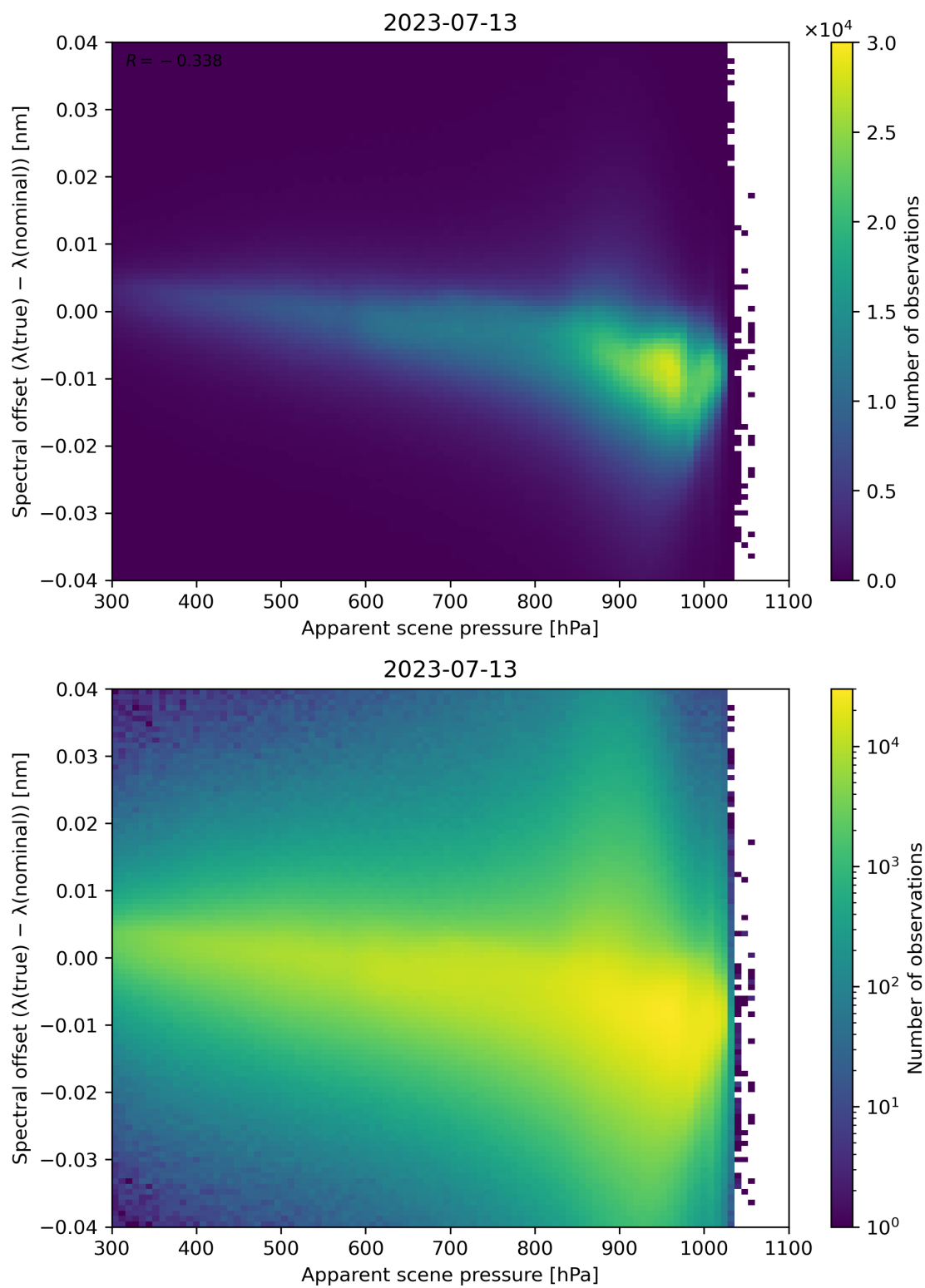
Figure 68: Scatter density plot of “Apparent scene pressure” against “Spectral offset ( \lambda(\text{true}) - \lambda(\text{nominal}) )” for 2023-07-13 to 2023-07-14.
