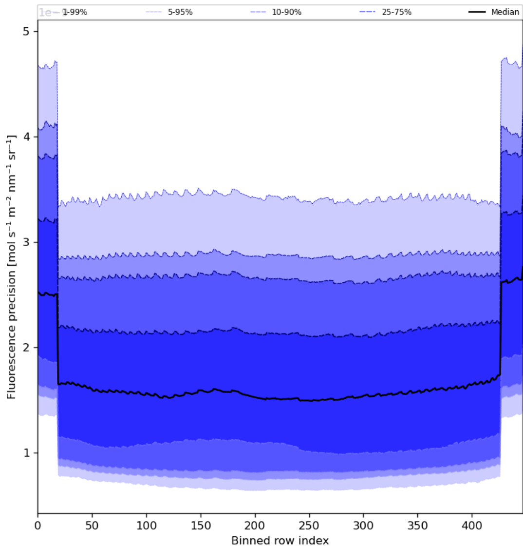
Figure 58: Along track statistics of “Fluorescence precision” for 2023-07-13 to 2023-07-14
