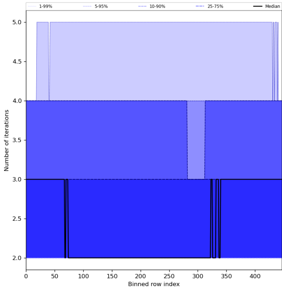
Figure 56: Along track statistics of “Number of iterations” for 2023-07-13 to 2023-07-14
