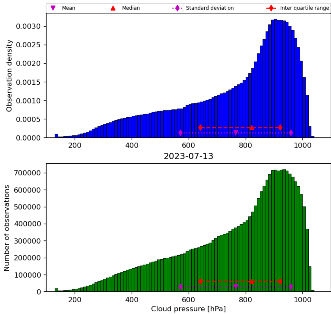
Figure 30: Histogram of “Cloud pressure” for 2023-07-13 to 2023-07-14
