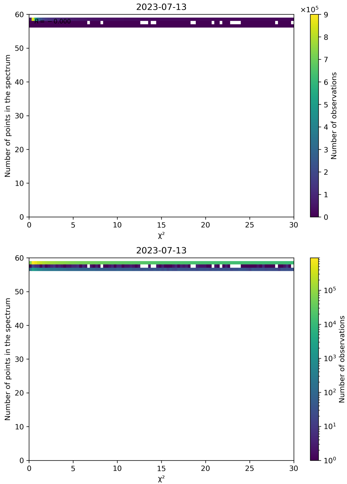
Figure 74: Scatter density plot of " \chi^2 " against "Number of points in the spectrum" for 2023-07-13 to 2023-07-14.
