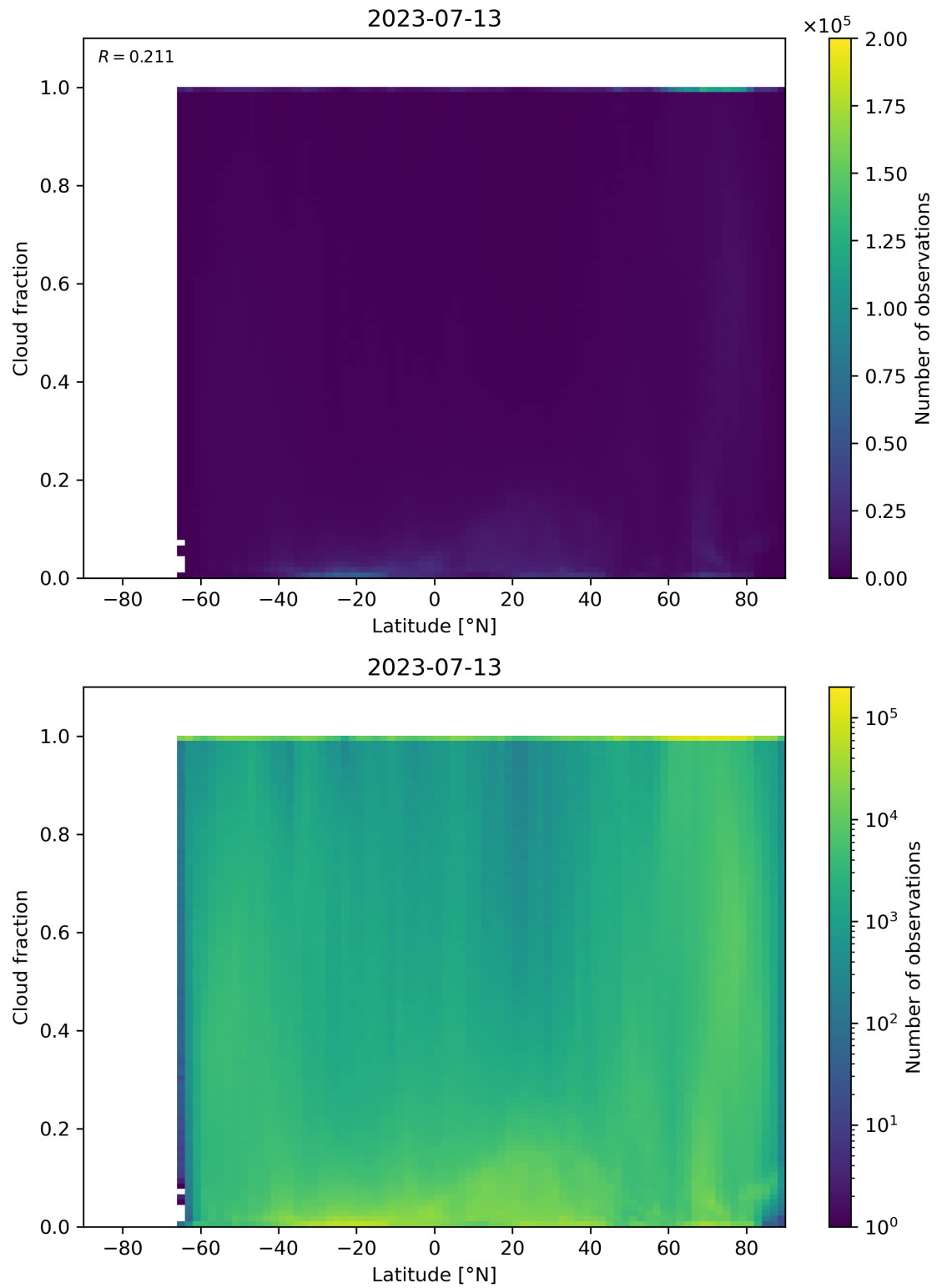
Figure 99: Scatter density plot of “Latitude” against “Cloud fraction” for 2023-07-13 to 2023-07-14.
