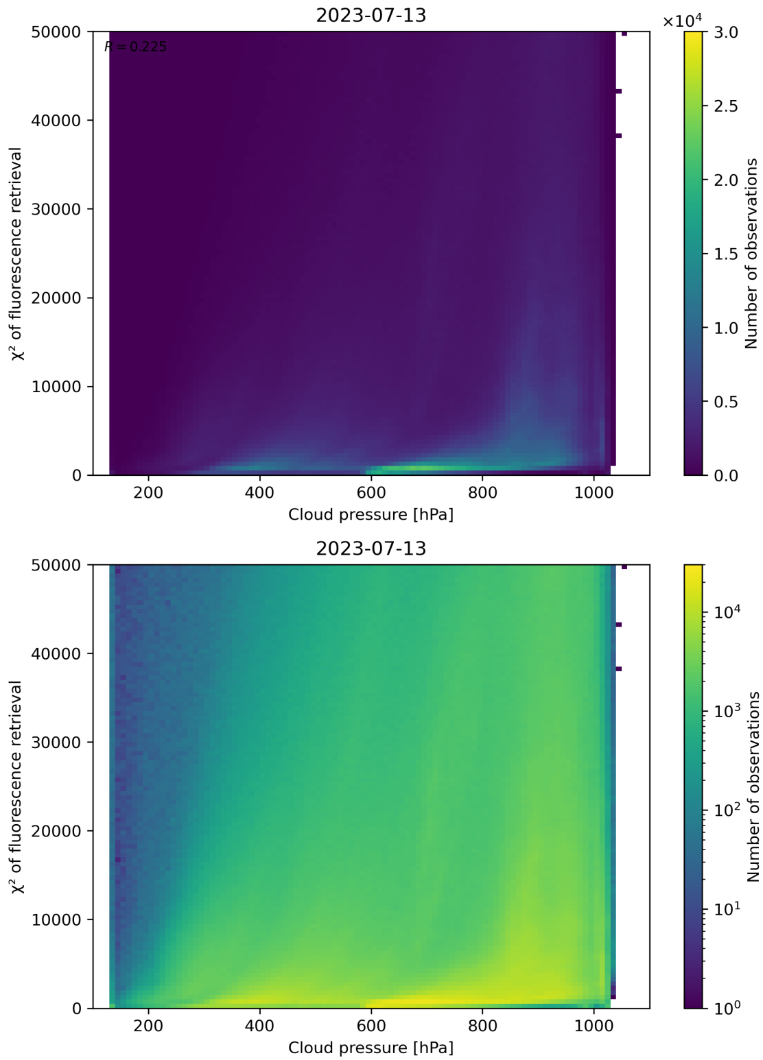
Figure 86: Scatter density plot of “Cloud pressure” against “ \chi^2 of fluorescence retrieval” for 2023-07-13 to 2023-07-14.
