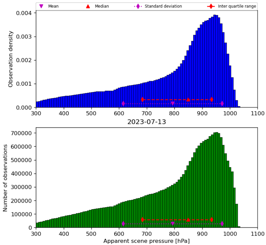
Figure 36: Histogram of “Apparent scene pressure” for 2023-07-13 to 2023-07-14
