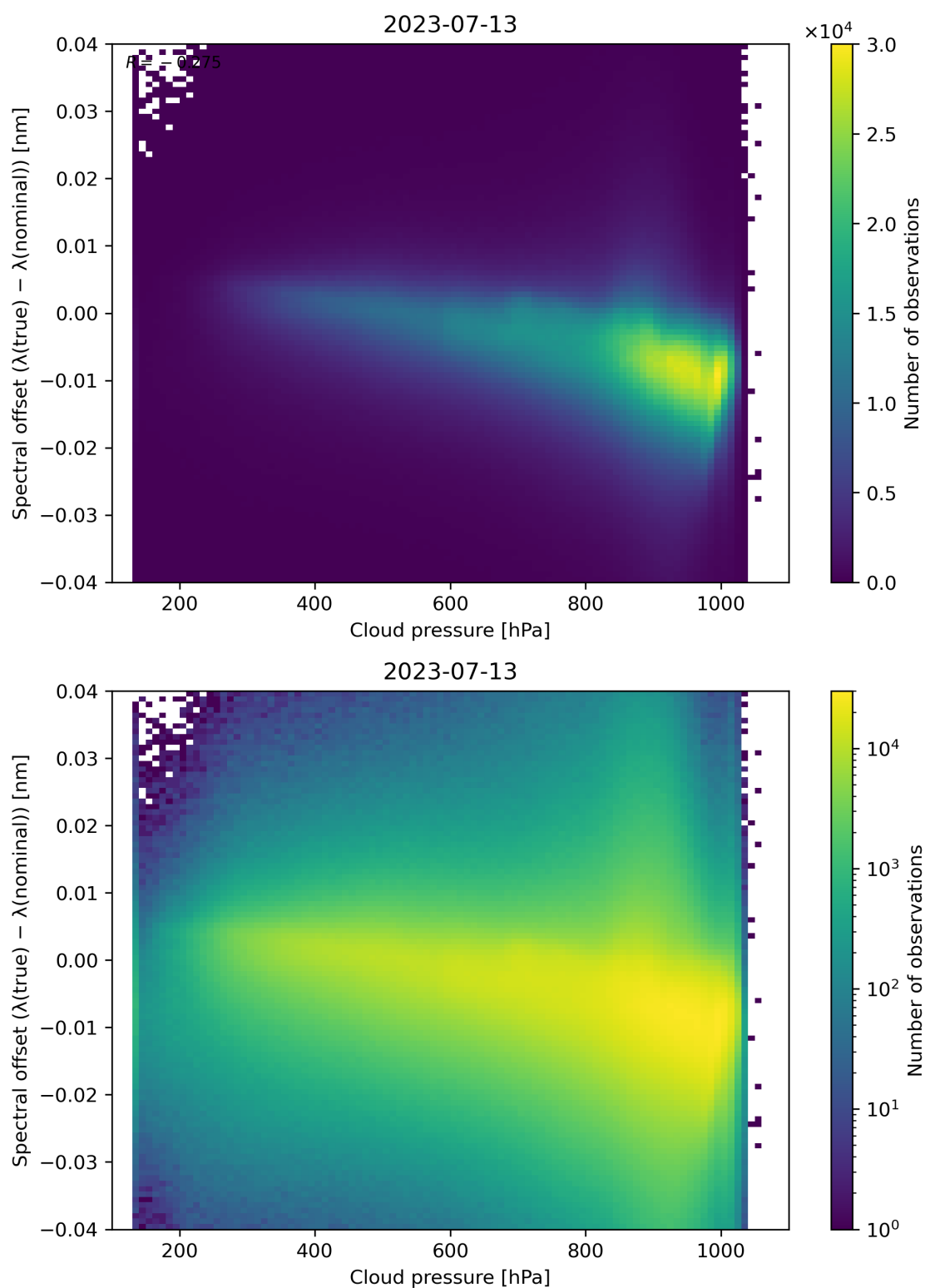
Figure 92: Scatter density plot of “Cloud pressure” against “Spectral offset ( \lambda(\text{true}) - \lambda(\text{nominal}) )” for 2023-07-13 to 2023-07-14.
