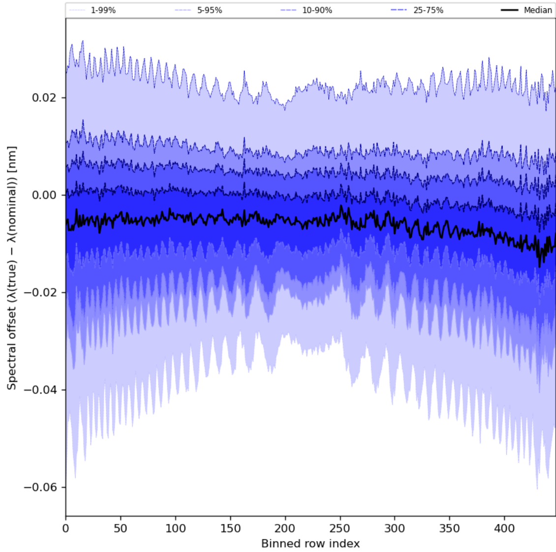
Figure 62: Along track statistics of “Spectral offset ( \lambda(\text{true}) - \lambda(\text{nominal}) )” for 2023-07-13 to 2023-07-14
