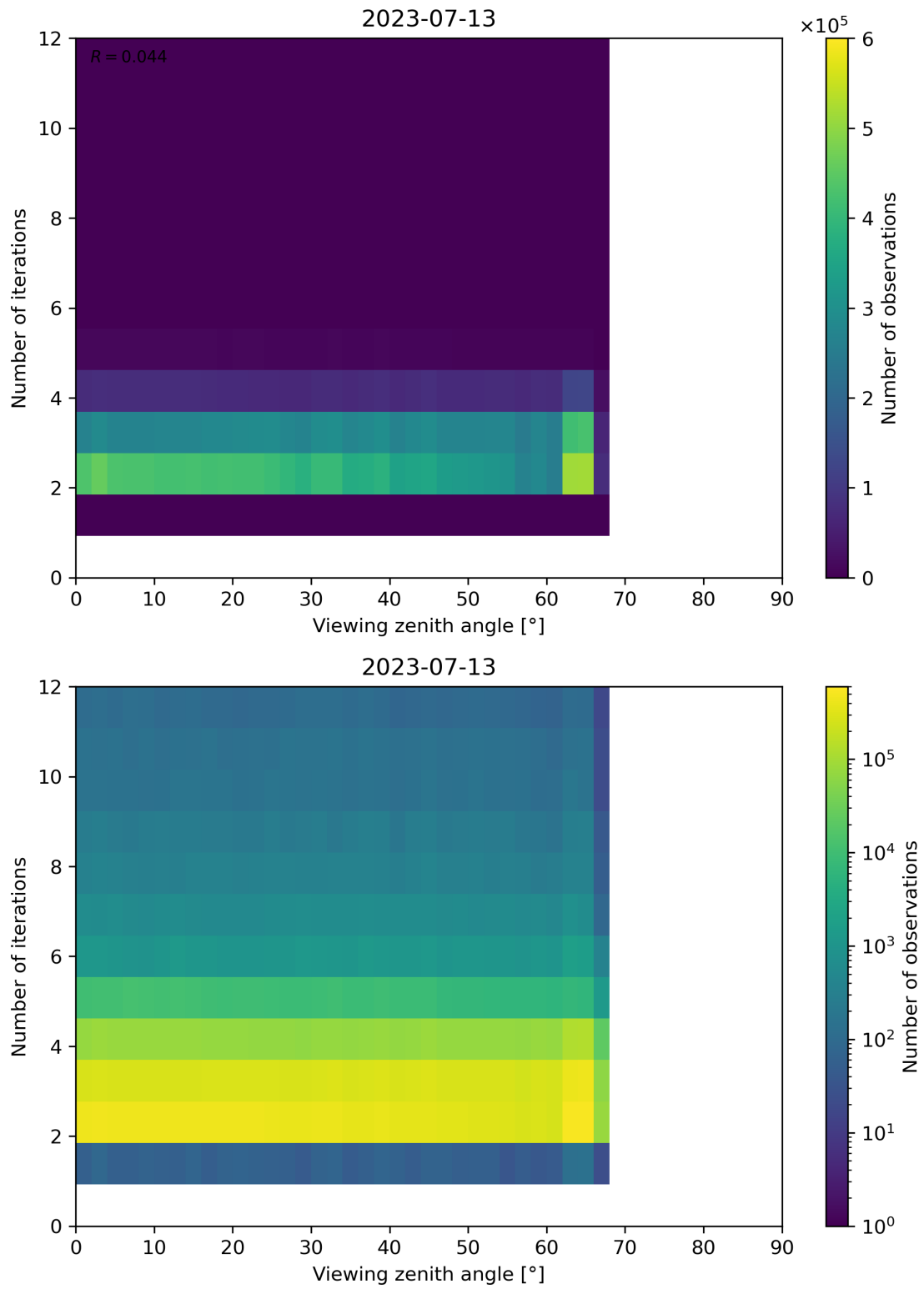
Figure 136: Scatter density plot of “Viewing zenith angle” against “Number of iterations” for 2023-07-13 to 2023-07-14.
