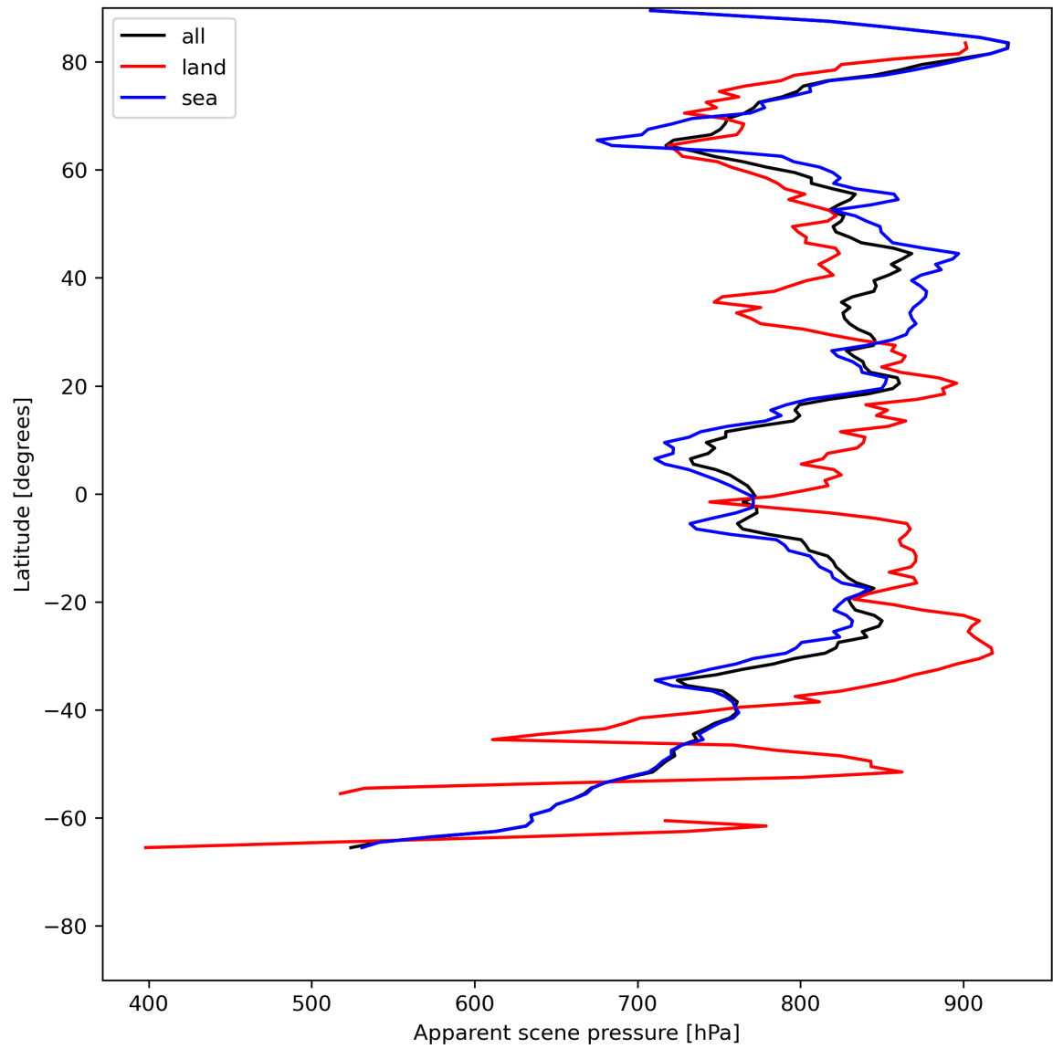
Figure 19: Zonal average of “Apparent scene pressure” for 2023-07-13 to 2023-07-14.
