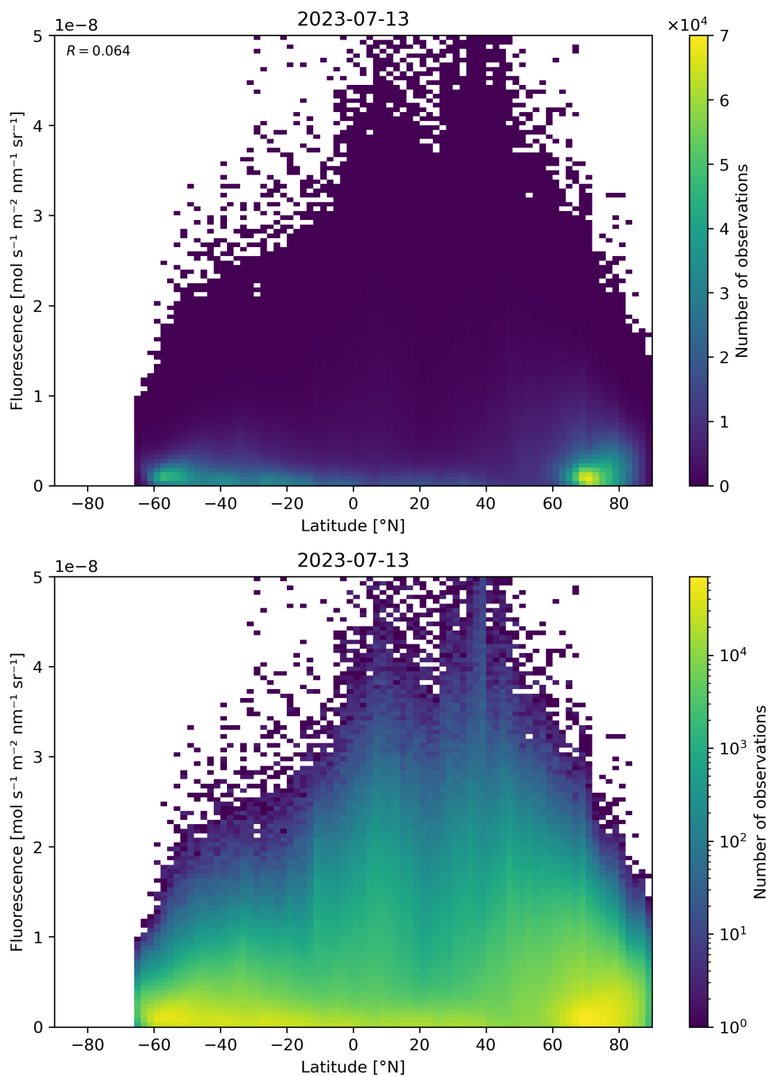
Figure 101: Scatter density plot of “Latitude” against “Fluorescence” for 2023-07-13 to 2023-07-14.
