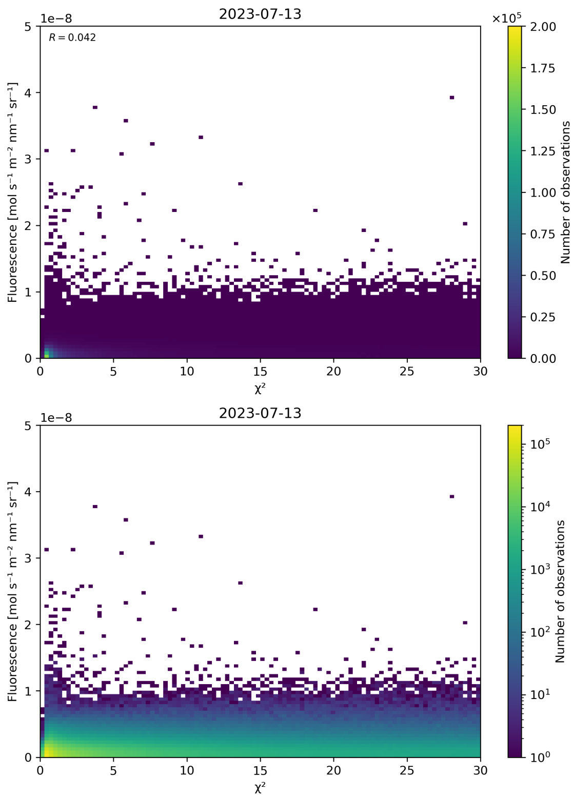
Figure 70: Scatter density plot of “ \chi^2 ” against “Fluorescence” for 2023-07-13 to 2023-07-14.
