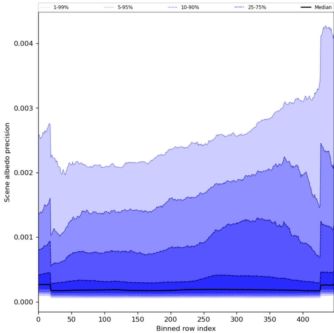
Figure 52: Along track statistics of “Scene albedo precision” for 2023-07-13 to 2023-07-14
