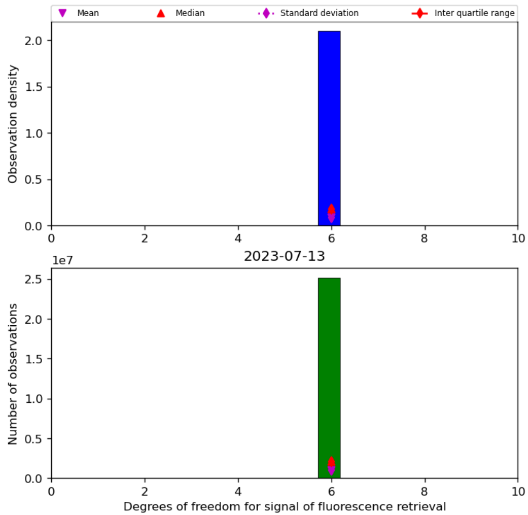
Figure 43: Histogram of “Degrees of freedom for signal of fluorescence retrieval” for 2023-07-13 to 2023-07-14
