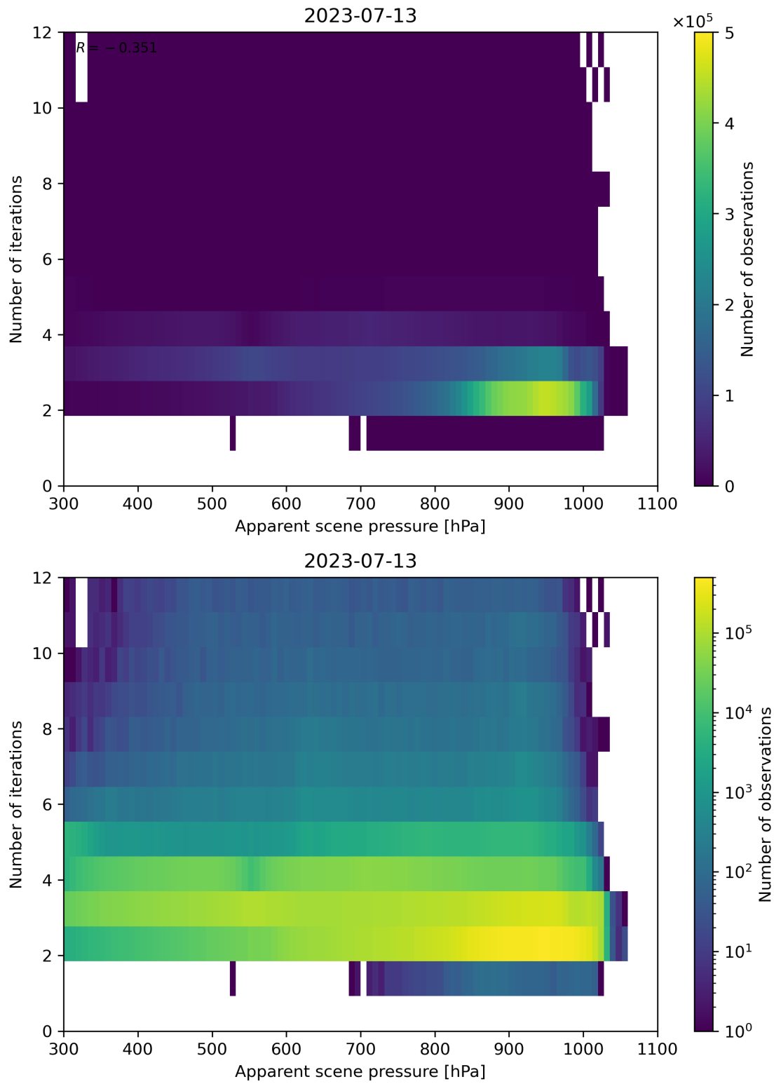
Figure 66: Scatter density plot of “Apparent scene pressure” against “Number of iterations” for 2023-07-13 to 2023-07-14.
