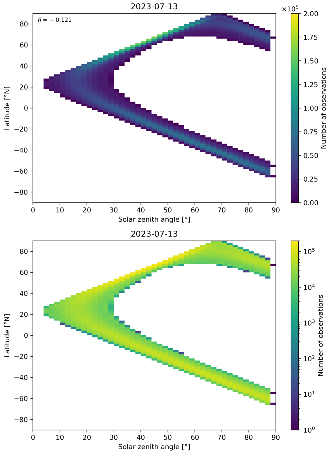
Figure 124: Scatter density plot of “Solar zenith angle” against “Latitude” for 2023-07-13 to 2023-07-14.
