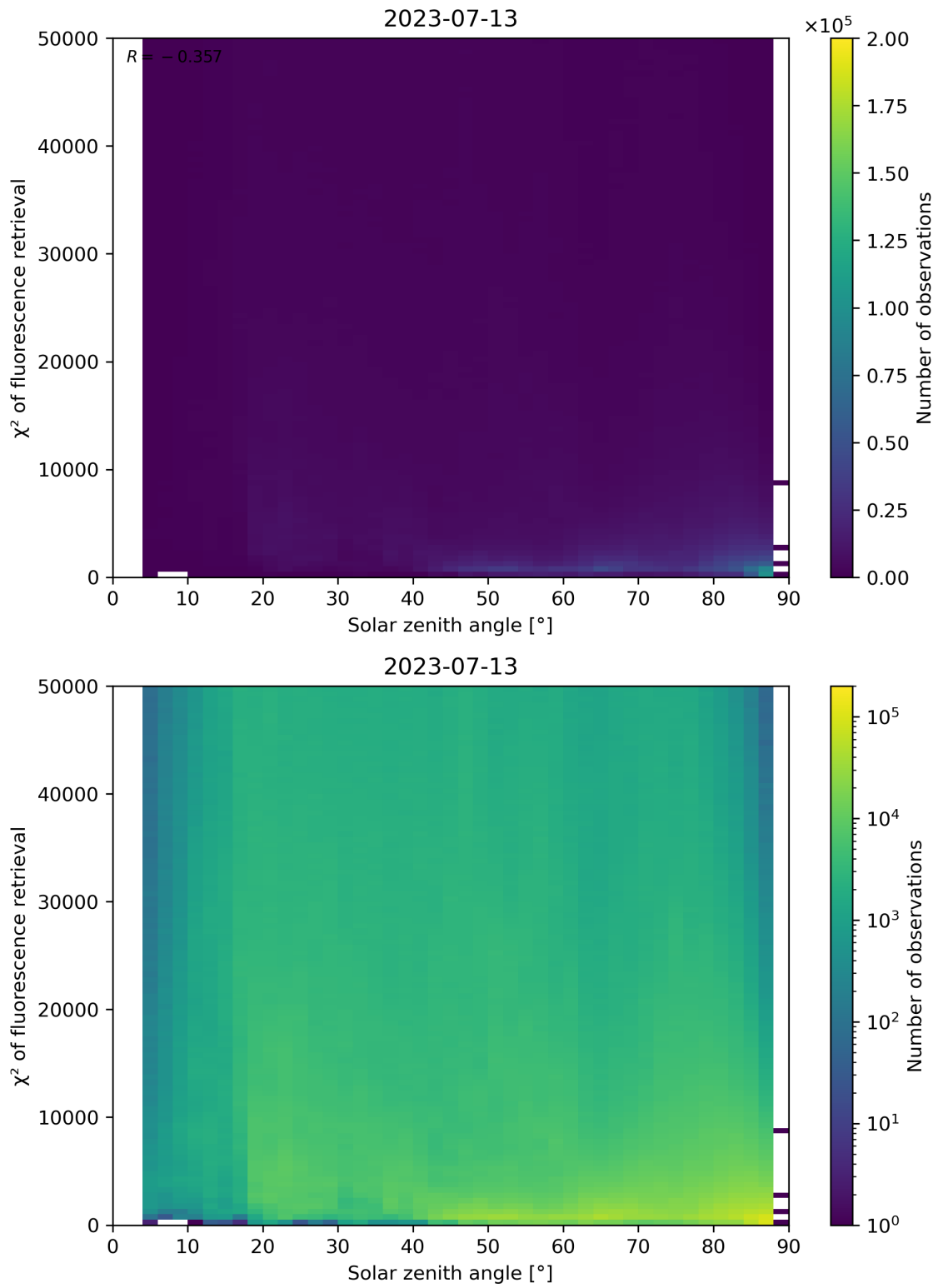
Figure 120: Scatter density plot of “Solar zenith angle” against “ \chi^2 of fluorescence retrieval” for 2023-07-13 to 2023-07-14.
