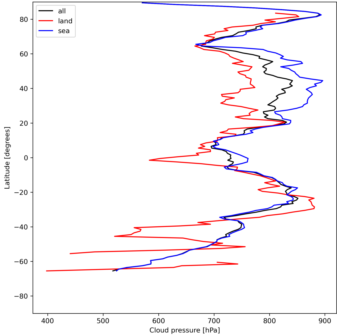
Figure 13: Zonal average of “Cloud pressure” for 2023-07-13 to 2023-07-14.
