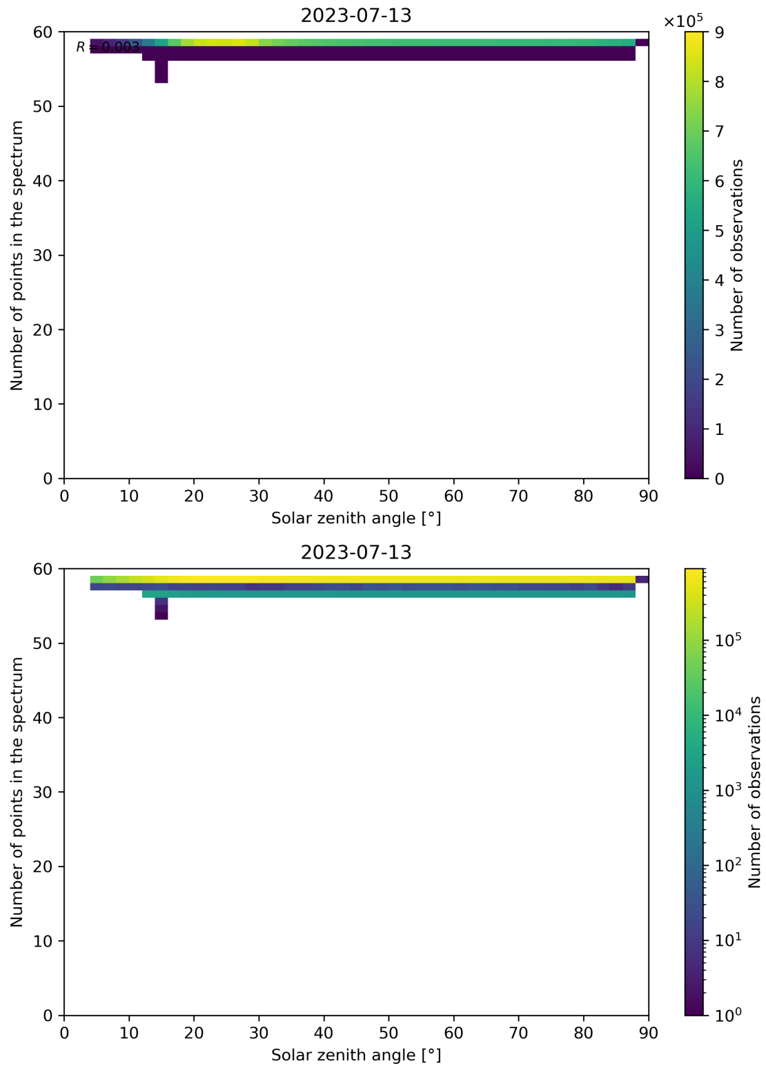
Figure 126: Scatter density plot of “Solar zenith angle” against “Number of points in the spectrum” for 2023-07-13 to 2023-07-14.
