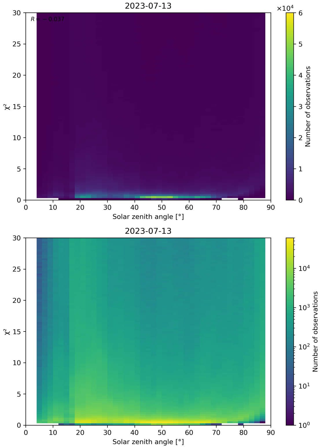
Figure 119: Scatter density plot of “Solar zenith angle” against “ \chi^2 ” for 2023-07-13 to 2023-07-14.
