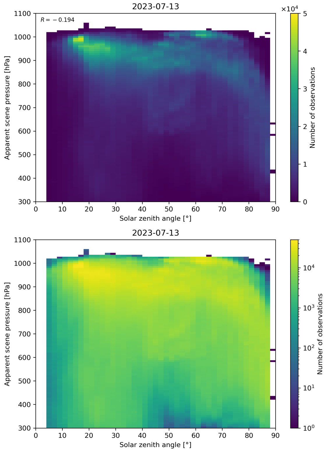
Figure 118: Scatter density plot of “Solar zenith angle” against “Apparent scene pressure” for 2023-07-13 to 2023-07-14.
