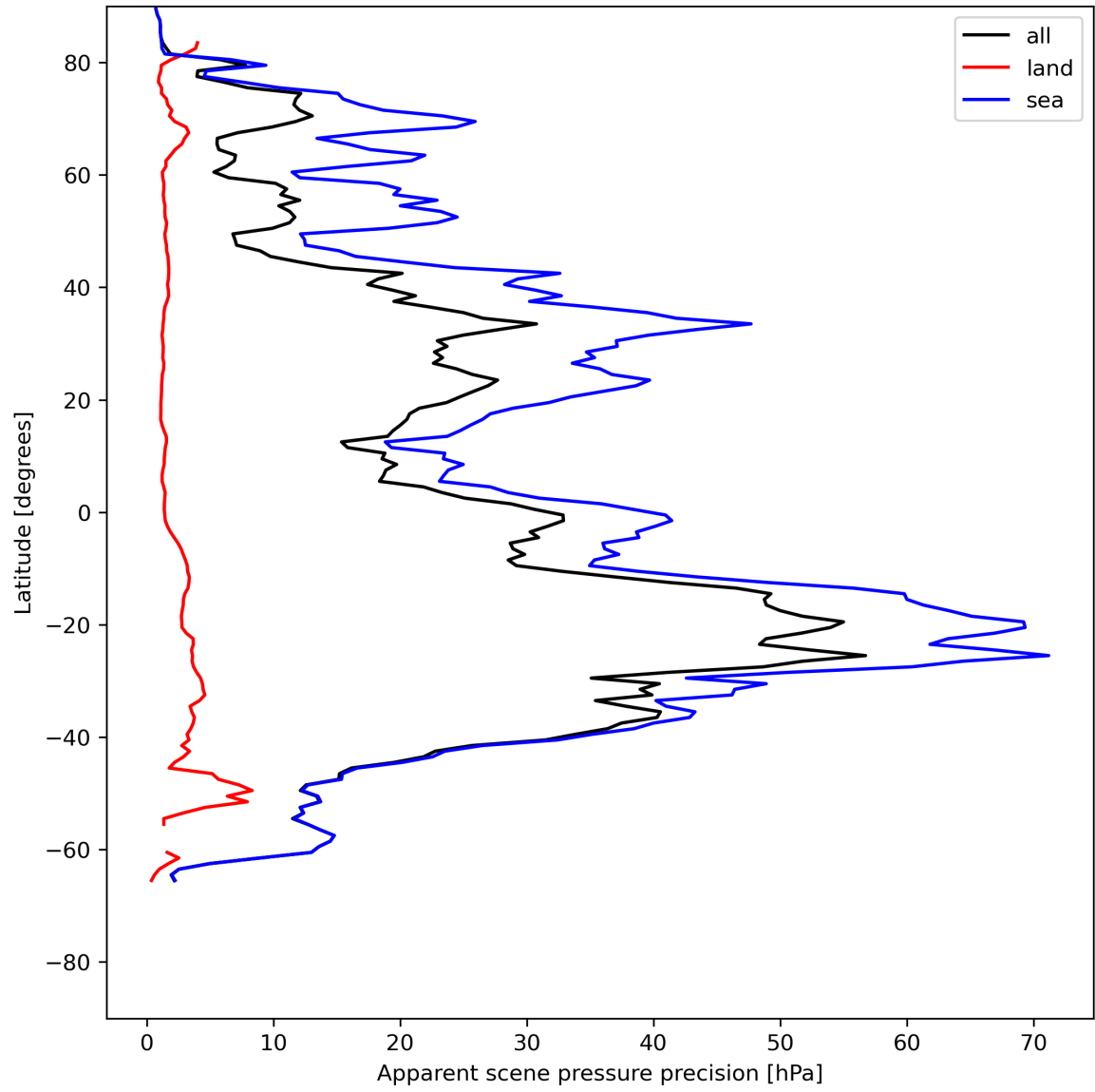
Figure 20: Zonal average of “Apparent scene pressure precision” for 2023-07-13 to 2023-07-14.
