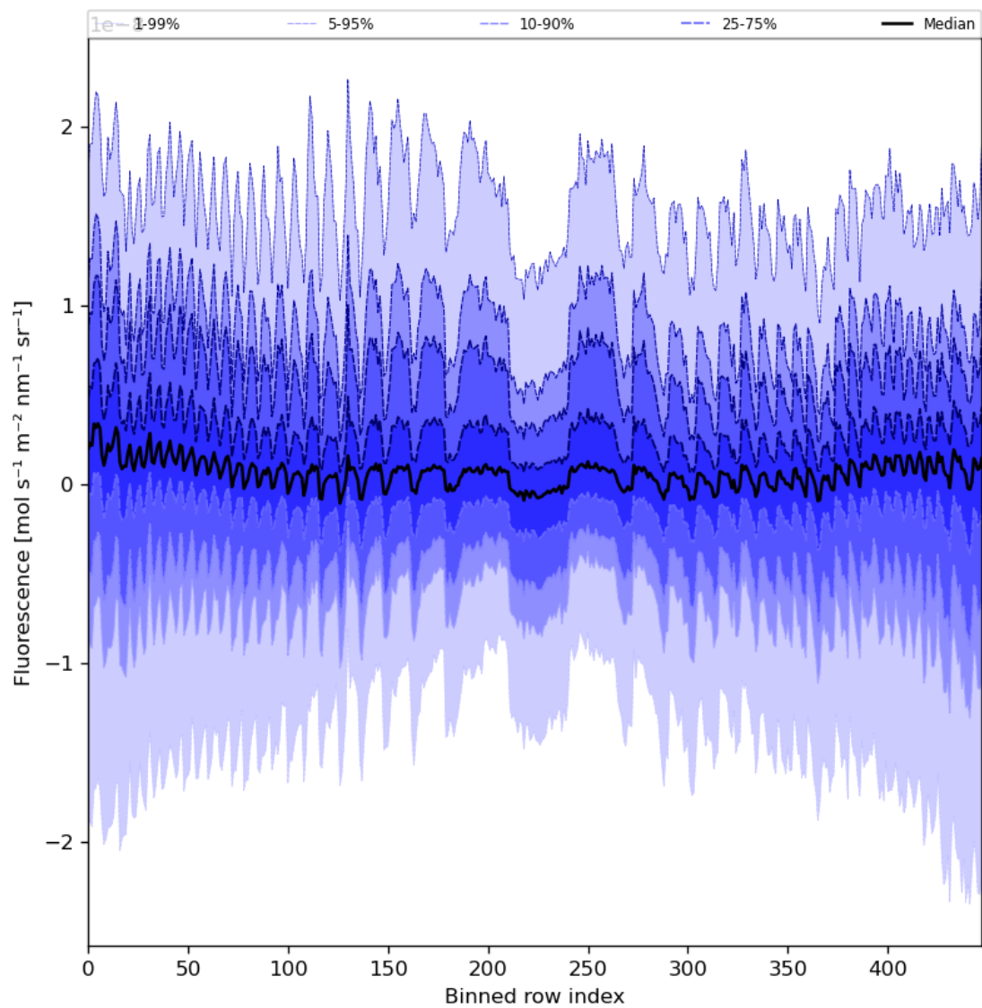
Figure 57: Along track statistics of “Fluorescence” for 2023-07-13 to 2023-07-14
