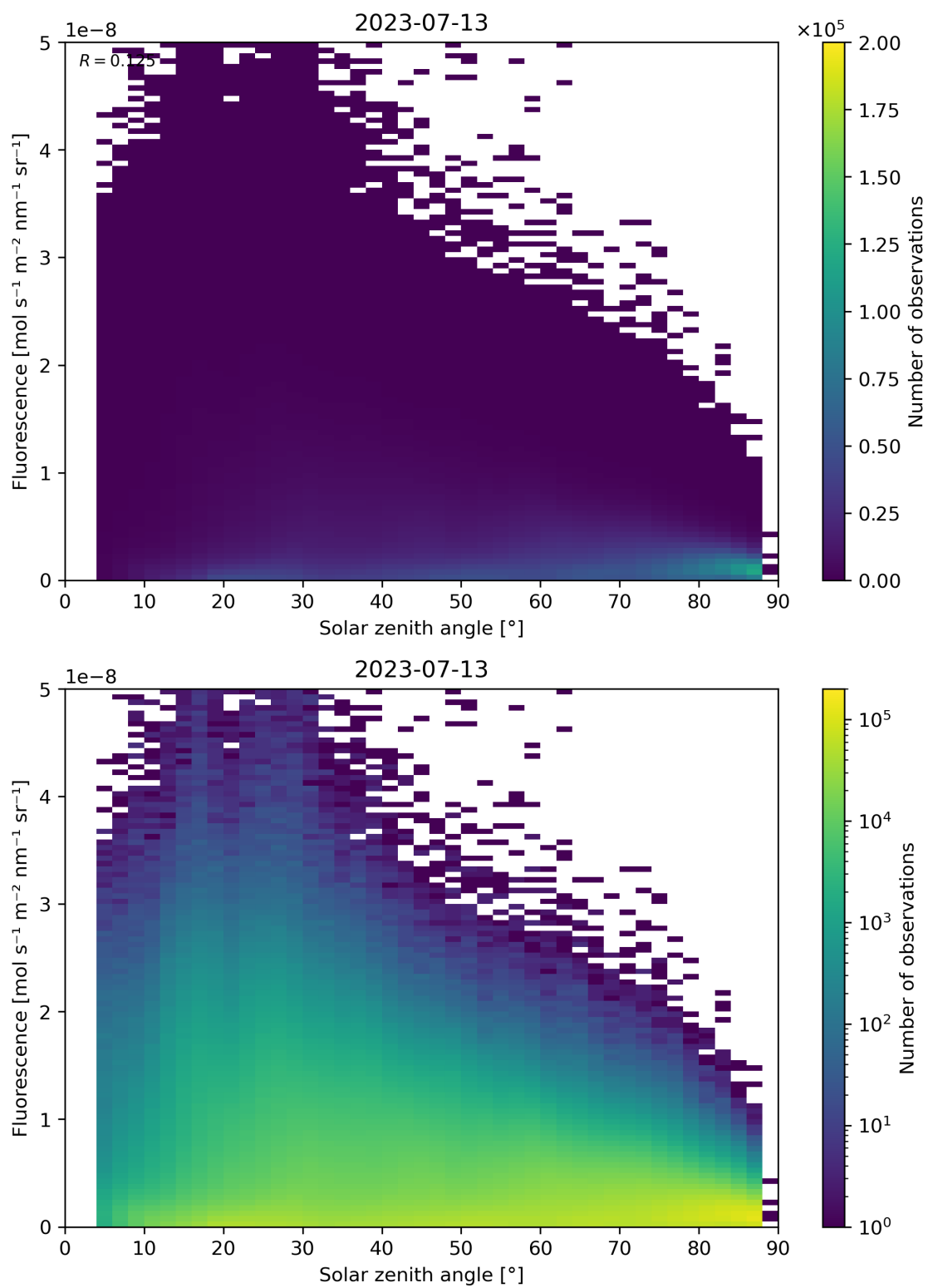
Figure 123: Scatter density plot of “Solar zenith angle” against “Fluorescence” for 2023-07-13 to 2023-07-14.
