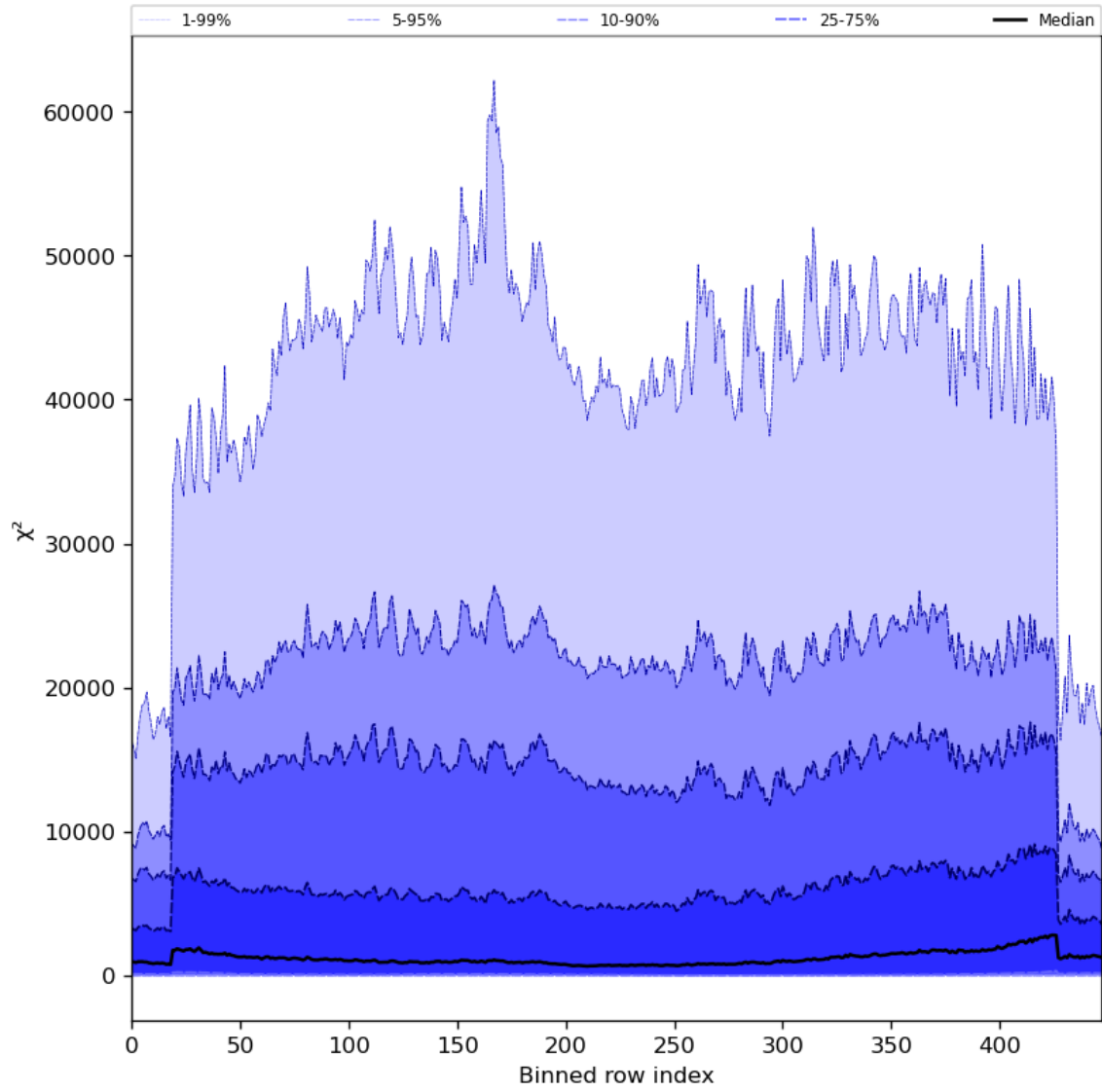
Figure 55: Along track statistics of “ \chi^2 ” for 2023-07-13 to 2023-07-14
