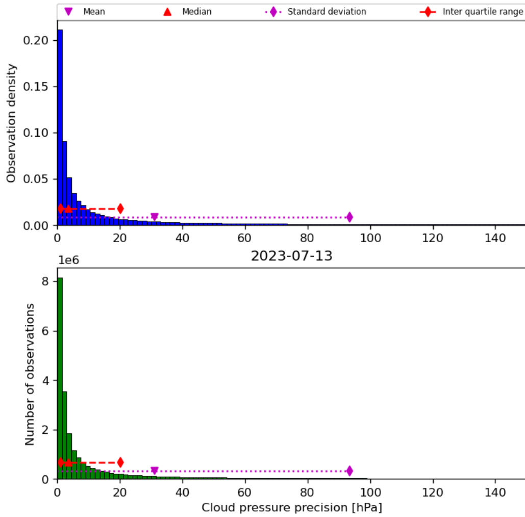
Figure 31: Histogram of “Cloud pressure precision” for 2023-07-13 to 2023-07-14
