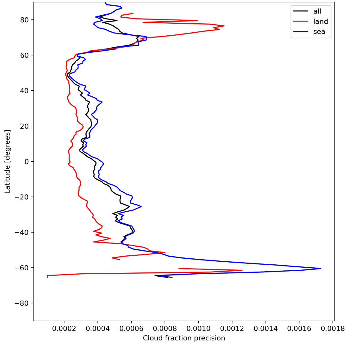
Figure 16: Zonal average of “Cloud fraction precision” for 2023-07-13 to 2023-07-14.
