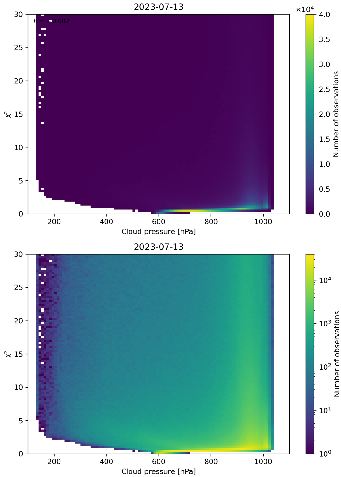
Figure 85: Scatter density plot of “Cloud pressure” against “ \chi^2 ” for 2023-07-13 to 2023-07-14.
