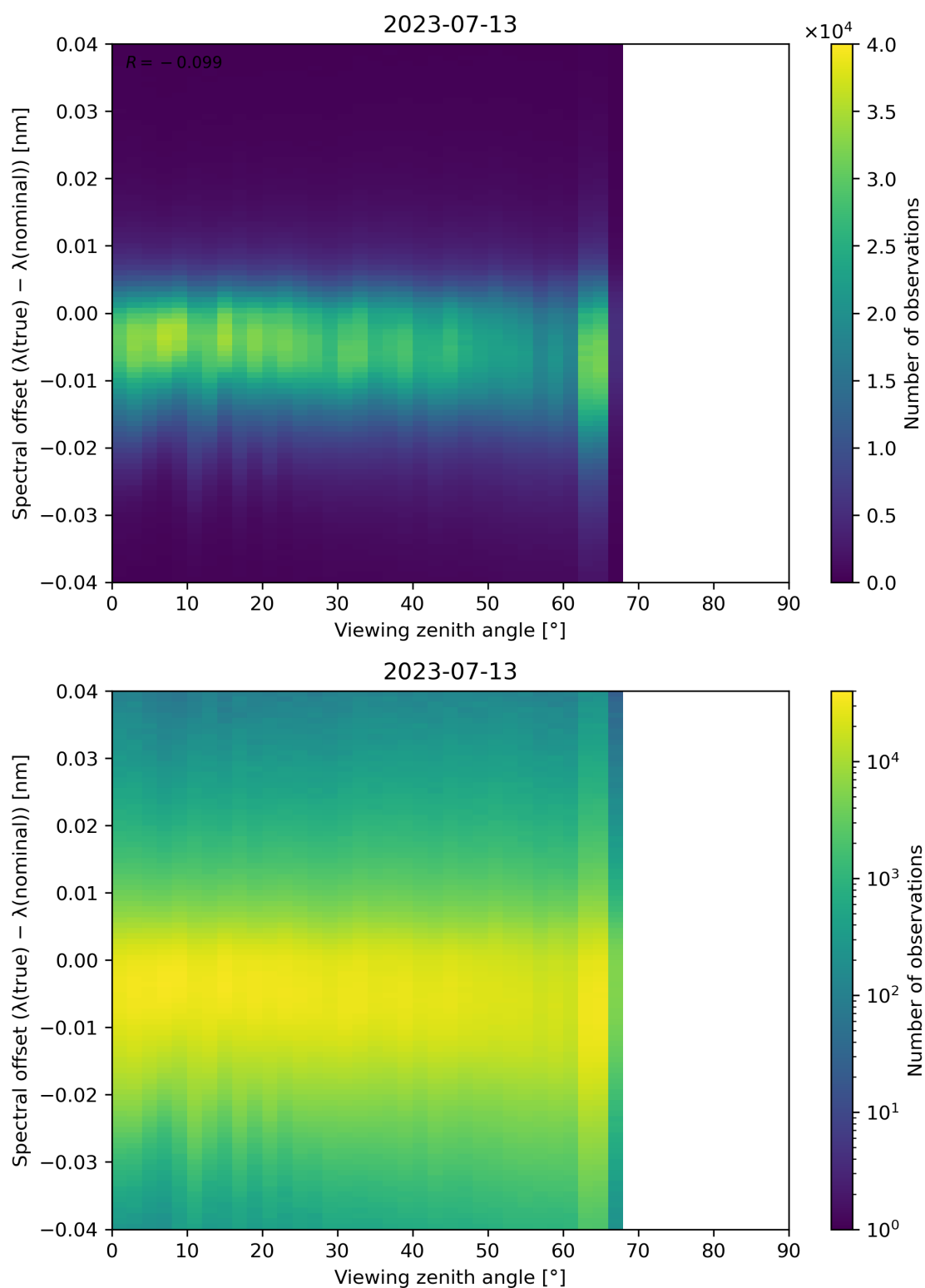
Figure 140: Scatter density plot of “Viewing zenith angle” against “Spectral offset ( \lambda(\text{true}) - \lambda(\text{nominal}) )” for 2023-07-13 to 2023-07-14.
