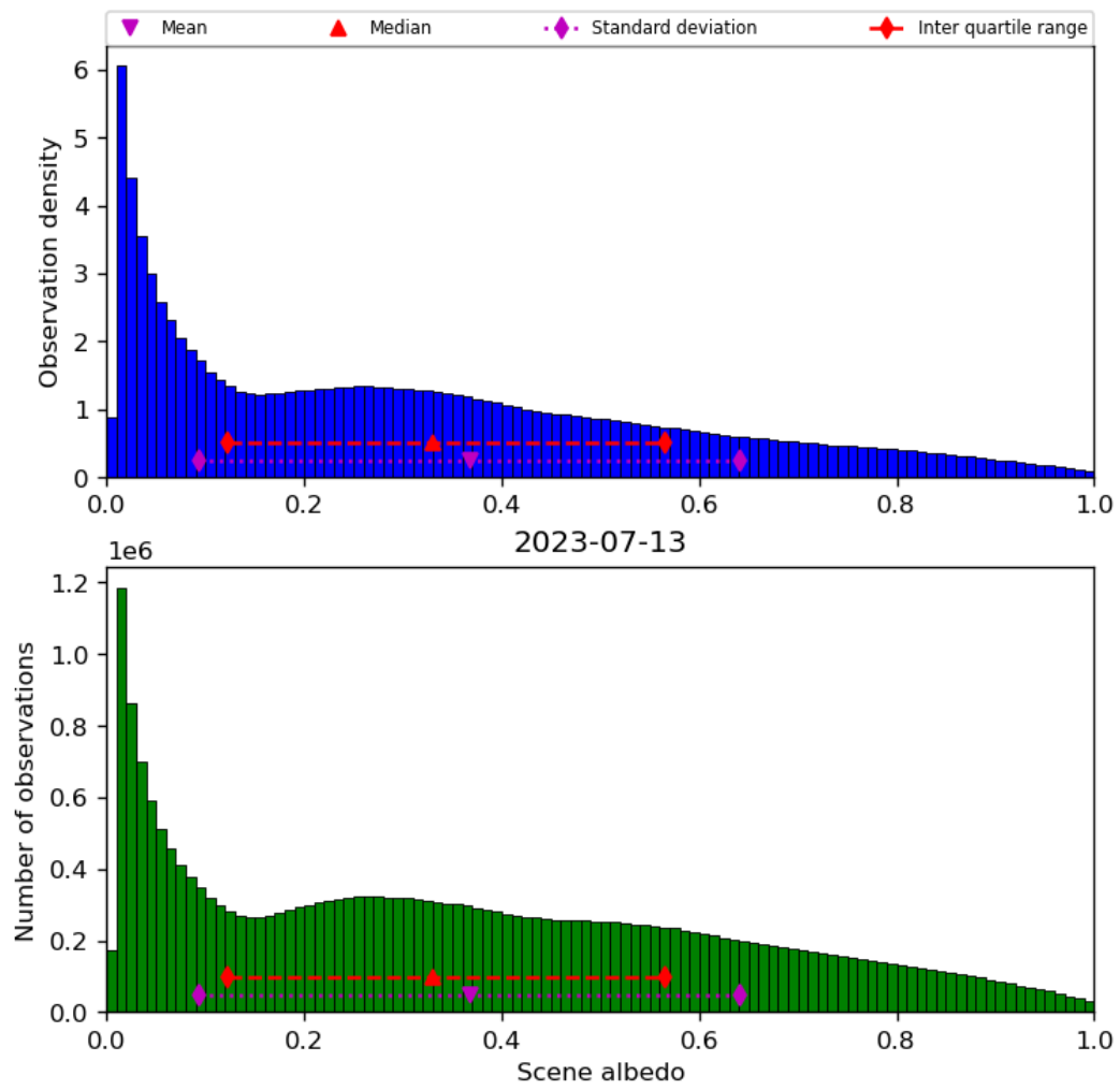
Figure 34: Histogram of “Scene albedo” for 2023-07-13 to 2023-07-14
