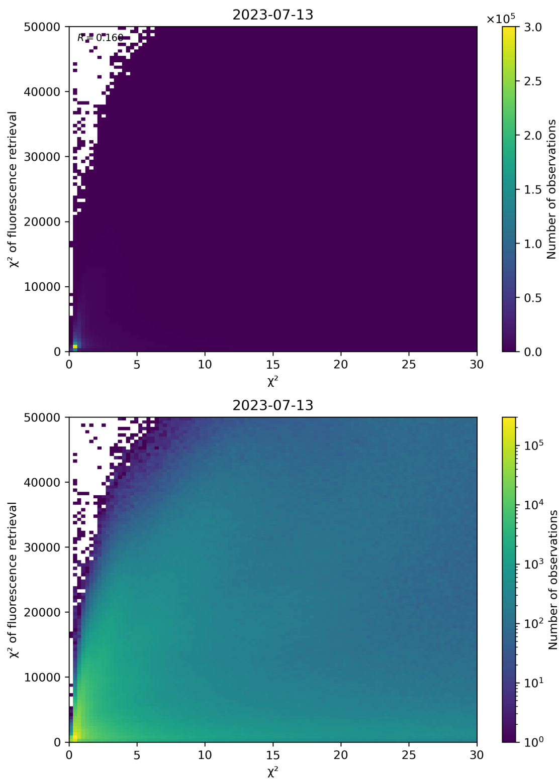
Figure 69: Scatter density plot of “ \chi^2 ” against “ \chi^2 of fluorescence retrieval” for 2023-07-13 to 2023-07-14.
