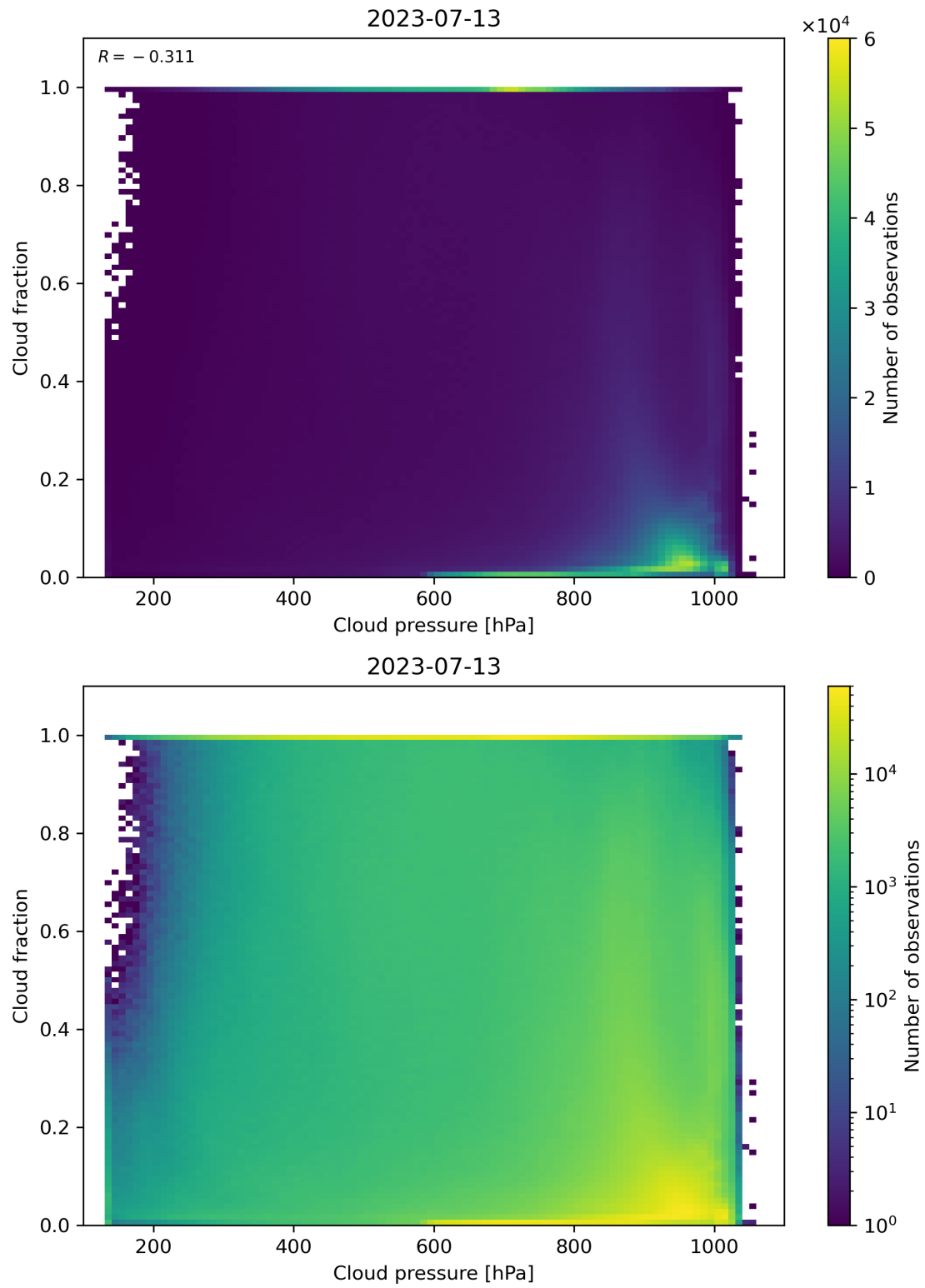
Figure 87: Scatter density plot of “Cloud pressure” against “Cloud fraction” for 2023-07-13 to 2023-07-14.
