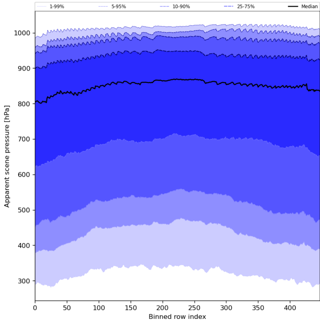
Figure 53: Along track statistics of “Apparent scene pressure” for 2023-07-13 to 2023-07-14
