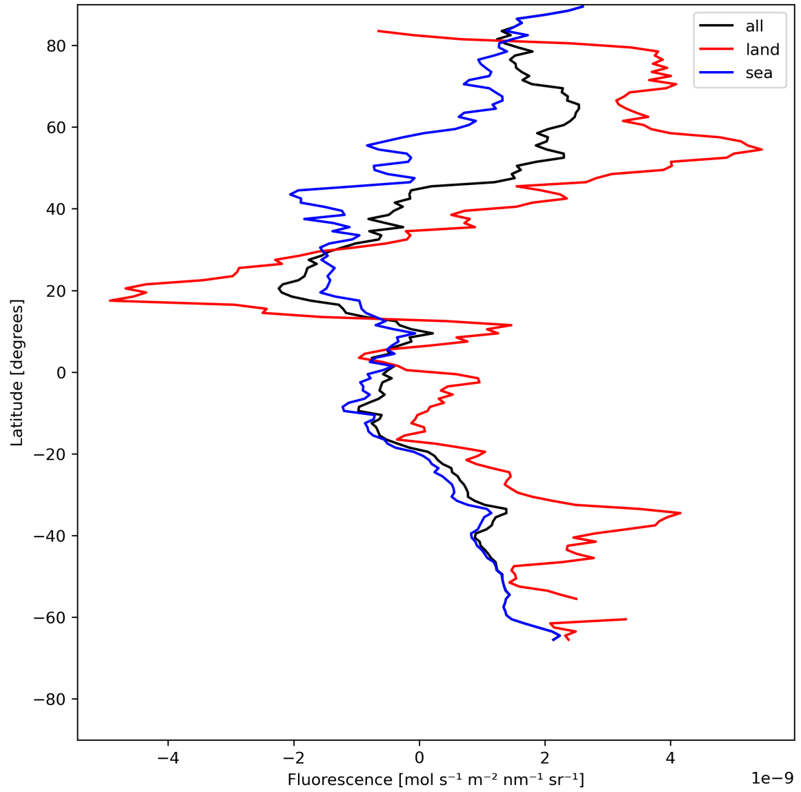
Figure 23: Zonal average of “Fluorescence” for 2023-07-13 to 2023-07-14.
