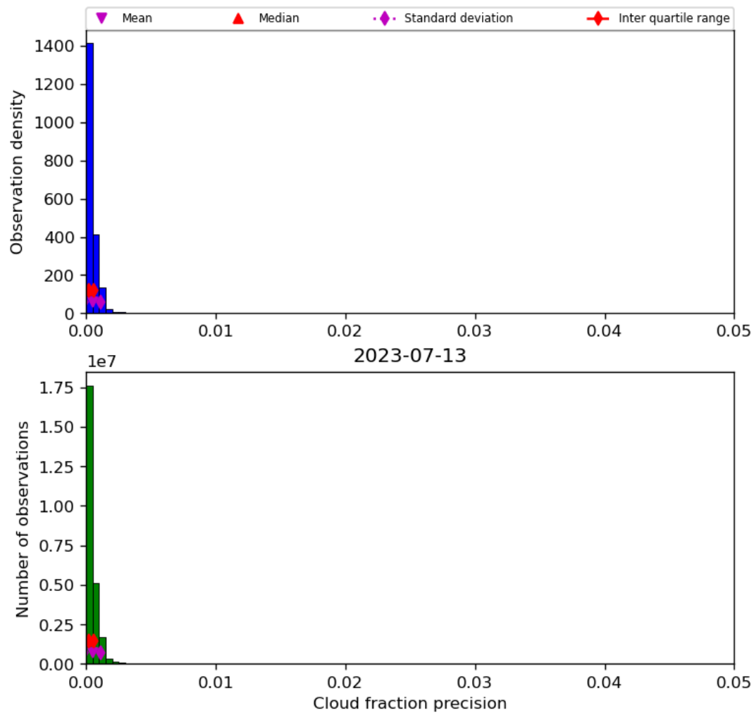
Figure 33: Histogram of “Cloud fraction precision” for 2023-07-13 to 2023-07-14
