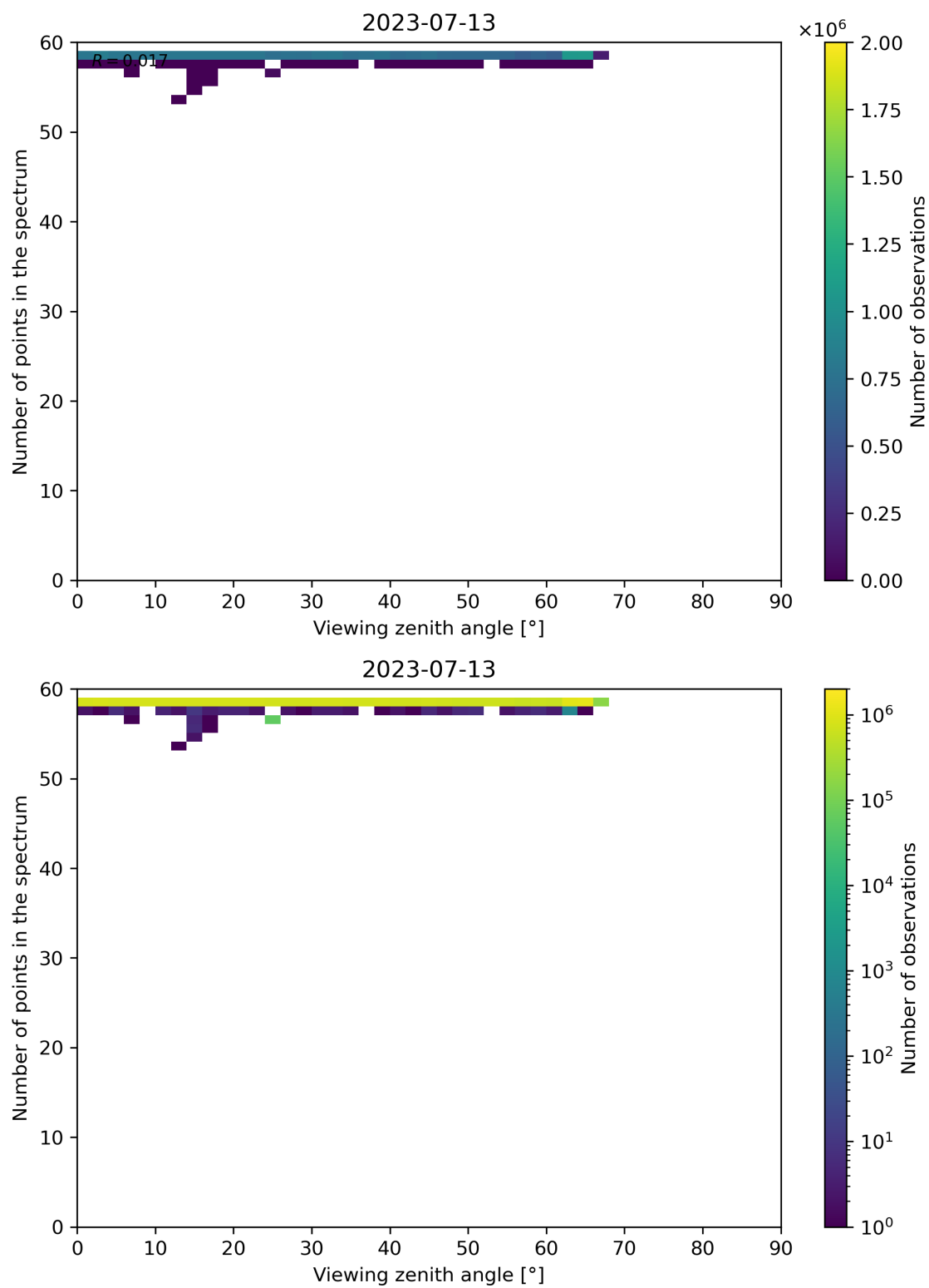
Figure 137: Scatter density plot of “Viewing zenith angle” against “Number of points in the spectrum” for 2023-07-13 to 2023-07-14.
