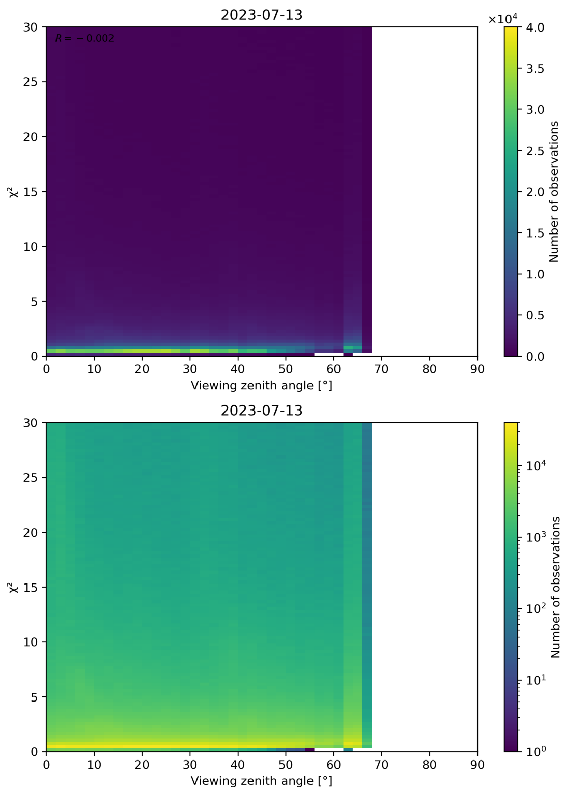
Figure 130: Scatter density plot of “Viewing zenith angle” against “ \chi^2 ” for 2023-07-13 to 2023-07-14.
