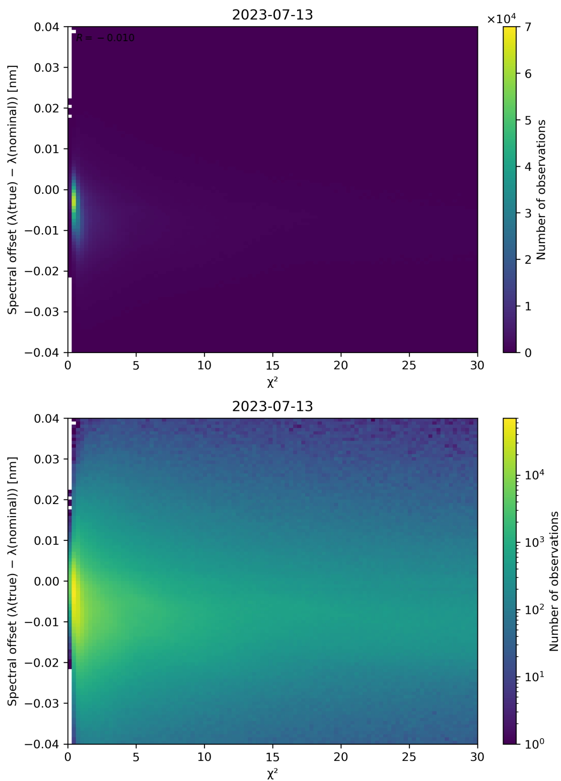
Figure 75: Scatter density plot of " \chi^2 " against "Spectral offset ( \lambda(\text{true}) - \lambda(\text{nominal})) " for 2023-07-13 to 2023-07-14.
