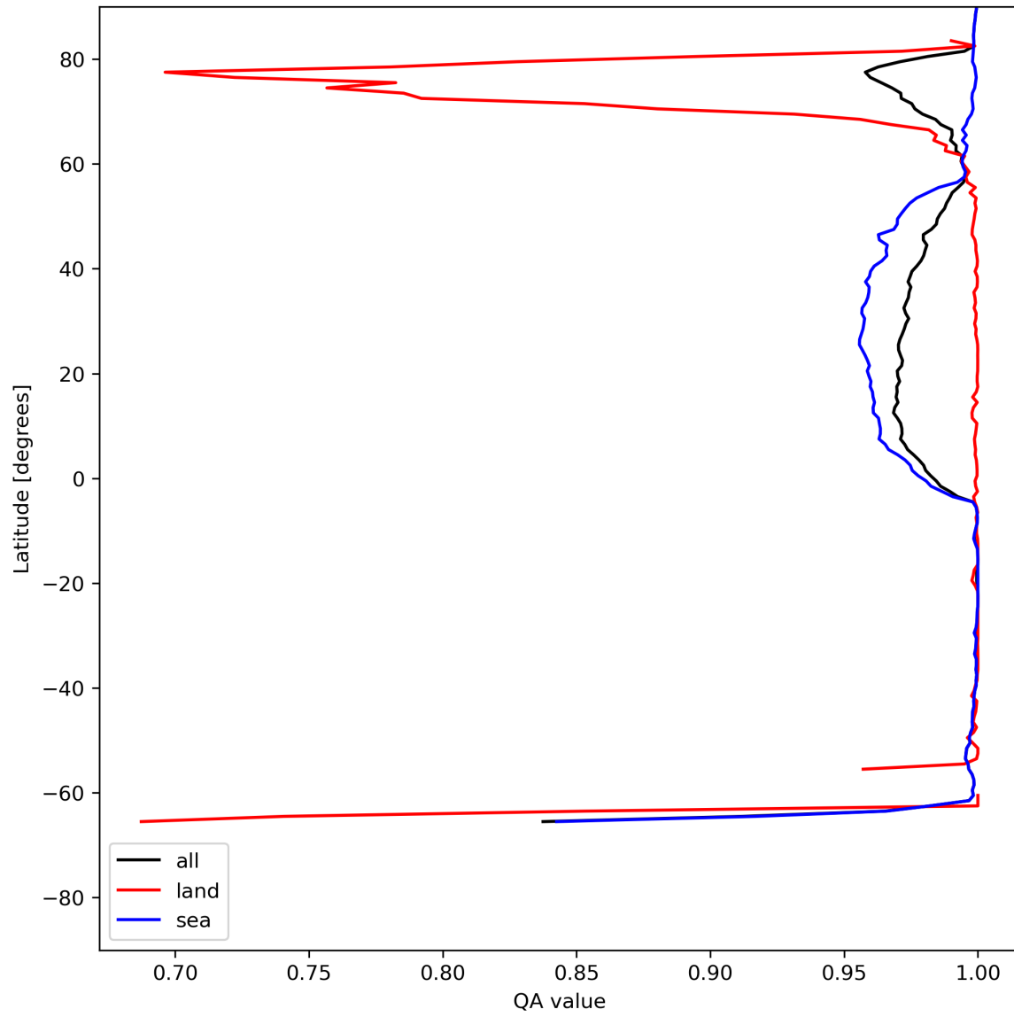
Figure 12: Zonal average of “QA value” for 2023-07-13 to 2023-07-14.
