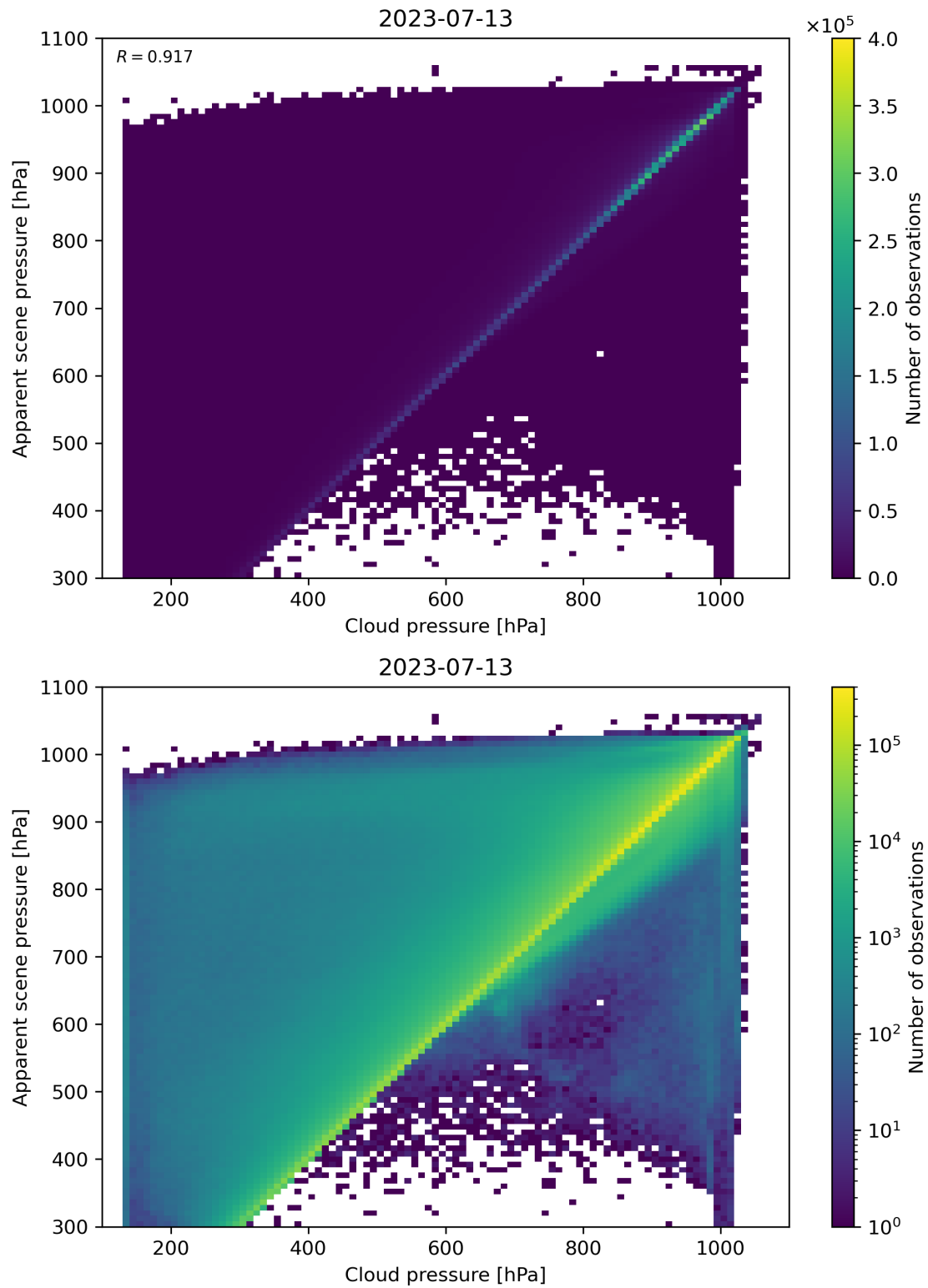
Figure 84: Scatter density plot of “Cloud pressure” against “Apparent scene pressure” for 2023-07-13 to 2023-07-14.
