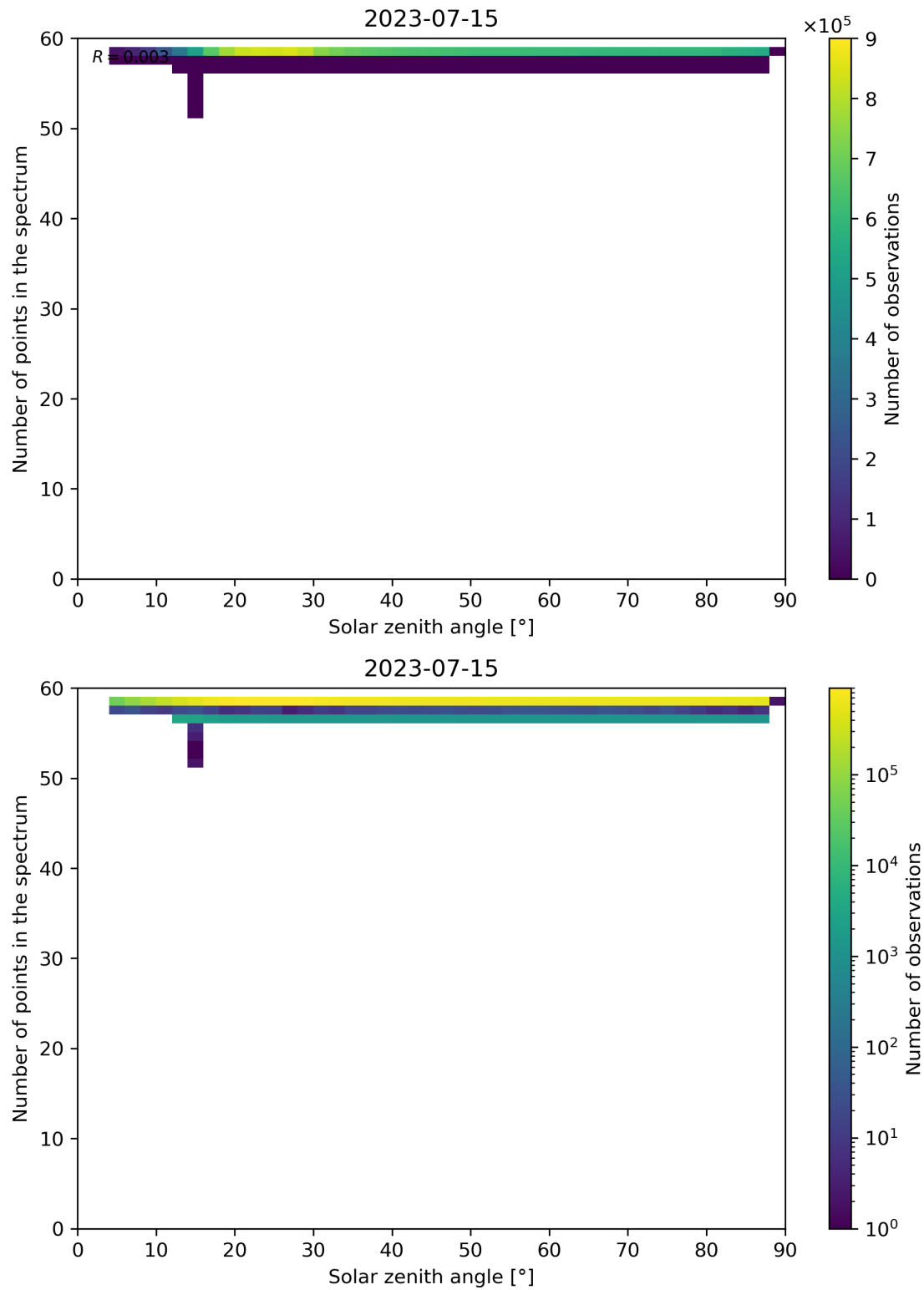
Figure 126: Scatter density plot of “Solar zenith angle” against “Number of points in the spectrum” for 2023-07-14 to 2023-07-16.
