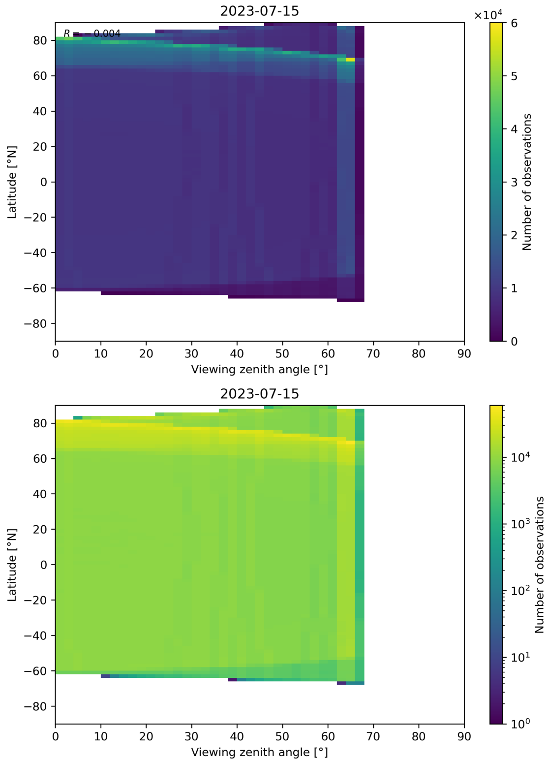
Figure 135: Scatter density plot of “Viewing zenith angle” against “Latitude” for 2023-07-14 to 2023-07-16.
