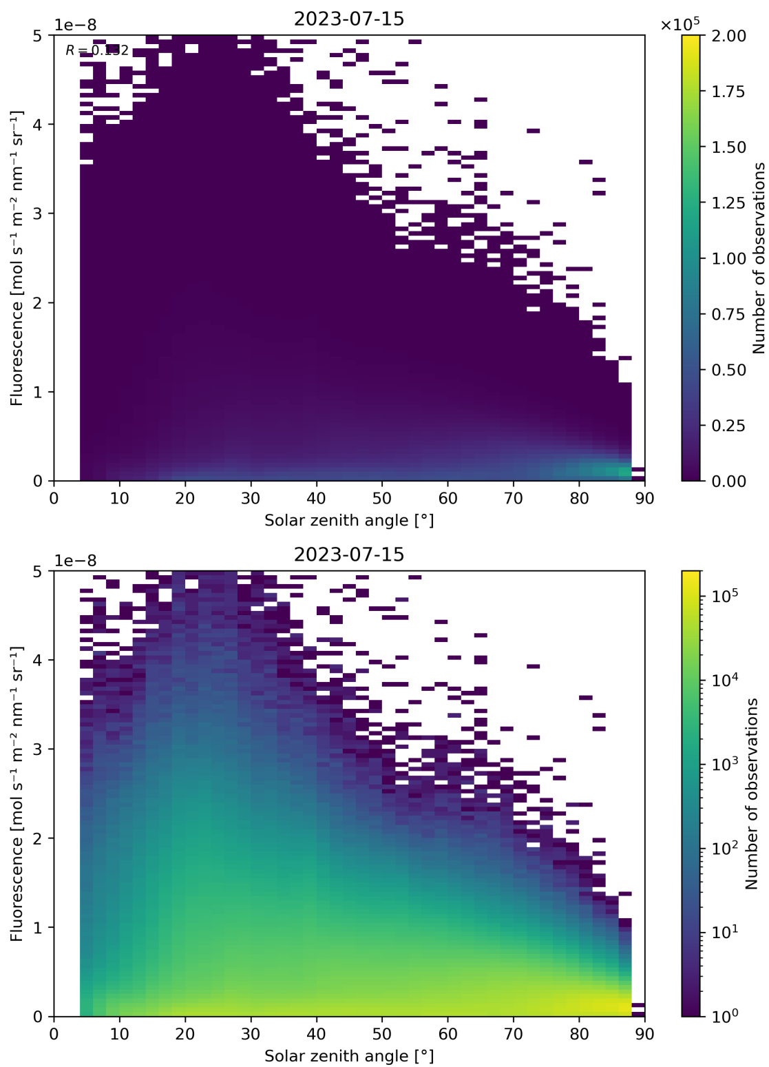
Figure 123: Scatter density plot of “Solar zenith angle” against “Fluorescence” for 2023-07-14 to 2023-07-16.
