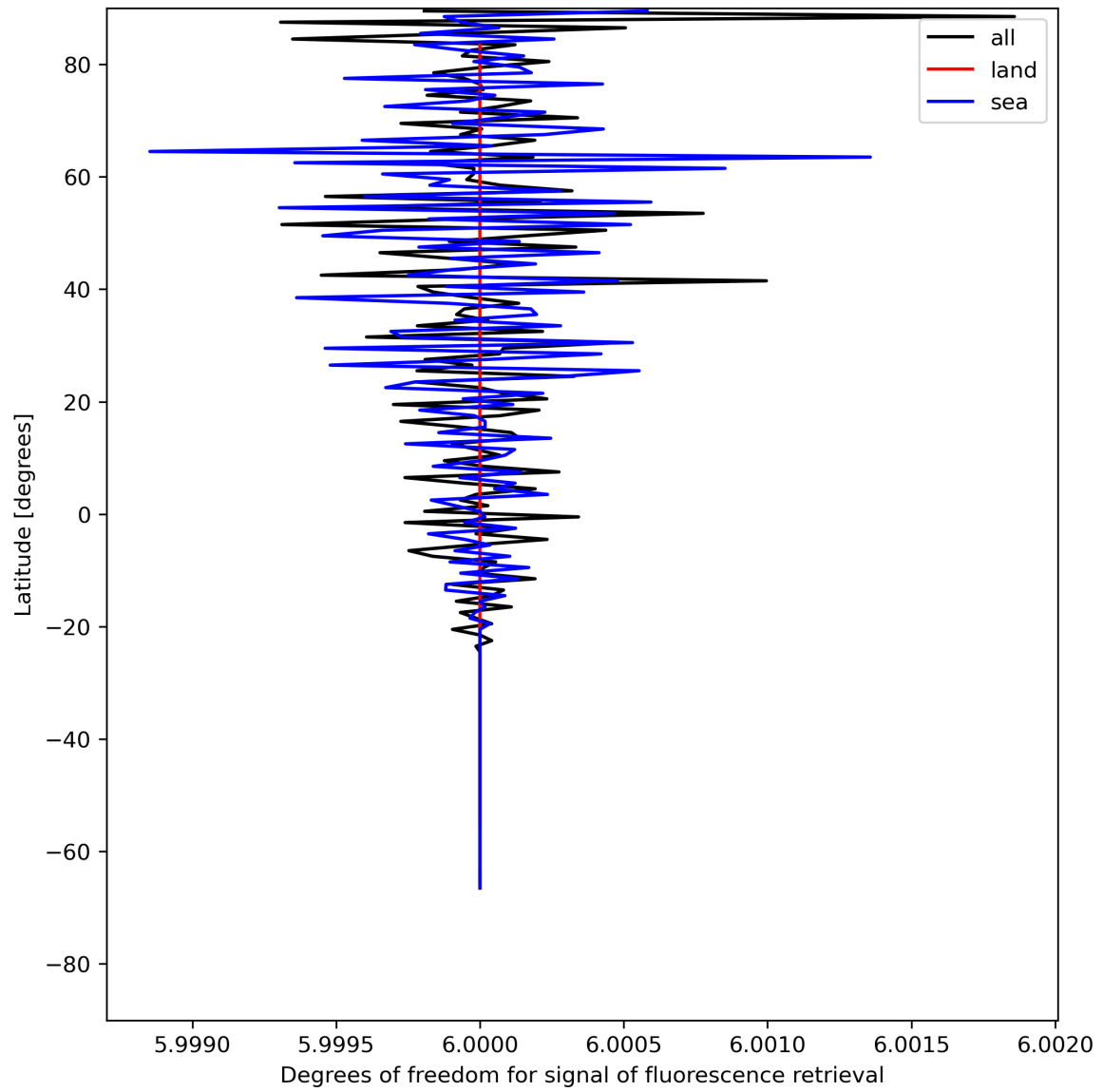
Figure 26: Zonal average of “Degrees of freedom for signal of fluorescence retrieval” for 2023-07-14 to 2023-07-16.
