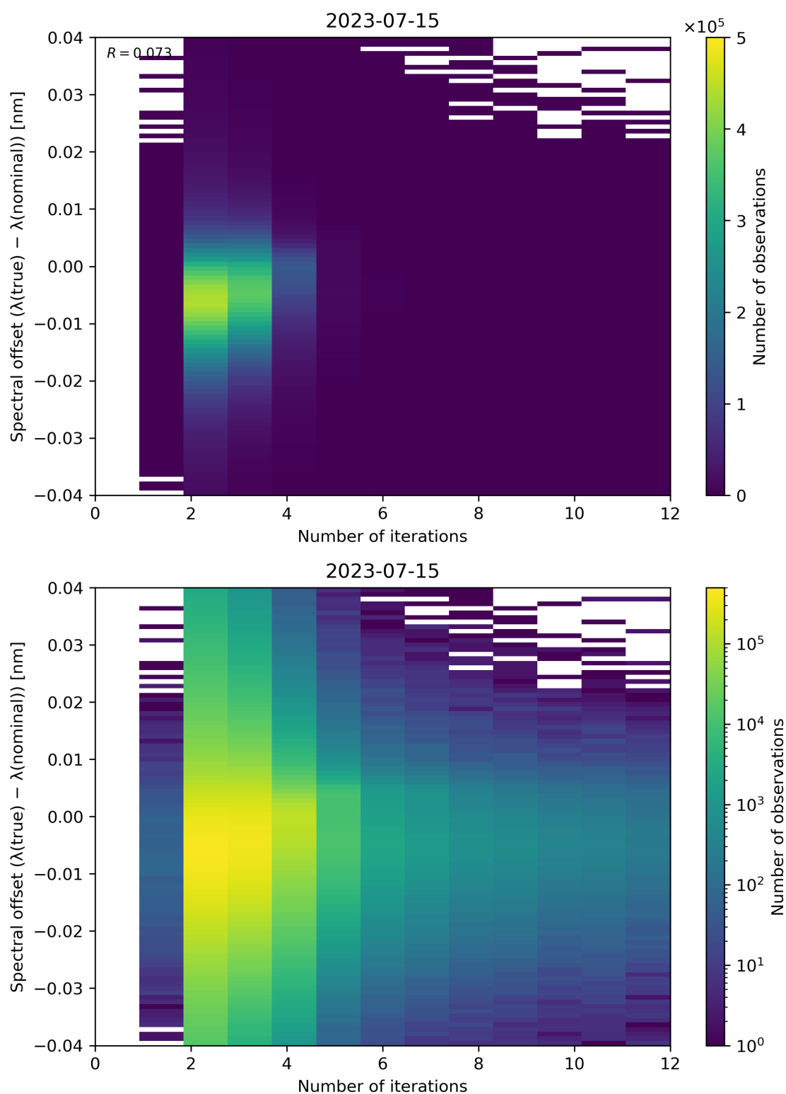
Figure 109: Scatter density plot of “Number of iterations” against “Spectral offset ( \lambda(\text{true}) - \lambda(\text{nominal}) )” for 2023-07-14 to 2023-07-16.
