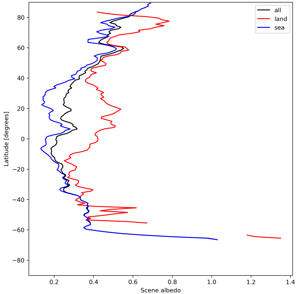
Figure 17: Zonal average of “Scene albedo” for 2023-07-14 to 2023-07-16.
