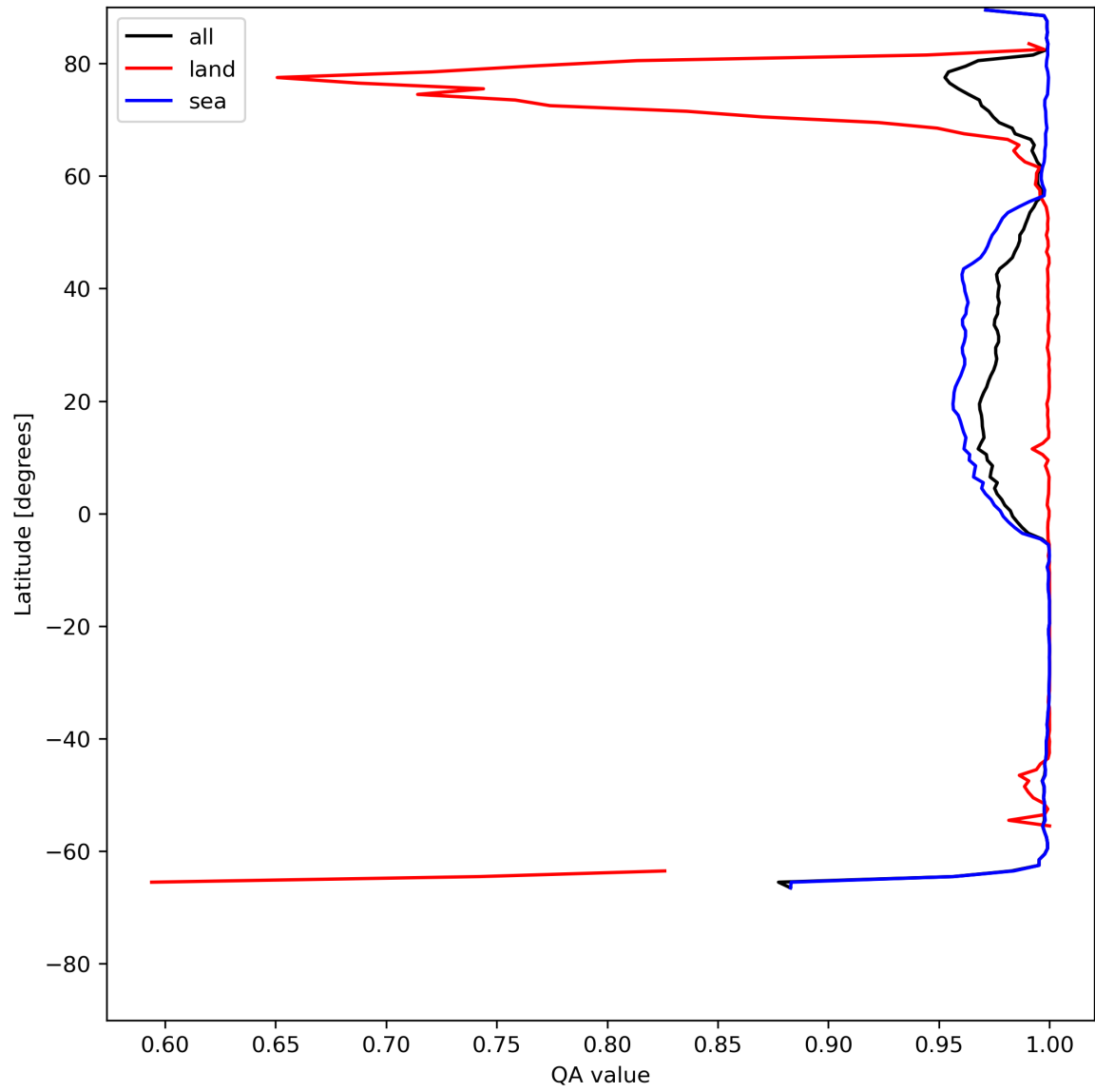
Figure 12: Zonal average of “QA value” for 2023-07-14 to 2023-07-16.
