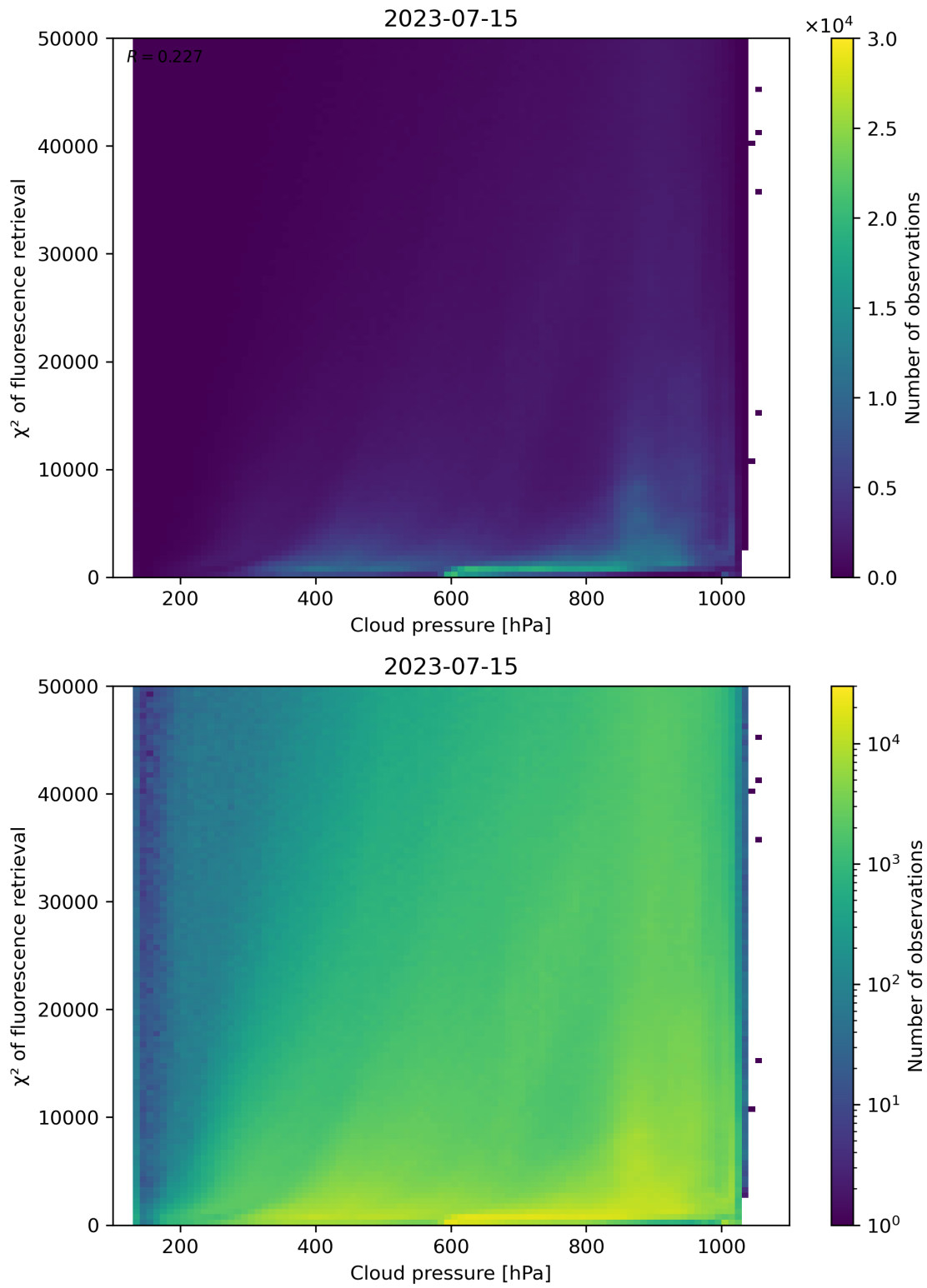
Figure 86: Scatter density plot of “Cloud pressure” against “ \chi^2 of fluorescence retrieval” for 2023-07-14 to 2023-07-16.
