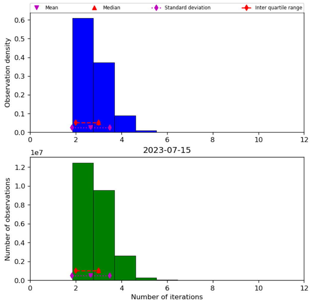
Figure 39: Histogram of “Number of iterations” for 2023-07-14 to 2023-07-16
