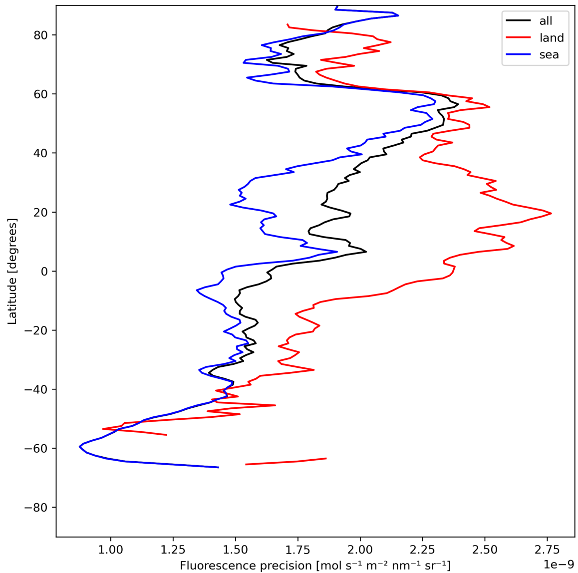
Figure 24: Zonal average of “Fluorescence precision” for 2023-07-14 to 2023-07-16.
