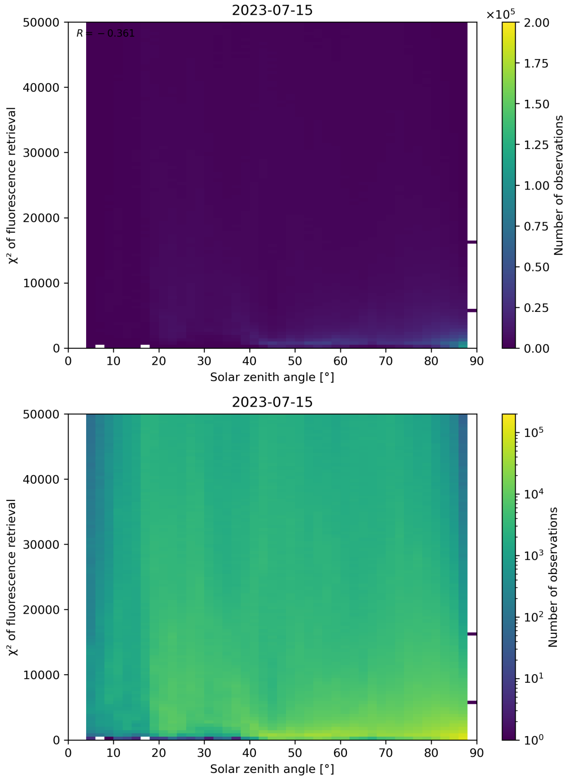
Figure 120: Scatter density plot of “Solar zenith angle” against “ \chi^2 of fluorescence retrieval” for 2023-07-14 to 2023-07-16.
