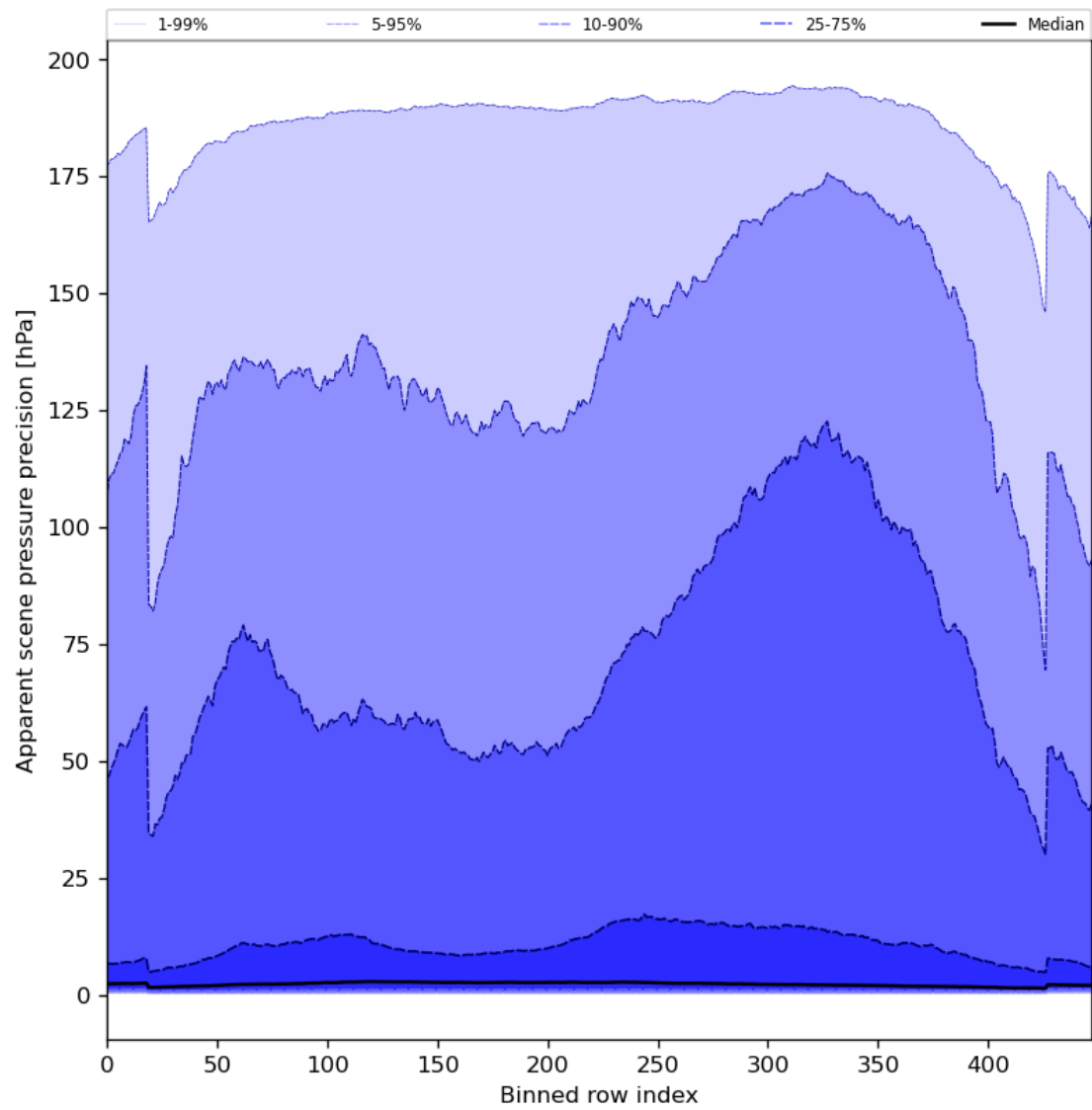
Figure 54: Along track statistics of “Apparent scene pressure precision” for 2023-07-14 to 2023-07-16
