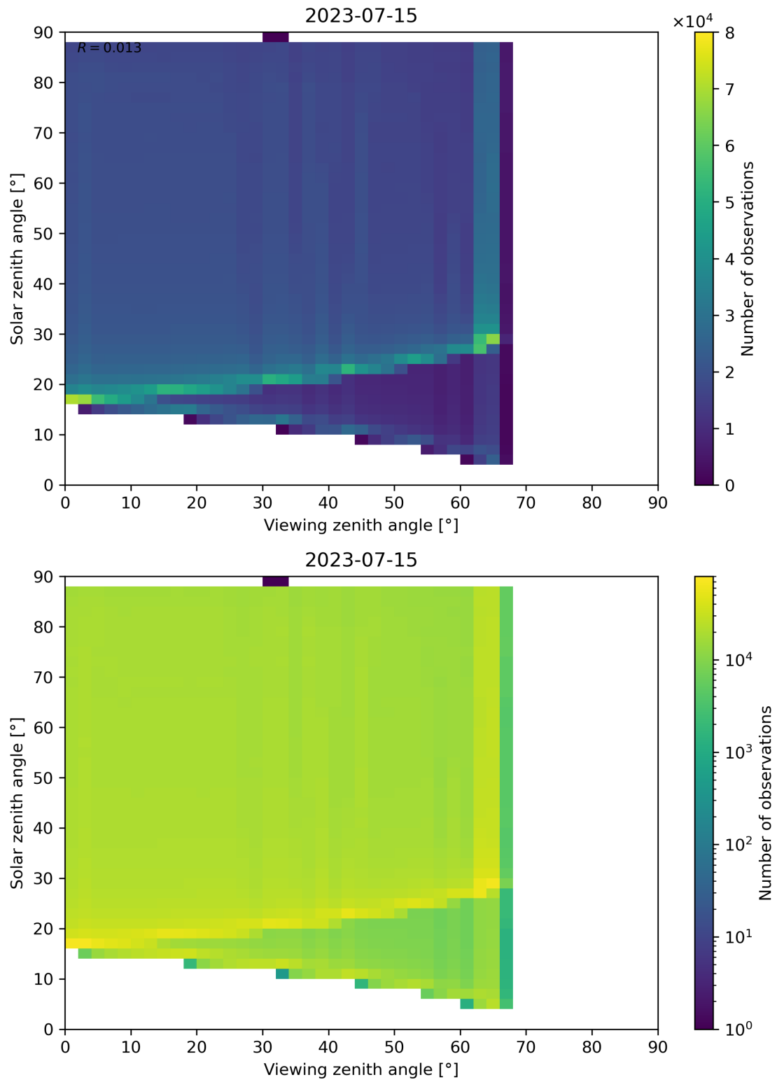
Figure 139: Scatter density plot of “Viewing zenith angle” against “Solar zenith angle” for 2023-07-14 to 2023-07-16.
