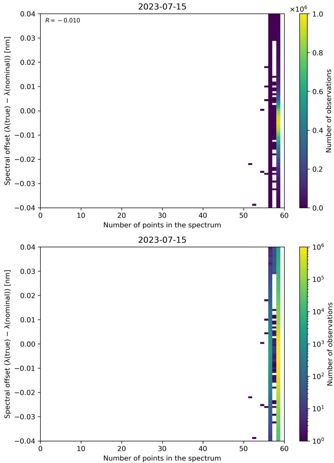
Figure 110: Scatter density plot of “Number of points in the spectrum” against “Spectral offset ( \lambda(\text{true}) - \lambda(\text{nominal}) )” for 2023-07-14 to 2023-07-16.
