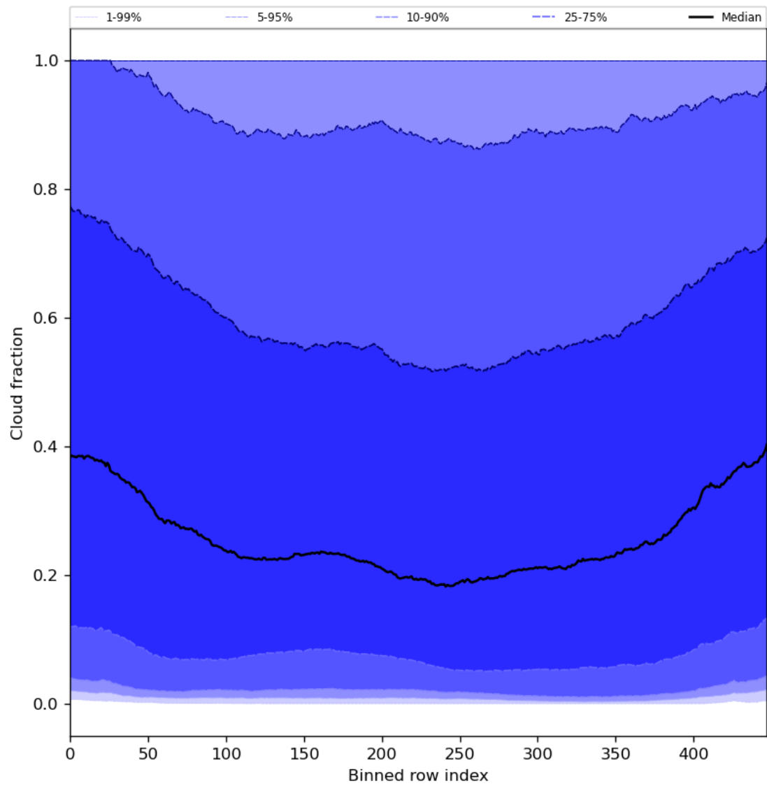
Figure 49: Along track statistics of “Cloud fraction” for 2023-07-14 to 2023-07-16
