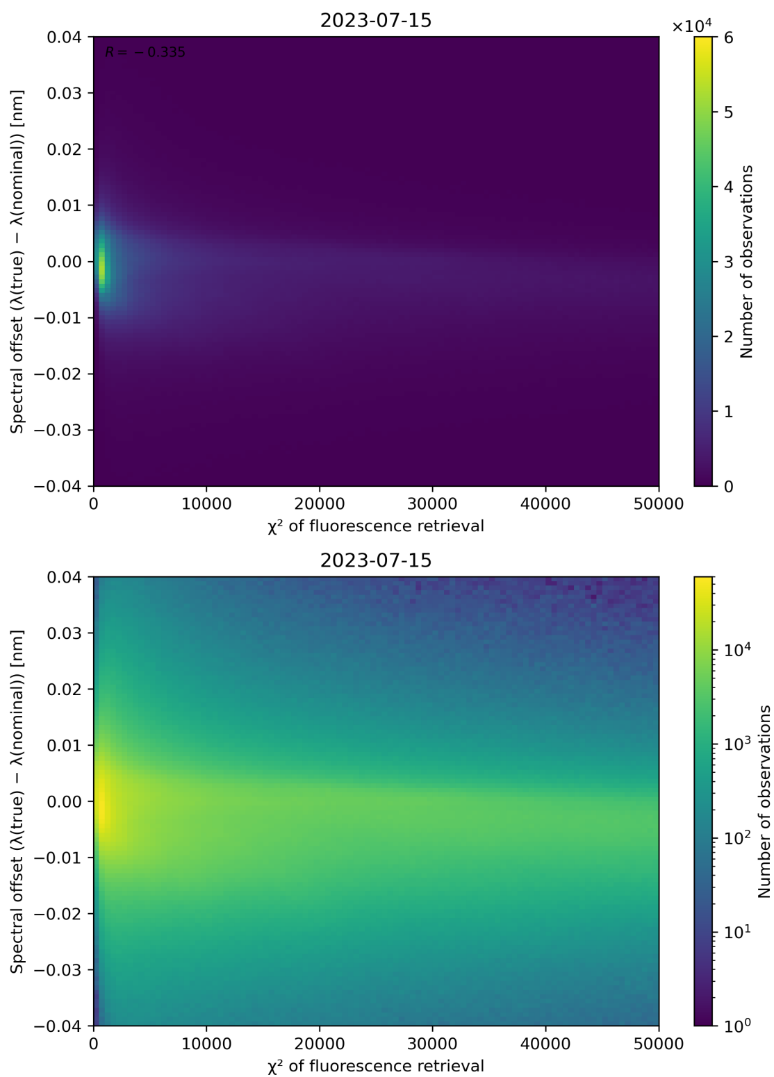
Figure 72: Scatter density plot of " \chi^2 of fluorescence retrieval" against "Spectral offset ( \lambda(\text{true}) - \lambda(\text{nominal}) )" for 2023-07-14 to 2023-07-16.
