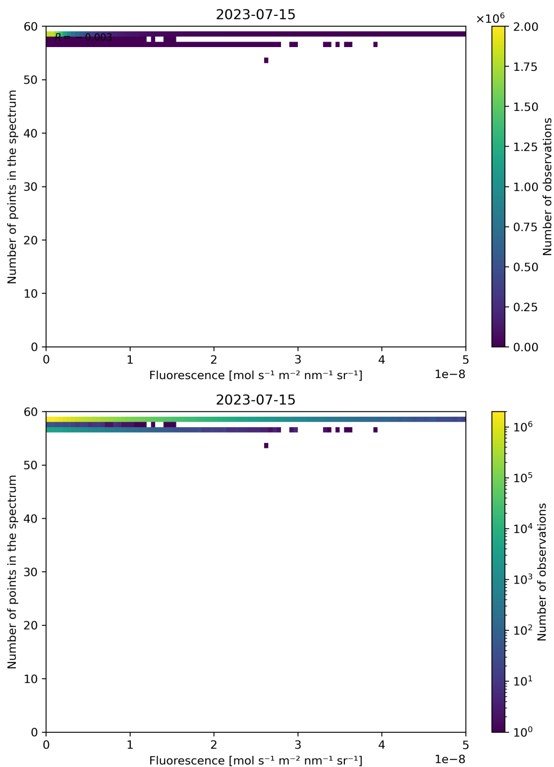
Figure 94: Scatter density plot of “Fluorescence” against “Number of points in the spectrum” for 2023-07-14 to 2023-07-16.
