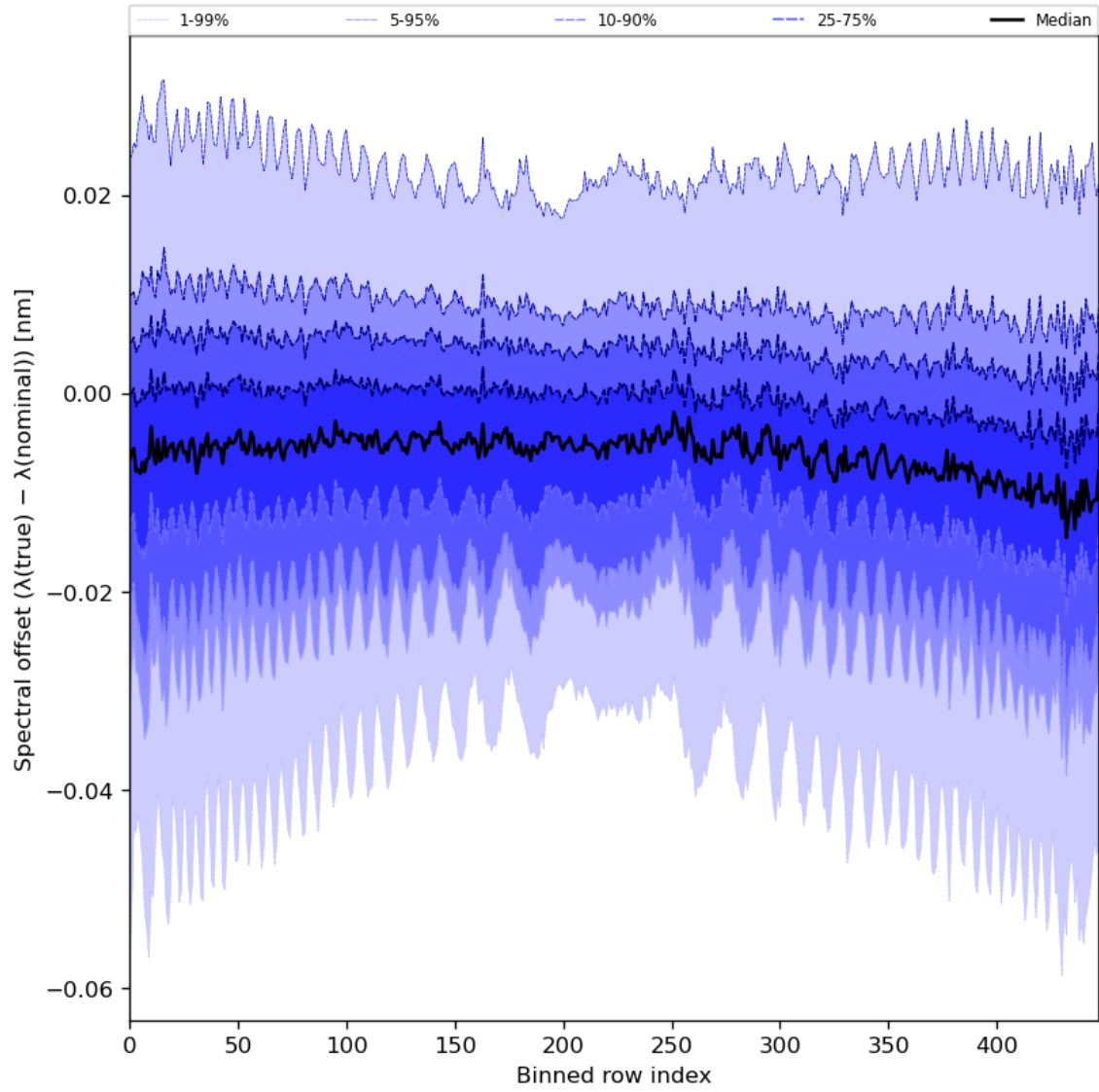
Figure 62: Along track statistics of “Spectral offset ( \lambda(\text{true}) - \lambda(\text{nominal}) )” for 2023-07-14 to 2023-07-16
