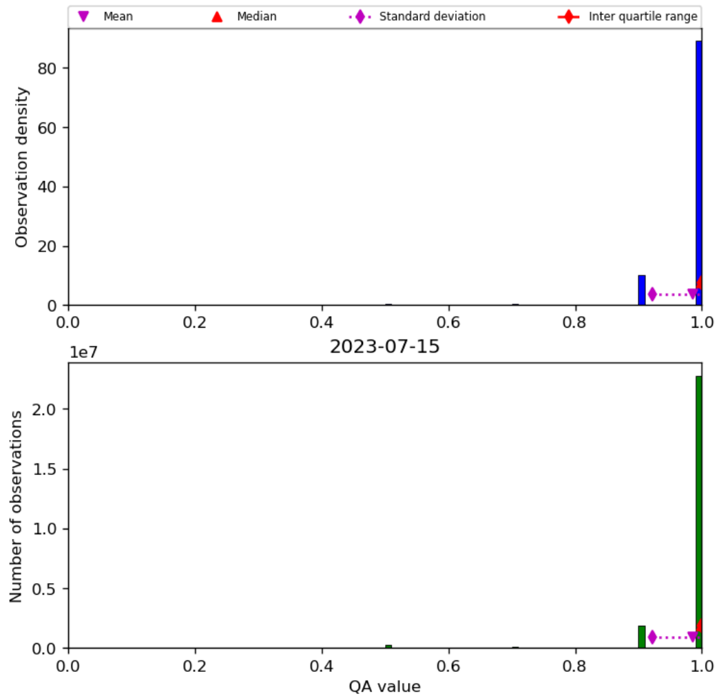
Figure 29: Histogram of “QA value” for 2023-07-14 to 2023-07-16
