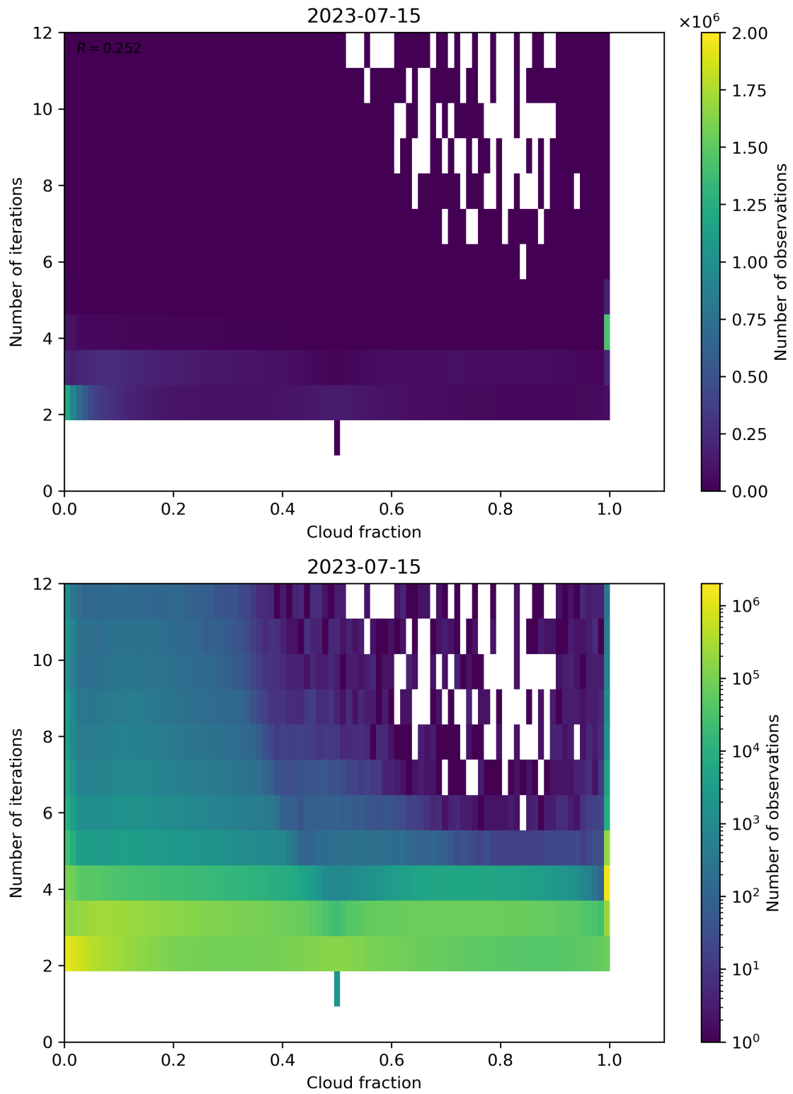
Figure 80: Scatter density plot of “Cloud fraction” against “Number of iterations” for 2023-07-14 to 2023-07-16.
