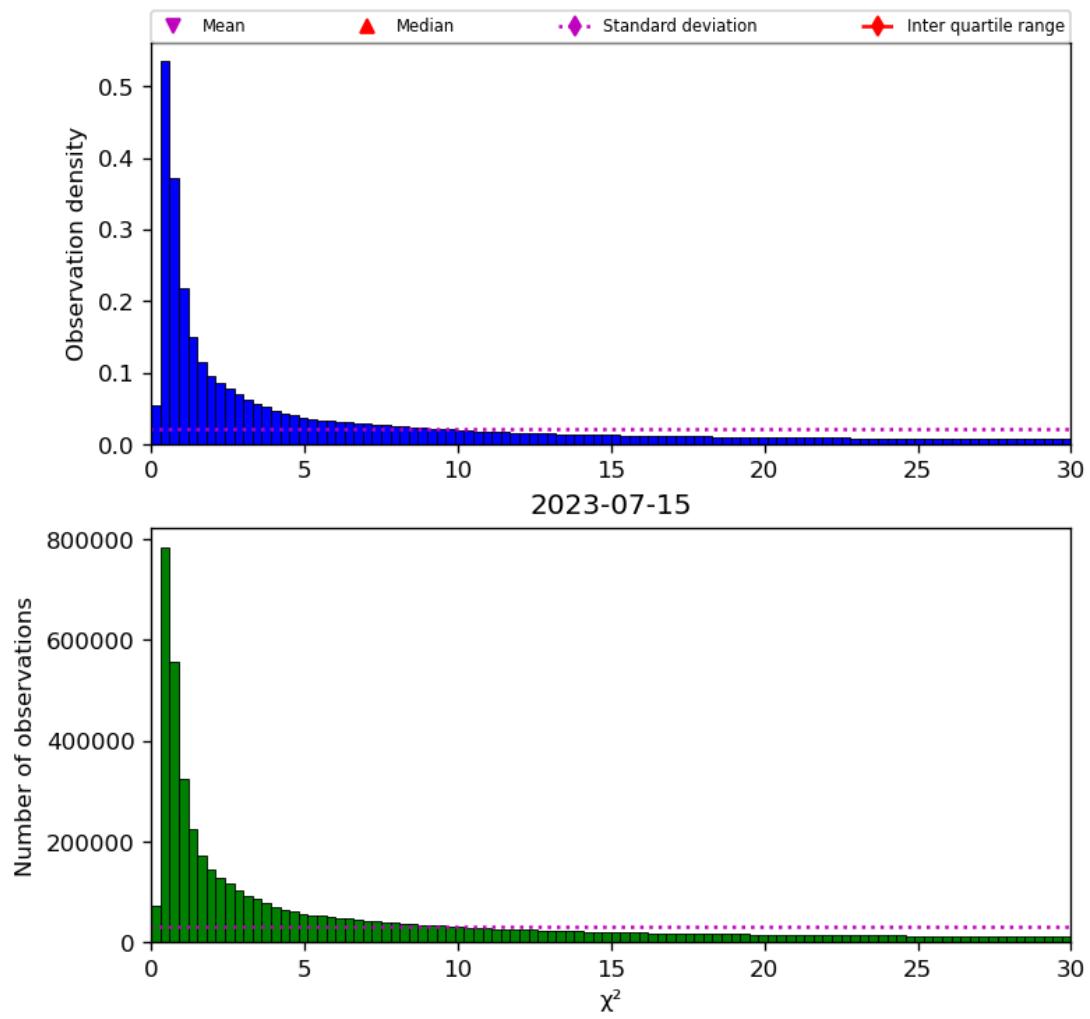
Figure 38: Histogram of “ \chi^2 ” for 2023-07-14 to 2023-07-16
