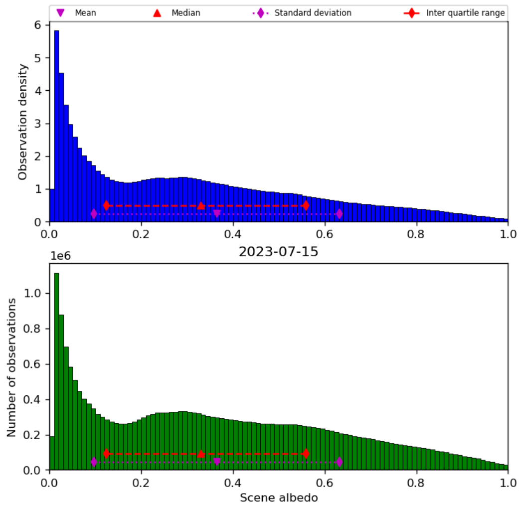
Figure 34: Histogram of “Scene albedo” for 2023-07-14 to 2023-07-16
