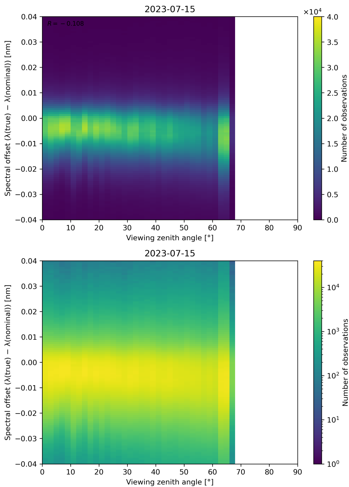
Figure 140: Scatter density plot of “Viewing zenith angle” against “Spectral offset ( \lambda(\text{true}) - \lambda(\text{nominal}) )” for 2023-07-14 to 2023-07-16.
