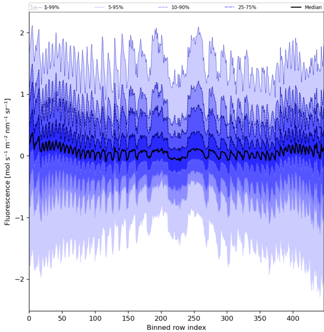
Figure 57: Along track statistics of “Fluorescence” for 2023-07-14 to 2023-07-16
