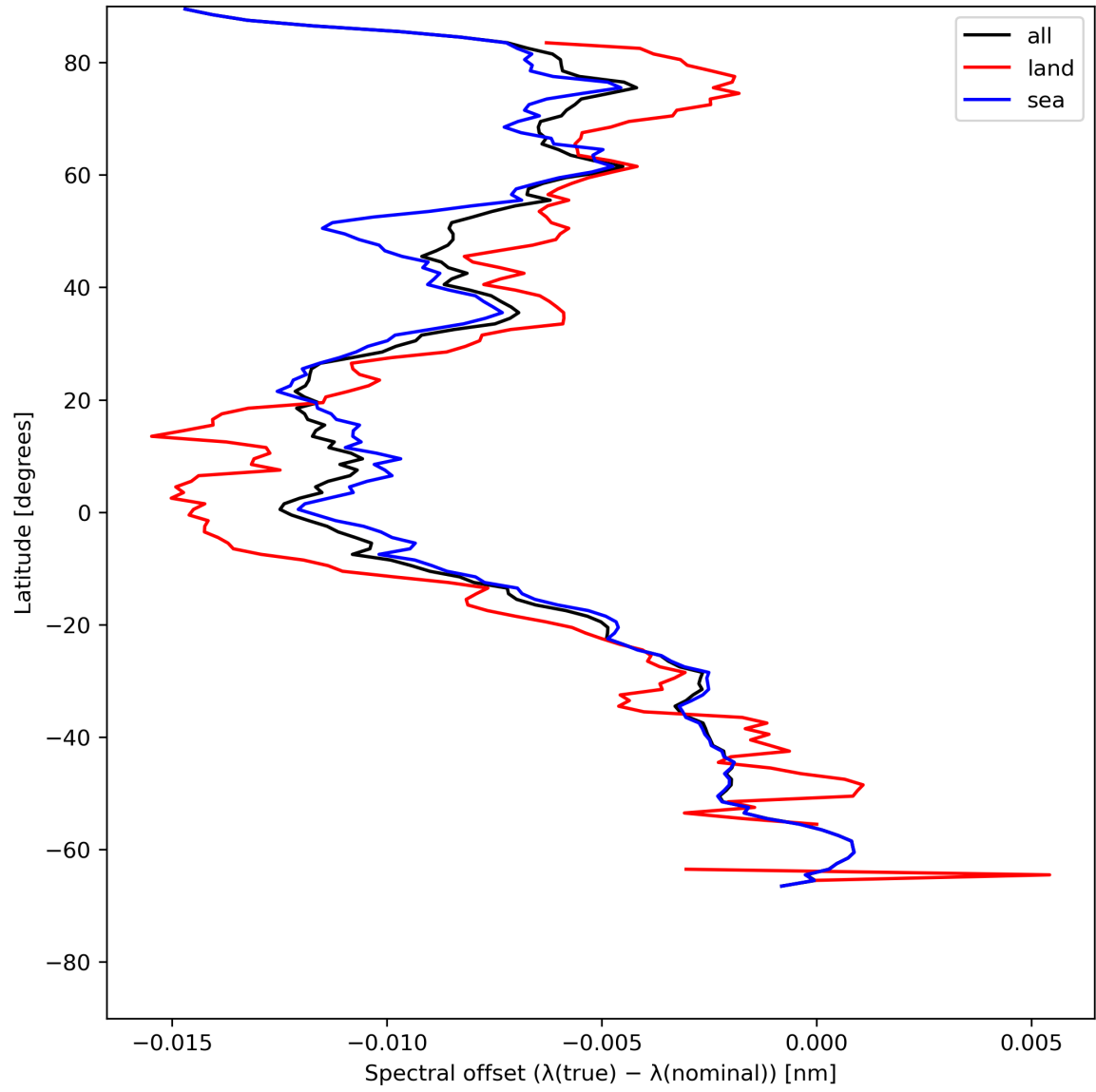
Figure 28: Zonal average of “Spectral offset ( \lambda(\text{true}) - \lambda(\text{nominal}) )” for 2023-07-14 to 2023-07-16.
