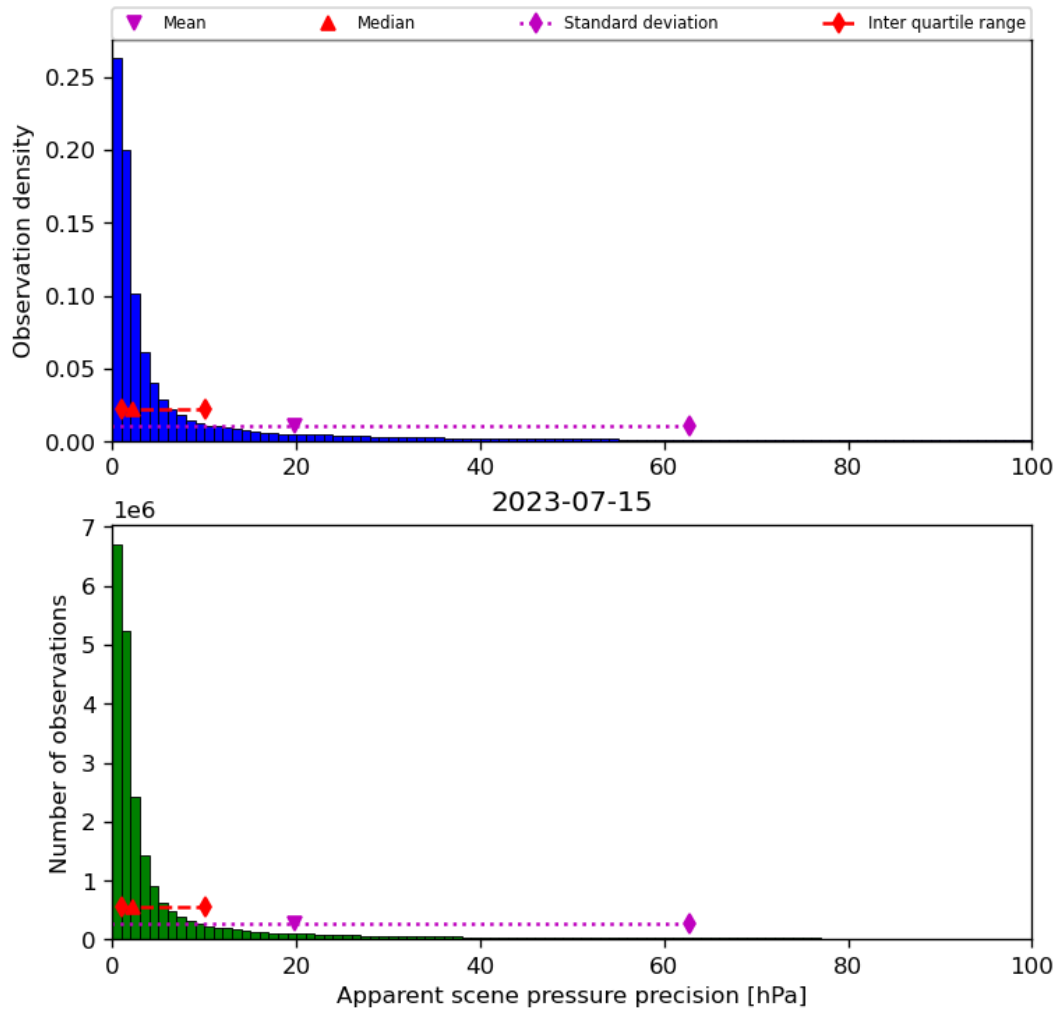
Figure 37: Histogram of “Apparent scene pressure precision” for 2023-07-14 to 2023-07-16
