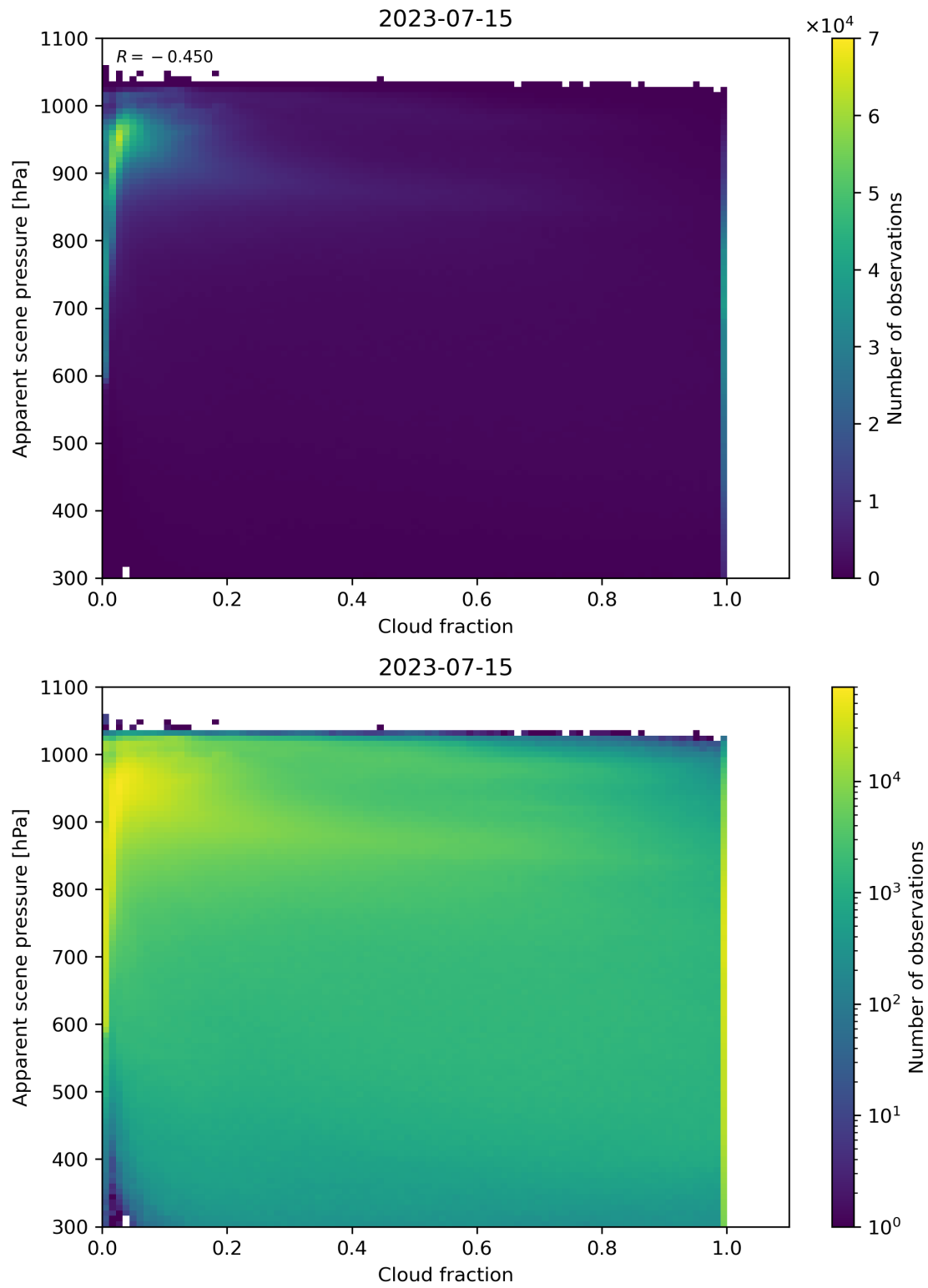
Figure 76: Scatter density plot of “Cloud fraction” against “Apparent scene pressure” for 2023-07-14 to 2023-07-16.
