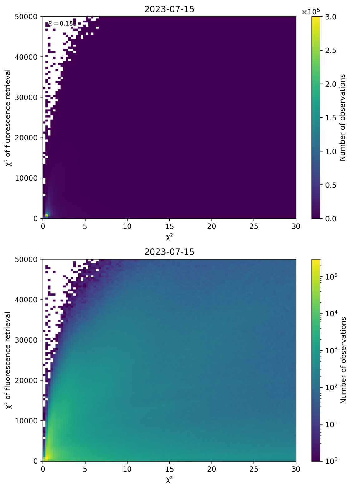
Figure 69: Scatter density plot of “ \chi^2 ” against “ \chi^2 of fluorescence retrieval” for 2023-07-14 to 2023-07-16.
