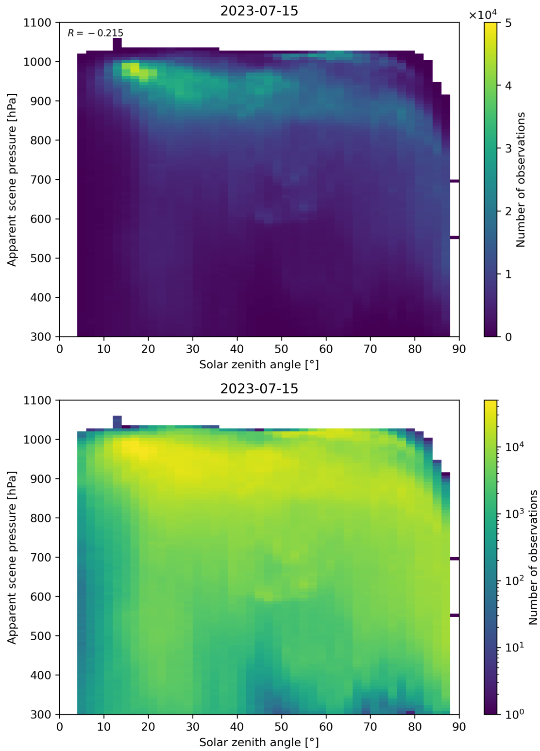
Figure 118: Scatter density plot of “Solar zenith angle” against “Apparent scene pressure” for 2023-07-14 to 2023-07-16.
