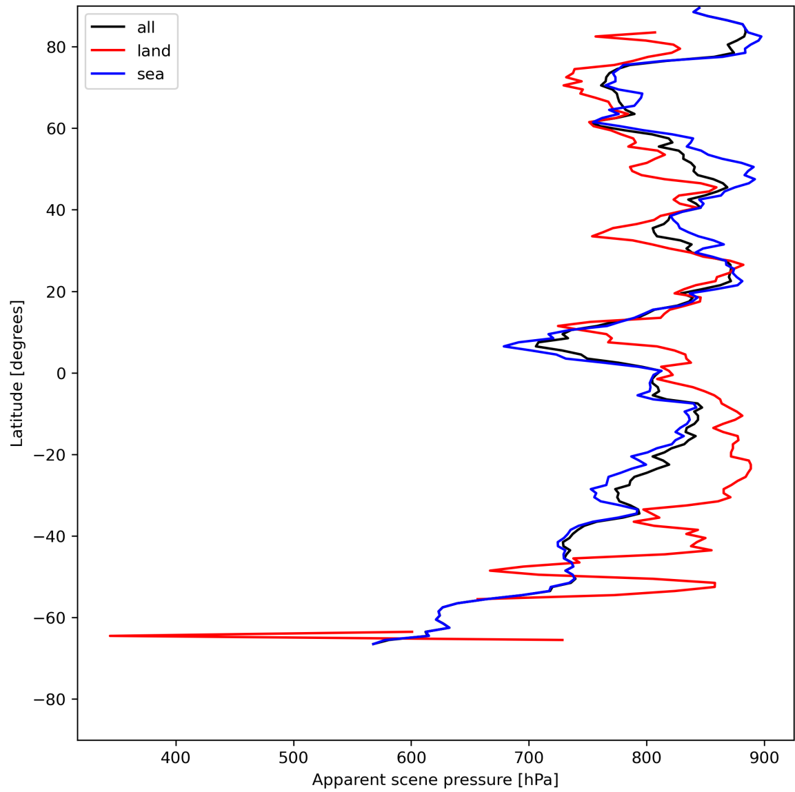
Figure 19: Zonal average of “Apparent scene pressure” for 2023-07-14 to 2023-07-16.
