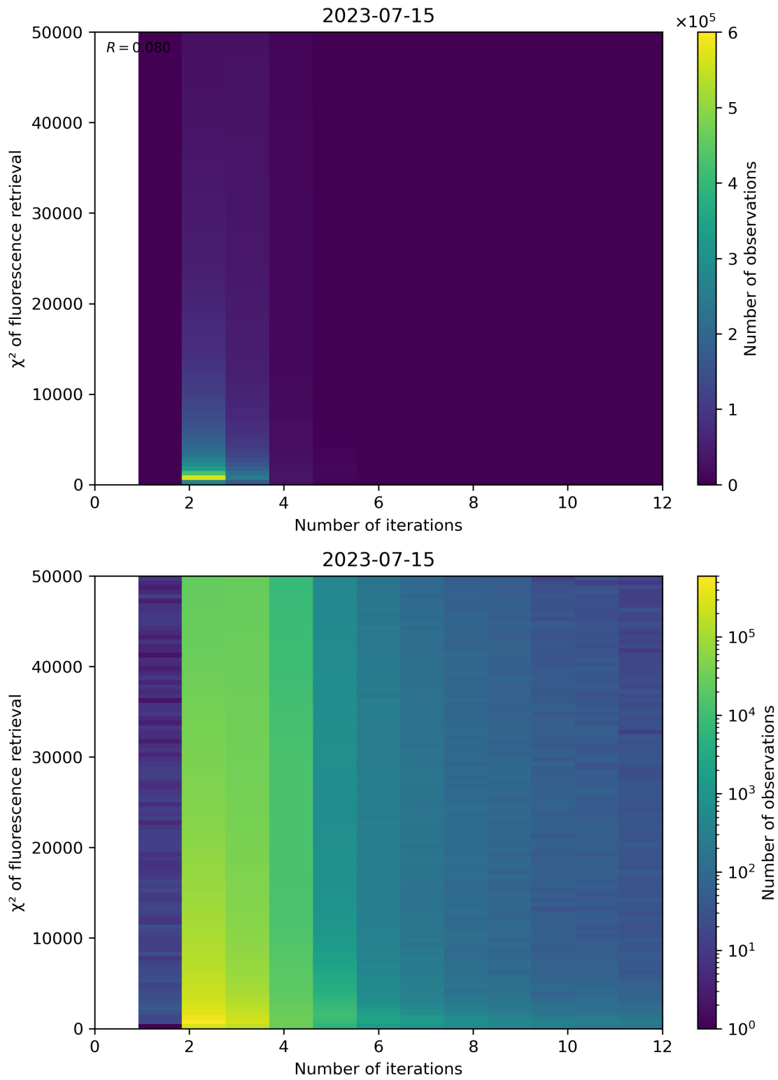
Figure 106: Scatter density plot of “Number of iterations” against “ \chi^2 of fluorescence retrieval” for 2023-07-14 to 2023-07-16.
