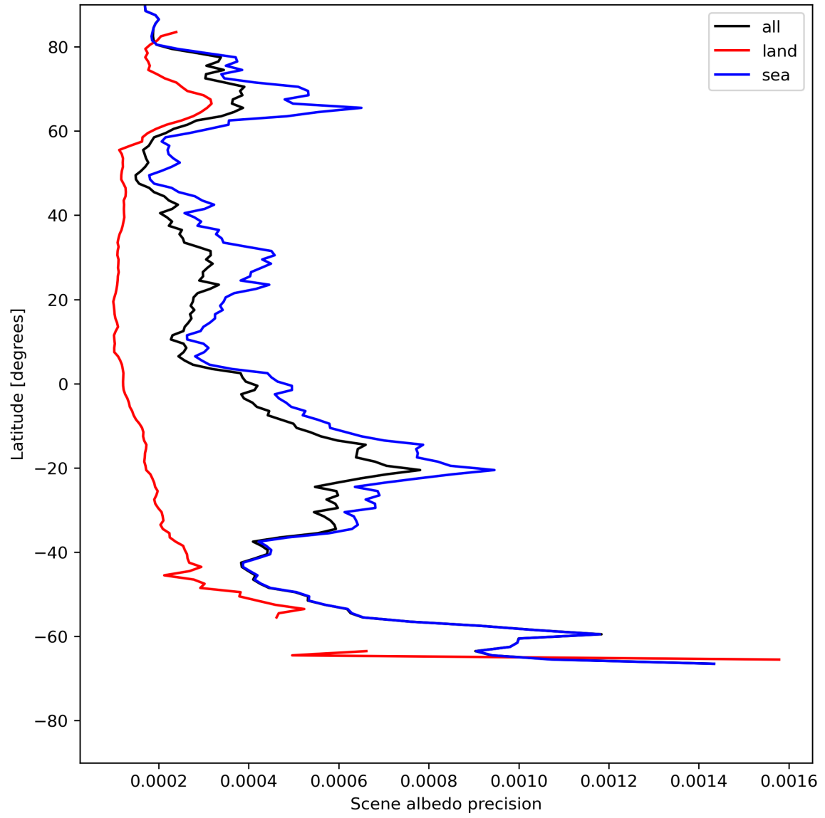
Figure 18: Zonal average of “Scene albedo precision” for 2023-07-14 to 2023-07-16.
