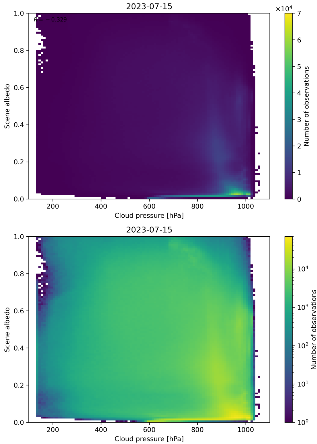
Figure 91: Scatter density plot of “Cloud pressure” against “Scene albedo” for 2023-07-14 to 2023-07-16.
