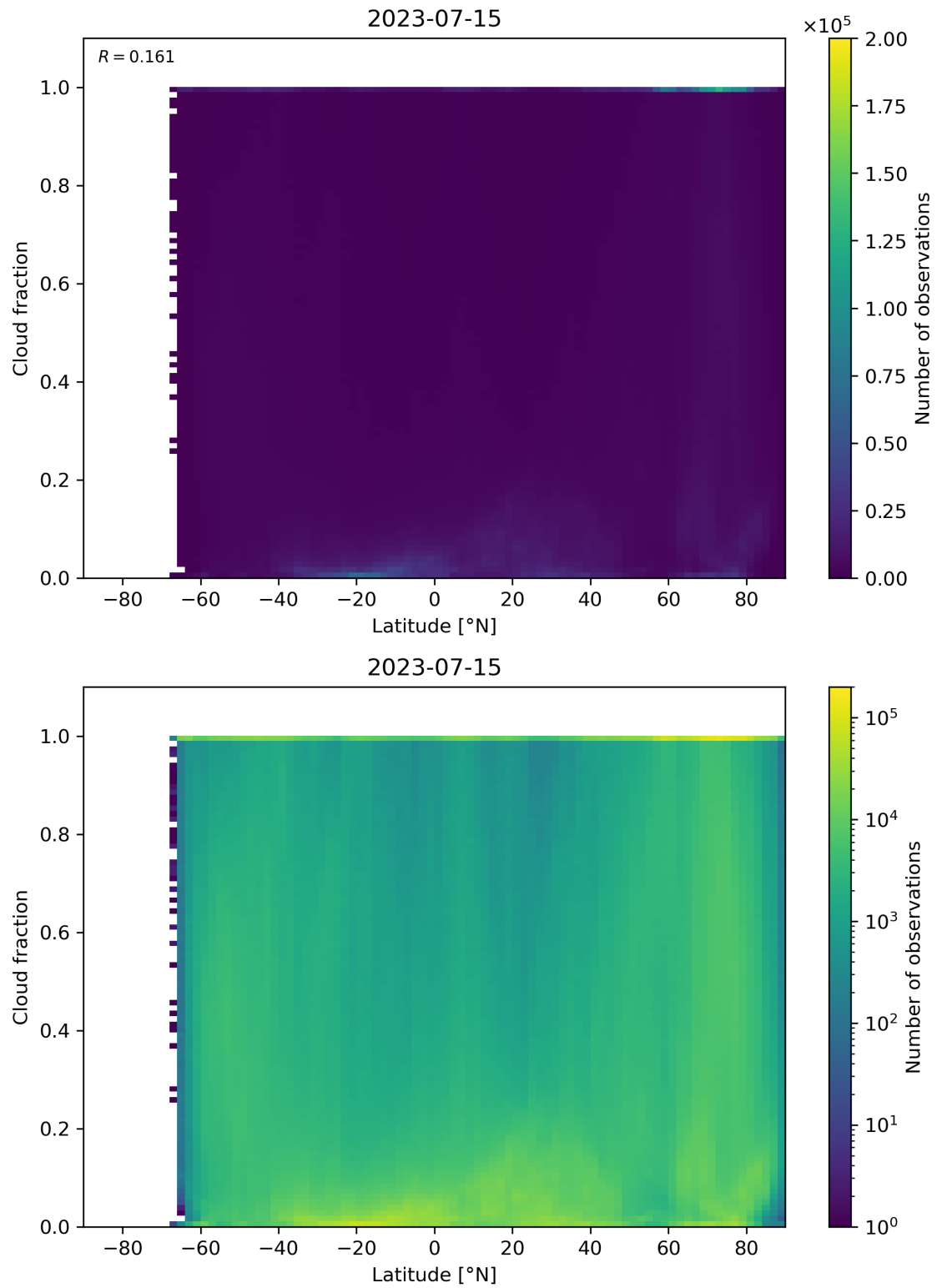
Figure 99: Scatter density plot of “Latitude” against “Cloud fraction” for 2023-07-14 to 2023-07-16.
