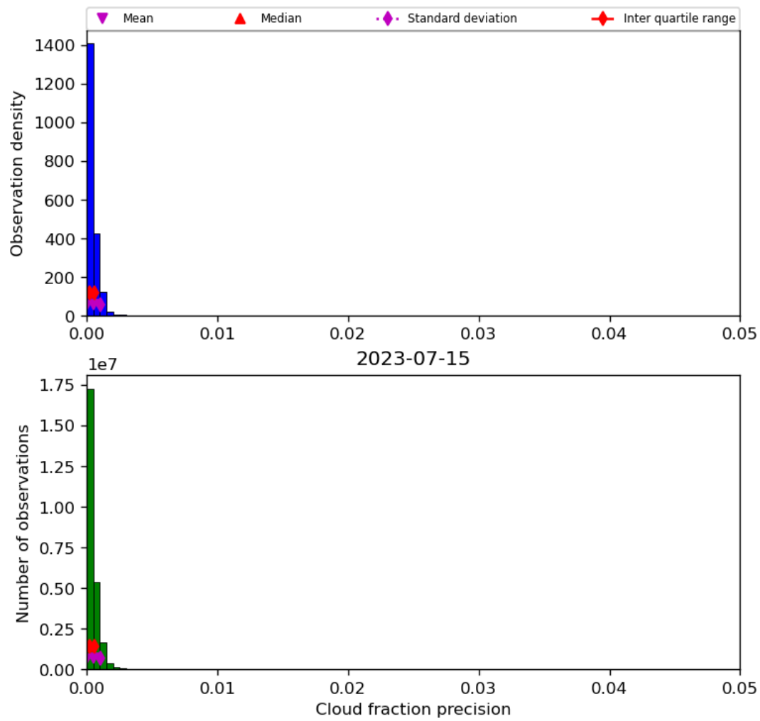
Figure 33: Histogram of “Cloud fraction precision” for 2023-07-14 to 2023-07-16
