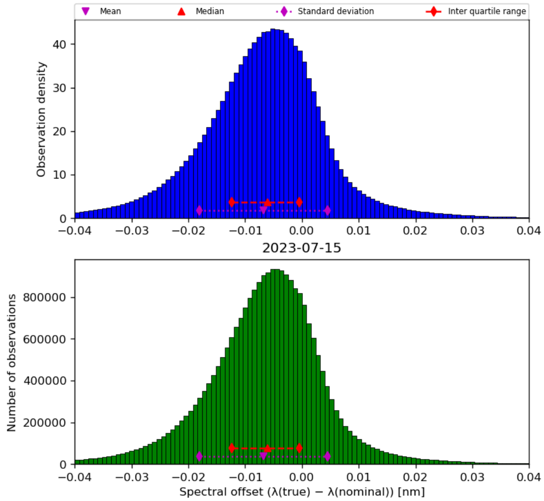
Figure 45: Histogram of “Spectral offset ( \lambda(\text{true}) - \lambda(\text{nominal}) )” for 2023-07-14 to 2023-07-16
