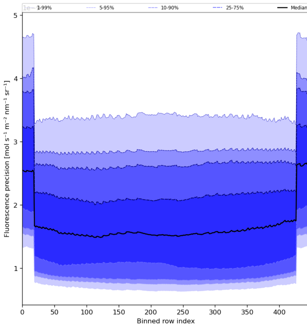
Figure 58: Along track statistics of “Fluorescence precision” for 2023-07-14 to 2023-07-16
