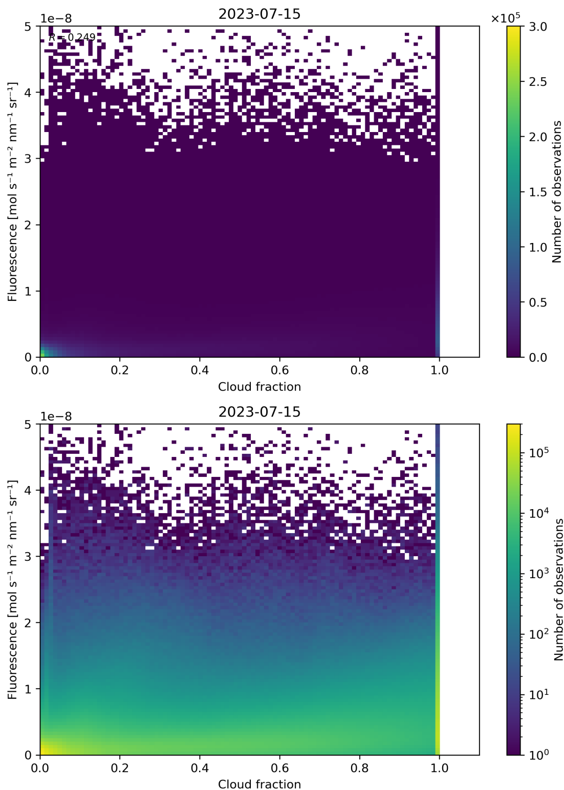
Figure 79: Scatter density plot of “Cloud fraction” against “Fluorescence” for 2023-07-14 to 2023-07-16.
