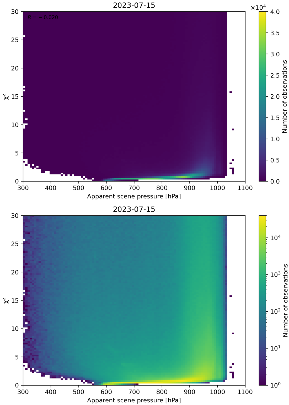
Figure 63: Scatter density plot of “Apparent scene pressure” against “ \chi^2 ” for 2023-07-14 to 2023-07-16.
