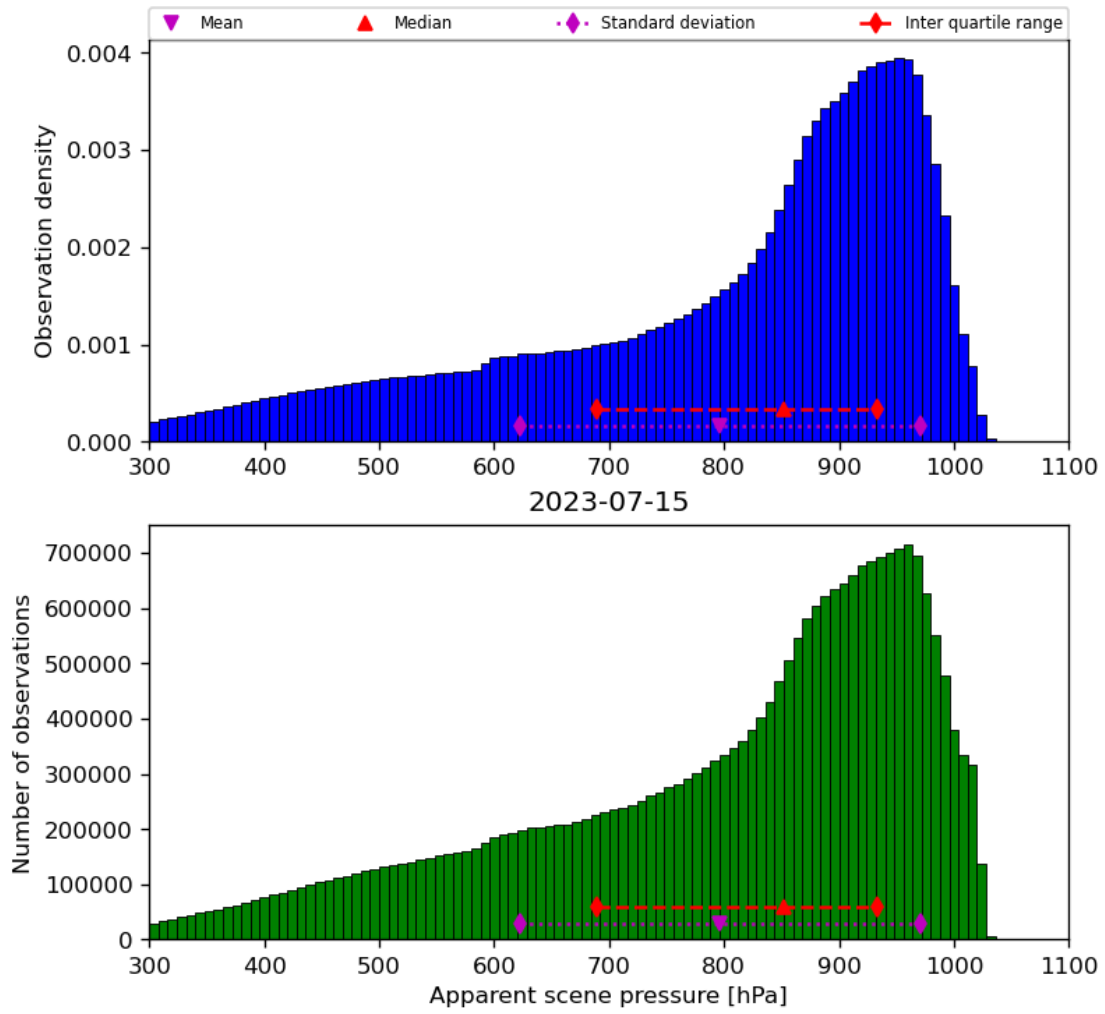
Figure 36: Histogram of “Apparent scene pressure” for 2023-07-14 to 2023-07-16
