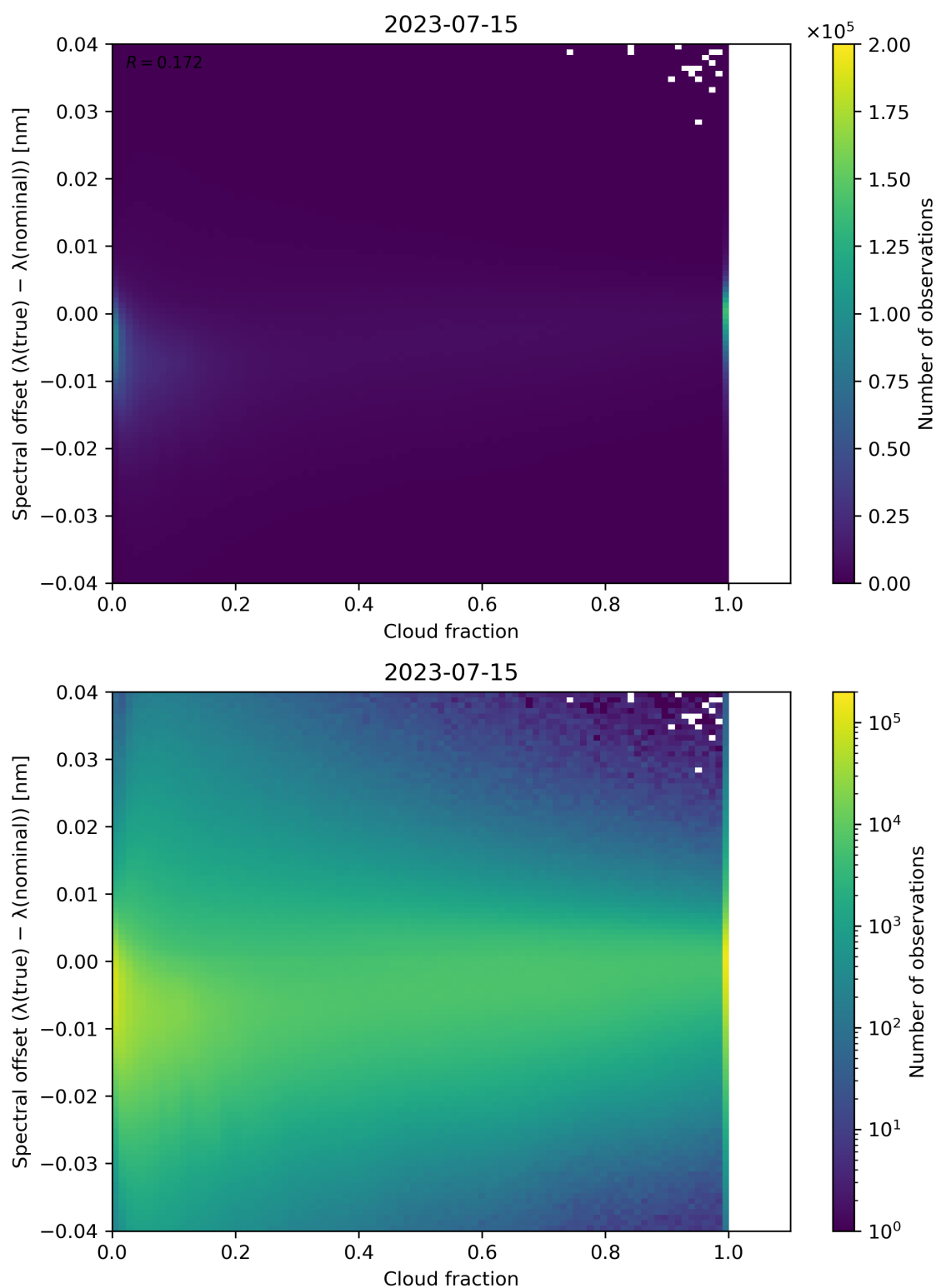
Figure 83: Scatter density plot of “Cloud fraction” against “Spectral offset ( \lambda(\text{true}) - \lambda(\text{nominal}) )” for 2023-07-14 to 2023-07-16.
