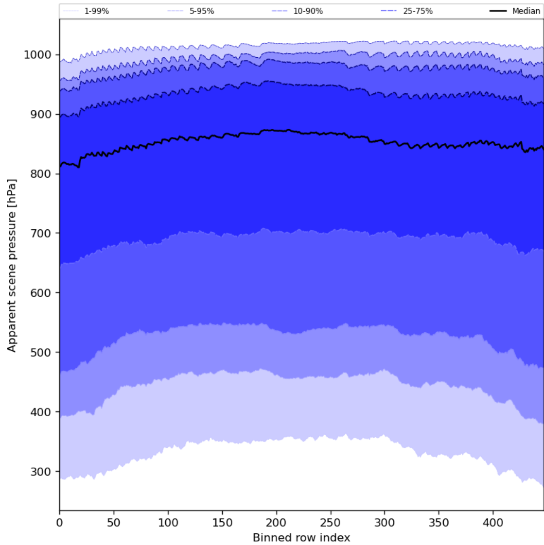
Figure 53: Along track statistics of “Apparent scene pressure” for 2023-07-14 to 2023-07-16
