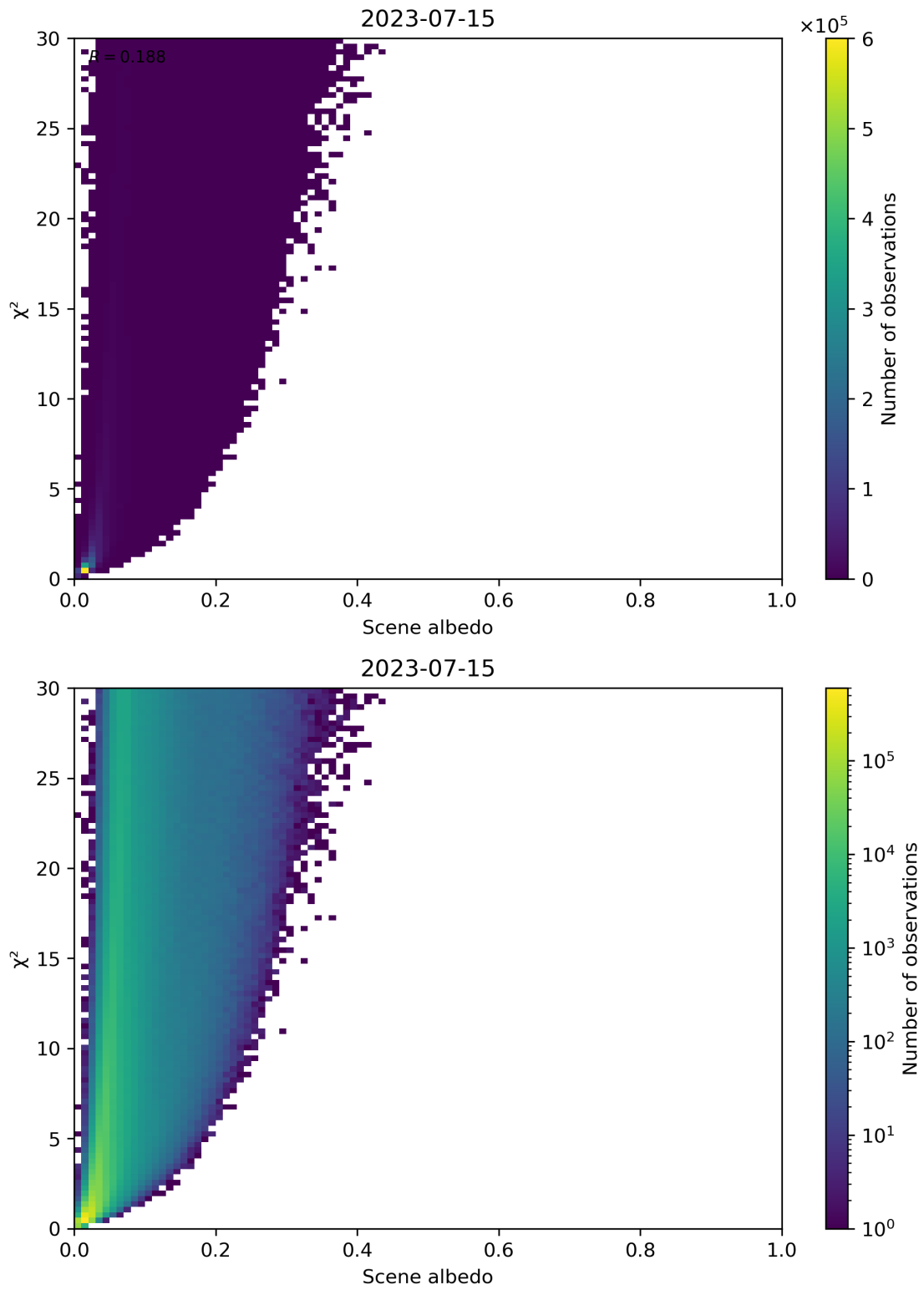
Figure 112: Scatter density plot of “Scene albedo” against “ \chi^2 ” for 2023-07-14 to 2023-07-16.
