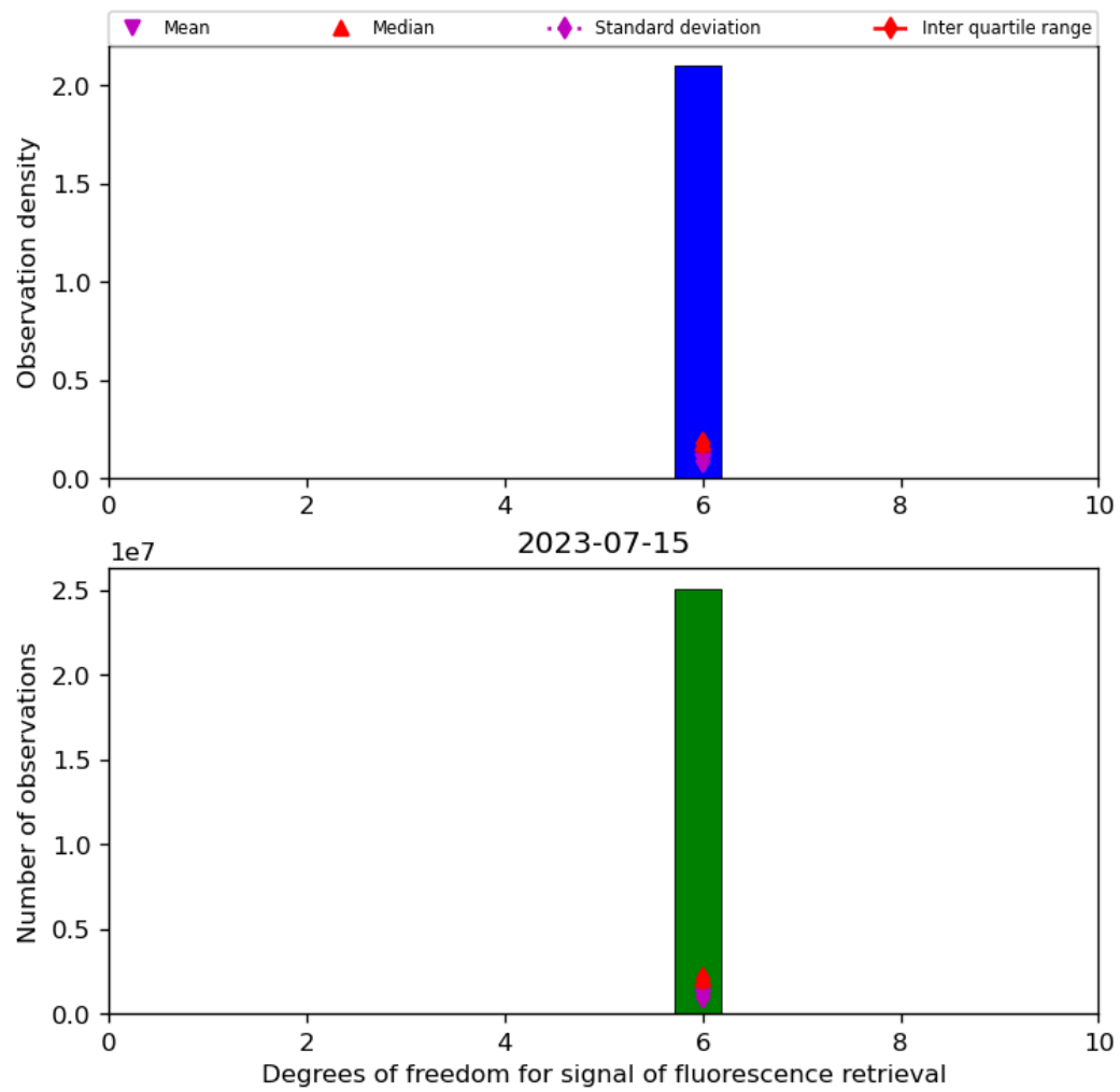
Figure 43: Histogram of “Degrees of freedom for signal of fluorescence retrieval” for 2023-07-14 to 2023-07-16
