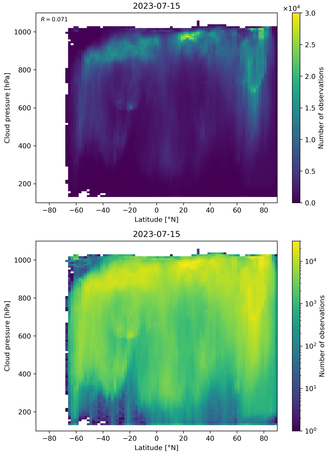
Figure 100: Scatter density plot of “Latitude” against “Cloud pressure” for 2023-07-14 to 2023-07-16.
