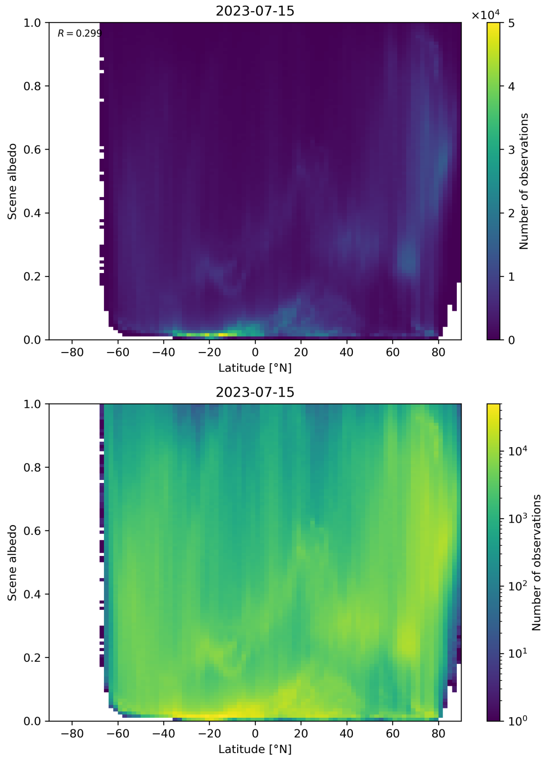
Figure 104: Scatter density plot of “Latitude” against “Scene albedo” for 2023-07-14 to 2023-07-16.
