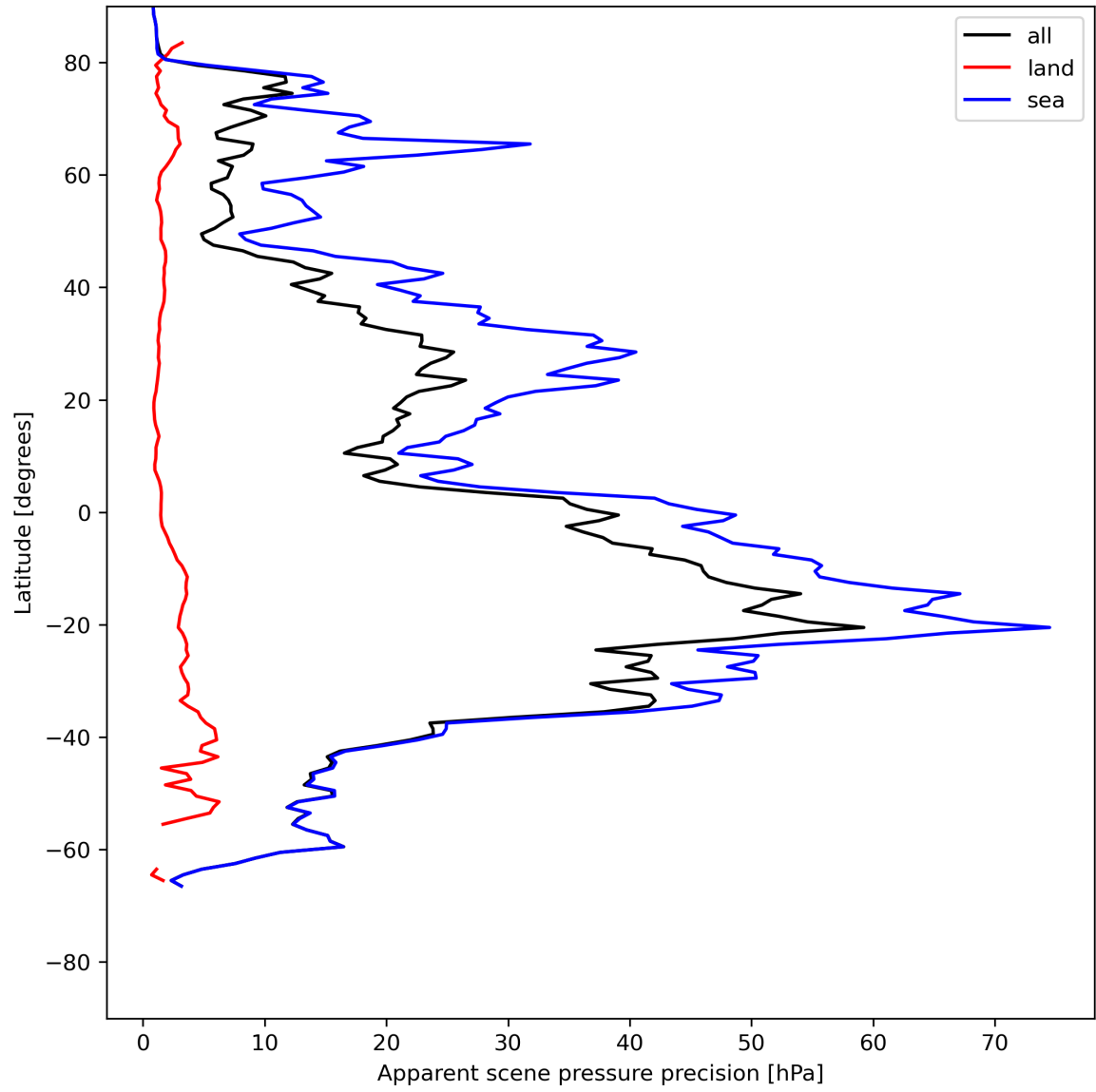
Figure 20: Zonal average of “Apparent scene pressure precision” for 2023-07-14 to 2023-07-16.
