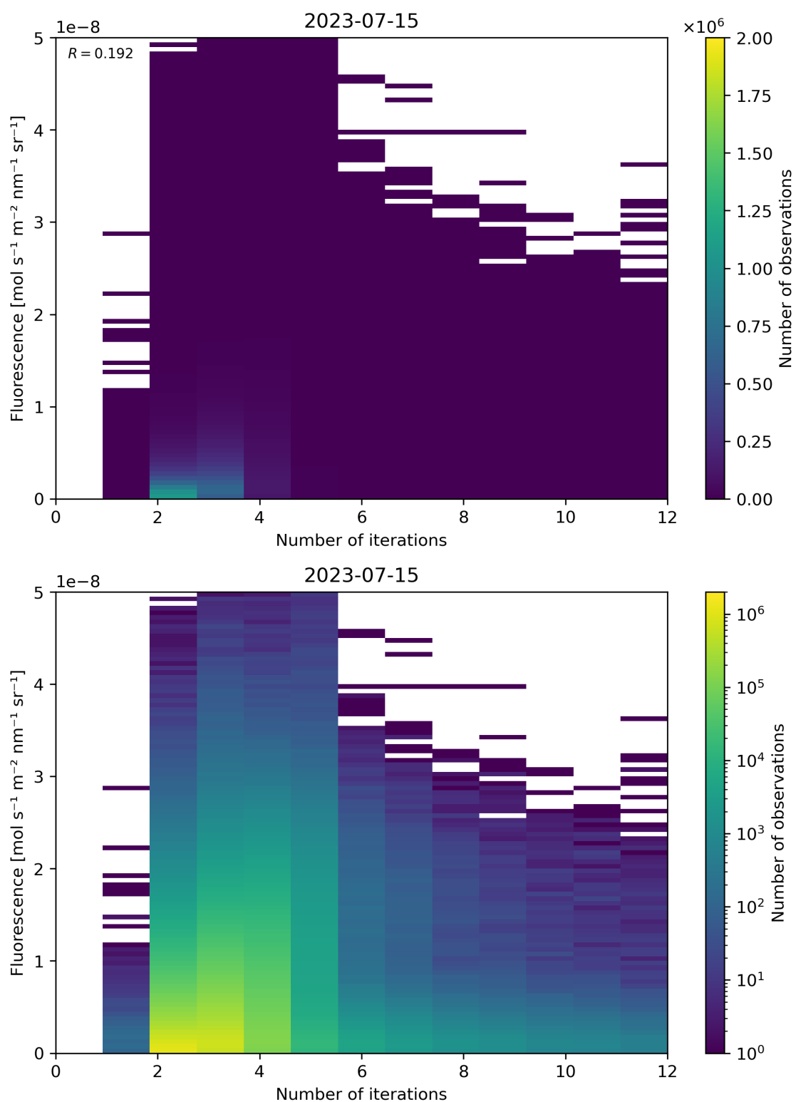
Figure 107: Scatter density plot of “Number of iterations” against “Fluorescence” for 2023-07-14 to 2023-07-16.
