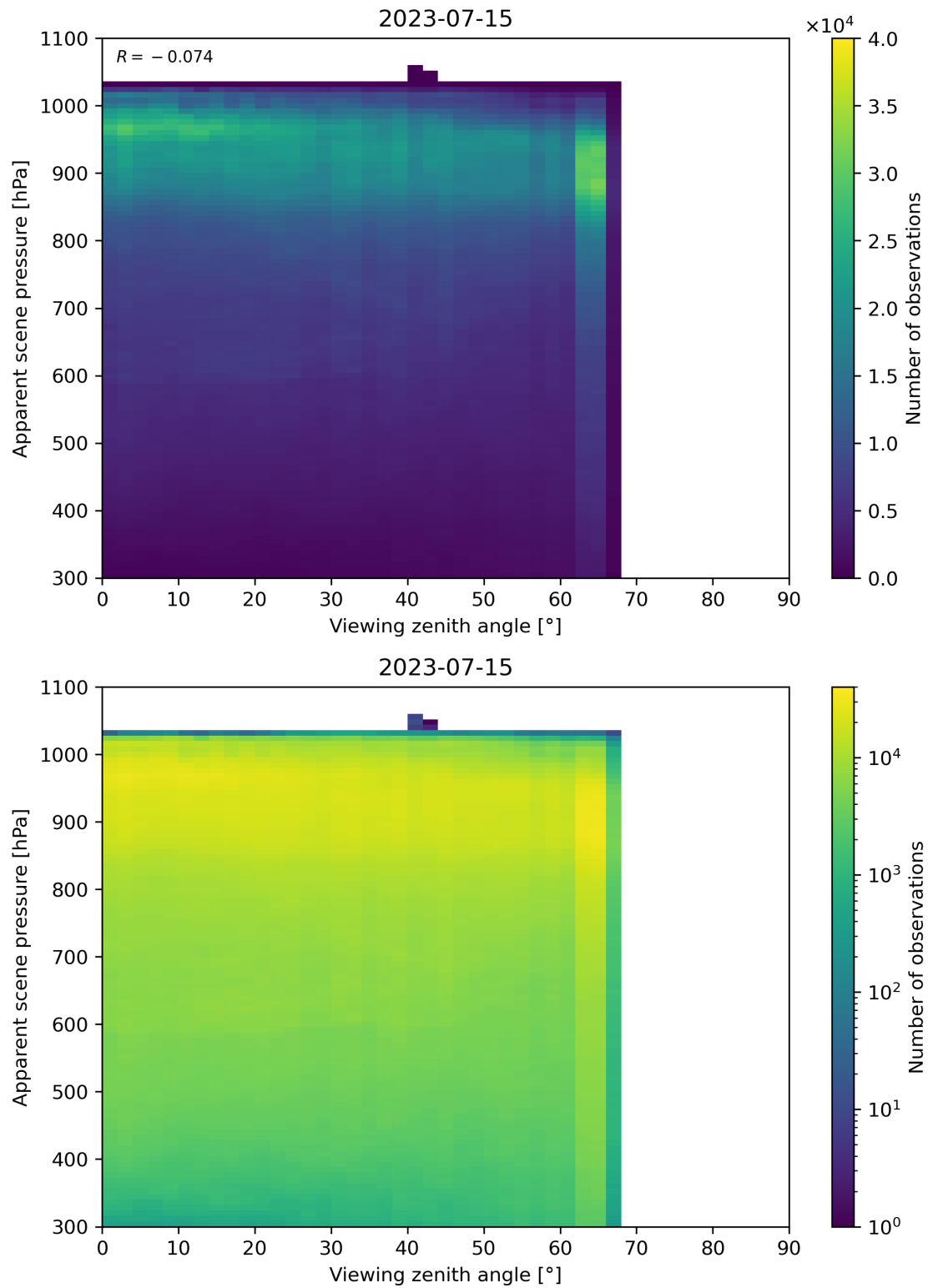
Figure 129: Scatter density plot of “Viewing zenith angle” against “Apparent scene pressure” for 2023-07-14 to 2023-07-16.
