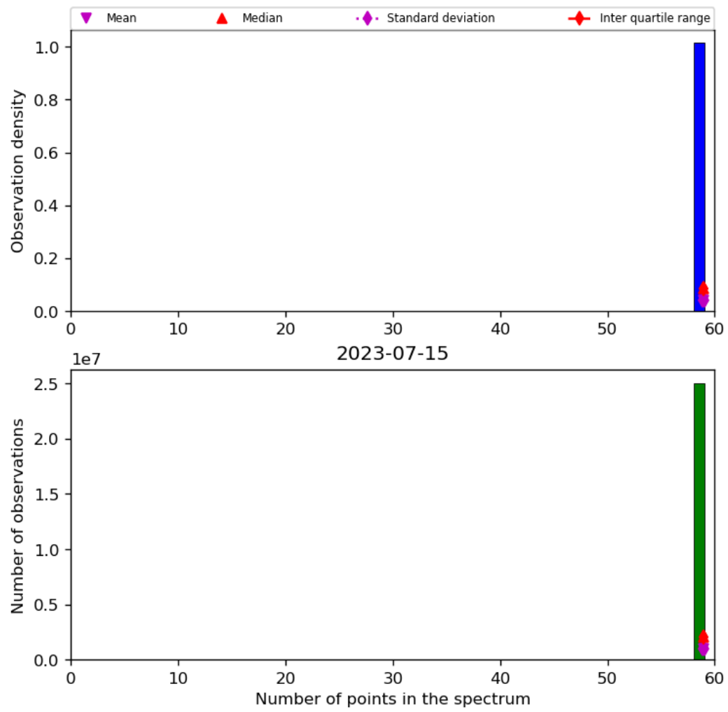
Figure 44: Histogram of “Number of points in the spectrum” for 2023-07-14 to 2023-07-16
