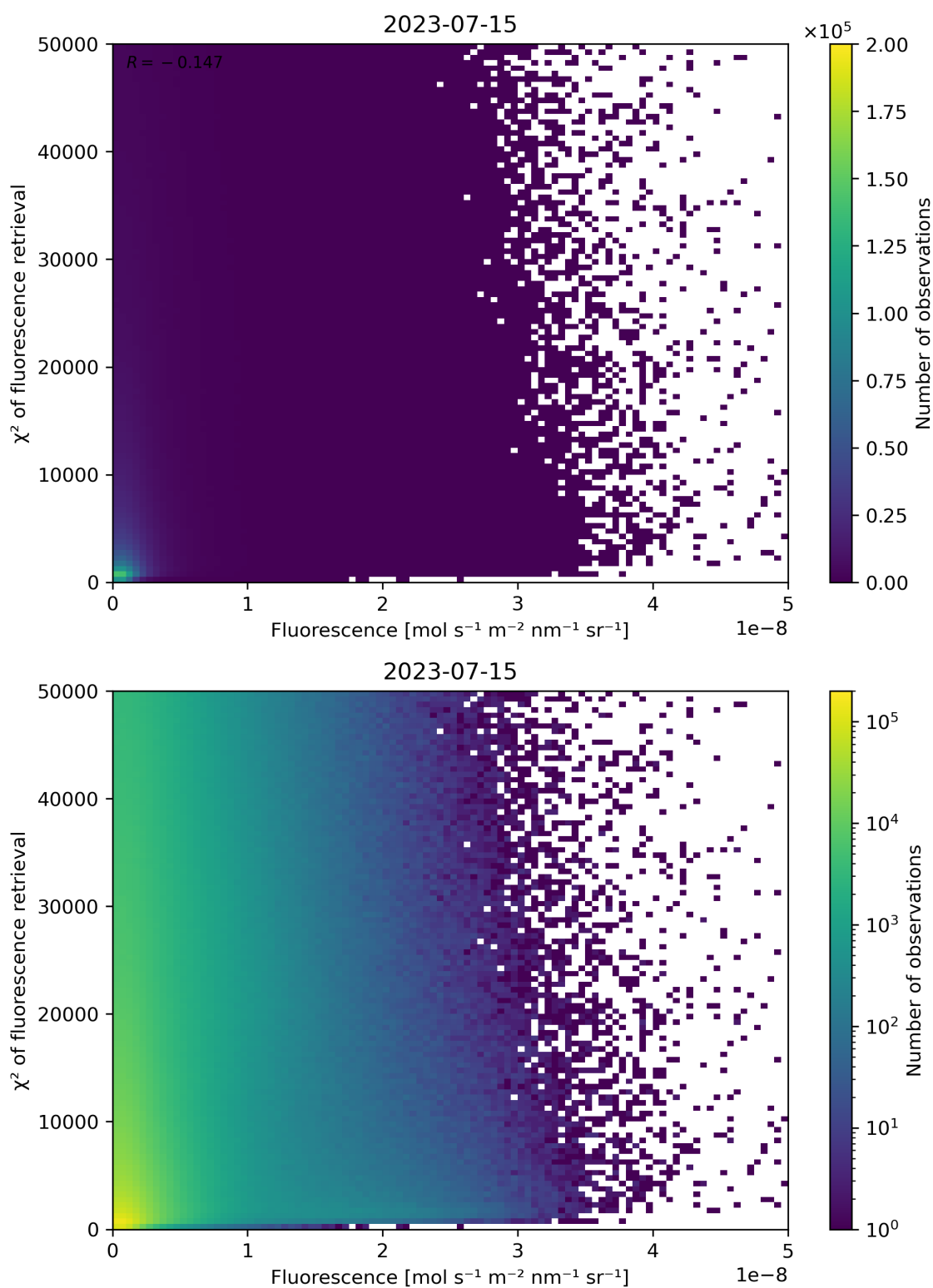
Figure 93: Scatter density plot of “Fluorescence” against “ \chi^2 of fluorescence retrieval” for 2023-07-14 to 2023-07-16.
