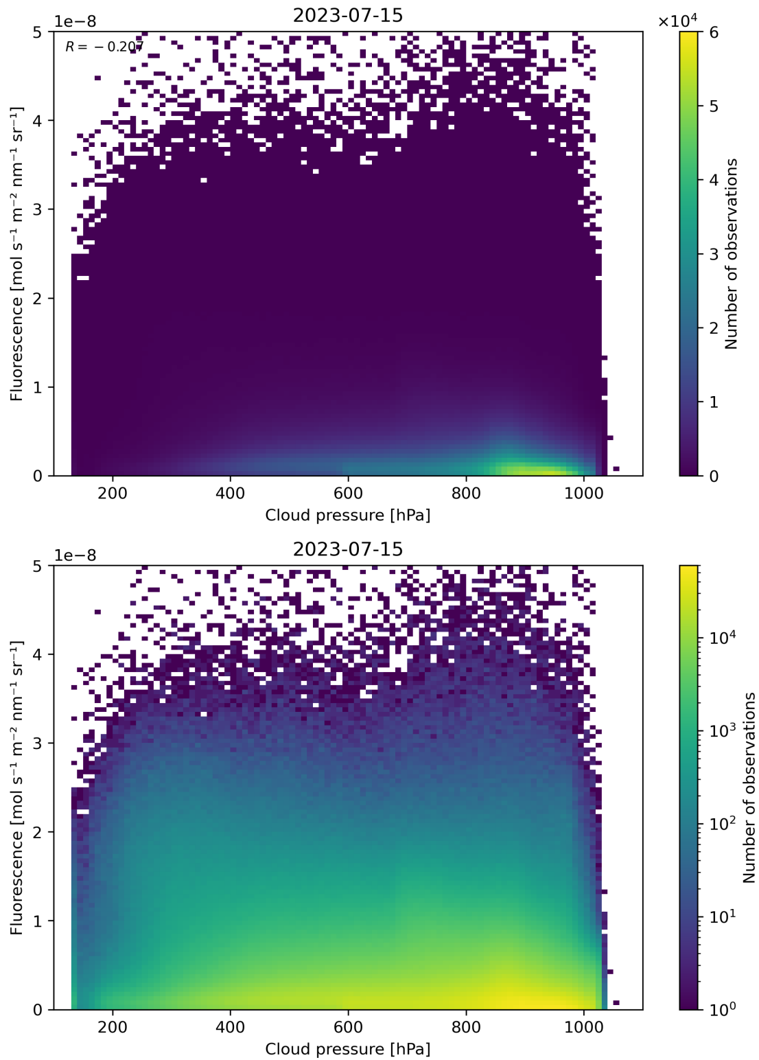
Figure 88: Scatter density plot of “Cloud pressure” against “Fluorescence” for 2023-07-14 to 2023-07-16.
