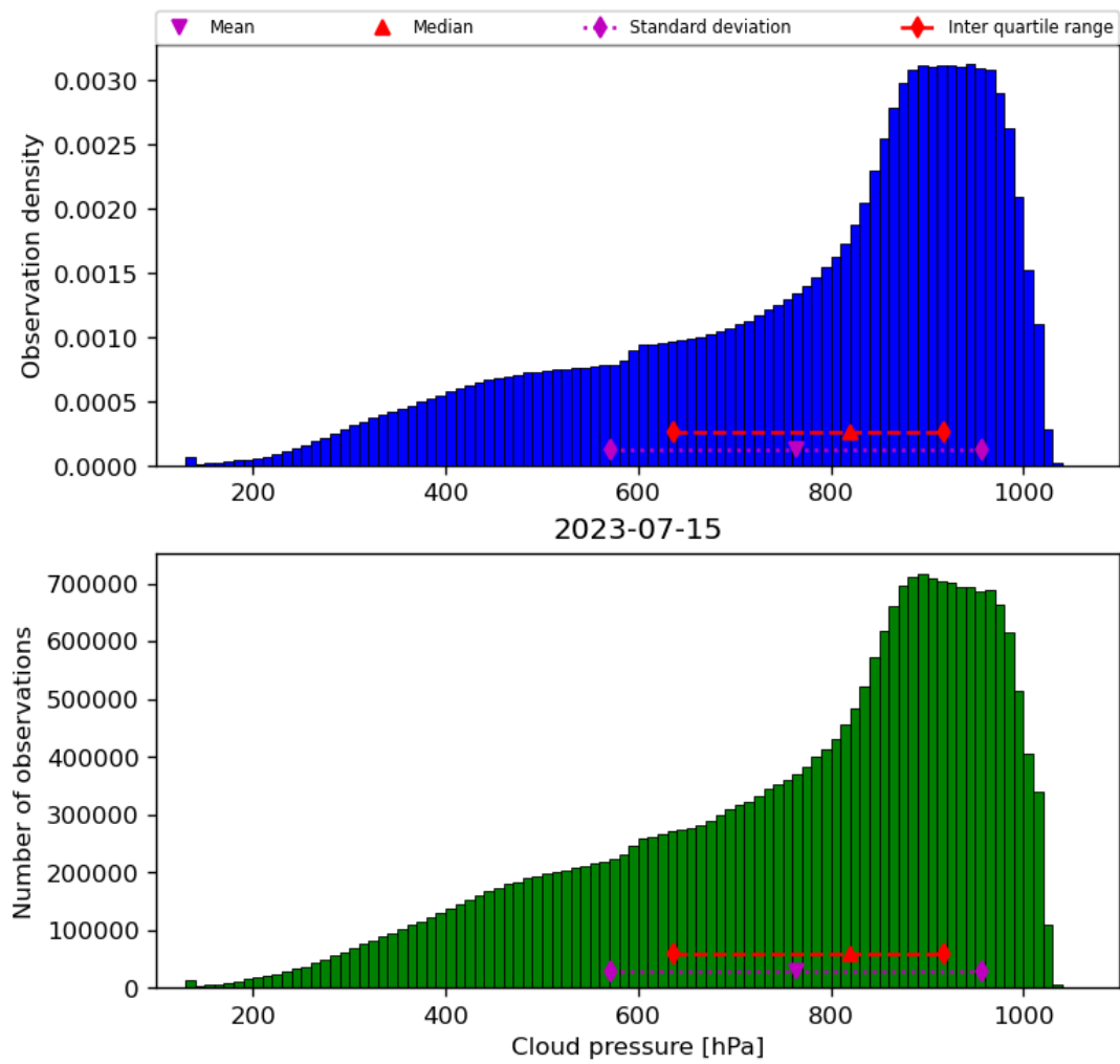
Figure 30: Histogram of “Cloud pressure” for 2023-07-14 to 2023-07-16
