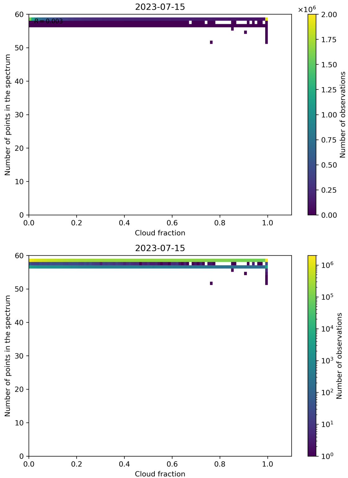
Figure 81: Scatter density plot of “Cloud fraction” against “Number of points in the spectrum” for 2023-07-14 to 2023-07-16.
