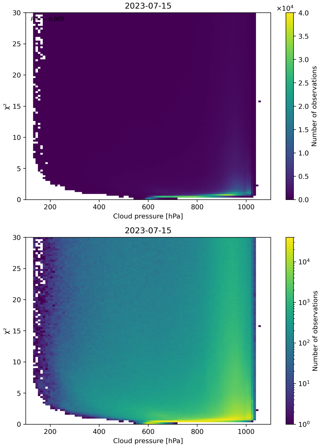
Figure 85: Scatter density plot of “Cloud pressure” against “ \chi^2 ” for 2023-07-14 to 2023-07-16.
