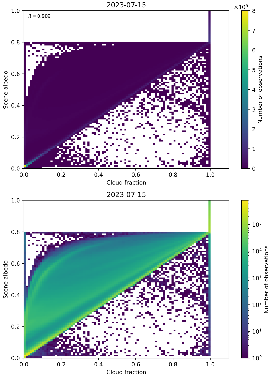
Figure 82: Scatter density plot of “Cloud fraction” against “Scene albedo” for 2023-07-14 to 2023-07-16.
