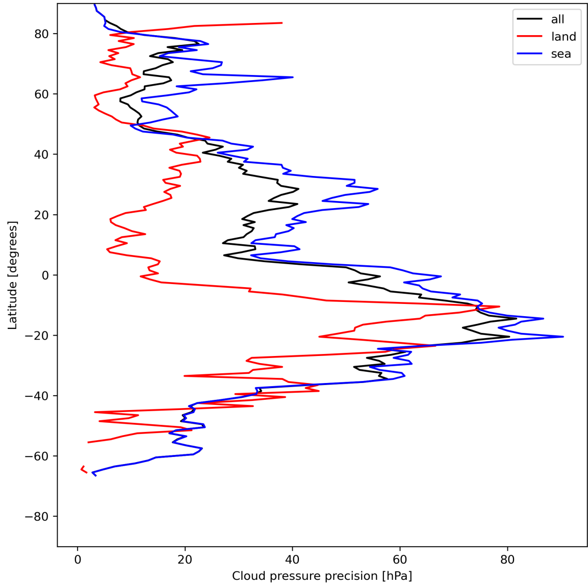
Figure 14: Zonal average of “Cloud pressure precision” for 2023-07-14 to 2023-07-16.
