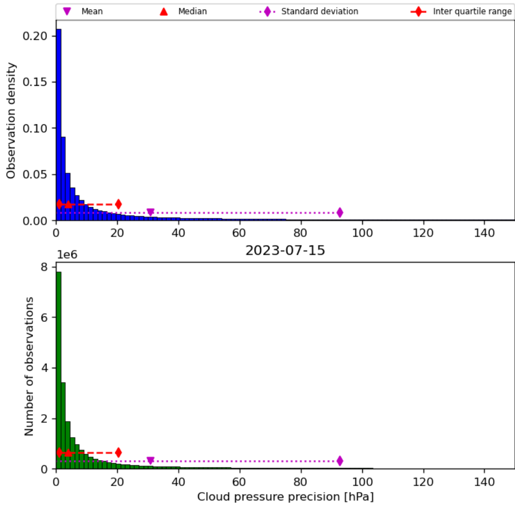
Figure 31: Histogram of “Cloud pressure precision” for 2023-07-14 to 2023-07-16
