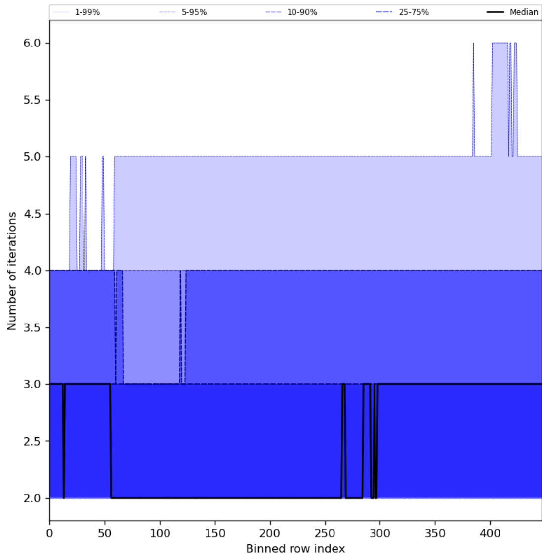
Figure 56: Along track statistics of “Number of iterations” for 2023-07-14 to 2023-07-16
