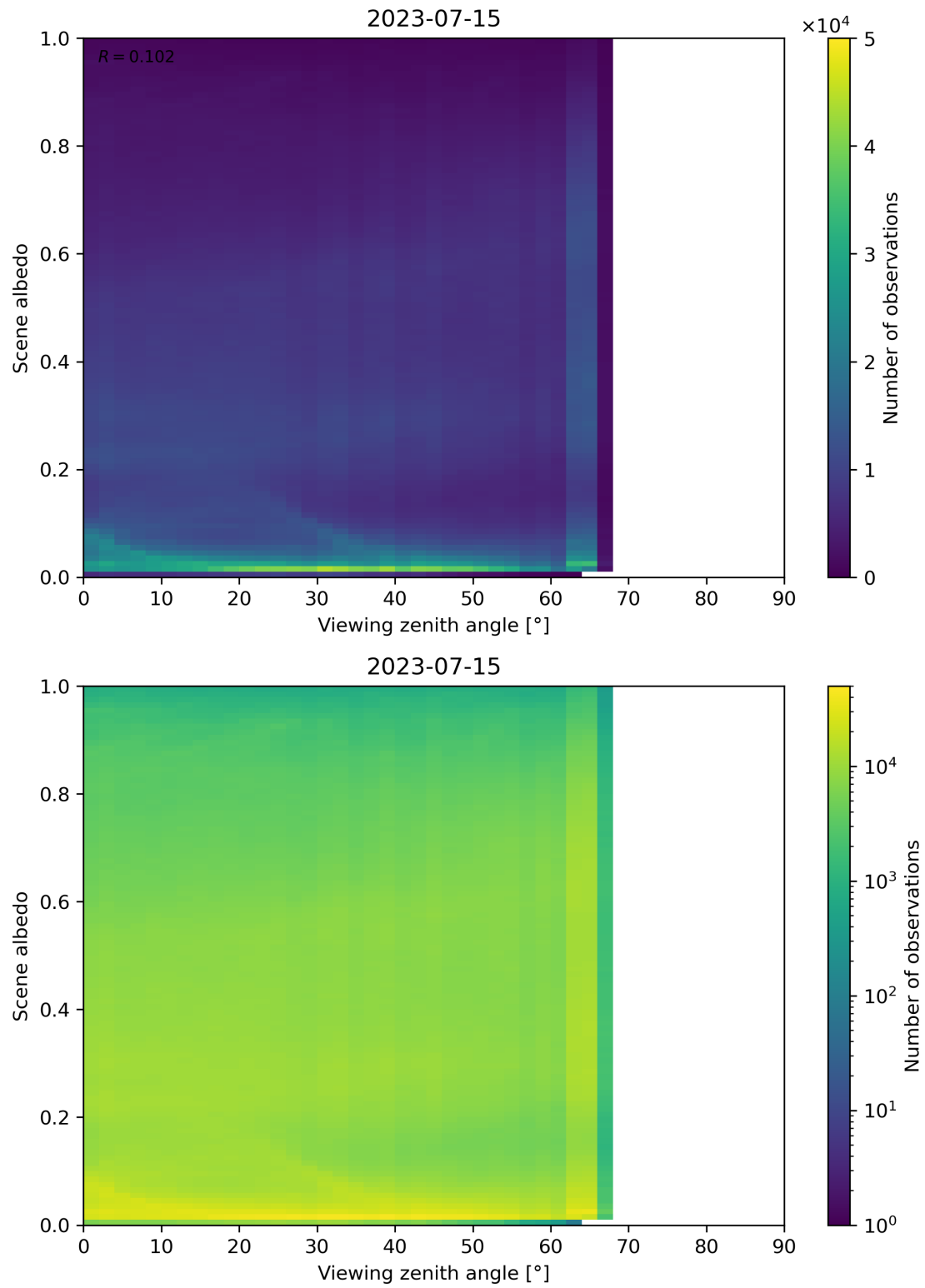
Figure 138: Scatter density plot of “Viewing zenith angle” against “Scene albedo” for 2023-07-14 to 2023-07-16.
