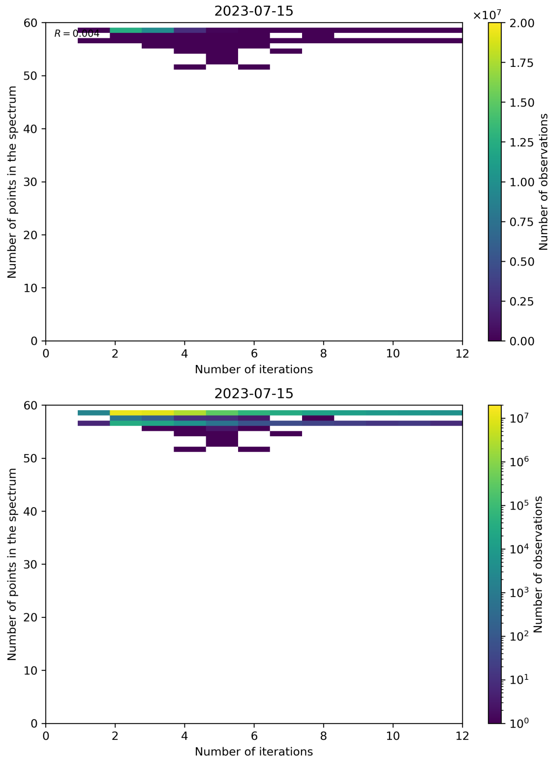
Figure 108: Scatter density plot of “Number of iterations” against “Number of points in the spectrum” for 2023-07-14 to 2023-07-16.
