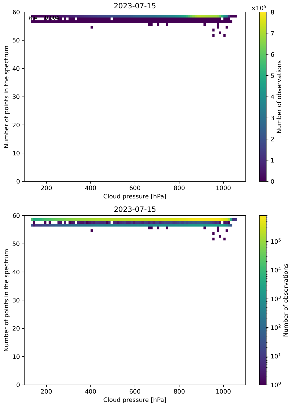
Figure 90: Scatter density plot of “Cloud pressure” against “Number of points in the spectrum” for 2023-07-14 to 2023-07-16.
