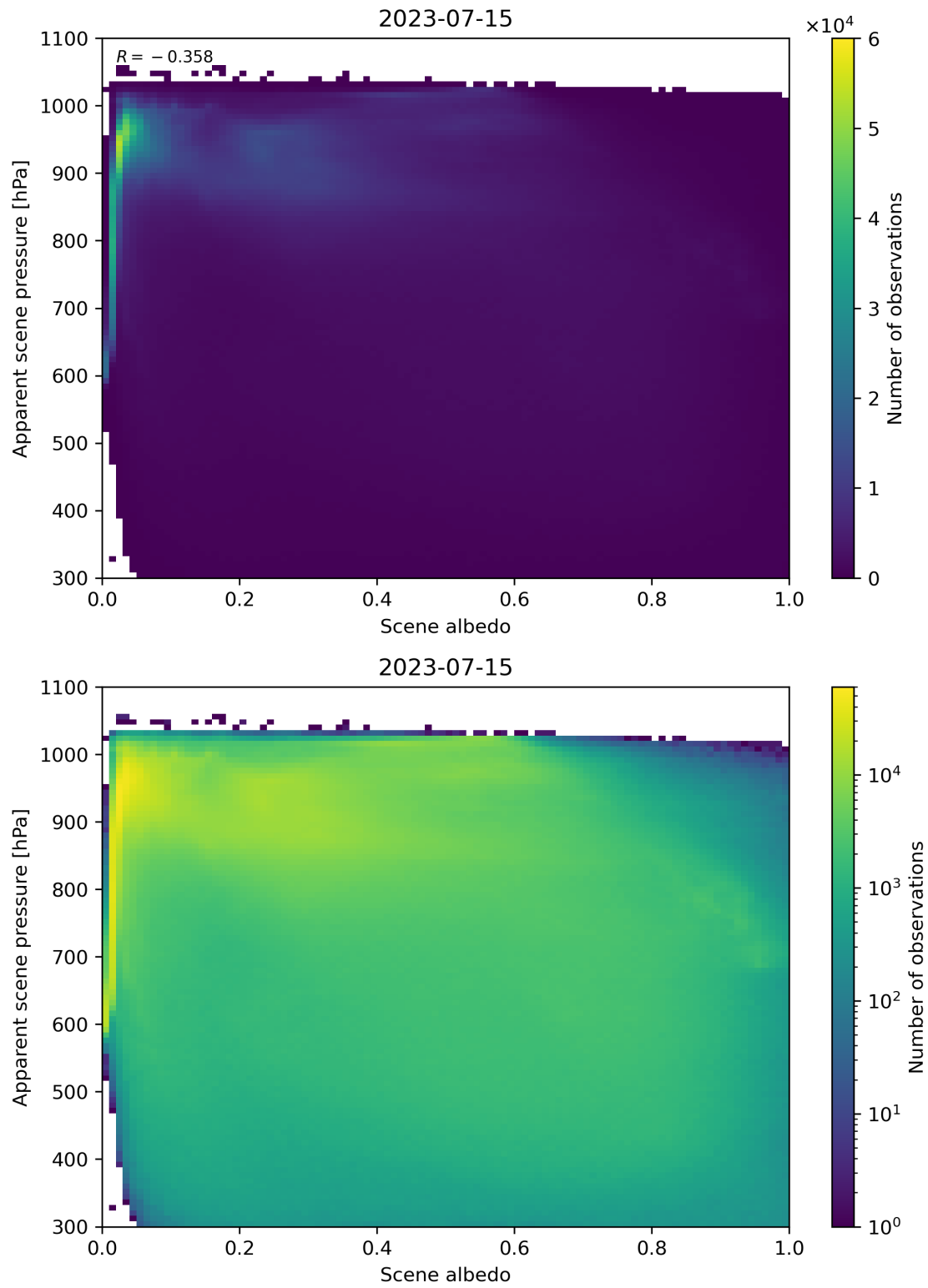
Figure 111: Scatter density plot of “Scene albedo” against “Apparent scene pressure” for 2023-07-14 to 2023-07-16.
