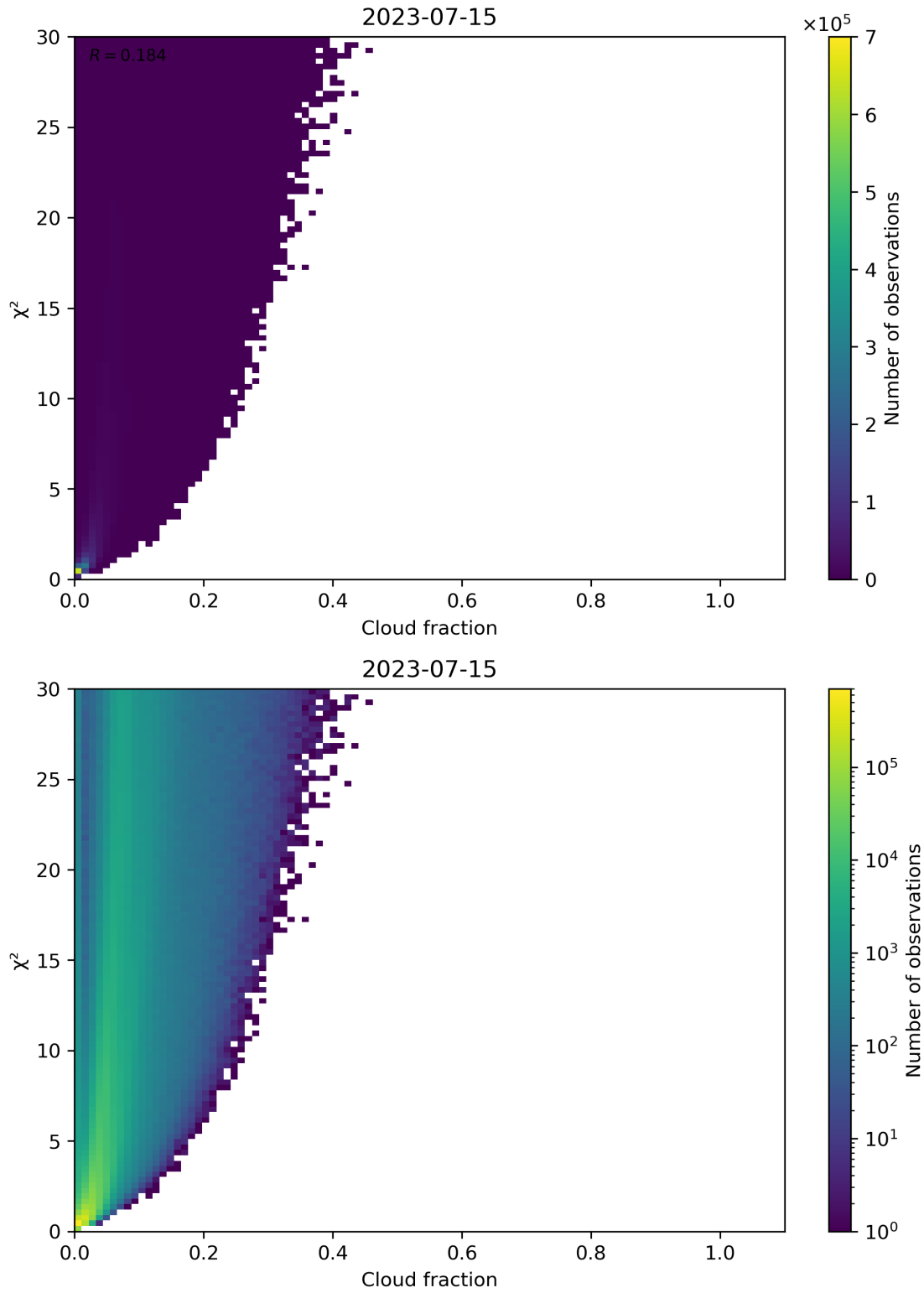
Figure 77: Scatter density plot of “Cloud fraction” against “ \chi^2 ” for 2023-07-14 to 2023-07-16.
