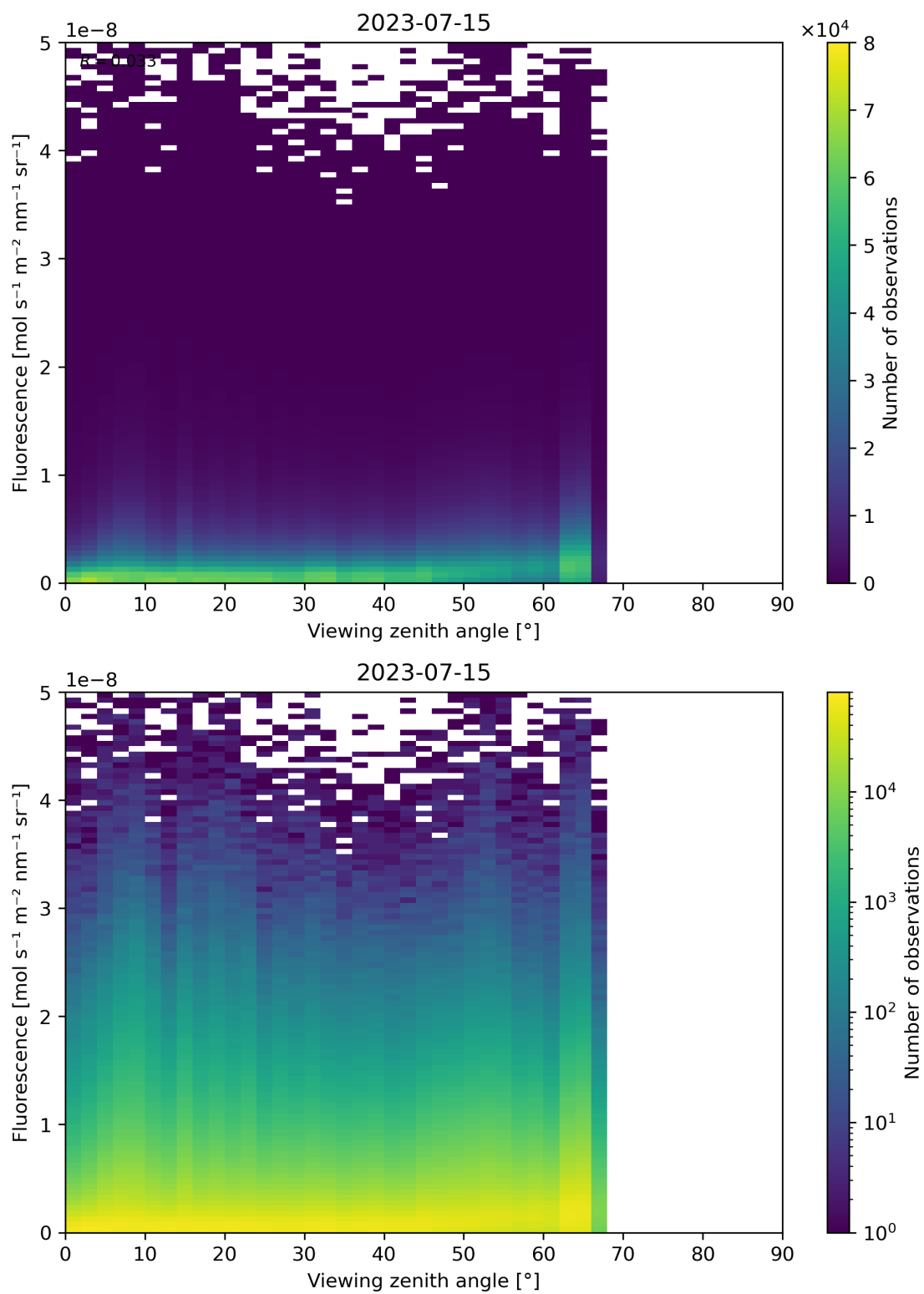
Figure 134: Scatter density plot of “Viewing zenith angle” against “Fluorescence” for 2023-07-14 to 2023-07-16.
