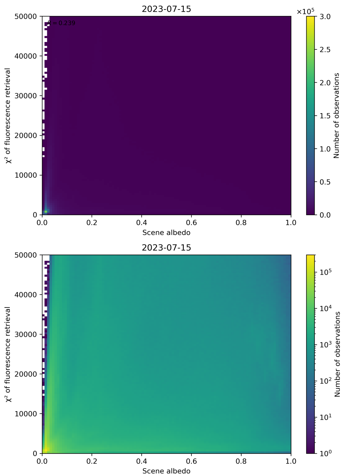
Figure 113: Scatter density plot of “Scene albedo” against “ \chi^2 of fluorescence retrieval” for 2023-07-14 to 2023-07-16.
