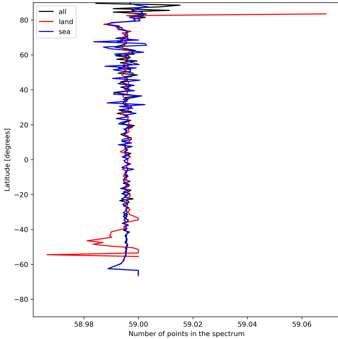
Figure 27: Zonal average of “Number of points in the spectrum” for 2023-07-14 to 2023-07-16.
