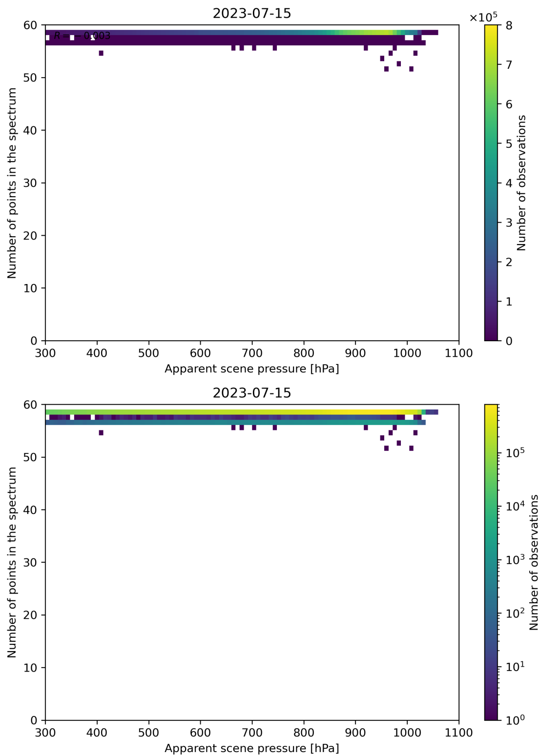
Figure 67: Scatter density plot of “Apparent scene pressure” against “Number of points in the spectrum” for 2023-07-14 to 2023-07-16.
