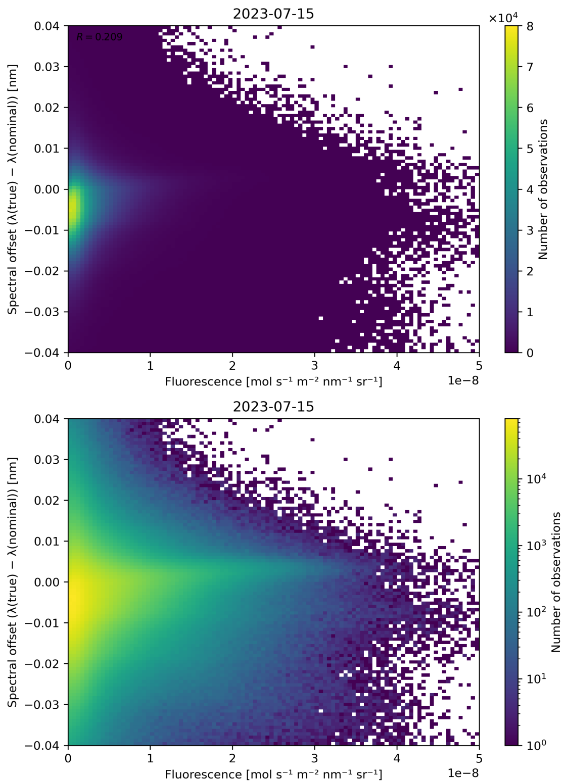
Figure 95: Scatter density plot of “Fluorescence” against “Spectral offset ( \lambda(\text{true}) - \lambda(\text{nominal}) )” for 2023-07-14 to 2023-07-16.
