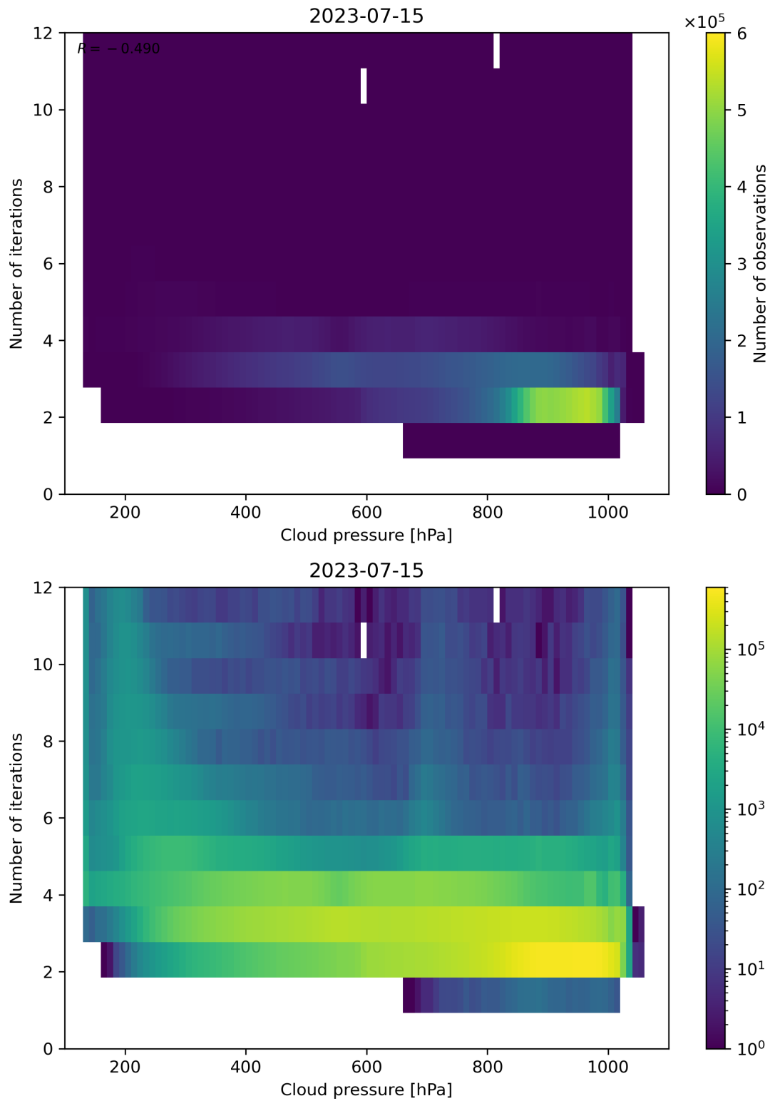
Figure 89: Scatter density plot of “Cloud pressure” against “Number of iterations” for 2023-07-14 to 2023-07-16.
