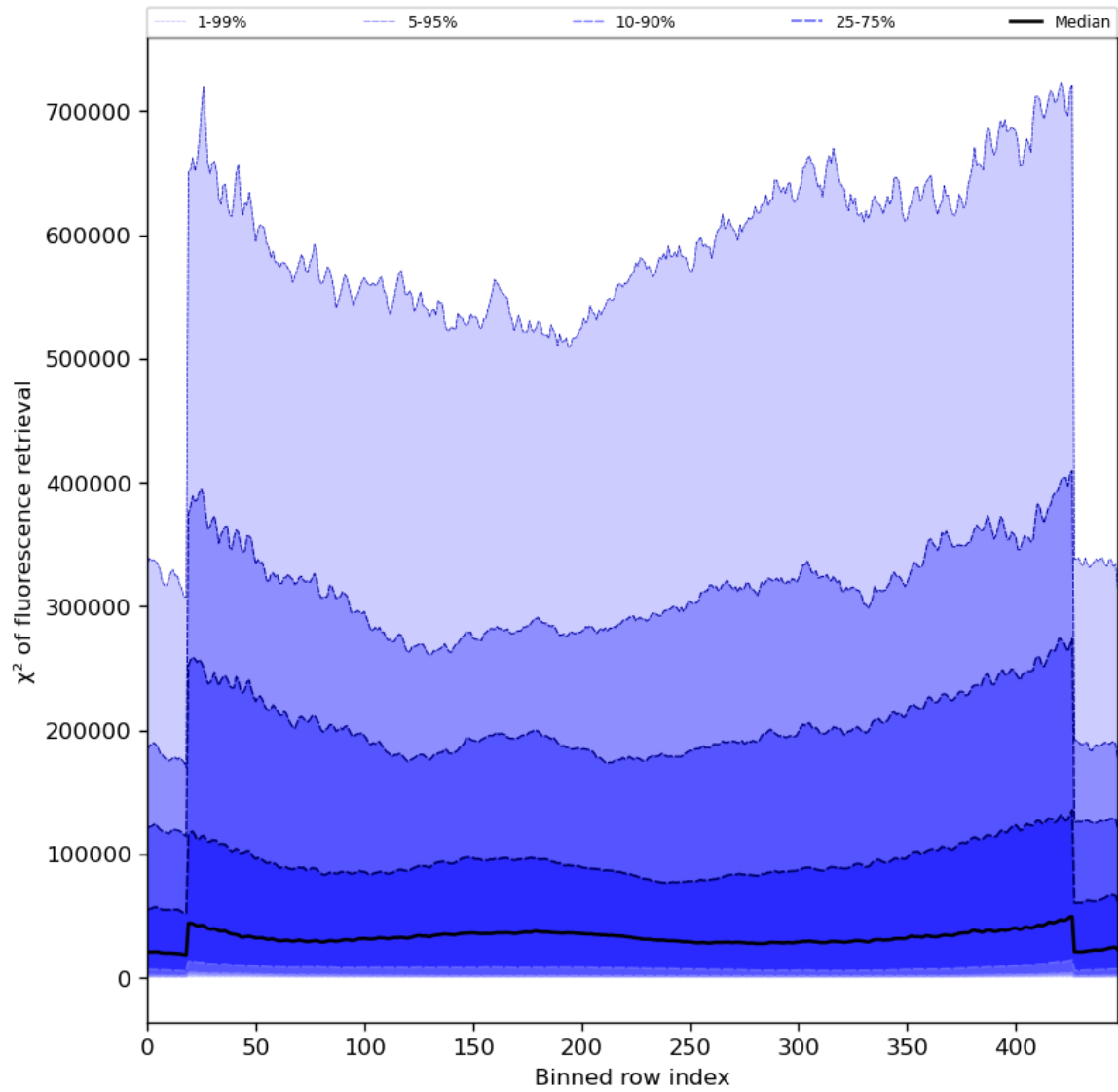
Figure 59: Along track statistics of “ \chi^2 of fluorescence retrieval” for 2023-07-14 to 2023-07-16
