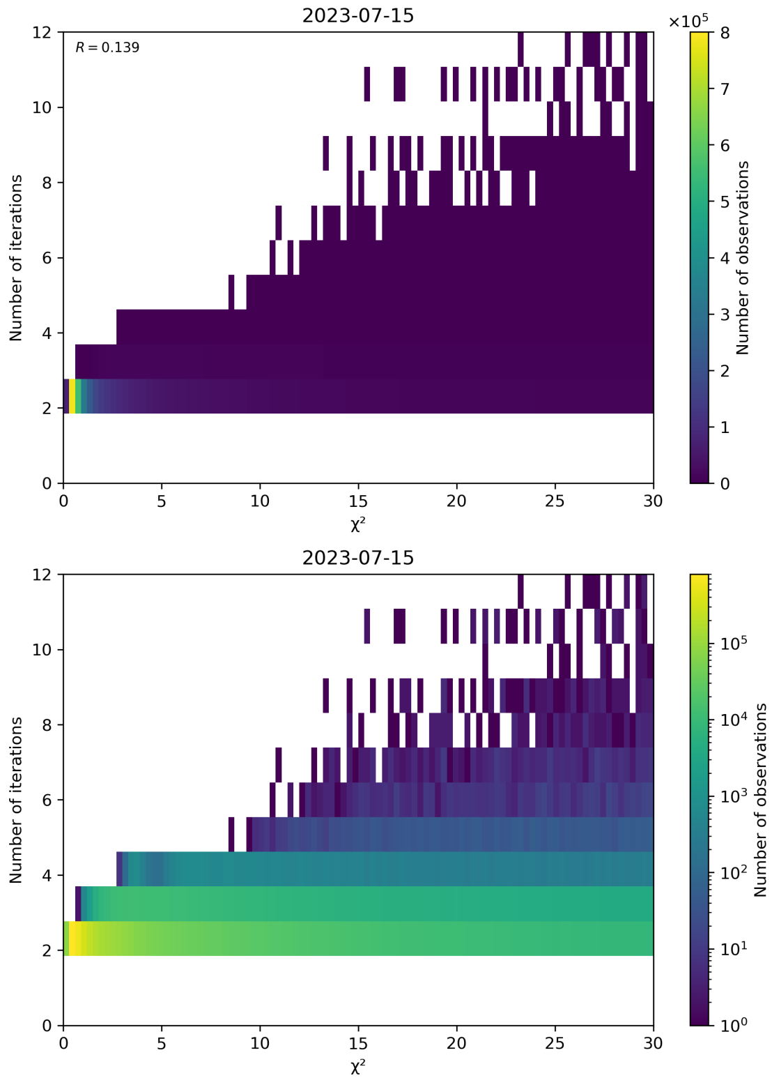
Figure 73: Scatter density plot of “ \chi^2 ” against “Number of iterations” for 2023-07-14 to 2023-07-16.
