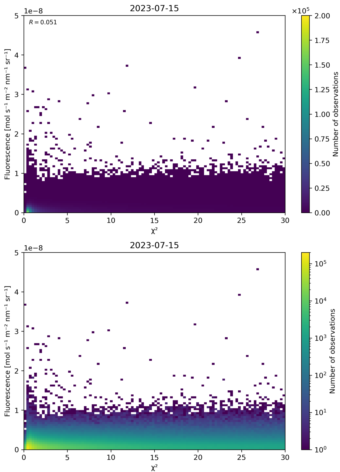
Figure 70: Scatter density plot of “ \chi^2 ” against “Fluorescence” for 2023-07-14 to 2023-07-16.
