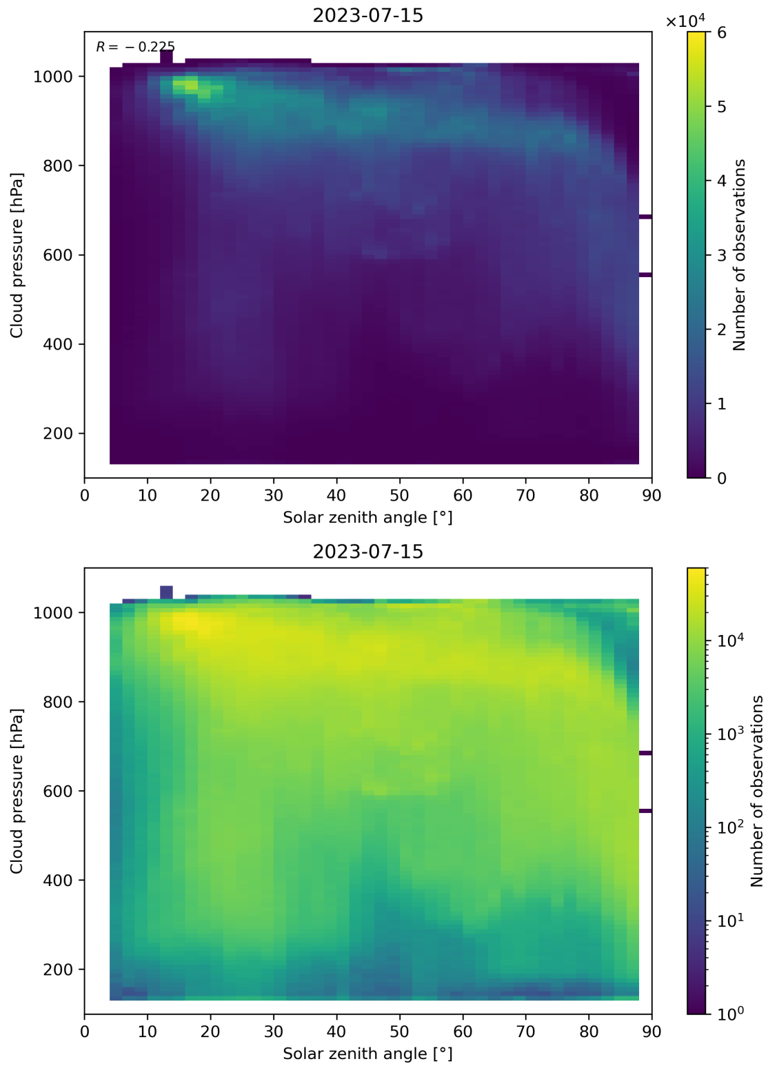
Figure 122: Scatter density plot of “Solar zenith angle” against “Cloud pressure” for 2023-07-14 to 2023-07-16.
