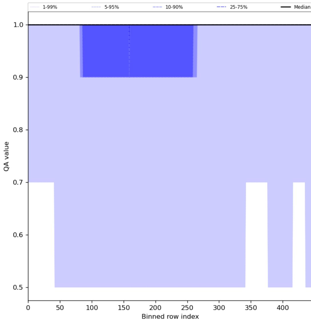
Figure 46: Along track statistics of “QA value” for 2023-07-14 to 2023-07-16
