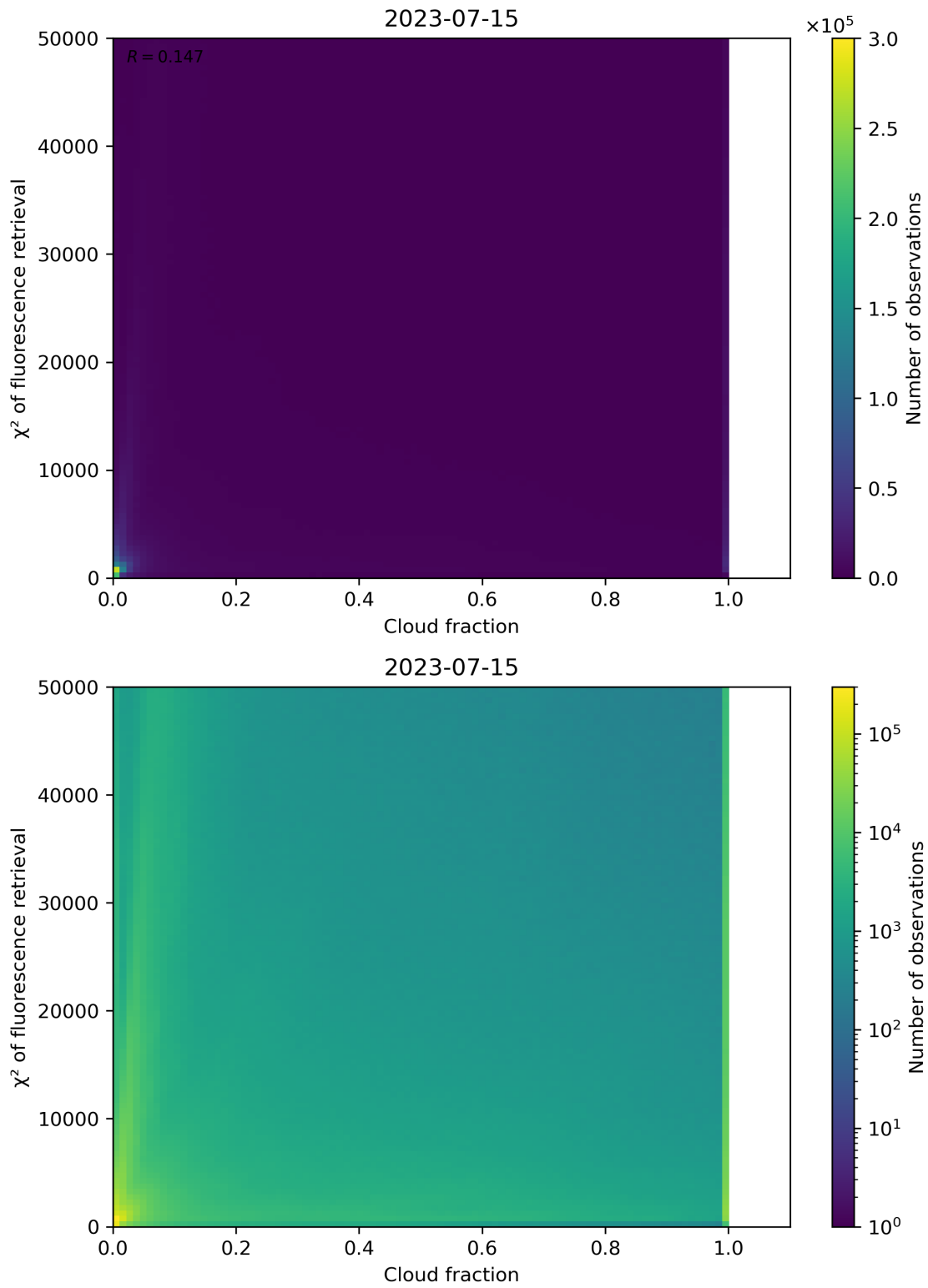
Figure 78: Scatter density plot of “Cloud fraction” against “ \chi^2 of fluorescence retrieval” for 2023-07-14 to 2023-07-16.
