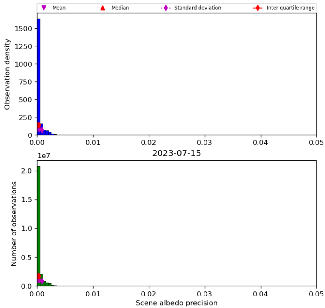
Figure 35: Histogram of “Scene albedo precision” for 2023-07-14 to 2023-07-16
