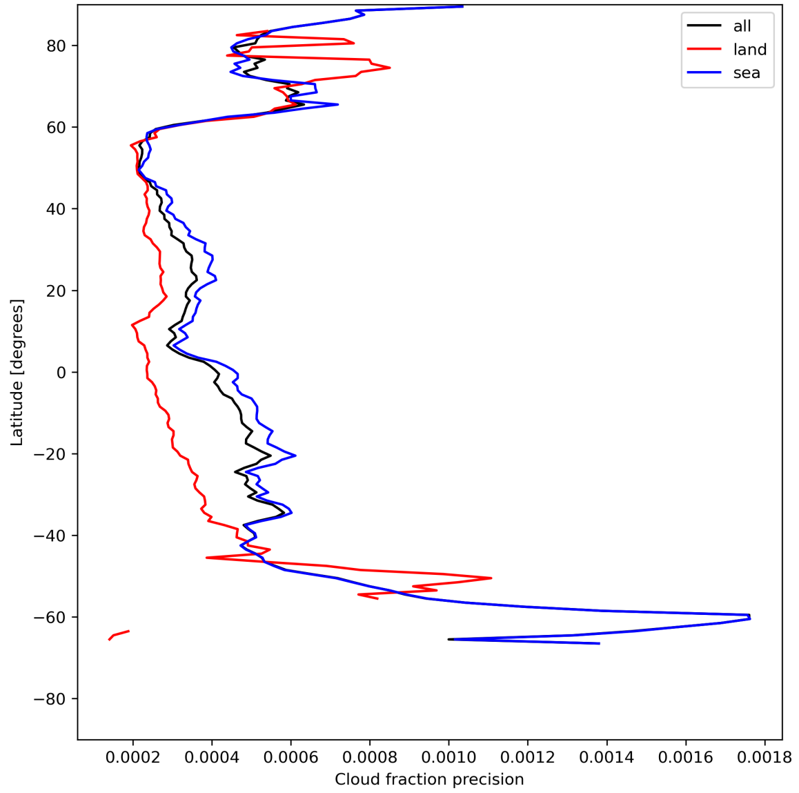
Figure 16: Zonal average of “Cloud fraction precision” for 2023-07-14 to 2023-07-16.
