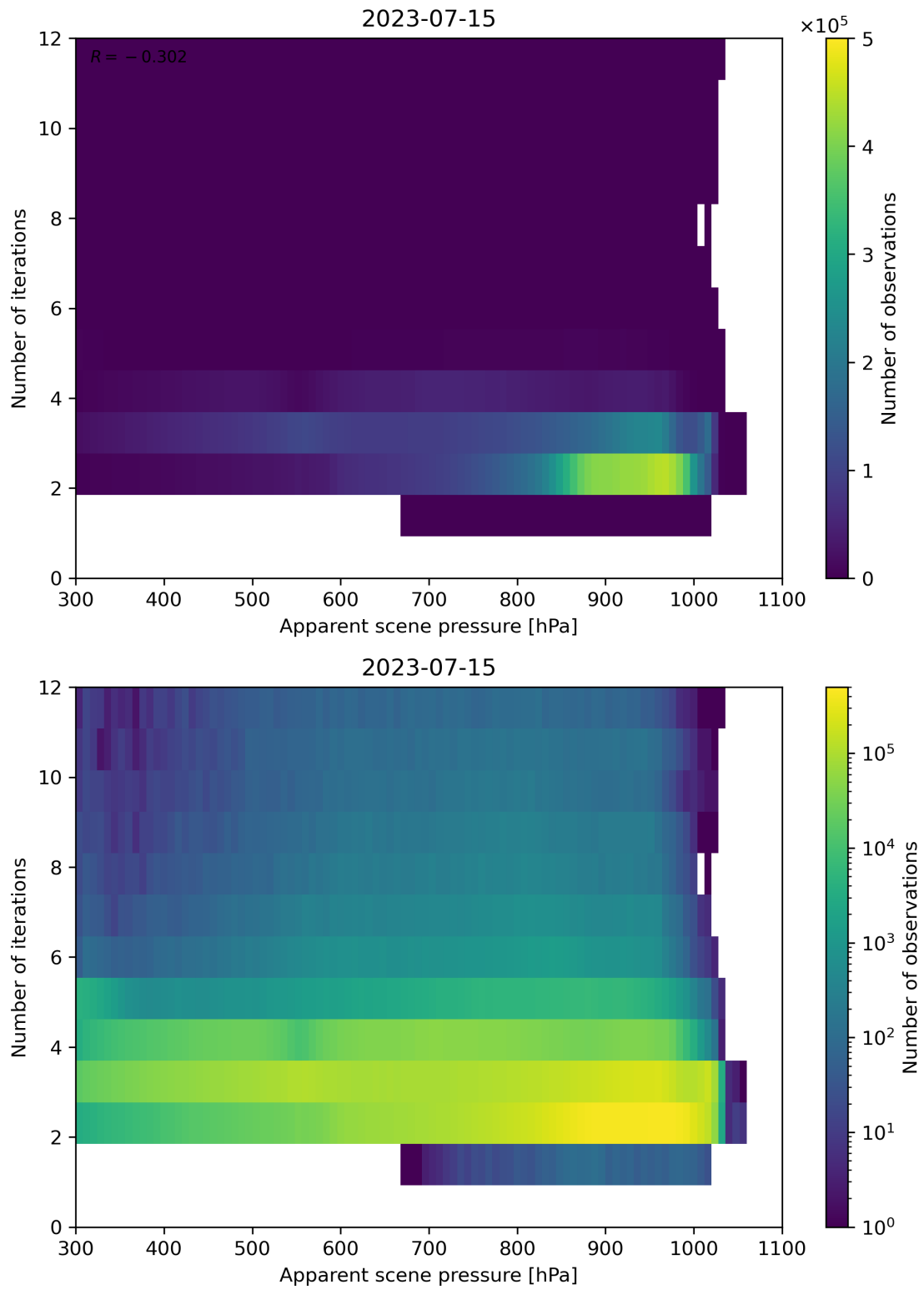
Figure 66: Scatter density plot of “Apparent scene pressure” against “Number of iterations” for 2023-07-14 to 2023-07-16.
