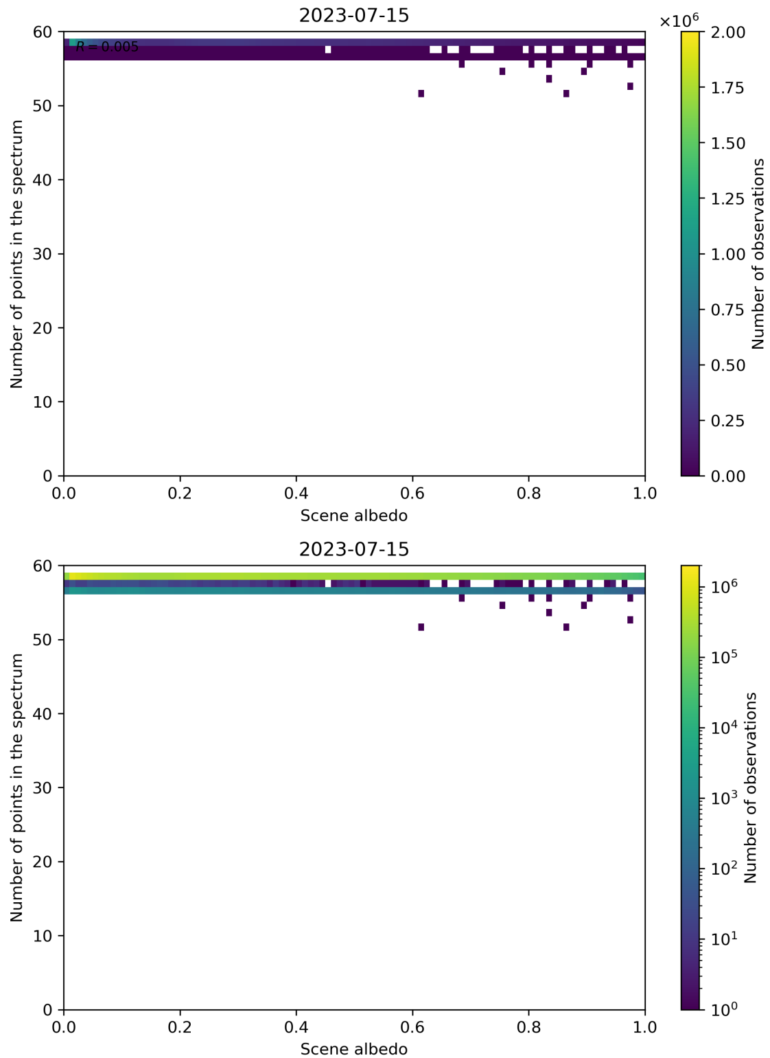
Figure 116: Scatter density plot of “Scene albedo” against “Number of points in the spectrum” for 2023-07-14 to 2023-07-16.
