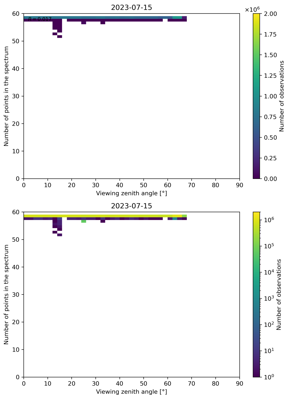
Figure 137: Scatter density plot of “Viewing zenith angle” against “Number of points in the spectrum” for 2023-07-14 to 2023-07-16.
