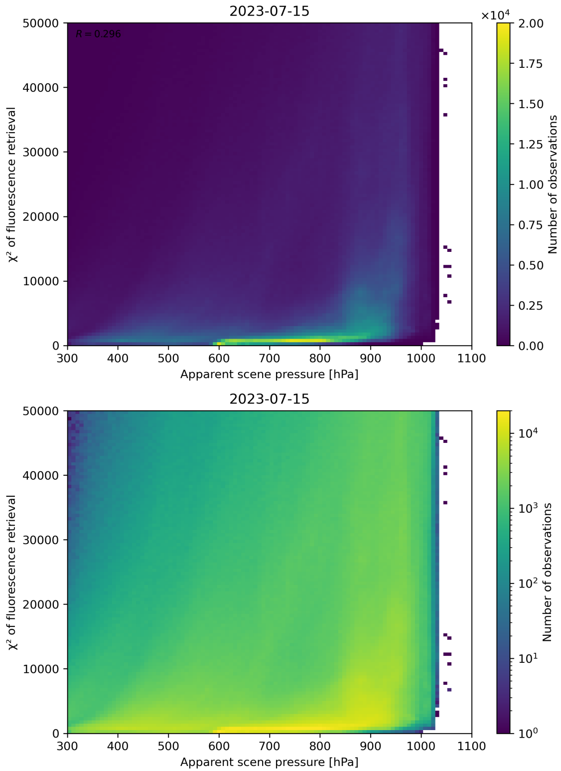
Figure 64: Scatter density plot of “Apparent scene pressure” against “ \chi^2 of fluorescence retrieval” for 2023-07-14 to 2023-07-16.
