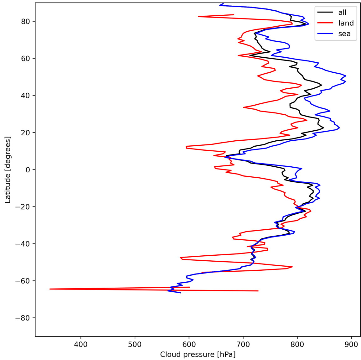
Figure 13: Zonal average of “Cloud pressure” for 2023-07-14 to 2023-07-16.
