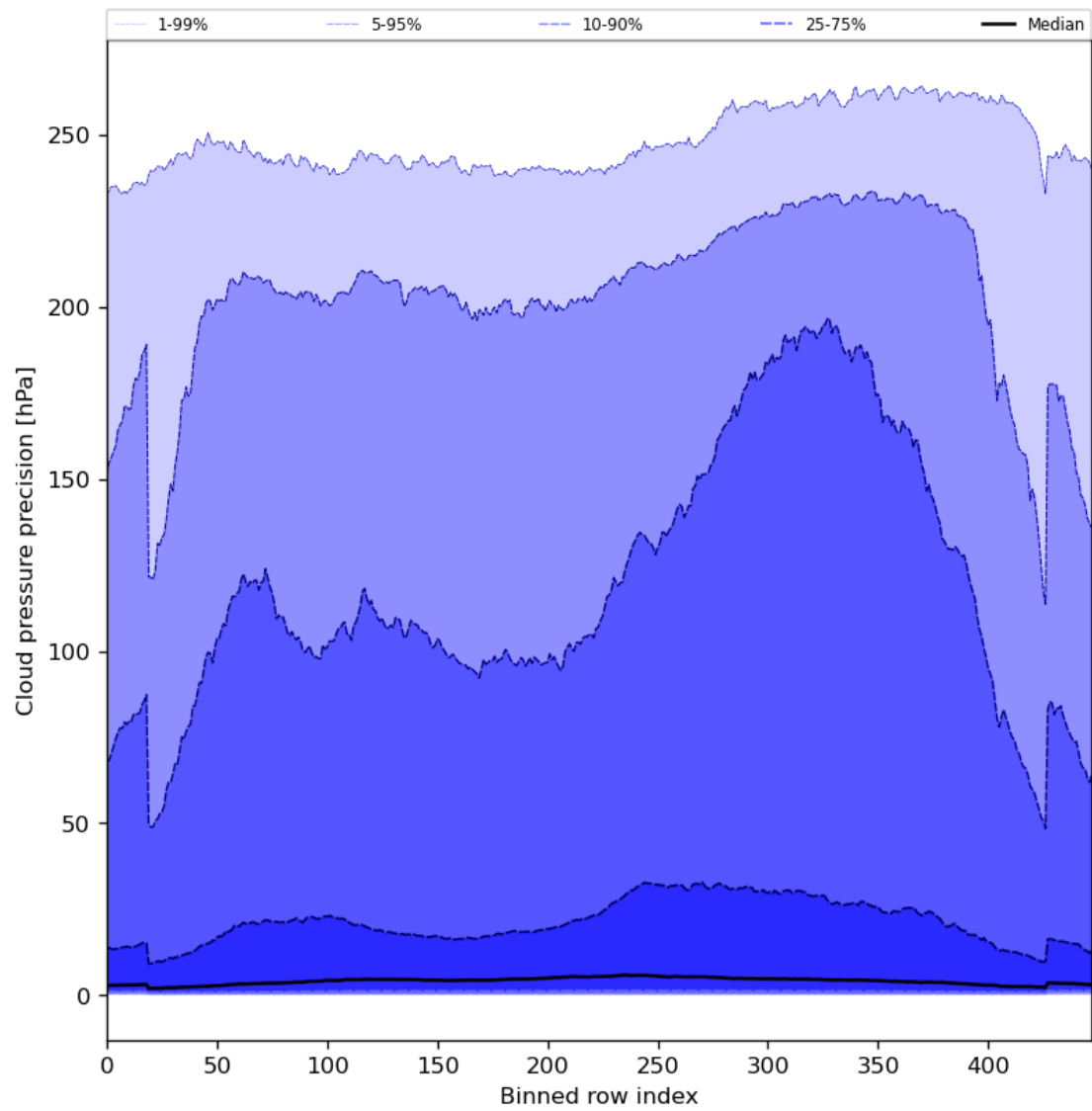
Figure 48: Along track statistics of “Cloud pressure precision” for 2023-07-14 to 2023-07-16
