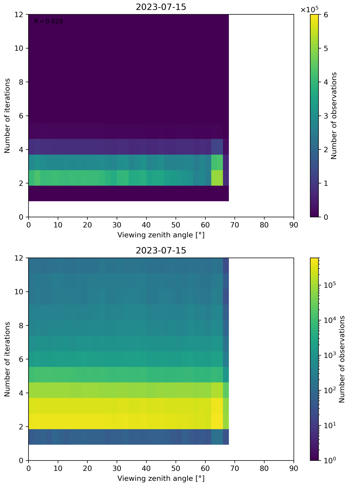
Figure 136: Scatter density plot of “Viewing zenith angle” against “Number of iterations” for 2023-07-14 to 2023-07-16.
