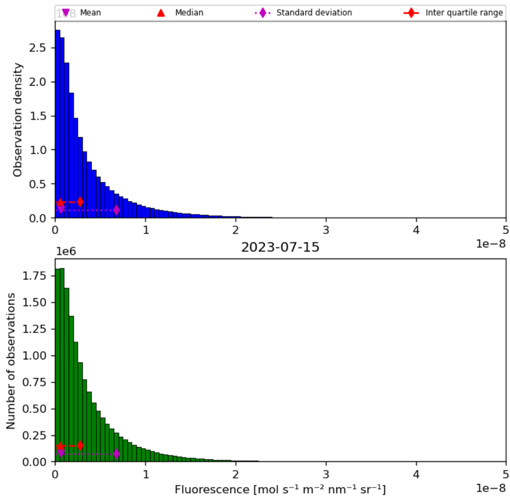
Figure 40: Histogram of “Fluorescence” for 2023-07-14 to 2023-07-16
