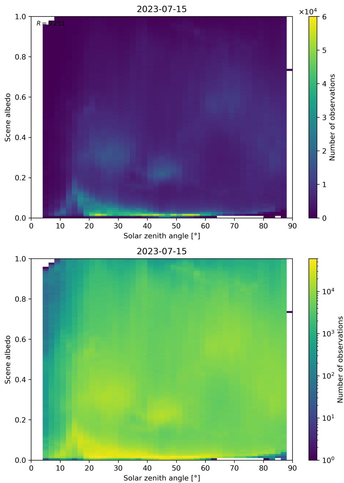
Figure 127: Scatter density plot of “Solar zenith angle” against “Scene albedo” for 2023-07-14 to 2023-07-16.
