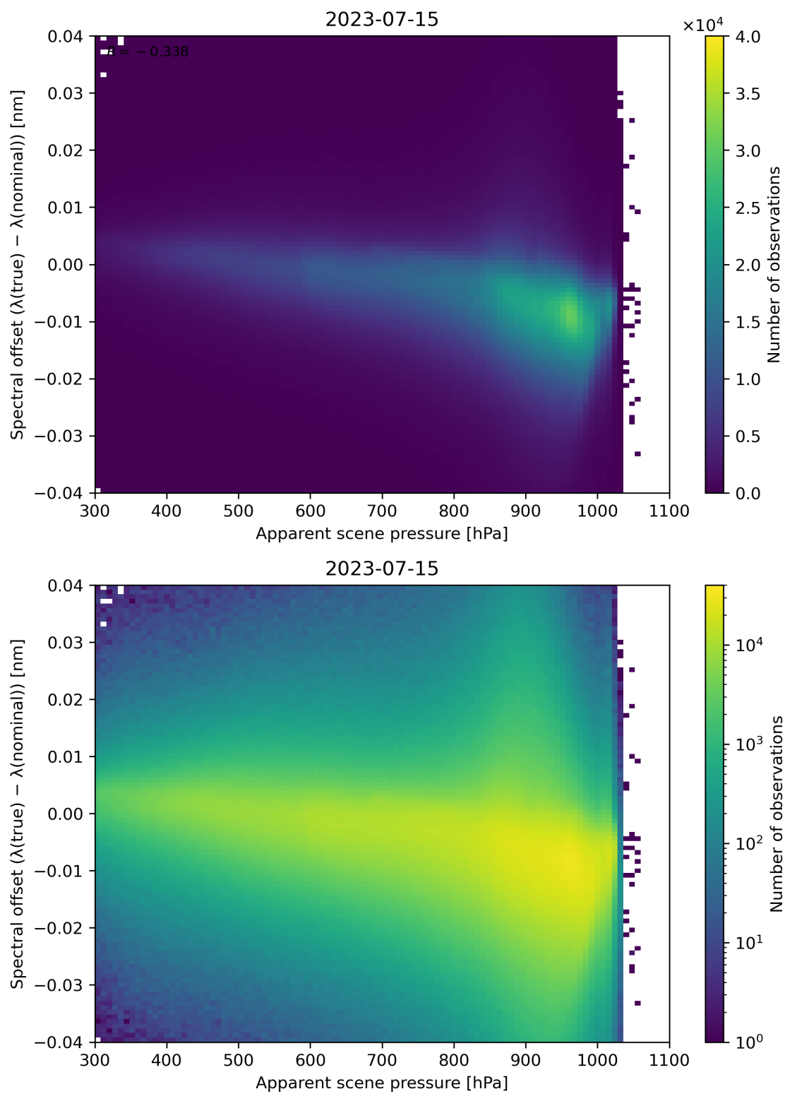
Figure 68: Scatter density plot of “Apparent scene pressure” against “Spectral offset ( \lambda(\text{true}) - \lambda(\text{nominal}) )” for 2023-07-14 to 2023-07-16.
