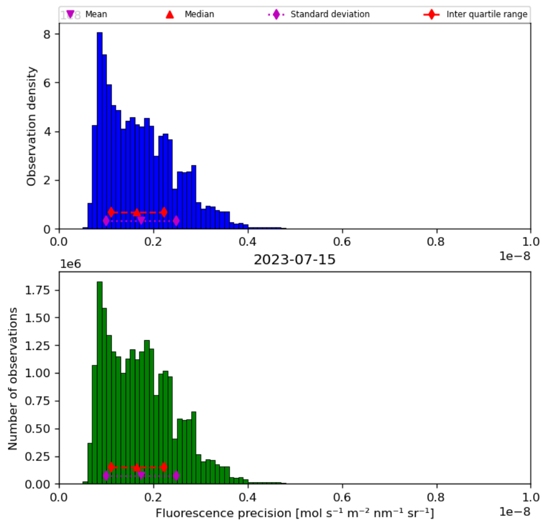
Figure 41: Histogram of “Fluorescence precision” for 2023-07-14 to 2023-07-16
