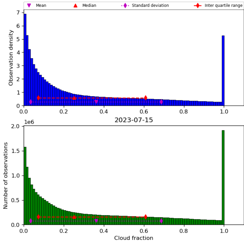
Figure 32: Histogram of “Cloud fraction” for 2023-07-14 to 2023-07-16
