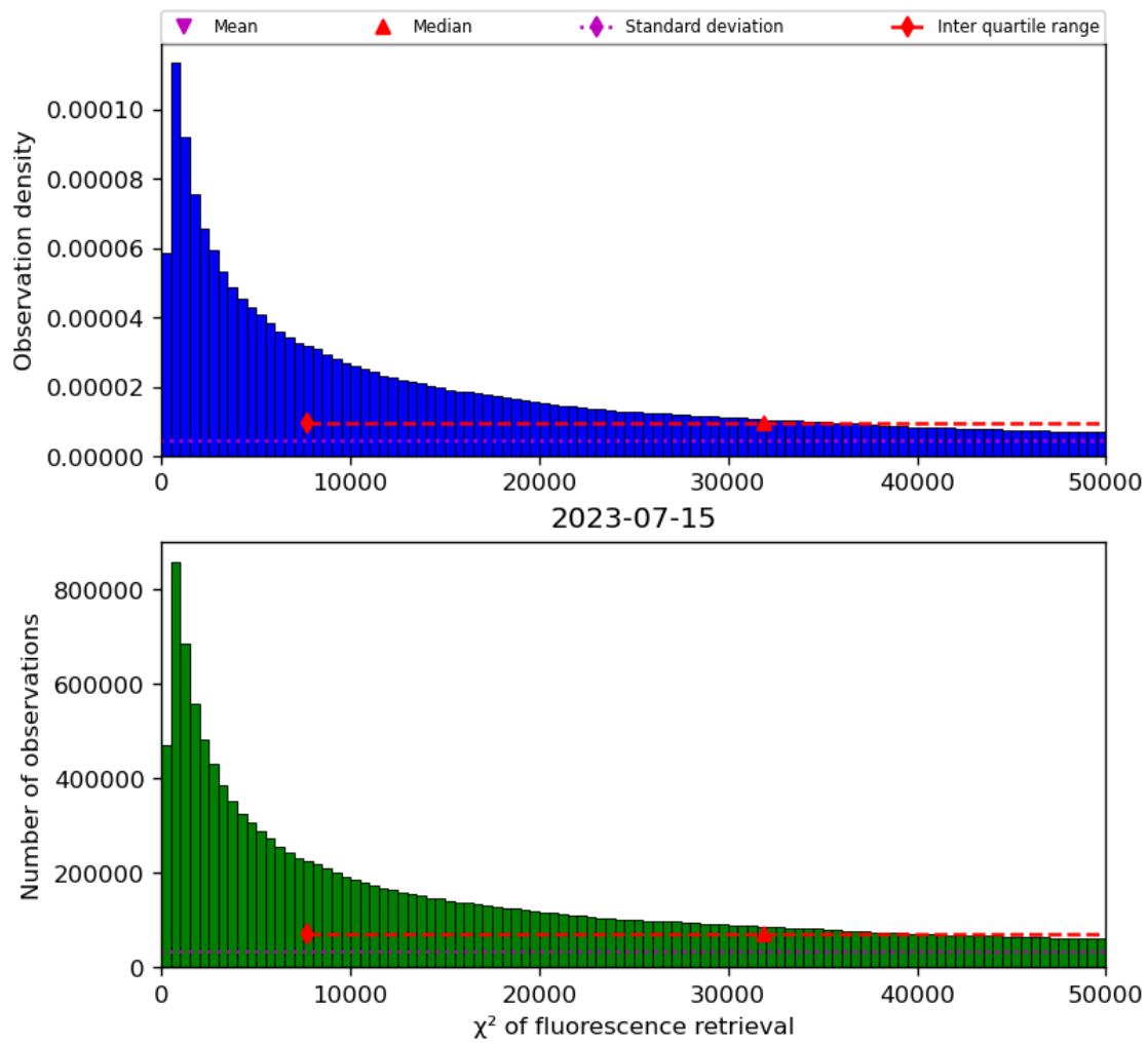
Figure 42: Histogram of “ \chi^2 of fluorescence retrieval” for 2023-07-14 to 2023-07-16
