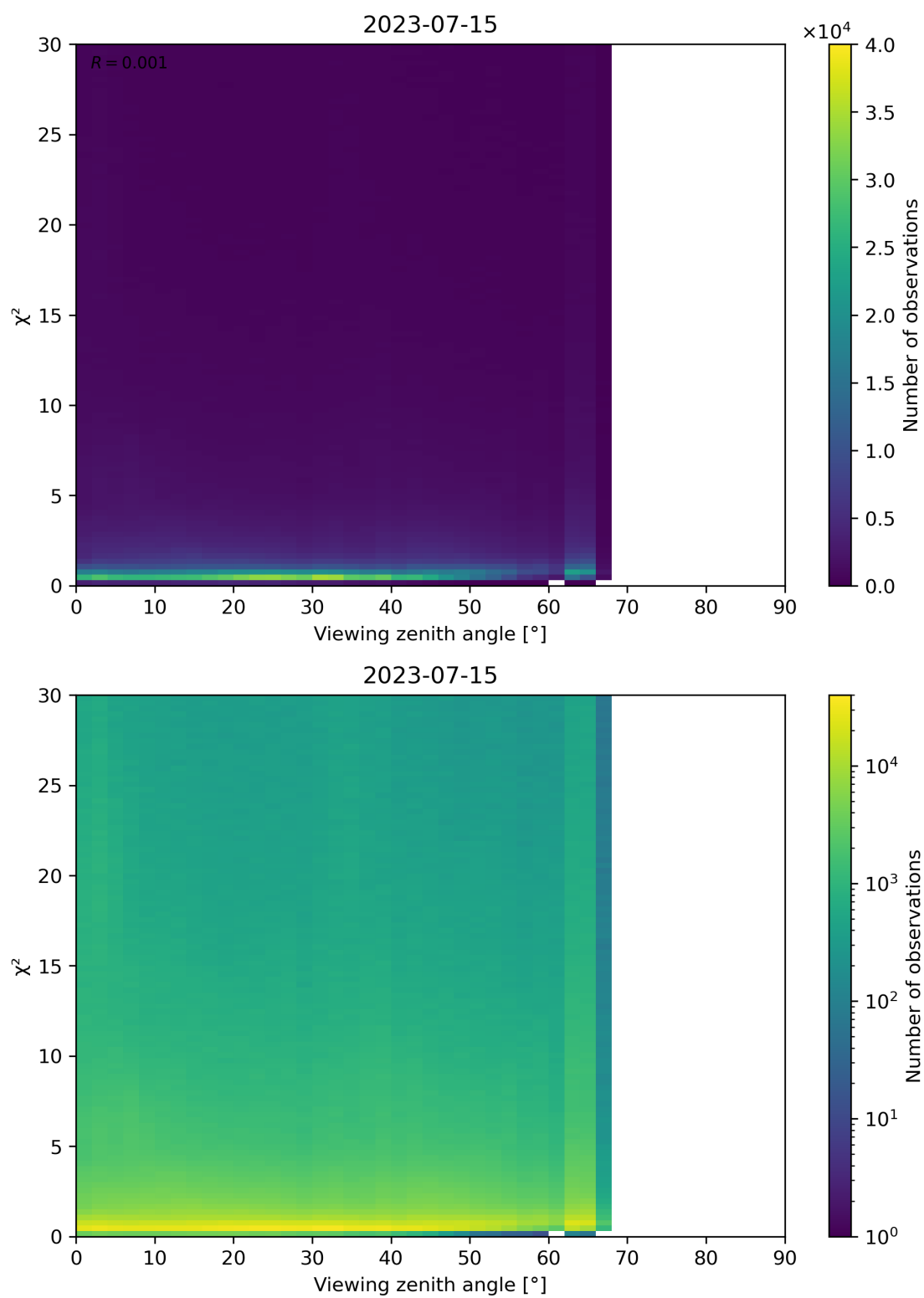
Figure 130: Scatter density plot of “Viewing zenith angle” against “ \chi^2 ” for 2023-07-14 to 2023-07-16.
