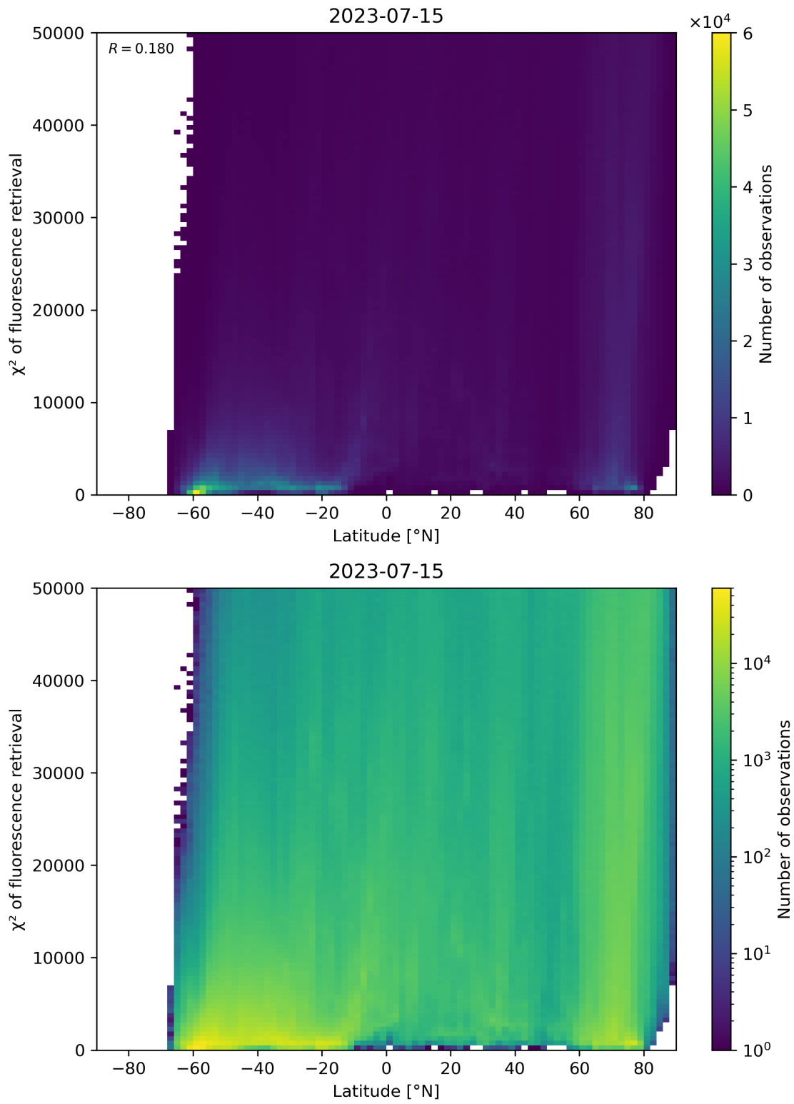
Figure 98: Scatter density plot of “Latitude” against “ \chi^2 of fluorescence retrieval” for 2023-07-14 to 2023-07-16.
