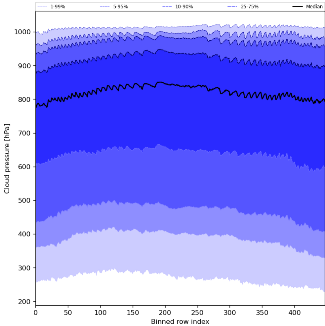
Figure 47: Along track statistics of “Cloud pressure” for 2023-07-14 to 2023-07-16
