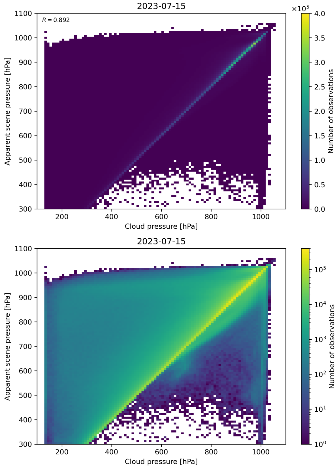
Figure 84: Scatter density plot of “Cloud pressure” against “Apparent scene pressure” for 2023-07-14 to 2023-07-16.
