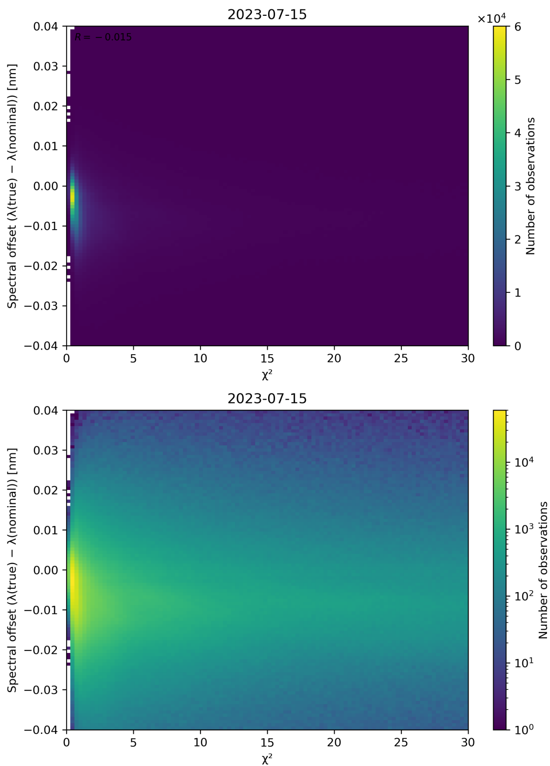
Figure 75: Scatter density plot of " \chi^2 " against "Spectral offset ( \lambda(\text{true}) - \lambda(\text{nominal}) )" for 2023-07-14 to 2023-07-16.
