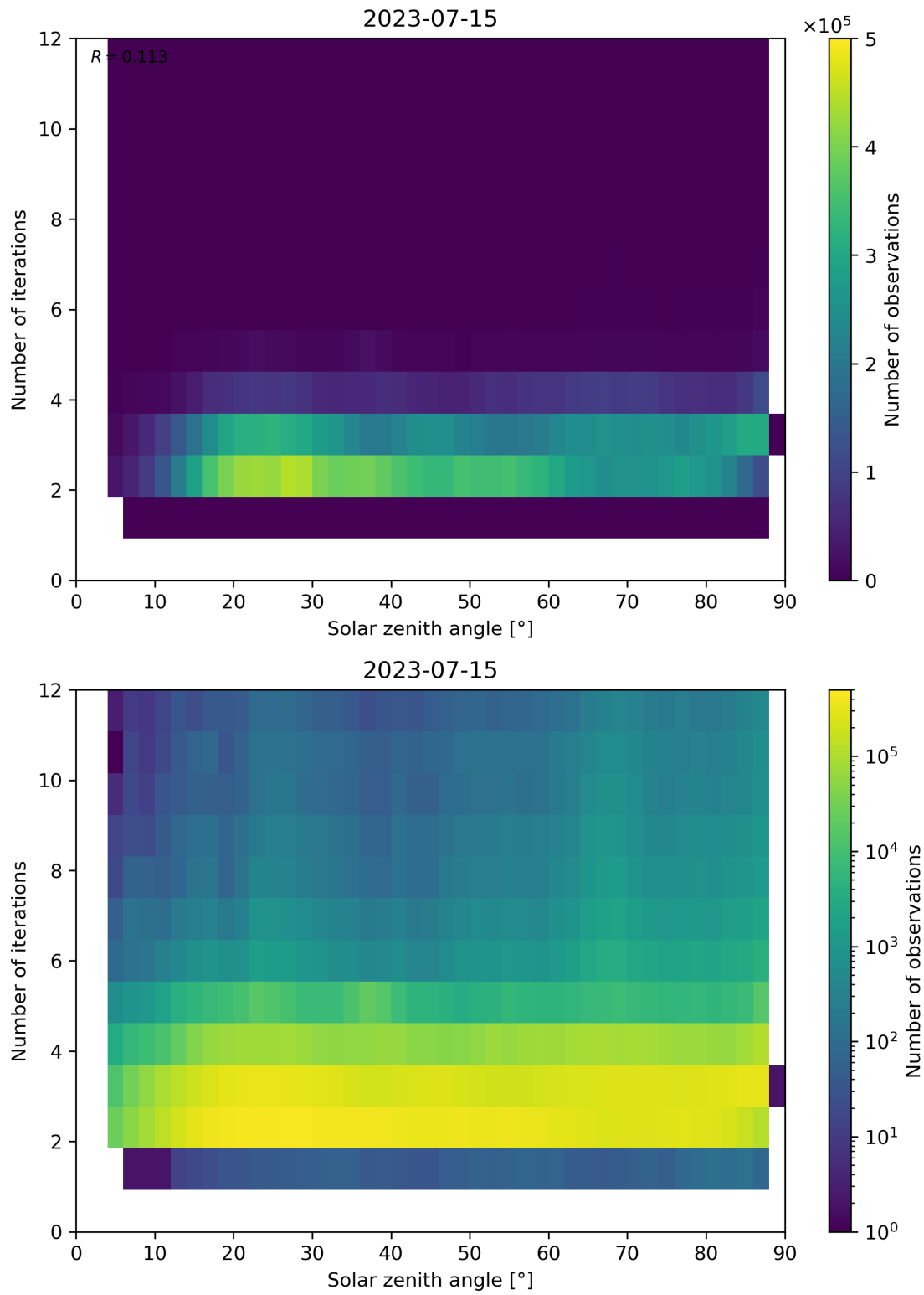
Figure 125: Scatter density plot of “Solar zenith angle” against “Number of iterations” for 2023-07-14 to 2023-07-16.
