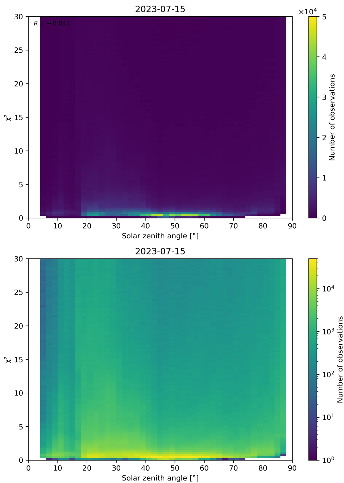
Figure 119: Scatter density plot of “Solar zenith angle” against “ \chi^2 ” for 2023-07-14 to 2023-07-16.
