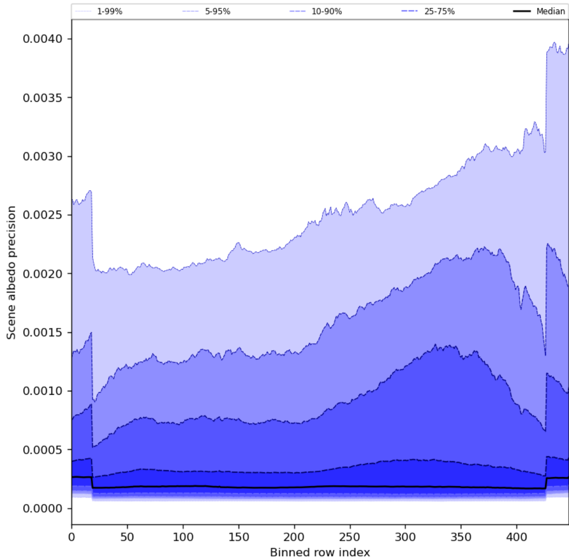
Figure 52: Along track statistics of “Scene albedo precision” for 2023-07-14 to 2023-07-16
