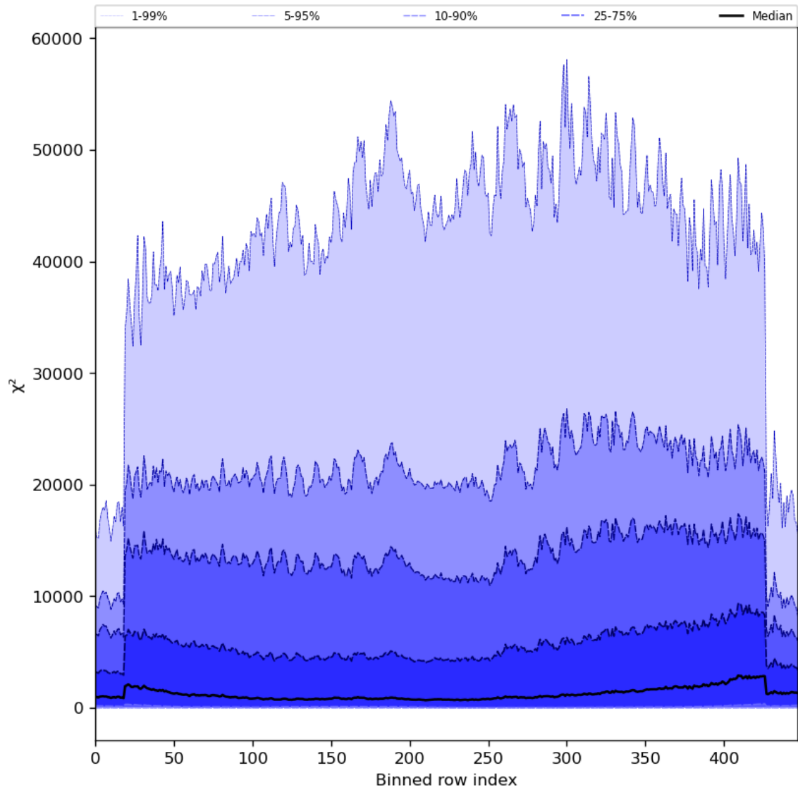
Figure 55: Along track statistics of “ \chi^2 ” for 2023-07-14 to 2023-07-16
