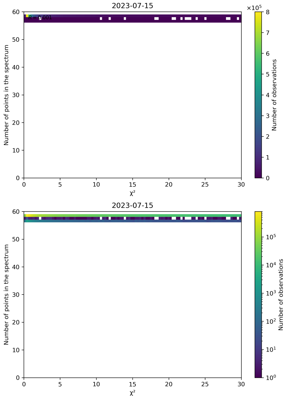
Figure 74: Scatter density plot of “ \chi^2 ” against “Number of points in the spectrum” for 2023-07-14 to 2023-07-16.
