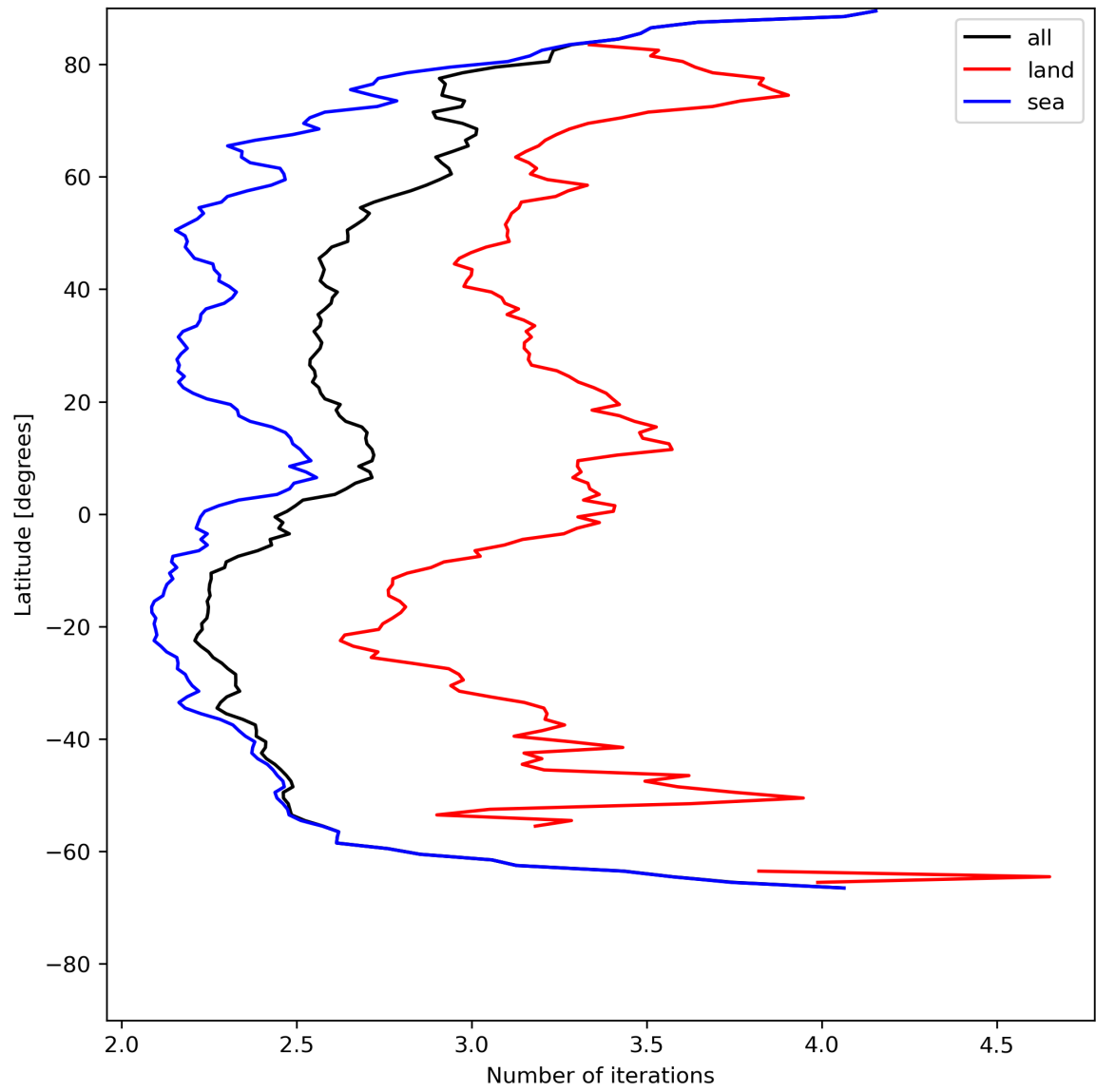
Figure 22: Zonal average of “Number of iterations” for 2023-07-14 to 2023-07-16.
