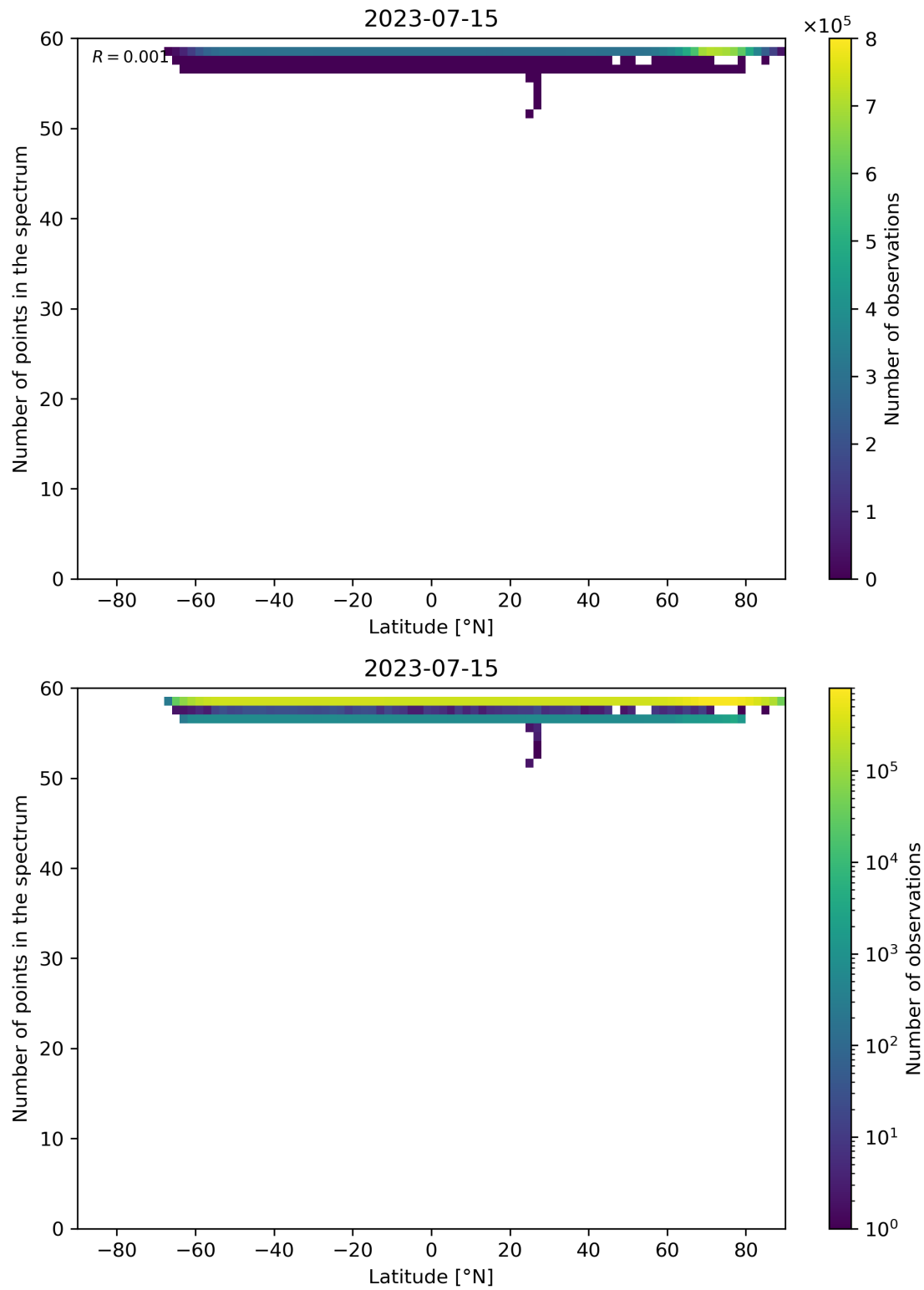
Figure 103: Scatter density plot of “Latitude” against “Number of points in the spectrum” for 2023-07-14 to 2023-07-16.
