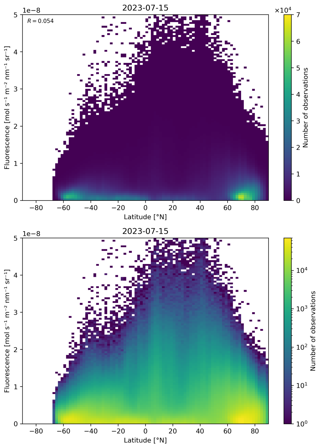
Figure 101: Scatter density plot of “Latitude” against “Fluorescence” for 2023-07-14 to 2023-07-16.
