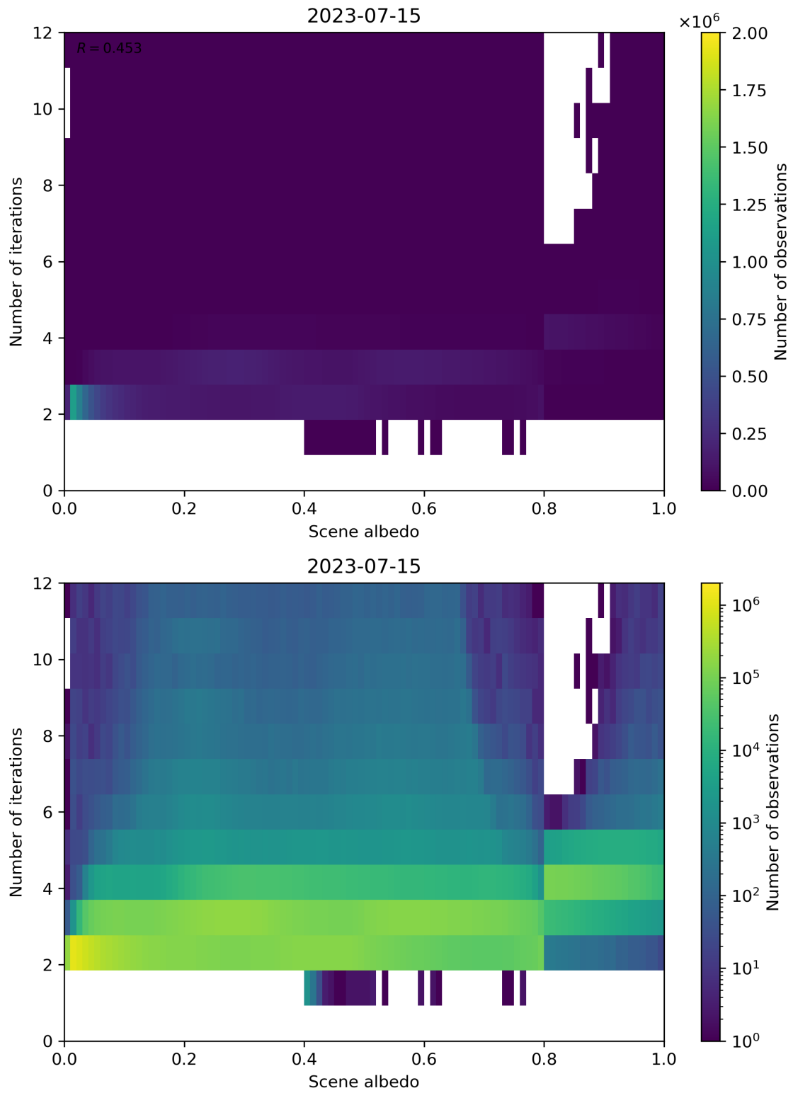
Figure 115: Scatter density plot of “Scene albedo” against “Number of iterations” for 2023-07-14 to 2023-07-16.
