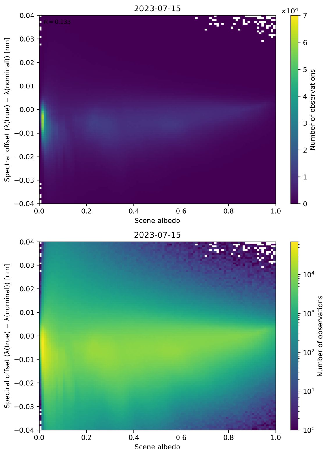
Figure 117: Scatter density plot of “Scene albedo” against “Spectral offset ( \lambda(\text{true}) - \lambda(\text{nominal}) )” for 2023-07-14 to 2023-07-16.
