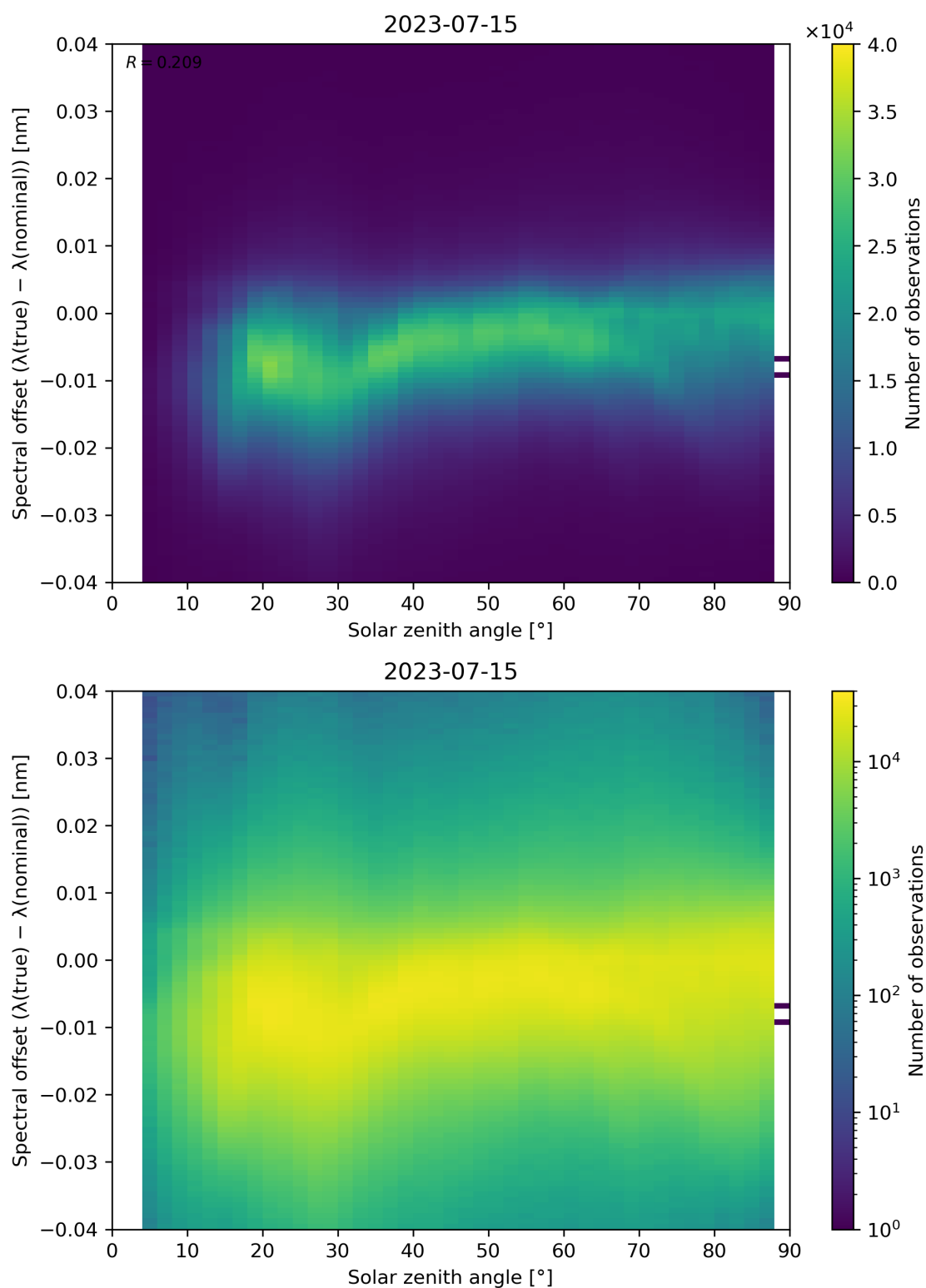
Figure 128: Scatter density plot of “Solar zenith angle” against “Spectral offset ( \lambda(\text{true}) - \lambda(\text{nominal}) )” for 2023-07-14 to 2023-07-16.
