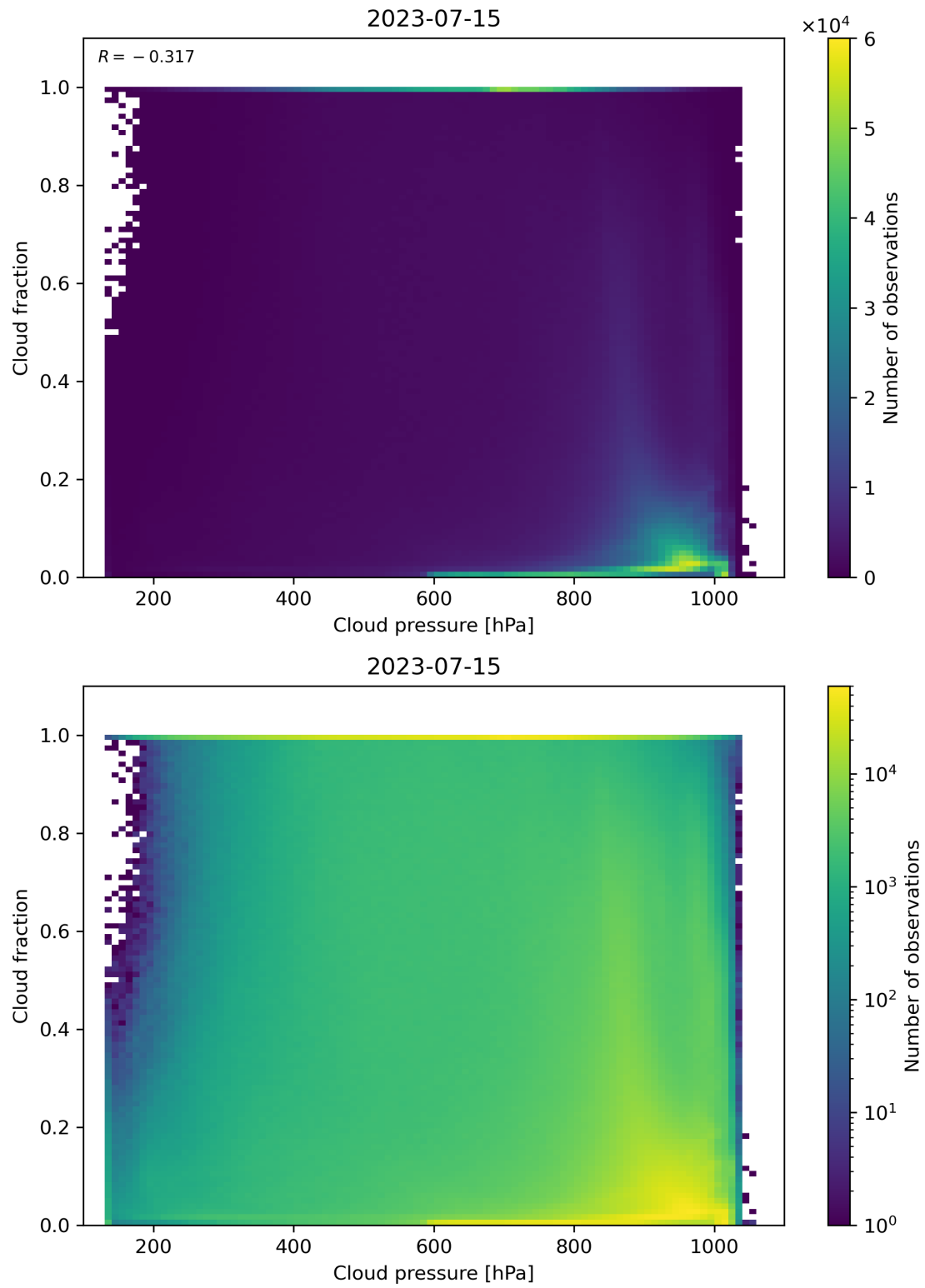
Figure 87: Scatter density plot of “Cloud pressure” against “Cloud fraction” for 2023-07-14 to 2023-07-16.
