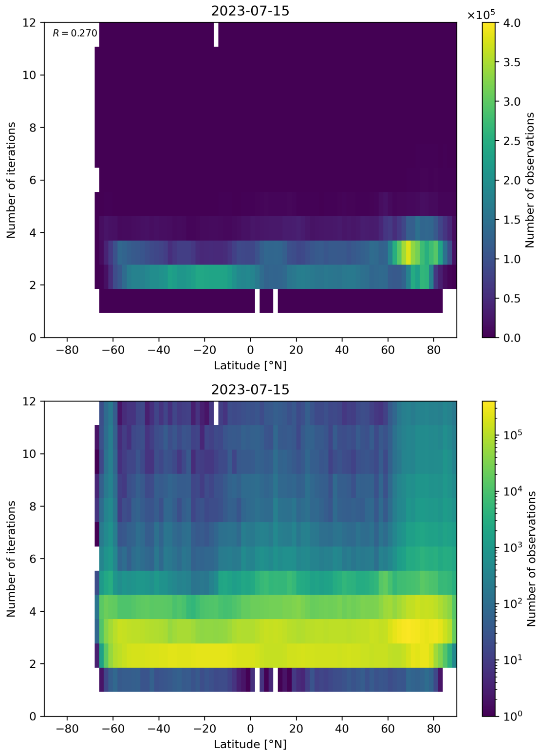
Figure 102: Scatter density plot of “Latitude” against “Number of iterations” for 2023-07-14 to 2023-07-16.
