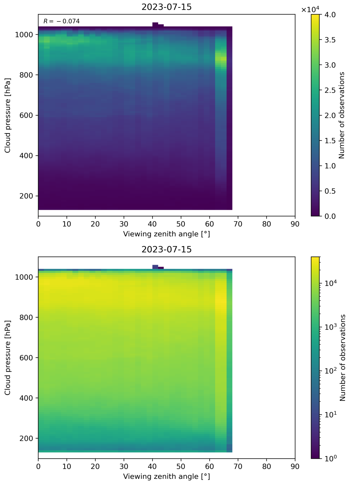
Figure 133: Scatter density plot of “Viewing zenith angle” against “Cloud pressure” for 2023-07-14 to 2023-07-16.
