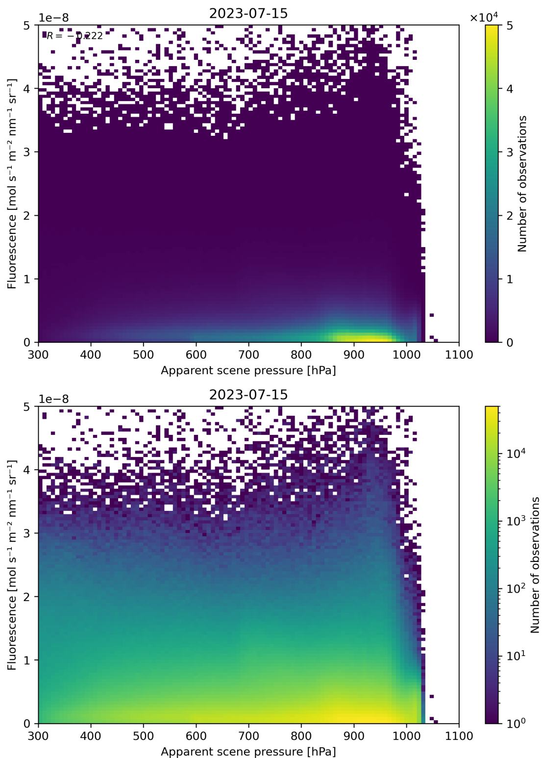
Figure 65: Scatter density plot of “Apparent scene pressure” against “Fluorescence” for 2023-07-14 to 2023-07-16.
