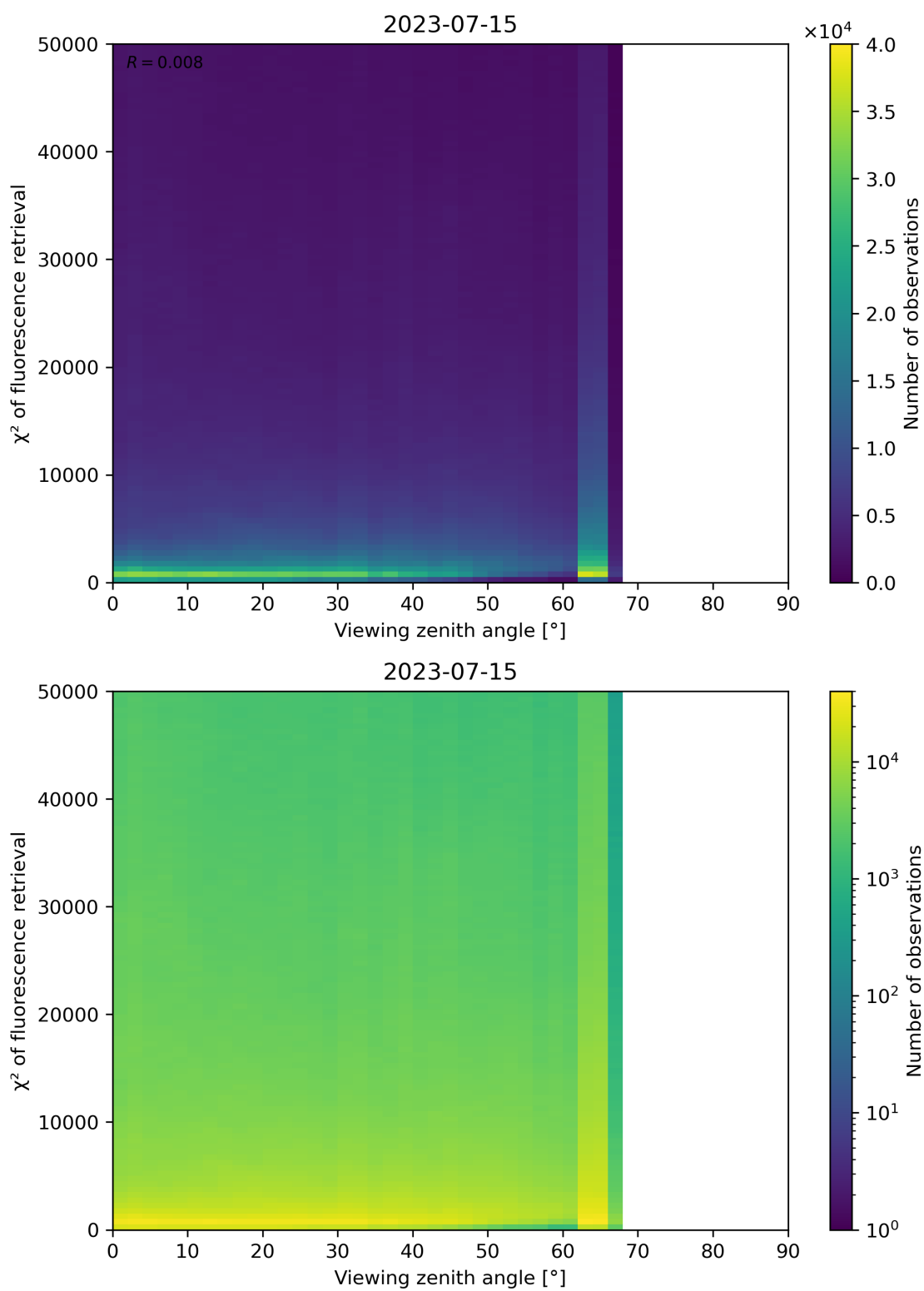
Figure 131: Scatter density plot of “Viewing zenith angle” against “ \chi^2 of fluorescence retrieval” for 2023-07-14 to 2023-07-16.
