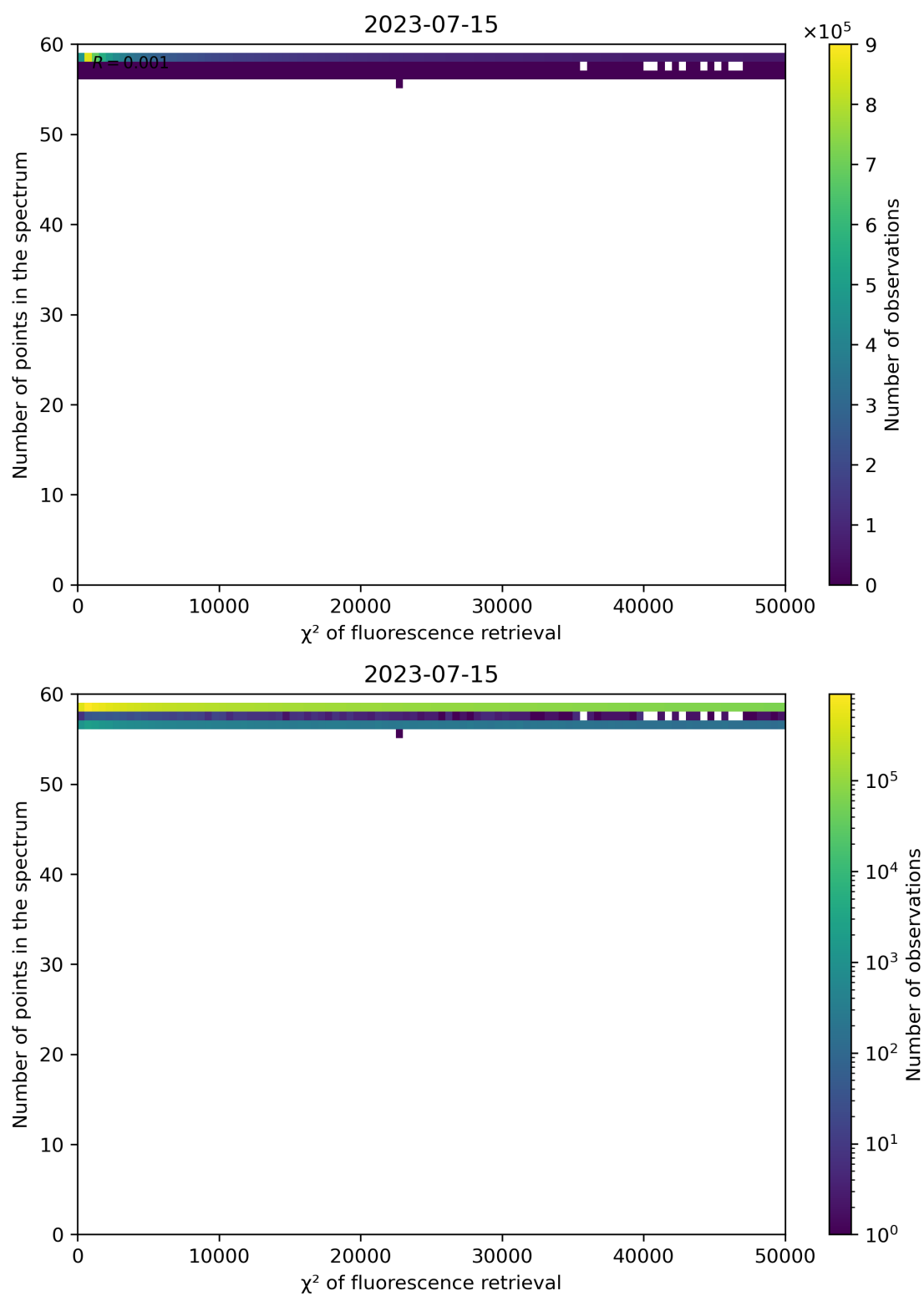
Figure 71: Scatter density plot of “ \chi^2 of fluorescence retrieval” against “Number of points in the spectrum” for 2023-07-14 to 2023-07-16.
