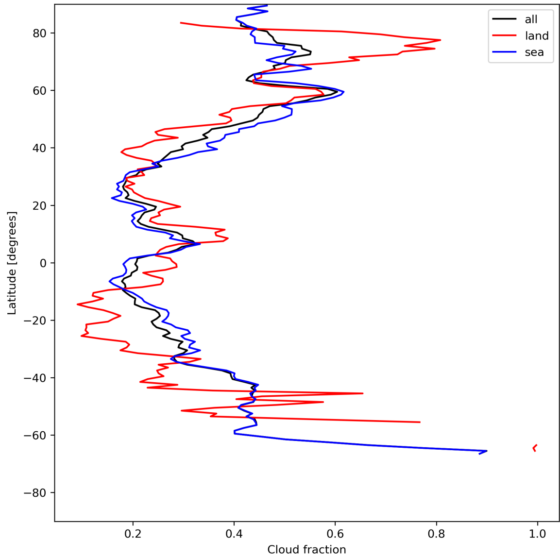
Figure 15: Zonal average of “Cloud fraction” for 2023-07-14 to 2023-07-16.
