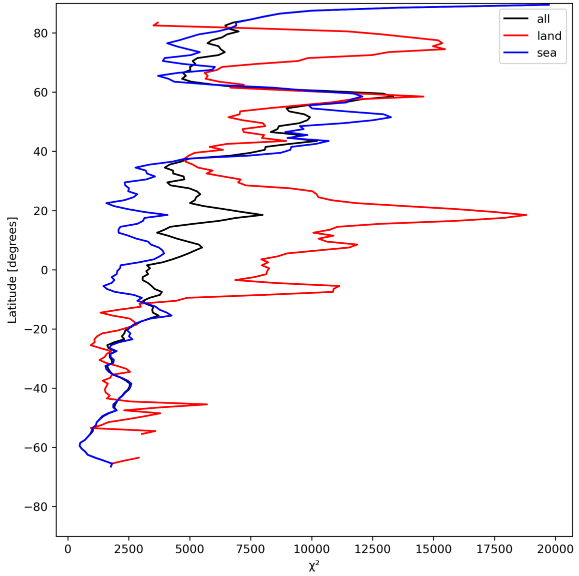
Figure 21: Zonal average of “ \chi^2 ” for 2023-07-14 to 2023-07-16.
