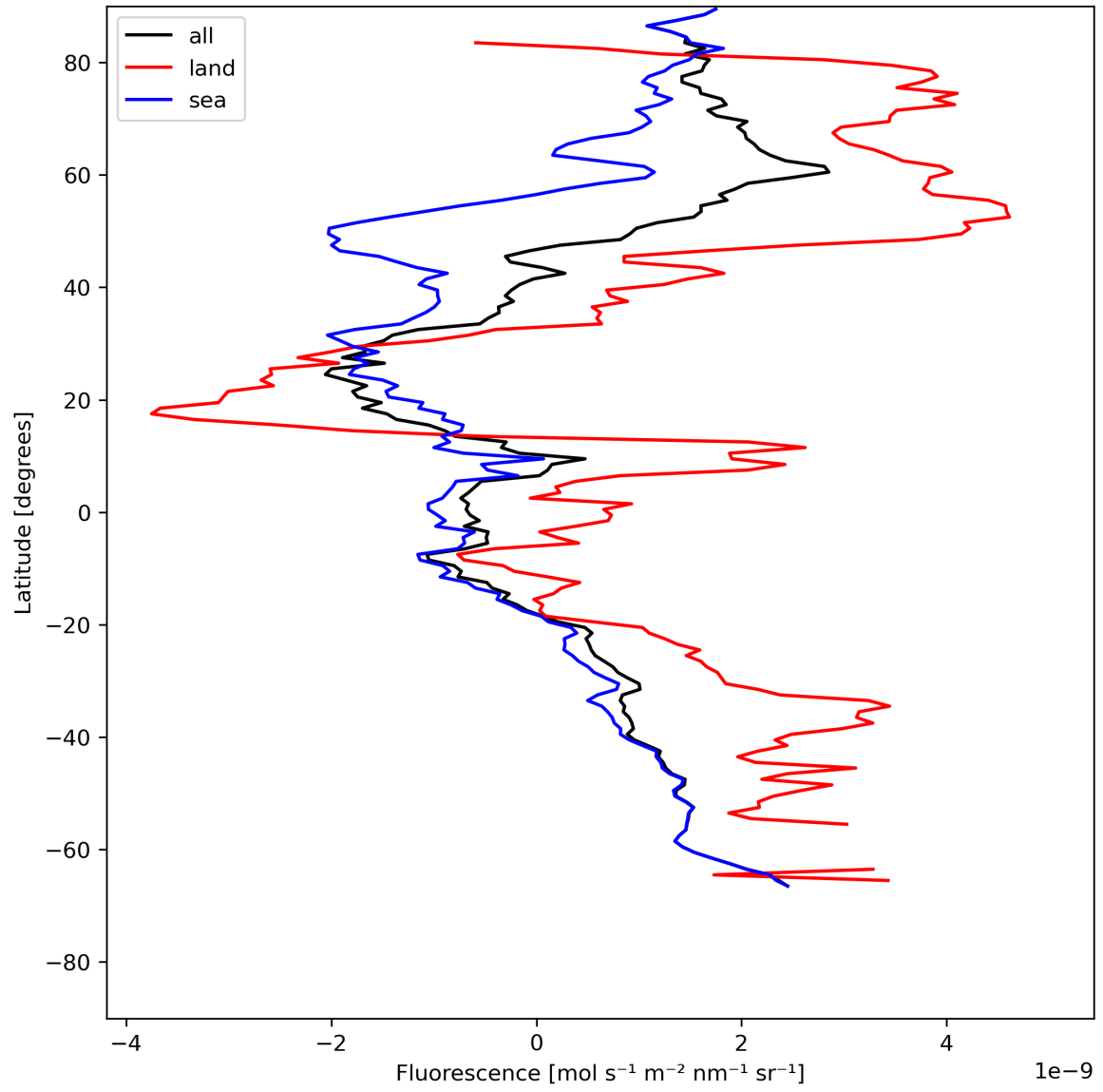
Figure 23: Zonal average of “Fluorescence” for 2023-07-14 to 2023-07-16.
