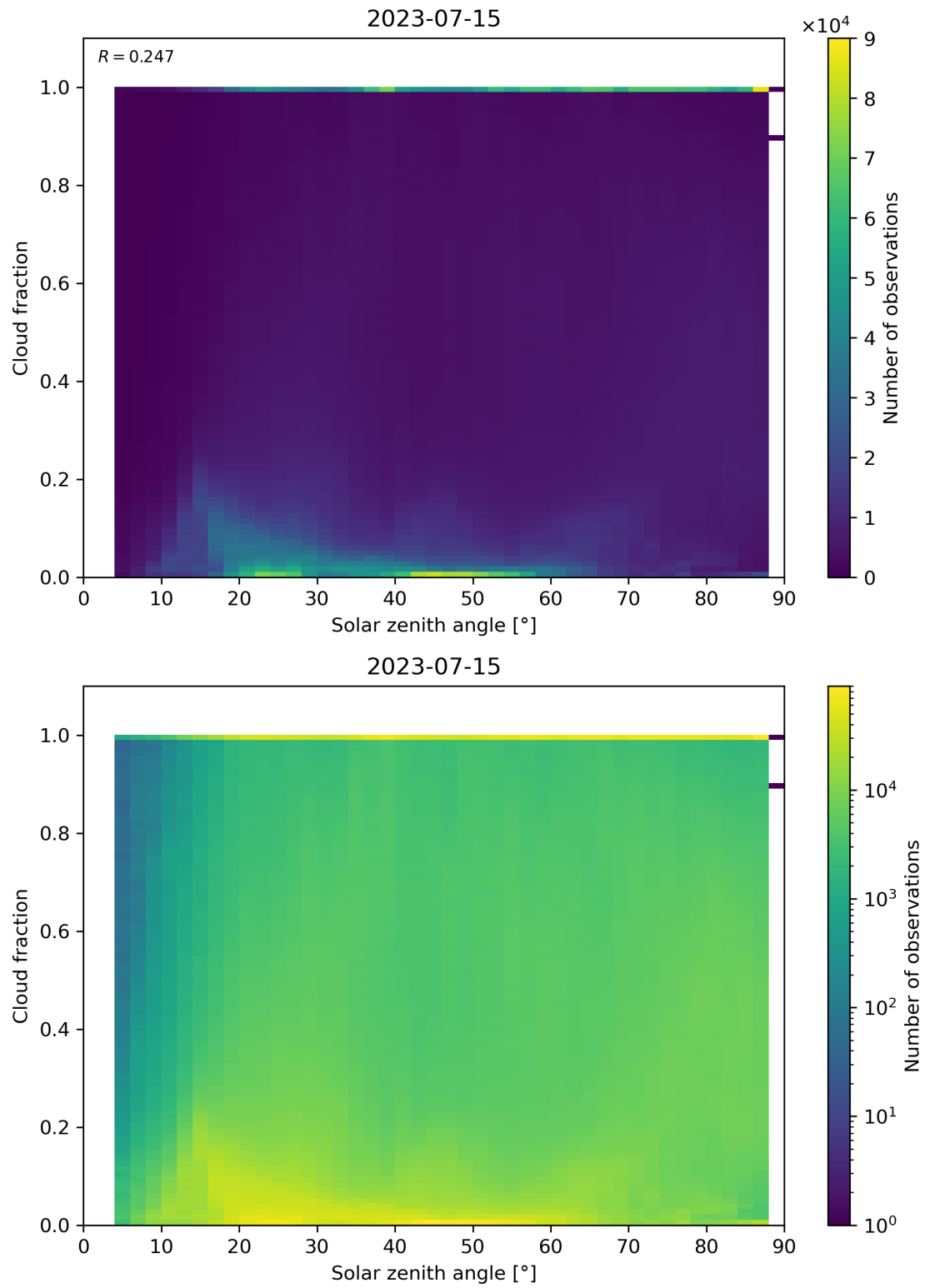
Figure 121: Scatter density plot of “Solar zenith angle” against “Cloud fraction” for 2023-07-14 to 2023-07-16.
