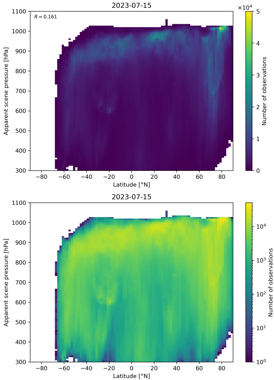
Figure 96: Scatter density plot of “Latitude” against “Apparent scene pressure” for 2023-07-14 to 2023-07-16.
