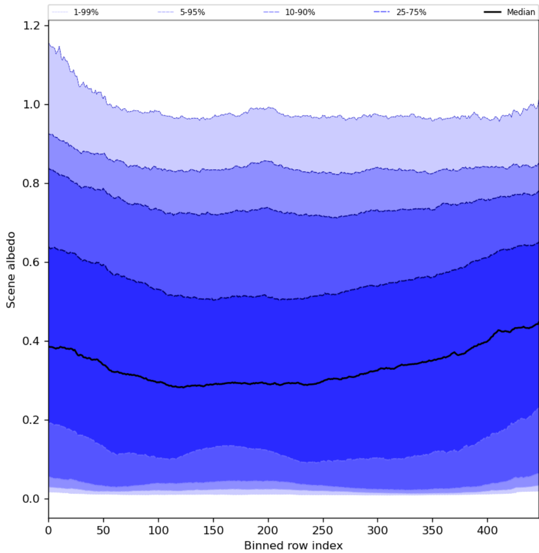
Figure 51: Along track statistics of “Scene albedo” for 2023-07-14 to 2023-07-16
