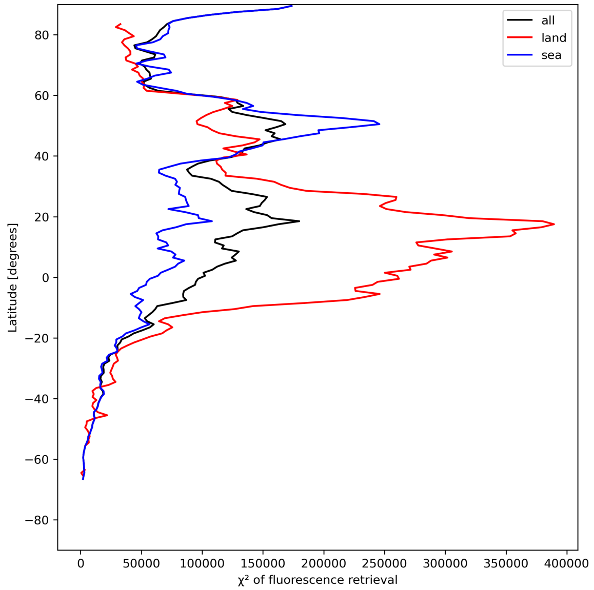
Figure 25: Zonal average of “ \chi^2 of fluorescence retrieval” for 2023-07-14 to 2023-07-16.
