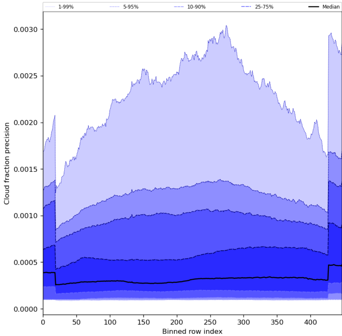
Figure 50: Along track statistics of “Cloud fraction precision” for 2023-07-14 to 2023-07-16
