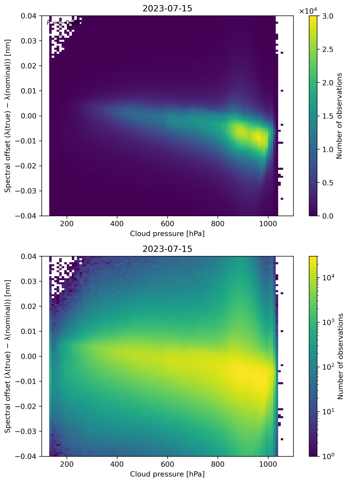
Figure 92: Scatter density plot of “Cloud pressure” against “Spectral offset ( \lambda(\text{true}) - \lambda(\text{nominal}) )” for 2023-07-14 to 2023-07-16.
