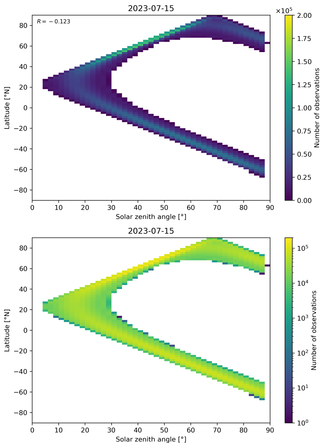
Figure 124: Scatter density plot of “Solar zenith angle” against “Latitude” for 2023-07-14 to 2023-07-16.
