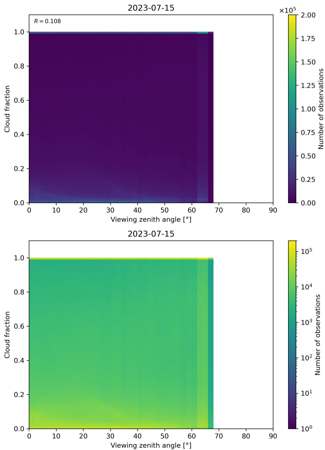
Figure 132: Scatter density plot of “Viewing zenith angle” against “Cloud fraction” for 2023-07-14 to 2023-07-16.
