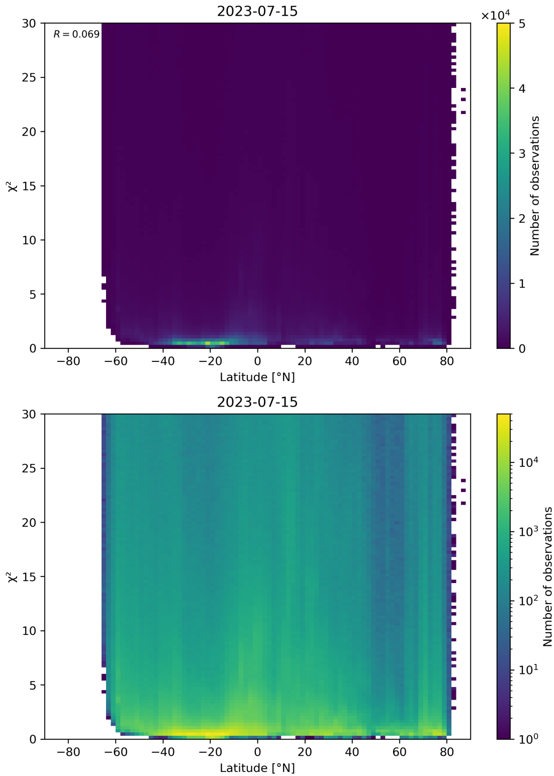
Figure 97: Scatter density plot of “Latitude” against “ \chi^2 ” for 2023-07-14 to 2023-07-16.
