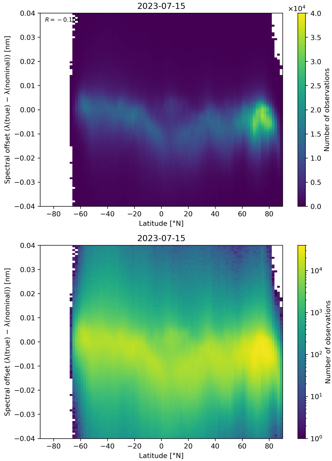
Figure 105: Scatter density plot of “Latitude” against “Spectral offset ( \lambda(\text{true}) - \lambda(\text{nominal}) )” for 2023-07-14 to 2023-07-16.
