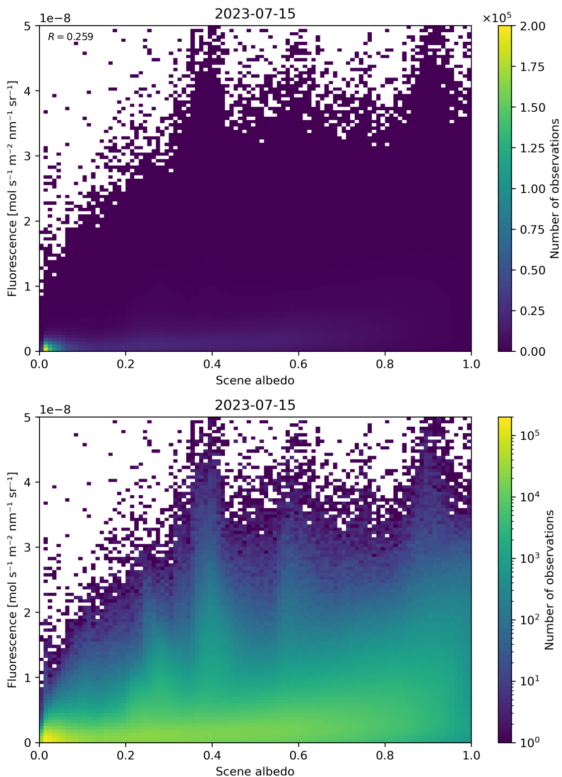
Figure 114: Scatter density plot of “Scene albedo” against “Fluorescence” for 2023-07-14 to 2023-07-16.
