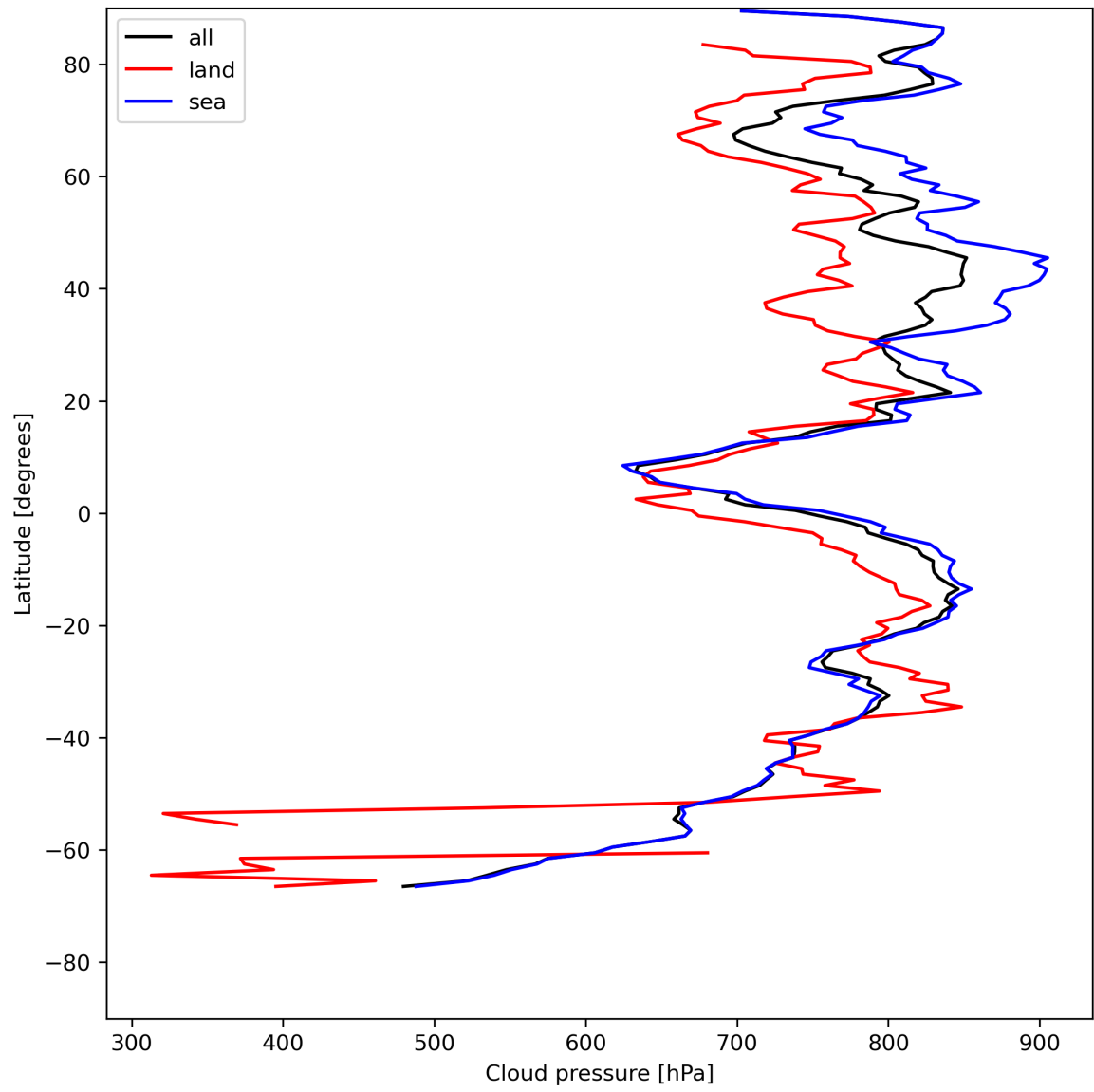
Figure 13: Zonal average of “Cloud pressure” for 2023-07-16 to 2023-07-18.
