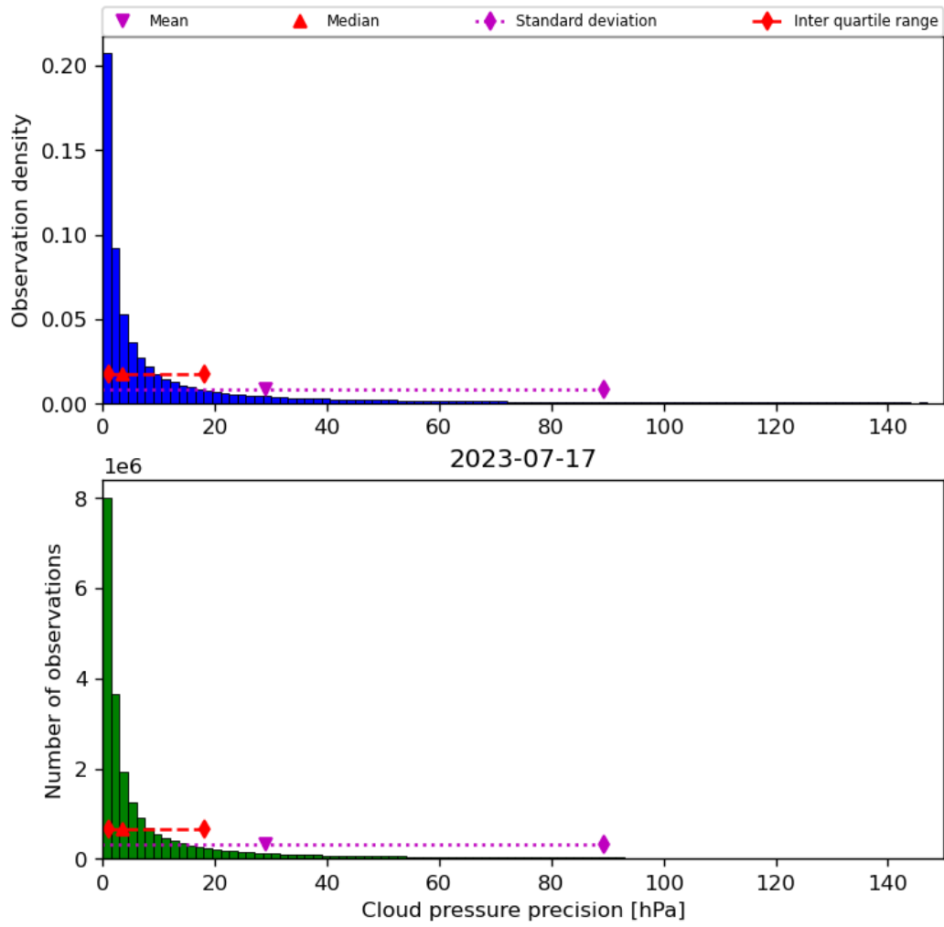
Figure 31: Histogram of “Cloud pressure precision” for 2023-07-16 to 2023-07-18
