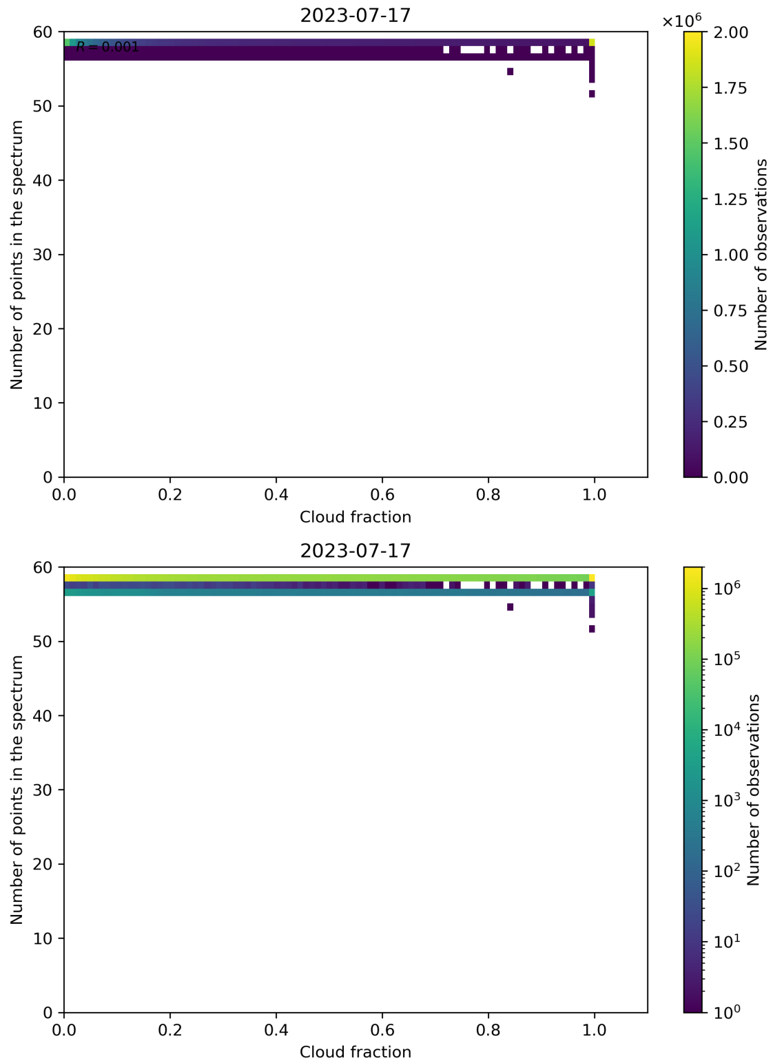
Figure 81: Scatter density plot of “Cloud fraction” against “Number of points in the spectrum” for 2023-07-16 to 2023-07-18.
