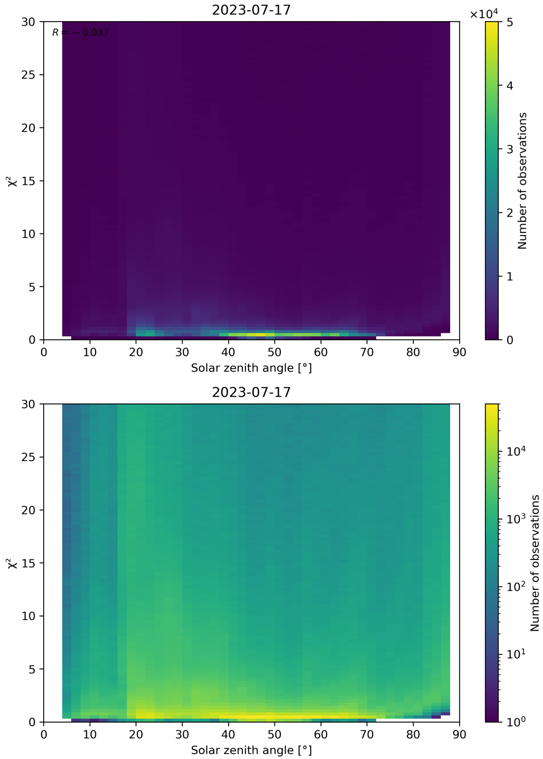
Figure 119: Scatter density plot of “Solar zenith angle” against “ \chi^2 ” for 2023-07-16 to 2023-07-18.
