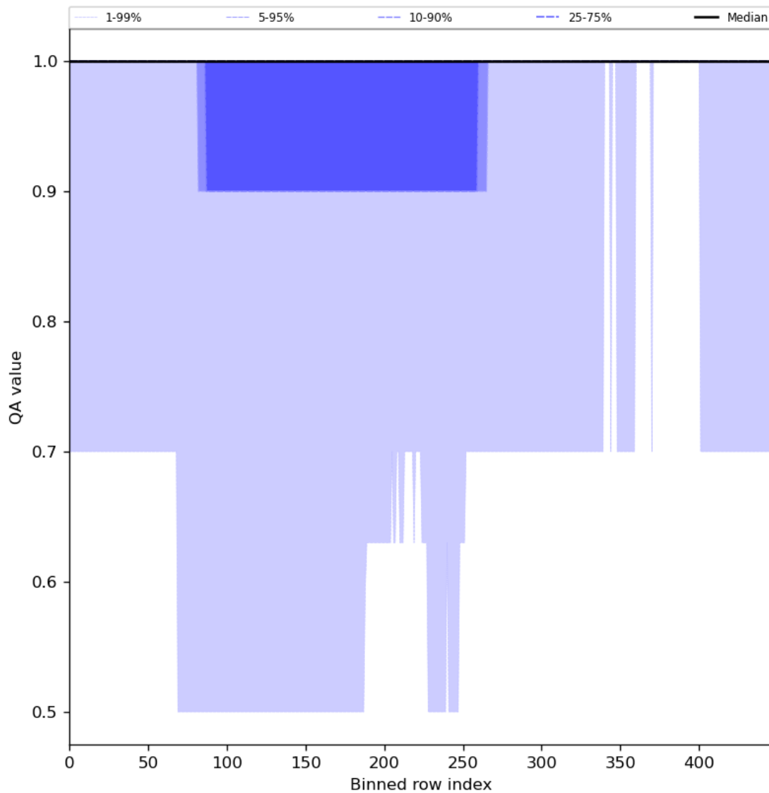
Figure 46: Along track statistics of “QA value” for 2023-07-16 to 2023-07-18
