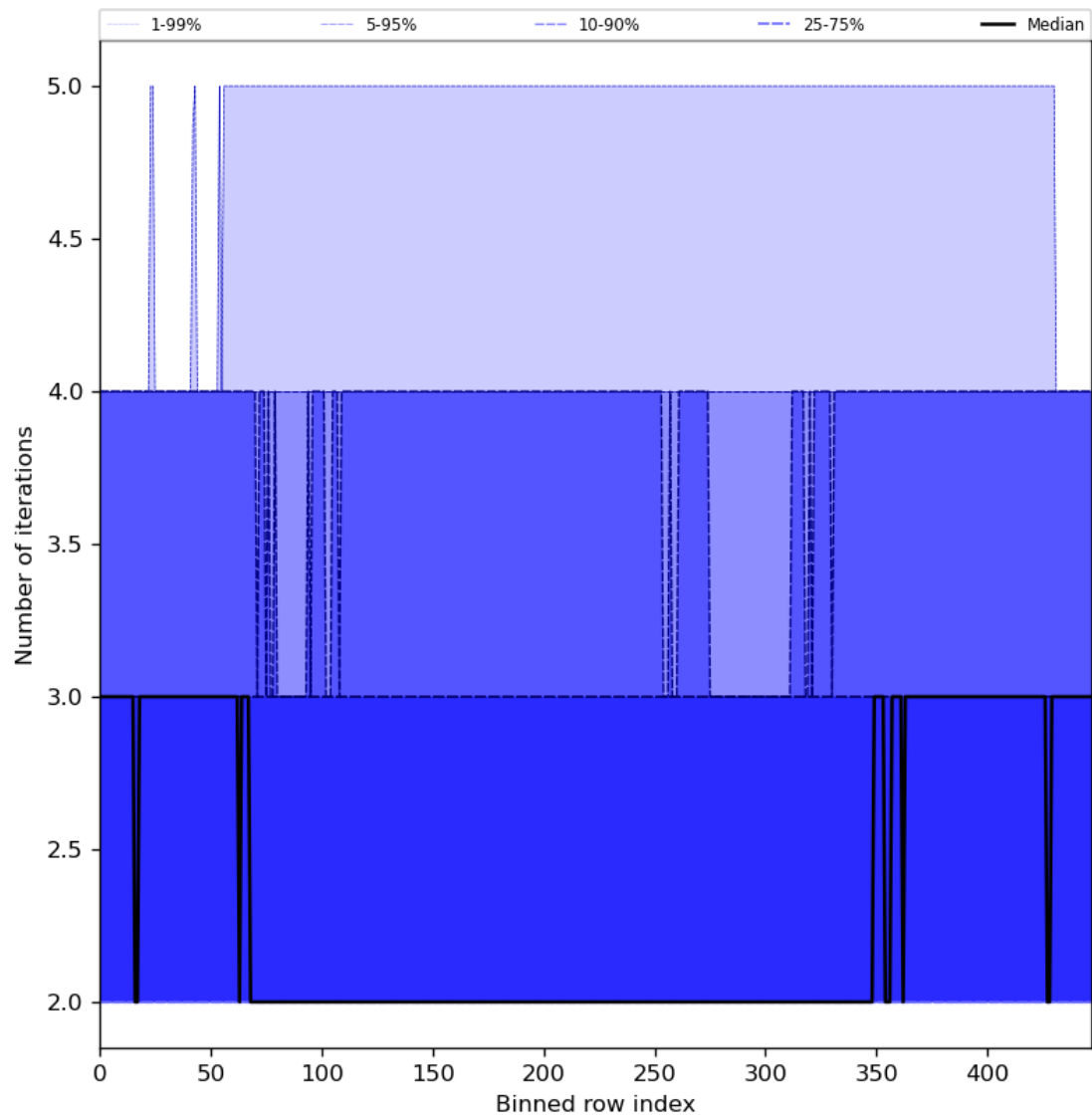
Figure 56: Along track statistics of “Number of iterations” for 2023-07-16 to 2023-07-18
