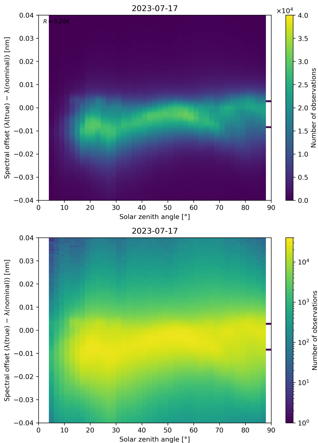
Figure 128: Scatter density plot of “Solar zenith angle” against “Spectral offset ( \lambda(\text{true}) - \lambda(\text{nominal}) )” for 2023-07-16 to 2023-07-18.
