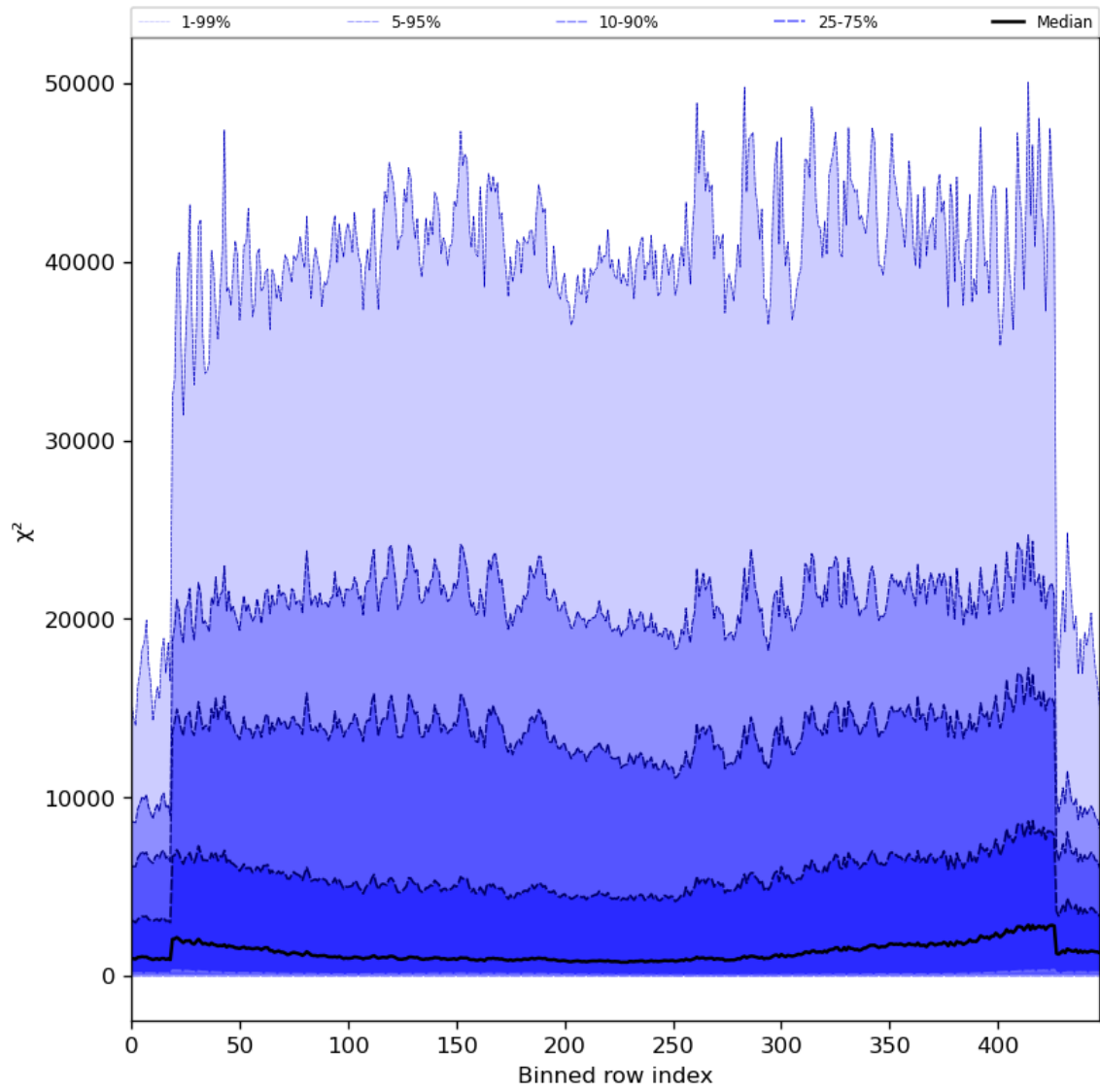
Figure 55: Along track statistics of “ \chi^2 ” for 2023-07-16 to 2023-07-18
