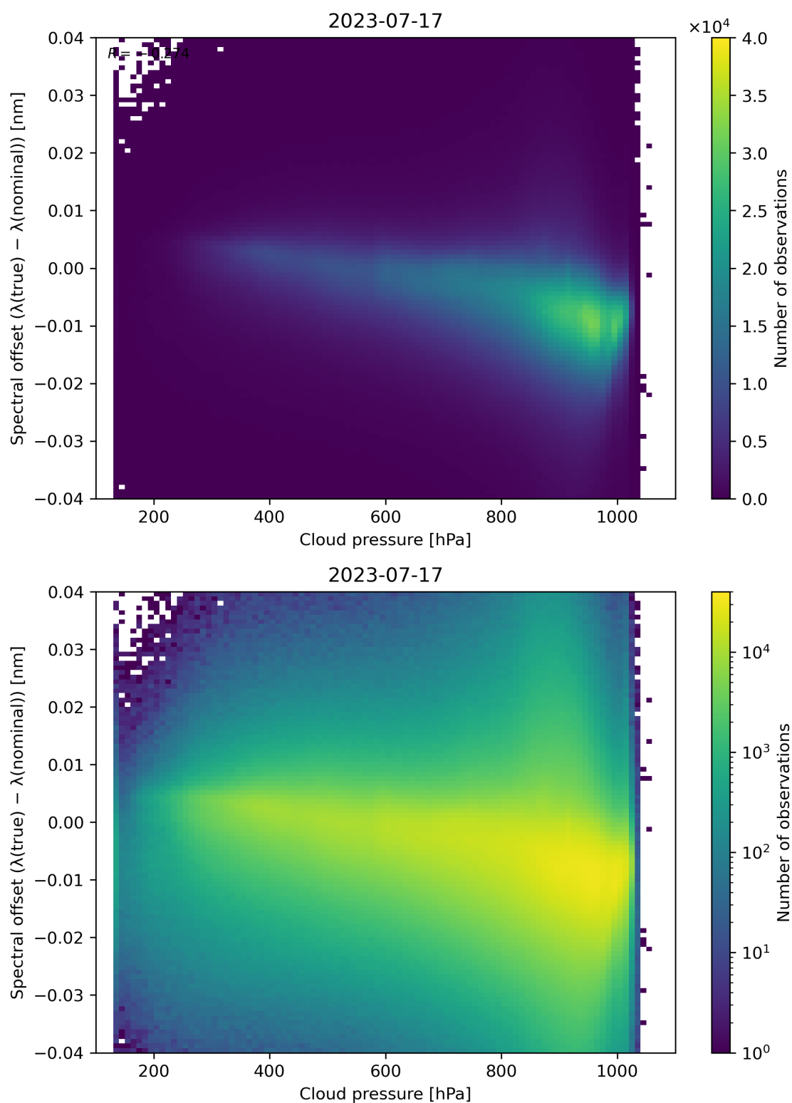
Figure 92: Scatter density plot of “Cloud pressure” against “Spectral offset ( \lambda(\text{true}) - \lambda(\text{nominal}) )” for 2023-07-16 to 2023-07-18.
