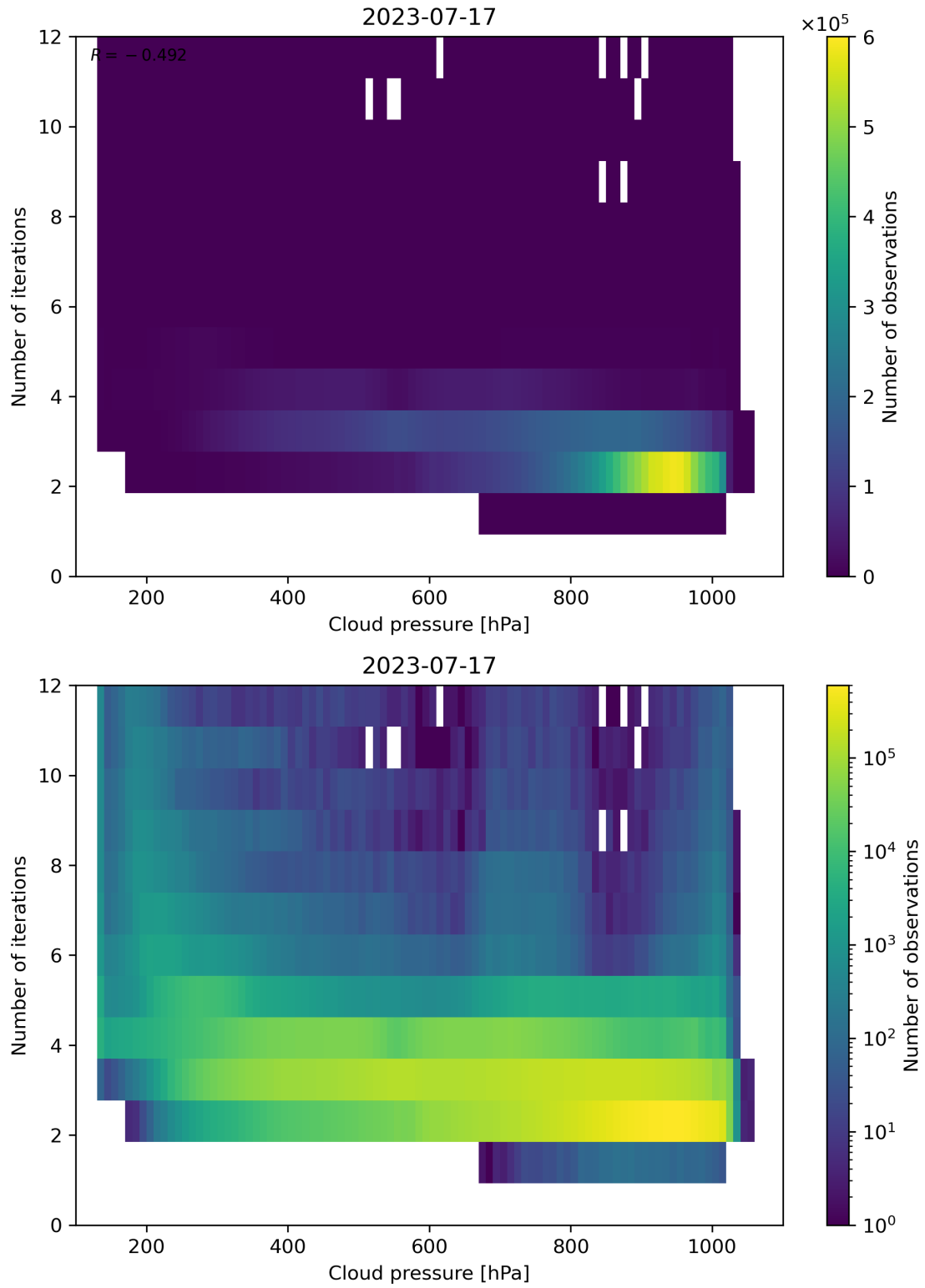
Figure 89: Scatter density plot of “Cloud pressure” against “Number of iterations” for 2023-07-16 to 2023-07-18.
