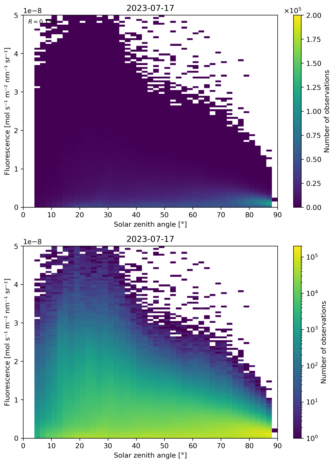
Figure 123: Scatter density plot of “Solar zenith angle” against “Fluorescence” for 2023-07-16 to 2023-07-18.
