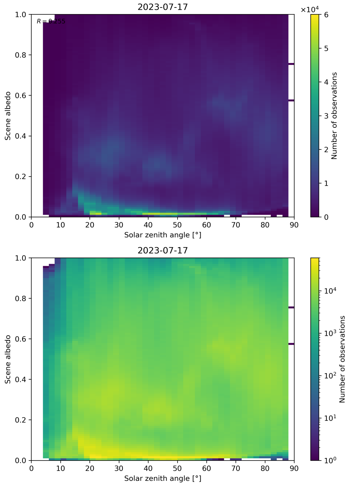
Figure 127: Scatter density plot of “Solar zenith angle” against “Scene albedo” for 2023-07-16 to 2023-07-18.
