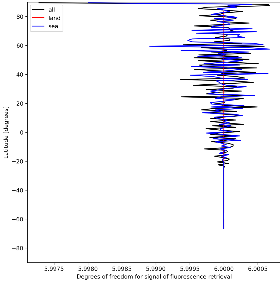
Figure 26: Zonal average of “Degrees of freedom for signal of fluorescence retrieval” for 2023-07-16 to 2023-07-18.
