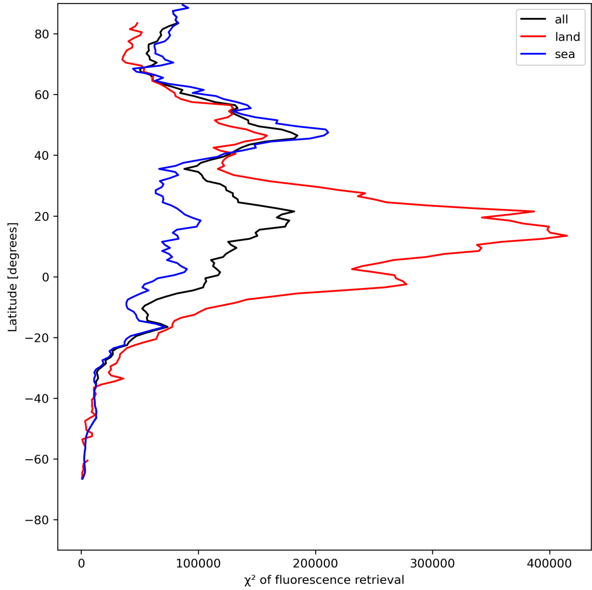
Figure 25: Zonal average of “ \chi^2 of fluorescence retrieval” for 2023-07-16 to 2023-07-18.
