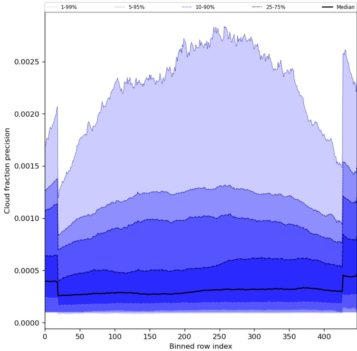
Figure 50: Along track statistics of “Cloud fraction precision” for 2023-07-16 to 2023-07-18
