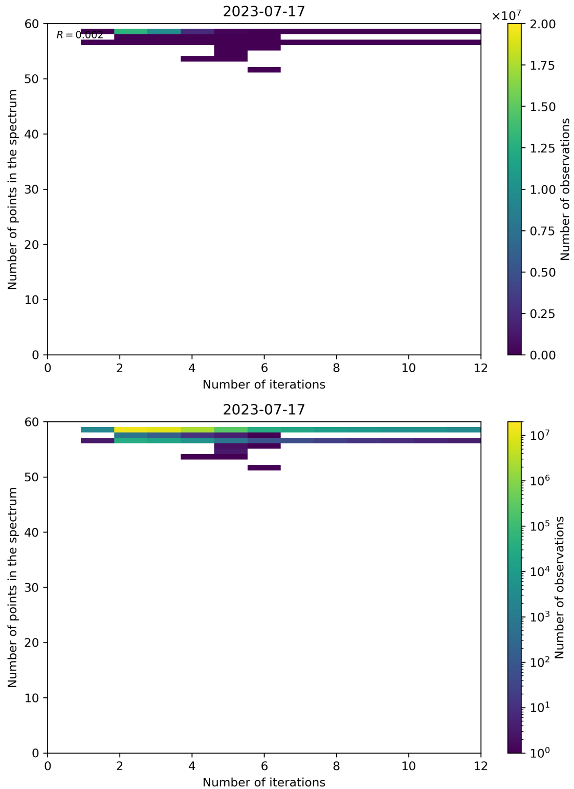
Figure 108: Scatter density plot of “Number of iterations” against “Number of points in the spectrum” for 2023-07-16 to 2023-07-18.
