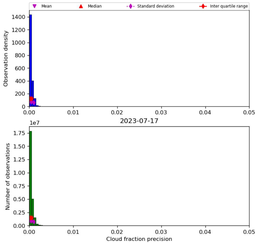
Figure 33: Histogram of “Cloud fraction precision” for 2023-07-16 to 2023-07-18
