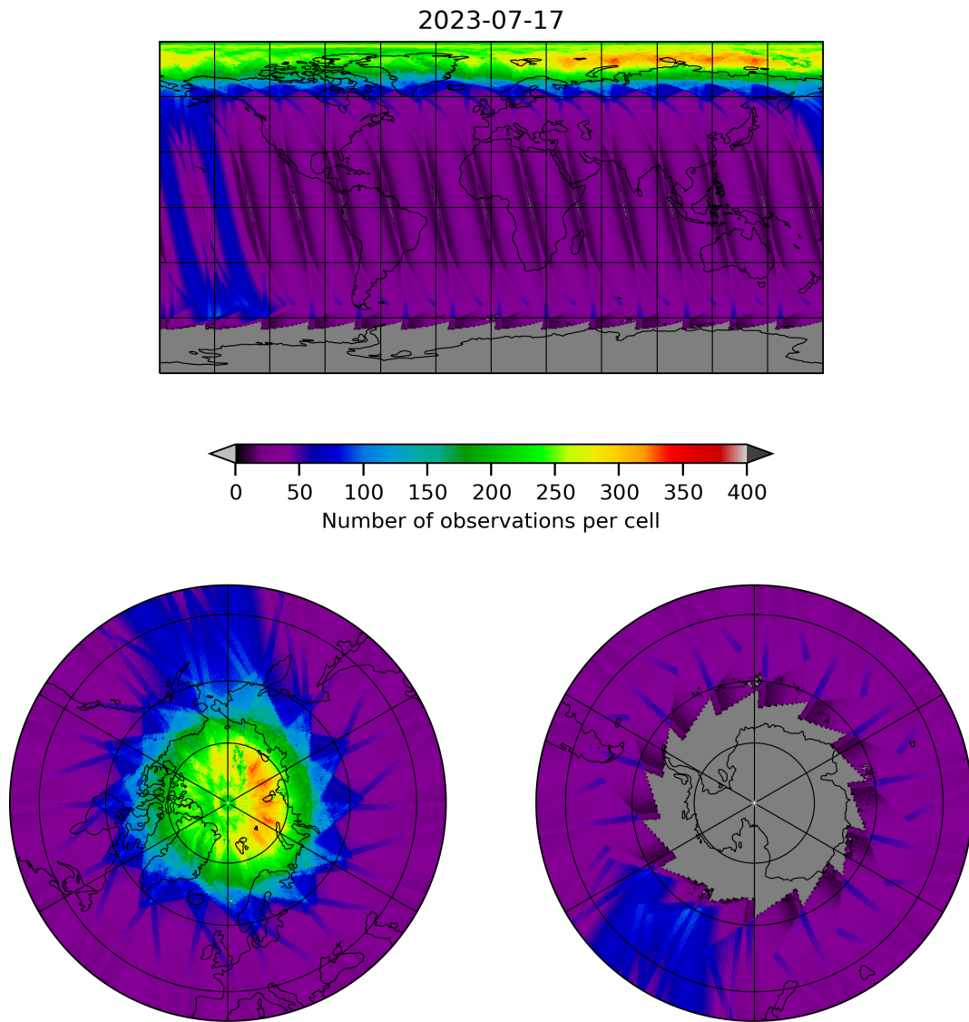
Figure 11: Map of the number of observations for 2023-07-16 to 2023-07-18
