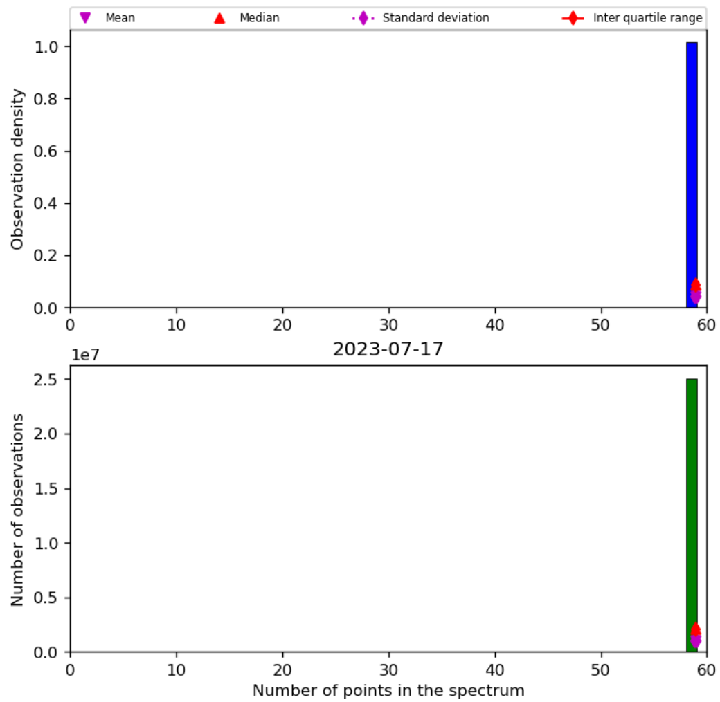
Figure 44: Histogram of “Number of points in the spectrum” for 2023-07-16 to 2023-07-18
