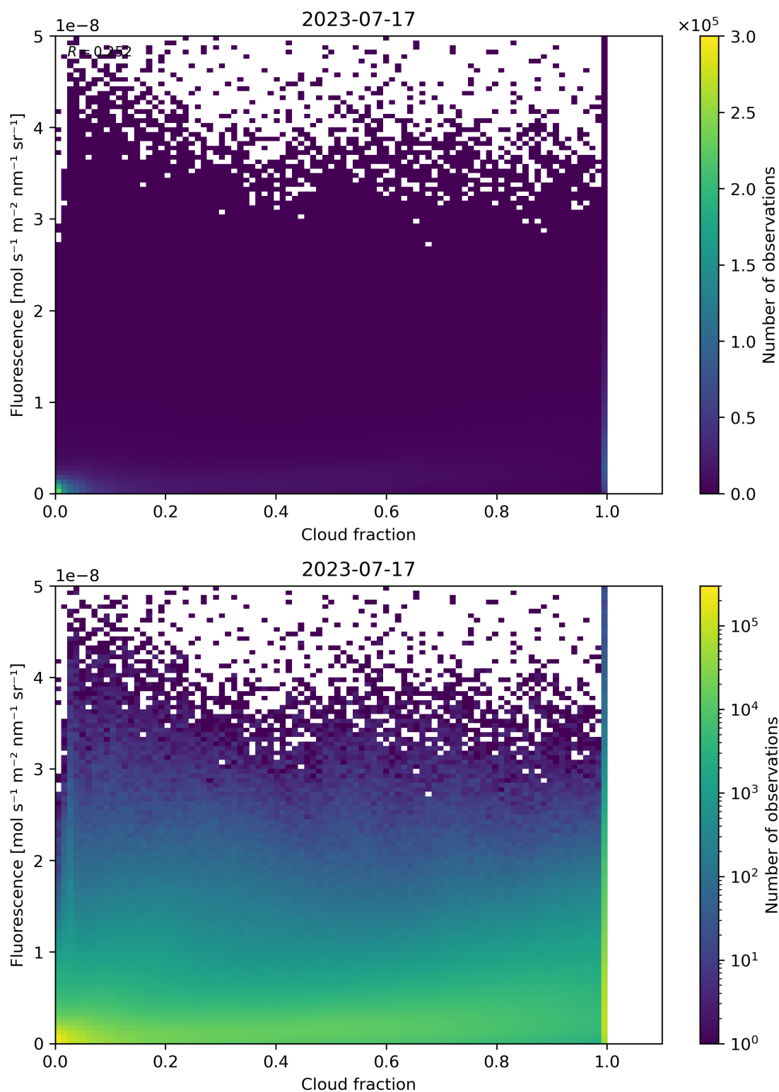
Figure 79: Scatter density plot of “Cloud fraction” against “Fluorescence” for 2023-07-16 to 2023-07-18.
