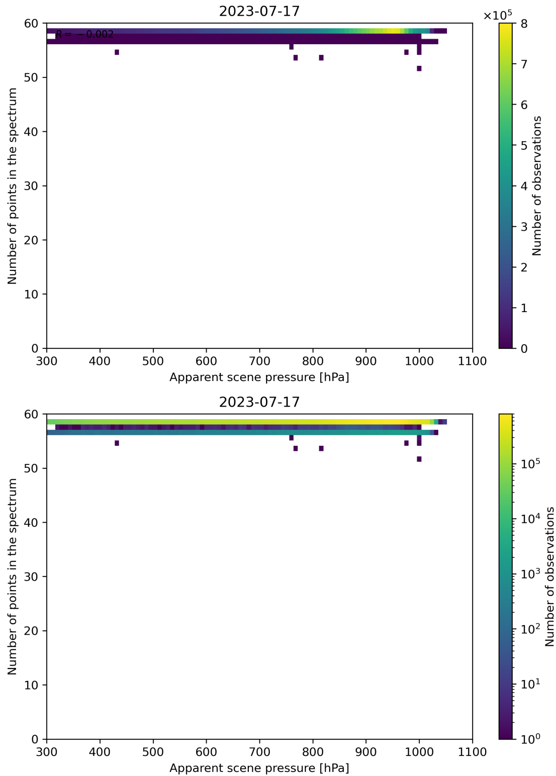
Figure 67: Scatter density plot of “Apparent scene pressure” against “Number of points in the spectrum” for 2023-07-16 to 2023-07-18.
