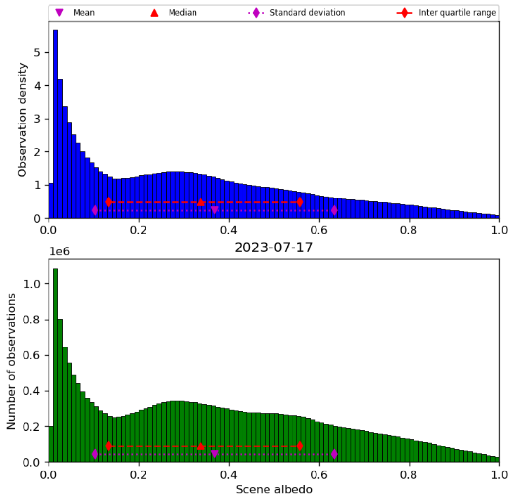
Figure 34: Histogram of “Scene albedo” for 2023-07-16 to 2023-07-18
