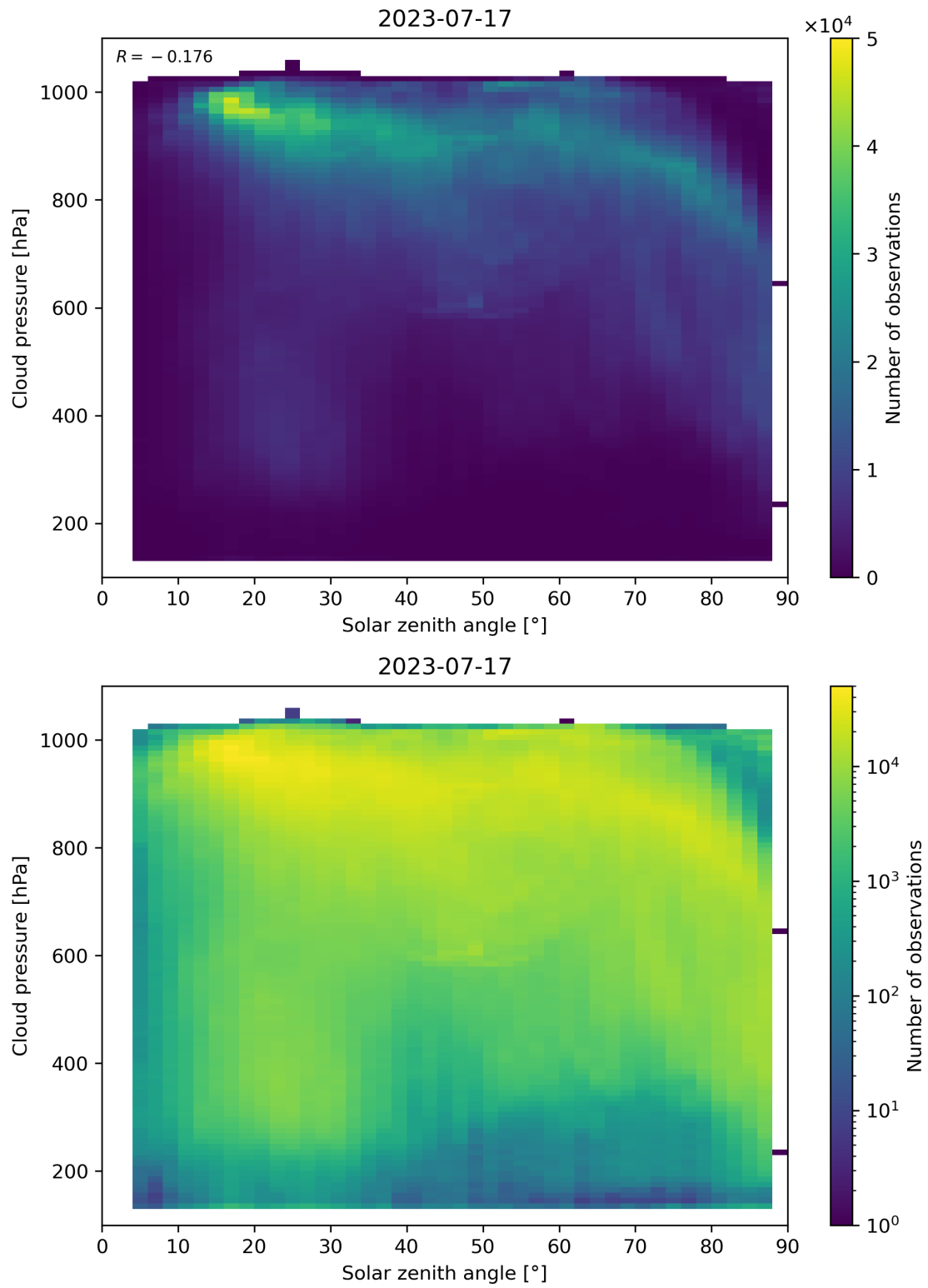
Figure 122: Scatter density plot of “Solar zenith angle” against “Cloud pressure” for 2023-07-16 to 2023-07-18.
