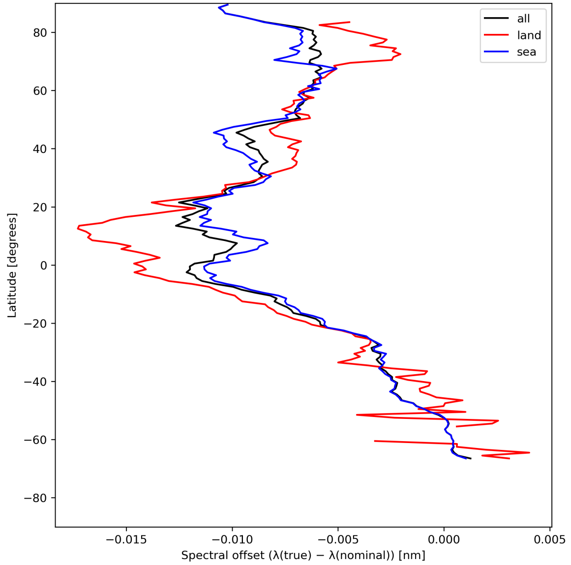
Figure 28: Zonal average of “Spectral offset ( \lambda(\text{true}) - \lambda(\text{nominal}) )” for 2023-07-16 to 2023-07-18.
