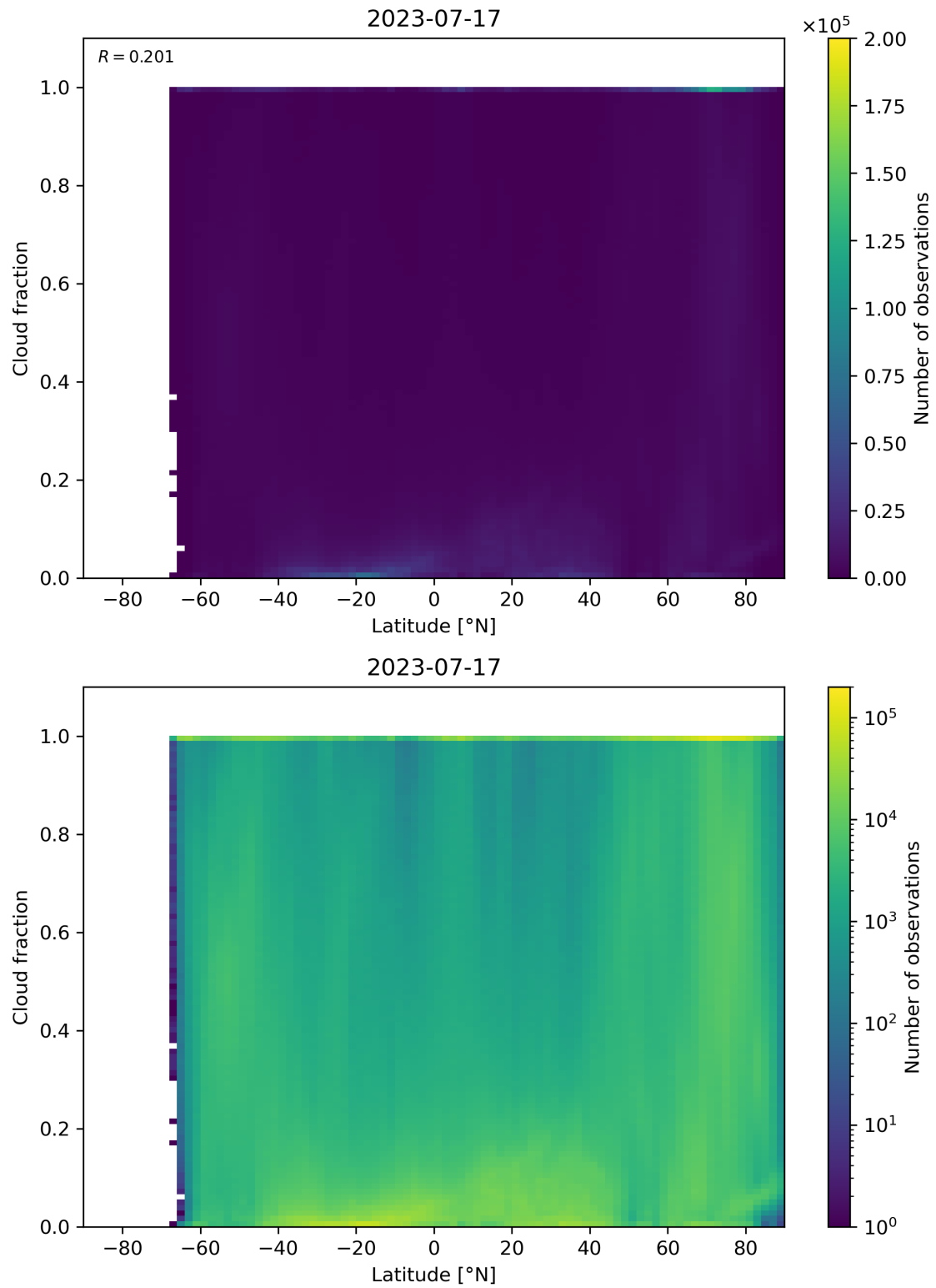
Figure 99: Scatter density plot of “Latitude” against “Cloud fraction” for 2023-07-16 to 2023-07-18.
