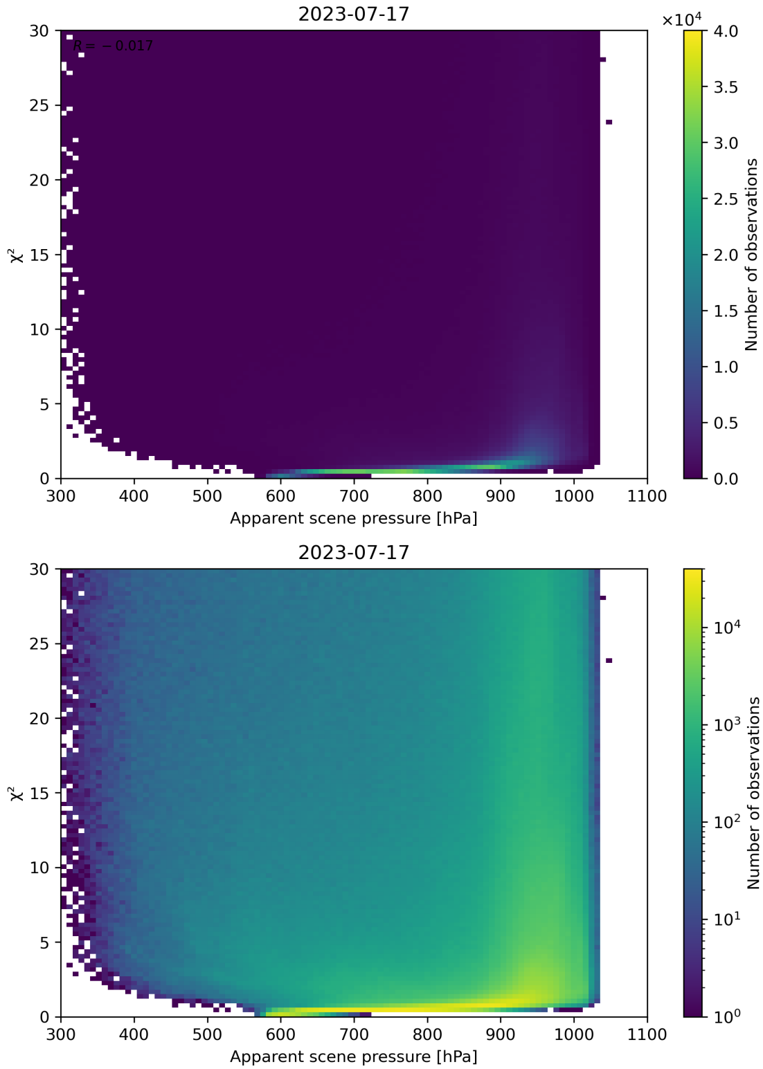
Figure 63: Scatter density plot of “Apparent scene pressure” against “ \chi^2 ” for 2023-07-16 to 2023-07-18.
