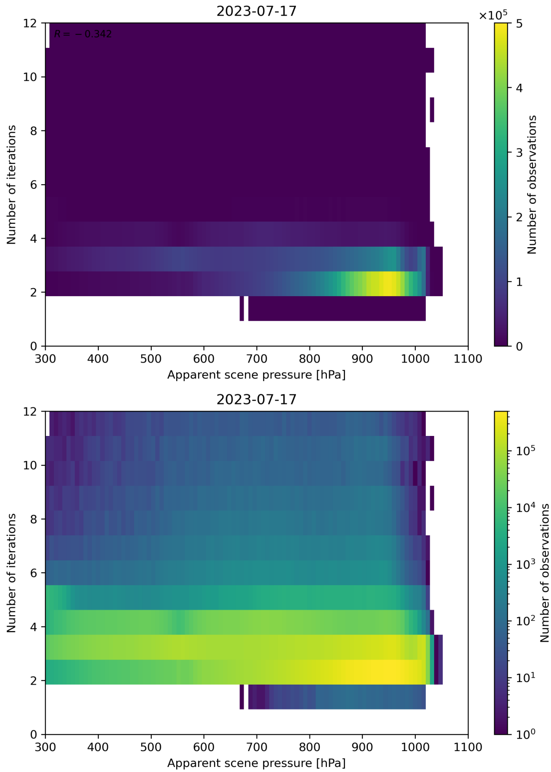
Figure 66: Scatter density plot of “Apparent scene pressure” against “Number of iterations” for 2023-07-16 to 2023-07-18.
