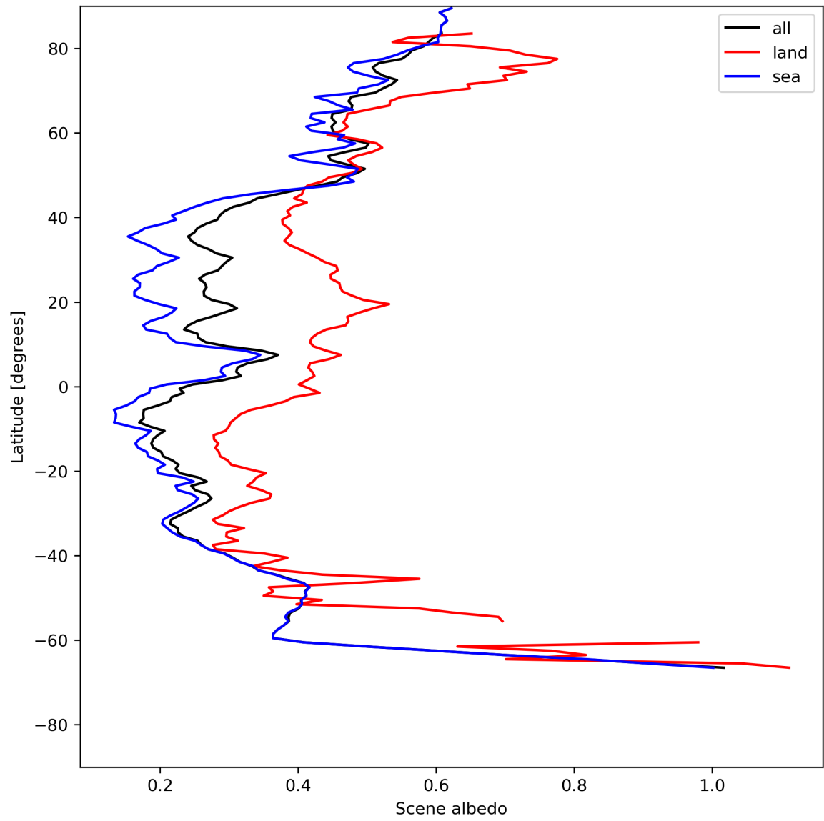
Figure 17: Zonal average of “Scene albedo” for 2023-07-16 to 2023-07-18.
