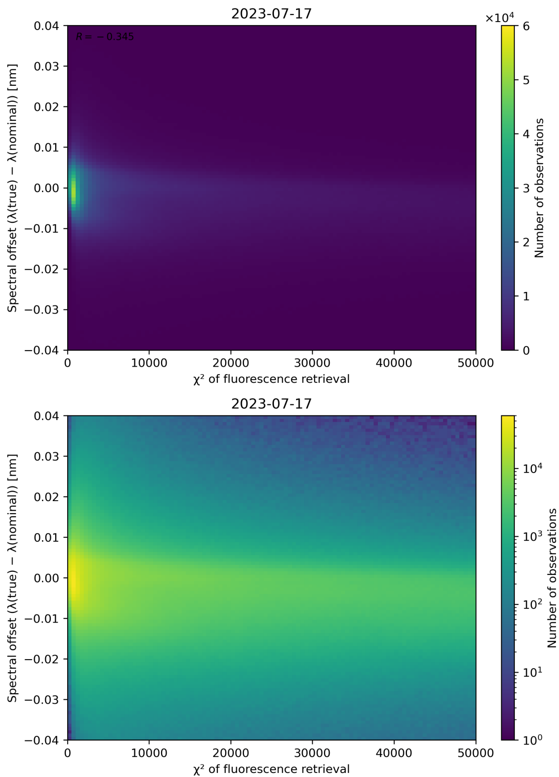
Figure 72: Scatter density plot of " \chi^2 of fluorescence retrieval" against "Spectral offset ( \lambda(\text{true}) - \lambda(\text{nominal}) )" for 2023-07-16 to 2023-07-18.
