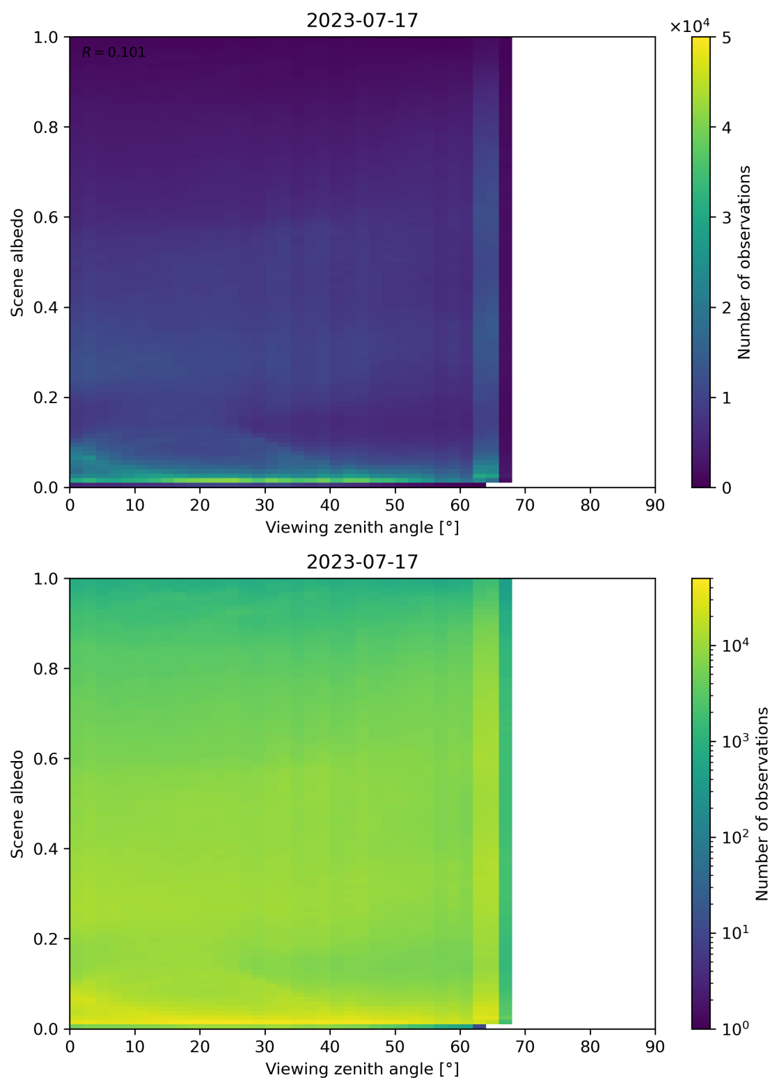
Figure 138: Scatter density plot of “Viewing zenith angle” against “Scene albedo” for 2023-07-16 to 2023-07-18.
