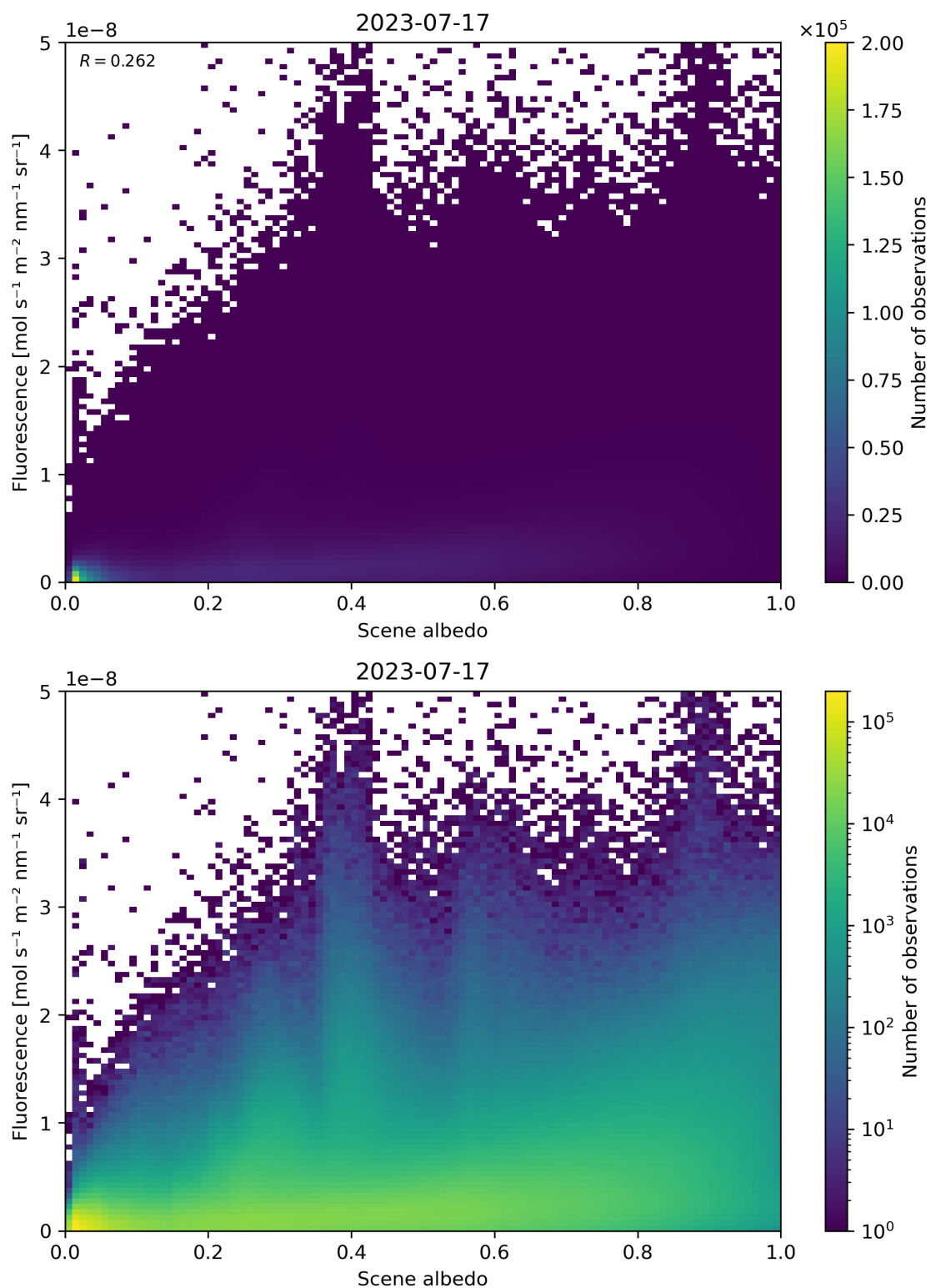
Figure 114: Scatter density plot of “Scene albedo” against “Fluorescence” for 2023-07-16 to 2023-07-18.
