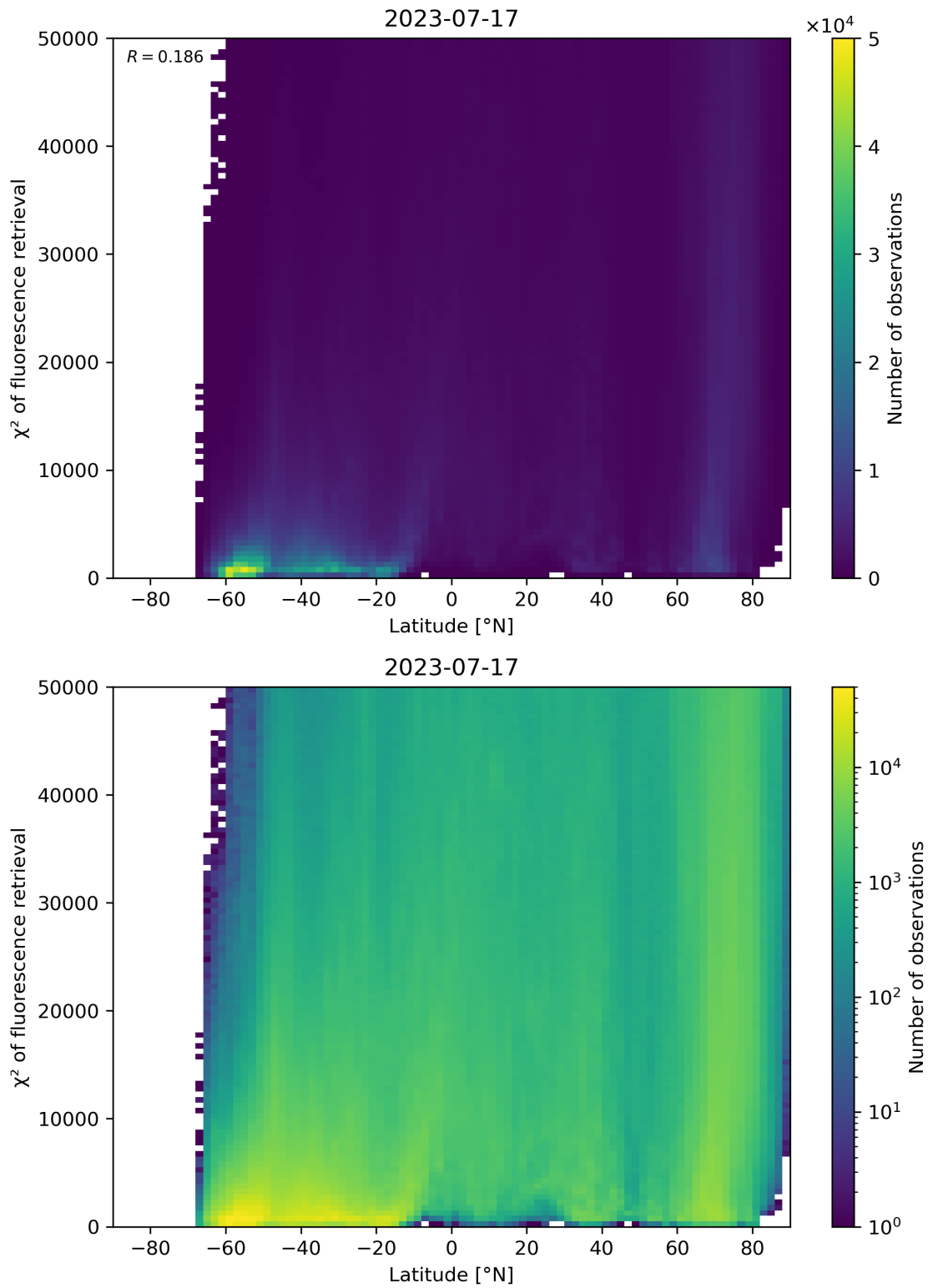
Figure 98: Scatter density plot of “Latitude” against “ \chi^2 of fluorescence retrieval” for 2023-07-16 to 2023-07-18.
