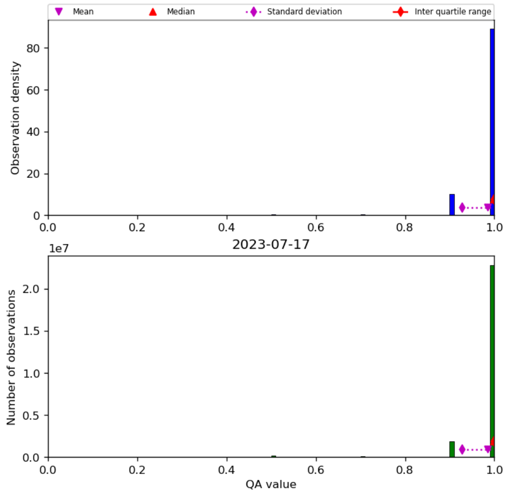
Figure 29: Histogram of “QA value” for 2023-07-16 to 2023-07-18
