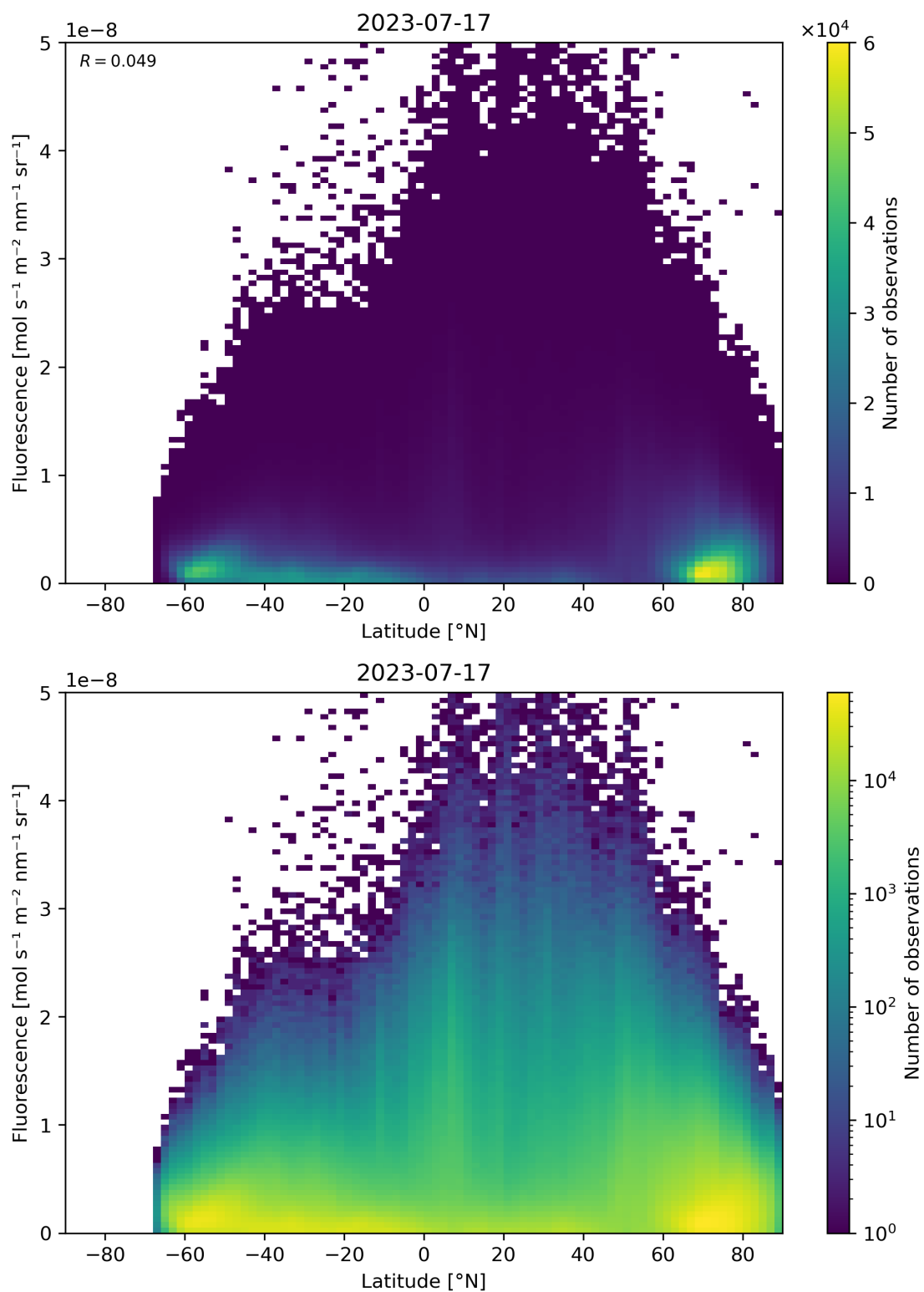
Figure 101: Scatter density plot of “Latitude” against “Fluorescence” for 2023-07-16 to 2023-07-18.
