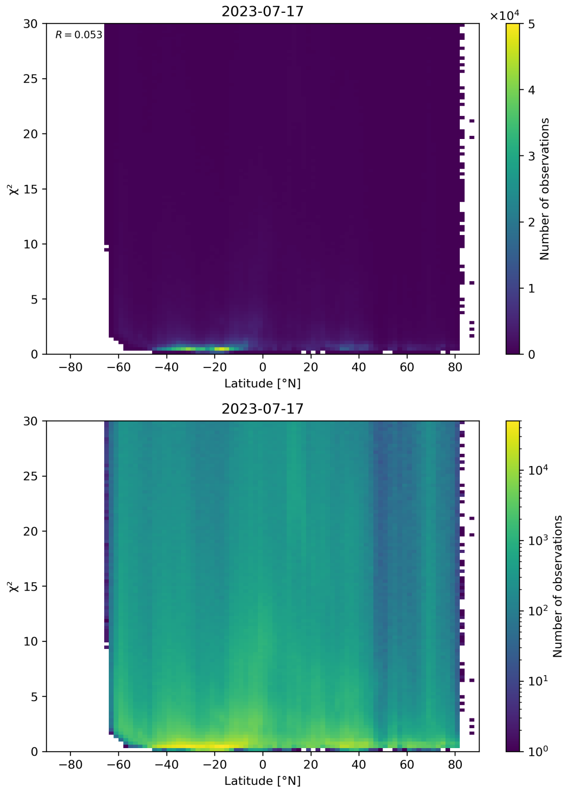
Figure 97: Scatter density plot of “Latitude” against “ \chi^2 ” for 2023-07-16 to 2023-07-18.
