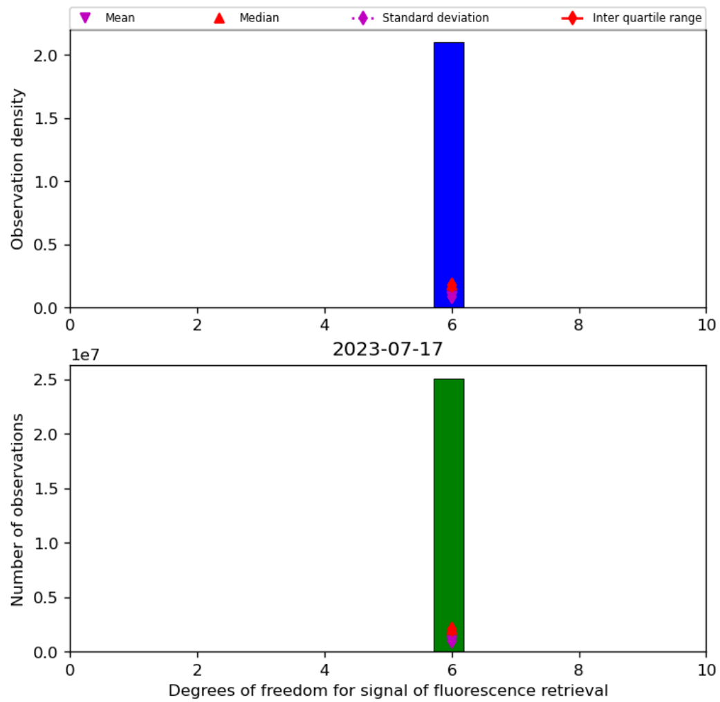
Figure 43: Histogram of “Degrees of freedom for signal of fluorescence retrieval” for 2023-07-16 to 2023-07-18
