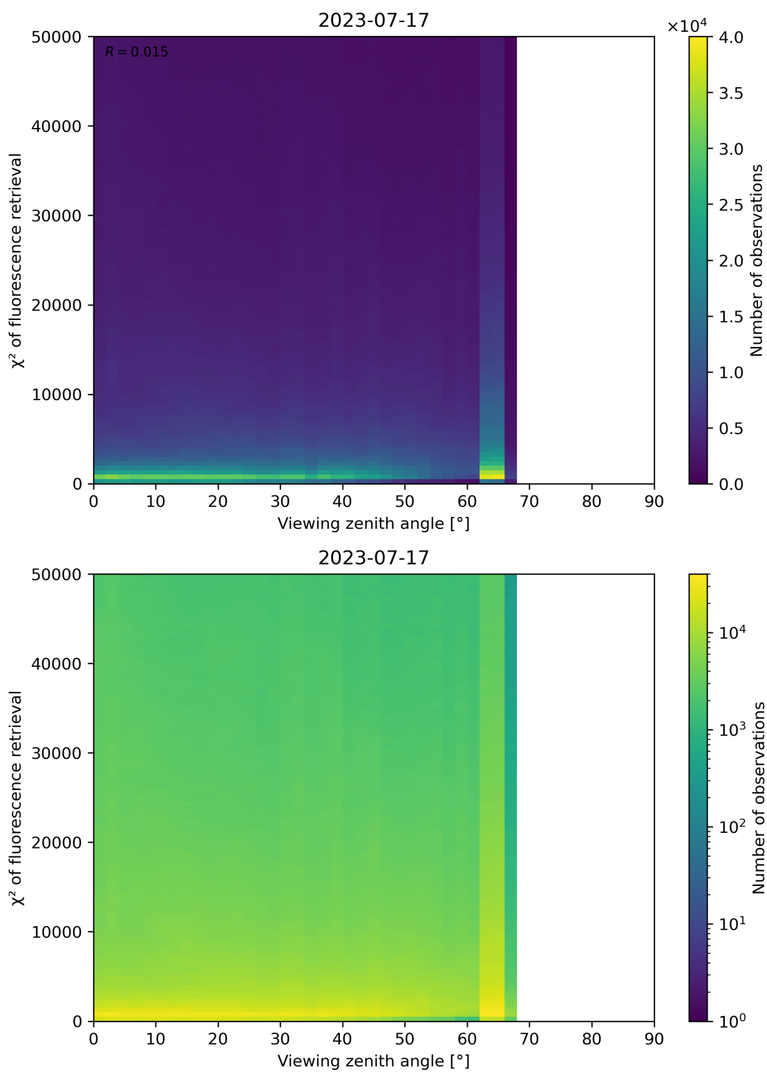
Figure 131: Scatter density plot of “Viewing zenith angle” against “ \chi^2 of fluorescence retrieval” for 2023-07-16 to 2023-07-18.
