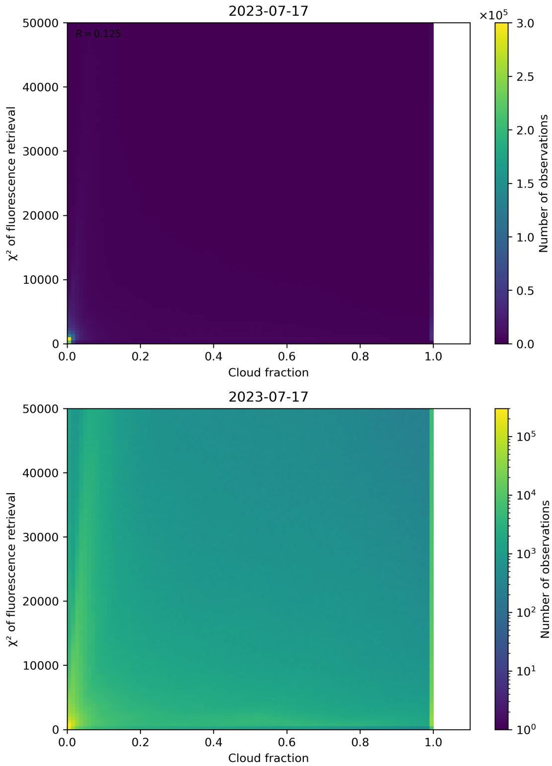
Figure 78: Scatter density plot of “Cloud fraction” against “ \chi^2 of fluorescence retrieval” for 2023-07-16 to 2023-07-18.
