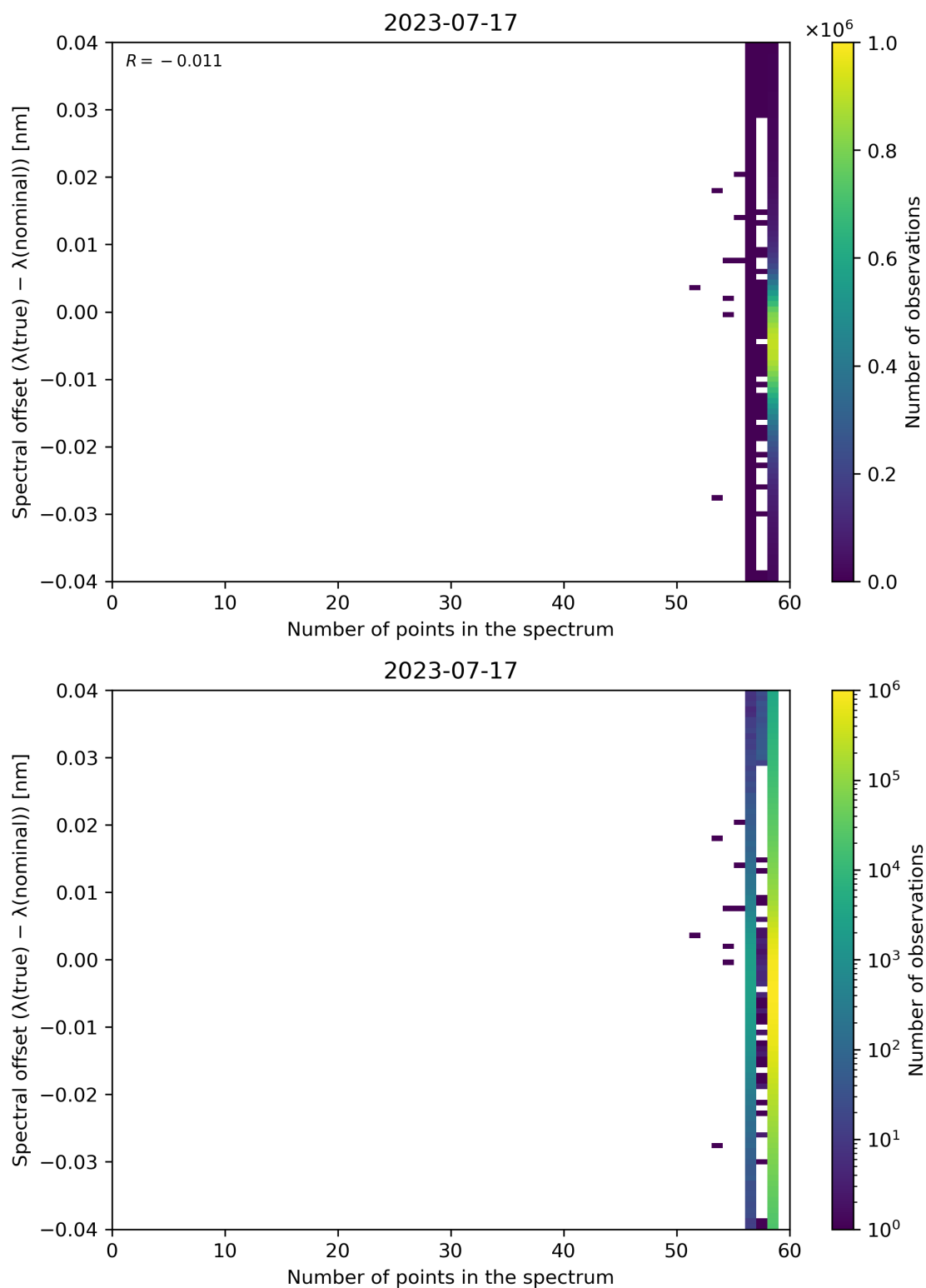
Figure 110: Scatter density plot of “Number of points in the spectrum” against “Spectral offset ( \lambda(\text{true}) - \lambda(\text{nominal}) )” for 2023-07-16 to 2023-07-18.
