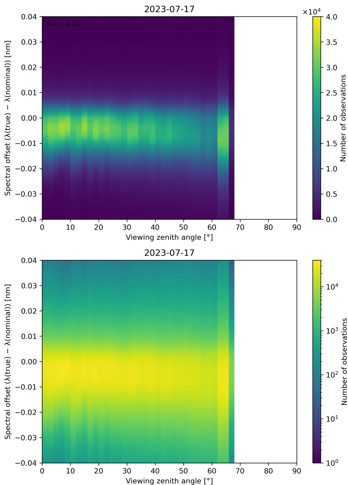
Figure 140: Scatter density plot of “Viewing zenith angle” against “Spectral offset ( \lambda(\text{true}) - \lambda(\text{nominal}) )” for 2023-07-16 to 2023-07-18.
