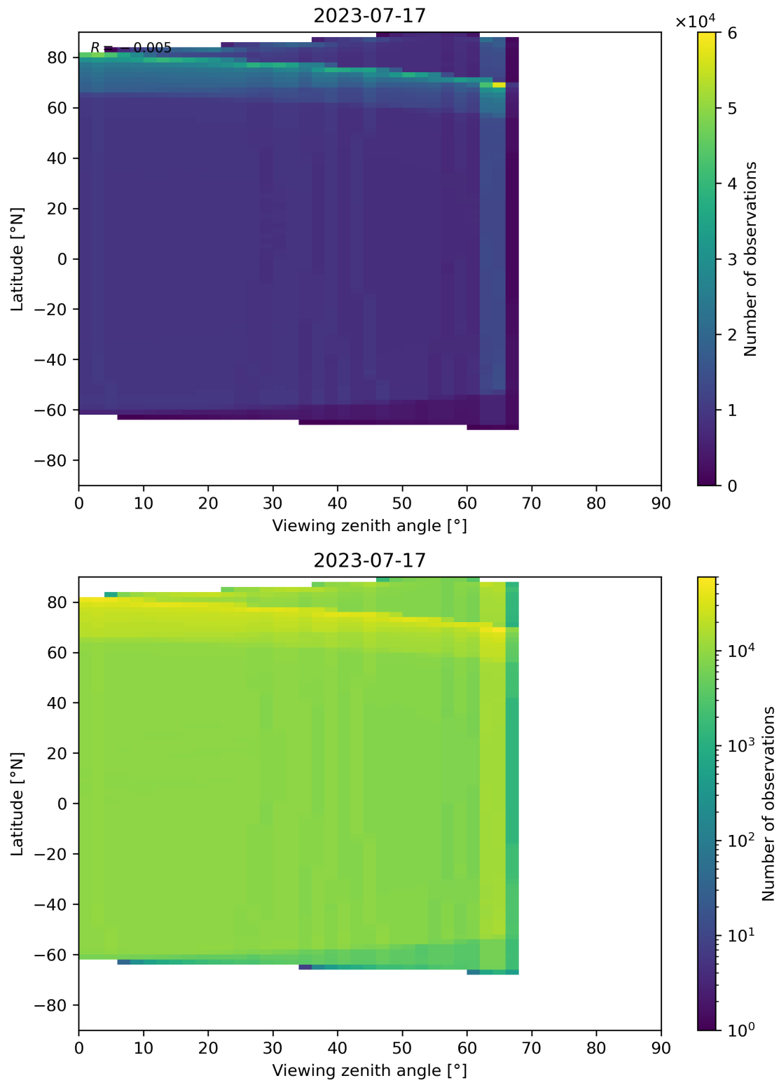
Figure 135: Scatter density plot of “Viewing zenith angle” against “Latitude” for 2023-07-16 to 2023-07-18.
