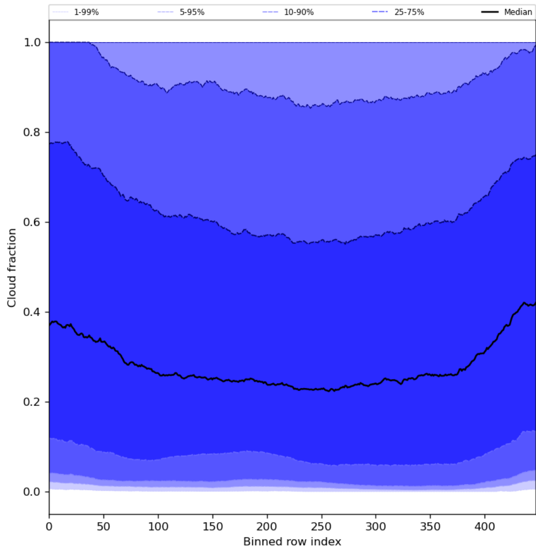
Figure 49: Along track statistics of “Cloud fraction” for 2023-07-16 to 2023-07-18
