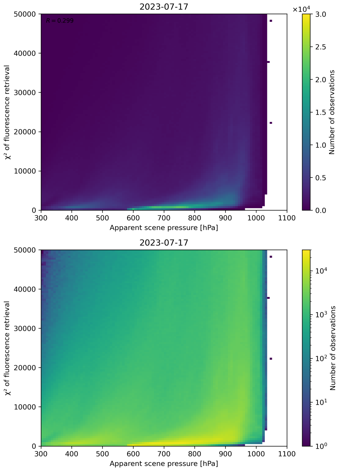
Figure 64: Scatter density plot of “Apparent scene pressure” against “ \chi^2 of fluorescence retrieval” for 2023-07-16 to 2023-07-18.
