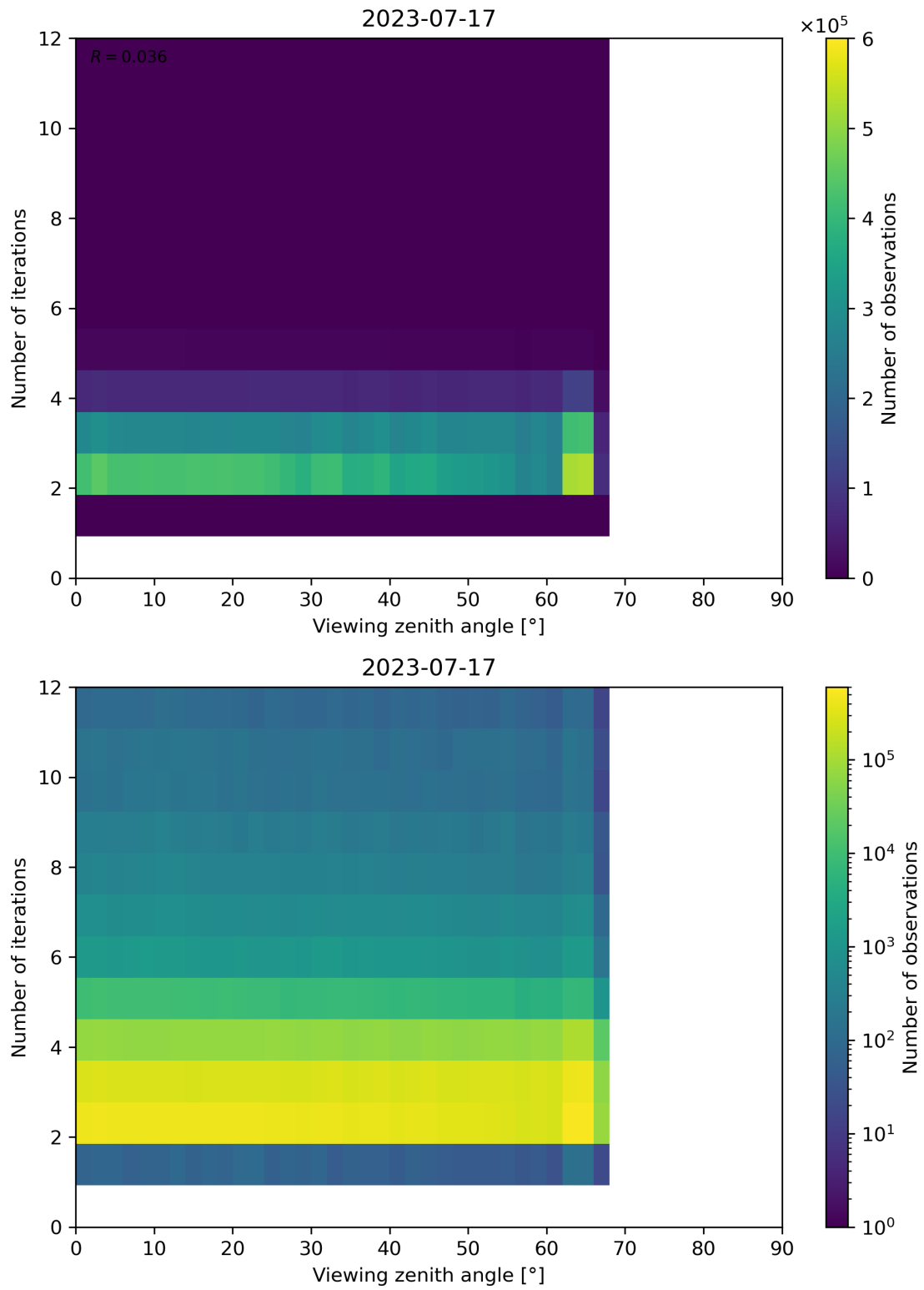
Figure 136: Scatter density plot of “Viewing zenith angle” against “Number of iterations” for 2023-07-16 to 2023-07-18.
