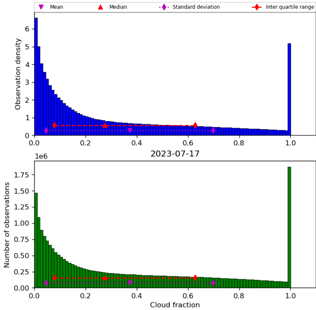
Figure 32: Histogram of “Cloud fraction” for 2023-07-16 to 2023-07-18
