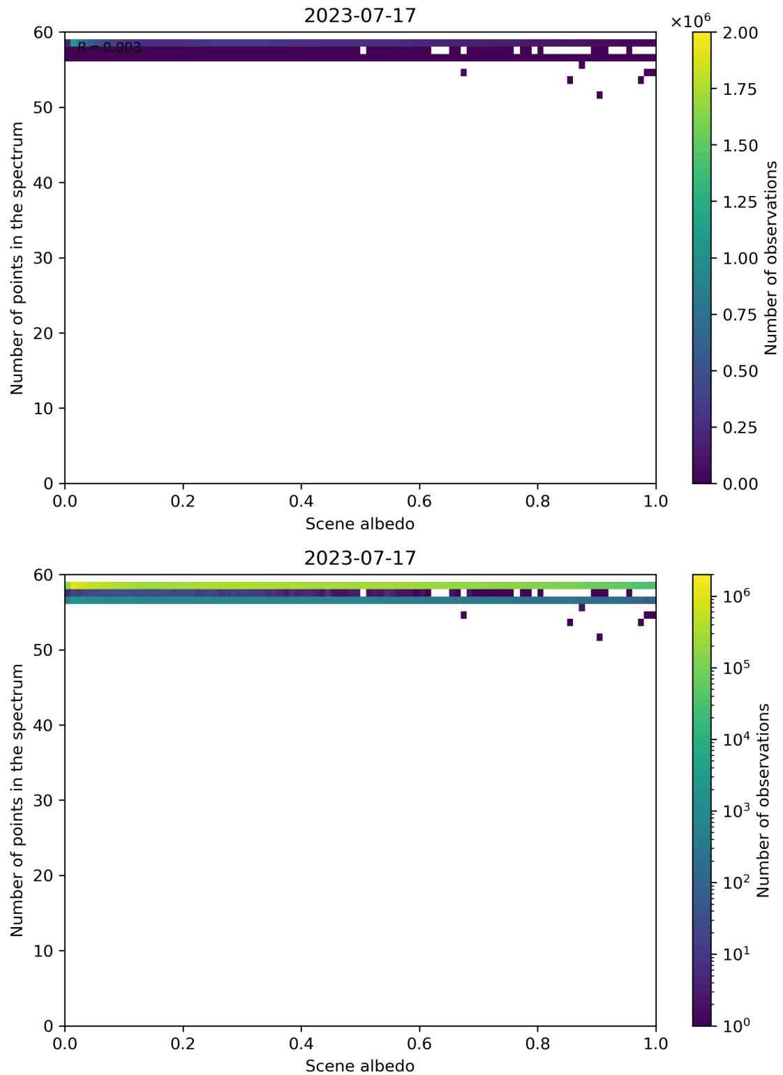
Figure 116: Scatter density plot of “Scene albedo” against “Number of points in the spectrum” for 2023-07-16 to 2023-07-18.
