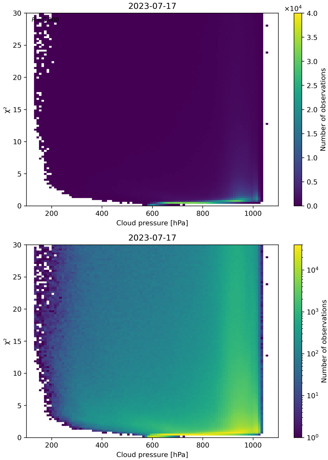
Figure 85: Scatter density plot of “Cloud pressure” against “ \chi^2 ” for 2023-07-16 to 2023-07-18.
