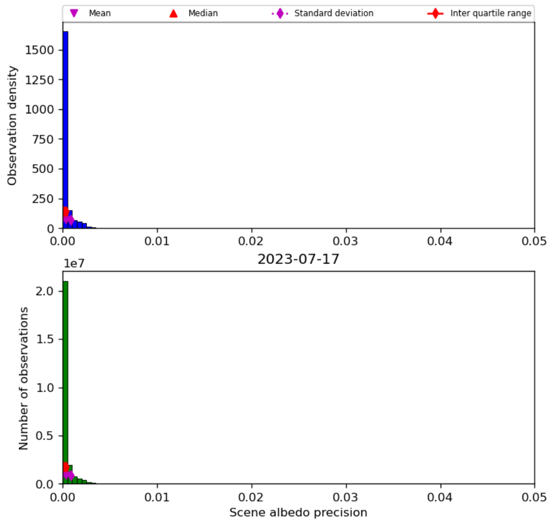
Figure 35: Histogram of “Scene albedo precision” for 2023-07-16 to 2023-07-18
