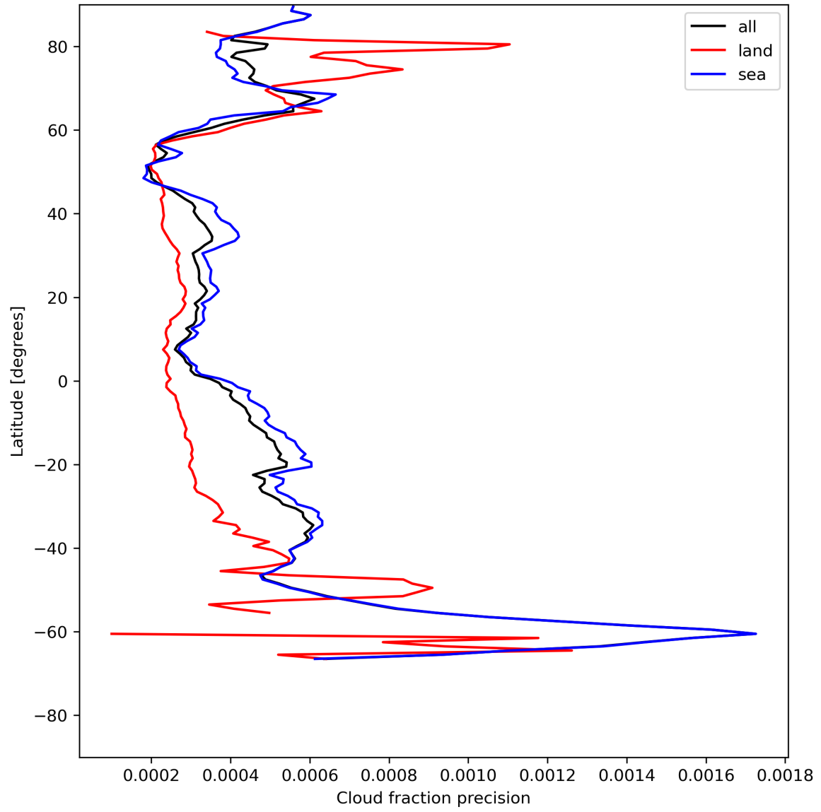
Figure 16: Zonal average of “Cloud fraction precision” for 2023-07-16 to 2023-07-18.
