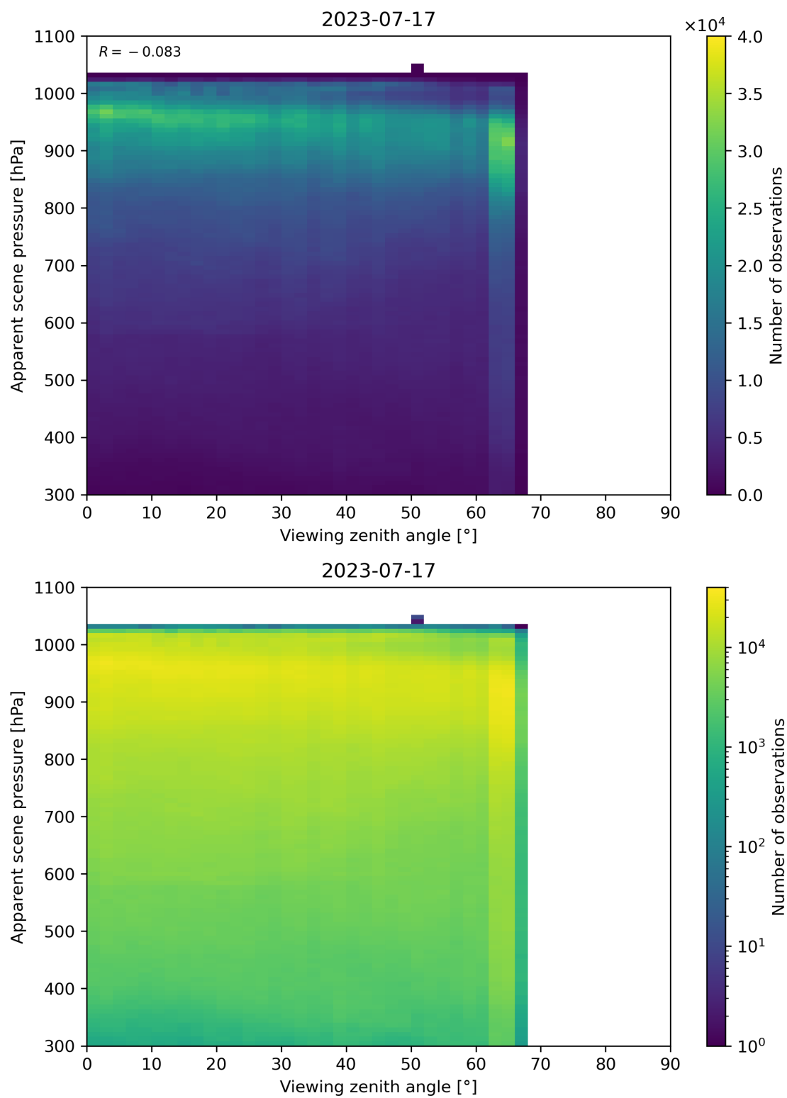
Figure 129: Scatter density plot of “Viewing zenith angle” against “Apparent scene pressure” for 2023-07-16 to 2023-07-18.
