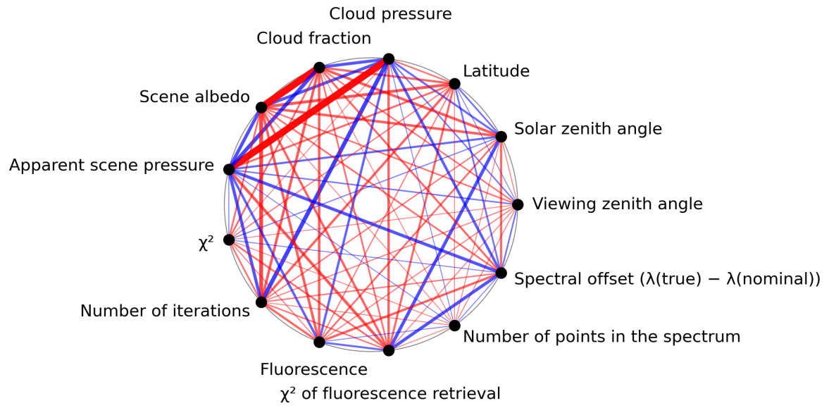
Figure 1: Map of correlation graph for 2023-07-16 to 2023-07-18.
