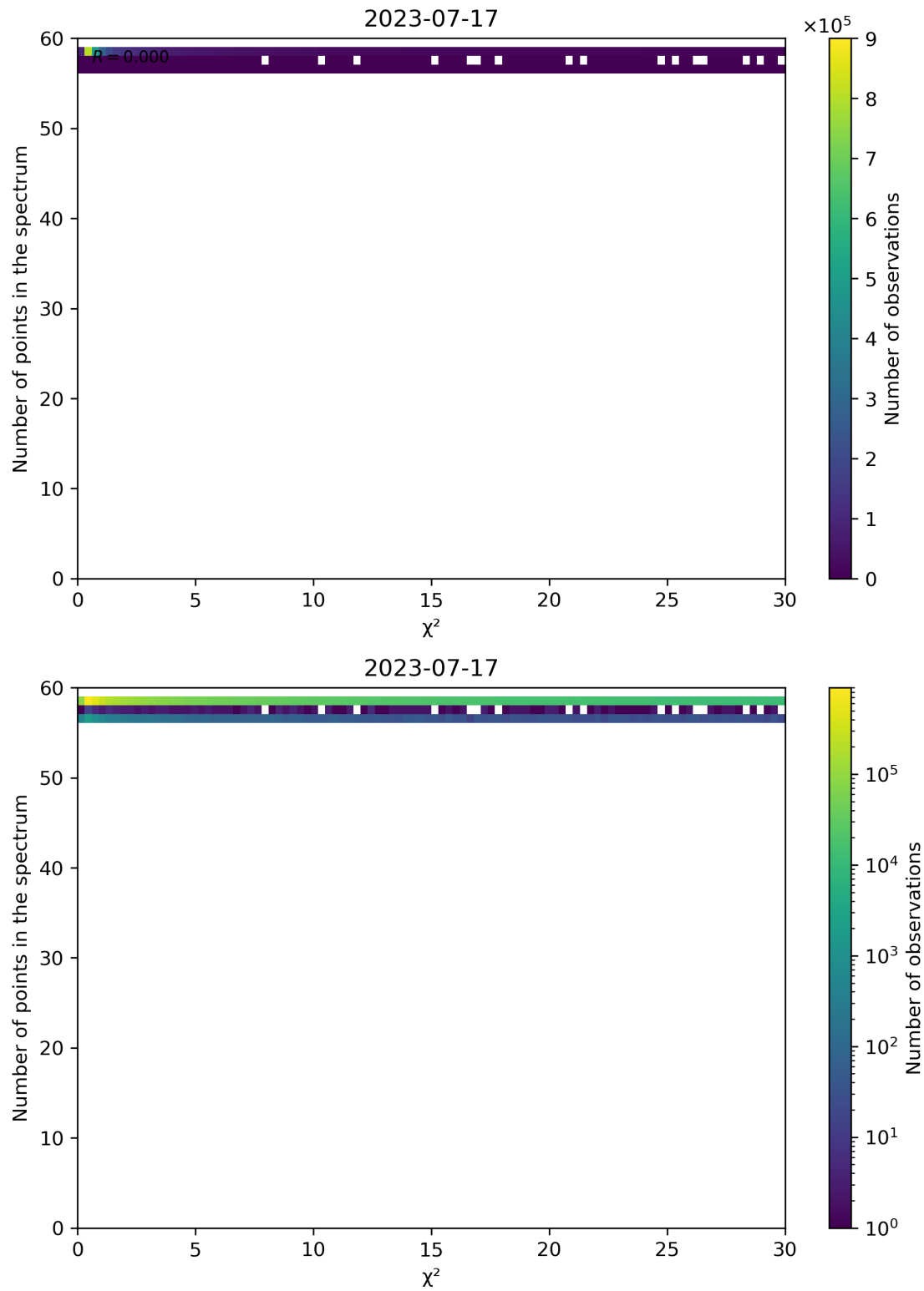
Figure 74: Scatter density plot of “ \chi^2 ” against “Number of points in the spectrum” for 2023-07-16 to 2023-07-18.
