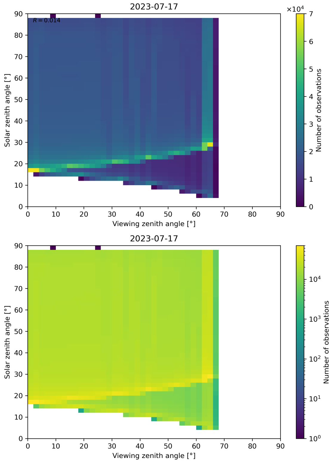
Figure 139: Scatter density plot of “Viewing zenith angle” against “Solar zenith angle” for 2023-07-16 to 2023-07-18.
