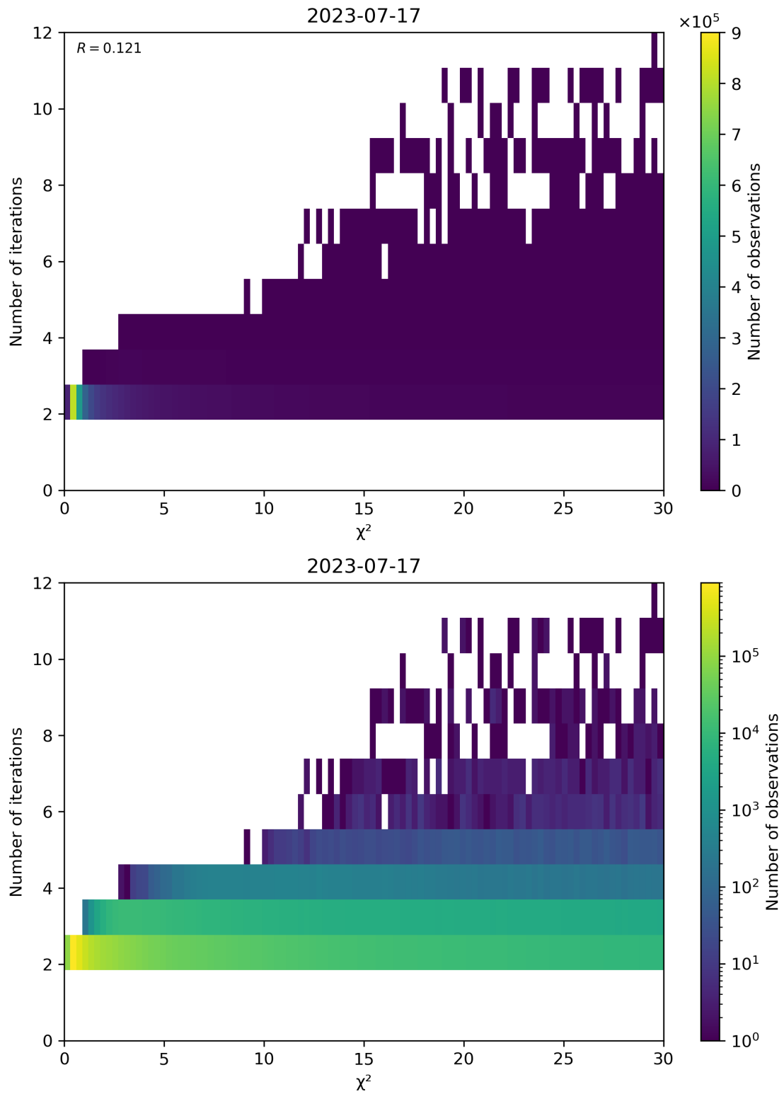
Figure 73: Scatter density plot of “ \chi^2 ” against “Number of iterations” for 2023-07-16 to 2023-07-18.
