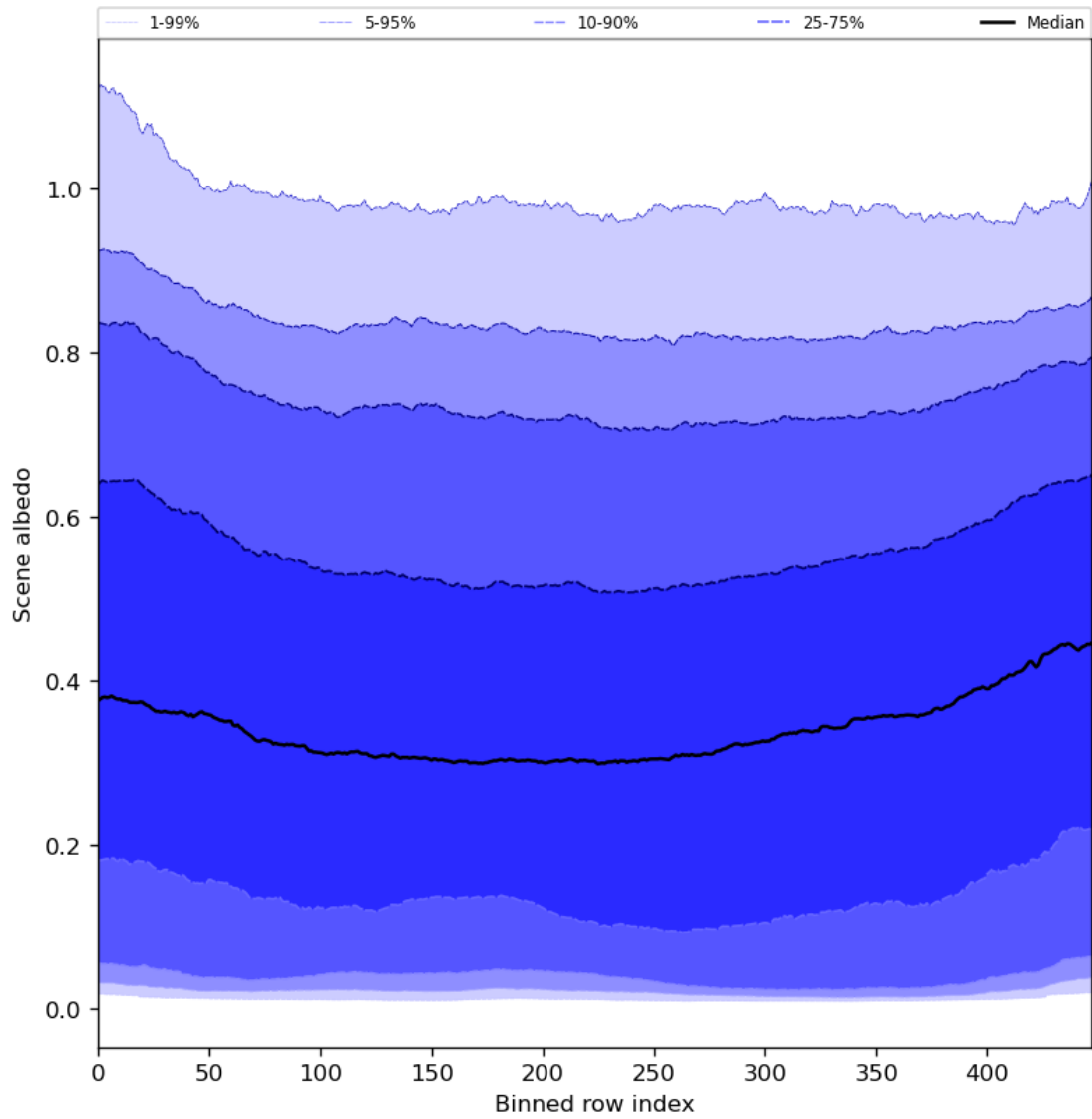
Figure 51: Along track statistics of “Scene albedo” for 2023-07-16 to 2023-07-18
