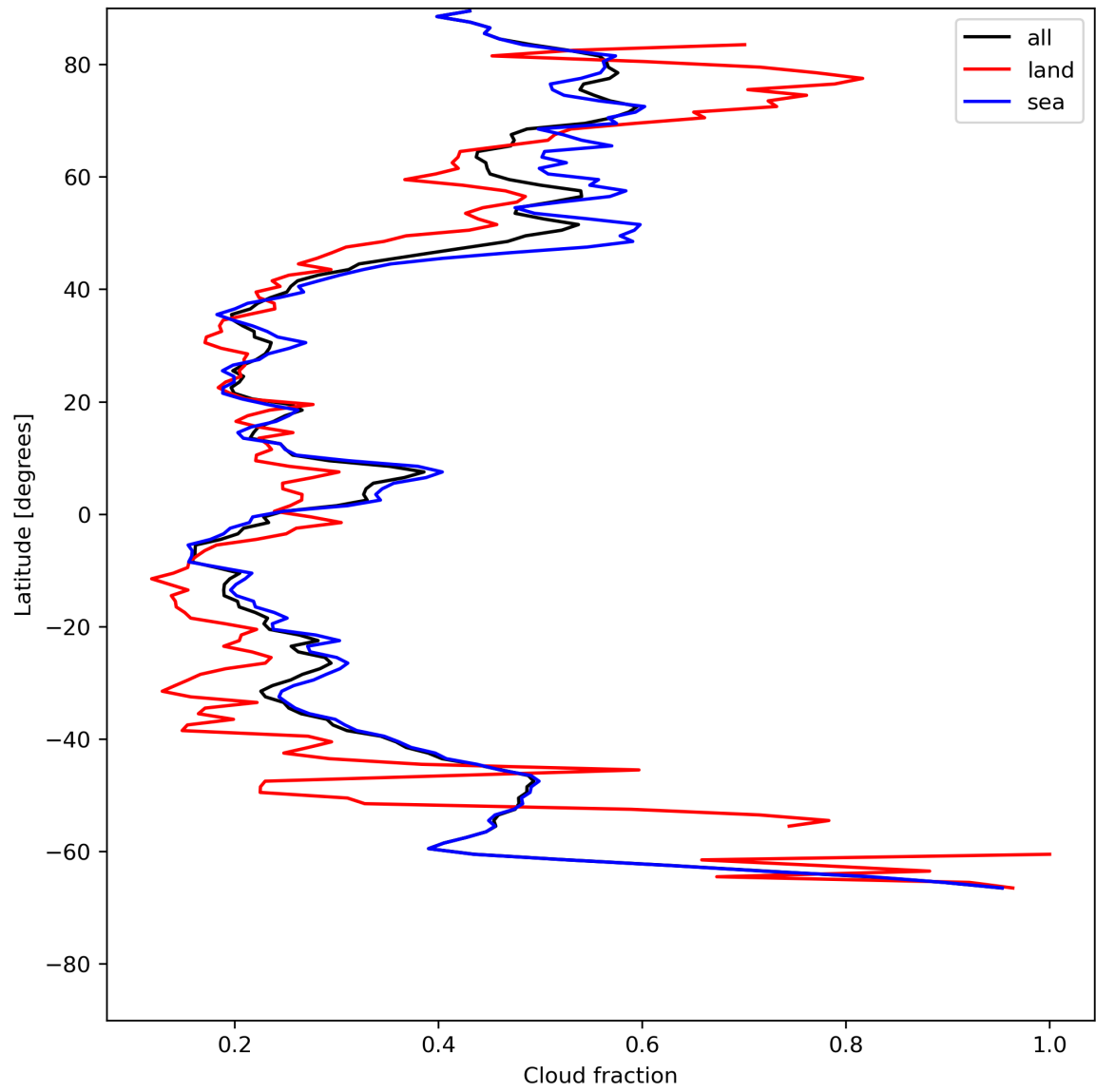
Figure 15: Zonal average of “Cloud fraction” for 2023-07-16 to 2023-07-18.
