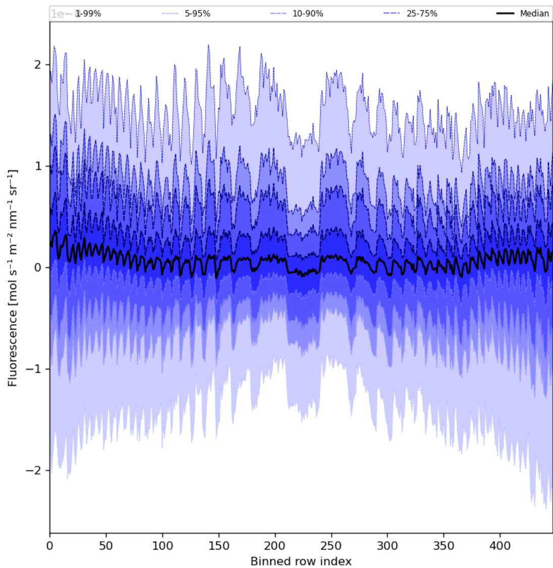
Figure 57: Along track statistics of “Fluorescence” for 2023-07-16 to 2023-07-18
