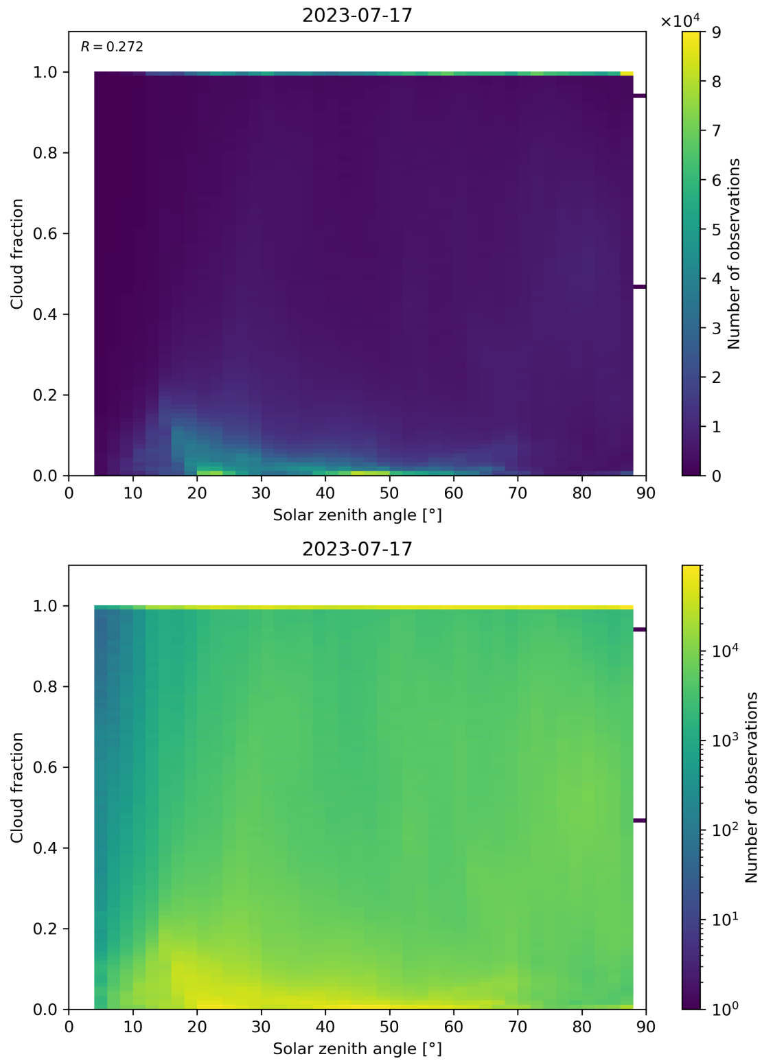
Figure 121: Scatter density plot of “Solar zenith angle” against “Cloud fraction” for 2023-07-16 to 2023-07-18.
