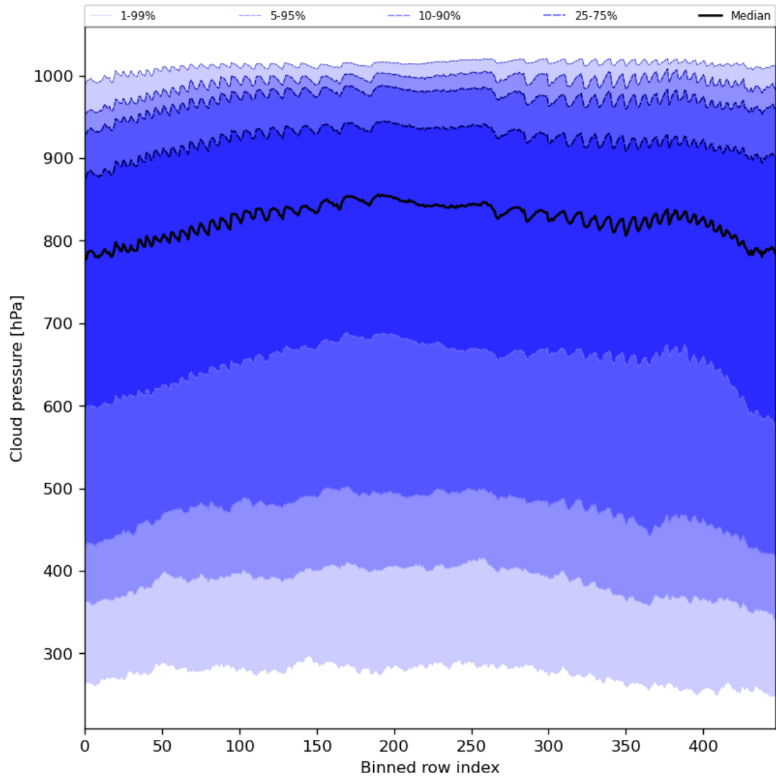
Figure 47: Along track statistics of “Cloud pressure” for 2023-07-16 to 2023-07-18
