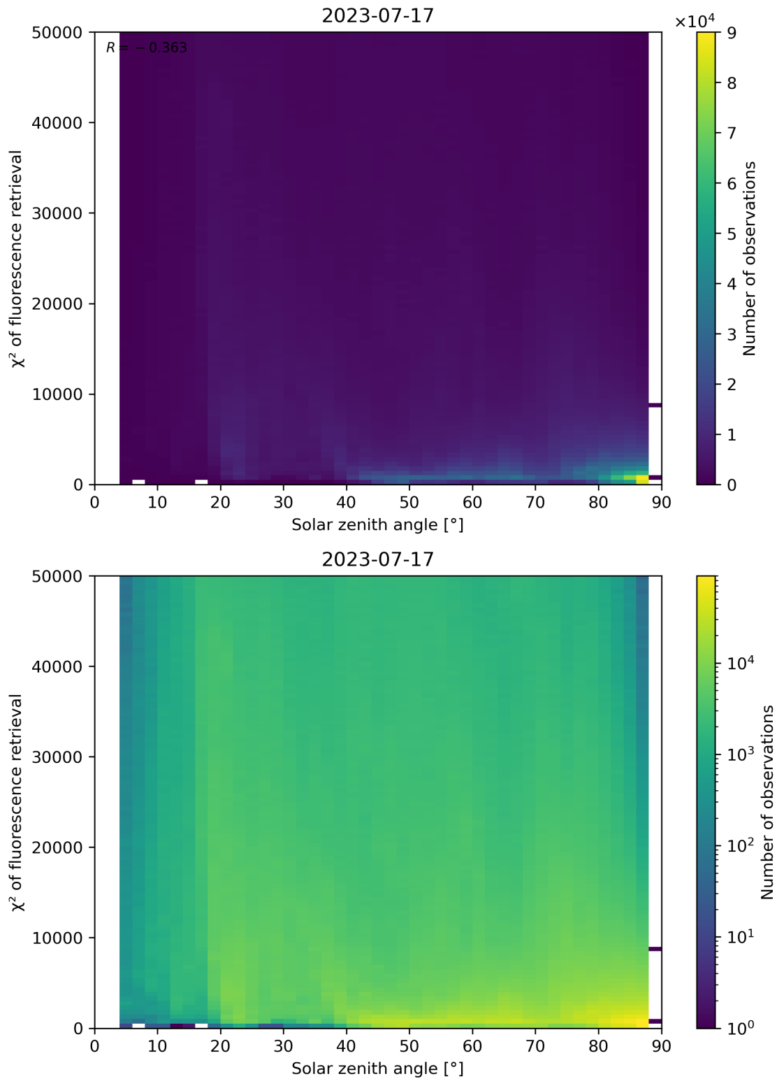
Figure 120: Scatter density plot of “Solar zenith angle” against “ \chi^2 of fluorescence retrieval” for 2023-07-16 to 2023-07-18.
