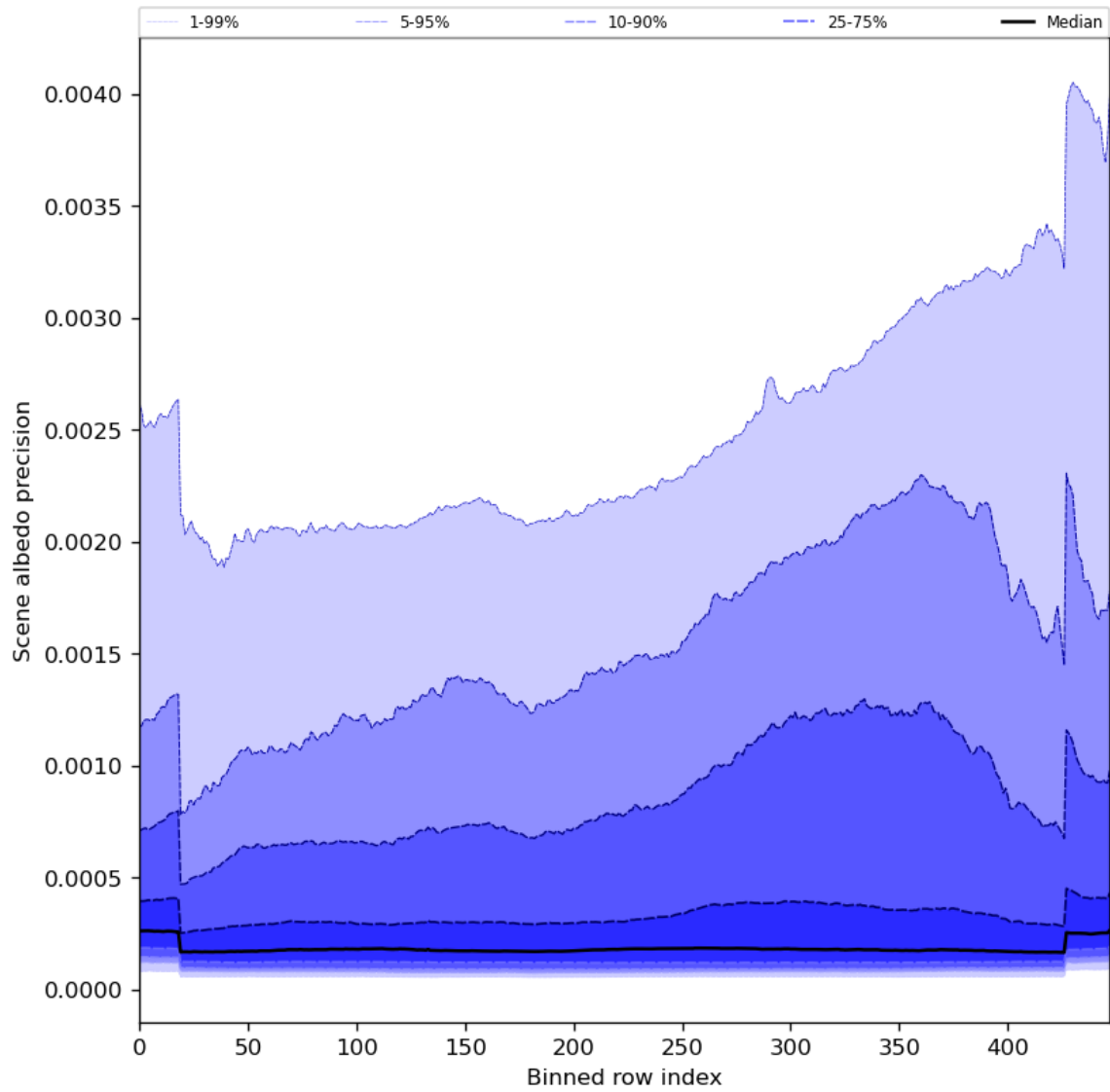
Figure 52: Along track statistics of “Scene albedo precision” for 2023-07-16 to 2023-07-18
