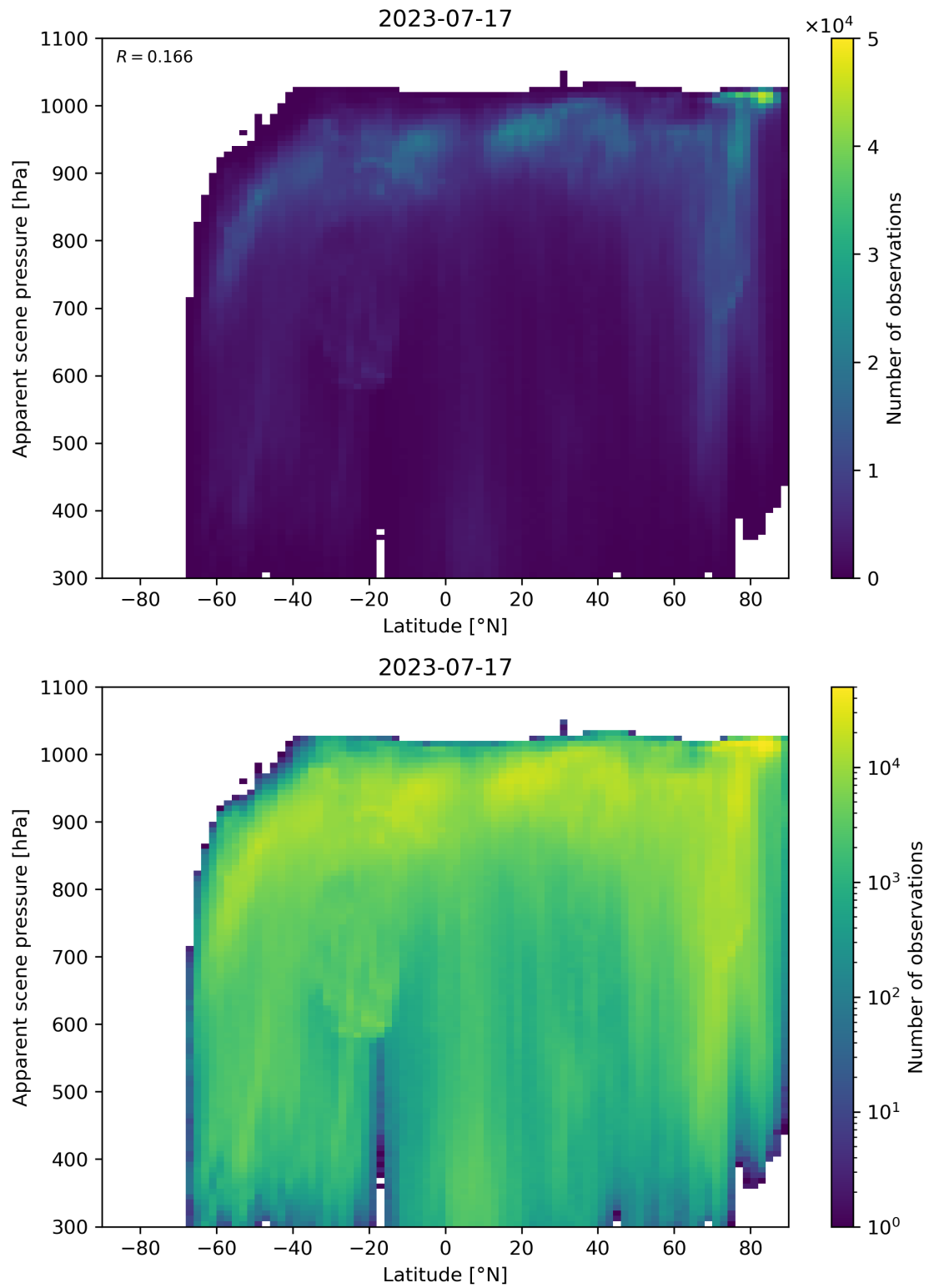
Figure 96: Scatter density plot of “Latitude” against “Apparent scene pressure” for 2023-07-16 to 2023-07-18.
