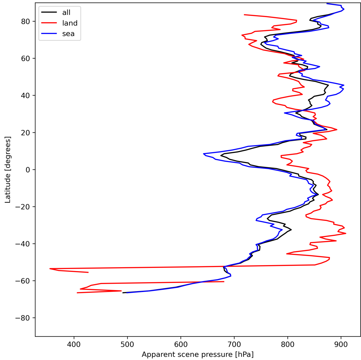
Figure 19: Zonal average of “Apparent scene pressure” for 2023-07-16 to 2023-07-18.
