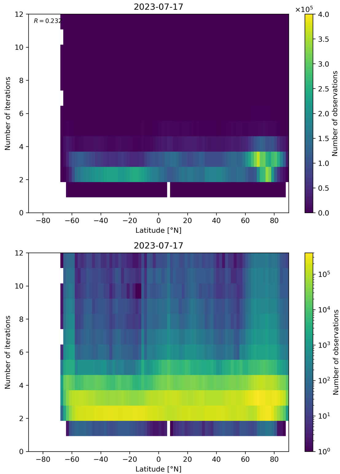
Figure 102: Scatter density plot of “Latitude” against “Number of iterations” for 2023-07-16 to 2023-07-18.
