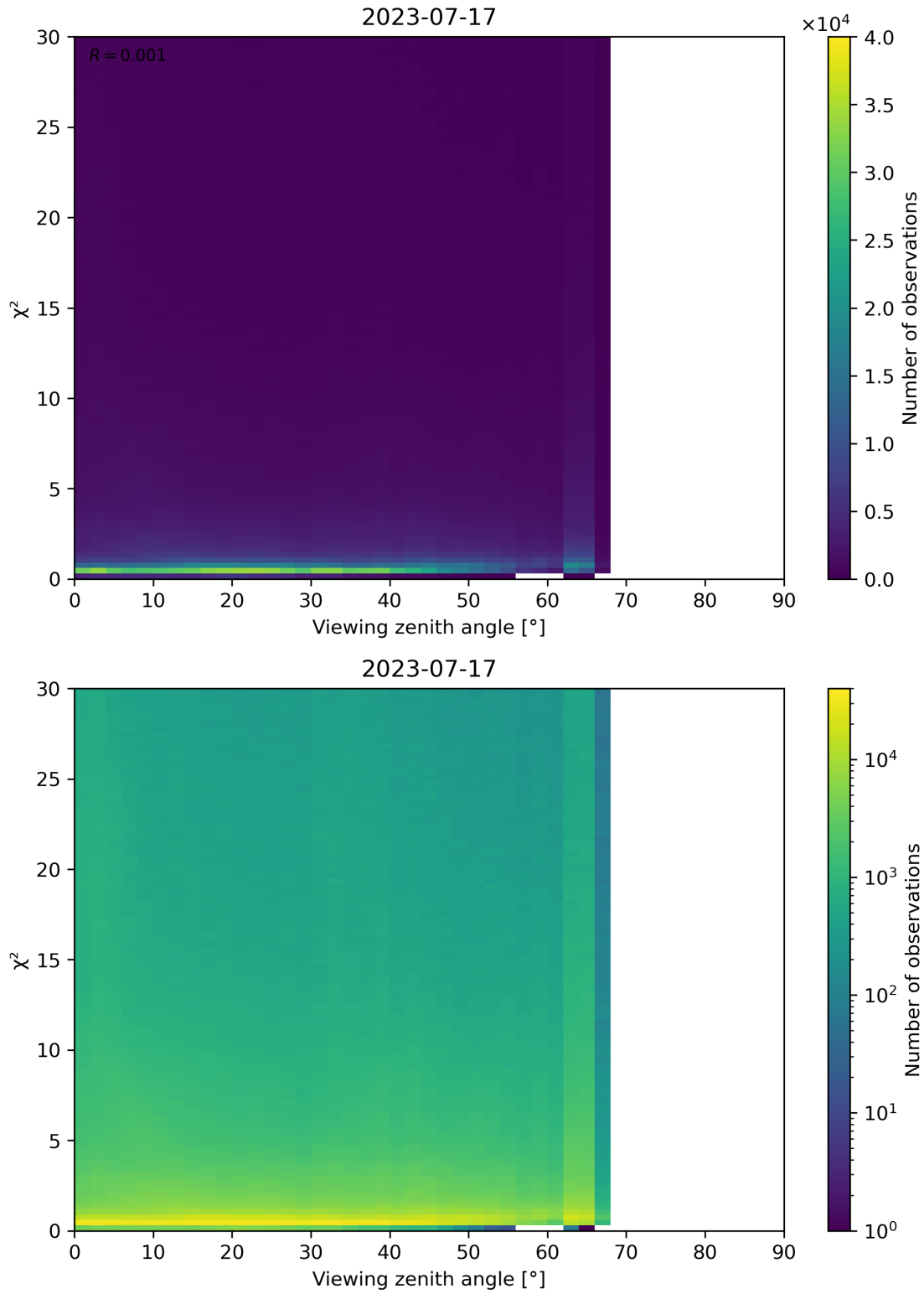
Figure 130: Scatter density plot of “Viewing zenith angle” against “ \chi^2 ” for 2023-07-16 to 2023-07-18.
