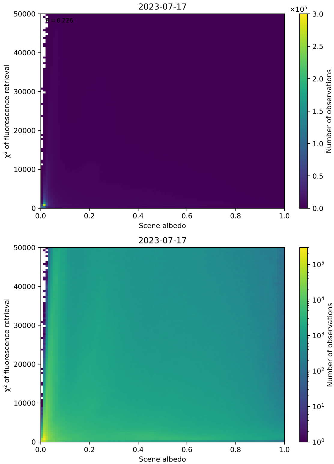
Figure 113: Scatter density plot of “Scene albedo” against “ \chi^2 of fluorescence retrieval” for 2023-07-16 to 2023-07-18.
