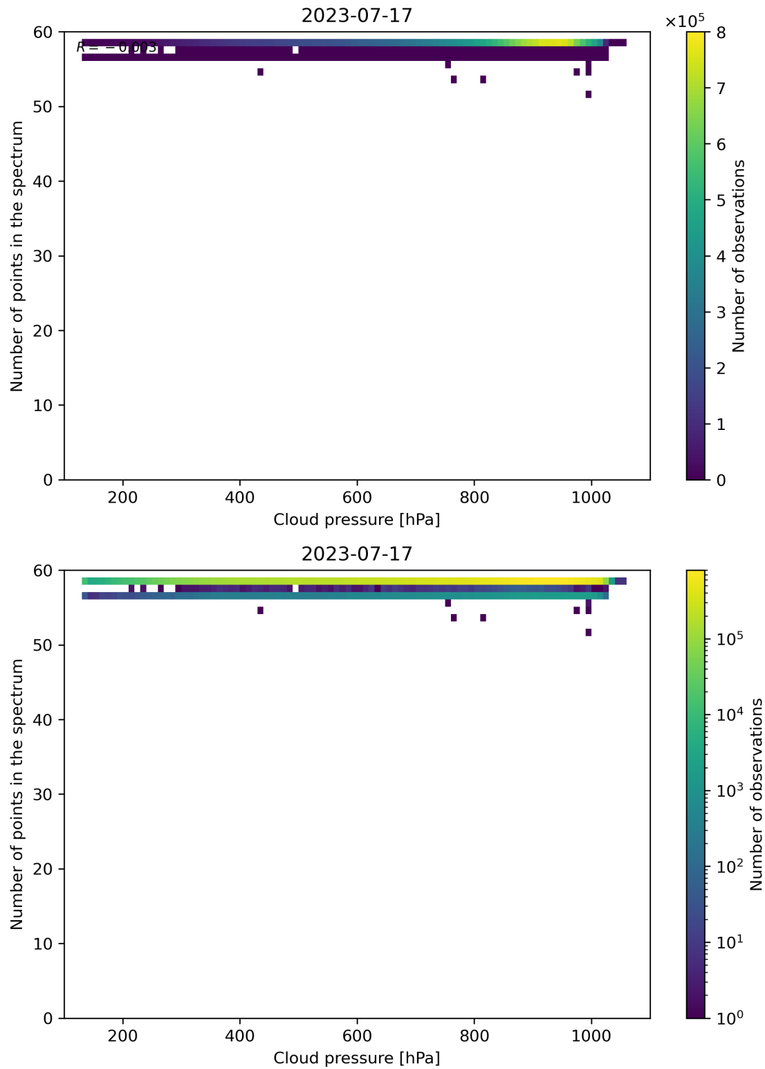
Figure 90: Scatter density plot of “Cloud pressure” against “Number of points in the spectrum” for 2023-07-16 to 2023-07-18.
