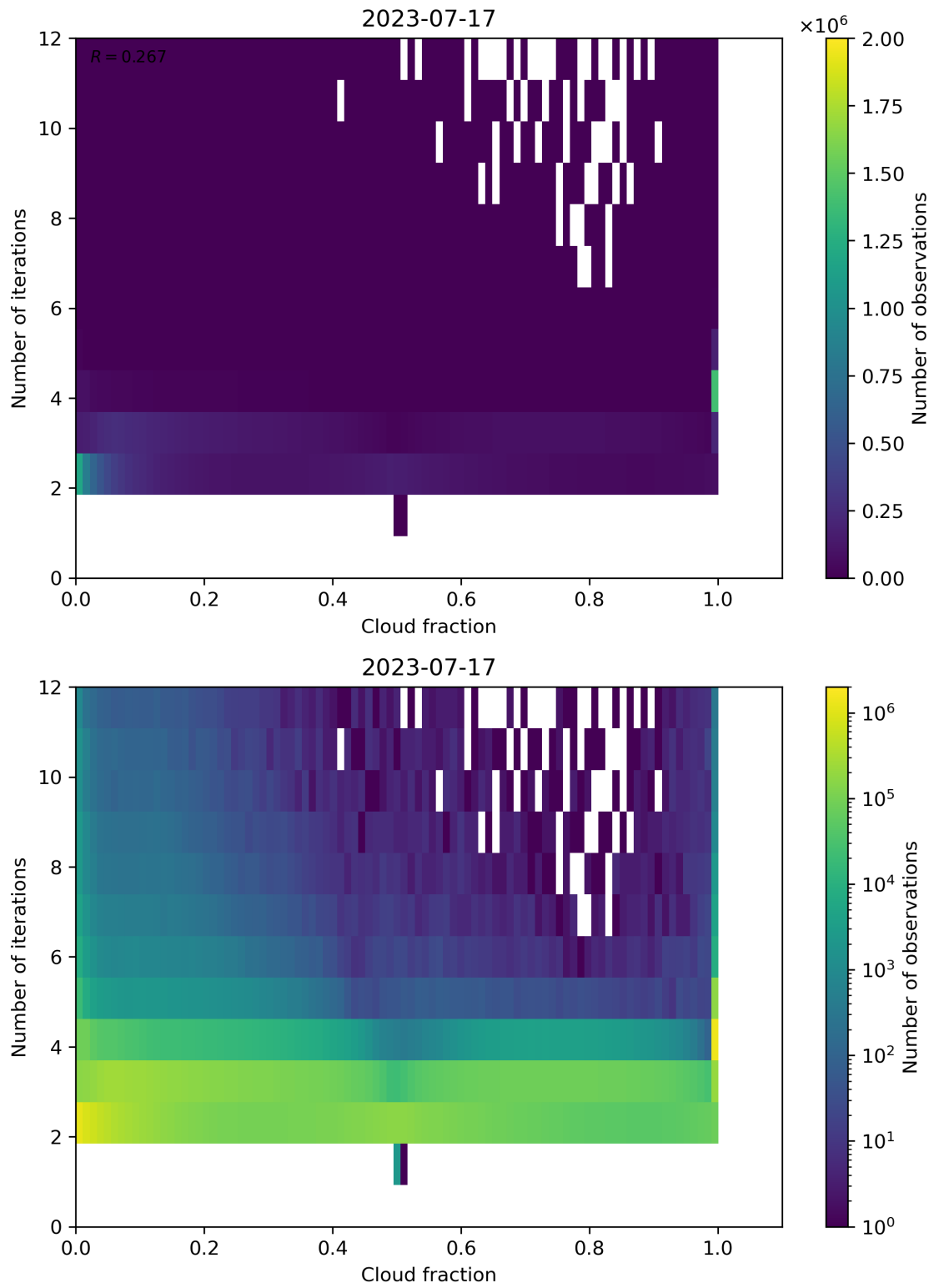
Figure 80: Scatter density plot of “Cloud fraction” against “Number of iterations” for 2023-07-16 to 2023-07-18.
