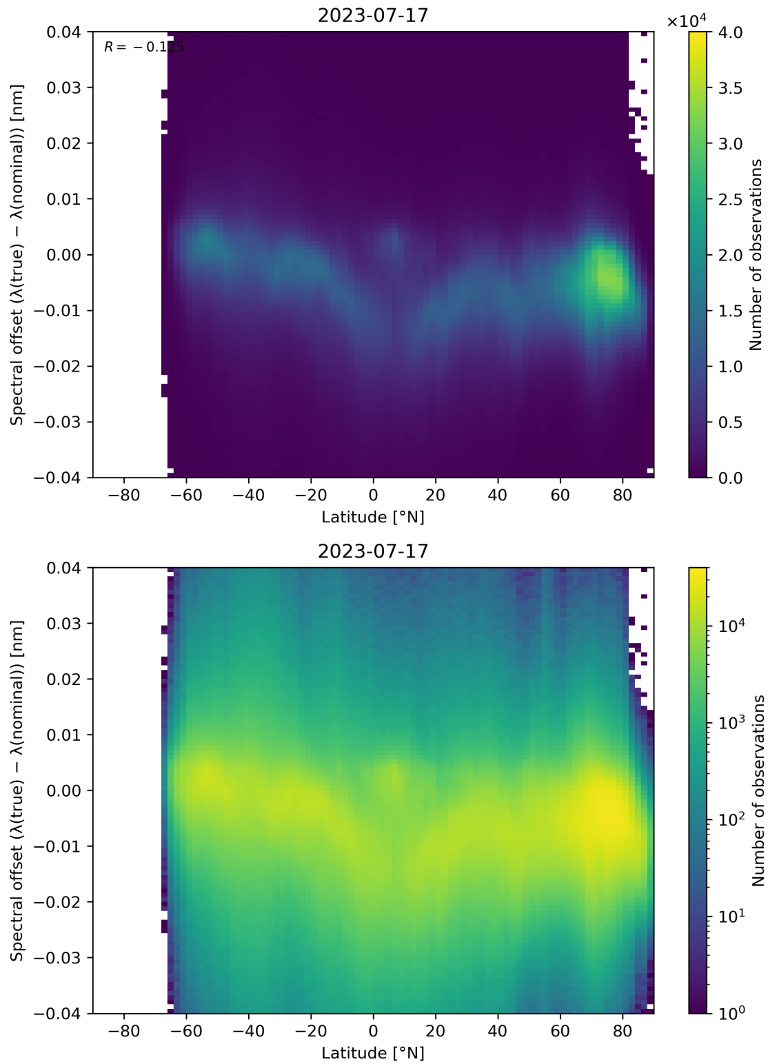
Figure 105: Scatter density plot of “Latitude” against “Spectral offset ( \lambda(\text{true}) - \lambda(\text{nominal}) )” for 2023-07-16 to 2023-07-18.
