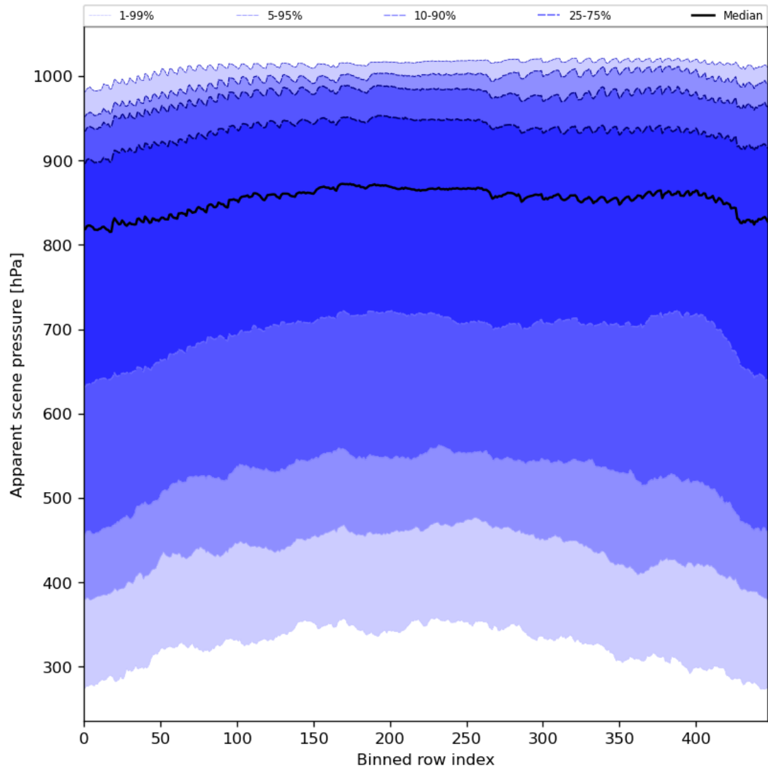
Figure 53: Along track statistics of “Apparent scene pressure” for 2023-07-16 to 2023-07-18
