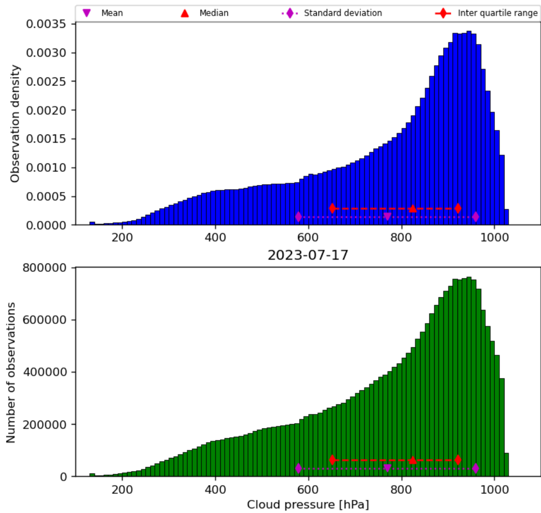
Figure 30: Histogram of “Cloud pressure” for 2023-07-16 to 2023-07-18
