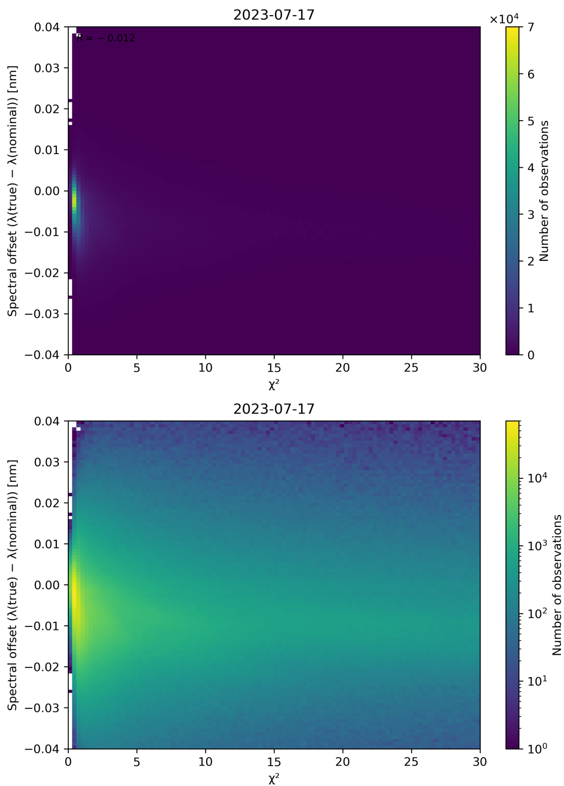
Figure 75: Scatter density plot of “ \chi^2 ” against “Spectral offset ( \lambda(\text{true}) - \lambda(\text{nominal}) )” for 2023-07-16 to 2023-07-18.
