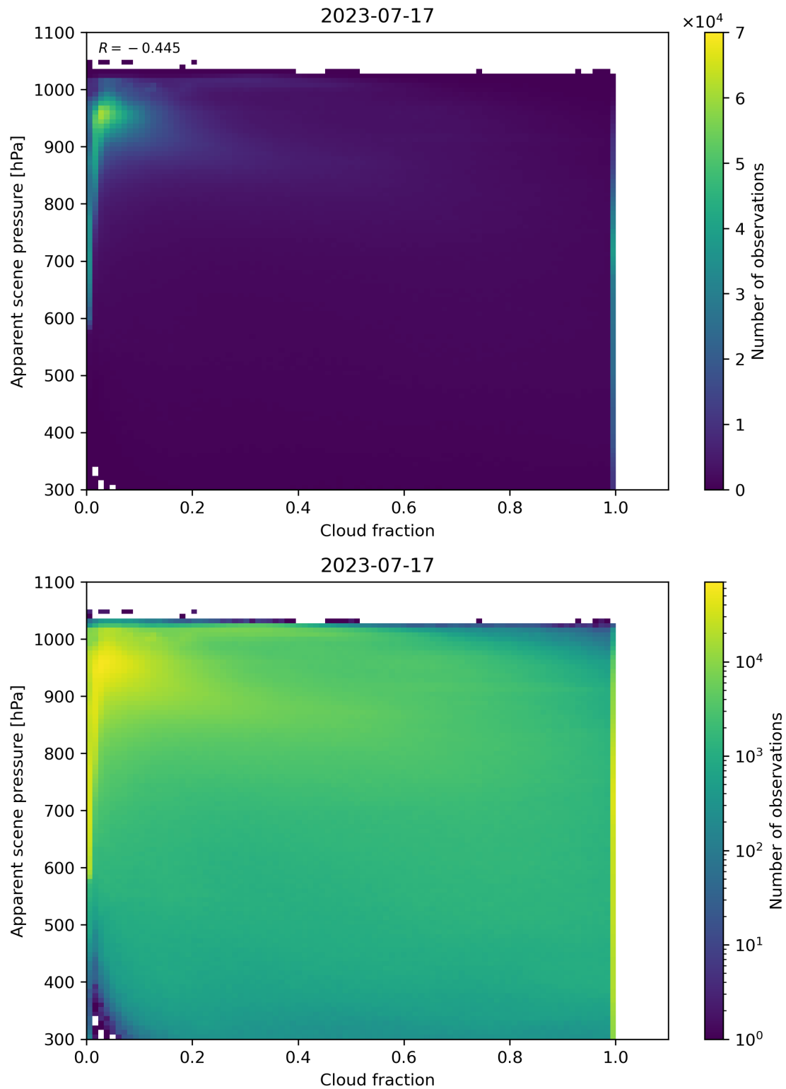
Figure 76: Scatter density plot of “Cloud fraction” against “Apparent scene pressure” for 2023-07-16 to 2023-07-18.
