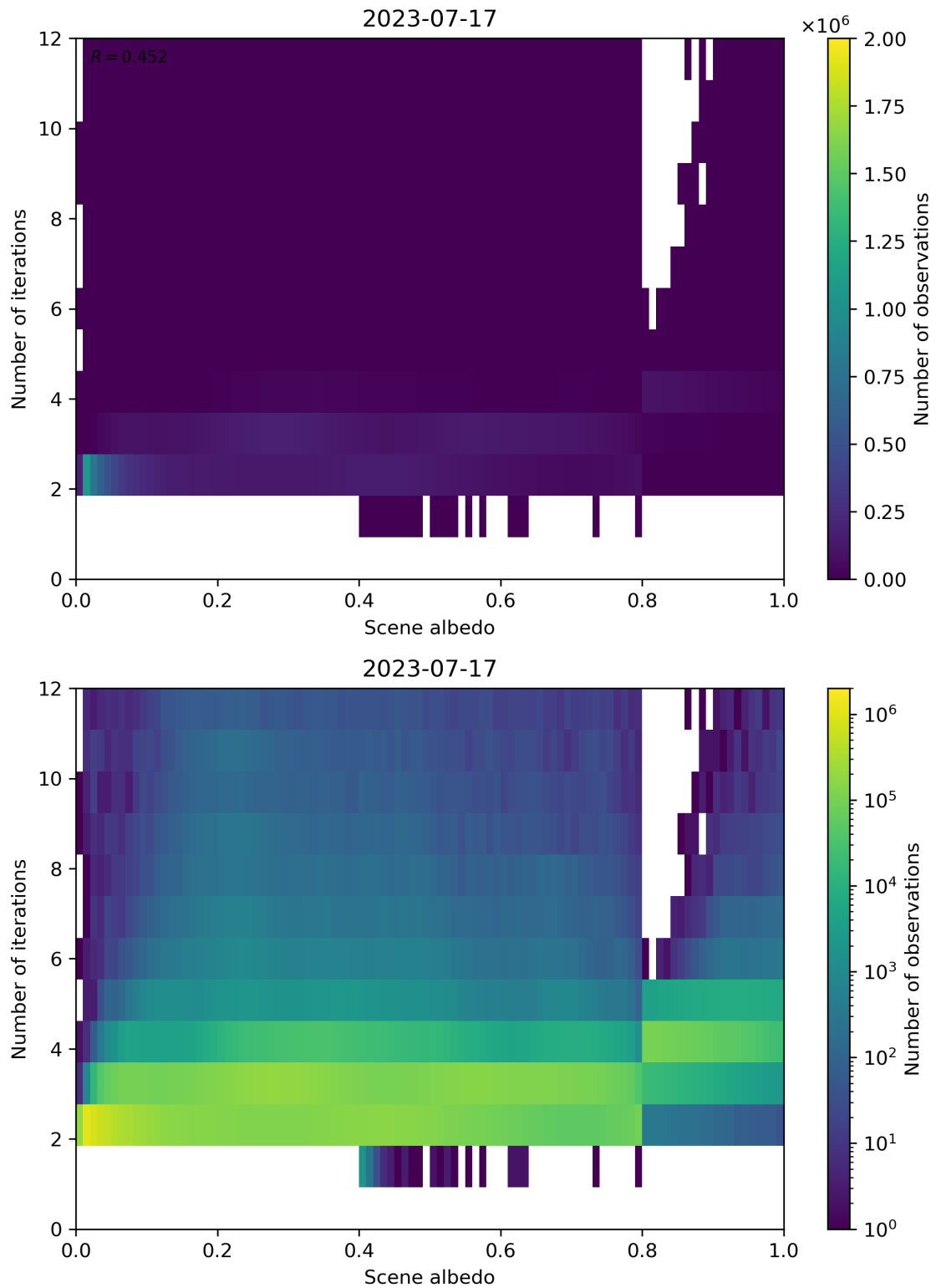
Figure 115: Scatter density plot of “Scene albedo” against “Number of iterations” for 2023-07-16 to 2023-07-18.
