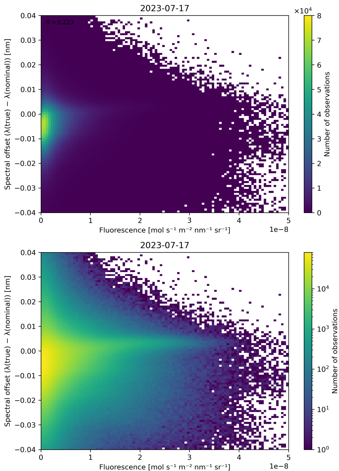
Figure 95: Scatter density plot of “Fluorescence” against “Spectral offset ( \lambda(\text{true}) - \lambda(\text{nominal}) )” for 2023-07-16 to 2023-07-18.
