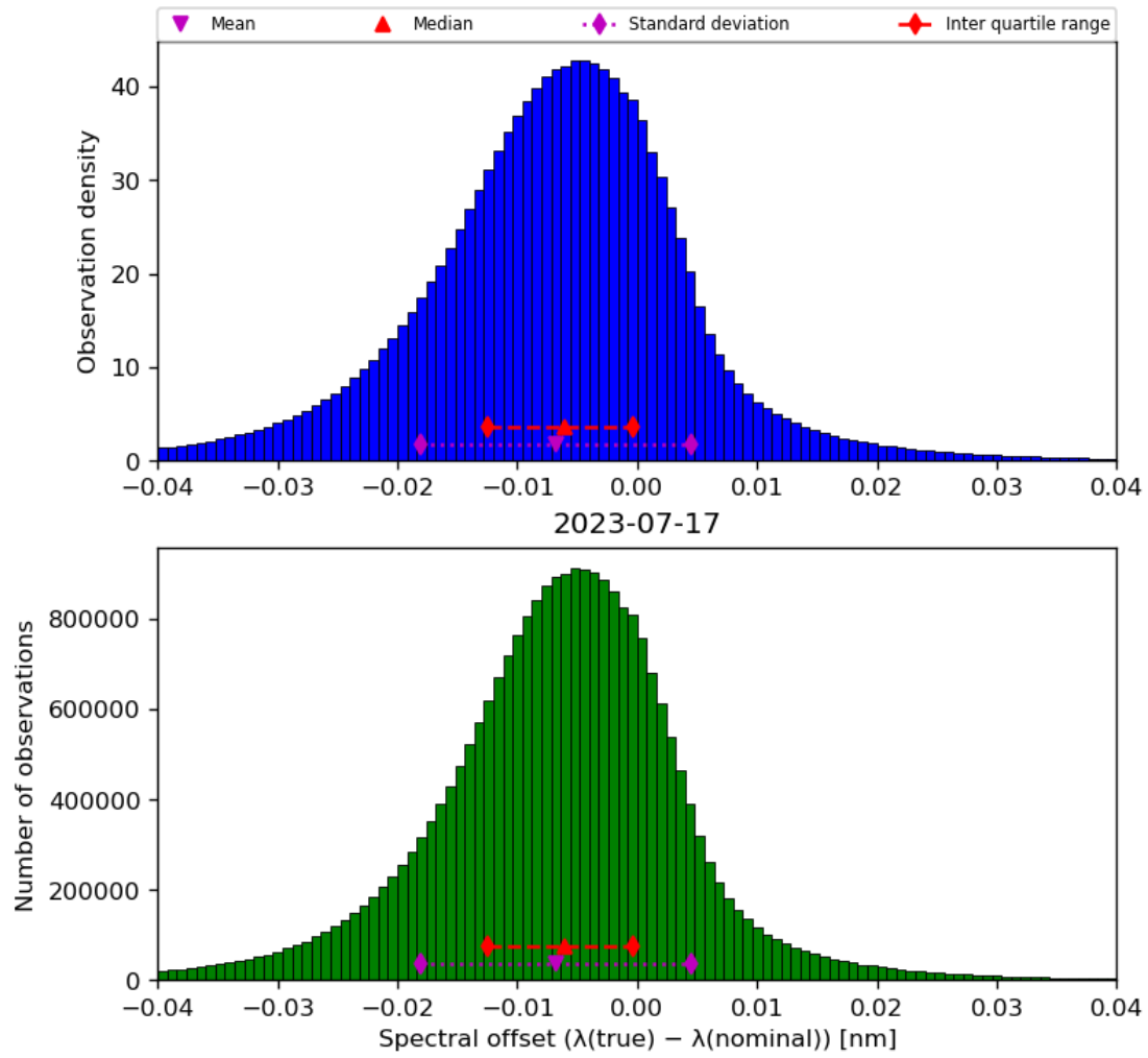
Figure 45: Histogram of “Spectral offset ( \lambda(\text{true}) - \lambda(\text{nominal}) )” for 2023-07-16 to 2023-07-18
