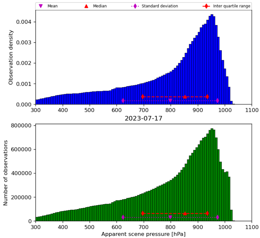
Figure 36: Histogram of “Apparent scene pressure” for 2023-07-16 to 2023-07-18
