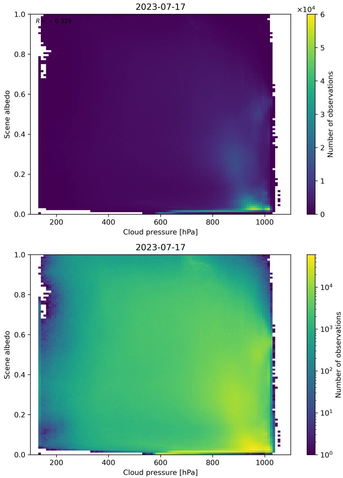
Figure 91: Scatter density plot of “Cloud pressure” against “Scene albedo” for 2023-07-16 to 2023-07-18.
