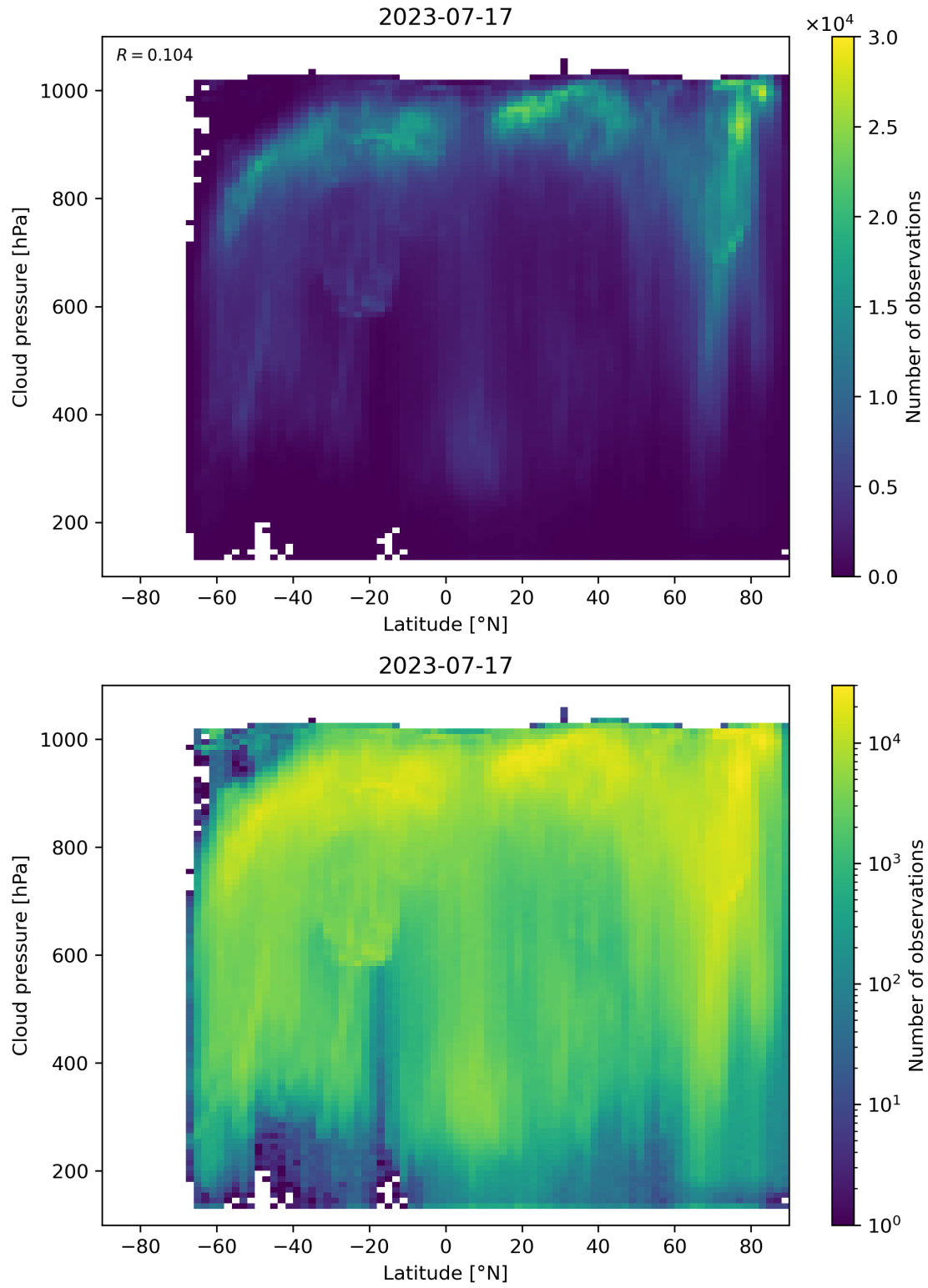
Figure 100: Scatter density plot of “Latitude” against “Cloud pressure” for 2023-07-16 to 2023-07-18.
