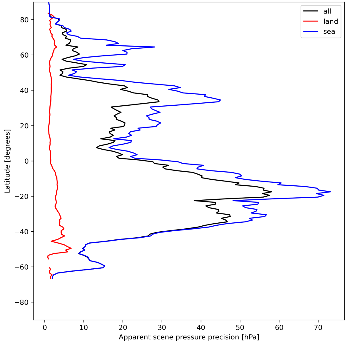
Figure 20: Zonal average of “Apparent scene pressure precision” for 2023-07-16 to 2023-07-18.
