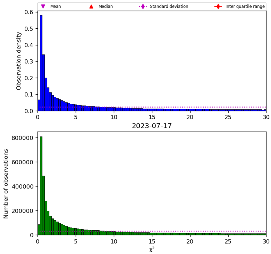
Figure 38: Histogram of “ \chi^2 ” for 2023-07-16 to 2023-07-18
