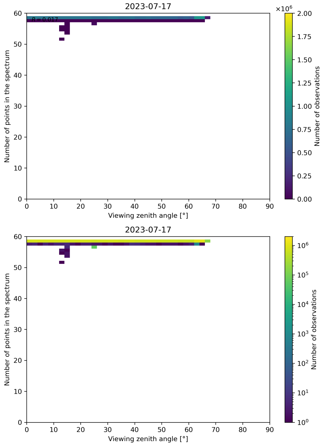
Figure 137: Scatter density plot of “Viewing zenith angle” against “Number of points in the spectrum” for 2023-07-16 to 2023-07-18.
