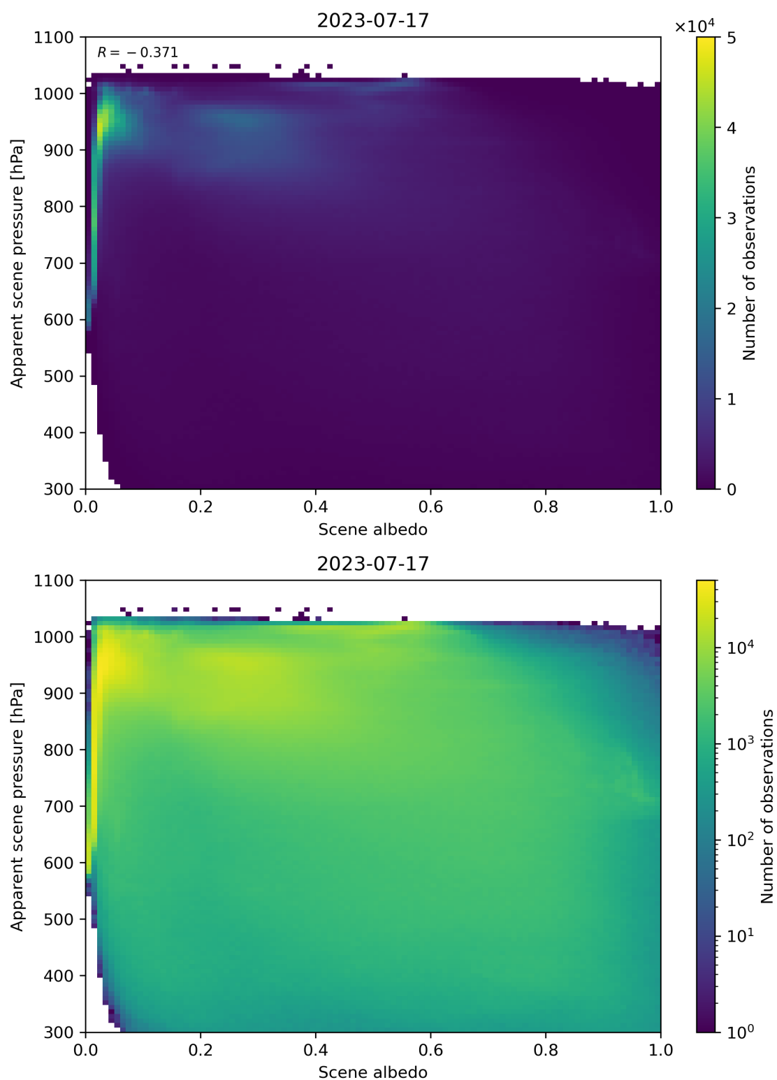
Figure 111: Scatter density plot of “Scene albedo” against “Apparent scene pressure” for 2023-07-16 to 2023-07-18.
