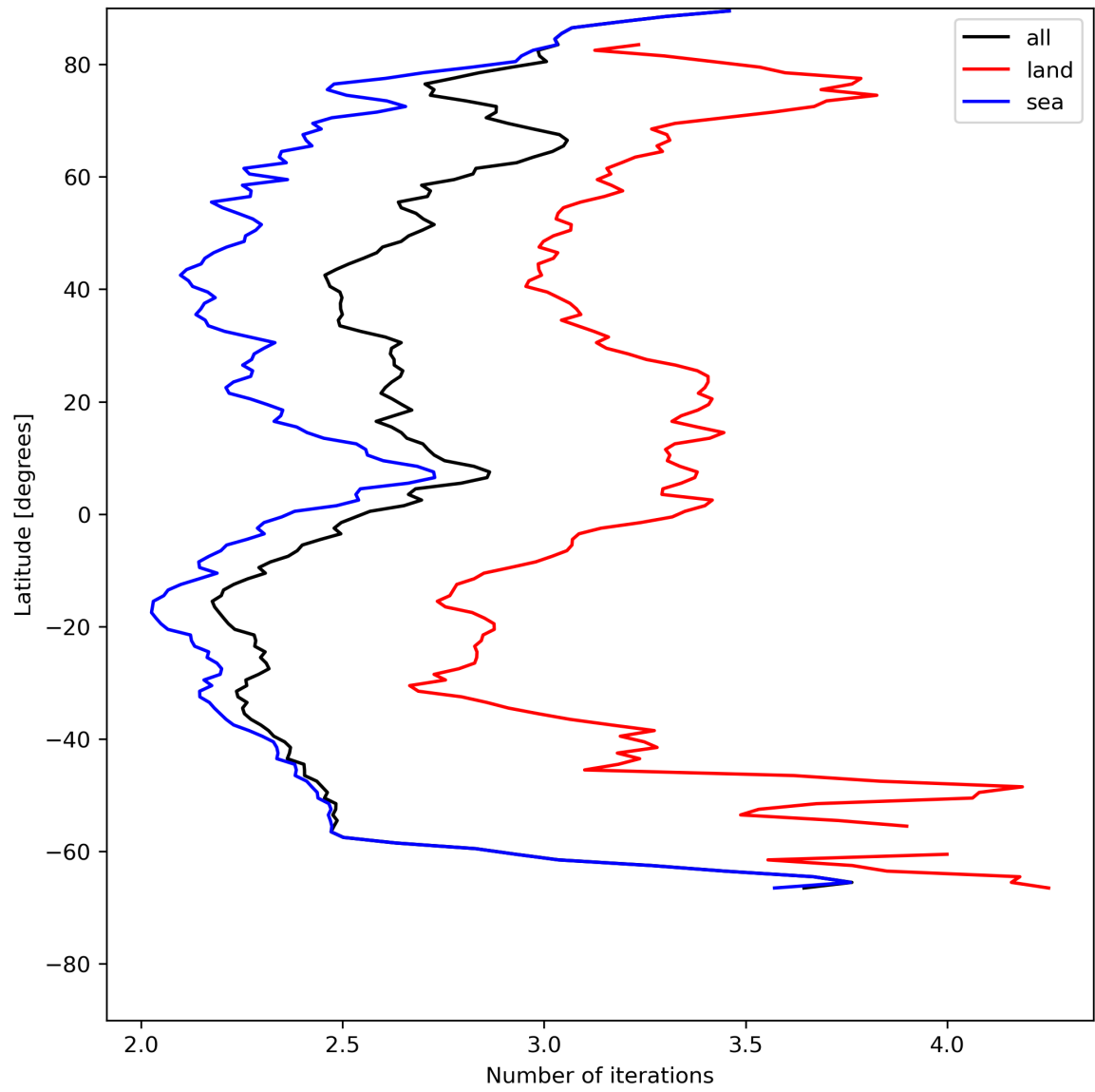
Figure 22: Zonal average of “Number of iterations” for 2023-07-16 to 2023-07-18.
