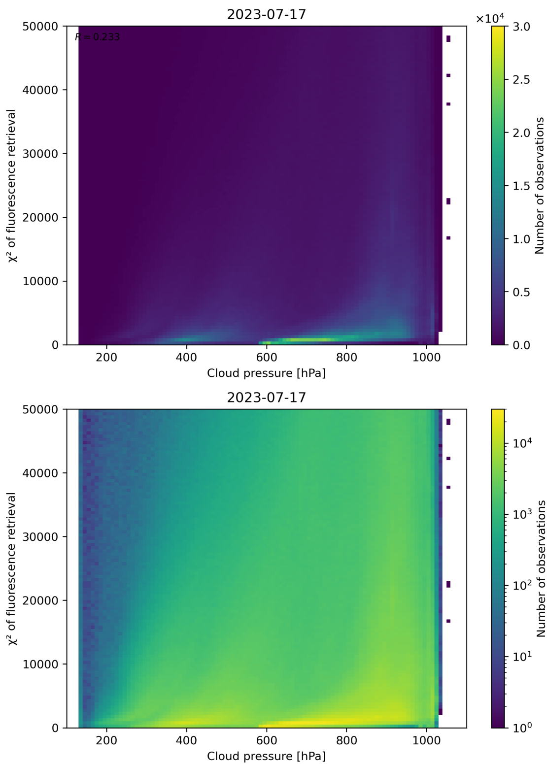
Figure 86: Scatter density plot of “Cloud pressure” against “ \chi^2 of fluorescence retrieval” for 2023-07-16 to 2023-07-18.
