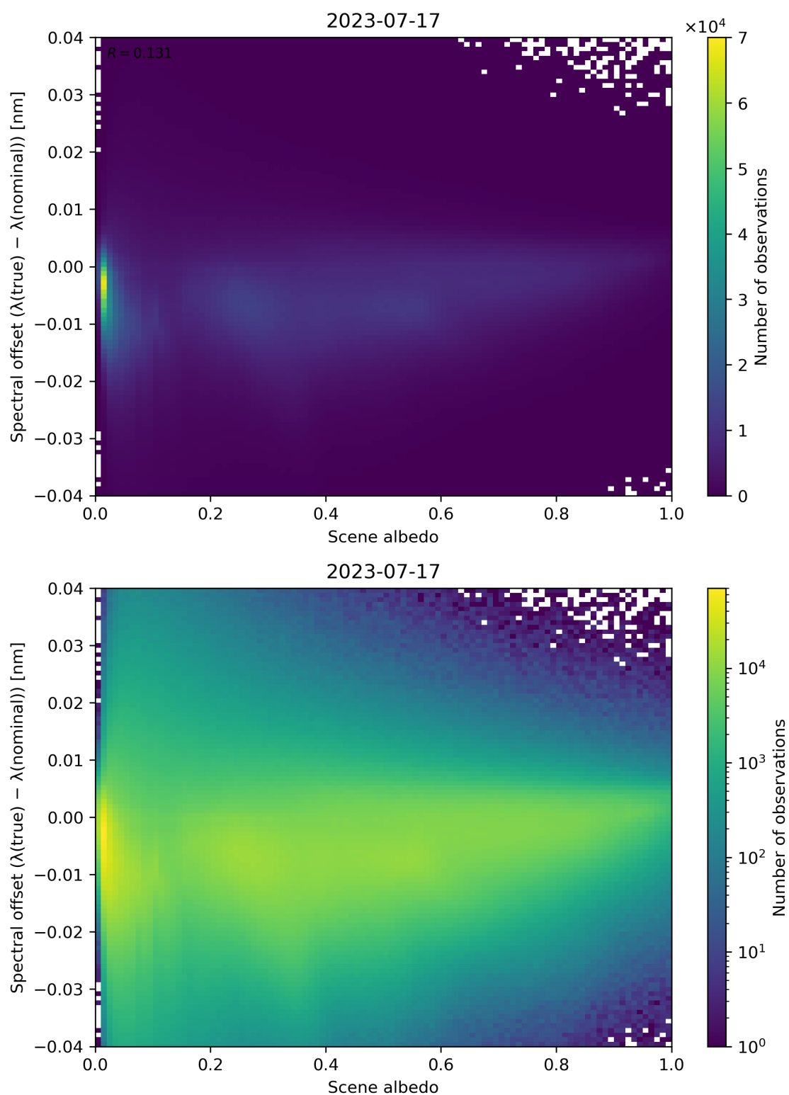
Figure 117: Scatter density plot of “Scene albedo” against “Spectral offset ( \lambda(\text{true}) - \lambda(\text{nominal}) )” for 2023-07-16 to 2023-07-18.
