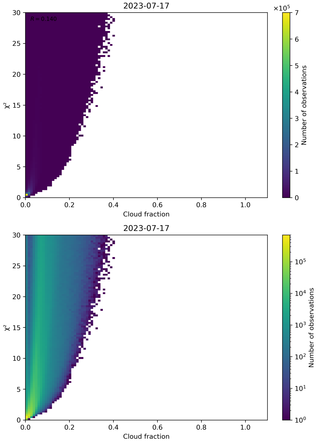
Figure 77: Scatter density plot of “Cloud fraction” against “ \chi^2 ” for 2023-07-16 to 2023-07-18.
