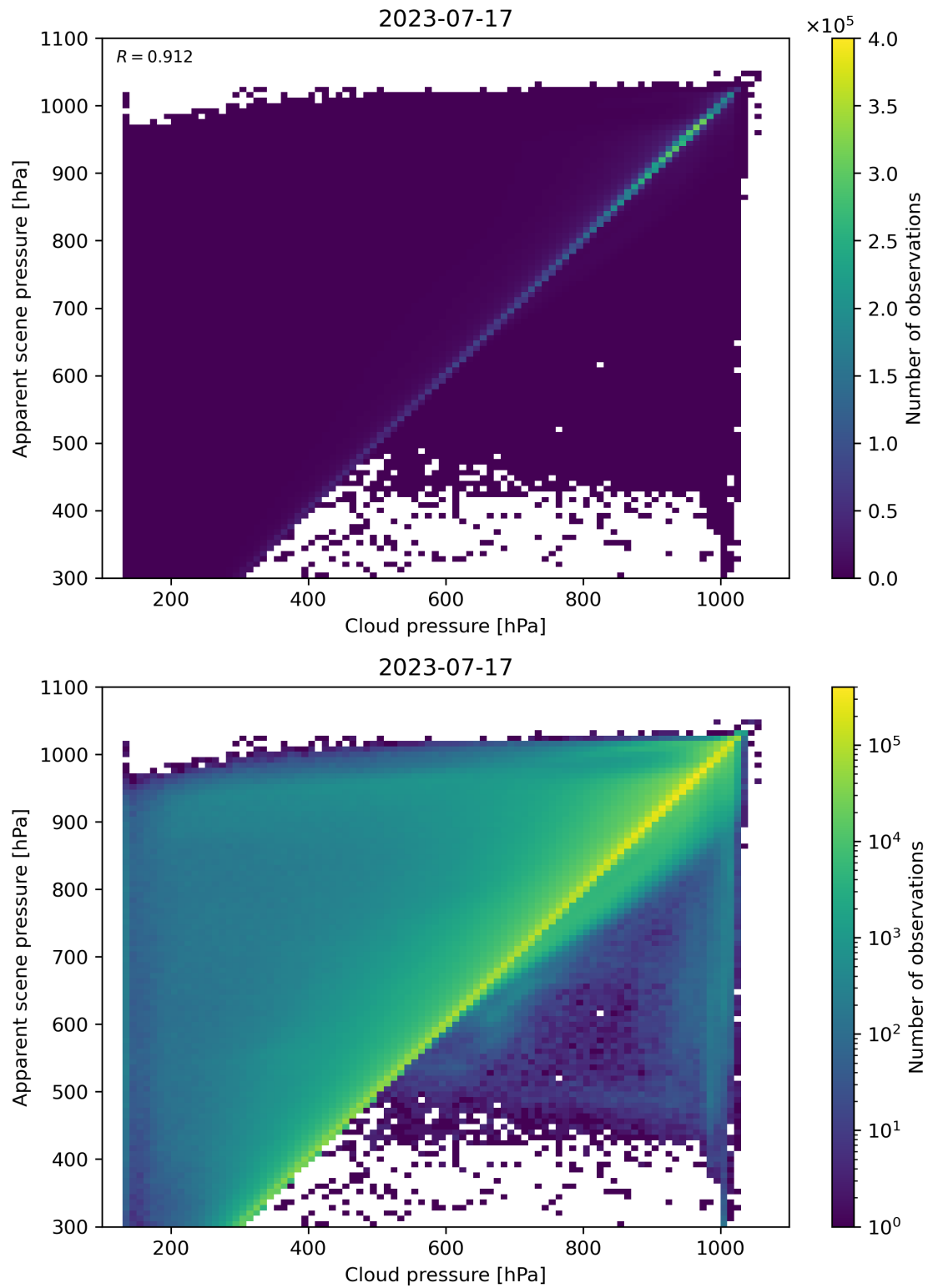
Figure 84: Scatter density plot of “Cloud pressure” against “Apparent scene pressure” for 2023-07-16 to 2023-07-18.
