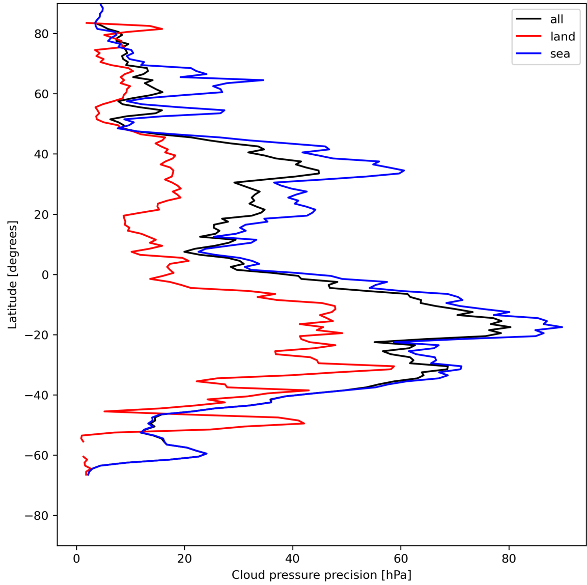
Figure 14: Zonal average of “Cloud pressure precision” for 2023-07-16 to 2023-07-18.
