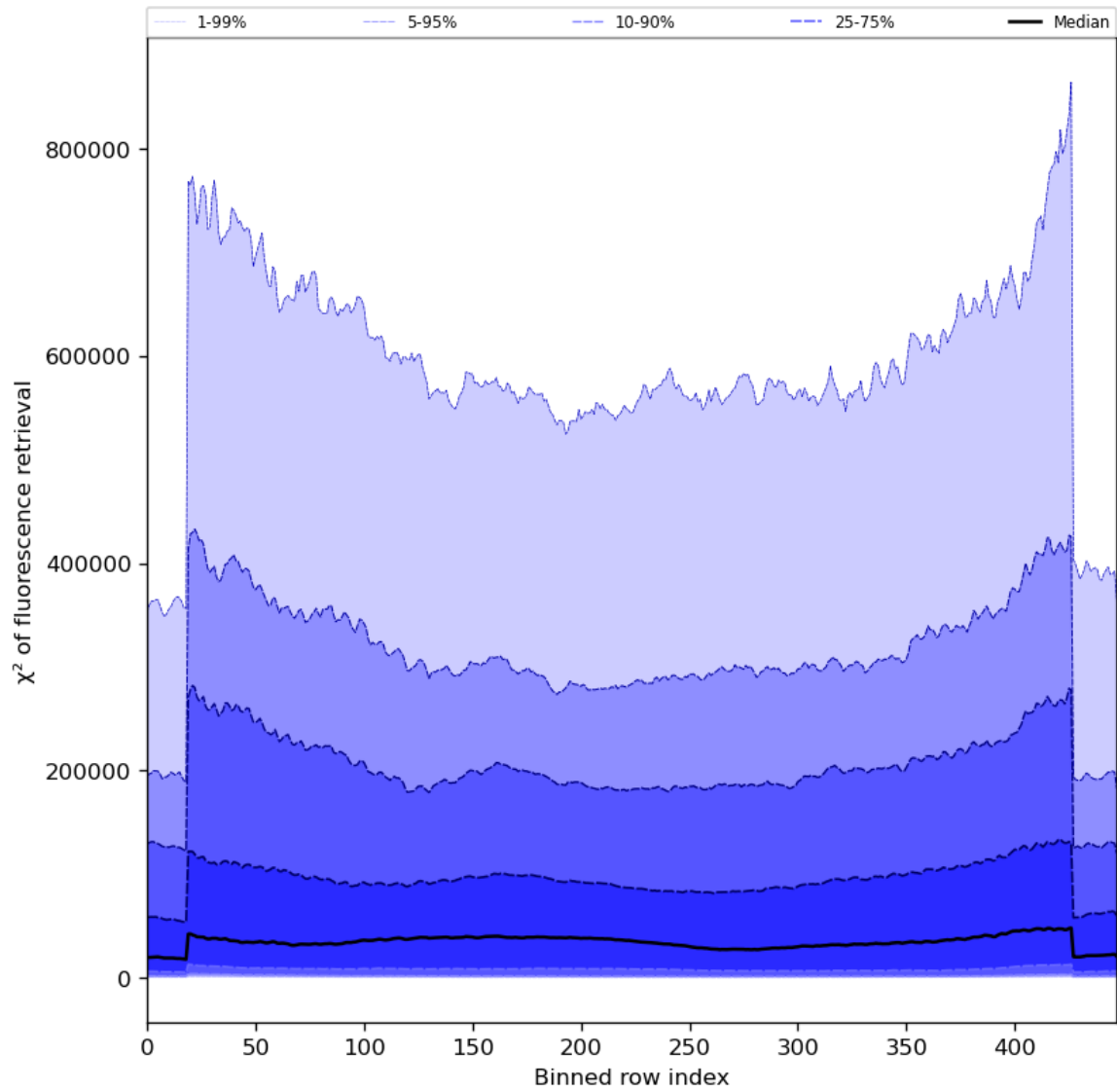
Figure 59: Along track statistics of “ \chi^2 of fluorescence retrieval” for 2023-07-16 to 2023-07-18
