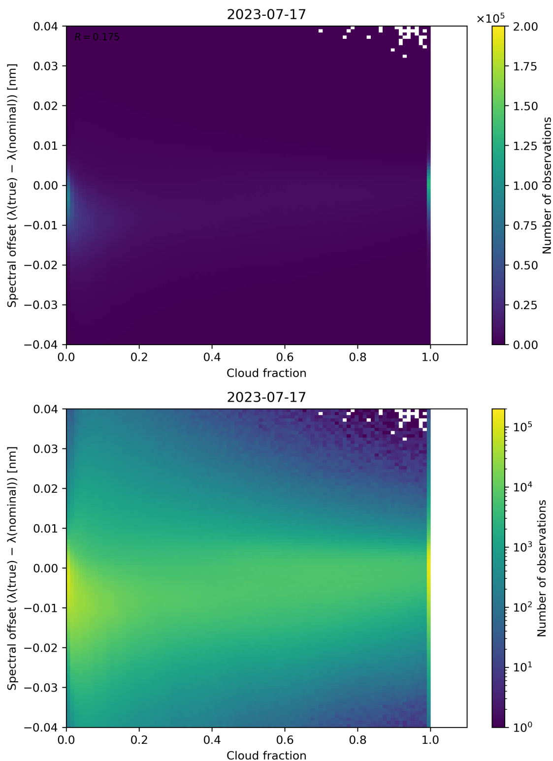
Figure 83: Scatter density plot of “Cloud fraction” against “Spectral offset ( \lambda(\text{true}) - \lambda(\text{nominal}) )” for 2023-07-16 to 2023-07-18.
