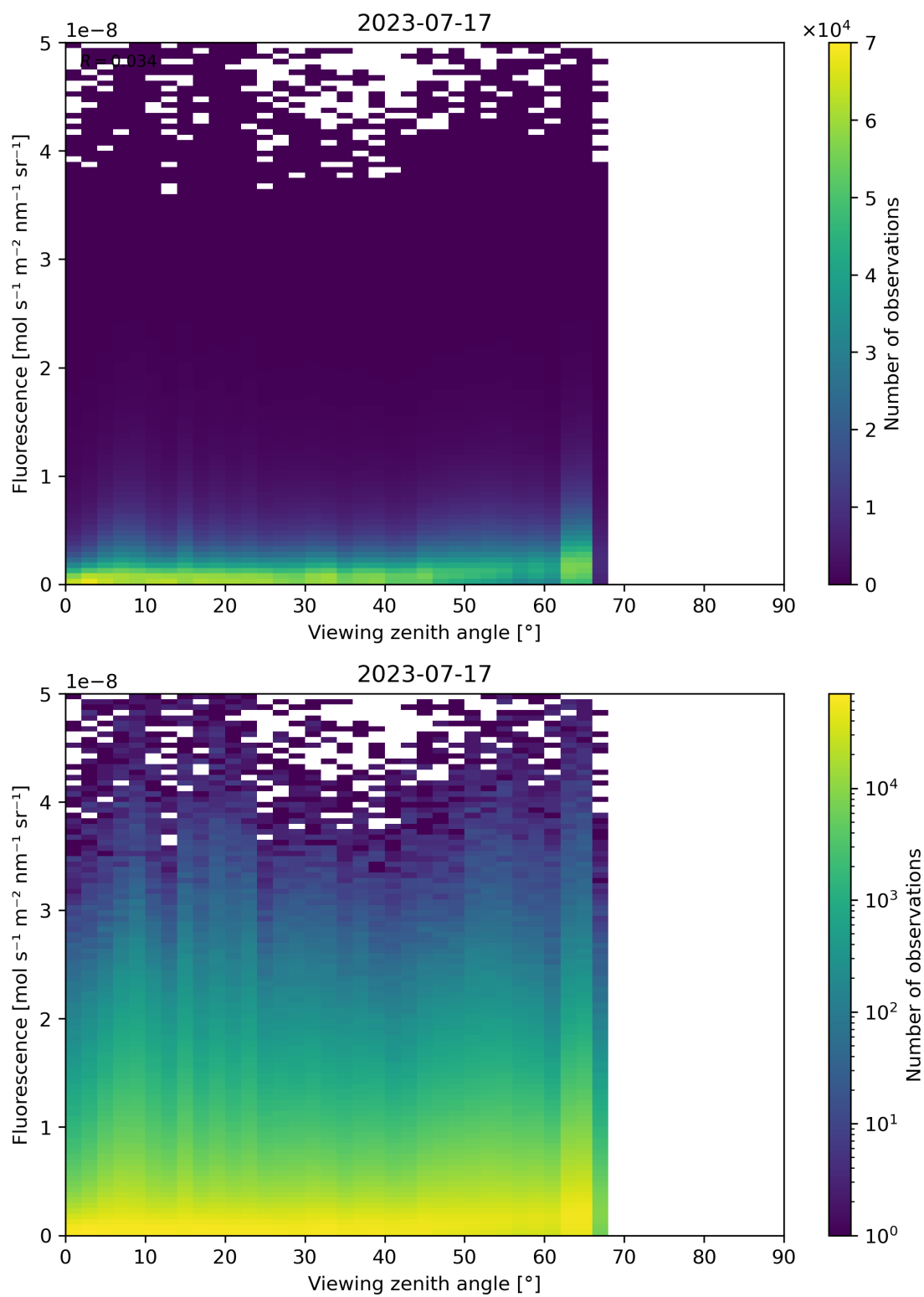
Figure 134: Scatter density plot of “Viewing zenith angle” against “Fluorescence” for 2023-07-16 to 2023-07-18.
