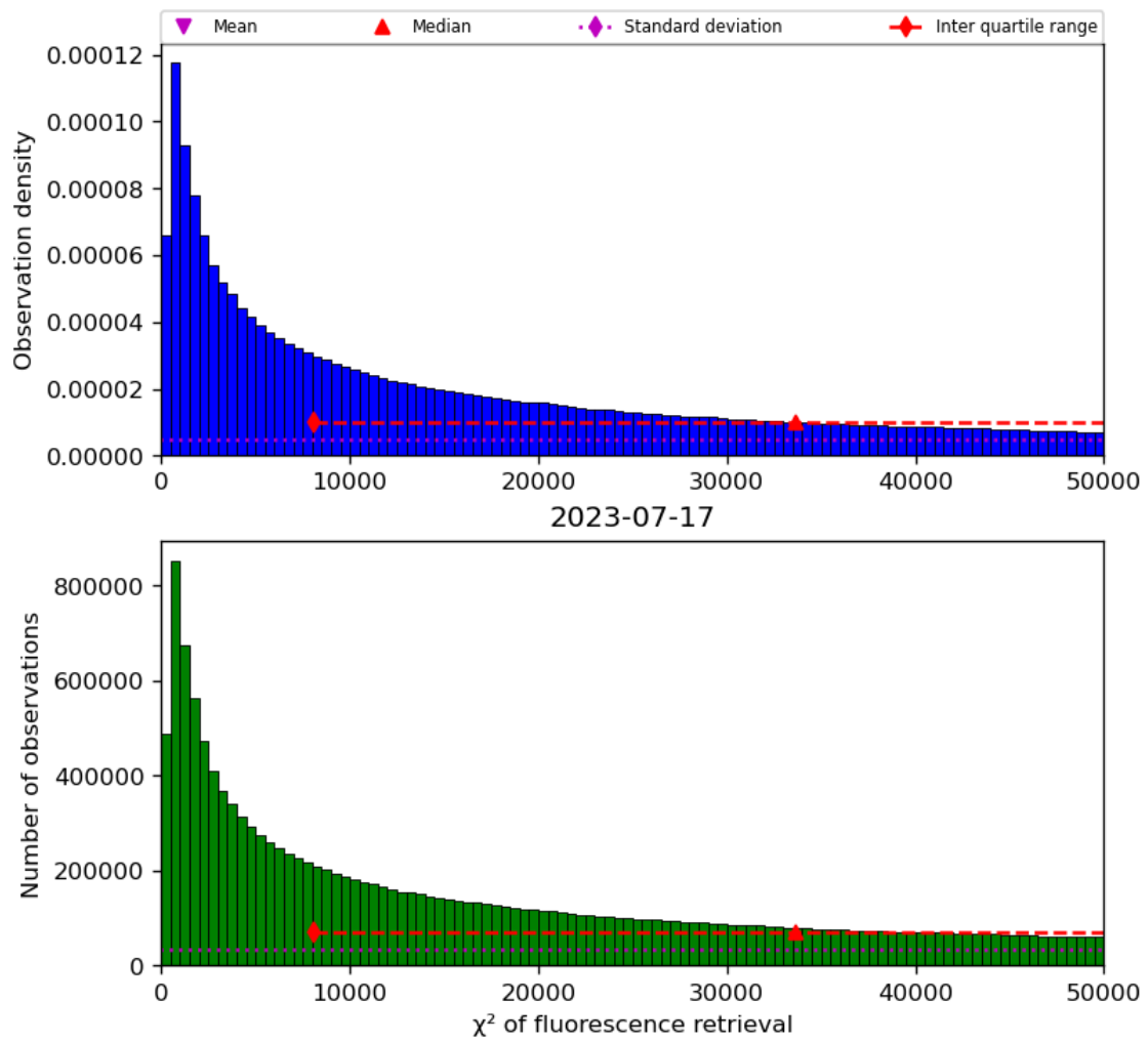
Figure 42: Histogram of “ \chi^2 of fluorescence retrieval” for 2023-07-16 to 2023-07-18
