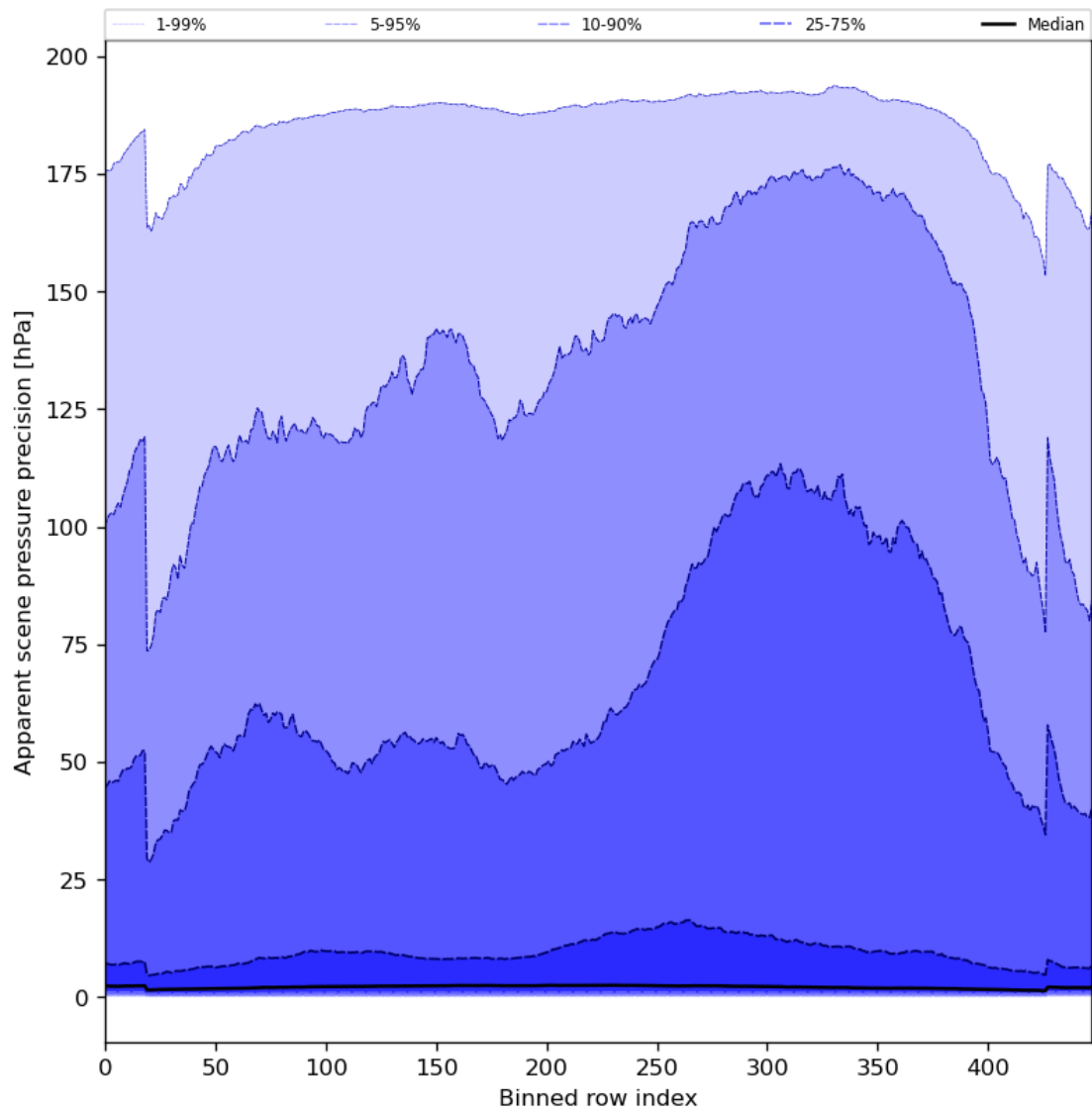
Figure 54: Along track statistics of “Apparent scene pressure precision” for 2023-07-16 to 2023-07-18
