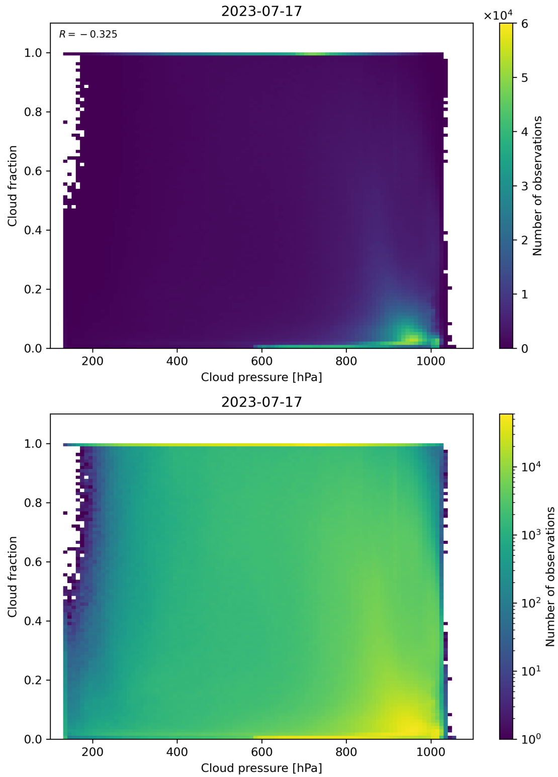
Figure 87: Scatter density plot of “Cloud pressure” against “Cloud fraction” for 2023-07-16 to 2023-07-18.
