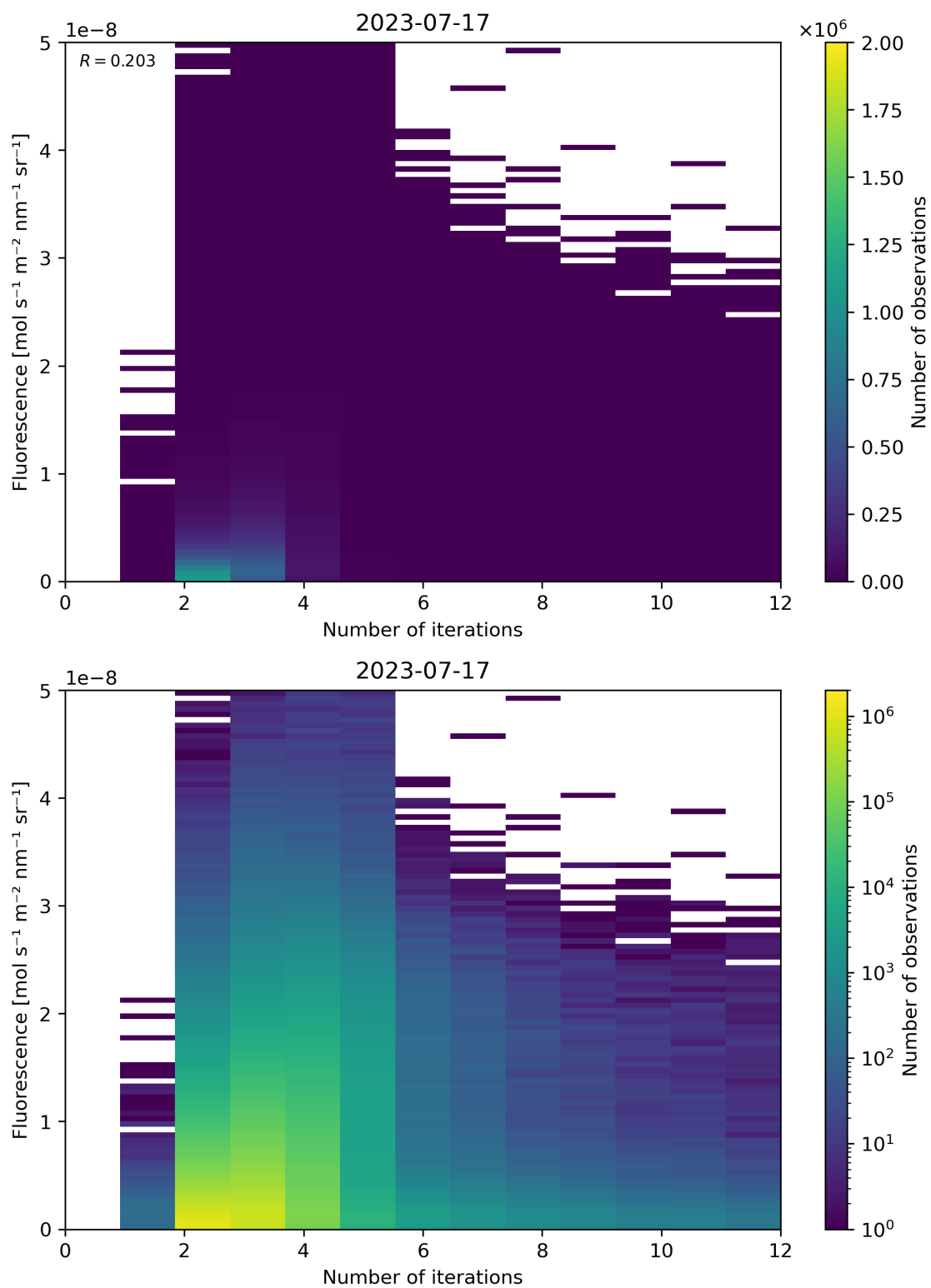
Figure 107: Scatter density plot of “Number of iterations” against “Fluorescence” for 2023-07-16 to 2023-07-18.
