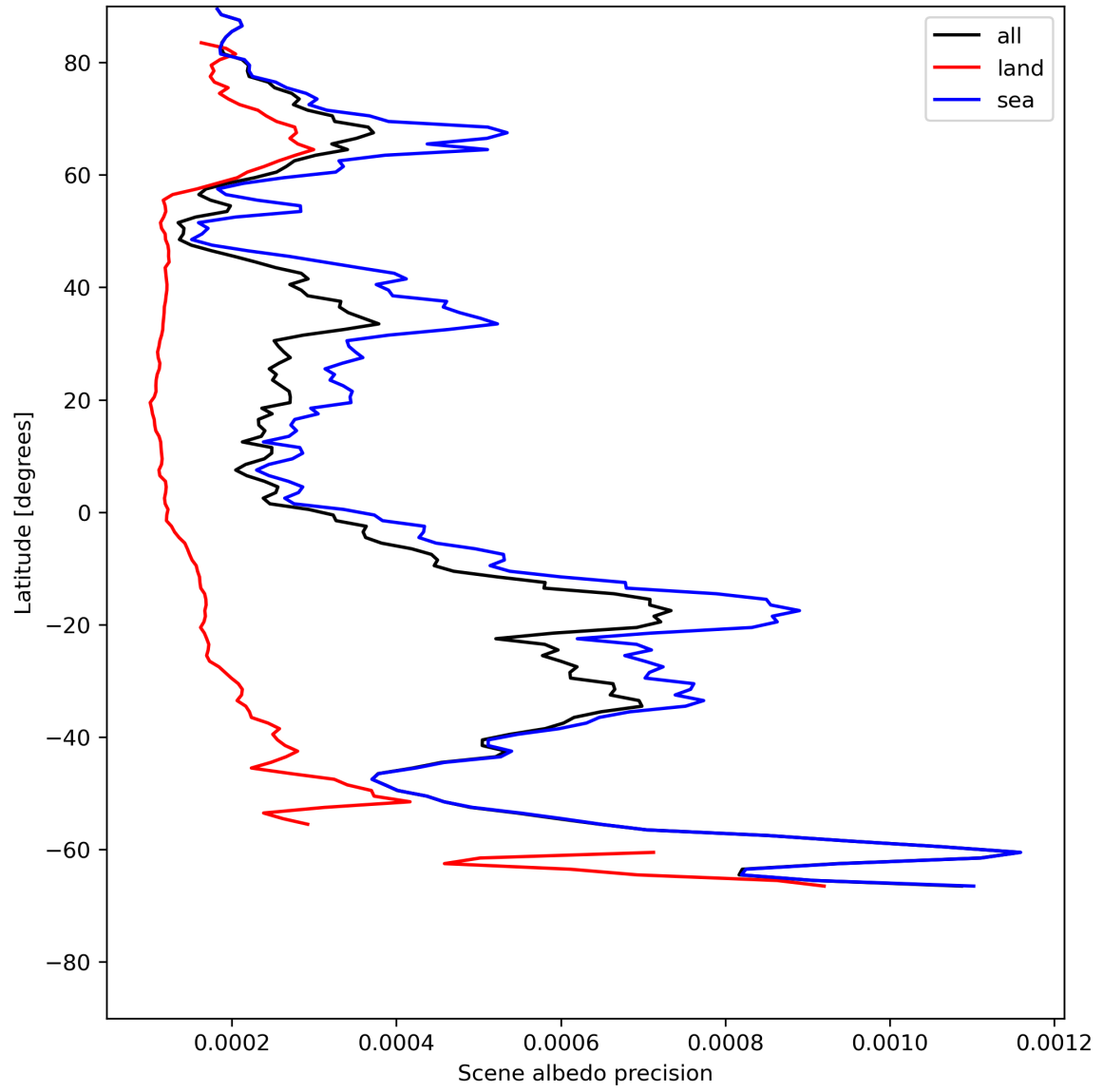
Figure 18: Zonal average of “Scene albedo precision” for 2023-07-16 to 2023-07-18.
