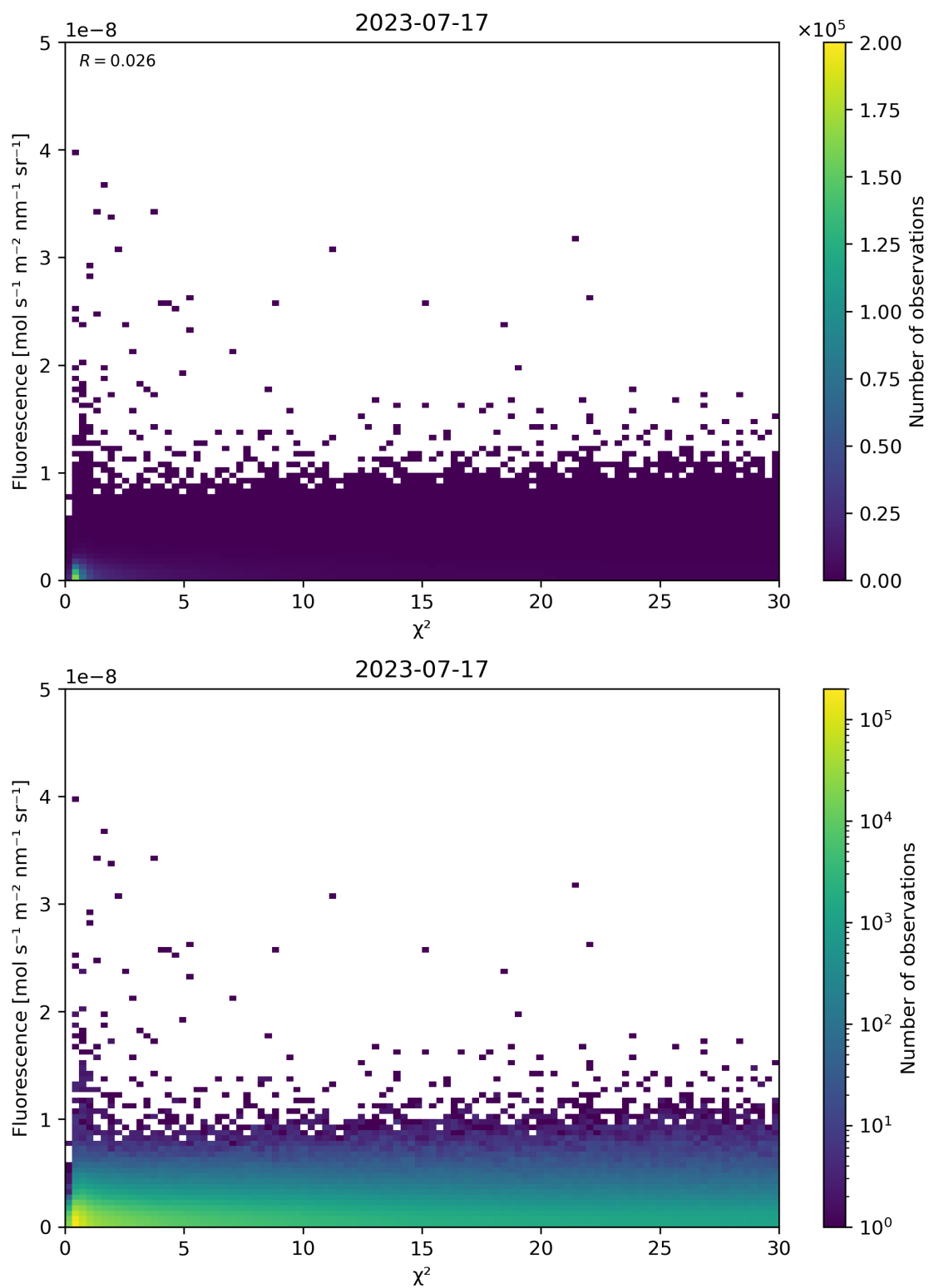
Figure 70: Scatter density plot of “ \chi^2 ” against “Fluorescence” for 2023-07-16 to 2023-07-18.
