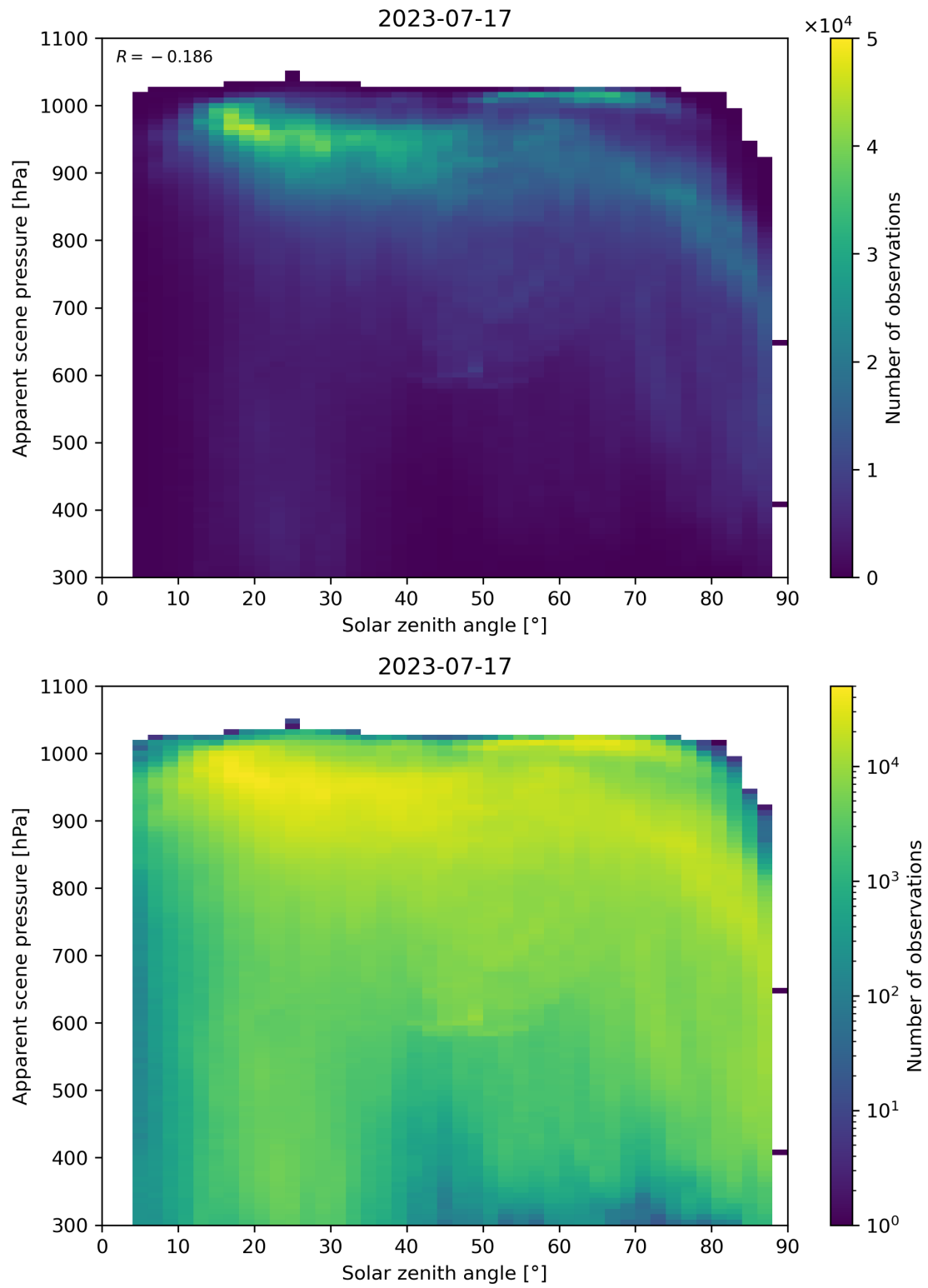
Figure 118: Scatter density plot of “Solar zenith angle” against “Apparent scene pressure” for 2023-07-16 to 2023-07-18.
