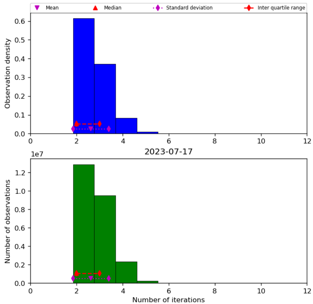
Figure 39: Histogram of “Number of iterations” for 2023-07-16 to 2023-07-18
