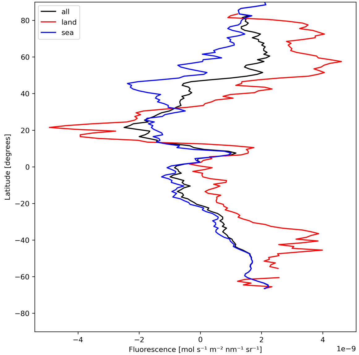
Figure 23: Zonal average of “Fluorescence” for 2023-07-16 to 2023-07-18.
