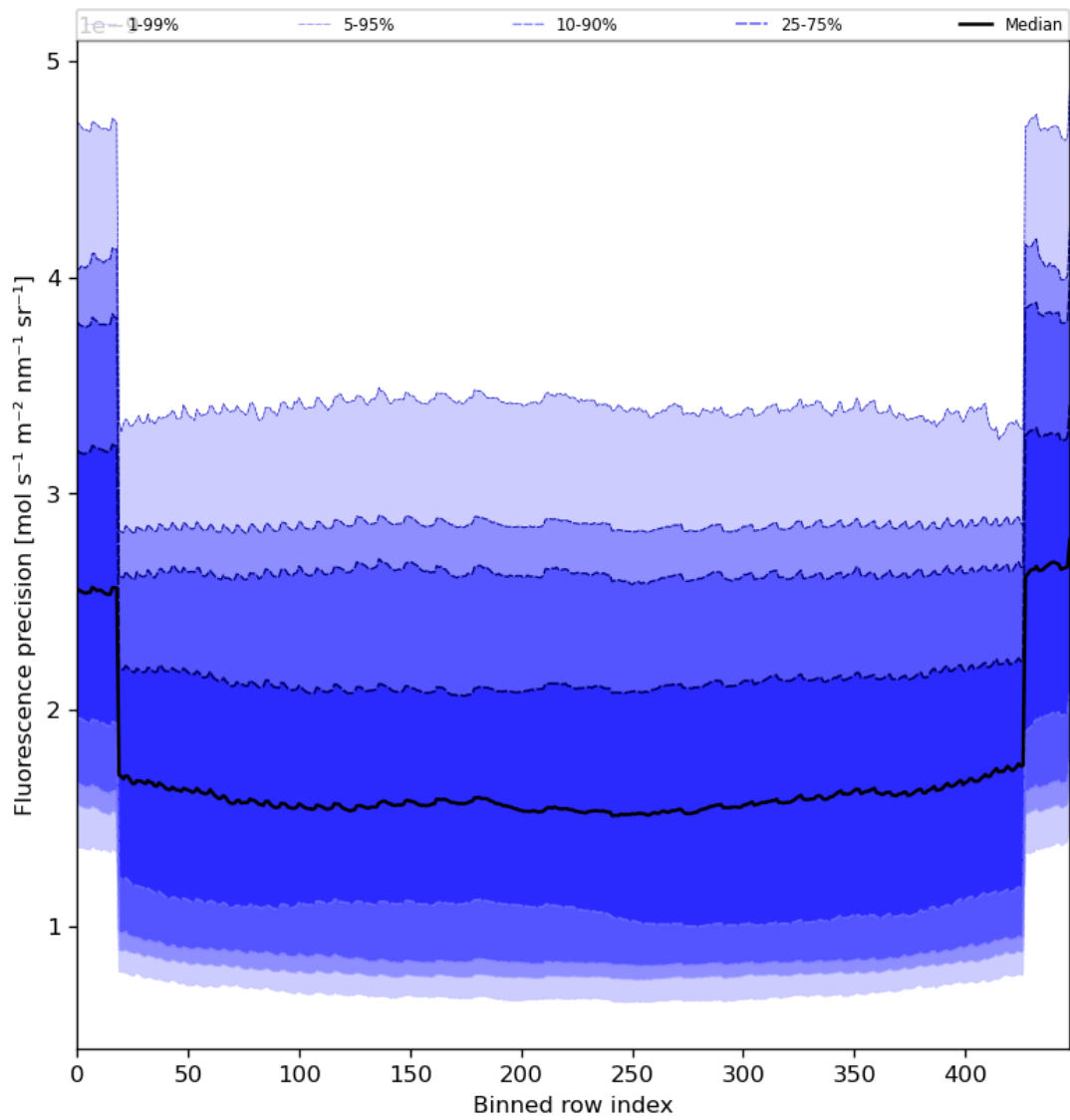
Figure 58: Along track statistics of “Fluorescence precision” for 2023-07-16 to 2023-07-18
