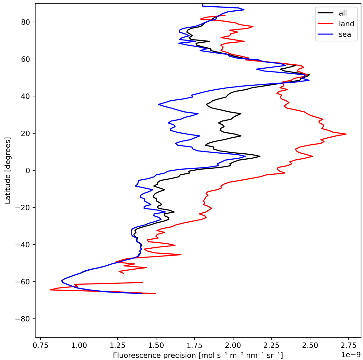
Figure 24: Zonal average of “Fluorescence precision” for 2023-07-16 to 2023-07-18.
