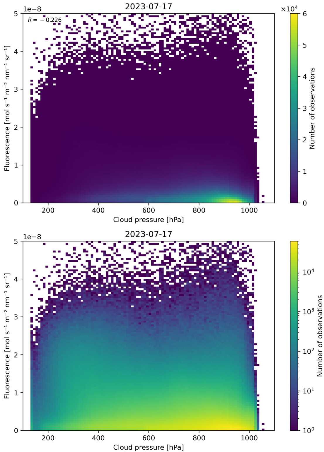
Figure 88: Scatter density plot of “Cloud pressure” against “Fluorescence” for 2023-07-16 to 2023-07-18.
