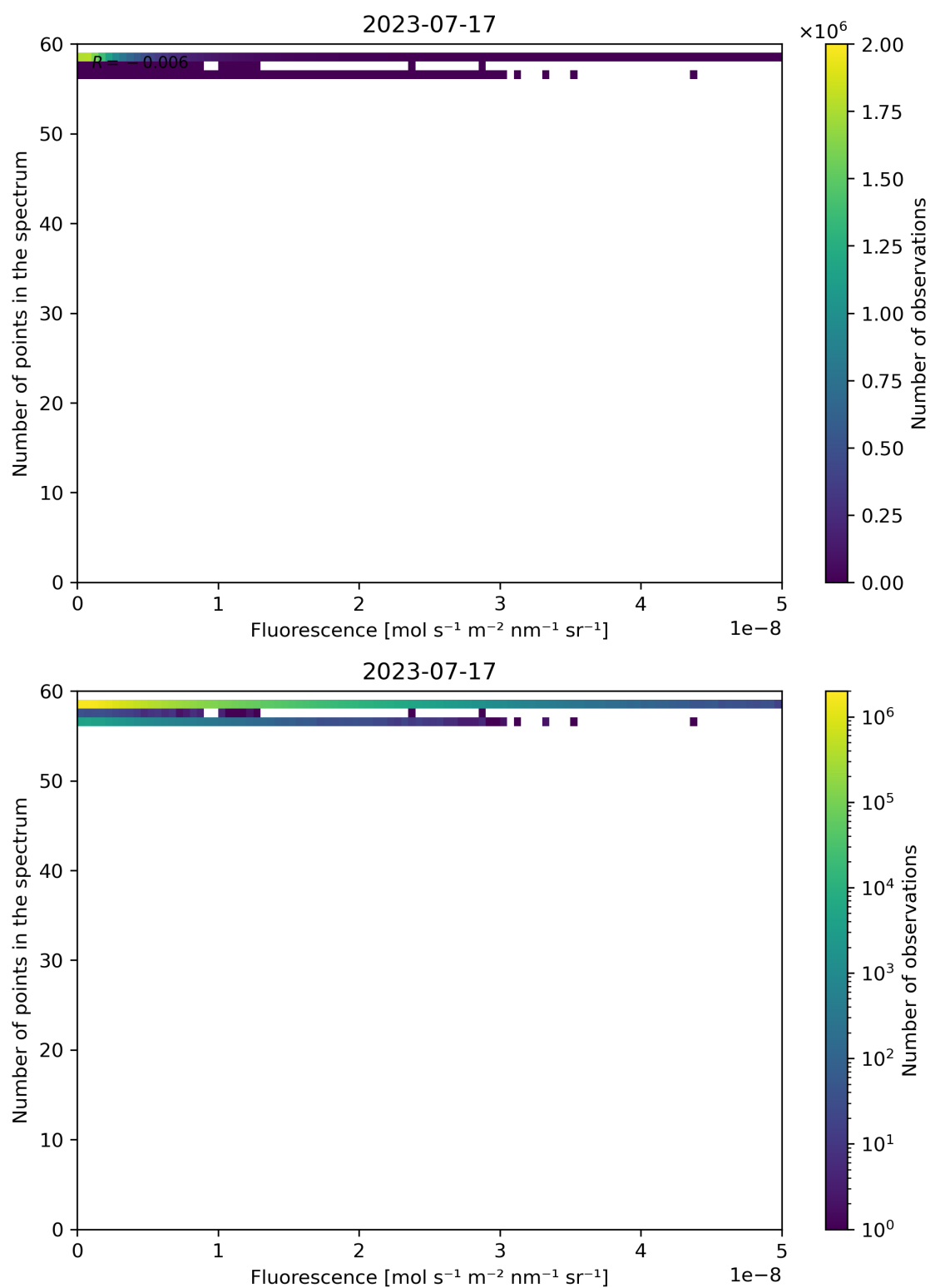
Figure 94: Scatter density plot of “Fluorescence” against “Number of points in the spectrum” for 2023-07-16 to 2023-07-18.
