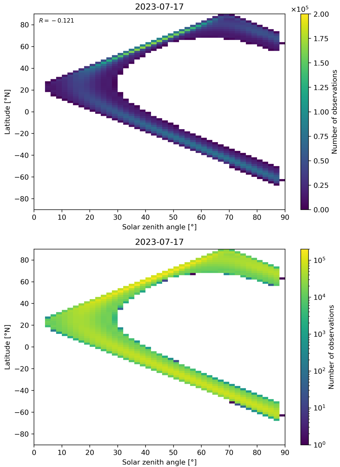
Figure 124: Scatter density plot of “Solar zenith angle” against “Latitude” for 2023-07-16 to 2023-07-18.
