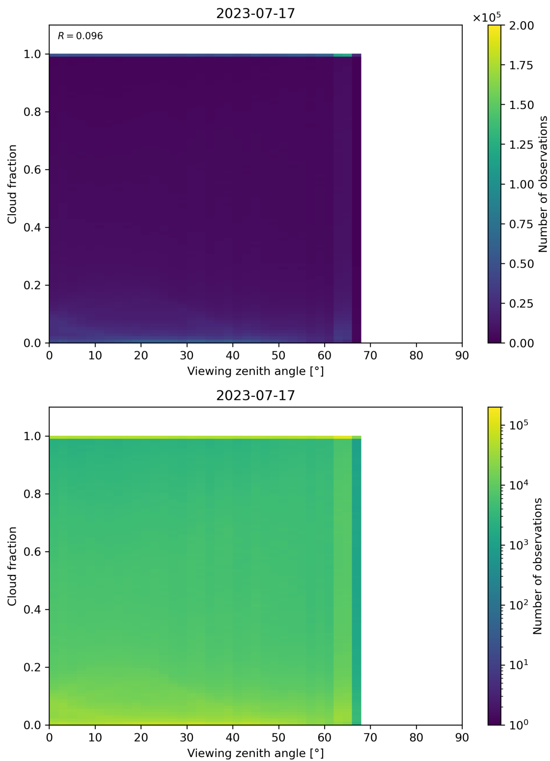
Figure 132: Scatter density plot of “Viewing zenith angle” against “Cloud fraction” for 2023-07-16 to 2023-07-18.
