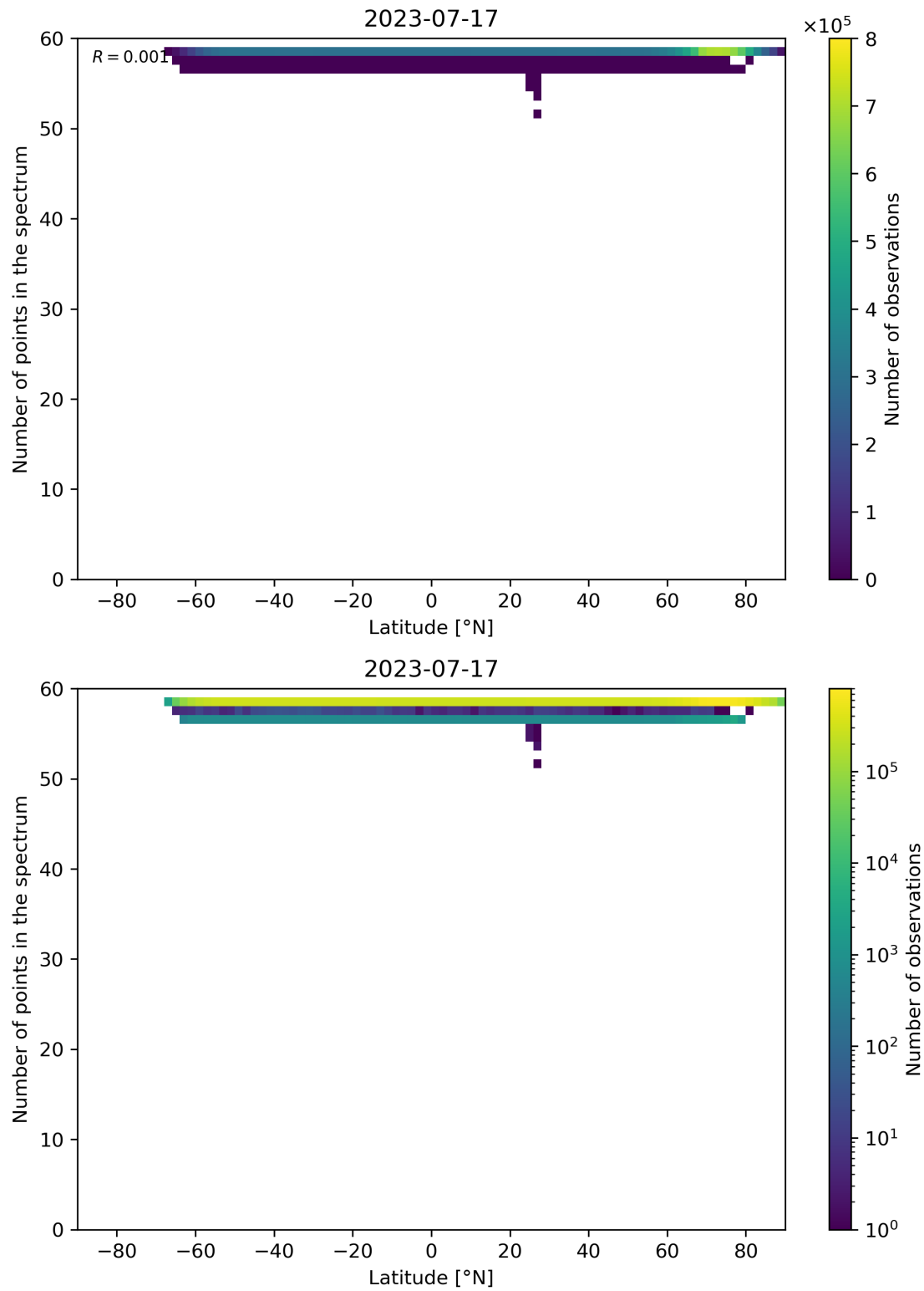
Figure 103: Scatter density plot of “Latitude” against “Number of points in the spectrum” for 2023-07-16 to 2023-07-18.
