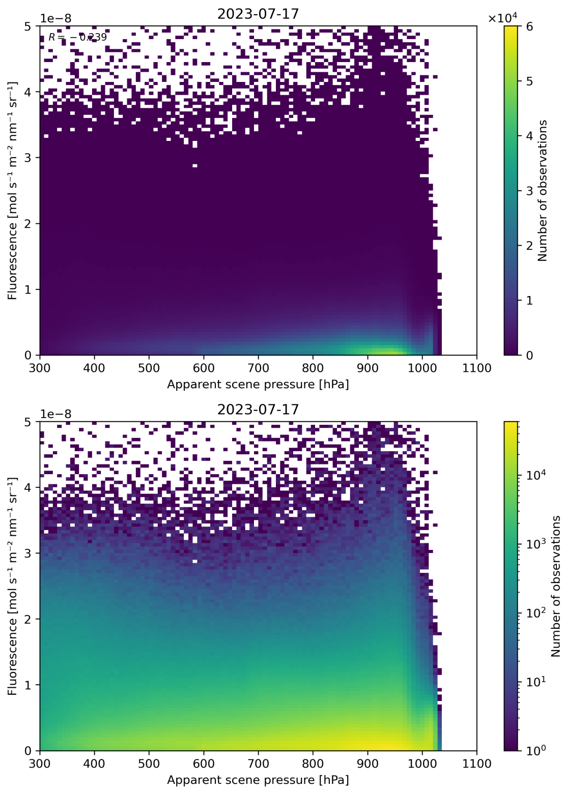
Figure 65: Scatter density plot of “Apparent scene pressure” against “Fluorescence” for 2023-07-16 to 2023-07-18.
