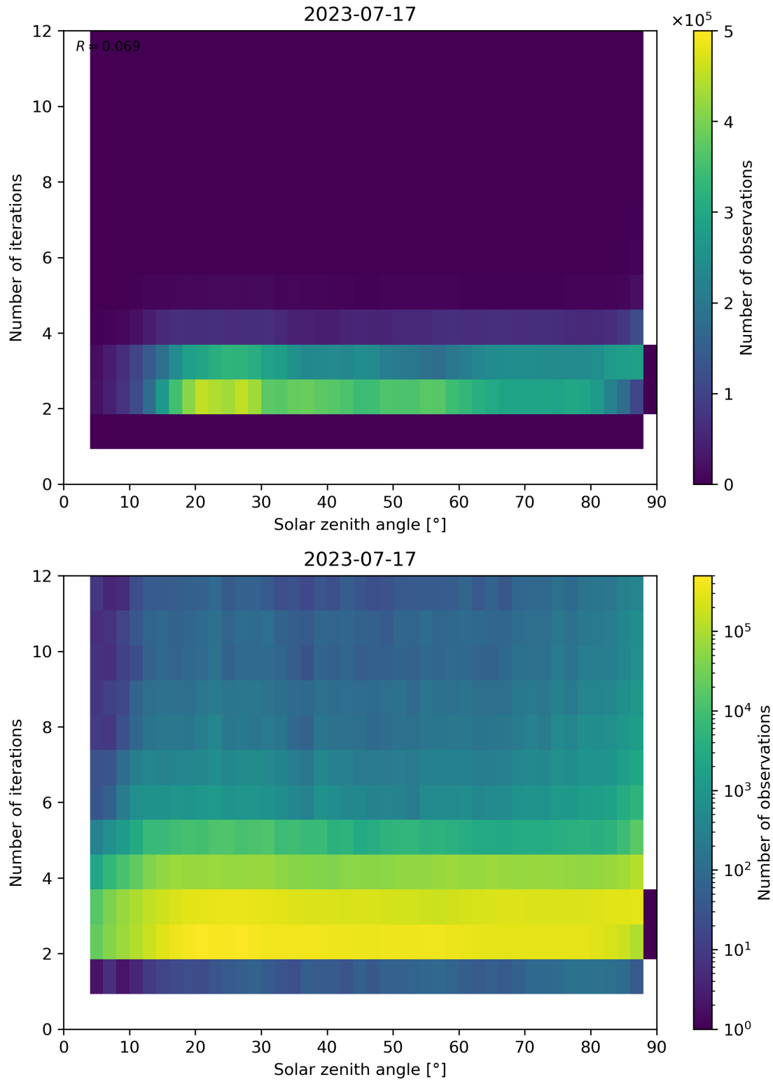
Figure 125: Scatter density plot of “Solar zenith angle” against “Number of iterations” for 2023-07-16 to 2023-07-18.
