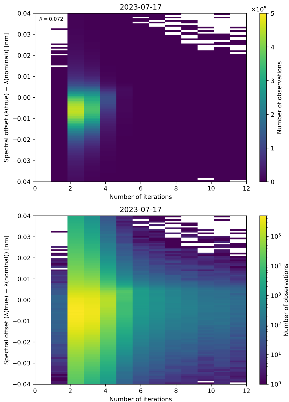
Figure 109: Scatter density plot of “Number of iterations” against “Spectral offset ( \lambda(\text{true}) - \lambda(\text{nominal}) )” for 2023-07-16 to 2023-07-18.
