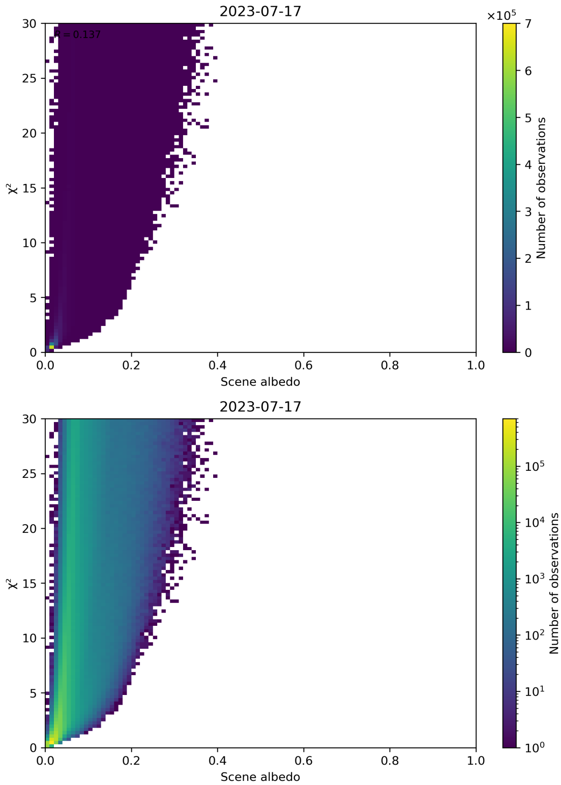
Figure 112: Scatter density plot of “Scene albedo” against “ \chi^2 ” for 2023-07-16 to 2023-07-18.
