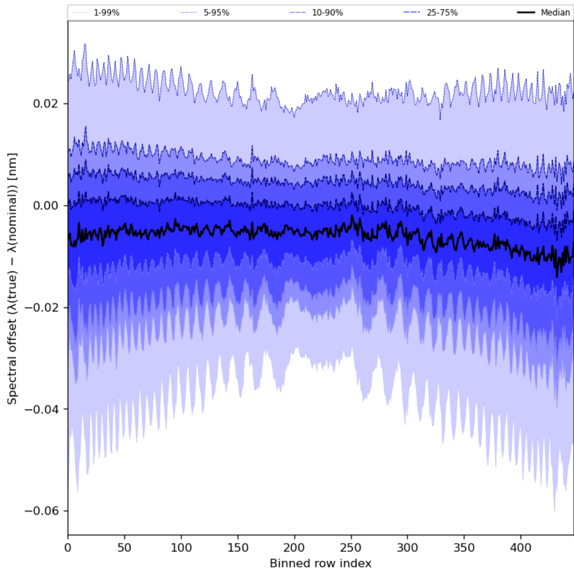
Figure 62: Along track statistics of “Spectral offset ( \lambda(\text{true}) - \lambda(\text{nominal}) )” for 2023-07-16 to 2023-07-18
