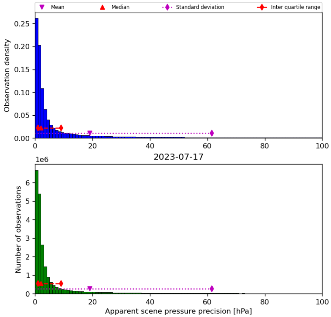
Figure 37: Histogram of “Apparent scene pressure precision” for 2023-07-16 to 2023-07-18
