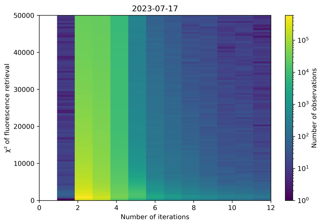
Figure 106: Scatter density plot of “Number of iterations” against “ \chi^2 of fluorescence retrieval” for 2023-07-16 to 2023-07-18.
