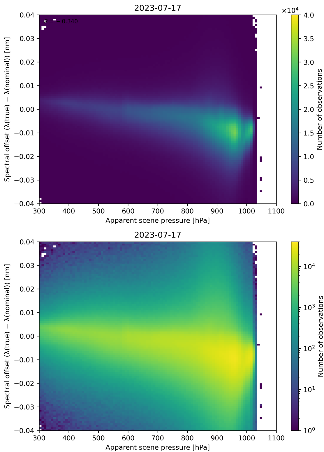
Figure 68: Scatter density plot of “Apparent scene pressure” against “Spectral offset ( \lambda(\text{true}) - \lambda(\text{nominal}) )” for 2023-07-16 to 2023-07-18.
