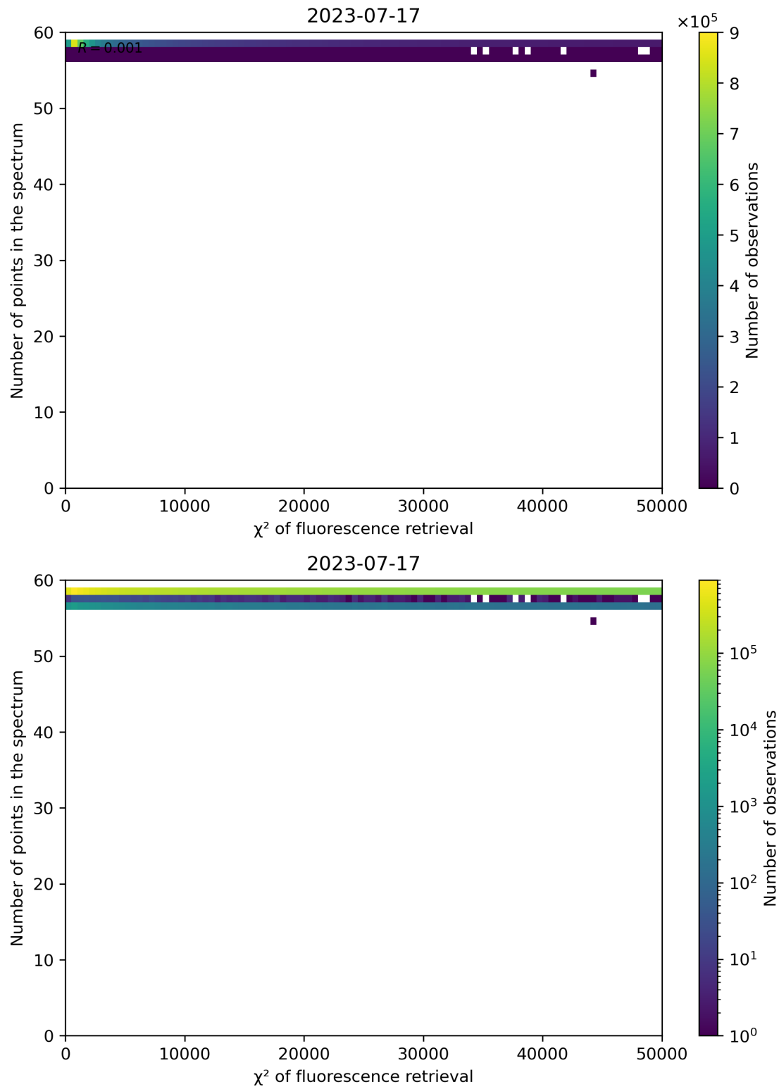
Figure 71: Scatter density plot of " \chi^2 of fluorescence retrieval" against "Number of points in the spectrum" for 2023-07-16 to 2023-07-18.
