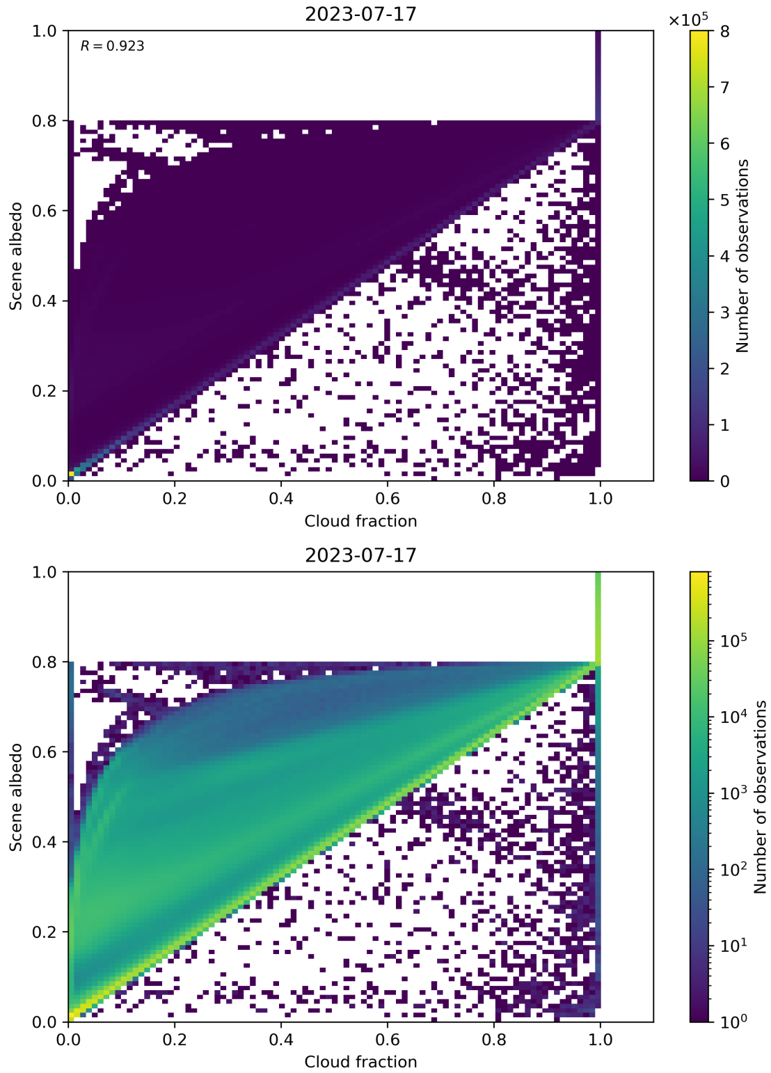
Figure 82: Scatter density plot of “Cloud fraction” against “Scene albedo” for 2023-07-16 to 2023-07-18.
