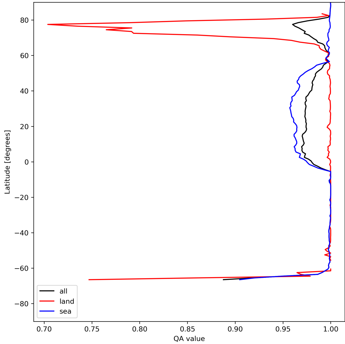
Figure 12: Zonal average of “QA value” for 2023-07-16 to 2023-07-18.
