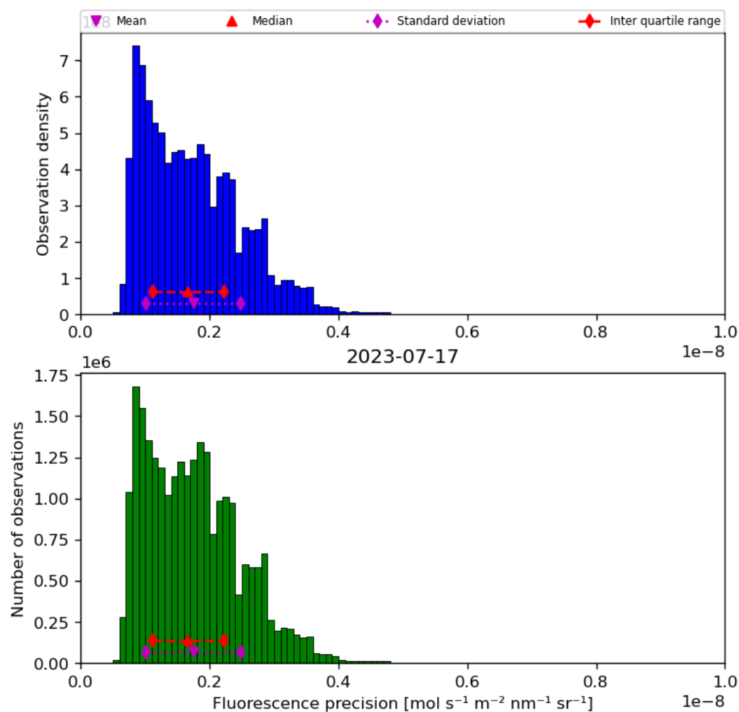
Figure 41: Histogram of “Fluorescence precision” for 2023-07-16 to 2023-07-18
