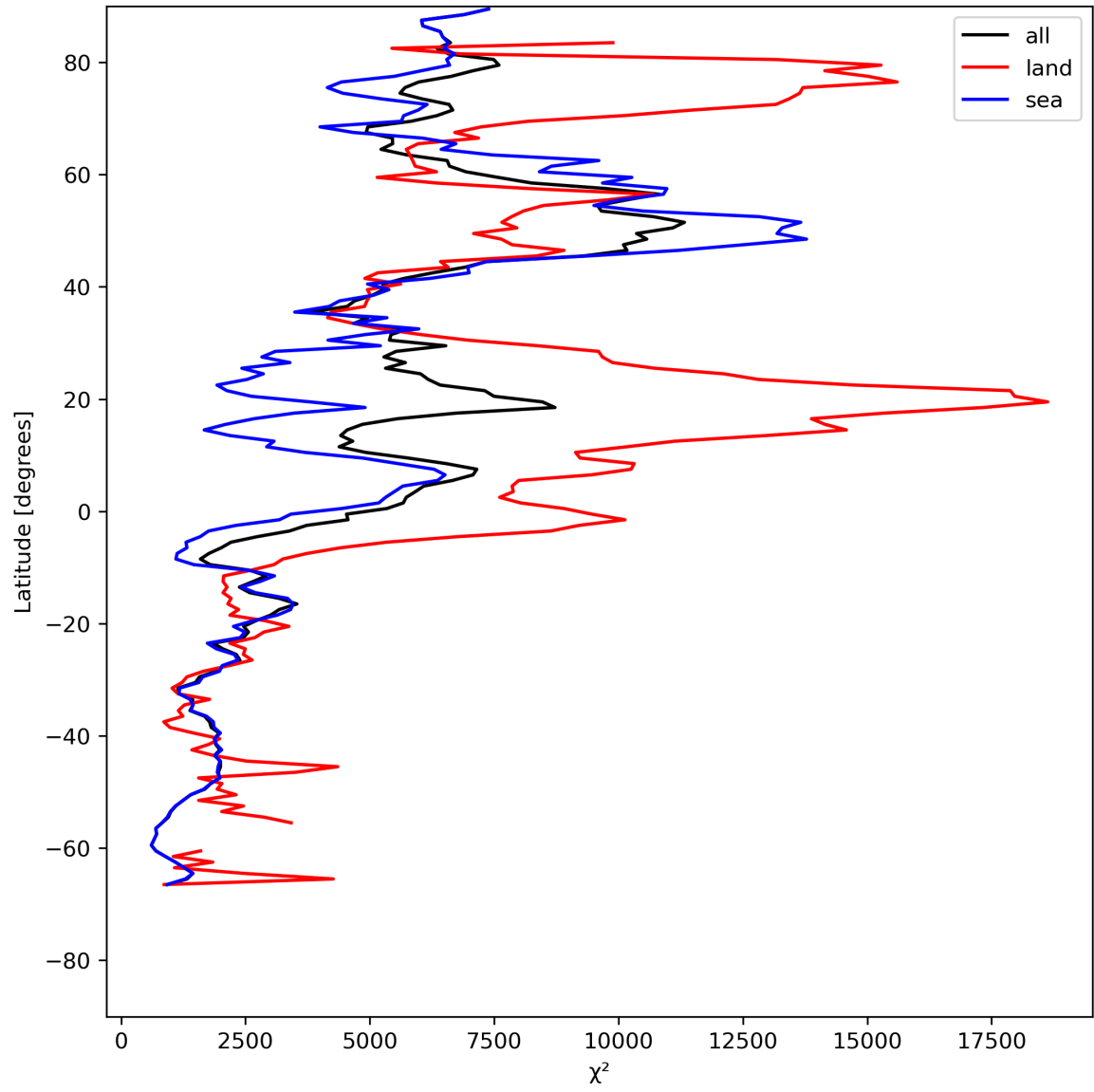
Figure 21: Zonal average of “ \chi^2 ” for 2023-07-16 to 2023-07-18.
