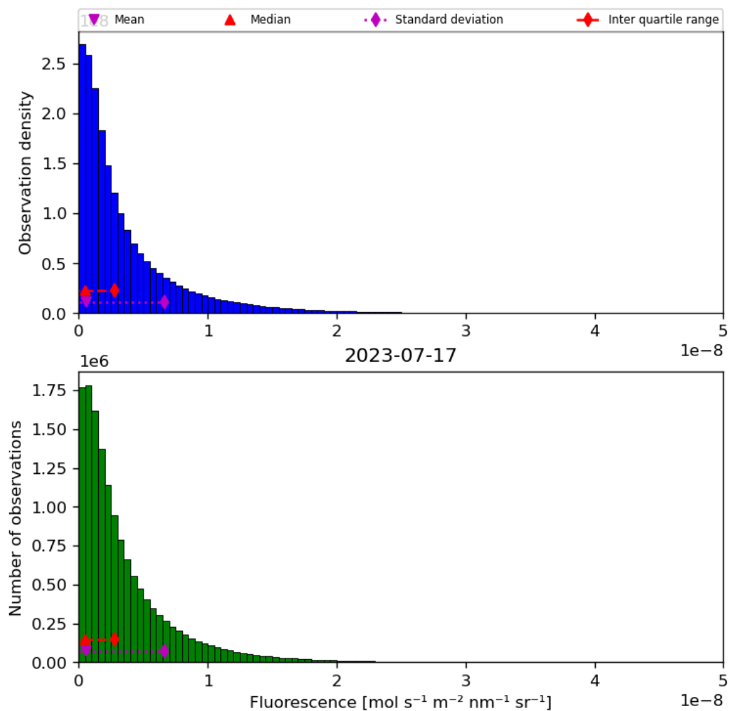
Figure 40: Histogram of “Fluorescence” for 2023-07-16 to 2023-07-18
