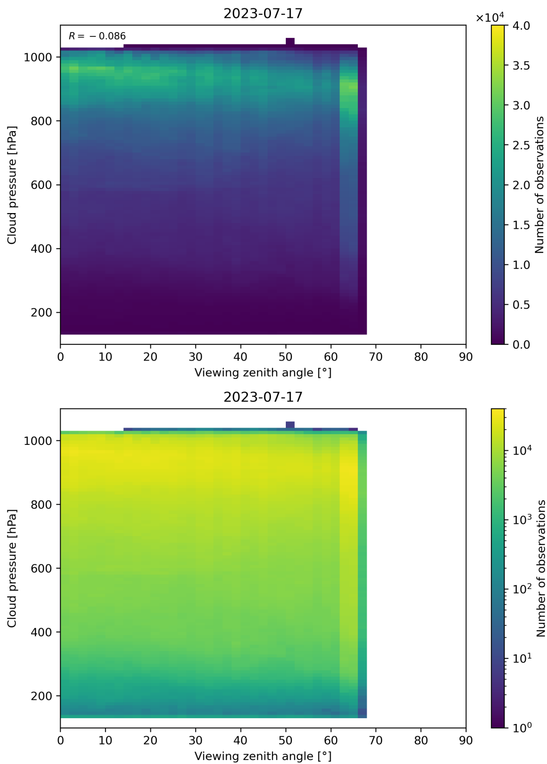
Figure 133: Scatter density plot of “Viewing zenith angle” against “Cloud pressure” for 2023-07-16 to 2023-07-18.
