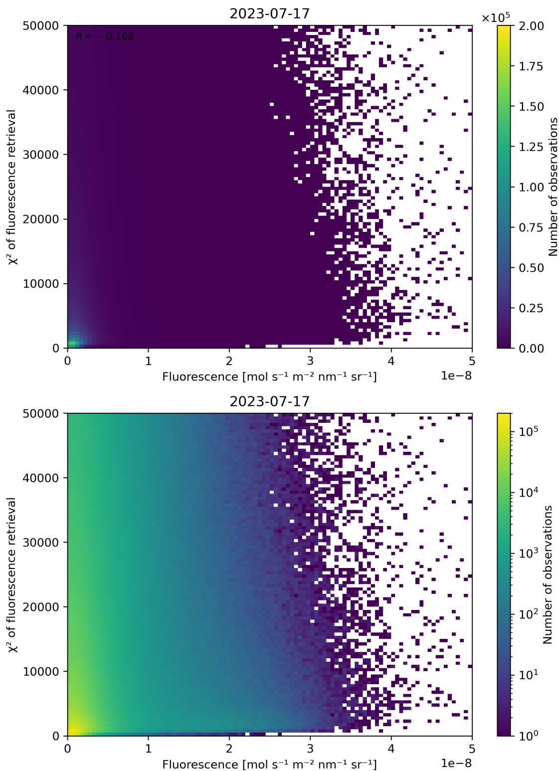
Figure 93: Scatter density plot of “Fluorescence” against “ \chi^2 of fluorescence retrieval” for 2023-07-16 to 2023-07-18.
