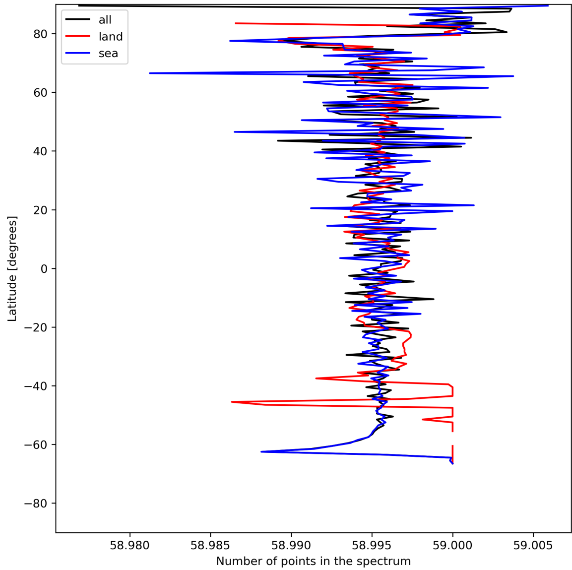
Figure 27: Zonal average of “Number of points in the spectrum” for 2023-07-16 to 2023-07-18.
