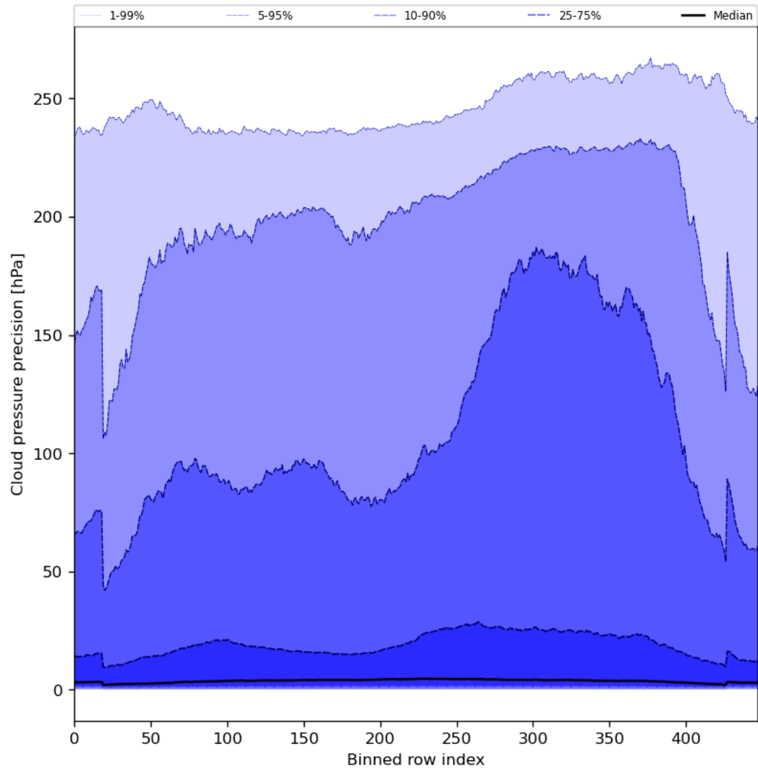
Figure 48: Along track statistics of “Cloud pressure precision” for 2023-07-16 to 2023-07-18
