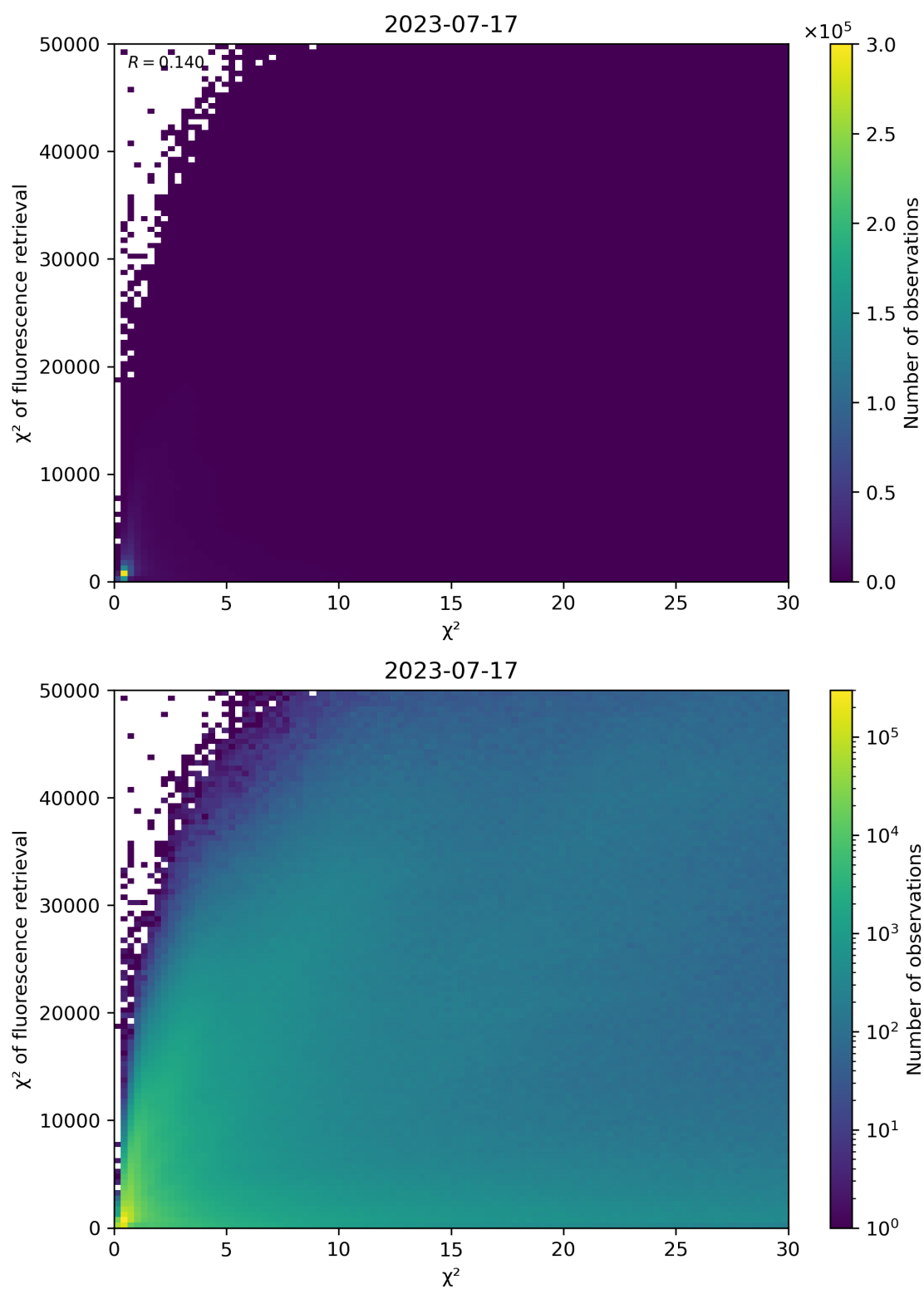
Figure 69: Scatter density plot of “ \chi^2 ” against “ \chi^2 of fluorescence retrieval” for 2023-07-16 to 2023-07-18.
