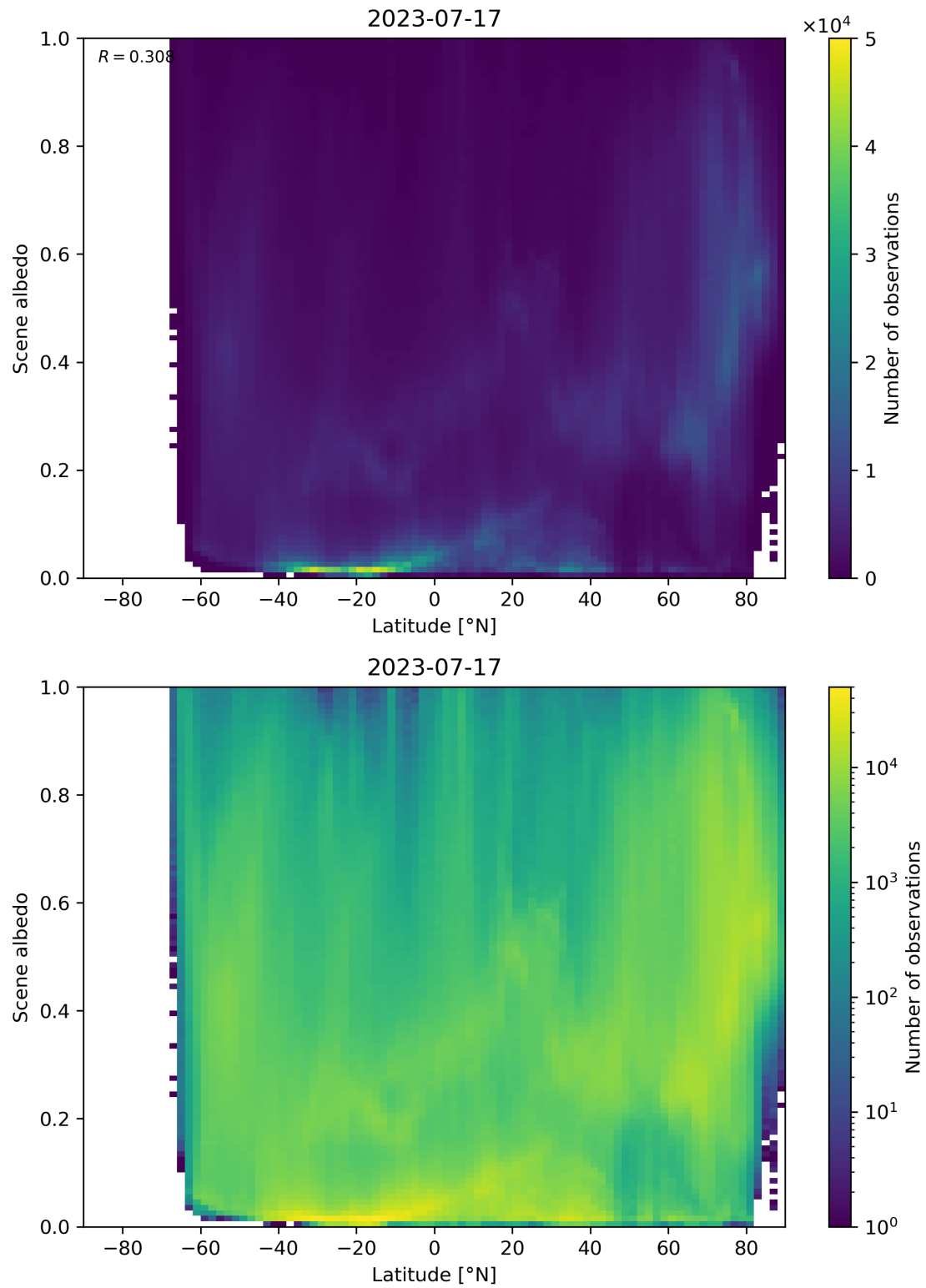
Figure 104: Scatter density plot of “Latitude” against “Scene albedo” for 2023-07-16 to 2023-07-18.
