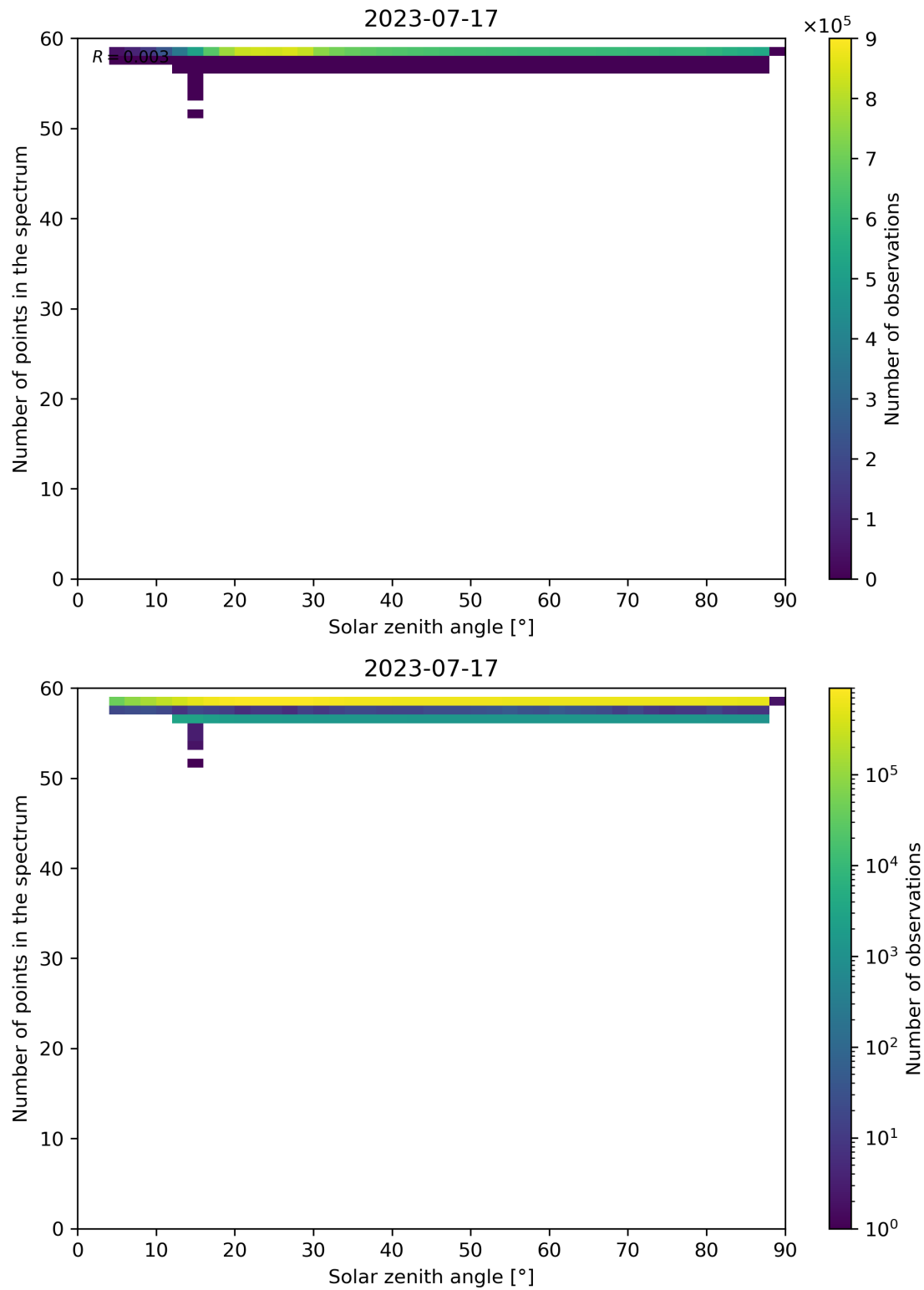
Figure 126: Scatter density plot of “Solar zenith angle” against “Number of points in the spectrum” for 2023-07-16 to 2023-07-18.
