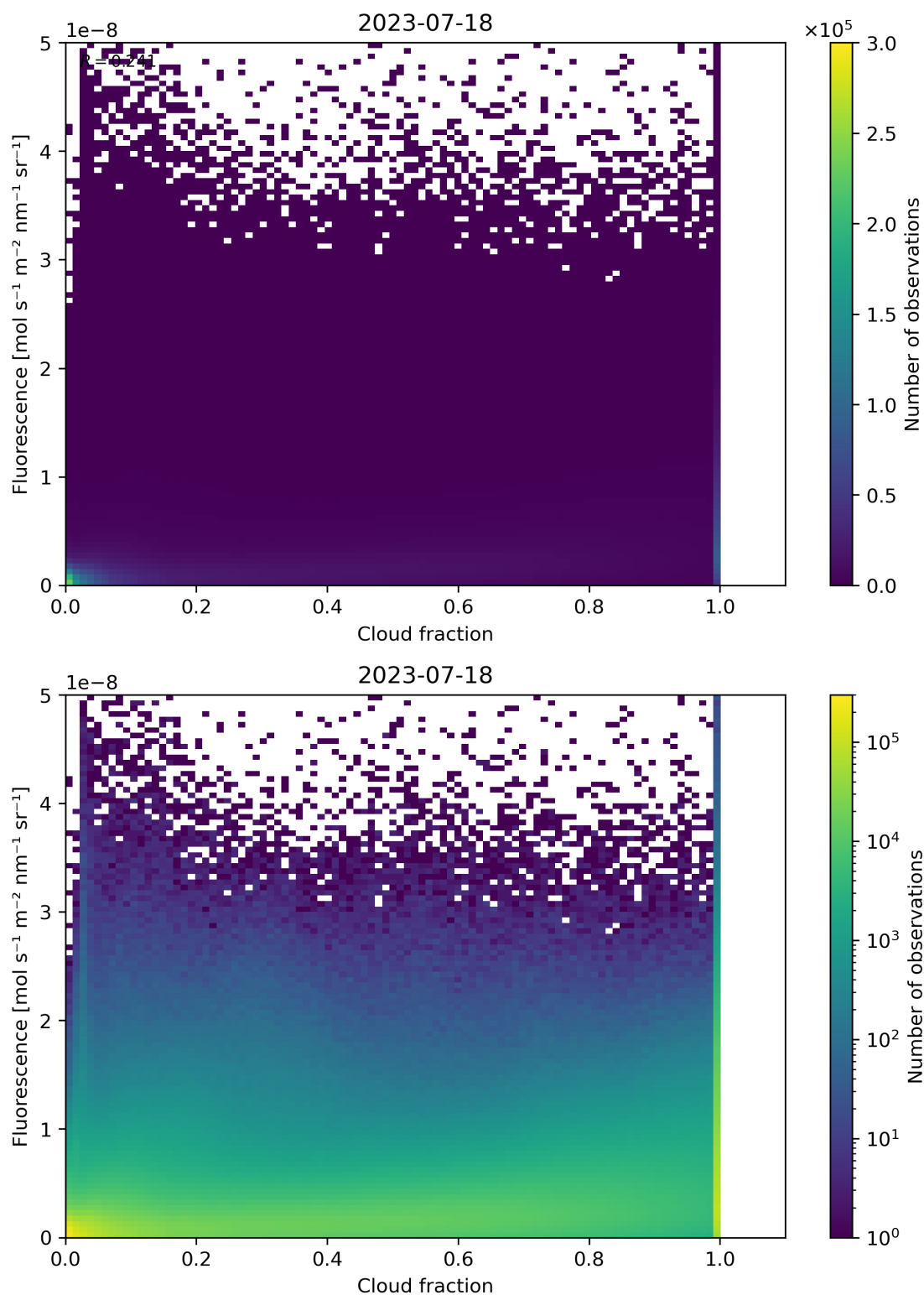
Figure 79: Scatter density plot of “Cloud fraction” against “Fluorescence” for 2023-07-17 to 2023-07-19.
