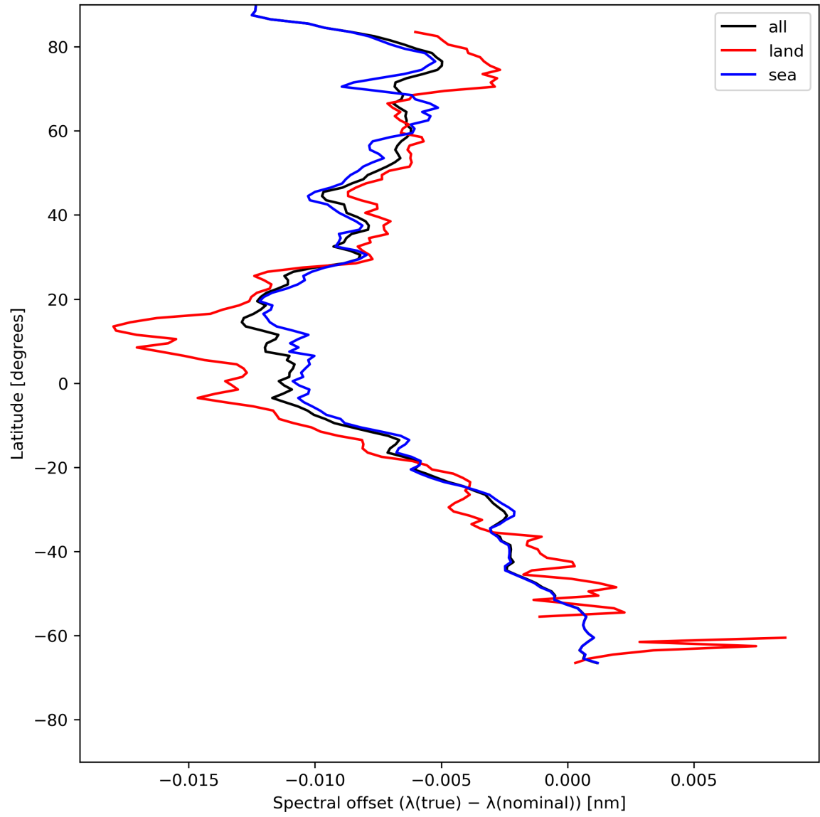
Figure 28: Zonal average of “Spectral offset ( \lambda(\text{true}) - \lambda(\text{nominal}) )” for 2023-07-17 to 2023-07-19.
