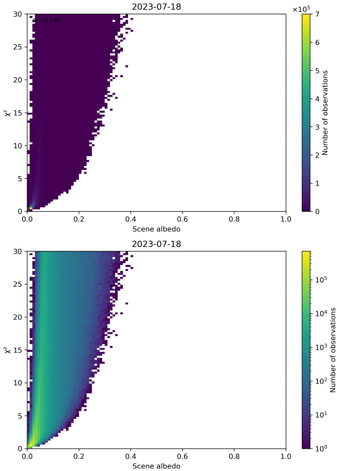
Figure 112: Scatter density plot of “Scene albedo” against “ \chi^2 ” for 2023-07-17 to 2023-07-19.
