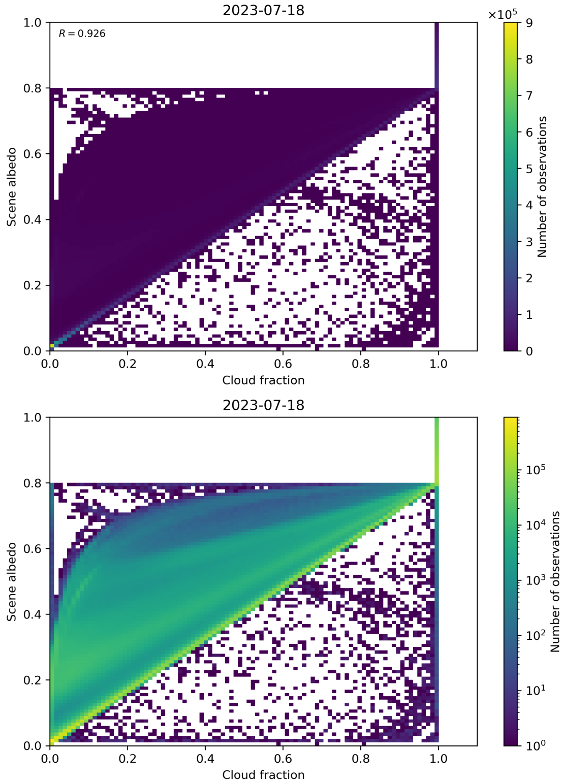
Figure 82: Scatter density plot of “Cloud fraction” against “Scene albedo” for 2023-07-17 to 2023-07-19.
