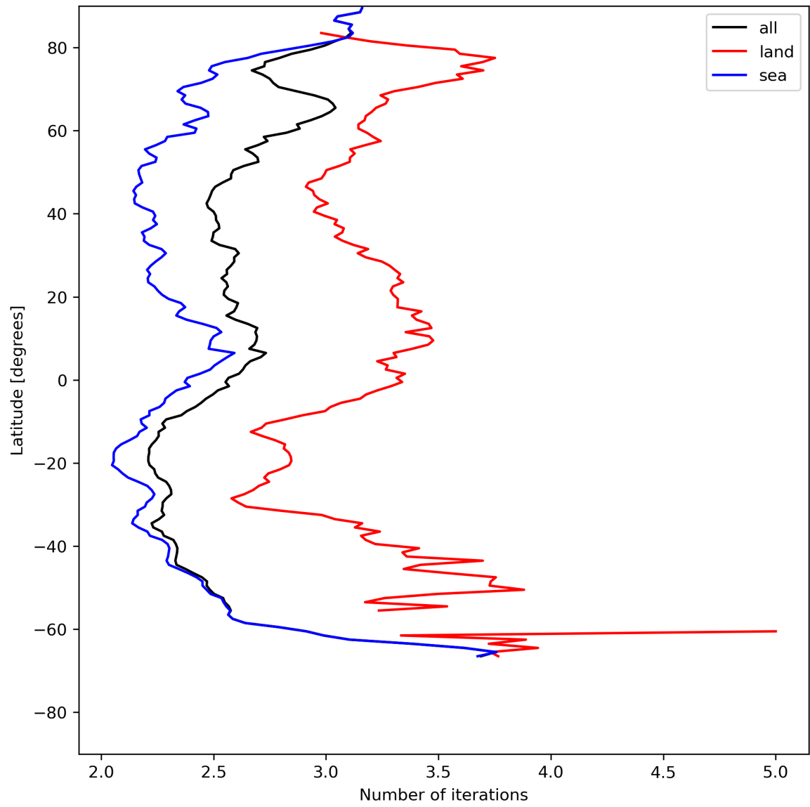
Figure 22: Zonal average of “Number of iterations” for 2023-07-17 to 2023-07-19.
