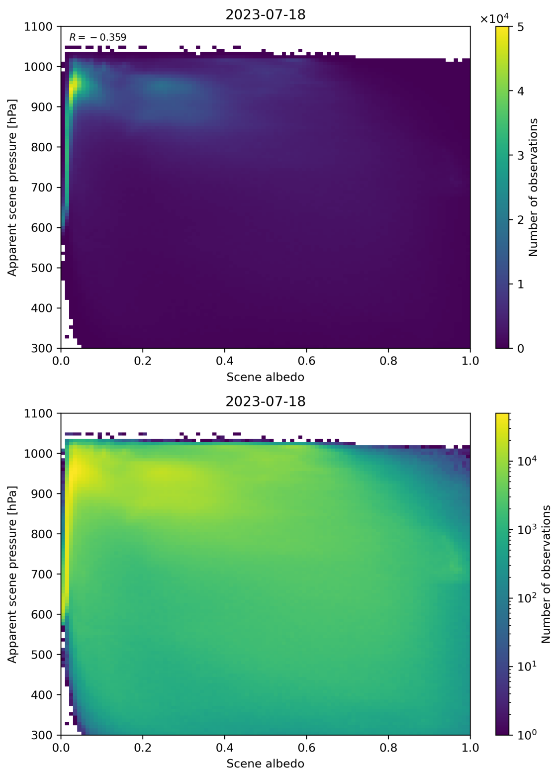
Figure 111: Scatter density plot of “Scene albedo” against “Apparent scene pressure” for 2023-07-17 to 2023-07-19.
