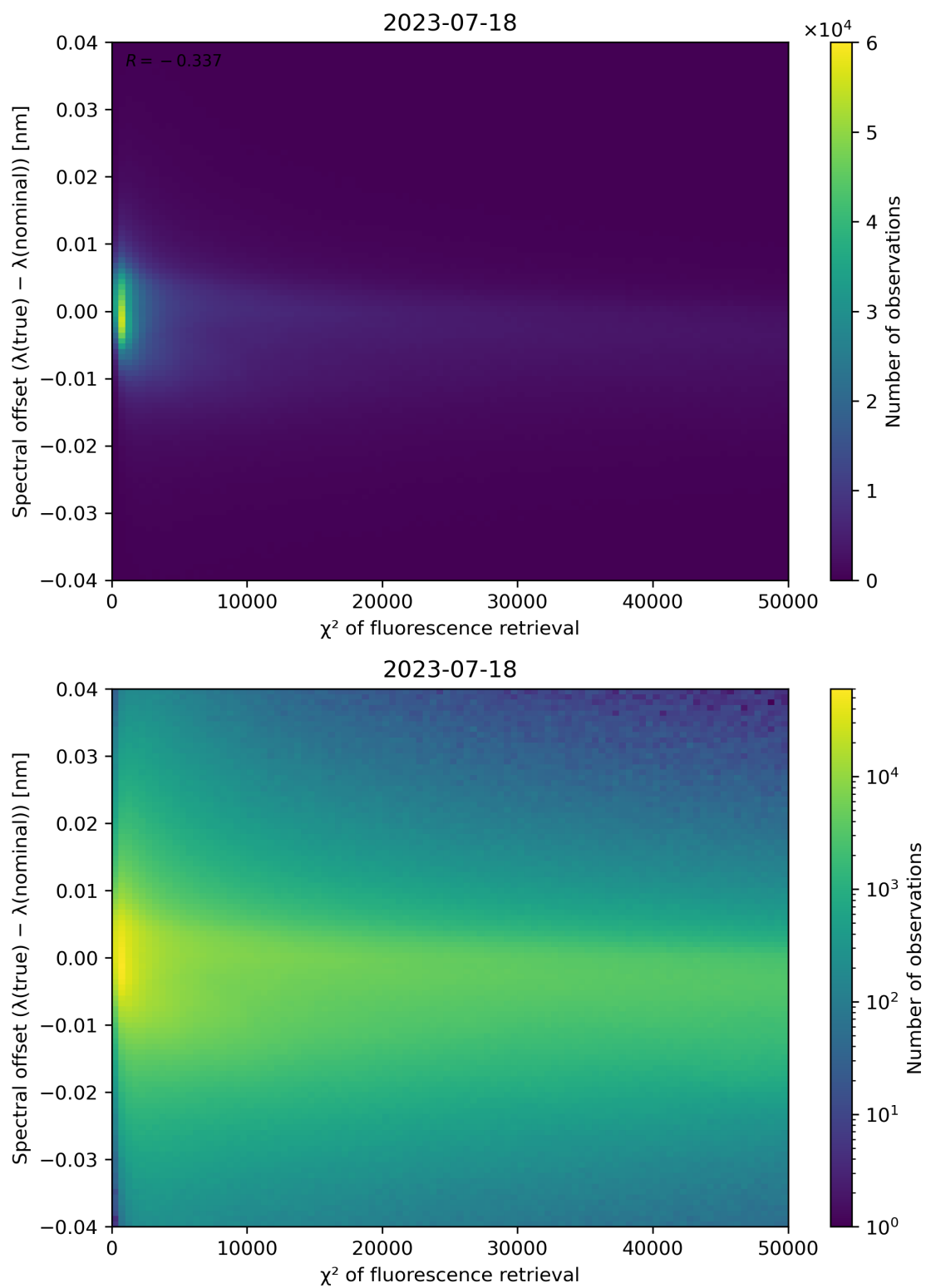
Figure 72: Scatter density plot of " \chi^2 of fluorescence retrieval" against "Spectral offset ( \lambda(\text{true}) - \lambda(\text{nominal}) )" for 2023-07-17 to 2023-07-19.
