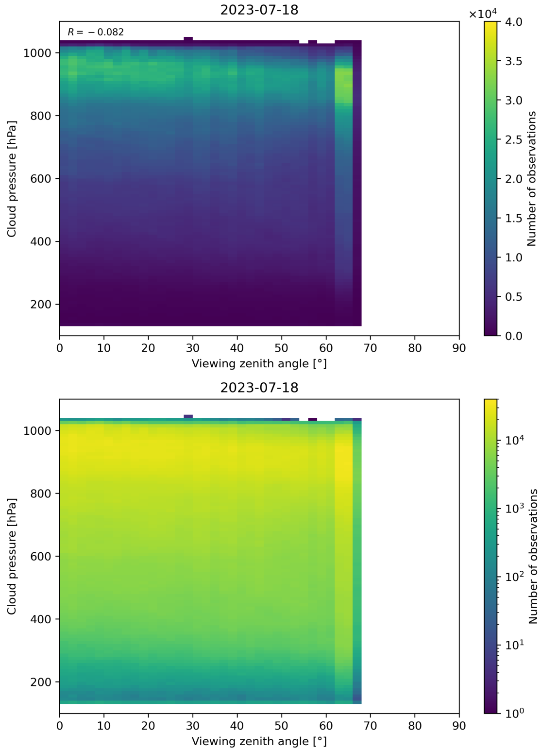
Figure 133: Scatter density plot of “Viewing zenith angle” against “Cloud pressure” for 2023-07-17 to 2023-07-19.
