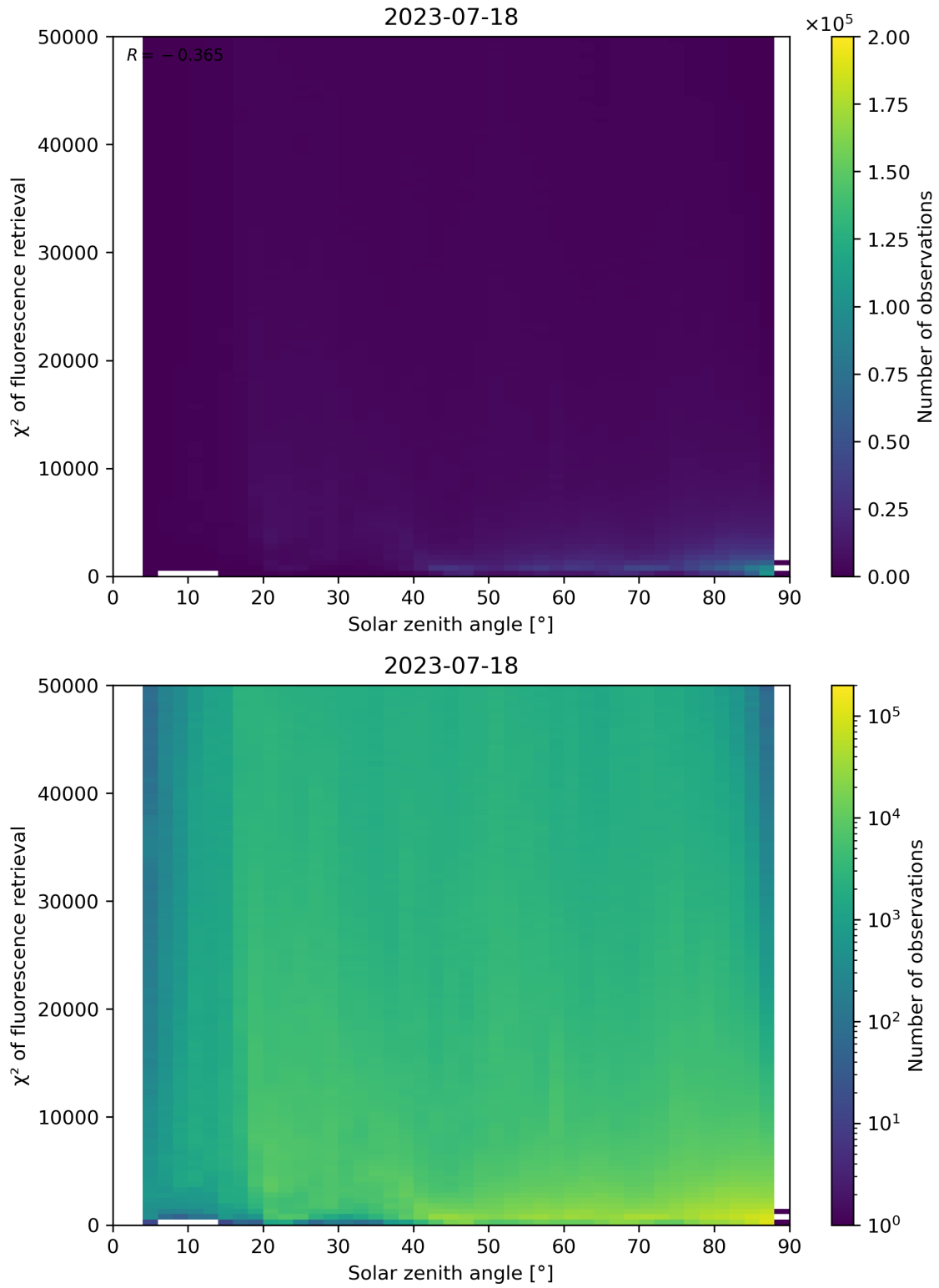
Figure 120: Scatter density plot of “Solar zenith angle” against “ \chi^2 of fluorescence retrieval” for 2023-07-17 to 2023-07-19.
