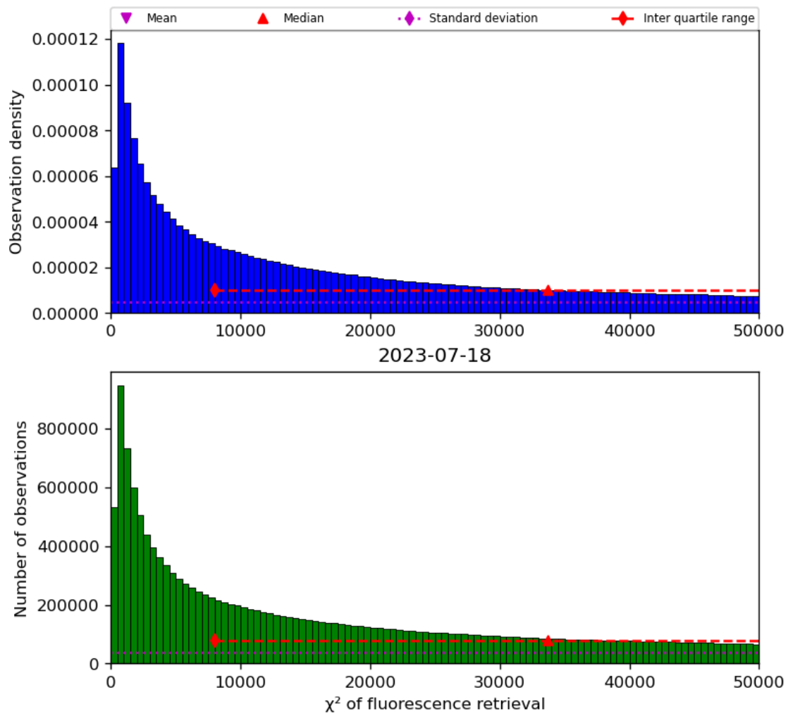
Figure 42: Histogram of “ \chi^2 of fluorescence retrieval” for 2023-07-17 to 2023-07-19
