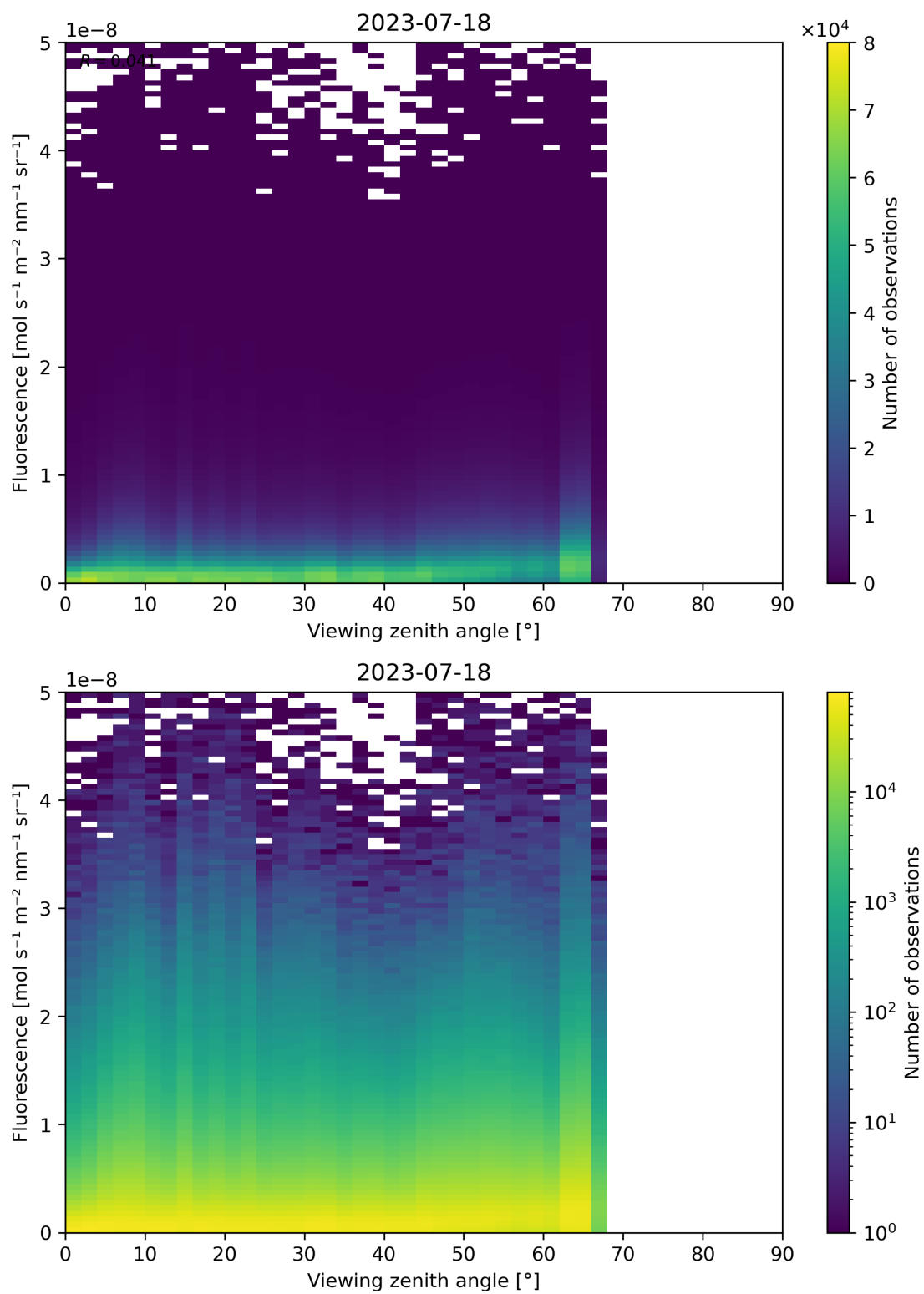
Figure 134: Scatter density plot of “Viewing zenith angle” against “Fluorescence” for 2023-07-17 to 2023-07-19.
