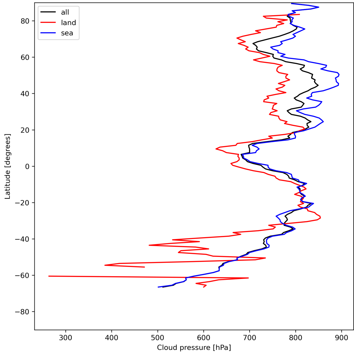
Figure 13: Zonal average of “Cloud pressure” for 2023-07-17 to 2023-07-19.
