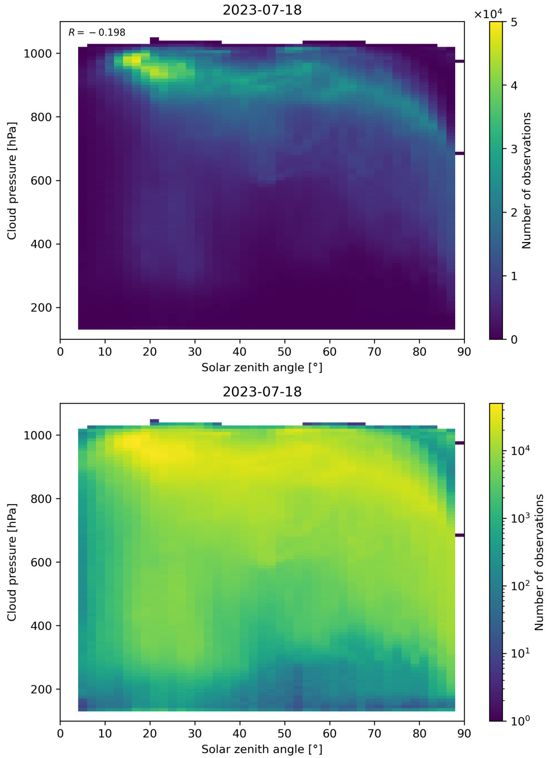
Figure 122: Scatter density plot of “Solar zenith angle” against “Cloud pressure” for 2023-07-17 to 2023-07-19.
