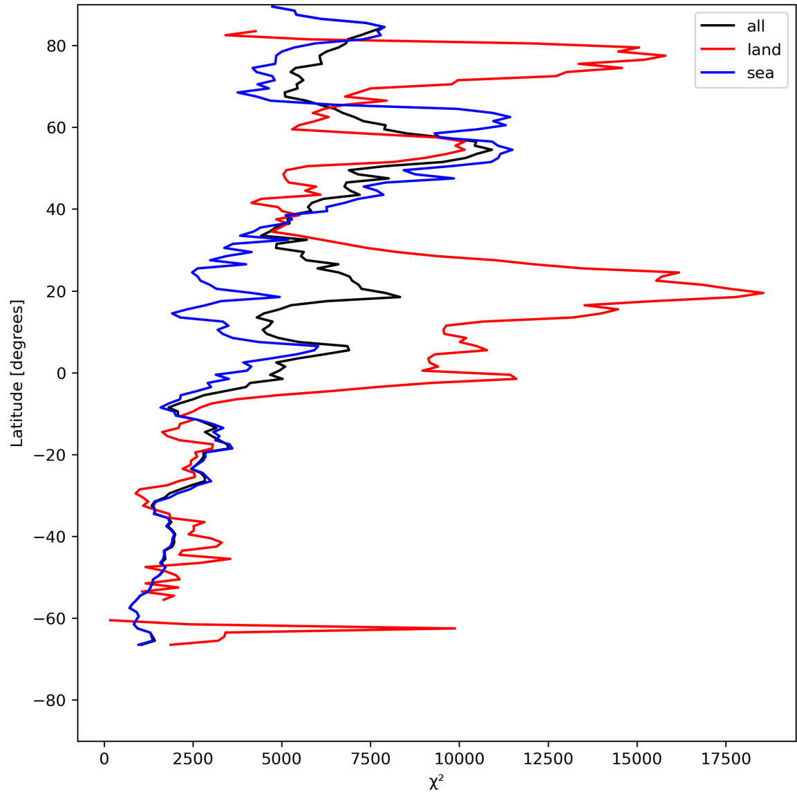
Figure 21: Zonal average of “ \chi^2 ” for 2023-07-17 to 2023-07-19.
