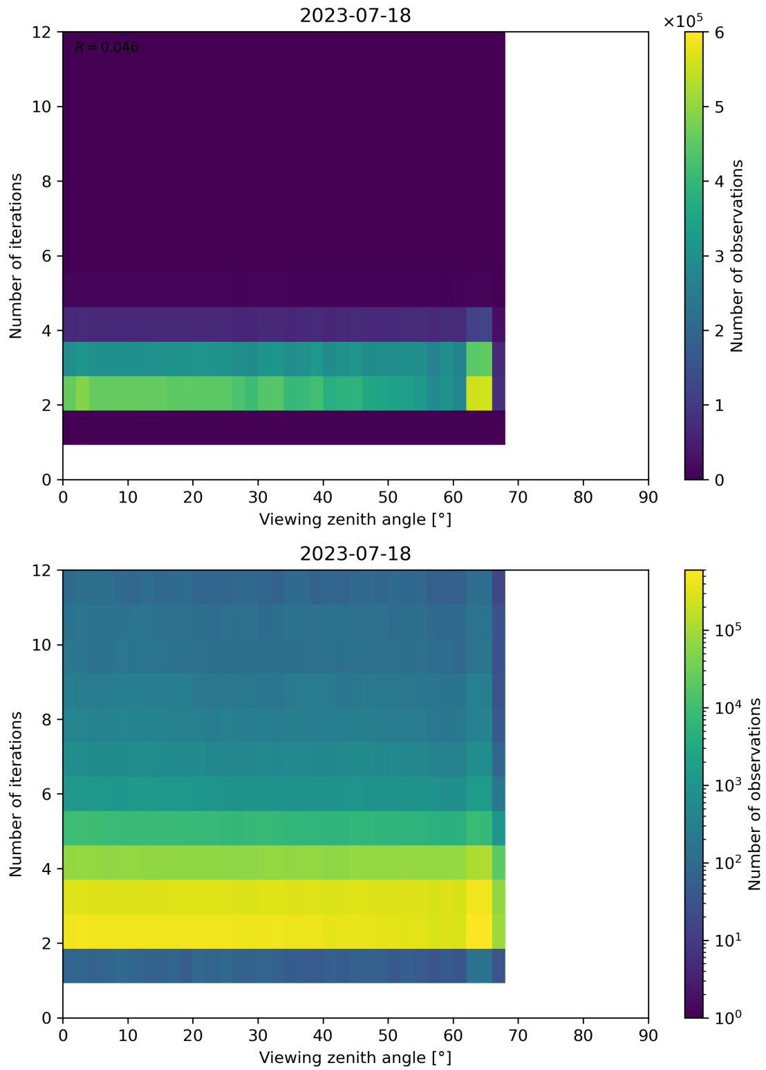
Figure 136: Scatter density plot of “Viewing zenith angle” against “Number of iterations” for 2023-07-17 to 2023-07-19.
