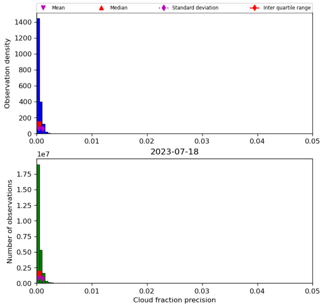
Figure 33: Histogram of “Cloud fraction precision” for 2023-07-17 to 2023-07-19
