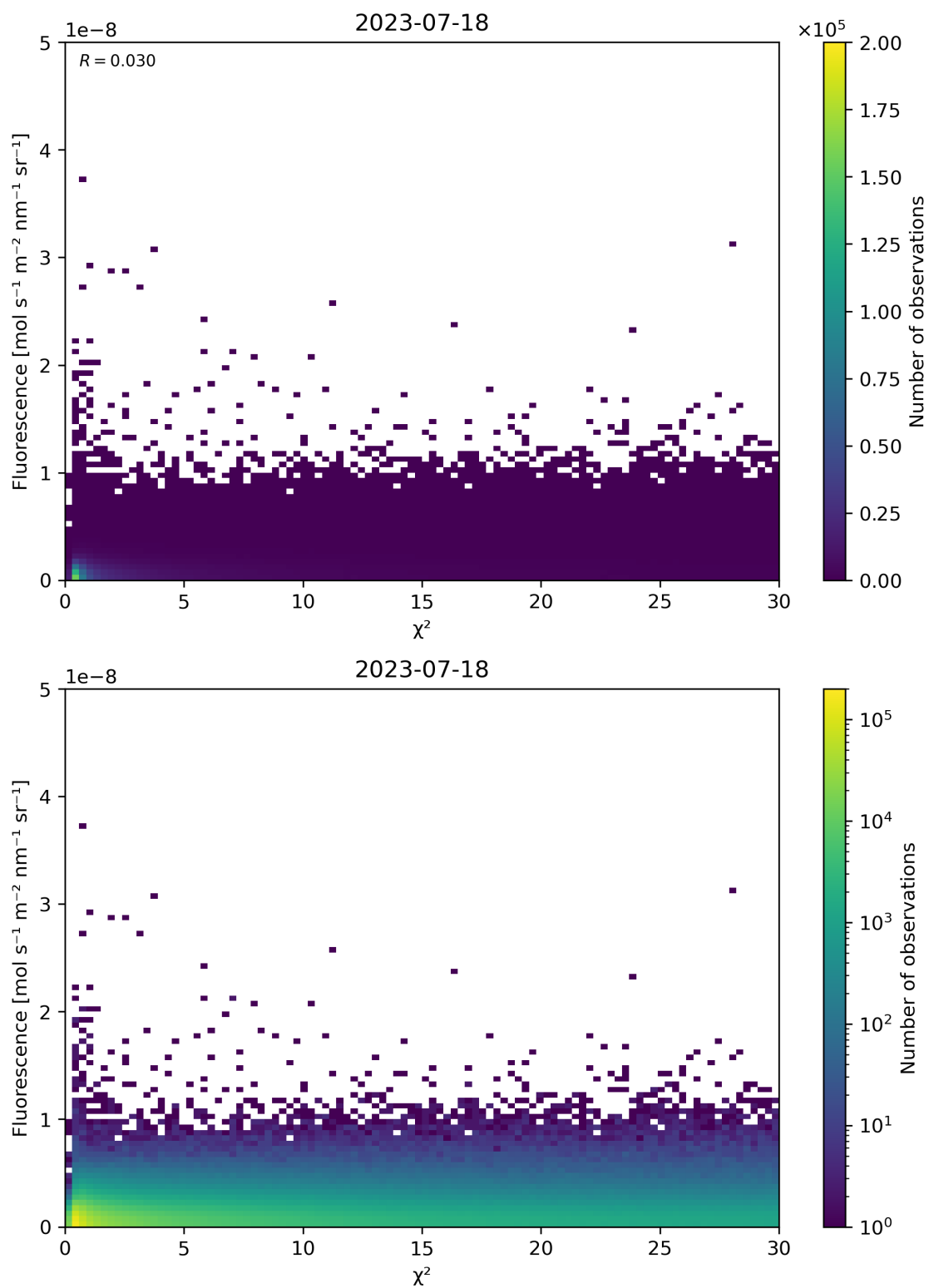
Figure 70: Scatter density plot of “ \chi^2 ” against “Fluorescence” for 2023-07-17 to 2023-07-19.
