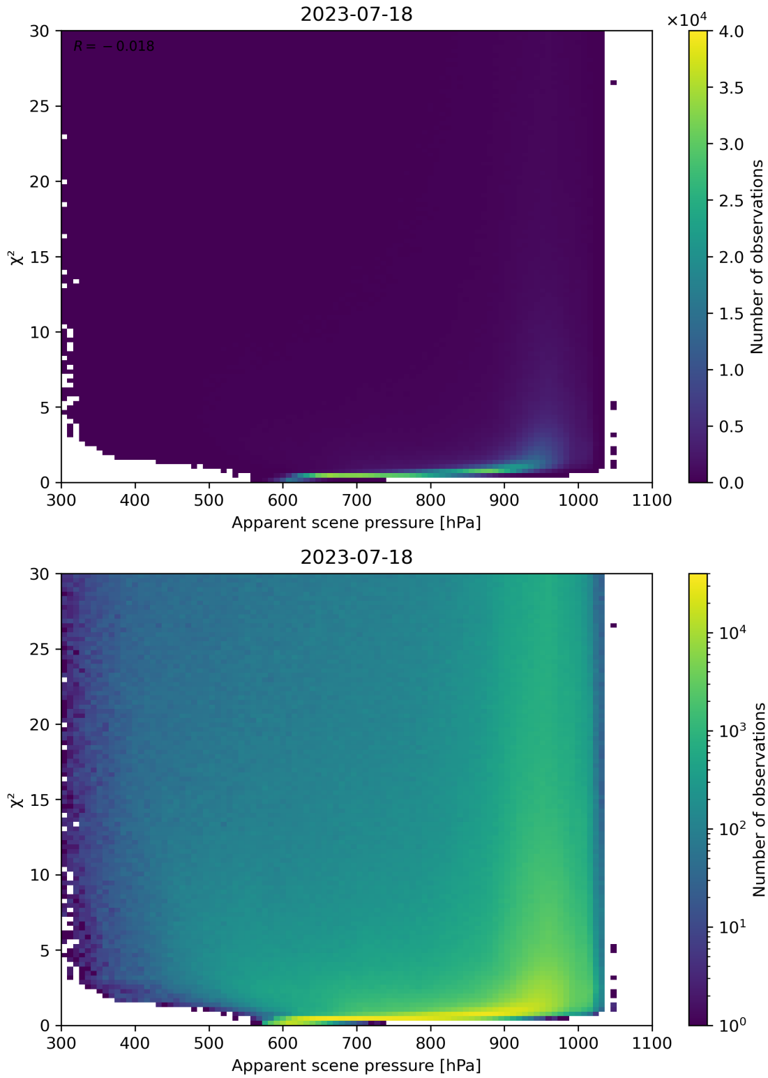
Figure 63: Scatter density plot of “Apparent scene pressure” against “ \chi^2 ” for 2023-07-17 to 2023-07-19.
