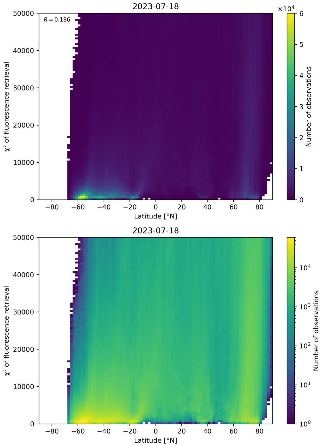
Figure 98: Scatter density plot of “Latitude” against “ \chi^2 of fluorescence retrieval” for 2023-07-17 to 2023-07-19.
