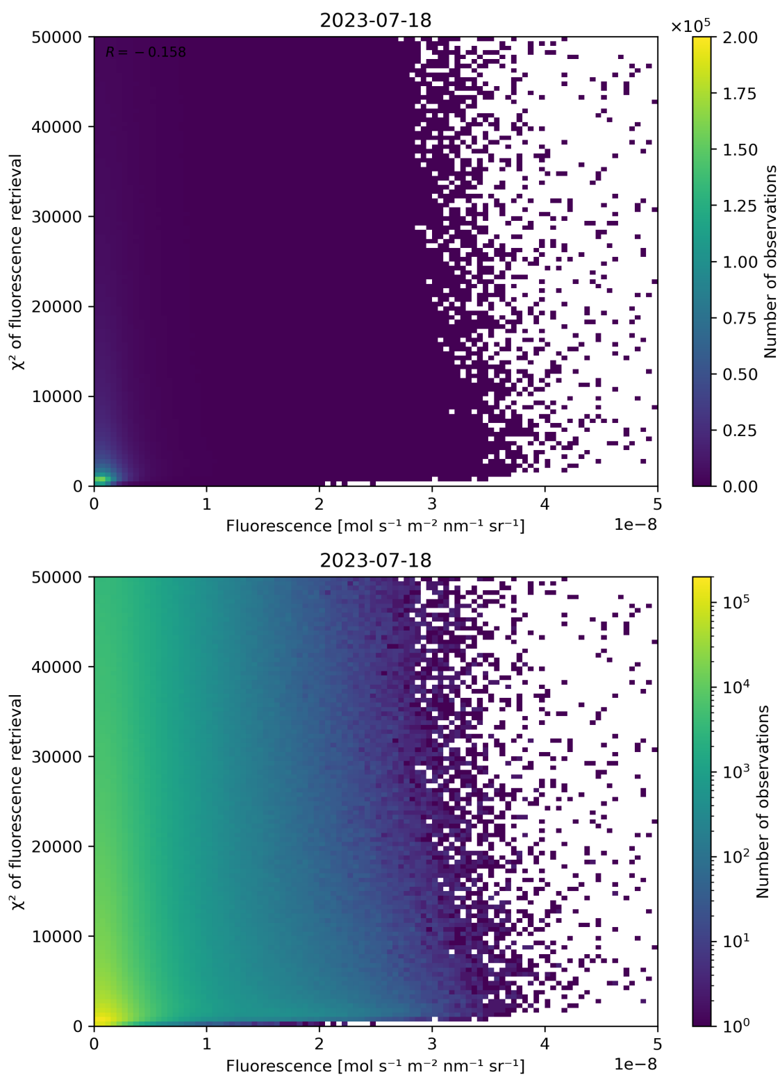
Figure 93: Scatter density plot of “Fluorescence” against “ \chi^2 of fluorescence retrieval” for 2023-07-17 to 2023-07-19.
