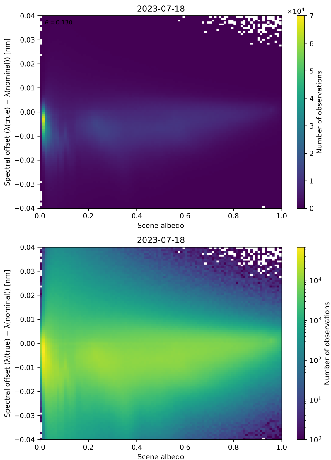
Figure 117: Scatter density plot of “Scene albedo” against “Spectral offset ( \lambda(\text{true}) - \lambda(\text{nominal}) )” for 2023-07-17 to 2023-07-19.
