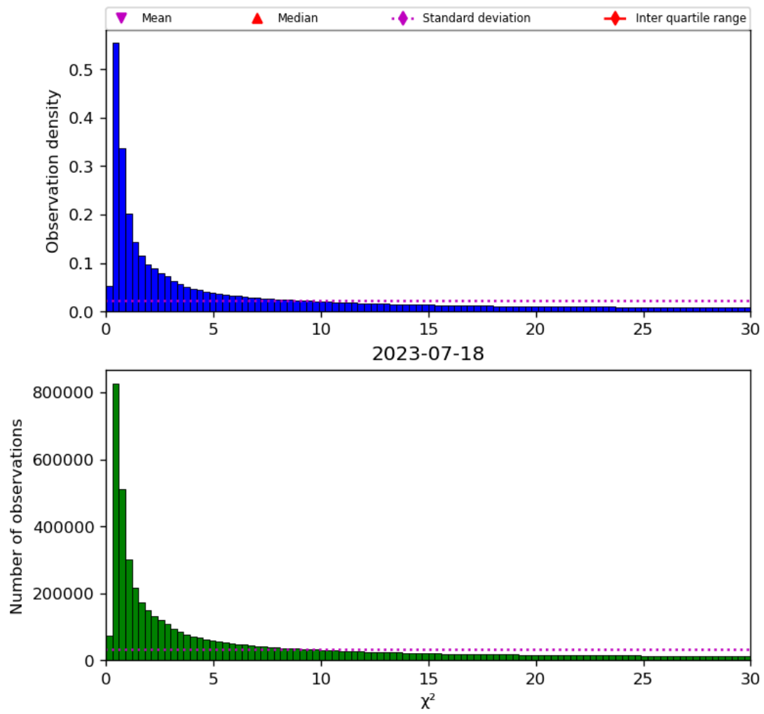
Figure 38: Histogram of “ \chi^2 ” for 2023-07-17 to 2023-07-19
