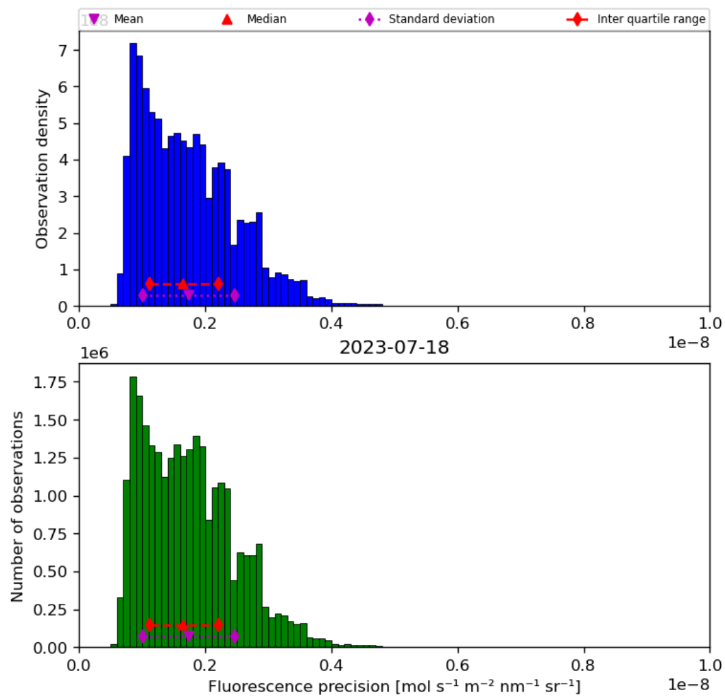
Figure 41: Histogram of “Fluorescence precision” for 2023-07-17 to 2023-07-19
