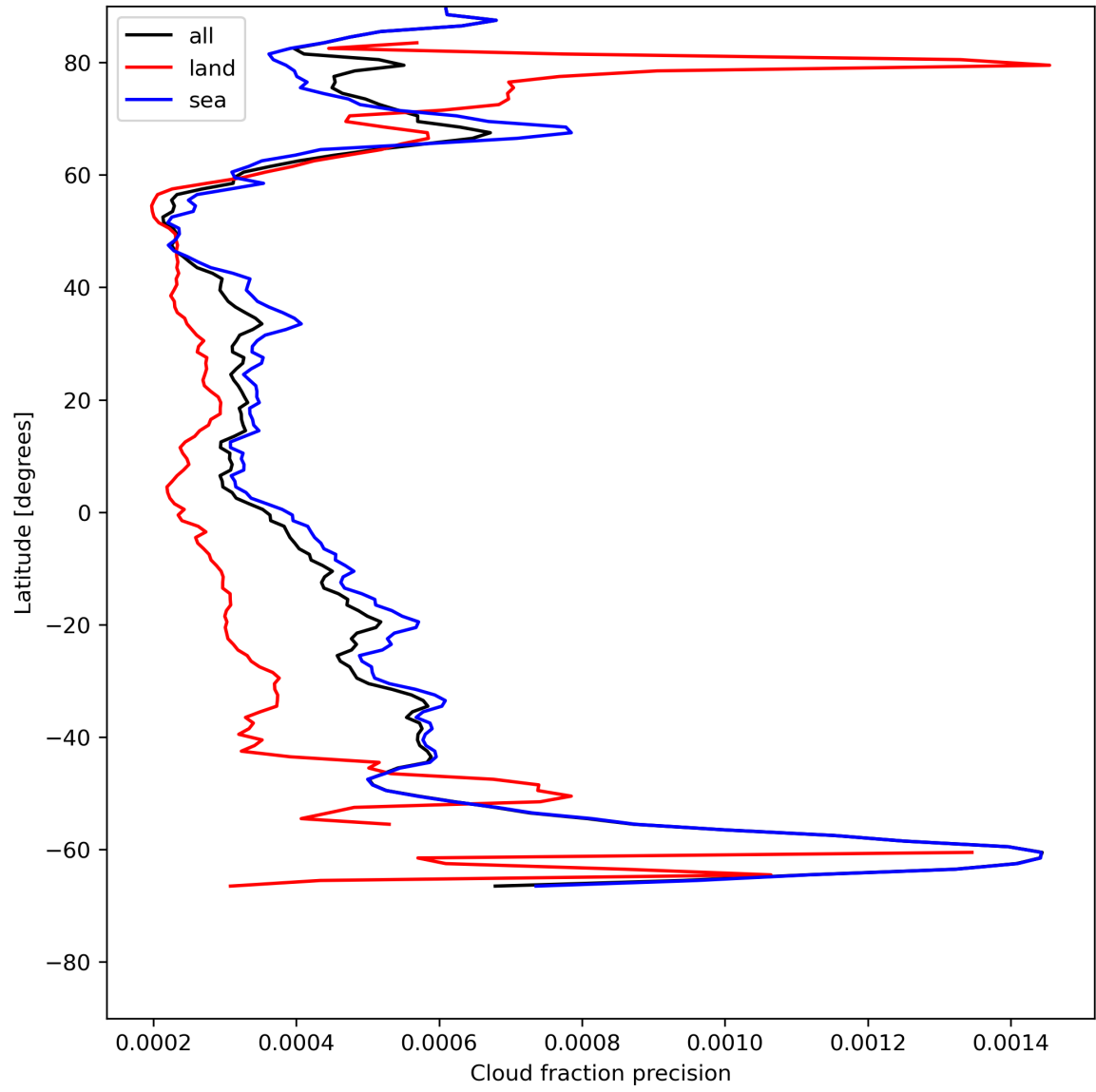
Figure 16: Zonal average of “Cloud fraction precision” for 2023-07-17 to 2023-07-19.
