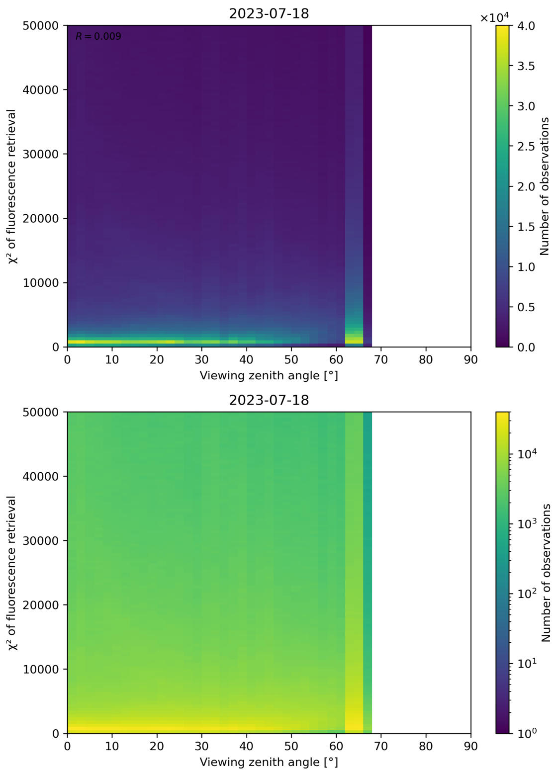
Figure 131: Scatter density plot of “Viewing zenith angle” against “ \chi^2 of fluorescence retrieval” for 2023-07-17 to 2023-07-19.
