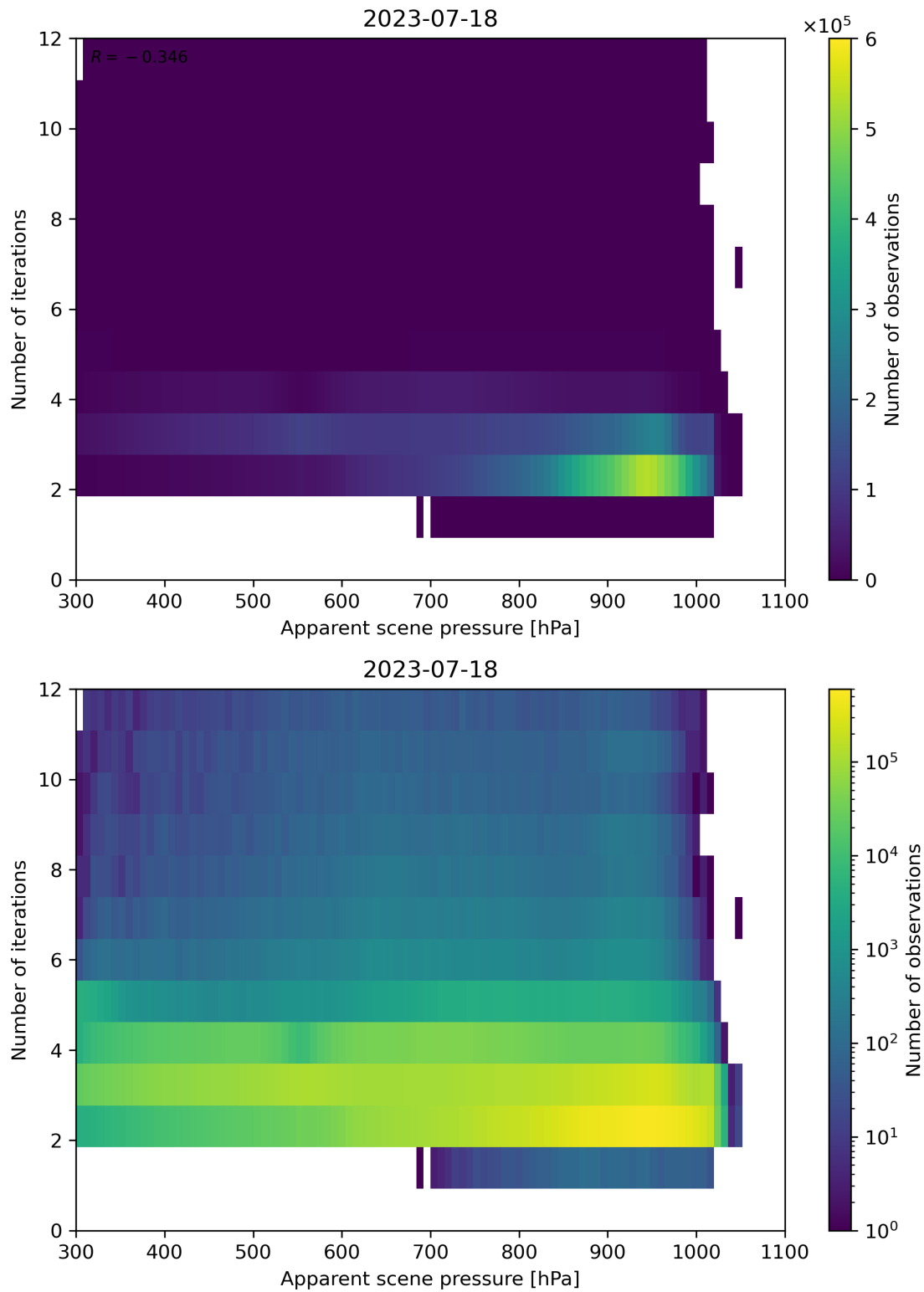
Figure 66: Scatter density plot of “Apparent scene pressure” against “Number of iterations” for 2023-07-17 to 2023-07-19.
