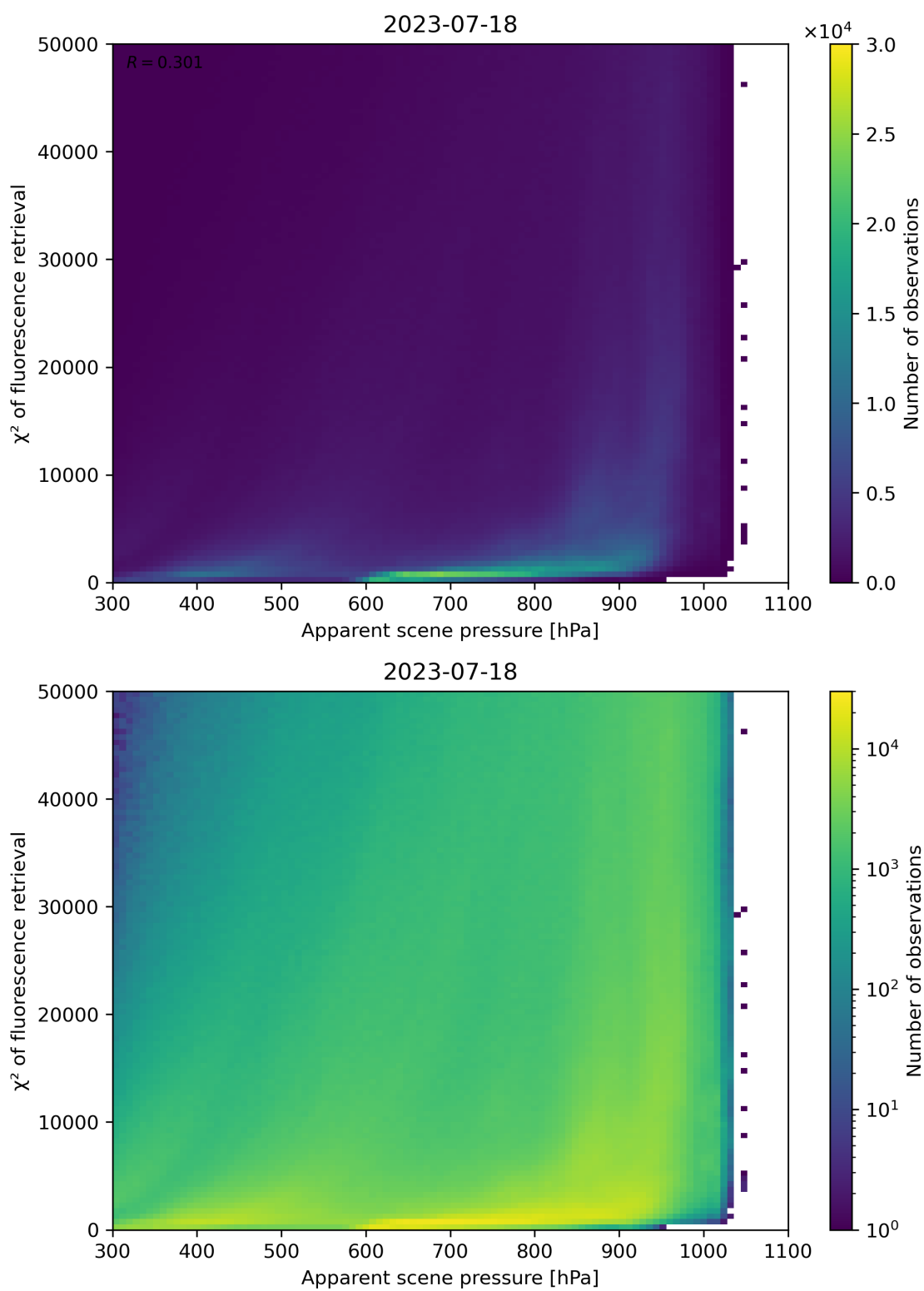
Figure 64: Scatter density plot of “Apparent scene pressure” against “ \chi^2 of fluorescence retrieval” for 2023-07-17 to 2023-07-19.
