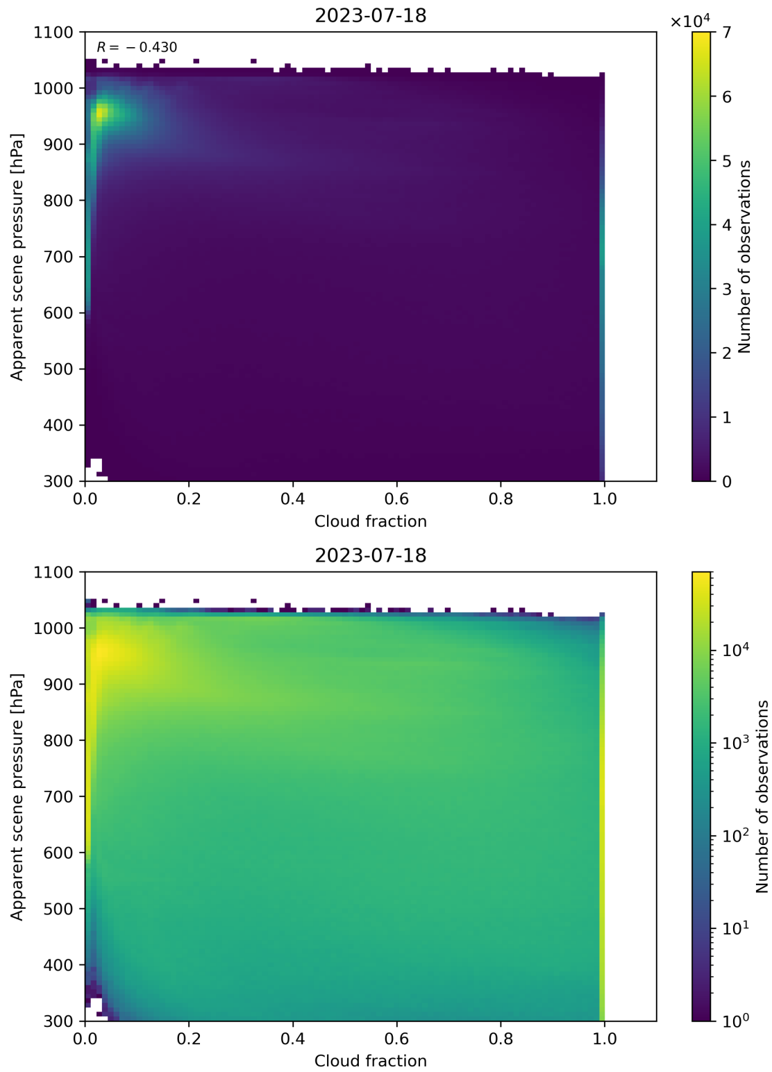
Figure 76: Scatter density plot of “Cloud fraction” against “Apparent scene pressure” for 2023-07-17 to 2023-07-19.
