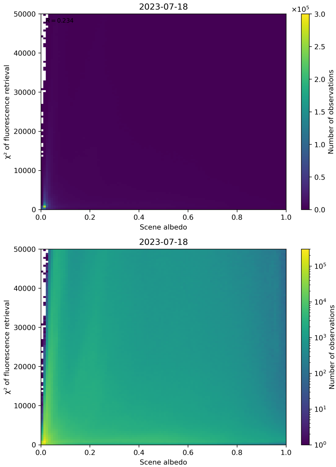
Figure 113: Scatter density plot of “Scene albedo” against “ \chi^2 of fluorescence retrieval” for 2023-07-17 to 2023-07-19.
