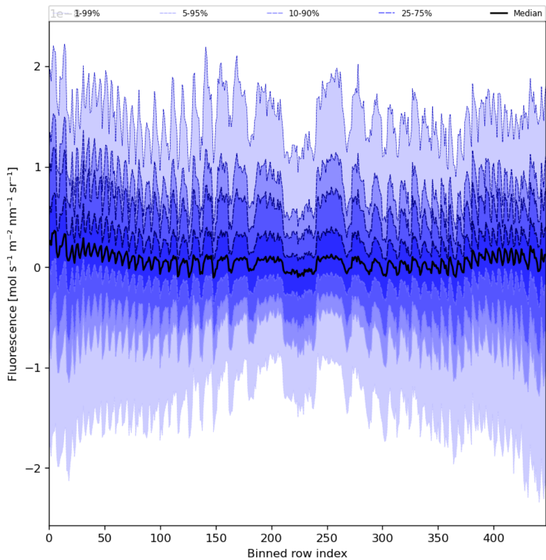
Figure 57: Along track statistics of "Fluorescence" for 2023-07-17 to 2023-07-19
