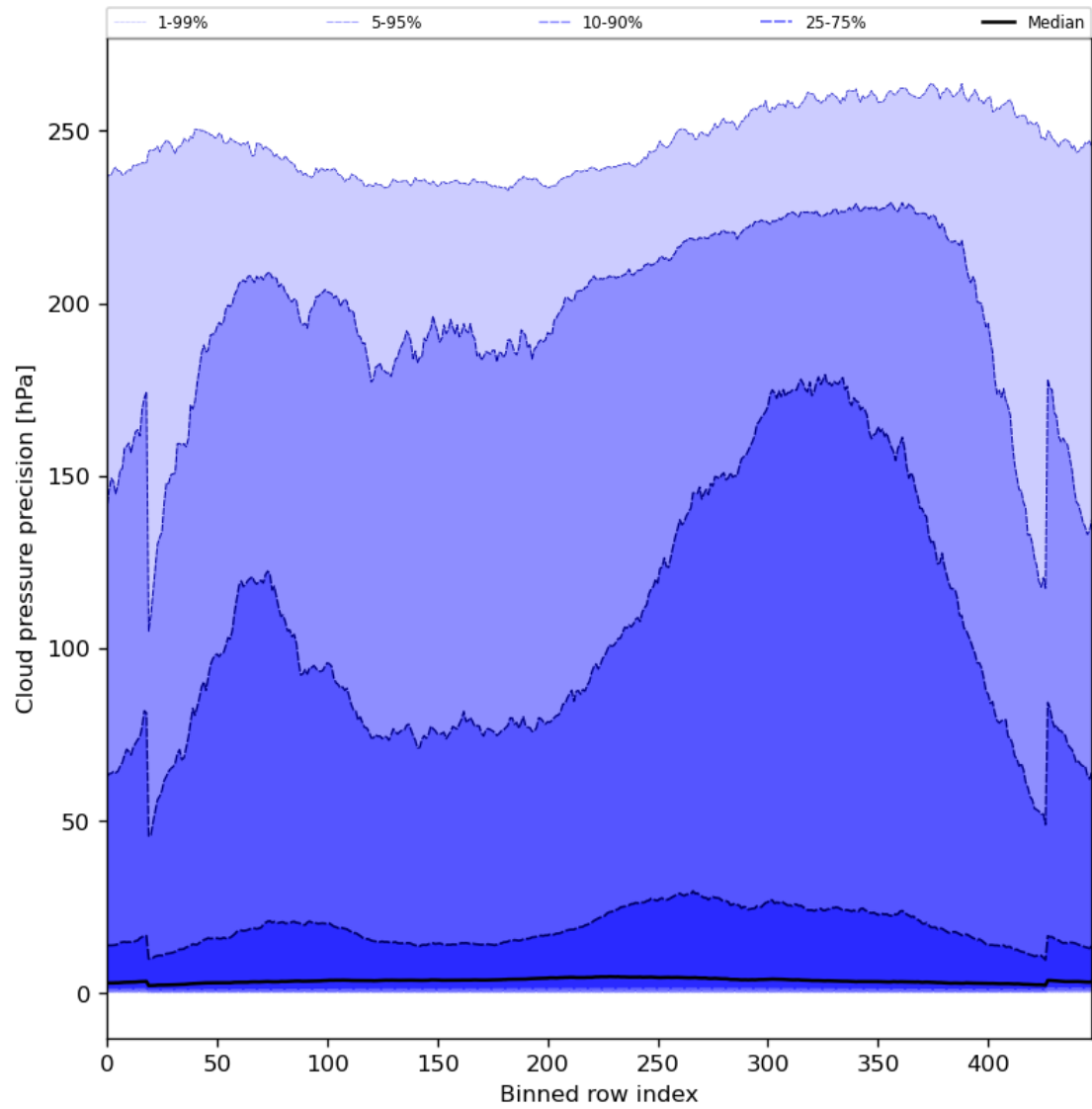
Figure 48: Along track statistics of “Cloud pressure precision” for 2023-07-17 to 2023-07-19
