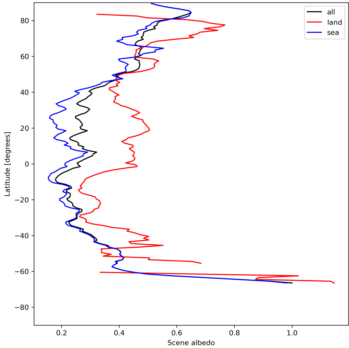
Figure 17: Zonal average of “Scene albedo” for 2023-07-17 to 2023-07-19.
