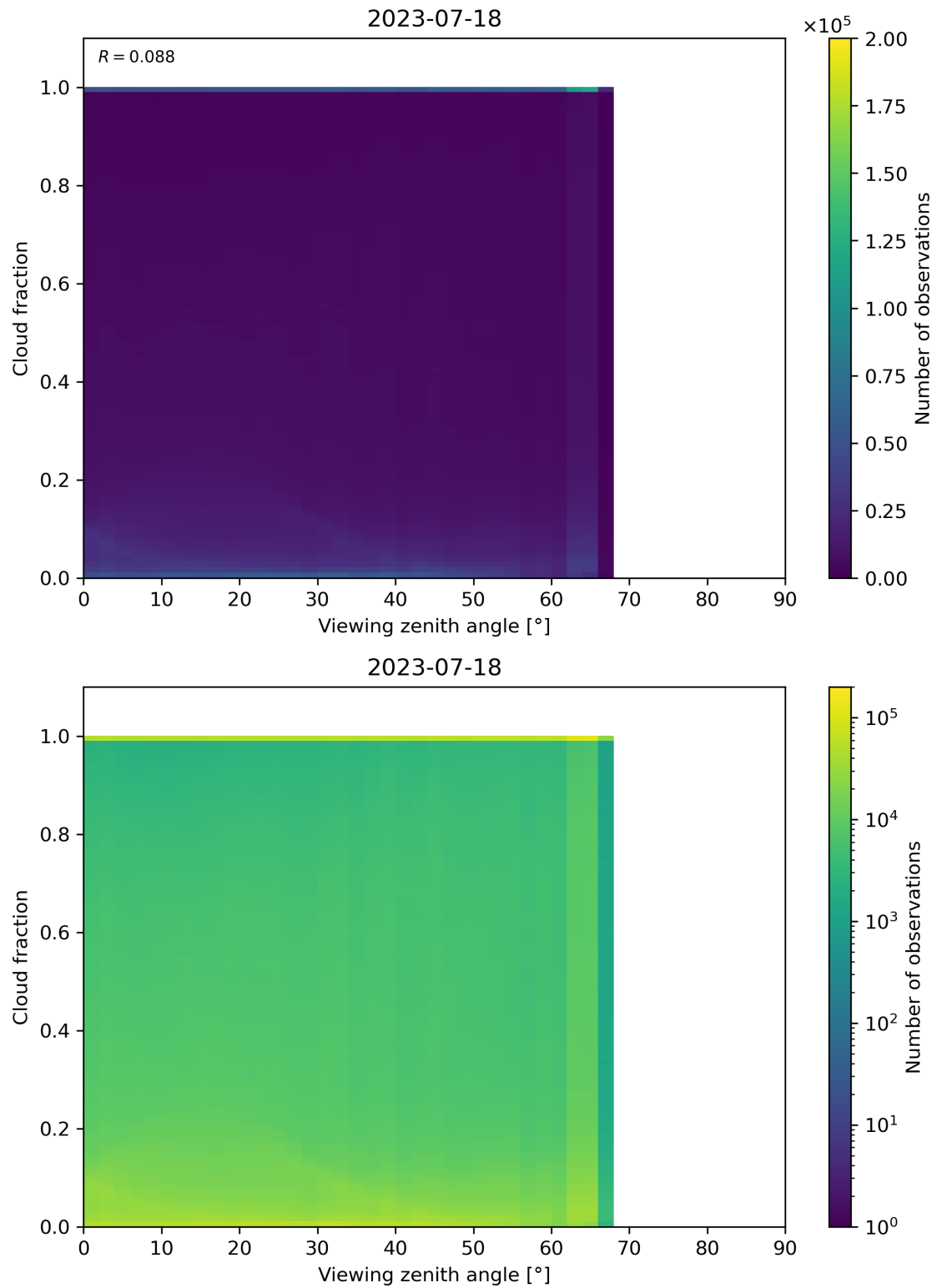
Figure 132: Scatter density plot of “Viewing zenith angle” against “Cloud fraction” for 2023-07-17 to 2023-07-19.
