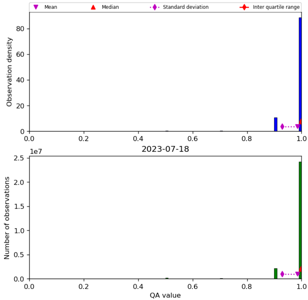
Figure 29: Histogram of “QA value” for 2023-07-17 to 2023-07-19
