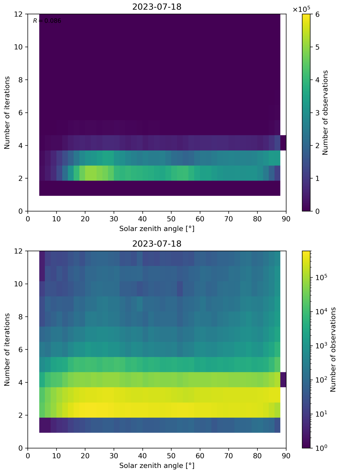
Figure 125: Scatter density plot of “Solar zenith angle” against “Number of iterations” for 2023-07-17 to 2023-07-19.
