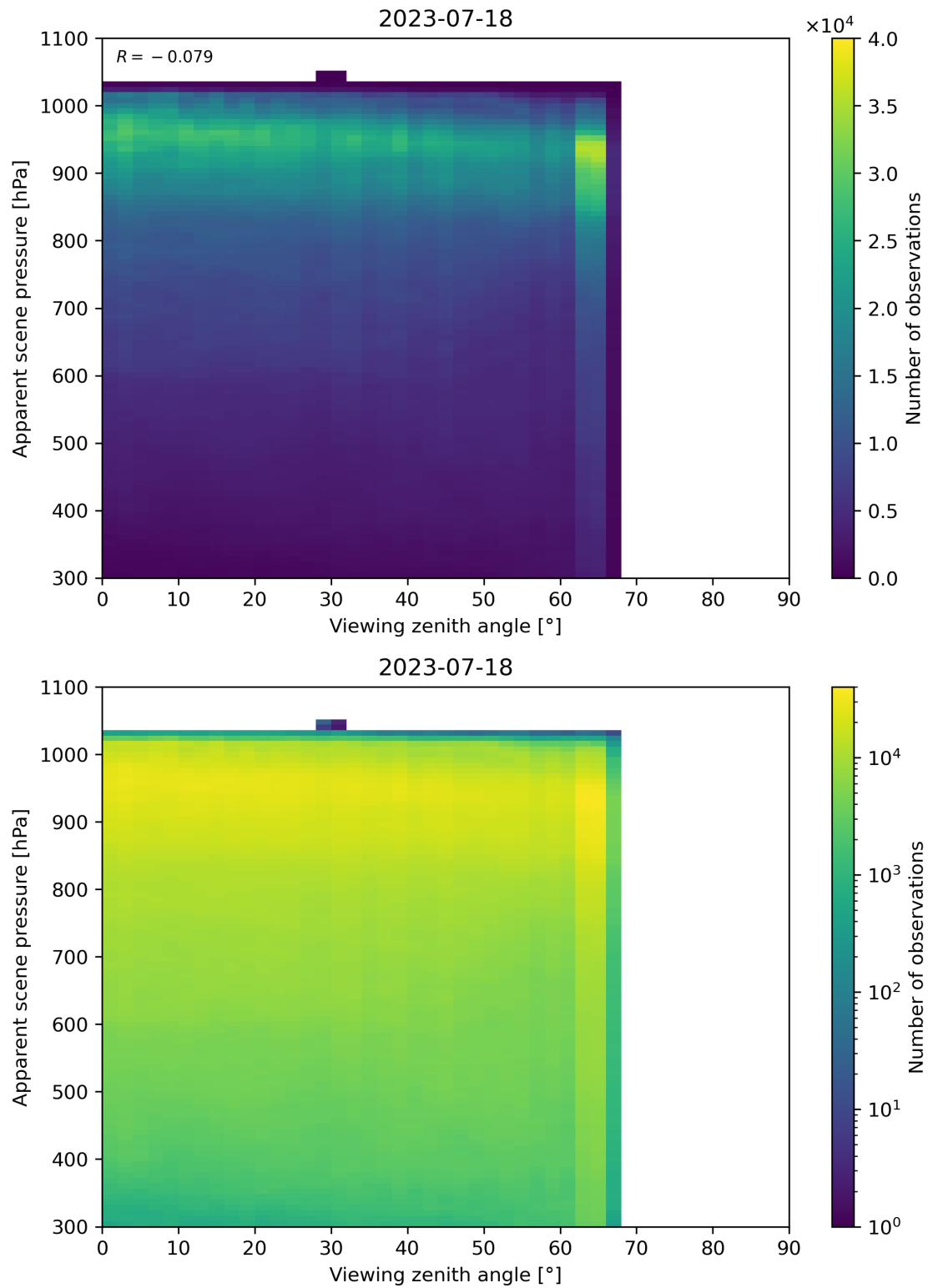
Figure 129: Scatter density plot of “Viewing zenith angle” against “Apparent scene pressure” for 2023-07-17 to 2023-07-19.
