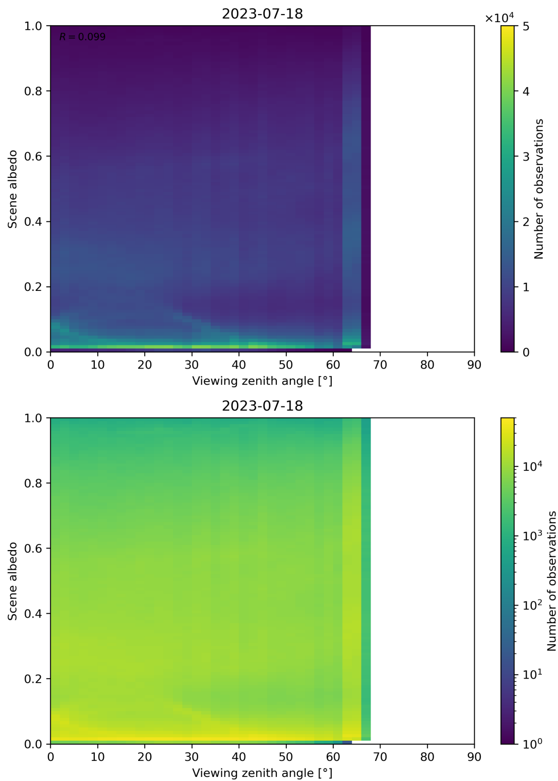
Figure 138: Scatter density plot of “Viewing zenith angle” against “Scene albedo” for 2023-07-17 to 2023-07-19.
