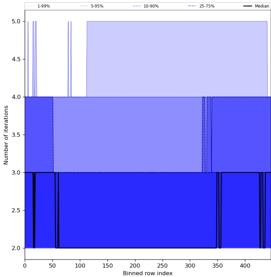
Figure 56: Along track statistics of “Number of iterations” for 2023-07-17 to 2023-07-19
