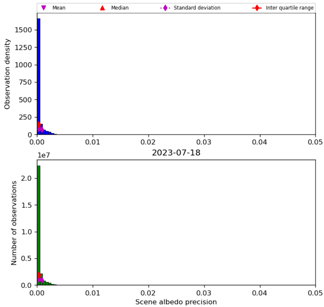
Figure 35: Histogram of “Scene albedo precision” for 2023-07-17 to 2023-07-19
