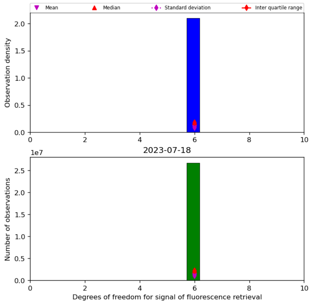
Figure 43: Histogram of “Degrees of freedom for signal of fluorescence retrieval” for 2023-07-17 to 2023-07-19
