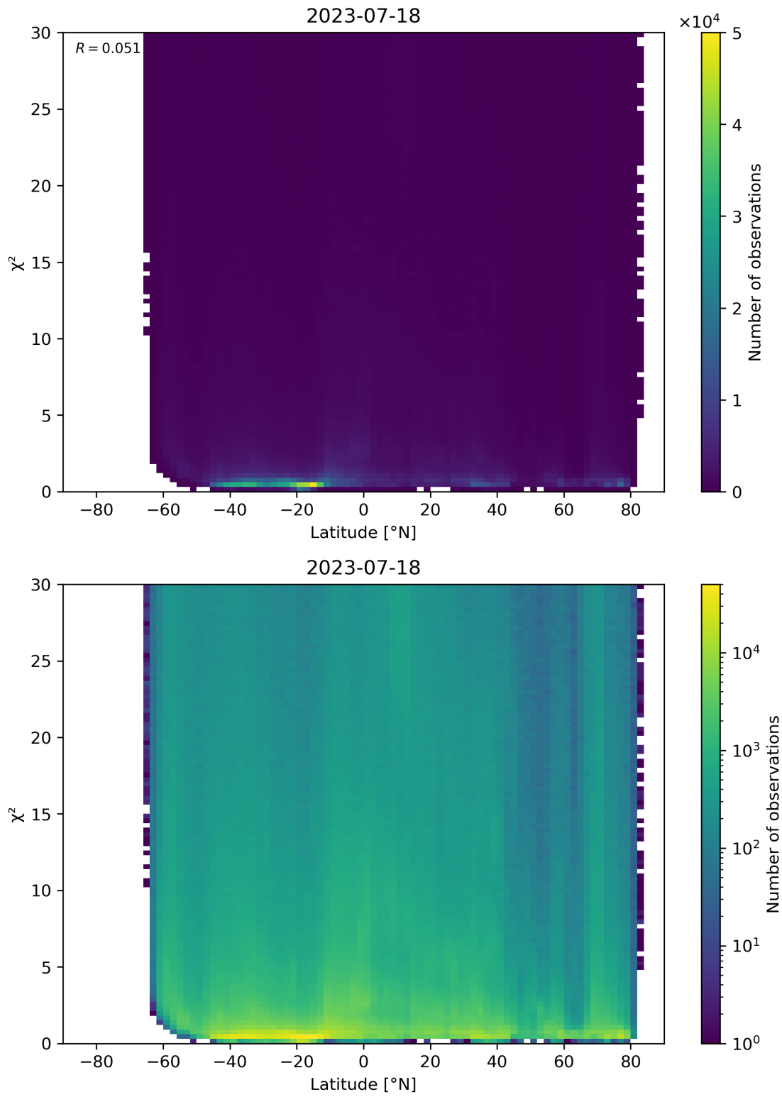
Figure 97: Scatter density plot of “Latitude” against “ \chi^2 ” for 2023-07-17 to 2023-07-19.
