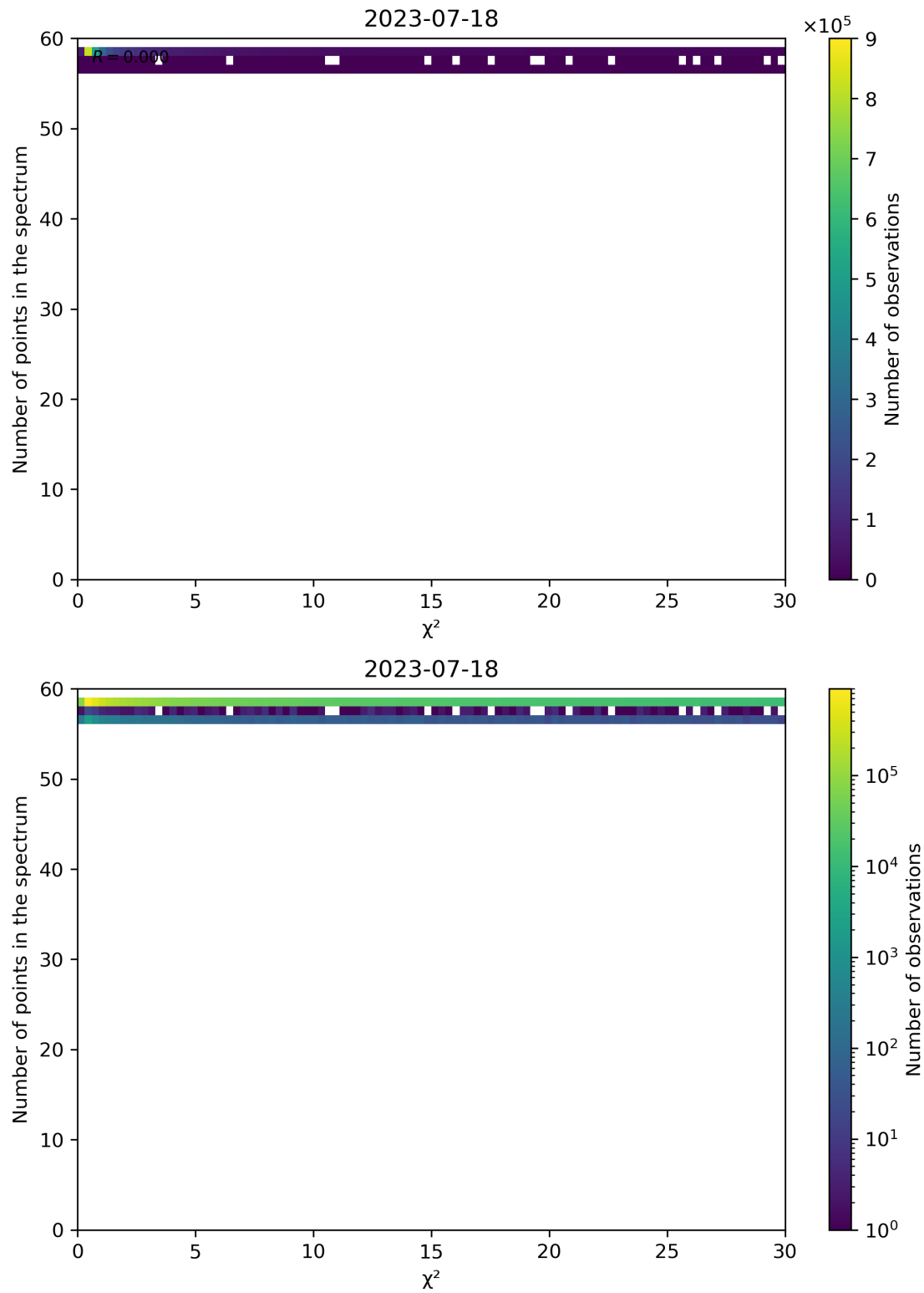
Figure 74: Scatter density plot of “ \chi^2 ” against “Number of points in the spectrum” for 2023-07-17 to 2023-07-19.
