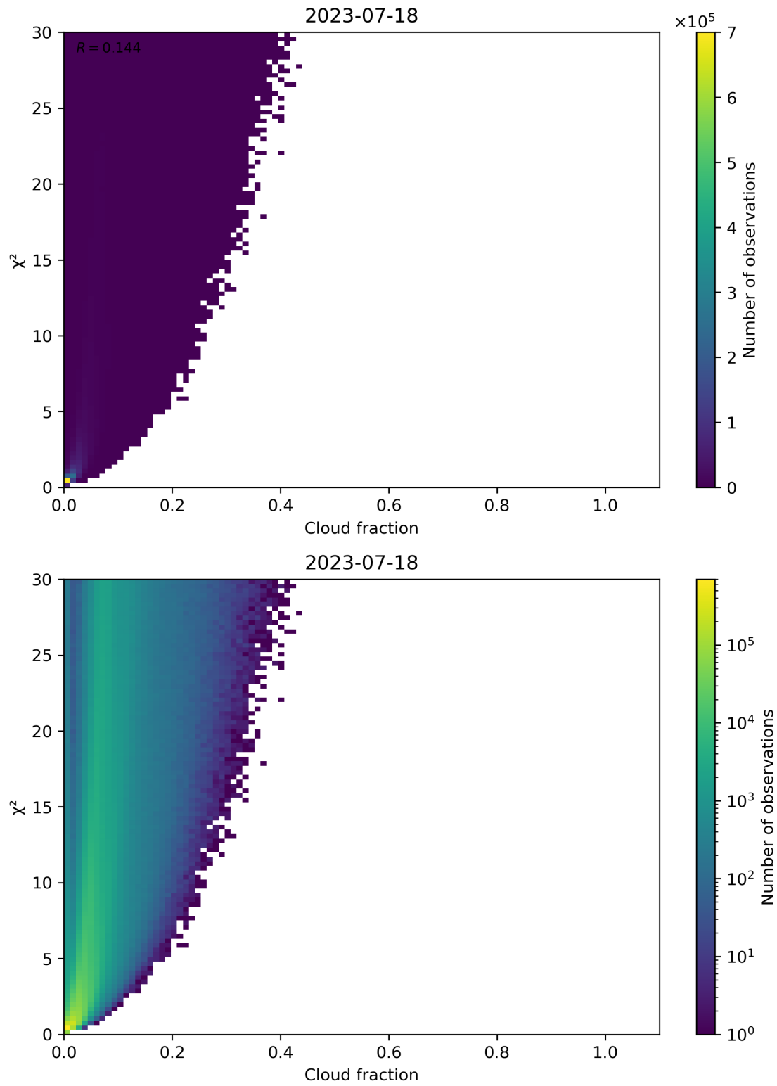
Figure 77: Scatter density plot of “Cloud fraction” against “ \chi^2 ” for 2023-07-17 to 2023-07-19.
