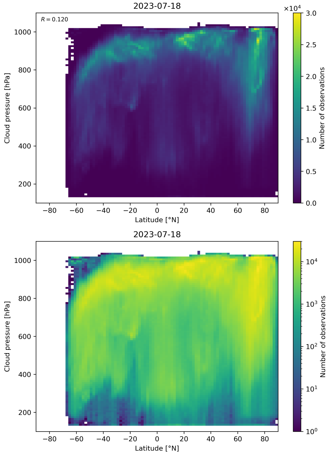
Figure 100: Scatter density plot of “Latitude” against “Cloud pressure” for 2023-07-17 to 2023-07-19.
