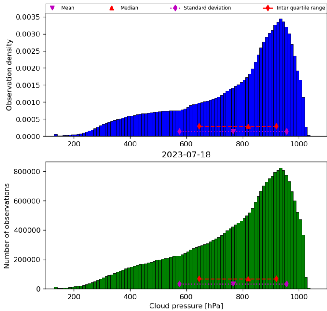
Figure 30: Histogram of “Cloud pressure” for 2023-07-17 to 2023-07-19
