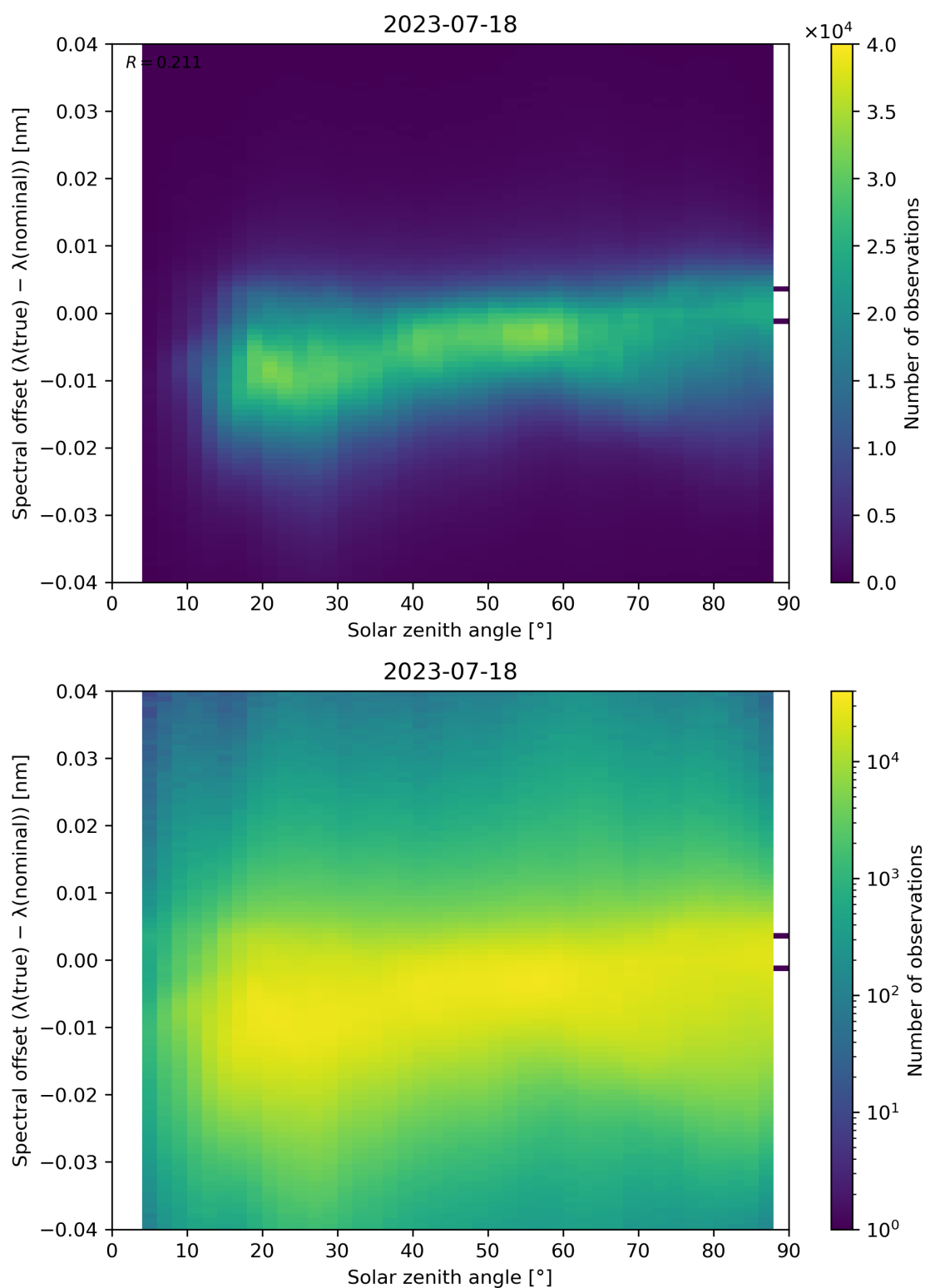
Figure 128: Scatter density plot of “Solar zenith angle” against “Spectral offset ( \lambda(\text{true}) - \lambda(\text{nominal}) )” for 2023-07-17 to 2023-07-19.
