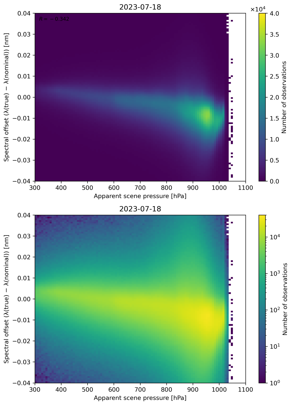
Figure 68: Scatter density plot of “Apparent scene pressure” against “Spectral offset ( \lambda(\text{true}) - \lambda(\text{nominal}) )” for 2023-07-17 to 2023-07-19.
