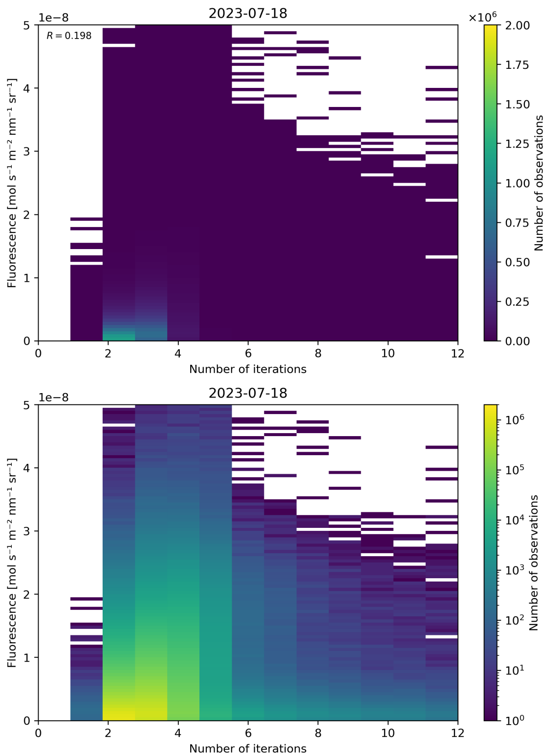
Figure 107: Scatter density plot of “Number of iterations” against “Fluorescence” for 2023-07-17 to 2023-07-19.
