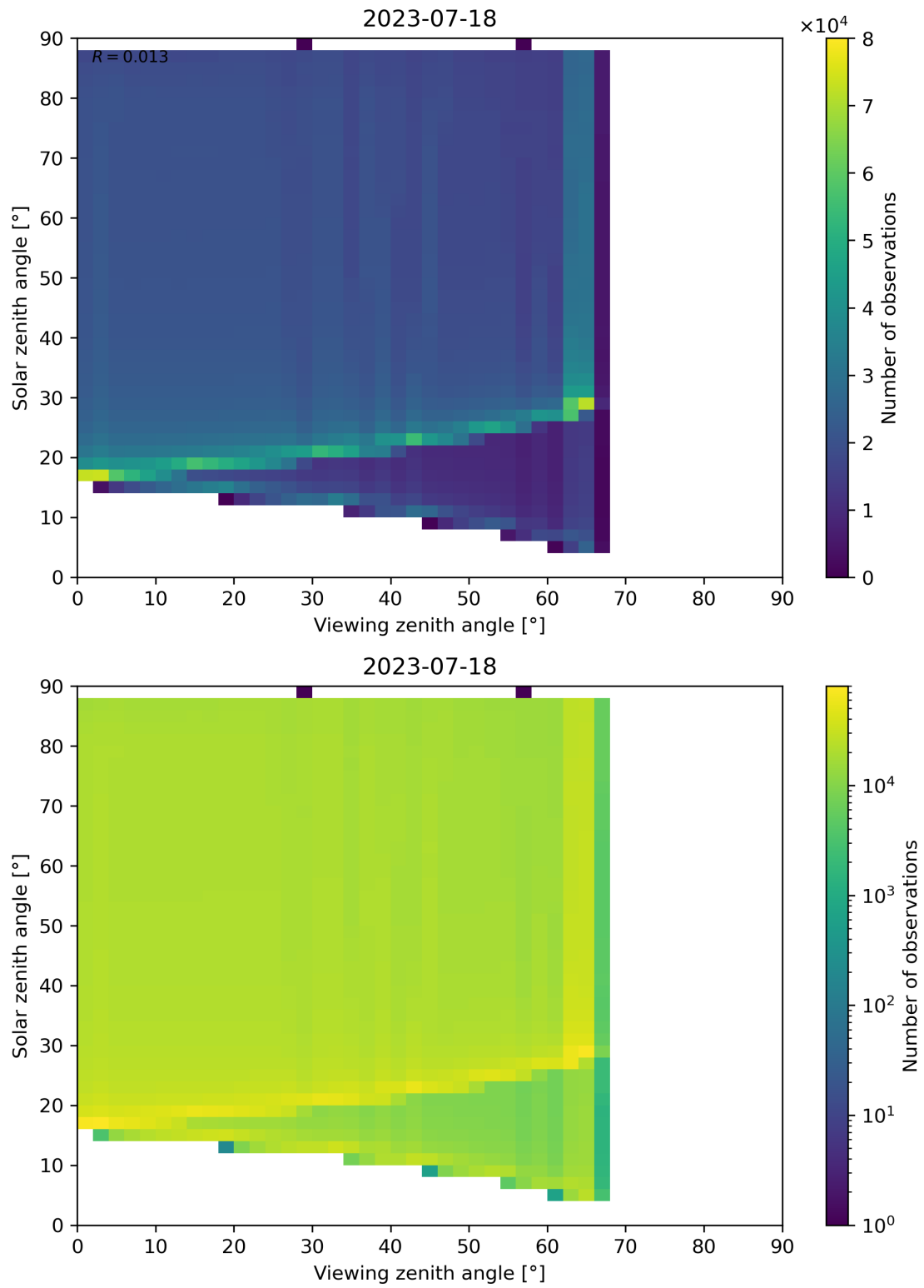
Figure 139: Scatter density plot of “Viewing zenith angle” against “Solar zenith angle” for 2023-07-17 to 2023-07-19.
