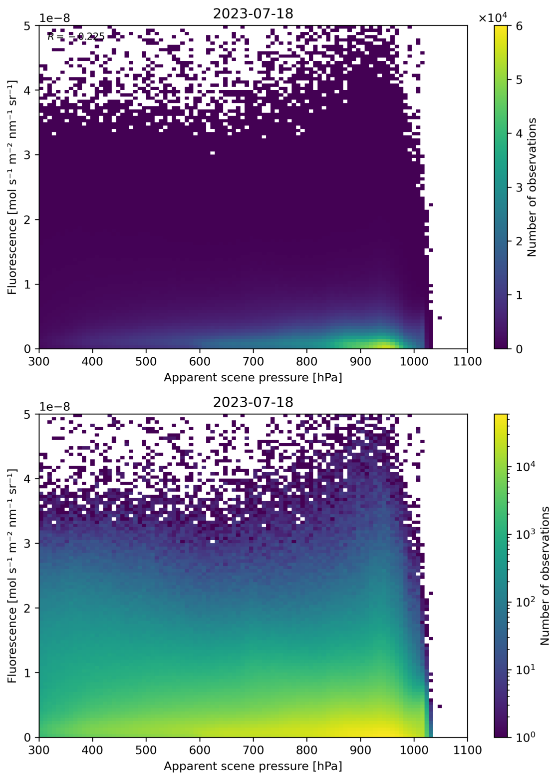
Figure 65: Scatter density plot of “Apparent scene pressure” against “Fluorescence” for 2023-07-17 to 2023-07-19.
