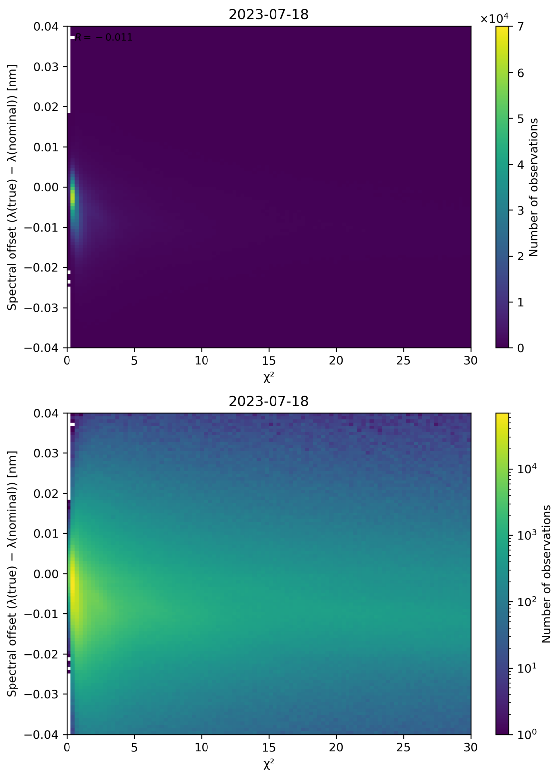
Figure 75: Scatter density plot of “ \chi^2 ” against “Spectral offset ( \lambda(\text{true}) - \lambda(\text{nominal}) )” for 2023-07-17 to 2023-07-19.
