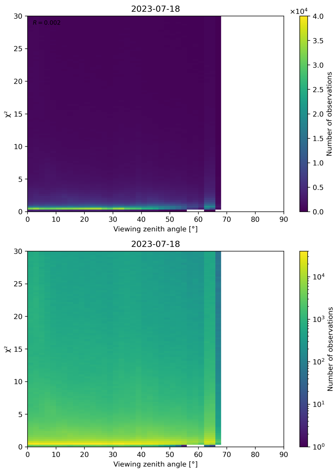
Figure 130: Scatter density plot of “Viewing zenith angle” against “ \chi^2 ” for 2023-07-17 to 2023-07-19.
