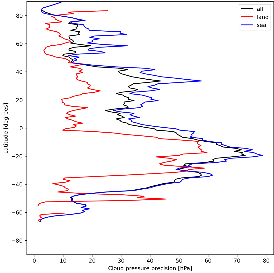
Figure 14: Zonal average of “Cloud pressure precision” for 2023-07-17 to 2023-07-19.
