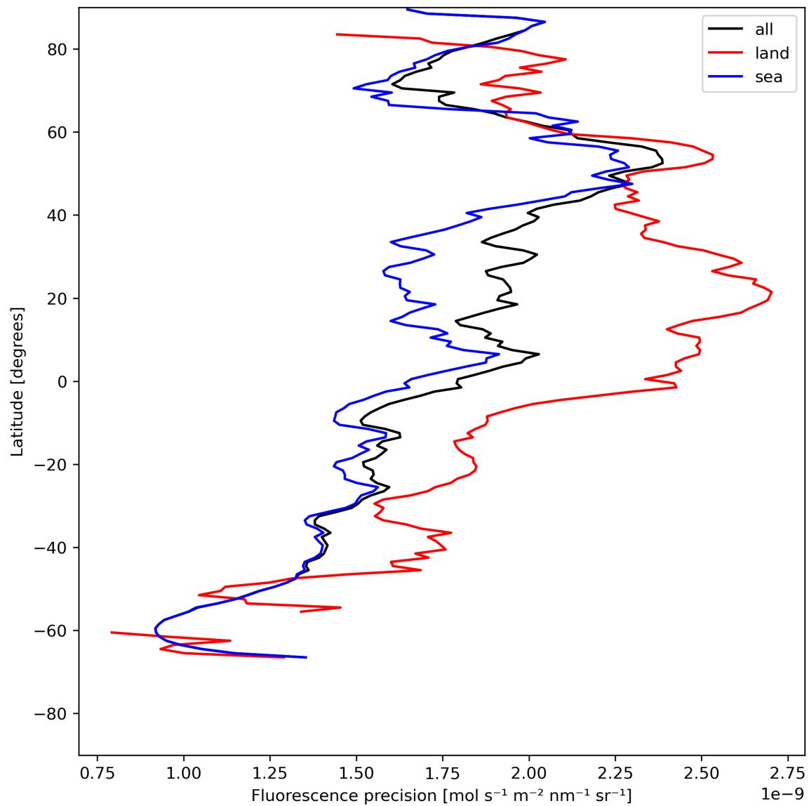
Figure 24: Zonal average of “Fluorescence precision” for 2023-07-17 to 2023-07-19.
