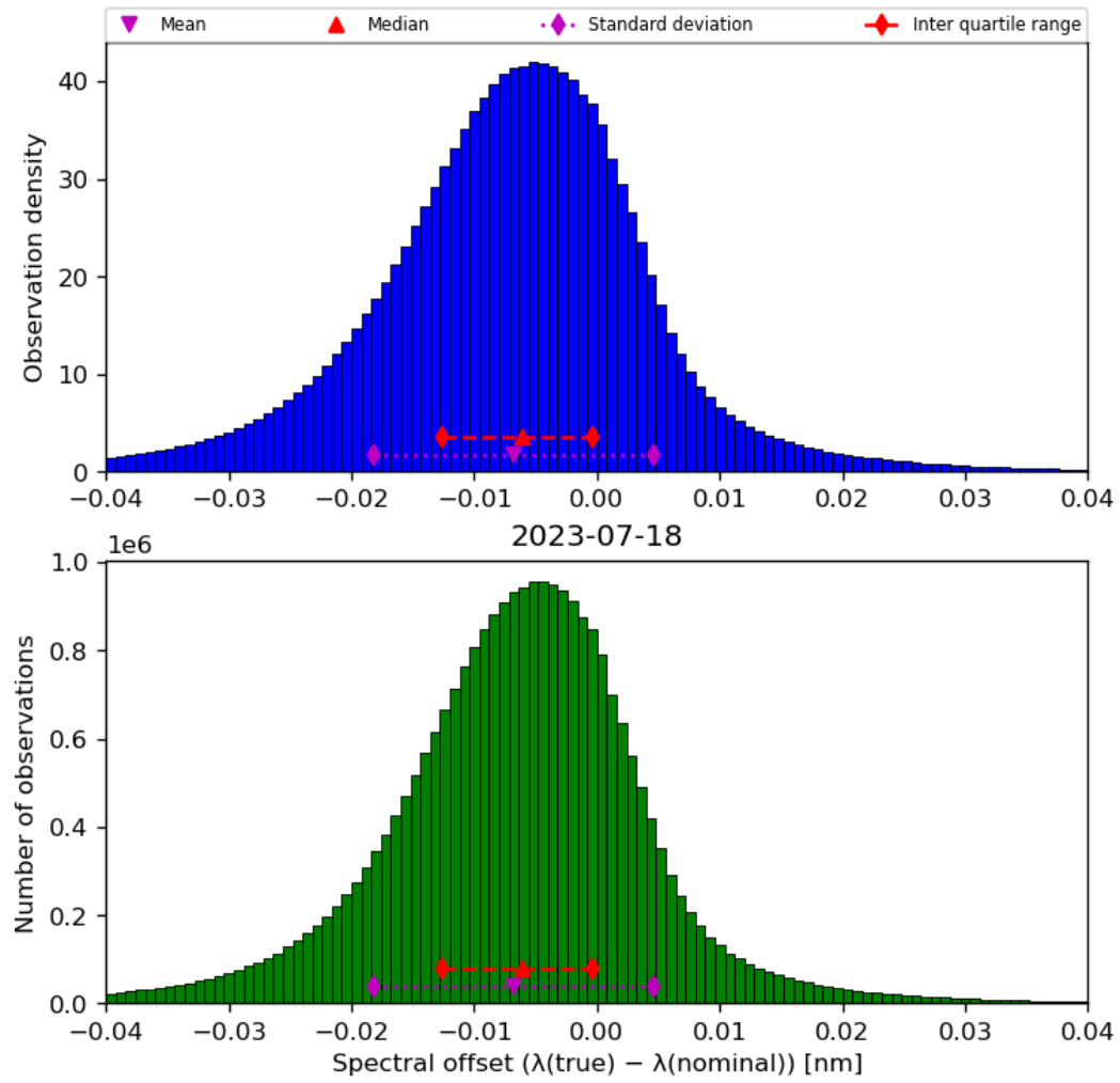
Figure 45: Histogram of “Spectral offset ( \lambda(\text{true}) - \lambda(\text{nominal}) )” for 2023-07-17 to 2023-07-19
