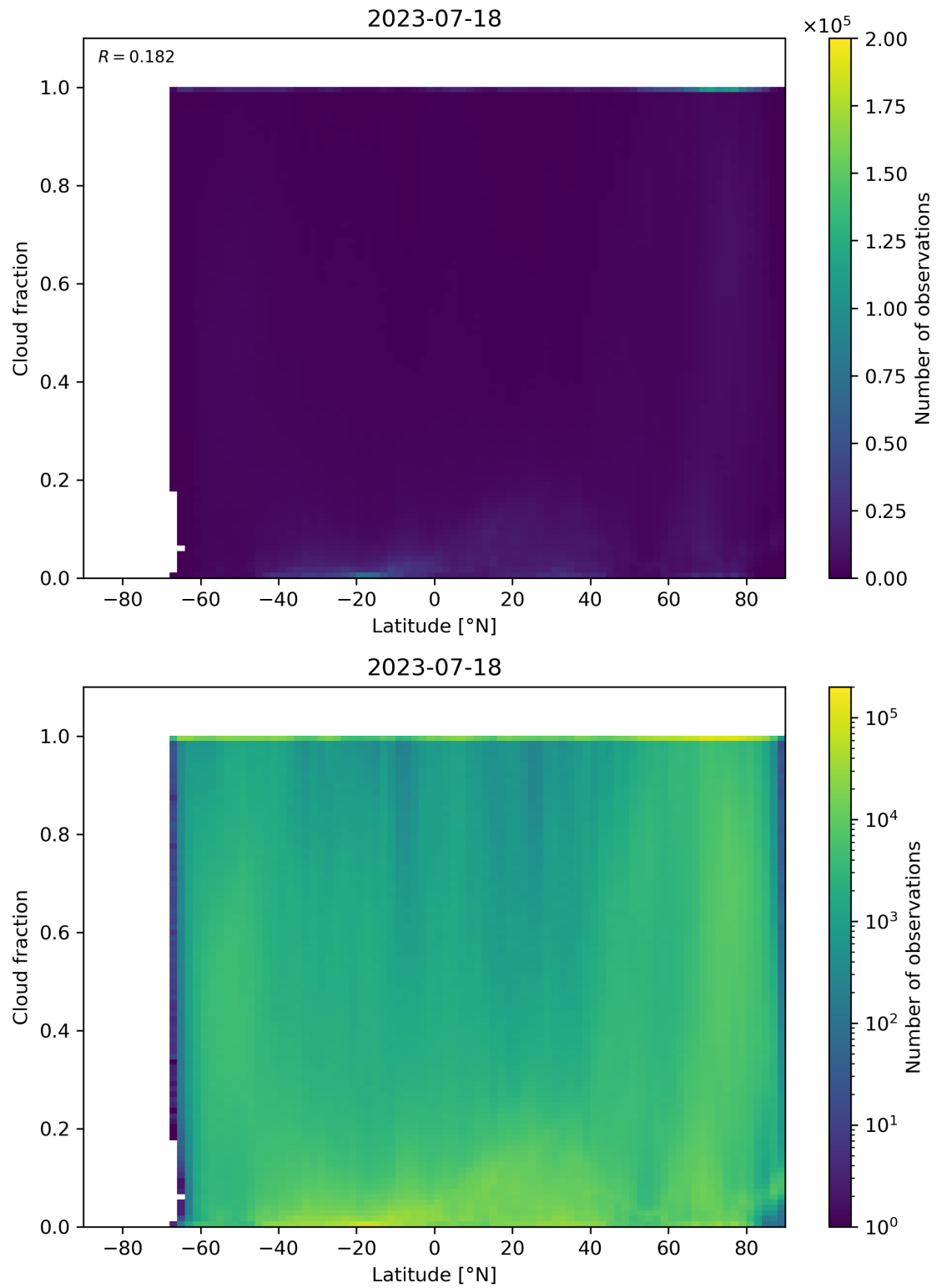
Figure 99: Scatter density plot of “Latitude” against “Cloud fraction” for 2023-07-17 to 2023-07-19.
