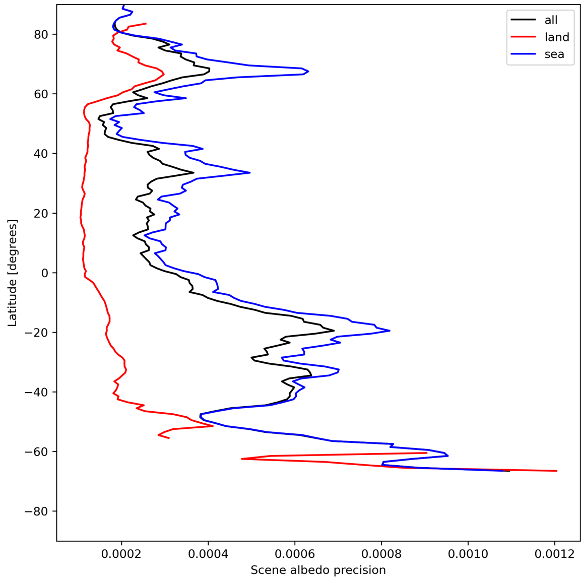
Figure 18: Zonal average of “Scene albedo precision” for 2023-07-17 to 2023-07-19.
