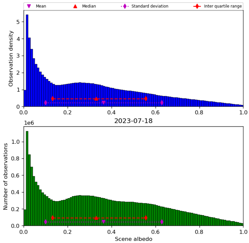
Figure 34: Histogram of “Scene albedo” for 2023-07-17 to 2023-07-19
