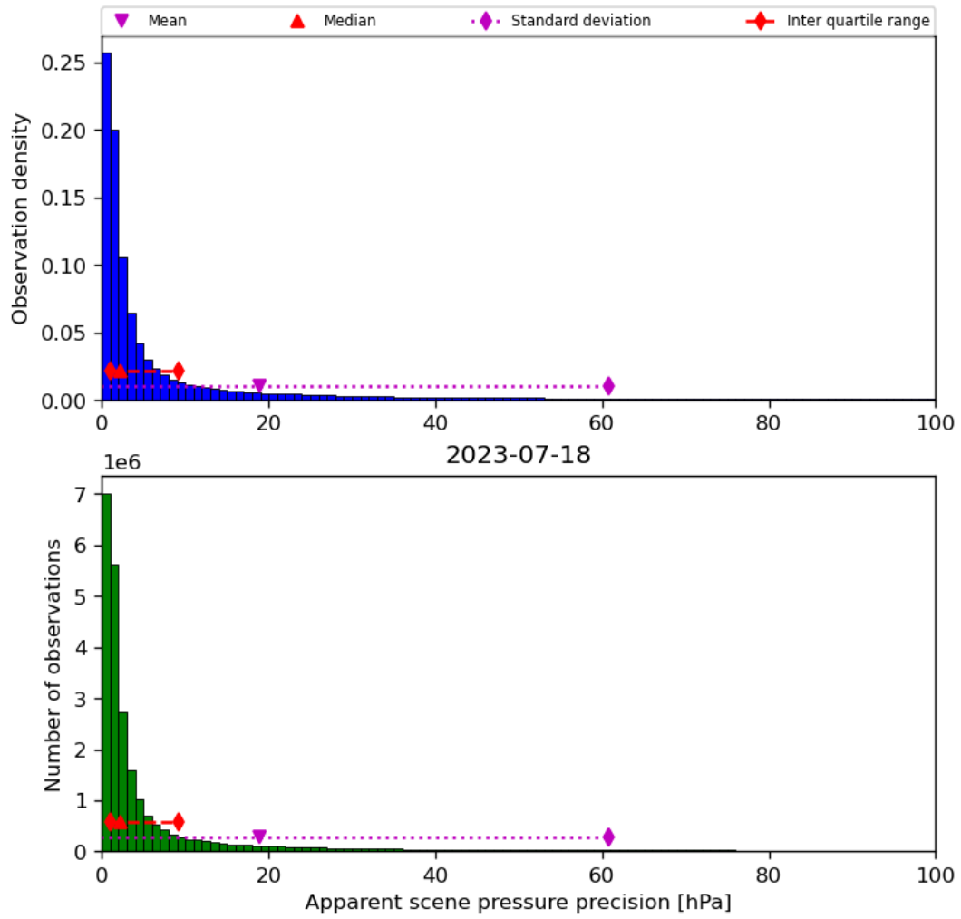
Figure 37: Histogram of “Apparent scene pressure precision” for 2023-07-17 to 2023-07-19
