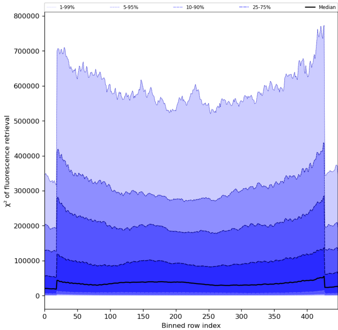
Figure 59: Along track statistics of “ \chi^2 of fluorescence retrieval” for 2023-07-17 to 2023-07-19
