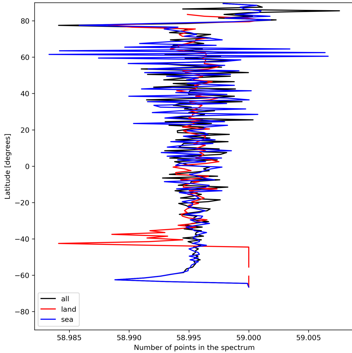
Figure 27: Zonal average of “Number of points in the spectrum” for 2023-07-17 to 2023-07-19.
