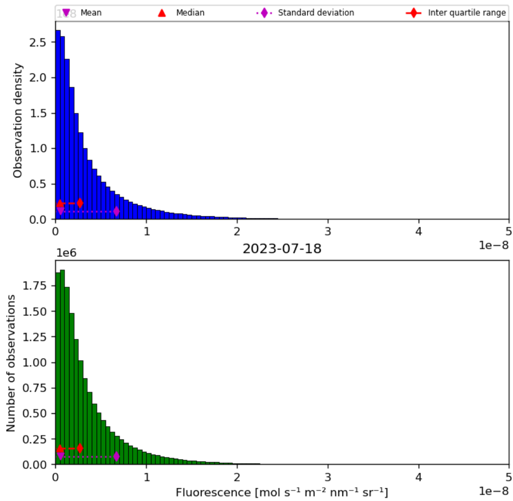
Figure 40: Histogram of “Fluorescence” for 2023-07-17 to 2023-07-19
