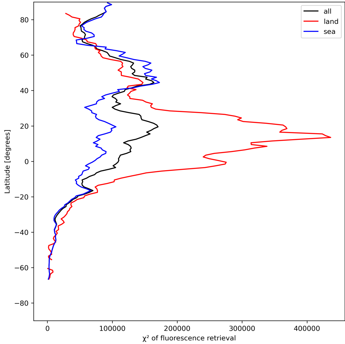
Figure 25: Zonal average of “ \chi^2 of fluorescence retrieval” for 2023-07-17 to 2023-07-19.
