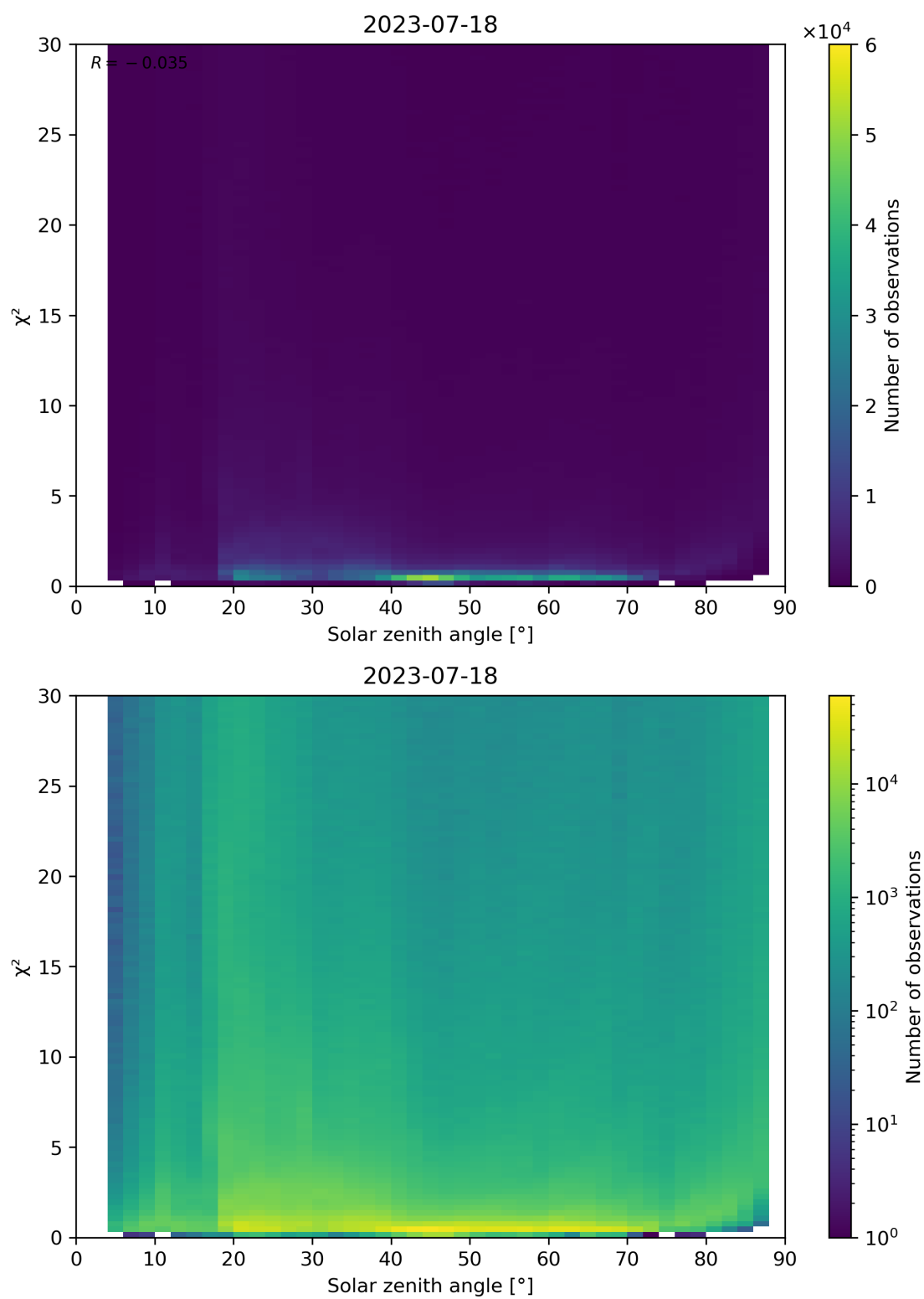
Figure 119: Scatter density plot of “Solar zenith angle” against “ \chi^2 ” for 2023-07-17 to 2023-07-19.
