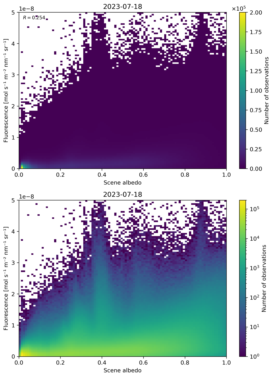
Figure 114: Scatter density plot of “Scene albedo” against “Fluorescence” for 2023-07-17 to 2023-07-19.
