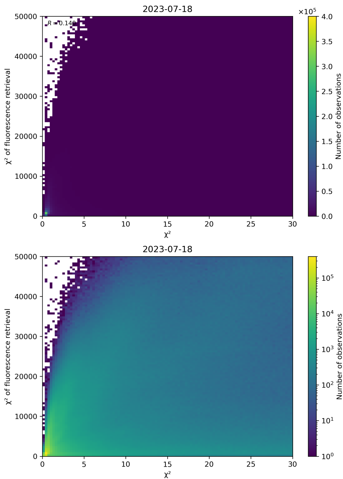
Figure 69: Scatter density plot of “ \chi^2 ” against “ \chi^2 of fluorescence retrieval” for 2023-07-17 to 2023-07-19.
