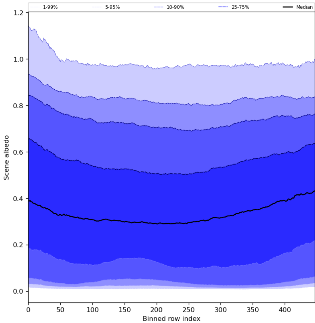
Figure 51: Along track statistics of “Scene albedo” for 2023-07-17 to 2023-07-19
