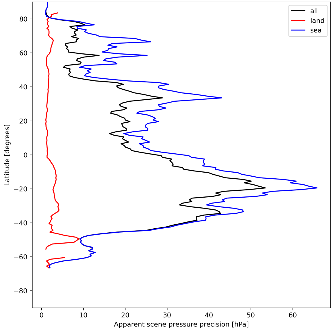
Figure 20: Zonal average of “Apparent scene pressure precision” for 2023-07-17 to 2023-07-19.
