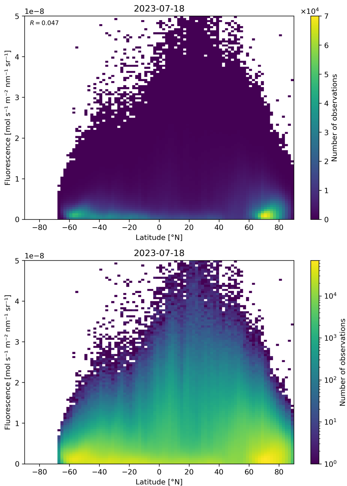
Figure 101: Scatter density plot of “Latitude” against “Fluorescence” for 2023-07-17 to 2023-07-19.
