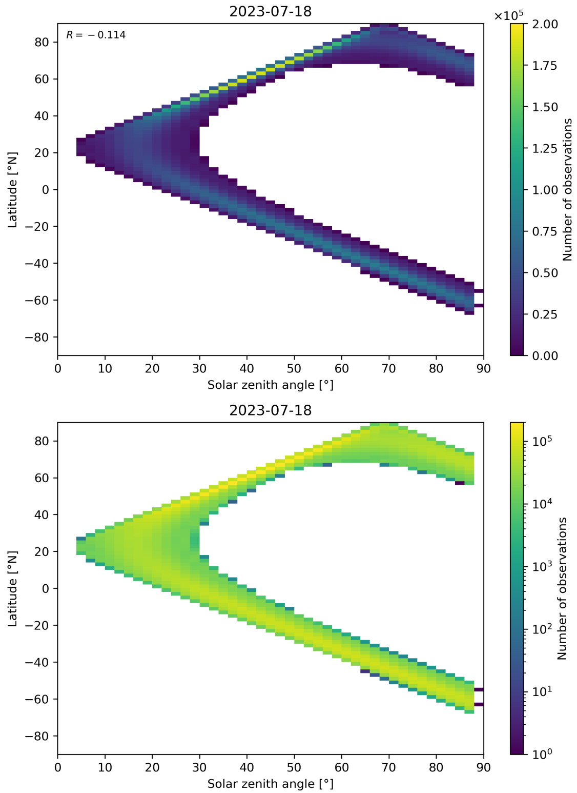
Figure 124: Scatter density plot of “Solar zenith angle” against “Latitude” for 2023-07-17 to 2023-07-19.
