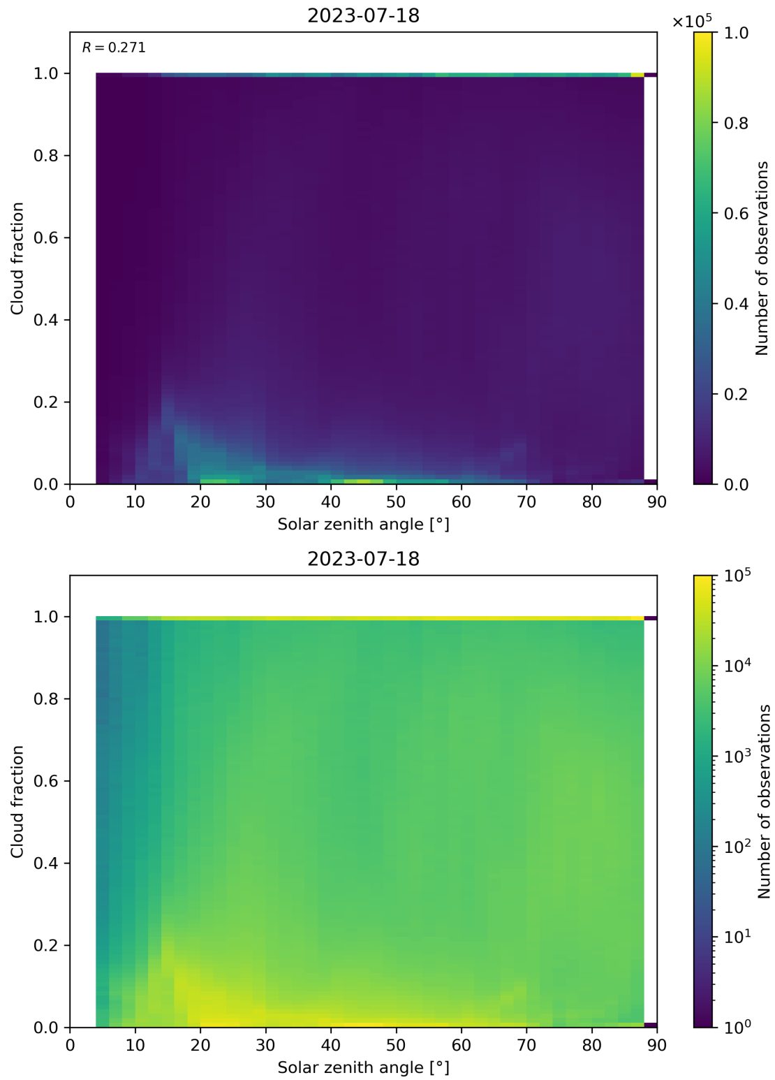
Figure 121: Scatter density plot of “Solar zenith angle” against “Cloud fraction” for 2023-07-17 to 2023-07-19.
