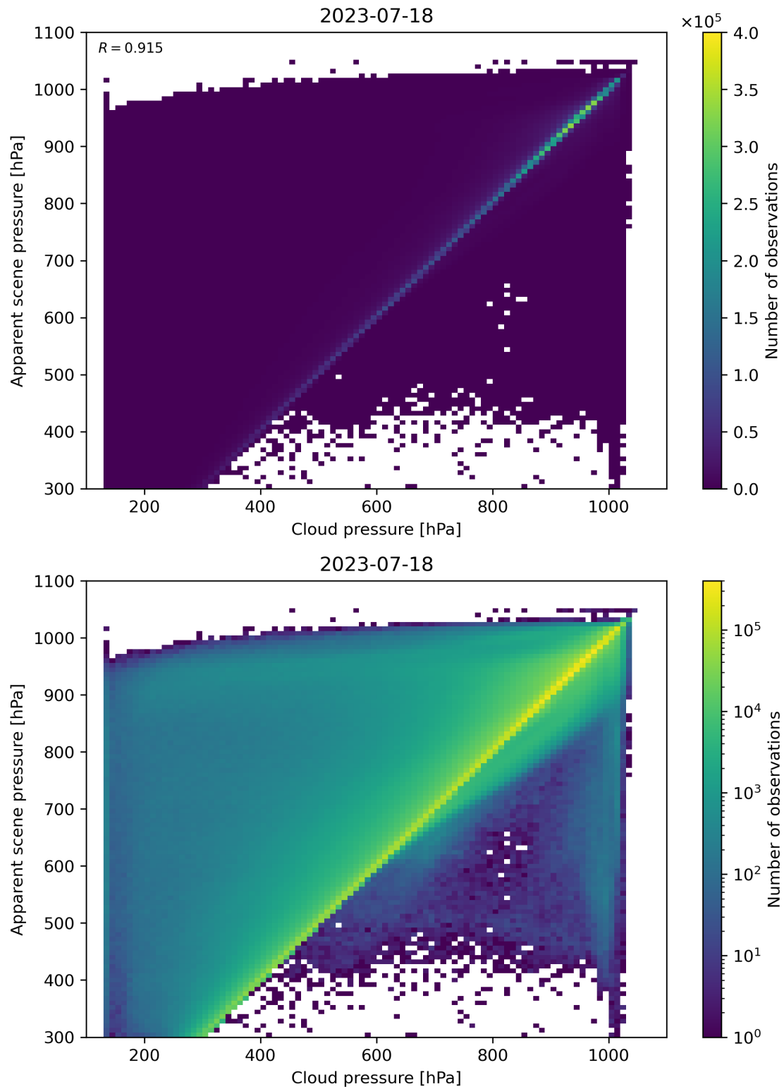
Figure 84: Scatter density plot of “Cloud pressure” against “Apparent scene pressure” for 2023-07-17 to 2023-07-19.
