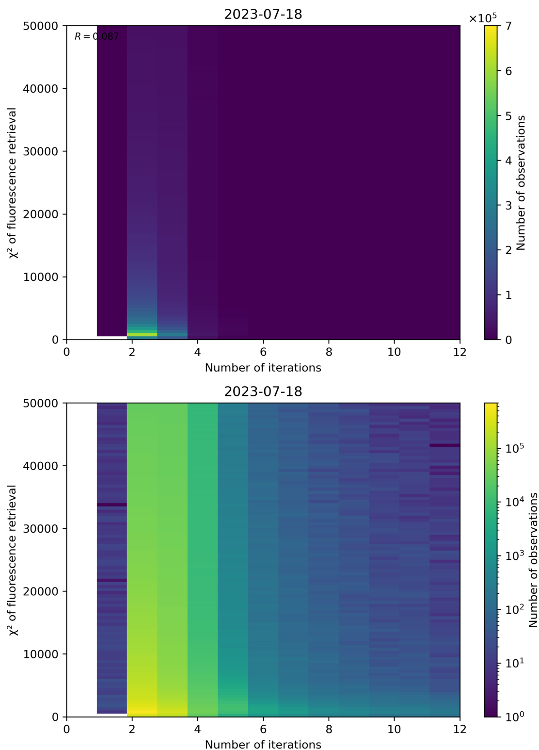
Figure 106: Scatter density plot of “Number of iterations” against “ \chi^2 of fluorescence retrieval” for 2023-07-17 to 2023-07-19.
