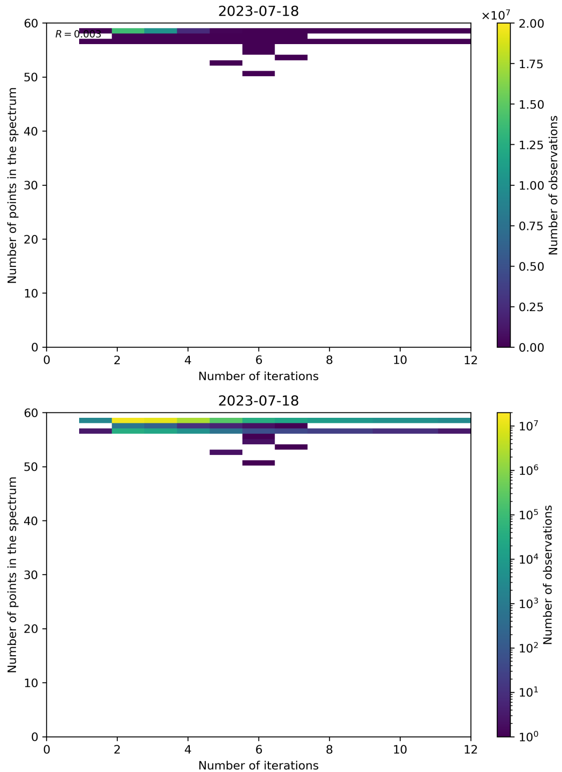
Figure 108: Scatter density plot of “Number of iterations” against “Number of points in the spectrum” for 2023-07-17 to 2023-07-19.
