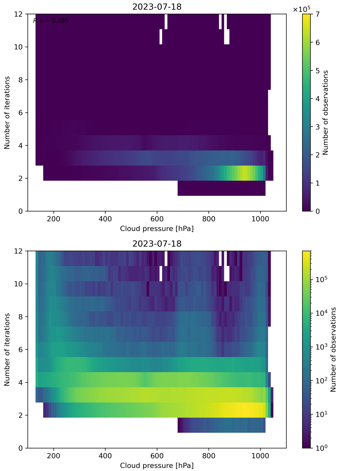
Figure 89: Scatter density plot of “Cloud pressure” against “Number of iterations” for 2023-07-17 to 2023-07-19.
