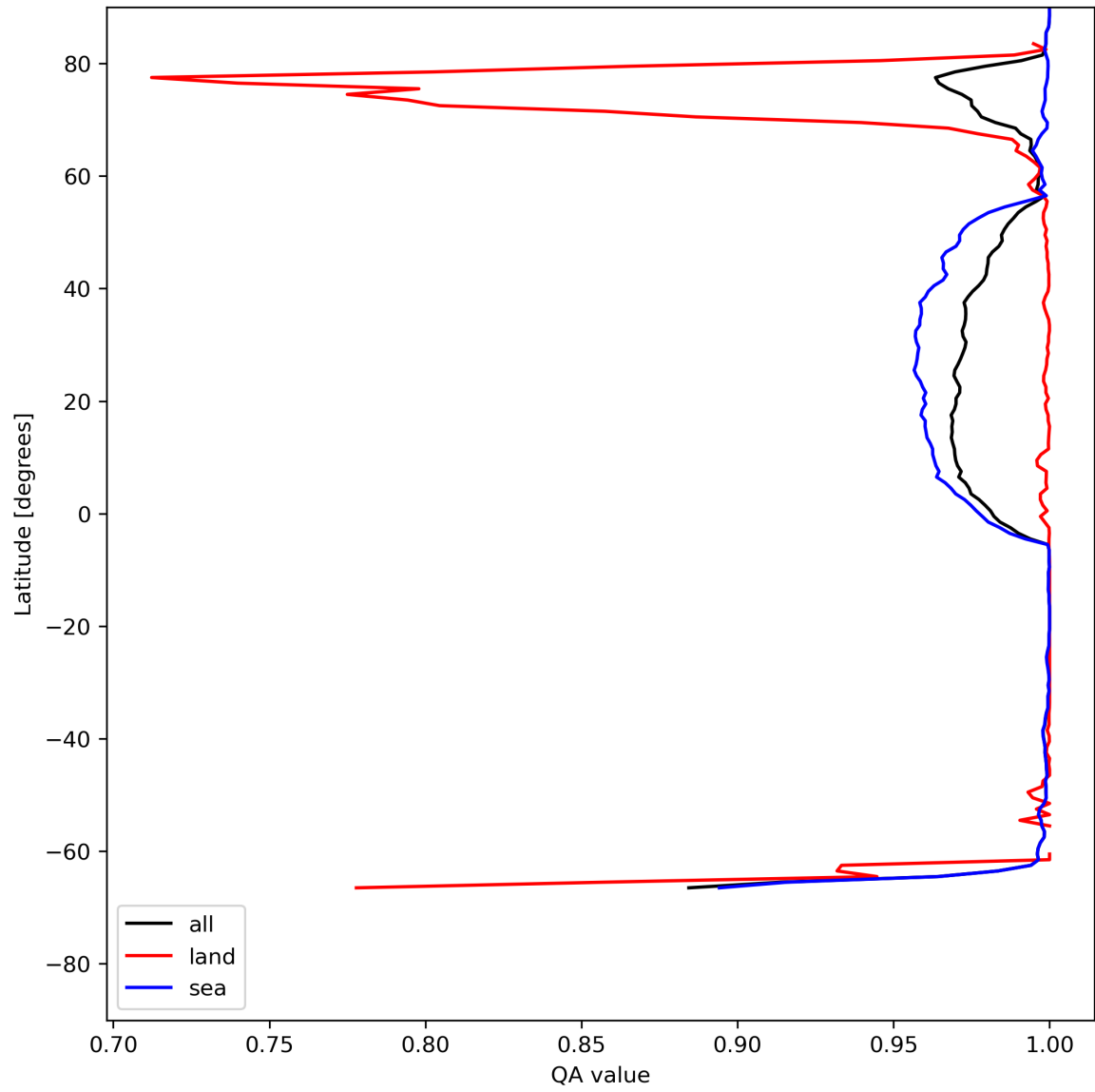
Figure 12: Zonal average of “QA value” for 2023-07-17 to 2023-07-19.
