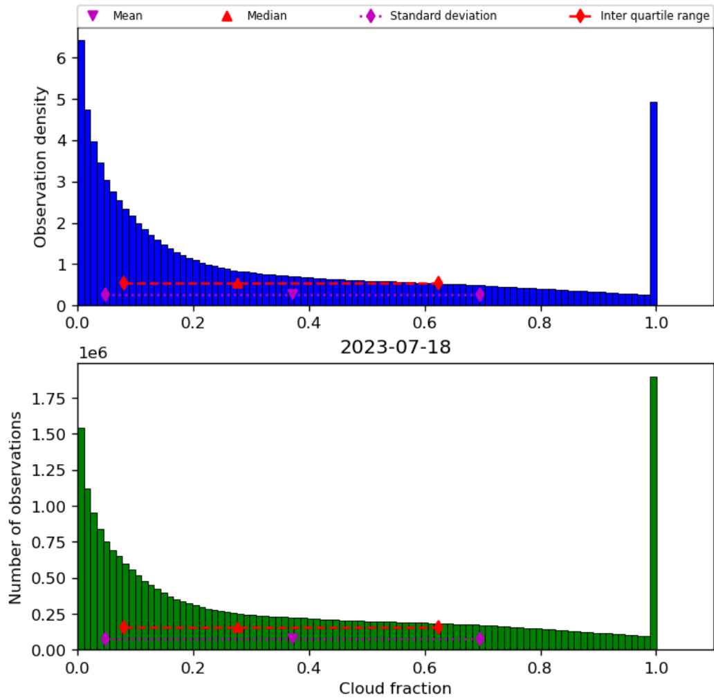
Figure 32: Histogram of “Cloud fraction” for 2023-07-17 to 2023-07-19
