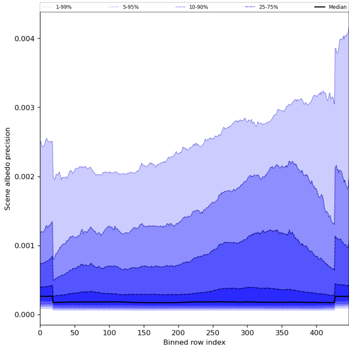
Figure 52: Along track statistics of “Scene albedo precision” for 2023-07-17 to 2023-07-19
