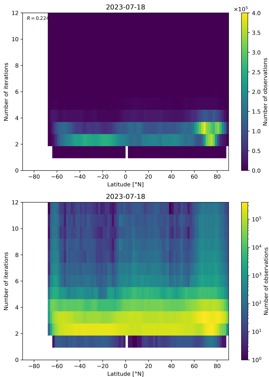
Figure 102: Scatter density plot of “Latitude” against “Number of iterations” for 2023-07-17 to 2023-07-19.
