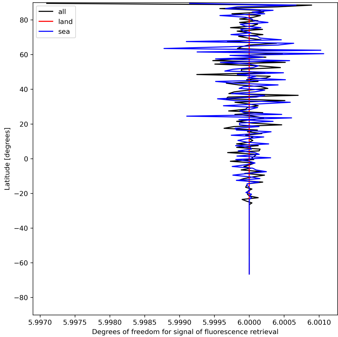
Figure 26: Zonal average of “Degrees of freedom for signal of fluorescence retrieval” for 2023-07-17 to 2023-07-19.
