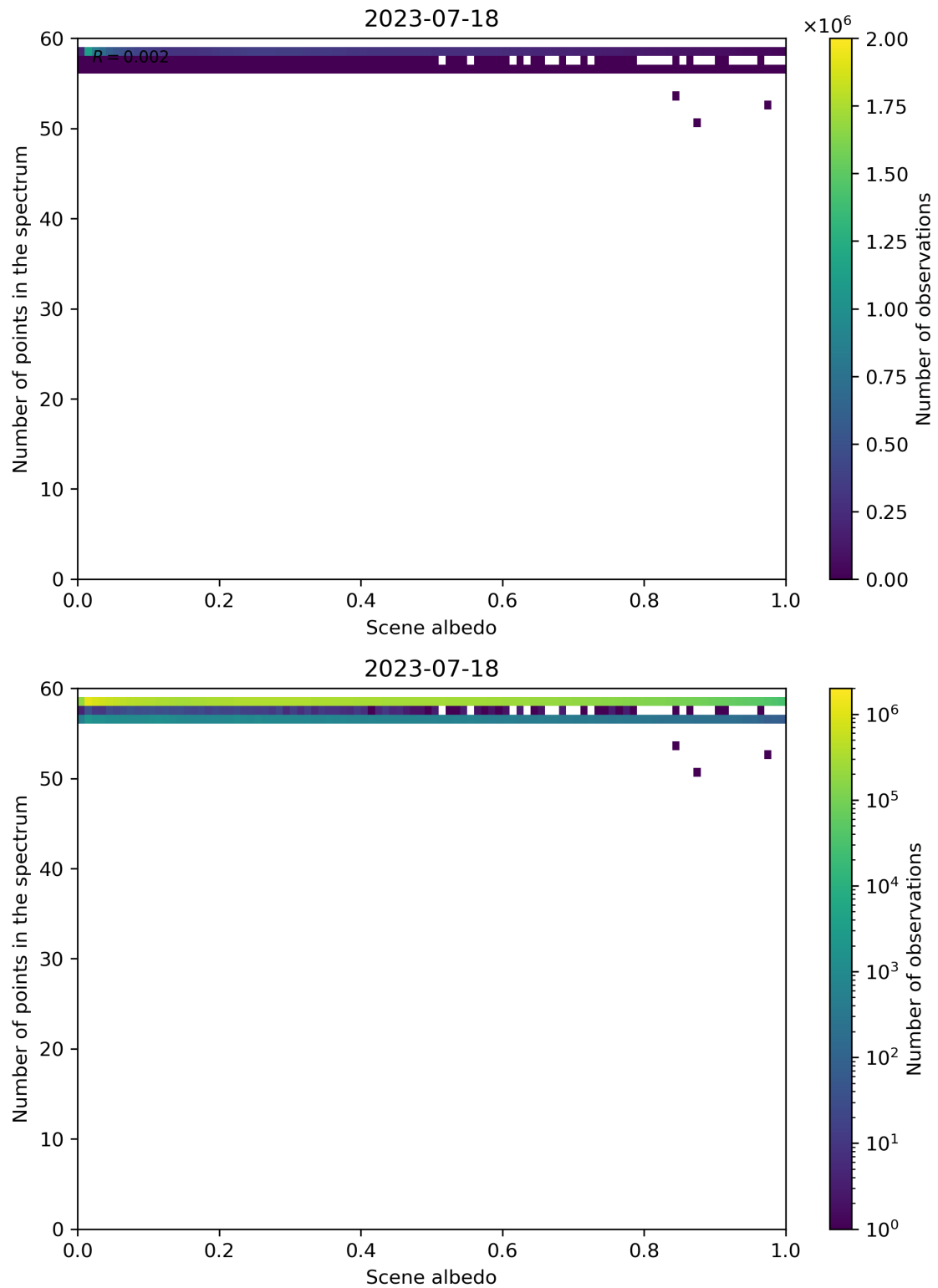
Figure 116: Scatter density plot of “Scene albedo” against “Number of points in the spectrum” for 2023-07-17 to 2023-07-19.
