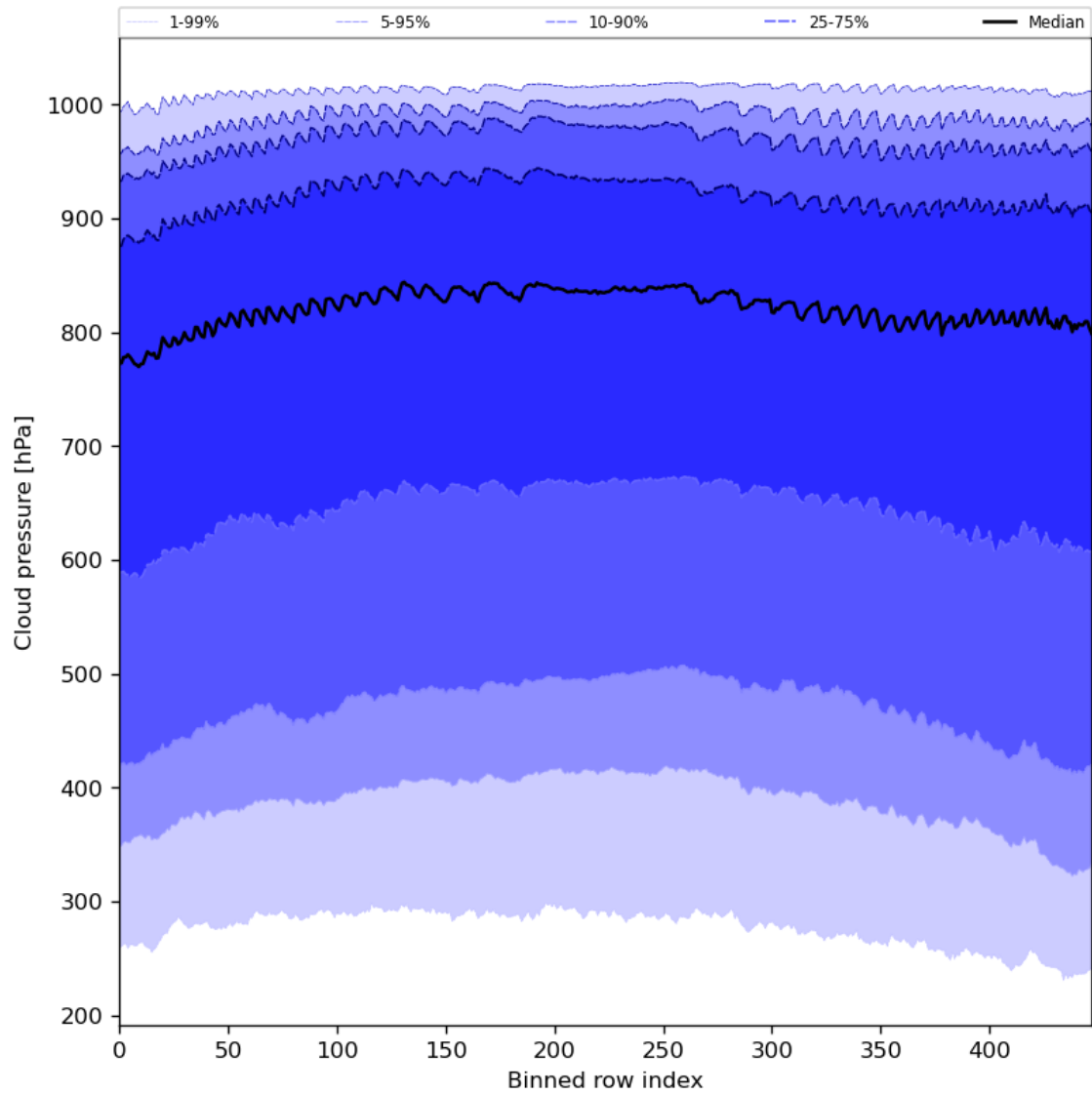
Figure 47: Along track statistics of “Cloud pressure” for 2023-07-17 to 2023-07-19
