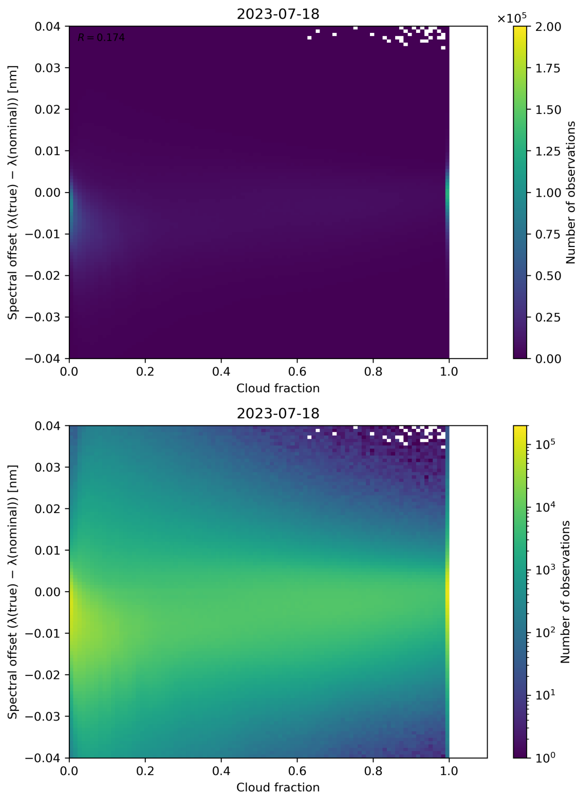
Figure 83: Scatter density plot of “Cloud fraction” against “Spectral offset ( \lambda(\text{true}) - \lambda(\text{nominal}) )” for 2023-07-17 to 2023-07-19.
