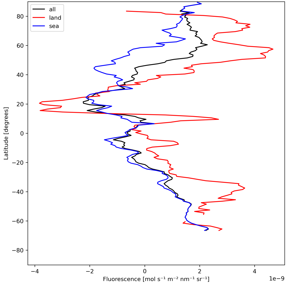
Figure 23: Zonal average of “Fluorescence” for 2023-07-17 to 2023-07-19.
