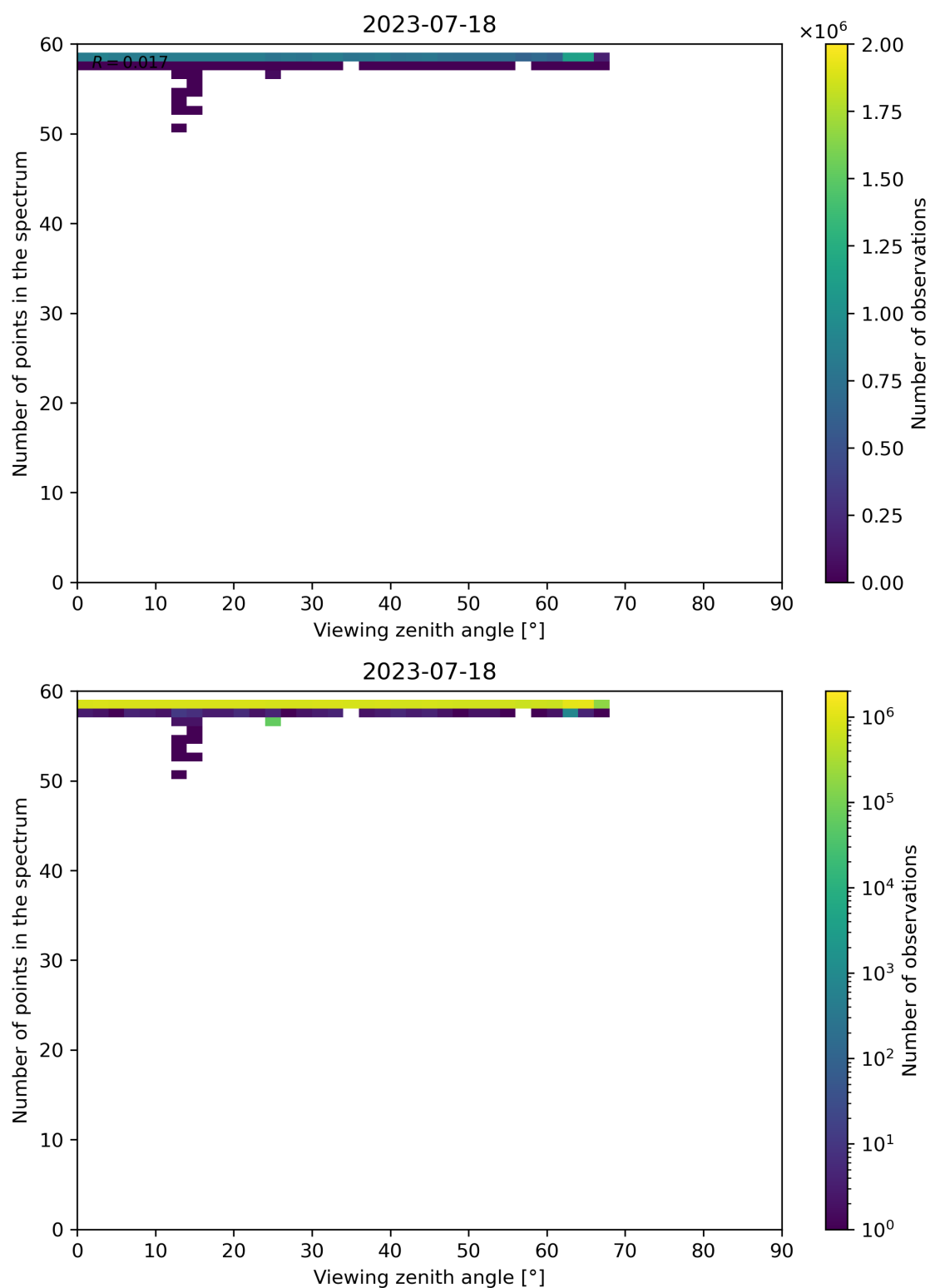
Figure 137: Scatter density plot of “Viewing zenith angle” against “Number of points in the spectrum” for 2023-07-17 to 2023-07-19.
