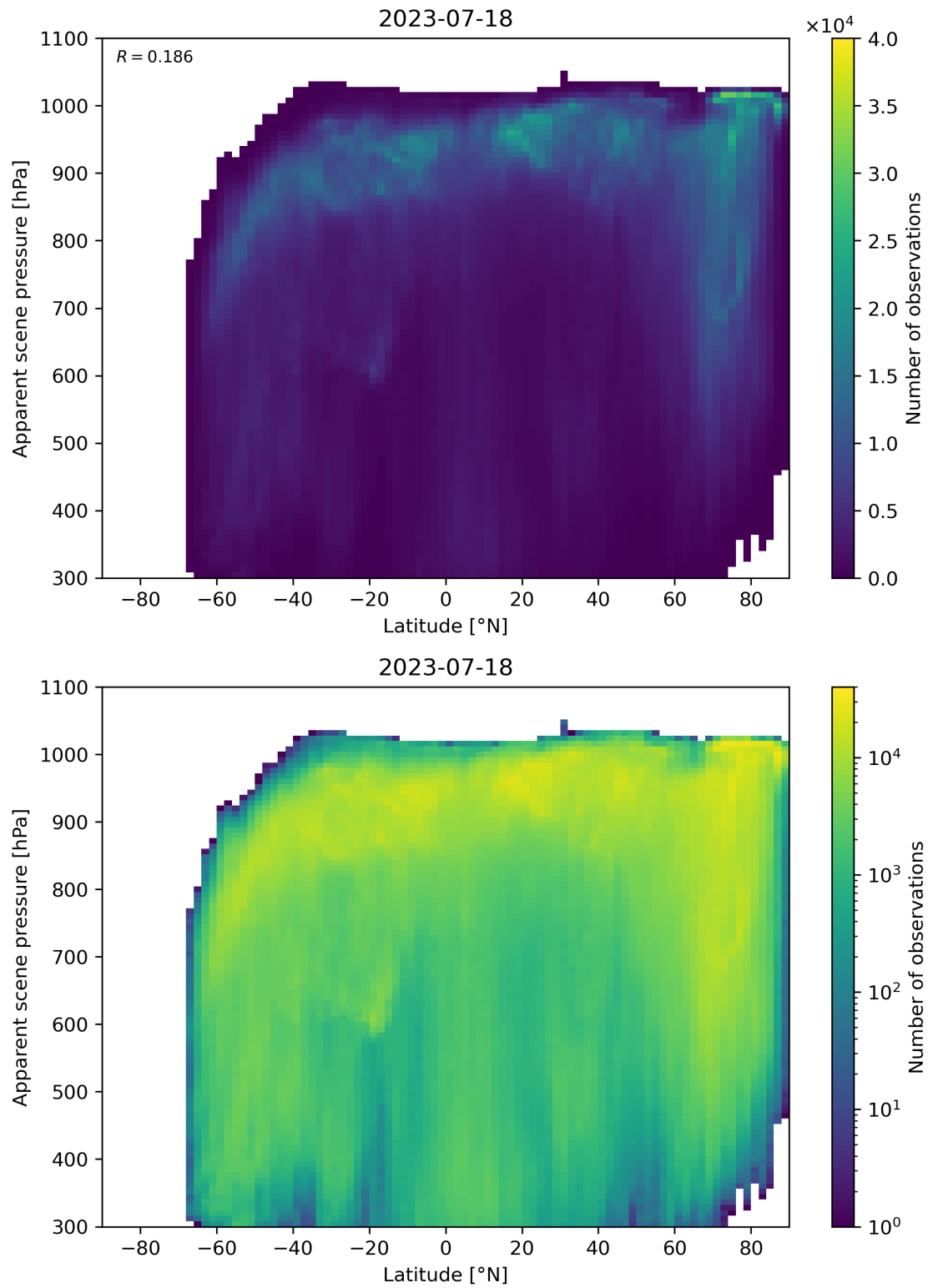
Figure 96: Scatter density plot of “Latitude” against “Apparent scene pressure” for 2023-07-17 to 2023-07-19.
