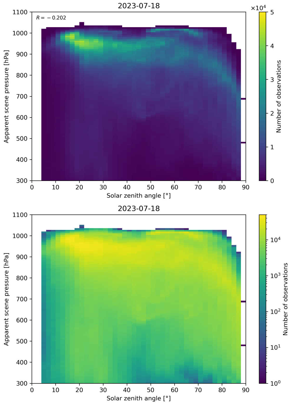
Figure 118: Scatter density plot of “Solar zenith angle” against “Apparent scene pressure” for 2023-07-17 to 2023-07-19.
