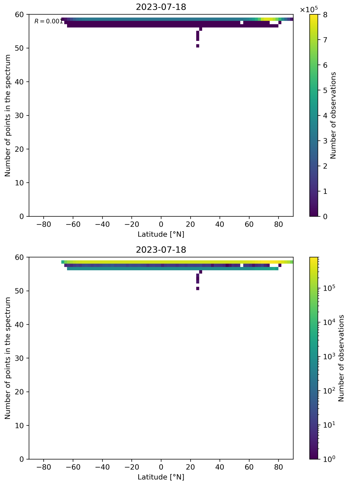
Figure 103: Scatter density plot of “Latitude” against “Number of points in the spectrum” for 2023-07-17 to 2023-07-19.
