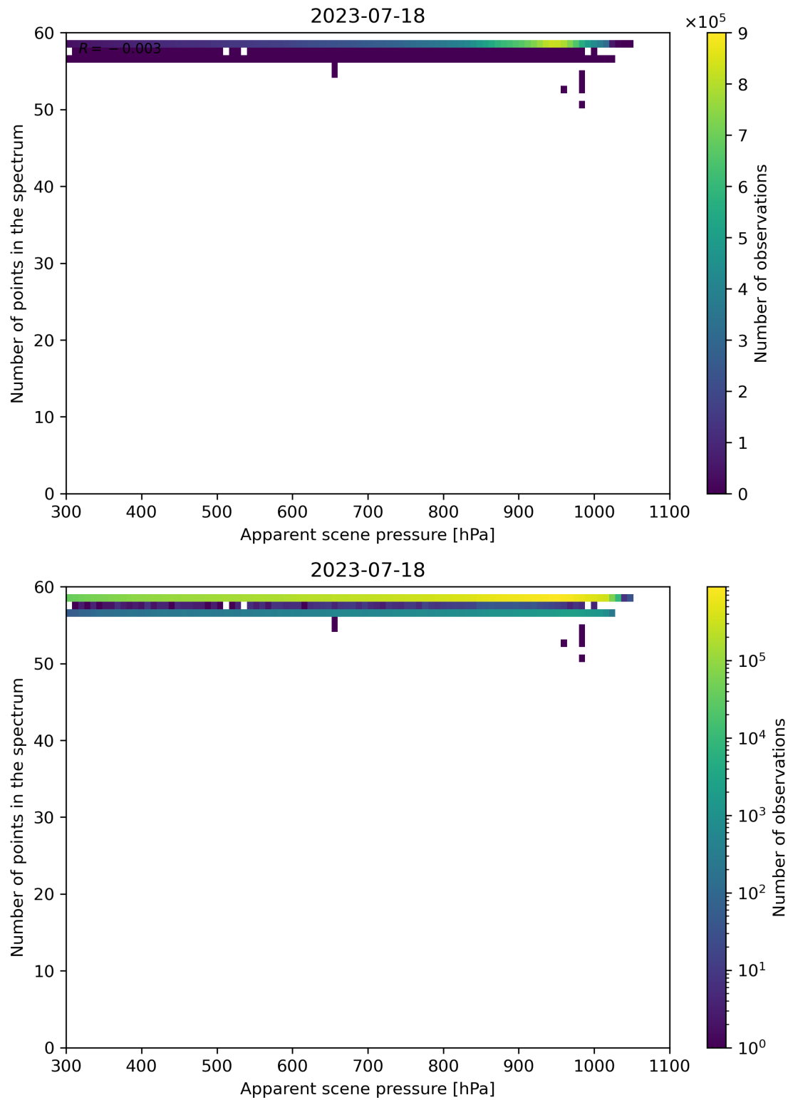
Figure 67: Scatter density plot of “Apparent scene pressure” against “Number of points in the spectrum” for 2023-07-17 to 2023-07-19.
