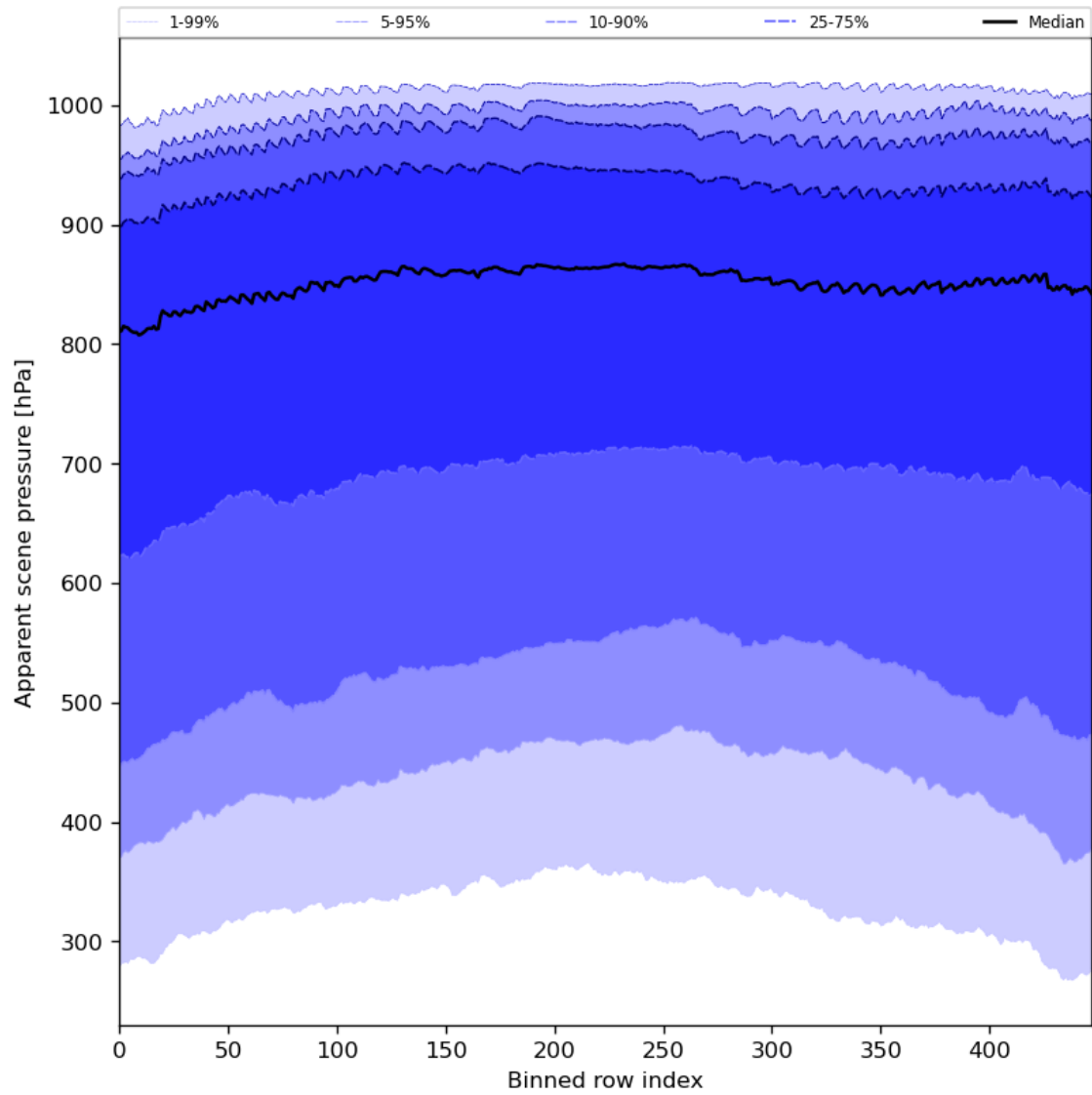
Figure 53: Along track statistics of “Apparent scene pressure” for 2023-07-17 to 2023-07-19
