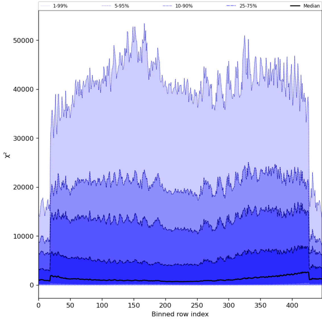
Figure 55: Along track statistics of “ \chi^2 ” for 2023-07-17 to 2023-07-19
