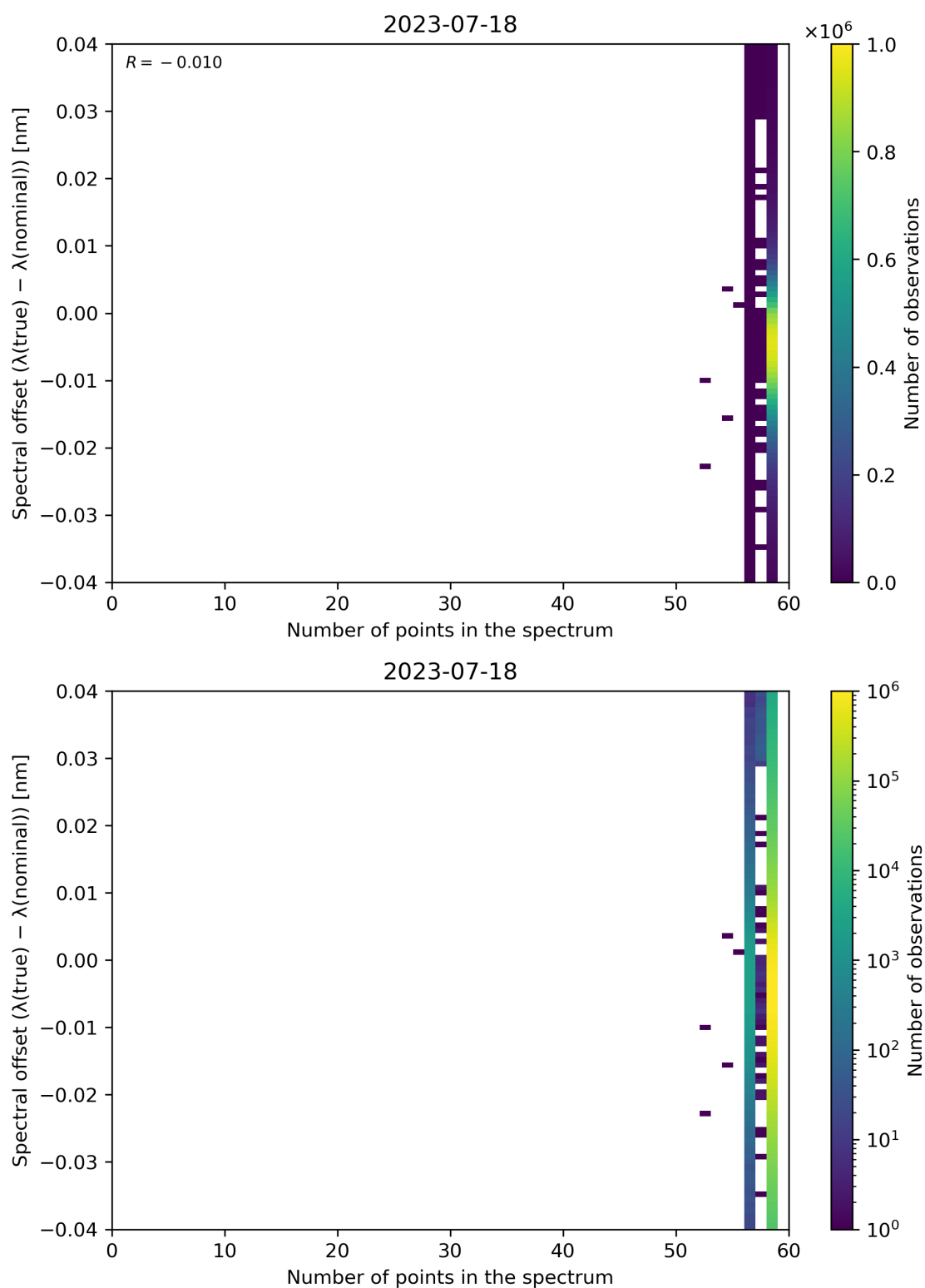
Figure 110: Scatter density plot of “Number of points in the spectrum” against “Spectral offset ( \lambda(\text{true}) - \lambda(\text{nominal}) )” for 2023-07-17 to 2023-07-19.
