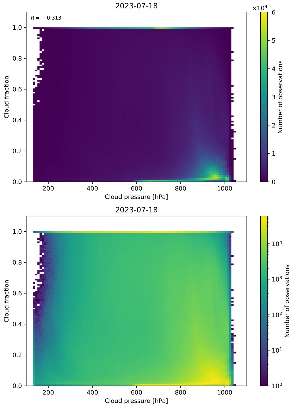
Figure 87: Scatter density plot of “Cloud pressure” against “Cloud fraction” for 2023-07-17 to 2023-07-19.
