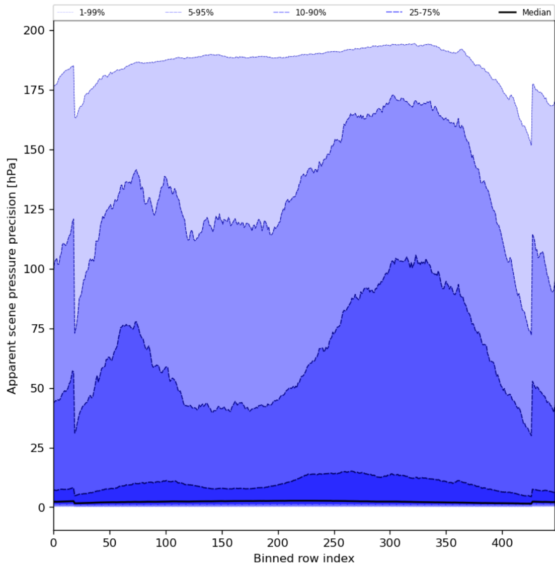
Figure 54: Along track statistics of “Apparent scene pressure precision” for 2023-07-17 to 2023-07-19
