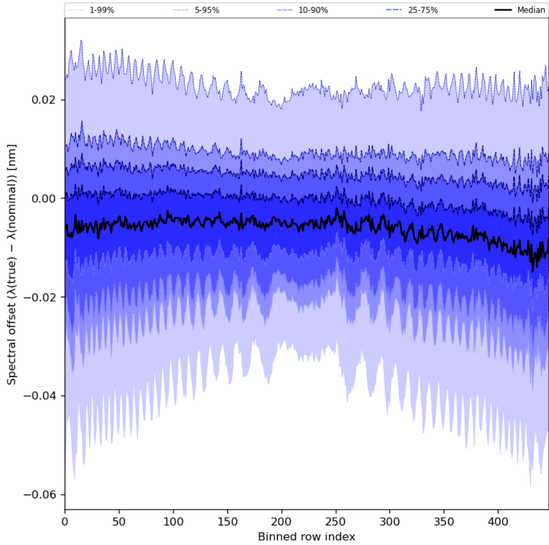
Figure 62: Along track statistics of “Spectral offset ( \lambda(\text{true}) - \lambda(\text{nominal}) )” for 2023-07-17 to 2023-07-19
