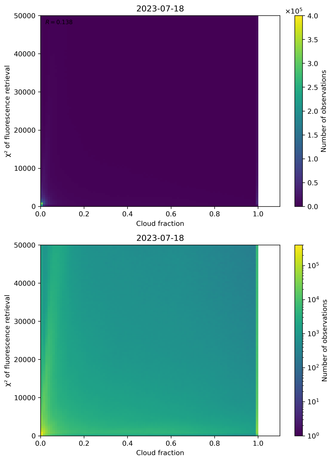
Figure 78: Scatter density plot of “Cloud fraction” against “ \chi^2 of fluorescence retrieval” for 2023-07-17 to 2023-07-19.
