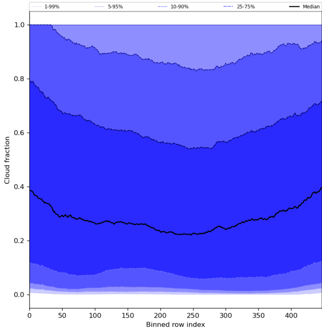
Figure 49: Along track statistics of “Cloud fraction” for 2023-07-17 to 2023-07-19
