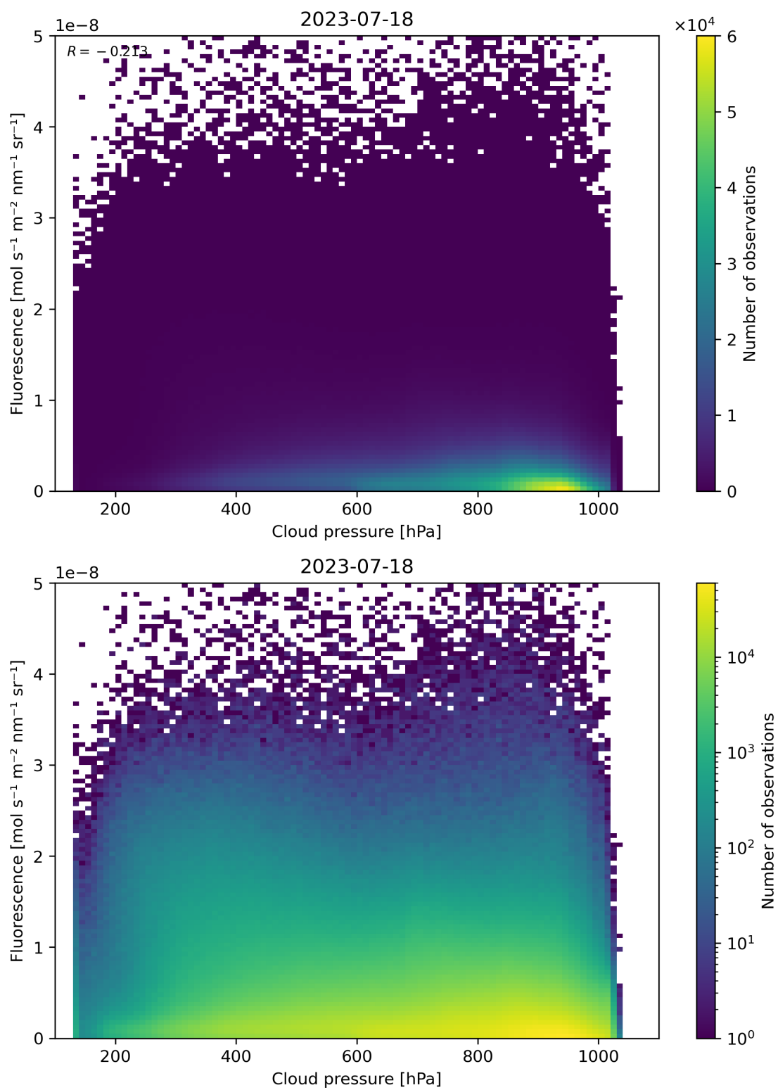
Figure 88: Scatter density plot of “Cloud pressure” against “Fluorescence” for 2023-07-17 to 2023-07-19.
