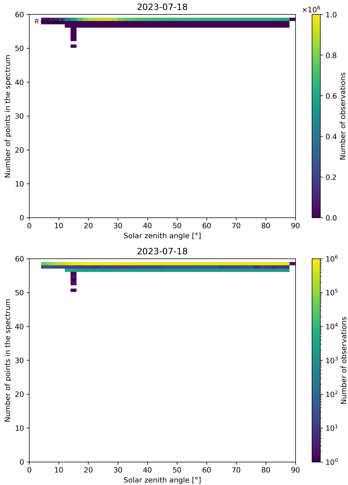
Figure 126: Scatter density plot of “Solar zenith angle” against “Number of points in the spectrum” for 2023-07-17 to 2023-07-19.
