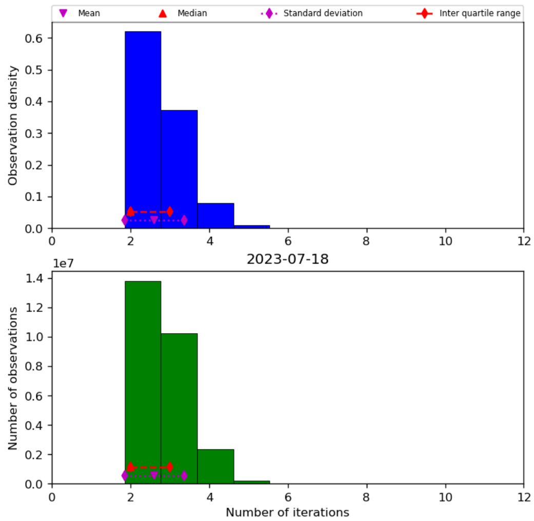
Figure 39: Histogram of “Number of iterations” for 2023-07-17 to 2023-07-19
