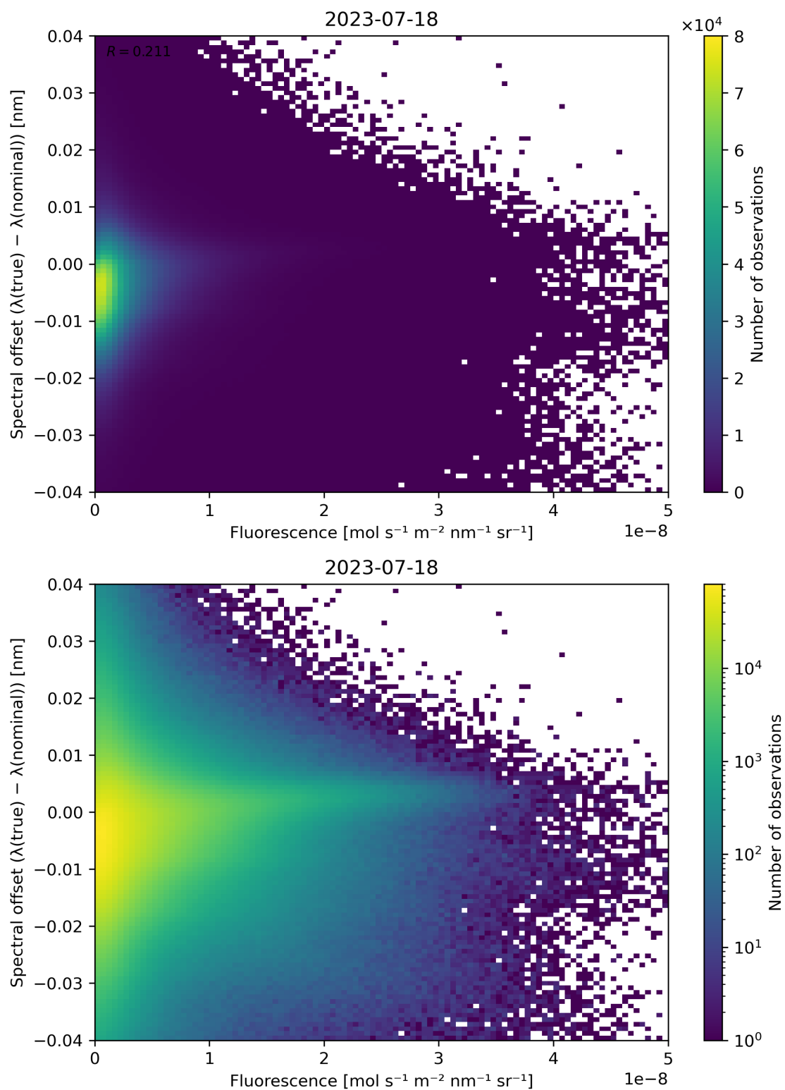
Figure 95: Scatter density plot of “Fluorescence” against “Spectral offset ( \lambda(\text{true}) - \lambda(\text{nominal}) )” for 2023-07-17 to 2023-07-19.
