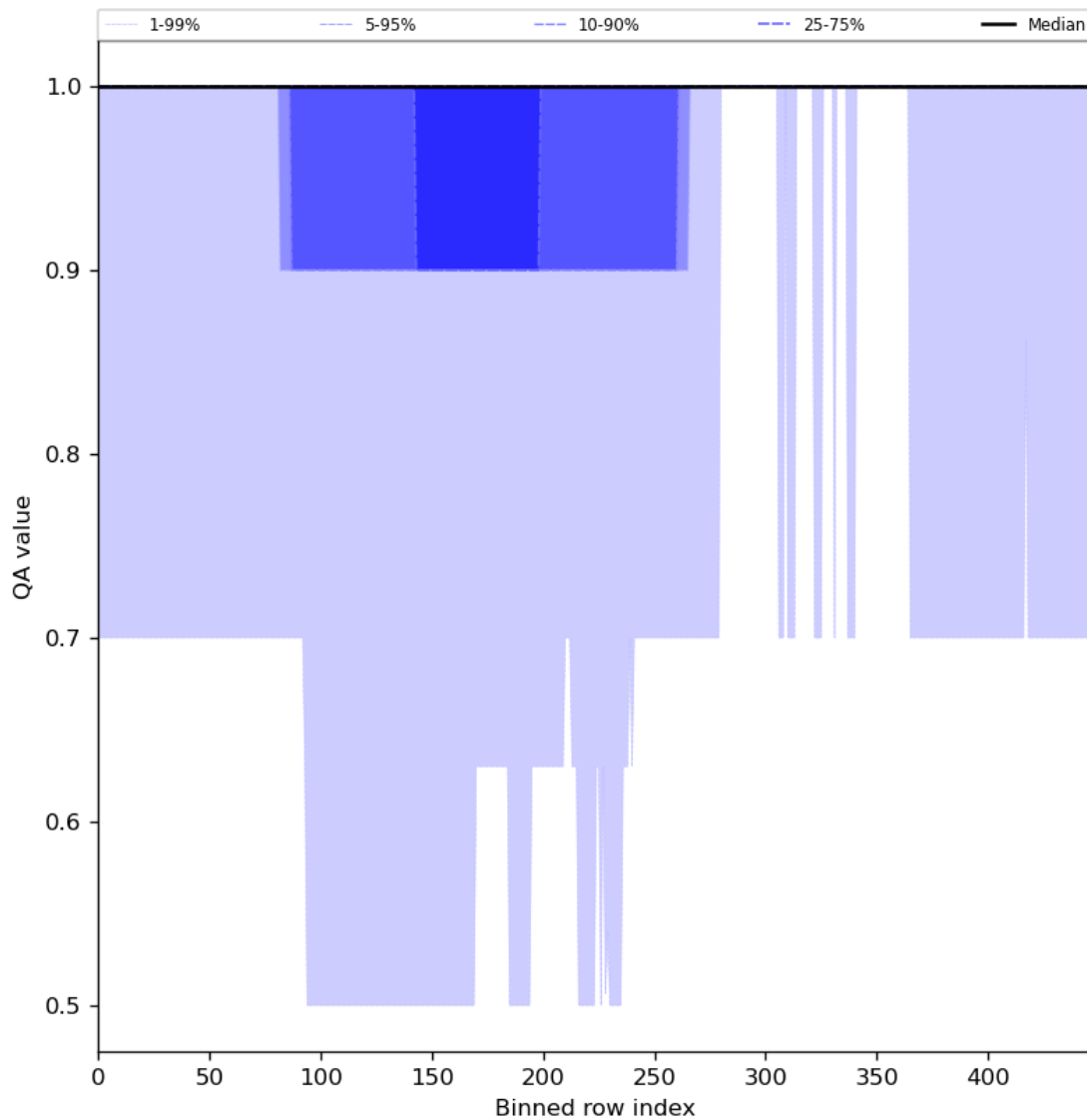
Figure 46: Along track statistics of “QA value” for 2023-07-17 to 2023-07-19
