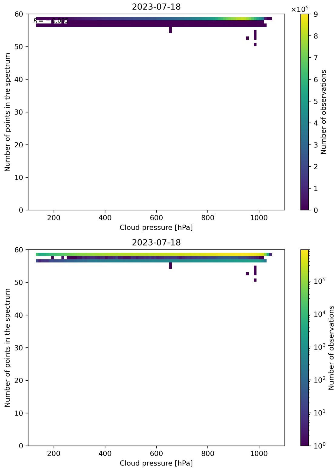
Figure 90: Scatter density plot of “Cloud pressure” against “Number of points in the spectrum” for 2023-07-17 to 2023-07-19.
