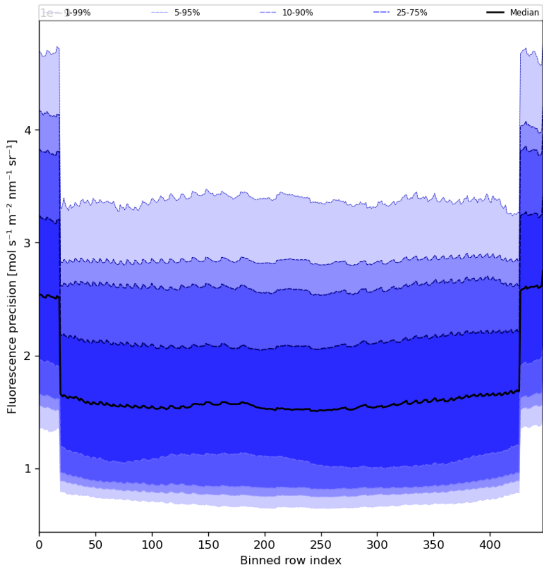
Figure 58: Along track statistics of “Fluorescence precision” for 2023-07-17 to 2023-07-19
