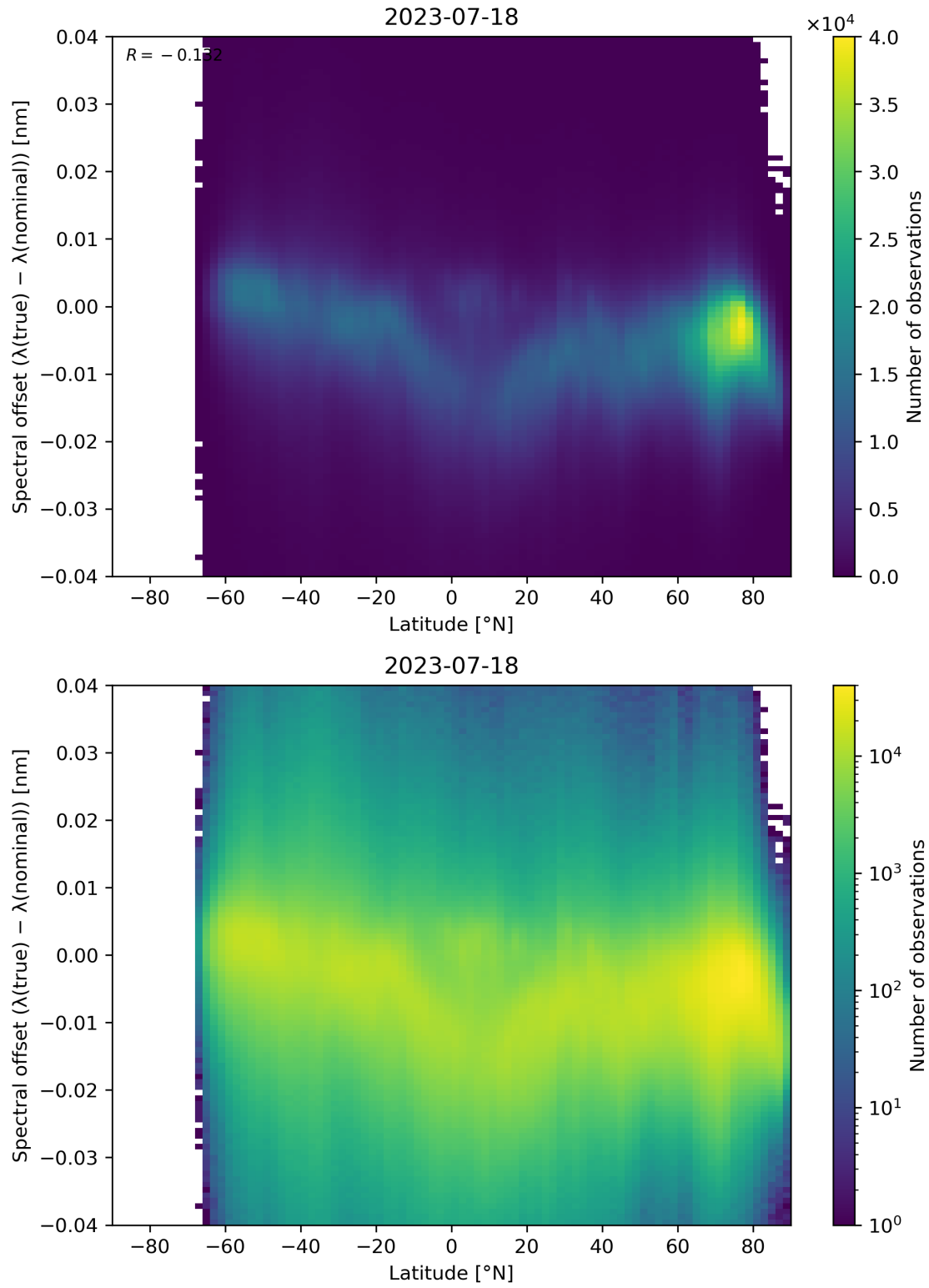
Figure 105: Scatter density plot of “Latitude” against “Spectral offset ( \lambda(\text{true}) - \lambda(\text{nominal}) )” for 2023-07-17 to 2023-07-19.
