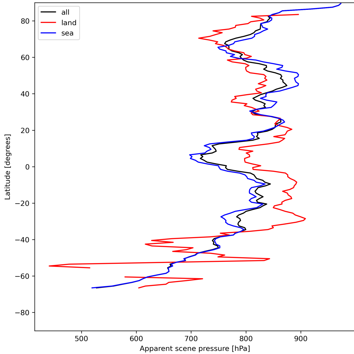
Figure 19: Zonal average of “Apparent scene pressure” for 2023-07-17 to 2023-07-19.
