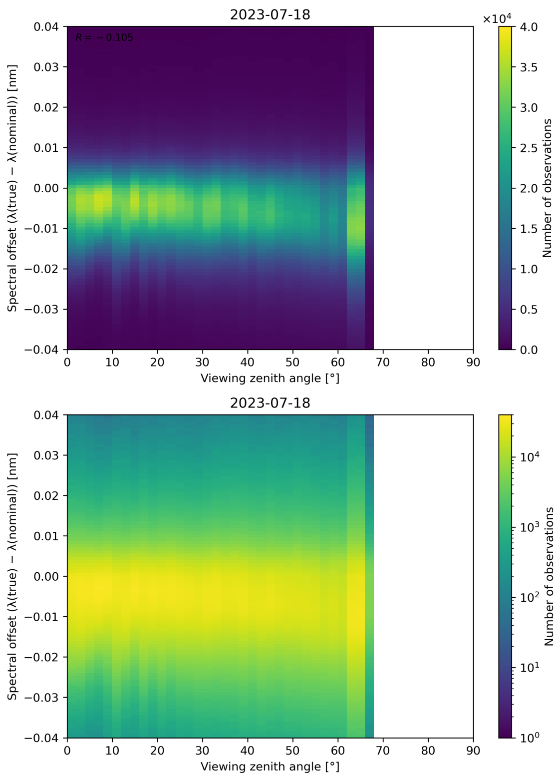
Figure 140: Scatter density plot of “Viewing zenith angle” against “Spectral offset ( \lambda(\text{true}) - \lambda(\text{nominal}) )” for 2023-07-17 to 2023-07-19.
