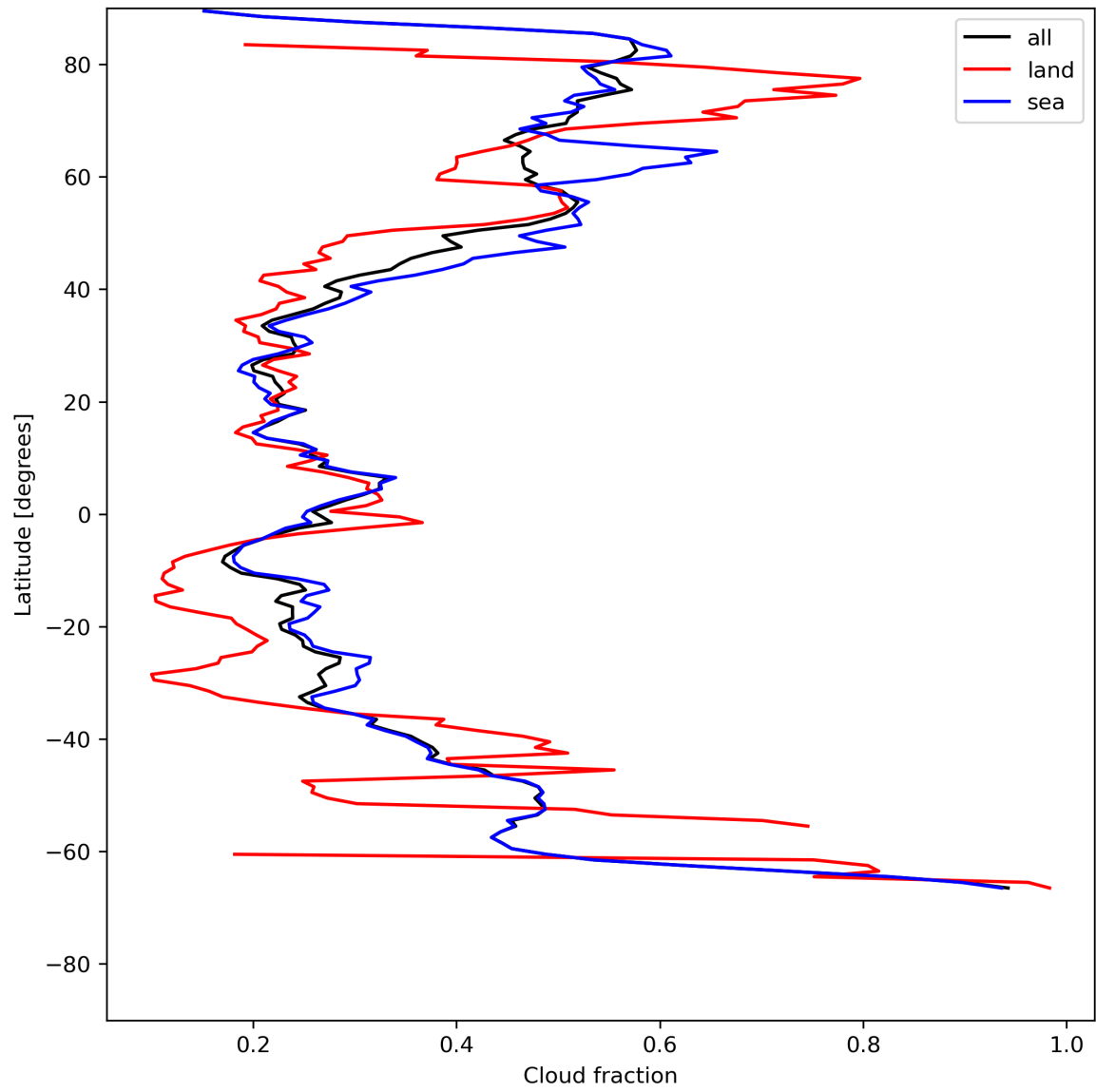
Figure 15: Zonal average of “Cloud fraction” for 2023-07-17 to 2023-07-19.
