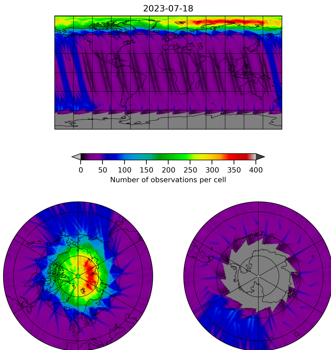
Figure 11: Map of the number of observations for 2023-07-17 to 2023-07-19
