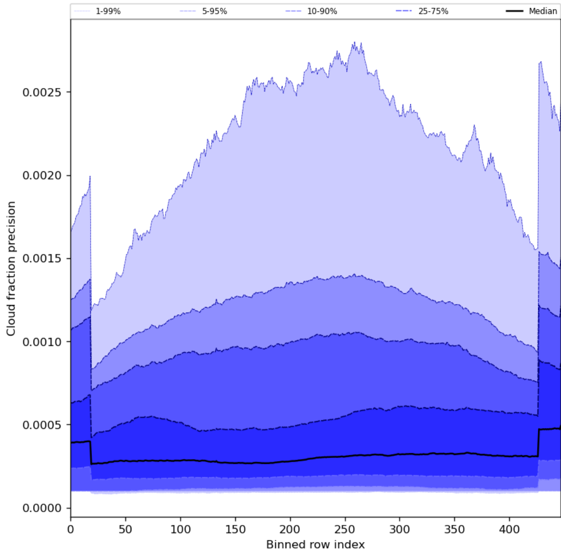
Figure 50: Along track statistics of “Cloud fraction precision” for 2023-07-17 to 2023-07-19
