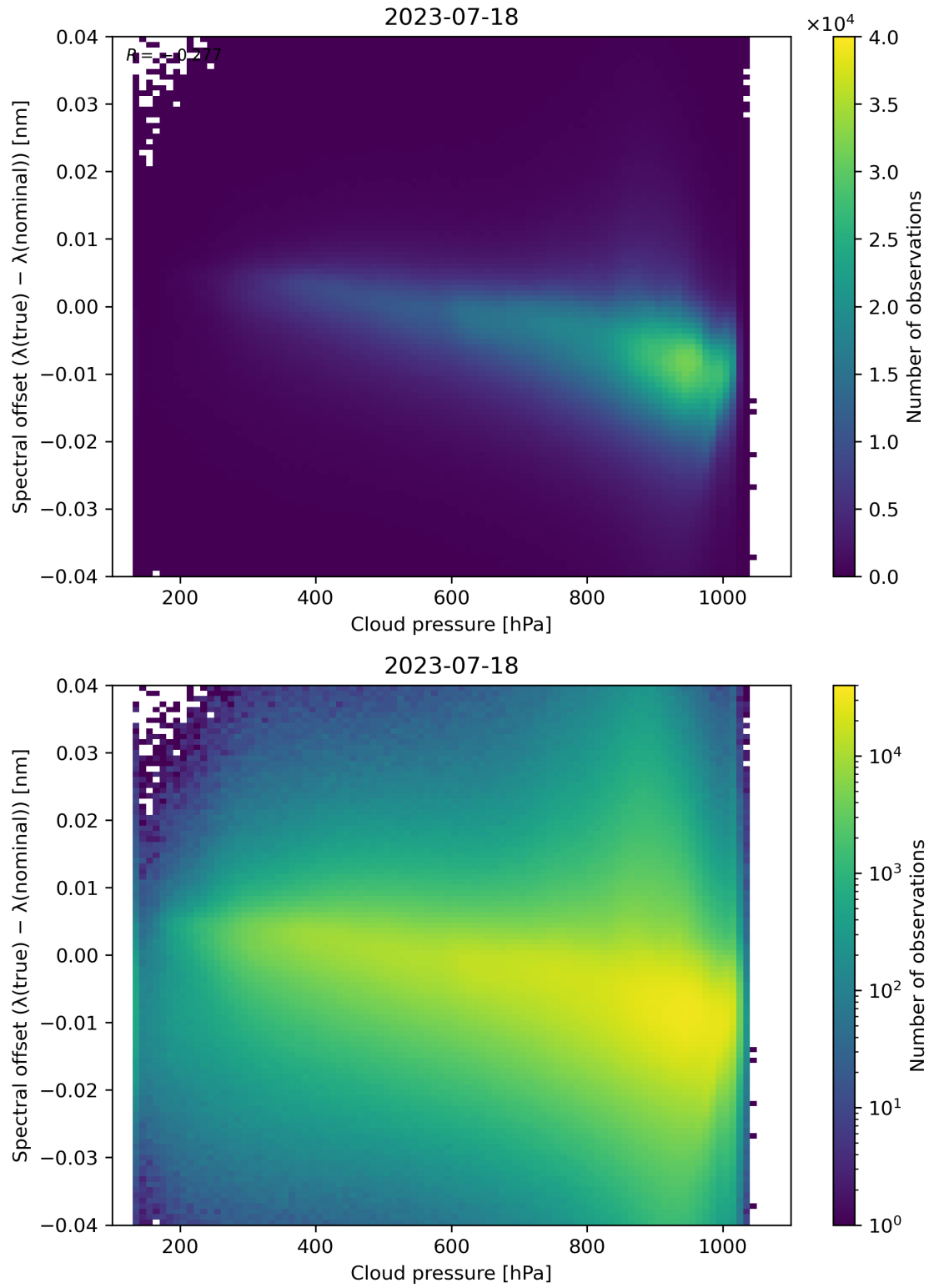
Figure 92: Scatter density plot of “Cloud pressure” against “Spectral offset ( \lambda(\text{true}) - \lambda(\text{nominal}) )” for 2023-07-17 to 2023-07-19.
