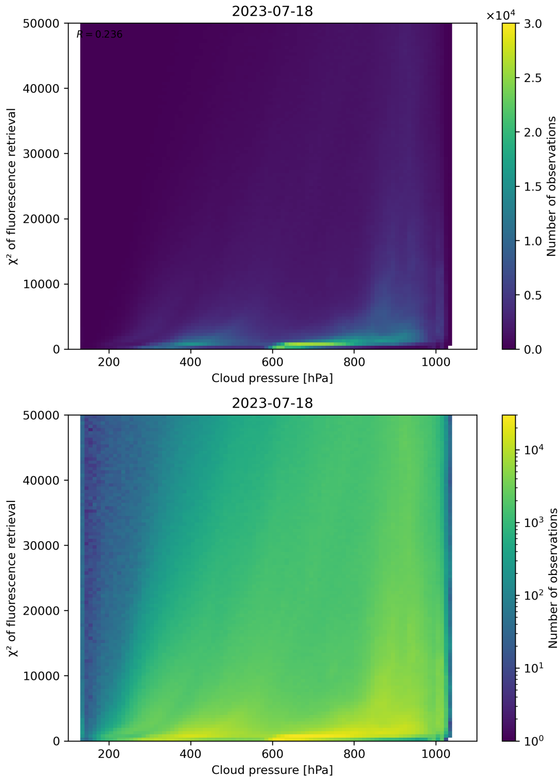
Figure 86: Scatter density plot of “Cloud pressure” against “ \chi^2 of fluorescence retrieval” for 2023-07-17 to 2023-07-19.
