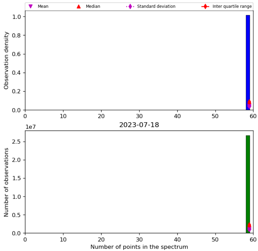
Figure 44: Histogram of “Number of points in the spectrum” for 2023-07-17 to 2023-07-19
