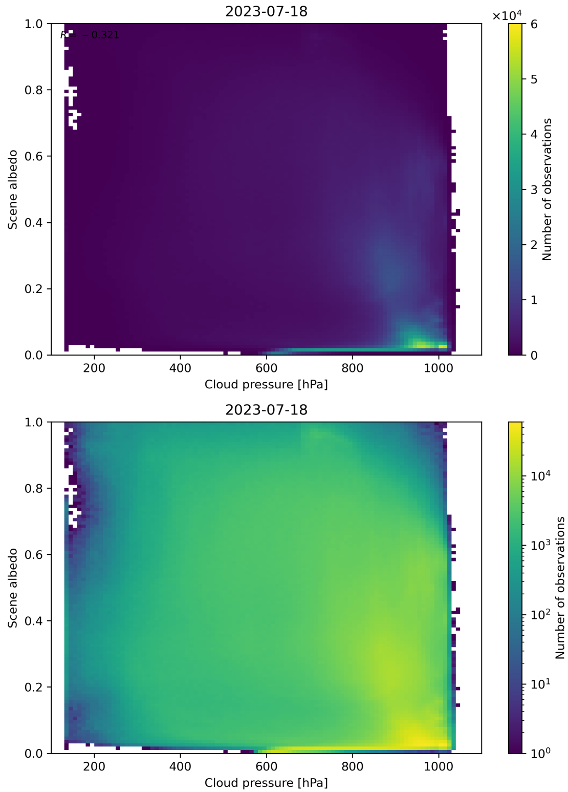
Figure 91: Scatter density plot of “Cloud pressure” against “Scene albedo” for 2023-07-17 to 2023-07-19.
