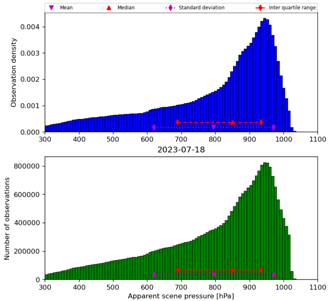
Figure 36: Histogram of “Apparent scene pressure” for 2023-07-17 to 2023-07-19
