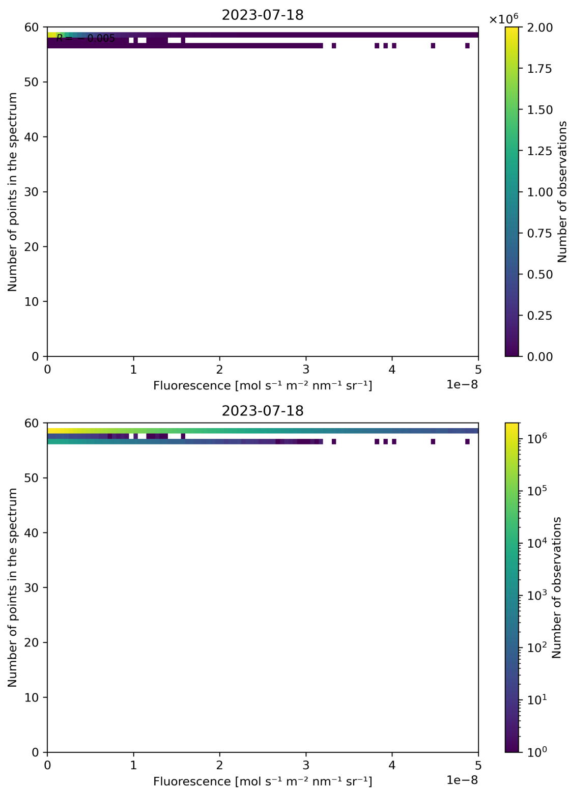
Figure 94: Scatter density plot of “Fluorescence” against “Number of points in the spectrum” for 2023-07-17 to 2023-07-19.
