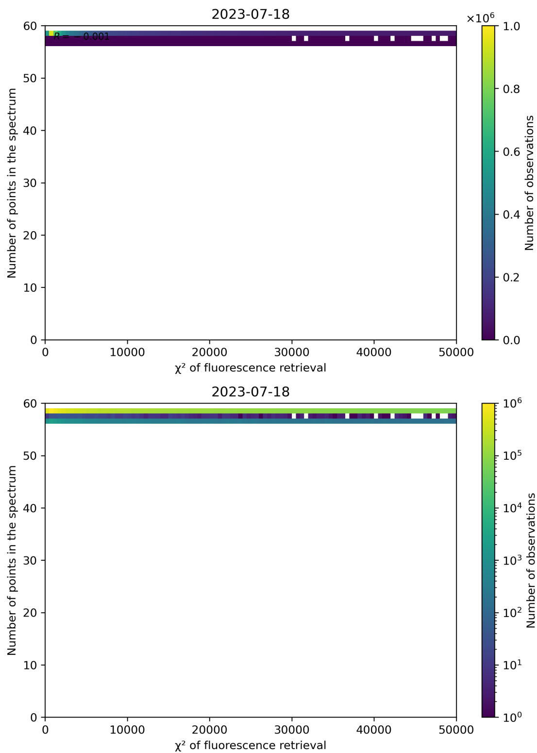
Figure 71: Scatter density plot of " \chi^2 of fluorescence retrieval" against "Number of points in the spectrum" for 2023-07-17 to 2023-07-19.
