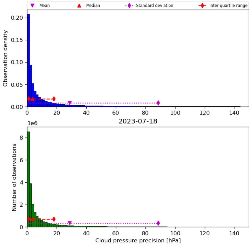
Figure 31: Histogram of “Cloud pressure precision” for 2023-07-17 to 2023-07-19
