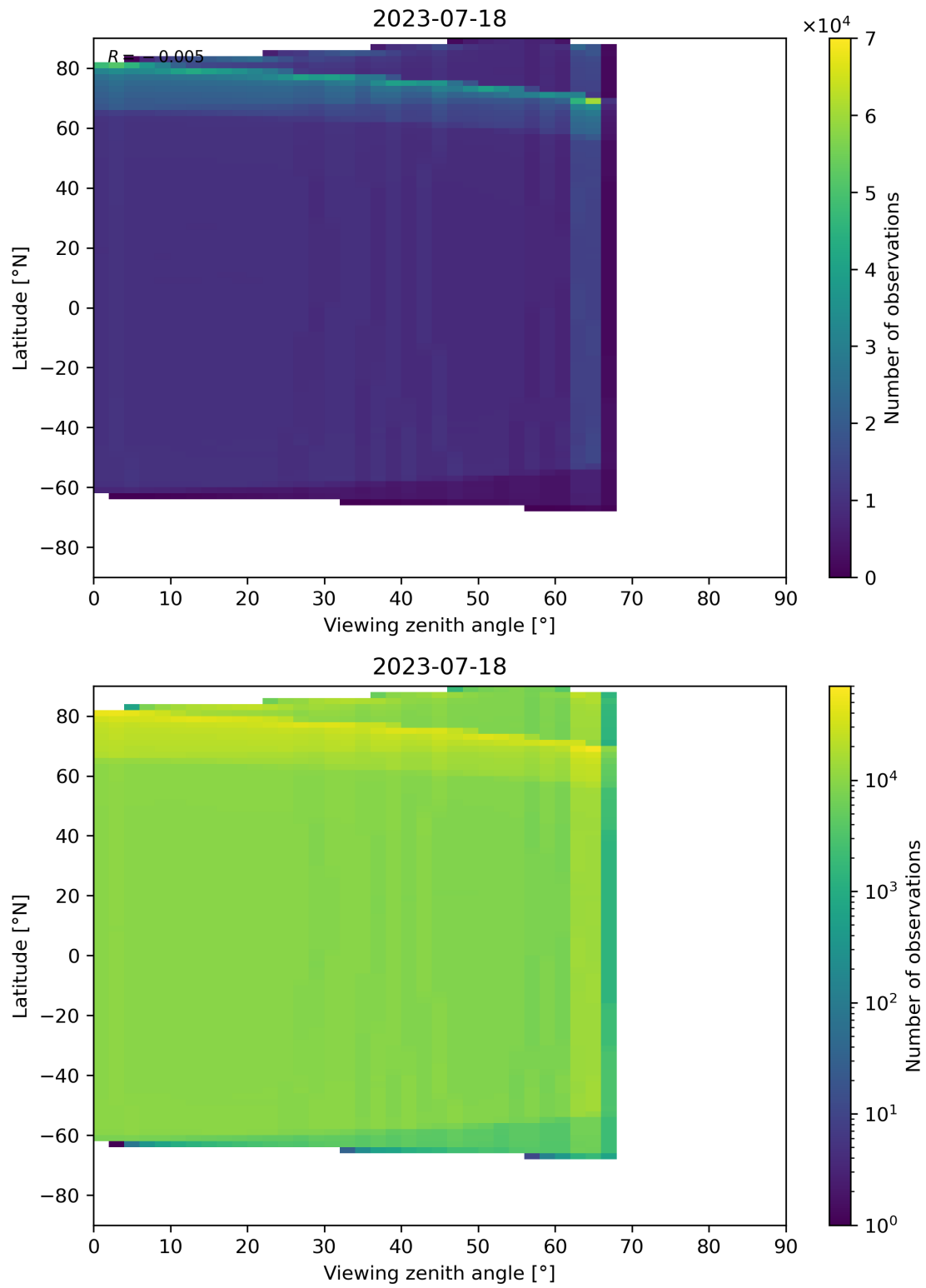
Figure 135: Scatter density plot of “Viewing zenith angle” against “Latitude” for 2023-07-17 to 2023-07-19.
