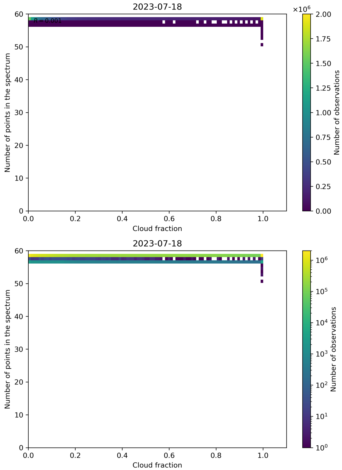
Figure 81: Scatter density plot of “Cloud fraction” against “Number of points in the spectrum” for 2023-07-17 to 2023-07-19.
