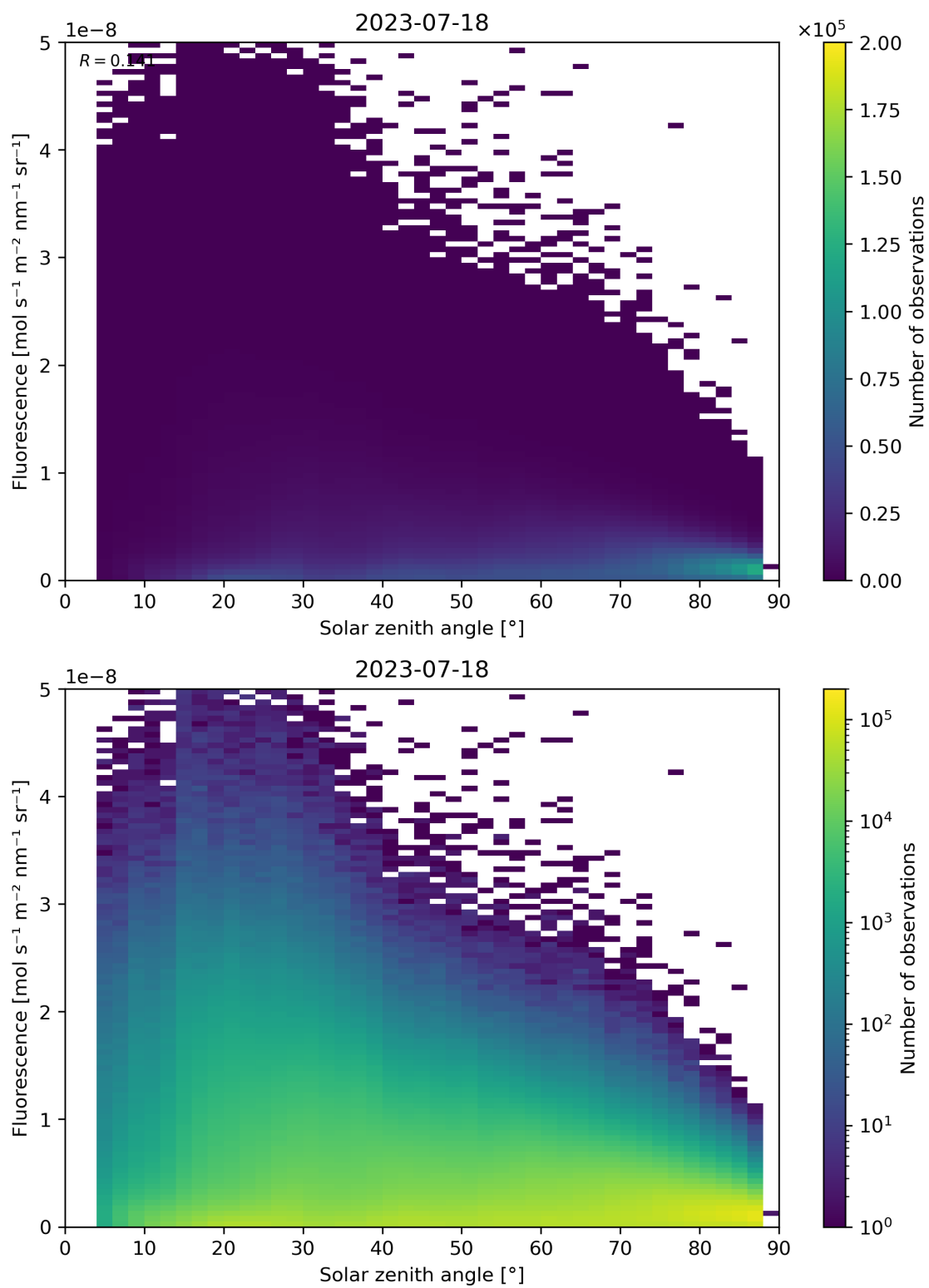
Figure 123: Scatter density plot of “Solar zenith angle” against “Fluorescence” for 2023-07-17 to 2023-07-19.
