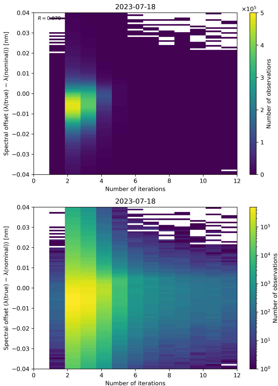
Figure 109: Scatter density plot of “Number of iterations” against “Spectral offset ( \lambda(\text{true}) - \lambda(\text{nominal}) )” for 2023-07-17 to 2023-07-19.
