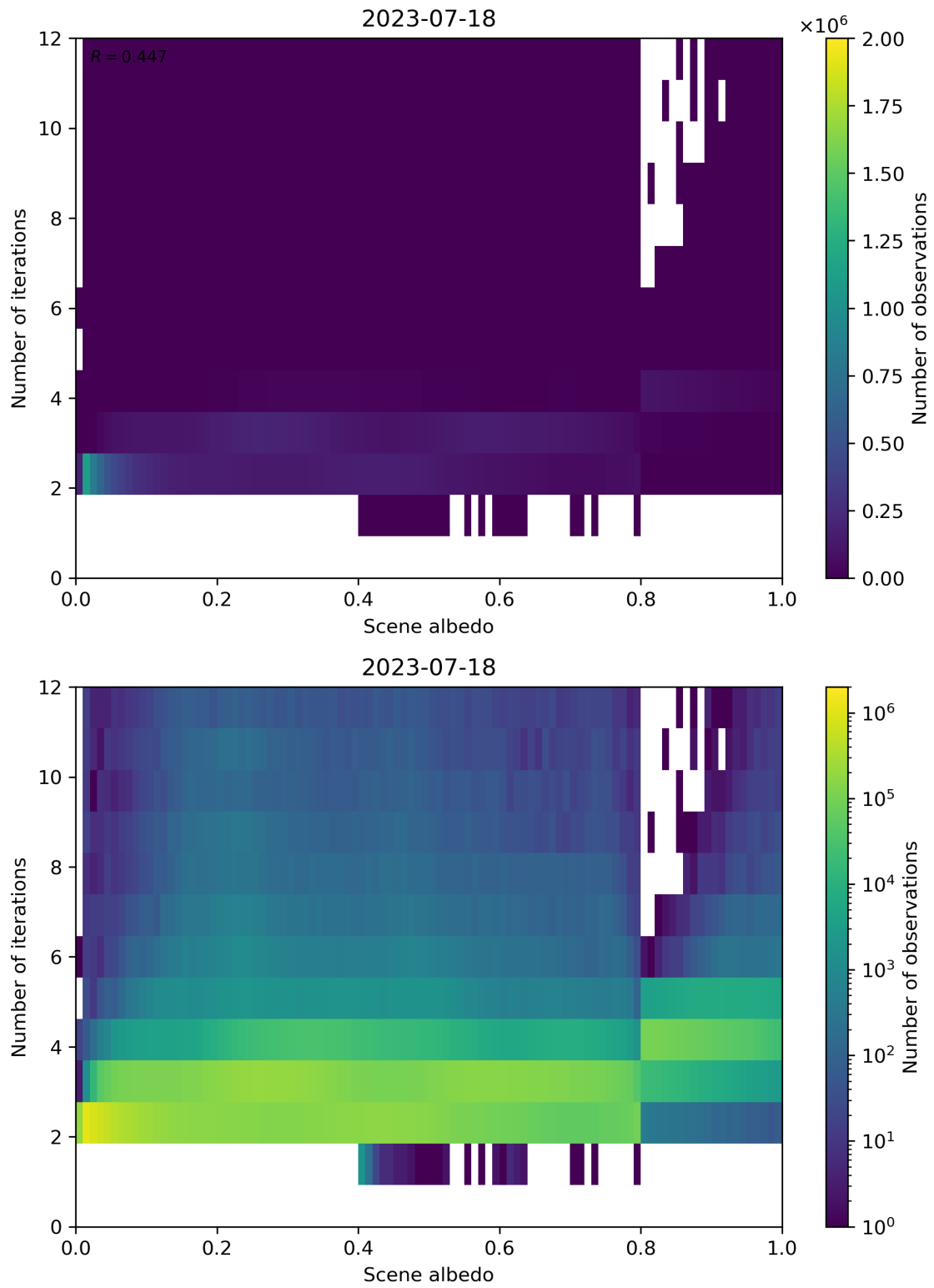
Figure 115: Scatter density plot of “Scene albedo” against “Number of iterations” for 2023-07-17 to 2023-07-19.
