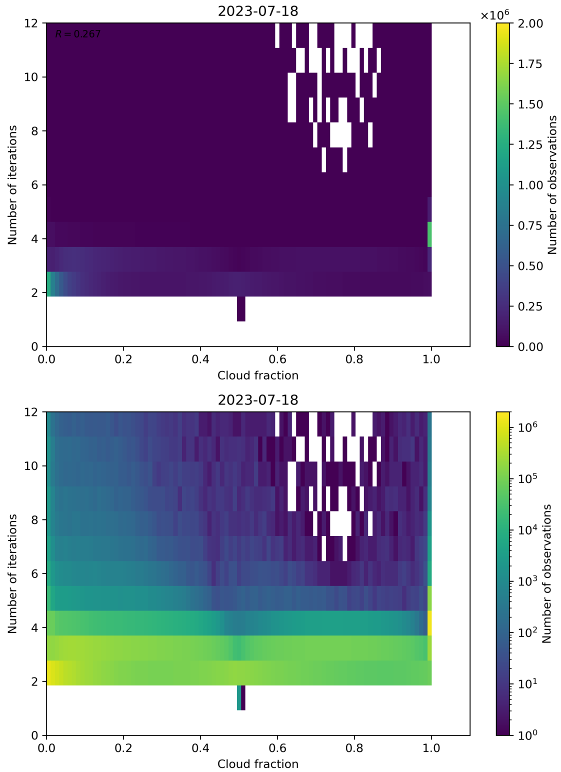
Figure 80: Scatter density plot of “Cloud fraction” against “Number of iterations” for 2023-07-17 to 2023-07-19.
