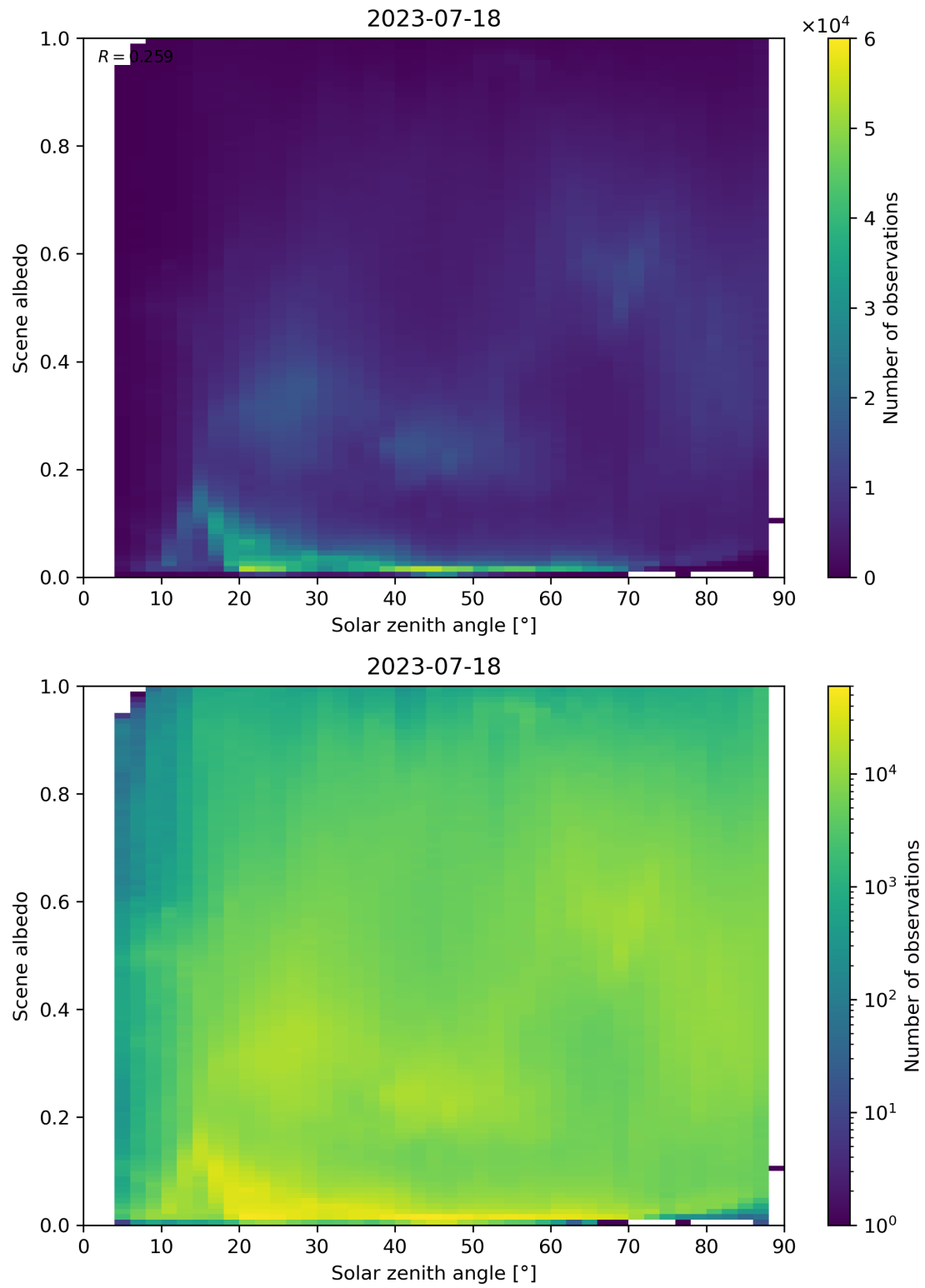
Figure 127: Scatter density plot of “Solar zenith angle” against “Scene albedo” for 2023-07-17 to 2023-07-19.
