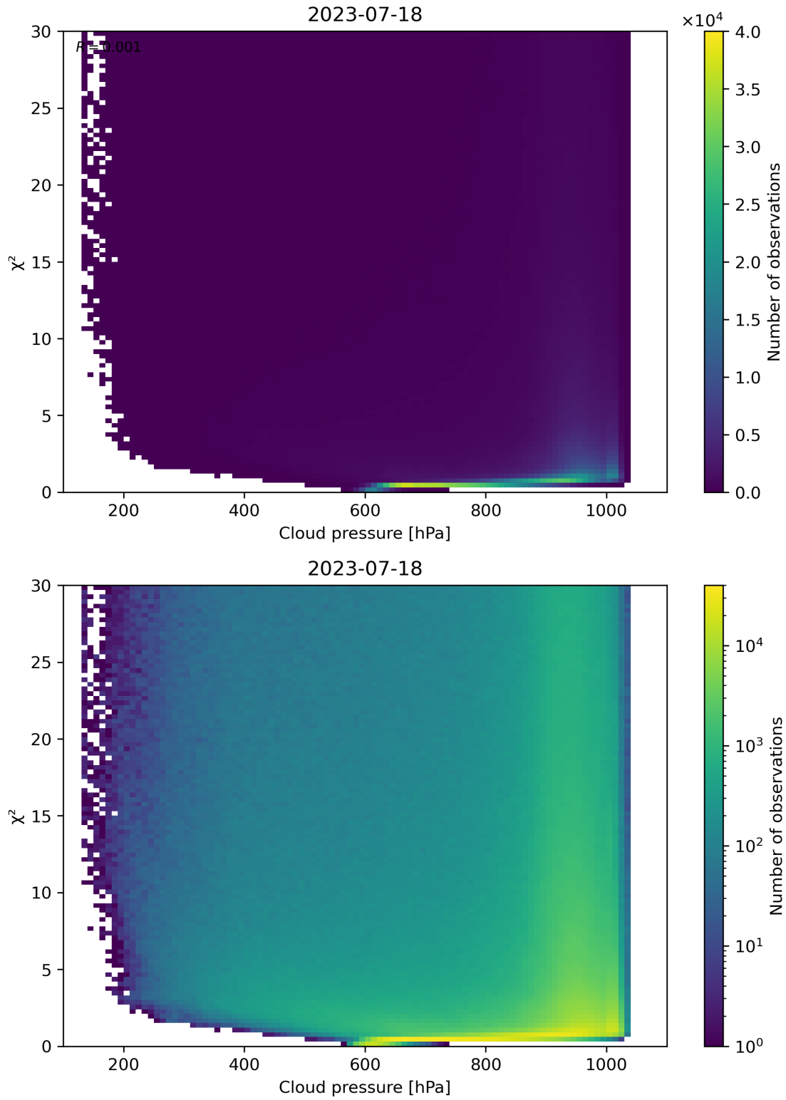
Figure 85: Scatter density plot of “Cloud pressure” against “ \chi^2 ” for 2023-07-17 to 2023-07-19.
