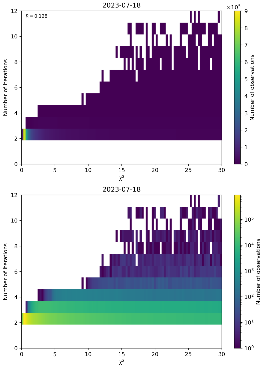
Figure 73: Scatter density plot of “ \chi^2 ” against “Number of iterations” for 2023-07-17 to 2023-07-19.
