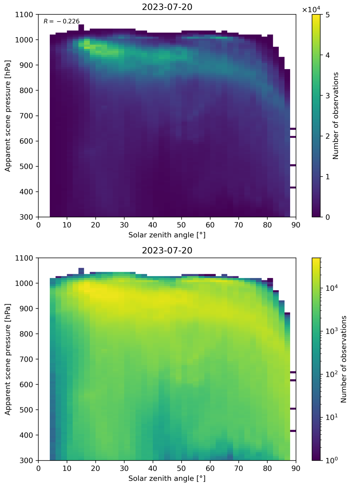
Figure 118: Scatter density plot of “Solar zenith angle” against “Apparent scene pressure” for 2023-07-19 to 2023-07-21.
