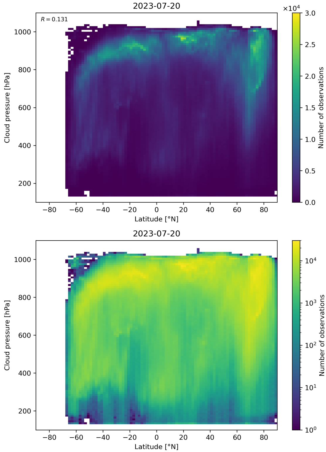
Figure 100: Scatter density plot of “Latitude” against “Cloud pressure” for 2023-07-19 to 2023-07-21.
