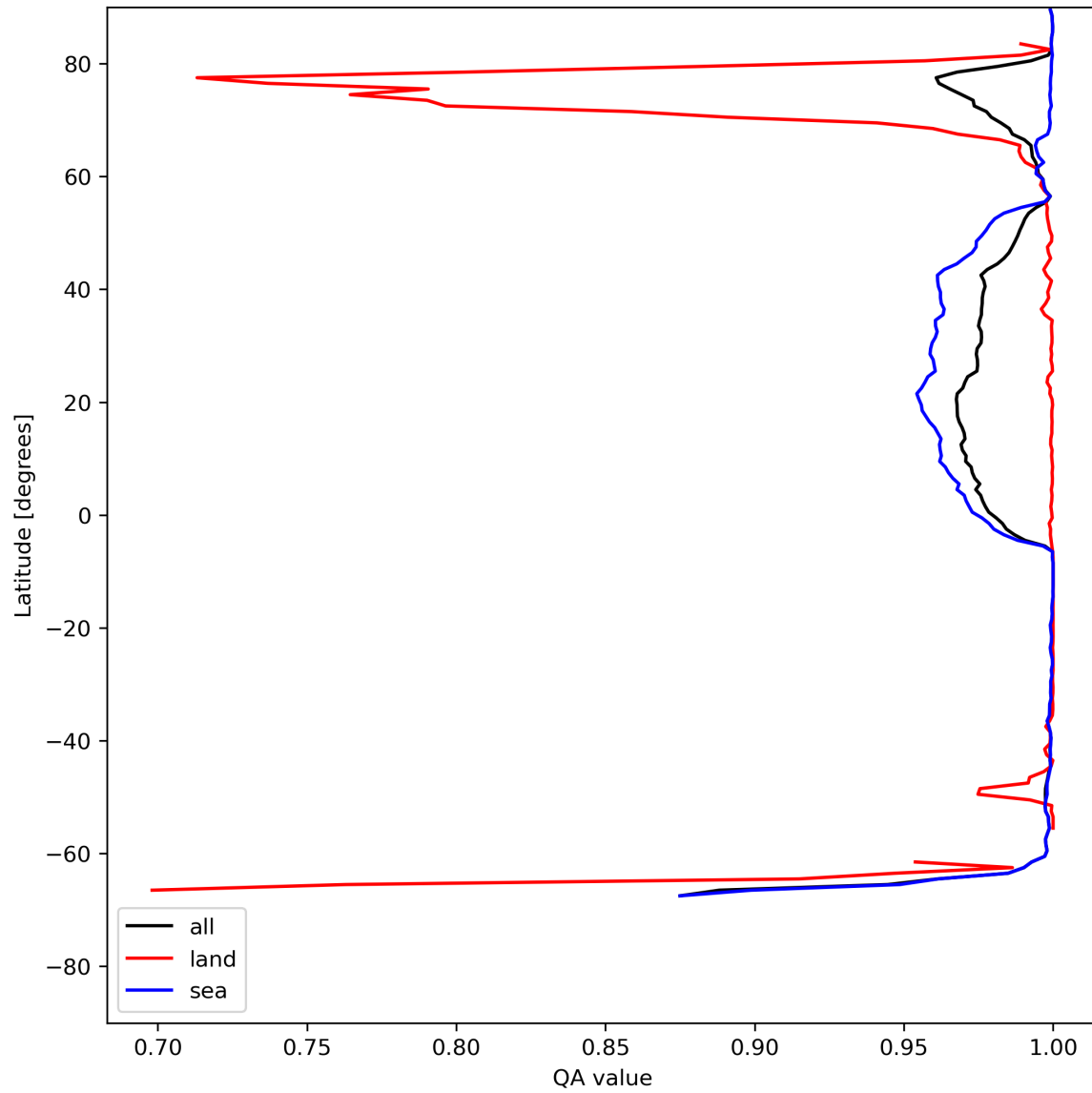
Figure 12: Zonal average of “QA value” for 2023-07-19 to 2023-07-21.
