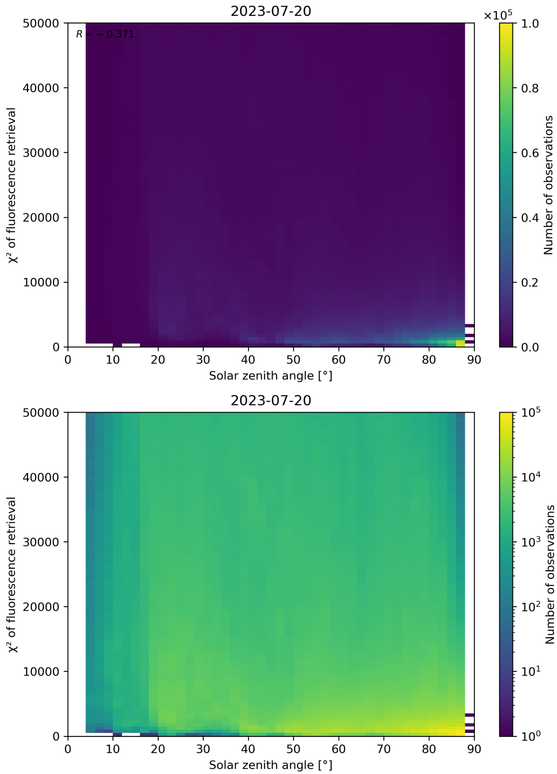
Figure 120: Scatter density plot of “Solar zenith angle” against “ \chi^2 of fluorescence retrieval” for 2023-07-19 to 2023-07-21.
