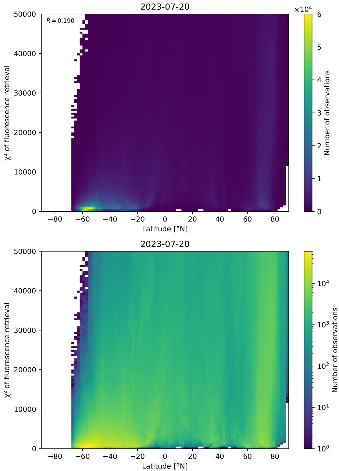
Figure 98: Scatter density plot of “Latitude” against “ \chi^2 of fluorescence retrieval” for 2023-07-19 to 2023-07-21.
