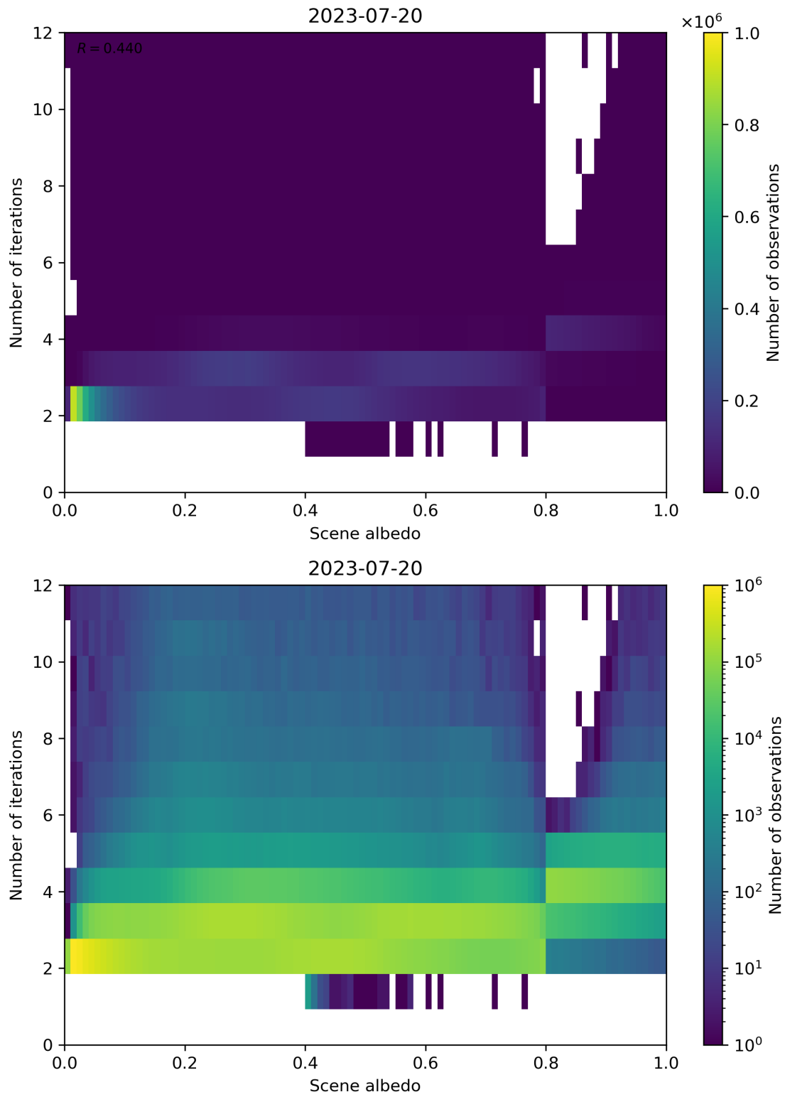
Figure 115: Scatter density plot of “Scene albedo” against “Number of iterations” for 2023-07-19 to 2023-07-21.
