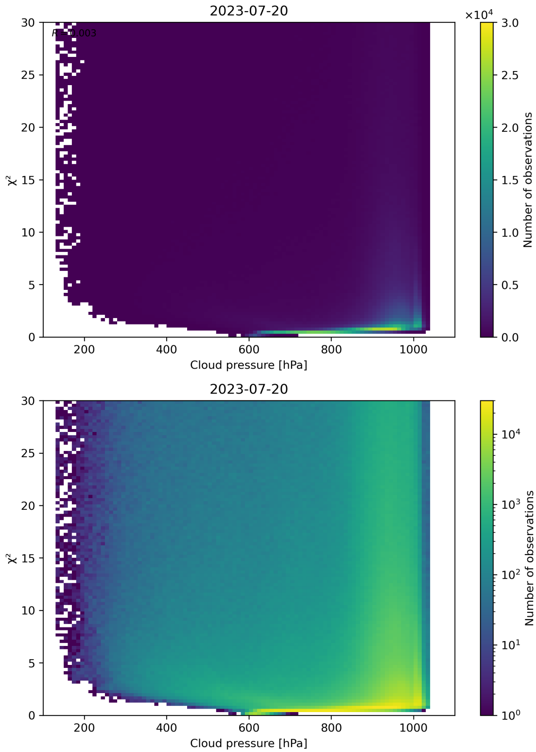
Figure 85: Scatter density plot of “Cloud pressure” against “ \chi^2 ” for 2023-07-19 to 2023-07-21.
