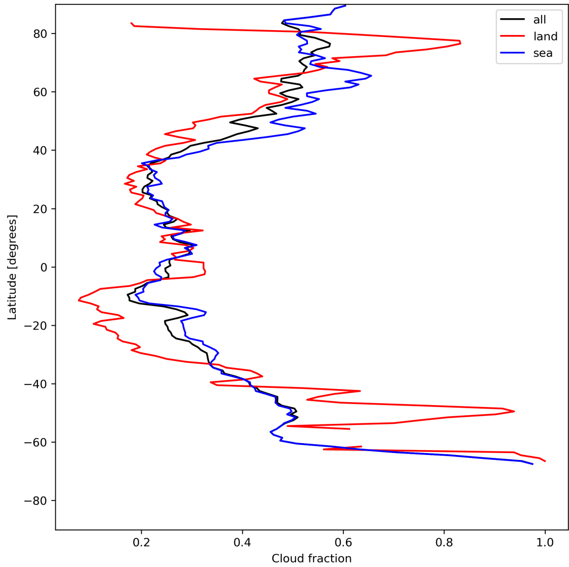
Figure 15: Zonal average of “Cloud fraction” for 2023-07-19 to 2023-07-21.
