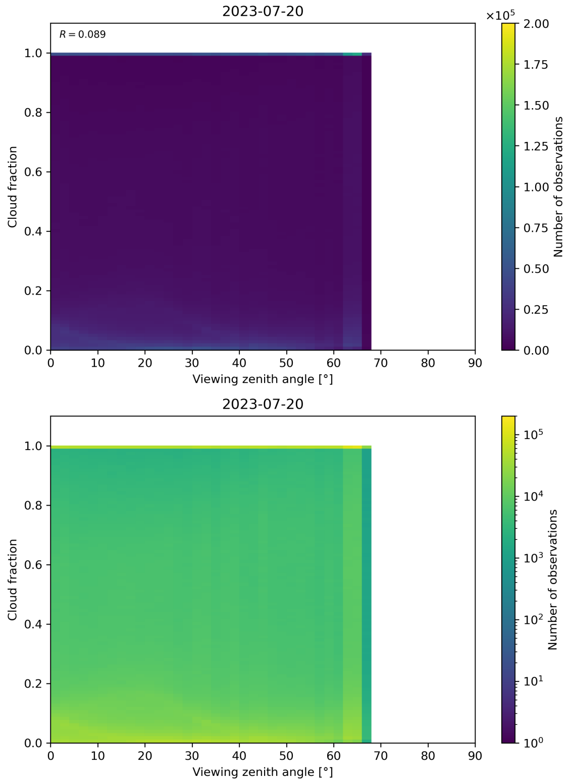
Figure 132: Scatter density plot of “Viewing zenith angle” against “Cloud fraction” for 2023-07-19 to 2023-07-21.
