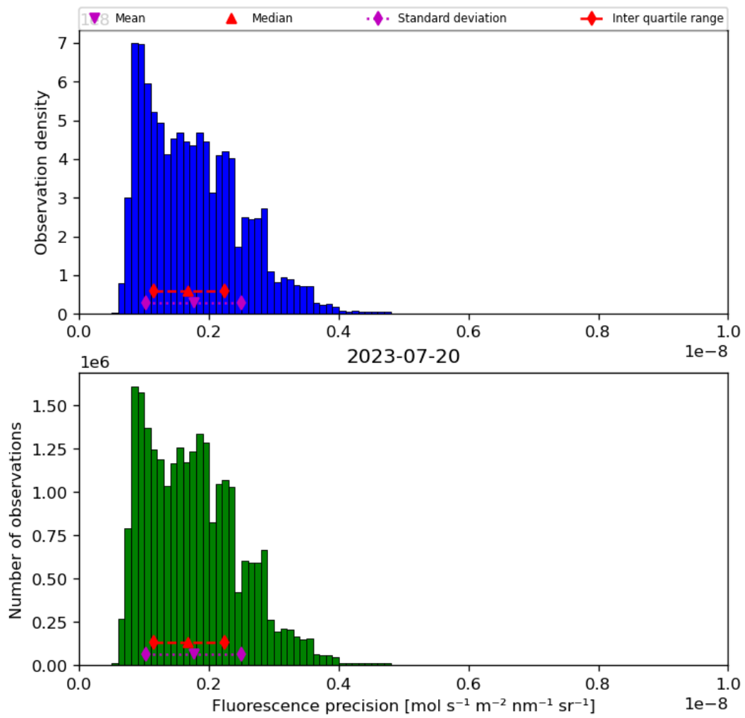
Figure 41: Histogram of “Fluorescence precision” for 2023-07-19 to 2023-07-21
