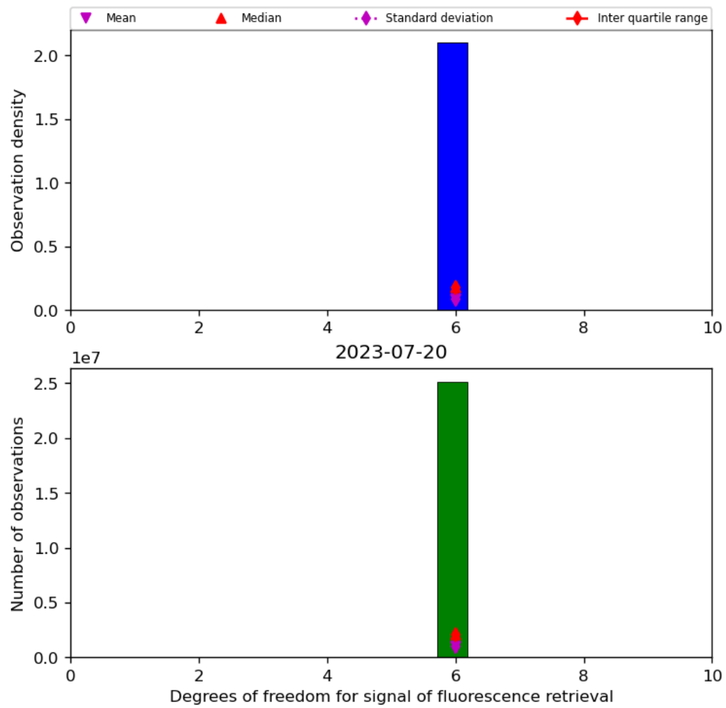
Figure 43: Histogram of "Degrees of freedom for signal of fluorescence retrieval" for 2023-07-19 to 2023-07-21
