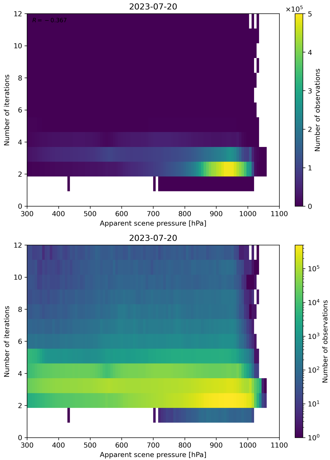
Figure 66: Scatter density plot of “Apparent scene pressure” against “Number of iterations” for 2023-07-19 to 2023-07-21.
