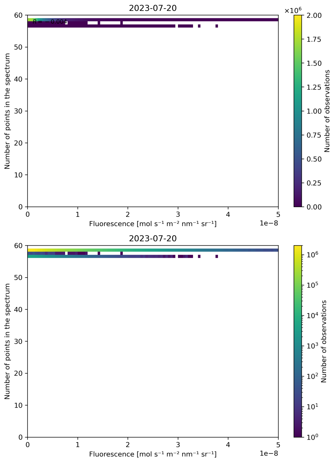
Figure 94: Scatter density plot of “Fluorescence” against “Number of points in the spectrum” for 2023-07-19 to 2023-07-21.
