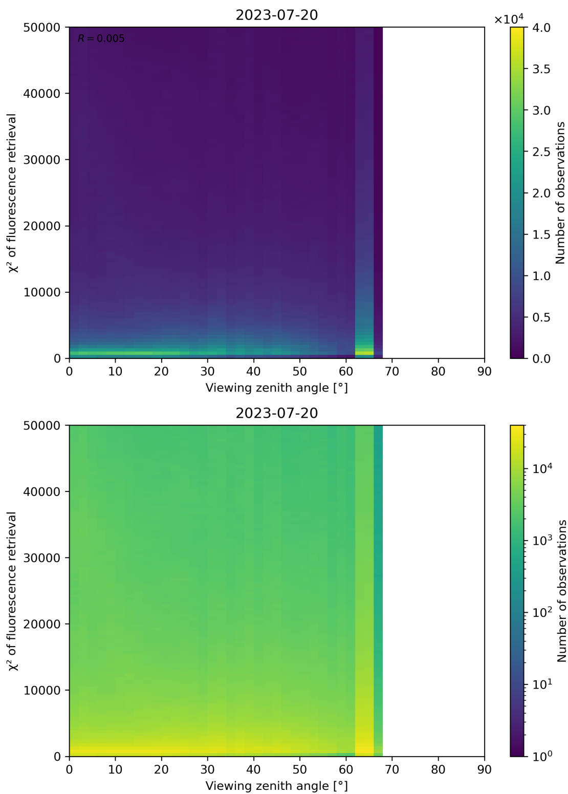
Figure 131: Scatter density plot of “Viewing zenith angle” against “ \chi^2 of fluorescence retrieval” for 2023-07-19 to 2023-07-21.
