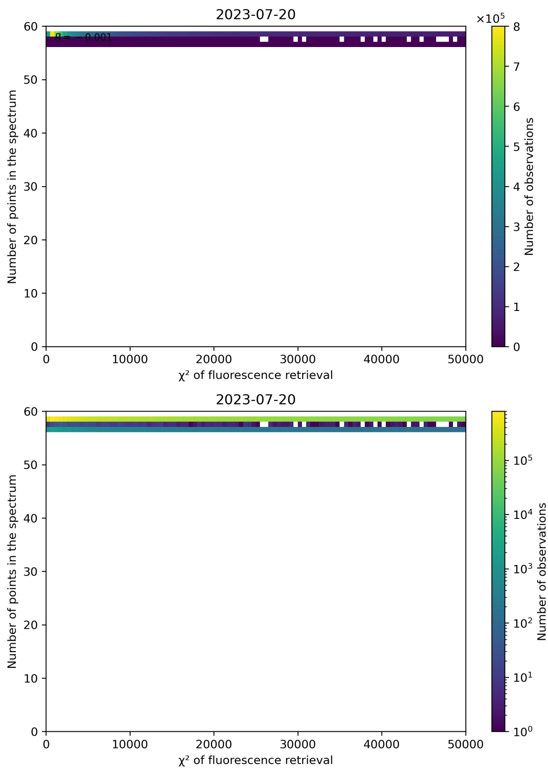
Figure 71: Scatter density plot of " \chi^2 of fluorescence retrieval" against "Number of points in the spectrum" for 2023-07-19 to 2023-07-21.
