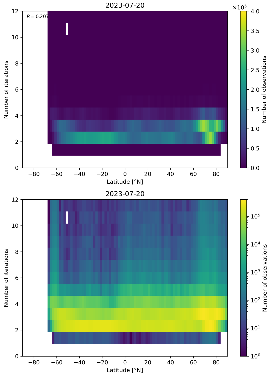
Figure 102: Scatter density plot of “Latitude” against “Number of iterations” for 2023-07-19 to 2023-07-21.
