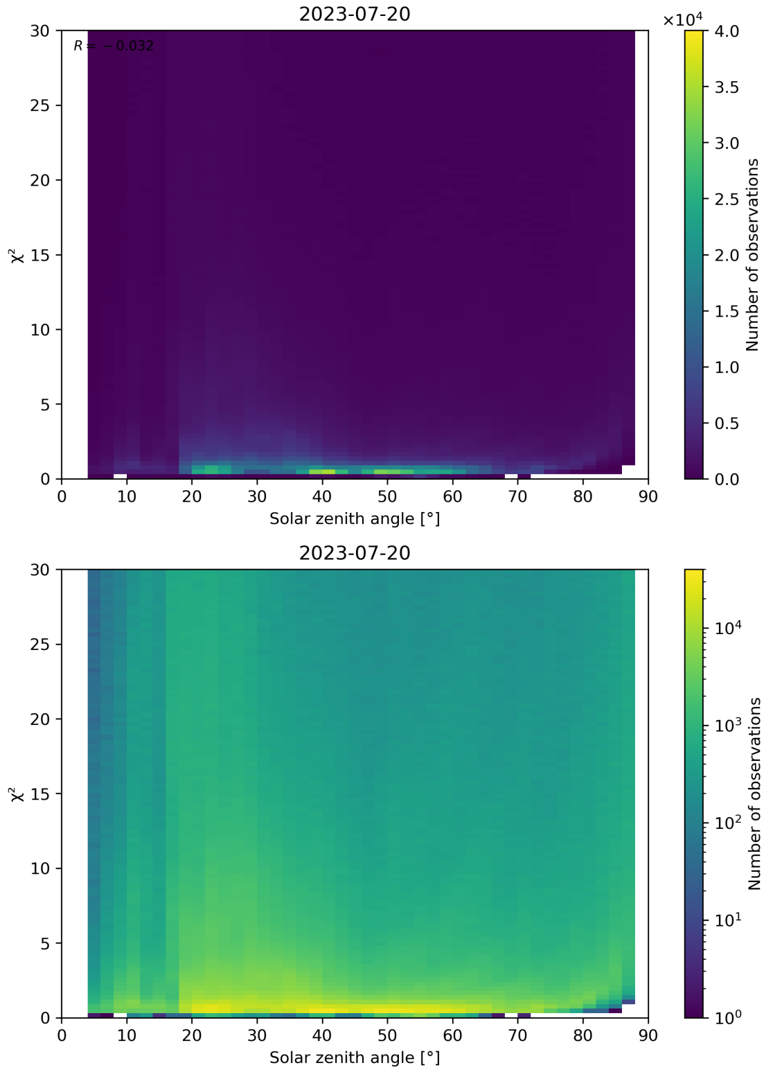
Figure 119: Scatter density plot of “Solar zenith angle” against “ \chi^2 ” for 2023-07-19 to 2023-07-21.
