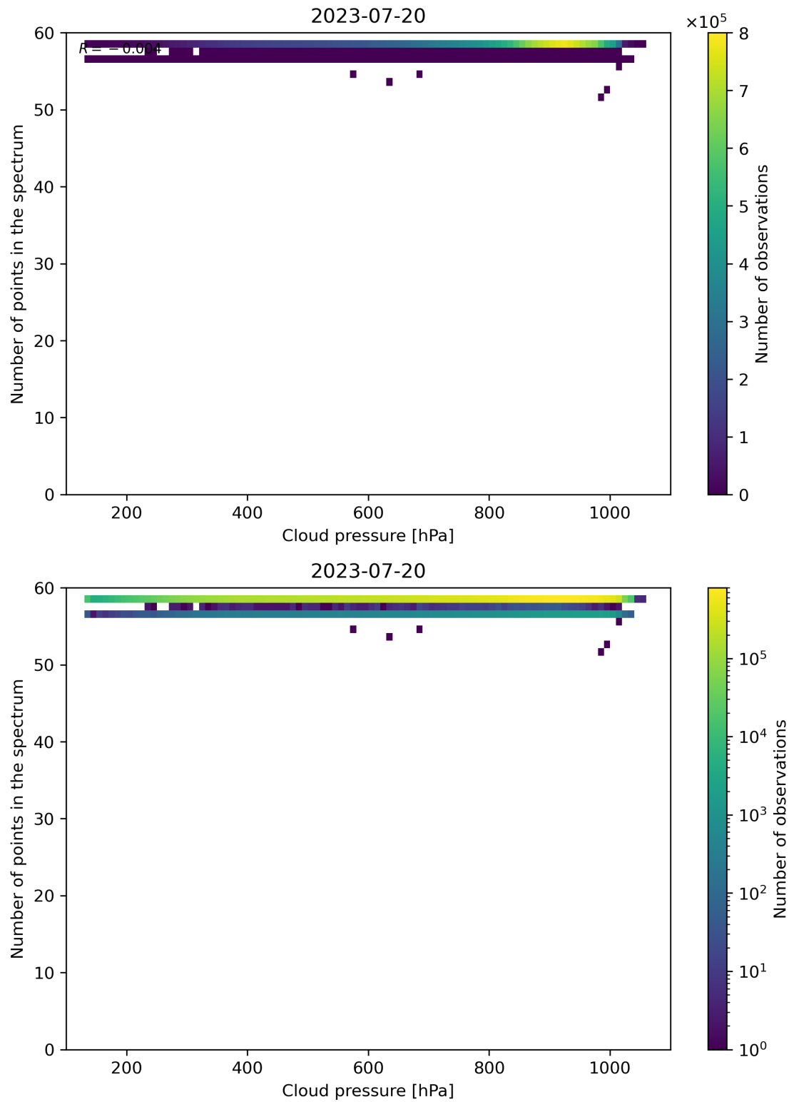
Figure 90: Scatter density plot of “Cloud pressure” against “Number of points in the spectrum” for 2023-07-19 to 2023-07-21.
