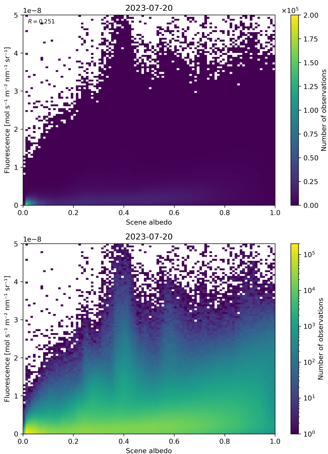
Figure 114: Scatter density plot of “Scene albedo” against “Fluorescence” for 2023-07-19 to 2023-07-21.
