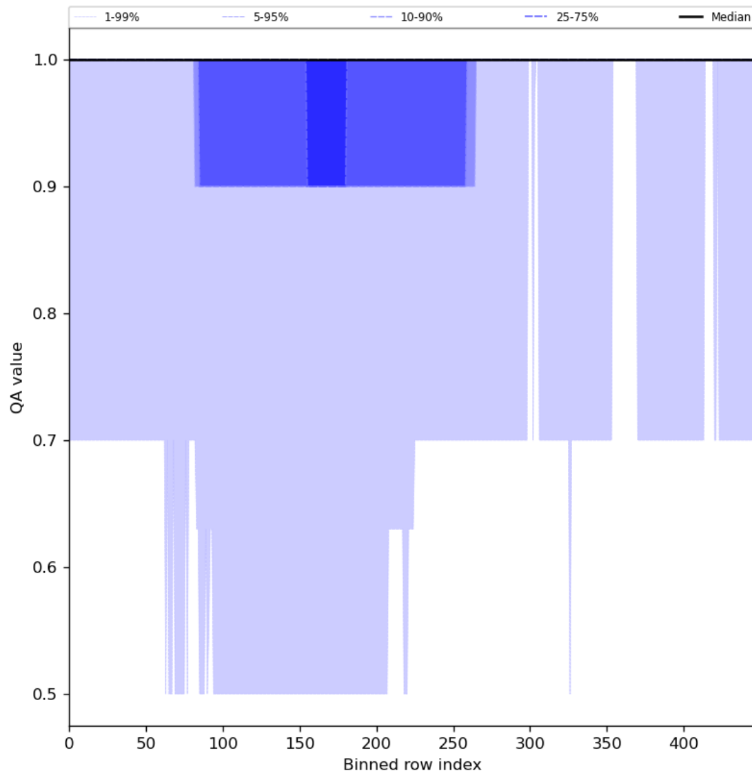
Figure 46: Along track statistics of “QA value” for 2023-07-19 to 2023-07-21
