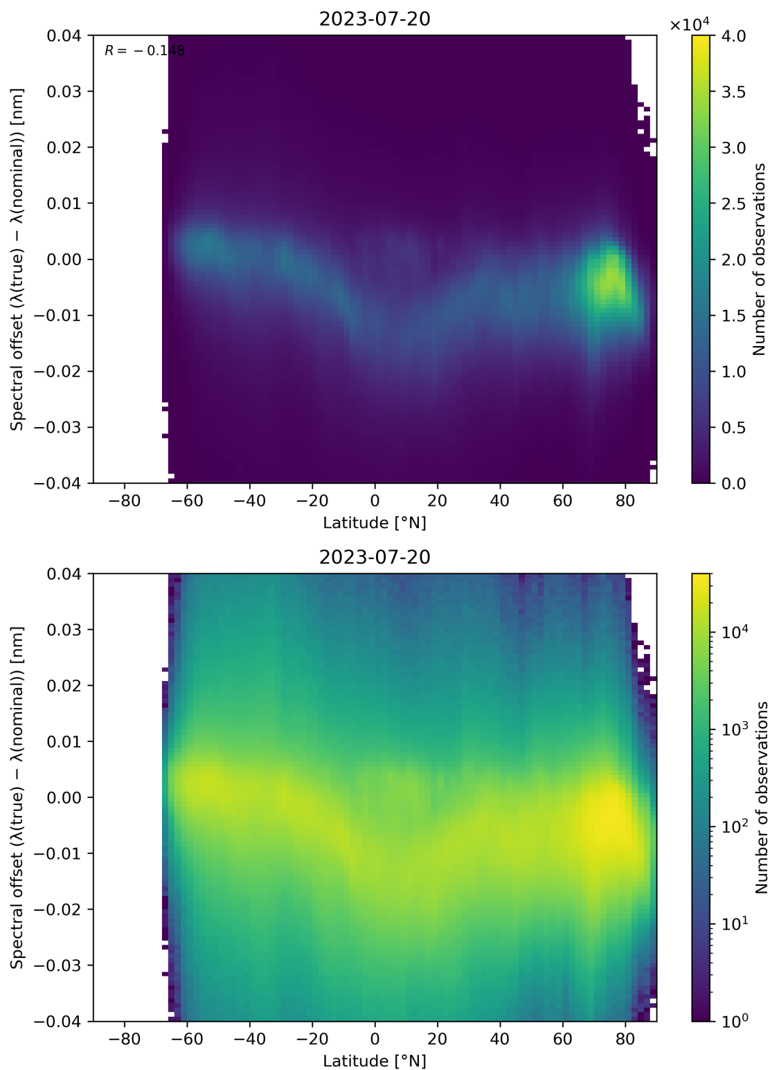
Figure 105: Scatter density plot of “Latitude” against “Spectral offset ( \lambda(\text{true}) - \lambda(\text{nominal}) )” for 2023-07-19 to 2023-07-21.
