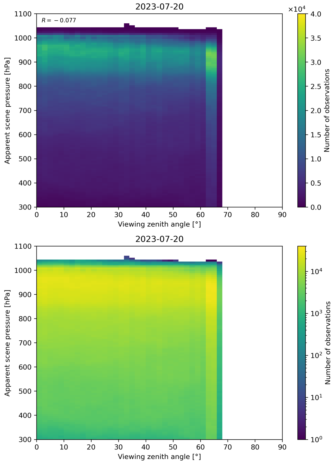
Figure 129: Scatter density plot of “Viewing zenith angle” against “Apparent scene pressure” for 2023-07-19 to 2023-07-21.
