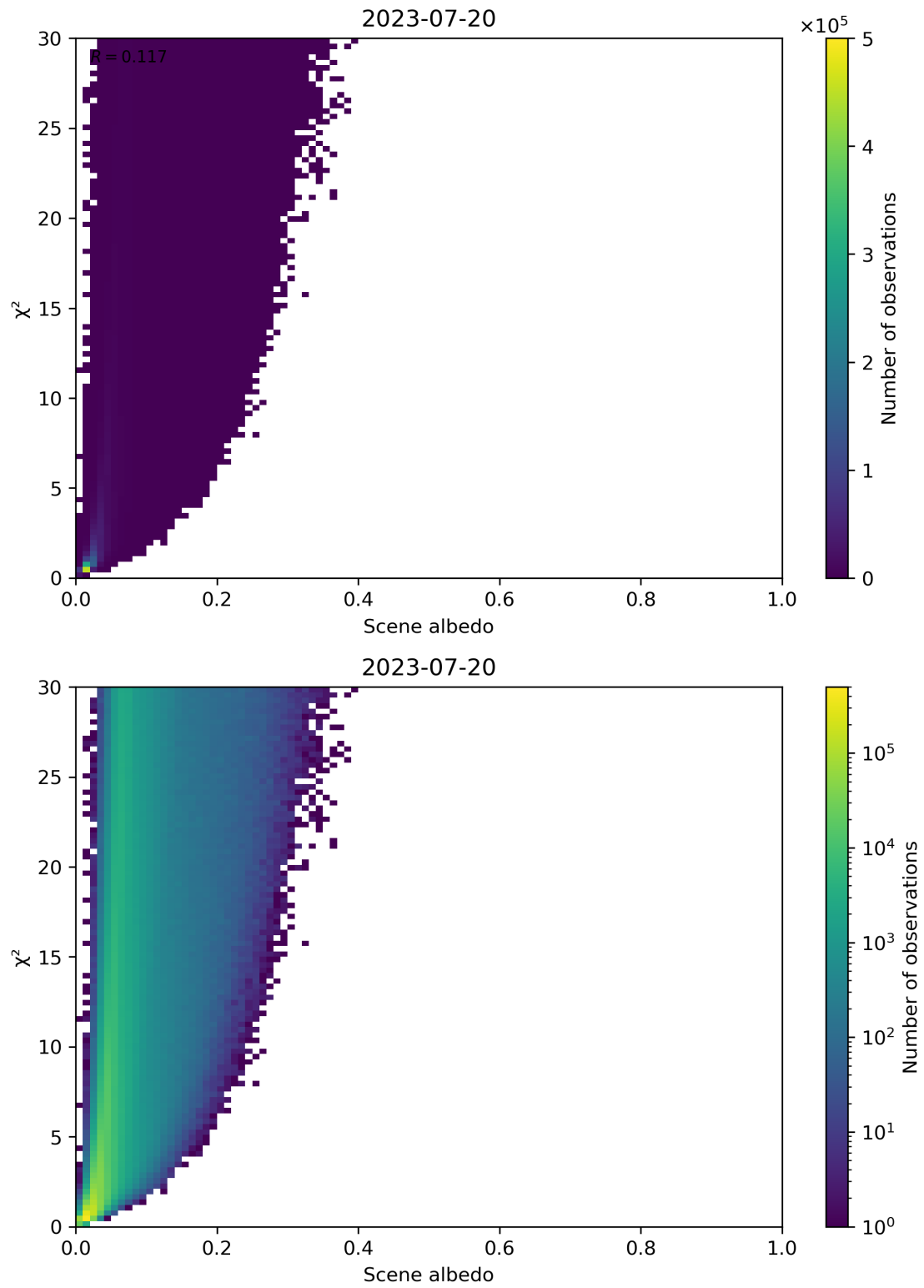
Figure 112: Scatter density plot of “Scene albedo” against “ \chi^2 ” for 2023-07-19 to 2023-07-21.
