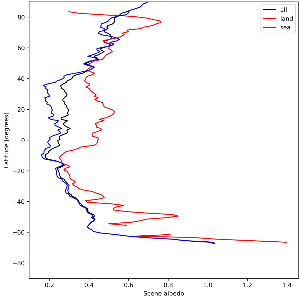
Figure 17: Zonal average of “Scene albedo” for 2023-07-19 to 2023-07-21.
