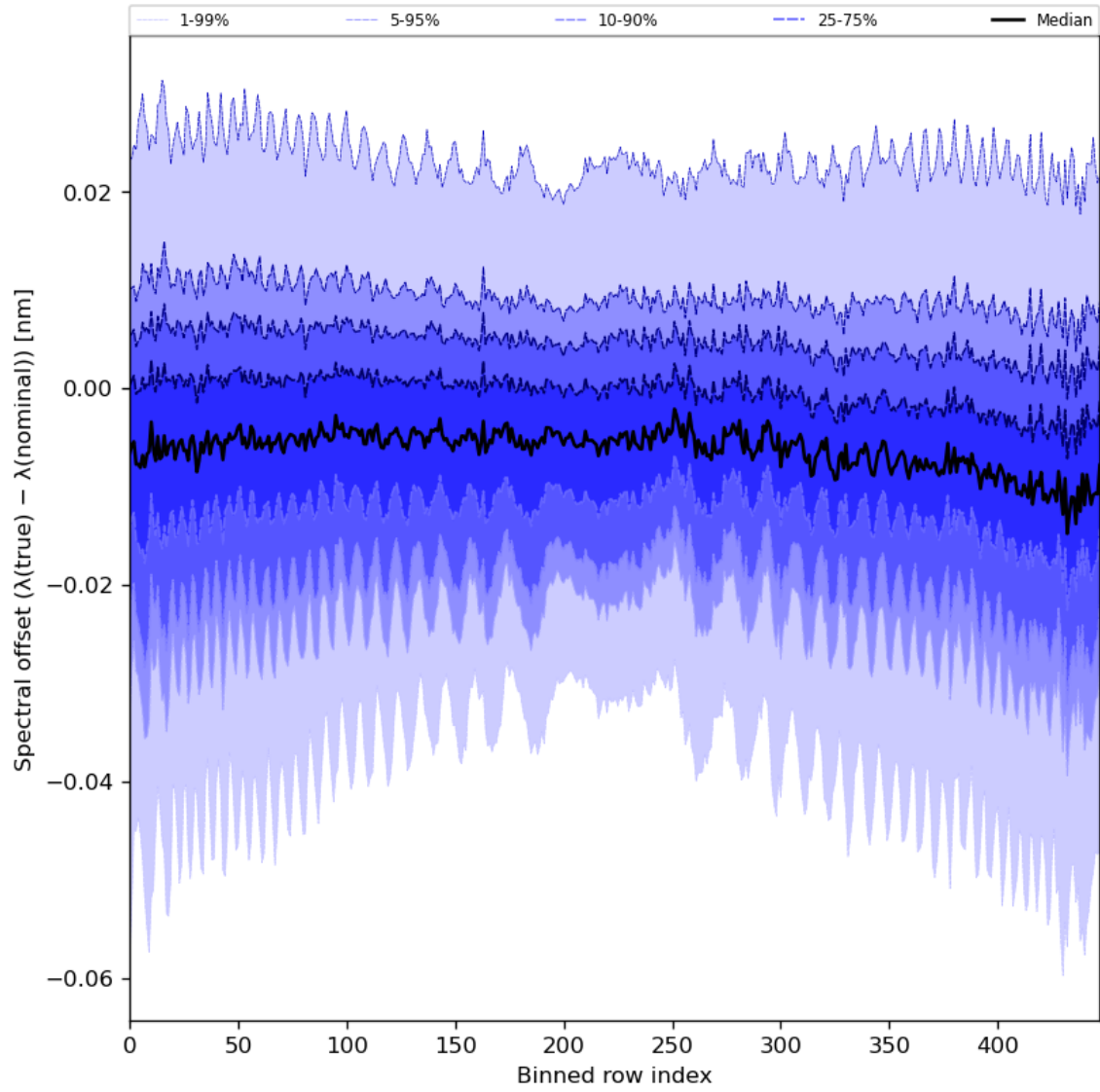
Figure 62: Along track statistics of “Spectral offset ( \lambda(\text{true}) - \lambda(\text{nominal}) )” for 2023-07-19 to 2023-07-21
