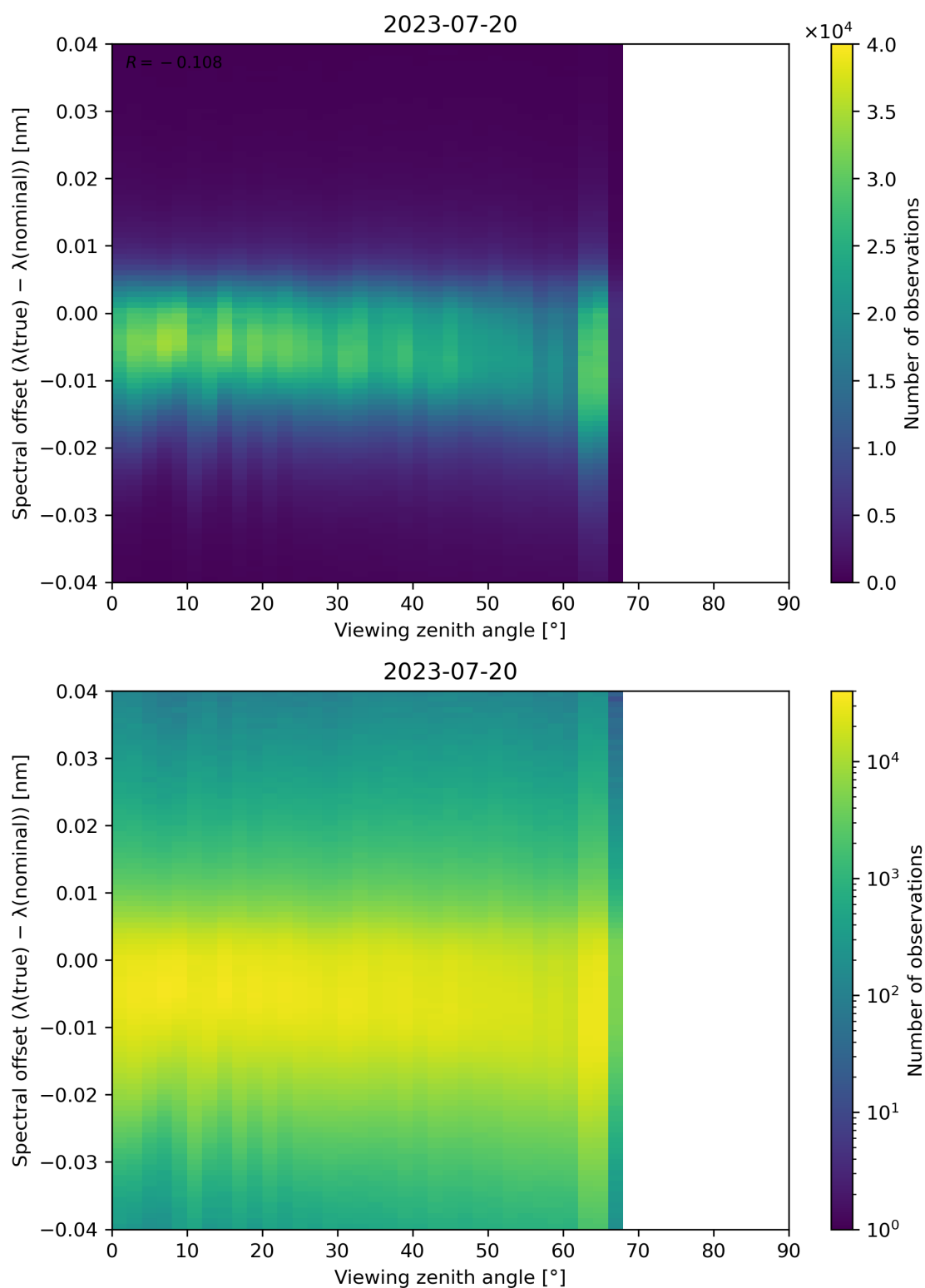
Figure 140: Scatter density plot of “Viewing zenith angle” against “Spectral offset ( \lambda(\text{true}) - \lambda(\text{nominal}) )” for 2023-07-19 to 2023-07-21.
