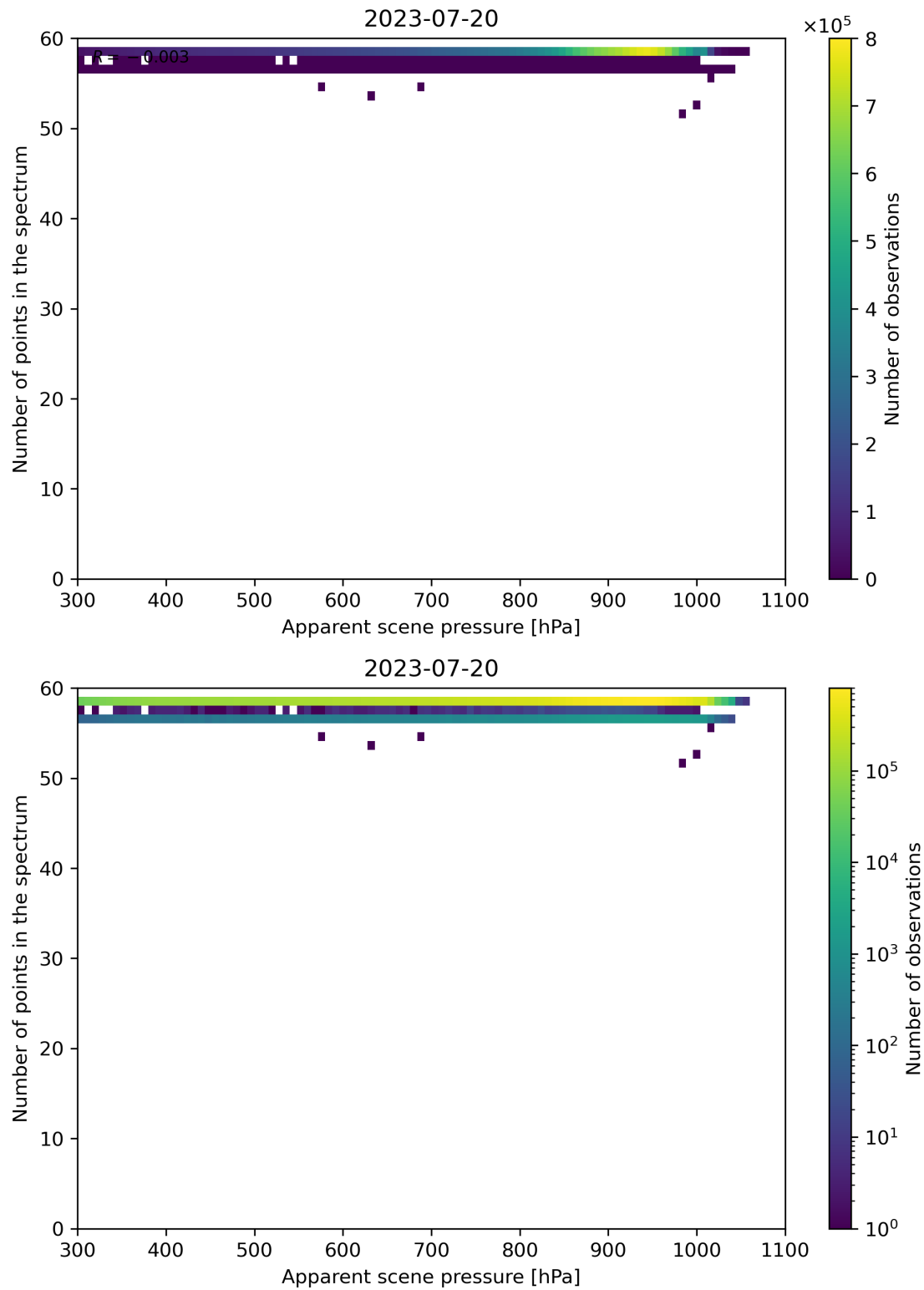
Figure 67: Scatter density plot of “Apparent scene pressure” against “Number of points in the spectrum” for 2023-07-19 to 2023-07-21.
