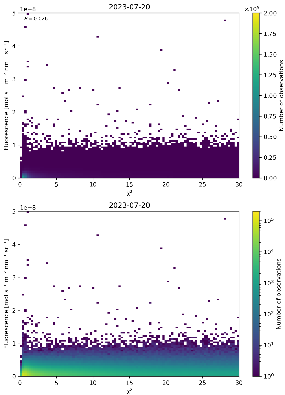
Figure 70: Scatter density plot of “ \chi^2 ” against “Fluorescence” for 2023-07-19 to 2023-07-21.
