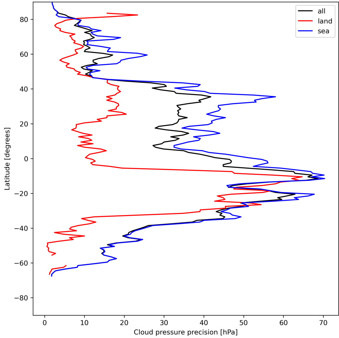
Figure 14: Zonal average of “Cloud pressure precision” for 2023-07-19 to 2023-07-21.
