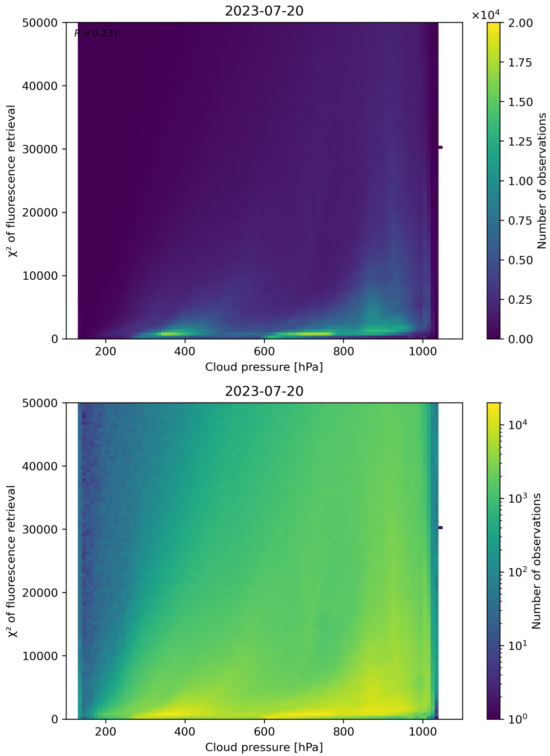
Figure 86: Scatter density plot of “Cloud pressure” against “ \chi^2 of fluorescence retrieval” for 2023-07-19 to 2023-07-21.
