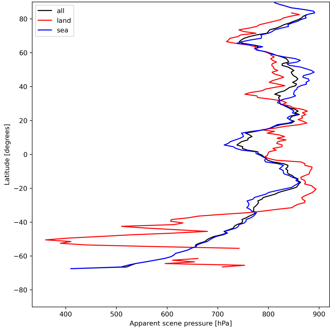
Figure 19: Zonal average of “Apparent scene pressure” for 2023-07-19 to 2023-07-21.
