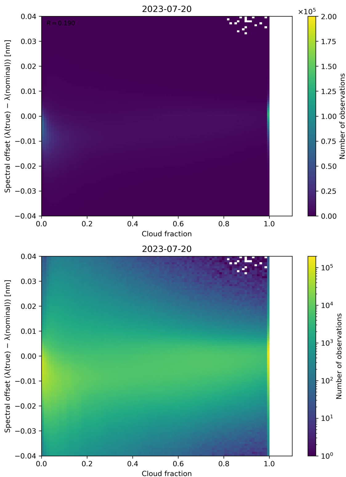
Figure 83: Scatter density plot of “Cloud fraction” against “Spectral offset ( \lambda(\text{true}) - \lambda(\text{nominal}) )” for 2023-07-19 to 2023-07-21.
