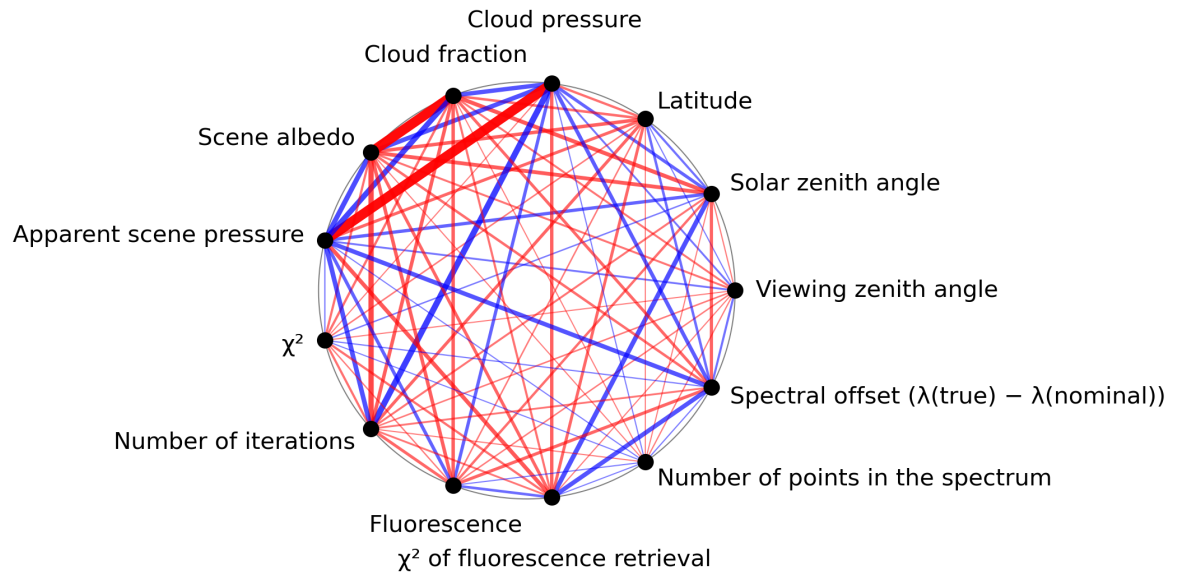
Figure 1: Map of correlation graph for 2023-07-19 to 2023-07-21.
