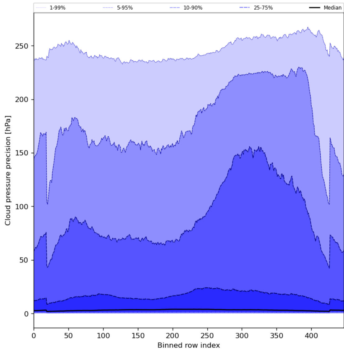
Figure 48: Along track statistics of “Cloud pressure precision” for 2023-07-19 to 2023-07-21
