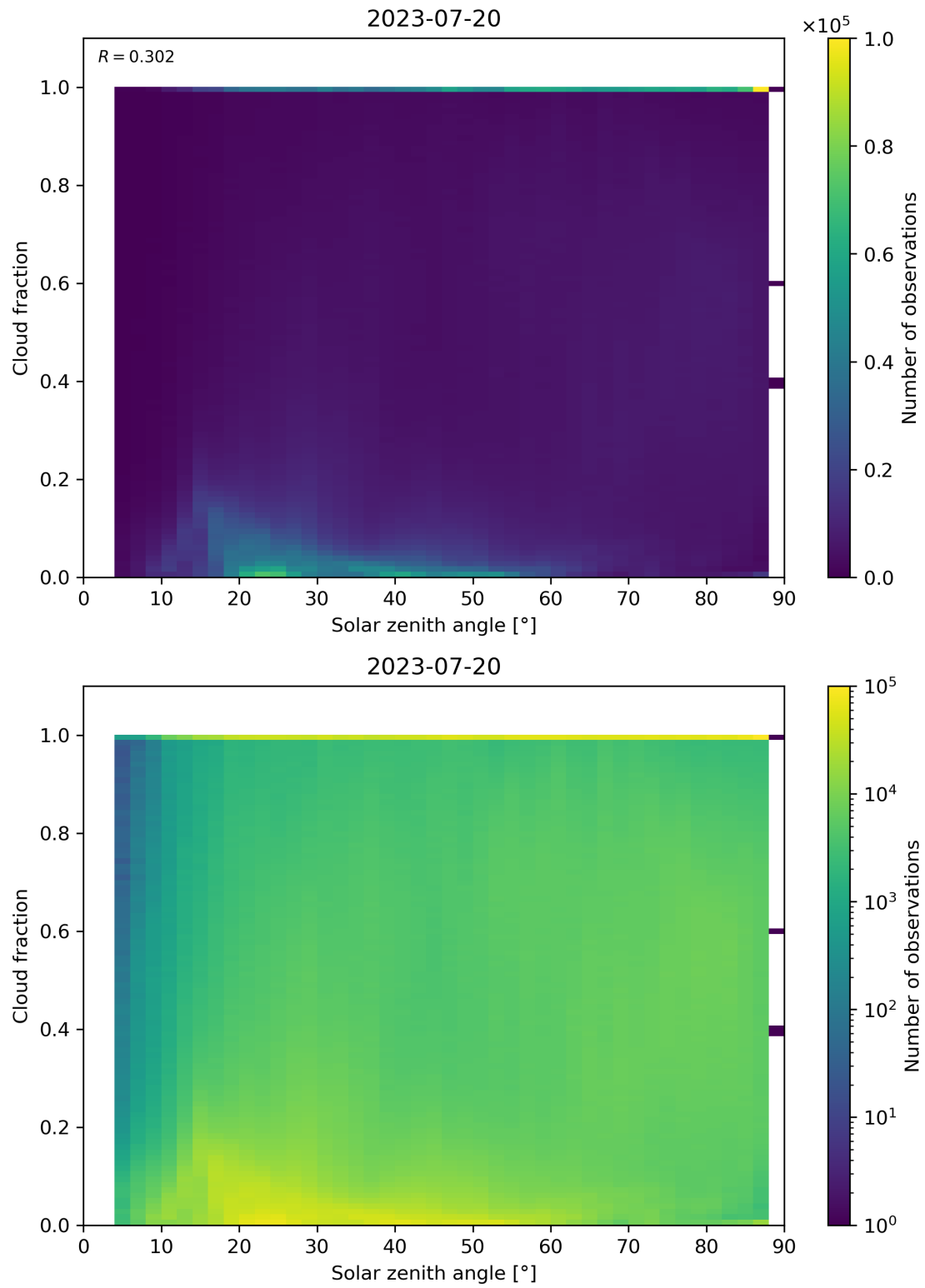
Figure 121: Scatter density plot of “Solar zenith angle” against “Cloud fraction” for 2023-07-19 to 2023-07-21.
