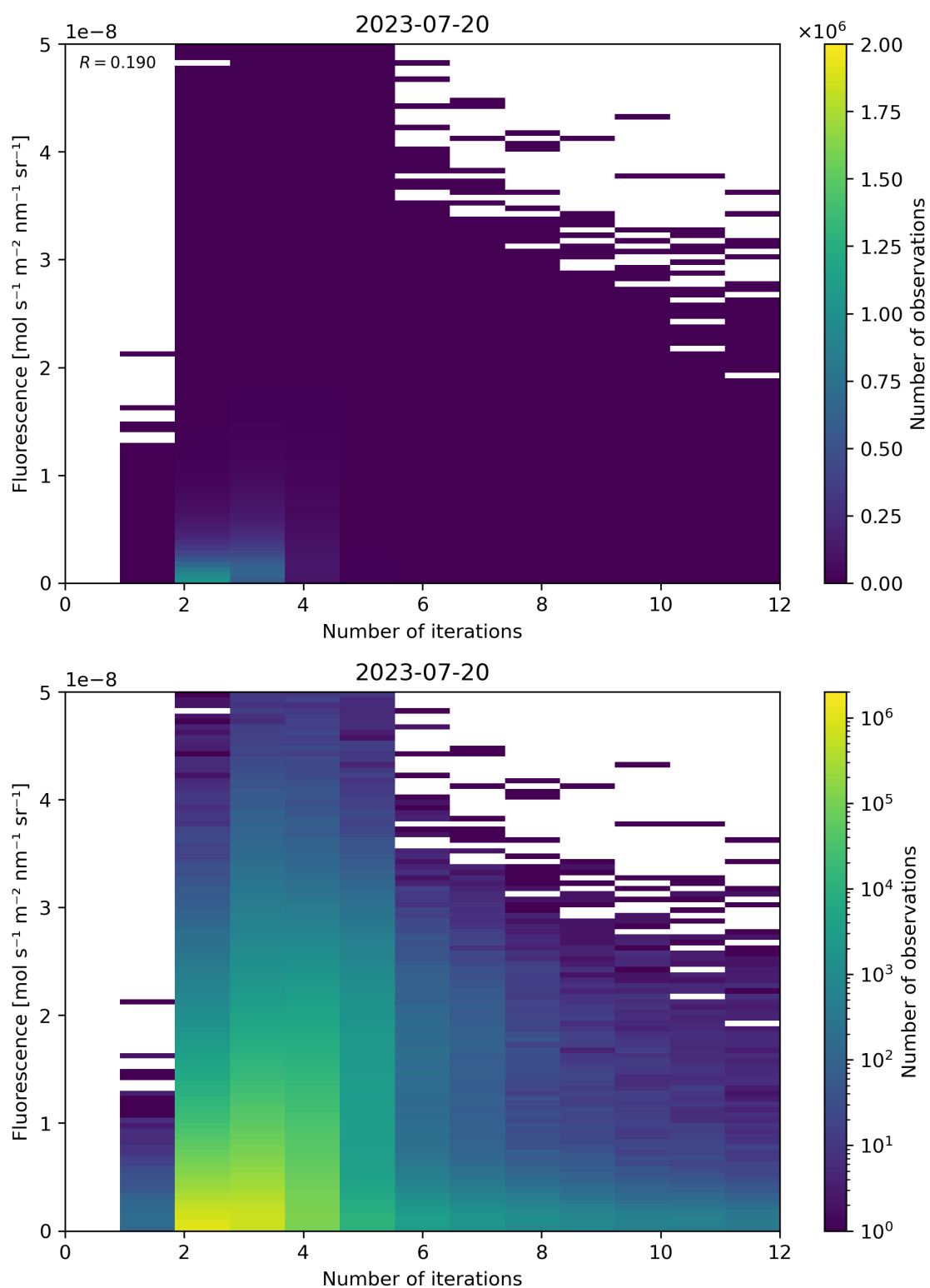
Figure 107: Scatter density plot of “Number of iterations” against “Fluorescence” for 2023-07-19 to 2023-07-21.
