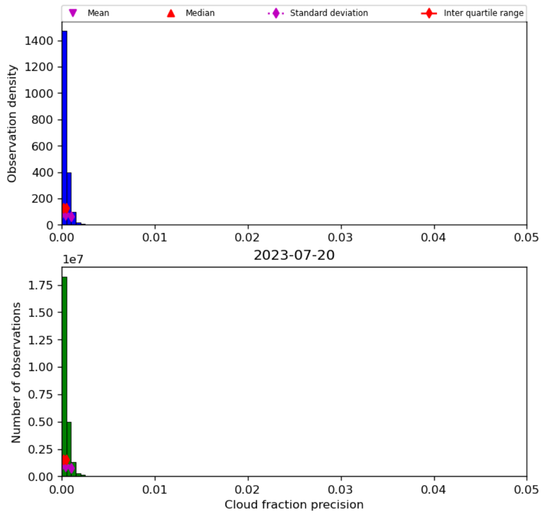
Figure 33: Histogram of “Cloud fraction precision” for 2023-07-19 to 2023-07-21
