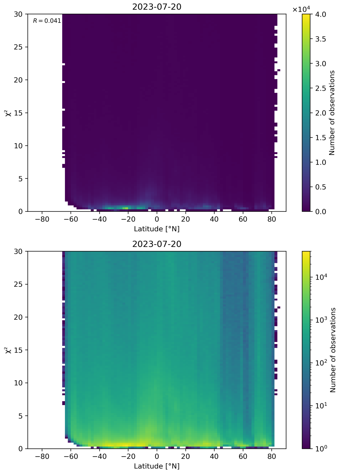
Figure 97: Scatter density plot of “Latitude” against “ \chi^2 ” for 2023-07-19 to 2023-07-21.
