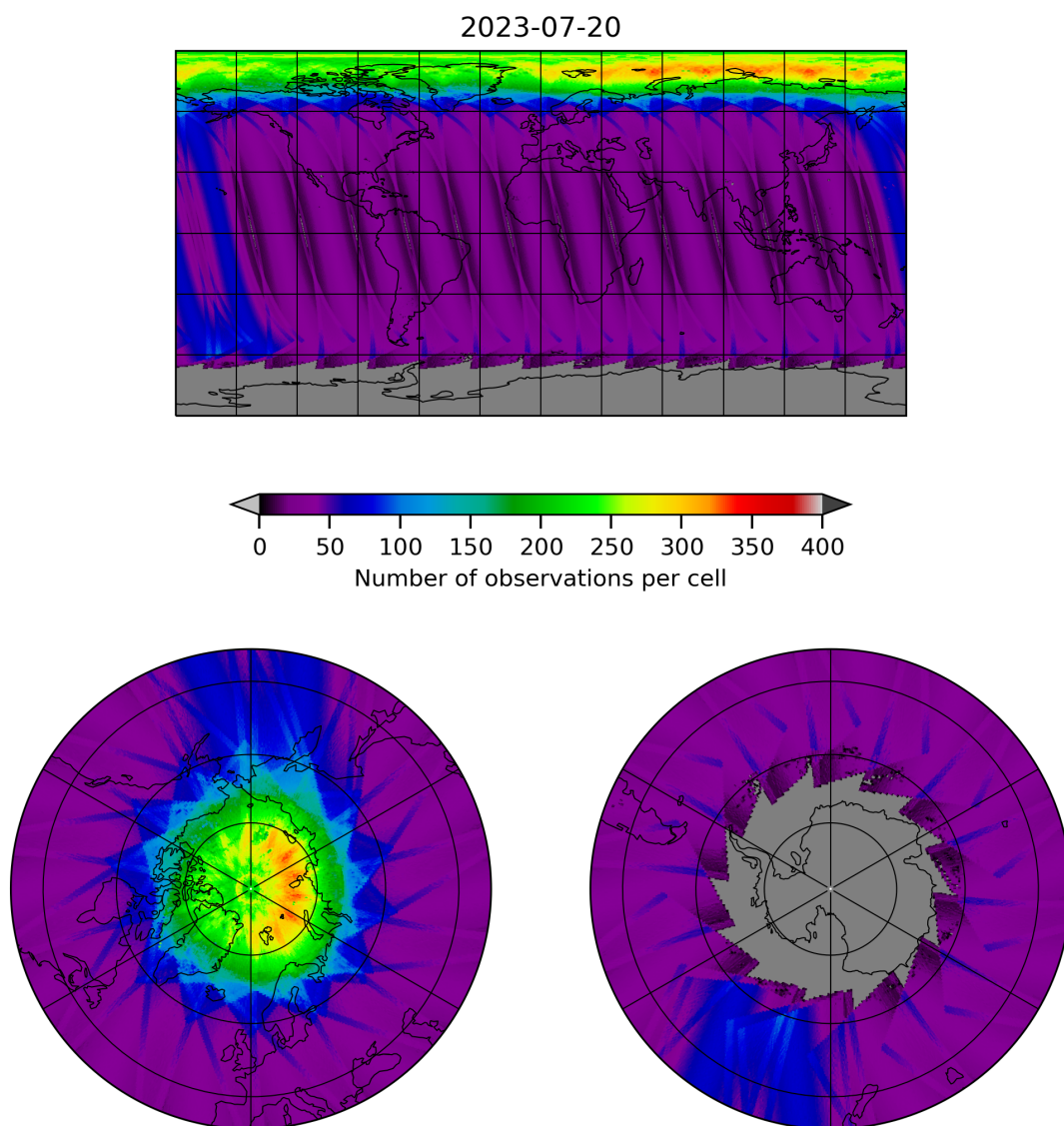
Figure 11: Map of the number of observations for 2023-07-19 to 2023-07-21
