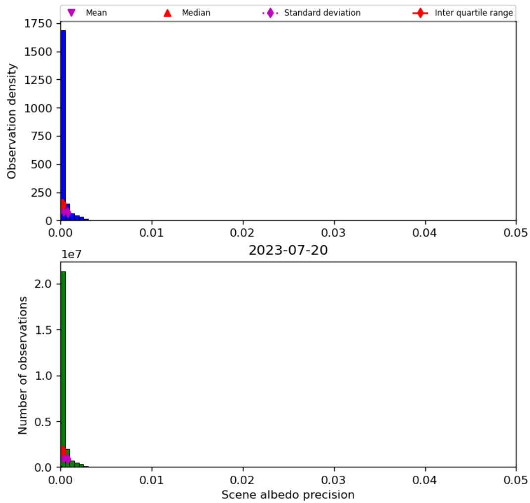
Figure 35: Histogram of “Scene albedo precision” for 2023-07-19 to 2023-07-21
