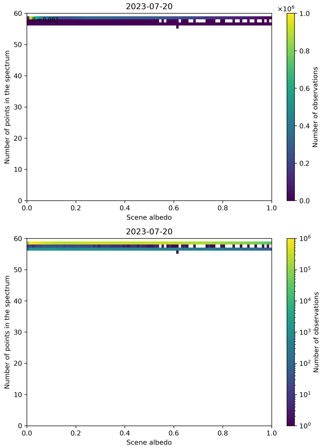
Figure 116: Scatter density plot of “Scene albedo” against “Number of points in the spectrum” for 2023-07-19 to 2023-07-21.
