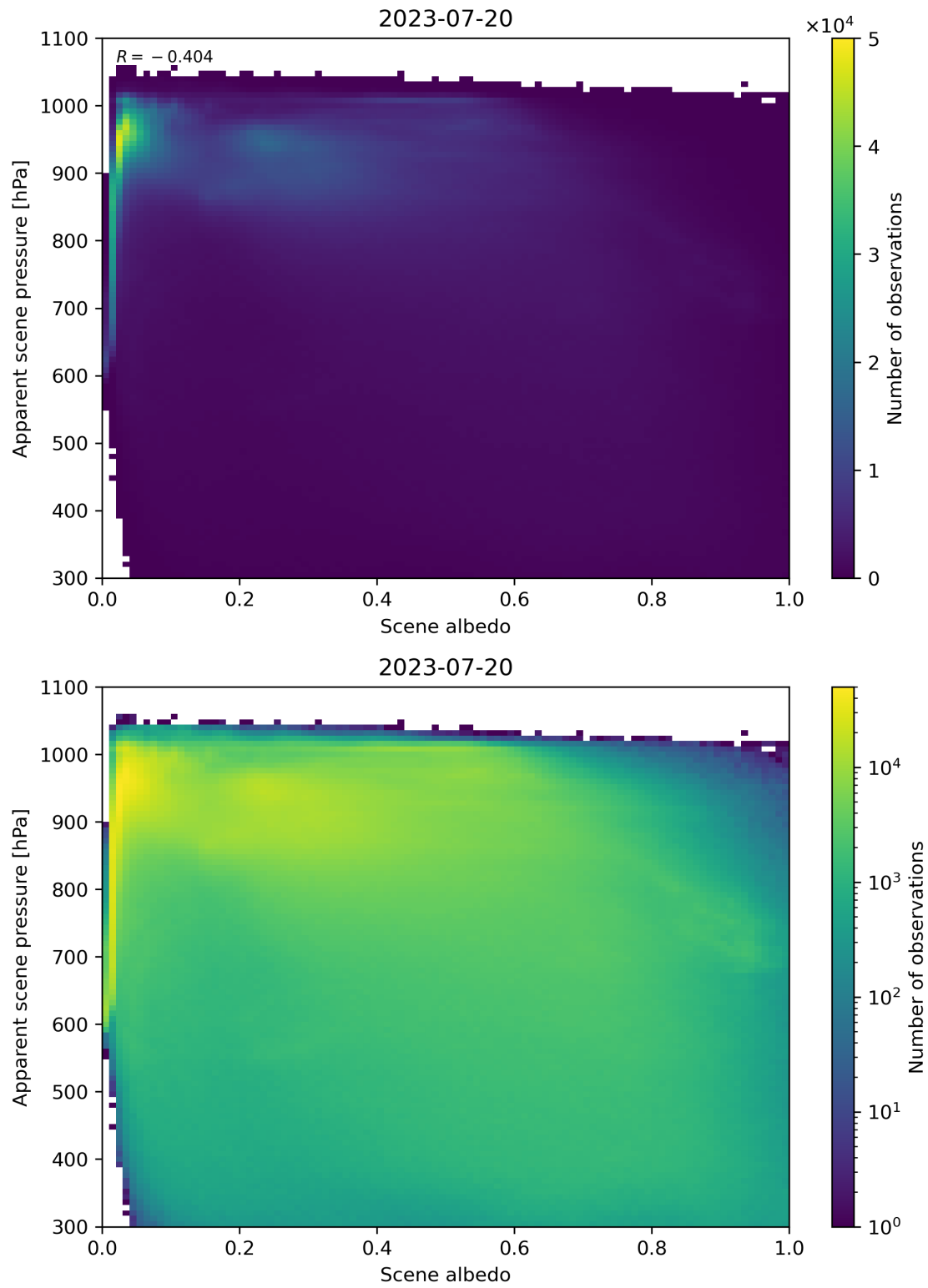
Figure 111: Scatter density plot of “Scene albedo” against “Apparent scene pressure” for 2023-07-19 to 2023-07-21.
