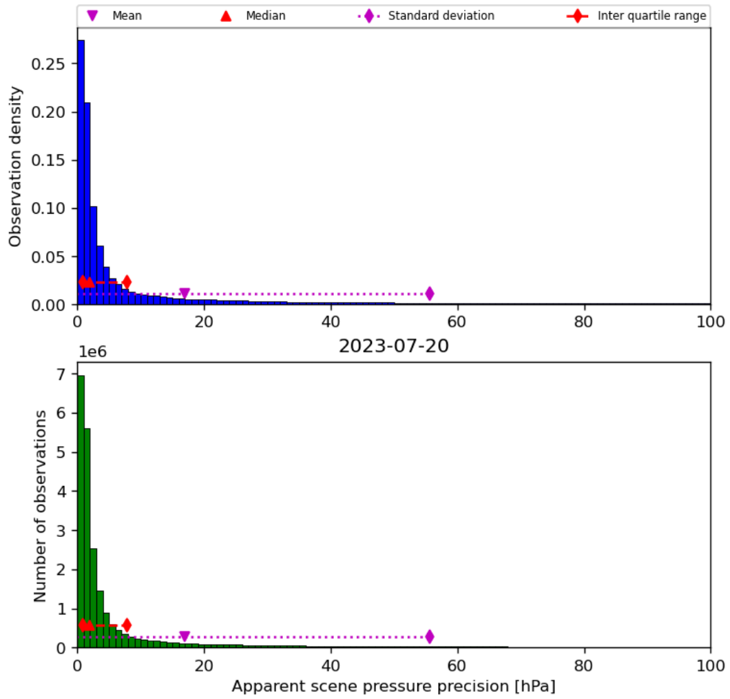
Figure 37: Histogram of “Apparent scene pressure precision” for 2023-07-19 to 2023-07-21
