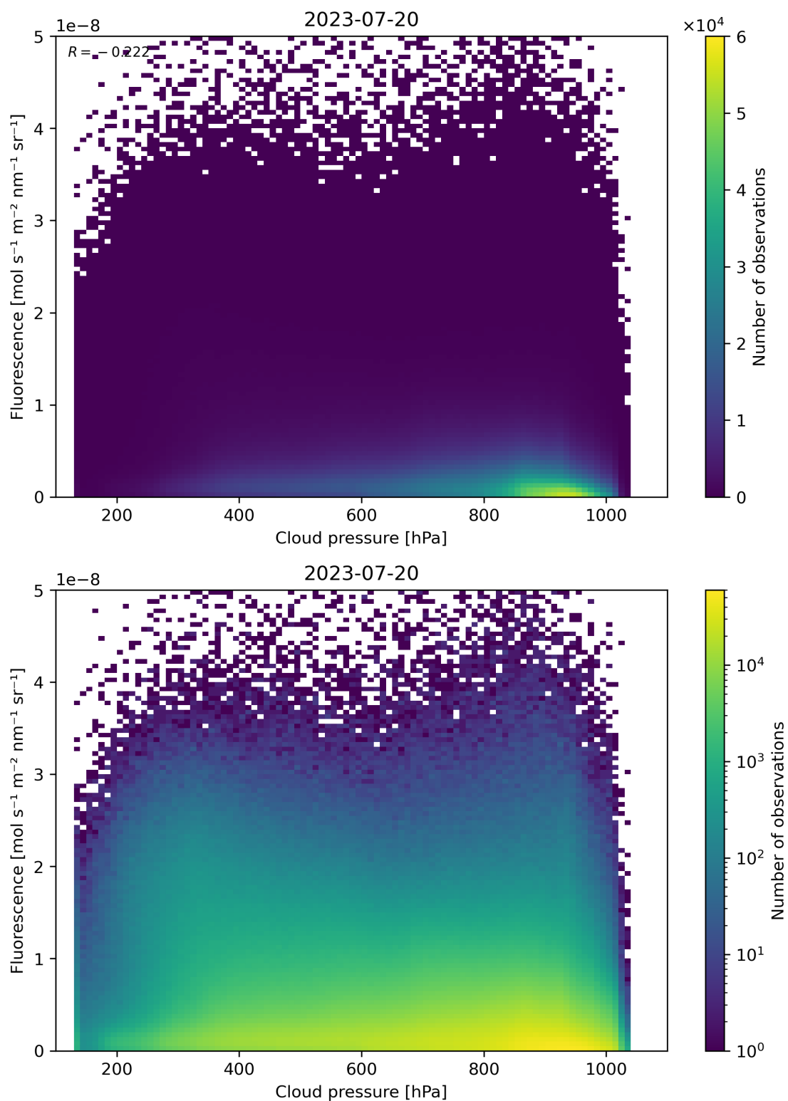
Figure 88: Scatter density plot of “Cloud pressure” against “Fluorescence” for 2023-07-19 to 2023-07-21.
