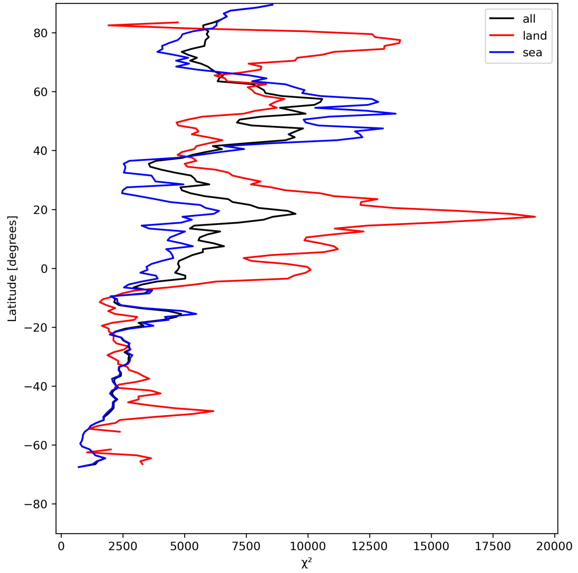
Figure 21: Zonal average of “ \chi^2 ” for 2023-07-19 to 2023-07-21.
