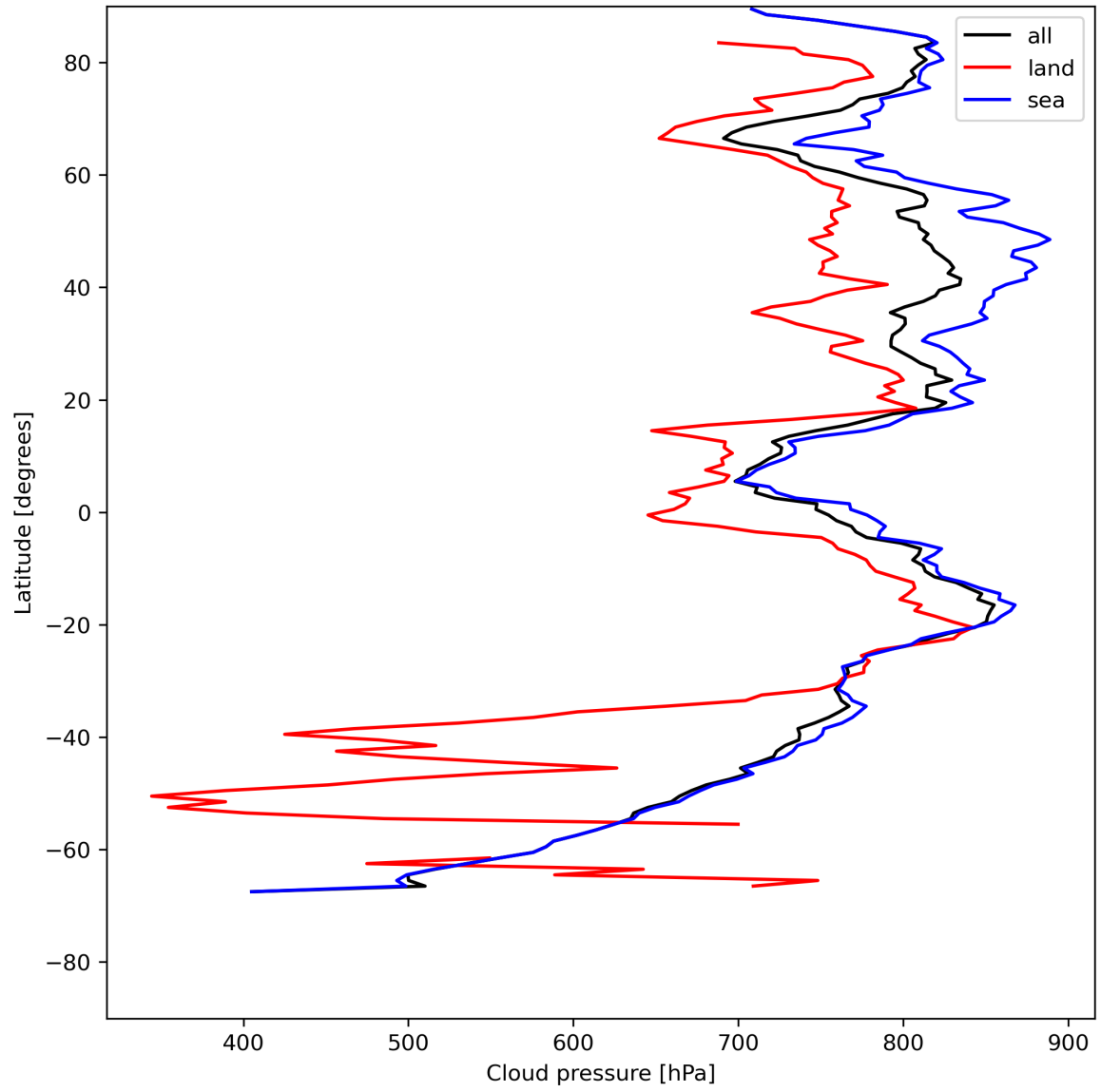
Figure 13: Zonal average of “Cloud pressure” for 2023-07-19 to 2023-07-21.
