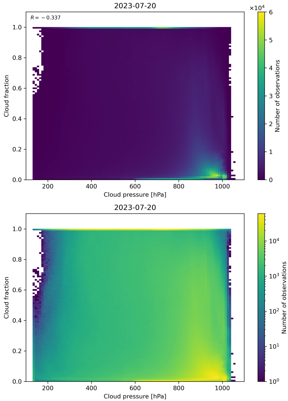
Figure 87: Scatter density plot of “Cloud pressure” against “Cloud fraction” for 2023-07-19 to 2023-07-21.
