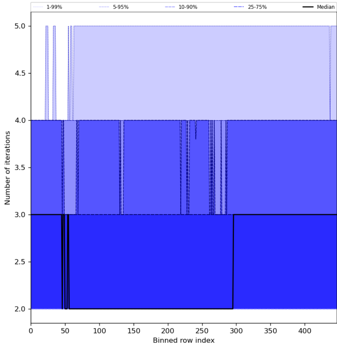
Figure 56: Along track statistics of “Number of iterations” for 2023-07-19 to 2023-07-21
