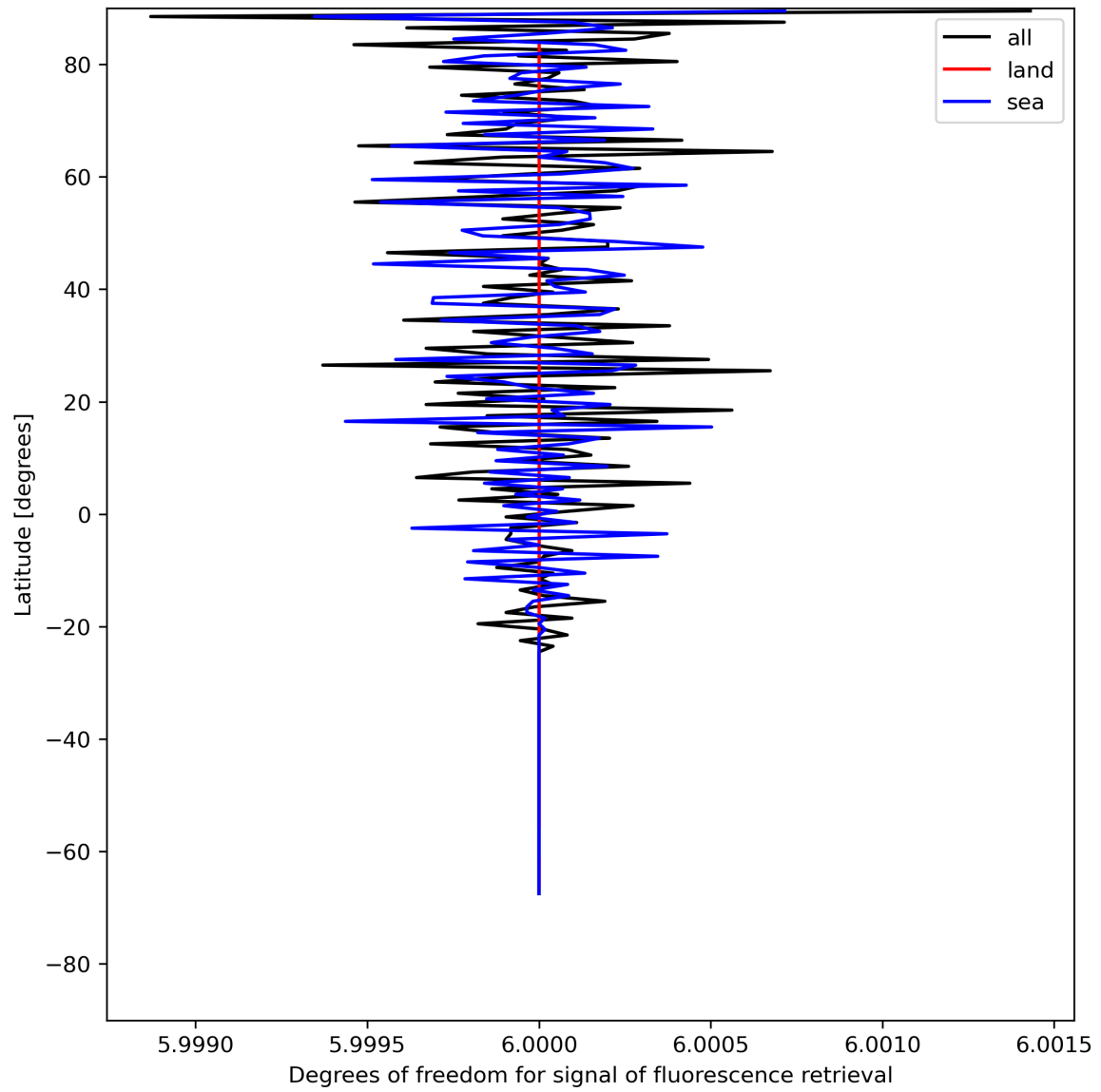
Figure 26: Zonal average of “Degrees of freedom for signal of fluorescence retrieval” for 2023-07-19 to 2023-07-21.
