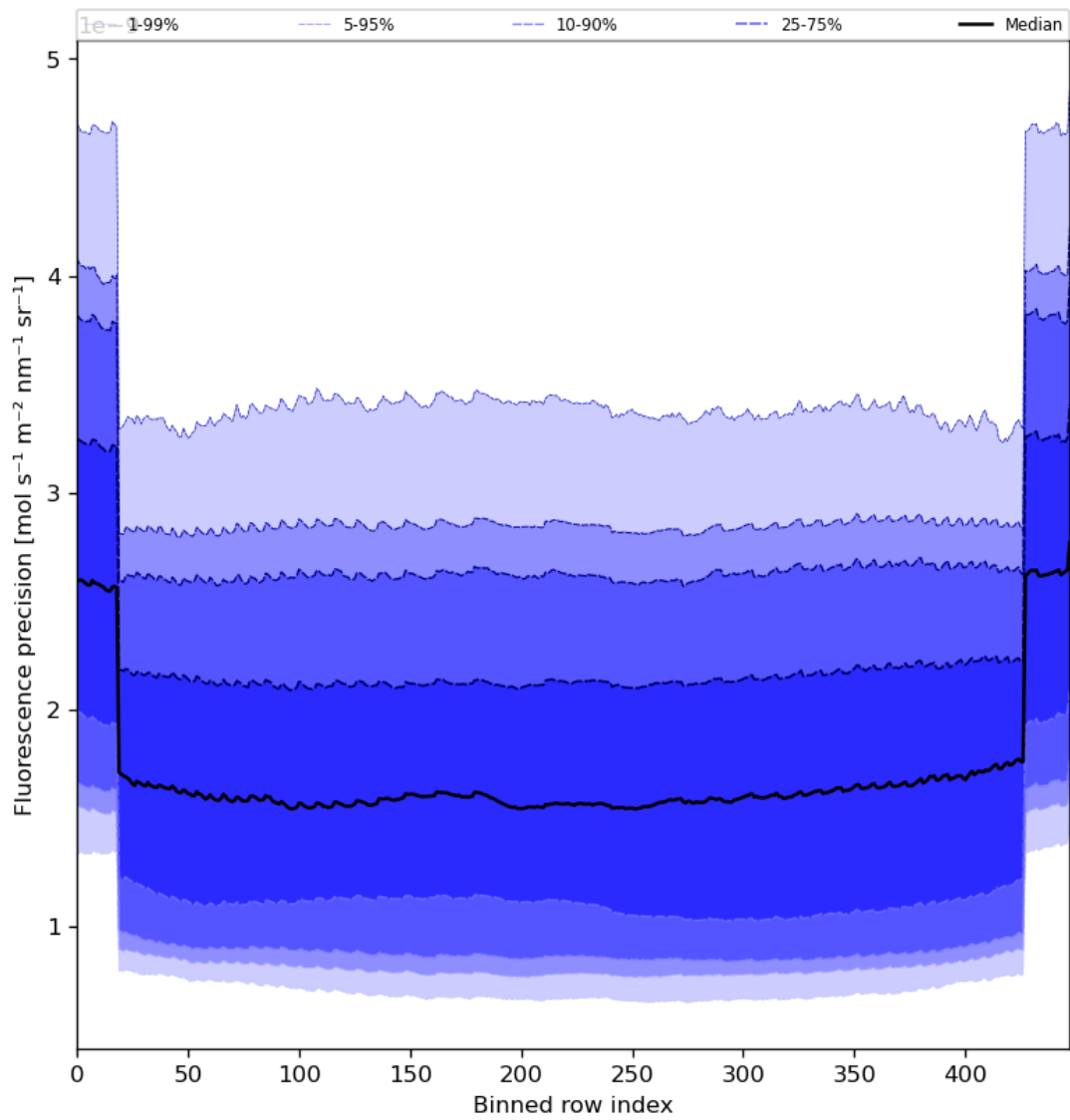
Figure 58: Along track statistics of “Fluorescence precision” for 2023-07-19 to 2023-07-21
