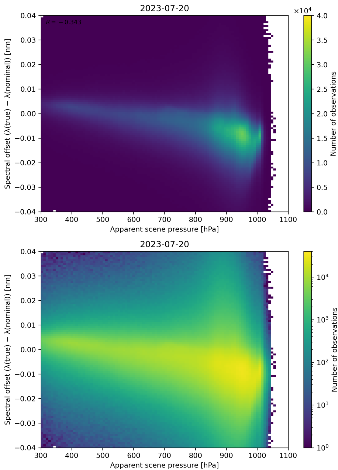
Figure 68: Scatter density plot of “Apparent scene pressure” against “Spectral offset ( \lambda(\text{true}) - \lambda(\text{nominal}) )” for 2023-07-19 to 2023-07-21.
