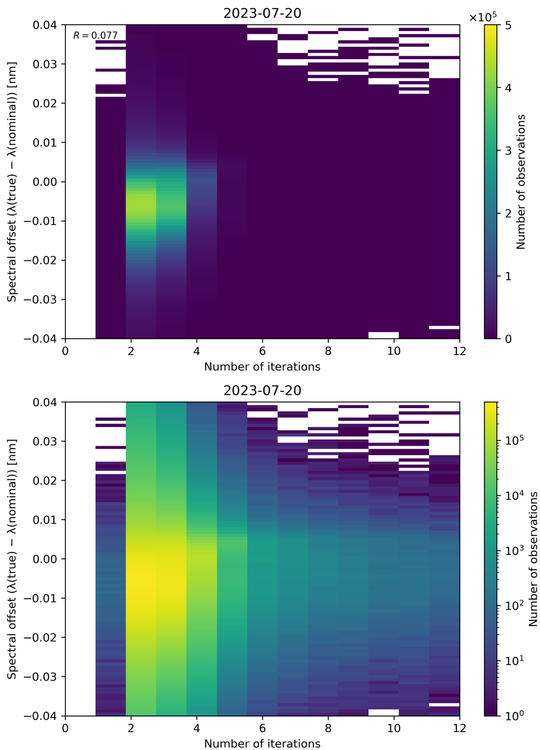
Figure 109: Scatter density plot of “Number of iterations” against “Spectral offset ( \lambda(\text{true}) - \lambda(\text{nominal}) )” for 2023-07-19 to 2023-07-21.
