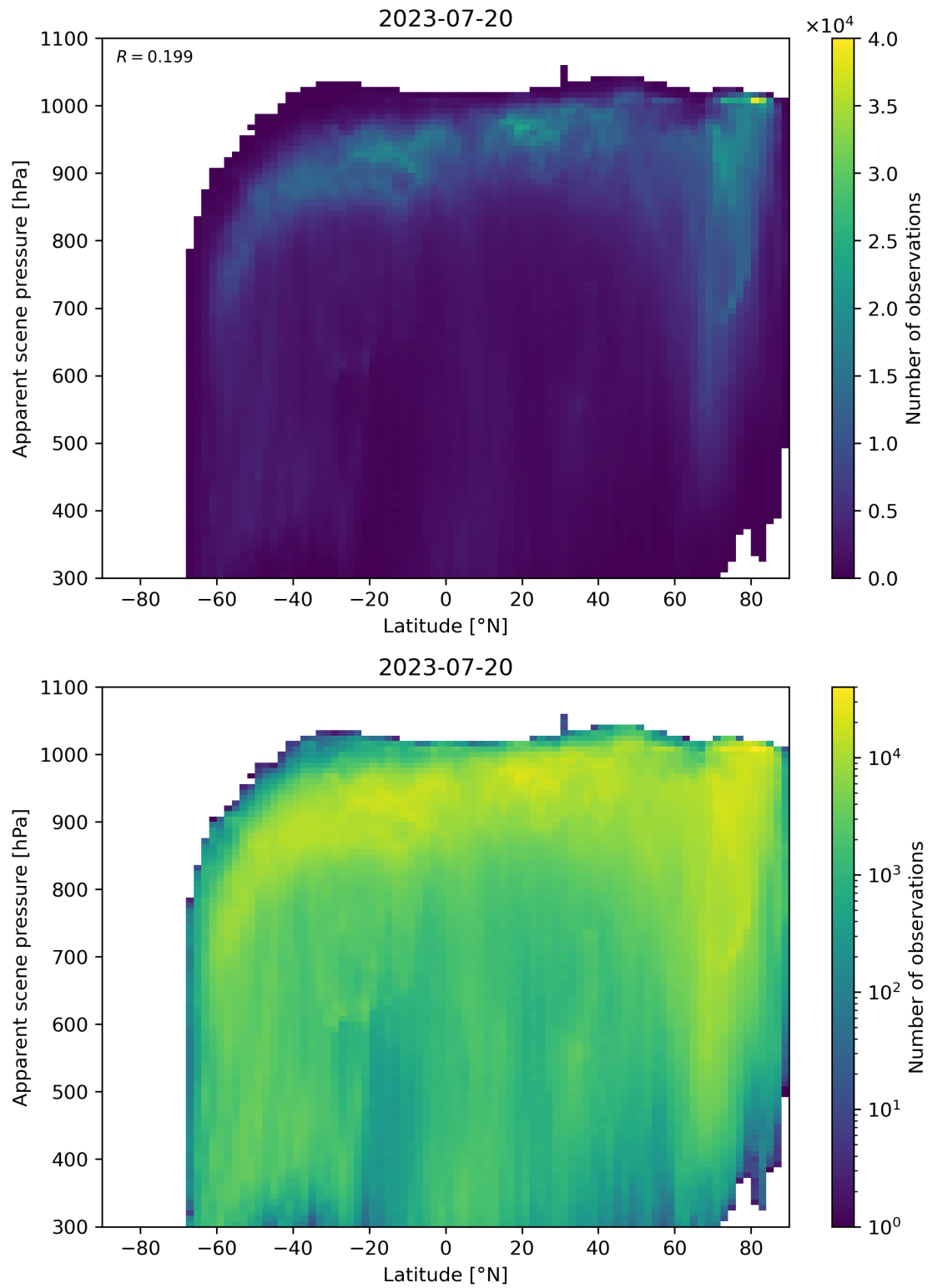
Figure 96: Scatter density plot of “Latitude” against “Apparent scene pressure” for 2023-07-19 to 2023-07-21.
