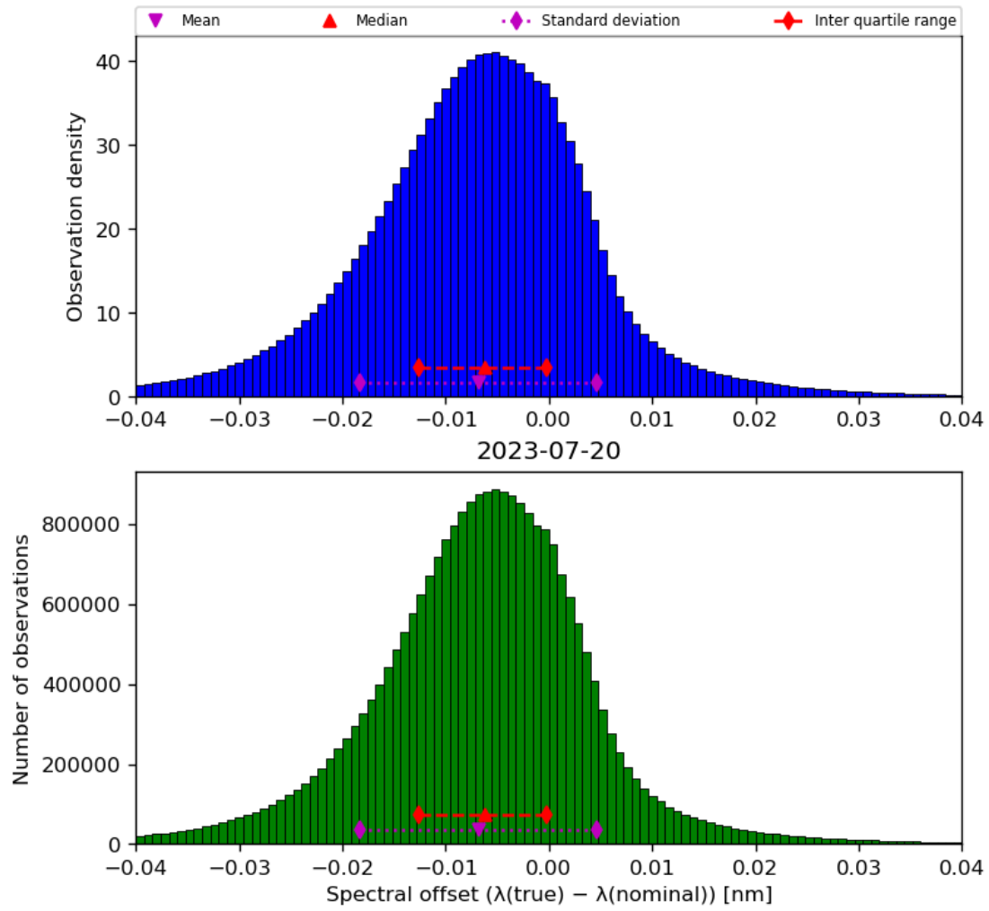
Figure 45: Histogram of “Spectral offset ( \lambda(\text{true}) - \lambda(\text{nominal}) )” for 2023-07-19 to 2023-07-21
