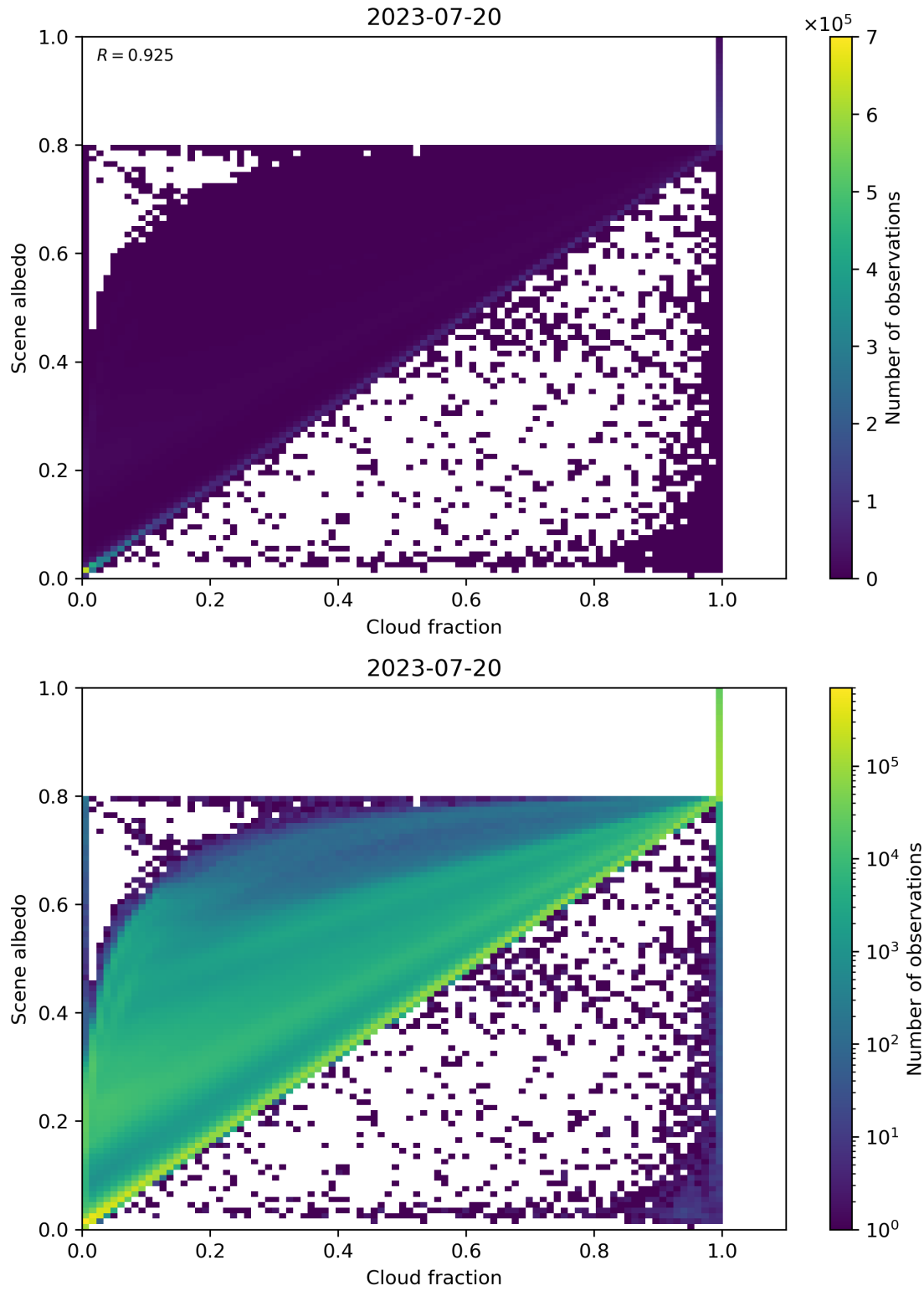
Figure 82: Scatter density plot of “Cloud fraction” against “Scene albedo” for 2023-07-19 to 2023-07-21.
