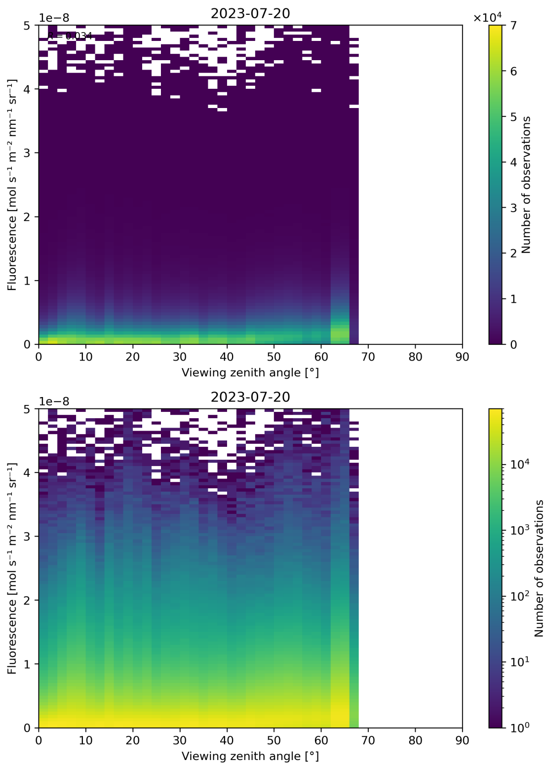
Figure 134: Scatter density plot of “Viewing zenith angle” against “Fluorescence” for 2023-07-19 to 2023-07-21.
