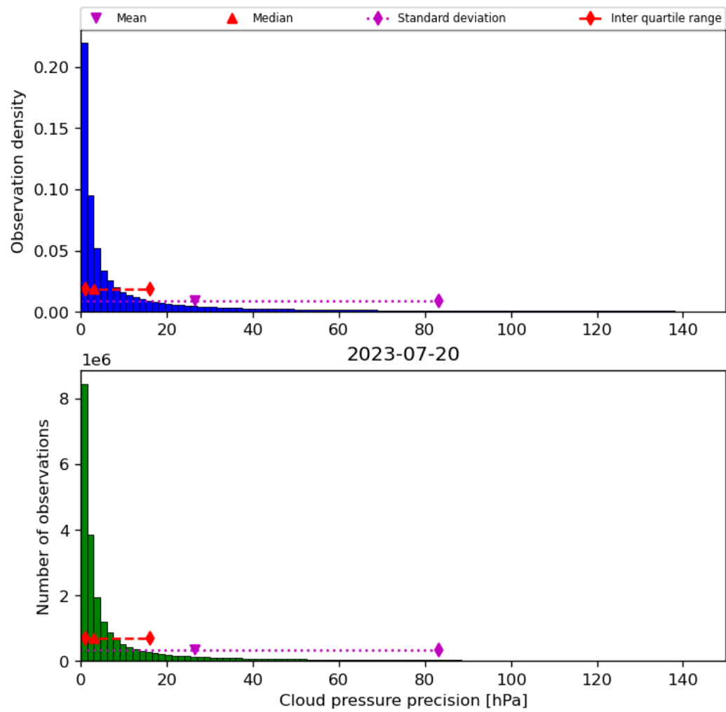
Figure 31: Histogram of “Cloud pressure precision” for 2023-07-19 to 2023-07-21
