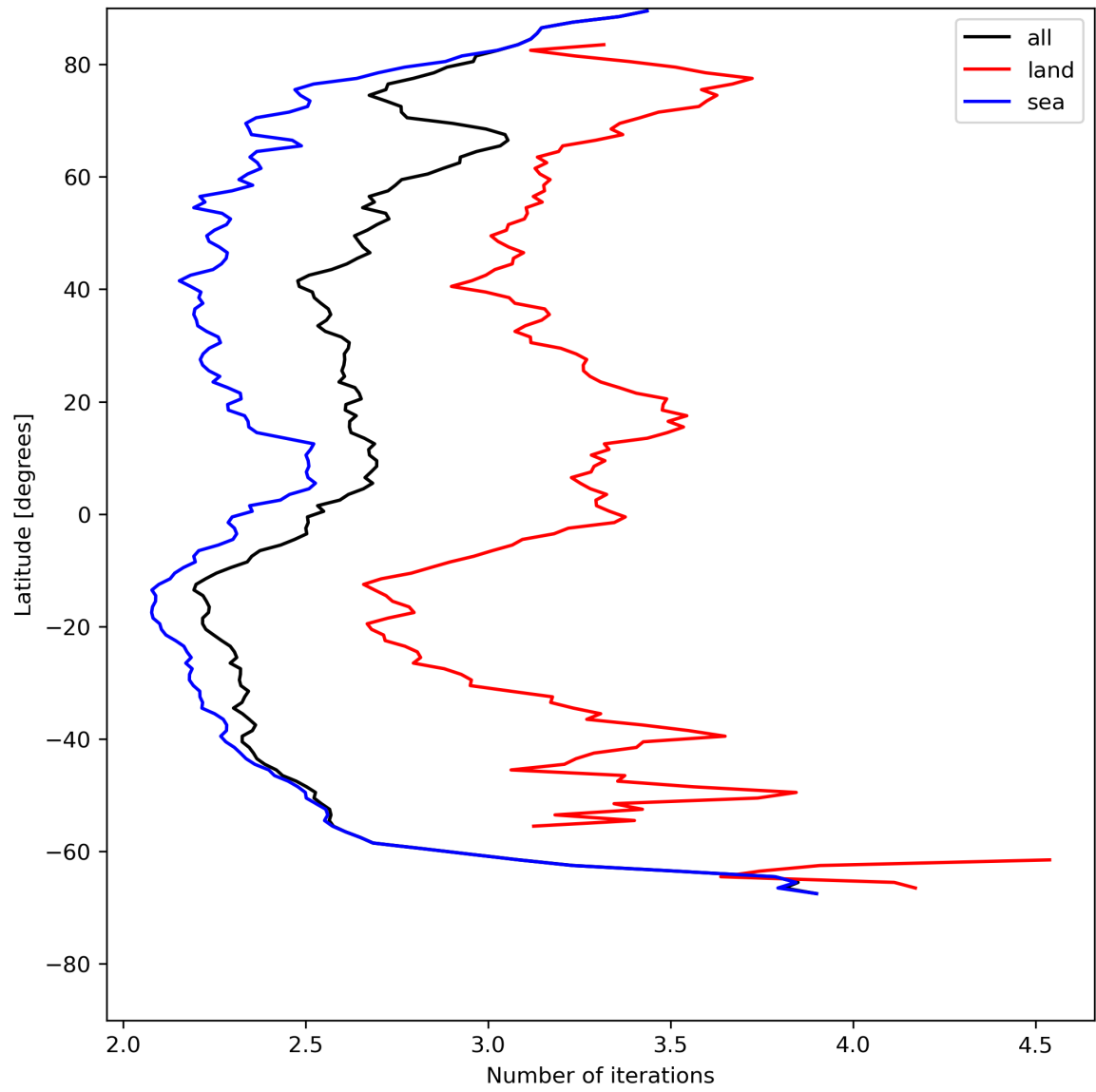
Figure 22: Zonal average of “Number of iterations” for 2023-07-19 to 2023-07-21.
