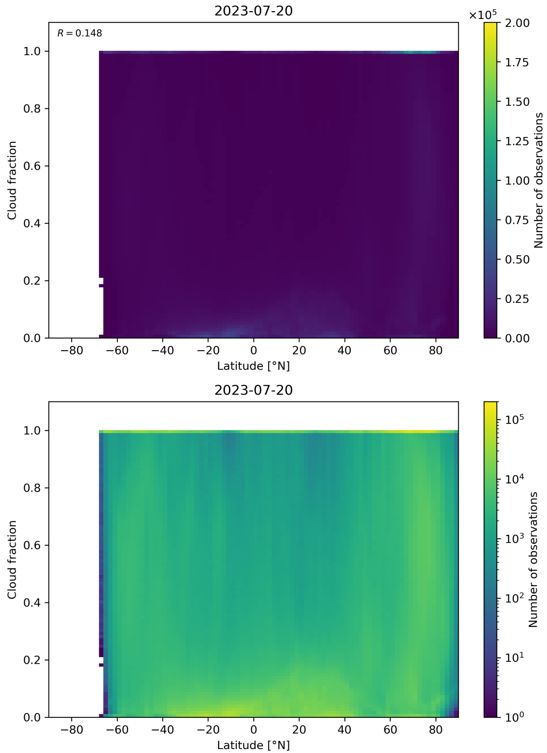
Figure 99: Scatter density plot of “Latitude” against “Cloud fraction” for 2023-07-19 to 2023-07-21.
