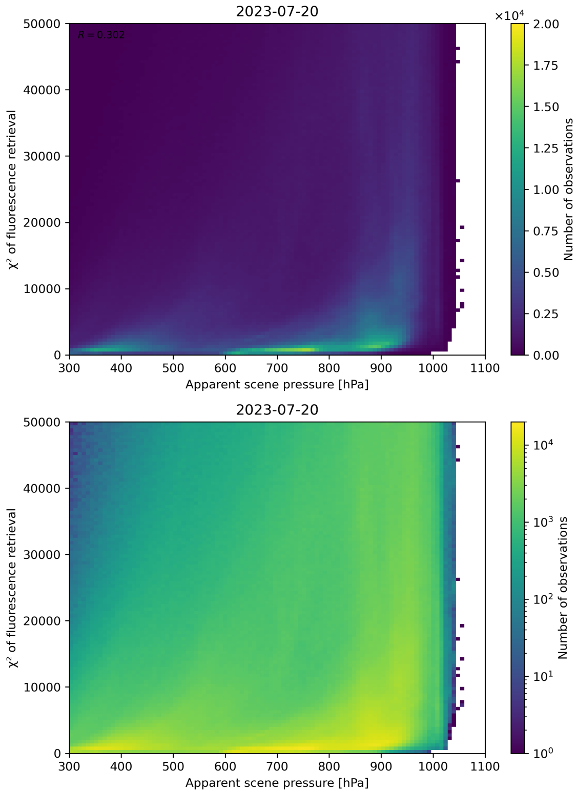
Figure 64: Scatter density plot of “Apparent scene pressure” against “ \chi^2 of fluorescence retrieval” for 2023-07-19 to 2023-07-21.
