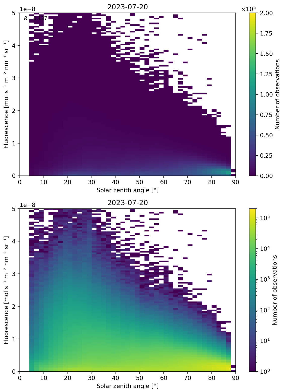
Figure 123: Scatter density plot of “Solar zenith angle” against “Fluorescence” for 2023-07-19 to 2023-07-21.
