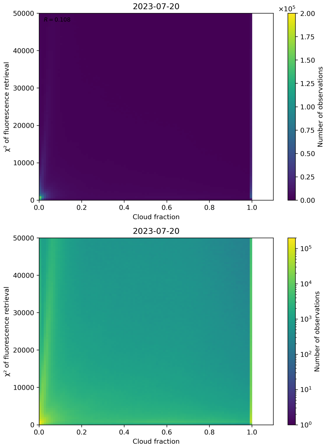
Figure 78: Scatter density plot of “Cloud fraction” against “ \chi^2 of fluorescence retrieval” for 2023-07-19 to 2023-07-21.
