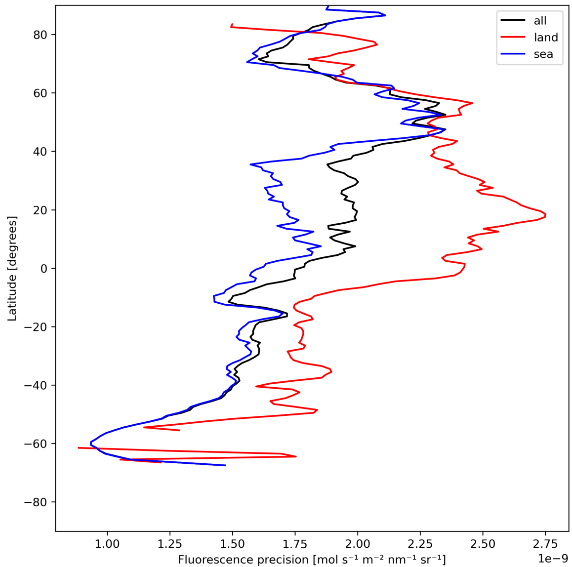
Figure 24: Zonal average of “Fluorescence precision” for 2023-07-19 to 2023-07-21.
