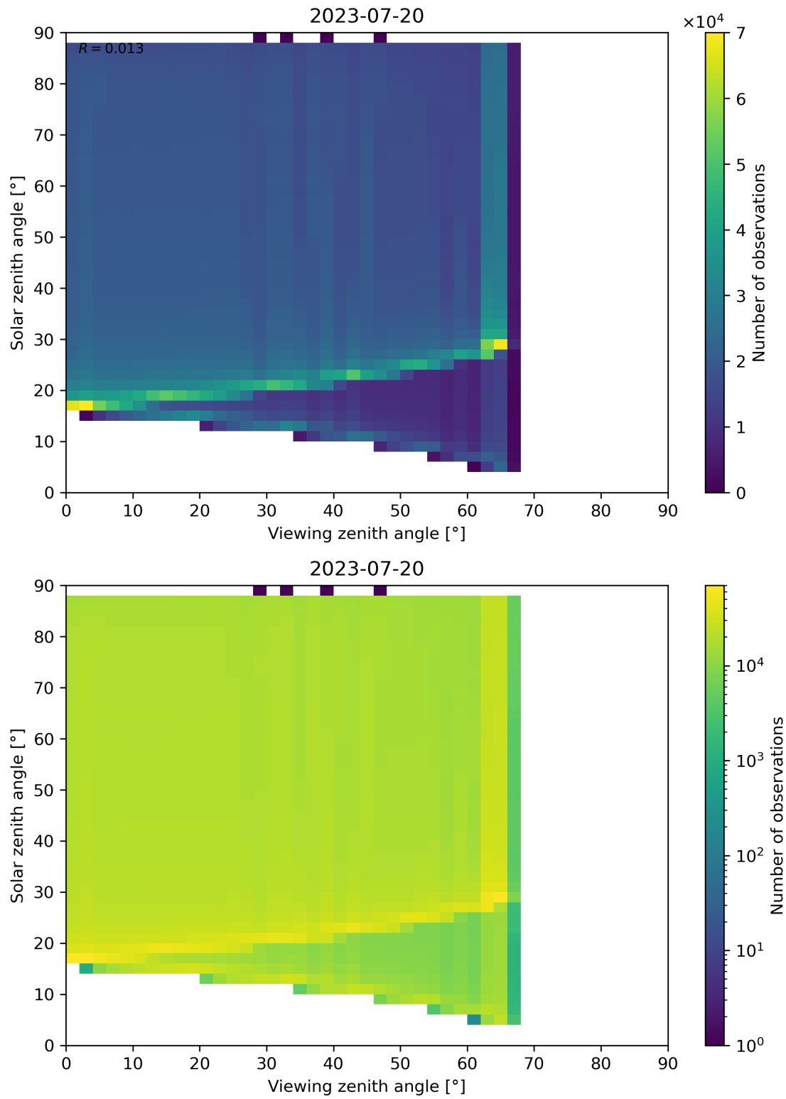
Figure 139: Scatter density plot of “Viewing zenith angle” against “Solar zenith angle” for 2023-07-19 to 2023-07-21.
