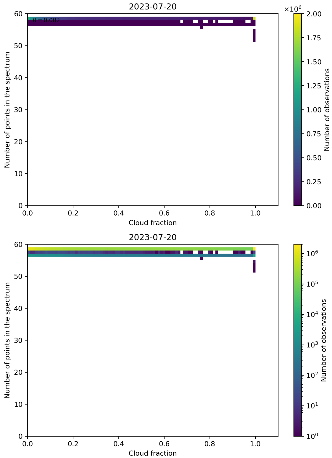
Figure 81: Scatter density plot of “Cloud fraction” against “Number of points in the spectrum” for 2023-07-19 to 2023-07-21.
