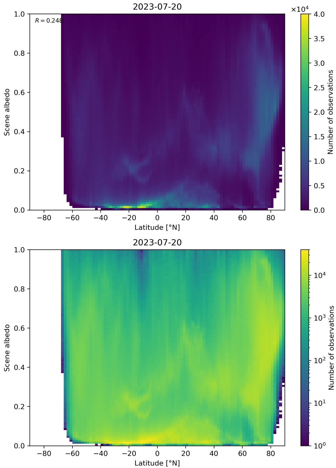
Figure 104: Scatter density plot of “Latitude” against “Scene albedo” for 2023-07-19 to 2023-07-21.
