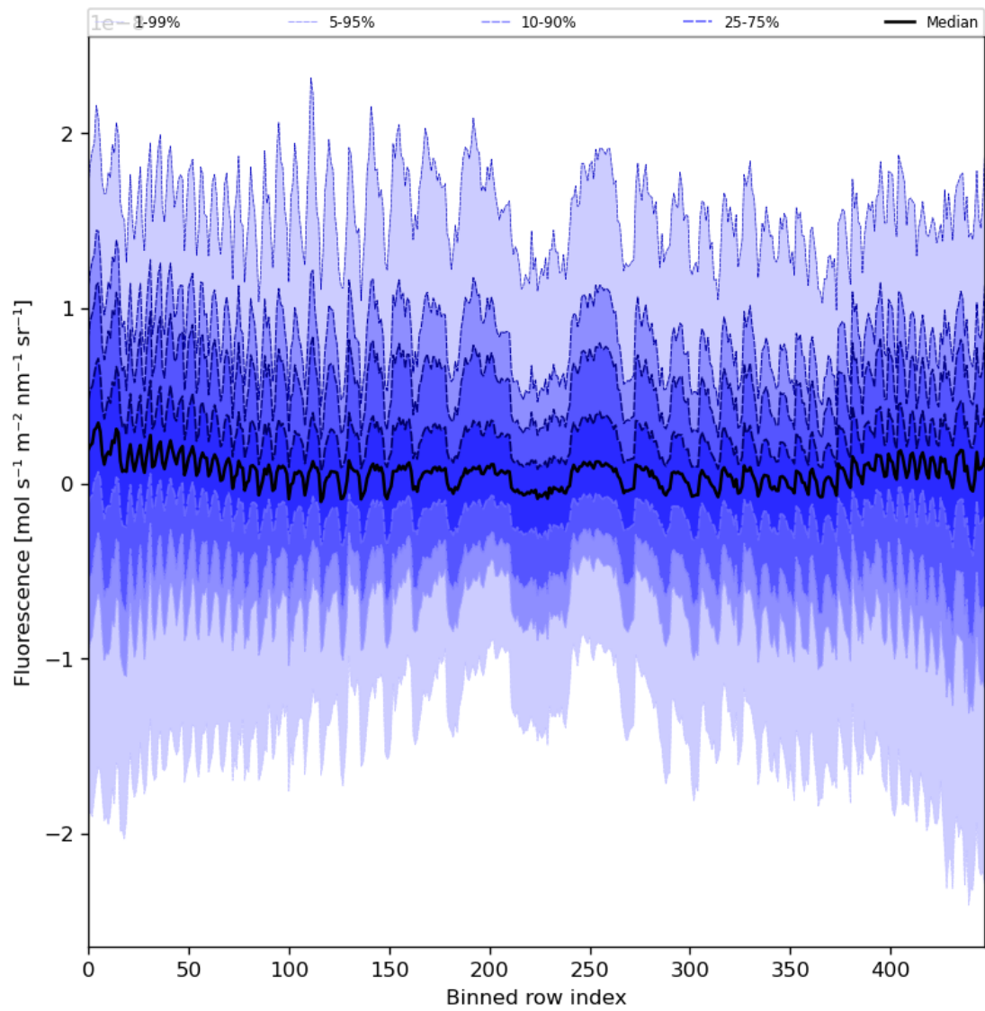
Figure 57: Along track statistics of “Fluorescence” for 2023-07-19 to 2023-07-21
