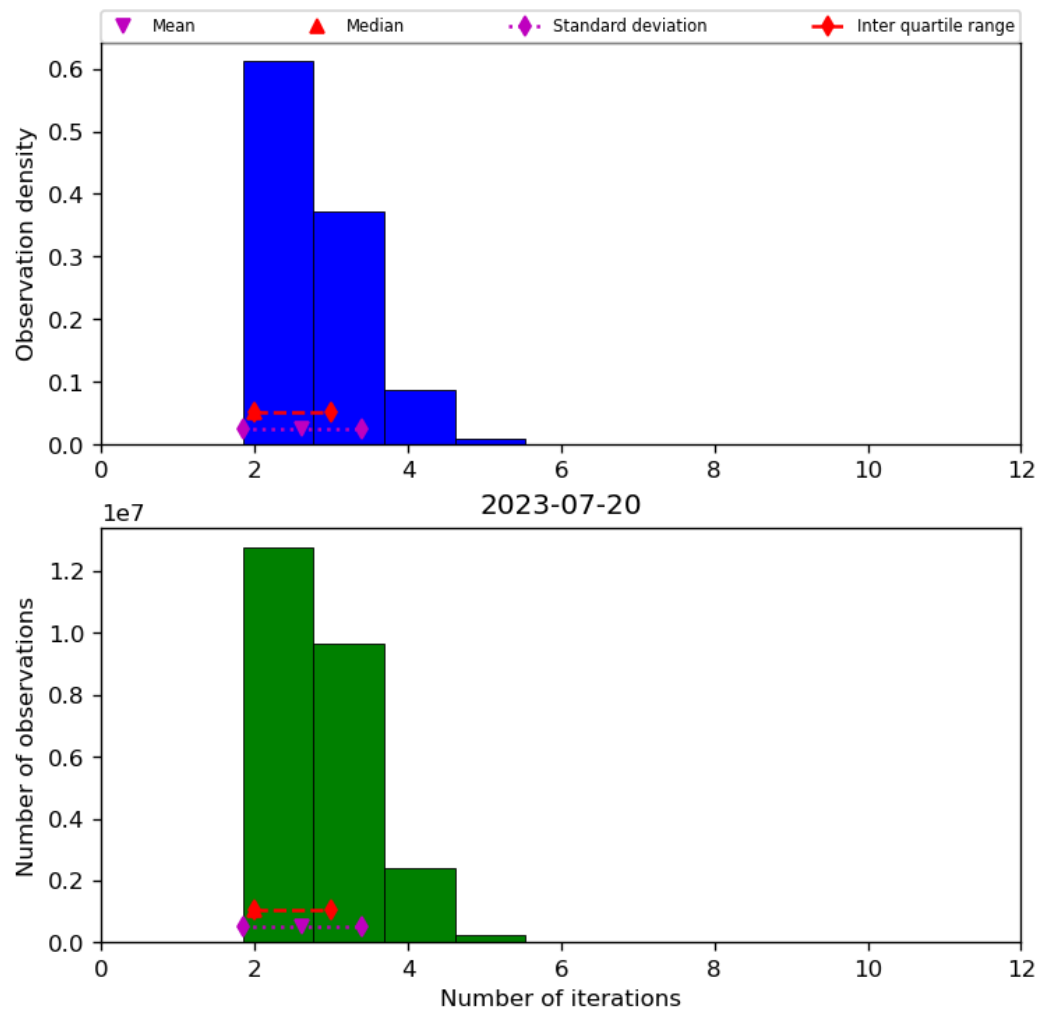
Figure 39: Histogram of “Number of iterations” for 2023-07-19 to 2023-07-21
