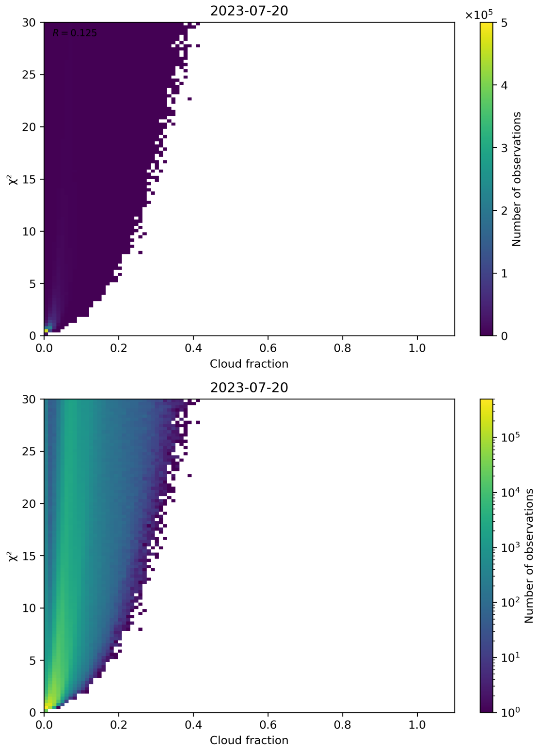
Figure 77: Scatter density plot of “Cloud fraction” against “ \chi^2 ” for 2023-07-19 to 2023-07-21.
