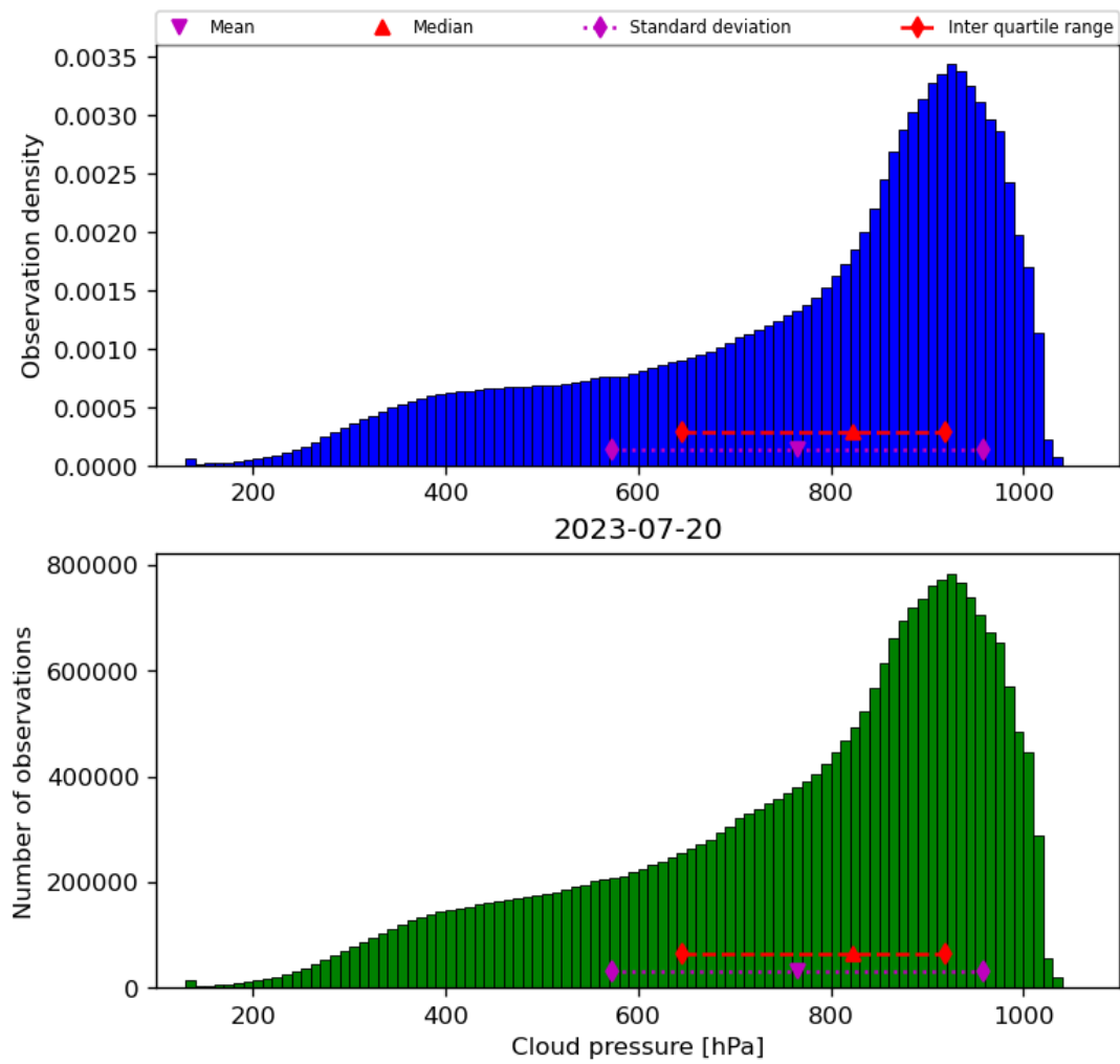
Figure 30: Histogram of “Cloud pressure” for 2023-07-19 to 2023-07-21
