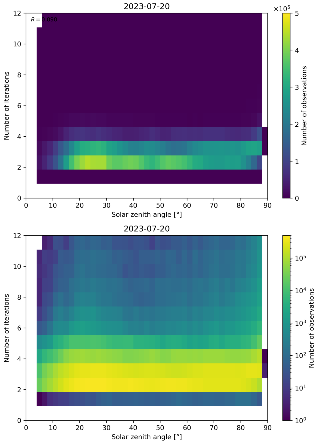
Figure 125: Scatter density plot of “Solar zenith angle” against “Number of iterations” for 2023-07-19 to 2023-07-21.
