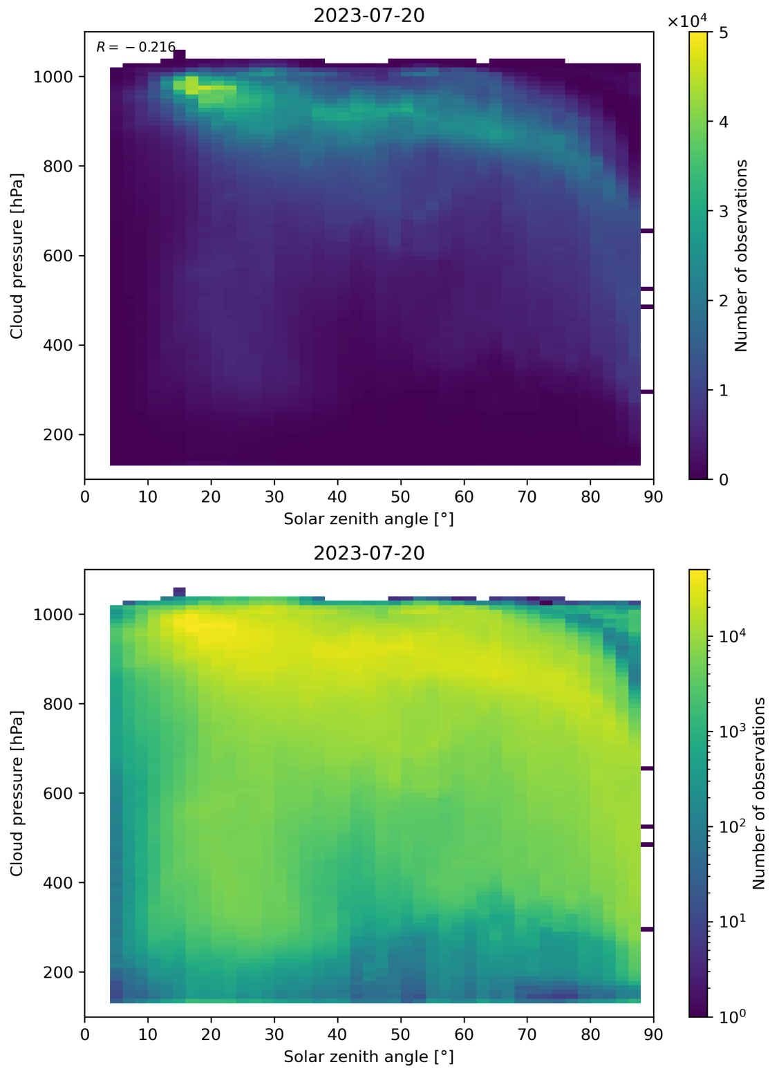
Figure 122: Scatter density plot of “Solar zenith angle” against “Cloud pressure” for 2023-07-19 to 2023-07-21.
