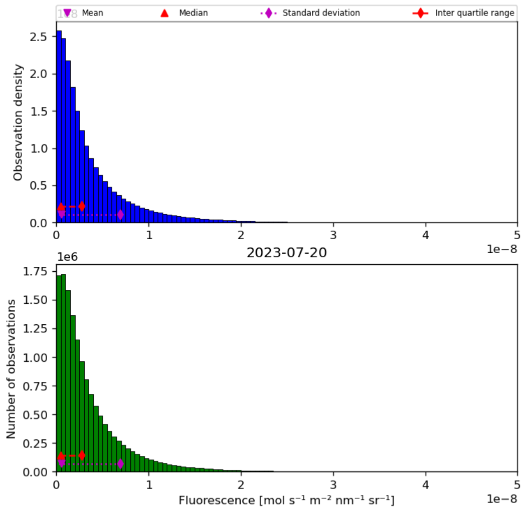
Figure 40: Histogram of “Fluorescence” for 2023-07-19 to 2023-07-21
