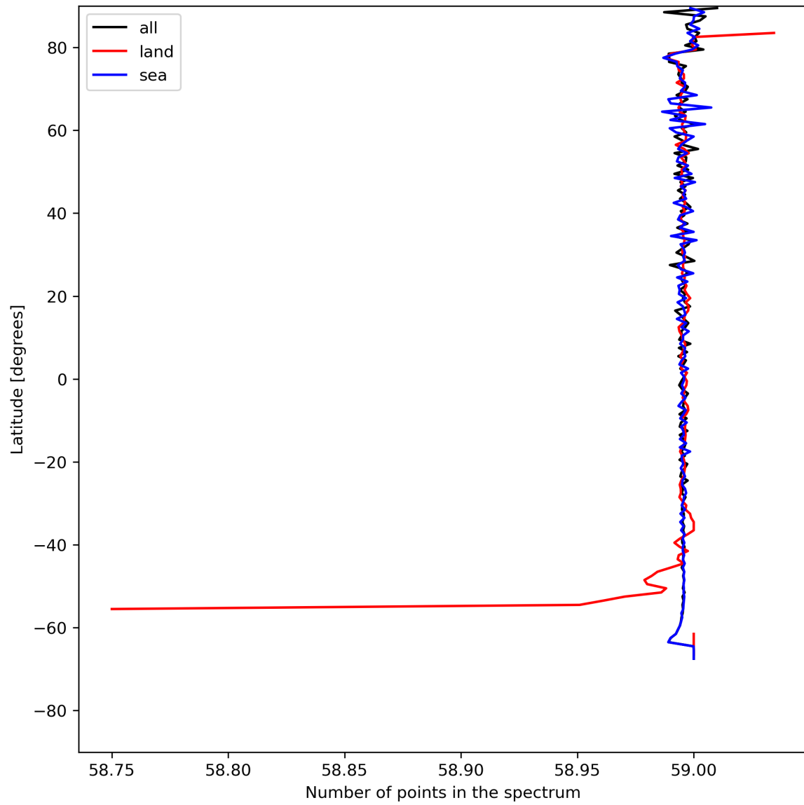
Figure 27: Zonal average of “Number of points in the spectrum” for 2023-07-19 to 2023-07-21.
