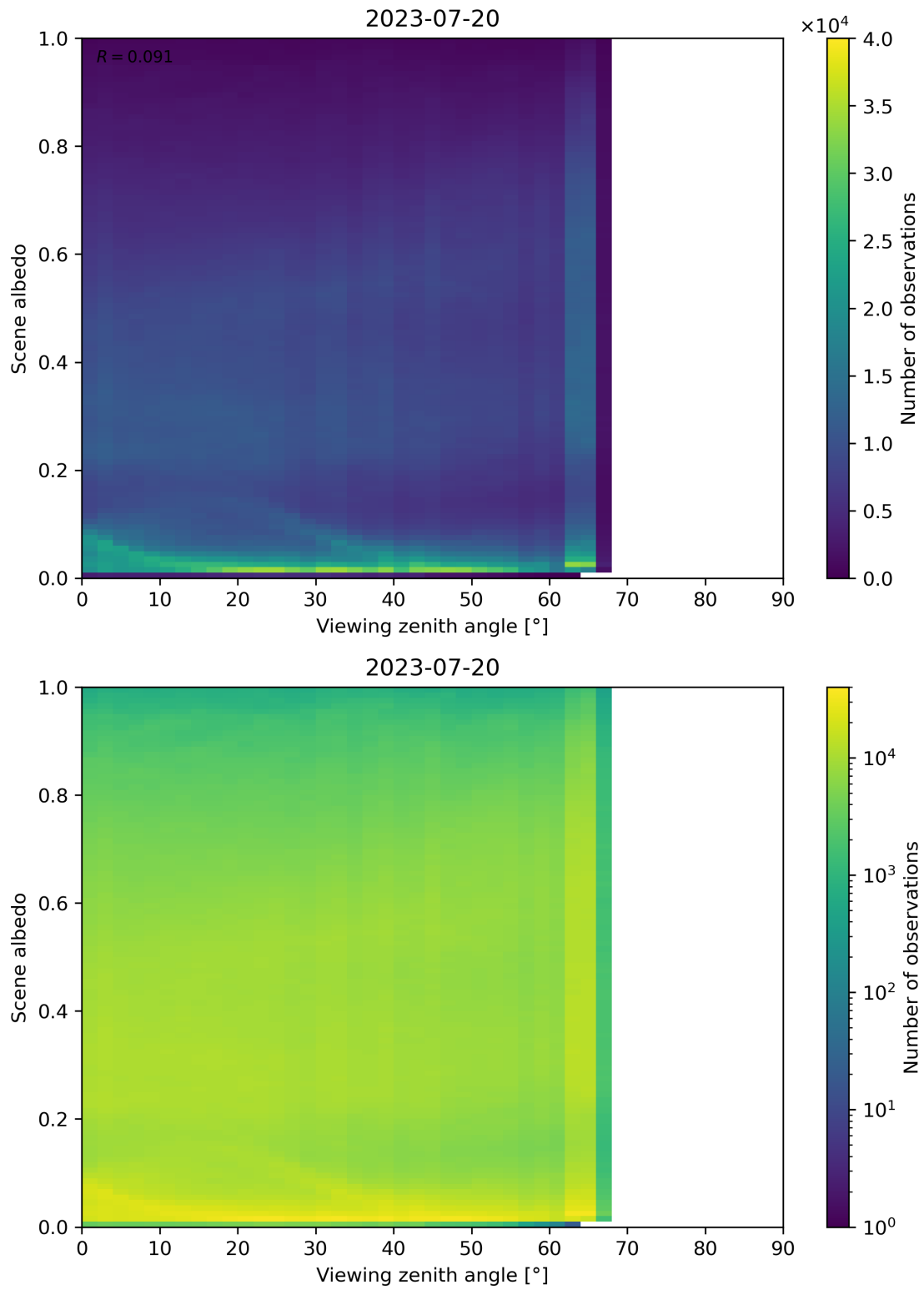
Figure 138: Scatter density plot of “Viewing zenith angle” against “Scene albedo” for 2023-07-19 to 2023-07-21.
