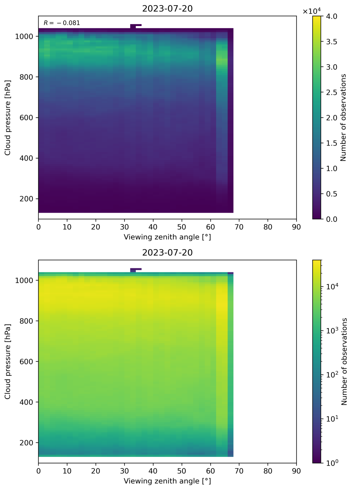
Figure 133: Scatter density plot of “Viewing zenith angle” against “Cloud pressure” for 2023-07-19 to 2023-07-21.
