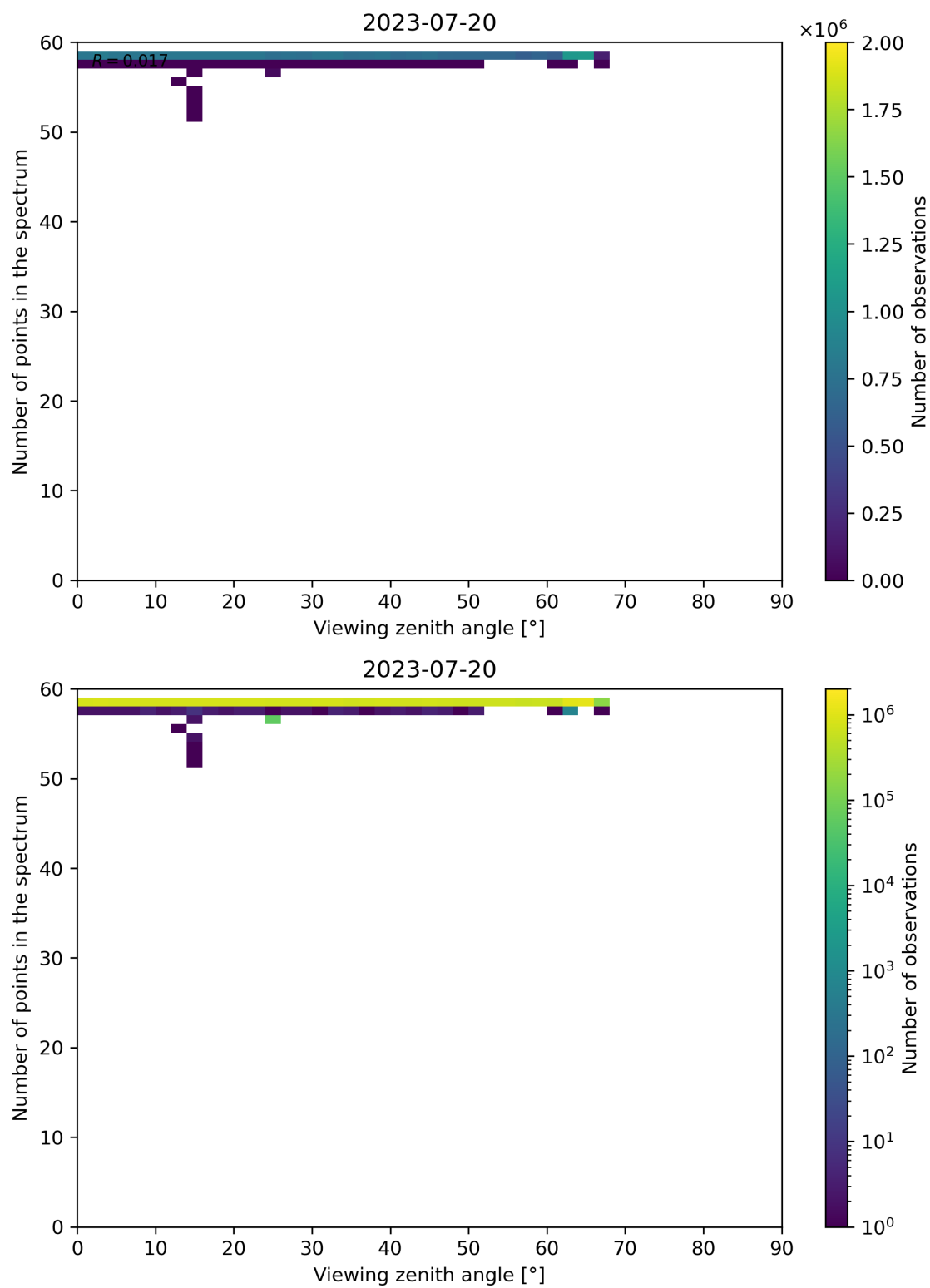
Figure 137: Scatter density plot of “Viewing zenith angle” against “Number of points in the spectrum” for 2023-07-19 to 2023-07-21.
