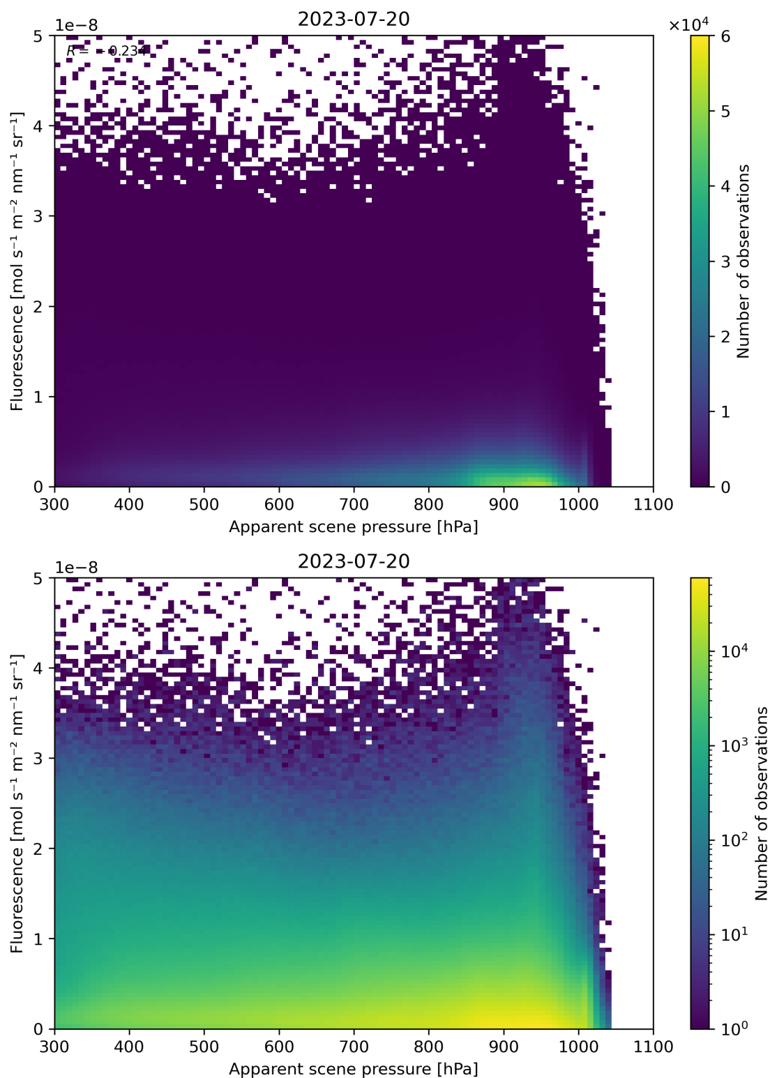
Figure 65: Scatter density plot of “Apparent scene pressure” against “Fluorescence” for 2023-07-19 to 2023-07-21.
