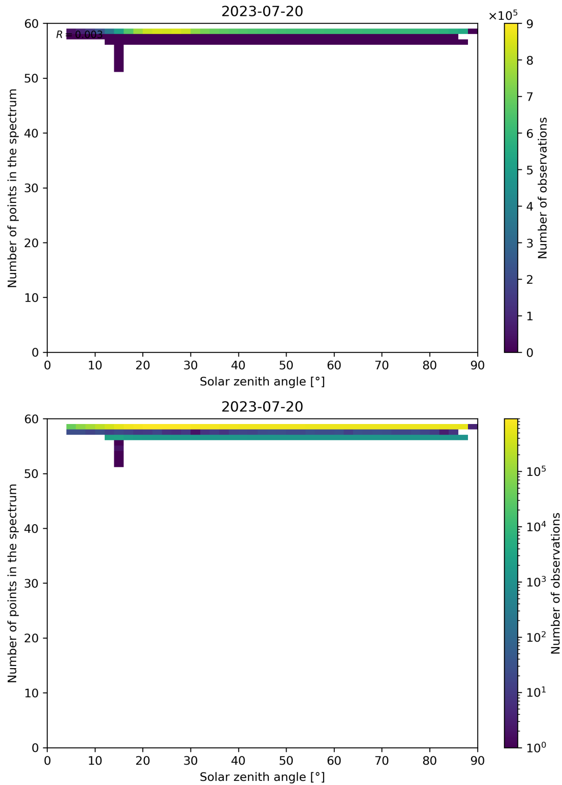
Figure 126: Scatter density plot of “Solar zenith angle” against “Number of points in the spectrum” for 2023-07-19 to 2023-07-21.
