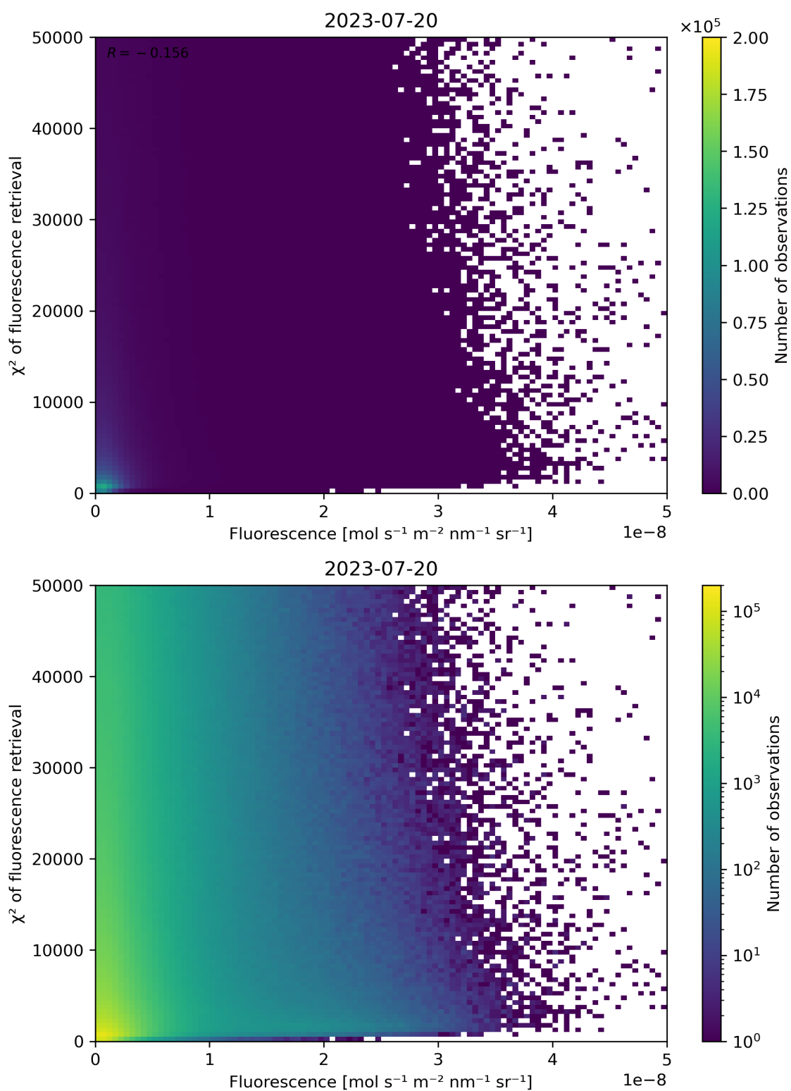
Figure 93: Scatter density plot of “Fluorescence” against “ \chi^2 of fluorescence retrieval” for 2023-07-19 to 2023-07-21.
