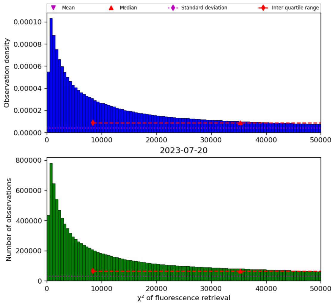
Figure 42: Histogram of “ \chi^2 of fluorescence retrieval” for 2023-07-19 to 2023-07-21
