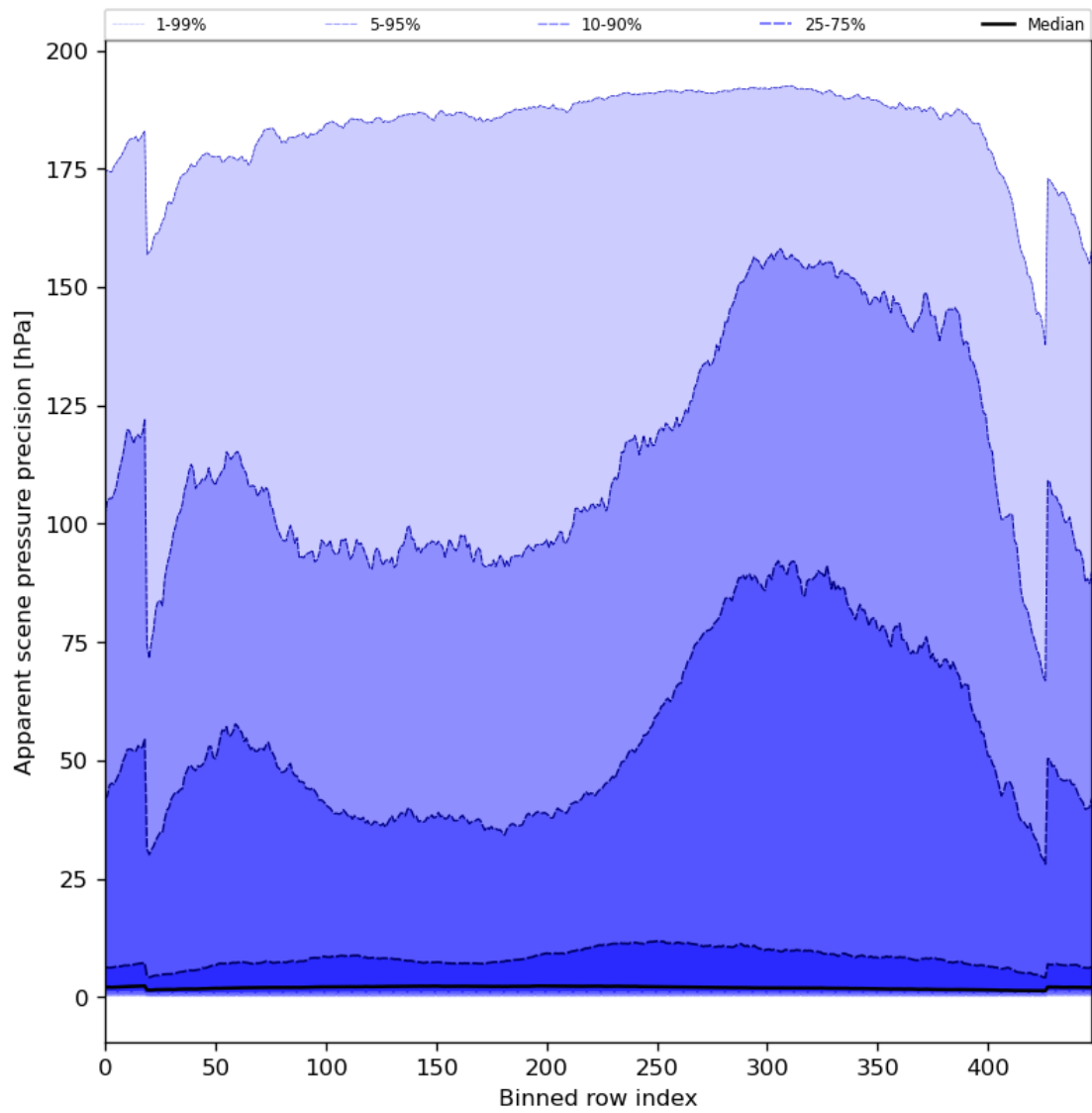
Figure 54: Along track statistics of “Apparent scene pressure precision” for 2023-07-19 to 2023-07-21
