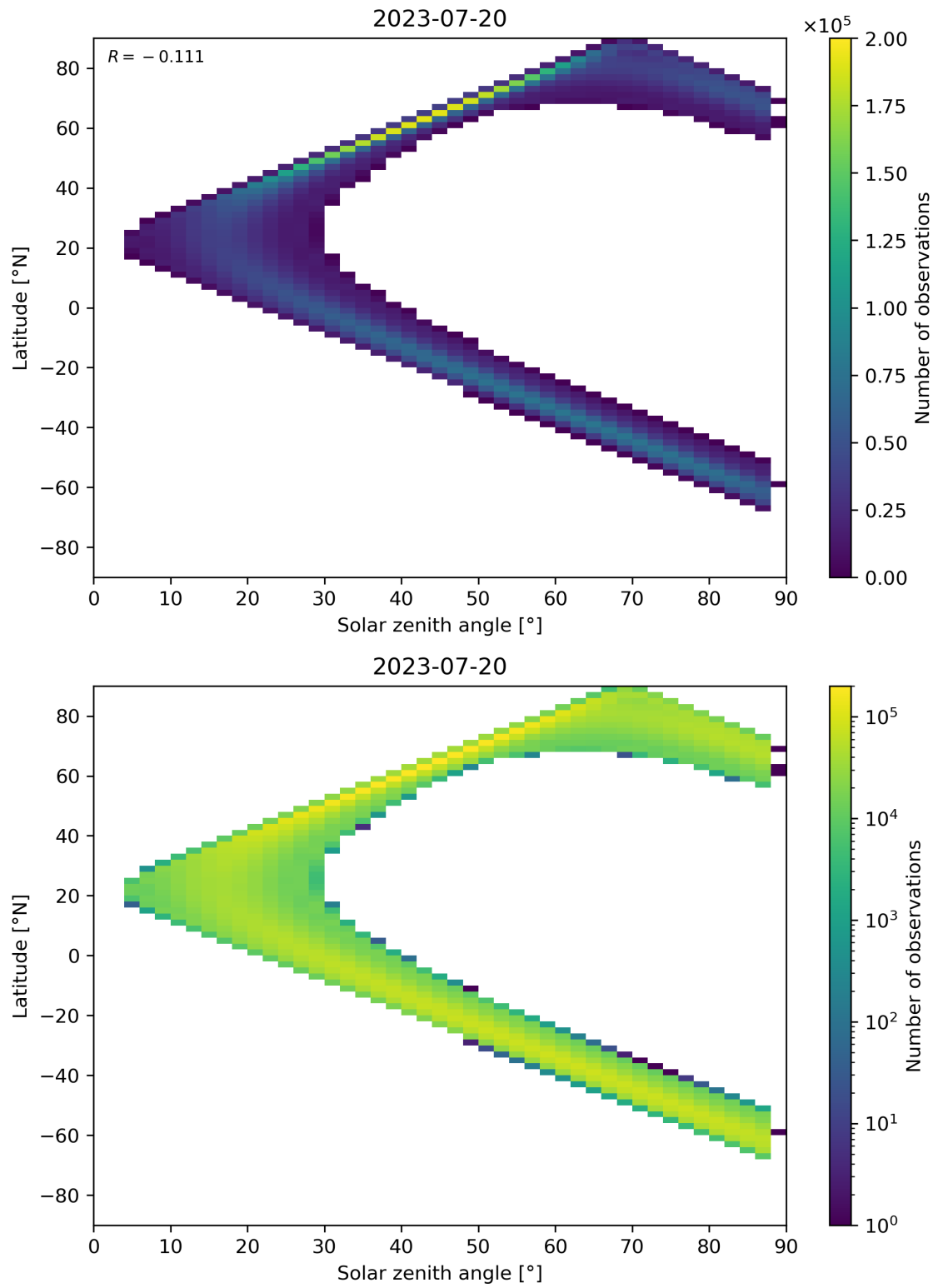
Figure 124: Scatter density plot of “Solar zenith angle” against “Latitude” for 2023-07-19 to 2023-07-21.
