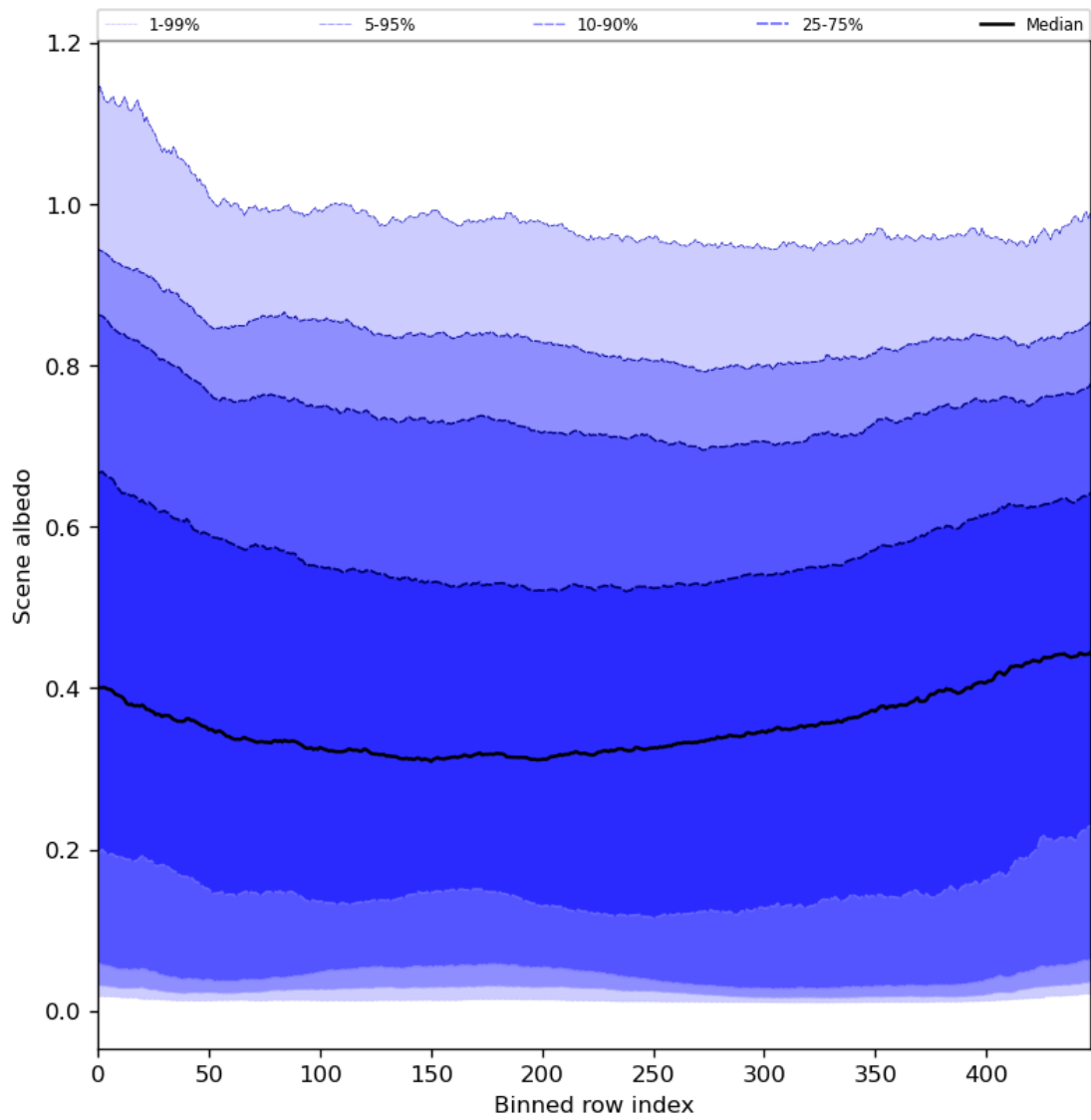
Figure 51: Along track statistics of “Scene albedo” for 2023-07-19 to 2023-07-21
