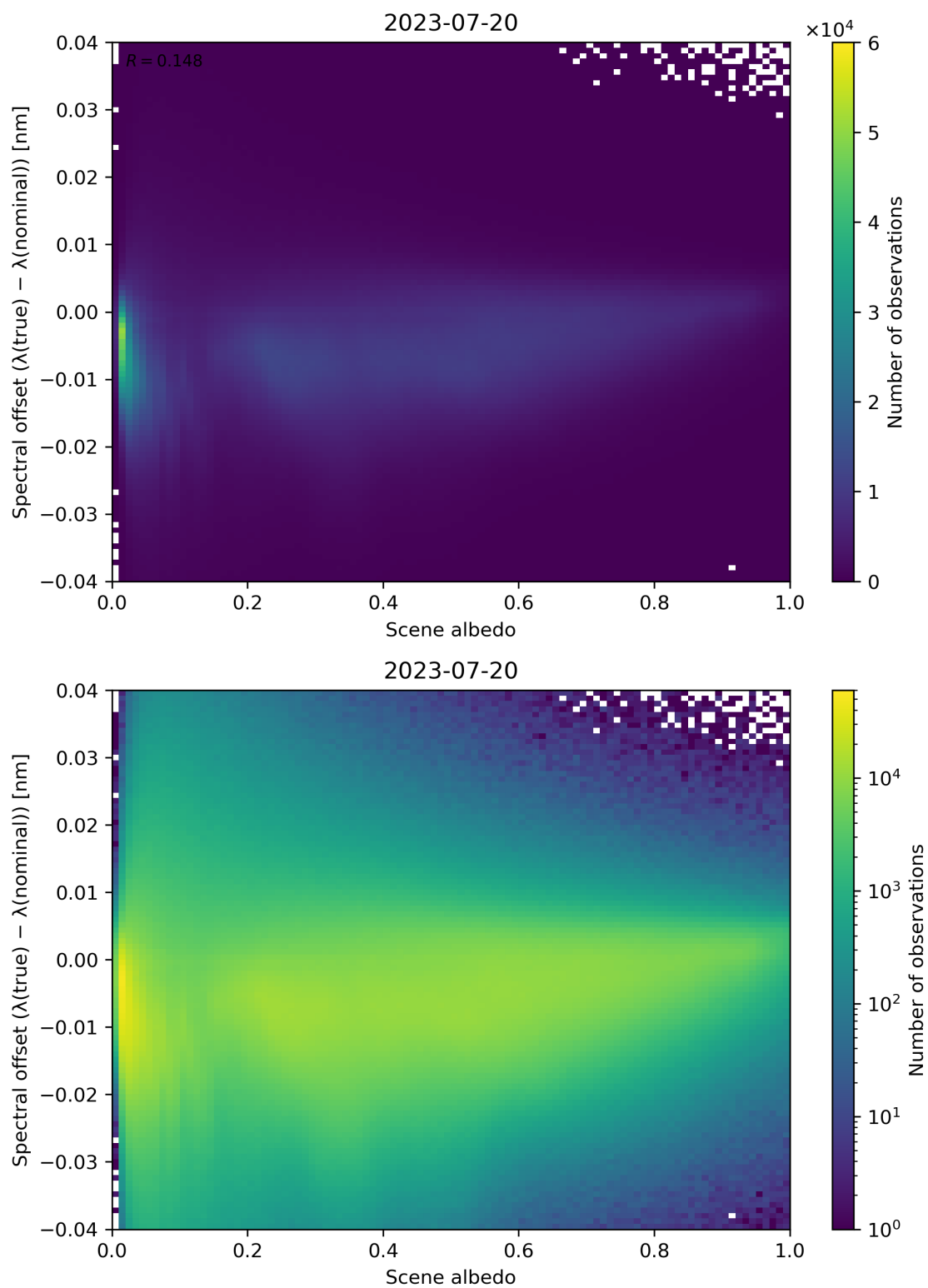
Figure 117: Scatter density plot of “Scene albedo” against “Spectral offset ( \lambda(\text{true}) - \lambda(\text{nominal}) )” for 2023-07-19 to 2023-07-21.
