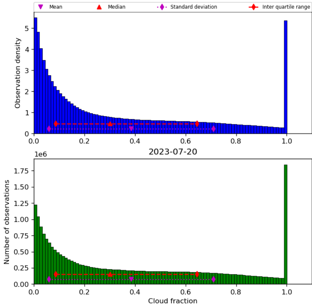
Figure 32: Histogram of “Cloud fraction” for 2023-07-19 to 2023-07-21
