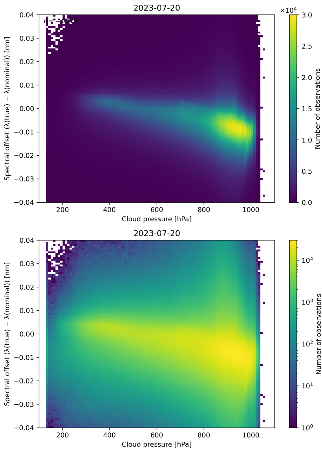
Figure 92: Scatter density plot of “Cloud pressure” against “Spectral offset ( \lambda(\text{true}) - \lambda(\text{nominal}) )” for 2023-07-19 to 2023-07-21.
