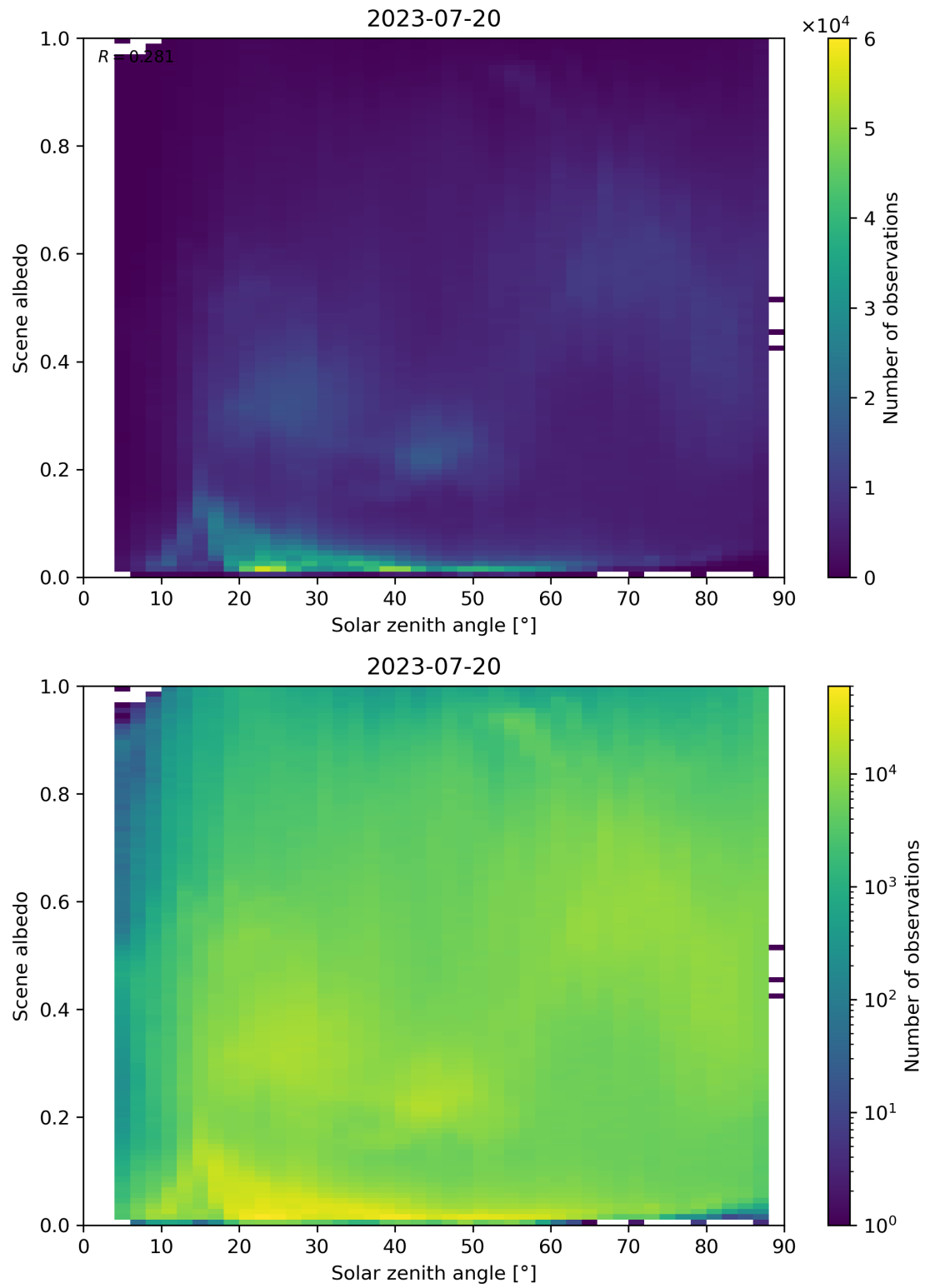
Figure 127: Scatter density plot of “Solar zenith angle” against “Scene albedo” for 2023-07-19 to 2023-07-21.
