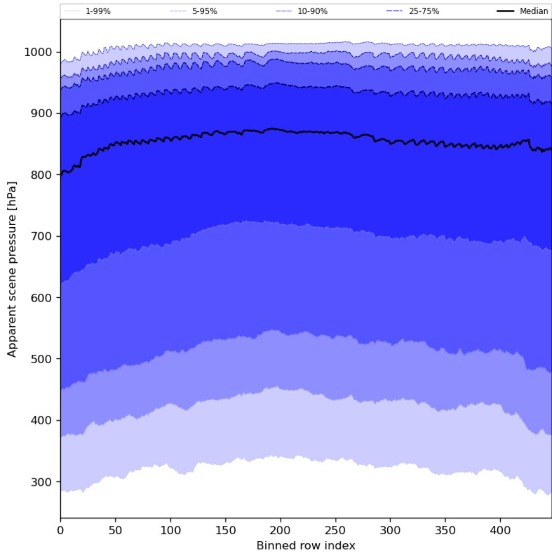
Figure 53: Along track statistics of “Apparent scene pressure” for 2023-07-19 to 2023-07-21
