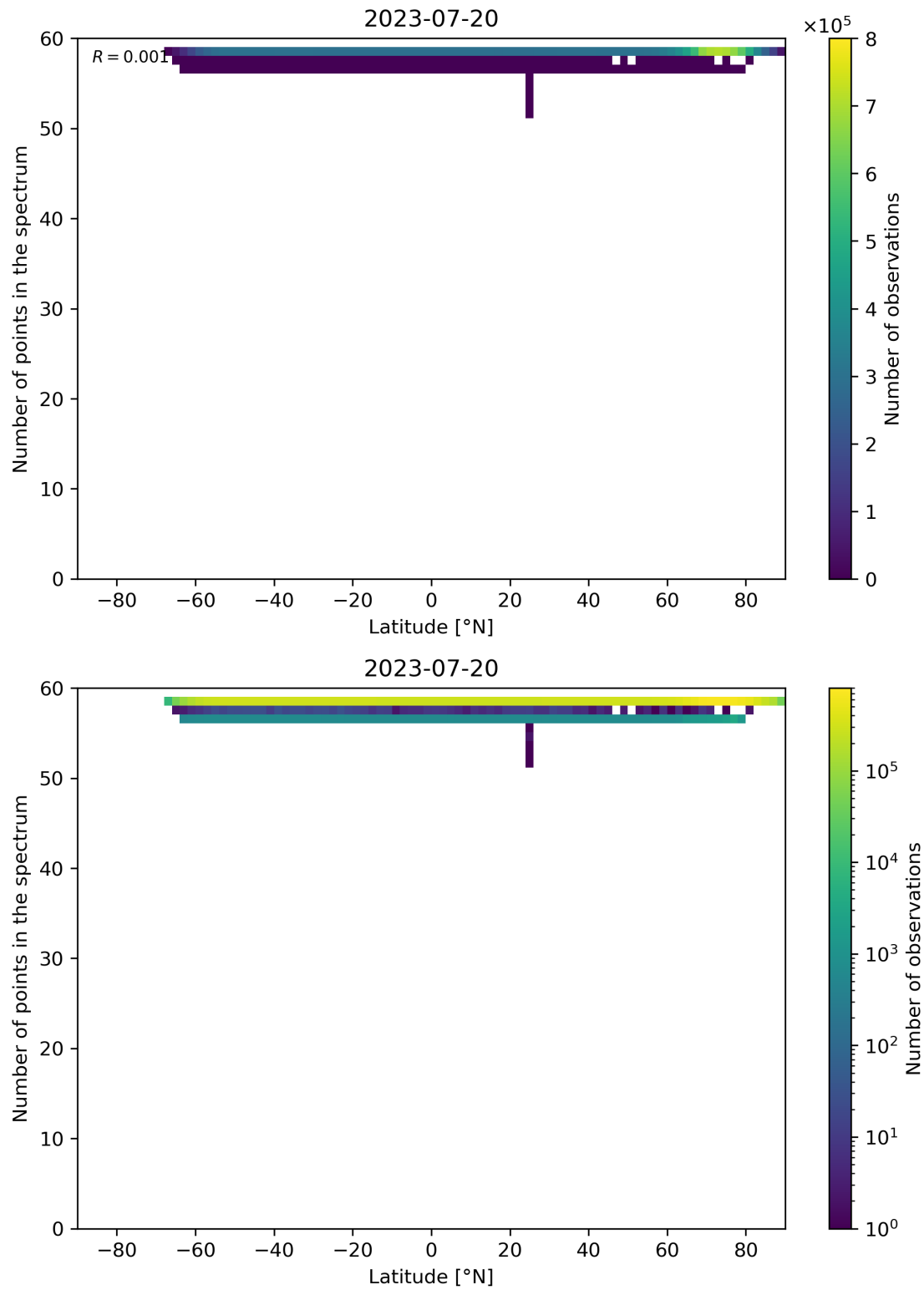
Figure 103: Scatter density plot of “Latitude” against “Number of points in the spectrum” for 2023-07-19 to 2023-07-21.
