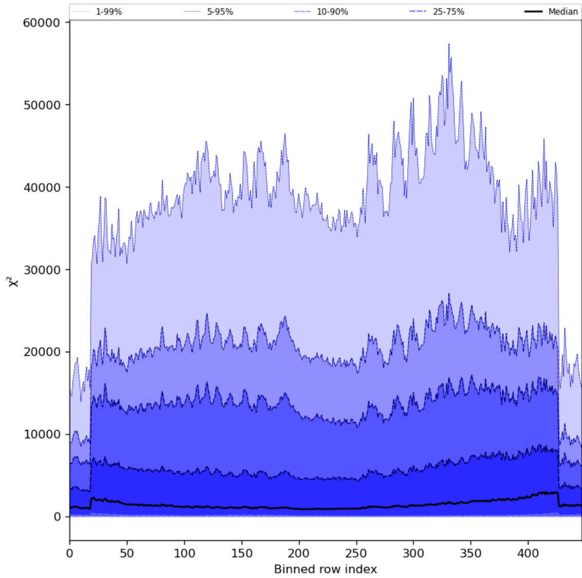
Figure 55: Along track statistics of “ \chi^2 ” for 2023-07-19 to 2023-07-21
