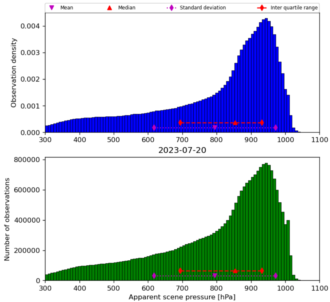
Figure 36: Histogram of “Apparent scene pressure” for 2023-07-19 to 2023-07-21
