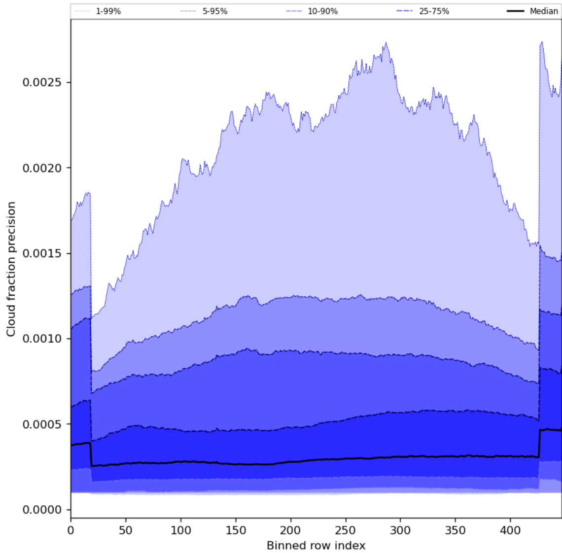
Figure 50: Along track statistics of “Cloud fraction precision” for 2023-07-19 to 2023-07-21
