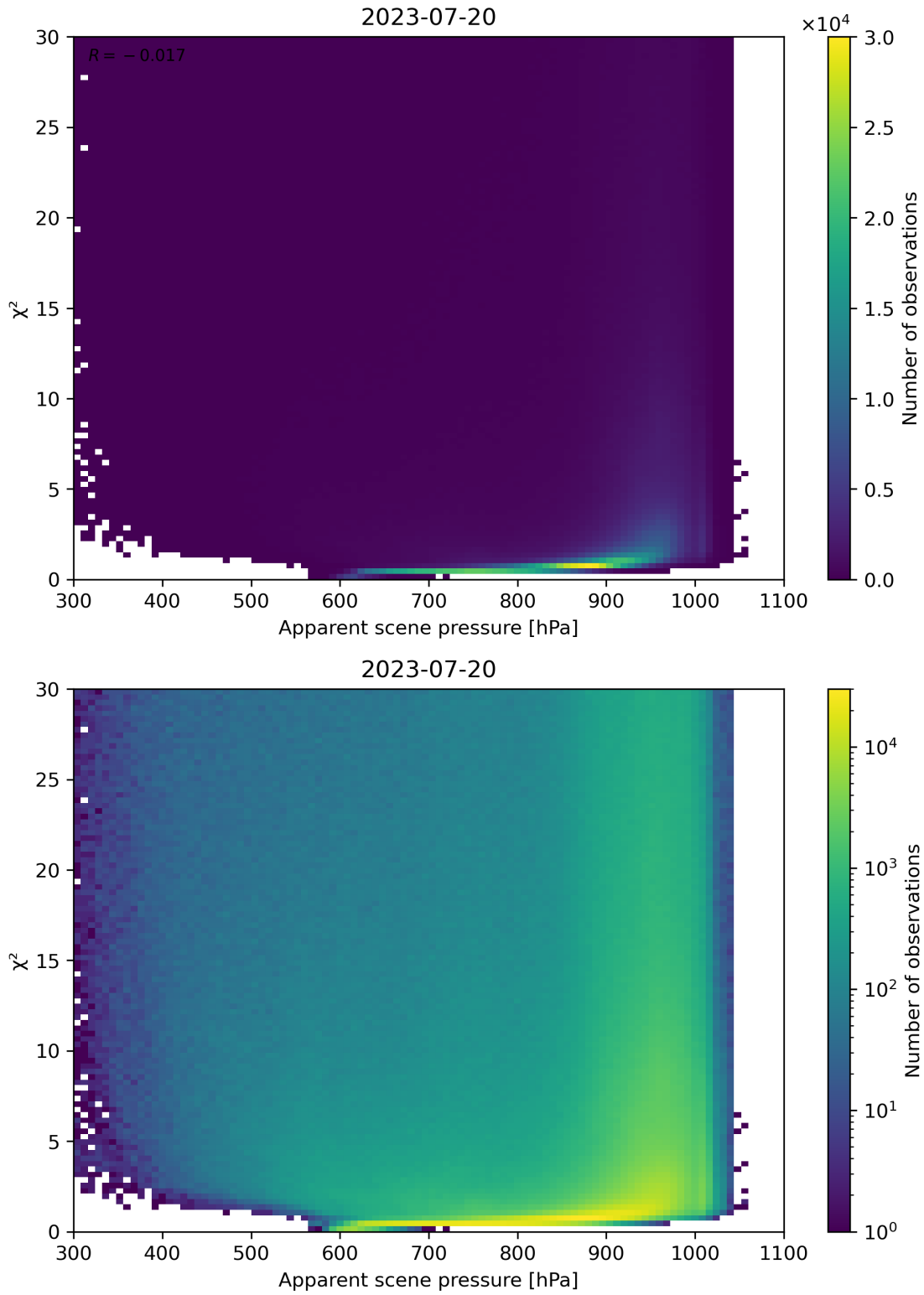
Figure 63: Scatter density plot of “Apparent scene pressure” against “ \chi^2 ” for 2023-07-19 to 2023-07-21.
