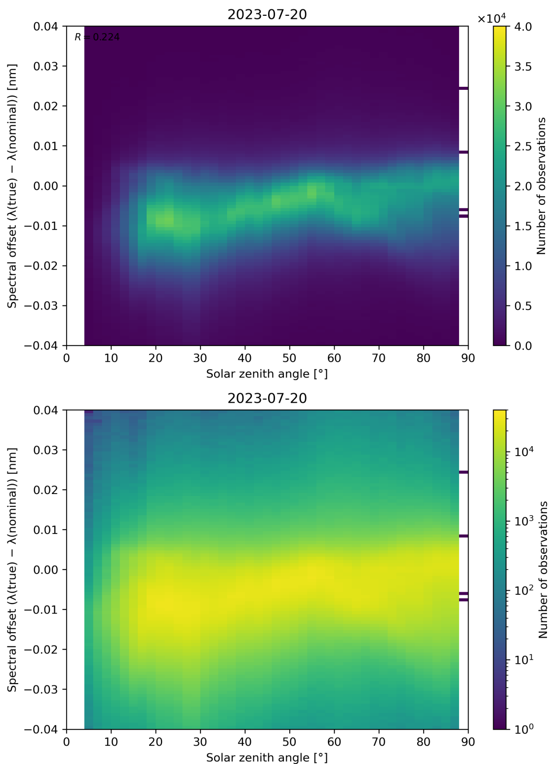
Figure 128: Scatter density plot of “Solar zenith angle” against “Spectral offset ( \lambda(\text{true}) - \lambda(\text{nominal}) )” for 2023-07-19 to 2023-07-21.
