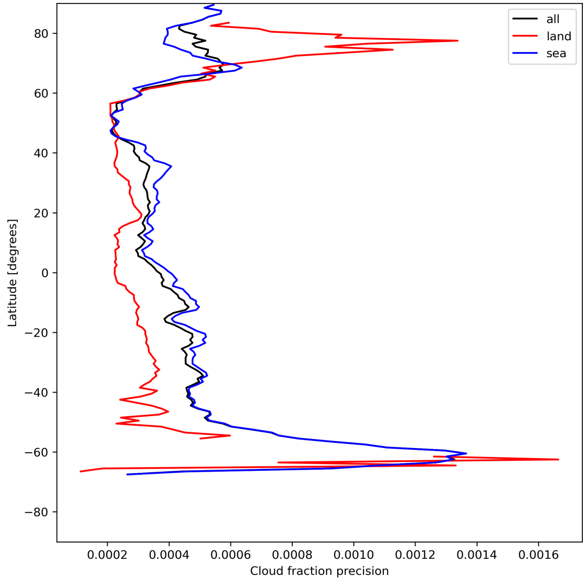
Figure 16: Zonal average of “Cloud fraction precision” for 2023-07-19 to 2023-07-21.
