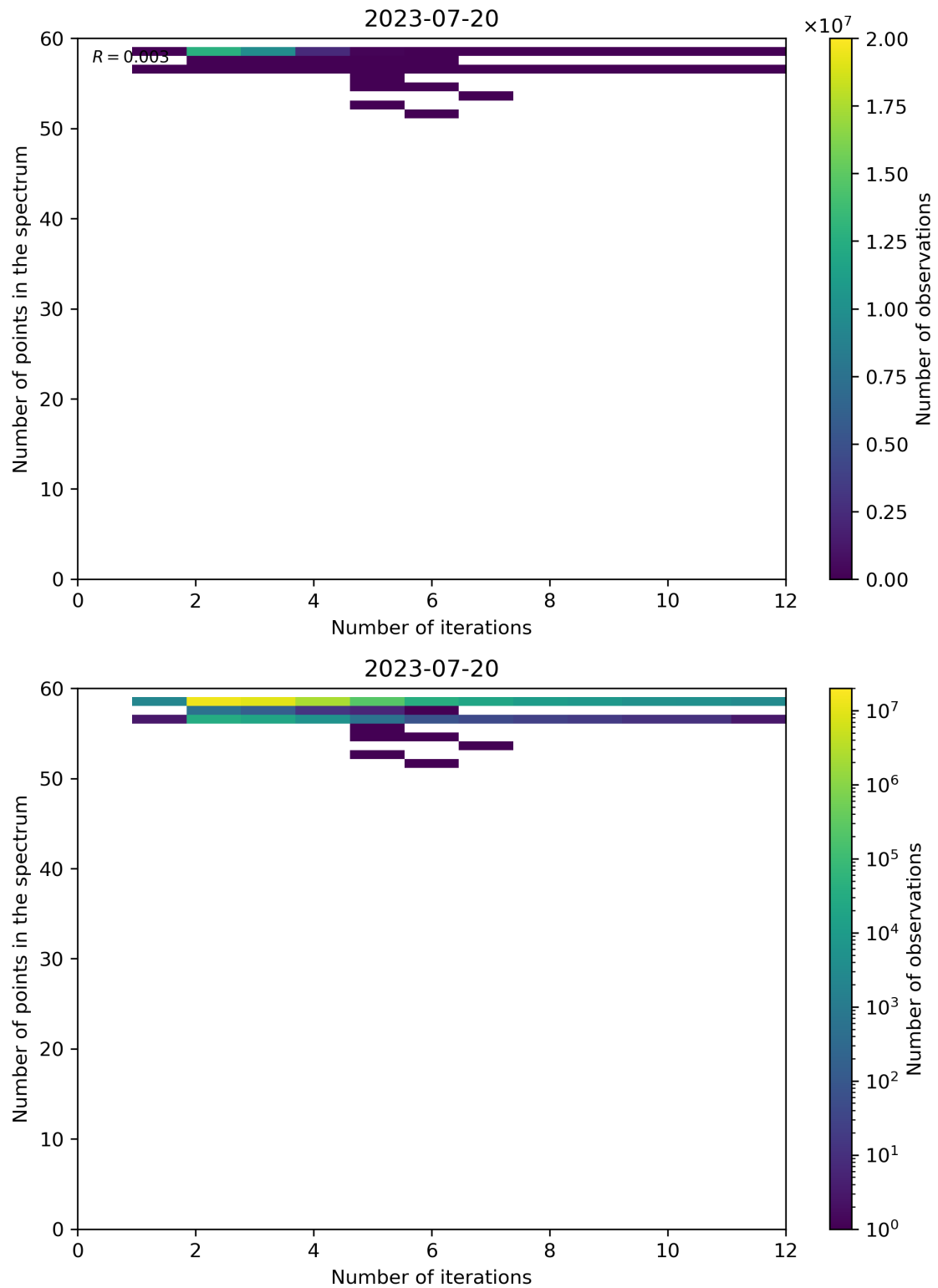
Figure 108: Scatter density plot of “Number of iterations” against “Number of points in the spectrum” for 2023-07-19 to 2023-07-21.
