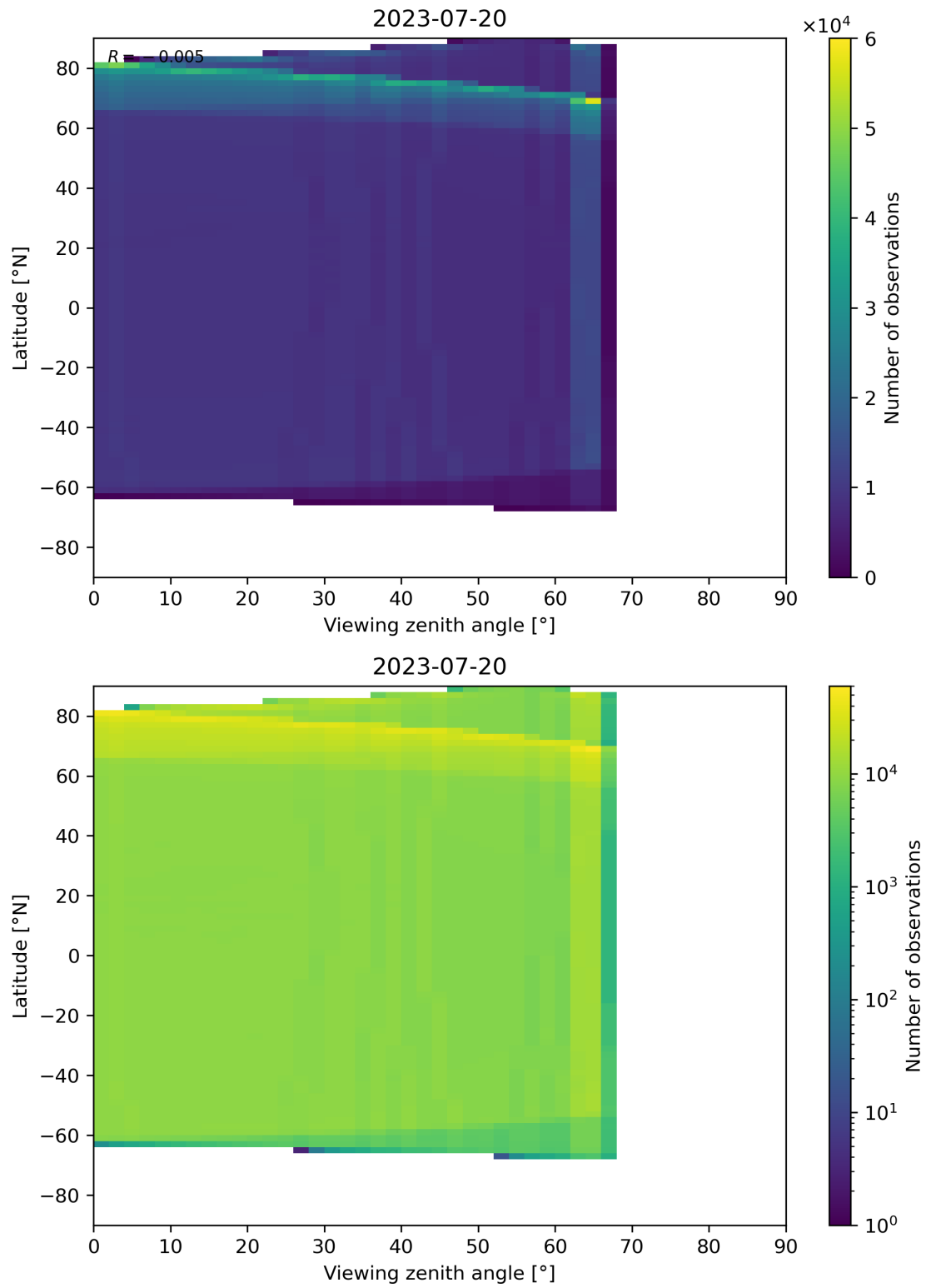
Figure 135: Scatter density plot of “Viewing zenith angle” against “Latitude” for 2023-07-19 to 2023-07-21.
