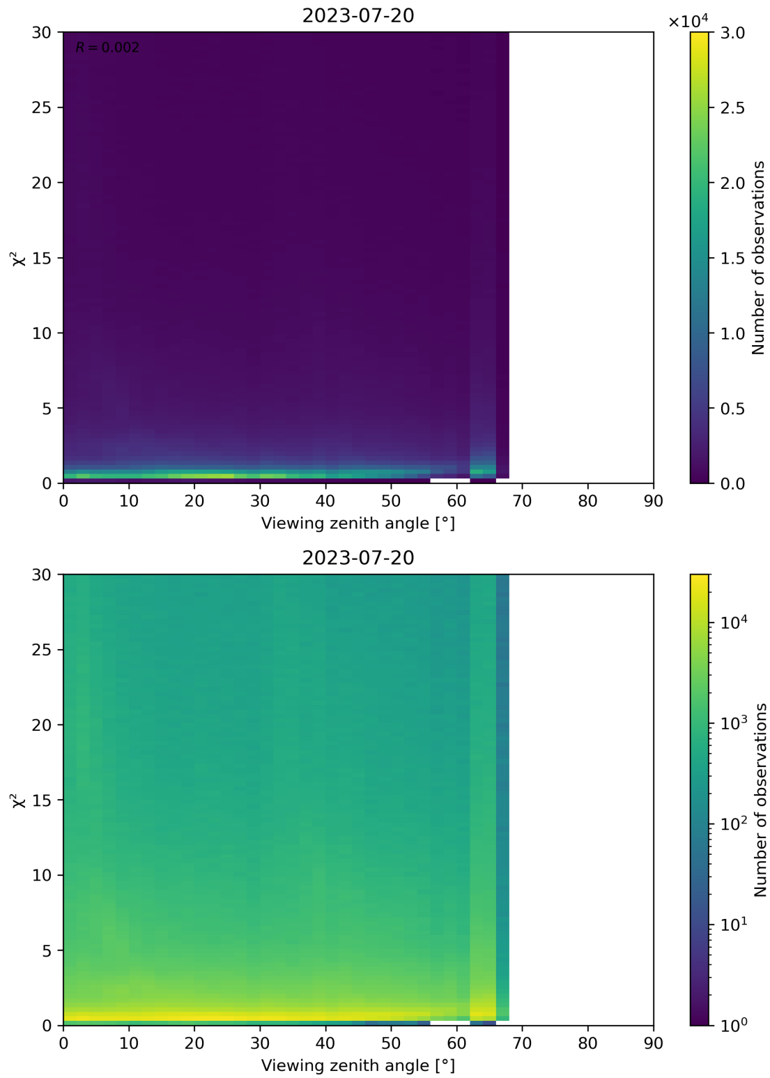
Figure 130: Scatter density plot of “Viewing zenith angle” against “ \chi^2 ” for 2023-07-19 to 2023-07-21.
