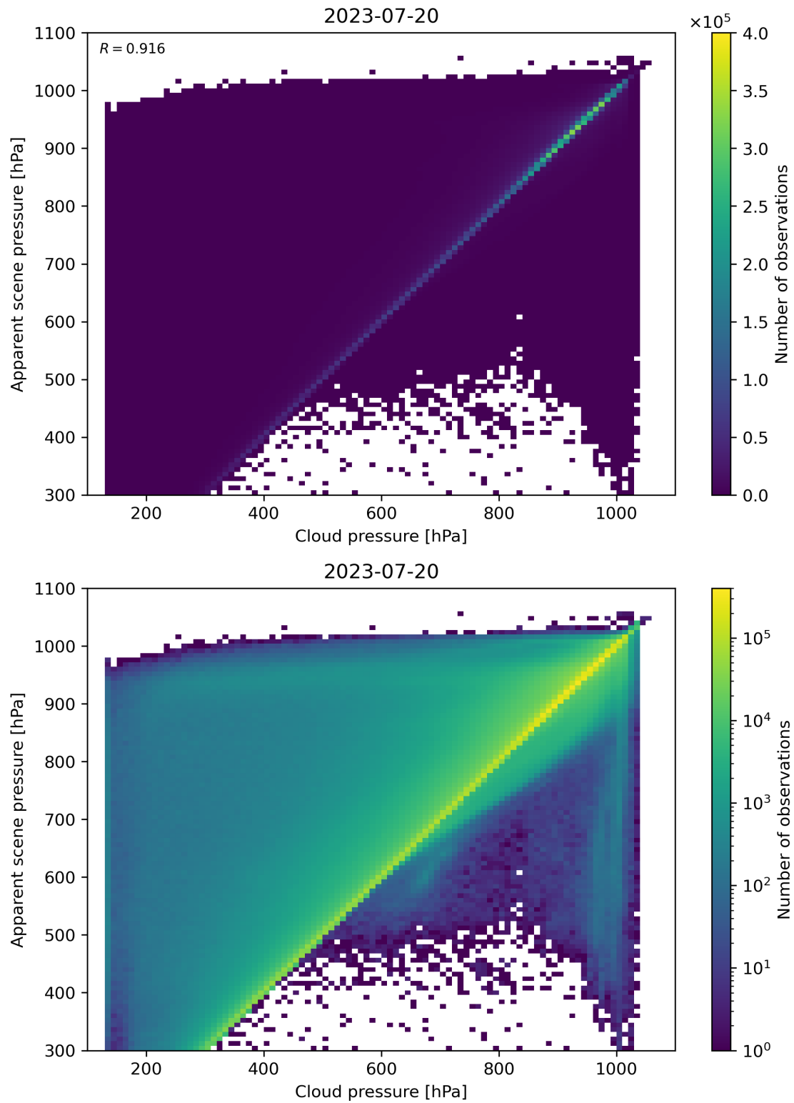
Figure 84: Scatter density plot of “Cloud pressure” against “Apparent scene pressure” for 2023-07-19 to 2023-07-21.
