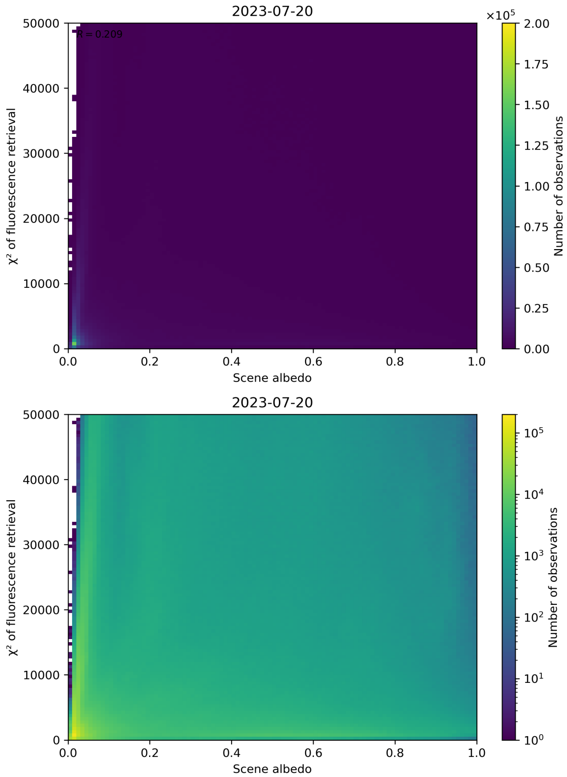
Figure 113: Scatter density plot of “Scene albedo” against “ \chi^2 of fluorescence retrieval” for 2023-07-19 to 2023-07-21.
