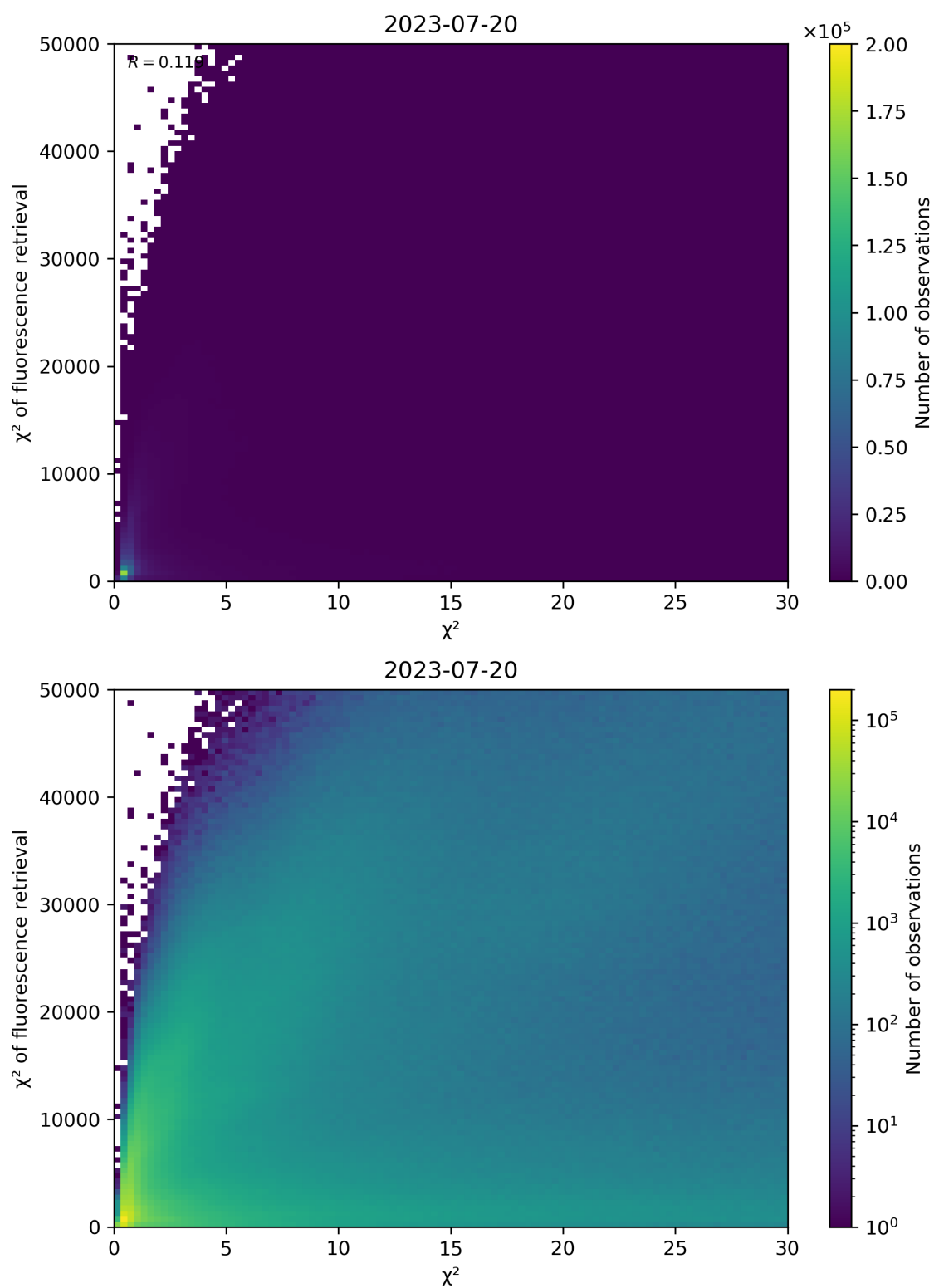
Figure 69: Scatter density plot of “ \chi^2 ” against “ \chi^2 of fluorescence retrieval” for 2023-07-19 to 2023-07-21.
