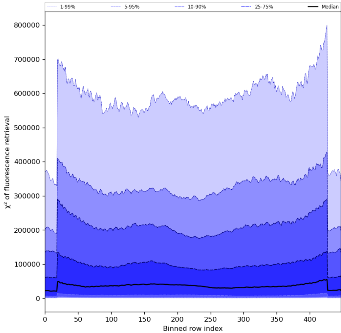
Figure 59: Along track statistics of “ \chi^2 of fluorescence retrieval” for 2023-07-19 to 2023-07-21
