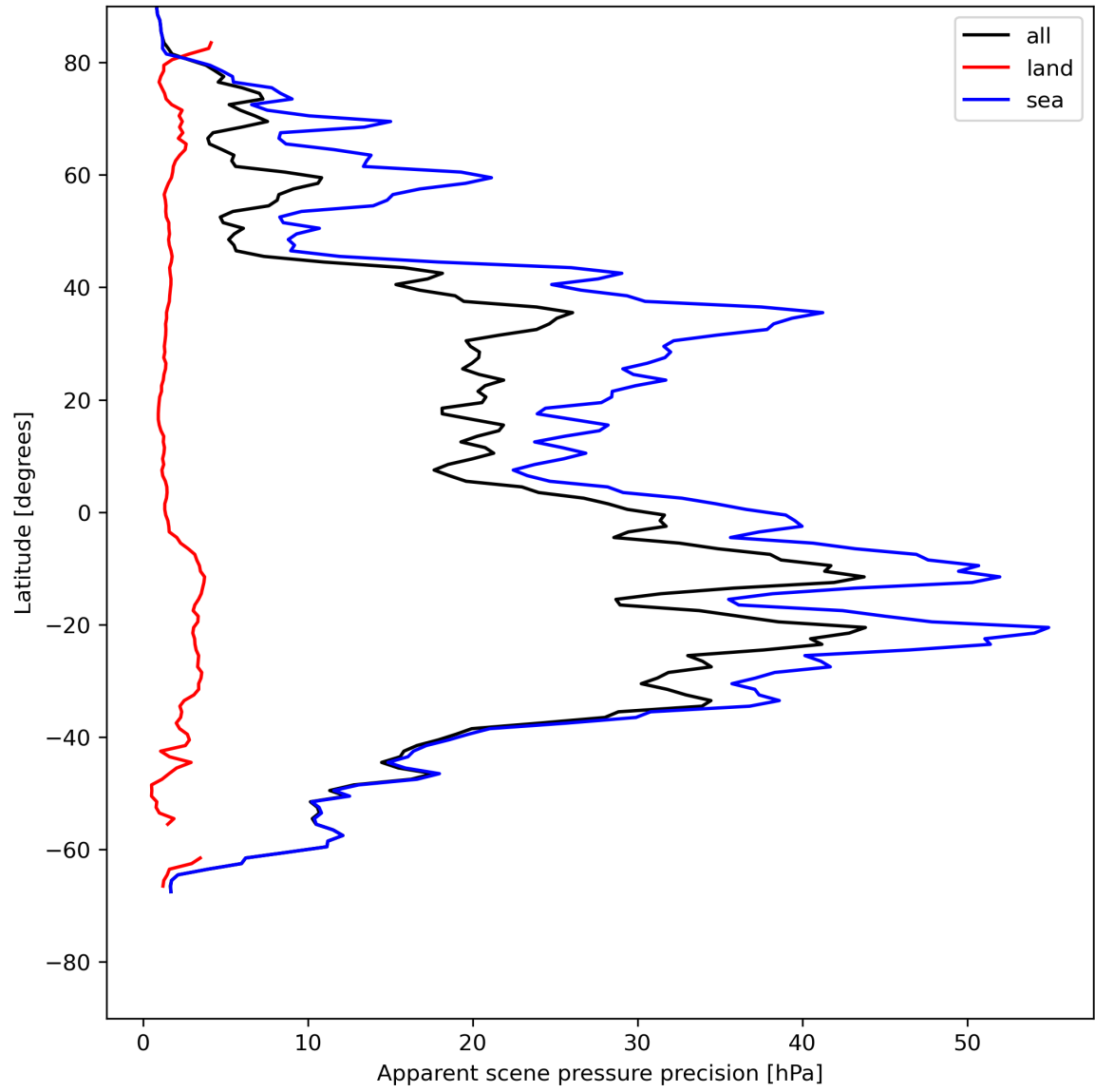
Figure 20: Zonal average of “Apparent scene pressure precision” for 2023-07-19 to 2023-07-21.
