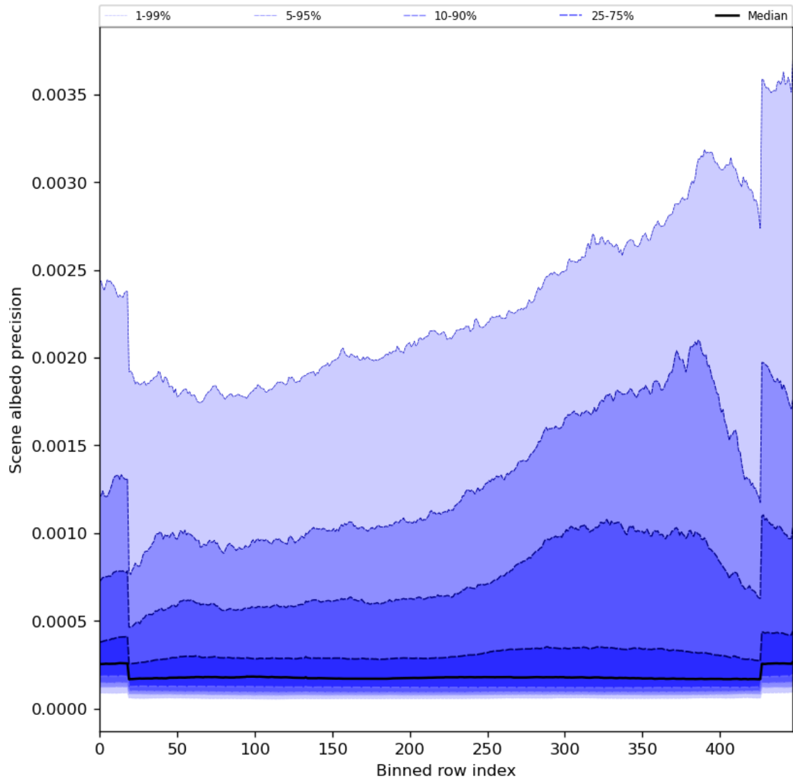
Figure 52: Along track statistics of “Scene albedo precision” for 2023-07-19 to 2023-07-21
