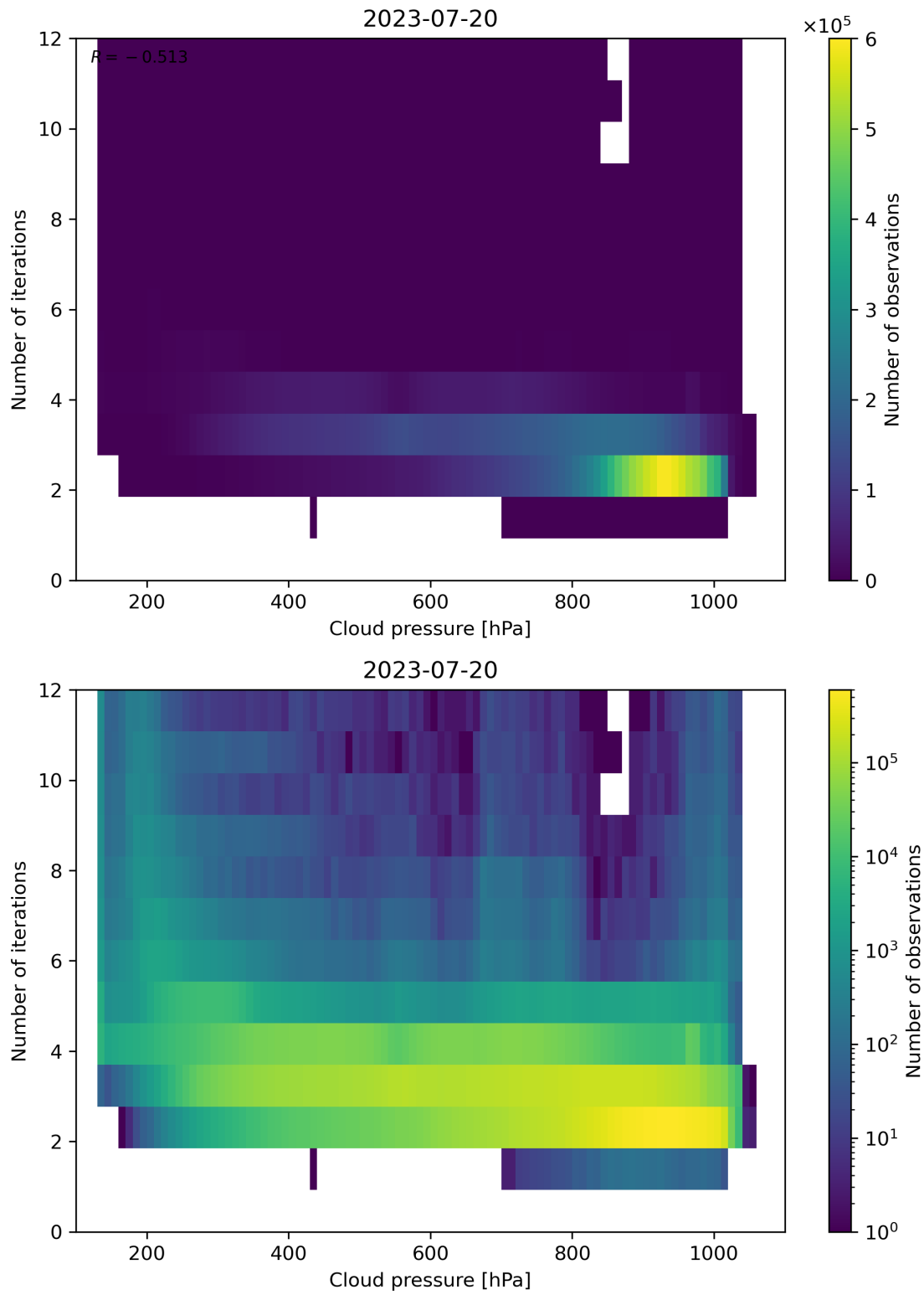
Figure 89: Scatter density plot of “Cloud pressure” against “Number of iterations” for 2023-07-19 to 2023-07-21.
