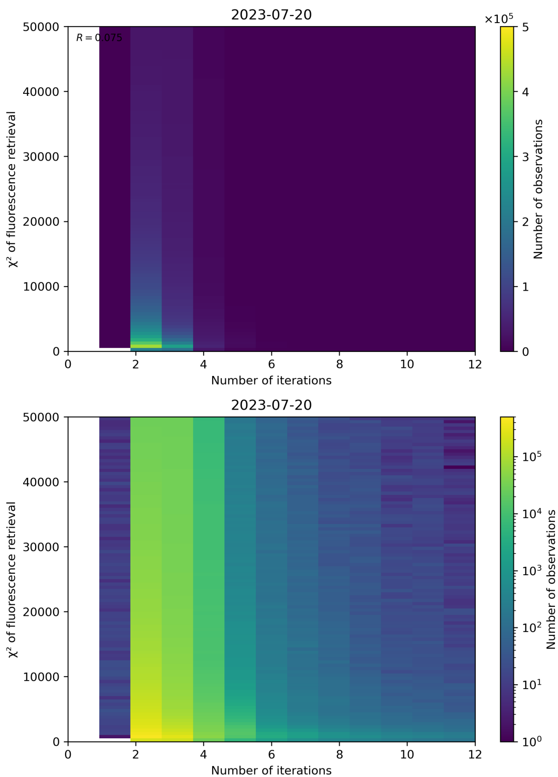
Figure 106: Scatter density plot of “Number of iterations” against “ \chi^2 of fluorescence retrieval” for 2023-07-19 to 2023-07-21.
