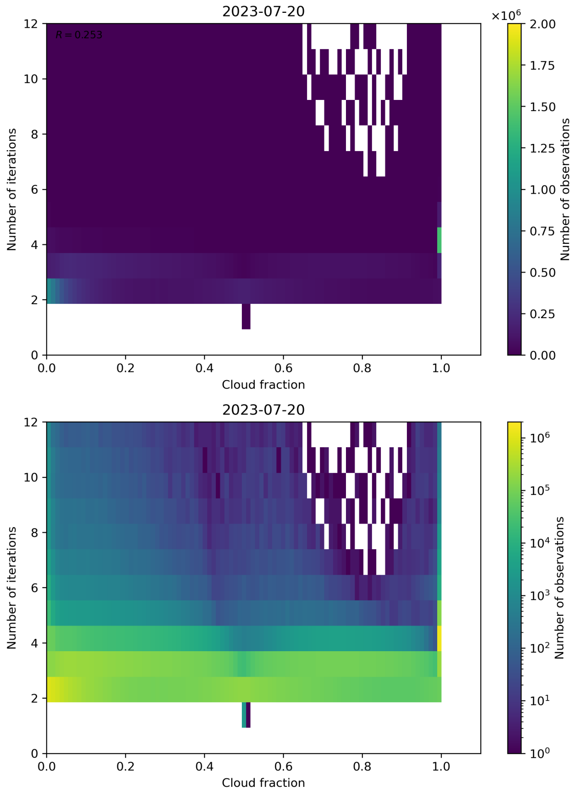
Figure 80: Scatter density plot of “Cloud fraction” against “Number of iterations” for 2023-07-19 to 2023-07-21.
