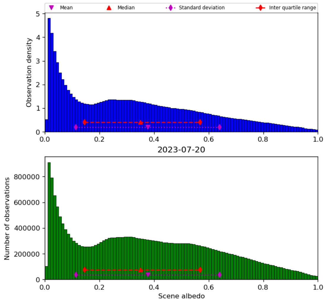
Figure 34: Histogram of “Scene albedo” for 2023-07-19 to 2023-07-21
