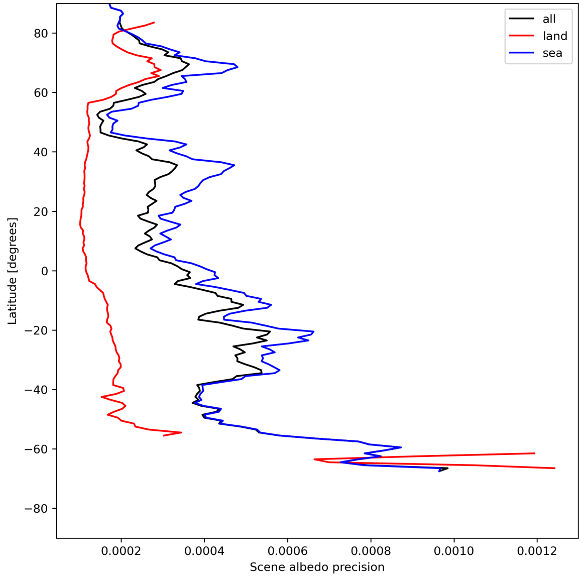
Figure 18: Zonal average of "Scene albedo precision" for 2023-07-19 to 2023-07-21.
