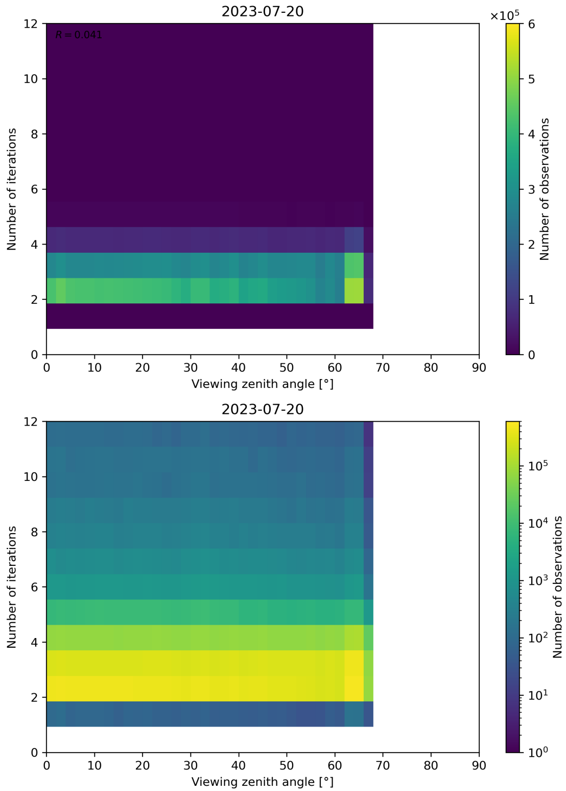
Figure 136: Scatter density plot of “Viewing zenith angle” against “Number of iterations” for 2023-07-19 to 2023-07-21.
