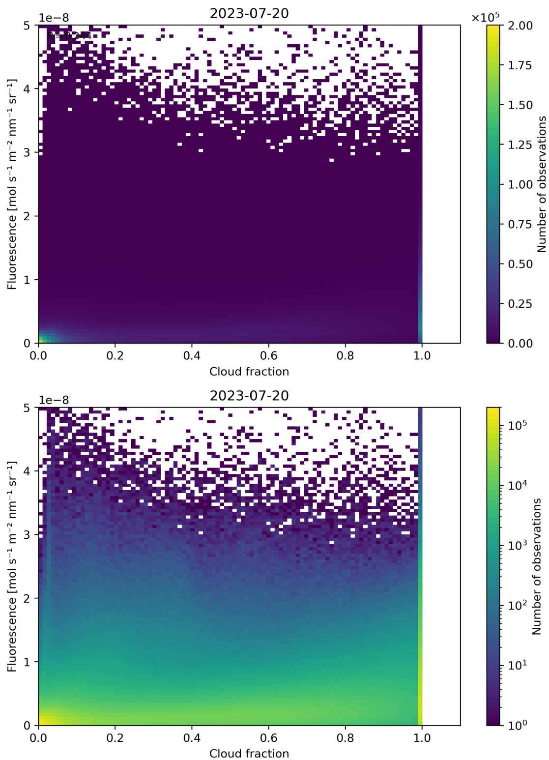
Figure 79: Scatter density plot of “Cloud fraction” against “Fluorescence” for 2023-07-19 to 2023-07-21.
