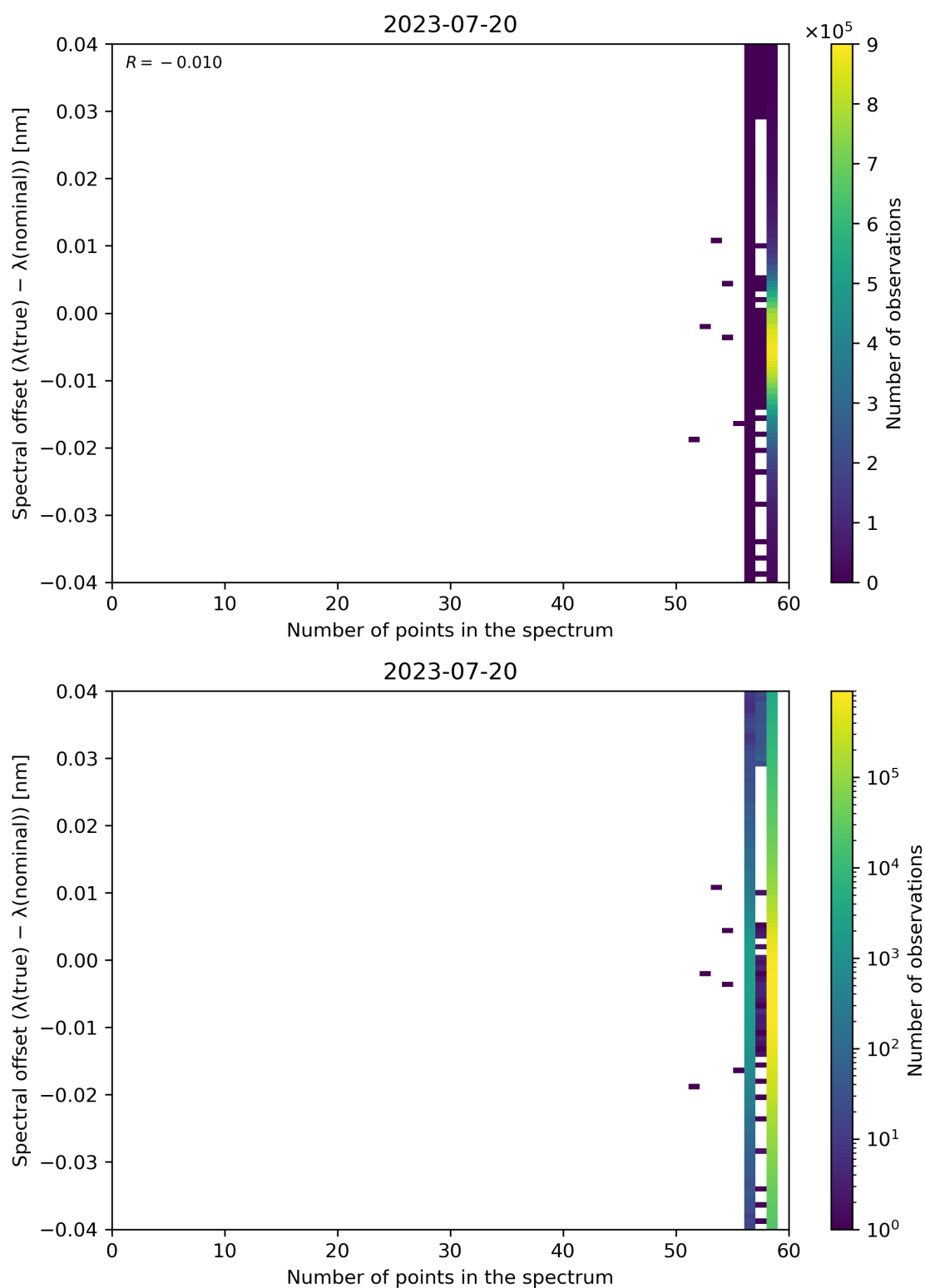
Figure 110: Scatter density plot of “Number of points in the spectrum” against “Spectral offset ( \lambda(\text{true}) - \lambda(\text{nominal}) )” for 2023-07-19 to 2023-07-21.
