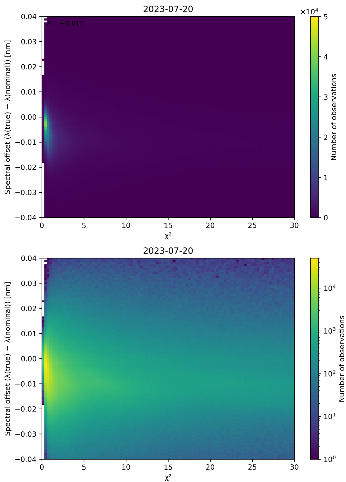
Figure 75: Scatter density plot of “ \chi^2 ” against “Spectral offset ( \lambda(\text{true}) - \lambda(\text{nominal}) )” for 2023-07-19 to 2023-07-21.
