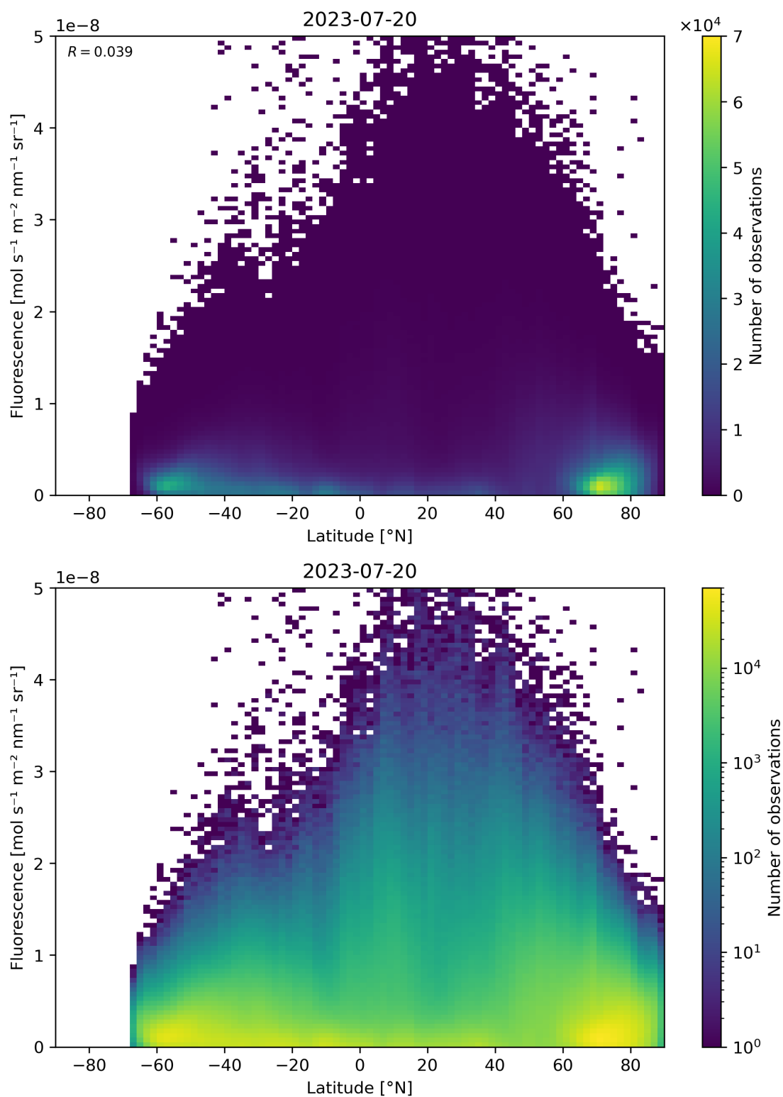
Figure 101: Scatter density plot of “Latitude” against “Fluorescence” for 2023-07-19 to 2023-07-21.
