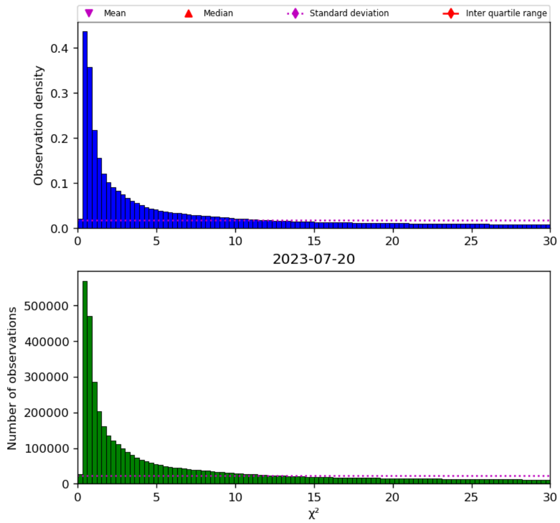
Figure 38: Histogram of " \chi^2 " for 2023-07-19 to 2023-07-21
