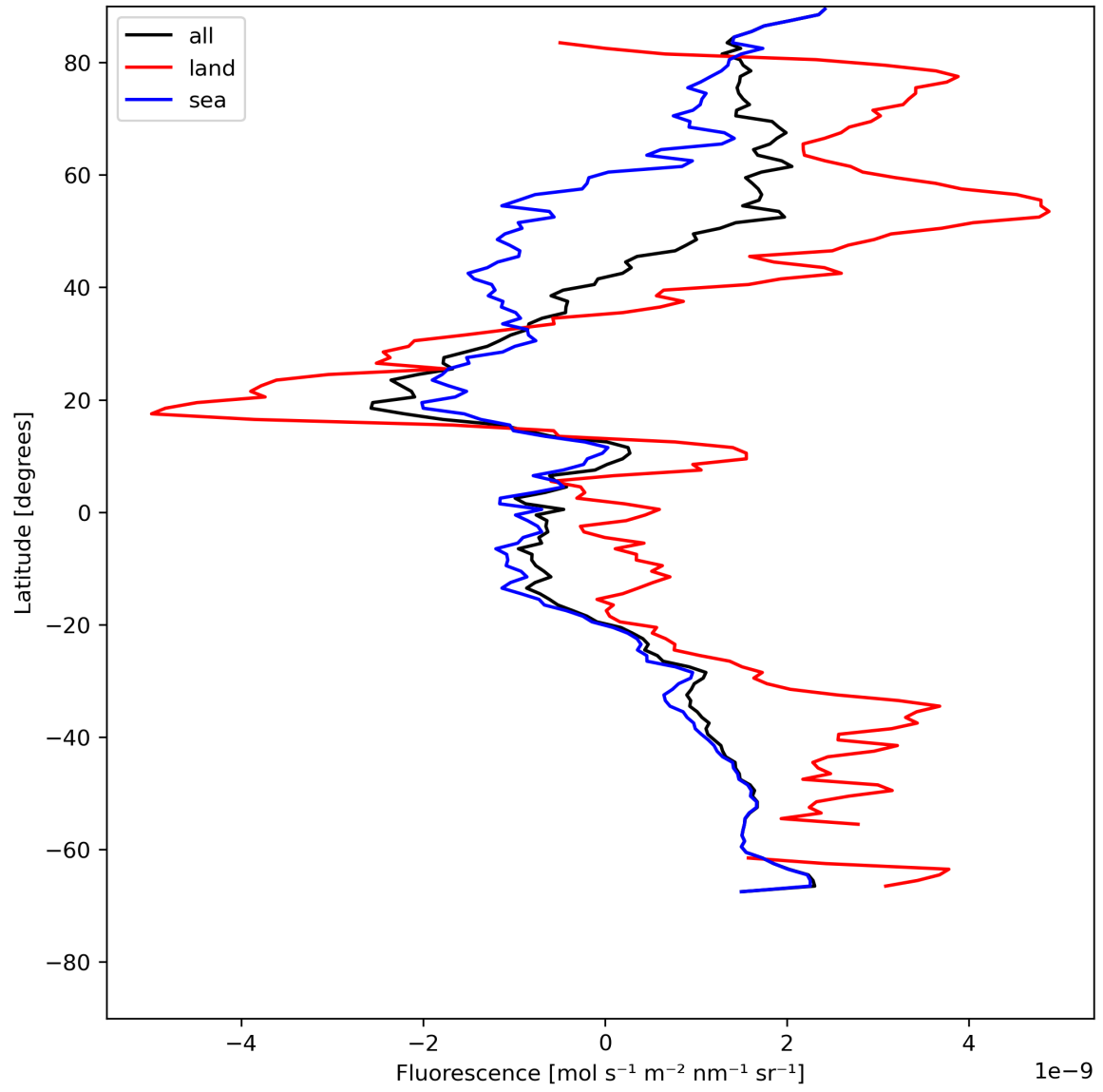
Figure 23: Zonal average of “Fluorescence” for 2023-07-19 to 2023-07-21.
