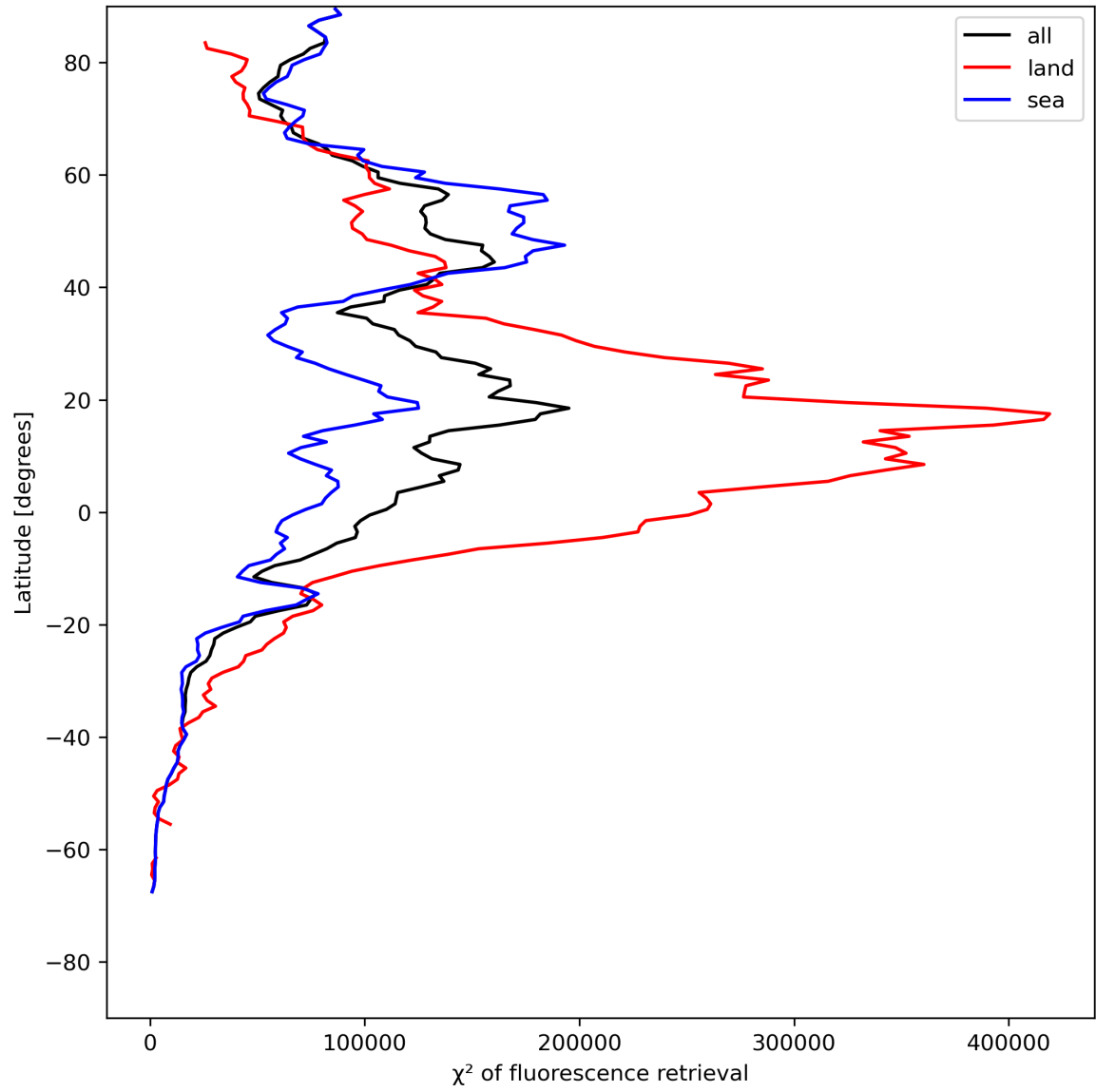
Figure 25: Zonal average of “ \chi^2 of fluorescence retrieval” for 2023-07-19 to 2023-07-21.
