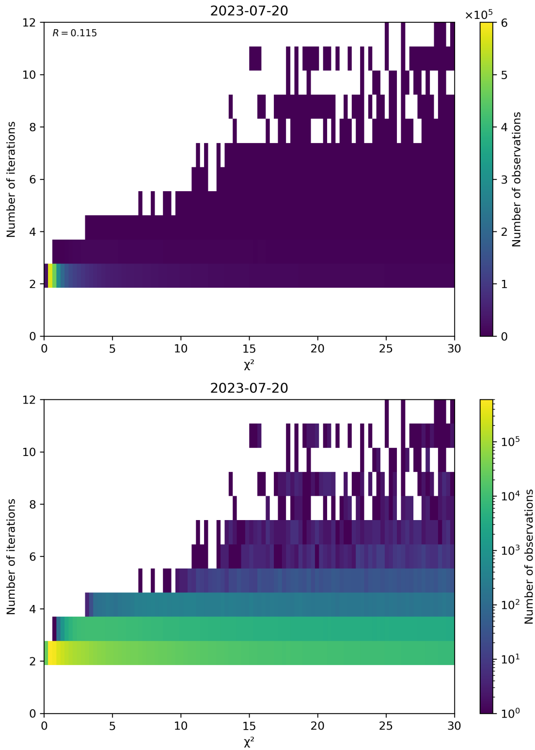
Figure 73: Scatter density plot of “ \chi^2 ” against “Number of iterations” for 2023-07-19 to 2023-07-21.
