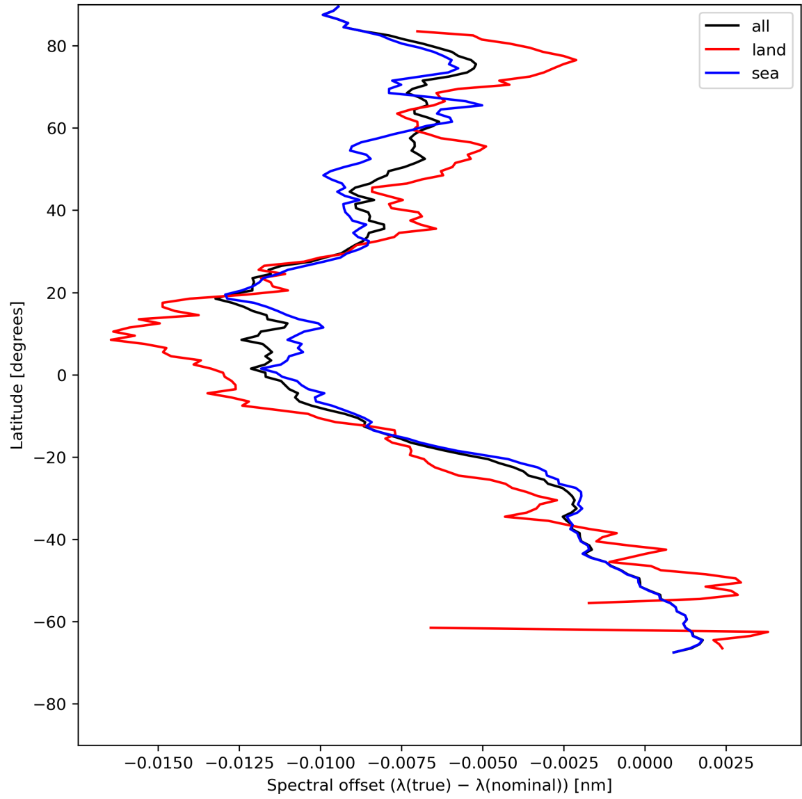
Figure 28: Zonal average of “Spectral offset ( \lambda(\text{true}) - \lambda(\text{nominal}) )” for 2023-07-19 to 2023-07-21.
