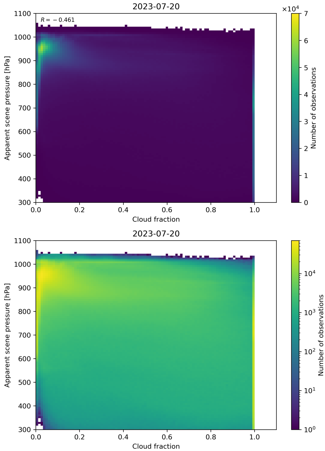
Figure 76: Scatter density plot of “Cloud fraction” against “Apparent scene pressure” for 2023-07-19 to 2023-07-21.
