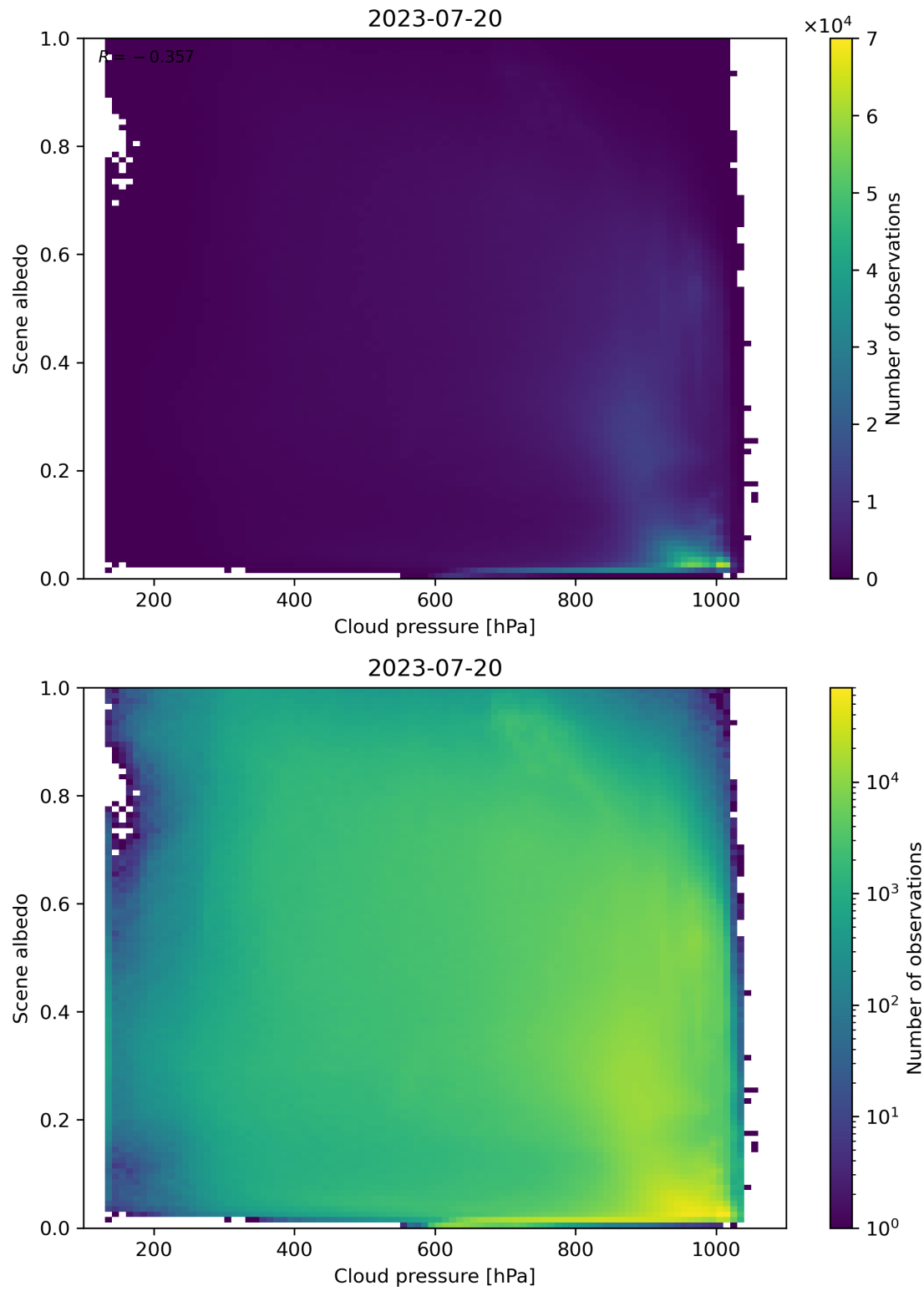
Figure 91: Scatter density plot of “Cloud pressure” against “Scene albedo” for 2023-07-19 to 2023-07-21.
