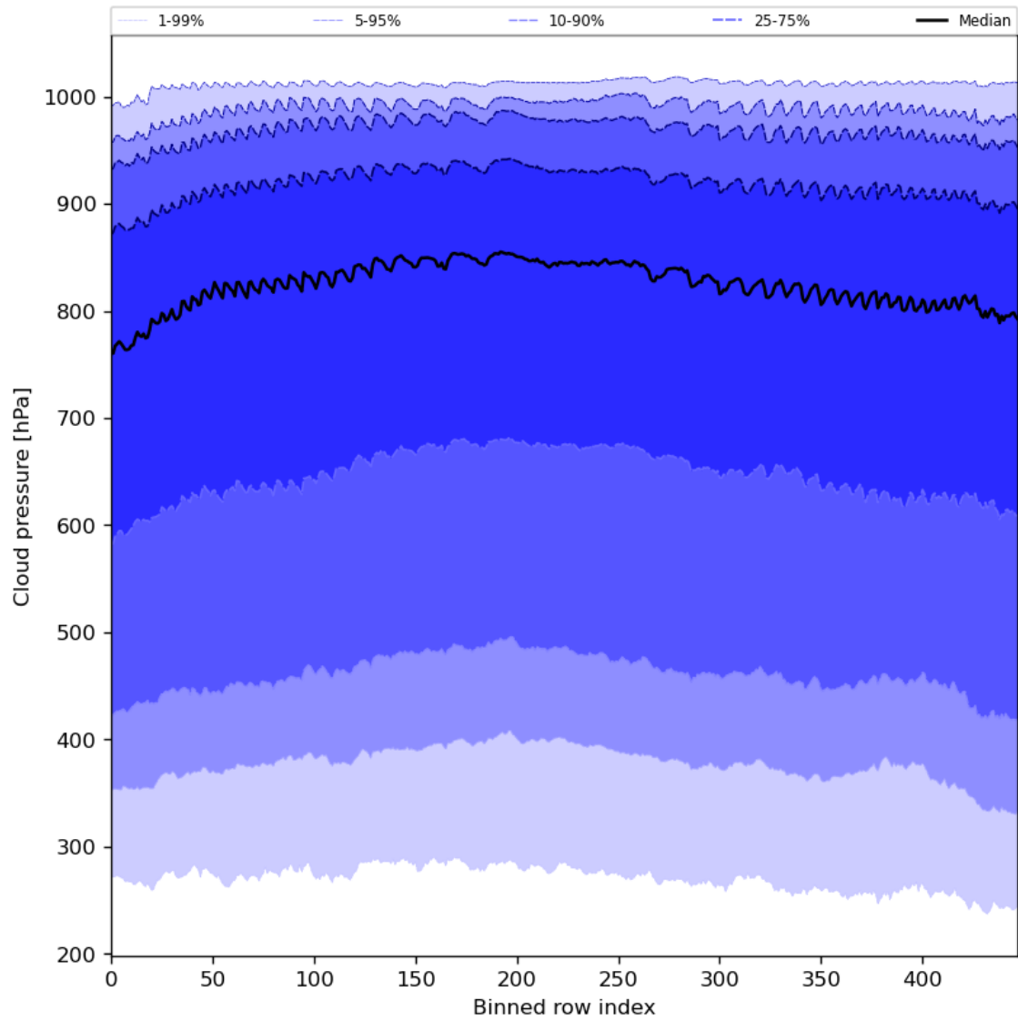
Figure 47: Along track statistics of “Cloud pressure” for 2023-07-19 to 2023-07-21
