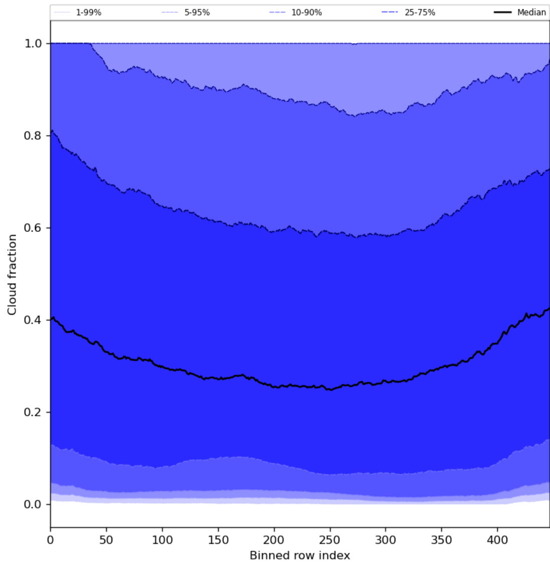
Figure 49: Along track statistics of “Cloud fraction” for 2023-07-19 to 2023-07-21
