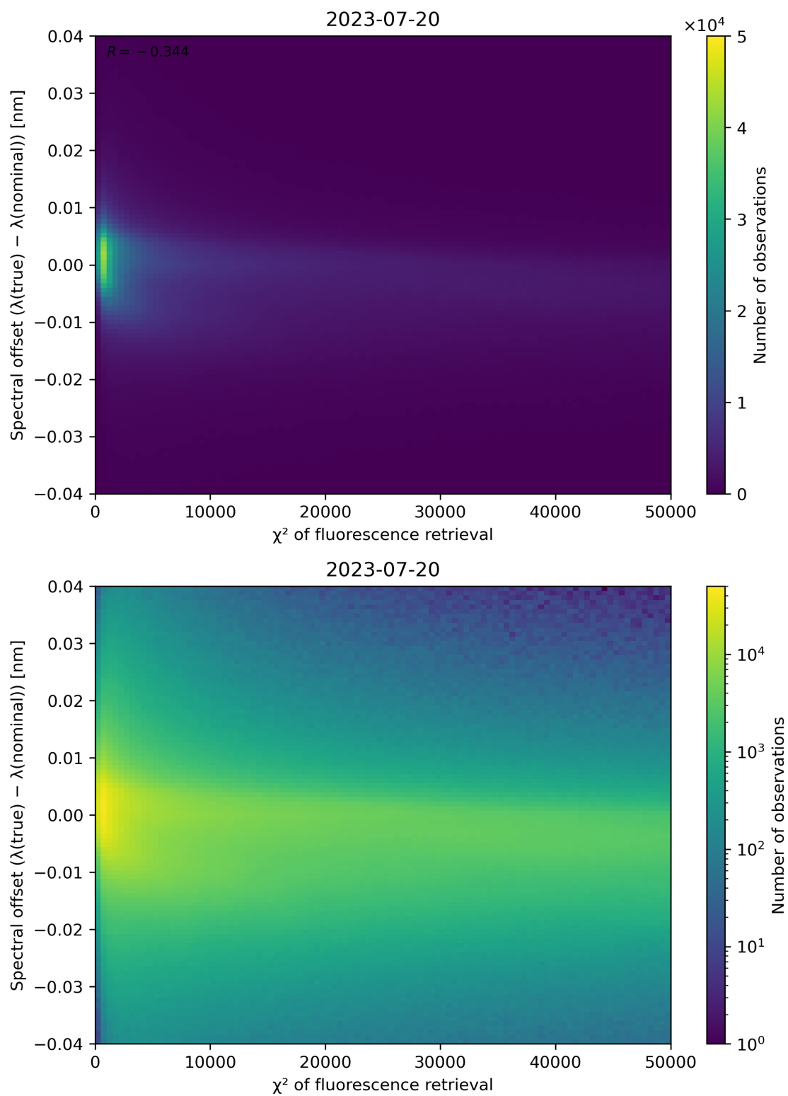
Figure 72: Scatter density plot of “ \chi^2 of fluorescence retrieval” against “Spectral offset ( \lambda(\text{true}) - \lambda(\text{nominal}) )” for 2023-07-19 to 2023-07-21.
