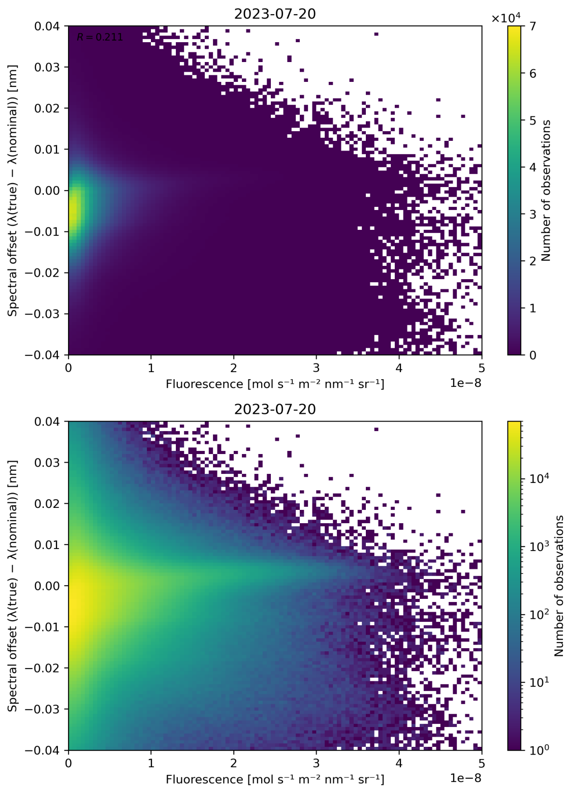
Figure 95: Scatter density plot of “Fluorescence” against “Spectral offset ( \lambda(\text{true}) - \lambda(\text{nominal}) )” for 2023-07-19 to 2023-07-21.
