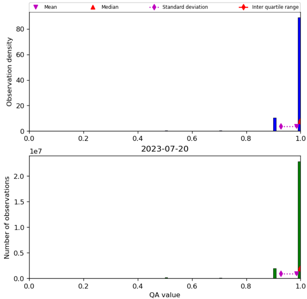
Figure 29: Histogram of “QA value” for 2023-07-19 to 2023-07-21
