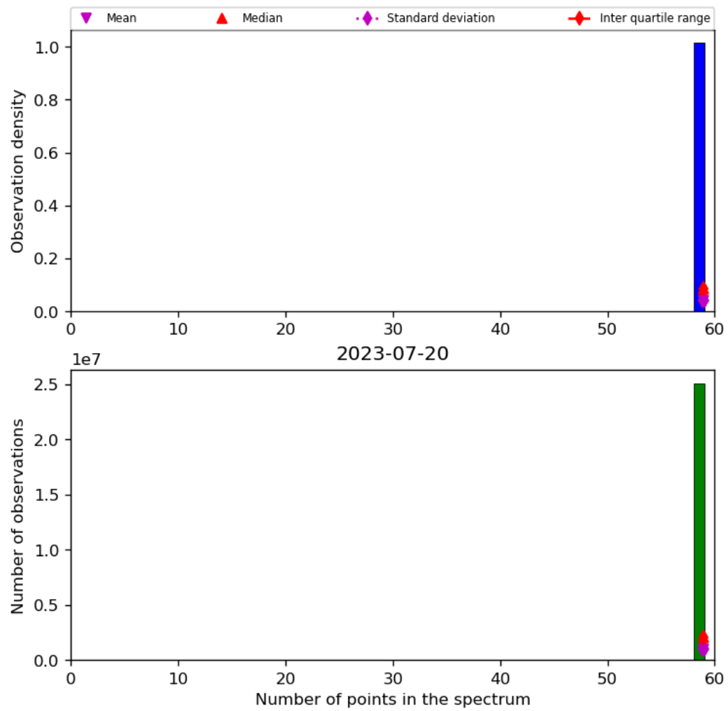
Figure 44: Histogram of “Number of points in the spectrum” for 2023-07-19 to 2023-07-21
