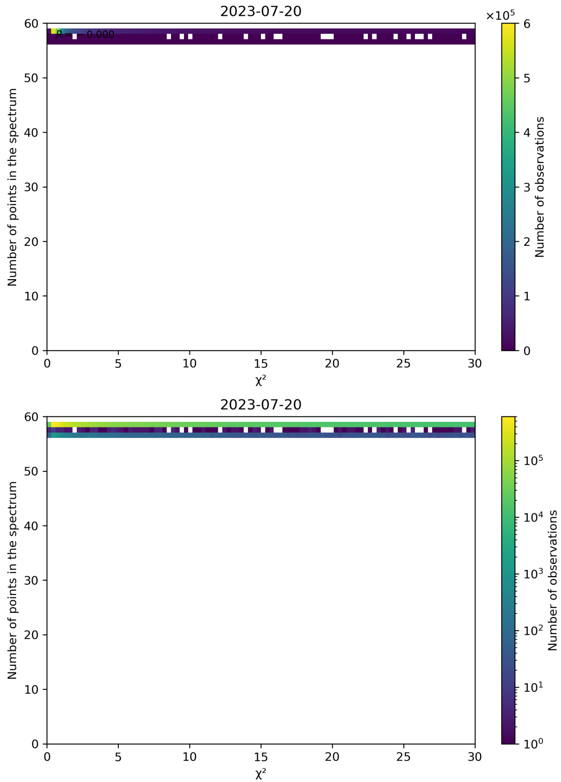
Figure 74: Scatter density plot of " \chi^2 " against "Number of points in the spectrum" for 2023-07-19 to 2023-07-21.
