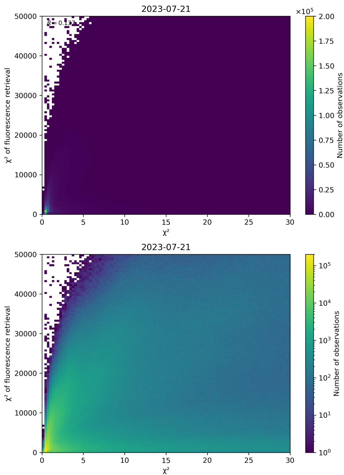
Figure 69: Scatter density plot of “ \chi^2 ” against “ \chi^2 of fluorescence retrieval” for 2023-07-20 to 2023-07-22.
