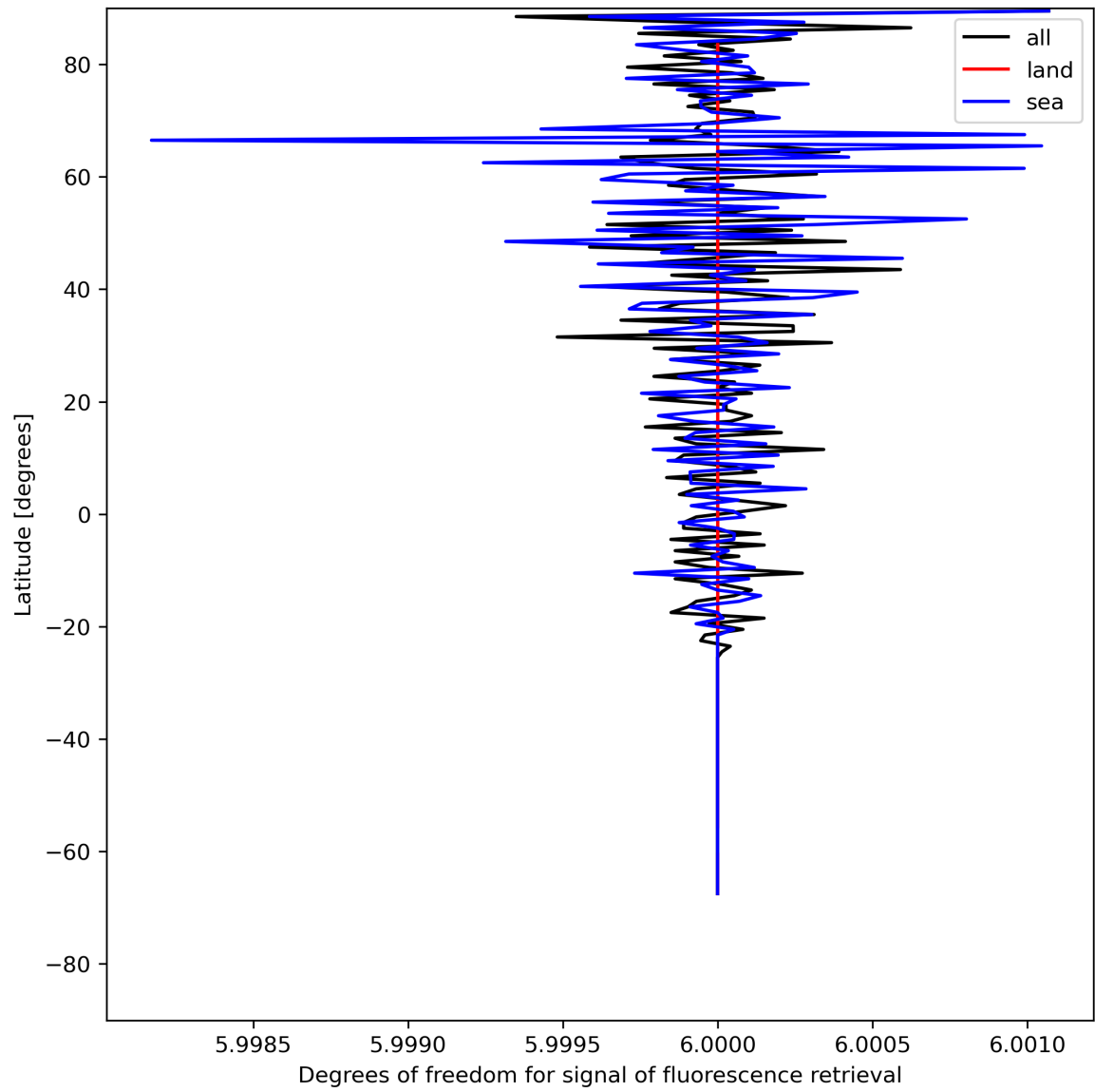
Figure 26: Zonal average of “Degrees of freedom for signal of fluorescence retrieval” for 2023-07-20 to 2023-07-22.
