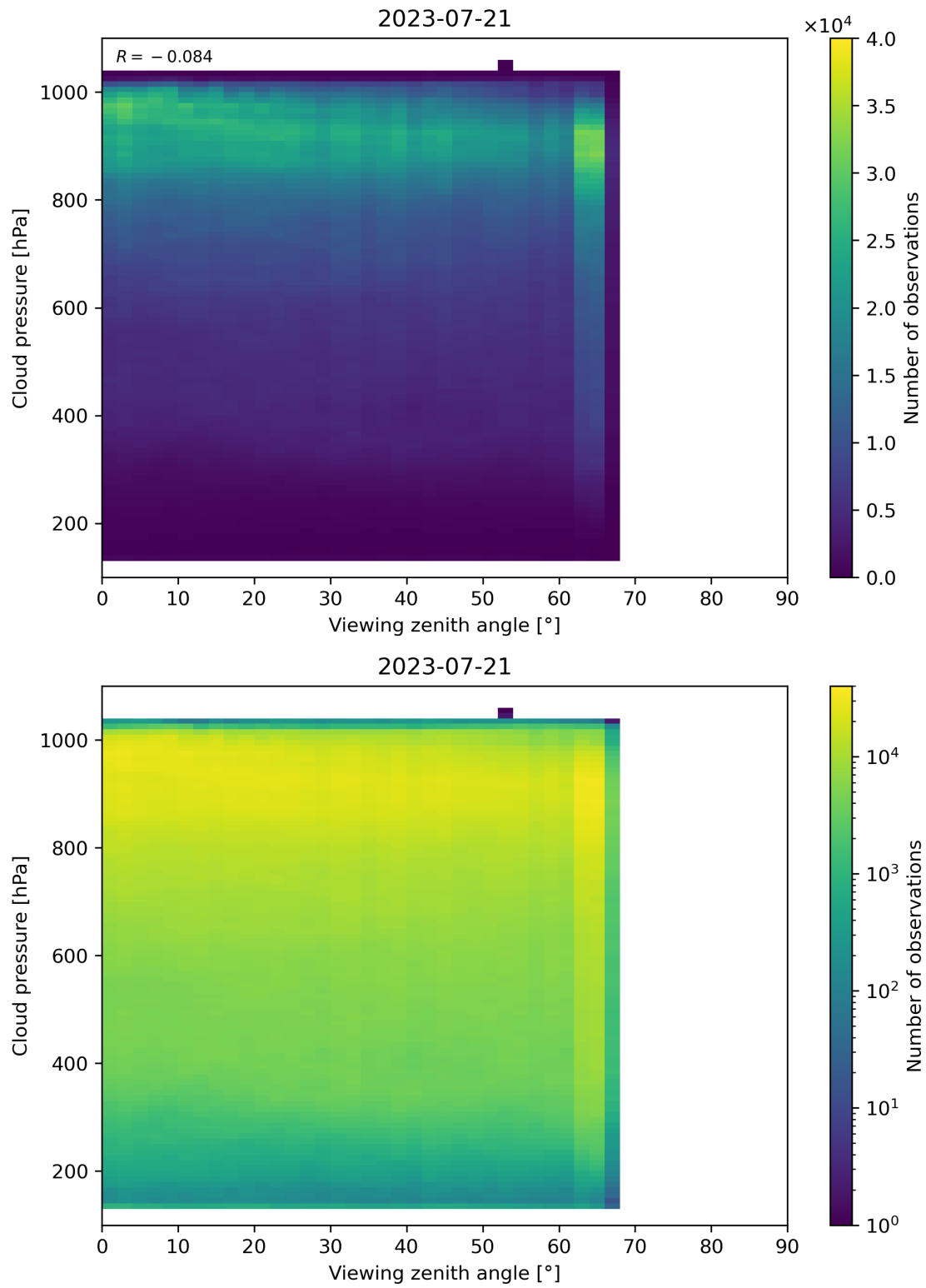
Figure 133: Scatter density plot of “Viewing zenith angle” against “Cloud pressure” for 2023-07-20 to 2023-07-22.
