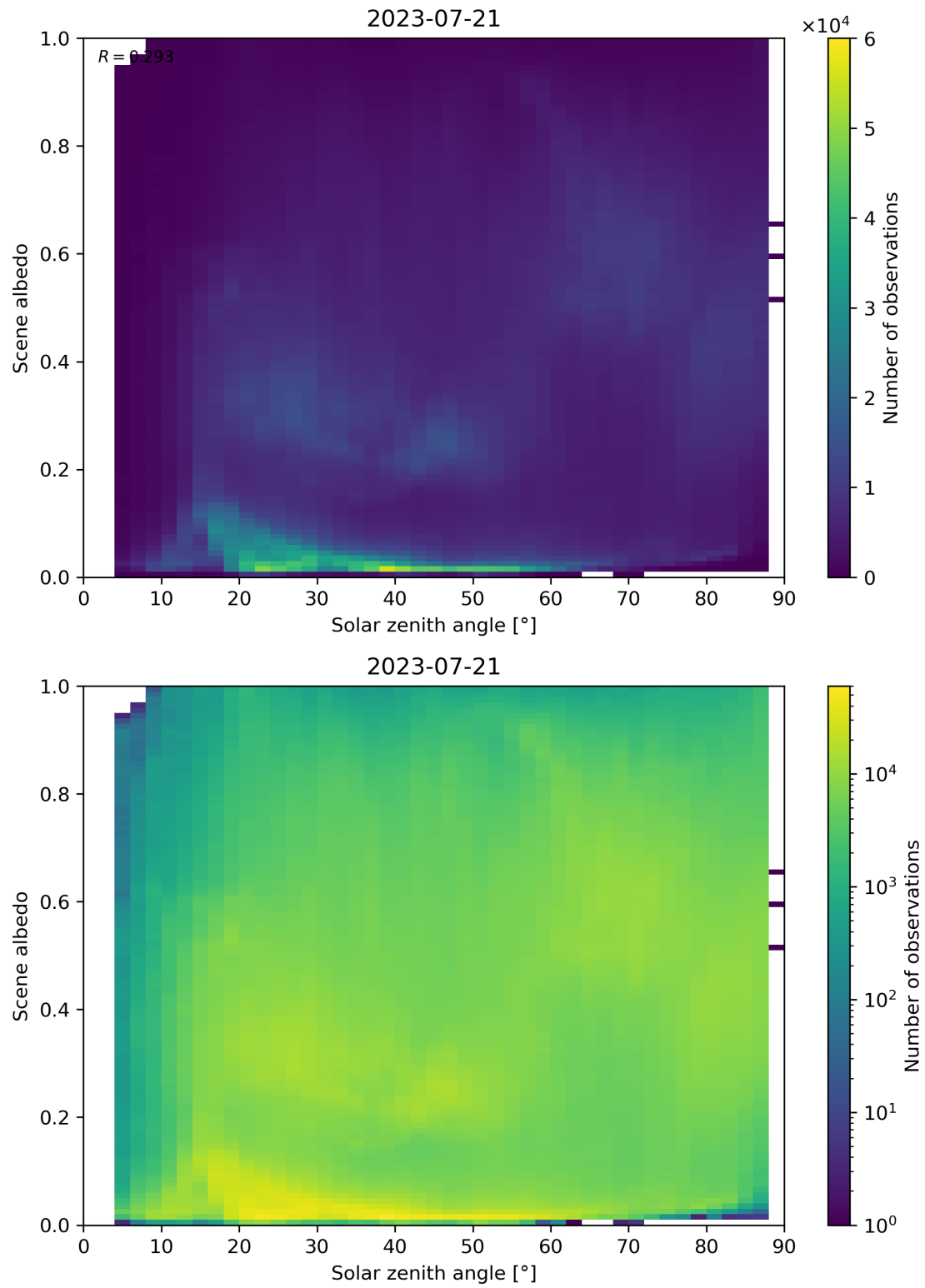
Figure 127: Scatter density plot of “Solar zenith angle” against “Scene albedo” for 2023-07-20 to 2023-07-22.
