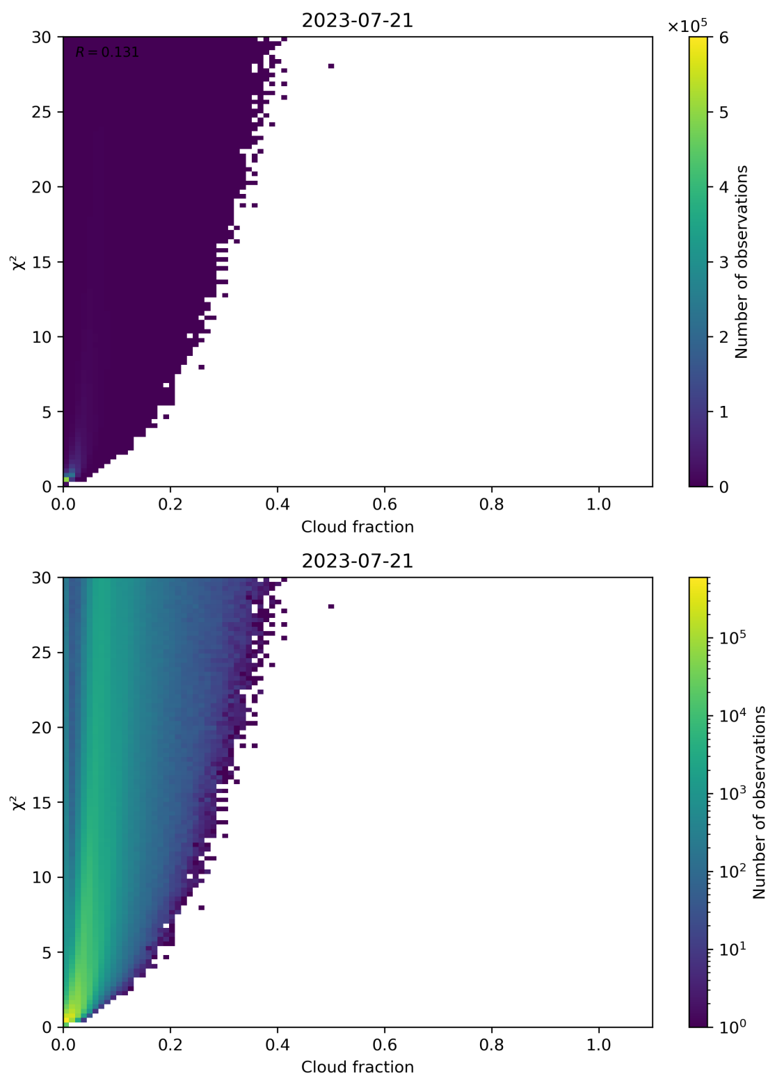
Figure 77: Scatter density plot of “Cloud fraction” against “ \chi^2 ” for 2023-07-20 to 2023-07-22.
