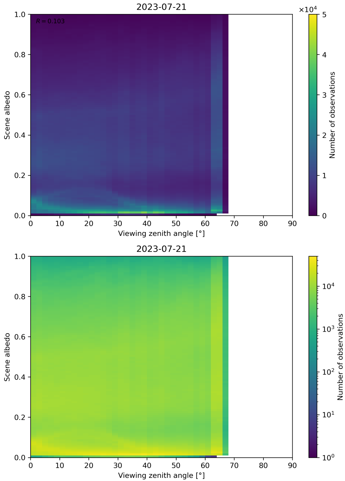
Figure 138: Scatter density plot of “Viewing zenith angle” against “Scene albedo” for 2023-07-20 to 2023-07-22.
