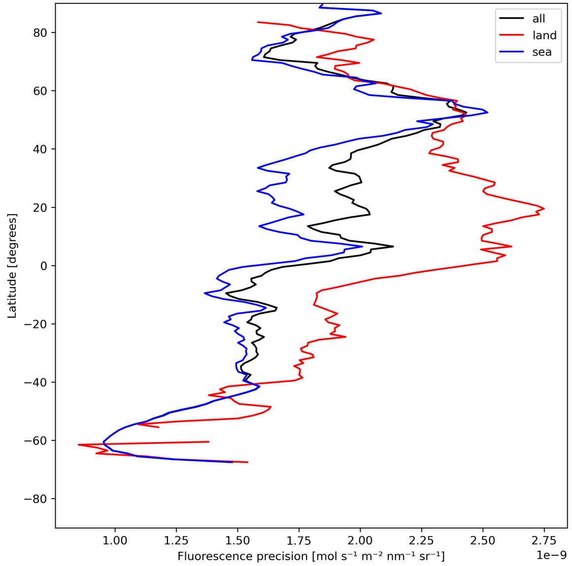
Figure 24: Zonal average of “Fluorescence precision” for 2023-07-20 to 2023-07-22.
