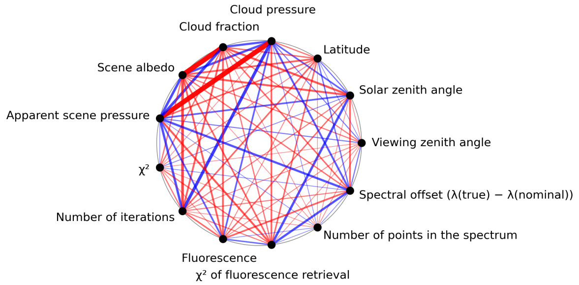
Figure 1: Map of correlation graph for 2023-07-20 to 2023-07-22.
