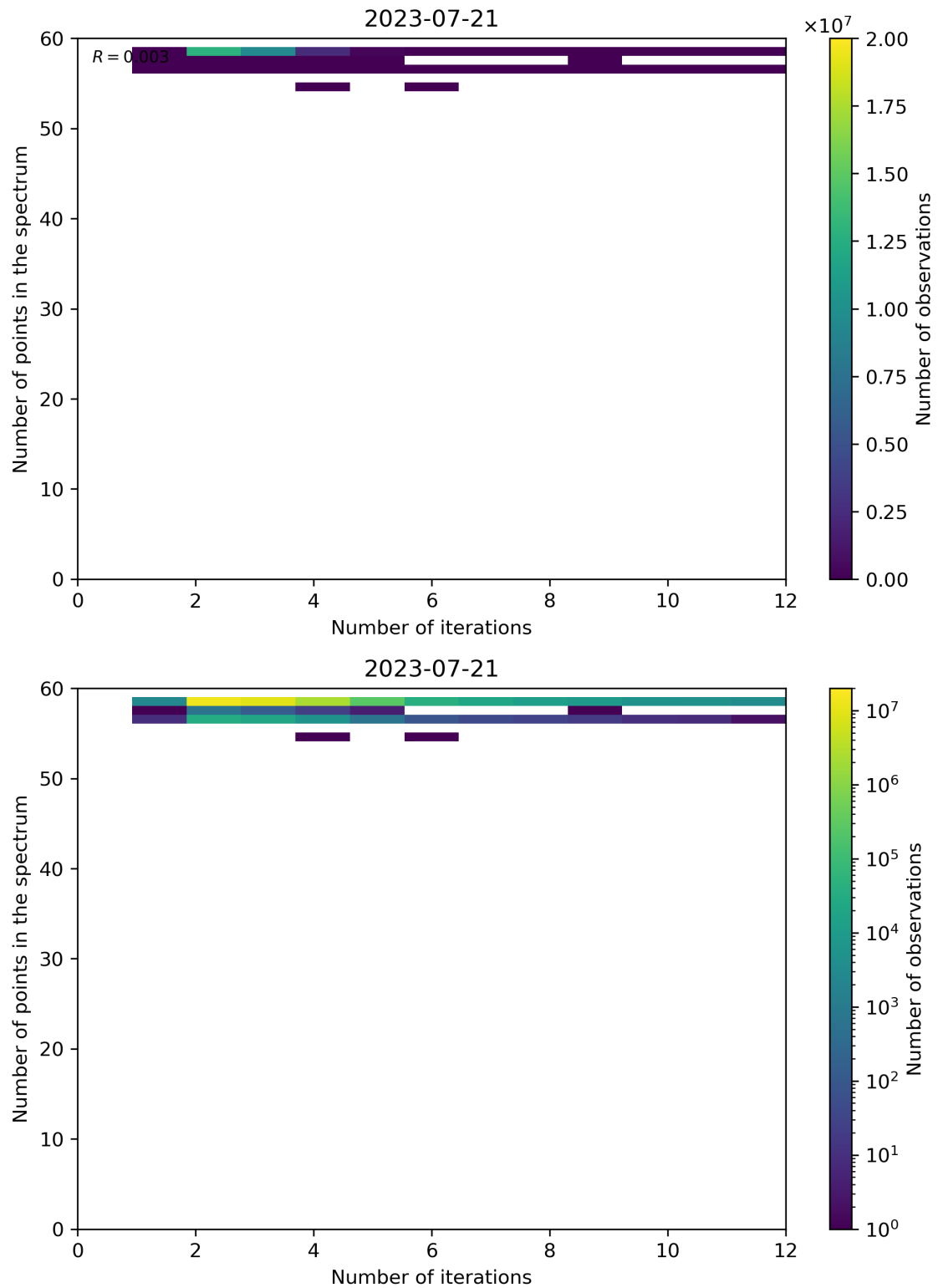
Figure 108: Scatter density plot of “Number of iterations” against “Number of points in the spectrum” for 2023-07-20 to 2023-07-22.
