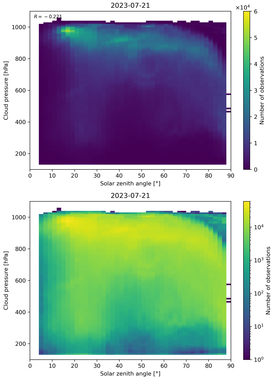
Figure 122: Scatter density plot of “Solar zenith angle” against “Cloud pressure” for 2023-07-20 to 2023-07-22.
