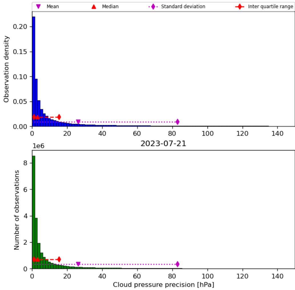
Figure 31: Histogram of “Cloud pressure precision” for 2023-07-20 to 2023-07-22
