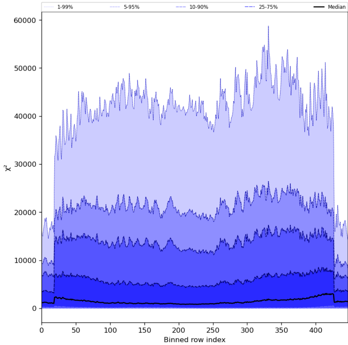
Figure 55: Along track statistics of “ \chi^2 ” for 2023-07-20 to 2023-07-22
