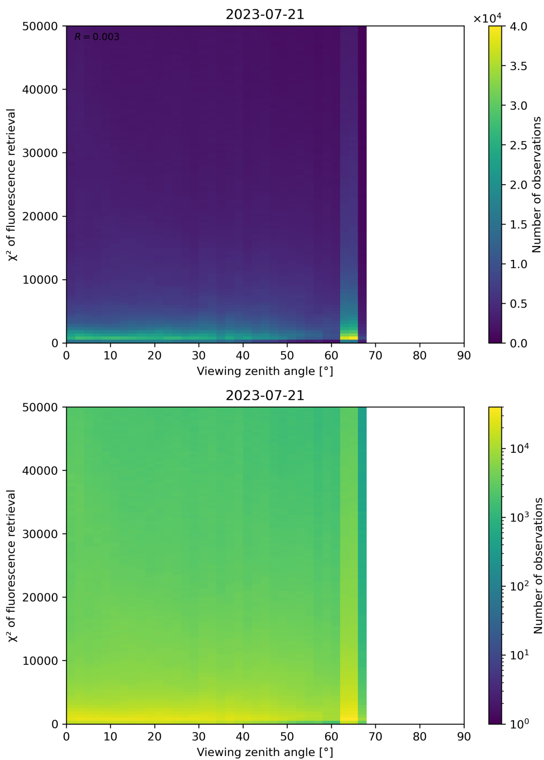
Figure 131: Scatter density plot of “Viewing zenith angle” against “ \chi^2 of fluorescence retrieval” for 2023-07-20 to 2023-07-22.
