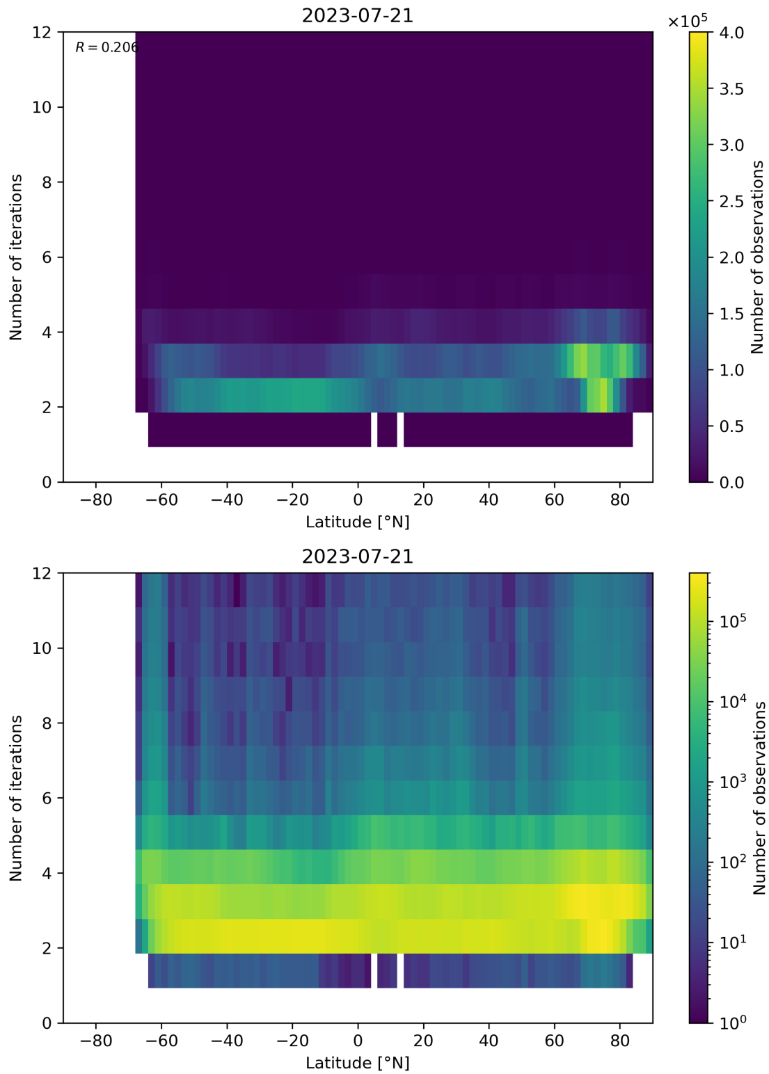
Figure 102: Scatter density plot of “Latitude” against “Number of iterations” for 2023-07-20 to 2023-07-22.
