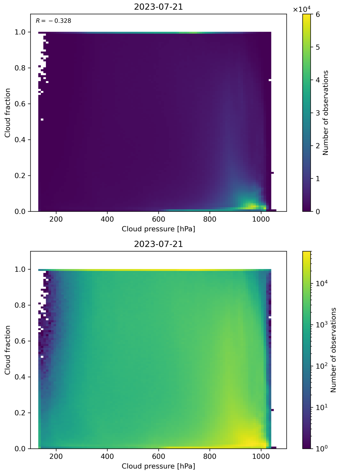
Figure 87: Scatter density plot of “Cloud pressure” against “Cloud fraction” for 2023-07-20 to 2023-07-22.
