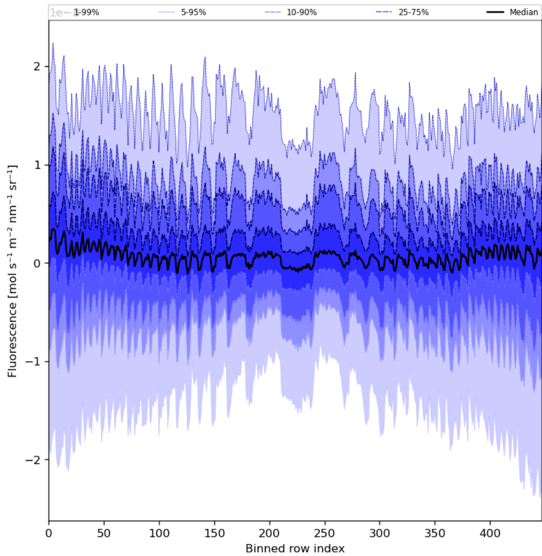
Figure 57: Along track statistics of “Fluorescence” for 2023-07-20 to 2023-07-22
