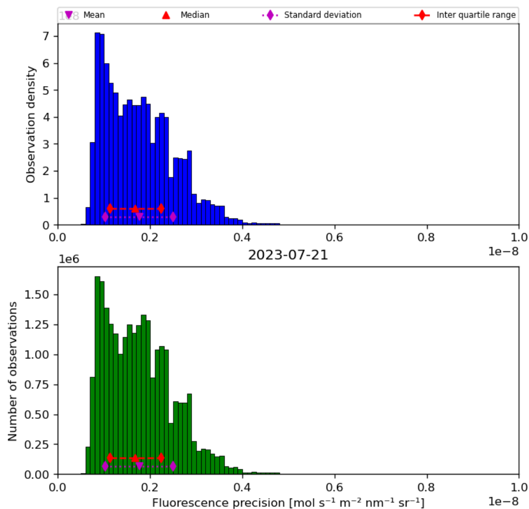
Figure 41: Histogram of “Fluorescence precision” for 2023-07-20 to 2023-07-22
