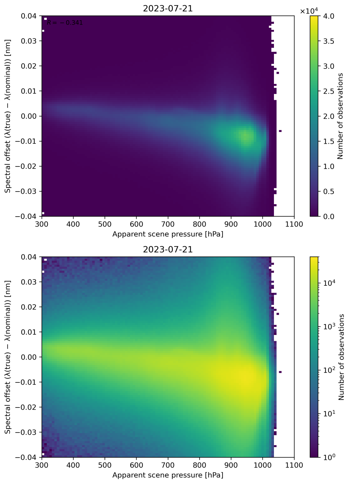
Figure 68: Scatter density plot of “Apparent scene pressure” against “Spectral offset ( \lambda(\text{true}) - \lambda(\text{nominal}) )” for 2023-07-20 to 2023-07-22.
