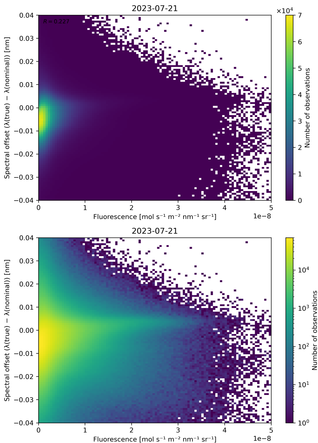
Figure 95: Scatter density plot of “Fluorescence” against “Spectral offset ( \lambda(\text{true}) - \lambda(\text{nominal}) )” for 2023-07-20 to 2023-07-22.
