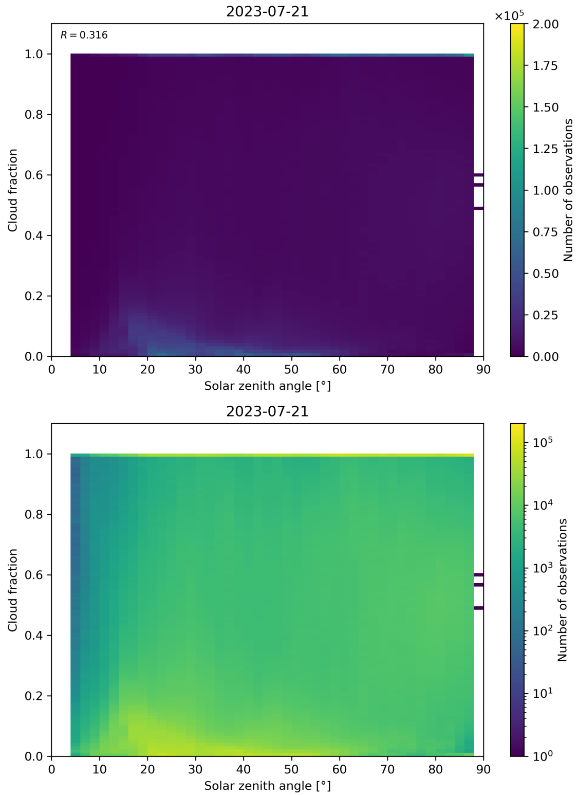
Figure 121: Scatter density plot of “Solar zenith angle” against “Cloud fraction” for 2023-07-20 to 2023-07-22.
