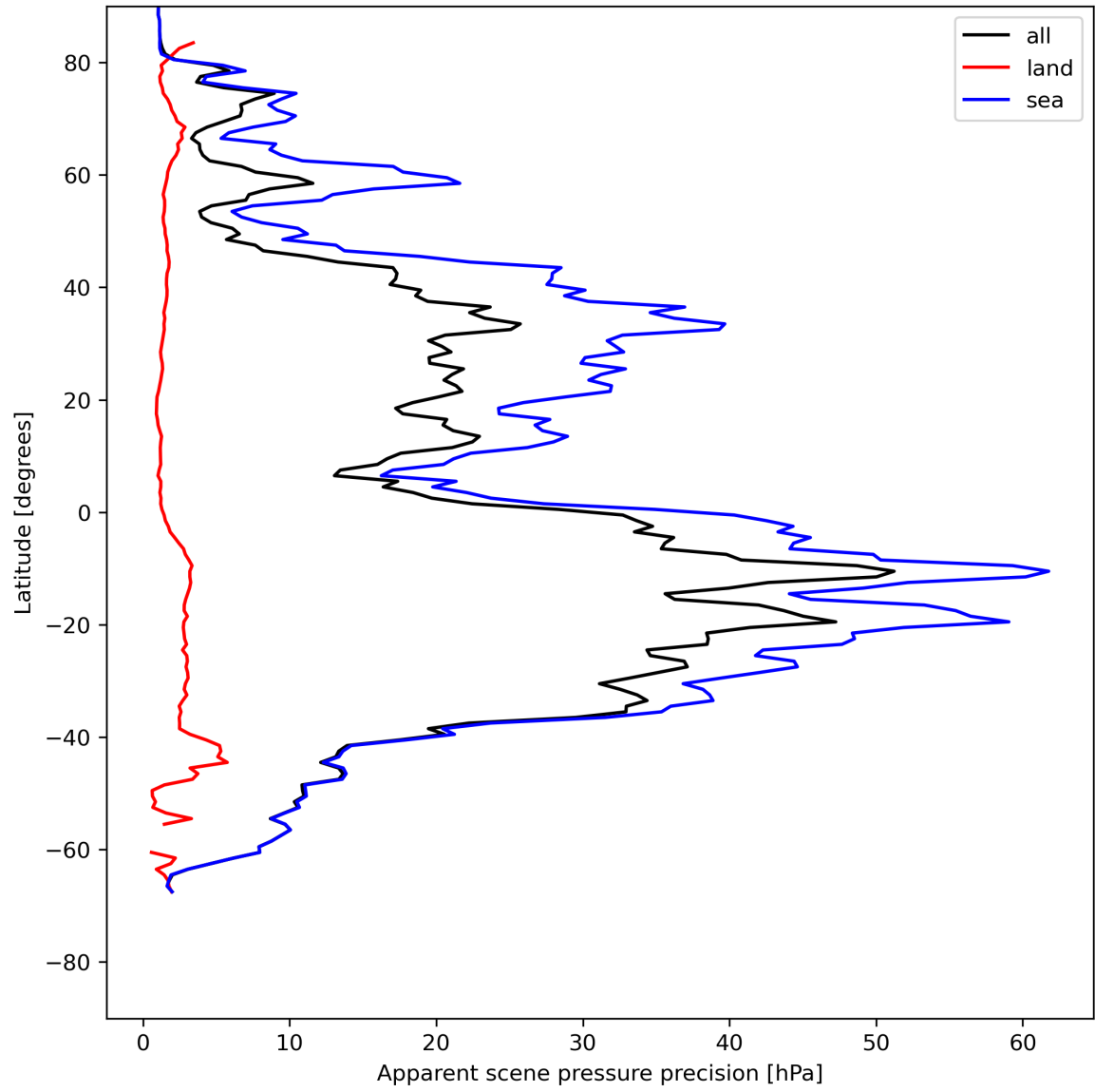
Figure 20: Zonal average of “Apparent scene pressure precision” for 2023-07-20 to 2023-07-22.
