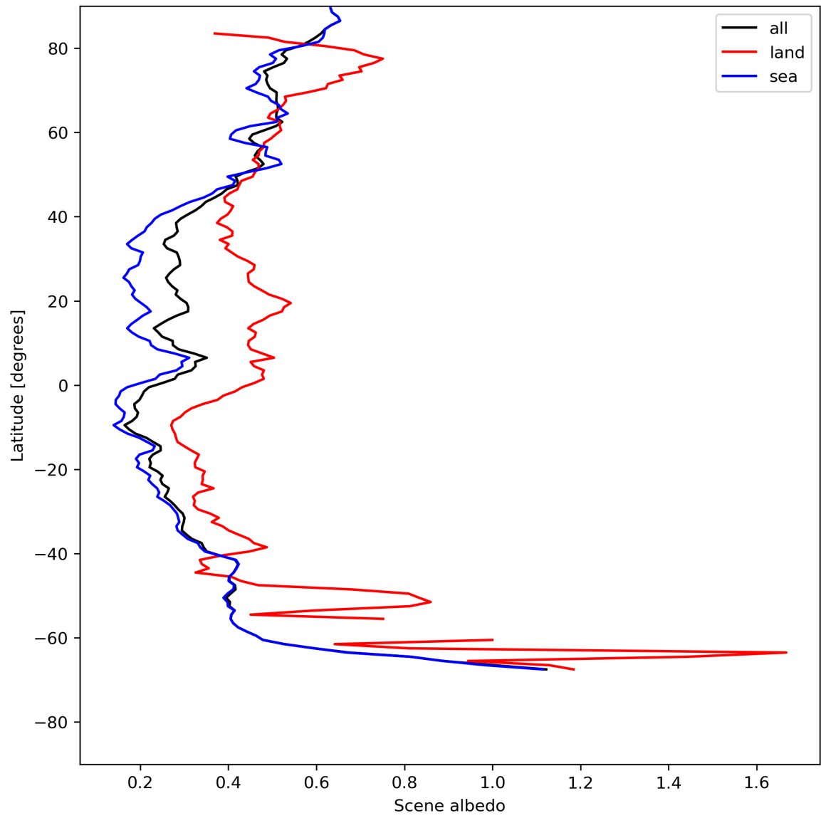
Figure 17: Zonal average of “Scene albedo” for 2023-07-20 to 2023-07-22.
