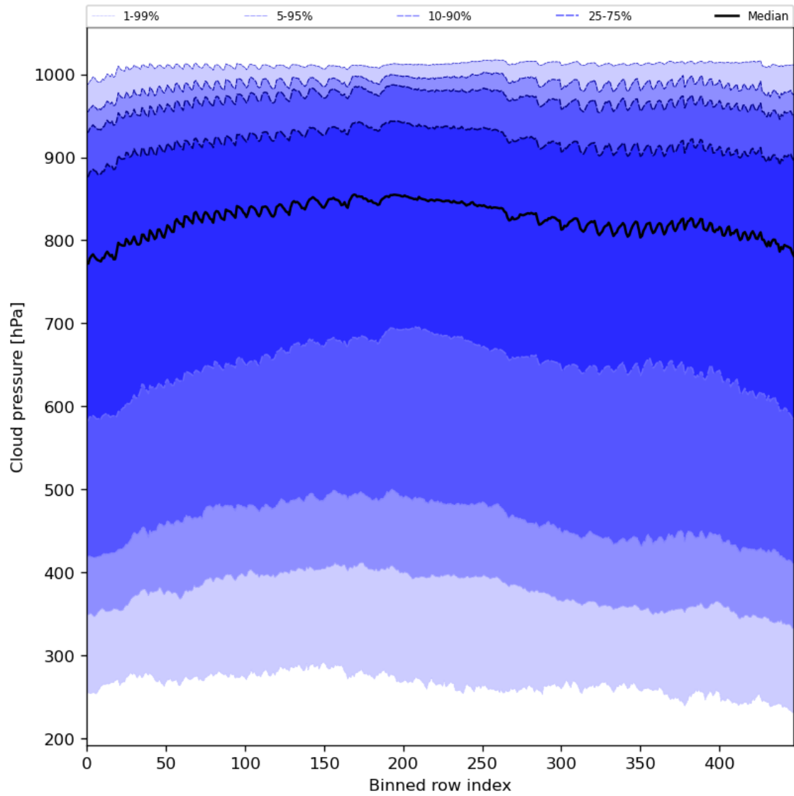
Figure 47: Along track statistics of “Cloud pressure” for 2023-07-20 to 2023-07-22
