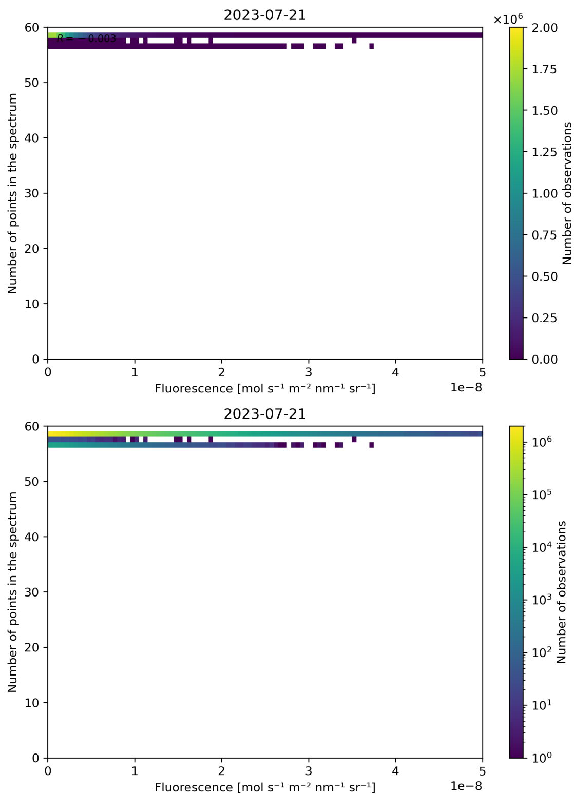
Figure 94: Scatter density plot of “Fluorescence” against “Number of points in the spectrum” for 2023-07-20 to 2023-07-22.
