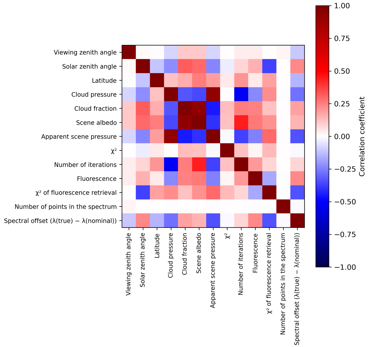
Figure 2: Map of correlation matrix for 2023-07-20 to 2023-07-22.
