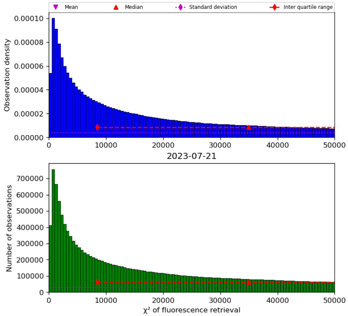
Figure 42: Histogram of “ \chi^2 of fluorescence retrieval” for 2023-07-20 to 2023-07-22
