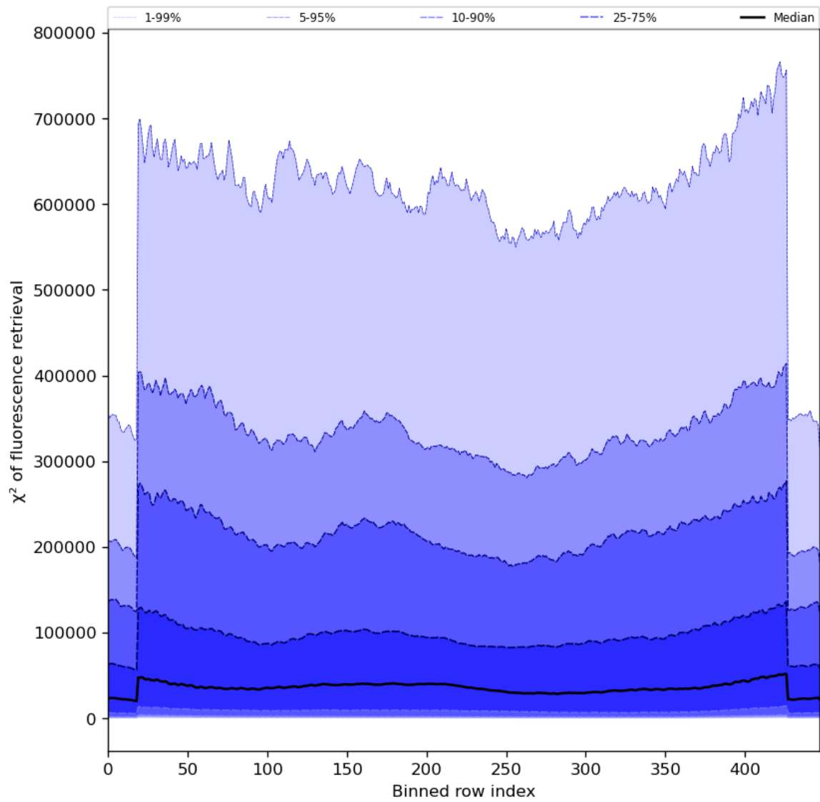
Figure 59: Along track statistics of “ \chi^2 of fluorescence retrieval” for 2023-07-20 to 2023-07-22
