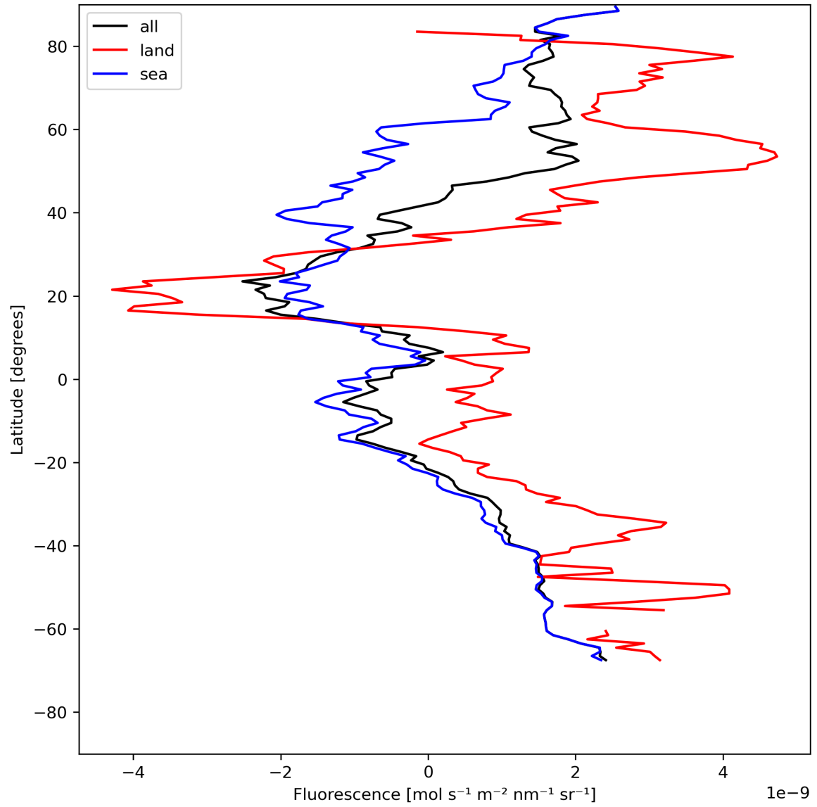
Figure 23: Zonal average of “Fluorescence” for 2023-07-20 to 2023-07-22.
