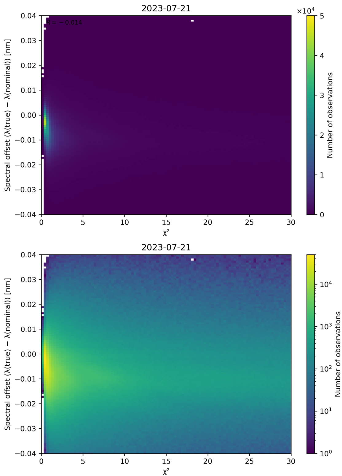
Figure 75: Scatter density plot of “ \chi^2 ” against “Spectral offset ( \lambda(\text{true}) - \lambda(\text{nominal}) )” for 2023-07-20 to 2023-07-22.
