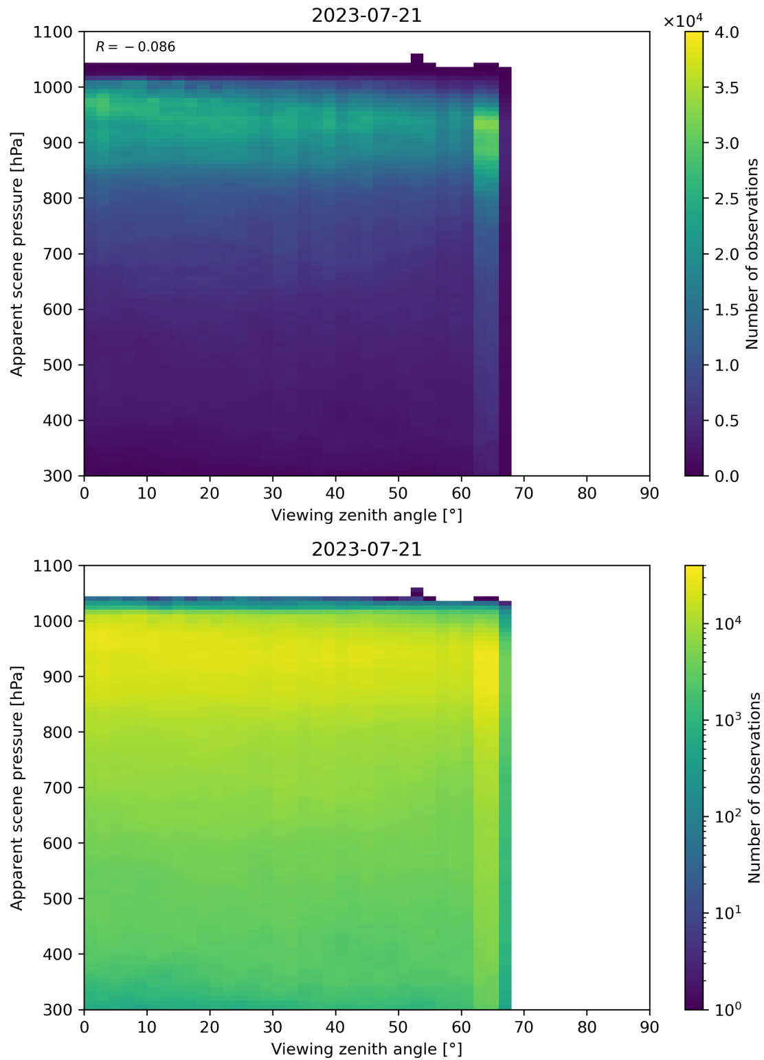
Figure 129: Scatter density plot of “Viewing zenith angle” against “Apparent scene pressure” for 2023-07-20 to 2023-07-22.
