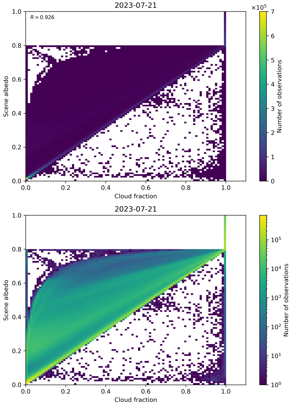
Figure 82: Scatter density plot of “Cloud fraction” against “Scene albedo” for 2023-07-20 to 2023-07-22.
