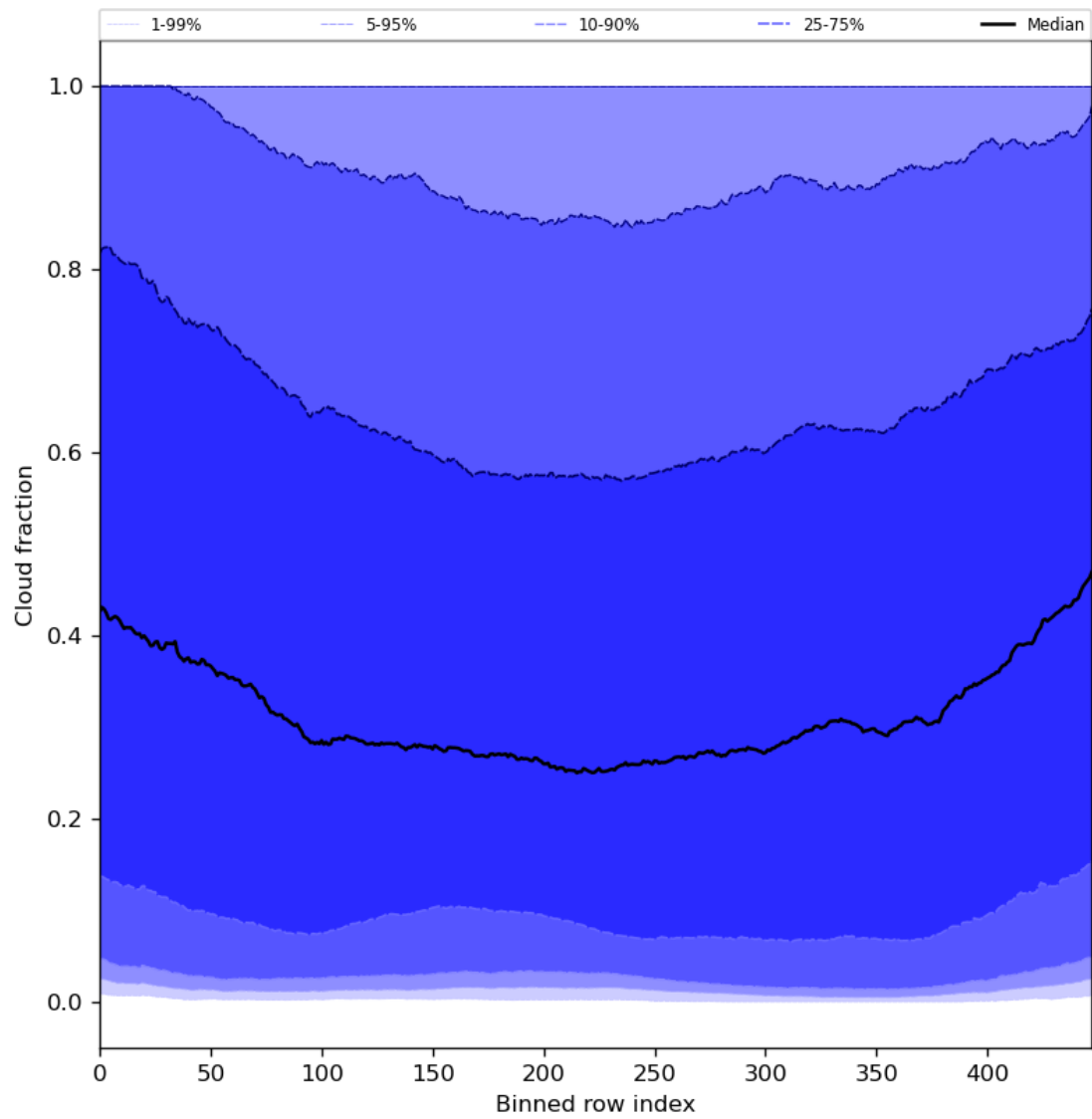
Figure 49: Along track statistics of “Cloud fraction” for 2023-07-20 to 2023-07-22
