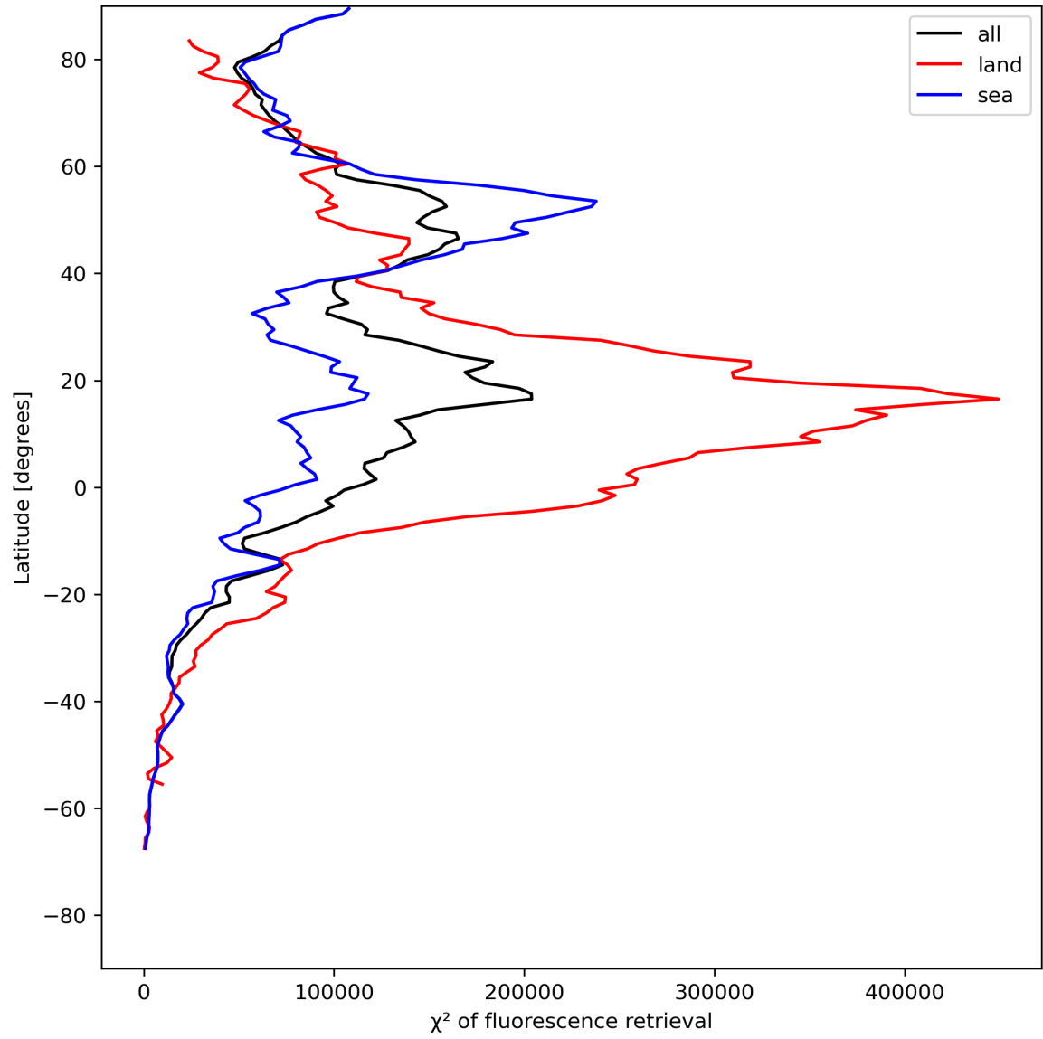
Figure 25: Zonal average of “ \chi^2 of fluorescence retrieval” for 2023-07-20 to 2023-07-22.
