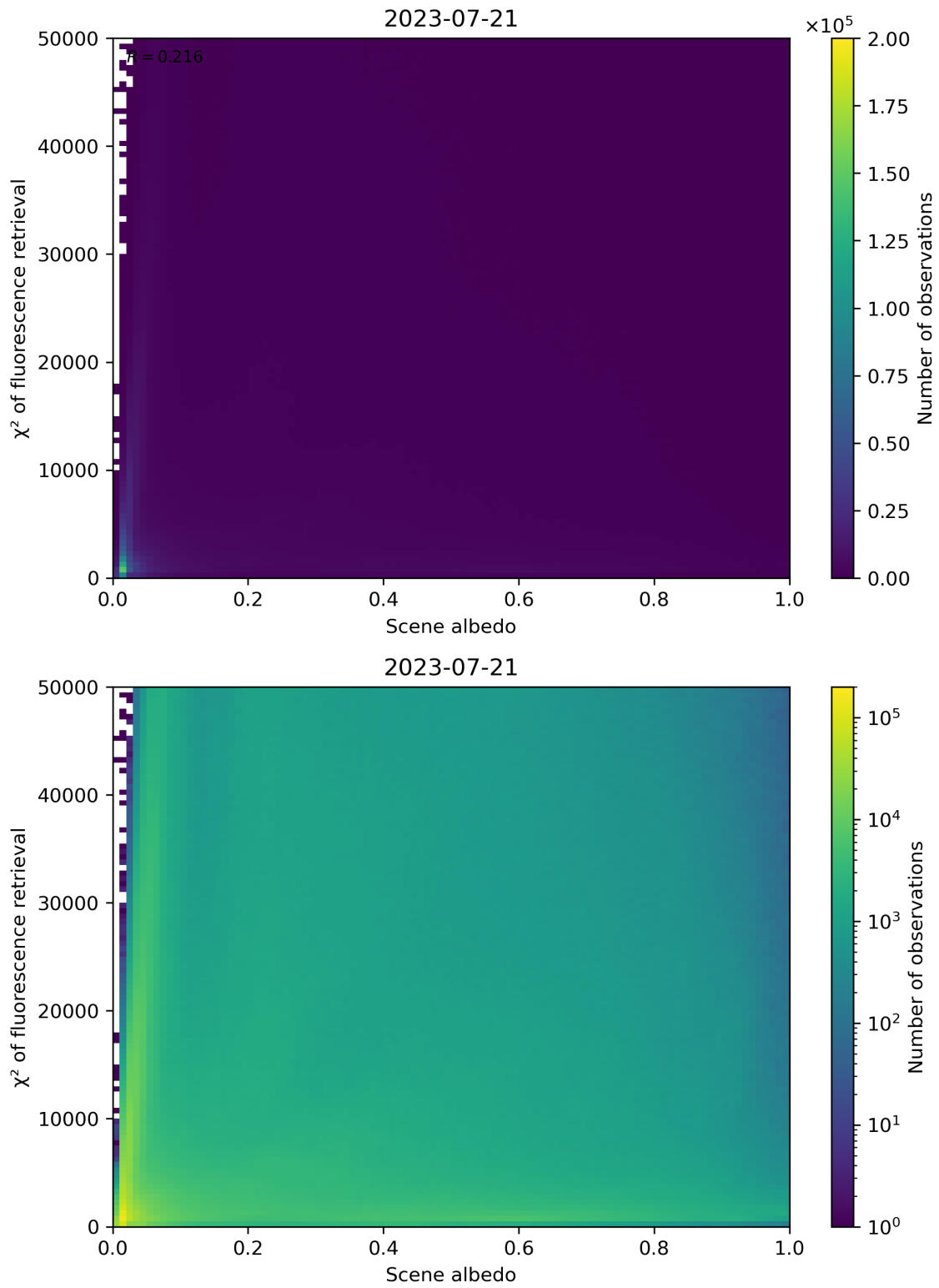
Figure 113: Scatter density plot of “Scene albedo” against “ \chi^2 of fluorescence retrieval” for 2023-07-20 to 2023-07-22.
