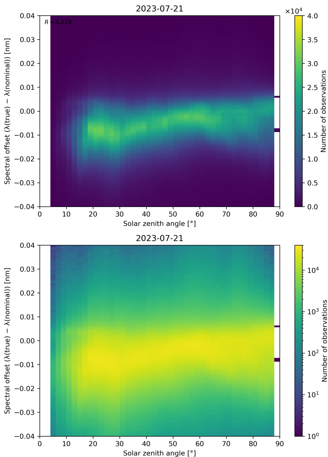
Figure 128: Scatter density plot of “Solar zenith angle” against “Spectral offset ( \lambda(\text{true}) - \lambda(\text{nominal}) )” for 2023-07-20 to 2023-07-22.
