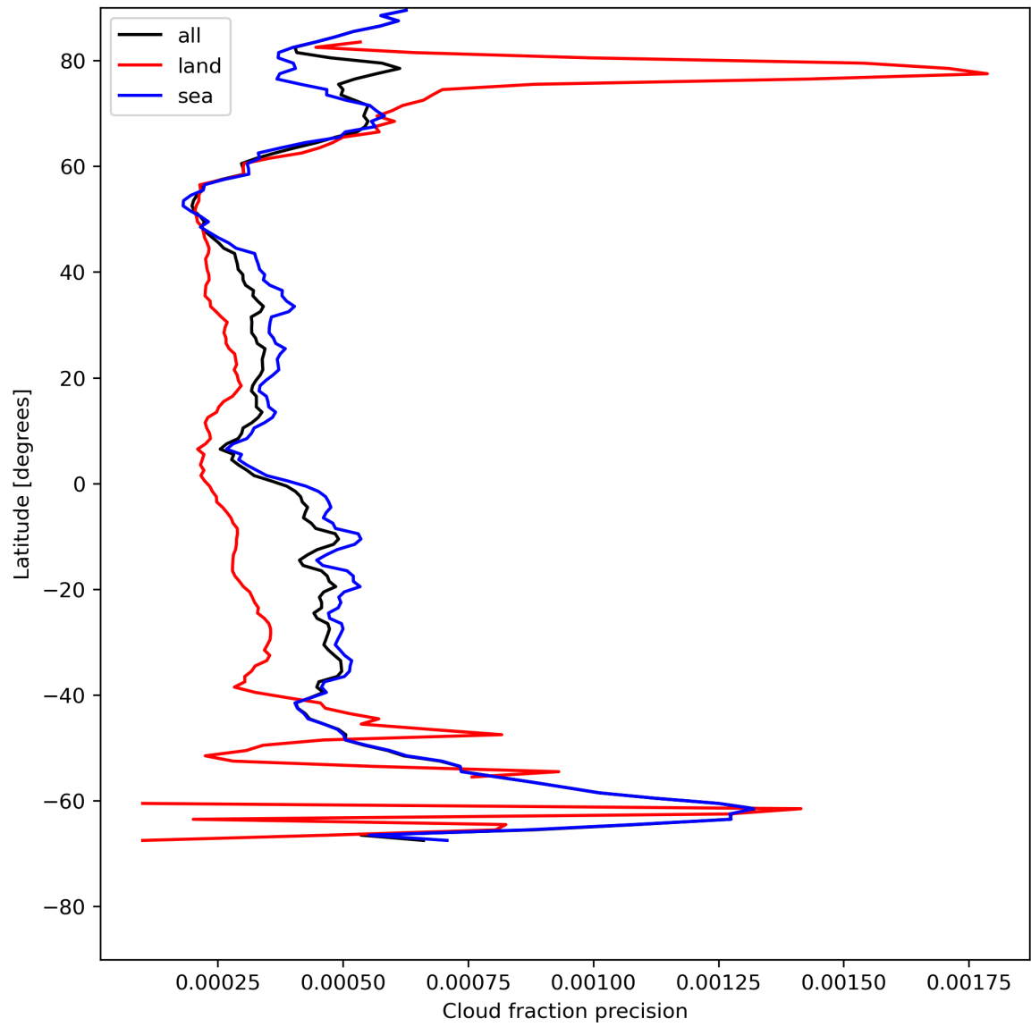
Figure 16: Zonal average of “Cloud fraction precision” for 2023-07-20 to 2023-07-22.
