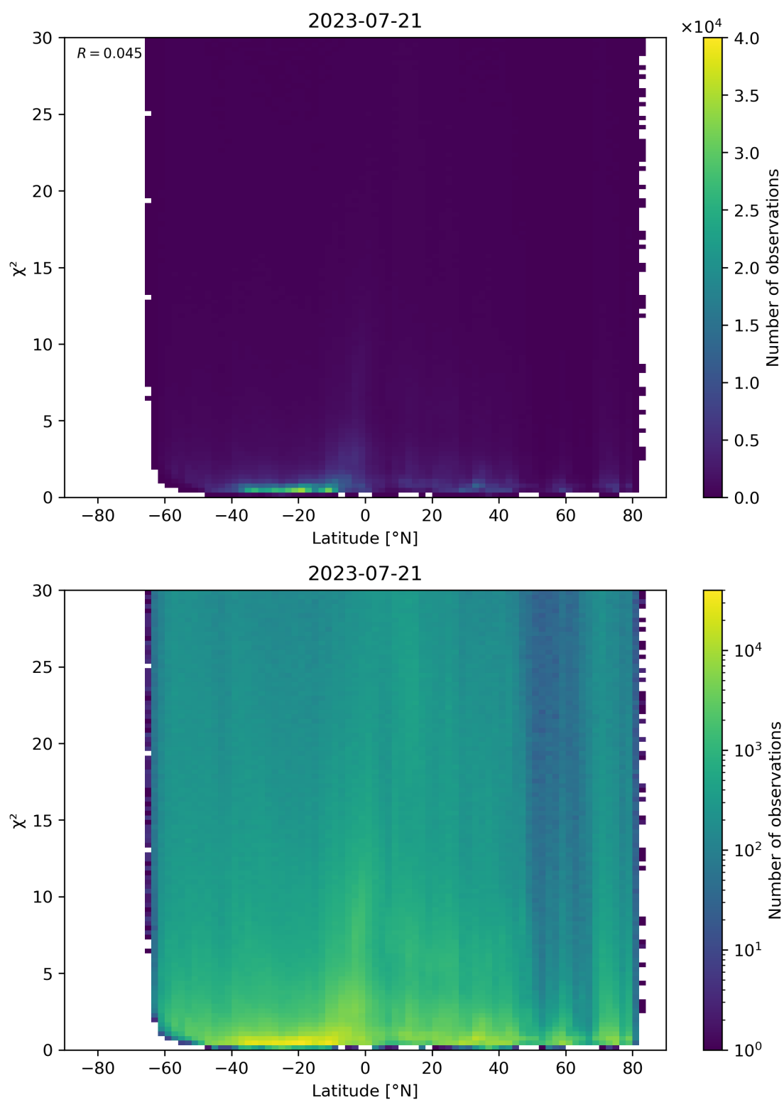
Figure 97: Scatter density plot of “Latitude” against “ \chi^2 ” for 2023-07-20 to 2023-07-22.
