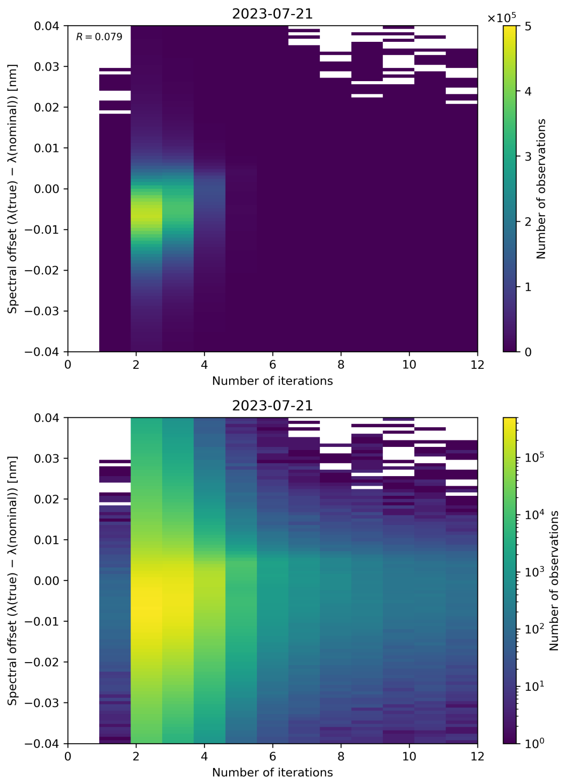
Figure 109: Scatter density plot of “Number of iterations” against “Spectral offset ( \lambda(\text{true}) - \lambda(\text{nominal}) )” for 2023-07-20 to 2023-07-22.
