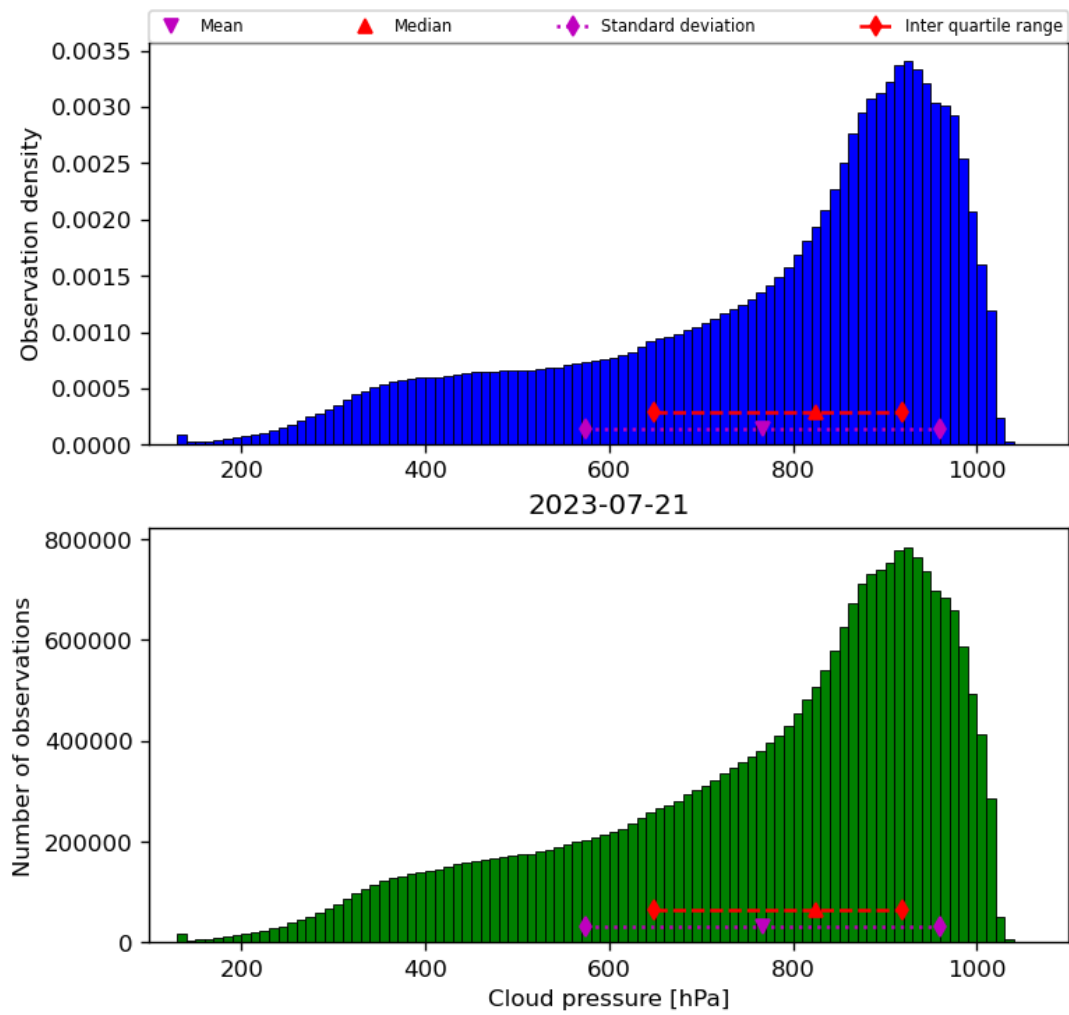
Figure 30: Histogram of “Cloud pressure” for 2023-07-20 to 2023-07-22
