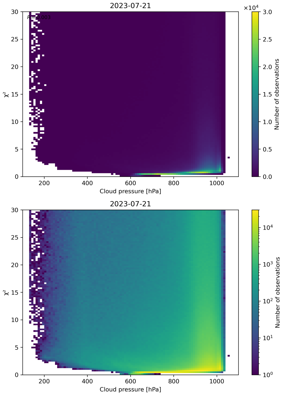
Figure 85: Scatter density plot of “Cloud pressure” against “ \chi^2 ” for 2023-07-20 to 2023-07-22.
