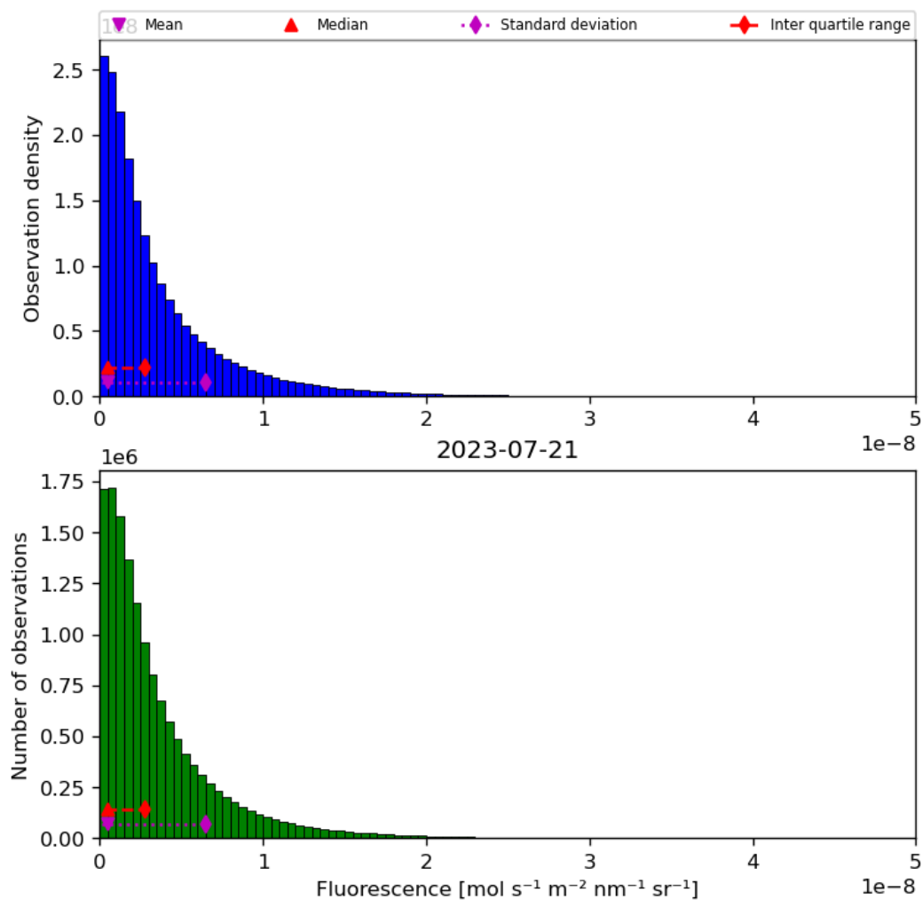
Figure 40: Histogram of “Fluorescence” for 2023-07-20 to 2023-07-22
