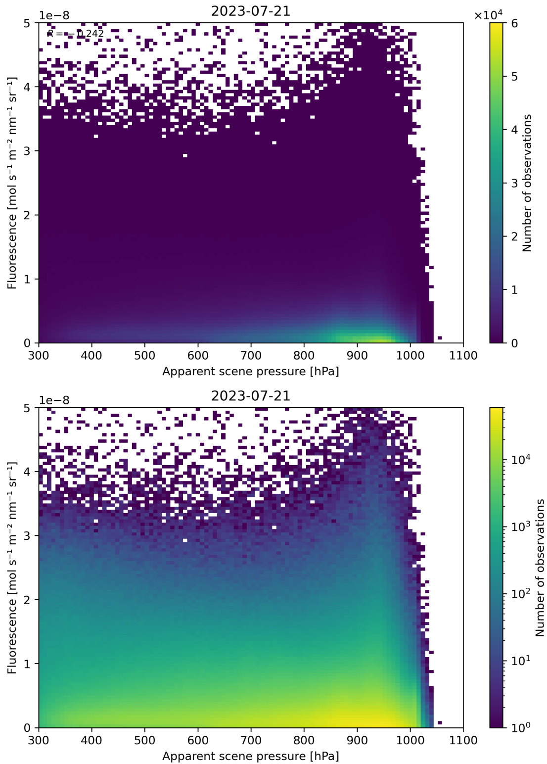
Figure 65: Scatter density plot of “Apparent scene pressure” against “Fluorescence” for 2023-07-20 to 2023-07-22.
