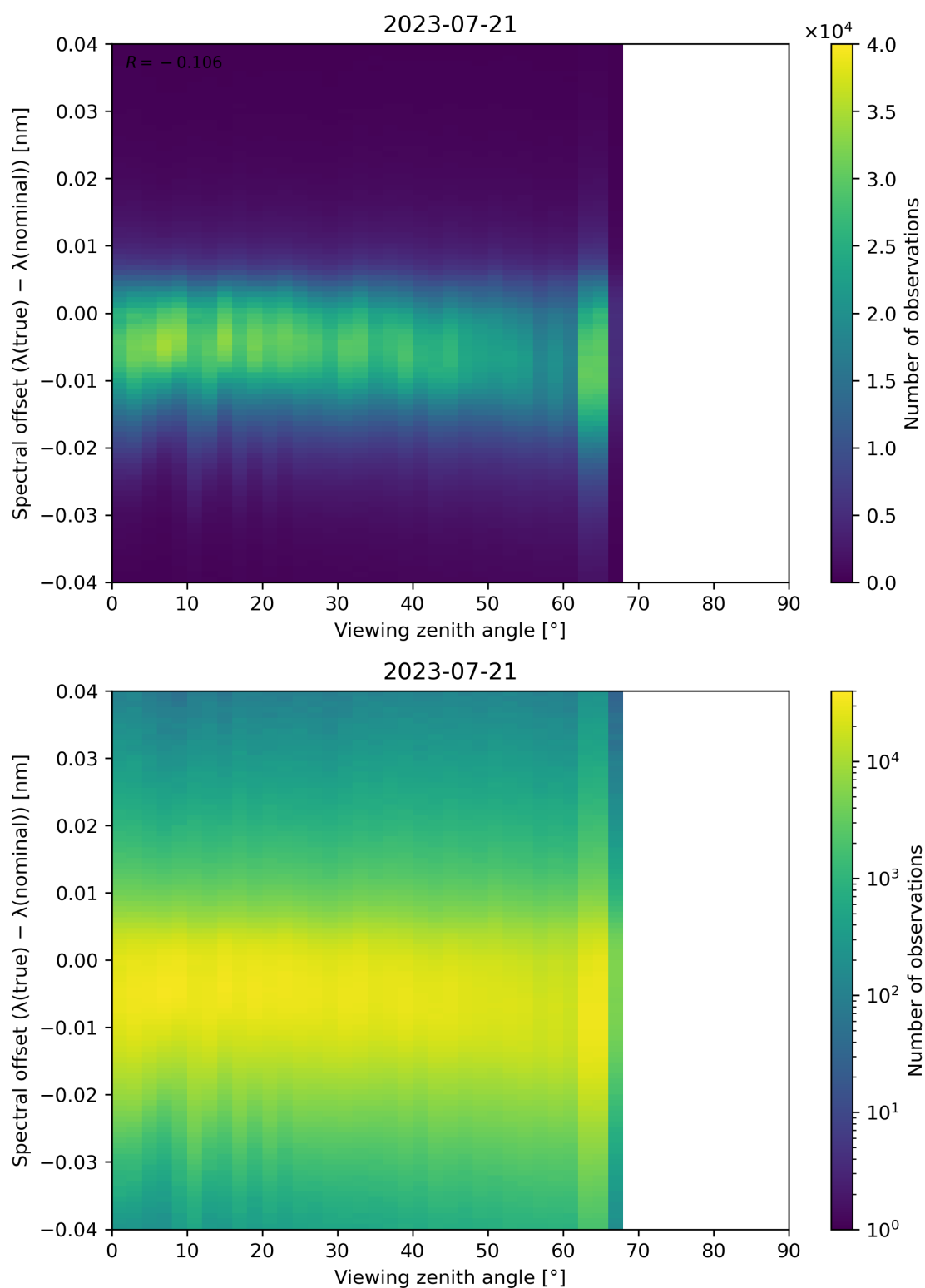
Figure 140: Scatter density plot of “Viewing zenith angle” against “Spectral offset ( \lambda(\text{true}) - \lambda(\text{nominal}) )” for 2023-07-20 to 2023-07-22.
