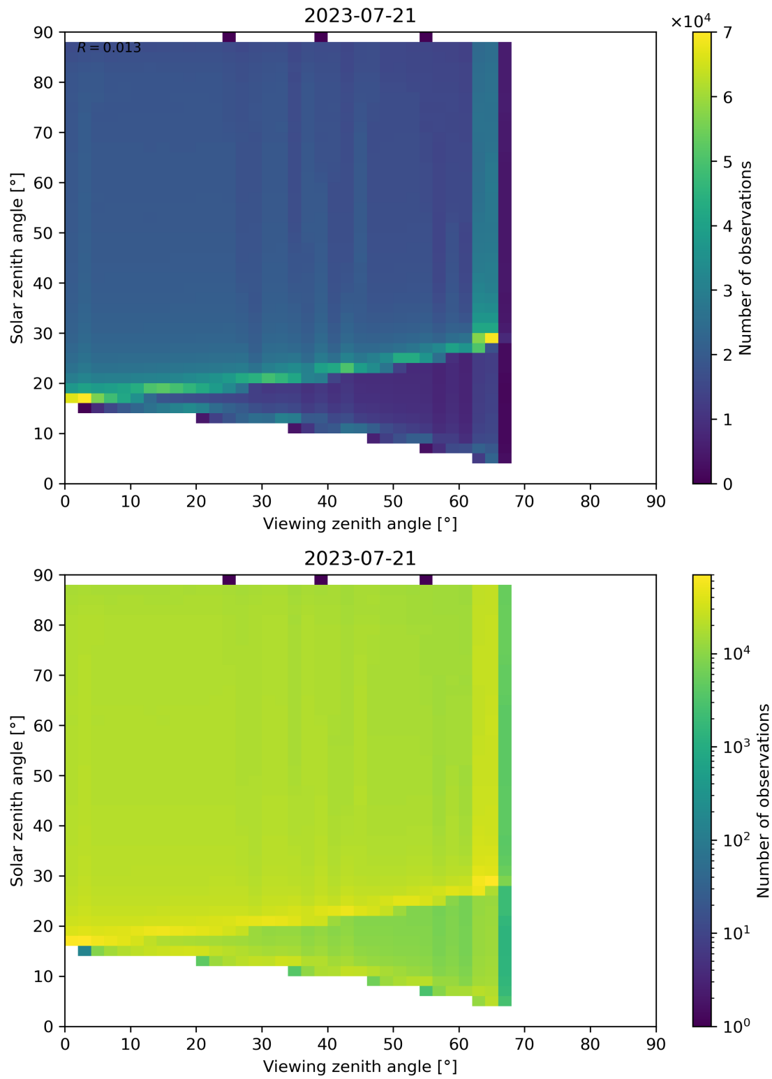
Figure 139: Scatter density plot of “Viewing zenith angle” against “Solar zenith angle” for 2023-07-20 to 2023-07-22.
