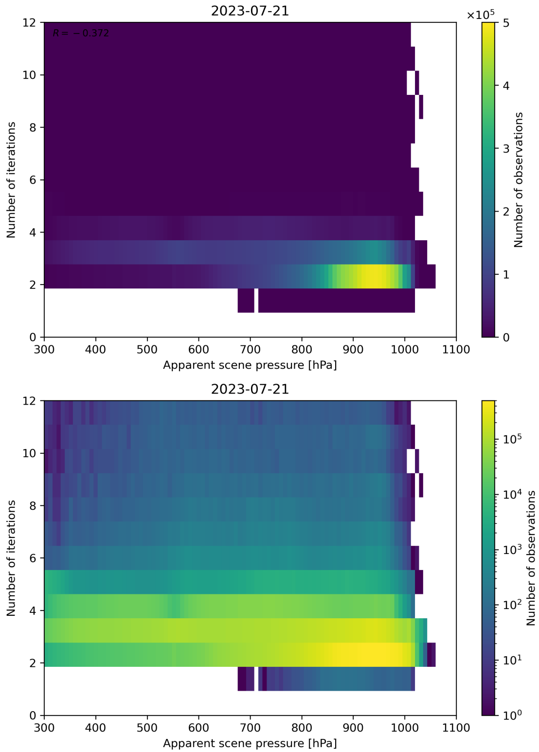
Figure 66: Scatter density plot of “Apparent scene pressure” against “Number of iterations” for 2023-07-20 to 2023-07-22.
