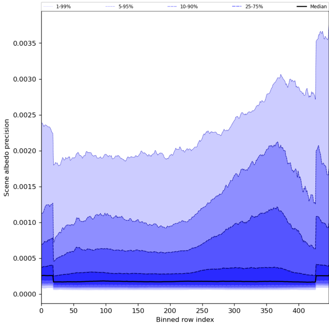
Figure 52: Along track statistics of “Scene albedo precision” for 2023-07-20 to 2023-07-22
