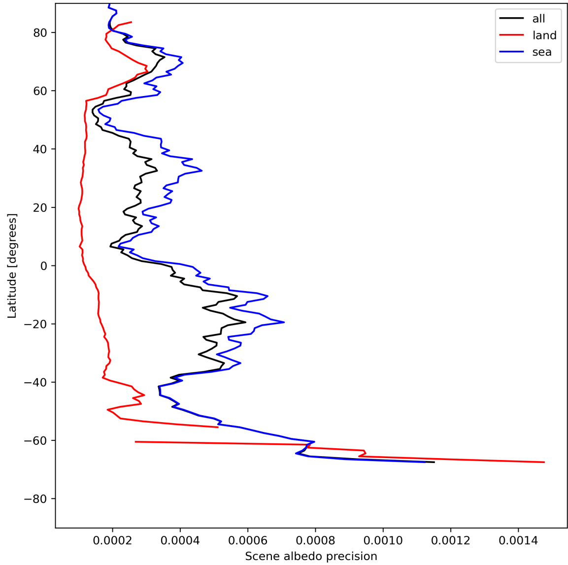
Figure 18: Zonal average of “Scene albedo precision” for 2023-07-20 to 2023-07-22.
