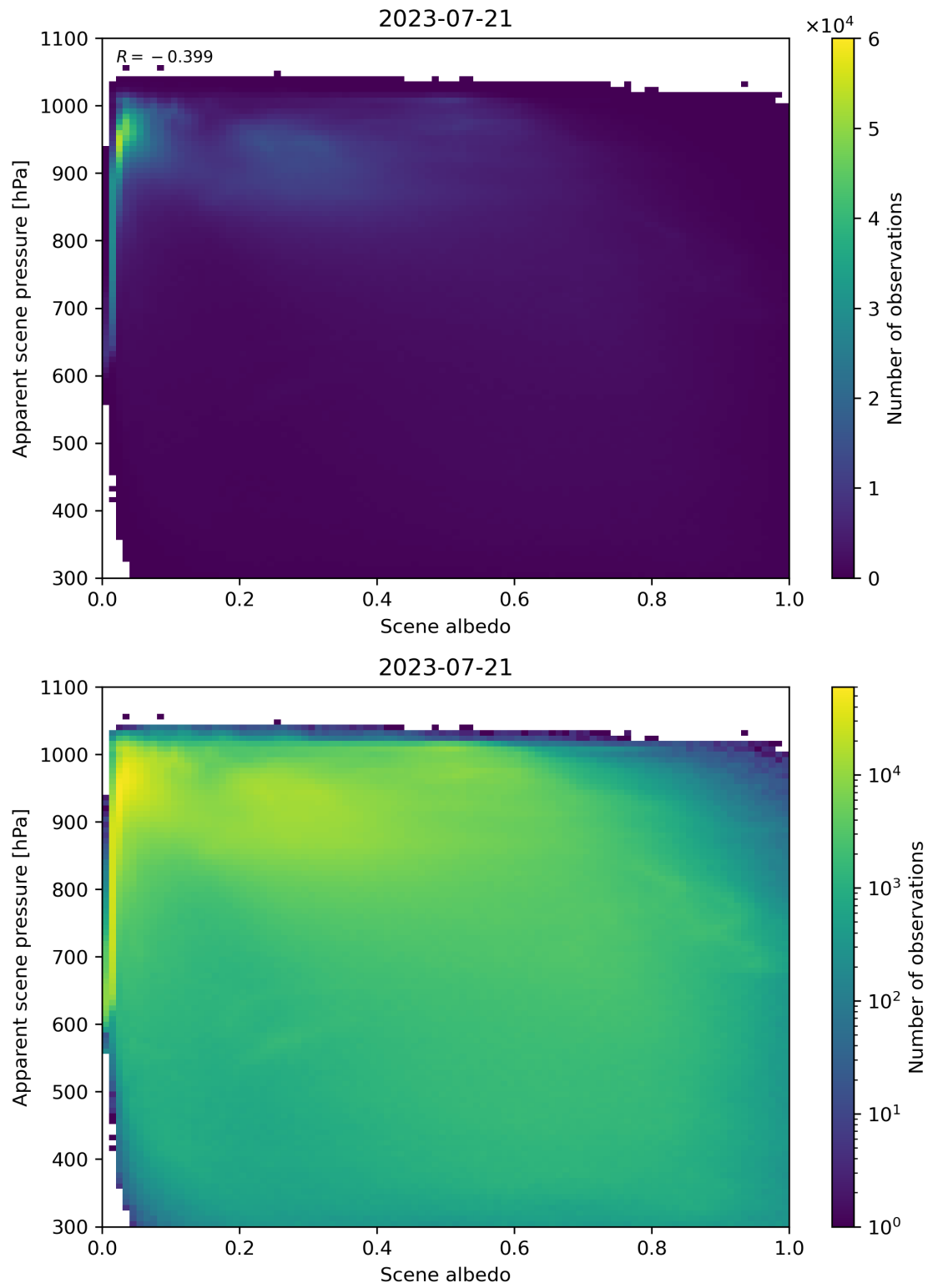
Figure 111: Scatter density plot of “Scene albedo” against “Apparent scene pressure” for 2023-07-20 to 2023-07-22.
