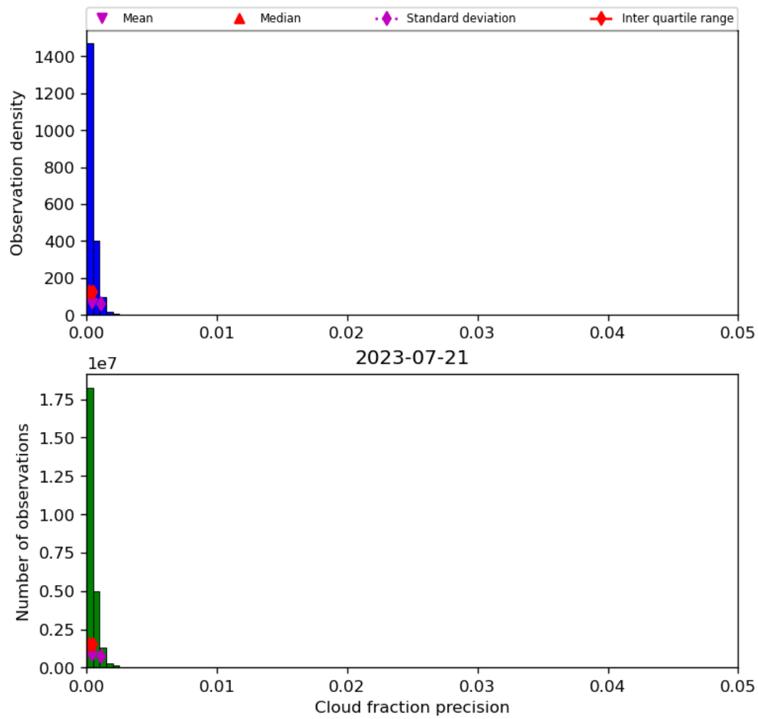
Figure 33: Histogram of “Cloud fraction precision” for 2023-07-20 to 2023-07-22
