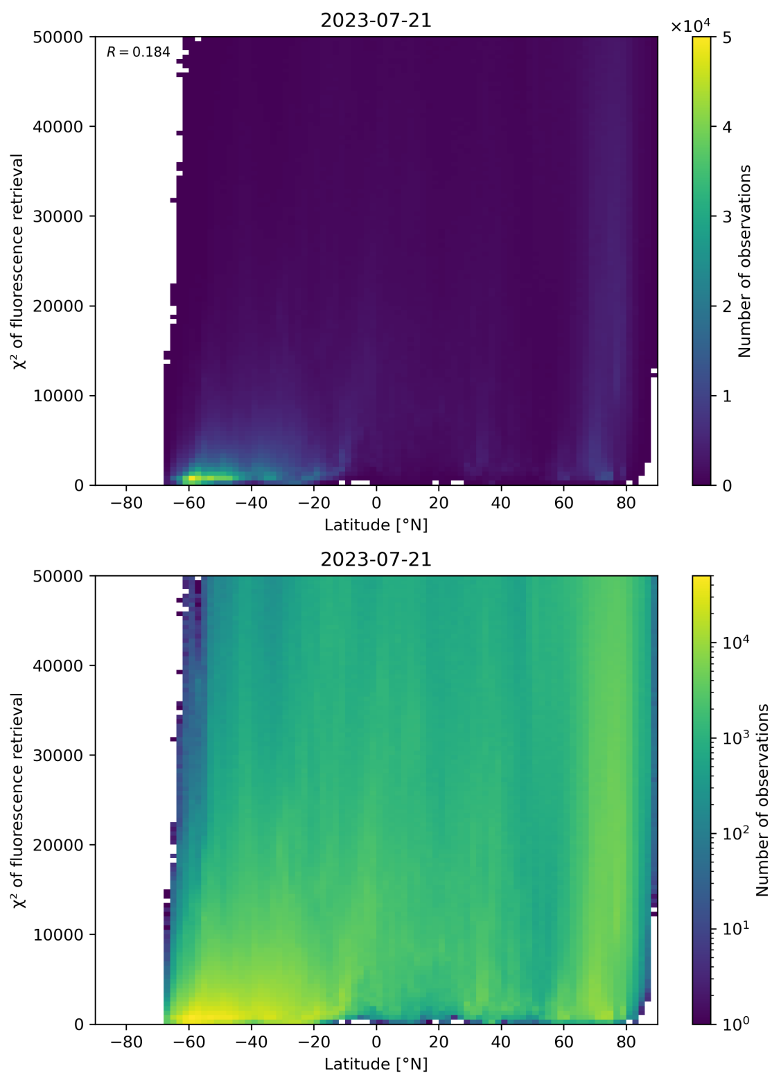
Figure 98: Scatter density plot of “Latitude” against “ \chi^2 of fluorescence retrieval” for 2023-07-20 to 2023-07-22.
