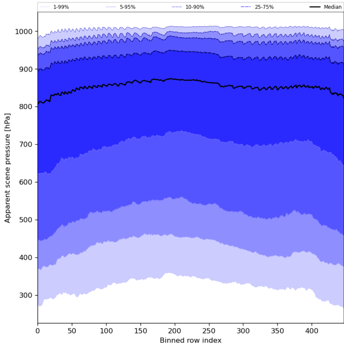
Figure 53: Along track statistics of “Apparent scene pressure” for 2023-07-20 to 2023-07-22
