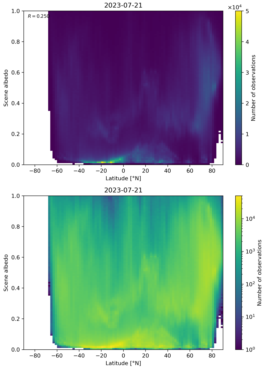
Figure 104: Scatter density plot of “Latitude” against “Scene albedo” for 2023-07-20 to 2023-07-22.
