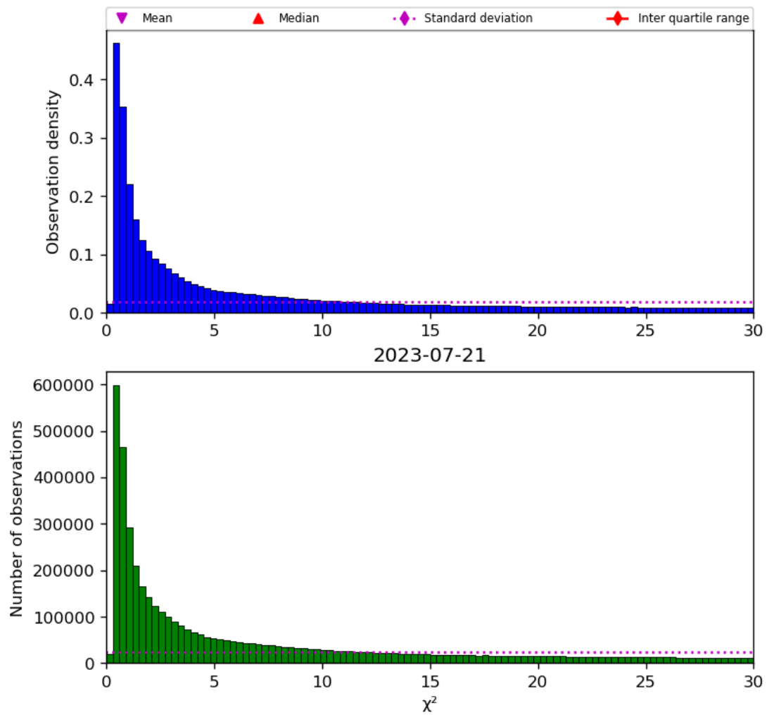
Figure 38: Histogram of “ \chi^2 ” for 2023-07-20 to 2023-07-22
