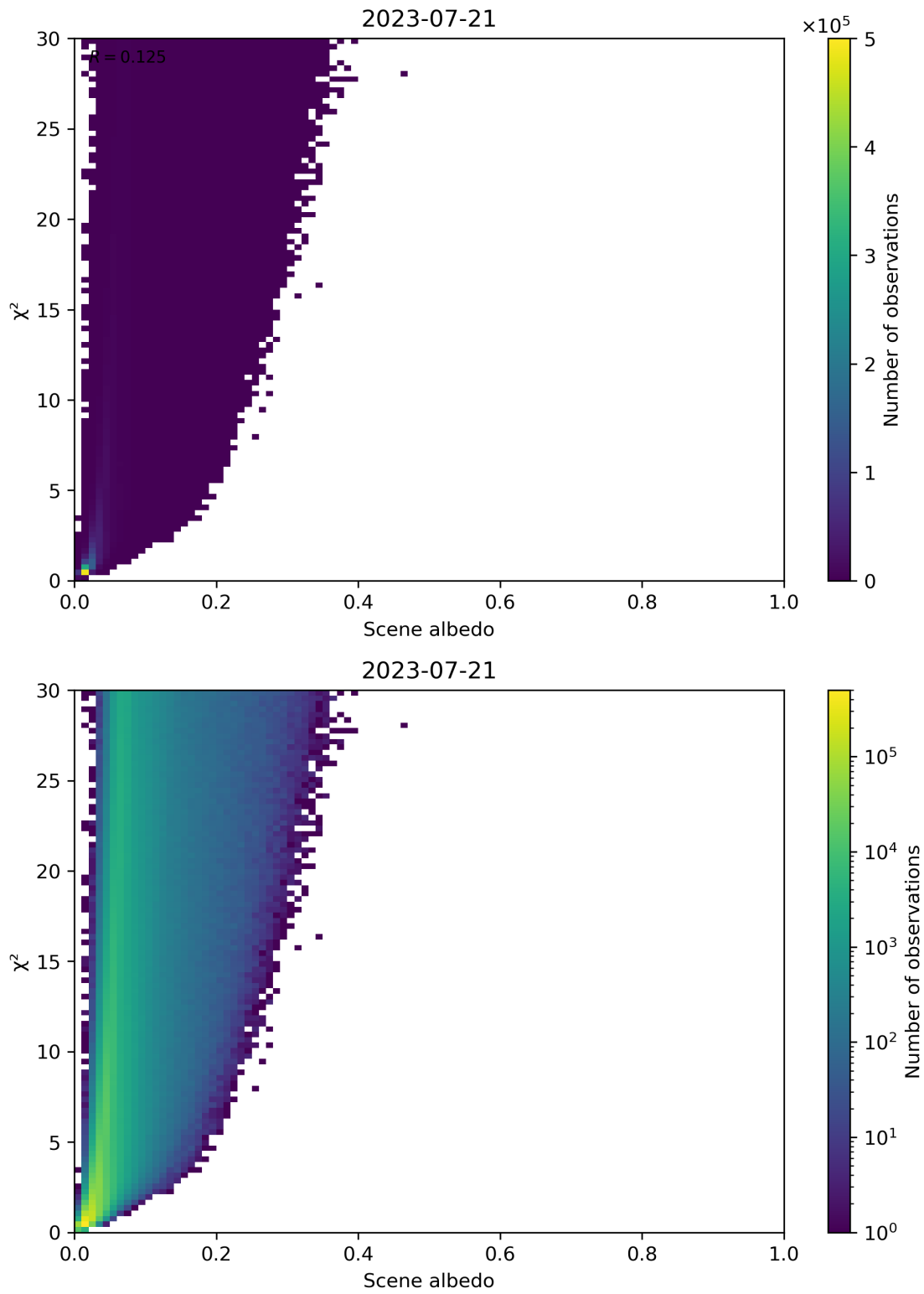
Figure 112: Scatter density plot of “Scene albedo” against “ \chi^2 ” for 2023-07-20 to 2023-07-22.
