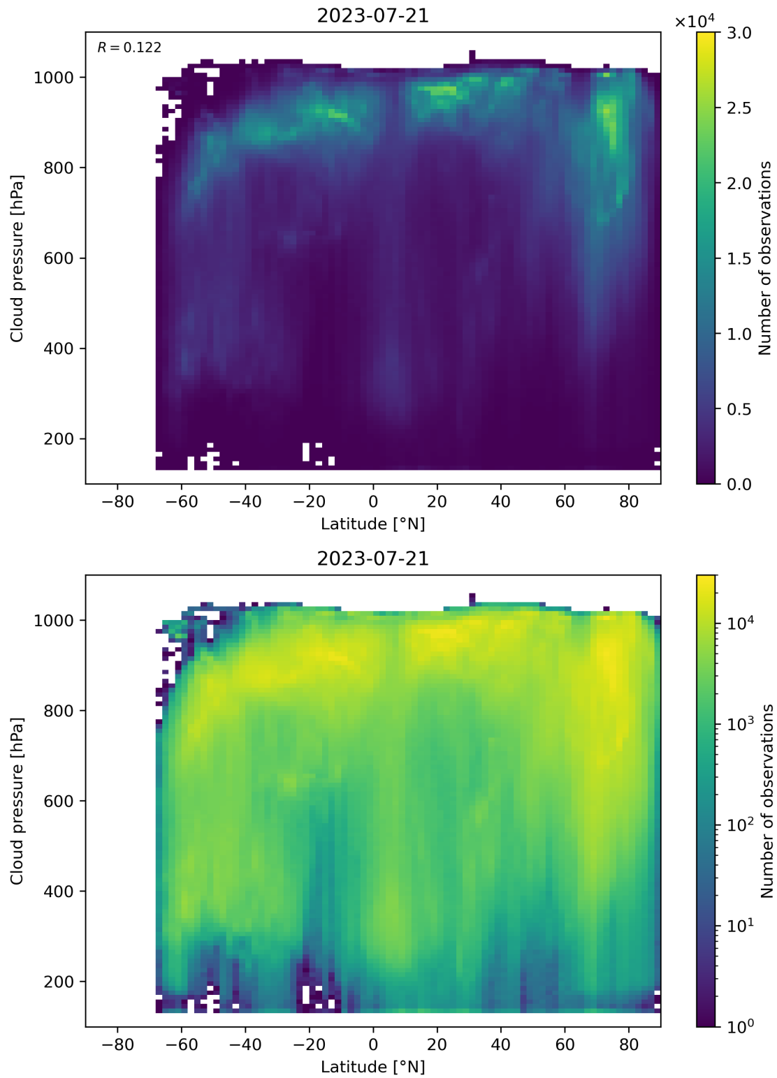
Figure 100: Scatter density plot of “Latitude” against “Cloud pressure” for 2023-07-20 to 2023-07-22.
