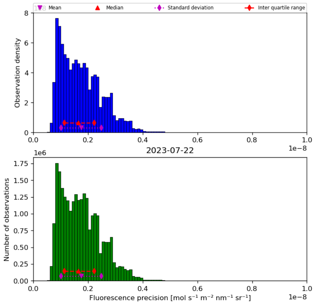
Figure 41: Histogram of “Fluorescence precision” for 2023-07-21 to 2023-07-23
