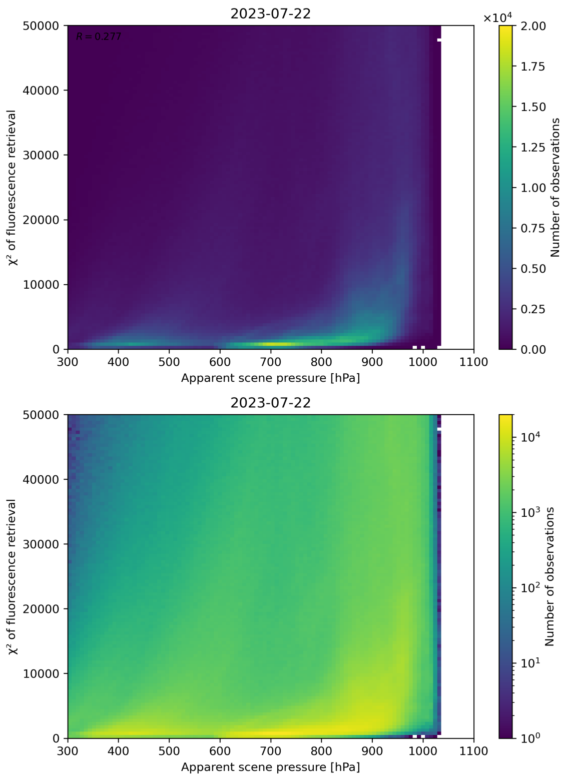
Figure 64: Scatter density plot of “Apparent scene pressure” against “ \chi^2 of fluorescence retrieval” for 2023-07-21 to 2023-07-23.
