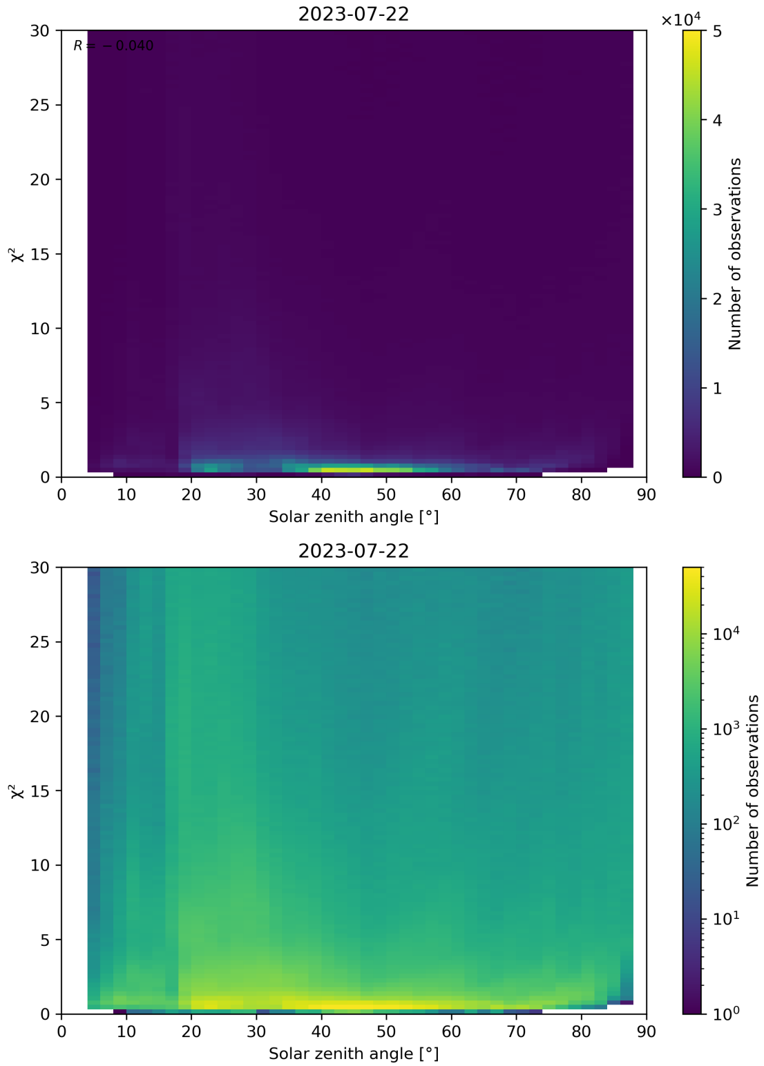
Figure 119: Scatter density plot of “Solar zenith angle” against “ \chi^2 ” for 2023-07-21 to 2023-07-23.
