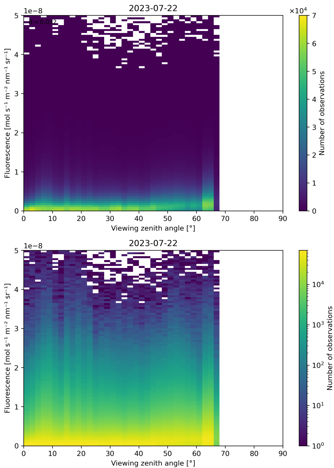
Figure 134: Scatter density plot of “Viewing zenith angle” against “Fluorescence” for 2023-07-21 to 2023-07-23.
