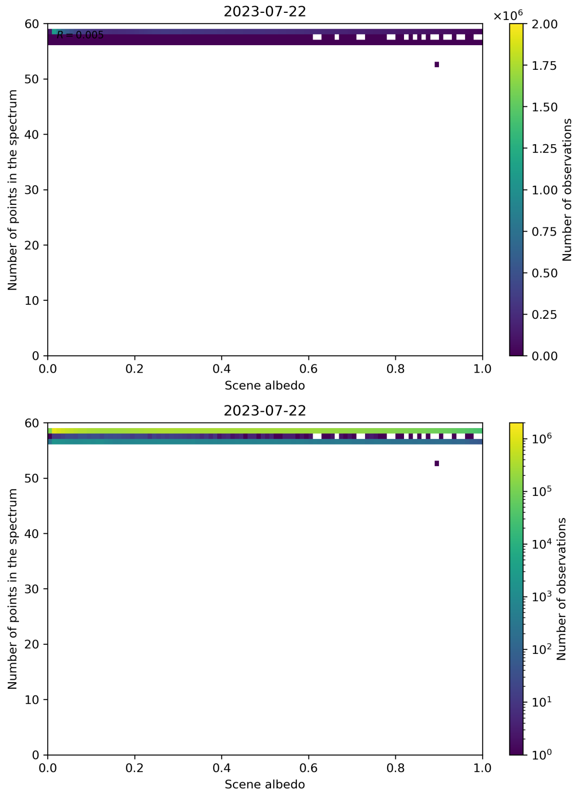
Figure 116: Scatter density plot of “Scene albedo” against “Number of points in the spectrum” for 2023-07-21 to 2023-07-23.
