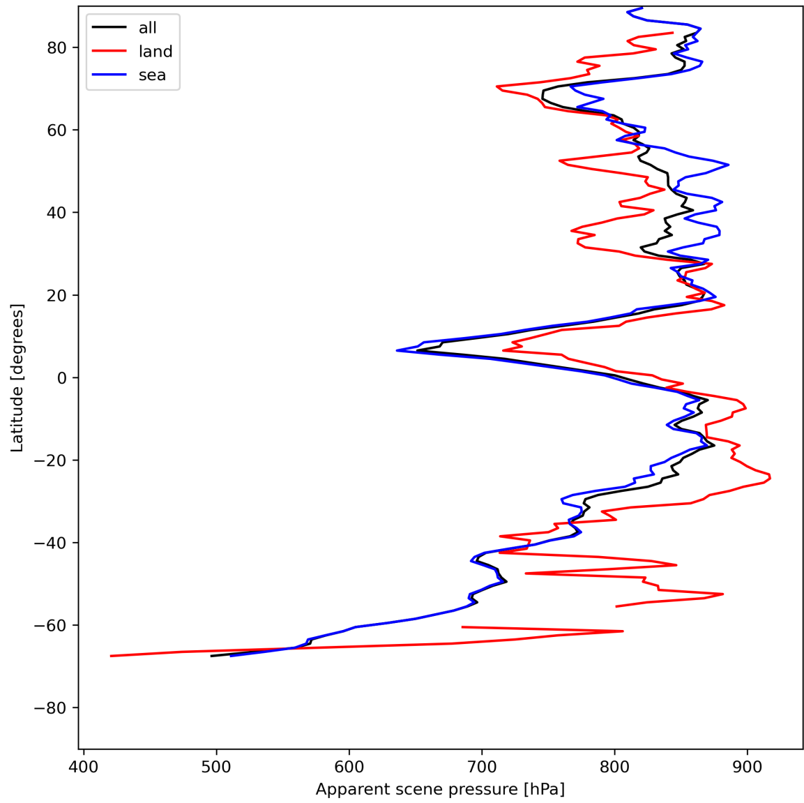
Figure 19: Zonal average of “Apparent scene pressure” for 2023-07-21 to 2023-07-23.
