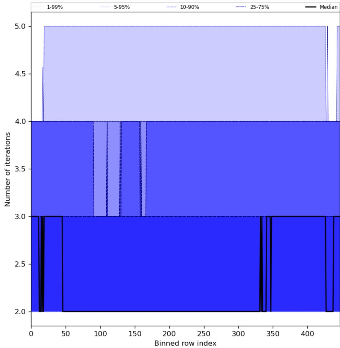
Figure 56: Along track statistics of “Number of iterations” for 2023-07-21 to 2023-07-23
