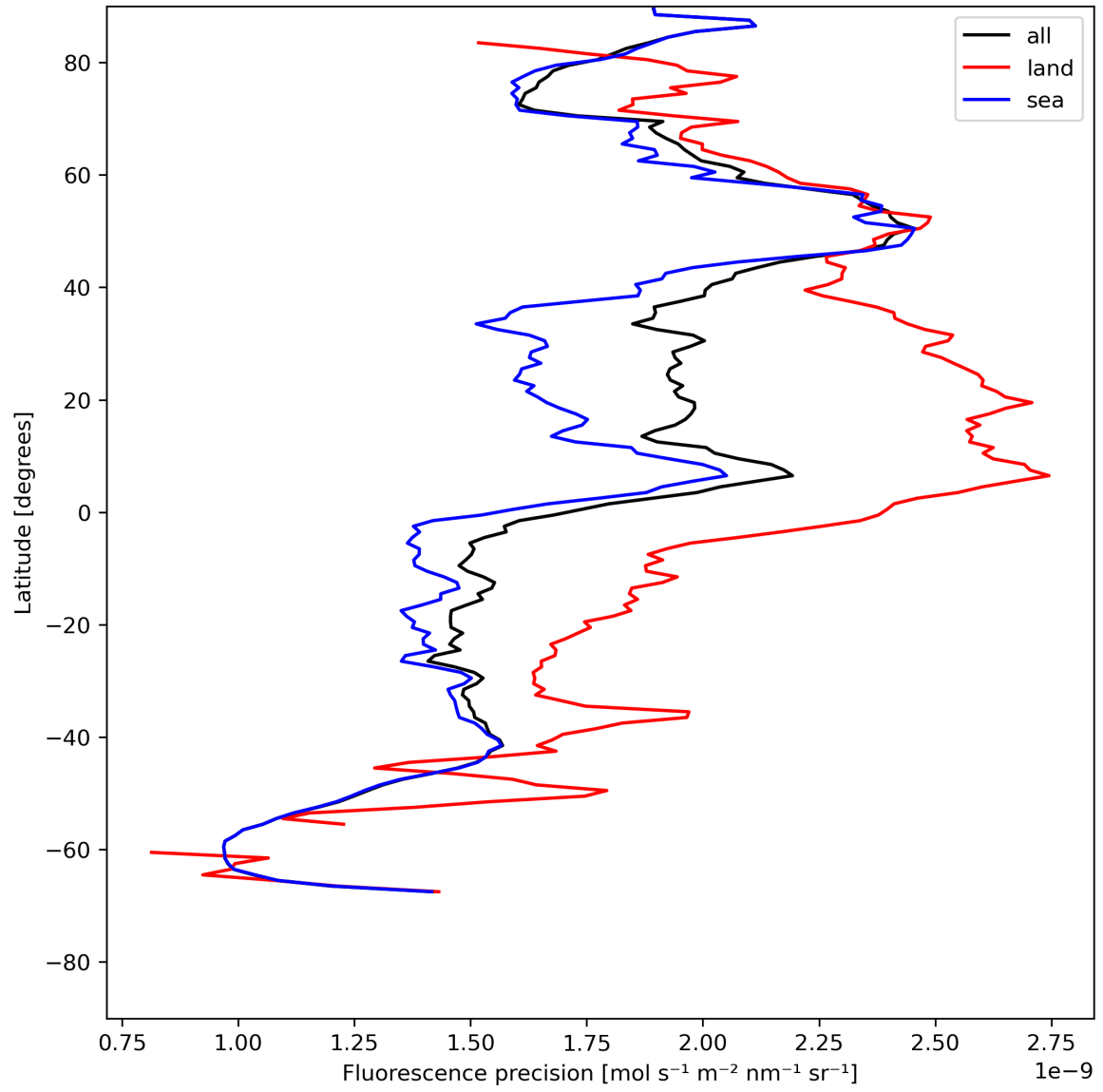
Figure 24: Zonal average of “Fluorescence precision” for 2023-07-21 to 2023-07-23.
