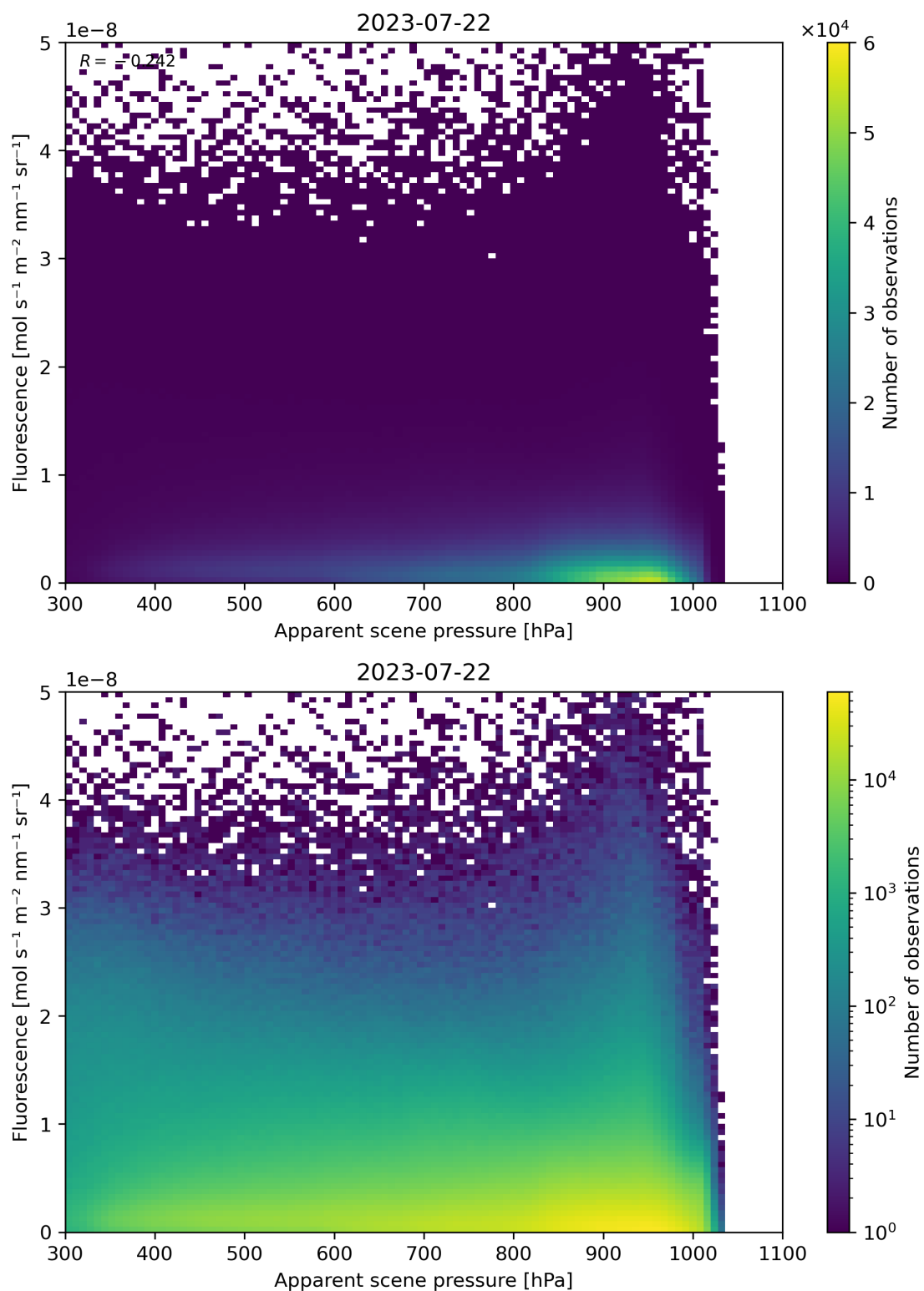
Figure 65: Scatter density plot of “Apparent scene pressure” against “Fluorescence” for 2023-07-21 to 2023-07-23.
