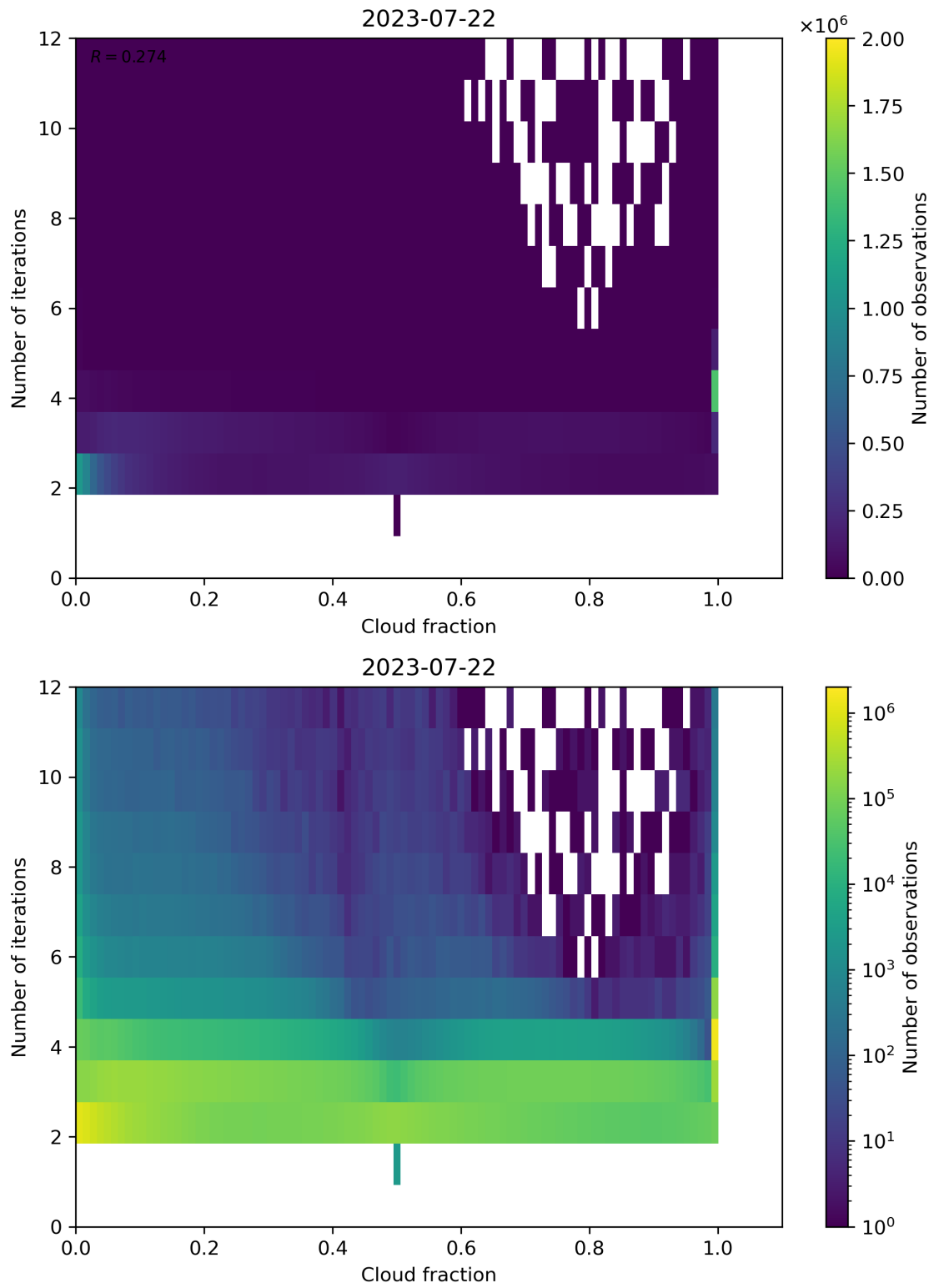
Figure 80: Scatter density plot of “Cloud fraction” against “Number of iterations” for 2023-07-21 to 2023-07-23.
