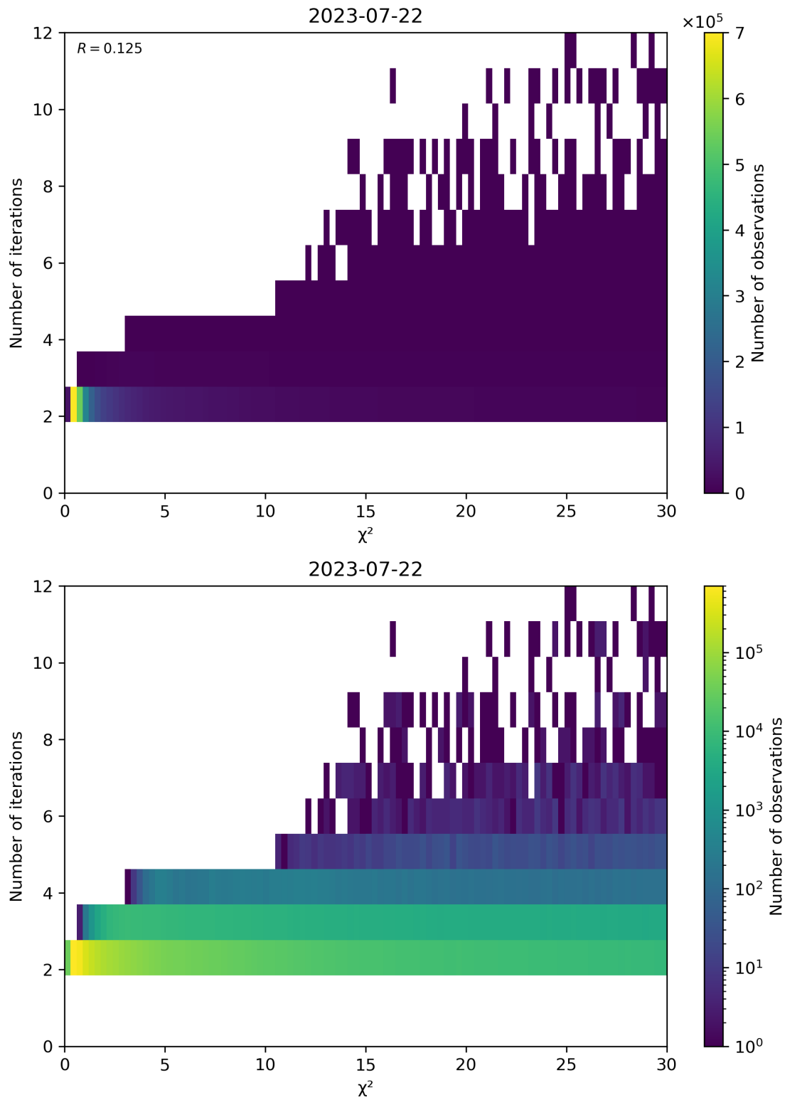
Figure 73: Scatter density plot of “ \chi^2 ” against “Number of iterations” for 2023-07-21 to 2023-07-23.
