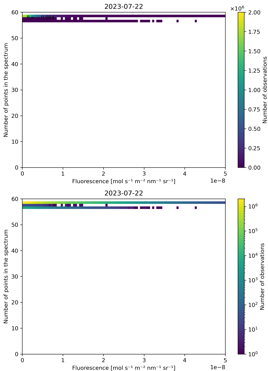
Figure 94: Scatter density plot of “Fluorescence” against “Number of points in the spectrum” for 2023-07-21 to 2023-07-23.
