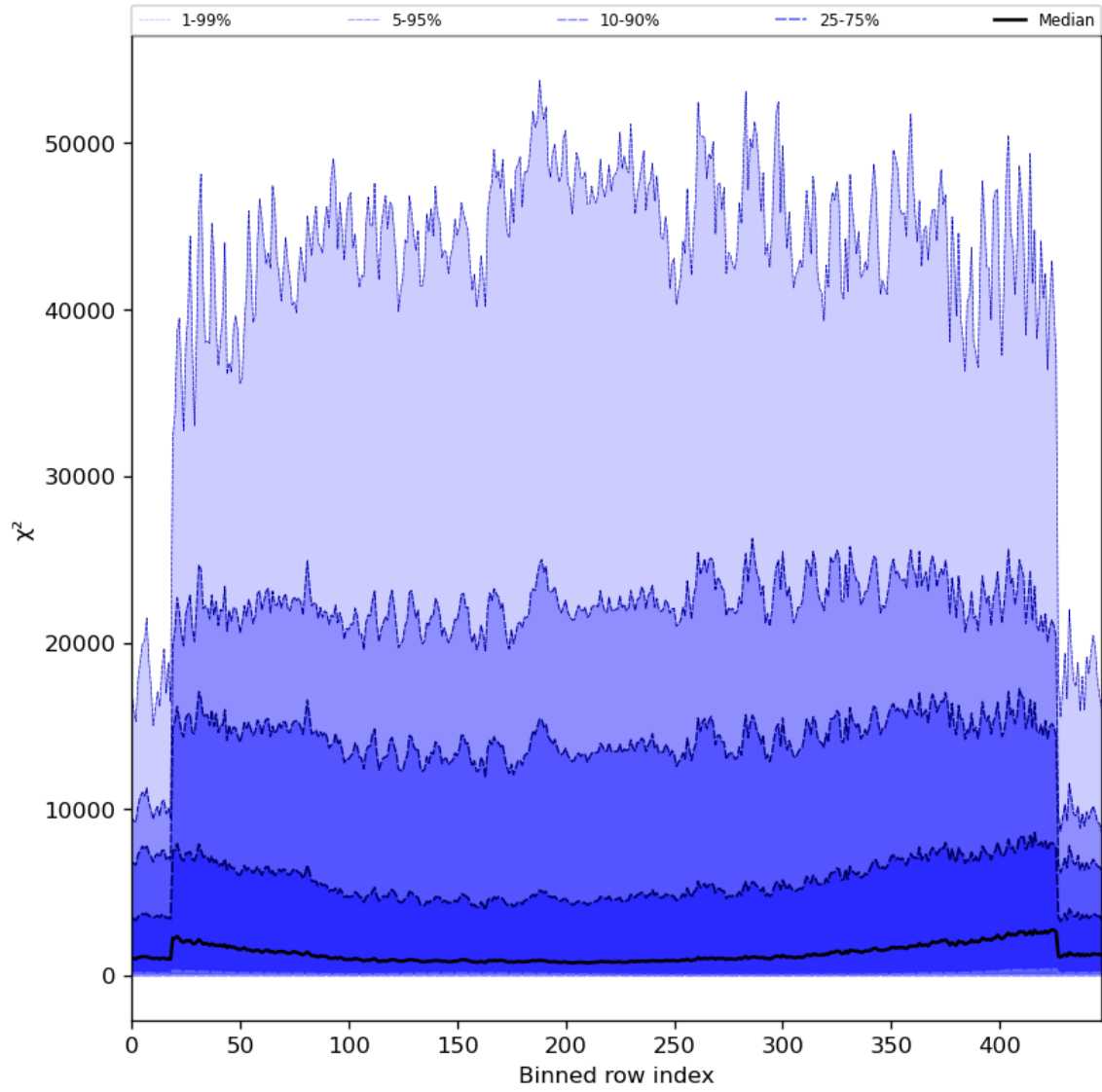
Figure 55: Along track statistics of “ \chi^2 ” for 2023-07-21 to 2023-07-23
