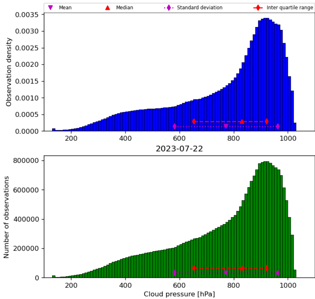
Figure 30: Histogram of “Cloud pressure” for 2023-07-21 to 2023-07-23
