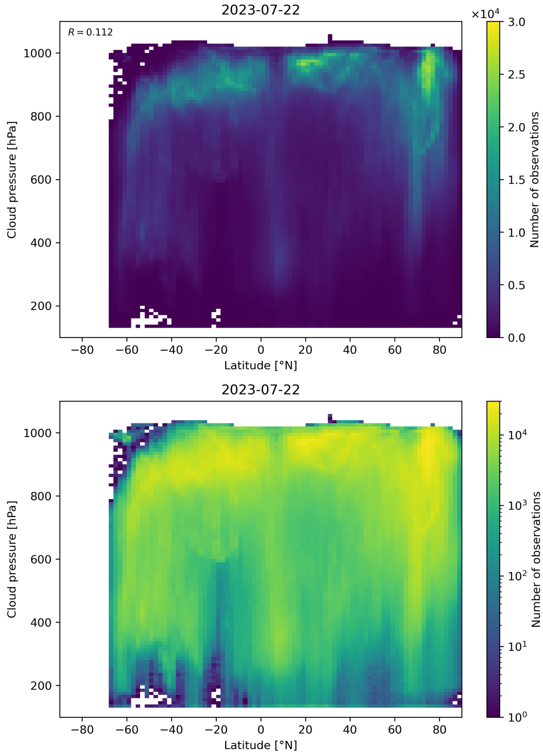
Figure 100: Scatter density plot of “Latitude” against “Cloud pressure” for 2023-07-21 to 2023-07-23.
