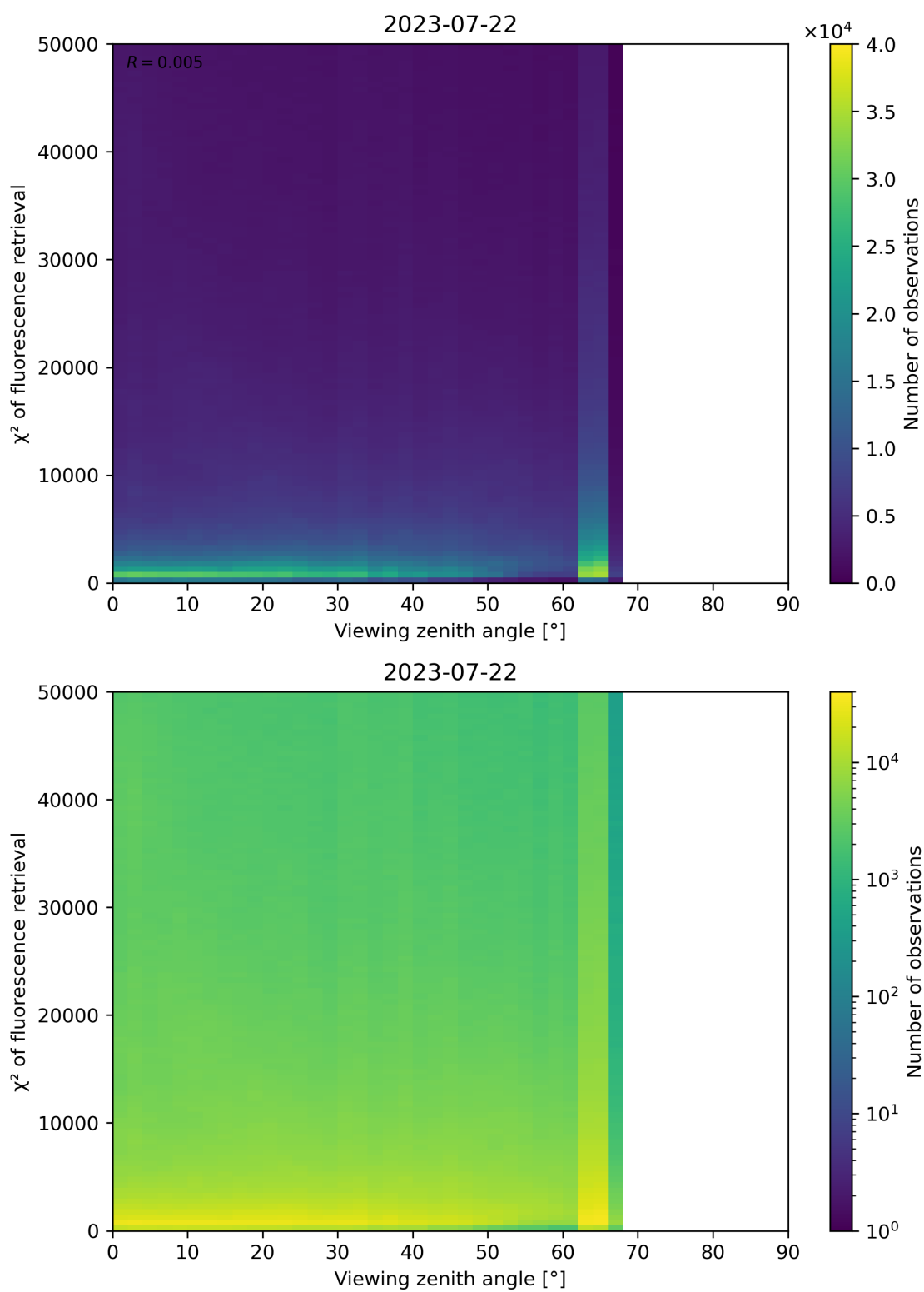
Figure 131: Scatter density plot of “Viewing zenith angle” against “ \chi^2 of fluorescence retrieval” for 2023-07-21 to 2023-07-23.
