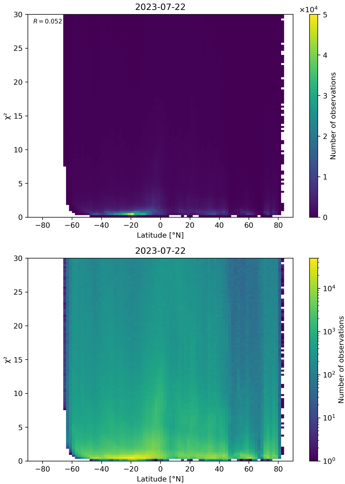
Figure 97: Scatter density plot of “Latitude” against “ \chi^2 ” for 2023-07-21 to 2023-07-23.
