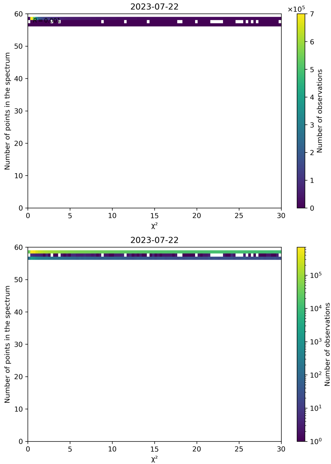
Figure 74: Scatter density plot of “ \chi^2 ” against “Number of points in the spectrum” for 2023-07-21 to 2023-07-23.
