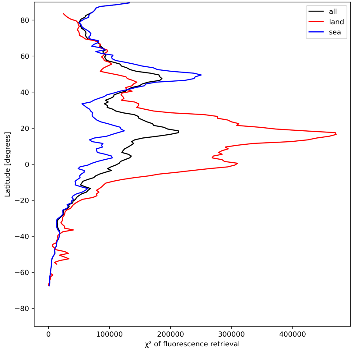
Figure 25: Zonal average of “ \chi^2 of fluorescence retrieval” for 2023-07-21 to 2023-07-23.
