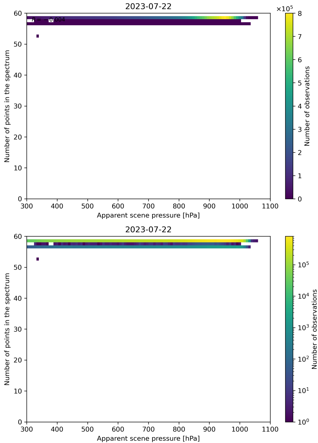
Figure 67: Scatter density plot of “Apparent scene pressure” against “Number of points in the spectrum” for 2023-07-21 to 2023-07-23.
