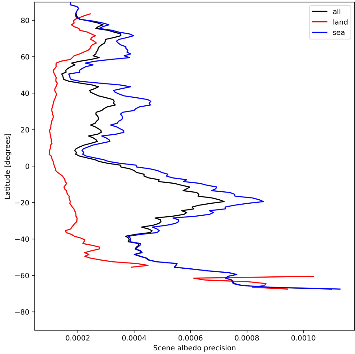
Figure 18: Zonal average of “Scene albedo precision” for 2023-07-21 to 2023-07-23.
