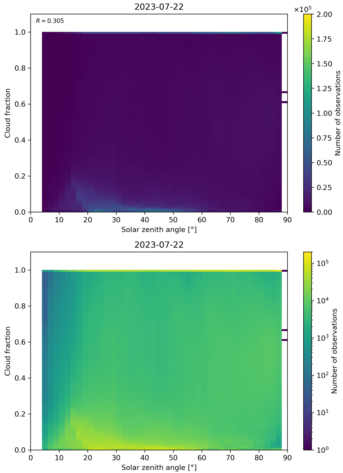
Figure 121: Scatter density plot of “Solar zenith angle” against “Cloud fraction” for 2023-07-21 to 2023-07-23.
