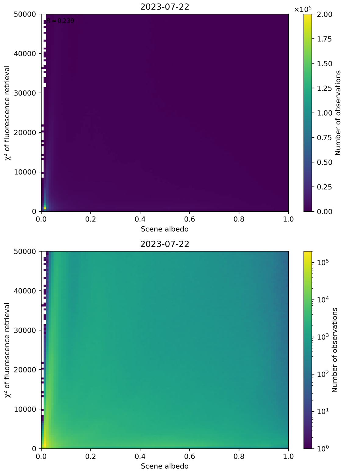
Figure 113: Scatter density plot of “Scene albedo” against “ \chi^2 of fluorescence retrieval” for 2023-07-21 to 2023-07-23.
