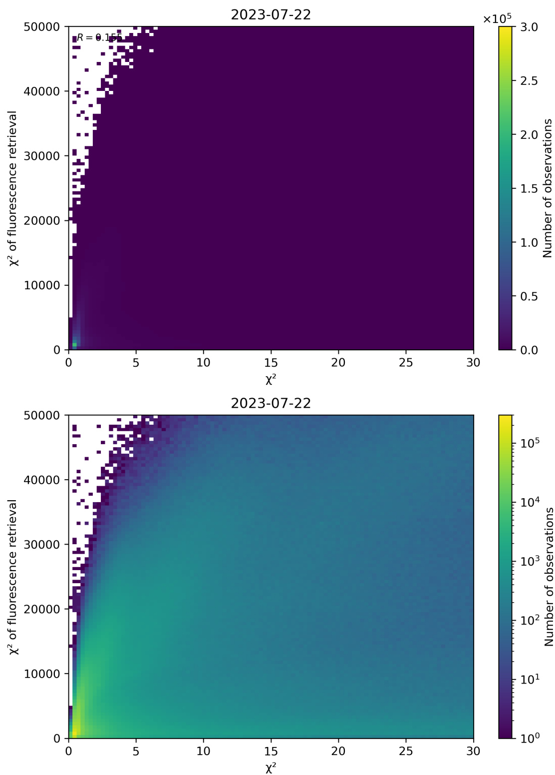
Figure 69: Scatter density plot of “ \chi^2 ” against “ \chi^2 of fluorescence retrieval” for 2023-07-21 to 2023-07-23.
