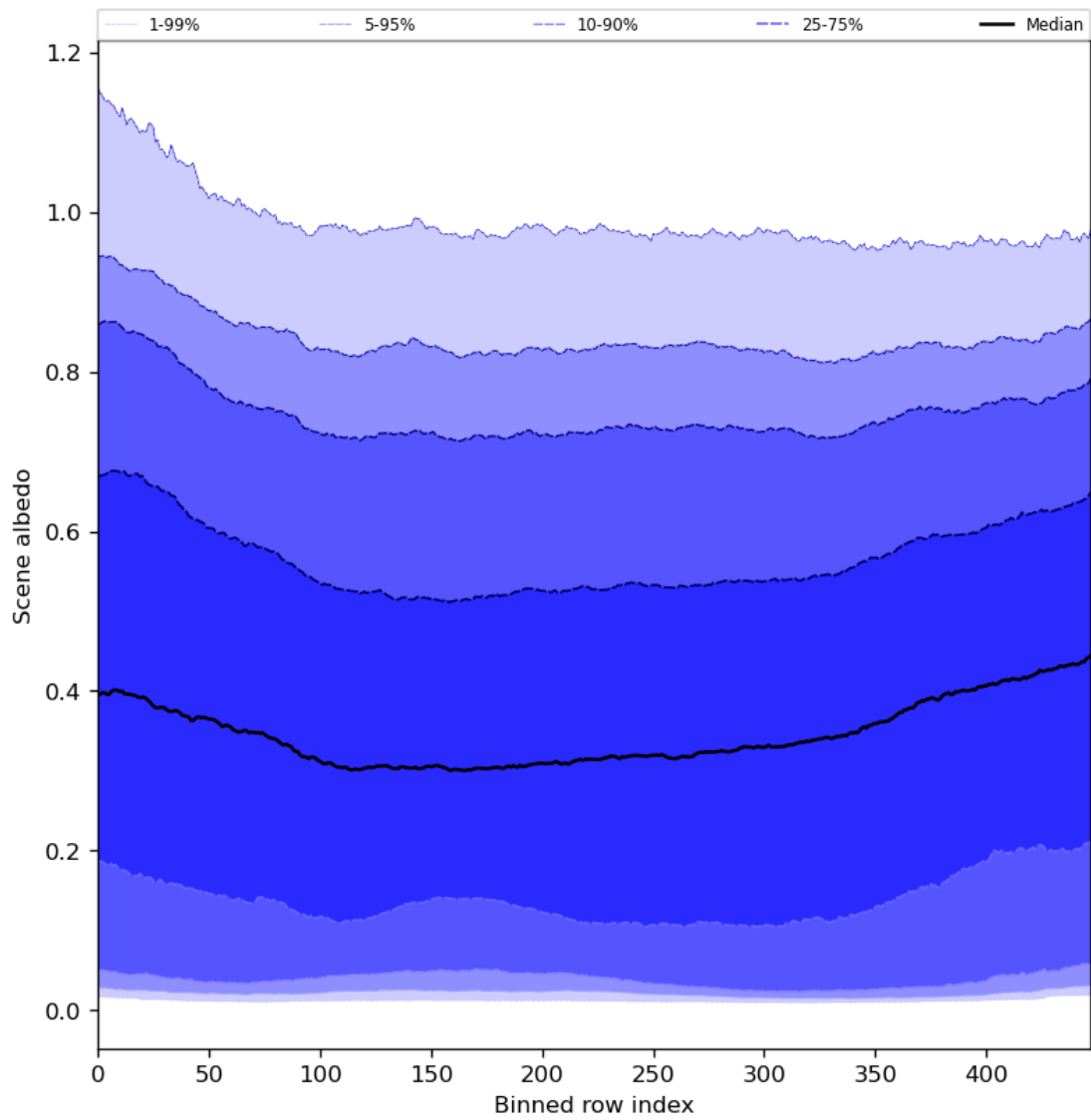
Figure 51: Along track statistics of “Scene albedo” for 2023-07-21 to 2023-07-23
