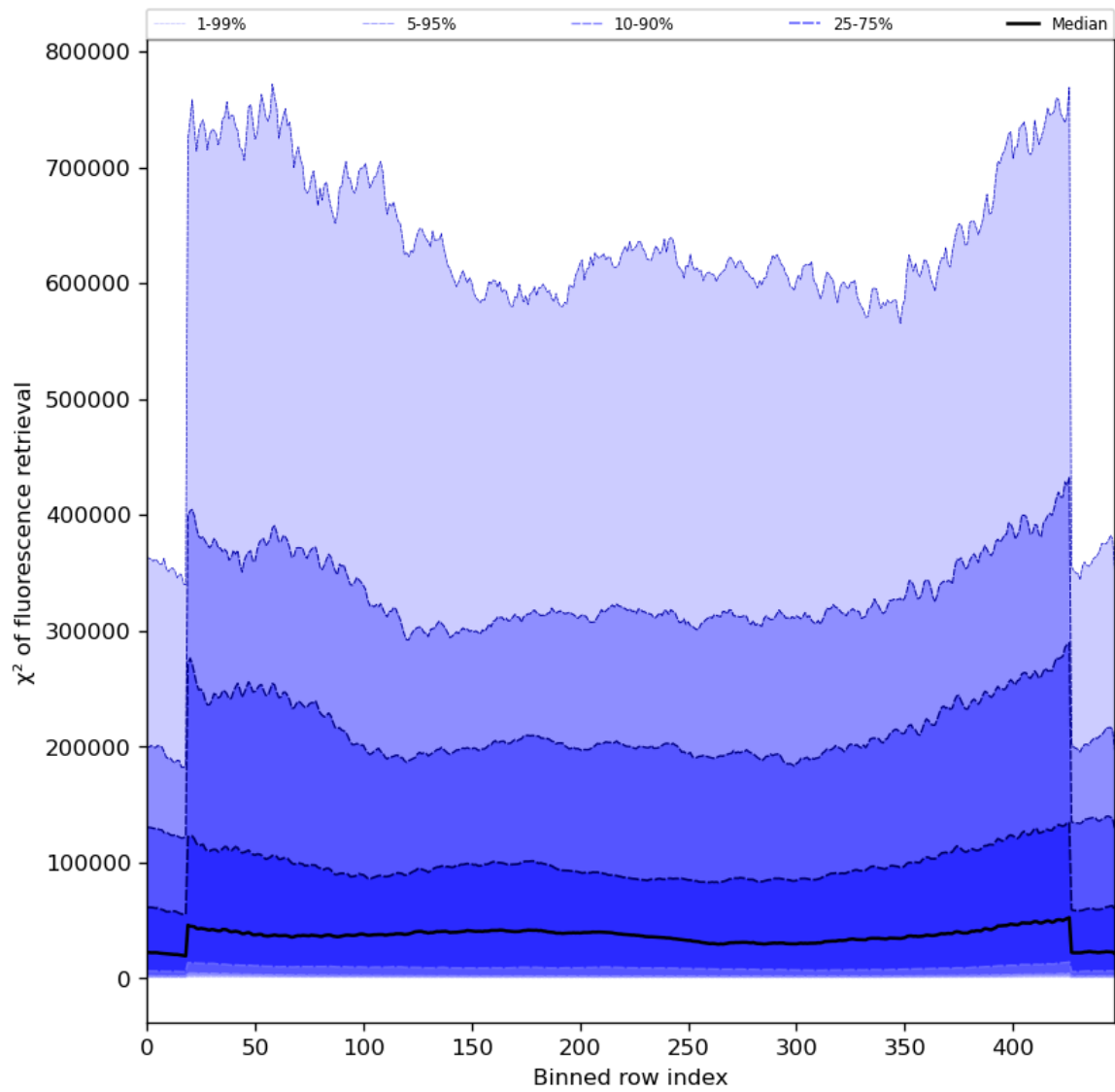
Figure 59: Along track statistics of “ \chi^2 of fluorescence retrieval” for 2023-07-21 to 2023-07-23
