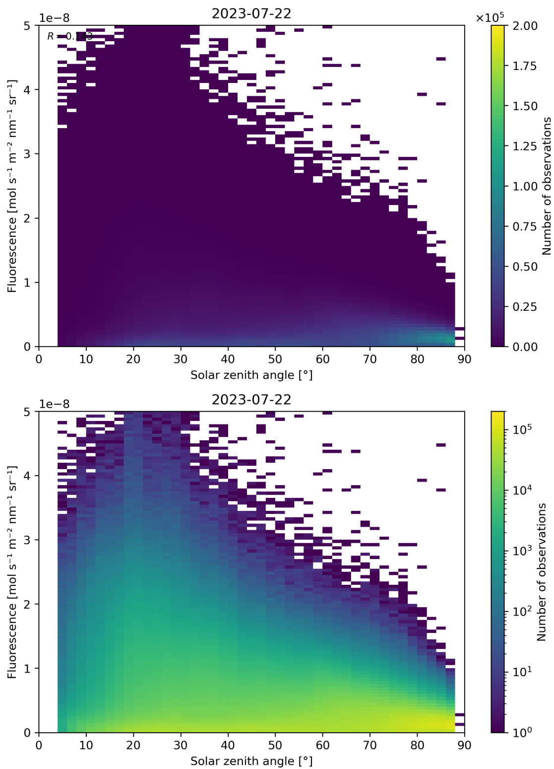
Figure 123: Scatter density plot of “Solar zenith angle” against “Fluorescence” for 2023-07-21 to 2023-07-23.
