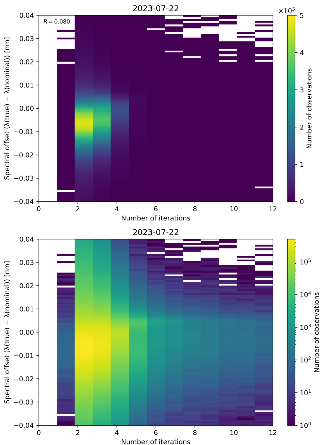
Figure 109: Scatter density plot of “Number of iterations” against “Spectral offset ( \lambda(\text{true}) - \lambda(\text{nominal}) )” for 2023-07-21 to 2023-07-23.
