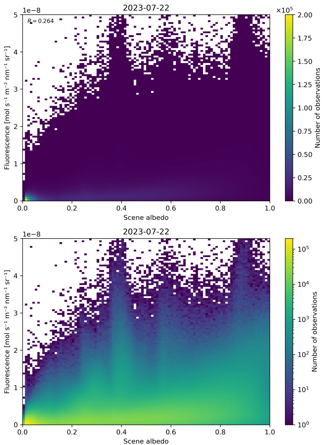
Figure 114: Scatter density plot of “Scene albedo” against “Fluorescence” for 2023-07-21 to 2023-07-23.
