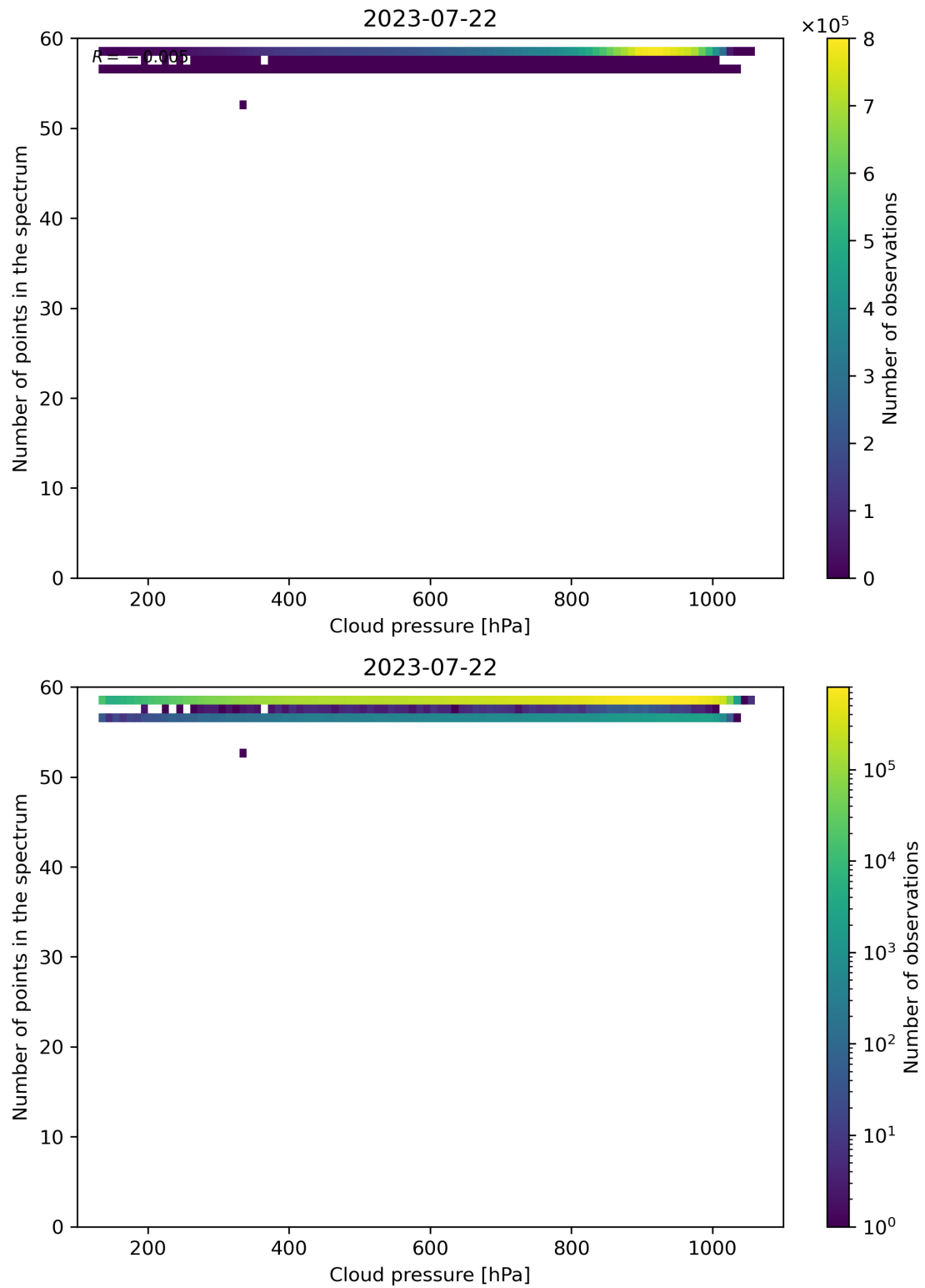
Figure 90: Scatter density plot of “Cloud pressure” against “Number of points in the spectrum” for 2023-07-21 to 2023-07-23.
