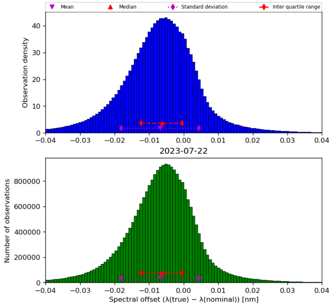
Figure 45: Histogram of “Spectral offset ( \lambda(\text{true}) - \lambda(\text{nominal}) )” for 2023-07-21 to 2023-07-23
