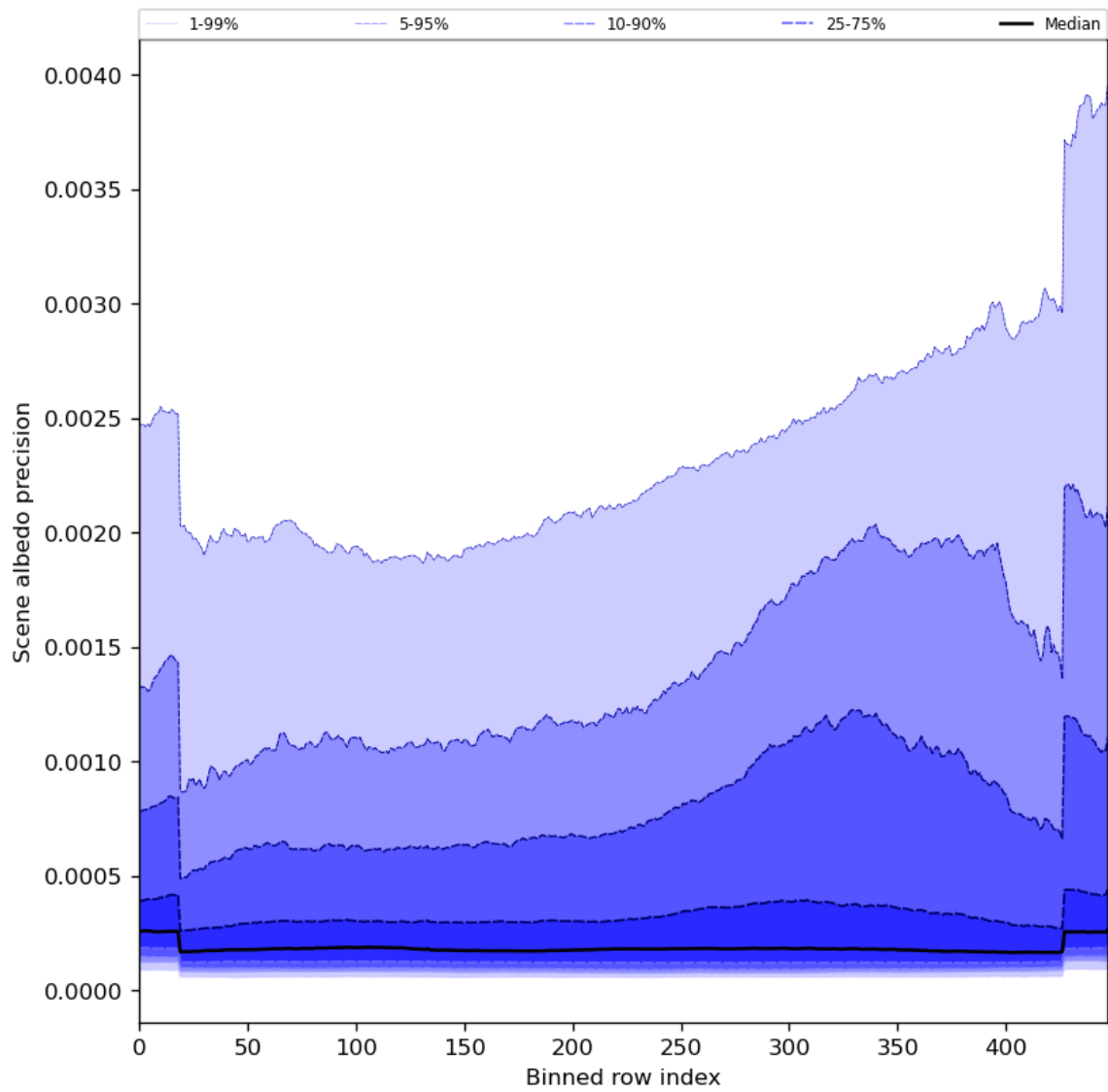
Figure 52: Along track statistics of “Scene albedo precision” for 2023-07-21 to 2023-07-23
