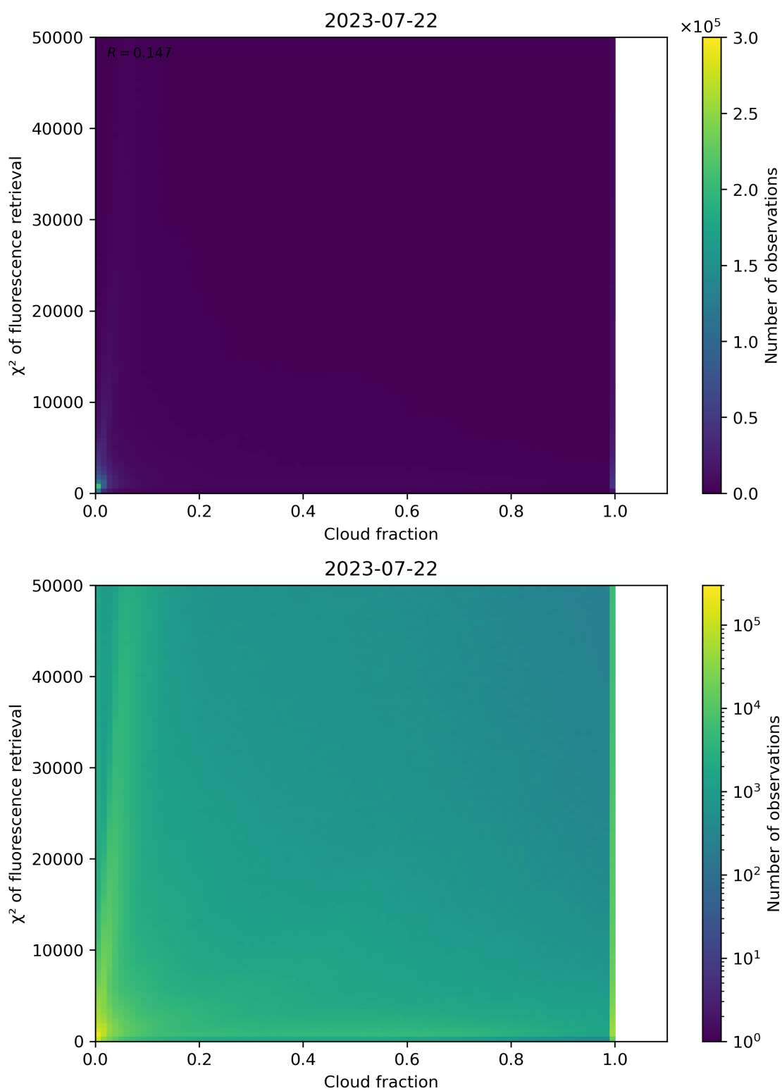
Figure 78: Scatter density plot of “Cloud fraction” against “ \chi^2 of fluorescence retrieval” for 2023-07-21 to 2023-07-23.
