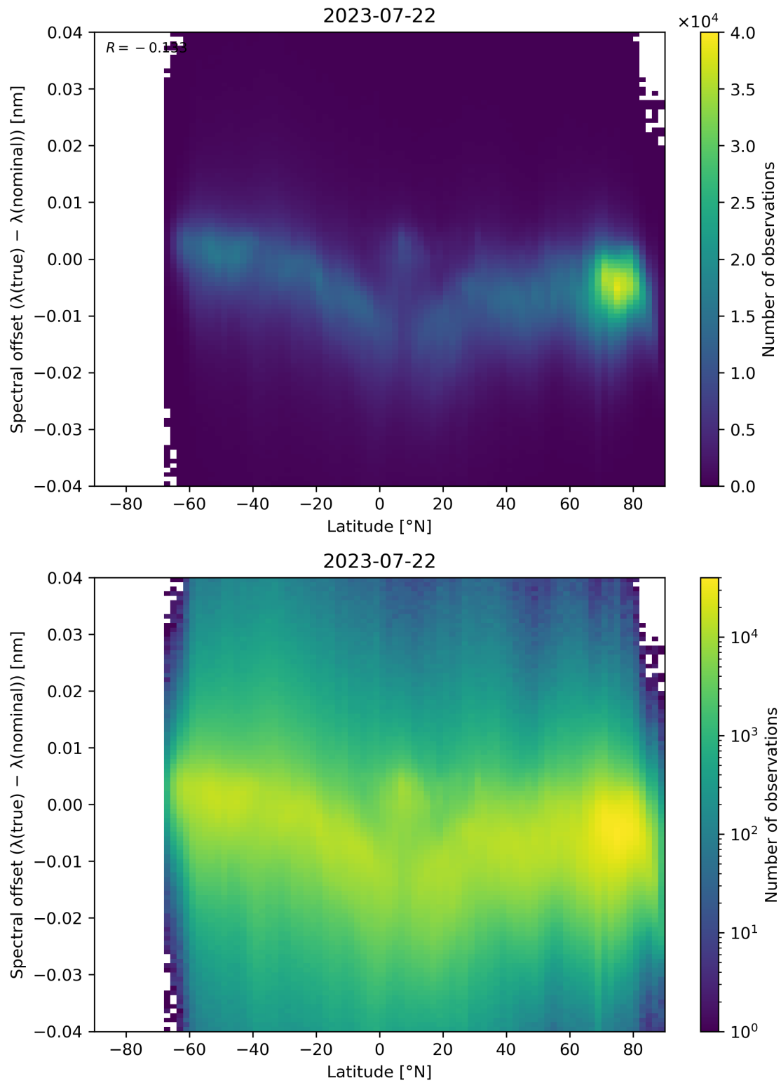
Figure 105: Scatter density plot of “Latitude” against “Spectral offset ( \lambda(\text{true}) - \lambda(\text{nominal}) )” for 2023-07-21 to 2023-07-23.
