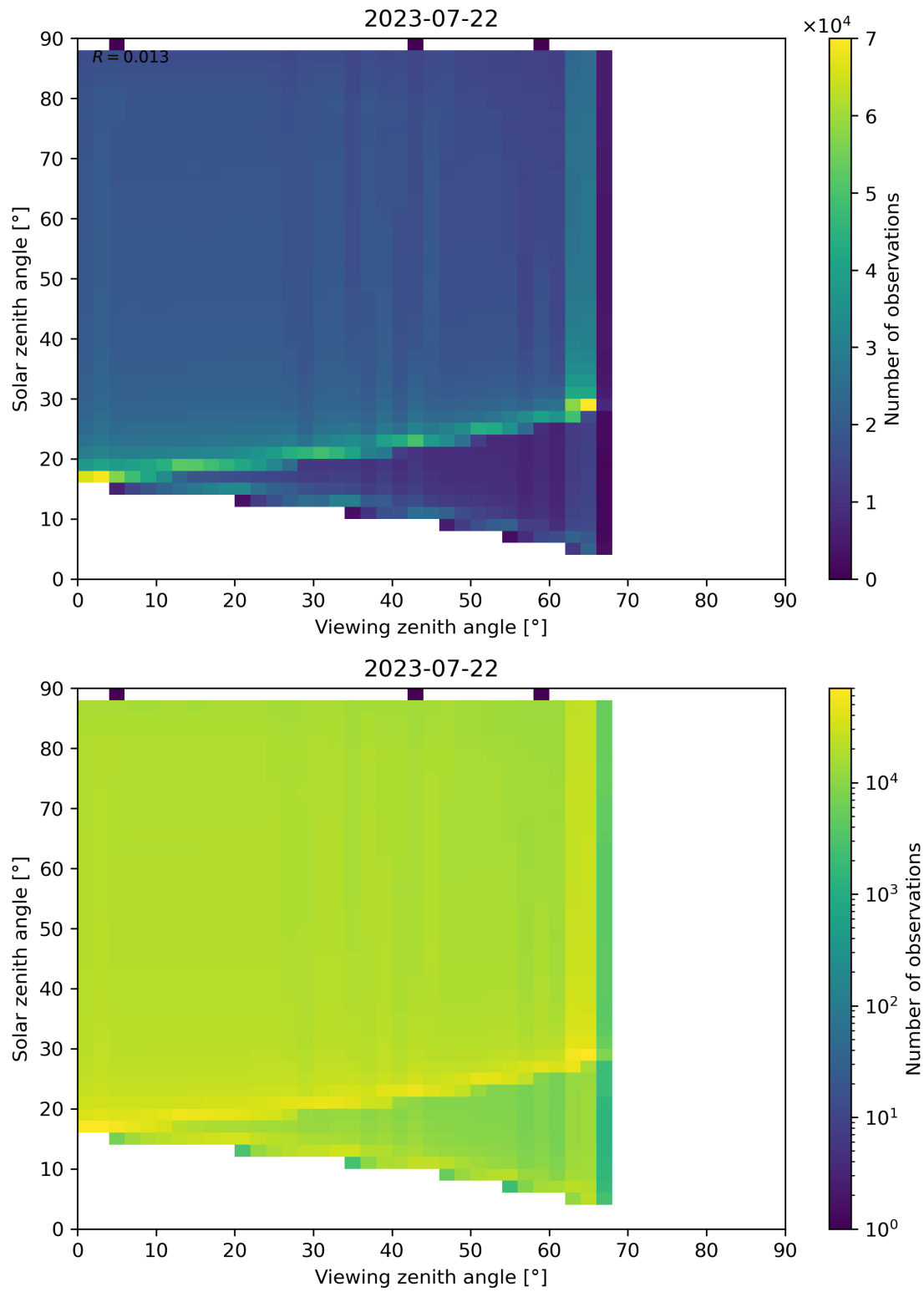
Figure 139: Scatter density plot of “Viewing zenith angle” against “Solar zenith angle” for 2023-07-21 to 2023-07-23.
