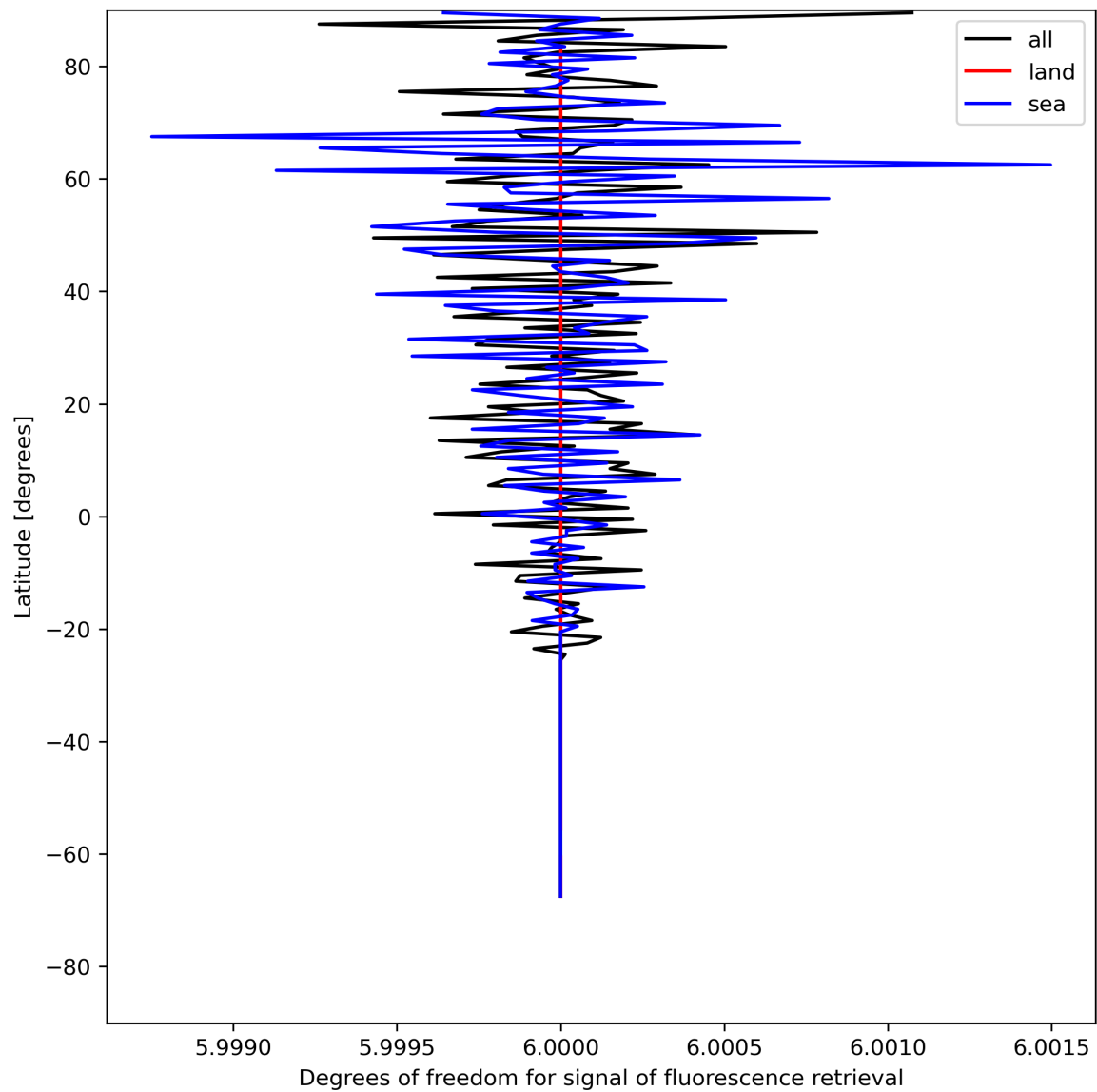
Figure 26: Zonal average of “Degrees of freedom for signal of fluorescence retrieval” for 2023-07-21 to 2023-07-23.
