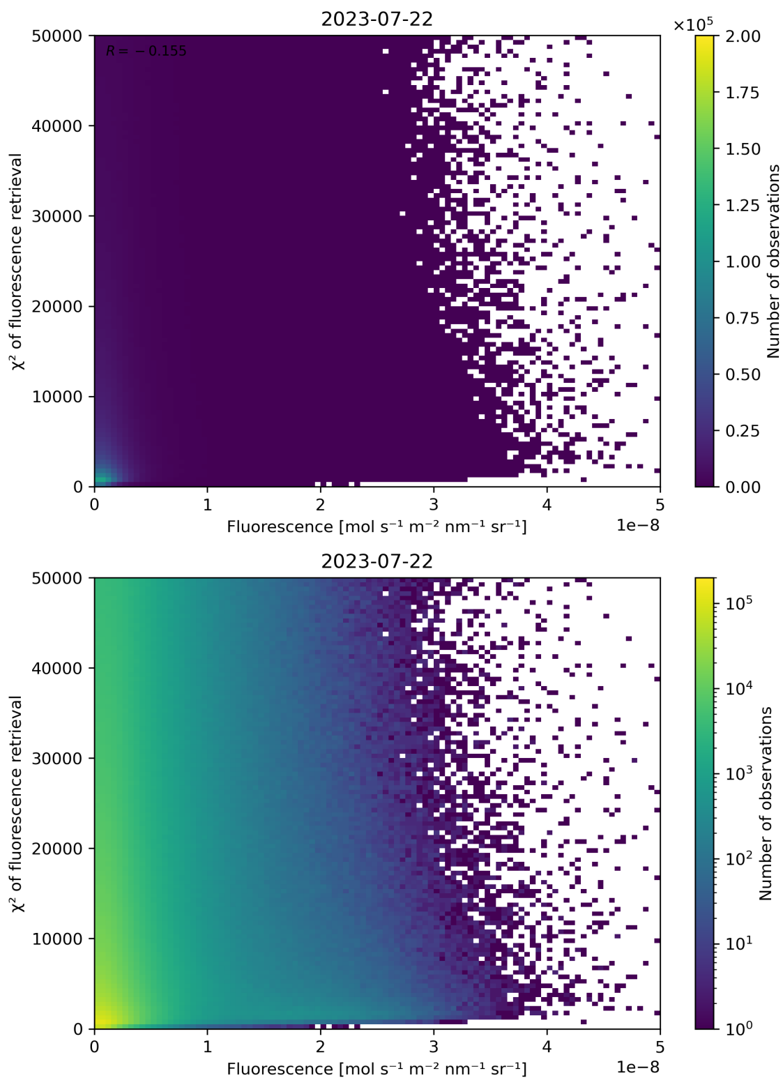
Figure 93: Scatter density plot of “Fluorescence” against “ \chi^2 of fluorescence retrieval” for 2023-07-21 to 2023-07-23.
