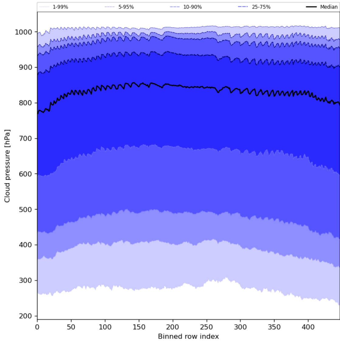
Figure 47: Along track statistics of “Cloud pressure” for 2023-07-21 to 2023-07-23
