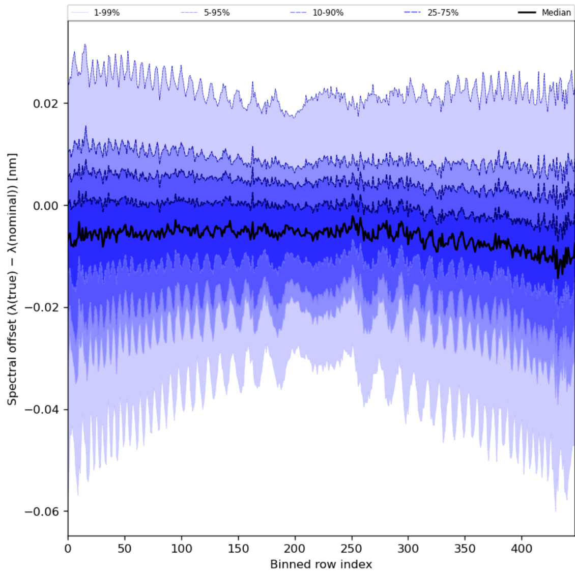
Figure 62: Along track statistics of “Spectral offset ( \lambda(\text{true}) - \lambda(\text{nominal}) )” for 2023-07-21 to 2023-07-23
