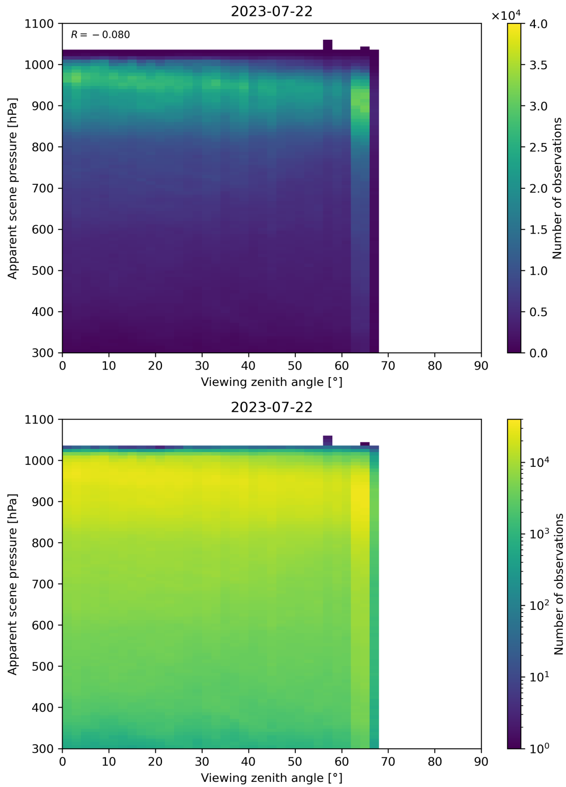
Figure 129: Scatter density plot of “Viewing zenith angle” against “Apparent scene pressure” for 2023-07-21 to 2023-07-23.
