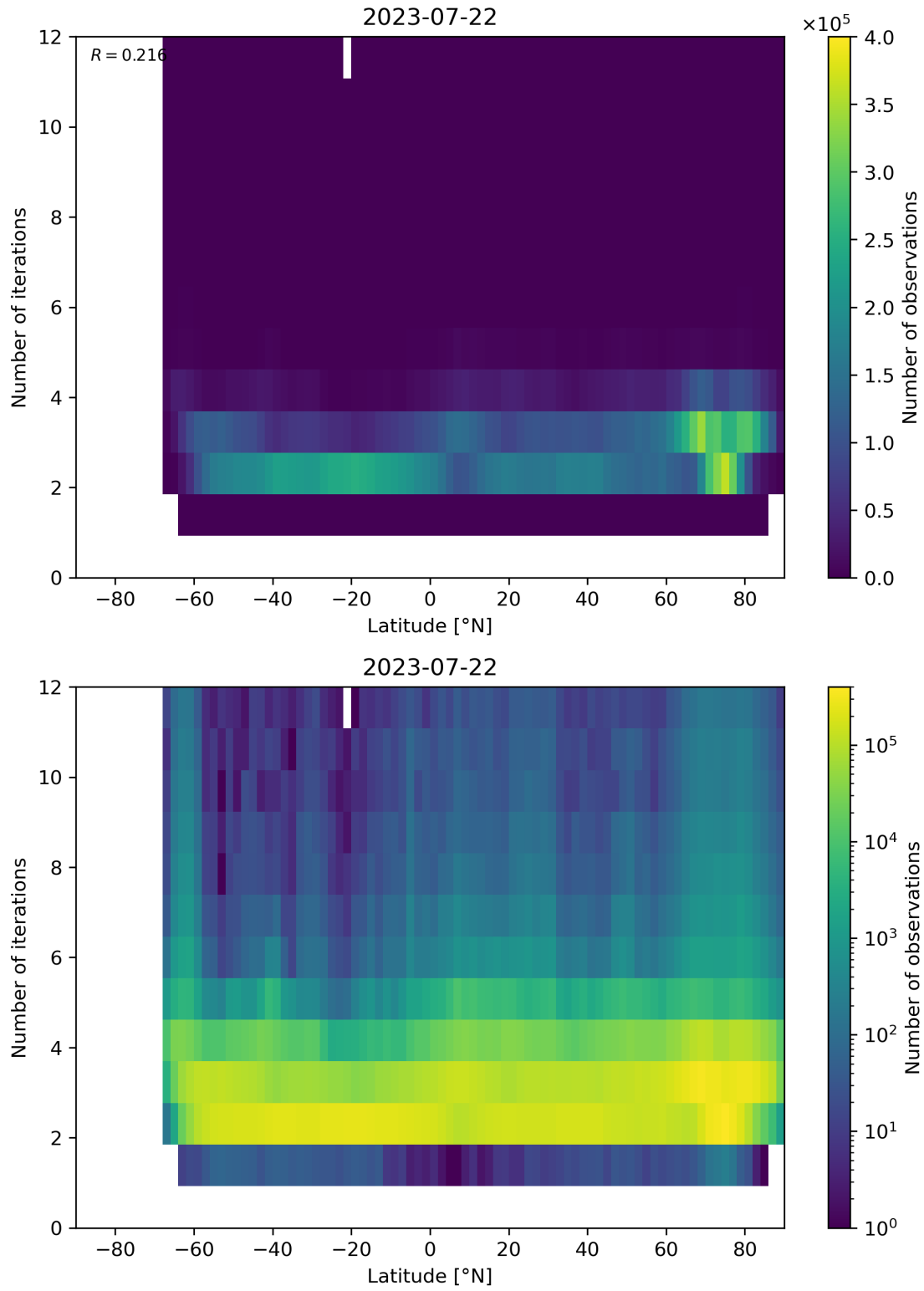
Figure 102: Scatter density plot of “Latitude” against “Number of iterations” for 2023-07-21 to 2023-07-23.
