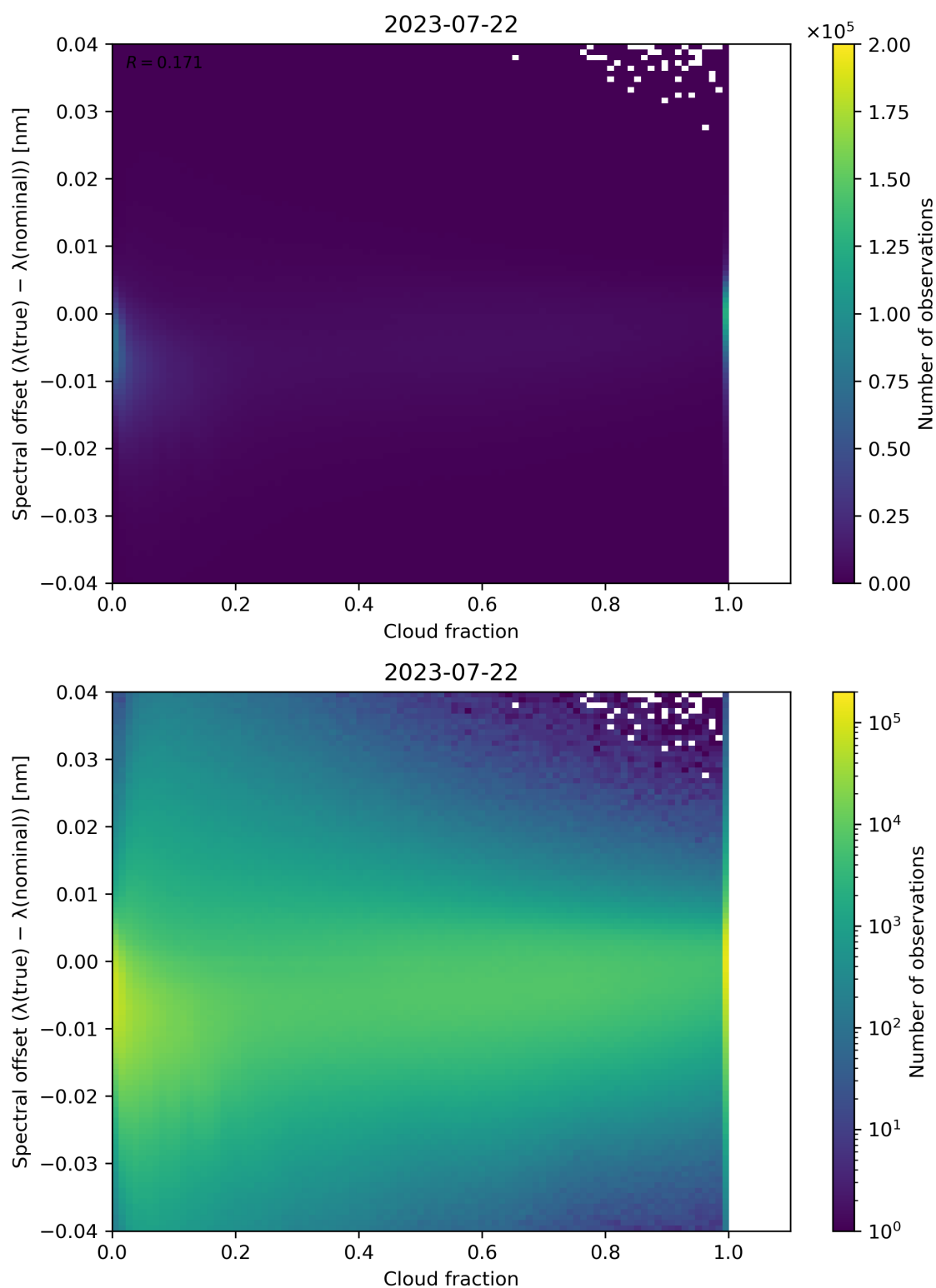
Figure 83: Scatter density plot of “Cloud fraction” against “Spectral offset ( \lambda(\text{true}) - \lambda(\text{nominal}) )” for 2023-07-21 to 2023-07-23.
