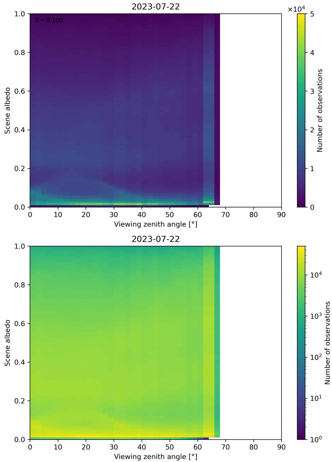
Figure 138: Scatter density plot of “Viewing zenith angle” against “Scene albedo” for 2023-07-21 to 2023-07-23.
