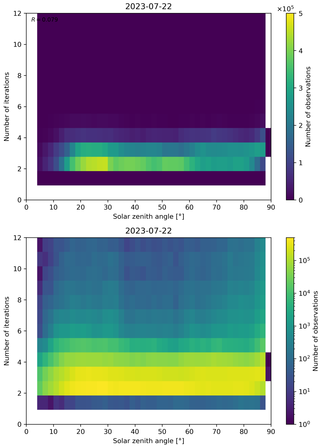
Figure 125: Scatter density plot of “Solar zenith angle” against “Number of iterations” for 2023-07-21 to 2023-07-23.
