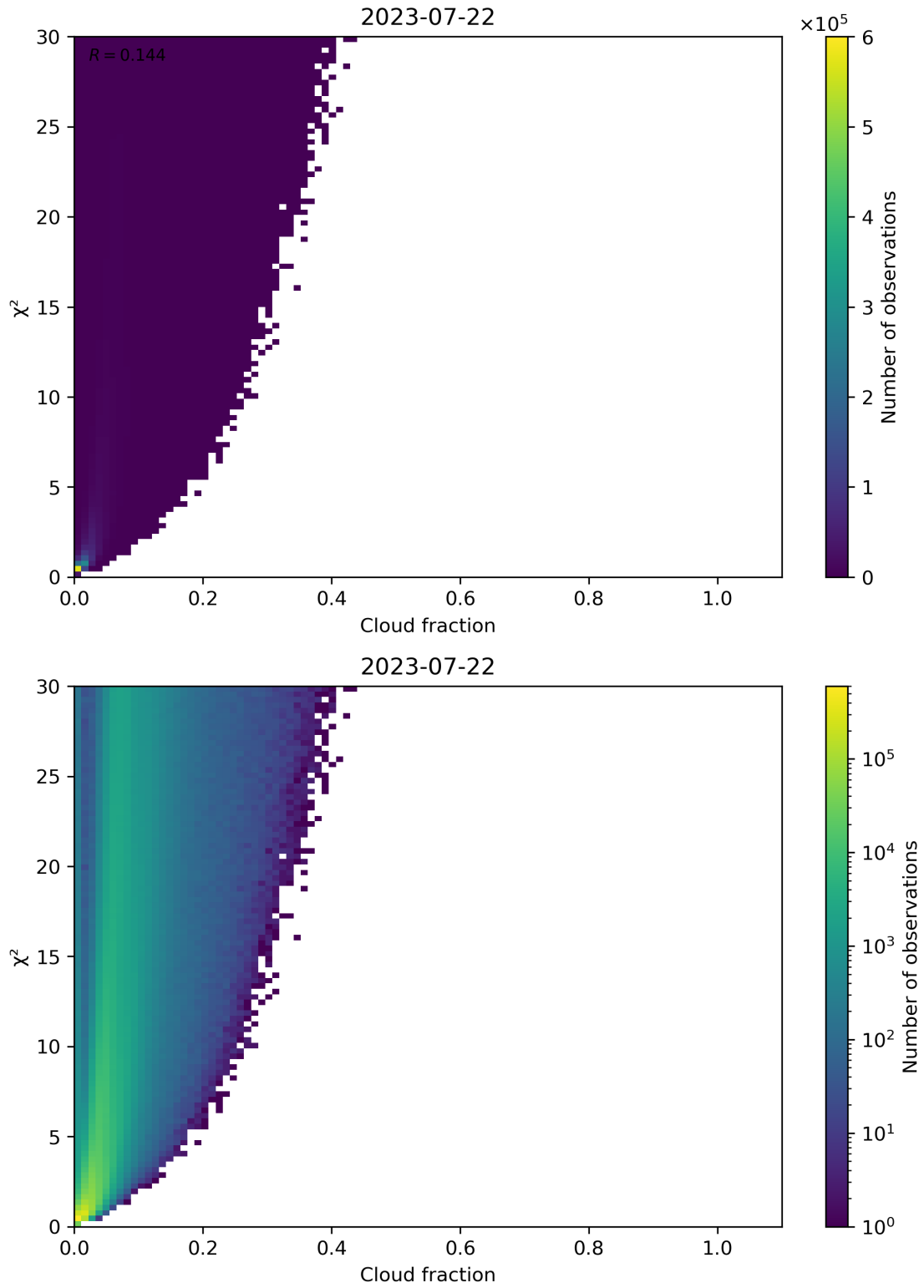
Figure 77: Scatter density plot of “Cloud fraction” against “ \chi^2 ” for 2023-07-21 to 2023-07-23.
