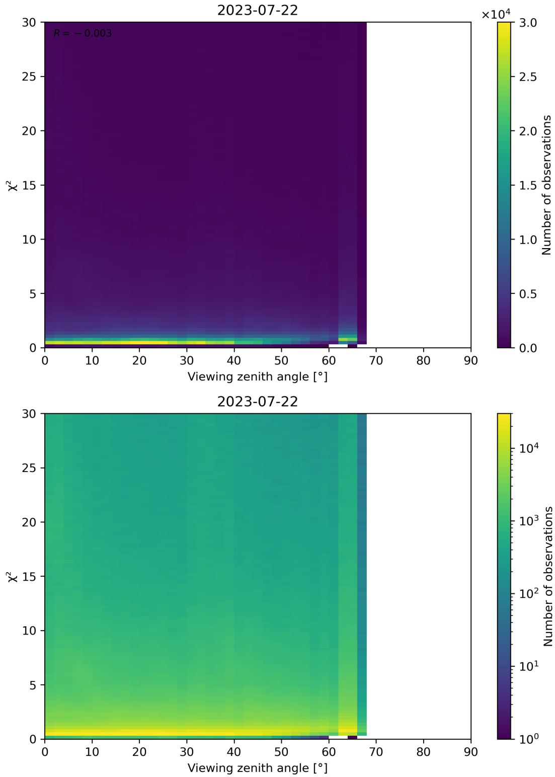
Figure 130: Scatter density plot of “Viewing zenith angle” against “ \chi^2 ” for 2023-07-21 to 2023-07-23.
