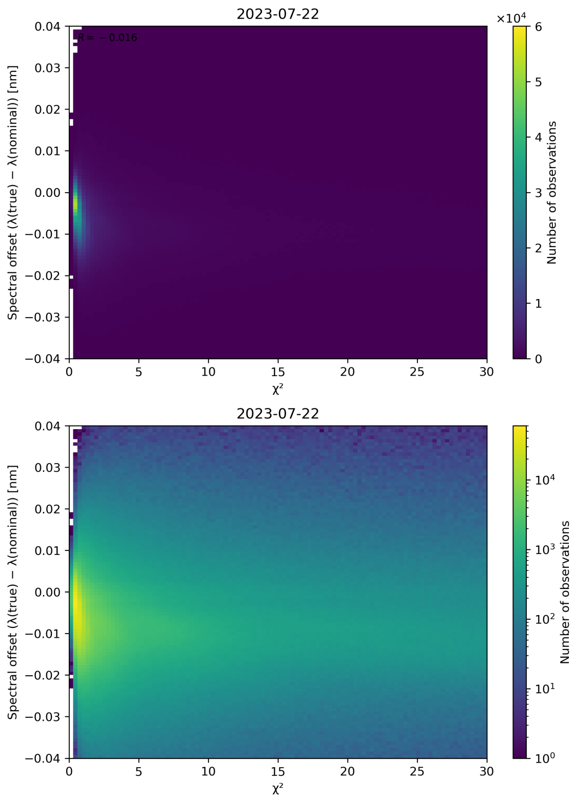
Figure 75: Scatter density plot of " \chi^2 " against "Spectral offset ( \lambda(\text{true}) - \lambda(\text{nominal}) )" for 2023-07-21 to 2023-07-23.
