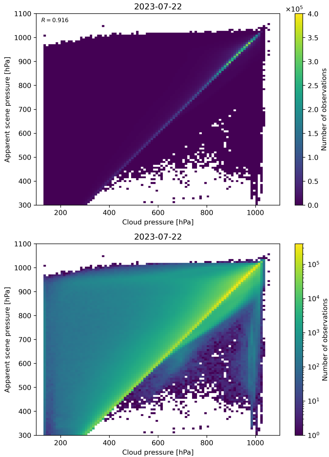
Figure 84: Scatter density plot of “Cloud pressure” against “Apparent scene pressure” for 2023-07-21 to 2023-07-23.
