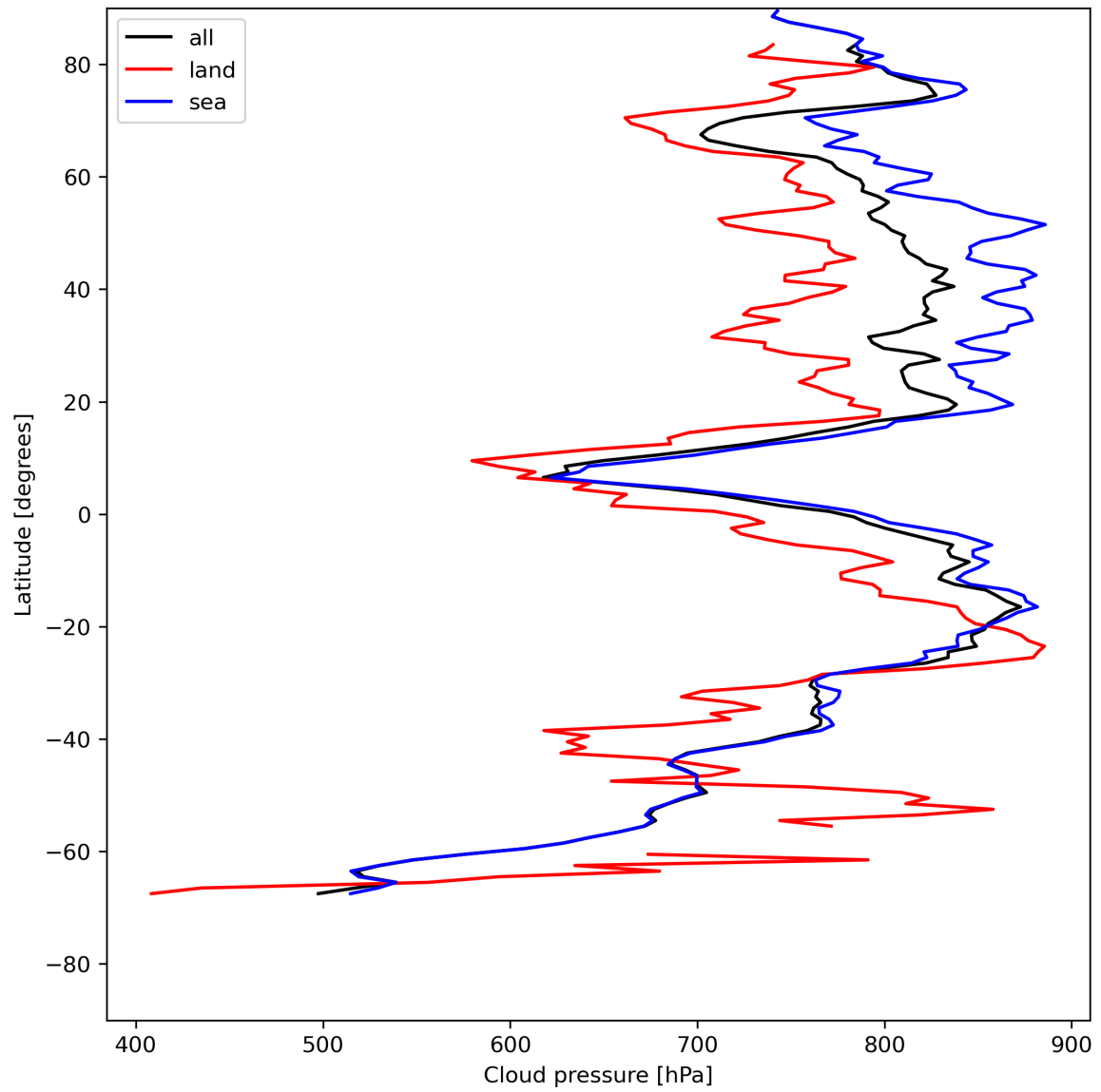
Figure 13: Zonal average of “Cloud pressure” for 2023-07-21 to 2023-07-23.
