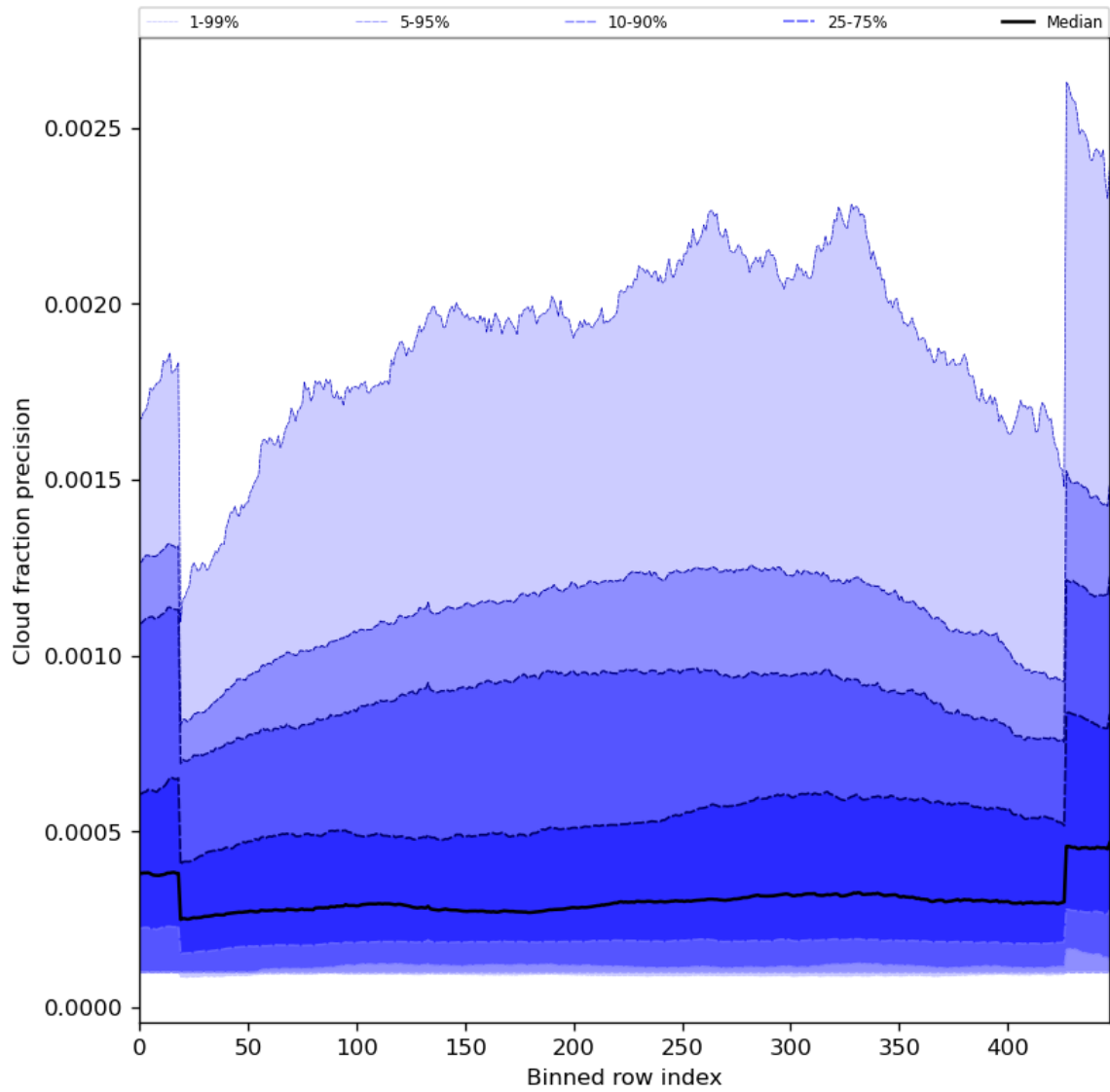
Figure 50: Along track statistics of “Cloud fraction precision” for 2023-07-21 to 2023-07-23
