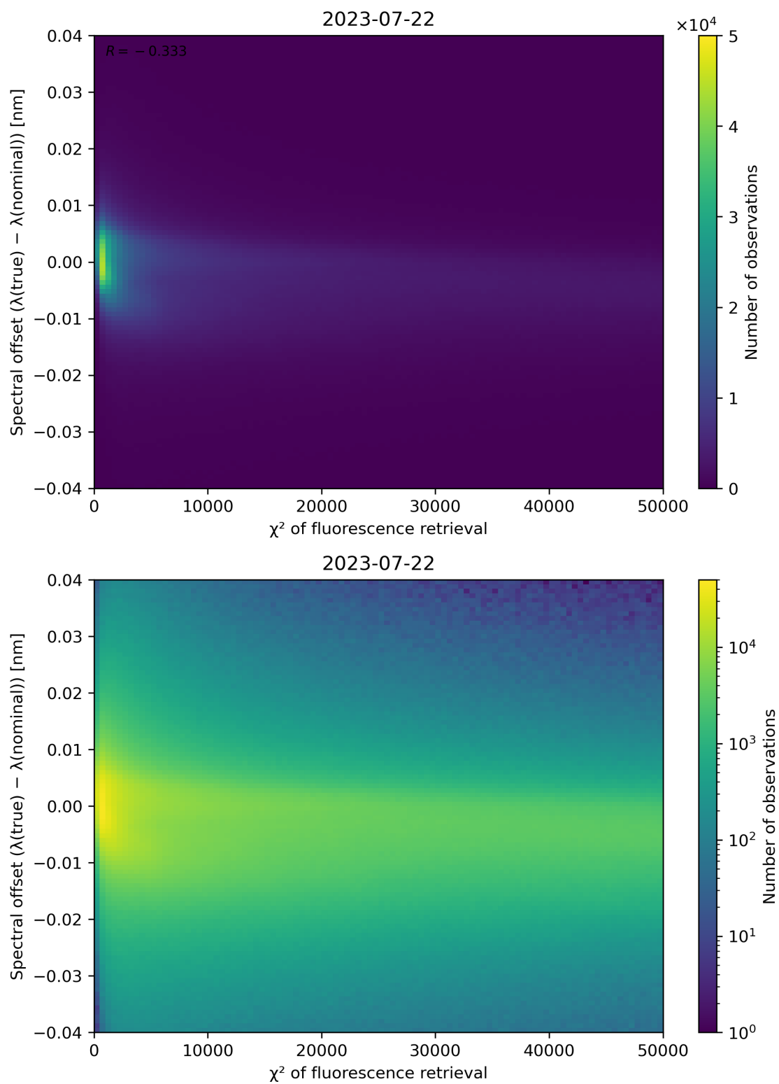
Figure 72: Scatter density plot of “ \chi^2 of fluorescence retrieval” against “Spectral offset ( \lambda(\text{true}) - \lambda(\text{nominal}) )” for 2023-07-21 to 2023-07-23.
