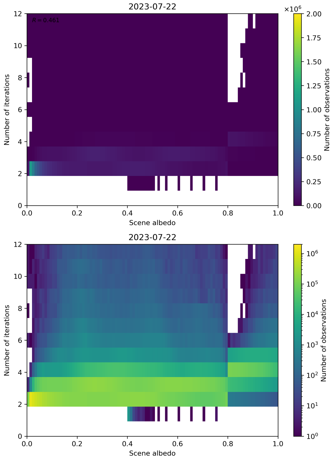
Figure 115: Scatter density plot of “Scene albedo” against “Number of iterations” for 2023-07-21 to 2023-07-23.
