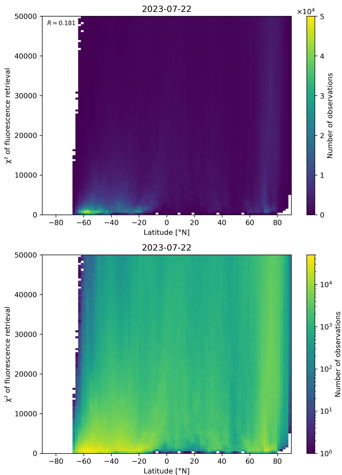
Figure 98: Scatter density plot of “Latitude” against “ \chi^2 of fluorescence retrieval” for 2023-07-21 to 2023-07-23.
