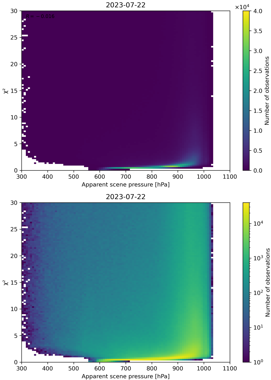
Figure 63: Scatter density plot of “Apparent scene pressure” against “ \chi^2 ” for 2023-07-21 to 2023-07-23.
