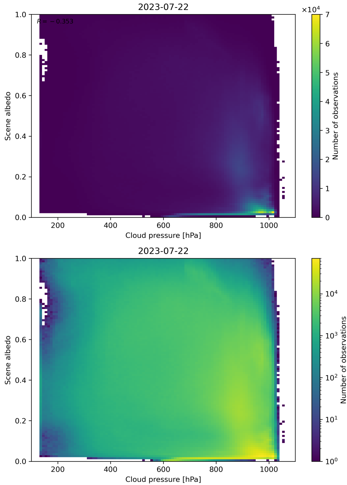
Figure 91: Scatter density plot of “Cloud pressure” against “Scene albedo” for 2023-07-21 to 2023-07-23.
