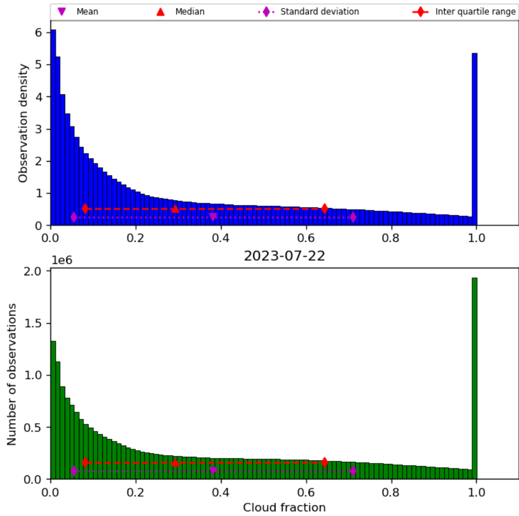
Figure 32: Histogram of “Cloud fraction” for 2023-07-21 to 2023-07-23
