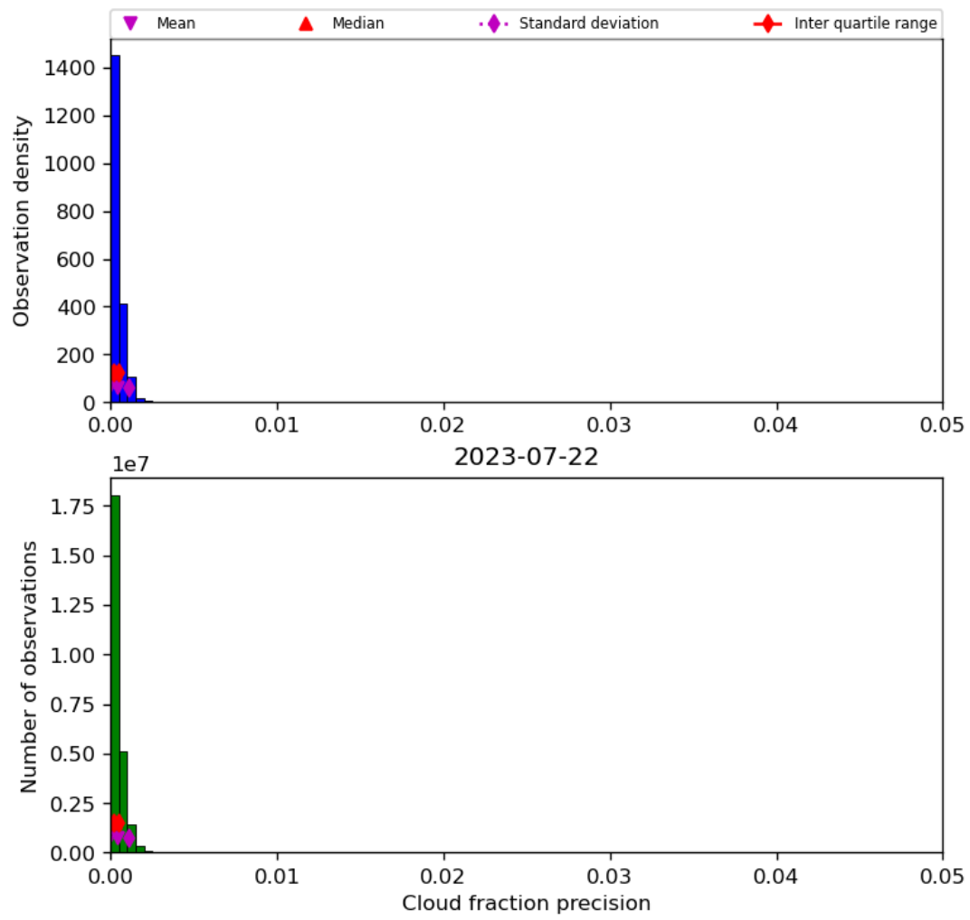
Figure 33: Histogram of “Cloud fraction precision” for 2023-07-21 to 2023-07-23
