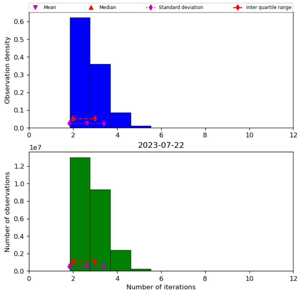
Figure 39: Histogram of “Number of iterations” for 2023-07-21 to 2023-07-23
