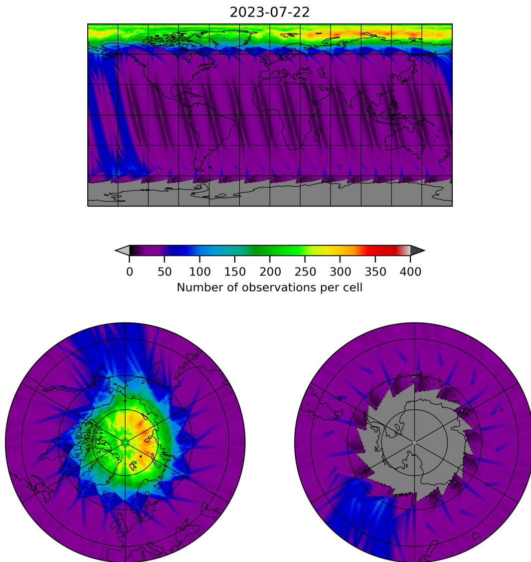
Figure 11: Map of the number of observations for 2023-07-21 to 2023-07-23
