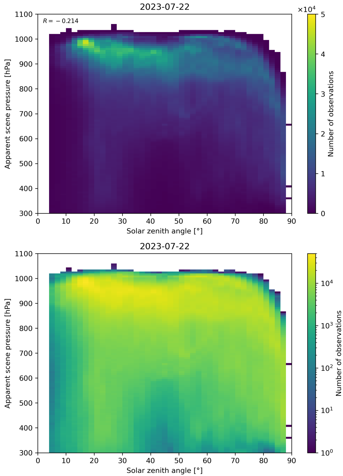
Figure 118: Scatter density plot of “Solar zenith angle” against “Apparent scene pressure” for 2023-07-21 to 2023-07-23.
