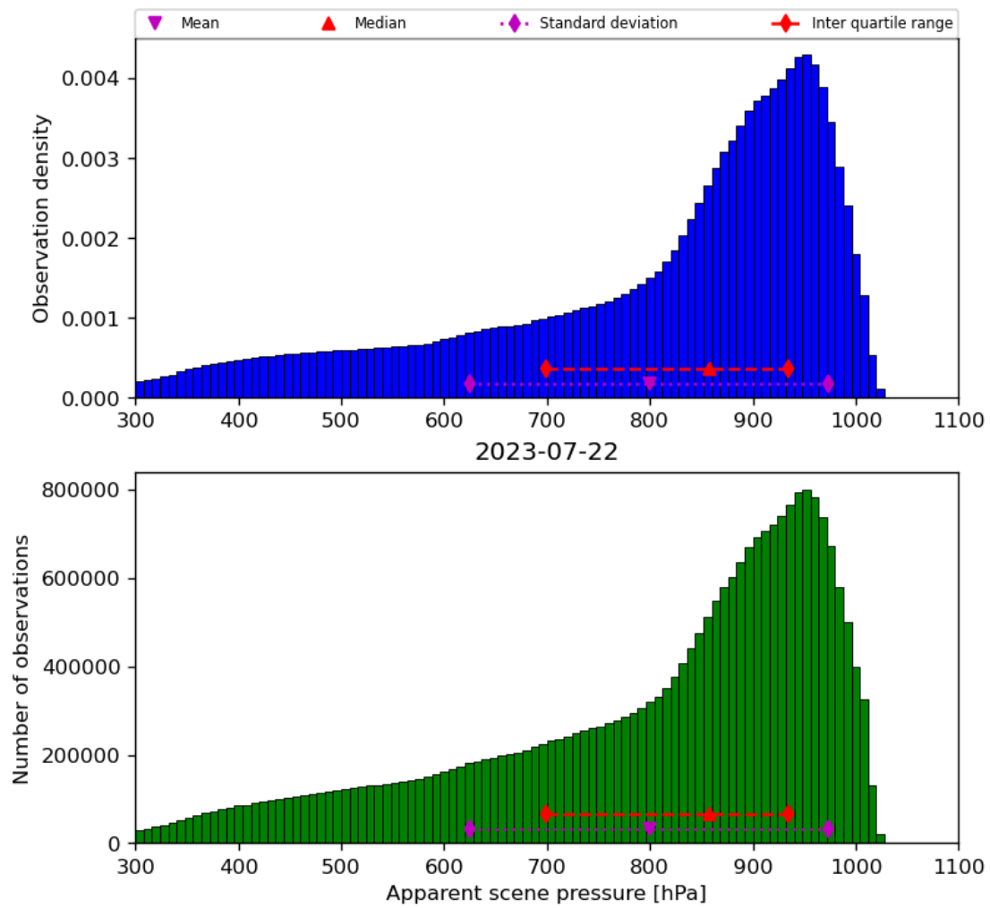
Figure 36: Histogram of “Apparent scene pressure” for 2023-07-21 to 2023-07-23
