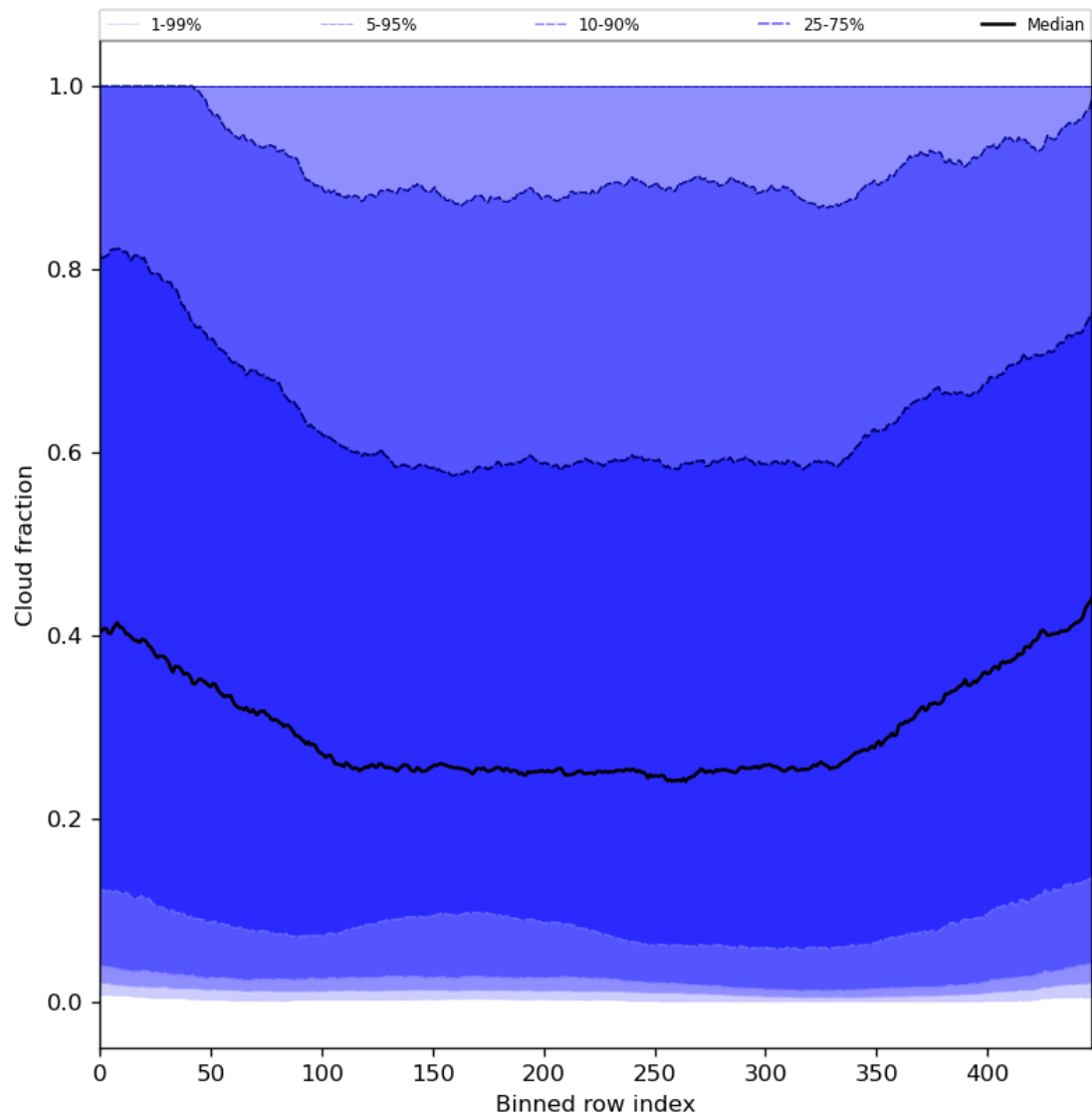
Figure 49: Along track statistics of “Cloud fraction” for 2023-07-21 to 2023-07-23
