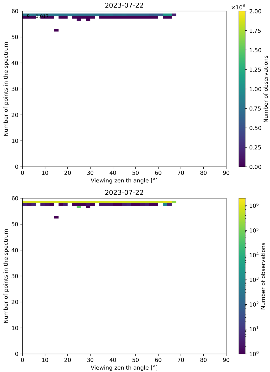
Figure 137: Scatter density plot of “Viewing zenith angle” against “Number of points in the spectrum” for 2023-07-21 to 2023-07-23.
