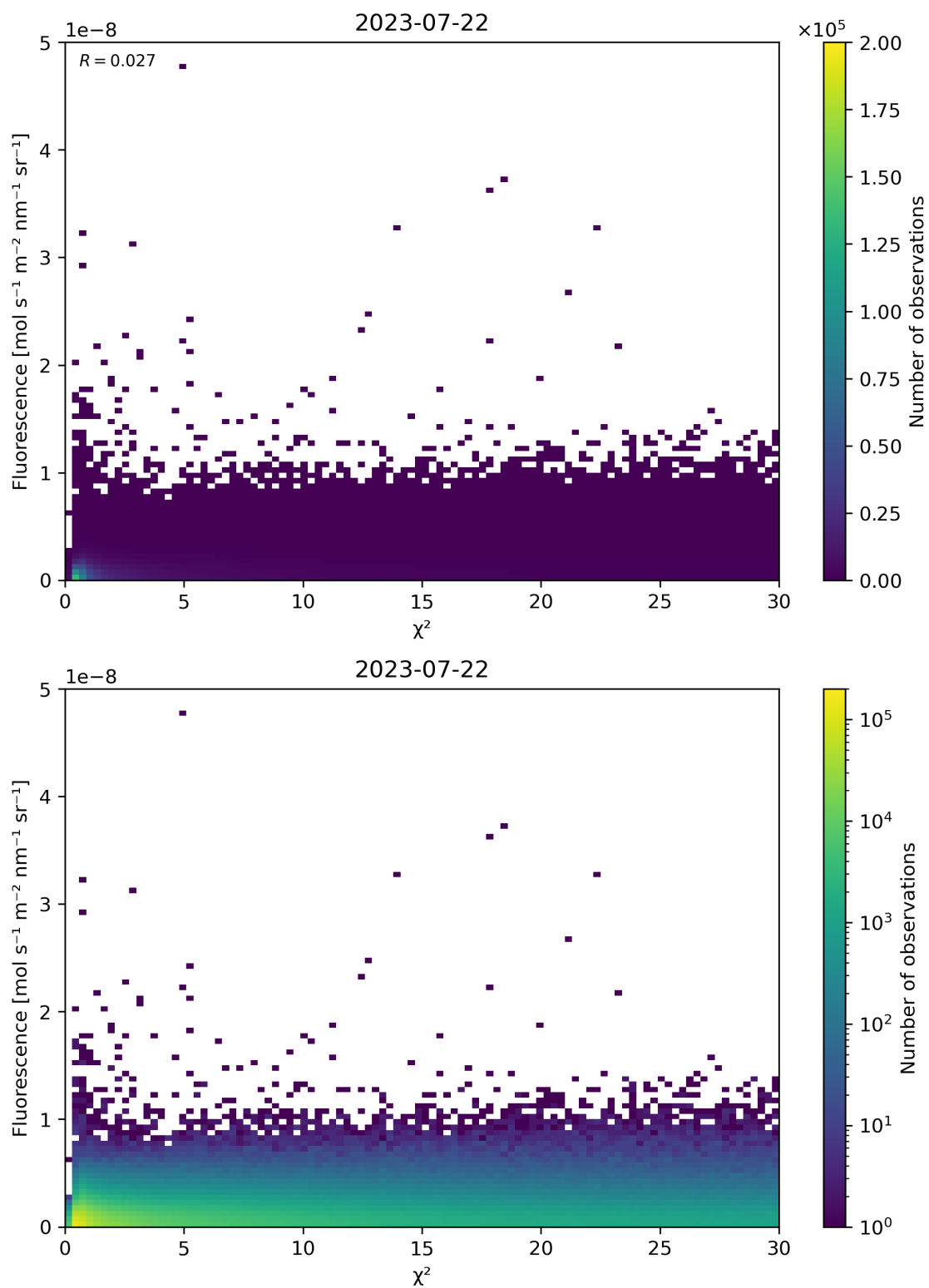
Figure 70: Scatter density plot of “ \chi^2 ” against “Fluorescence” for 2023-07-21 to 2023-07-23.
