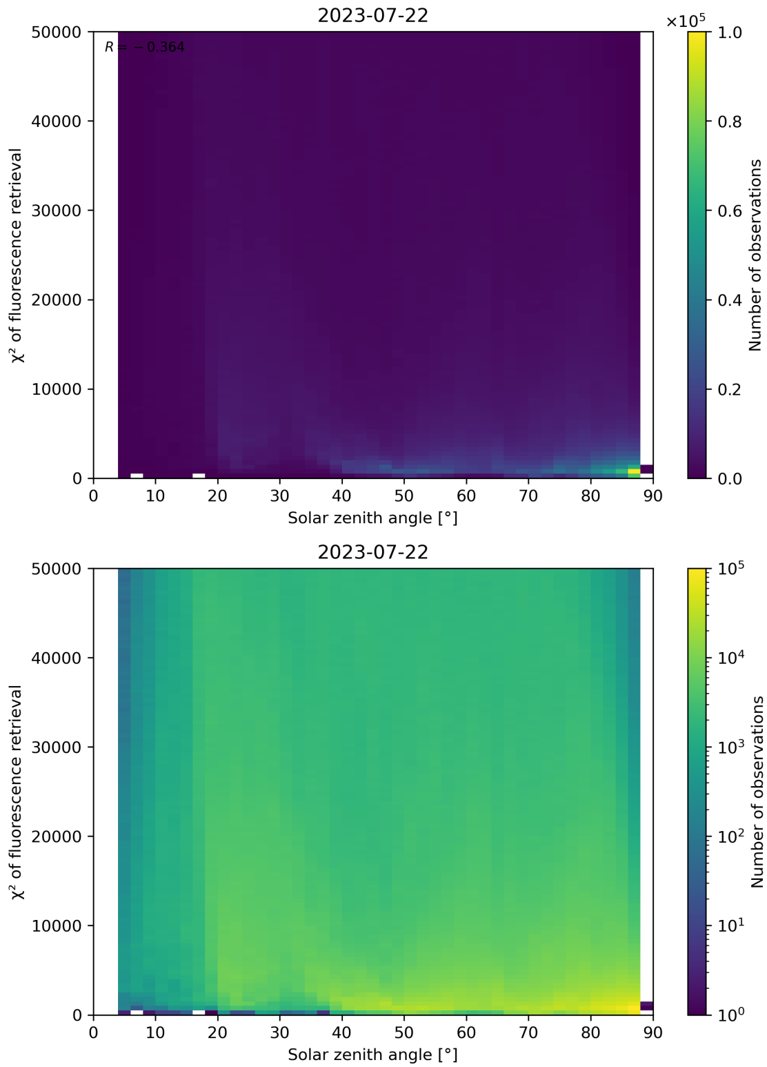
Figure 120: Scatter density plot of “Solar zenith angle” against “ \chi^2 of fluorescence retrieval” for 2023-07-21 to 2023-07-23.
