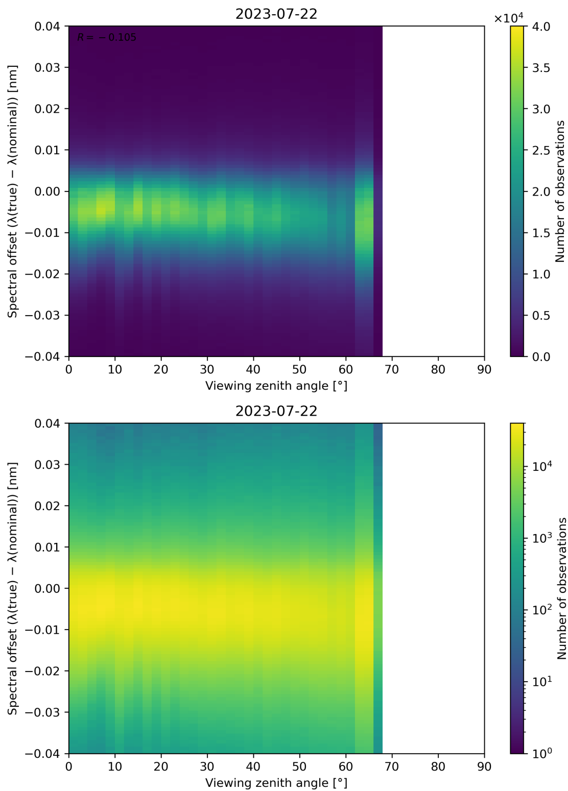
Figure 140: Scatter density plot of “Viewing zenith angle” against “Spectral offset ( \lambda(\text{true}) - \lambda(\text{nominal}) )” for 2023-07-21 to 2023-07-23.
