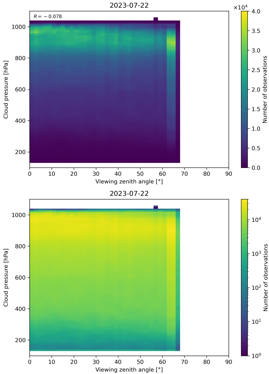
Figure 133: Scatter density plot of “Viewing zenith angle” against “Cloud pressure” for 2023-07-21 to 2023-07-23.
