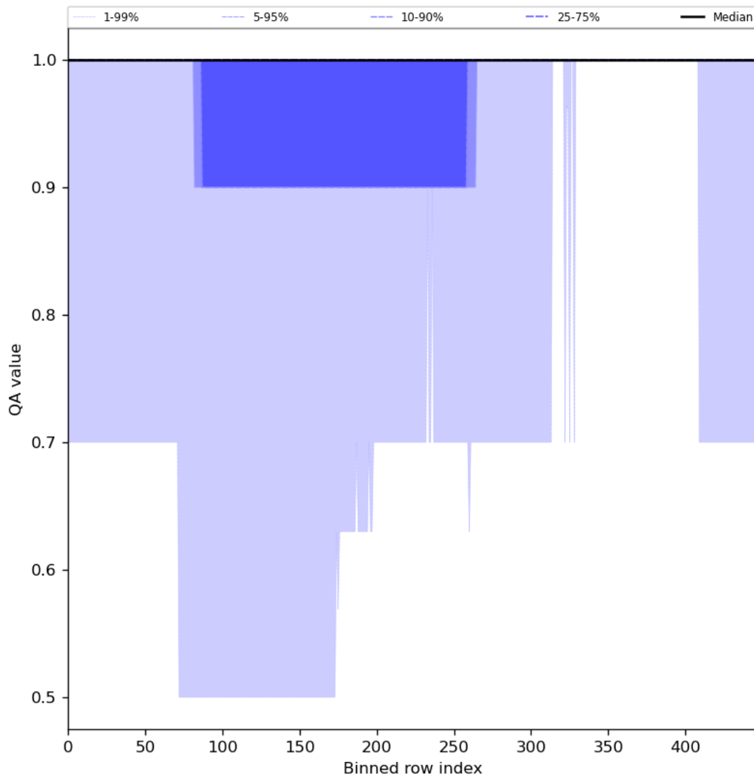
Figure 46: Along track statistics of “QA value” for 2023-07-21 to 2023-07-23
