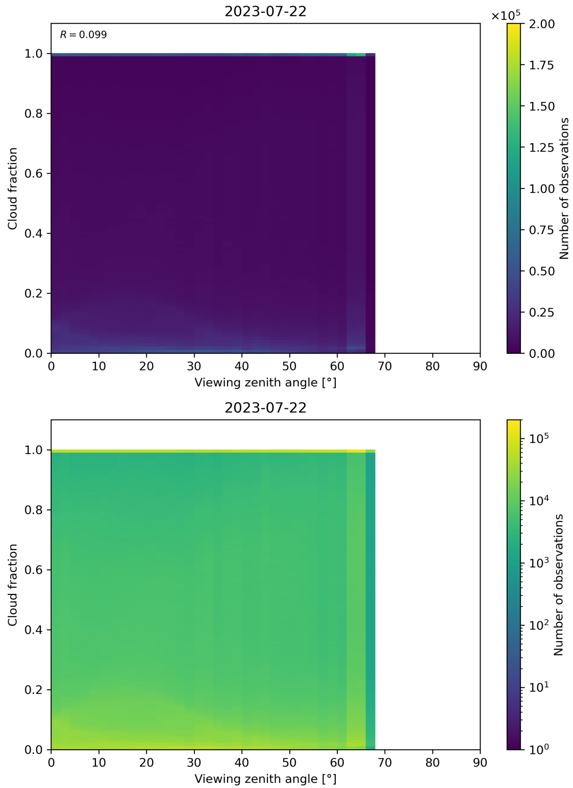
Figure 132: Scatter density plot of “Viewing zenith angle” against “Cloud fraction” for 2023-07-21 to 2023-07-23.
