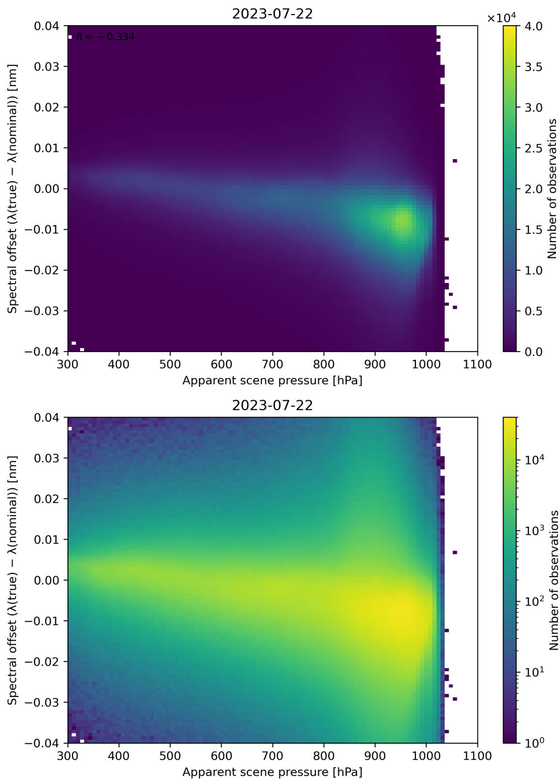
Figure 68: Scatter density plot of “Apparent scene pressure” against “Spectral offset ( \lambda(\text{true}) - \lambda(\text{nominal}) )” for 2023-07-21 to 2023-07-23.
