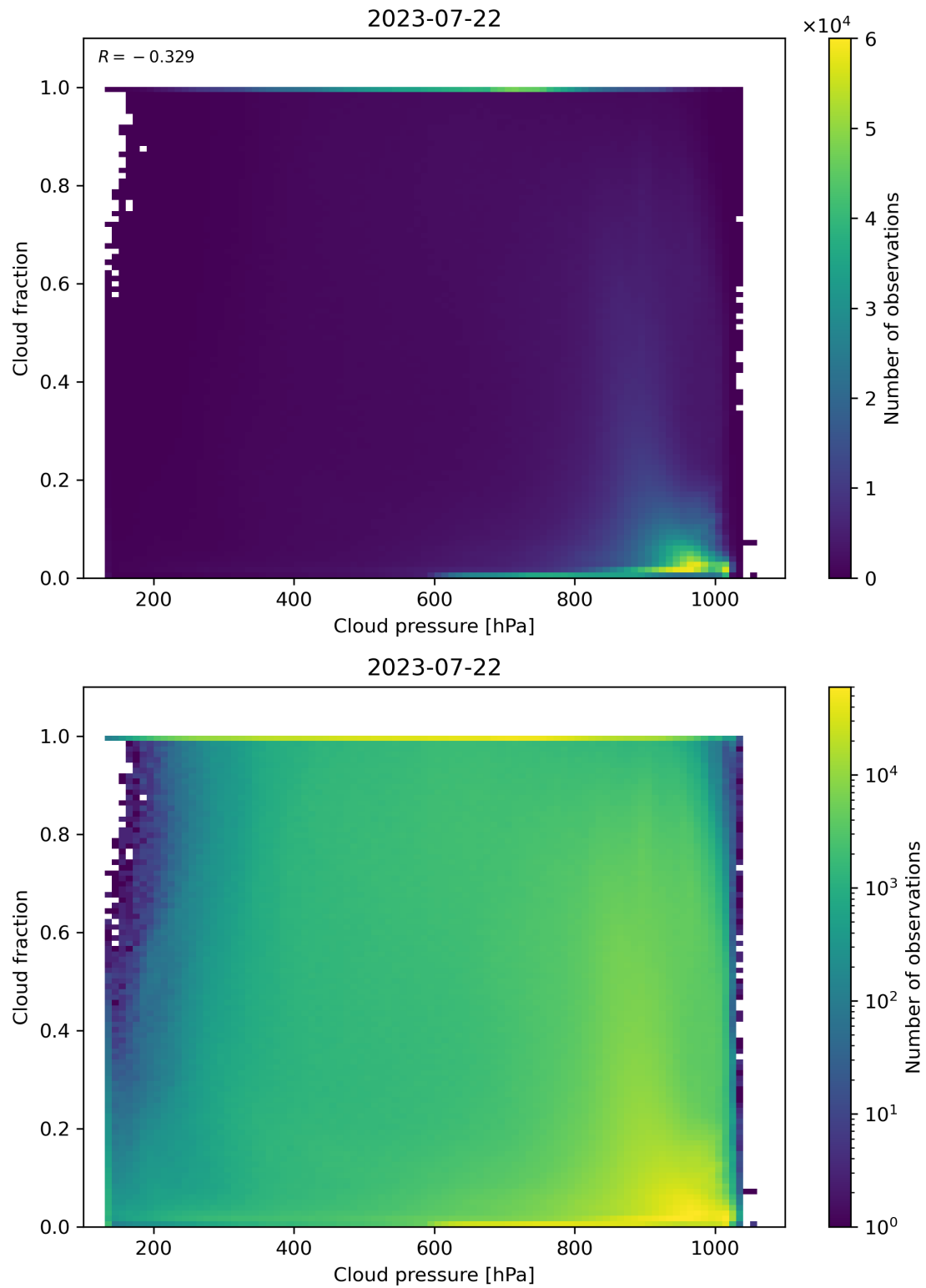
Figure 87: Scatter density plot of “Cloud pressure” against “Cloud fraction” for 2023-07-21 to 2023-07-23.
