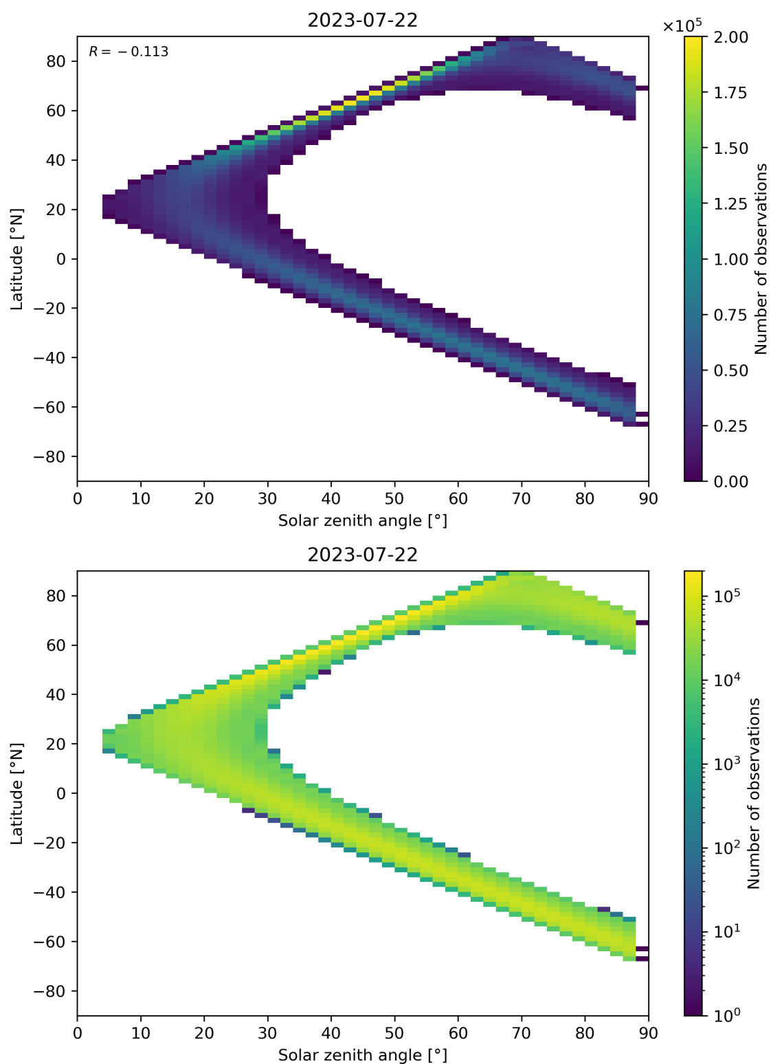
Figure 124: Scatter density plot of “Solar zenith angle” against “Latitude” for 2023-07-21 to 2023-07-23.
