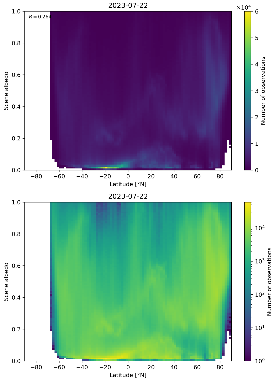
Figure 104: Scatter density plot of “Latitude” against “Scene albedo” for 2023-07-21 to 2023-07-23.
