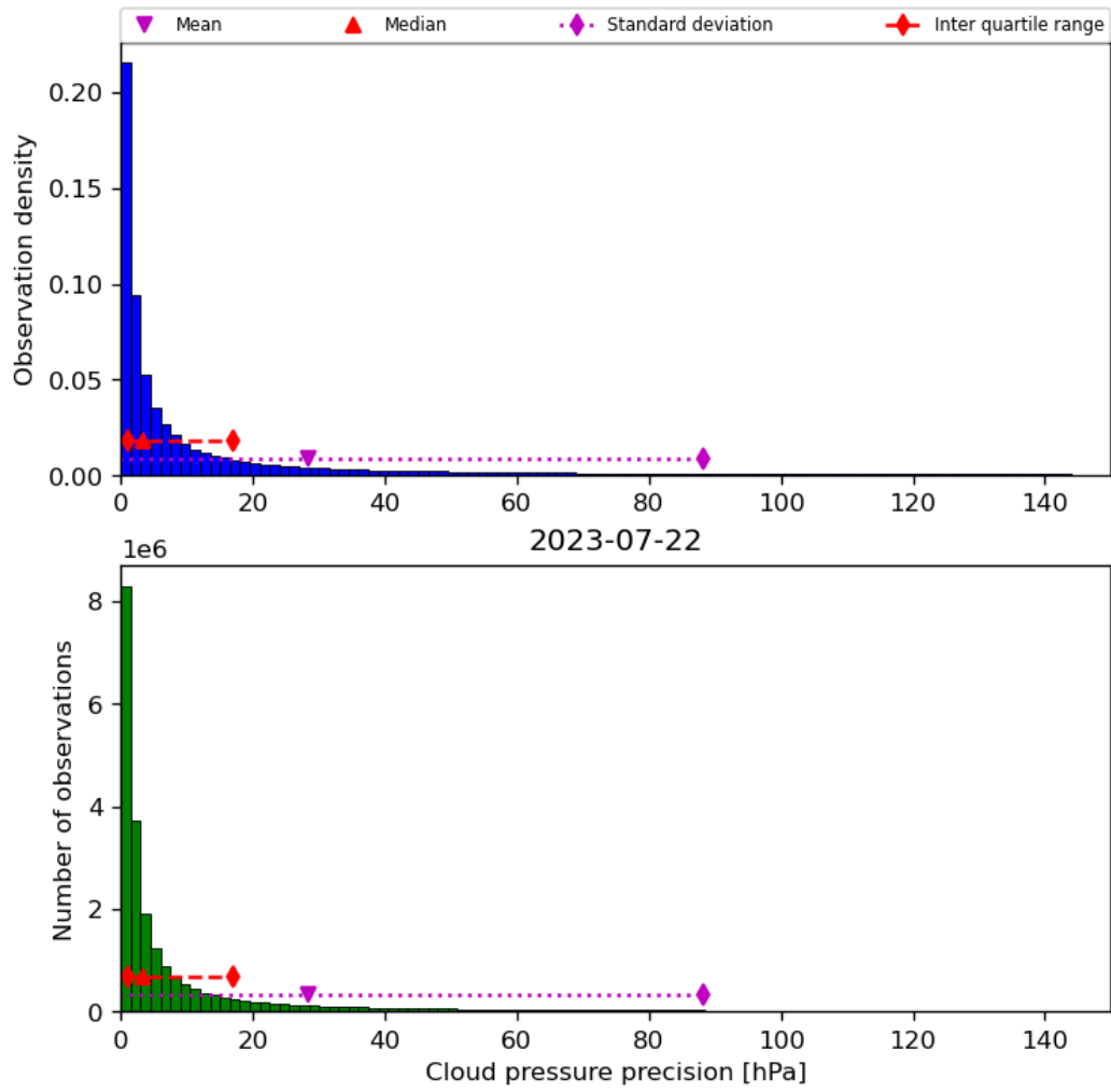
Figure 31: Histogram of “Cloud pressure precision” for 2023-07-21 to 2023-07-23
