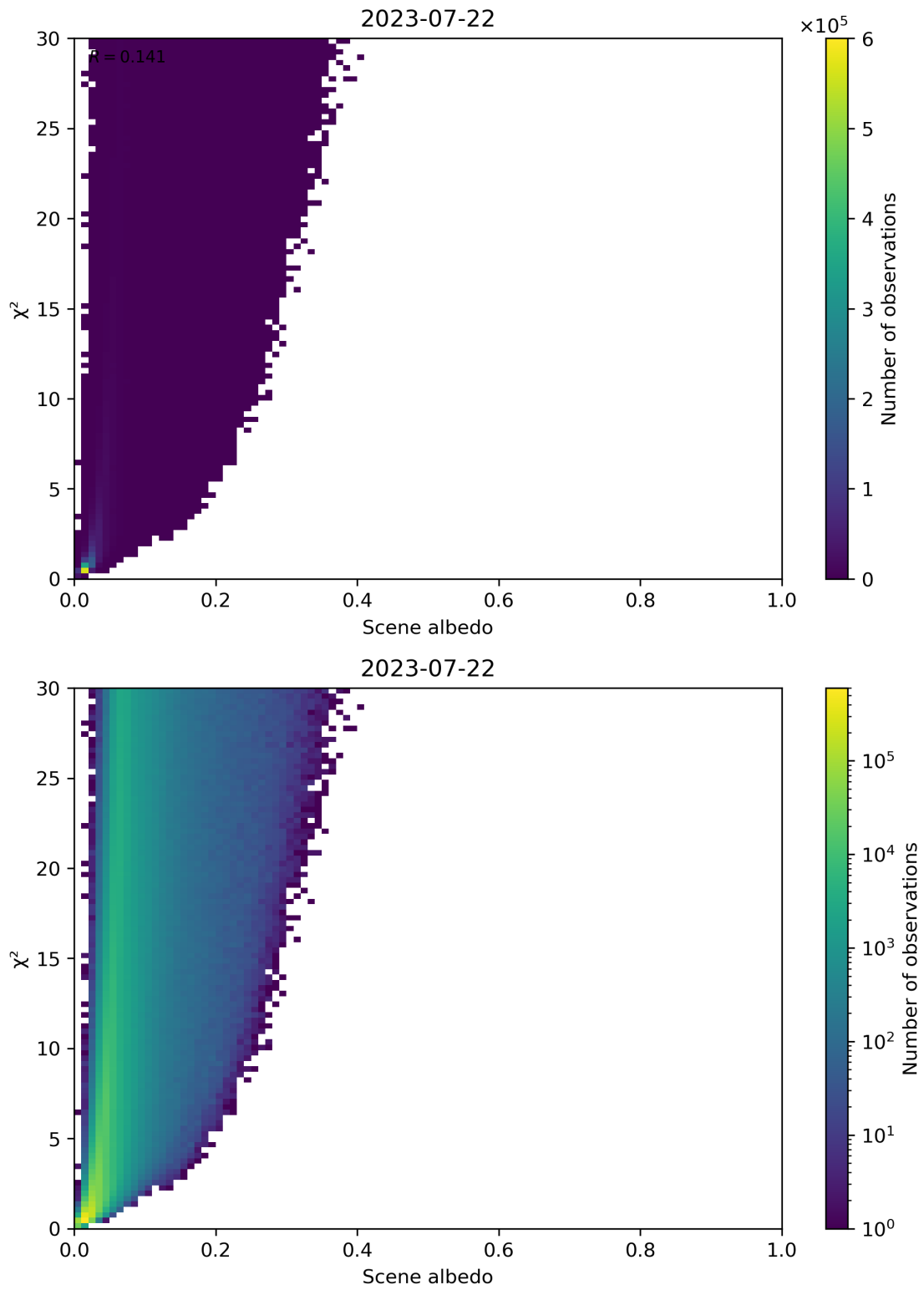
Figure 112: Scatter density plot of “Scene albedo” against “ \chi^2 ” for 2023-07-21 to 2023-07-23.
