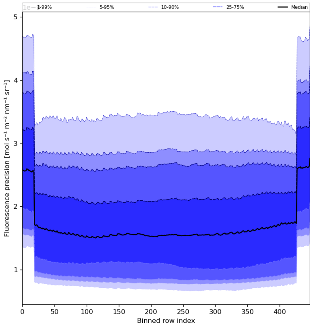
Figure 58: Along track statistics of “Fluorescence precision” for 2023-07-21 to 2023-07-23
