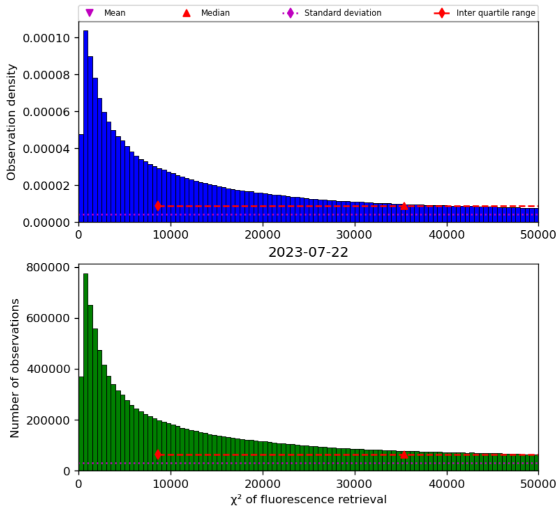
Figure 42: Histogram of “ \chi^2 of fluorescence retrieval” for 2023-07-21 to 2023-07-23
