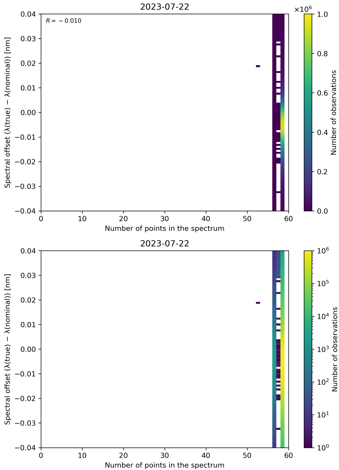
Figure 110: Scatter density plot of “Number of points in the spectrum” against “Spectral offset ( \lambda(\text{true}) - \lambda(\text{nominal}) )” for 2023-07-21 to 2023-07-23.
