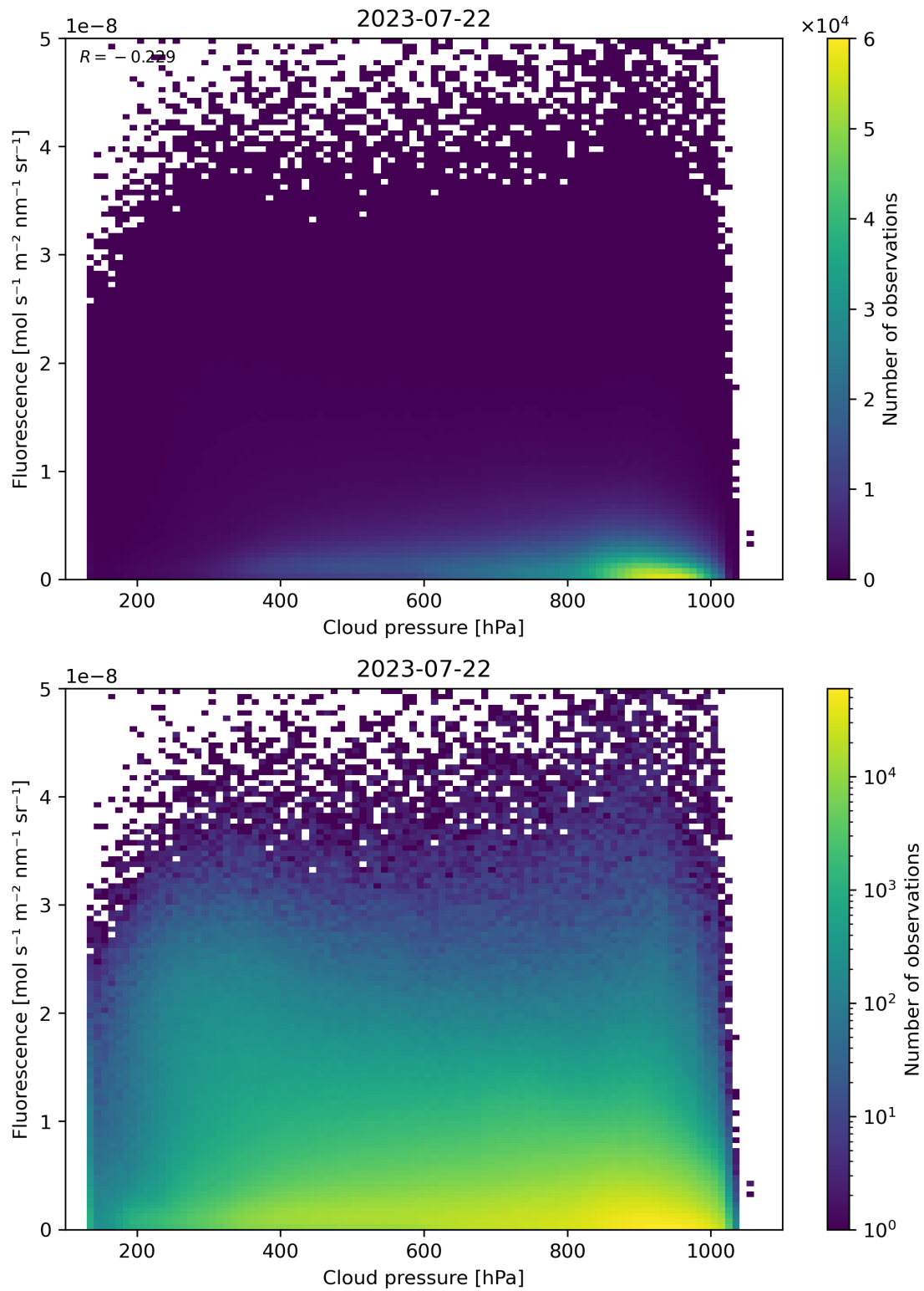
Figure 88: Scatter density plot of “Cloud pressure” against “Fluorescence” for 2023-07-21 to 2023-07-23.
