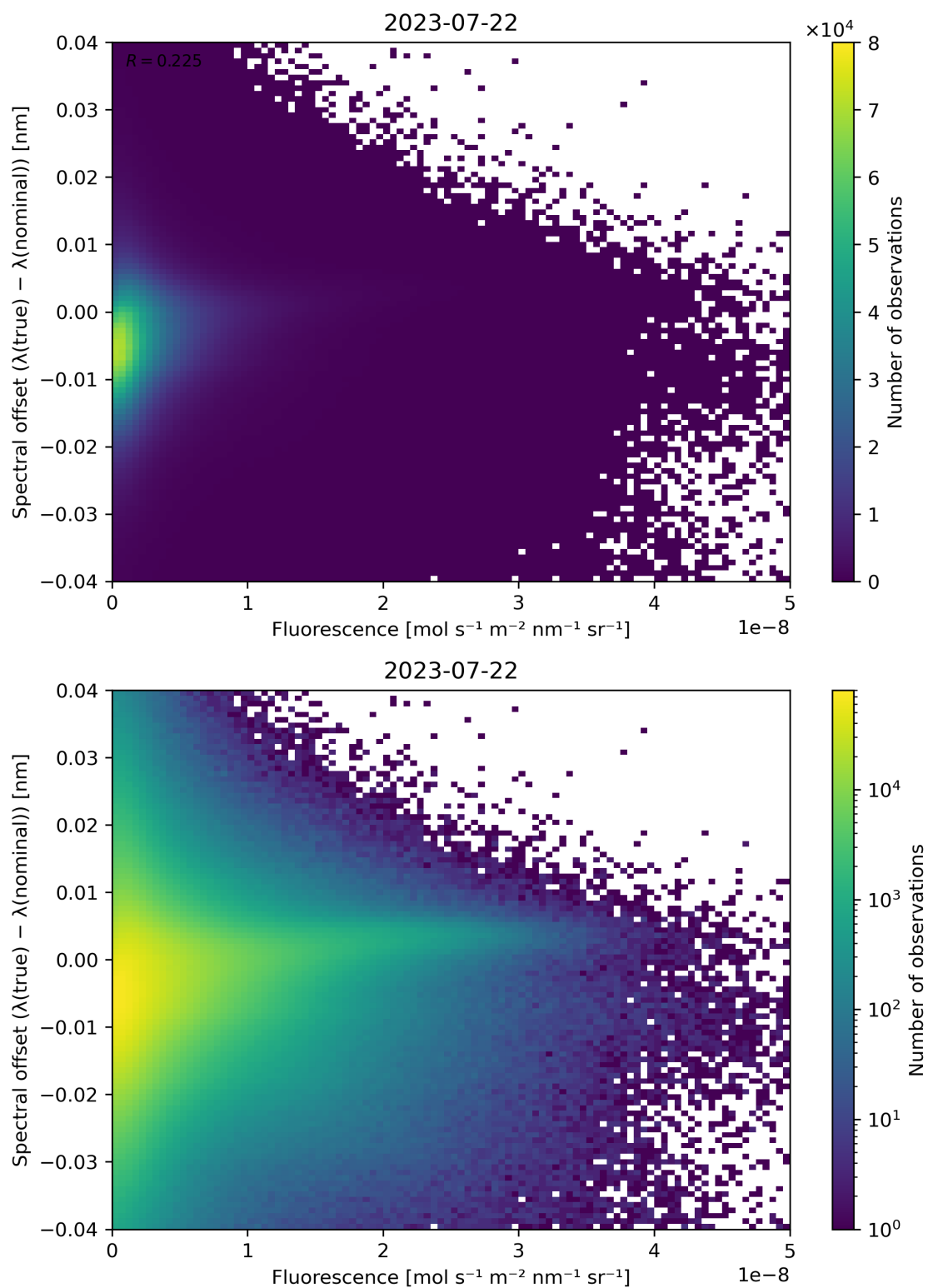
Figure 95: Scatter density plot of “Fluorescence” against “Spectral offset ( \lambda(\text{true}) - \lambda(\text{nominal}) )” for 2023-07-21 to 2023-07-23.
