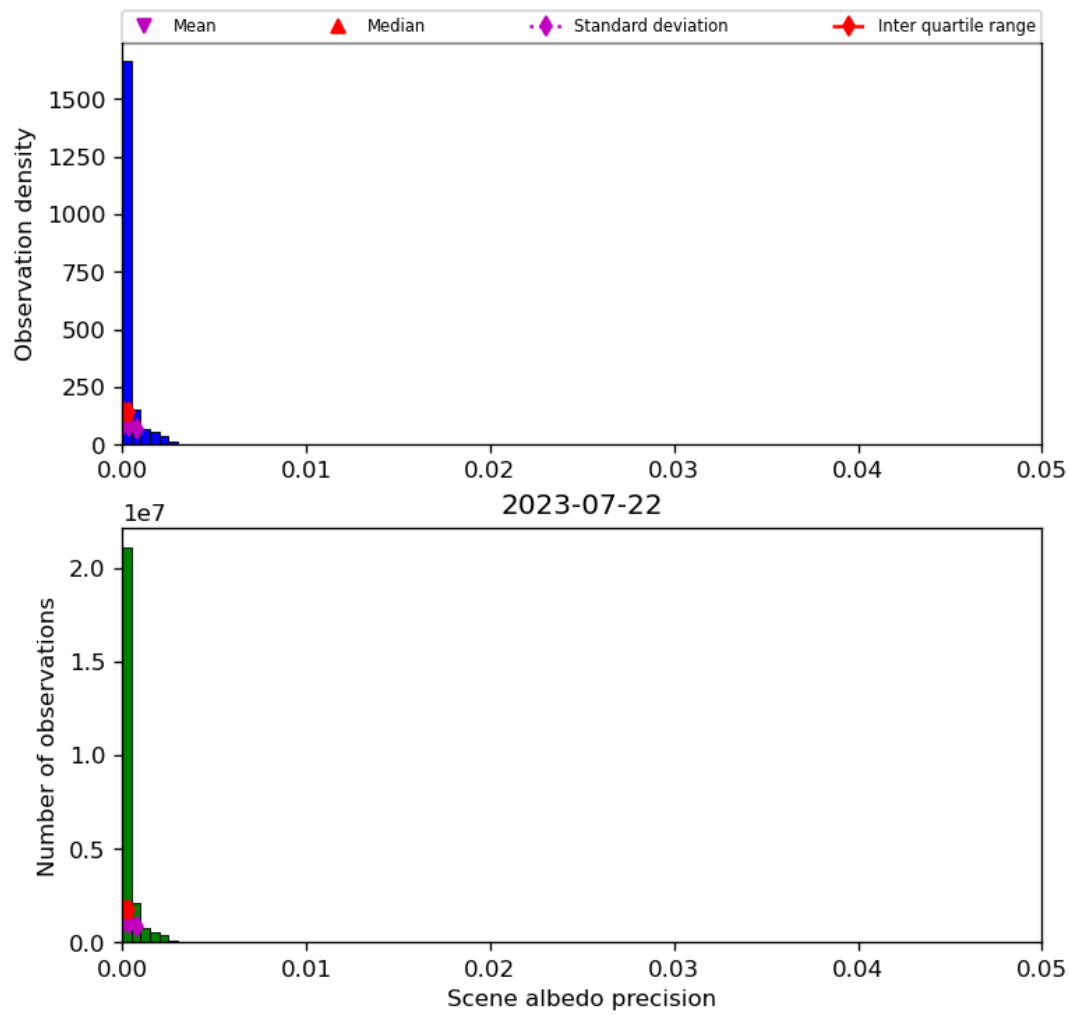
Figure 35: Histogram of “Scene albedo precision” for 2023-07-21 to 2023-07-23
