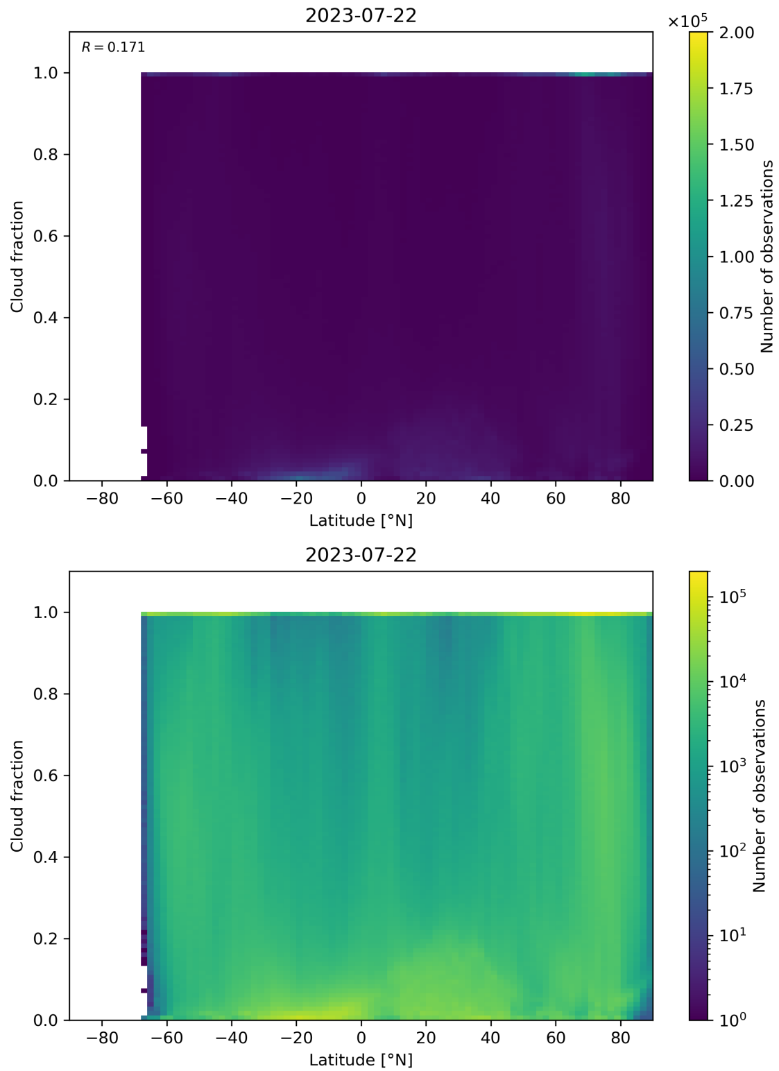
Figure 99: Scatter density plot of “Latitude” against “Cloud fraction” for 2023-07-21 to 2023-07-23.
