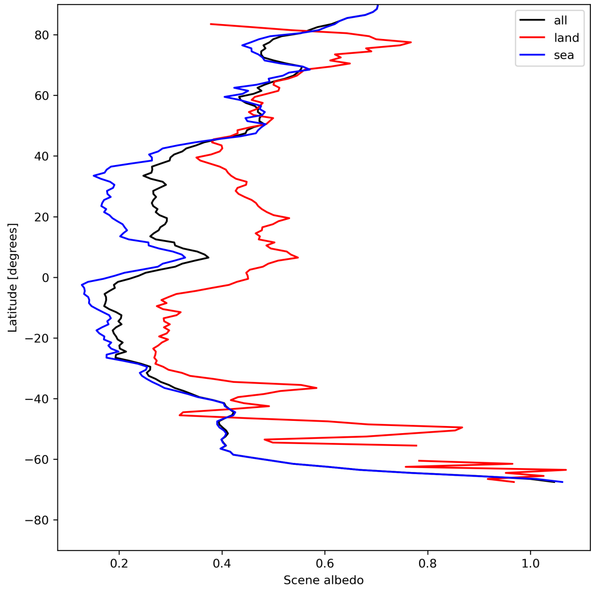
Figure 17: Zonal average of “Scene albedo” for 2023-07-21 to 2023-07-23.
