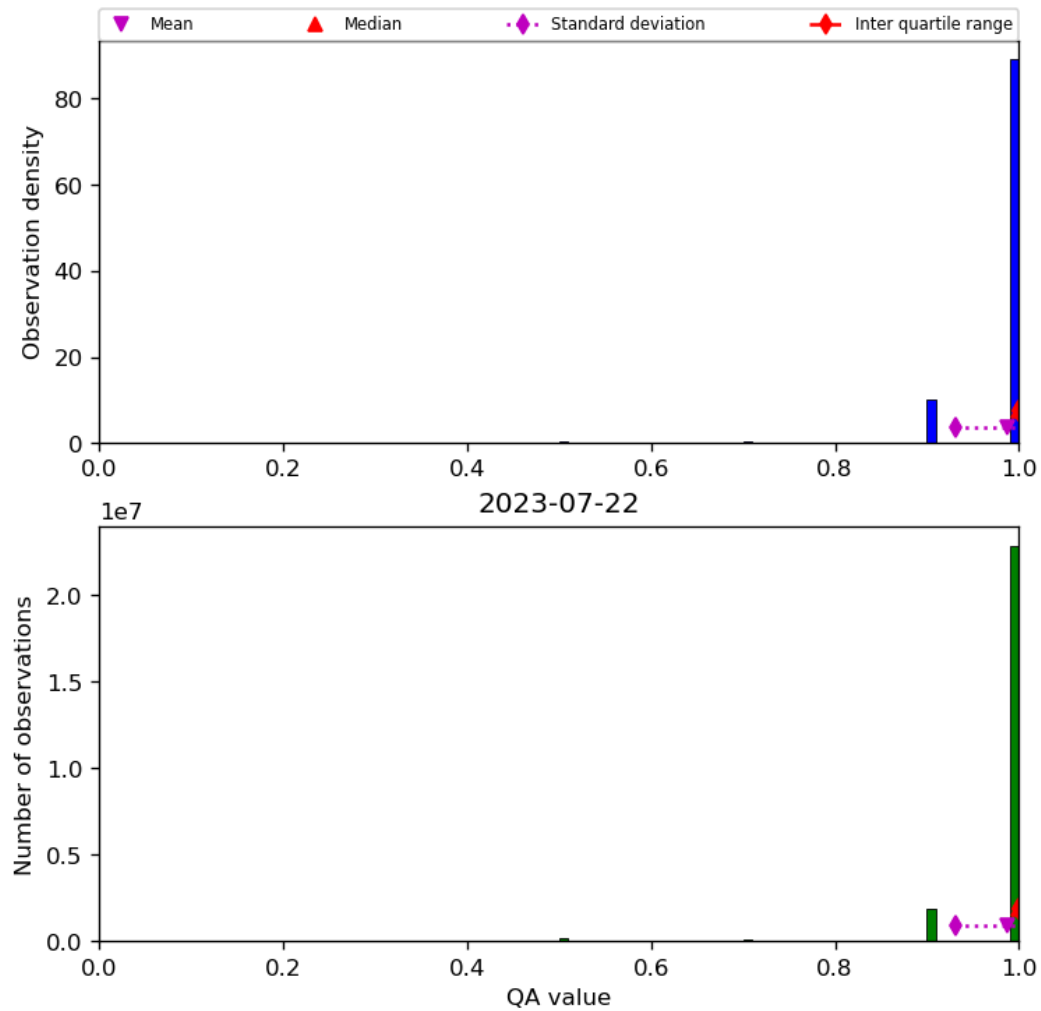
Figure 29: Histogram of “QA value” for 2023-07-21 to 2023-07-23
