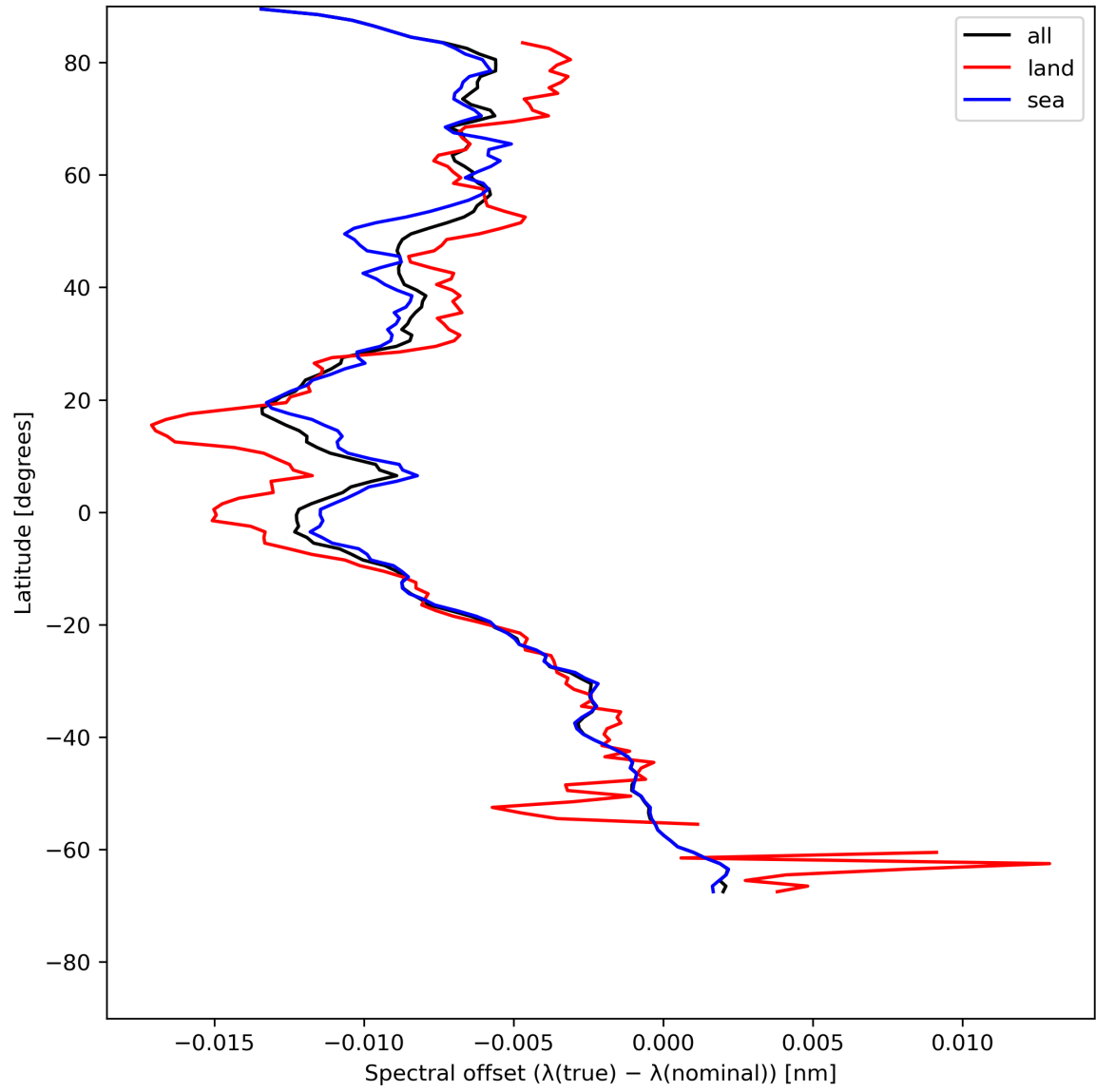
Figure 28: Zonal average of “Spectral offset ( \lambda(\text{true}) - \lambda(\text{nominal}) )” for 2023-07-21 to 2023-07-23.
