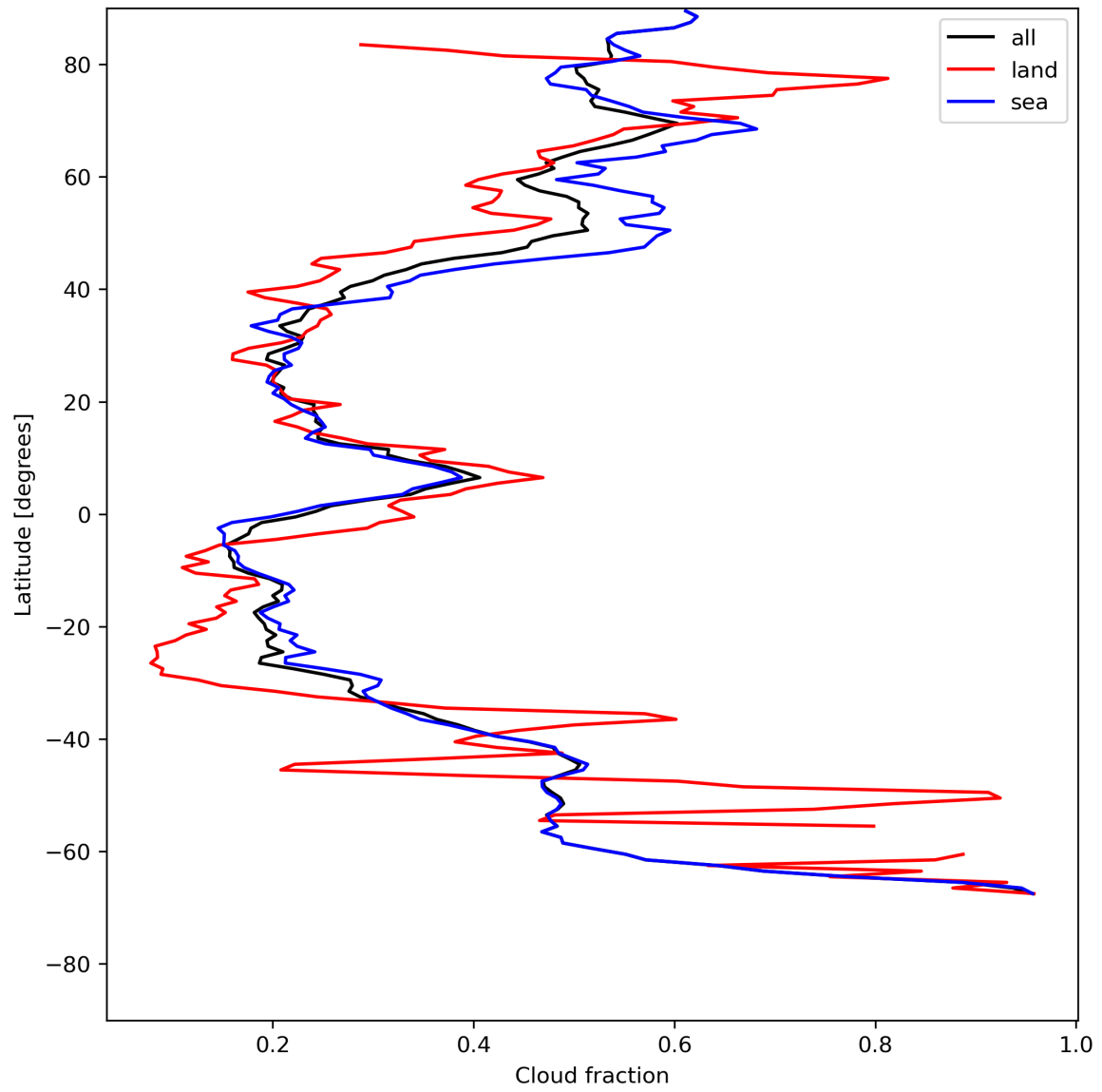
Figure 15: Zonal average of “Cloud fraction” for 2023-07-21 to 2023-07-23.
