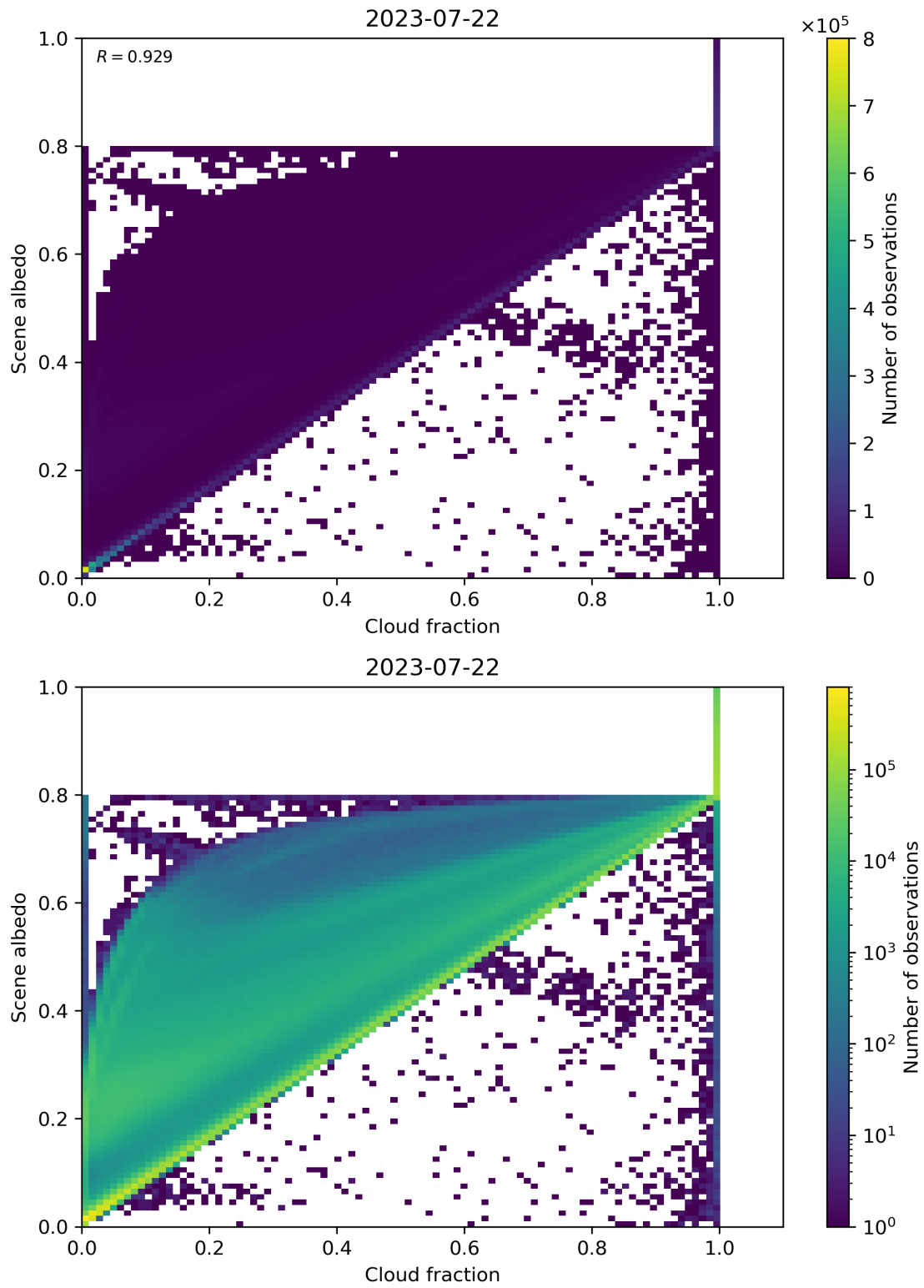
Figure 82: Scatter density plot of “Cloud fraction” against “Scene albedo” for 2023-07-21 to 2023-07-23.
