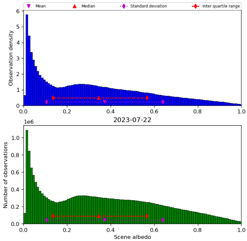
Figure 34: Histogram of “Scene albedo” for 2023-07-21 to 2023-07-23
