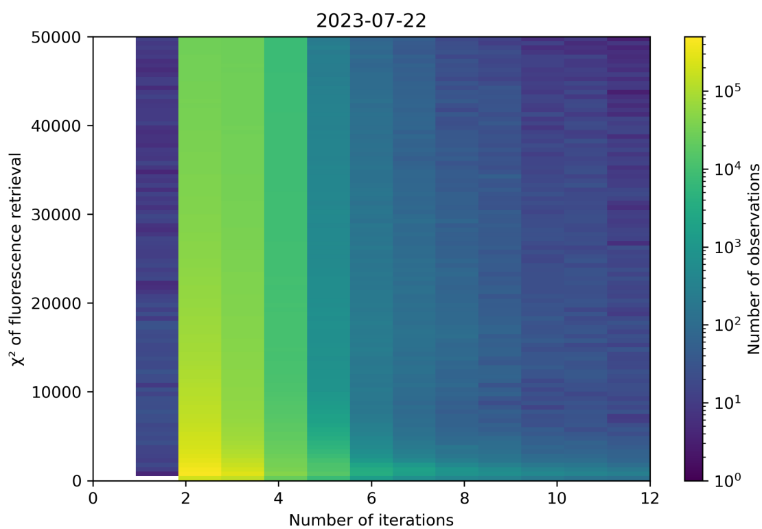
Figure 106: Scatter density plot of “Number of iterations” against “ \chi^2 of fluorescence retrieval” for 2023-07-21 to 2023-07-23.
