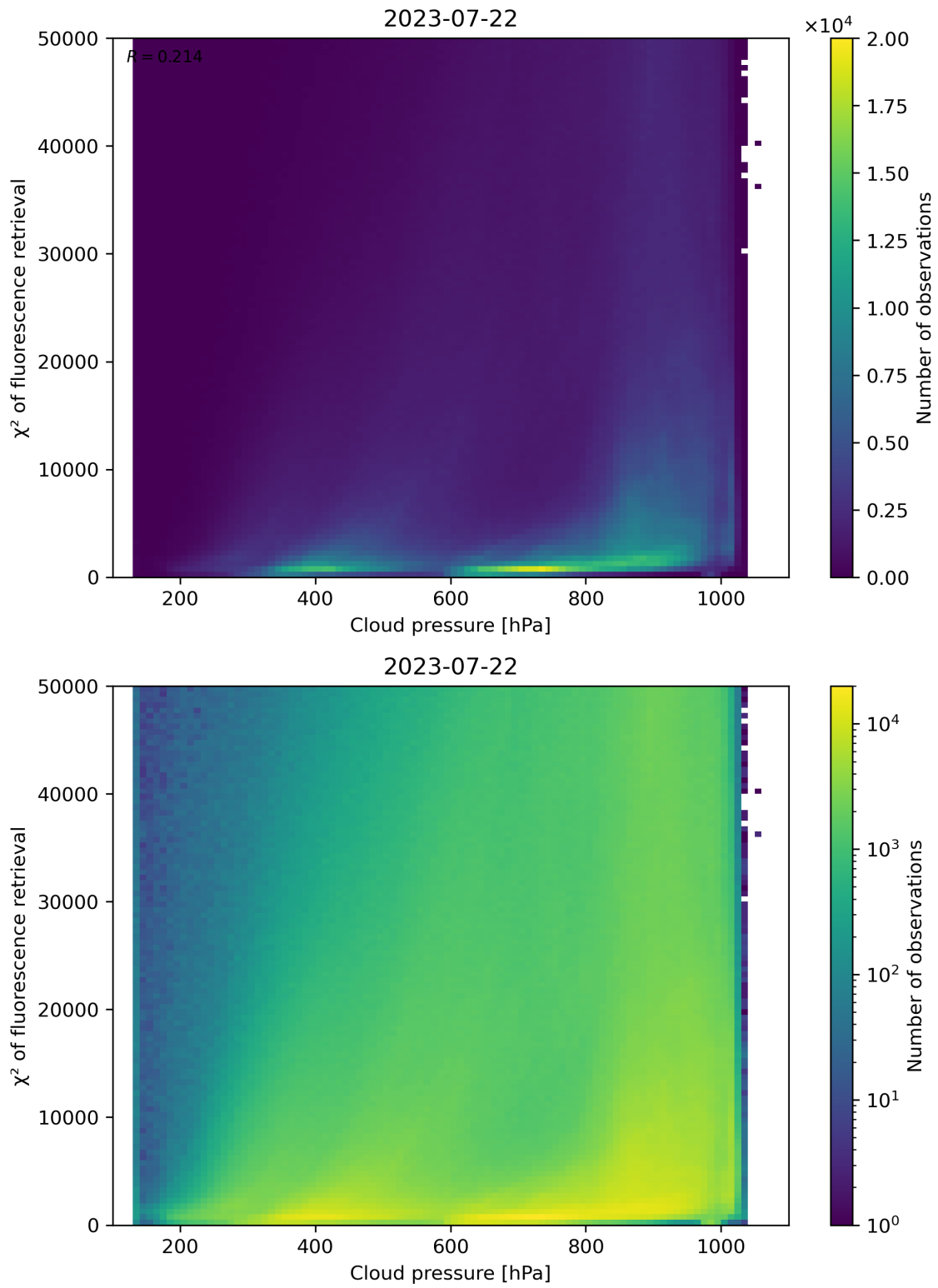
Figure 86: Scatter density plot of “Cloud pressure” against “ \chi^2 of fluorescence retrieval” for 2023-07-21 to 2023-07-23.
