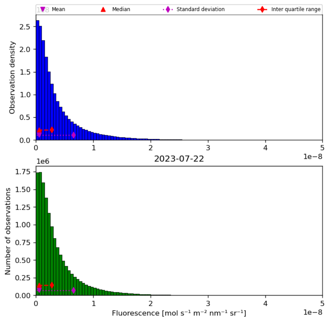
Figure 40: Histogram of “Fluorescence” for 2023-07-21 to 2023-07-23
