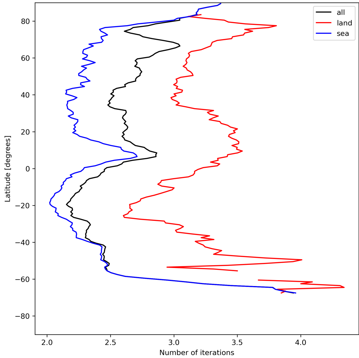
Figure 22: Zonal average of “Number of iterations” for 2023-07-21 to 2023-07-23.
