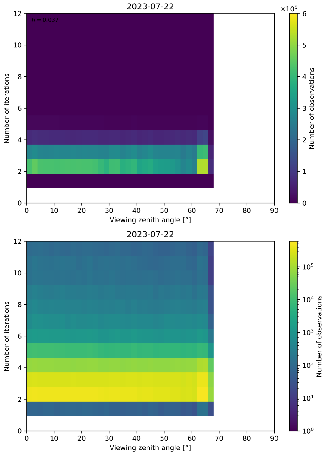
Figure 136: Scatter density plot of “Viewing zenith angle” against “Number of iterations” for 2023-07-21 to 2023-07-23.
