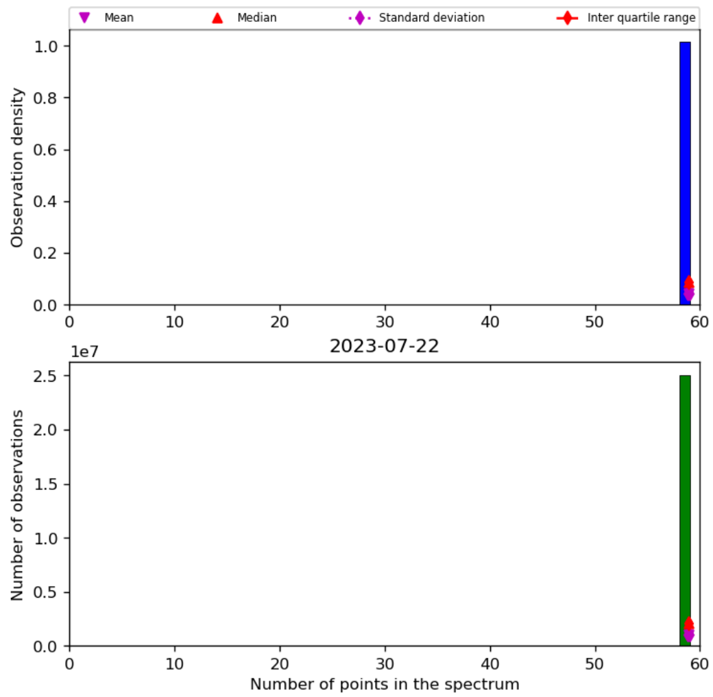
Figure 44: Histogram of “Number of points in the spectrum” for 2023-07-21 to 2023-07-23
