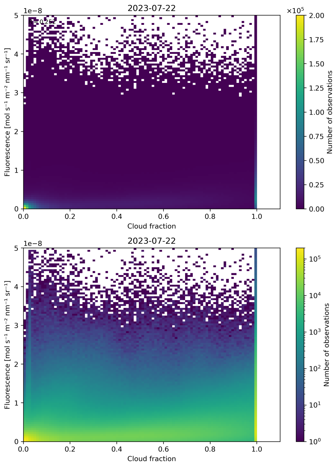
Figure 79: Scatter density plot of “Cloud fraction” against “Fluorescence” for 2023-07-21 to 2023-07-23.
