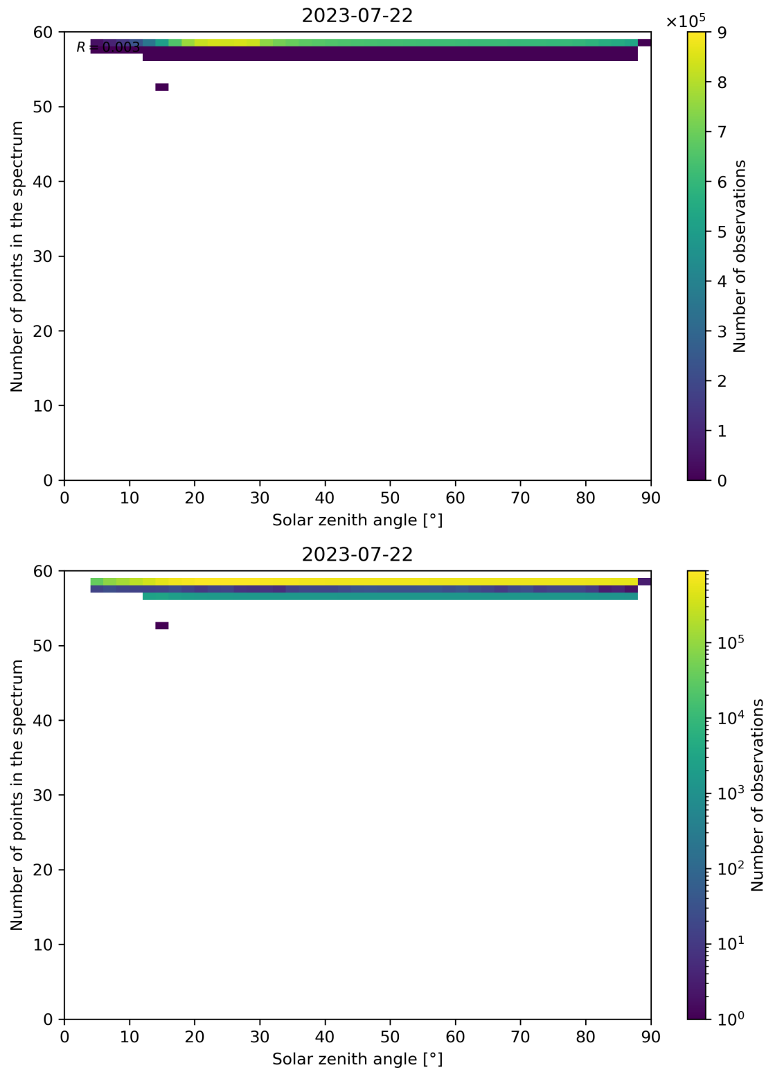
Figure 126: Scatter density plot of “Solar zenith angle” against “Number of points in the spectrum” for 2023-07-21 to 2023-07-23.
