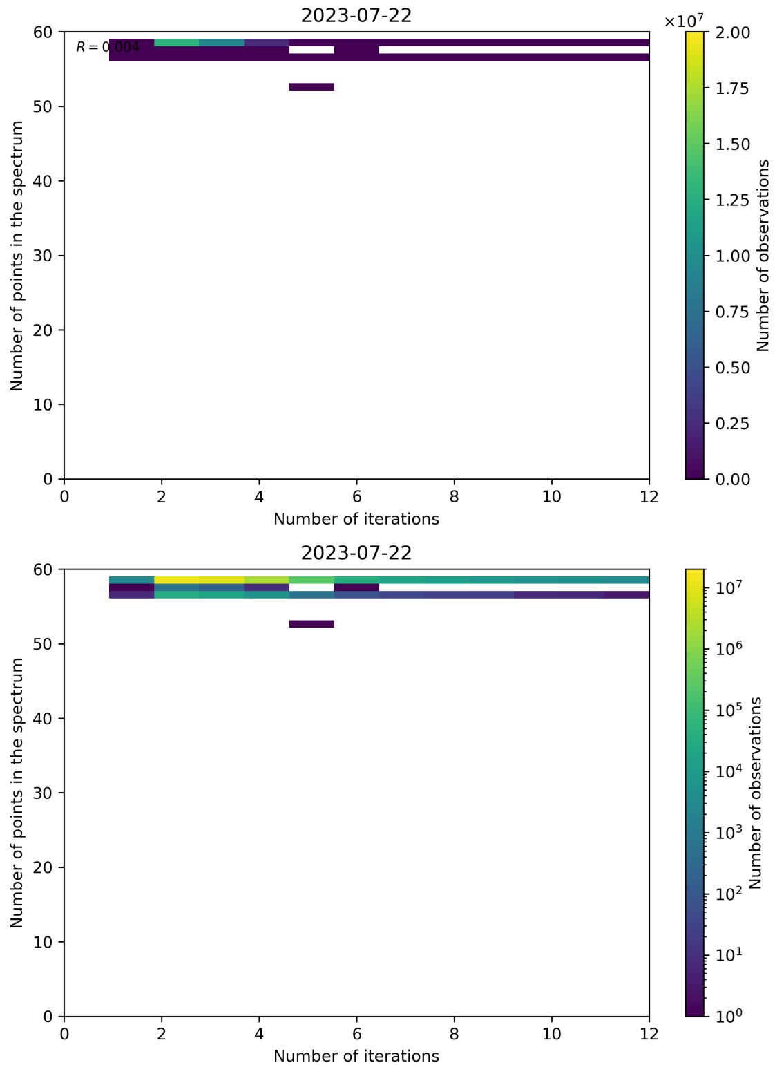
Figure 108: Scatter density plot of “Number of iterations” against “Number of points in the spectrum” for 2023-07-21 to 2023-07-23.
