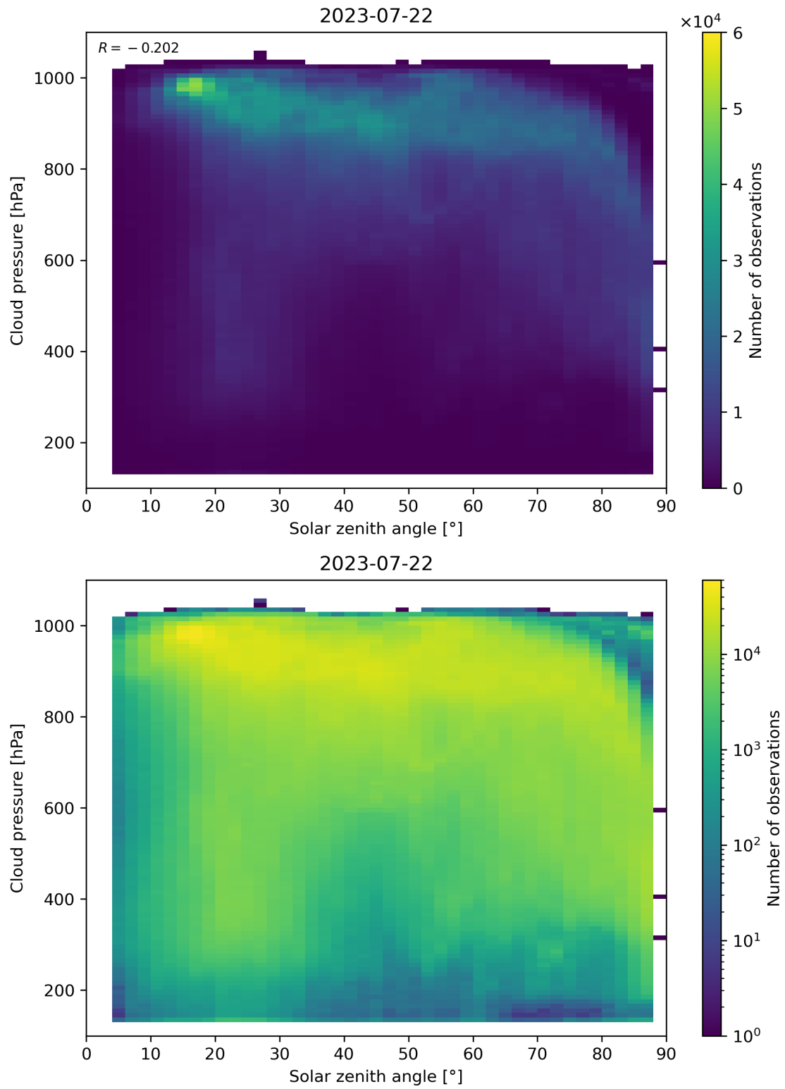
Figure 122: Scatter density plot of “Solar zenith angle” against “Cloud pressure” for 2023-07-21 to 2023-07-23.
