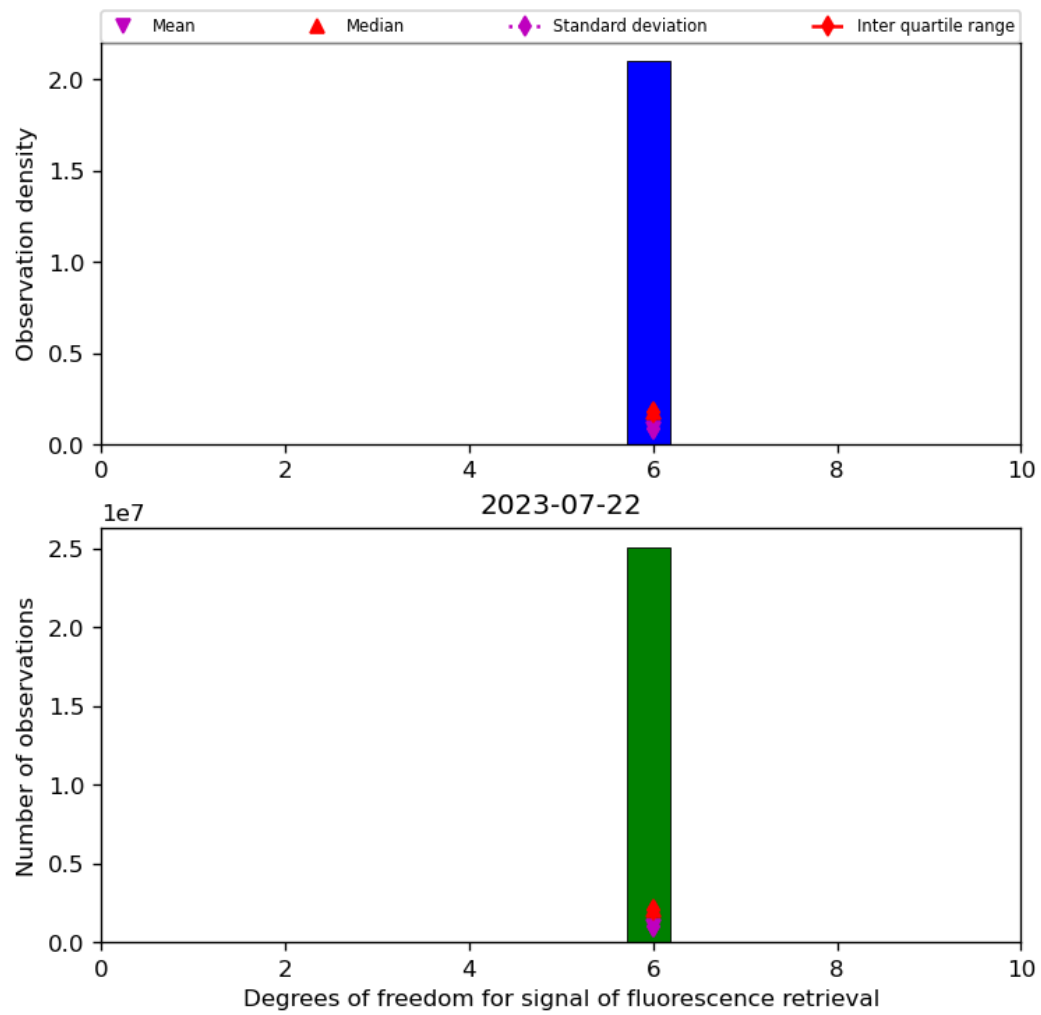
Figure 43: Histogram of “Degrees of freedom for signal of fluorescence retrieval” for 2023-07-21 to 2023-07-23
