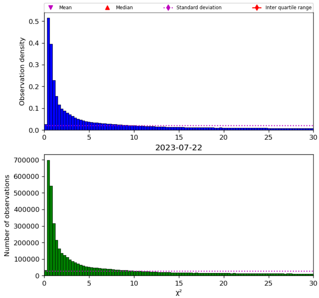
Figure 38: Histogram of “ \chi^2 ” for 2023-07-21 to 2023-07-23
