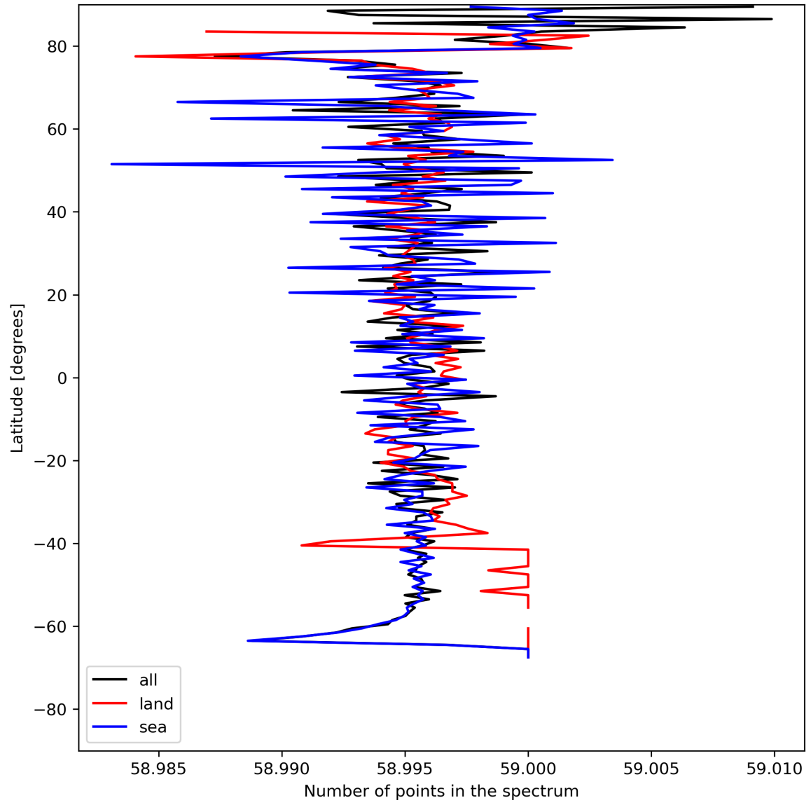
Figure 27: Zonal average of “Number of points in the spectrum” for 2023-07-21 to 2023-07-23.
