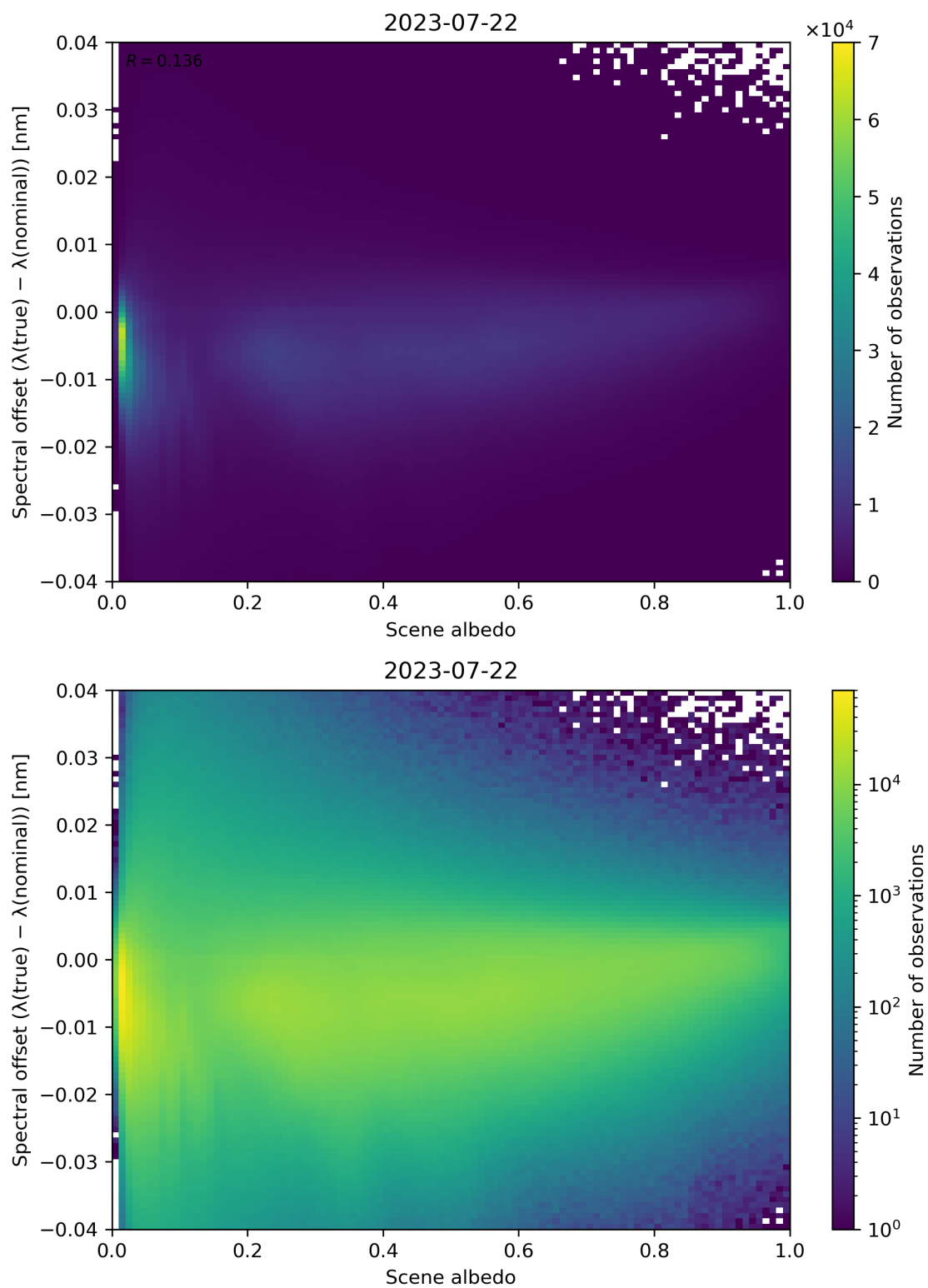
Figure 117: Scatter density plot of “Scene albedo” against “Spectral offset ( \lambda(\text{true}) - \lambda(\text{nominal}) )” for 2023-07-21 to 2023-07-23.
