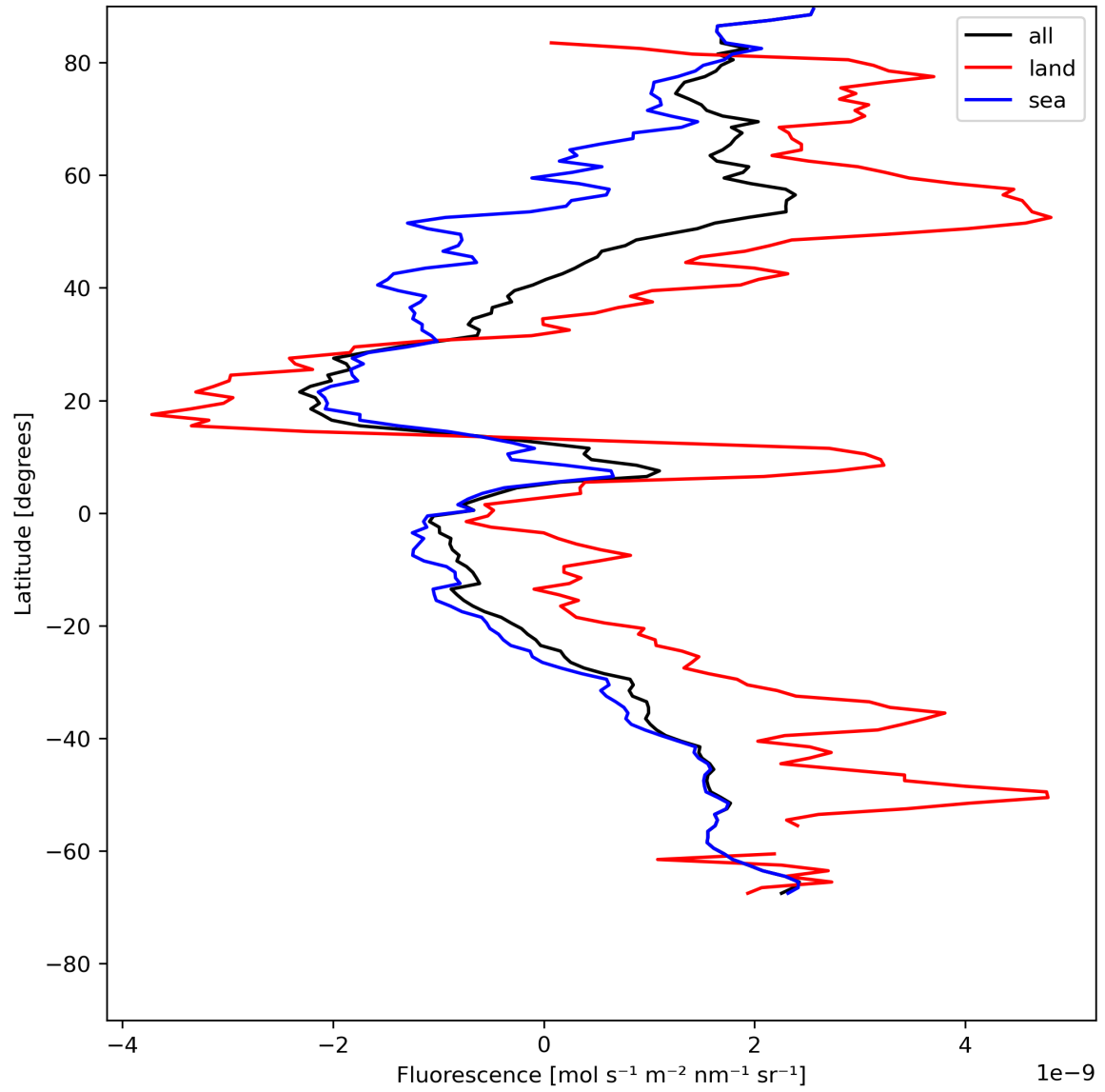
Figure 23: Zonal average of “Fluorescence” for 2023-07-21 to 2023-07-23.
