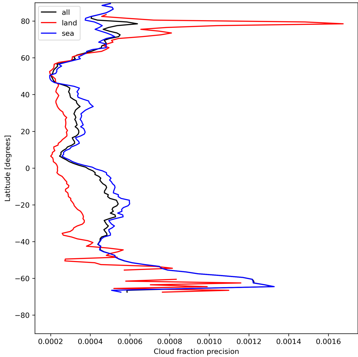
Figure 16: Zonal average of “Cloud fraction precision” for 2023-07-21 to 2023-07-23.
