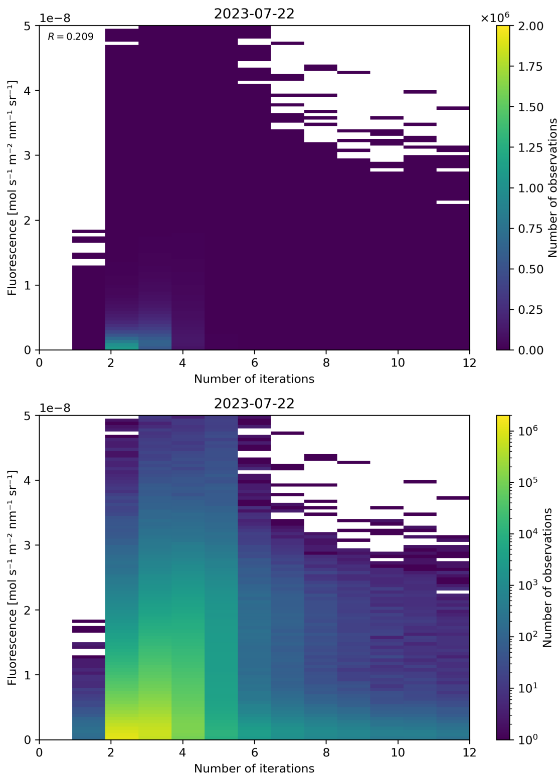
Figure 107: Scatter density plot of “Number of iterations” against “Fluorescence” for 2023-07-21 to 2023-07-23.
