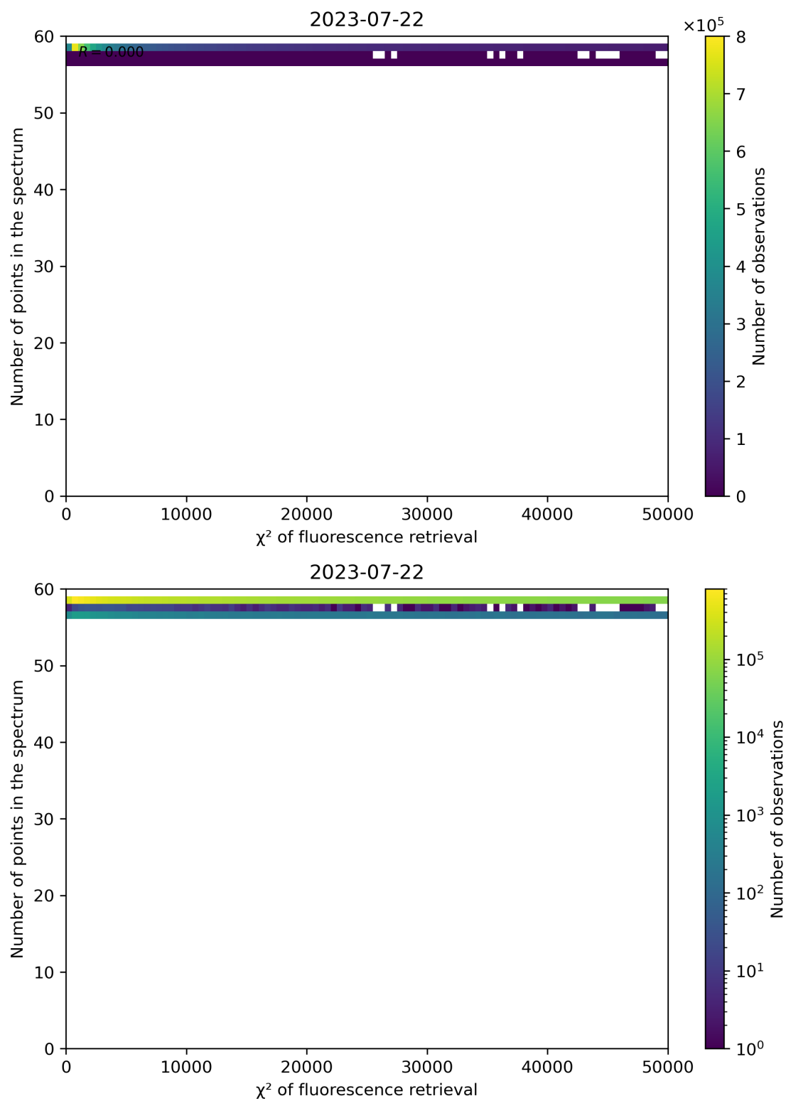
Figure 71: Scatter density plot of “ \chi^2 of fluorescence retrieval” against “Number of points in the spectrum” for 2023-07-21 to 2023-07-23.
