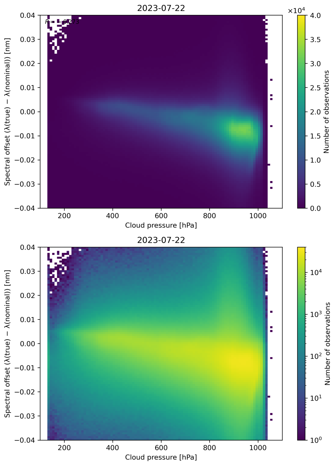
Figure 92: Scatter density plot of “Cloud pressure” against “Spectral offset ( \lambda(\text{true}) - \lambda(\text{nominal}) )” for 2023-07-21 to 2023-07-23.
