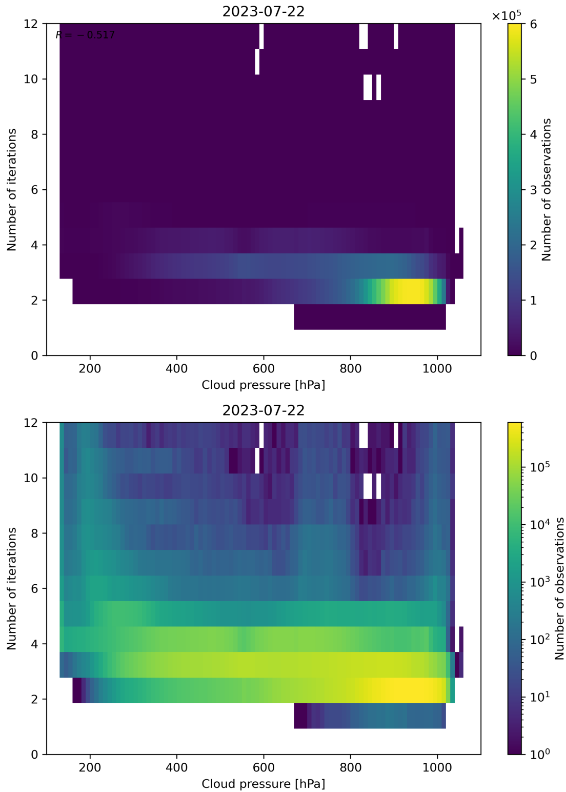
Figure 89: Scatter density plot of “Cloud pressure” against “Number of iterations” for 2023-07-21 to 2023-07-23.
