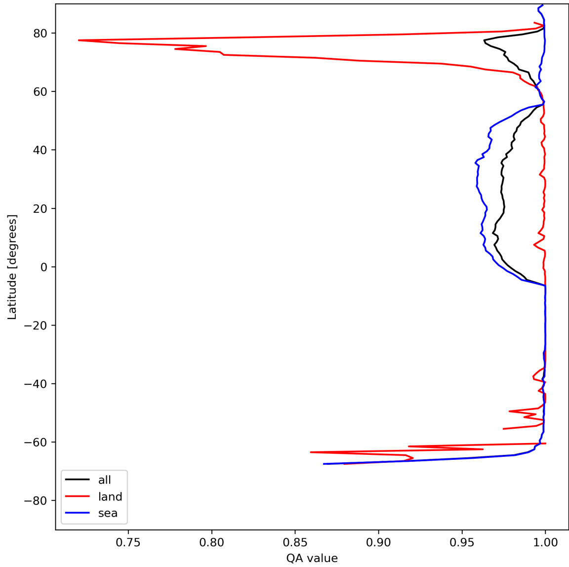
Figure 12: Zonal average of “QA value” for 2023-07-21 to 2023-07-23.
