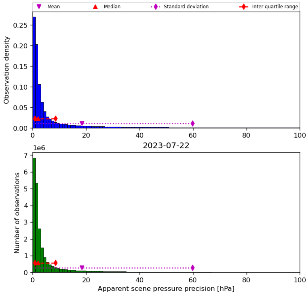
Figure 37: Histogram of “Apparent scene pressure precision” for 2023-07-21 to 2023-07-23
