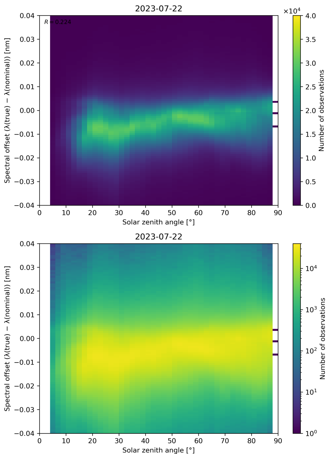
Figure 128: Scatter density plot of “Solar zenith angle” against “Spectral offset ( \lambda(\text{true}) - \lambda(\text{nominal}) )” for 2023-07-21 to 2023-07-23.
