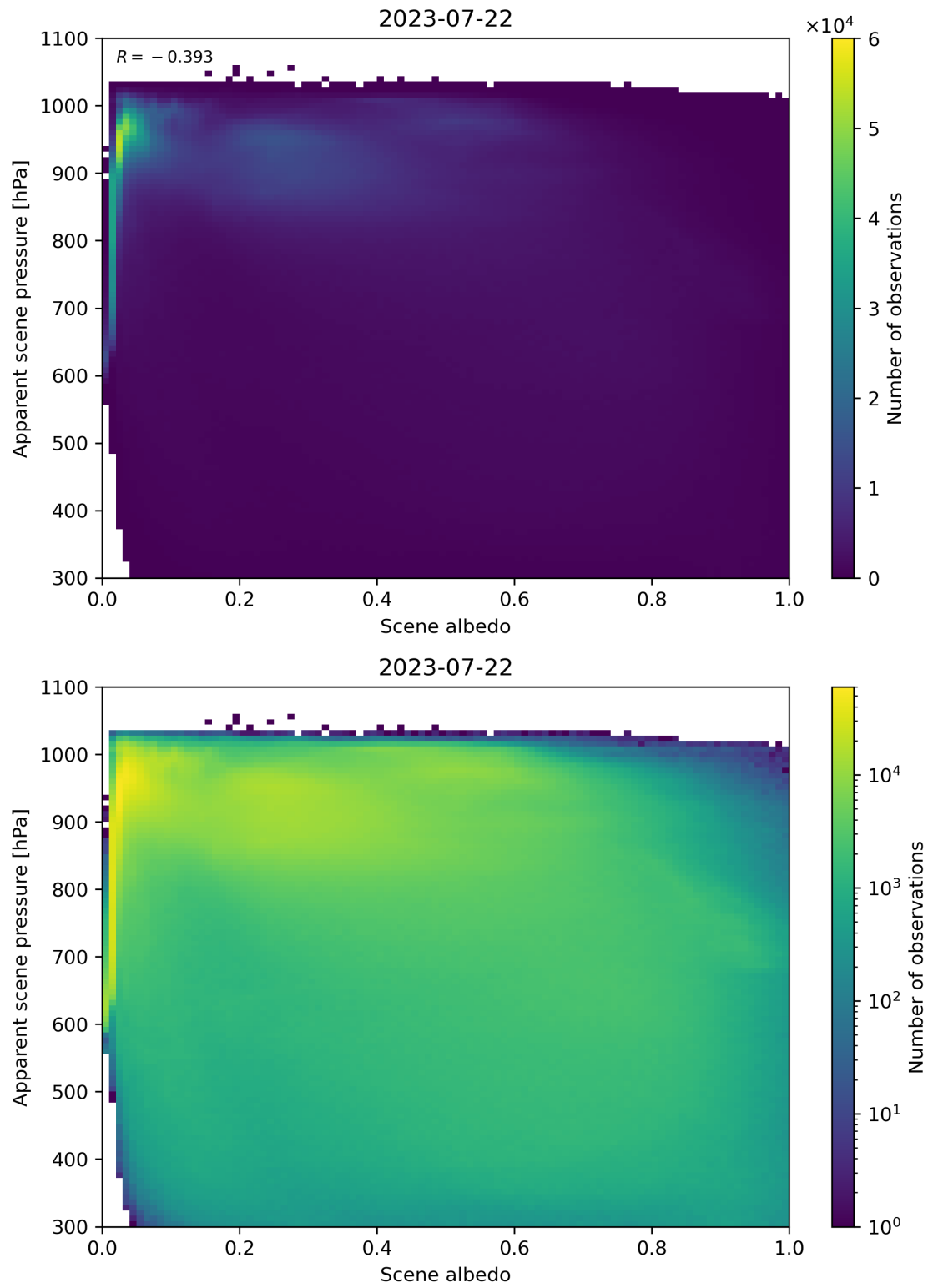
Figure 111: Scatter density plot of “Scene albedo” against “Apparent scene pressure” for 2023-07-21 to 2023-07-23.
