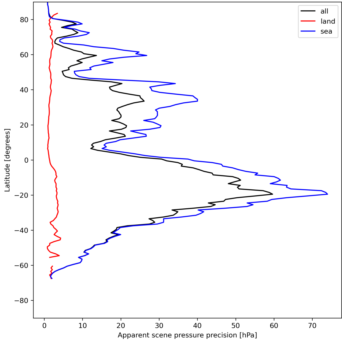
Figure 20: Zonal average of “Apparent scene pressure precision” for 2023-07-21 to 2023-07-23.
