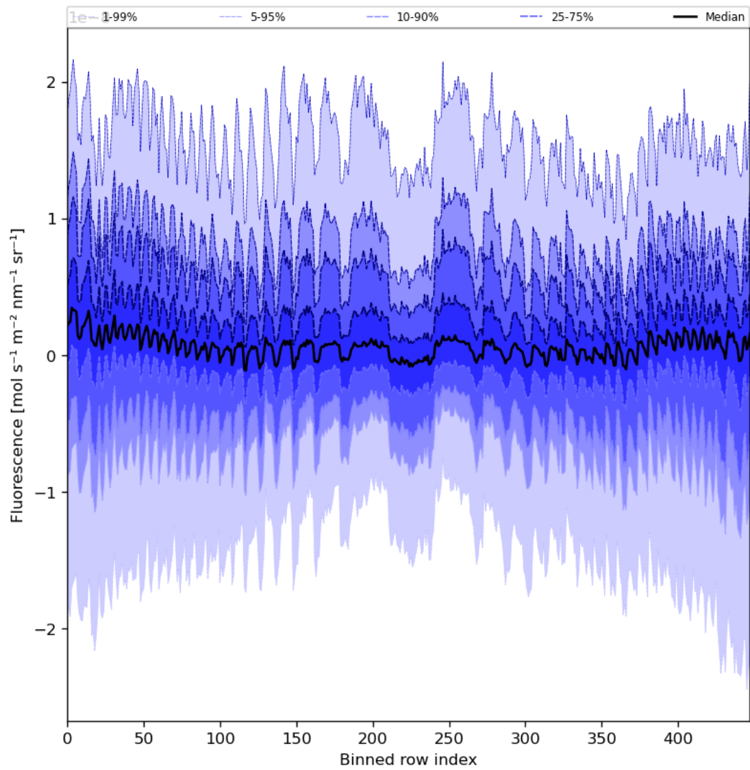
Figure 57: Along track statistics of “Fluorescence” for 2023-07-21 to 2023-07-23
