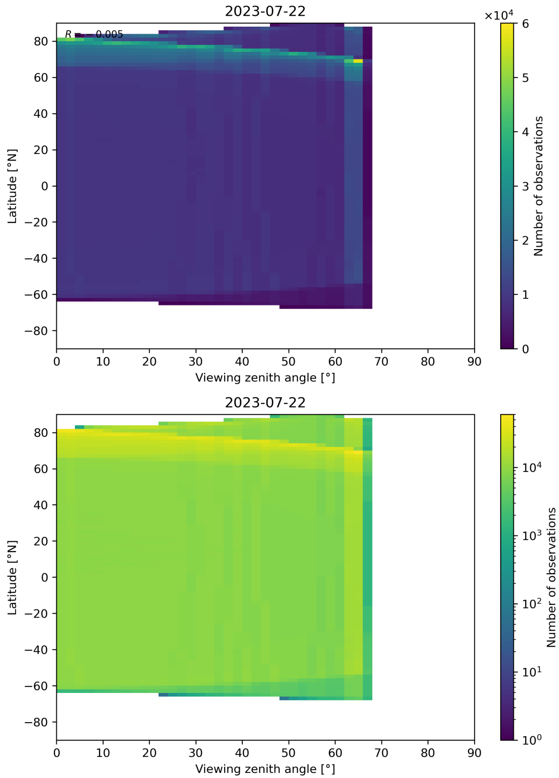
Figure 135: Scatter density plot of “Viewing zenith angle” against “Latitude” for 2023-07-21 to 2023-07-23.
