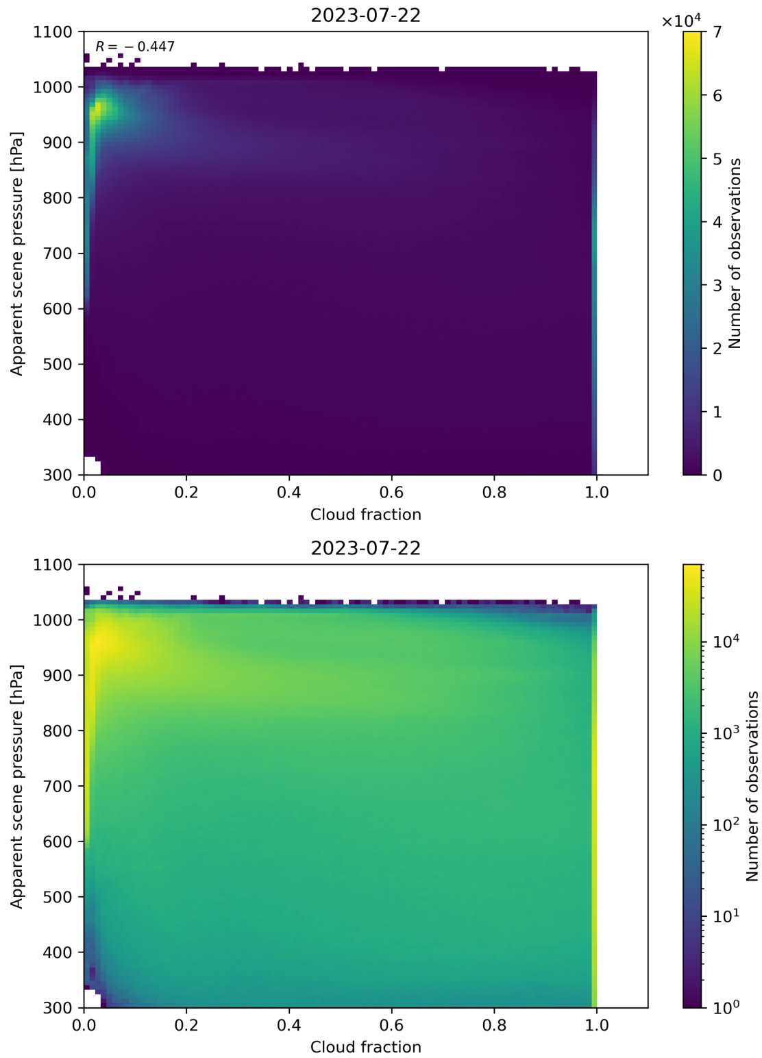
Figure 76: Scatter density plot of “Cloud fraction” against “Apparent scene pressure” for 2023-07-21 to 2023-07-23.
