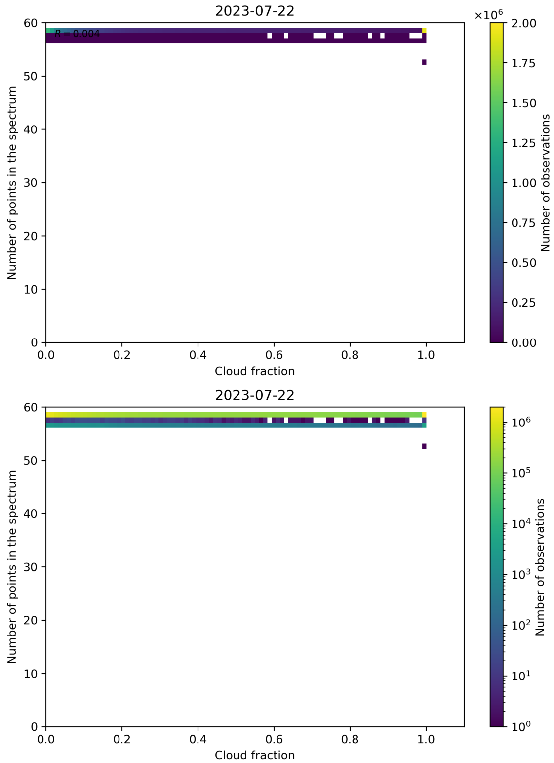
Figure 81: Scatter density plot of “Cloud fraction” against “Number of points in the spectrum” for 2023-07-21 to 2023-07-23.
