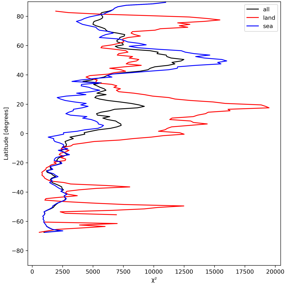
Figure 21: Zonal average of “ \chi^2 ” for 2023-07-21 to 2023-07-23.
