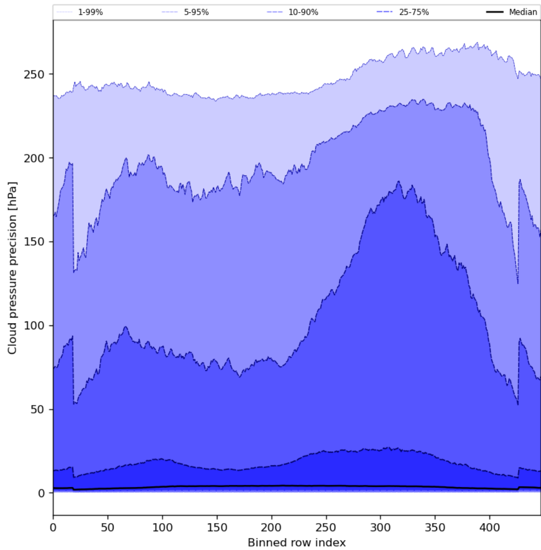
Figure 48: Along track statistics of “Cloud pressure precision” for 2023-07-21 to 2023-07-23
