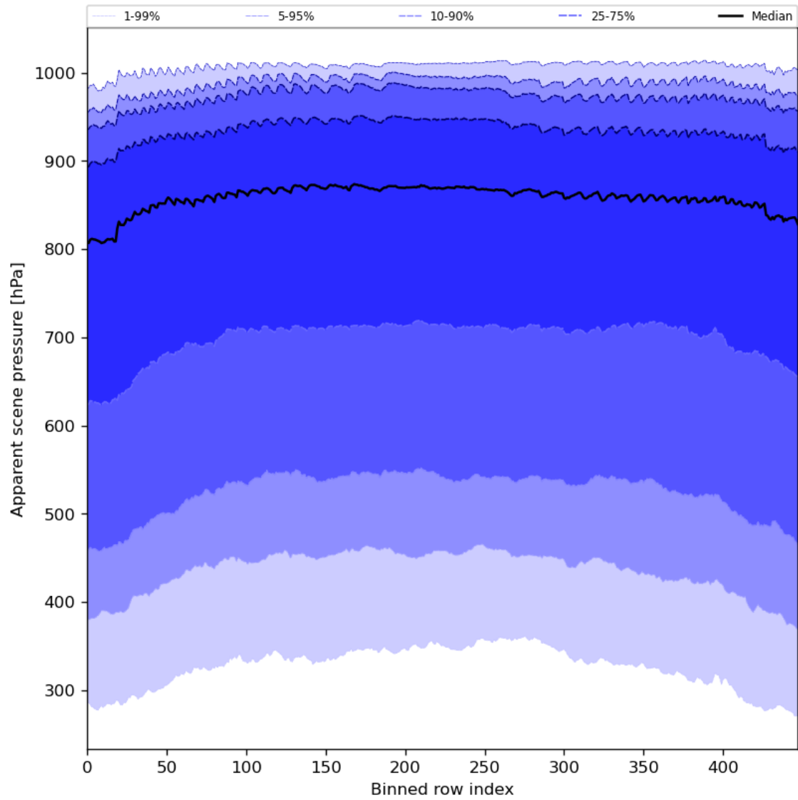
Figure 53: Along track statistics of “Apparent scene pressure” for 2023-07-21 to 2023-07-23
