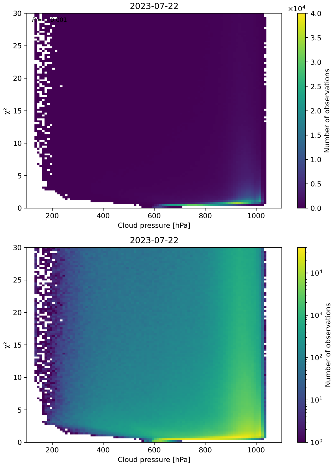
Figure 85: Scatter density plot of “Cloud pressure” against “ \chi^2 ” for 2023-07-21 to 2023-07-23.
