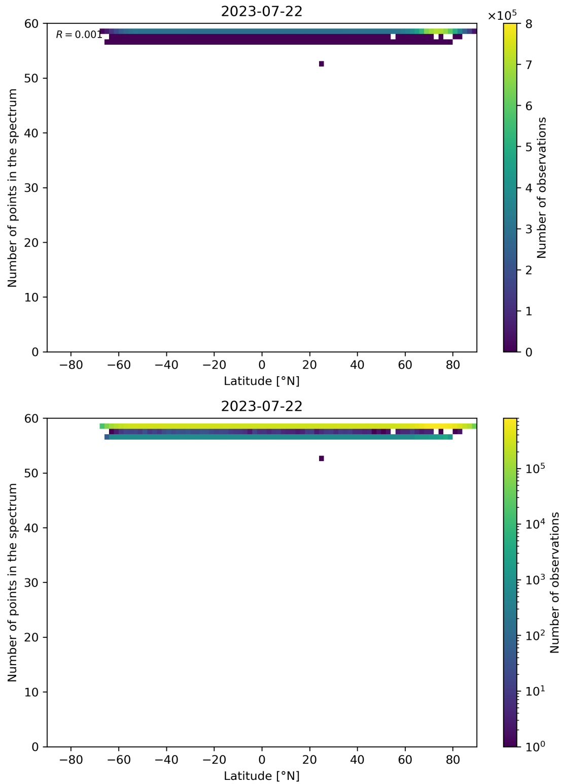
Figure 103: Scatter density plot of “Latitude” against “Number of points in the spectrum” for 2023-07-21 to 2023-07-23.
