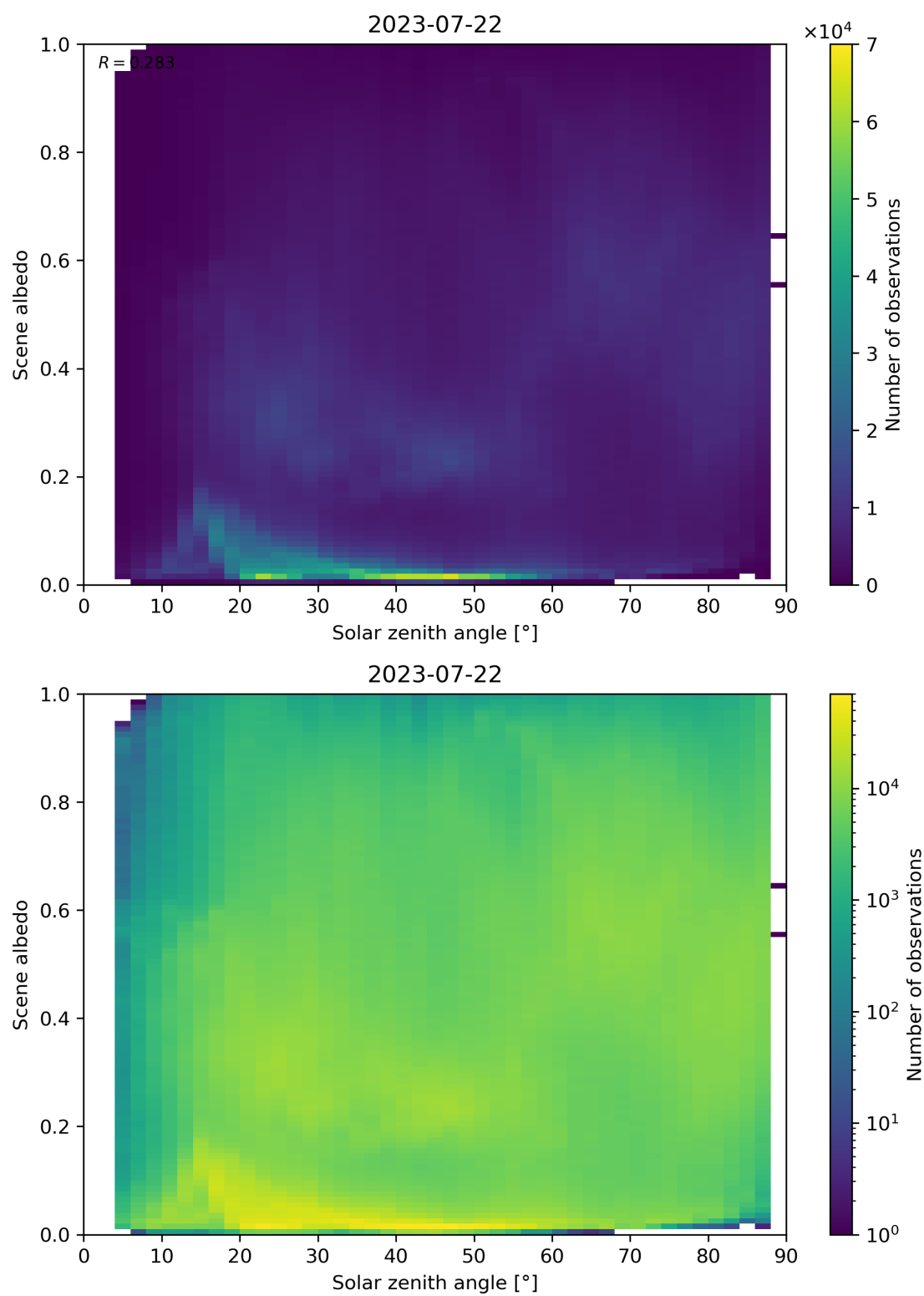
Figure 127: Scatter density plot of “Solar zenith angle” against “Scene albedo” for 2023-07-21 to 2023-07-23.
