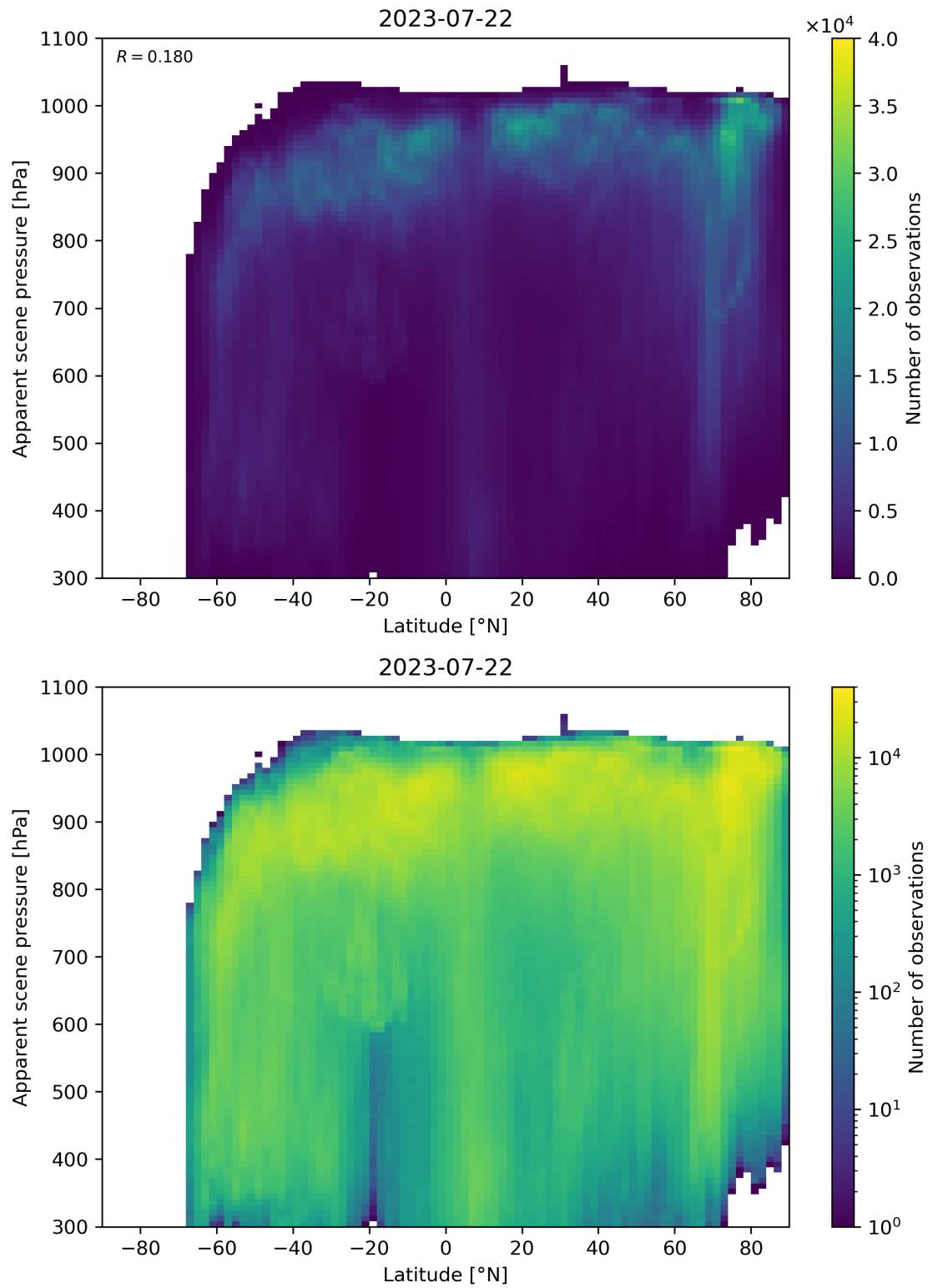
Figure 96: Scatter density plot of “Latitude” against “Apparent scene pressure” for 2023-07-21 to 2023-07-23.
