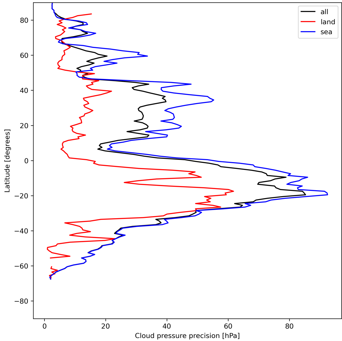
Figure 14: Zonal average of “Cloud pressure precision” for 2023-07-21 to 2023-07-23.
