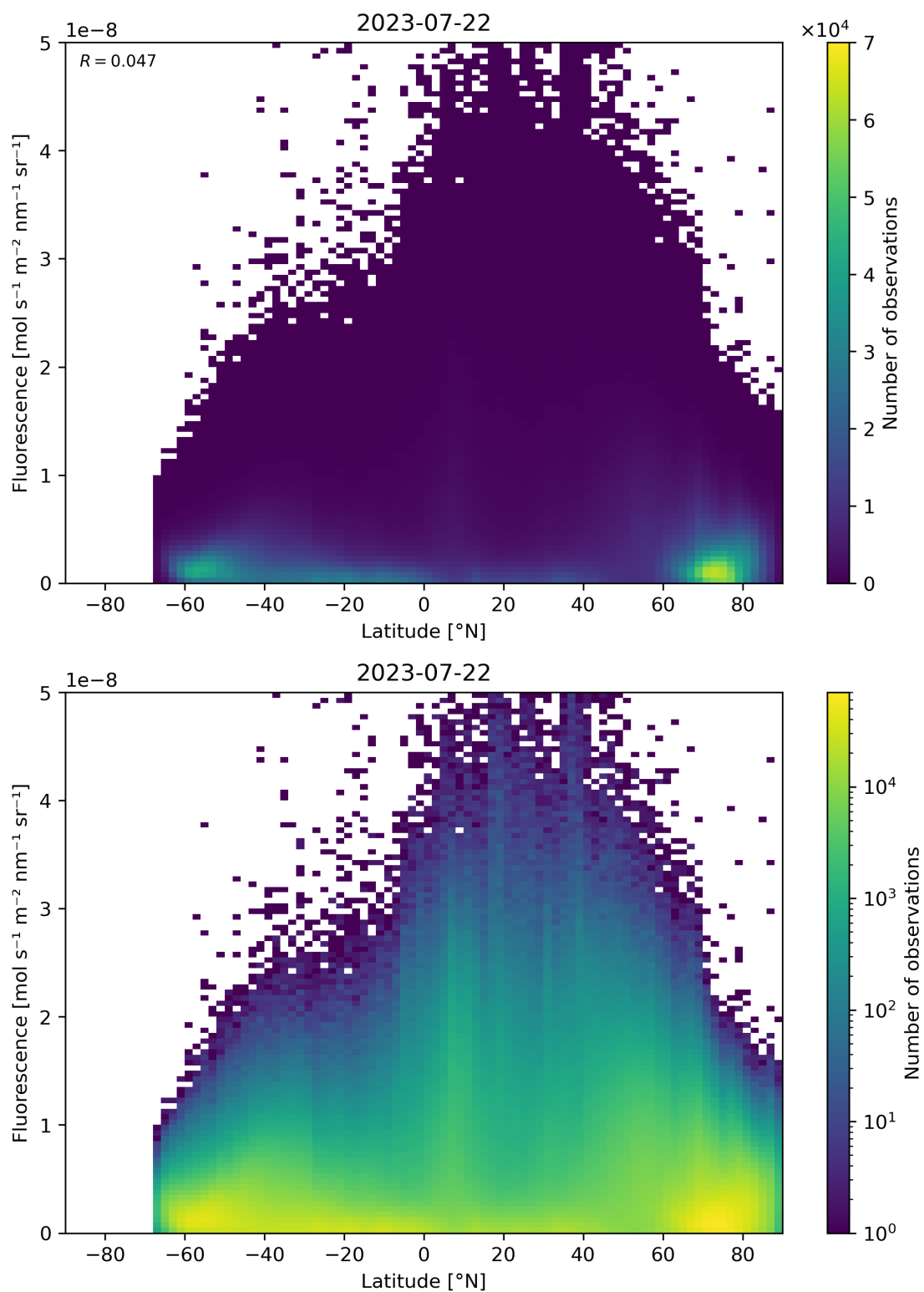
Figure 101: Scatter density plot of “Latitude” against “Fluorescence” for 2023-07-21 to 2023-07-23.
