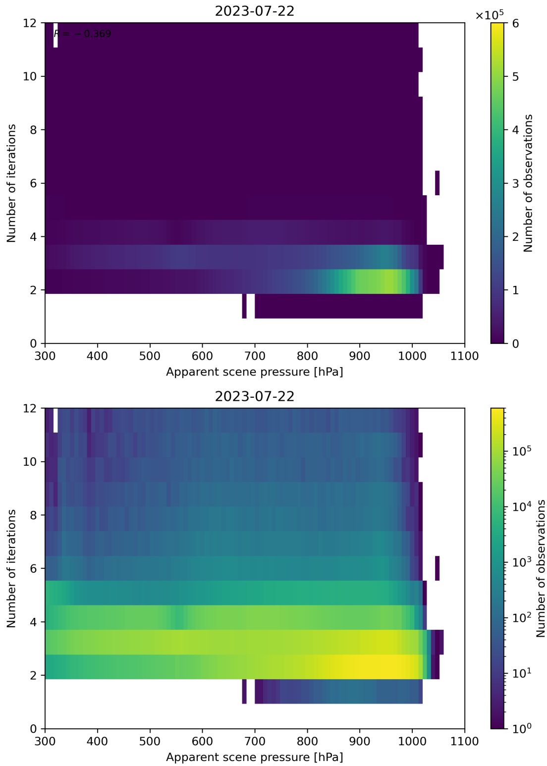
Figure 66: Scatter density plot of “Apparent scene pressure” against “Number of iterations” for 2023-07-21 to 2023-07-23.
