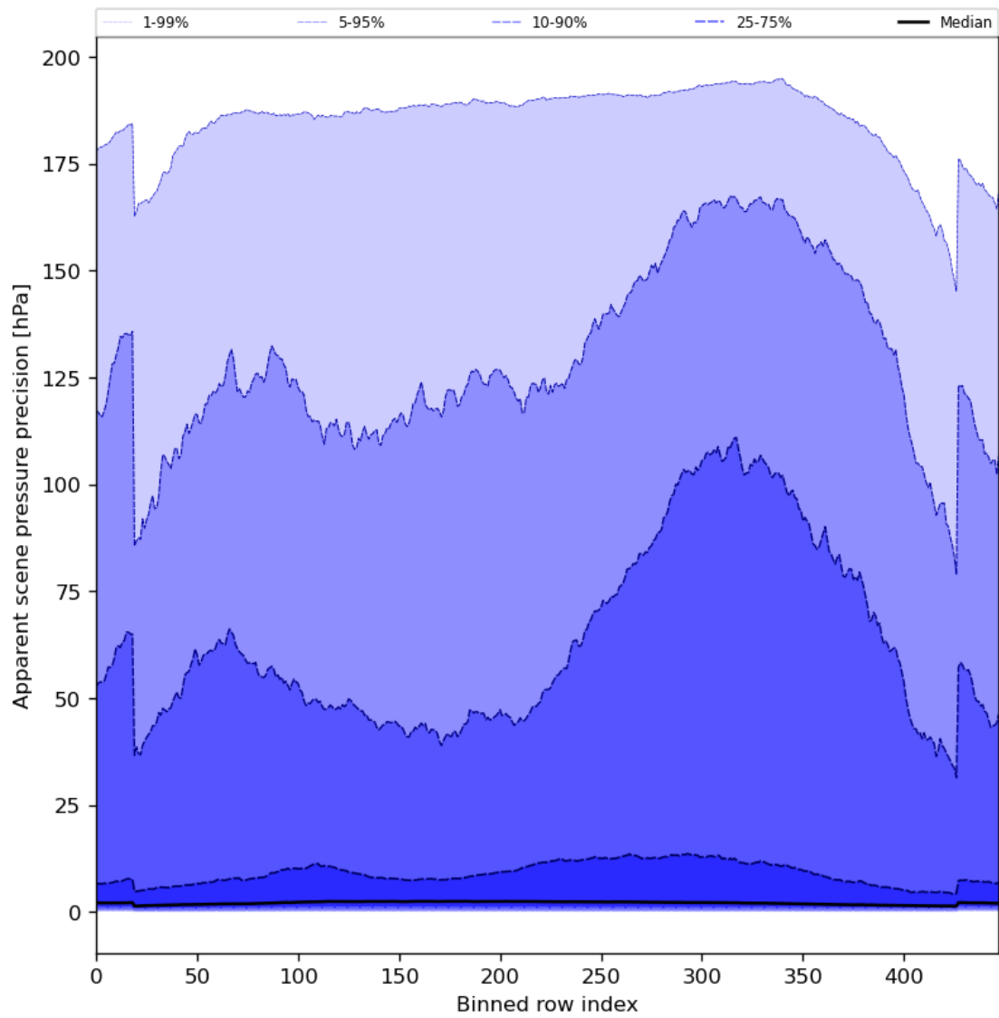
Figure 54: Along track statistics of “Apparent scene pressure precision” for 2023-07-21 to 2023-07-23
