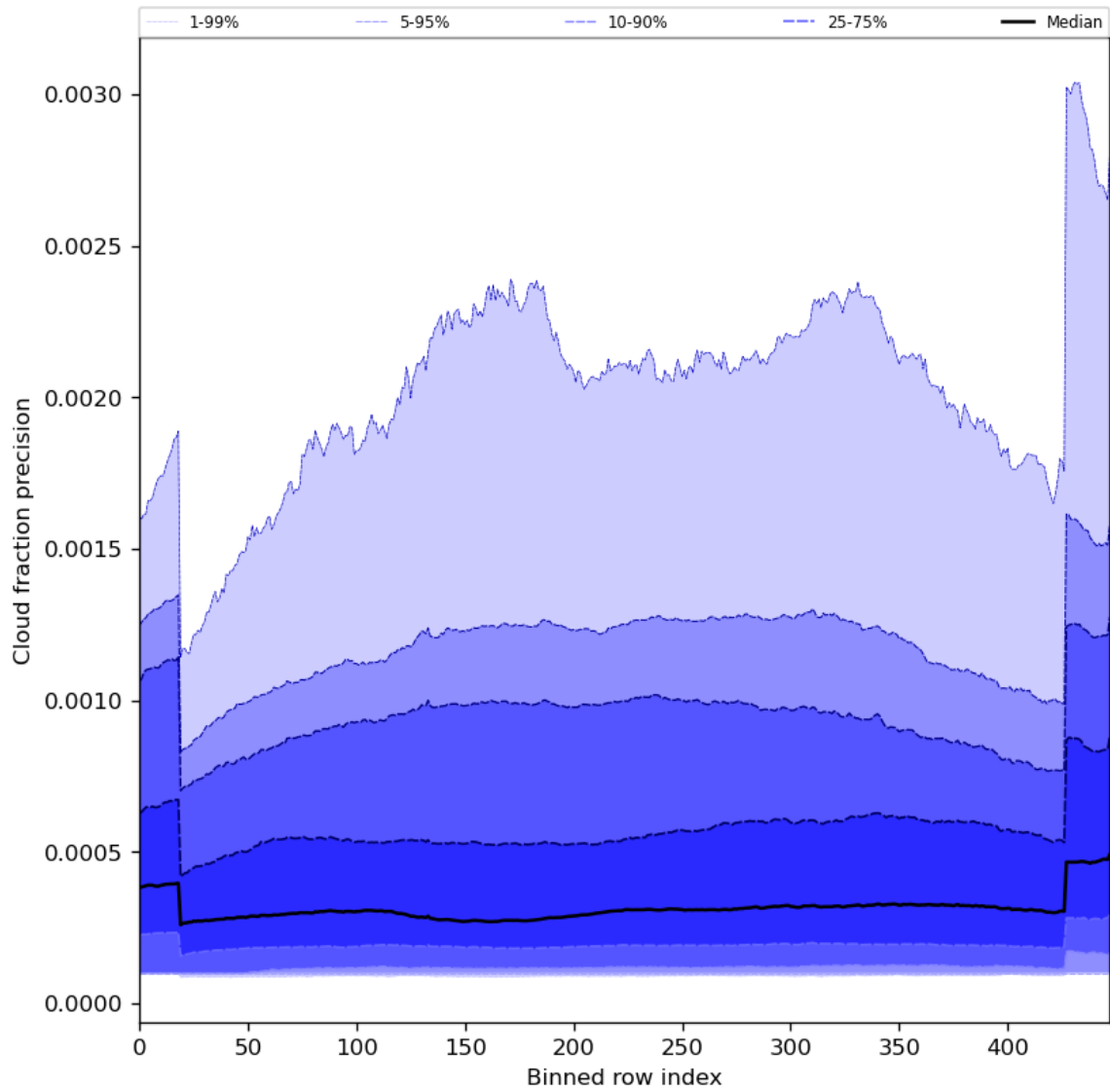
Figure 50: Along track statistics of “Cloud fraction precision” for 2023-07-22 to 2023-07-24
