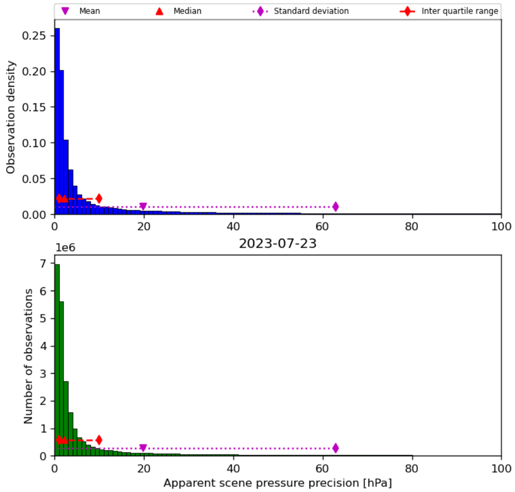
Figure 37: Histogram of “Apparent scene pressure precision” for 2023-07-22 to 2023-07-24
