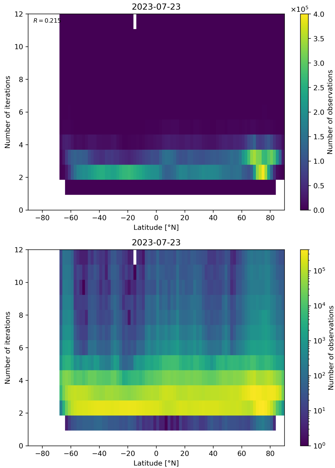
Figure 102: Scatter density plot of “Latitude” against “Number of iterations” for 2023-07-22 to 2023-07-24.
