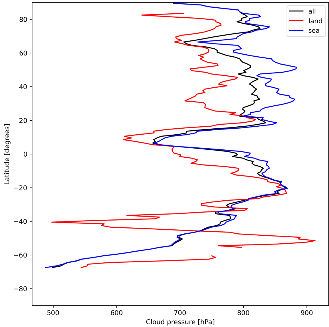
Figure 13: Zonal average of “Cloud pressure” for 2023-07-22 to 2023-07-24.
