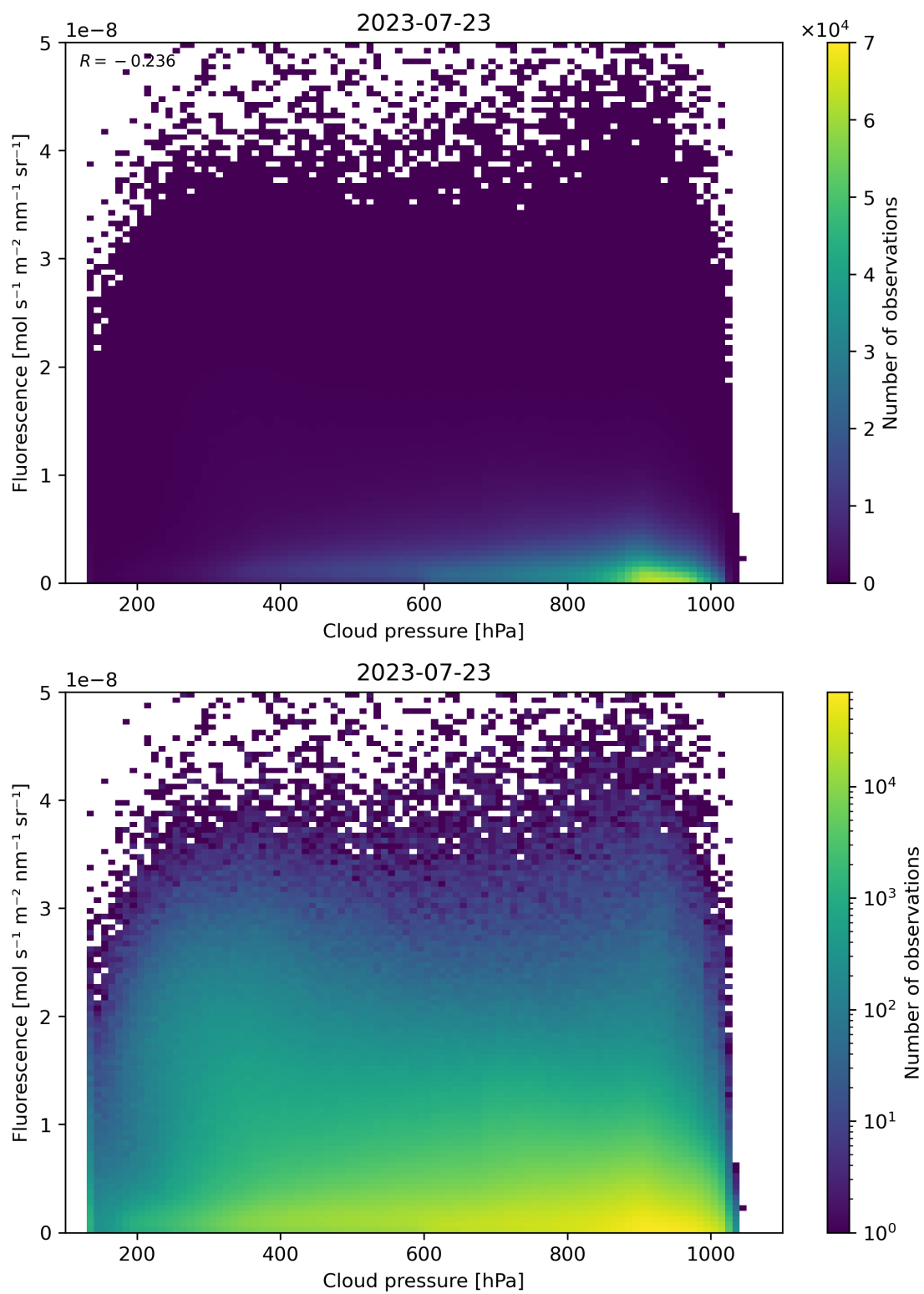
Figure 88: Scatter density plot of “Cloud pressure” against “Fluorescence” for 2023-07-22 to 2023-07-24.
