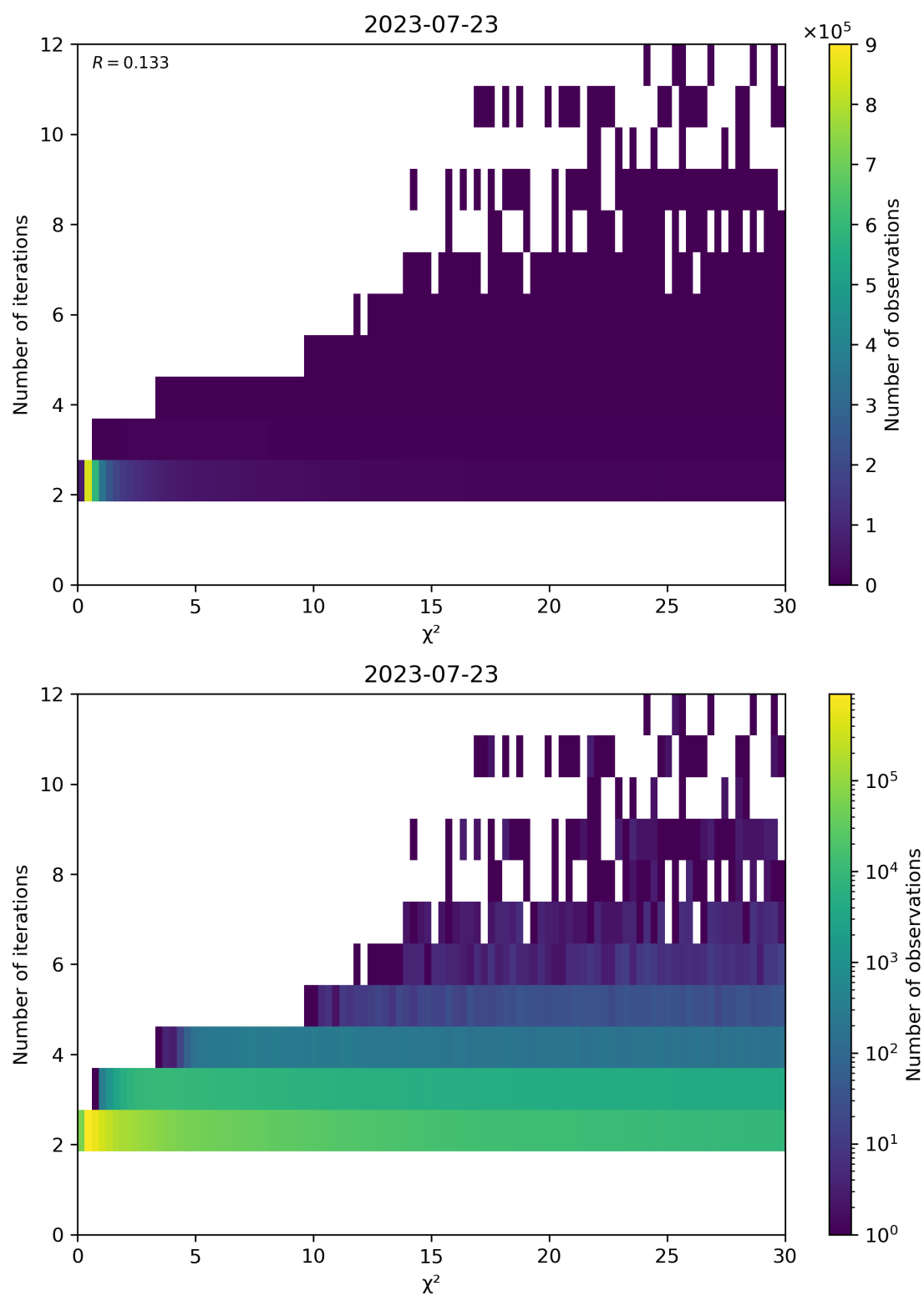
Figure 73: Scatter density plot of “ \chi^2 ” against “Number of iterations” for 2023-07-22 to 2023-07-24.
