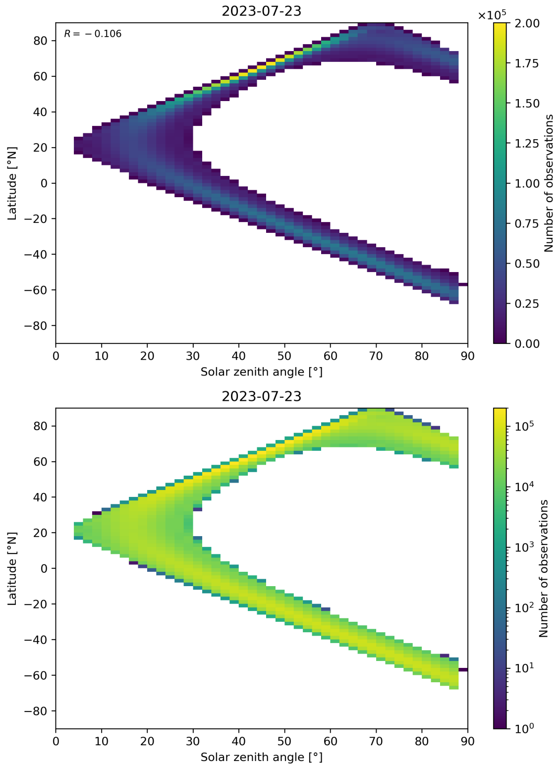
Figure 124: Scatter density plot of “Solar zenith angle” against “Latitude” for 2023-07-22 to 2023-07-24.
