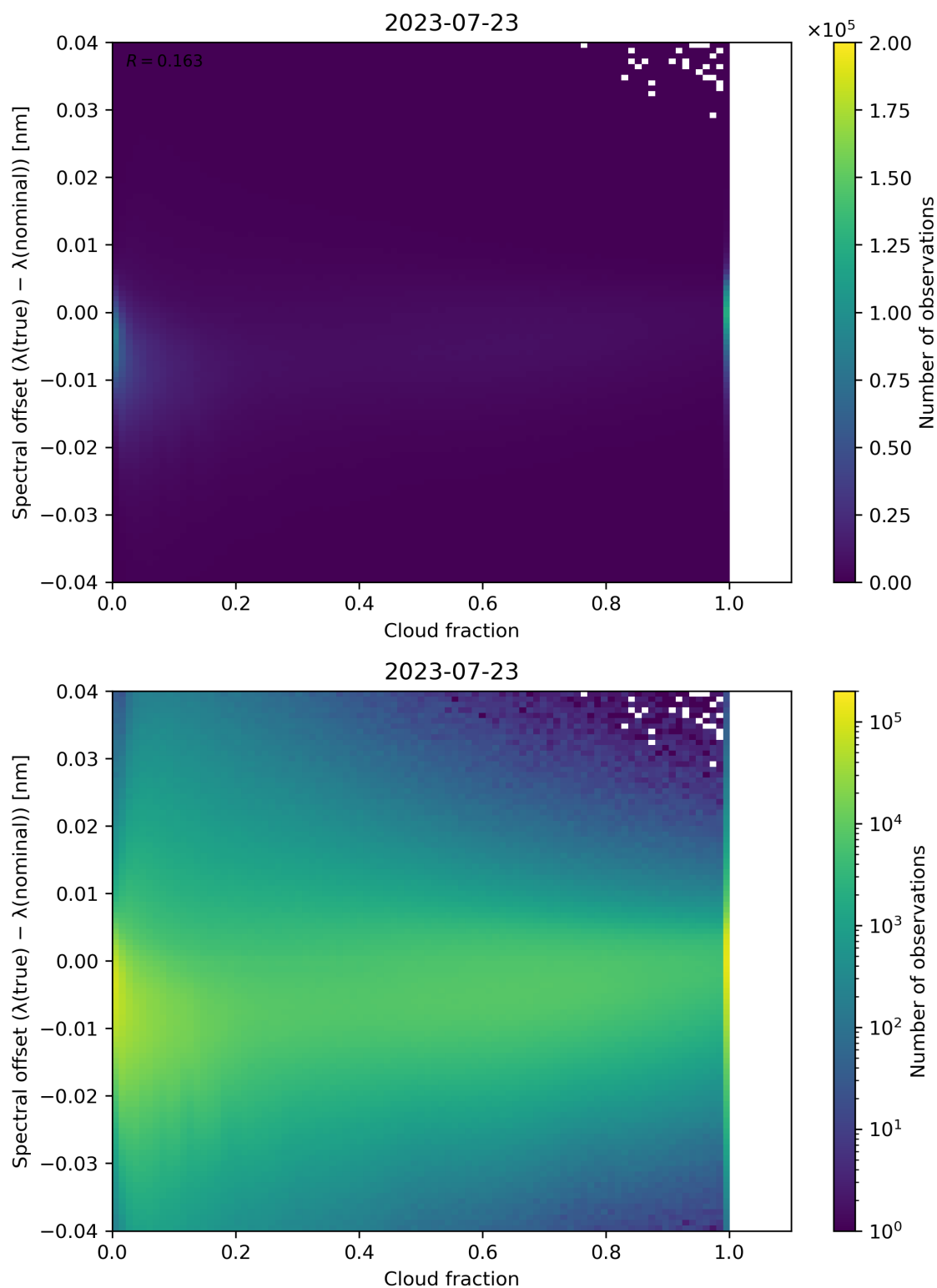
Figure 83: Scatter density plot of “Cloud fraction” against “Spectral offset ( \lambda(\text{true}) - \lambda(\text{nominal}) )” for 2023-07-22 to 2023-07-24.
