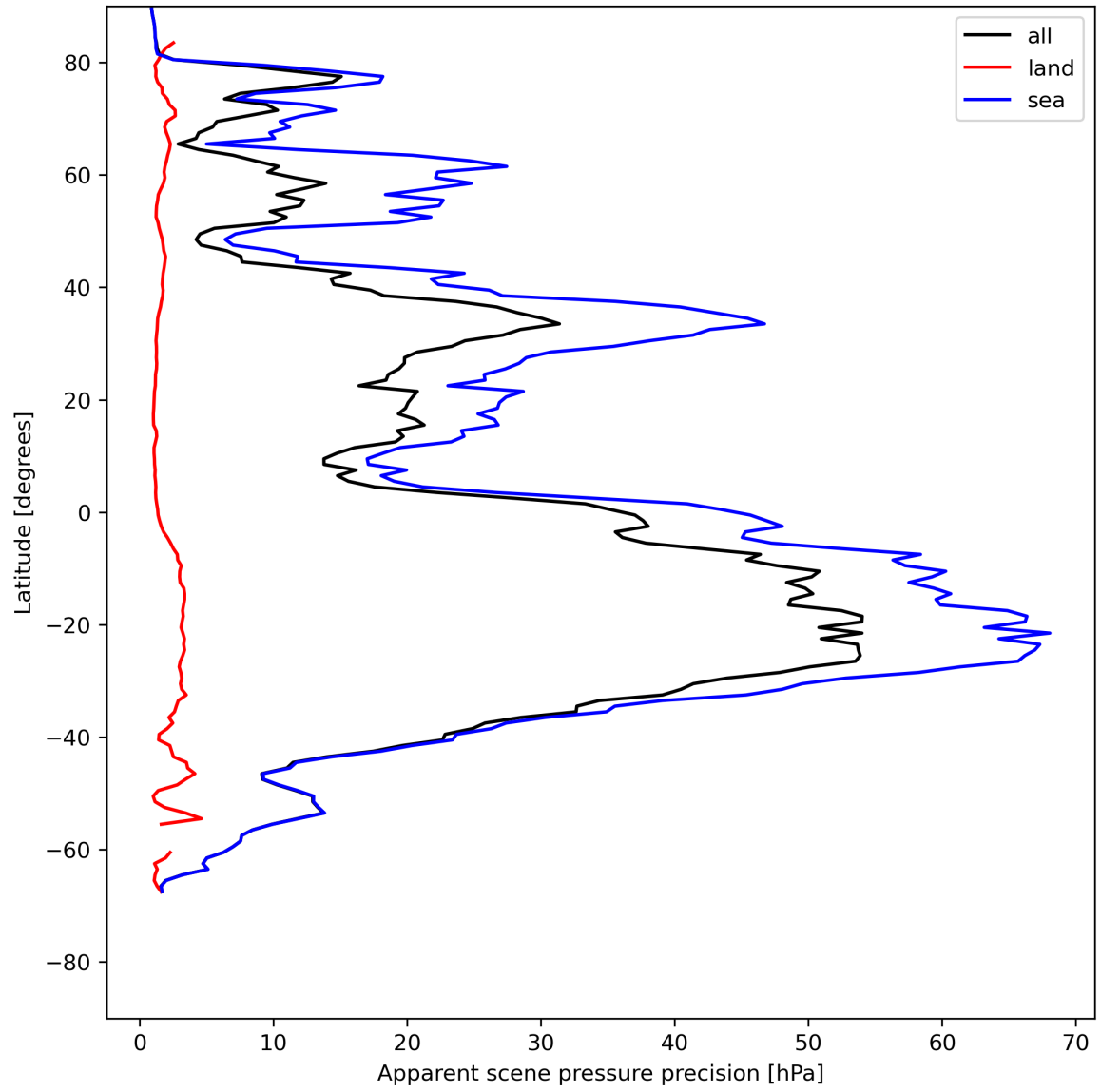
Figure 20: Zonal average of “Apparent scene pressure precision” for 2023-07-22 to 2023-07-24.
