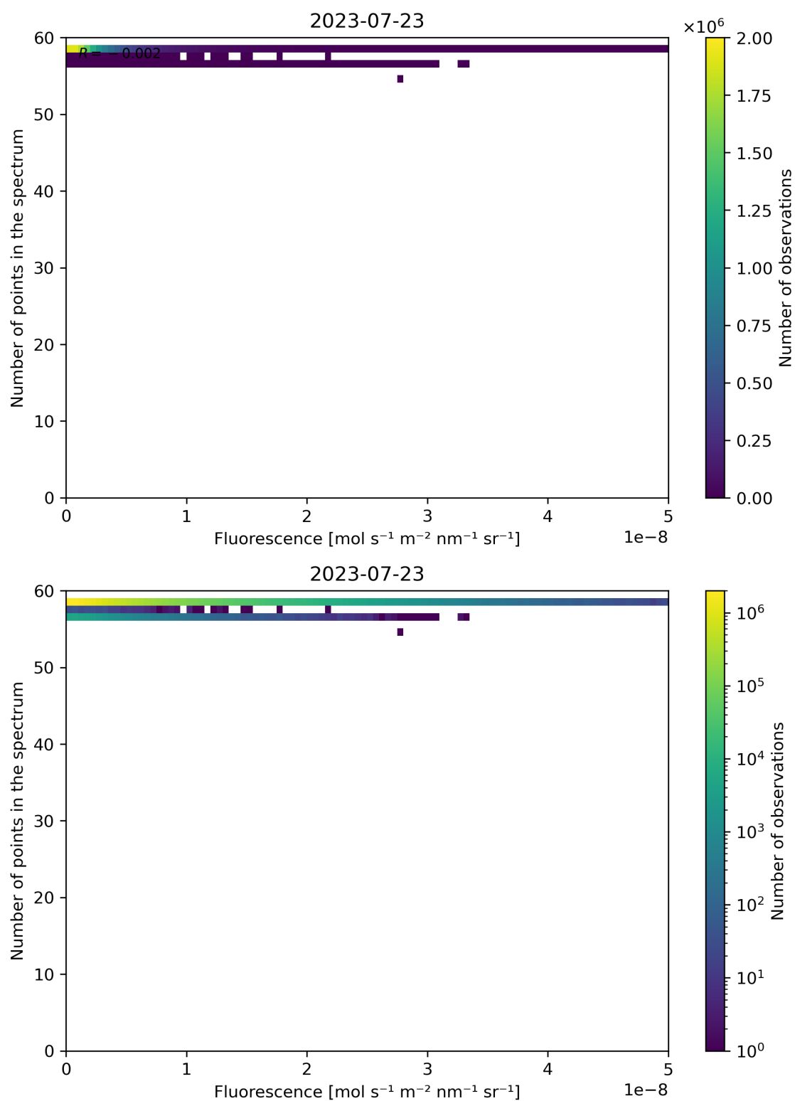
Figure 94: Scatter density plot of “Fluorescence” against “Number of points in the spectrum” for 2023-07-22 to 2023-07-24.
