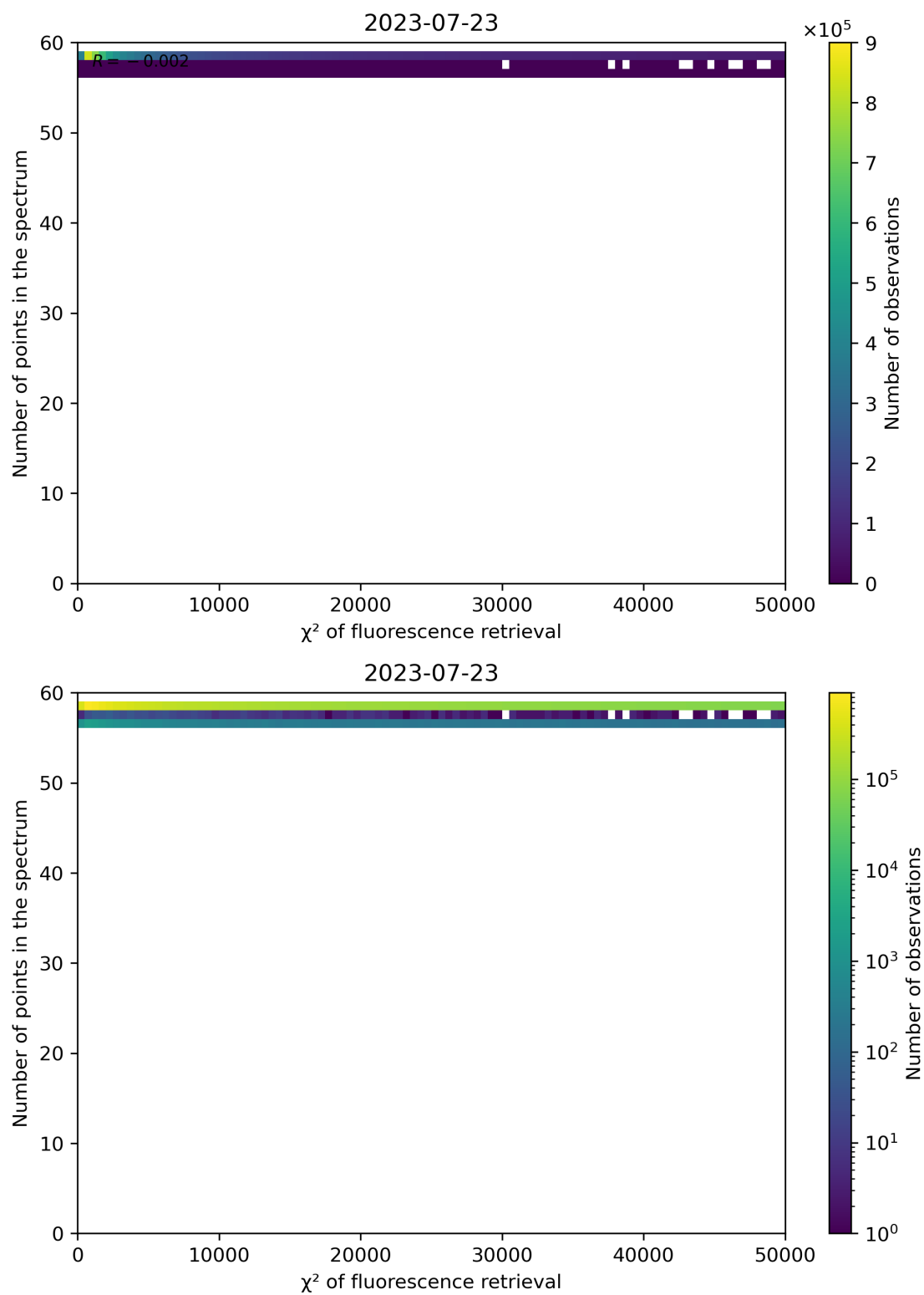
Figure 71: Scatter density plot of " \chi^2 of fluorescence retrieval" against "Number of points in the spectrum" for 2023-07-22 to 2023-07-24.
