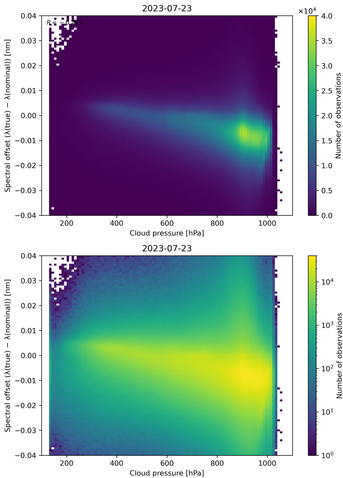
Figure 92: Scatter density plot of “Cloud pressure” against “Spectral offset ( \lambda(\text{true}) - \lambda(\text{nominal}) )” for 2023-07-22 to 2023-07-24.
