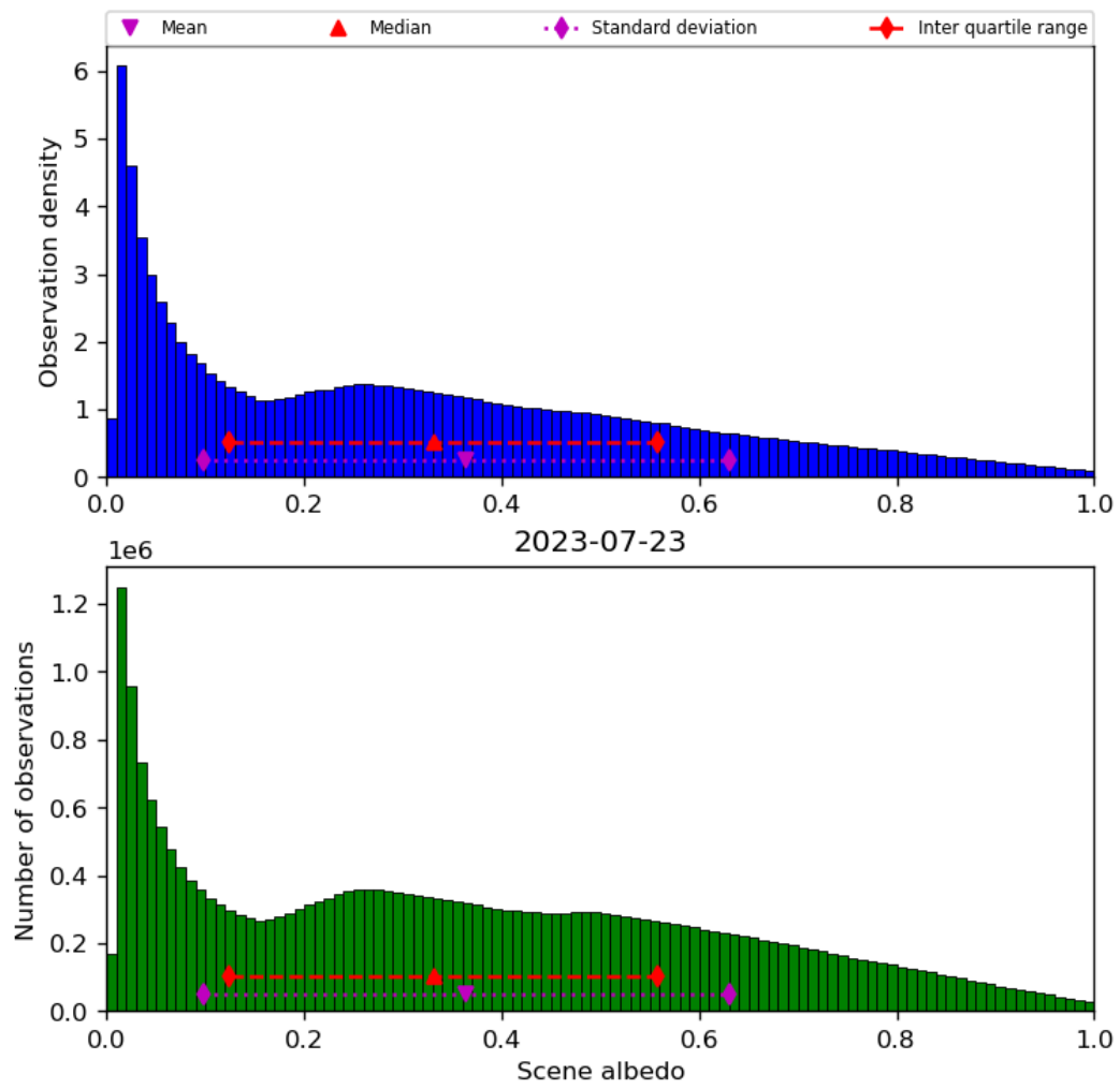
Figure 34: Histogram of “Scene albedo” for 2023-07-22 to 2023-07-24
