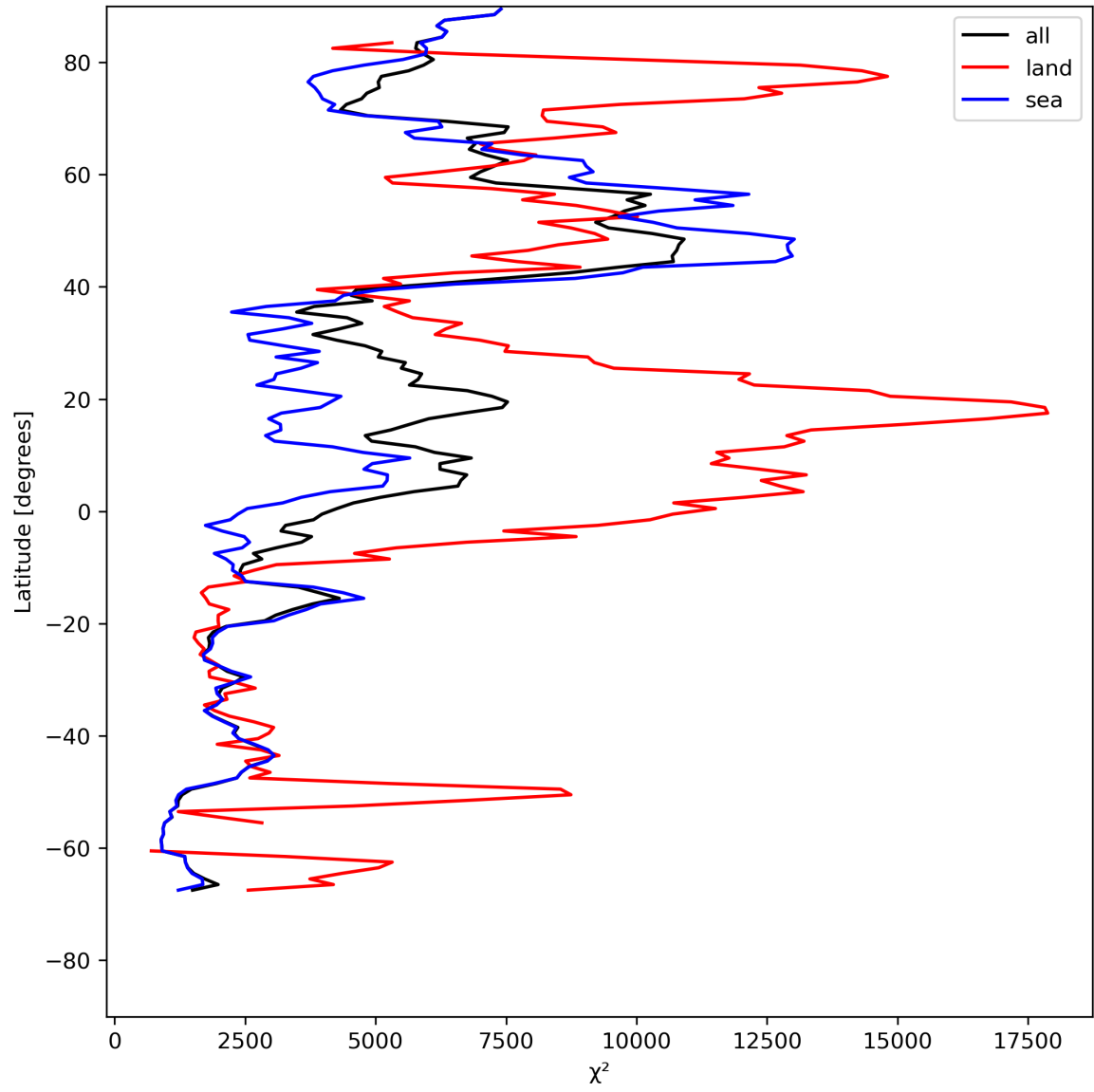
Figure 21: Zonal average of “ \chi^2 ” for 2023-07-22 to 2023-07-24.
