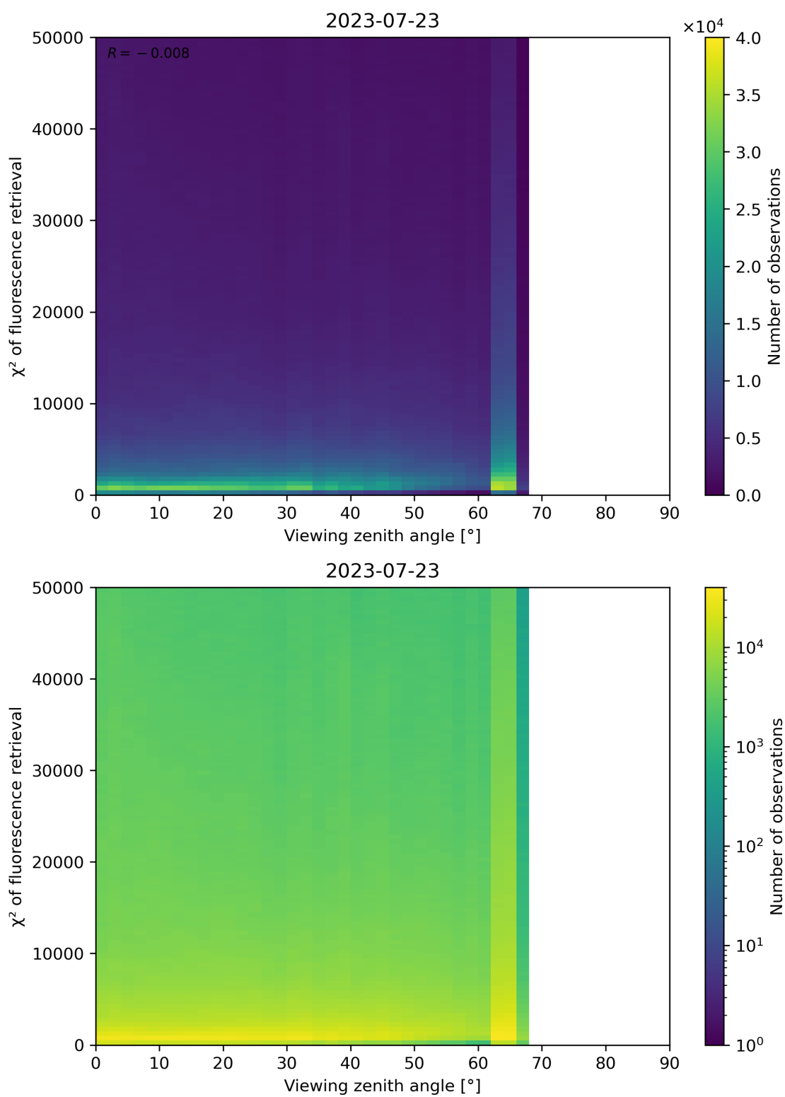
Figure 131: Scatter density plot of “Viewing zenith angle” against “ \chi^2 of fluorescence retrieval” for 2023-07-22 to 2023-07-24.
