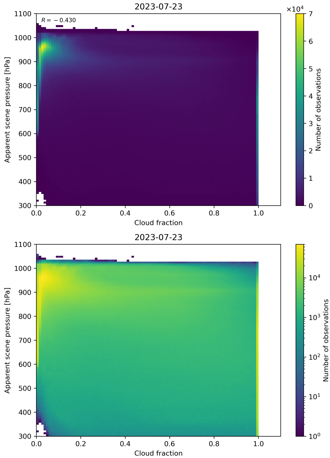
Figure 76: Scatter density plot of “Cloud fraction” against “Apparent scene pressure” for 2023-07-22 to 2023-07-24.
