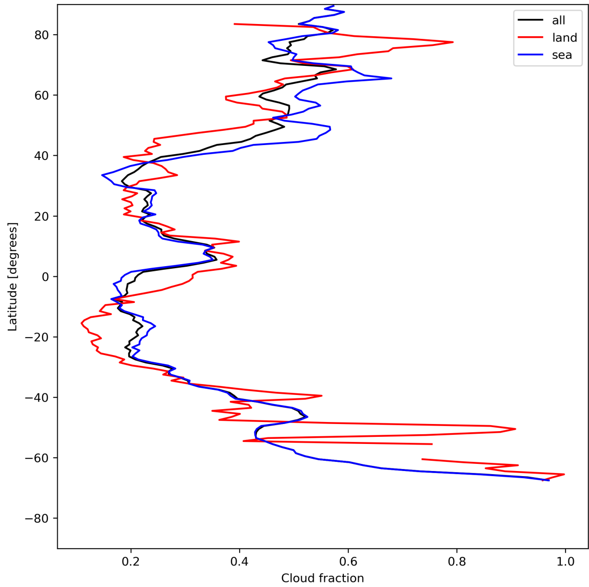
Figure 15: Zonal average of “Cloud fraction” for 2023-07-22 to 2023-07-24.
