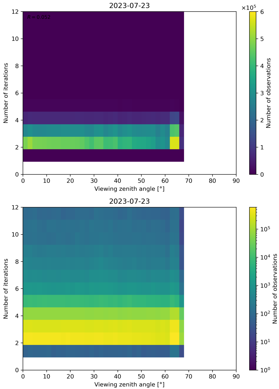
Figure 136: Scatter density plot of “Viewing zenith angle” against “Number of iterations” for 2023-07-22 to 2023-07-24.
