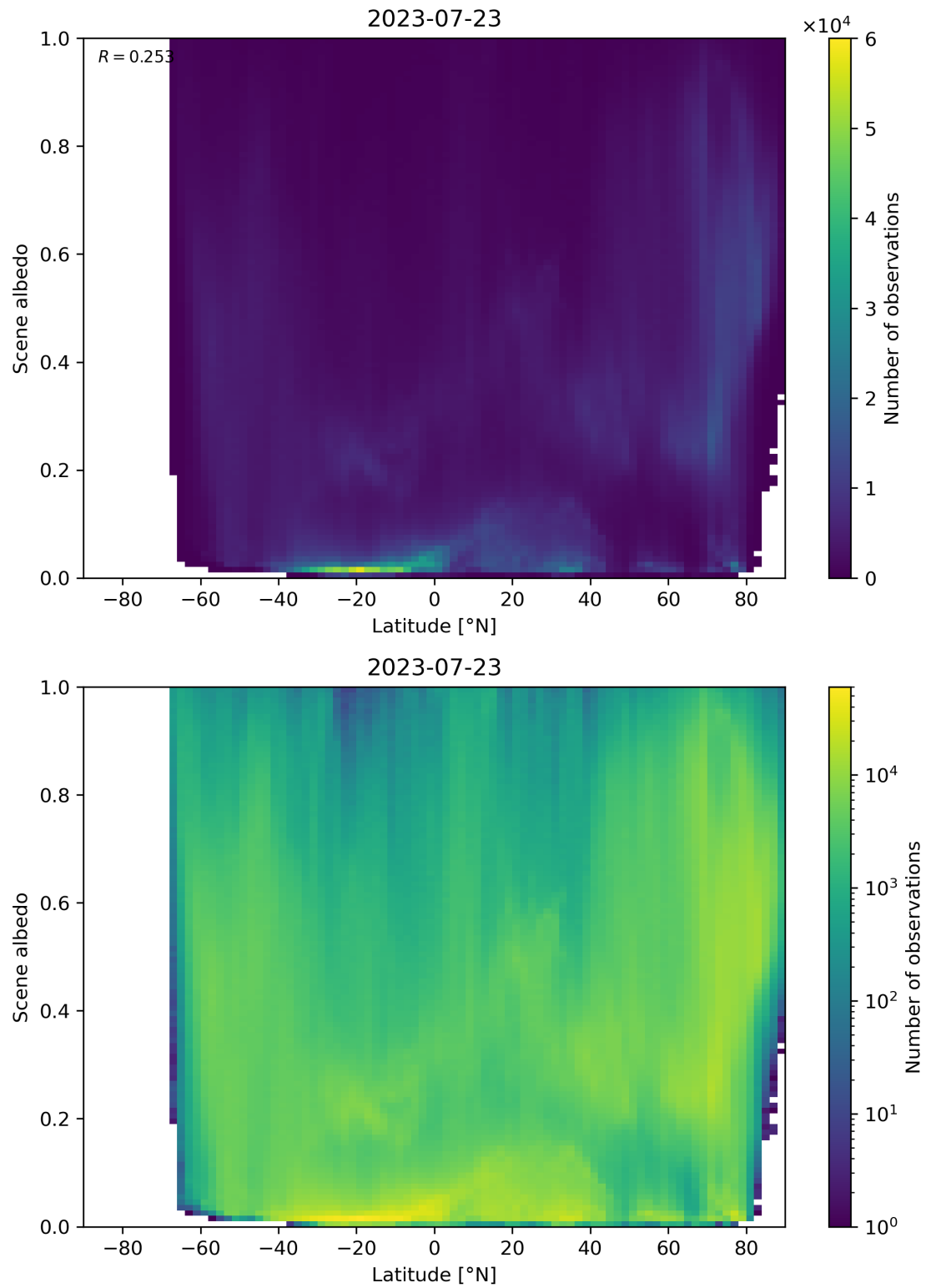
Figure 104: Scatter density plot of “Latitude” against “Scene albedo” for 2023-07-22 to 2023-07-24.
