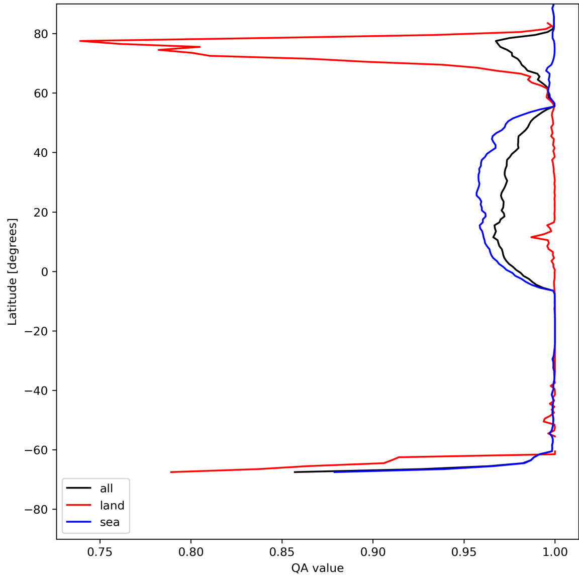
Figure 12: Zonal average of “QA value” for 2023-07-22 to 2023-07-24.
