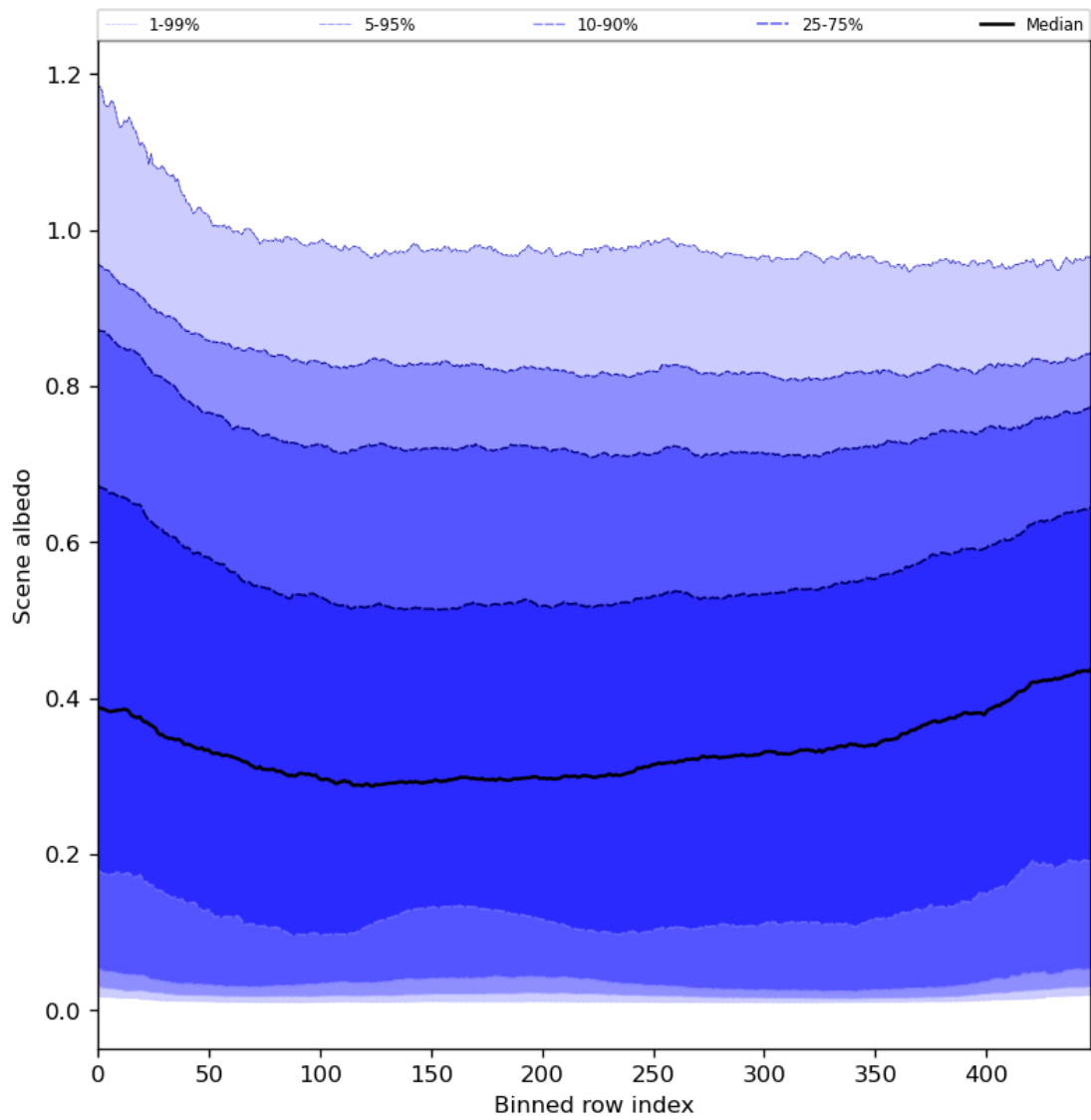
Figure 51: Along track statistics of “Scene albedo” for 2023-07-22 to 2023-07-24
