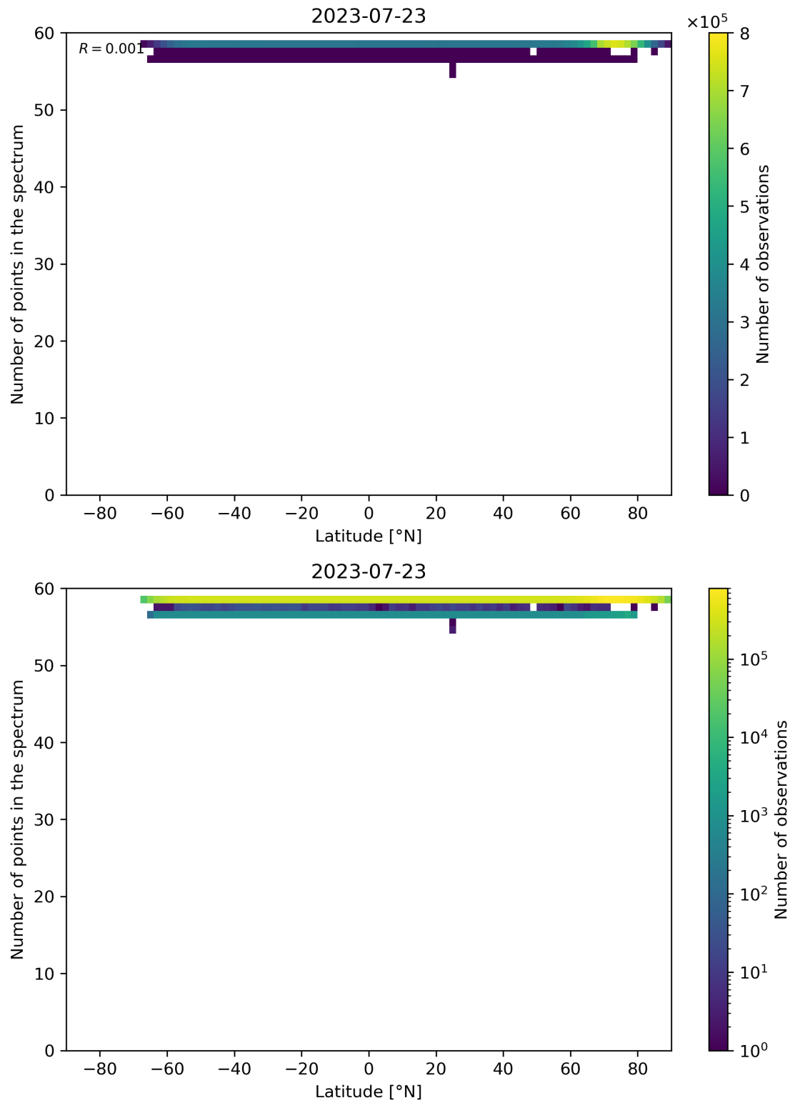
Figure 103: Scatter density plot of “Latitude” against “Number of points in the spectrum” for 2023-07-22 to 2023-07-24.
