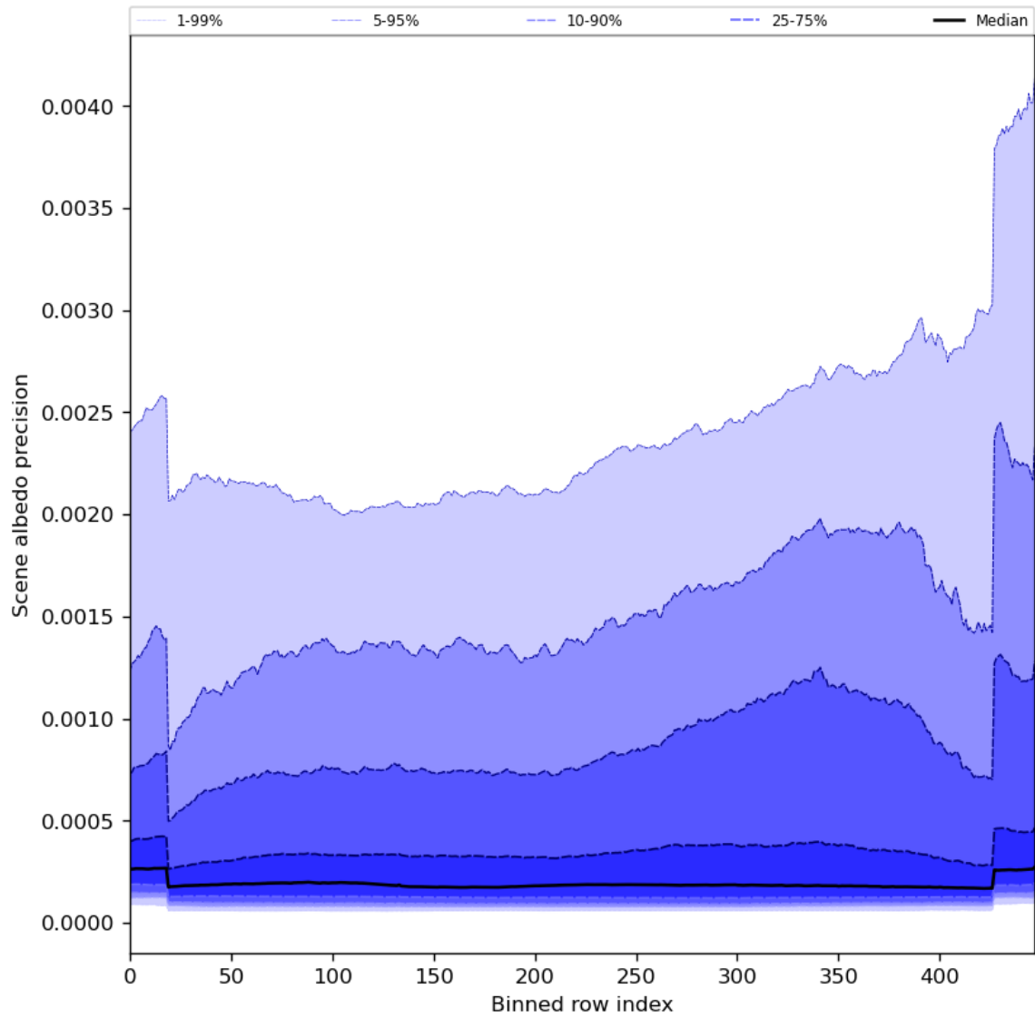
Figure 52: Along track statistics of “Scene albedo precision” for 2023-07-22 to 2023-07-24
