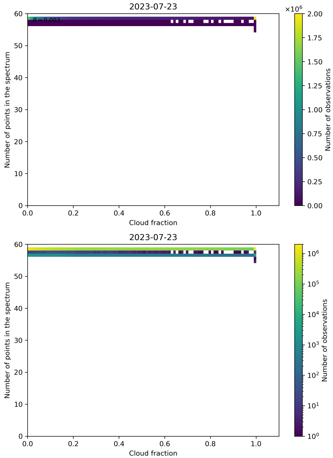
Figure 81: Scatter density plot of “Cloud fraction” against “Number of points in the spectrum” for 2023-07-22 to 2023-07-24.
