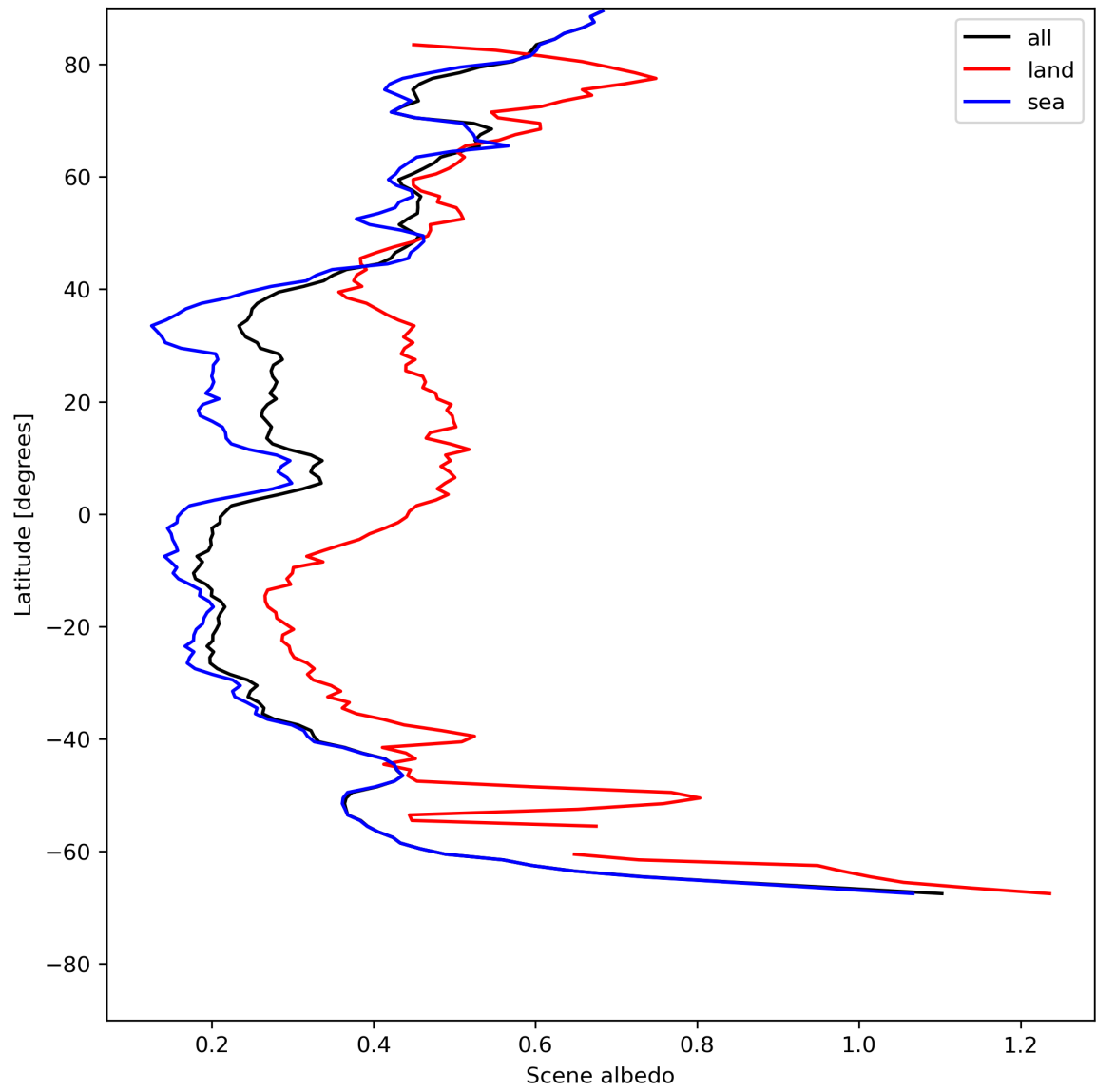
Figure 17: Zonal average of “Scene albedo” for 2023-07-22 to 2023-07-24.
