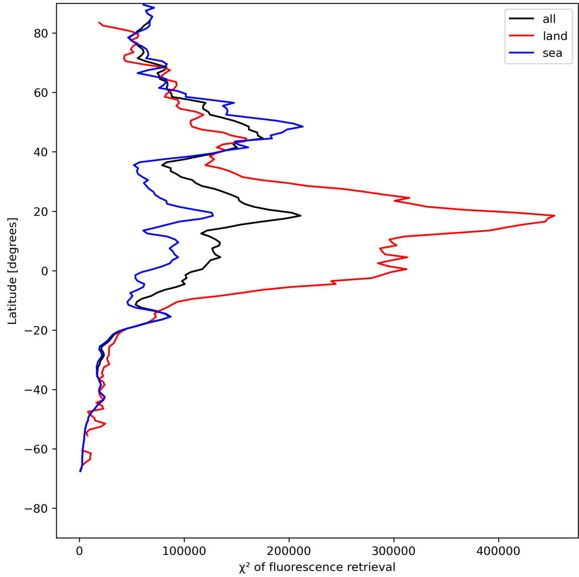
Figure 25: Zonal average of “ \chi^2 of fluorescence retrieval” for 2023-07-22 to 2023-07-24.
