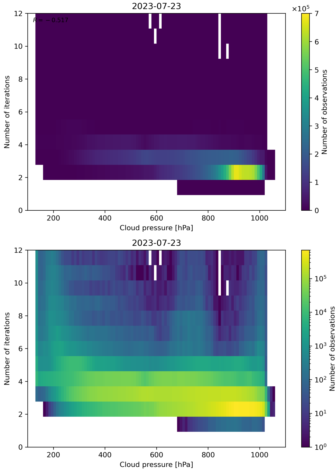
Figure 89: Scatter density plot of “Cloud pressure” against “Number of iterations” for 2023-07-22 to 2023-07-24.
