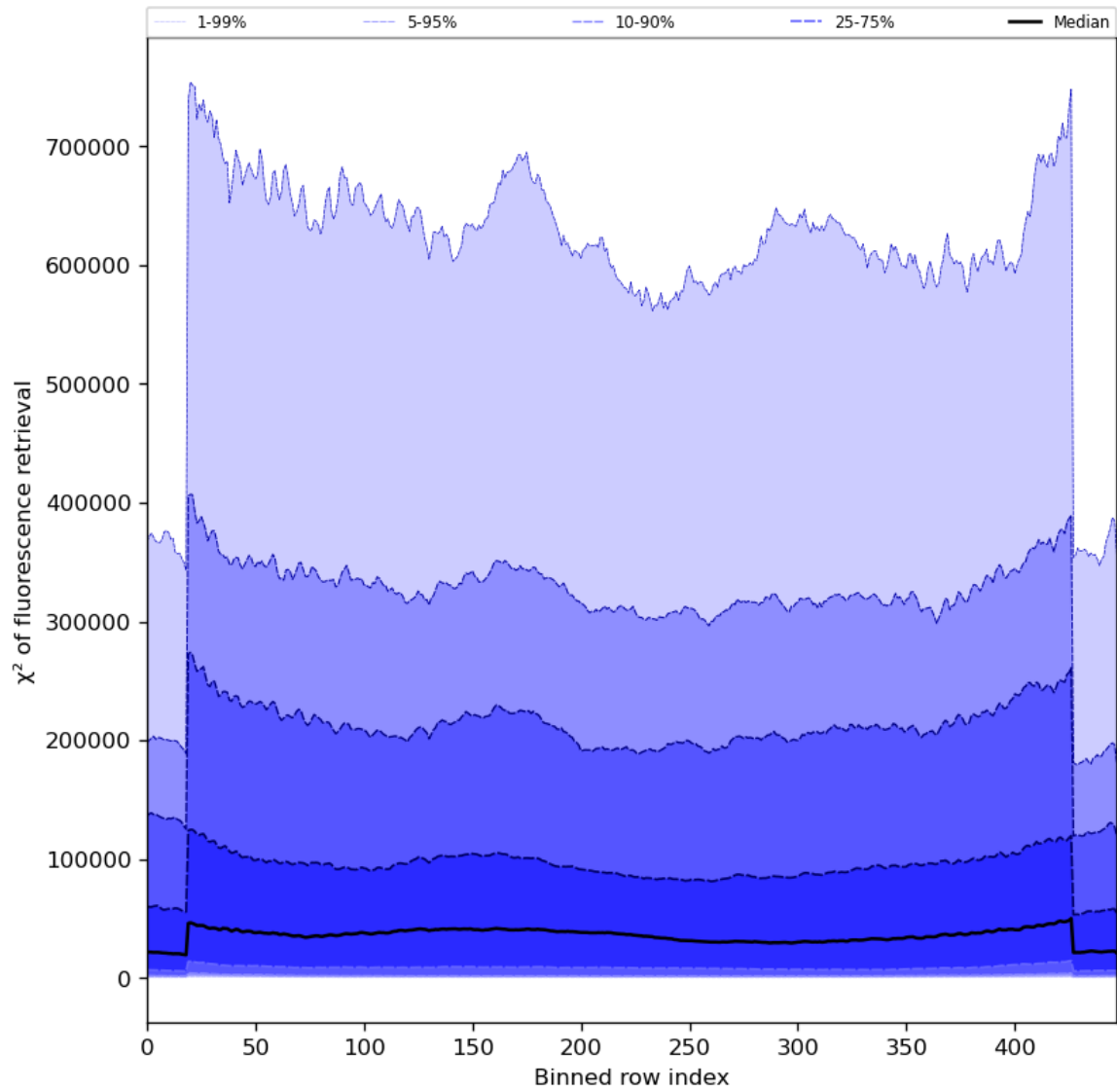
Figure 59: Along track statistics of “ \chi^2 of fluorescence retrieval” for 2023-07-22 to 2023-07-24
