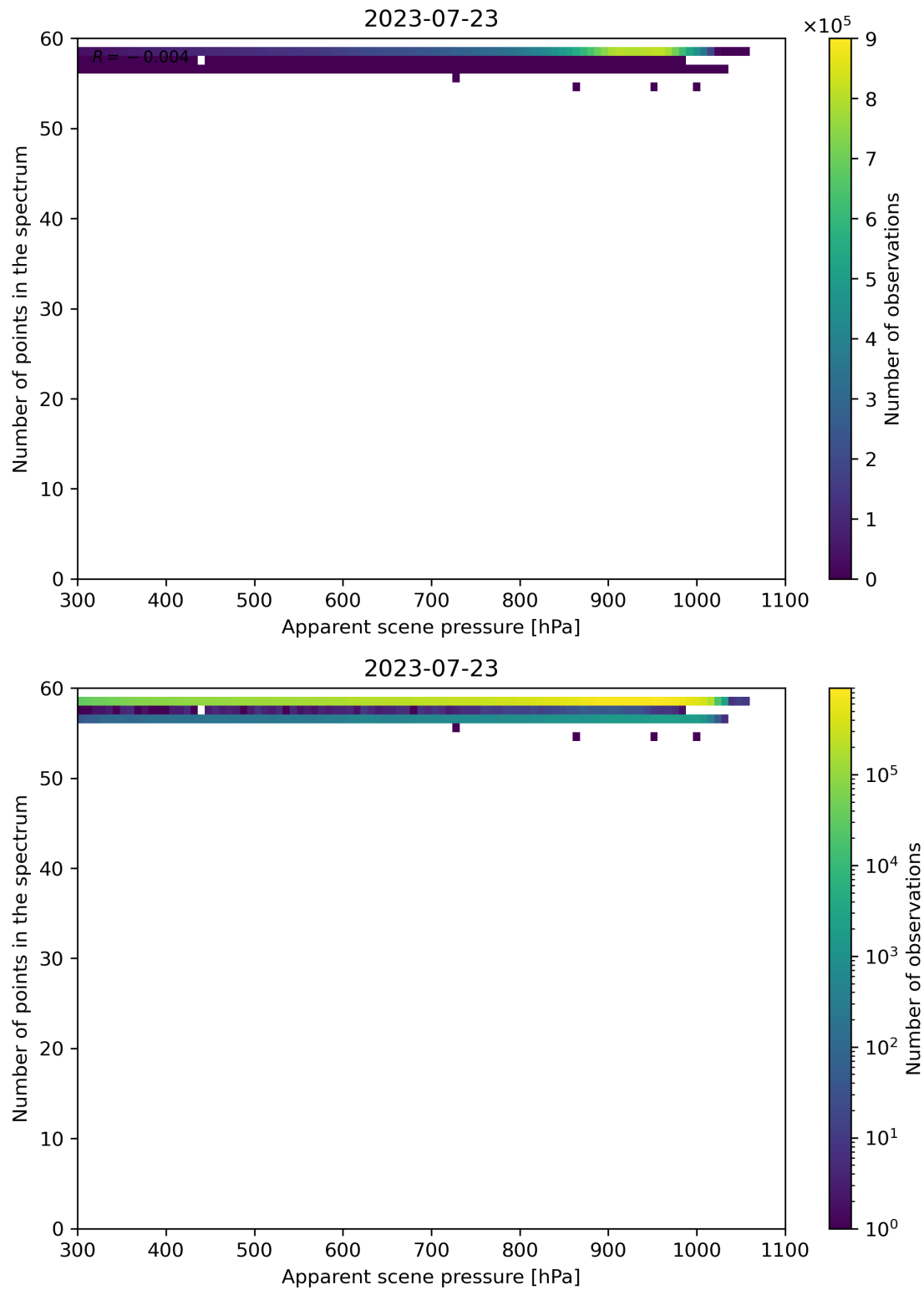
Figure 67: Scatter density plot of “Apparent scene pressure” against “Number of points in the spectrum” for 2023-07-22 to 2023-07-24.
