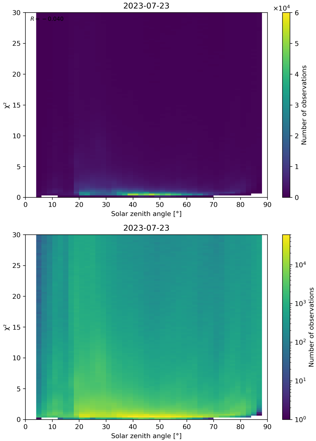
Figure 119: Scatter density plot of “Solar zenith angle” against “ \chi^2 ” for 2023-07-22 to 2023-07-24.
