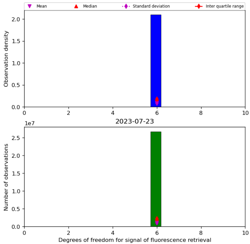
Figure 43: Histogram of “Degrees of freedom for signal of fluorescence retrieval” for 2023-07-22 to 2023-07-24
