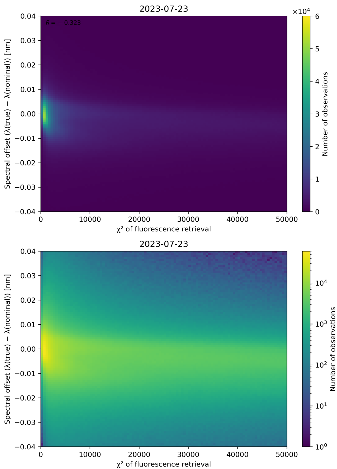
Figure 72: Scatter density plot of " \chi^2 of fluorescence retrieval" against "Spectral offset ( \lambda(\text{true}) - \lambda(\text{nominal}) )" for 2023-07-22 to 2023-07-24.
