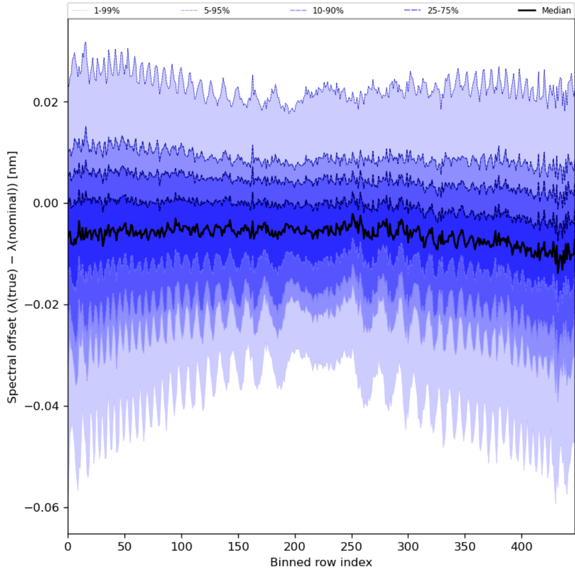
Figure 62: Along track statistics of “Spectral offset ( \lambda(\text{true}) - \lambda(\text{nominal}) )” for 2023-07-22 to 2023-07-24
