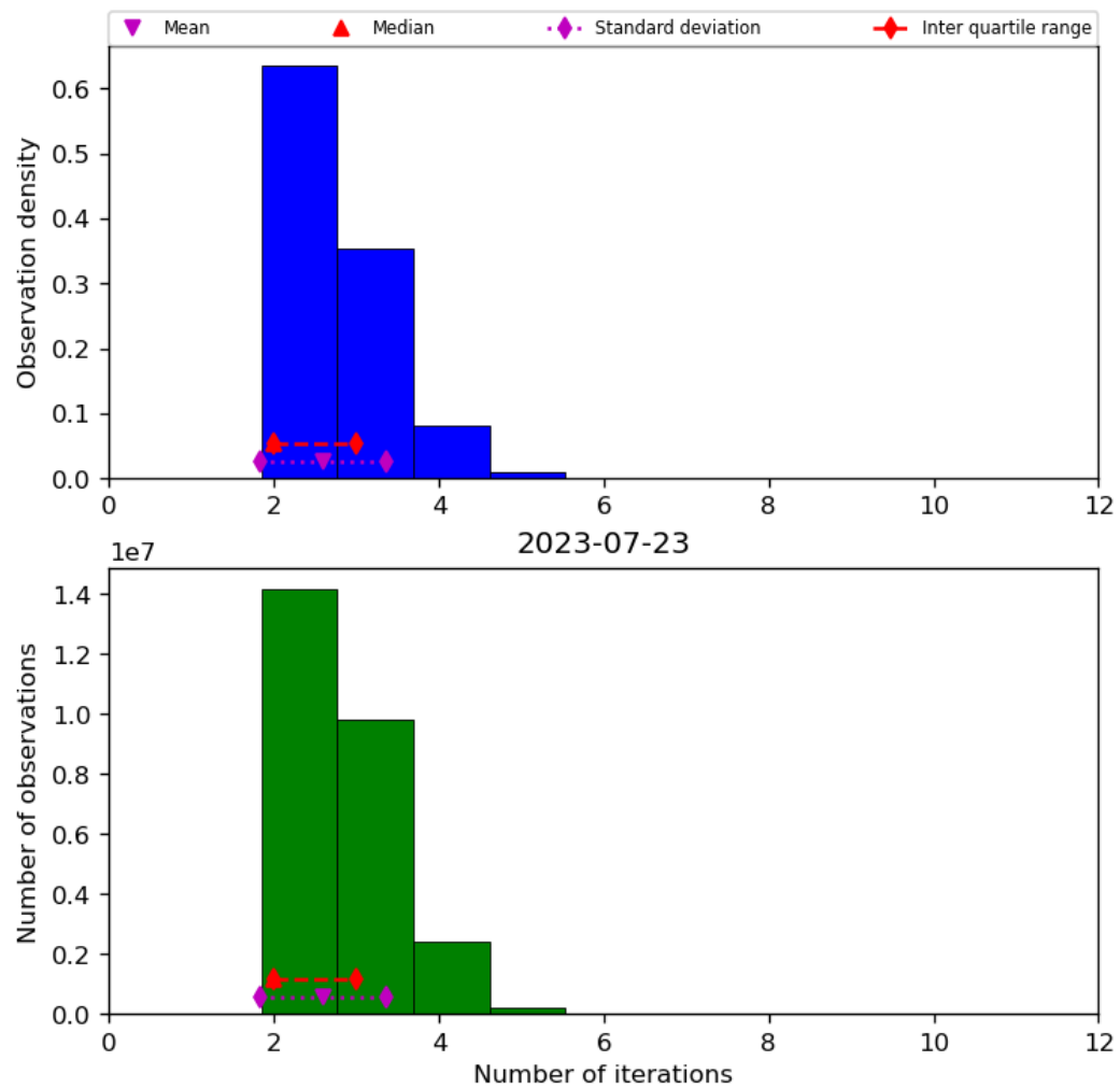
Figure 39: Histogram of “Number of iterations” for 2023-07-22 to 2023-07-24
