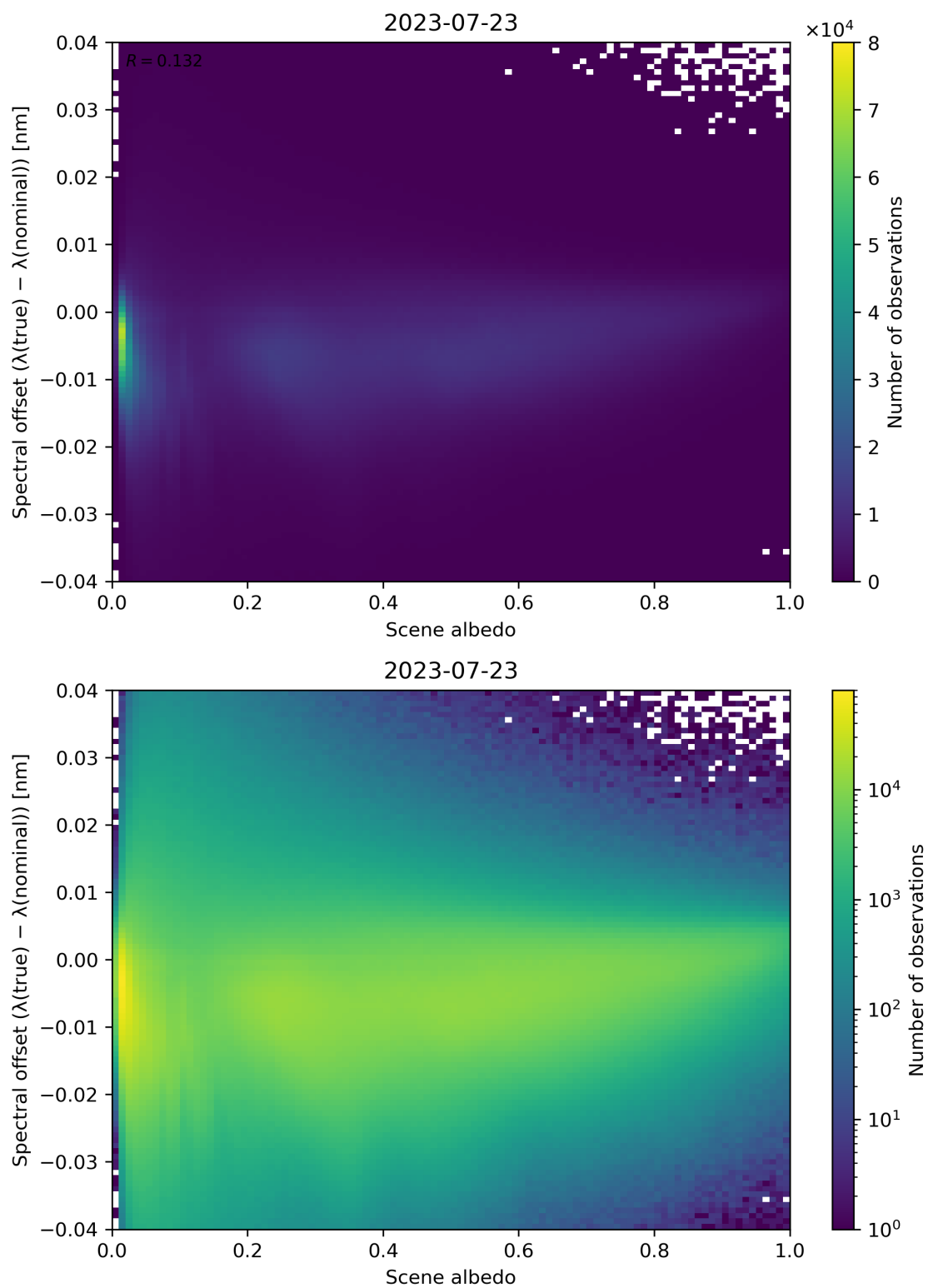
Figure 117: Scatter density plot of “Scene albedo” against “Spectral offset ( \lambda(\text{true}) - \lambda(\text{nominal}) )” for 2023-07-22 to 2023-07-24.
