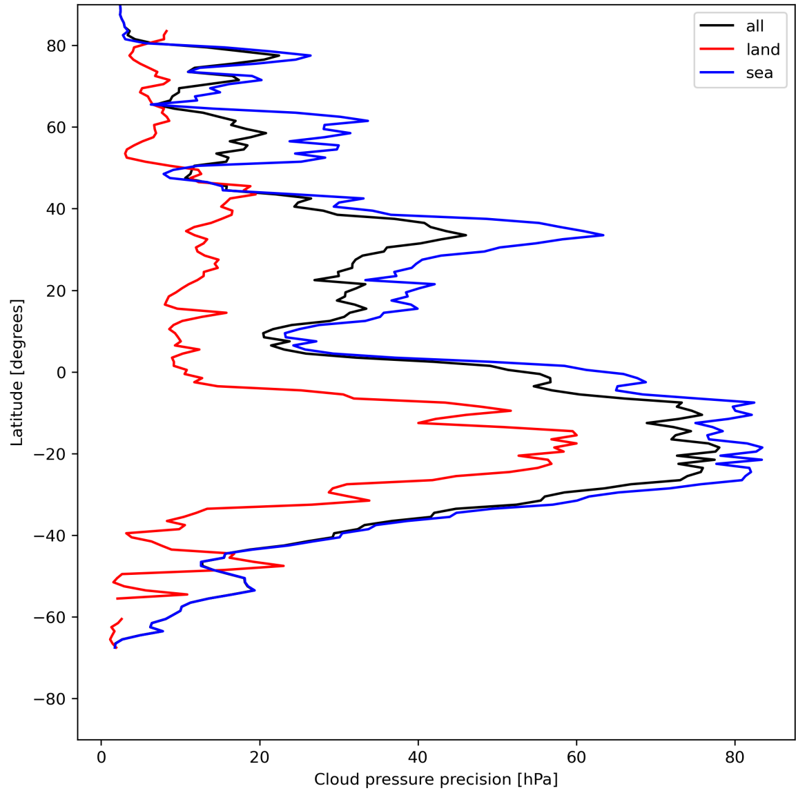
Figure 14: Zonal average of “Cloud pressure precision” for 2023-07-22 to 2023-07-24.
