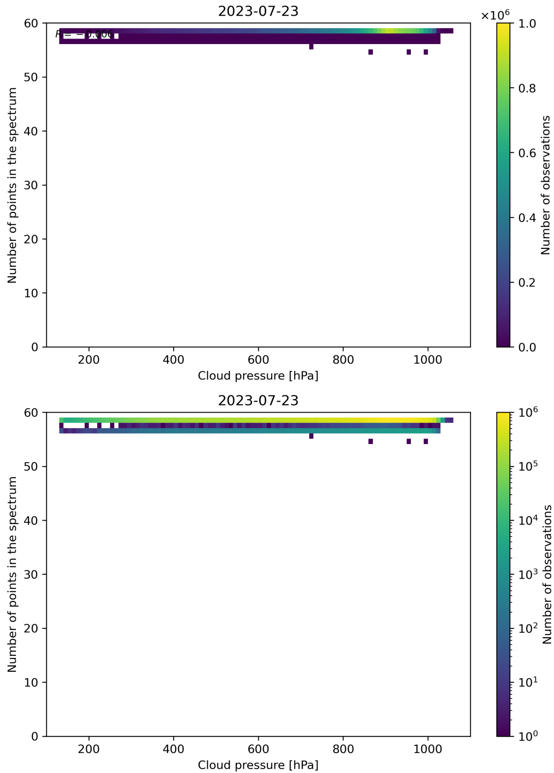
Figure 90: Scatter density plot of “Cloud pressure” against “Number of points in the spectrum” for 2023-07-22 to 2023-07-24.
