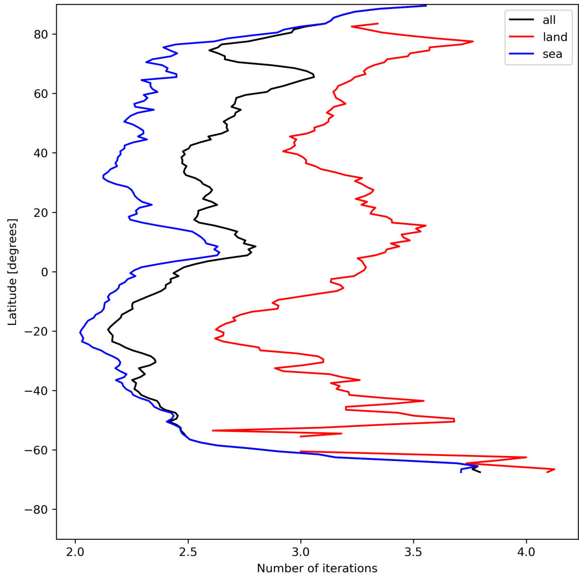
Figure 22: Zonal average of “Number of iterations” for 2023-07-22 to 2023-07-24.
