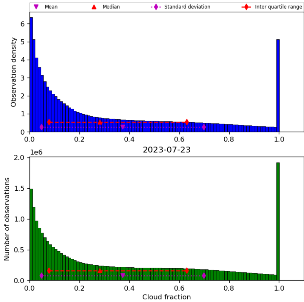
Figure 32: Histogram of “Cloud fraction” for 2023-07-22 to 2023-07-24
