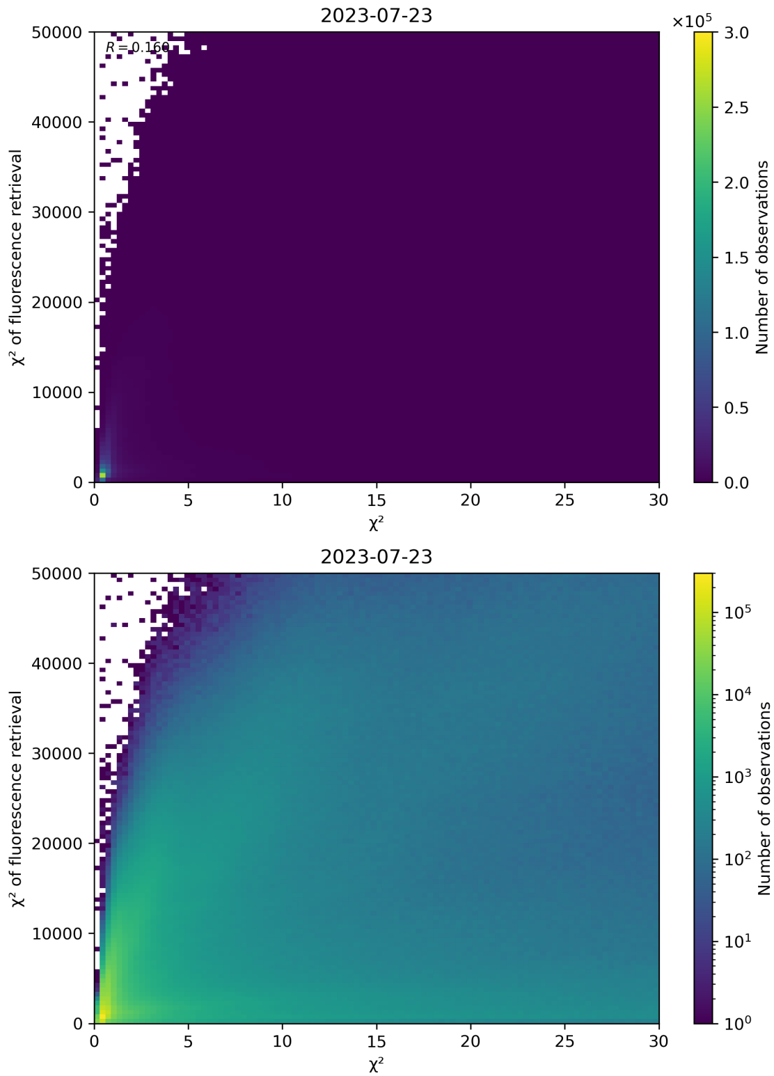
Figure 69: Scatter density plot of “ \chi^2 ” against “ \chi^2 of fluorescence retrieval” for 2023-07-22 to 2023-07-24.
