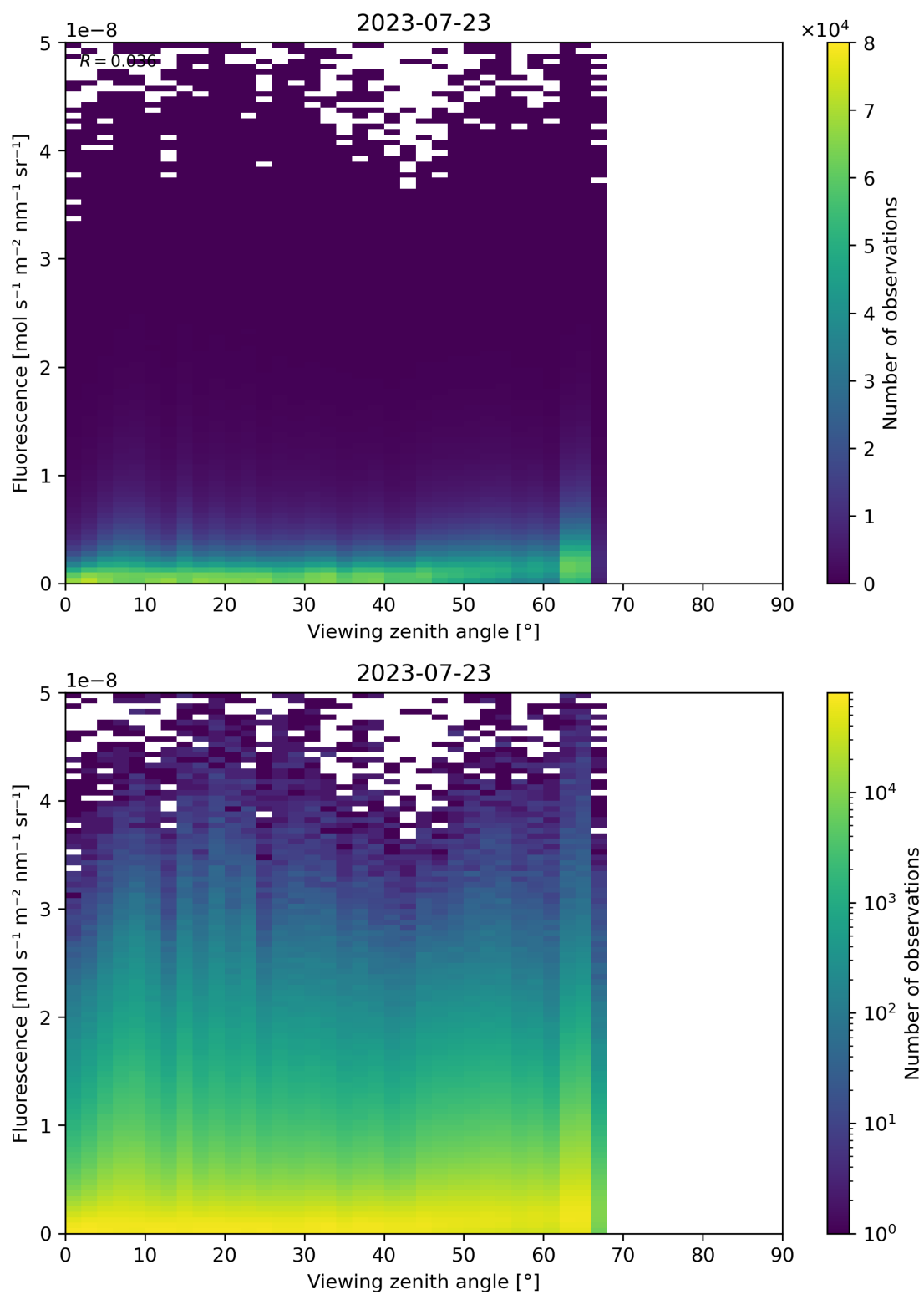
Figure 134: Scatter density plot of “Viewing zenith angle” against “Fluorescence” for 2023-07-22 to 2023-07-24.
