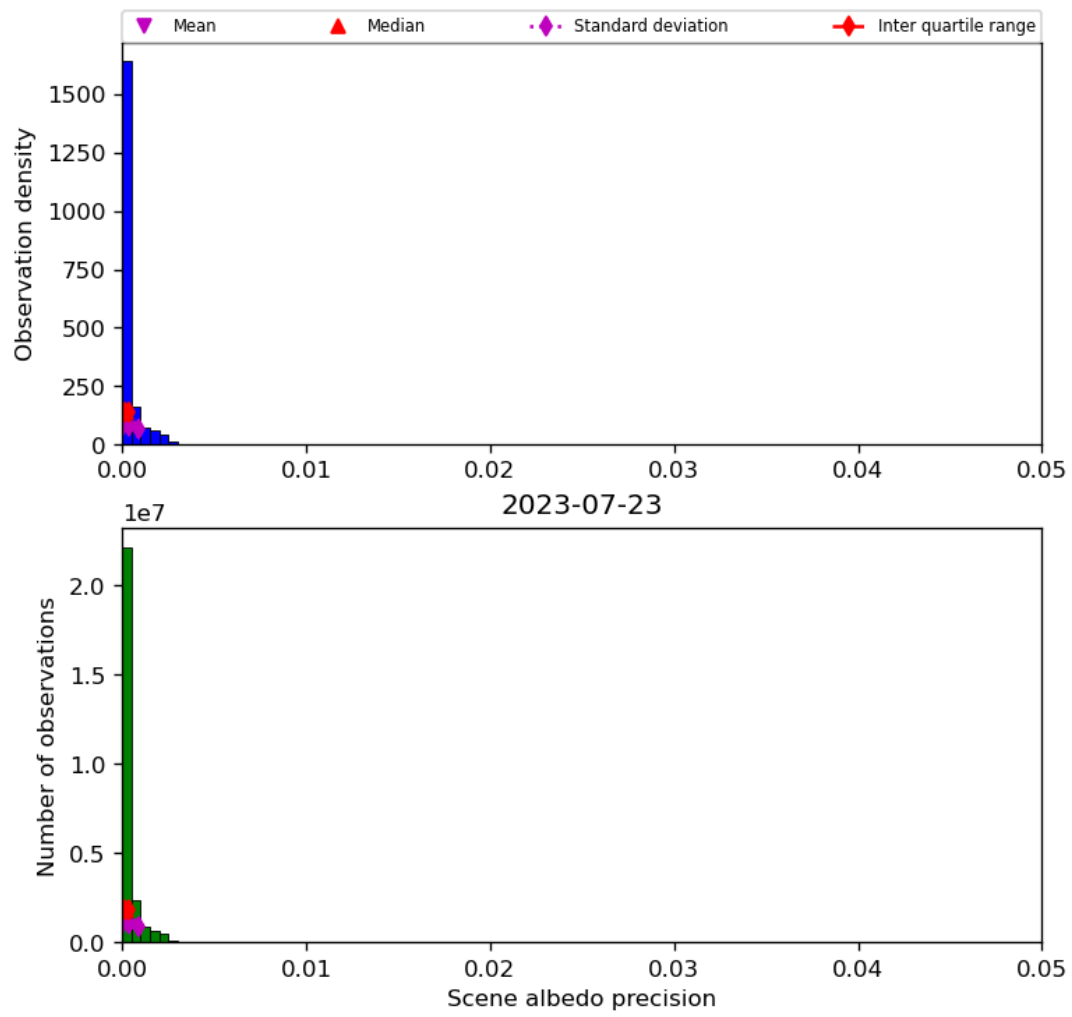
Figure 35: Histogram of “Scene albedo precision” for 2023-07-22 to 2023-07-24
