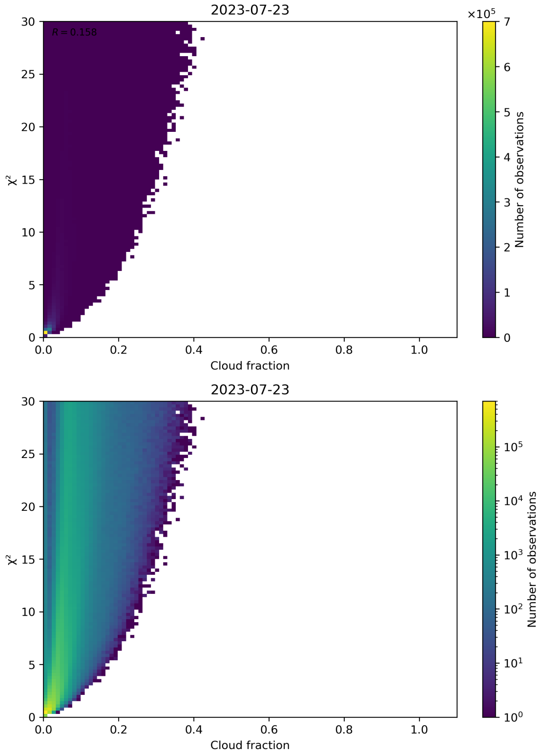
Figure 77: Scatter density plot of “Cloud fraction” against “ \chi^2 ” for 2023-07-22 to 2023-07-24.
