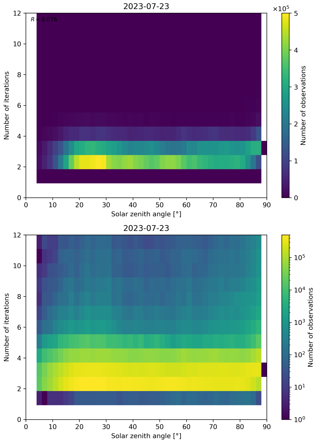
Figure 125: Scatter density plot of “Solar zenith angle” against “Number of iterations” for 2023-07-22 to 2023-07-24.
