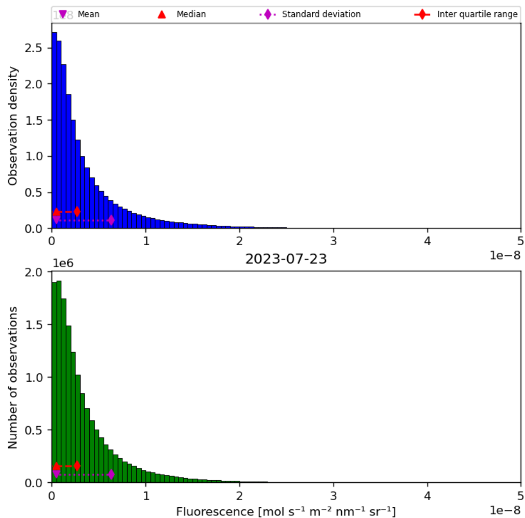
Figure 40: Histogram of “Fluorescence” for 2023-07-22 to 2023-07-24
