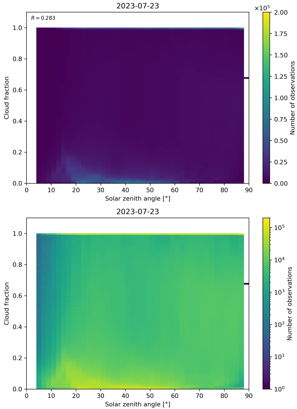
Figure 121: Scatter density plot of “Solar zenith angle” against “Cloud fraction” for 2023-07-22 to 2023-07-24.
