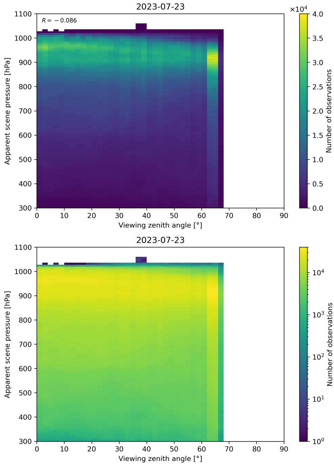
Figure 129: Scatter density plot of “Viewing zenith angle” against “Apparent scene pressure” for 2023-07-22 to 2023-07-24.
