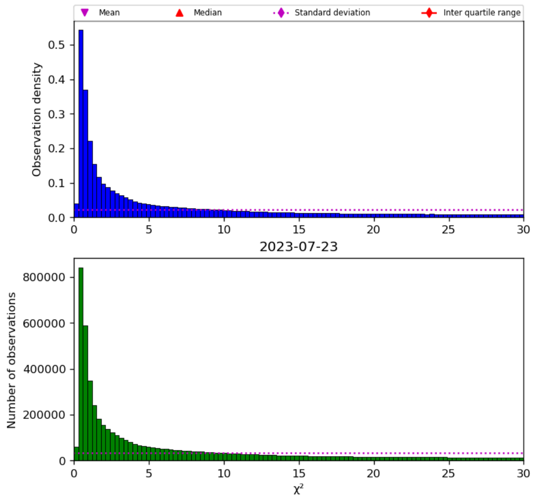
Figure 38: Histogram of “ \chi^2 ” for 2023-07-22 to 2023-07-24
