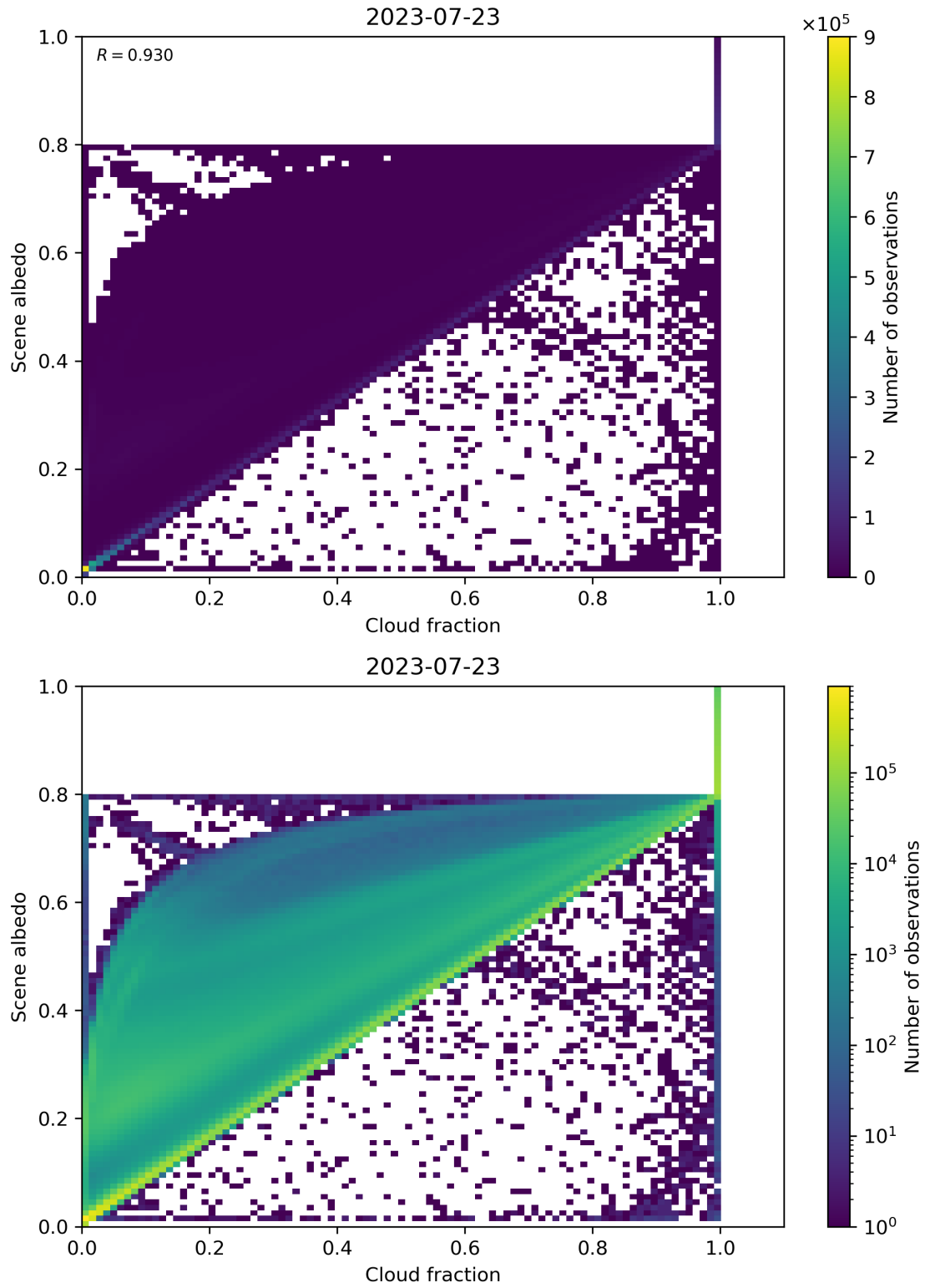
Figure 82: Scatter density plot of “Cloud fraction” against “Scene albedo” for 2023-07-22 to 2023-07-24.
