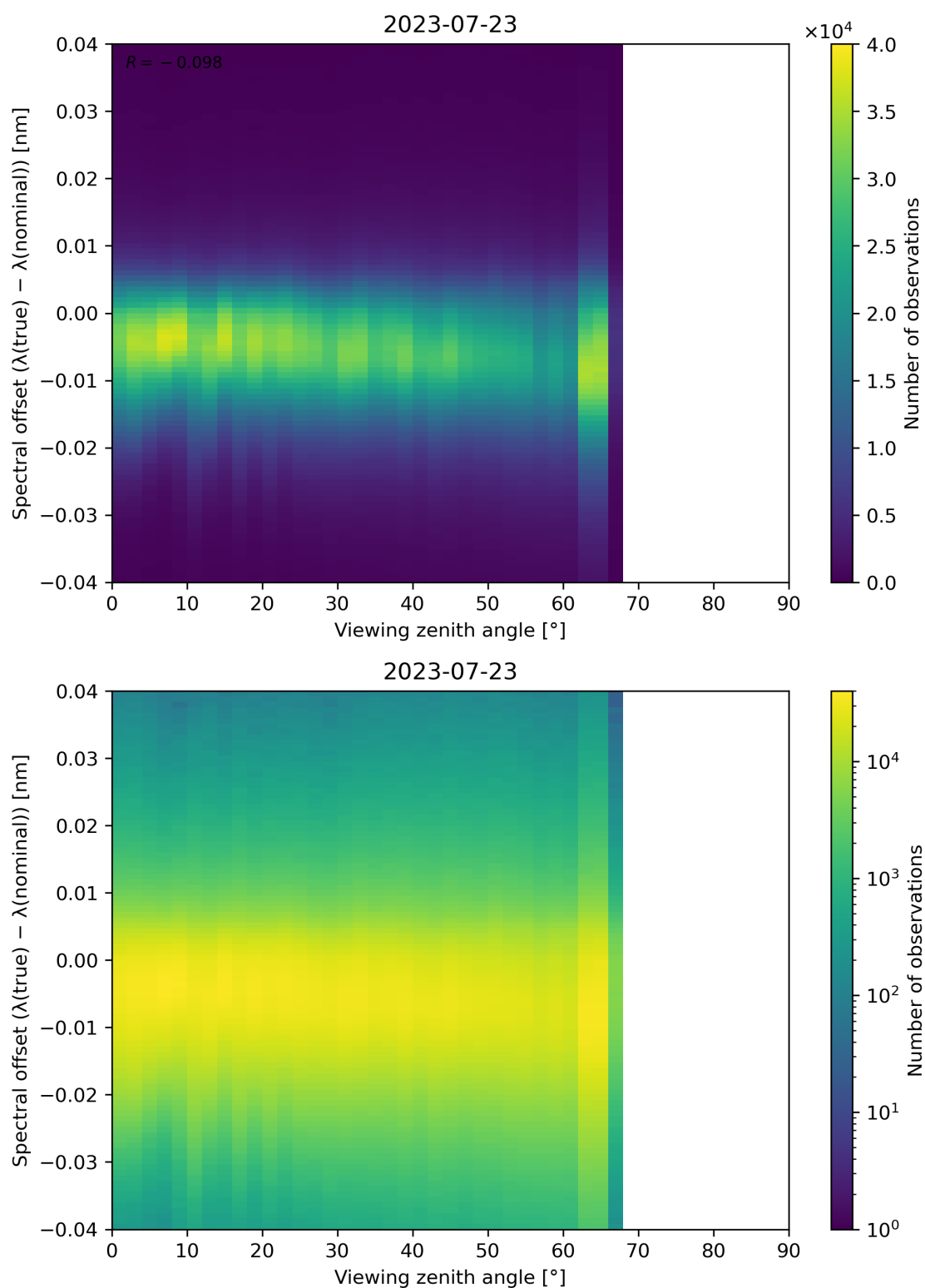
Figure 140: Scatter density plot of “Viewing zenith angle” against “Spectral offset ( \lambda(\text{true}) - \lambda(\text{nominal}) )” for 2023-07-22 to 2023-07-24.
