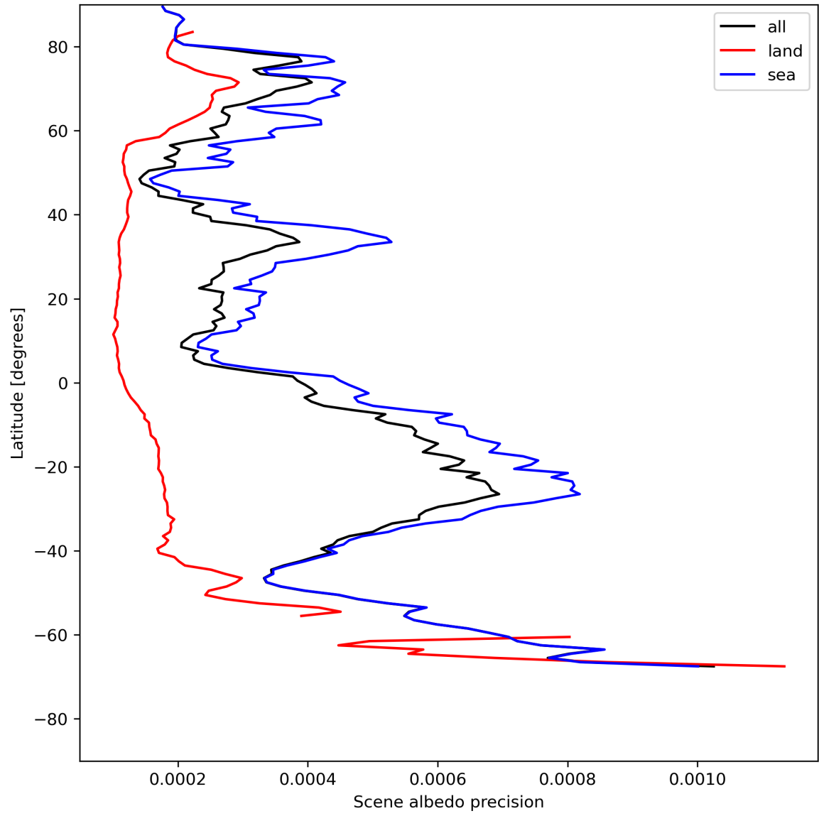
Figure 18: Zonal average of “Scene albedo precision” for 2023-07-22 to 2023-07-24.
