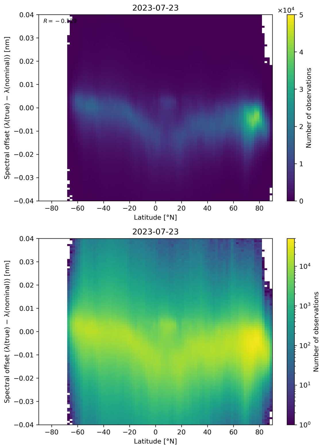
Figure 105: Scatter density plot of “Latitude” against “Spectral offset ( \lambda(\text{true}) - \lambda(\text{nominal}) )” for 2023-07-22 to 2023-07-24.
