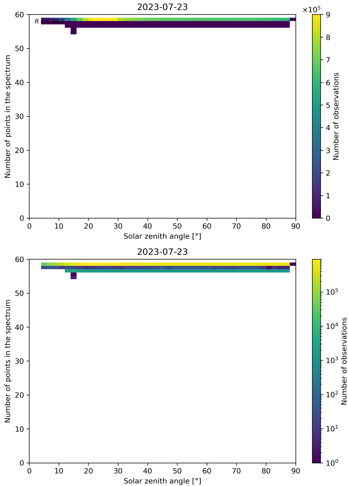
Figure 126: Scatter density plot of “Solar zenith angle” against “Number of points in the spectrum” for 2023-07-22 to 2023-07-24.
