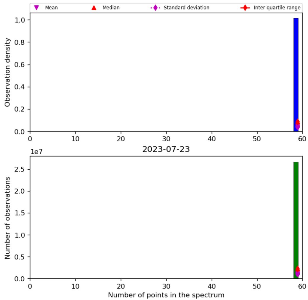
Figure 44: Histogram of “Number of points in the spectrum” for 2023-07-22 to 2023-07-24
