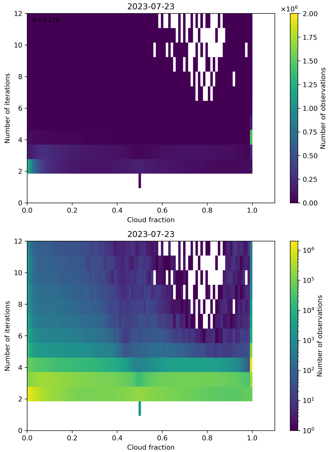
Figure 80: Scatter density plot of “Cloud fraction” against “Number of iterations” for 2023-07-22 to 2023-07-24.
