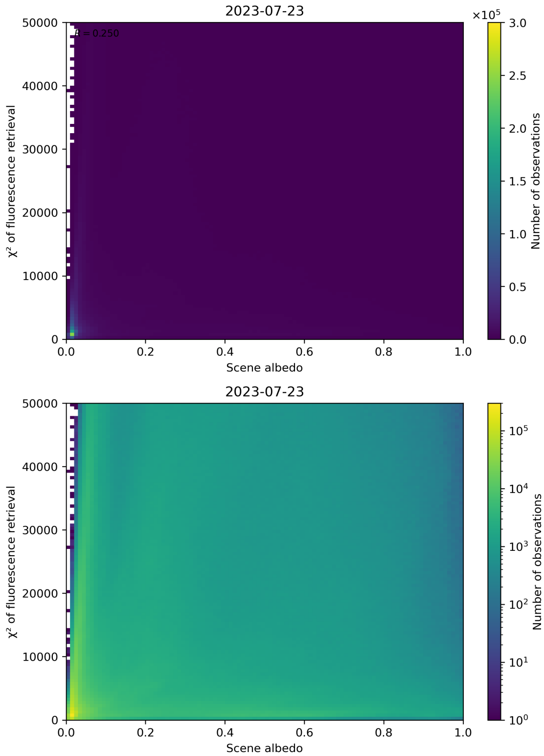
Figure 113: Scatter density plot of “Scene albedo” against “ \chi^2 of fluorescence retrieval” for 2023-07-22 to 2023-07-24.
