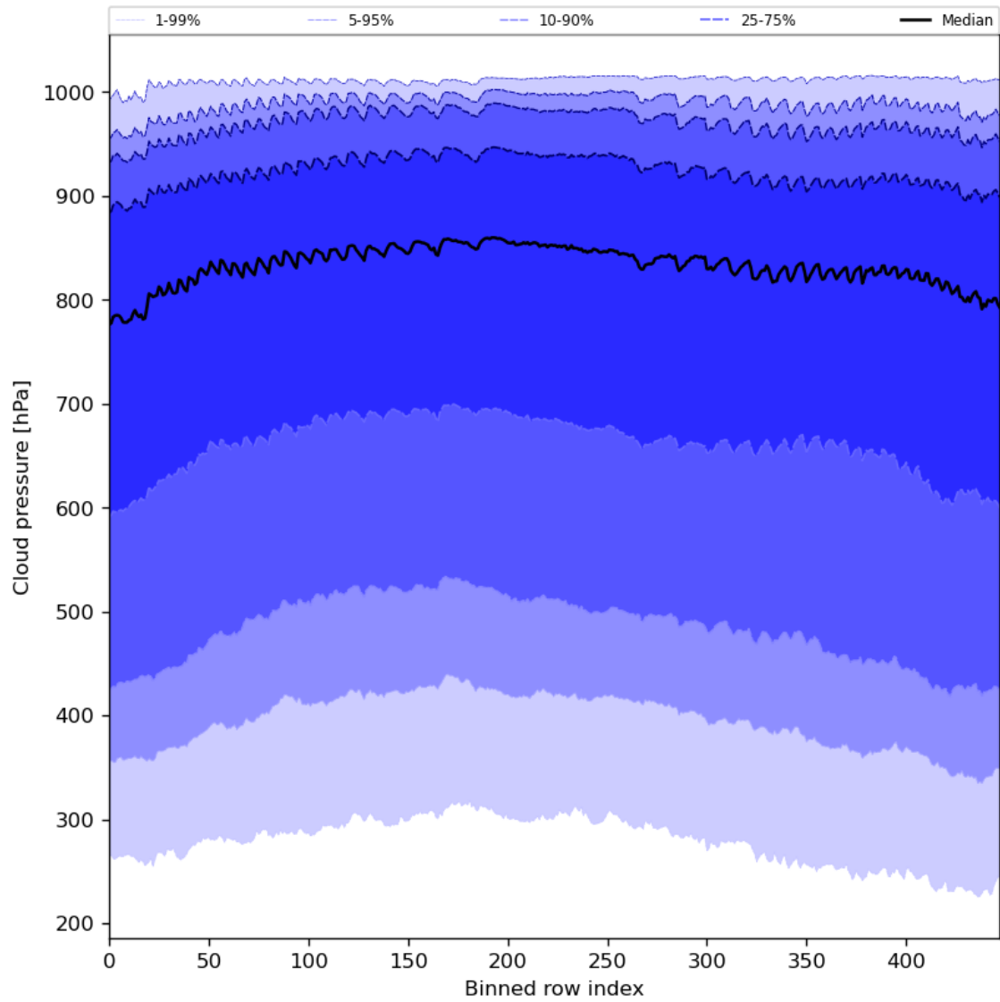
Figure 47: Along track statistics of “Cloud pressure” for 2023-07-22 to 2023-07-24
