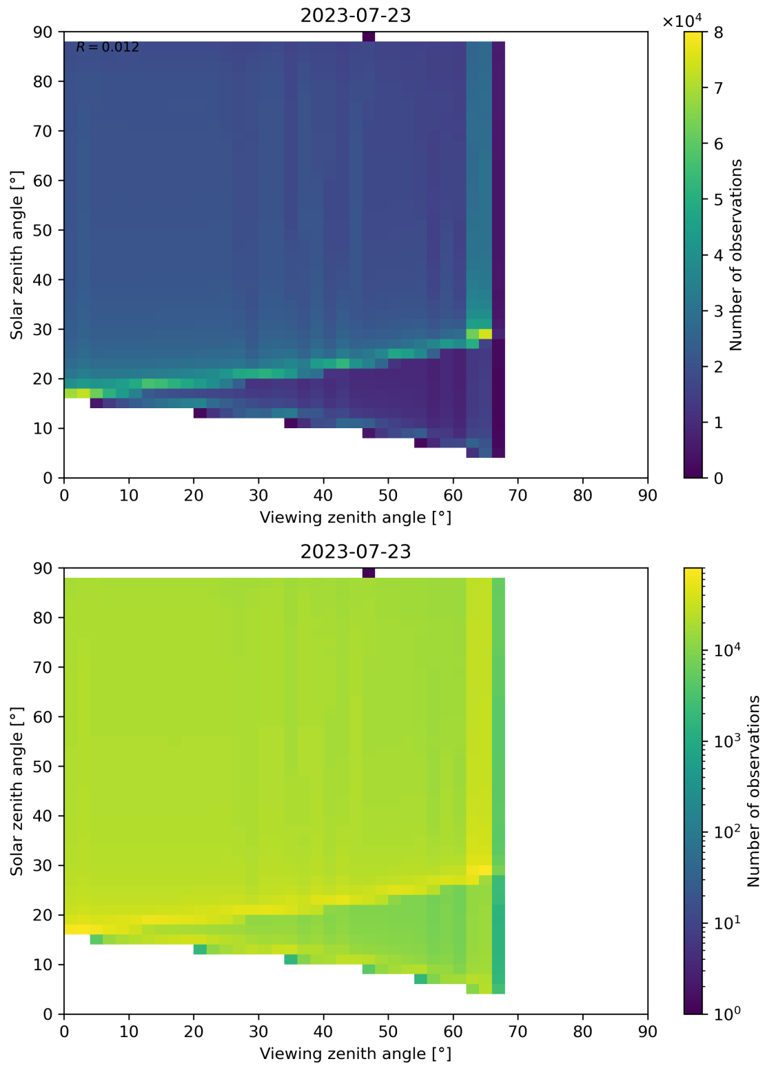
Figure 139: Scatter density plot of “Viewing zenith angle” against “Solar zenith angle” for 2023-07-22 to 2023-07-24.
