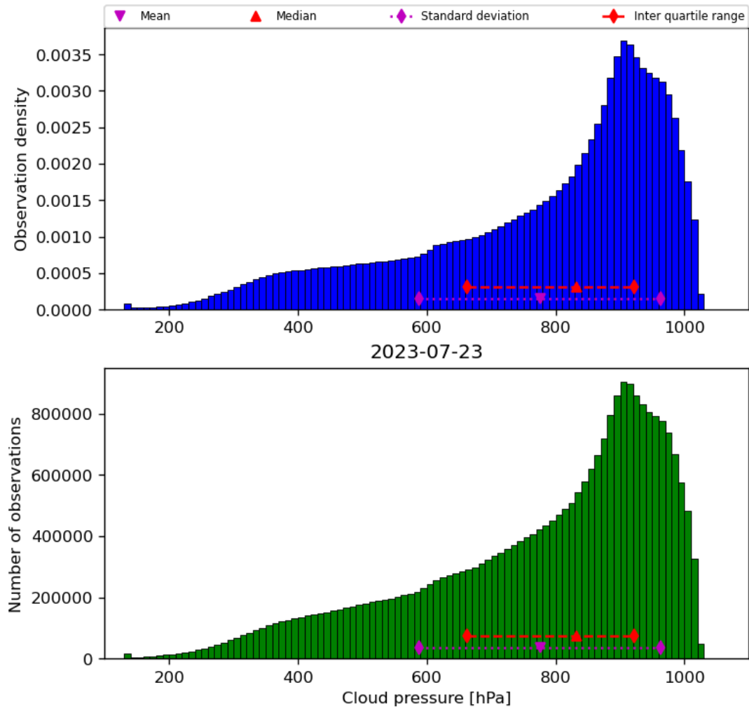
Figure 30: Histogram of “Cloud pressure” for 2023-07-22 to 2023-07-24
