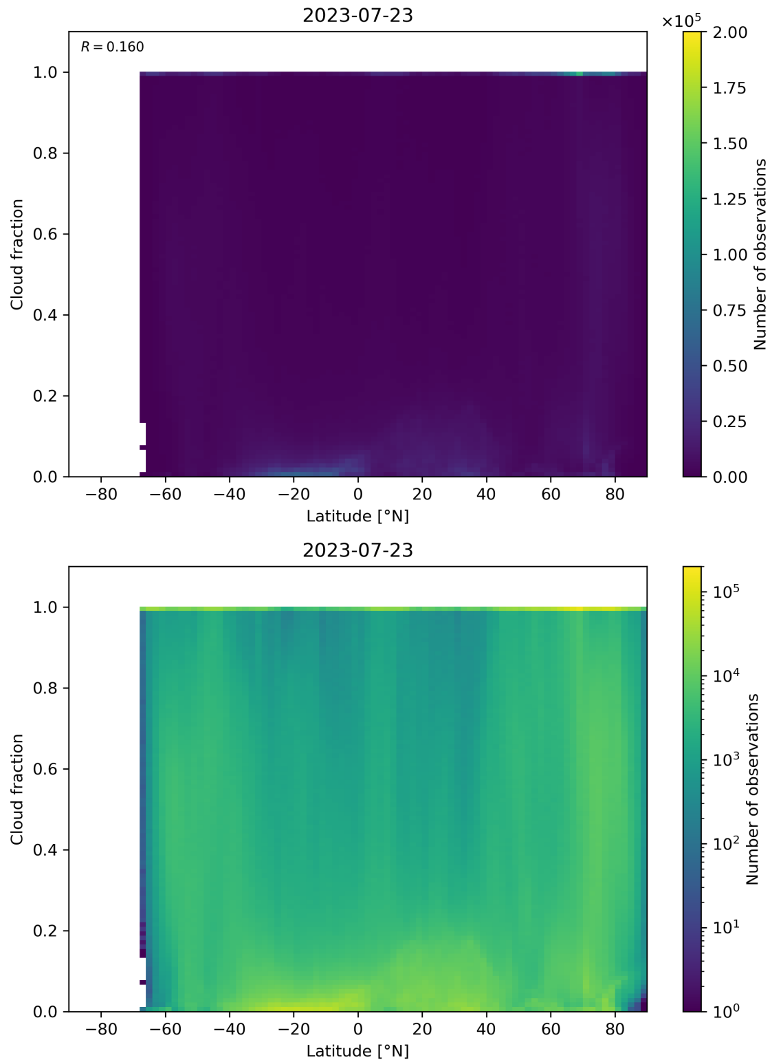
Figure 99: Scatter density plot of “Latitude” against “Cloud fraction” for 2023-07-22 to 2023-07-24.
