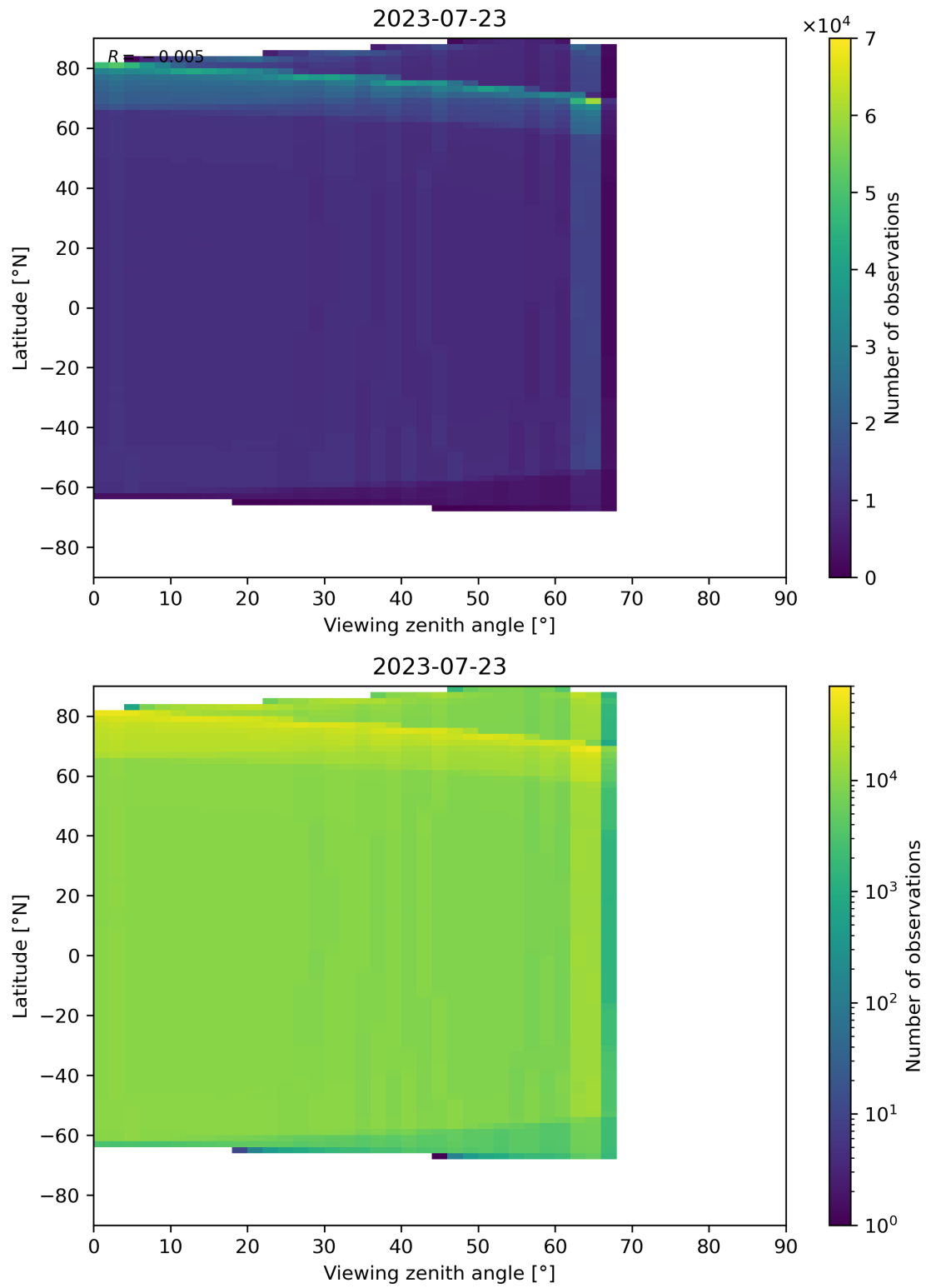
Figure 135: Scatter density plot of “Viewing zenith angle” against “Latitude” for 2023-07-22 to 2023-07-24.
