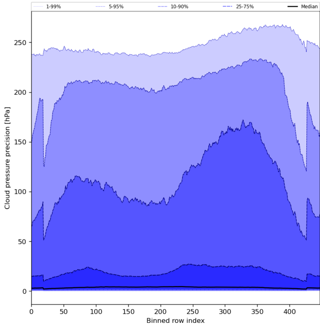
Figure 48: Along track statistics of “Cloud pressure precision” for 2023-07-22 to 2023-07-24
