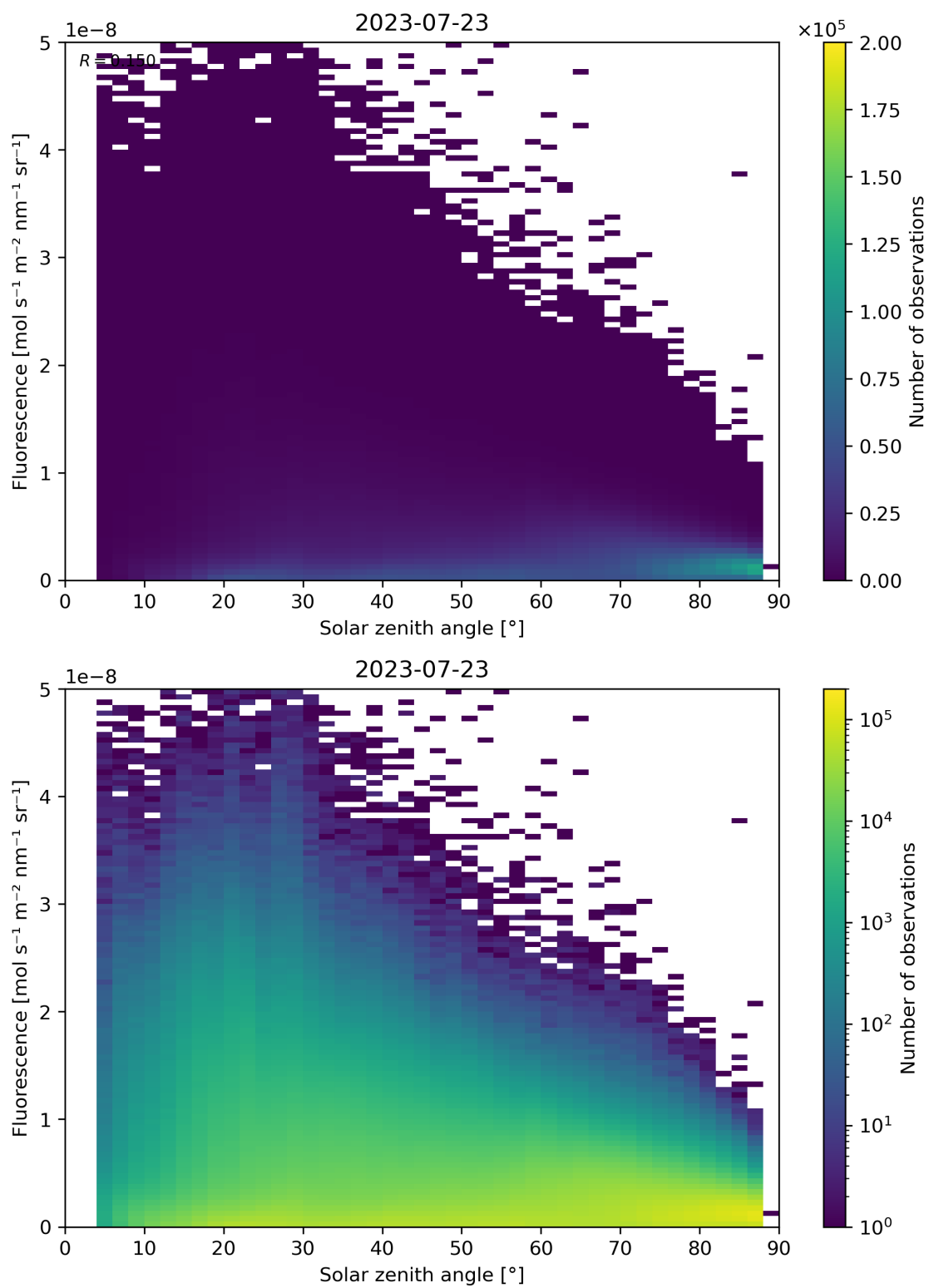
Figure 123: Scatter density plot of “Solar zenith angle” against “Fluorescence” for 2023-07-22 to 2023-07-24.
