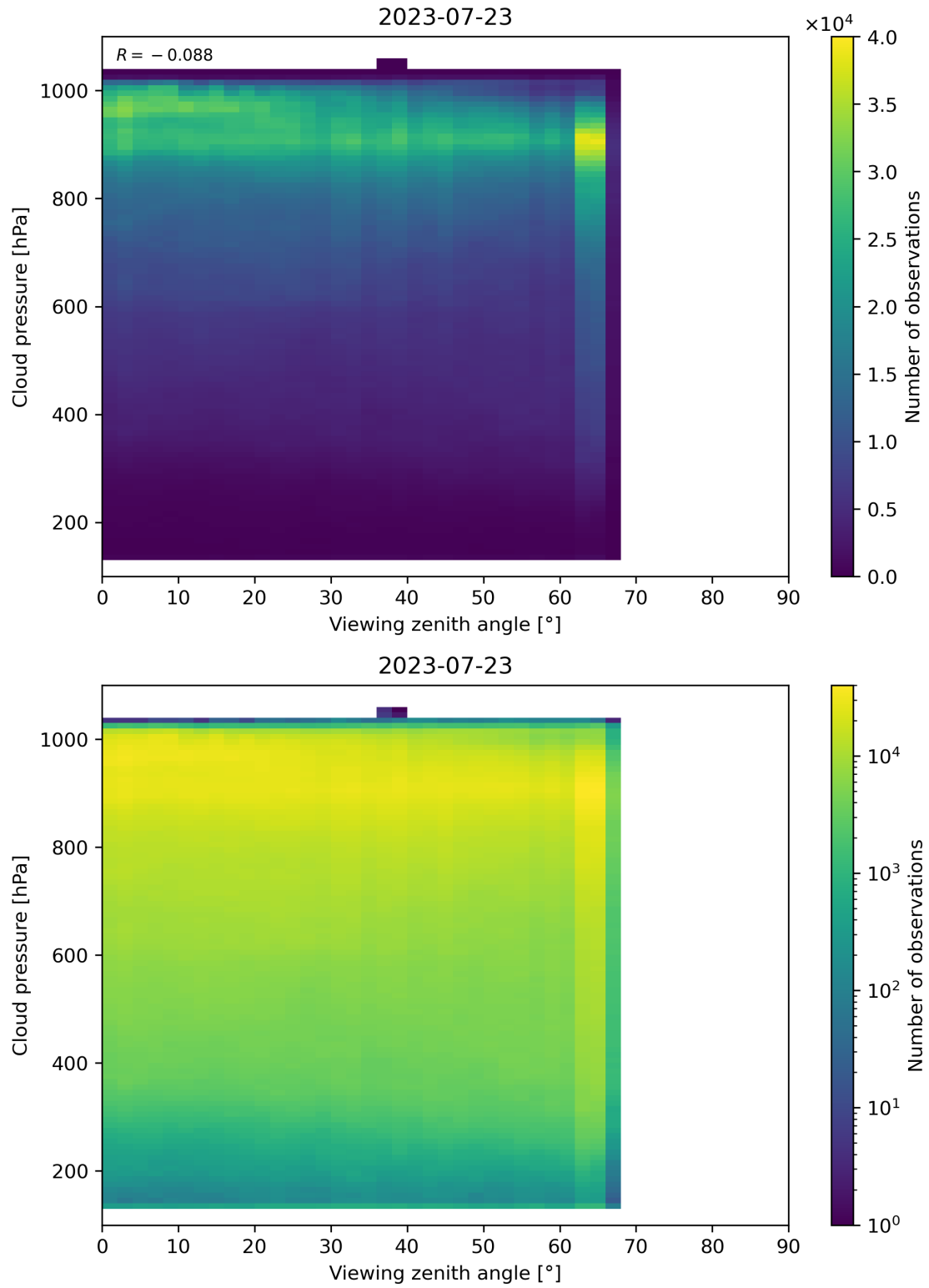
Figure 133: Scatter density plot of “Viewing zenith angle” against “Cloud pressure” for 2023-07-22 to 2023-07-24.
