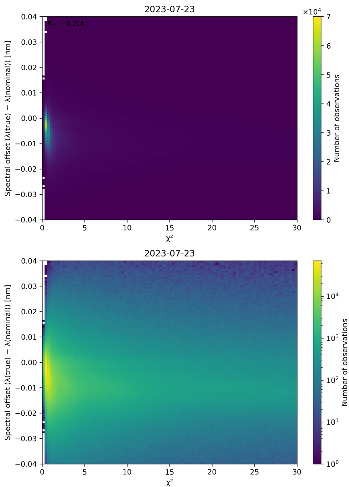
Figure 75: Scatter density plot of “ \chi^2 ” against “Spectral offset ( \lambda(\text{true}) - \lambda(\text{nominal}) )” for 2023-07-22 to 2023-07-24.
