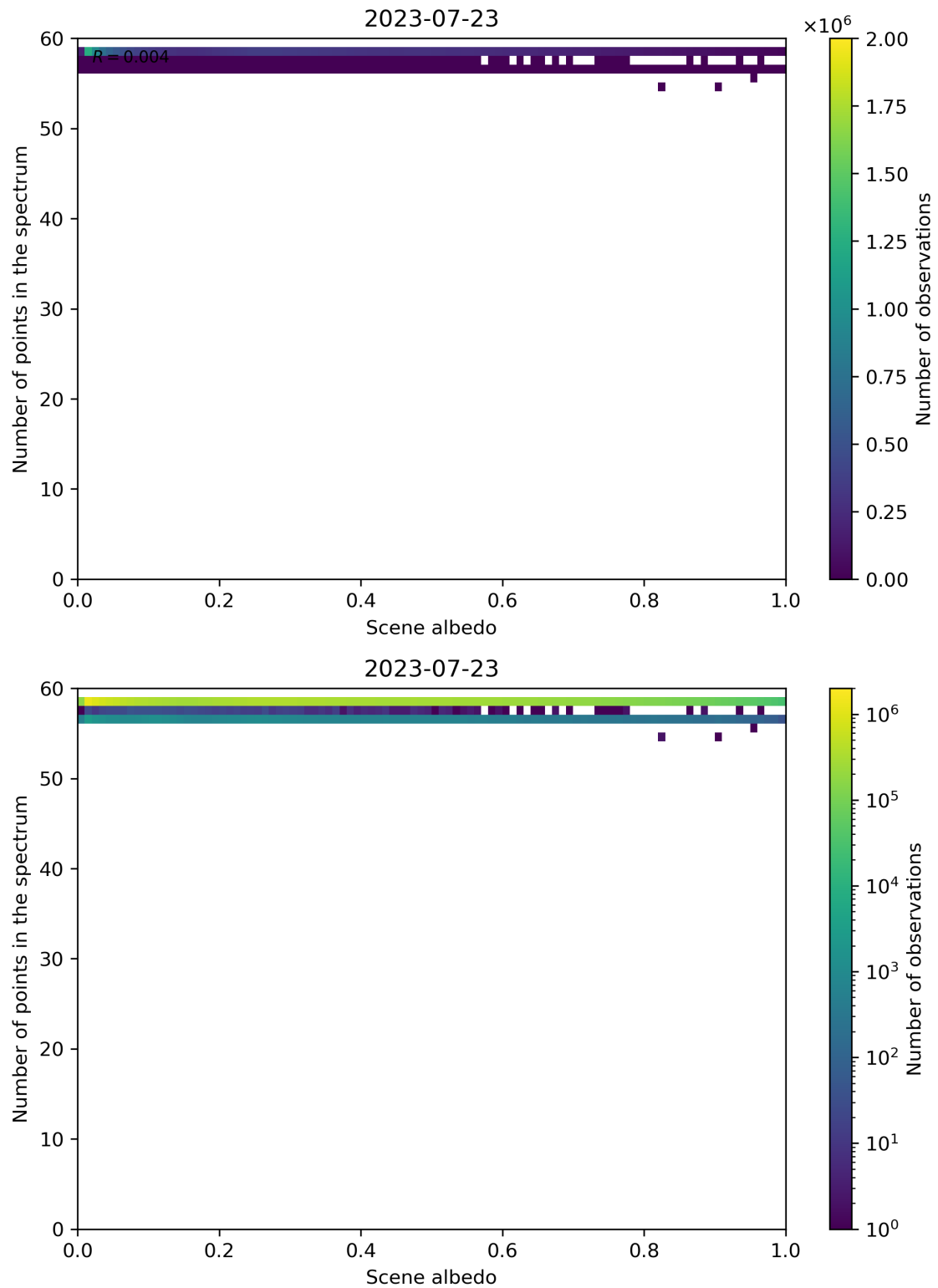
Figure 116: Scatter density plot of “Scene albedo” against “Number of points in the spectrum” for 2023-07-22 to 2023-07-24.
