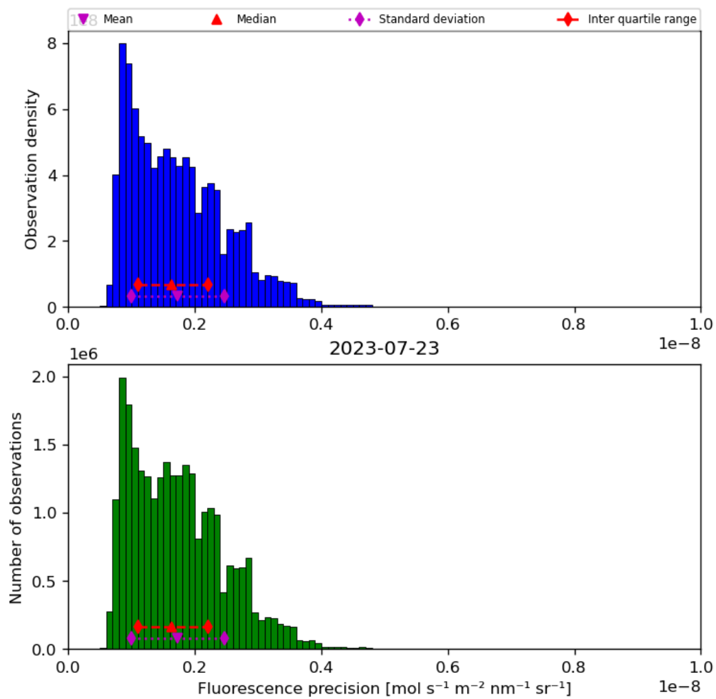
Figure 41: Histogram of “Fluorescence precision” for 2023-07-22 to 2023-07-24
