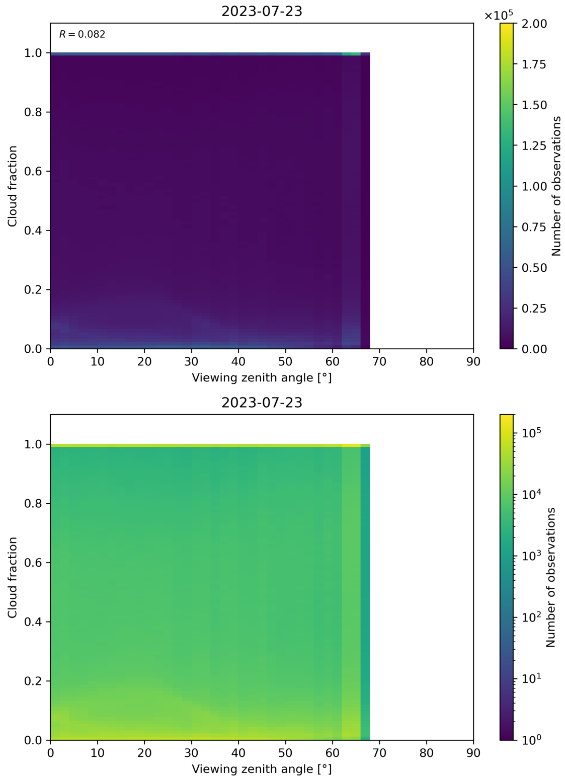
Figure 132: Scatter density plot of “Viewing zenith angle” against “Cloud fraction” for 2023-07-22 to 2023-07-24.
