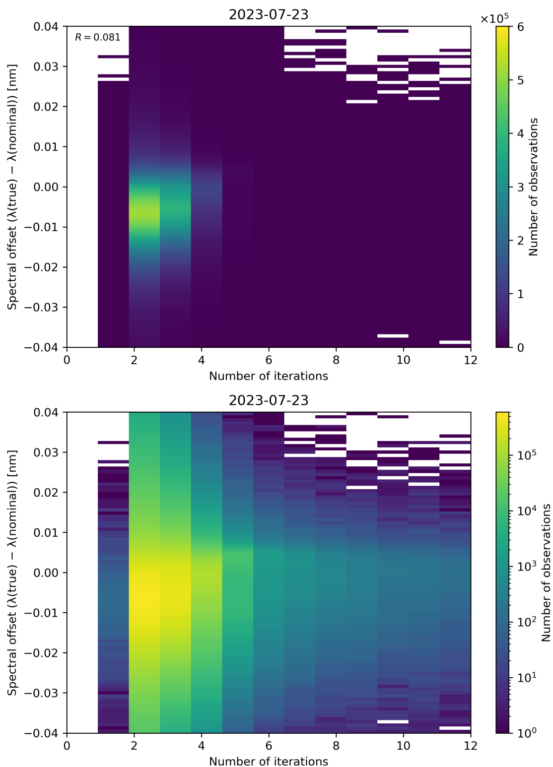
Figure 109: Scatter density plot of “Number of iterations” against “Spectral offset ( \lambda(\text{true}) - \lambda(\text{nominal}) )” for 2023-07-22 to 2023-07-24.
