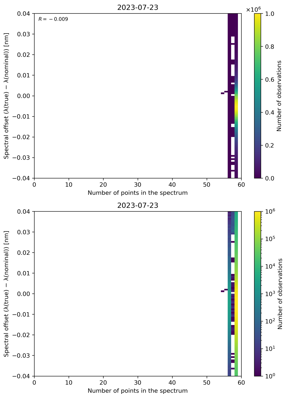
Figure 110: Scatter density plot of “Number of points in the spectrum” against “Spectral offset ( \lambda(\text{true}) - \lambda(\text{nominal}) )” for 2023-07-22 to 2023-07-24.
