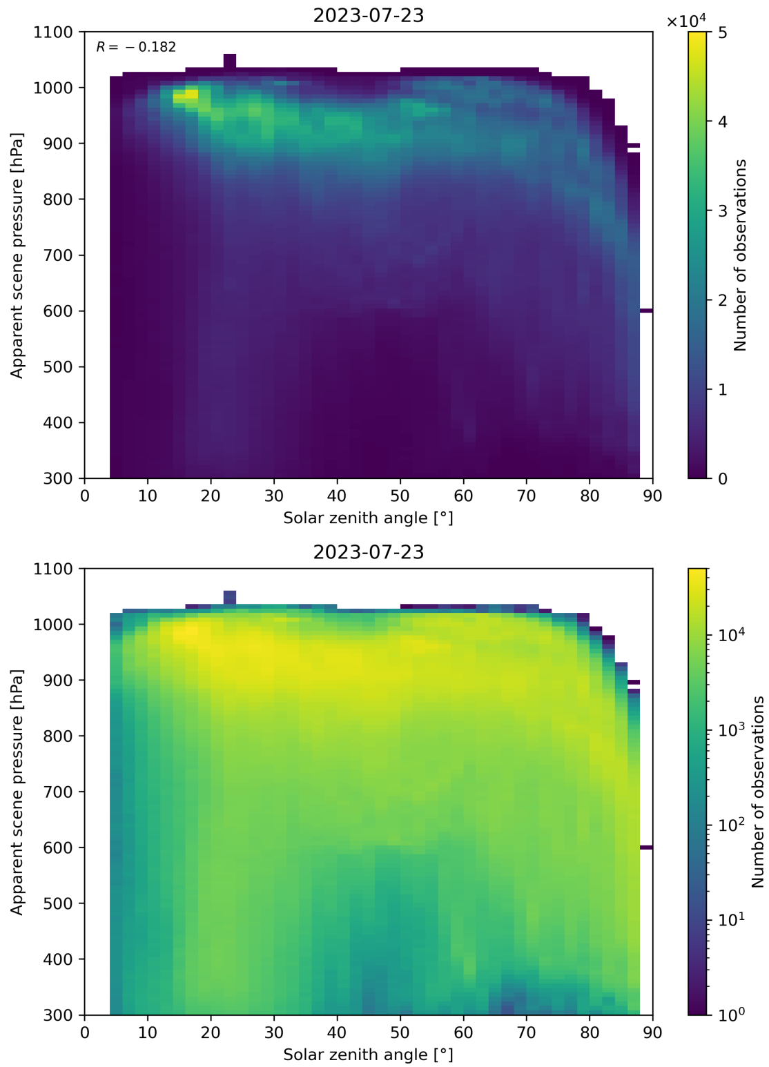
Figure 118: Scatter density plot of “Solar zenith angle” against “Apparent scene pressure” for 2023-07-22 to 2023-07-24.
