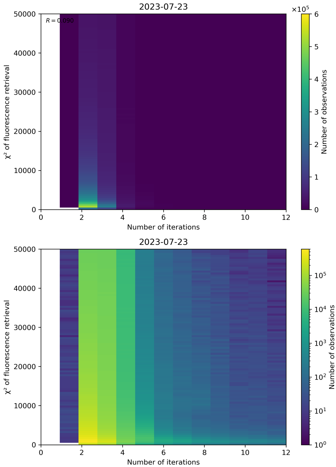
Figure 106: Scatter density plot of “Number of iterations” against “ \chi^2 of fluorescence retrieval” for 2023-07-22 to 2023-07-24.
