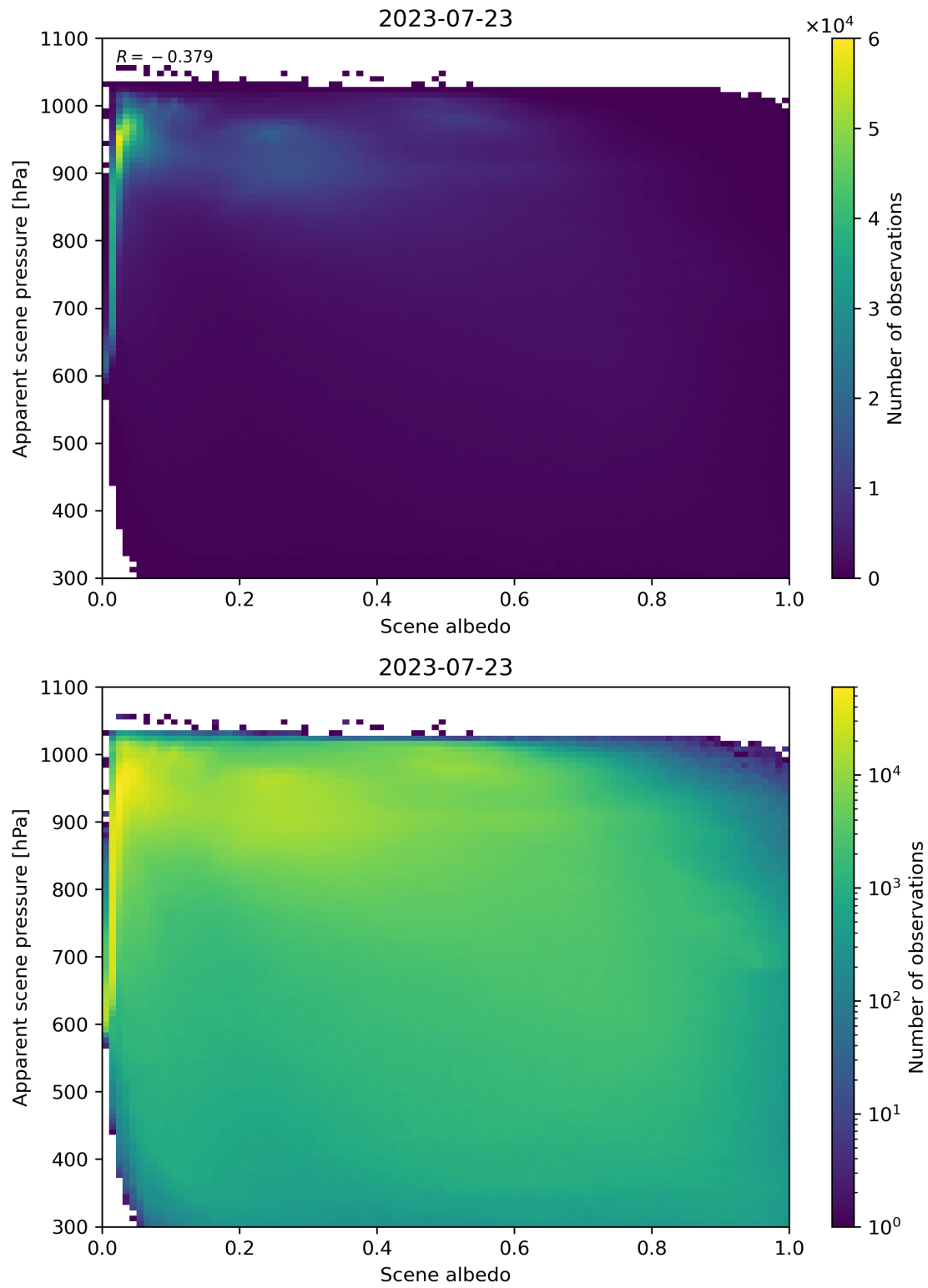
Figure 111: Scatter density plot of “Scene albedo” against “Apparent scene pressure” for 2023-07-22 to 2023-07-24.
