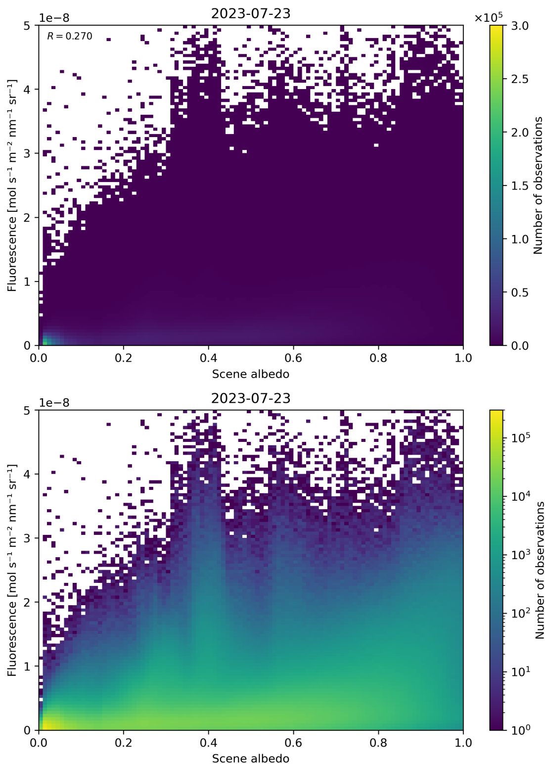
Figure 114: Scatter density plot of “Scene albedo” against “Fluorescence” for 2023-07-22 to 2023-07-24.
