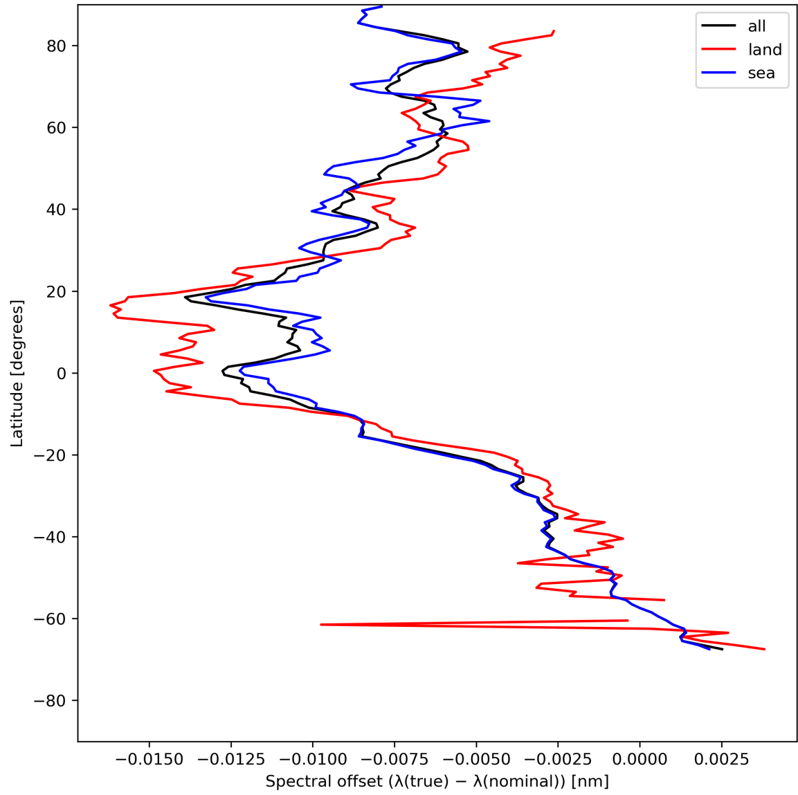
Figure 28: Zonal average of “Spectral offset ( \lambda(\text{true}) - \lambda(\text{nominal}) )” for 2023-07-22 to 2023-07-24.
