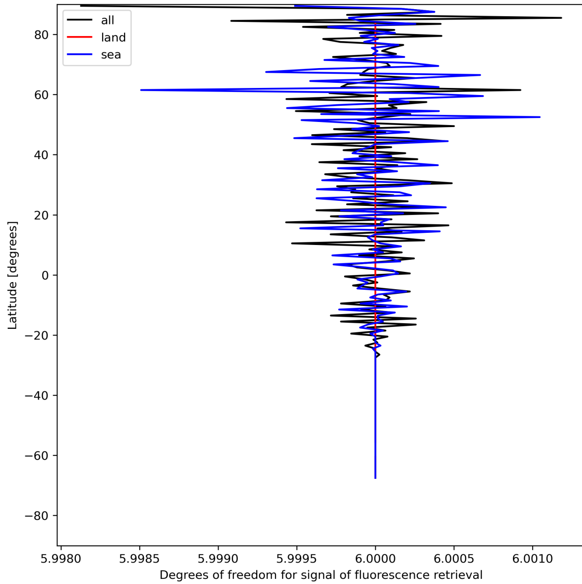
Figure 26: Zonal average of “Degrees of freedom for signal of fluorescence retrieval” for 2023-07-22 to 2023-07-24.
