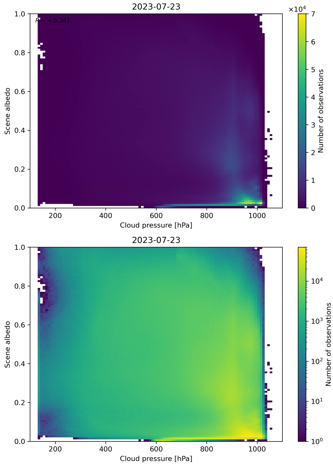
Figure 91: Scatter density plot of “Cloud pressure” against “Scene albedo” for 2023-07-22 to 2023-07-24.
