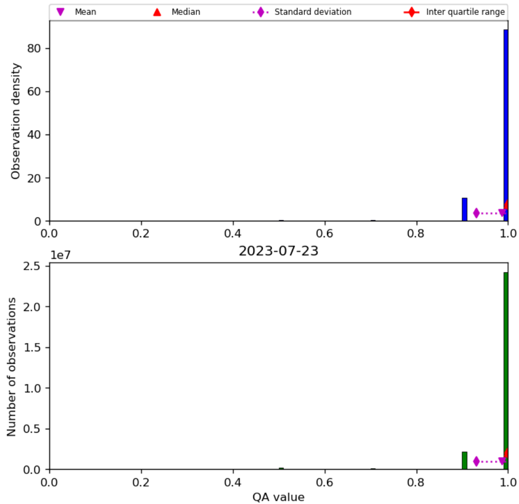
Figure 29: Histogram of “QA value” for 2023-07-22 to 2023-07-24
