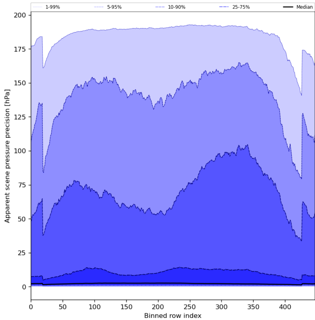
Figure 54: Along track statistics of “Apparent scene pressure precision” for 2023-07-22 to 2023-07-24
