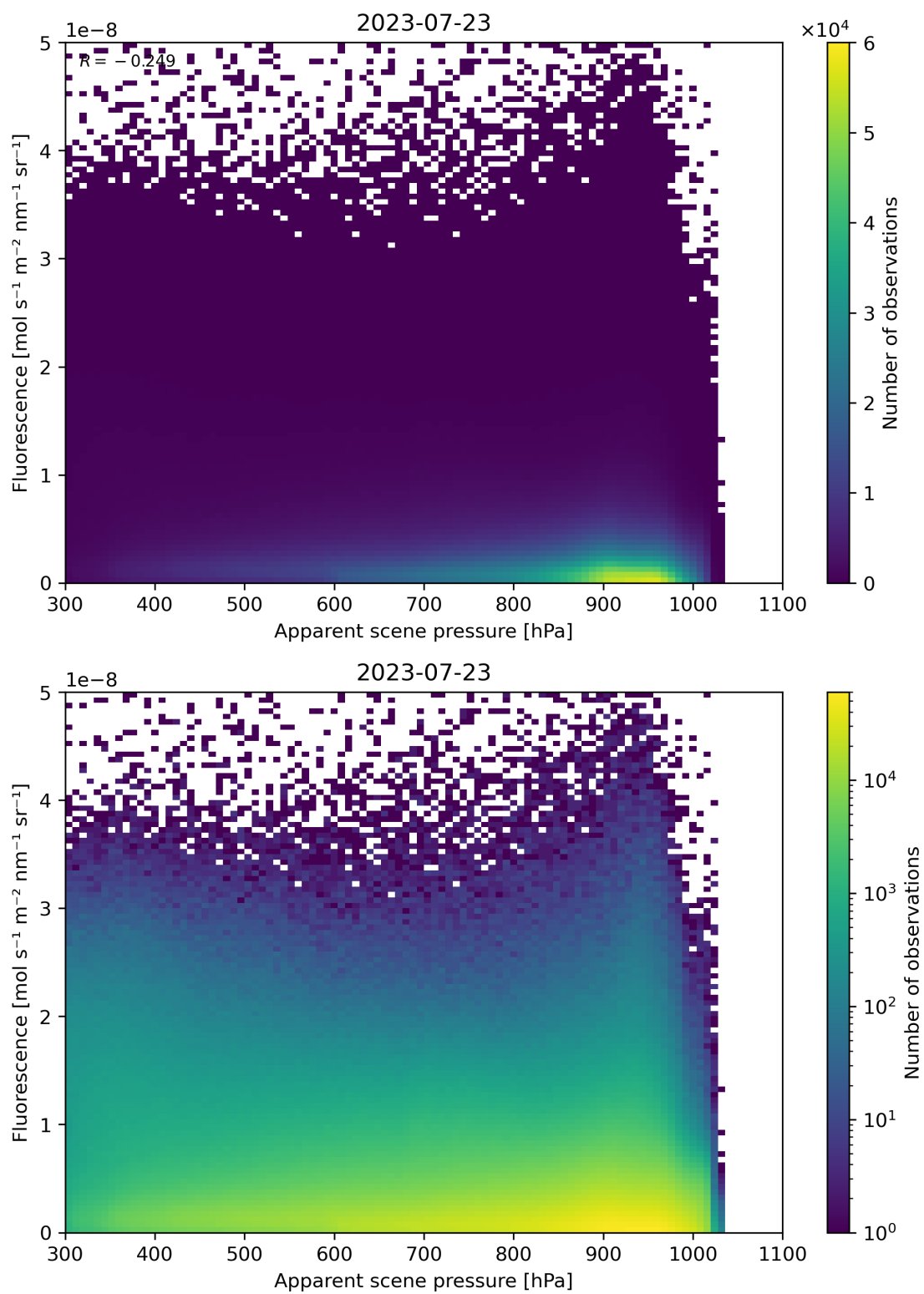
Figure 65: Scatter density plot of “Apparent scene pressure” against “Fluorescence” for 2023-07-22 to 2023-07-24.
