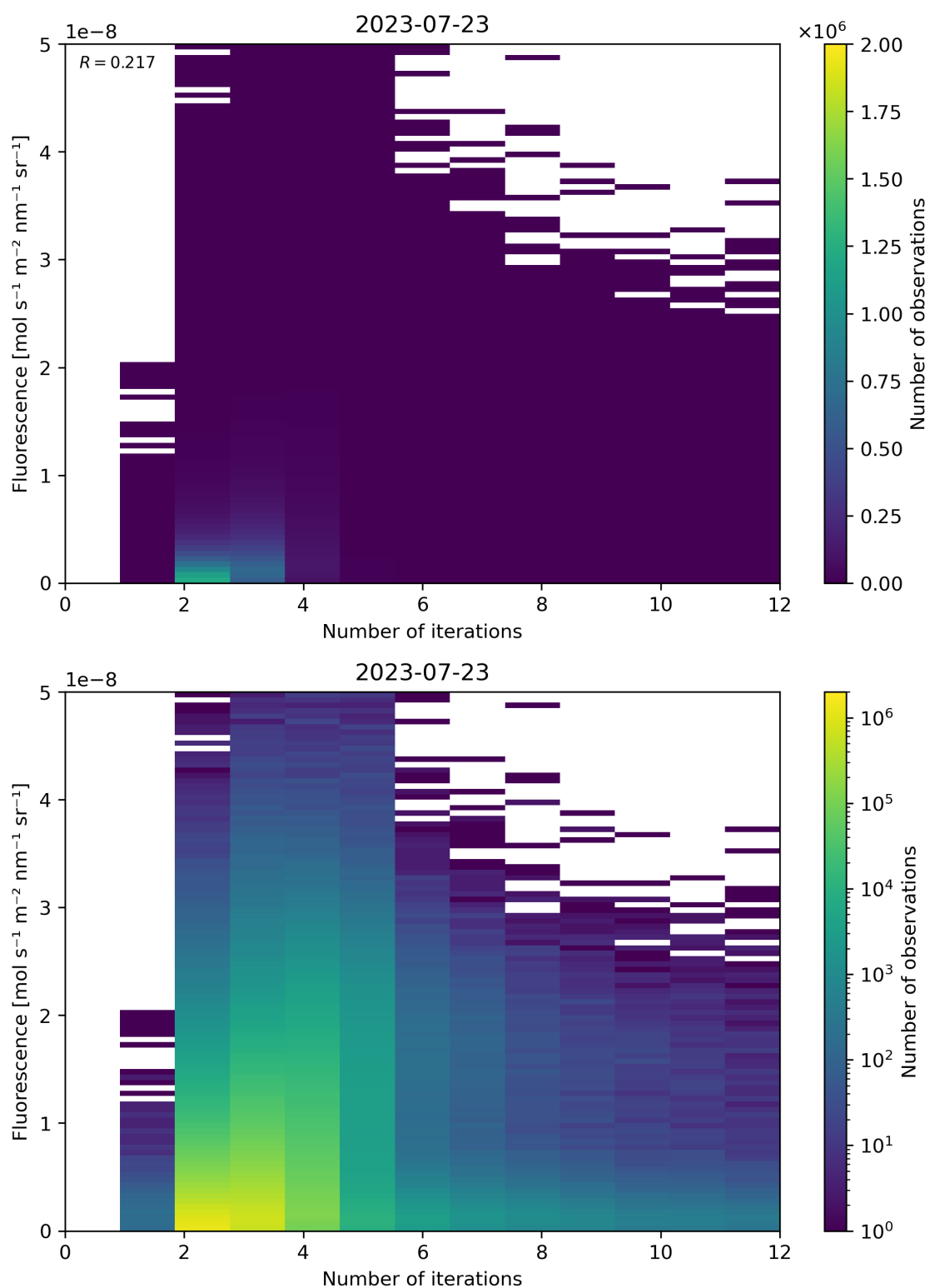
Figure 107: Scatter density plot of “Number of iterations” against “Fluorescence” for 2023-07-22 to 2023-07-24.
