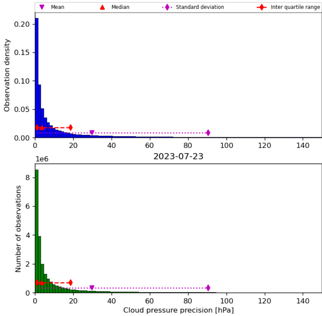
Figure 31: Histogram of “Cloud pressure precision” for 2023-07-22 to 2023-07-24
