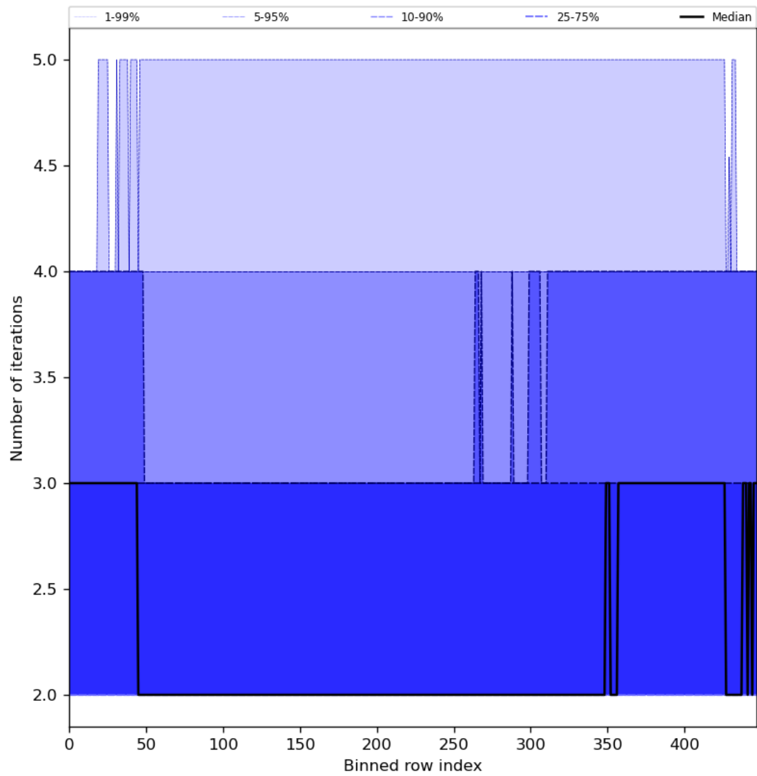
Figure 56: Along track statistics of “Number of iterations” for 2023-07-22 to 2023-07-24
