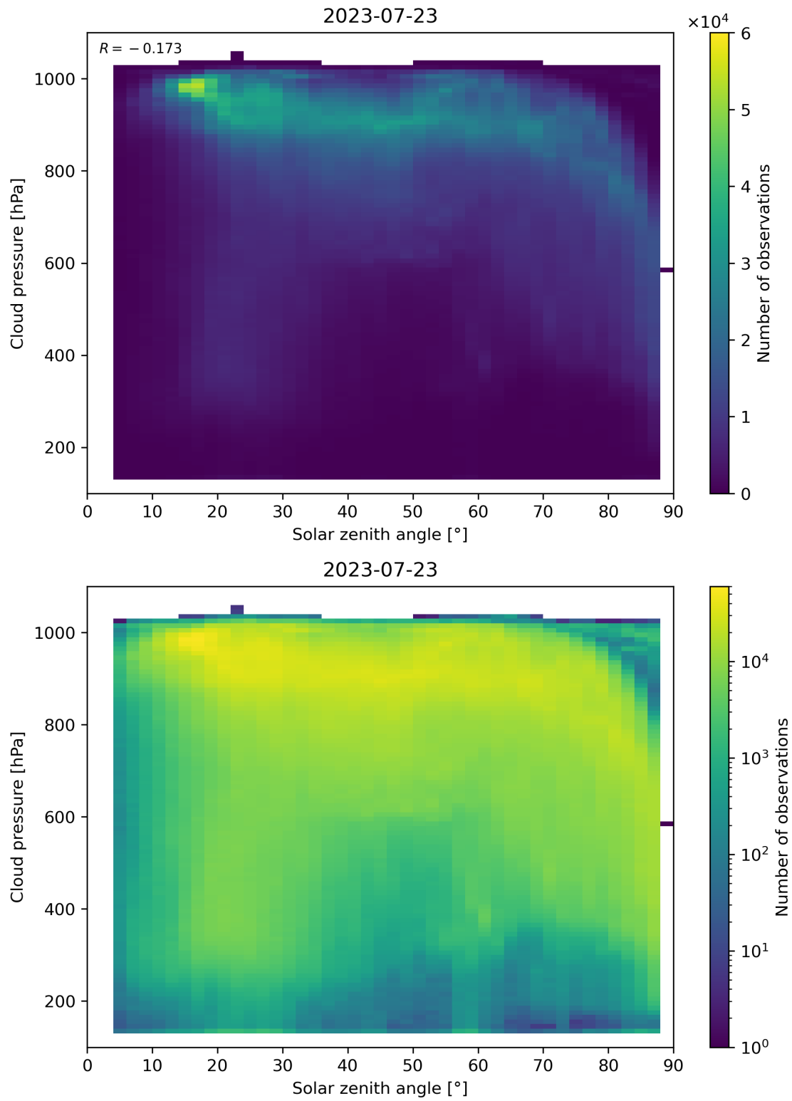
Figure 122: Scatter density plot of “Solar zenith angle” against “Cloud pressure” for 2023-07-22 to 2023-07-24.
