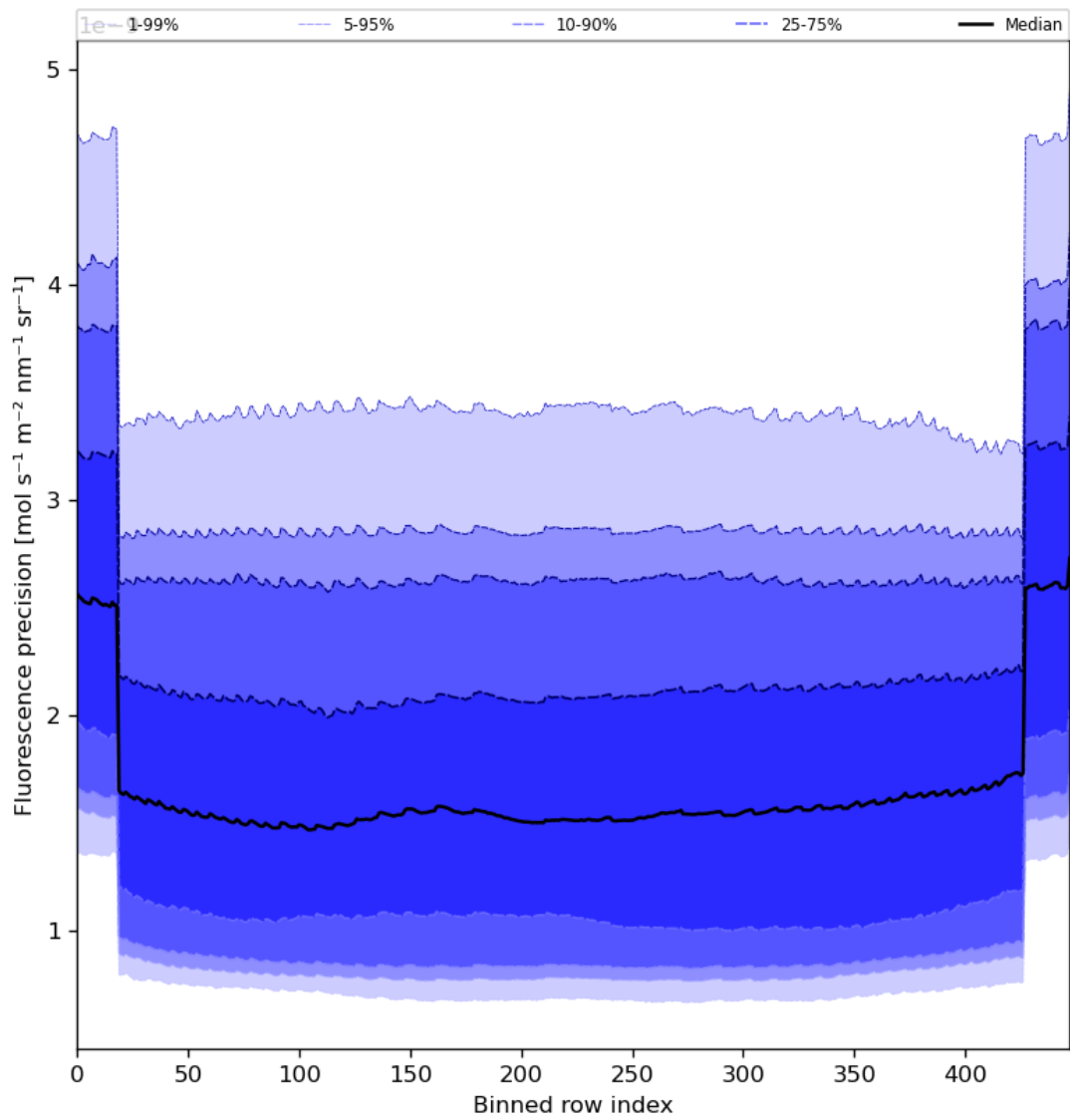
Figure 58: Along track statistics of “Fluorescence precision” for 2023-07-22 to 2023-07-24
