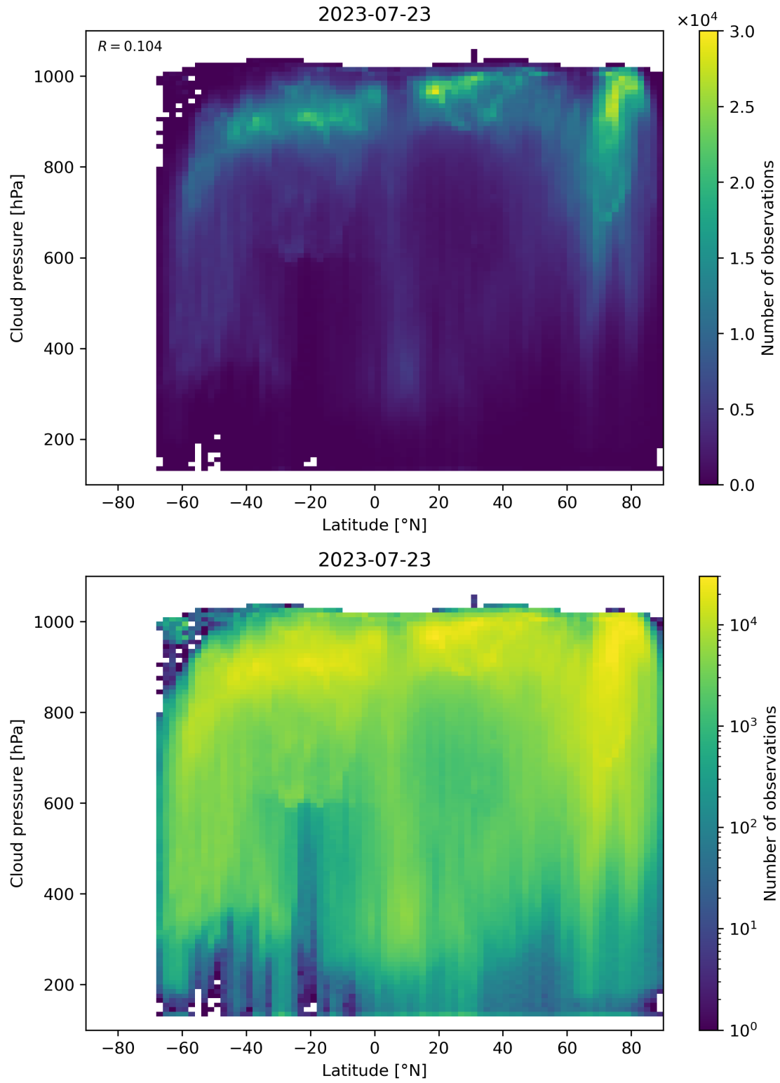
Figure 100: Scatter density plot of “Latitude” against “Cloud pressure” for 2023-07-22 to 2023-07-24.
