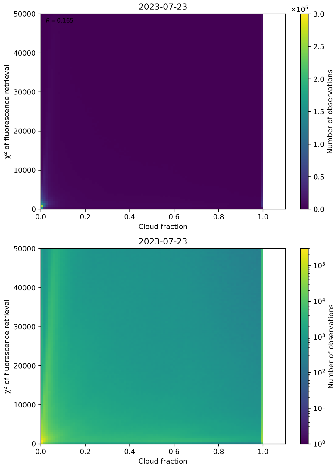
Figure 78: Scatter density plot of “Cloud fraction” against “ \chi^2 of fluorescence retrieval” for 2023-07-22 to 2023-07-24.
