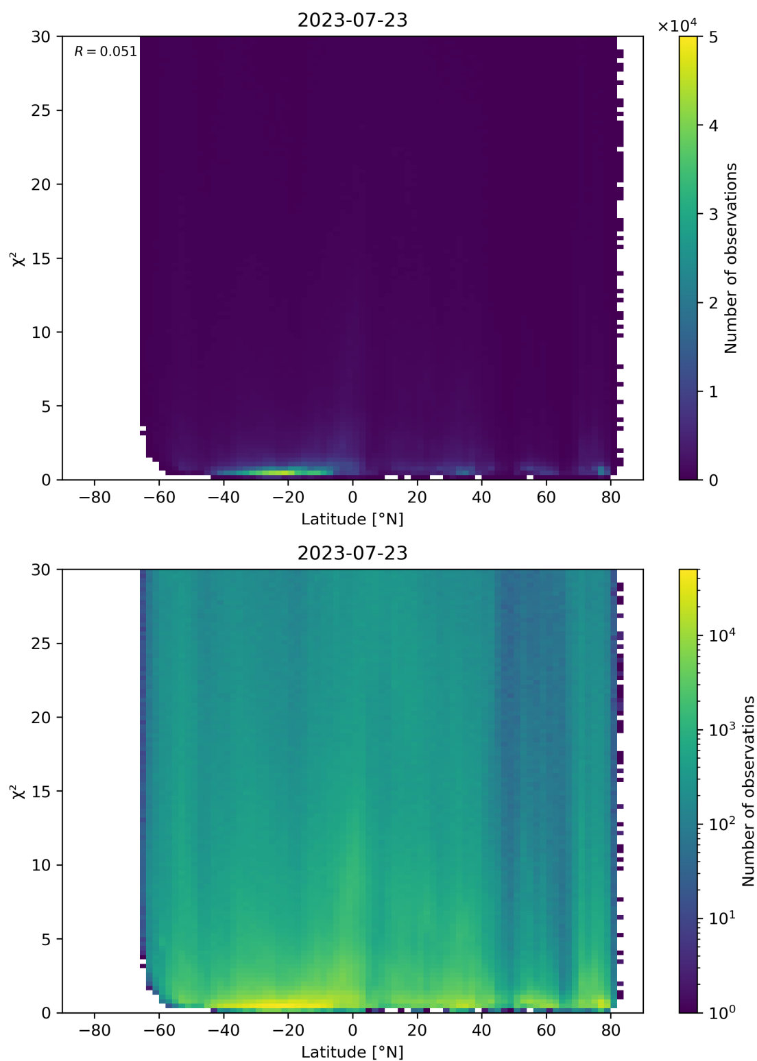
Figure 97: Scatter density plot of “Latitude” against “ \chi^2 ” for 2023-07-22 to 2023-07-24.
