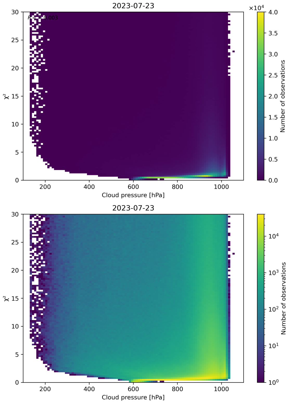
Figure 85: Scatter density plot of “Cloud pressure” against “ \chi^2 ” for 2023-07-22 to 2023-07-24.
