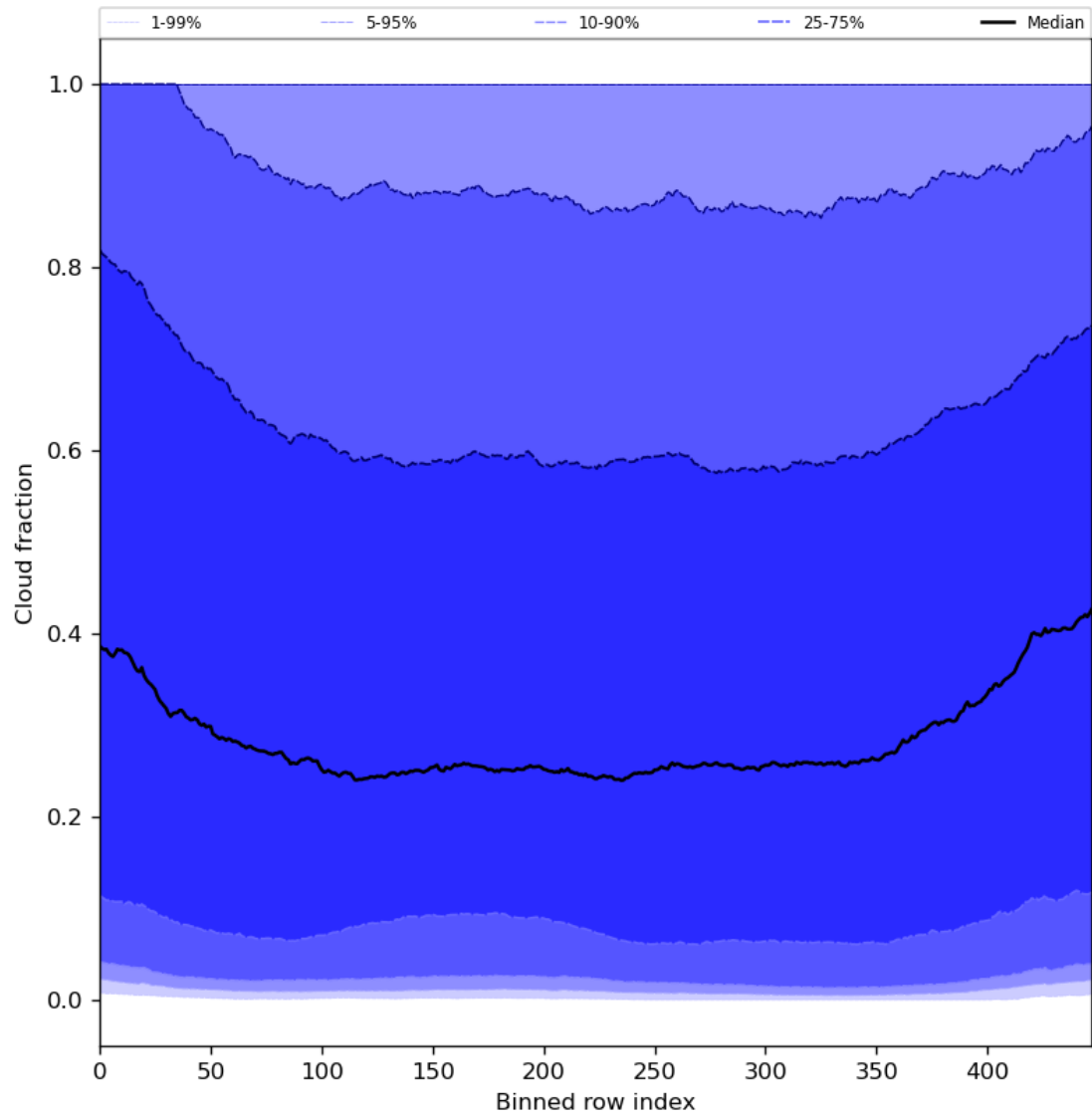
Figure 49: Along track statistics of “Cloud fraction” for 2023-07-22 to 2023-07-24
