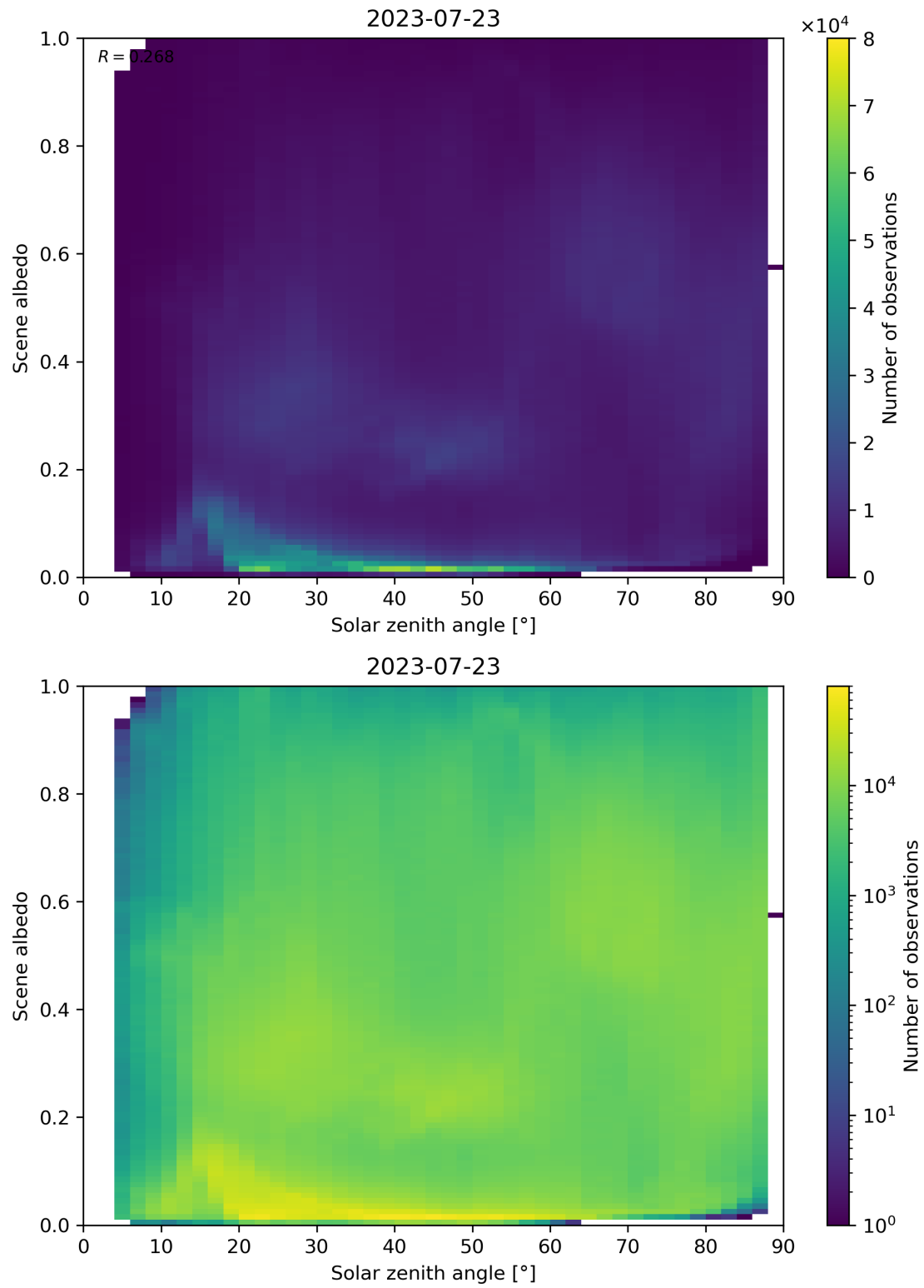
Figure 127: Scatter density plot of “Solar zenith angle” against “Scene albedo” for 2023-07-22 to 2023-07-24.
