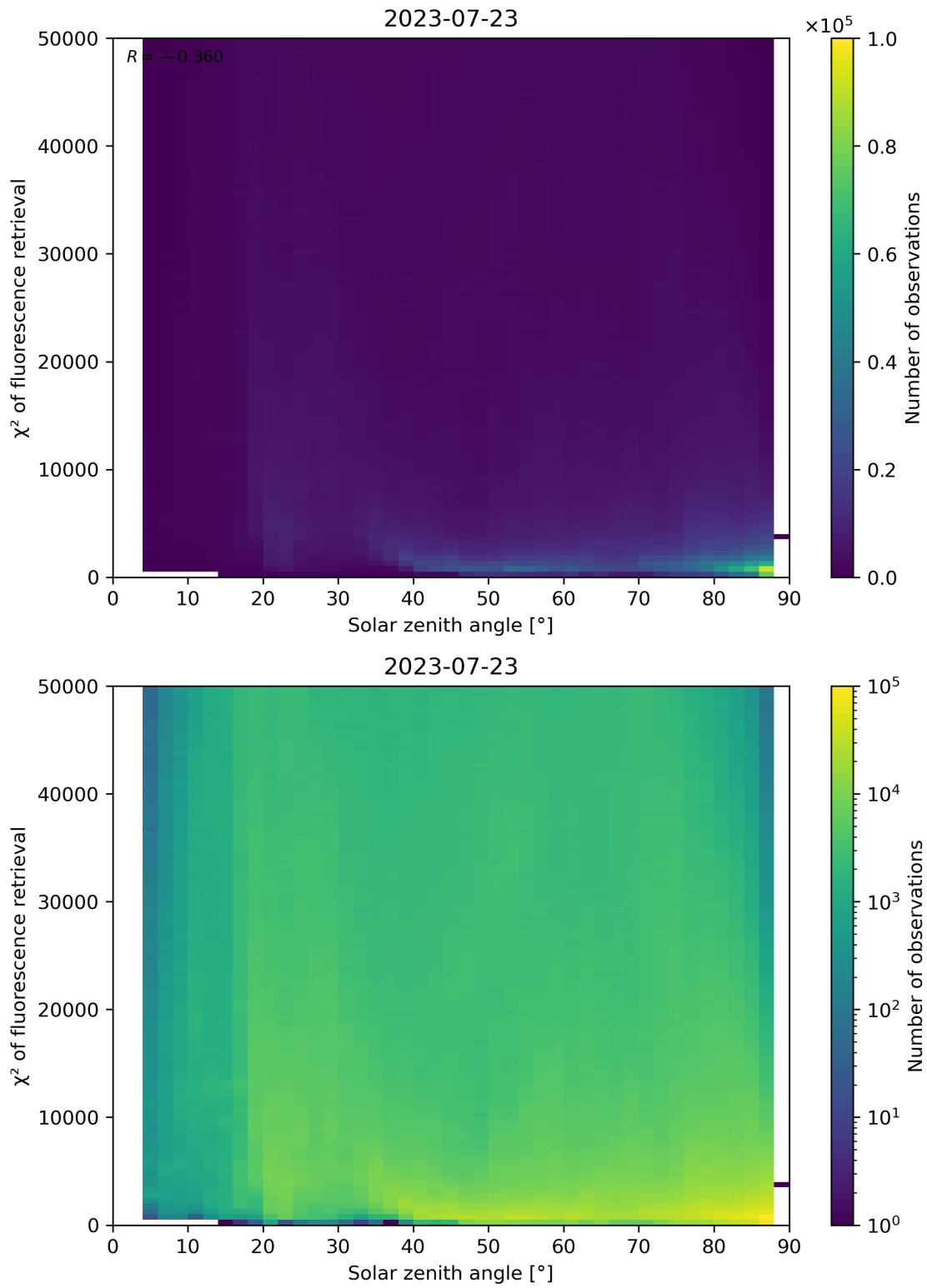
Figure 120: Scatter density plot of “Solar zenith angle” against “ \chi^2 of fluorescence retrieval” for 2023-07-22 to 2023-07-24.
