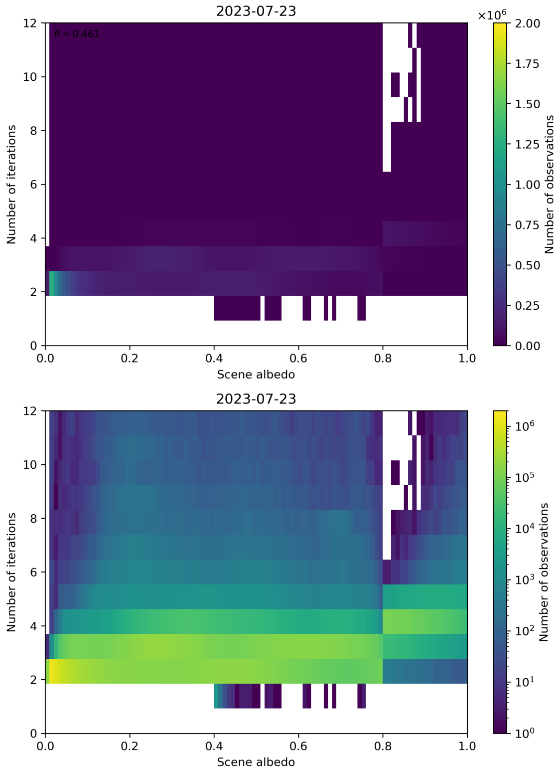
Figure 115: Scatter density plot of “Scene albedo” against “Number of iterations” for 2023-07-22 to 2023-07-24.
