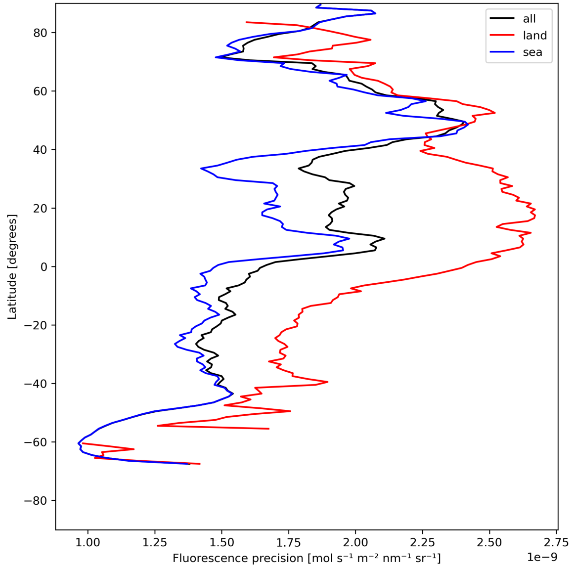
Figure 24: Zonal average of “Fluorescence precision” for 2023-07-22 to 2023-07-24.
