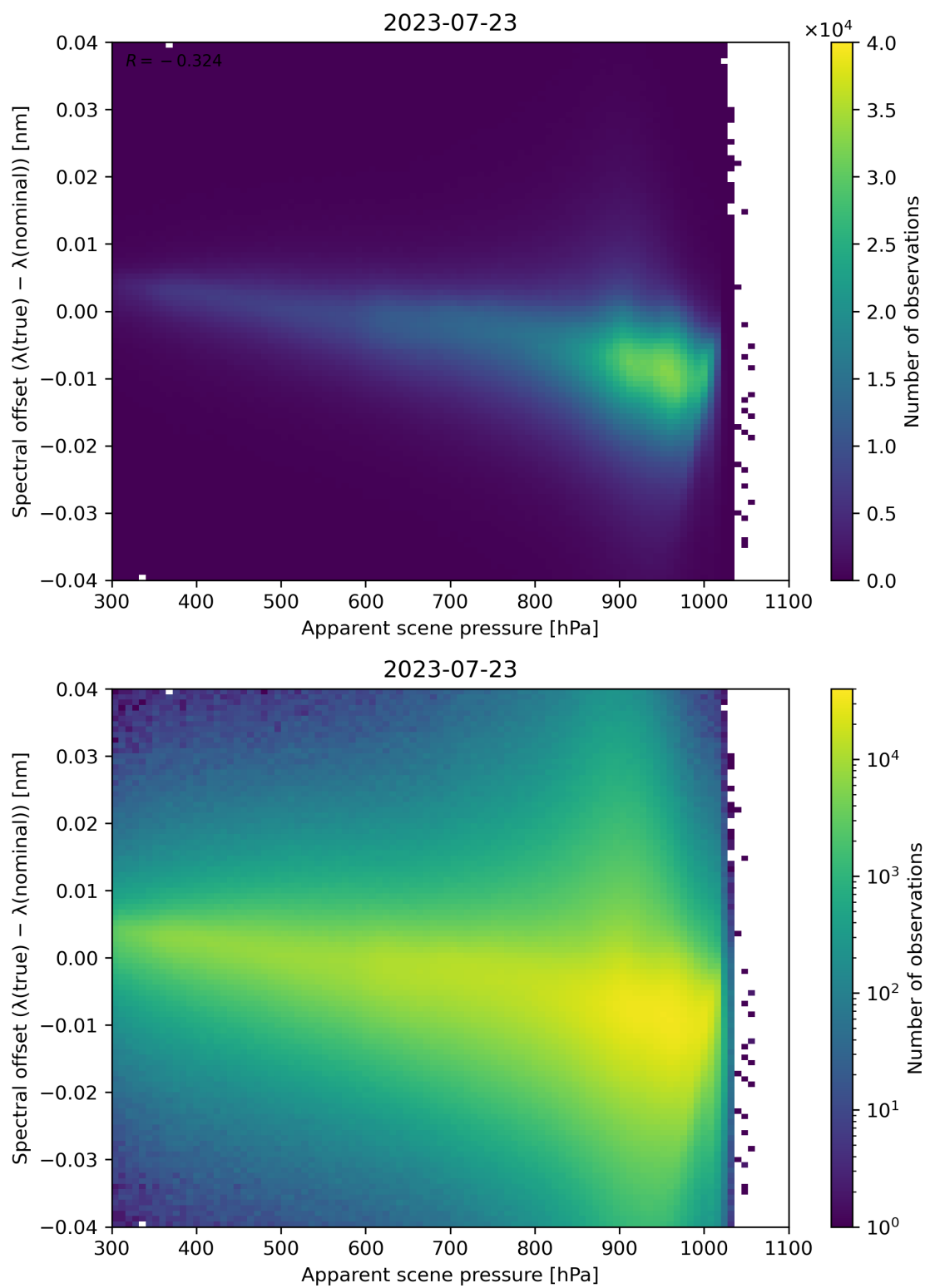
Figure 68: Scatter density plot of “Apparent scene pressure” against “Spectral offset ( \lambda(\text{true}) - \lambda(\text{nominal}) )” for 2023-07-22 to 2023-07-24.
