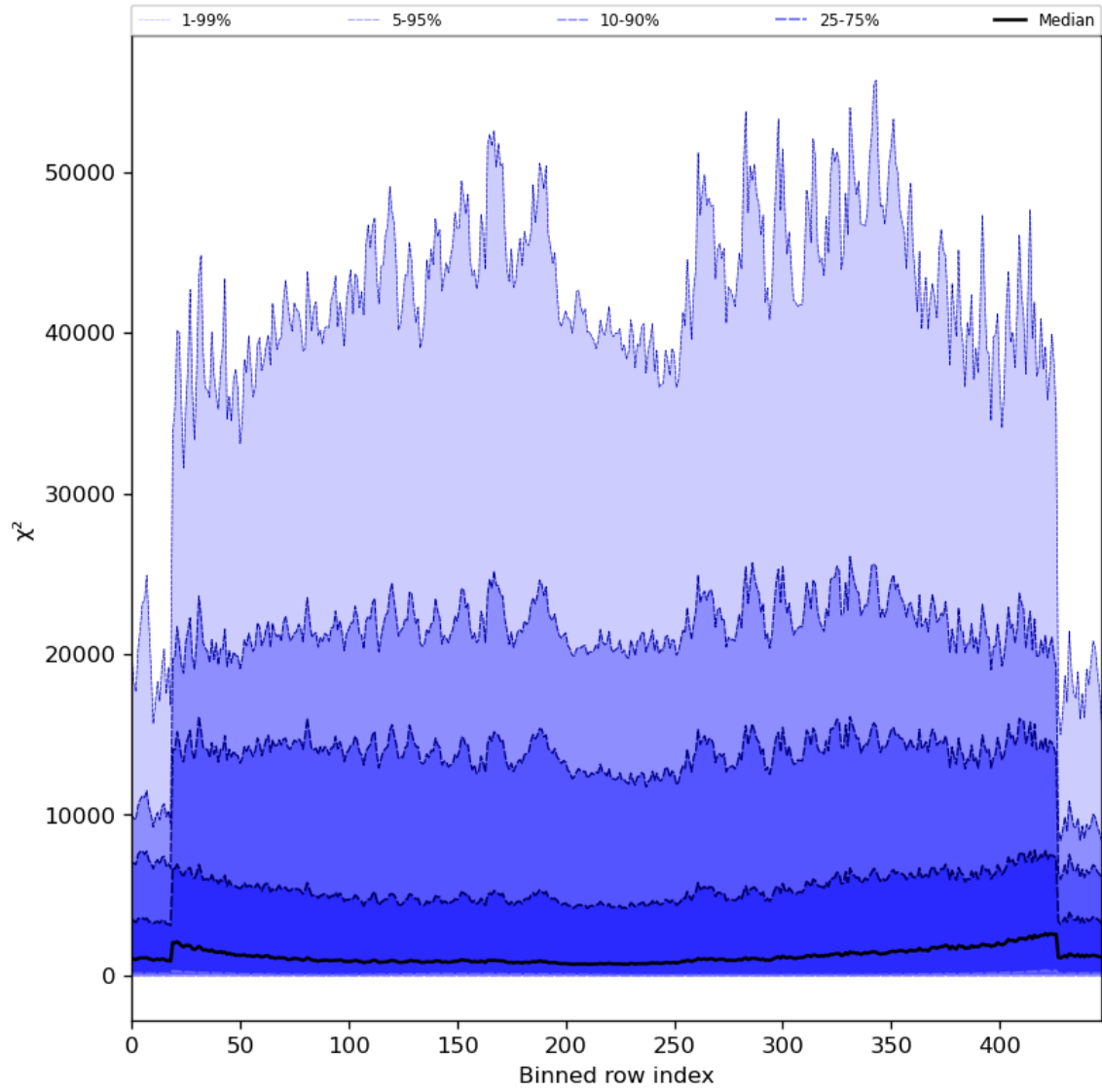
Figure 55: Along track statistics of “ \chi^2 ” for 2023-07-22 to 2023-07-24
