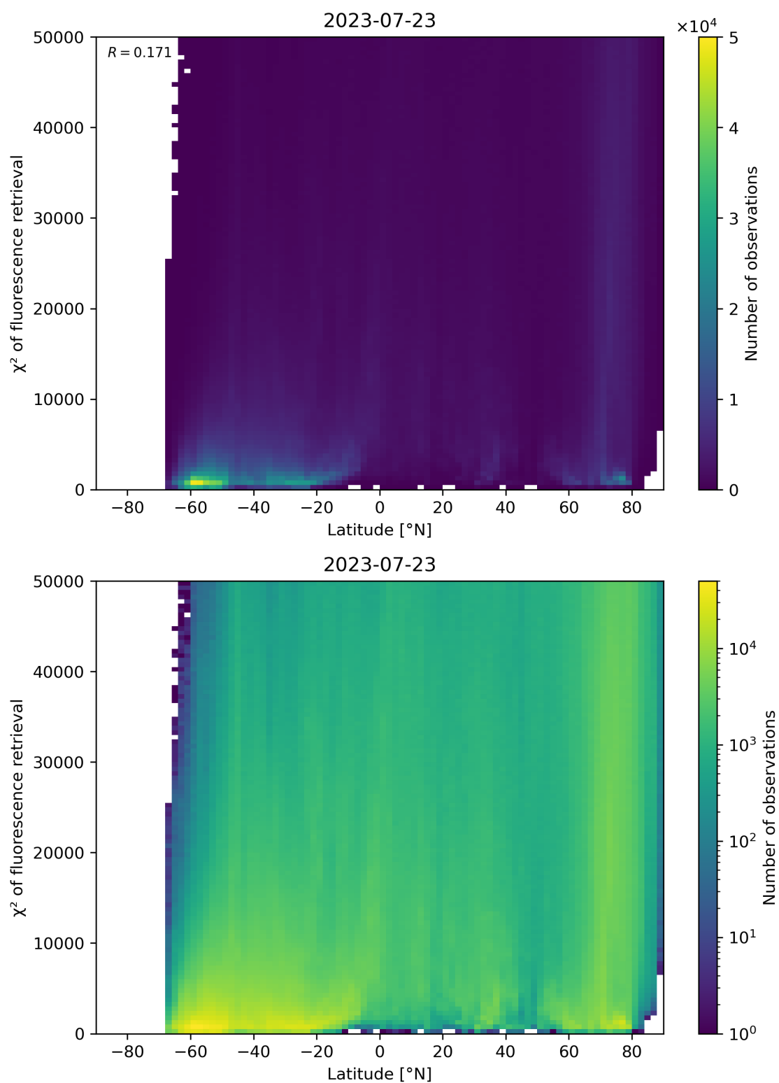
Figure 98: Scatter density plot of “Latitude” against “ \chi^2 of fluorescence retrieval” for 2023-07-22 to 2023-07-24.
