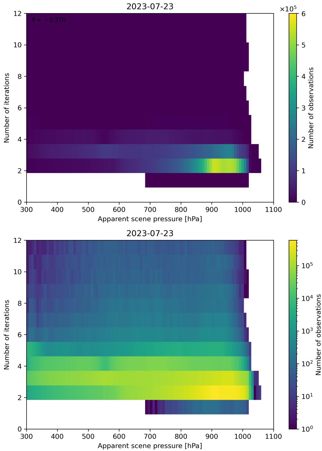
Figure 66: Scatter density plot of “Apparent scene pressure” against “Number of iterations” for 2023-07-22 to 2023-07-24.
