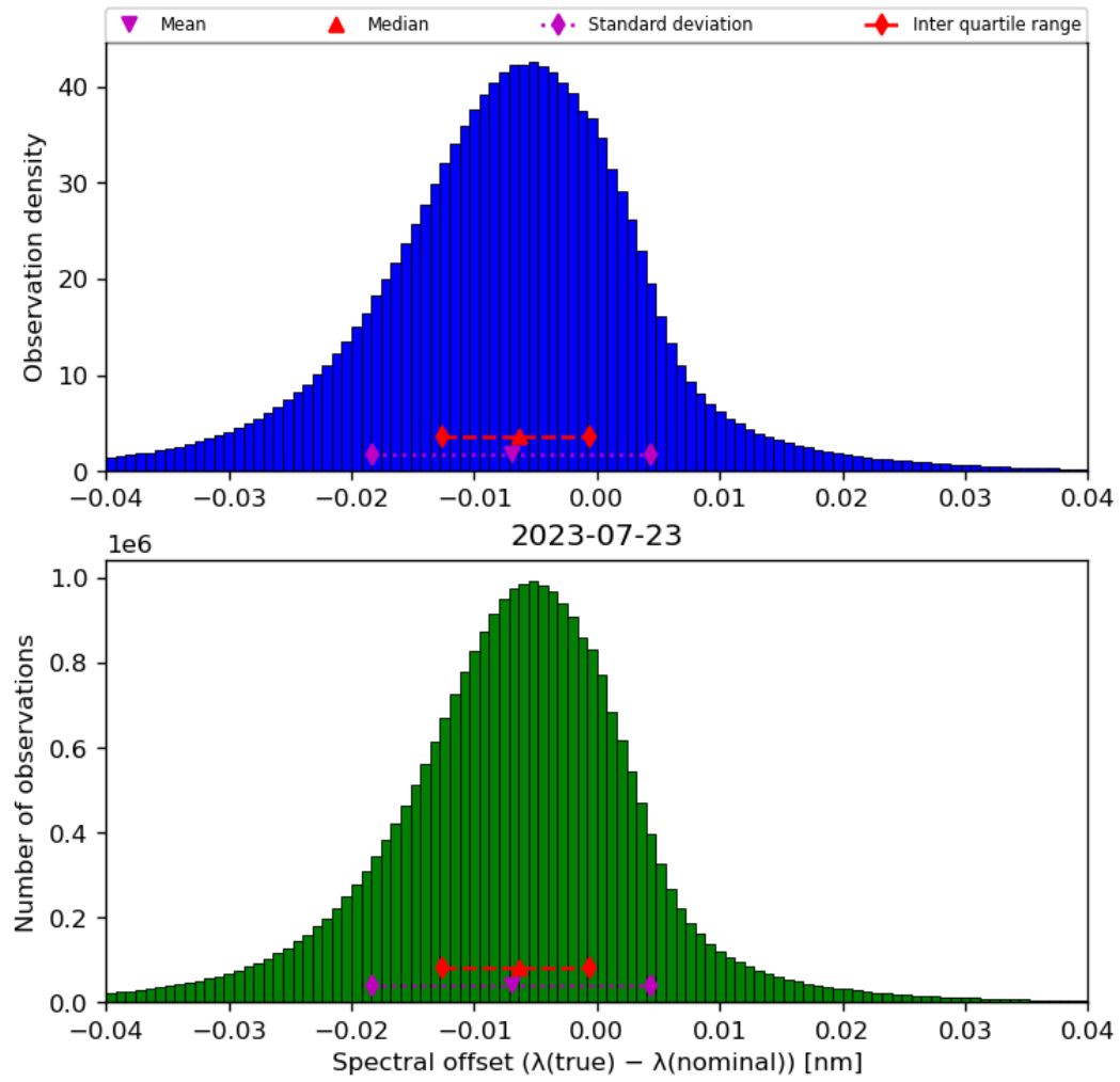
Figure 45: Histogram of “Spectral offset ( \lambda(\text{true}) - \lambda(\text{nominal}) )” for 2023-07-22 to 2023-07-24
