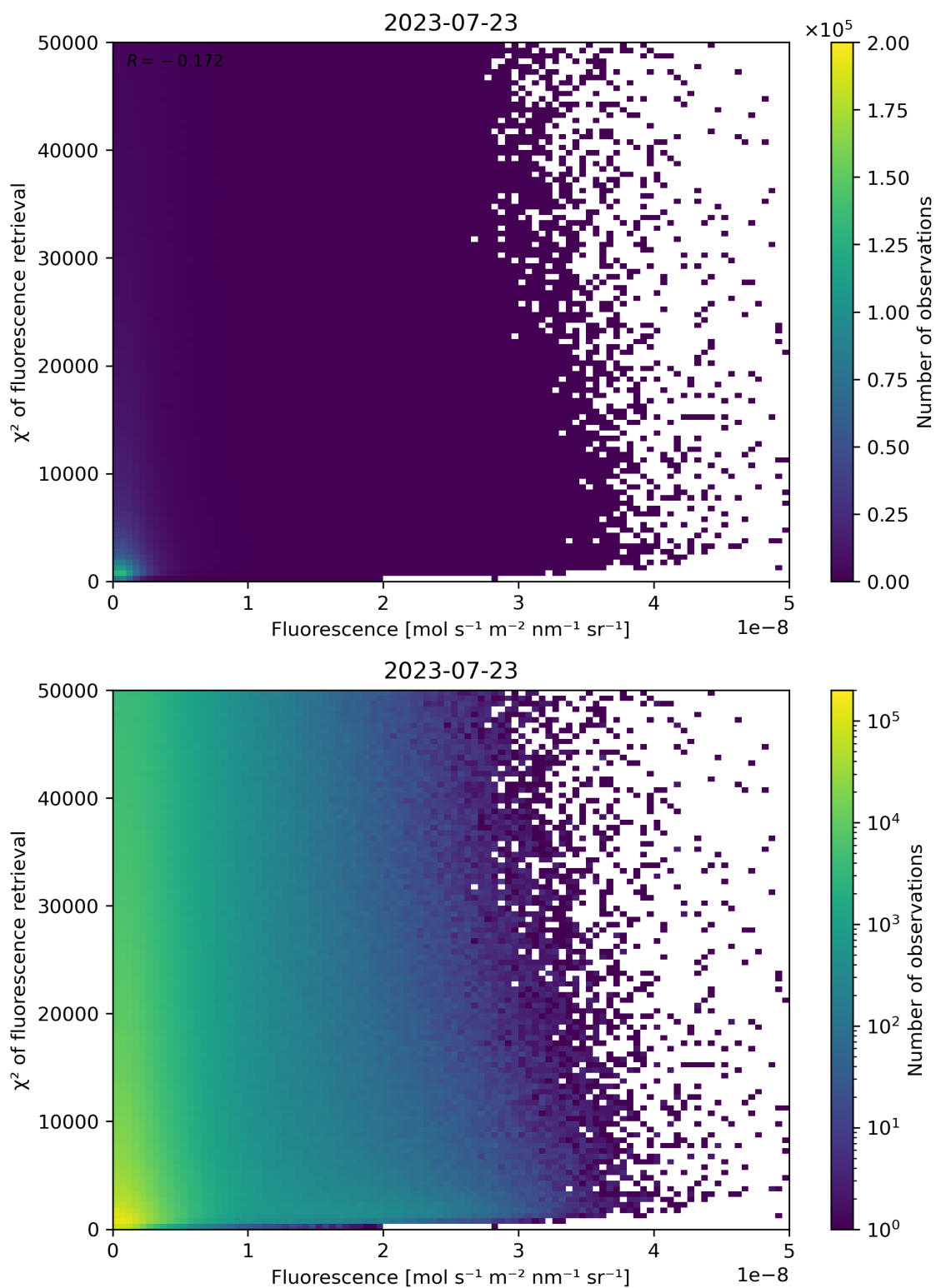
Figure 93: Scatter density plot of “Fluorescence” against “ \chi^2 of fluorescence retrieval” for 2023-07-22 to 2023-07-24.
