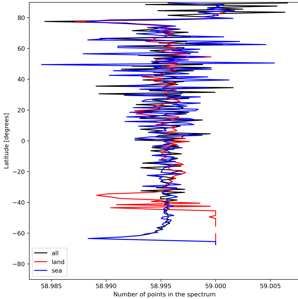
Figure 27: Zonal average of “Number of points in the spectrum” for 2023-07-22 to 2023-07-24.
