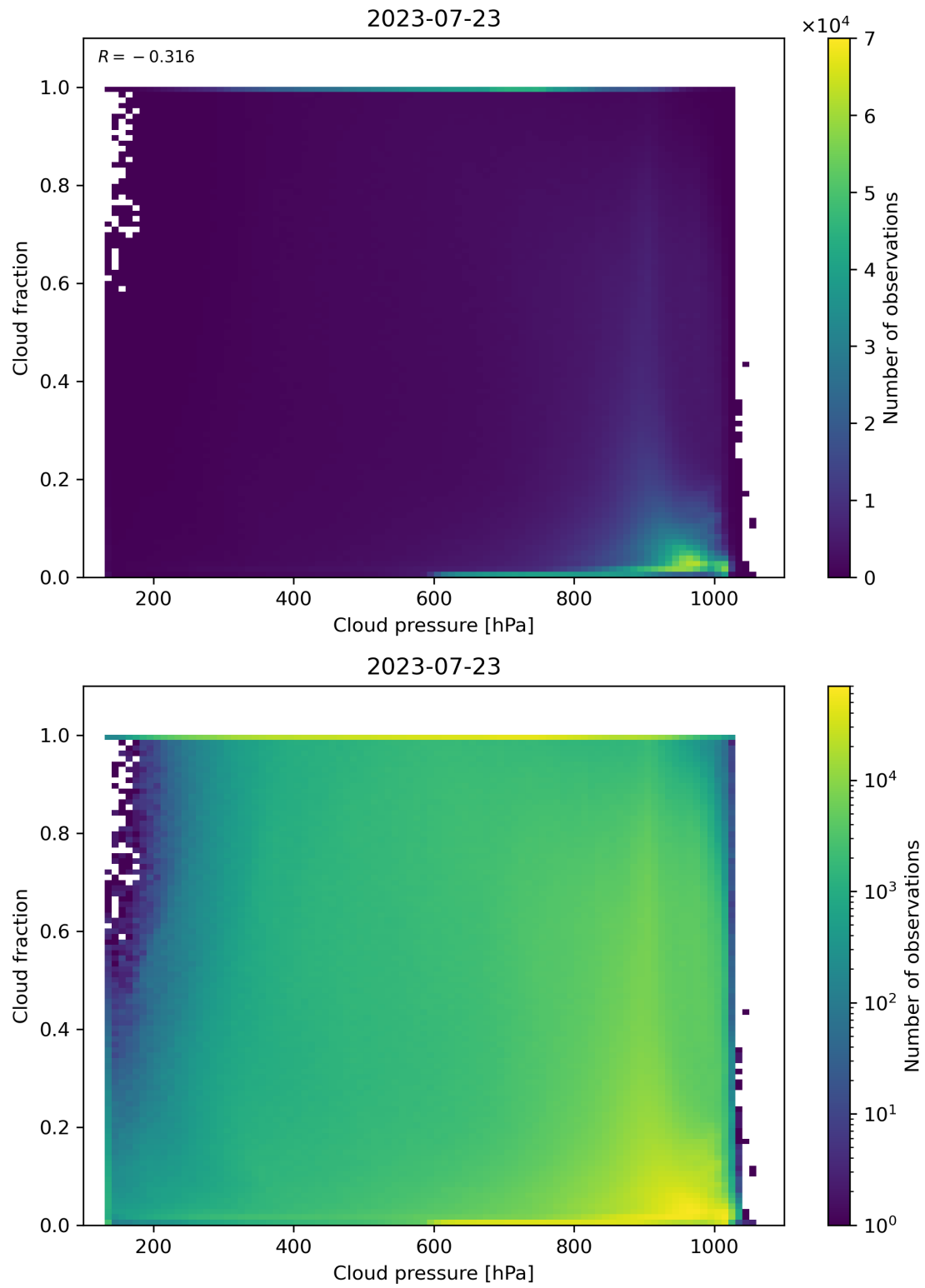
Figure 87: Scatter density plot of “Cloud pressure” against “Cloud fraction” for 2023-07-22 to 2023-07-24.
