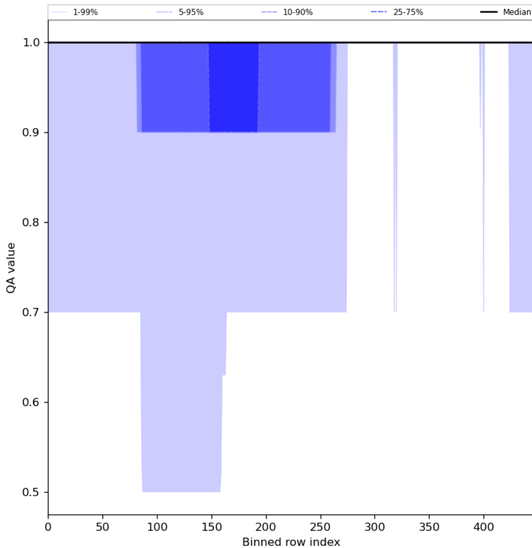
Figure 46: Along track statistics of “QA value” for 2023-07-22 to 2023-07-24
