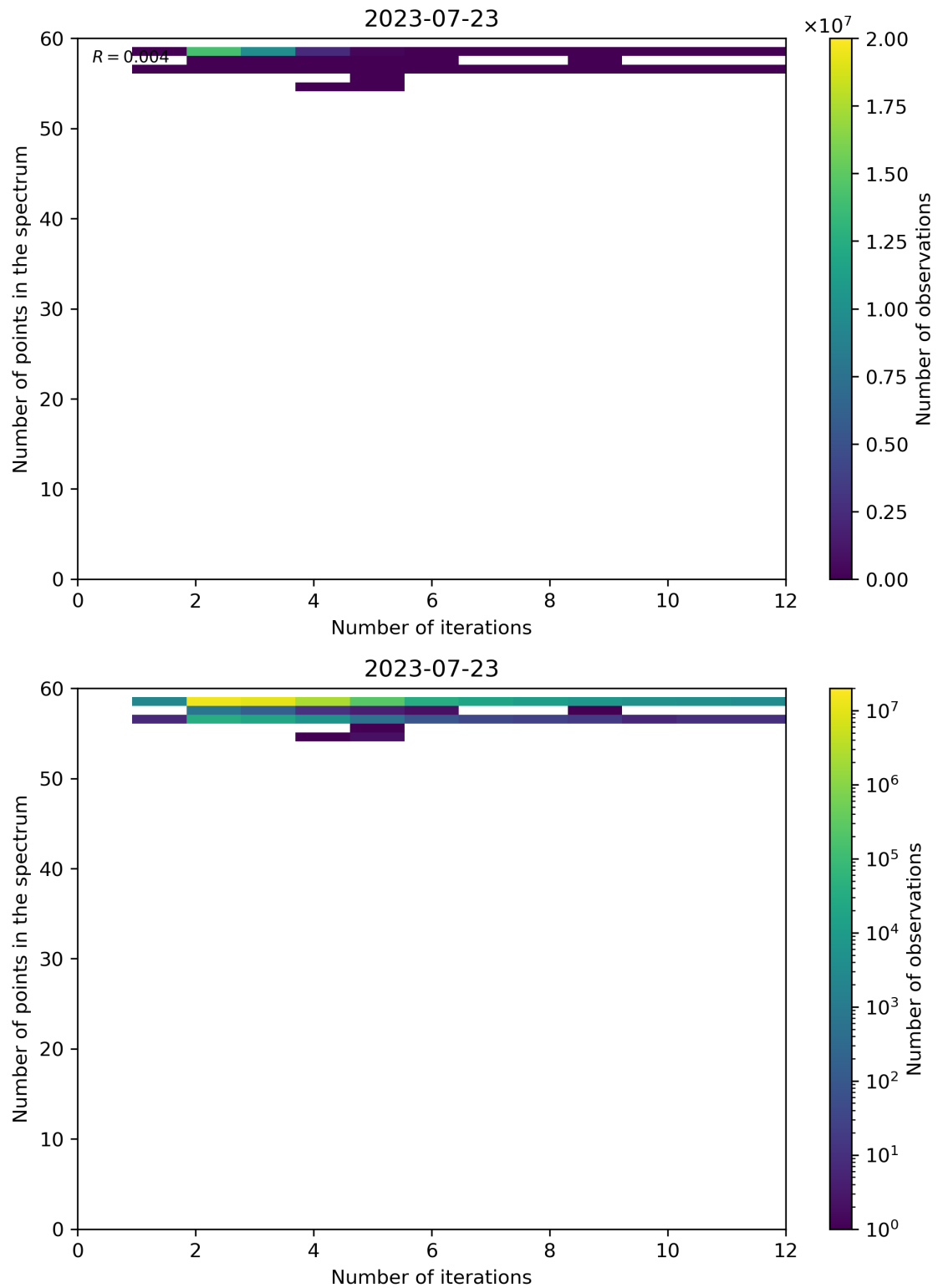
Figure 108: Scatter density plot of “Number of iterations” against “Number of points in the spectrum” for 2023-07-22 to 2023-07-24.
