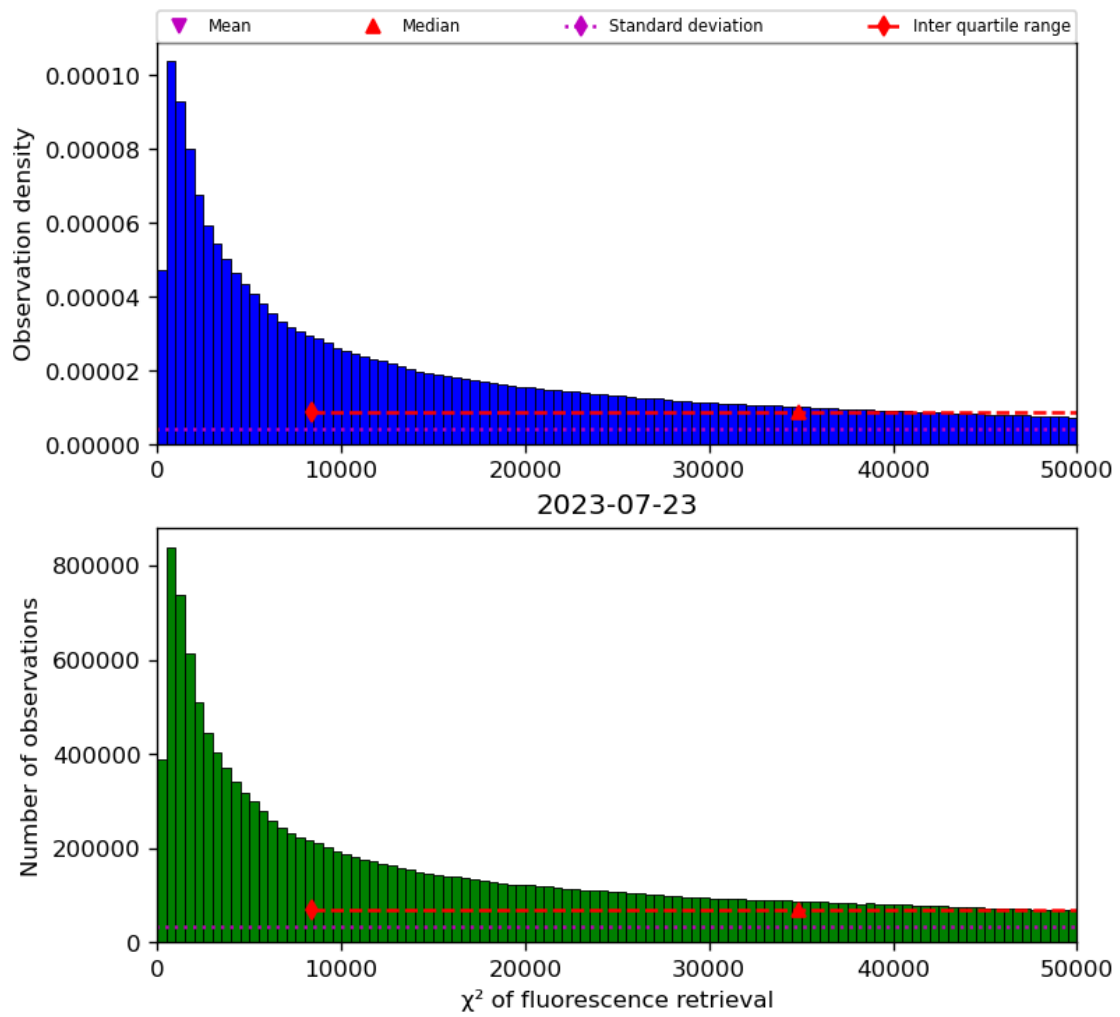
Figure 42: Histogram of “ \chi^2 of fluorescence retrieval” for 2023-07-22 to 2023-07-24
