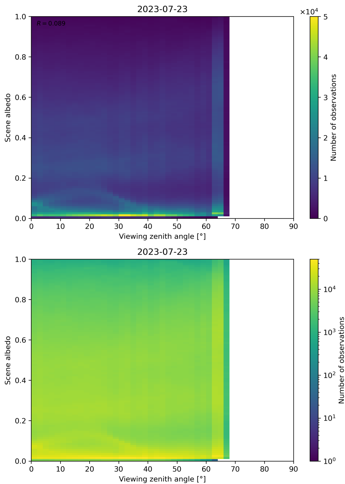
Figure 138: Scatter density plot of “Viewing zenith angle” against “Scene albedo” for 2023-07-22 to 2023-07-24.
