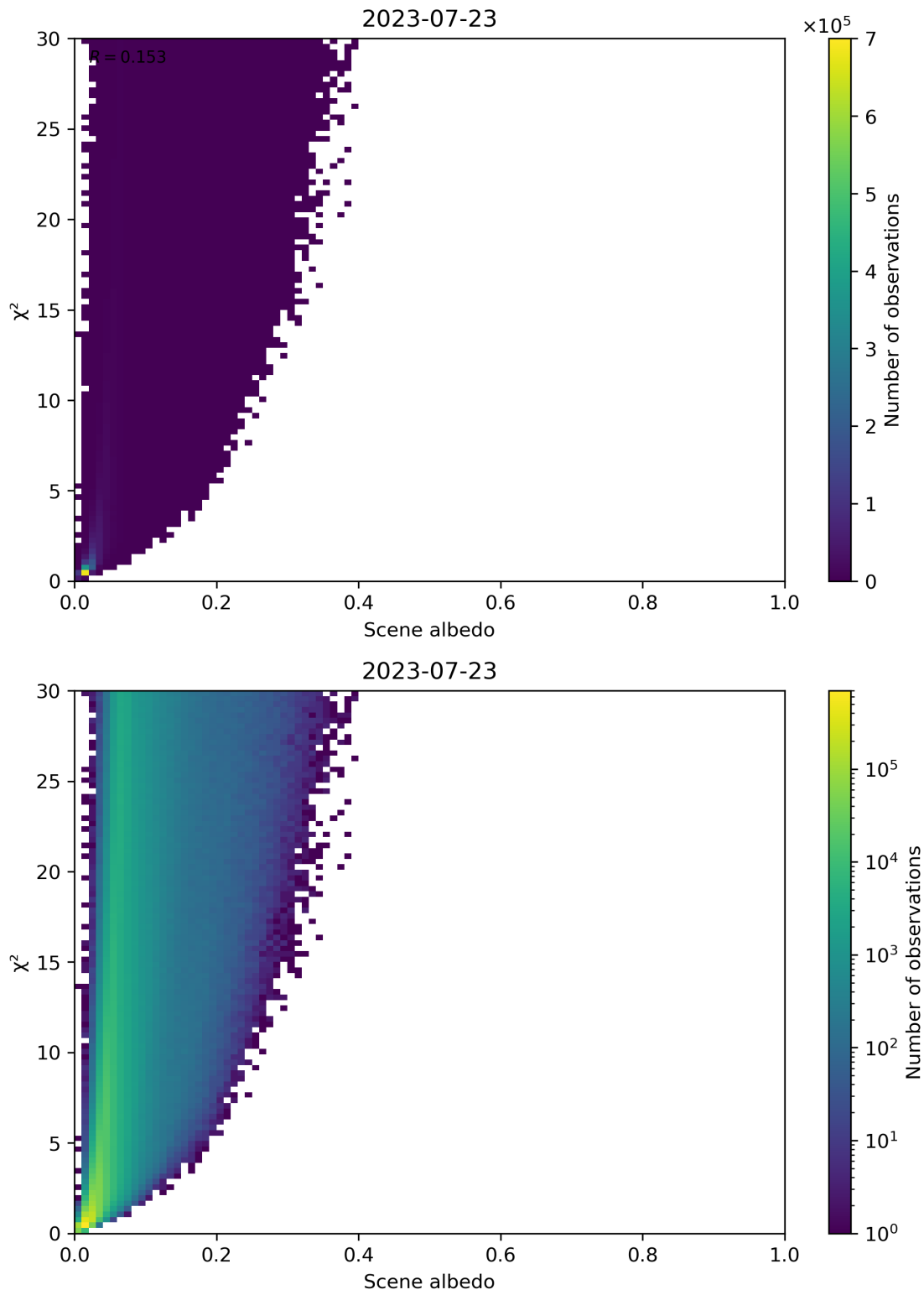
Figure 112: Scatter density plot of “Scene albedo” against “ \chi^2 ” for 2023-07-22 to 2023-07-24.
