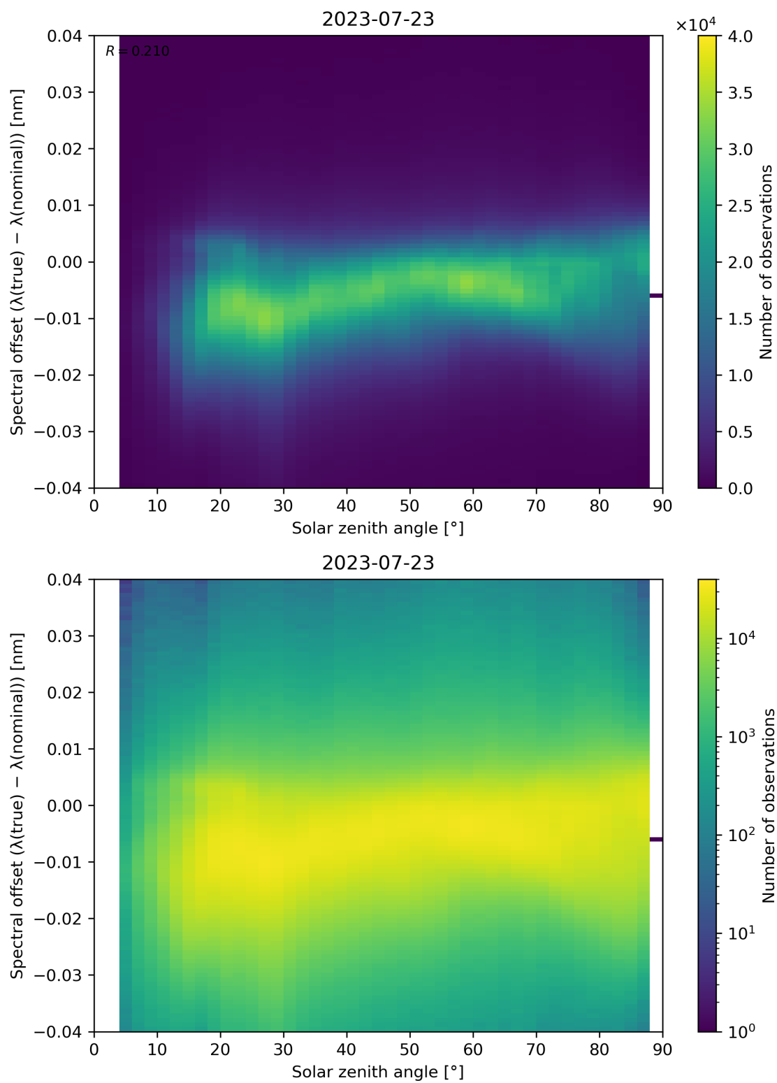
Figure 128: Scatter density plot of “Solar zenith angle” against “Spectral offset ( \lambda(\text{true}) - \lambda(\text{nominal}) )” for 2023-07-22 to 2023-07-24.
