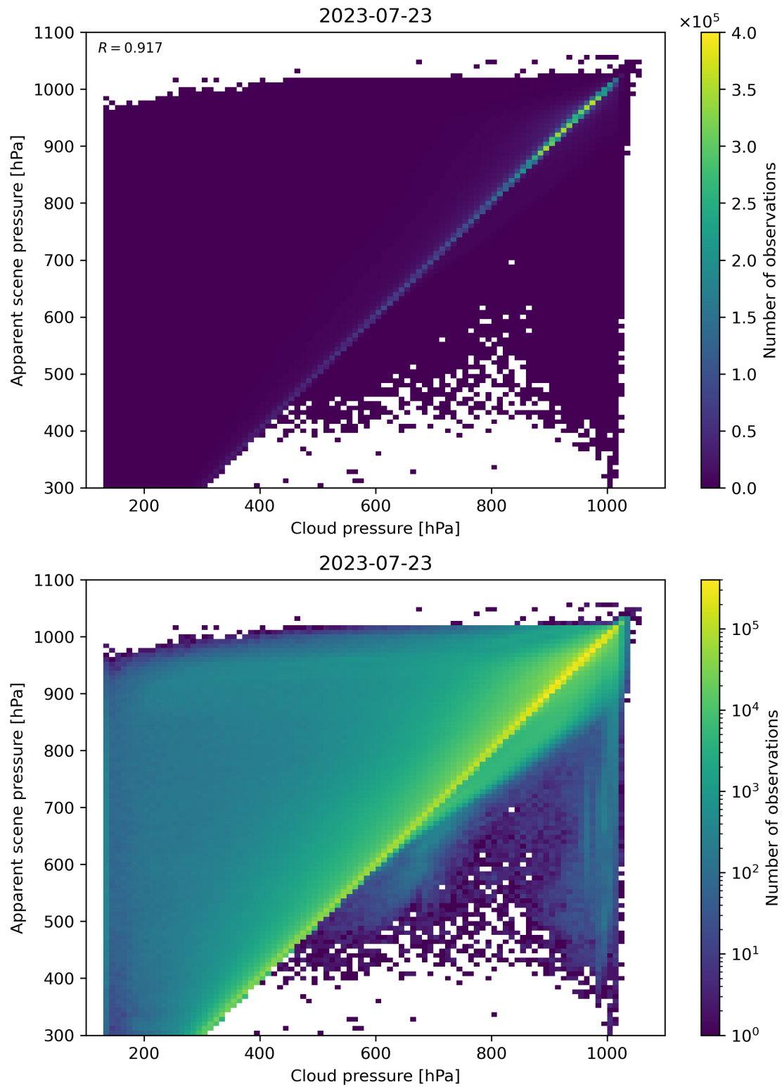
Figure 84: Scatter density plot of “Cloud pressure” against “Apparent scene pressure” for 2023-07-22 to 2023-07-24.
