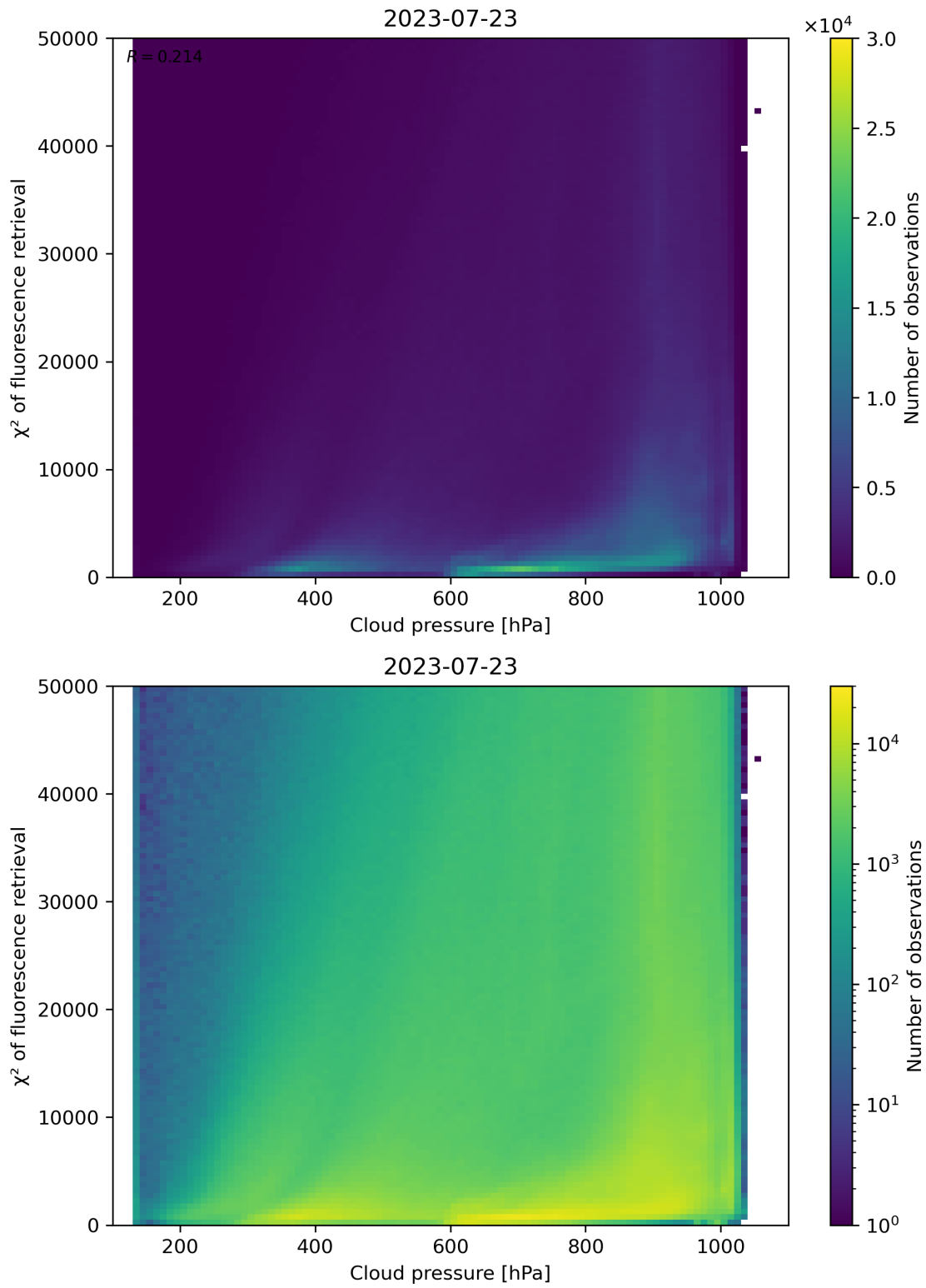
Figure 86: Scatter density plot of “Cloud pressure” against “ \chi^2 of fluorescence retrieval” for 2023-07-22 to 2023-07-24.
