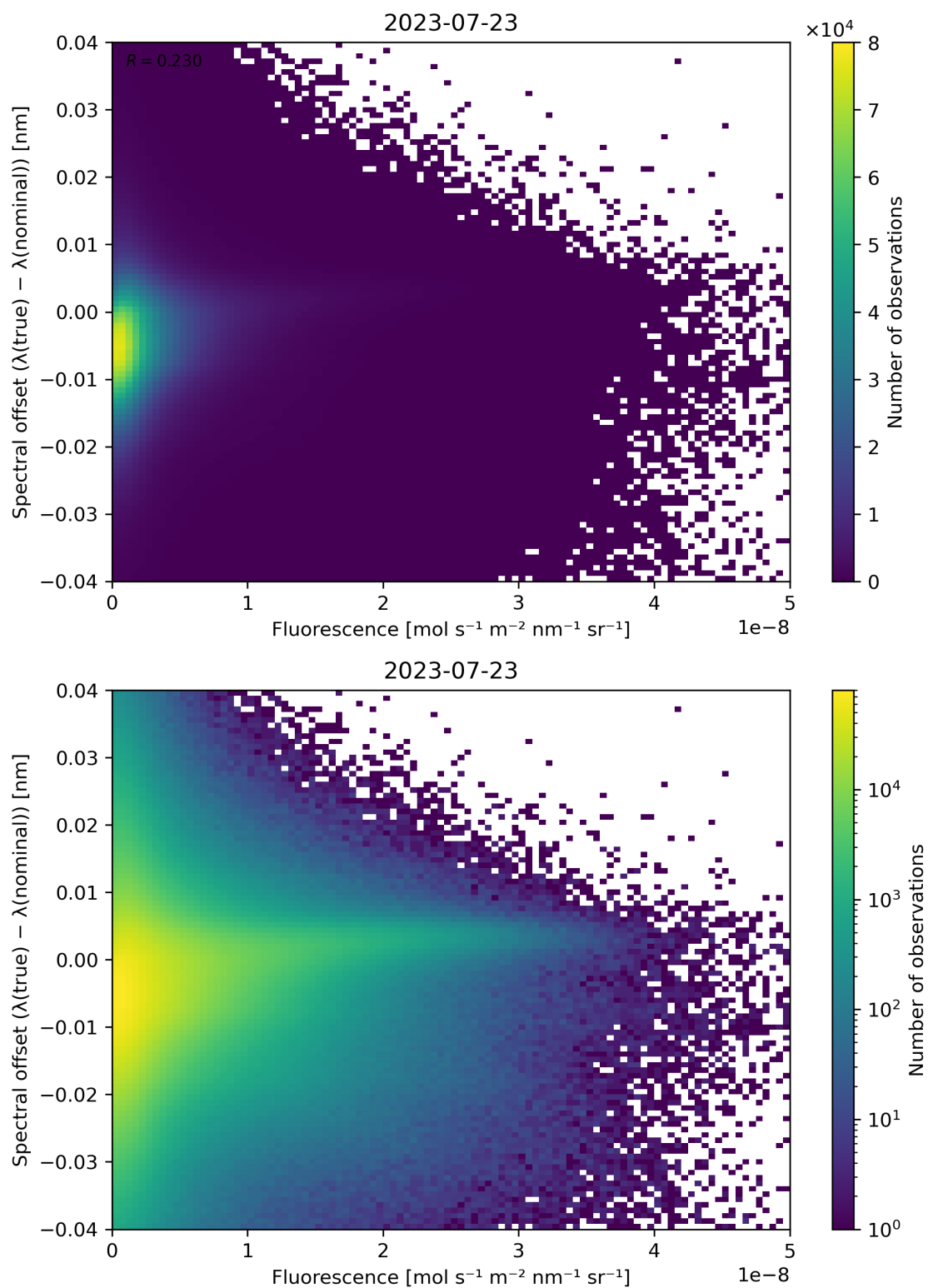
Figure 95: Scatter density plot of “Fluorescence” against “Spectral offset ( \lambda(\text{true}) - \lambda(\text{nominal}) )” for 2023-07-22 to 2023-07-24.
