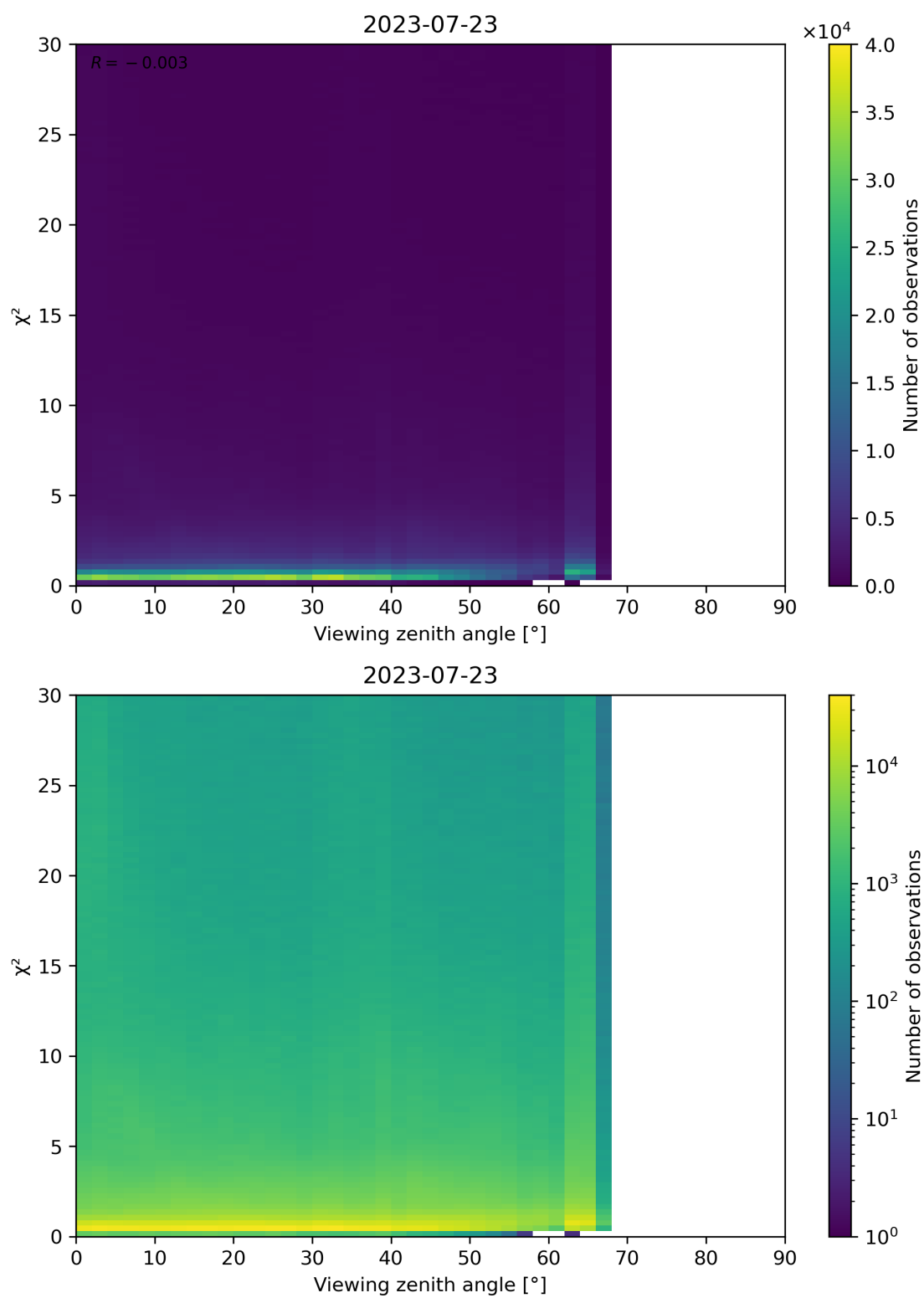
Figure 130: Scatter density plot of “Viewing zenith angle” against “ \chi^2 ” for 2023-07-22 to 2023-07-24.
