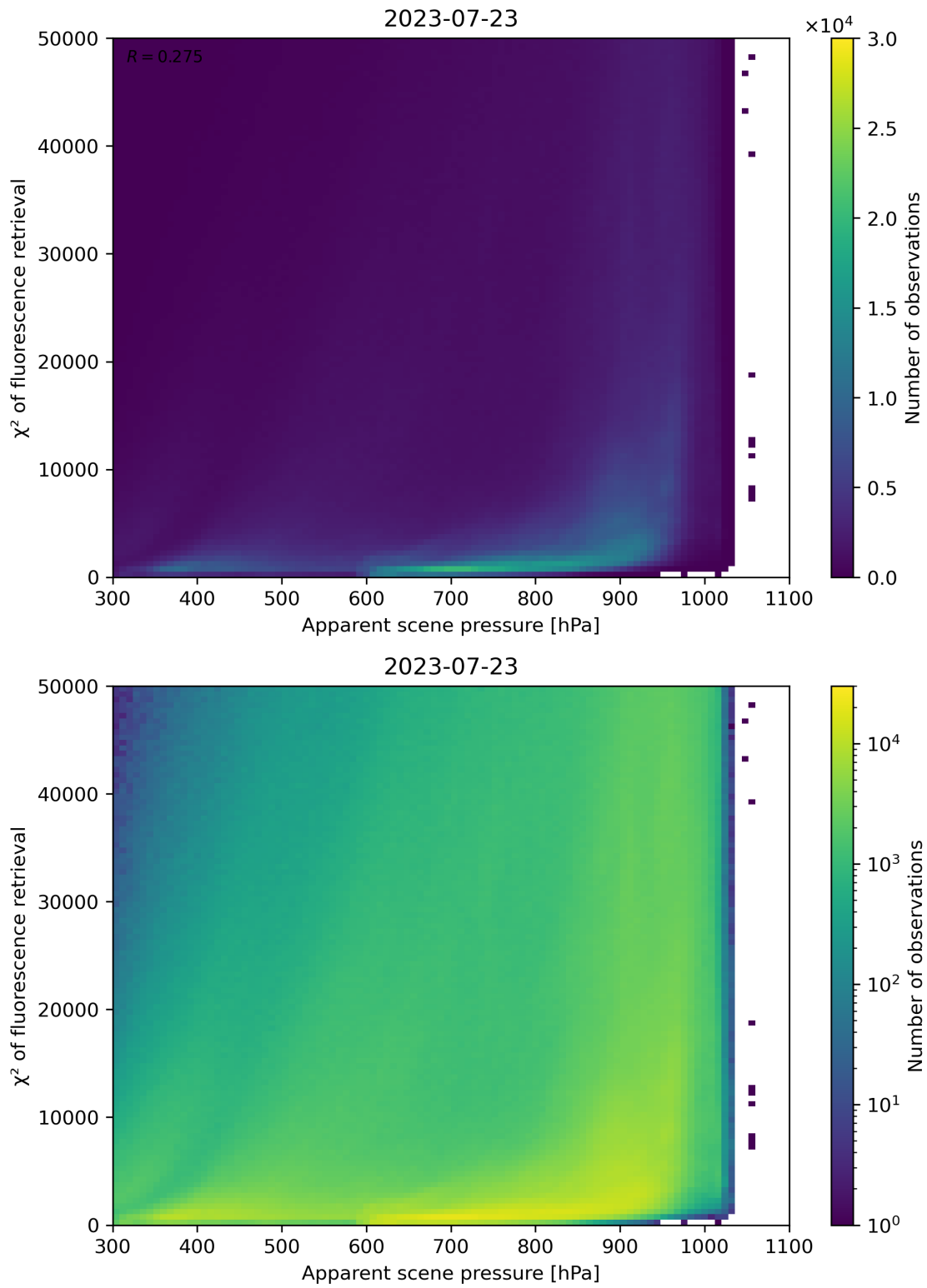
Figure 64: Scatter density plot of “Apparent scene pressure” against “ \chi^2 of fluorescence retrieval” for 2023-07-22 to 2023-07-24.
