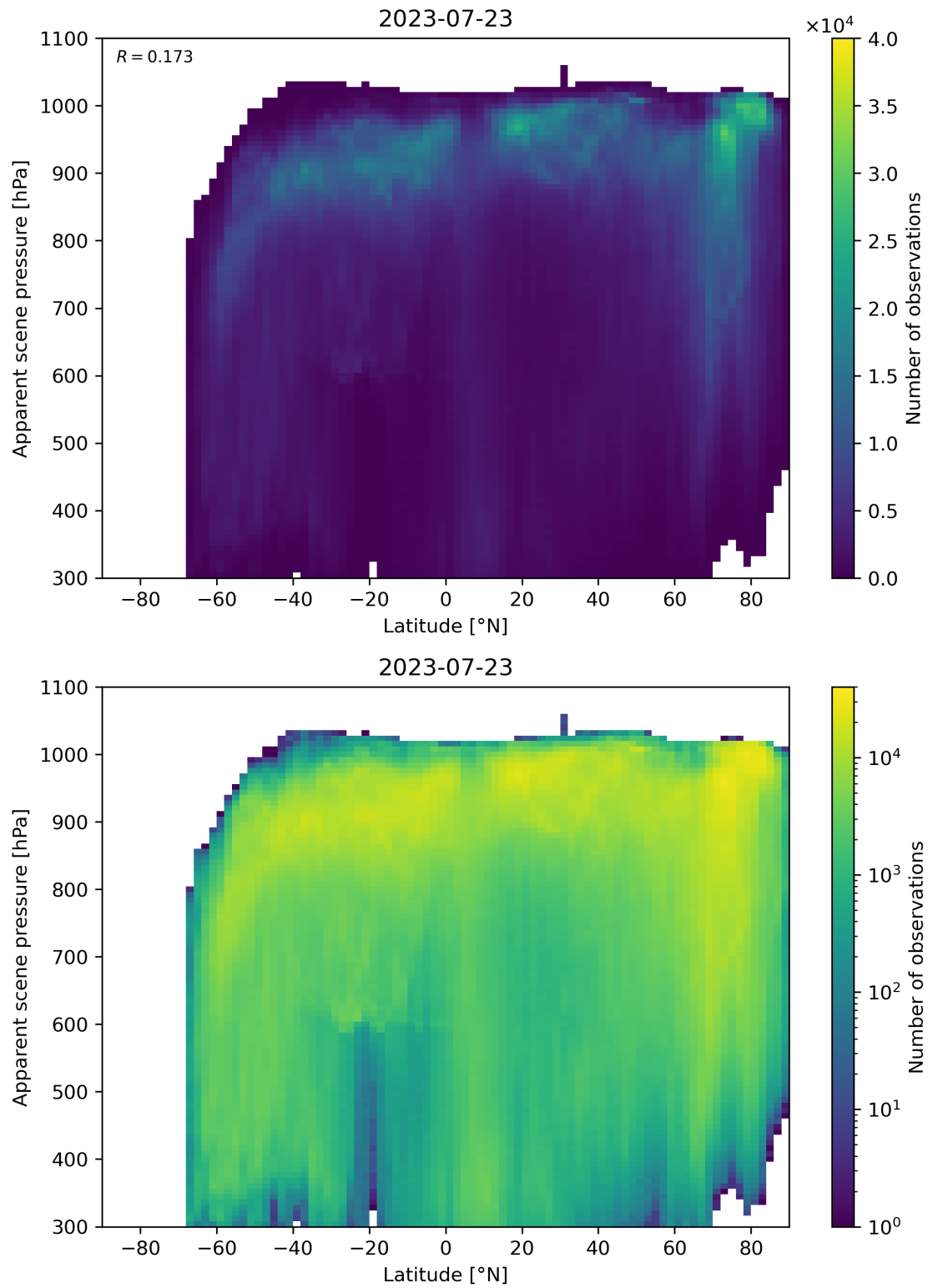
Figure 96: Scatter density plot of “Latitude” against “Apparent scene pressure” for 2023-07-22 to 2023-07-24.
