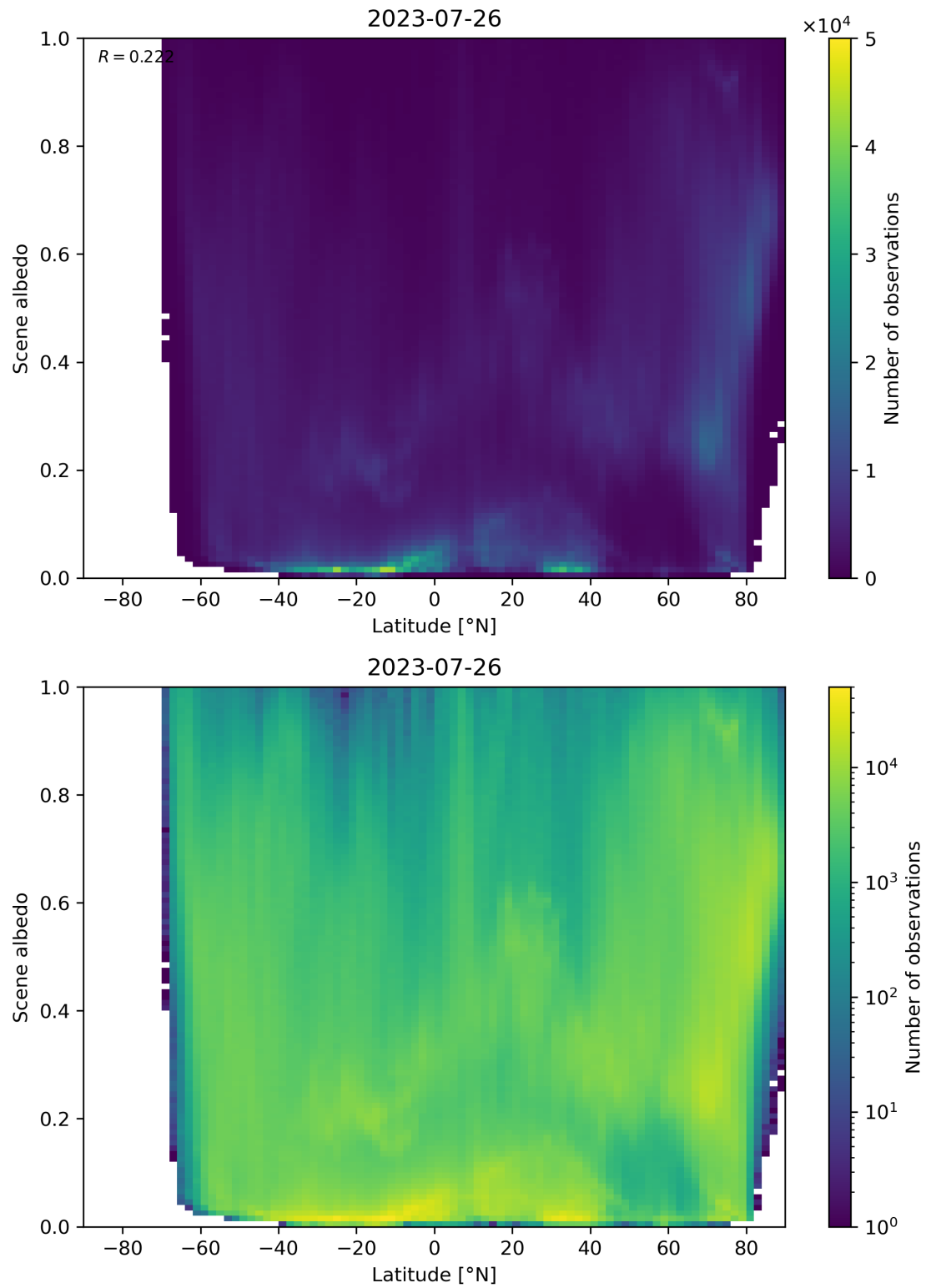
Figure 104: Scatter density plot of “Latitude” against “Scene albedo” for 2023-07-25 to 2023-07-27.
