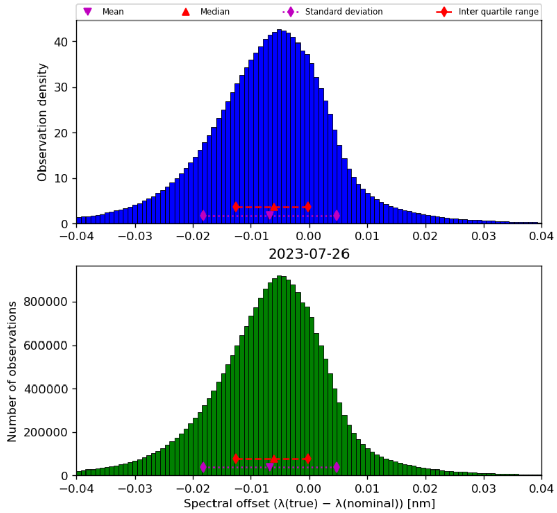
Figure 45: Histogram of “Spectral offset ( \lambda(\text{true}) - \lambda(\text{nominal}) )” for 2023-07-25 to 2023-07-27
