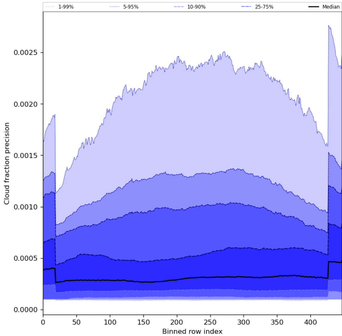
Figure 50: Along track statistics of “Cloud fraction precision” for 2023-07-25 to 2023-07-27
