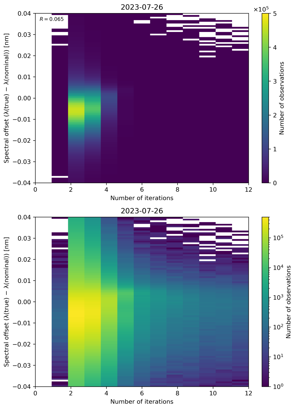
Figure 109: Scatter density plot of “Number of iterations” against “Spectral offset ( \lambda(\text{true}) - \lambda(\text{nominal}) )” for 2023-07-25 to 2023-07-27.
