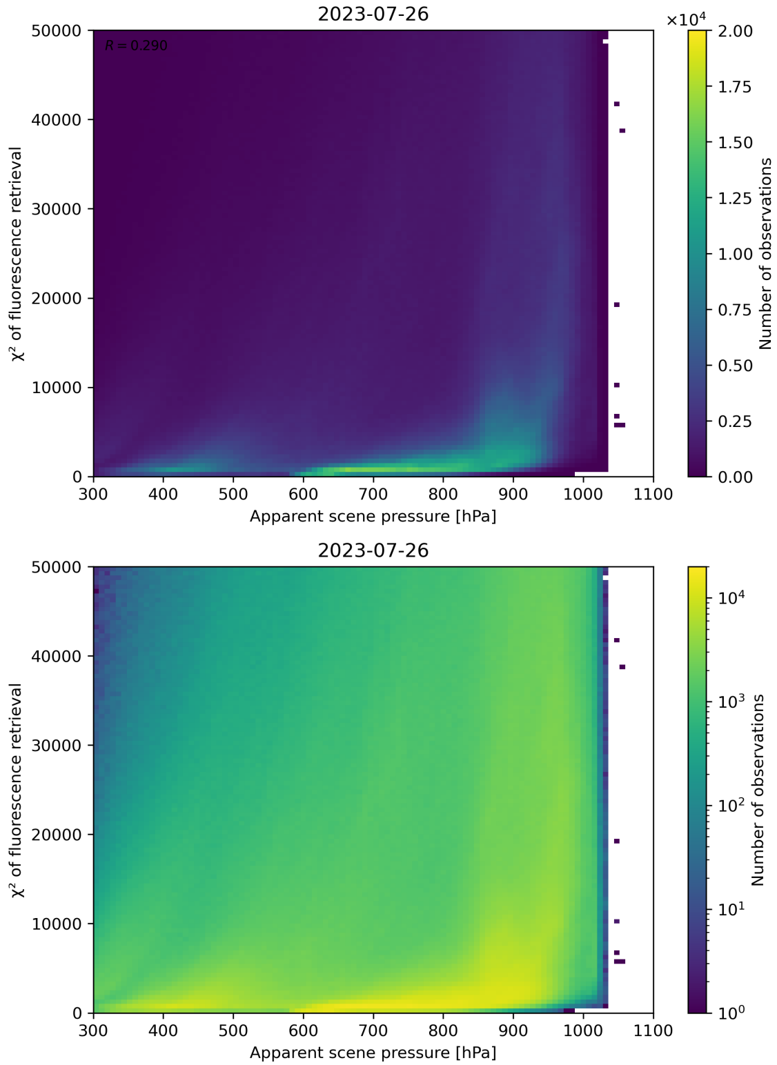
Figure 64: Scatter density plot of “Apparent scene pressure” against “ \chi^2 of fluorescence retrieval” for 2023-07-25 to 2023-07-27.
