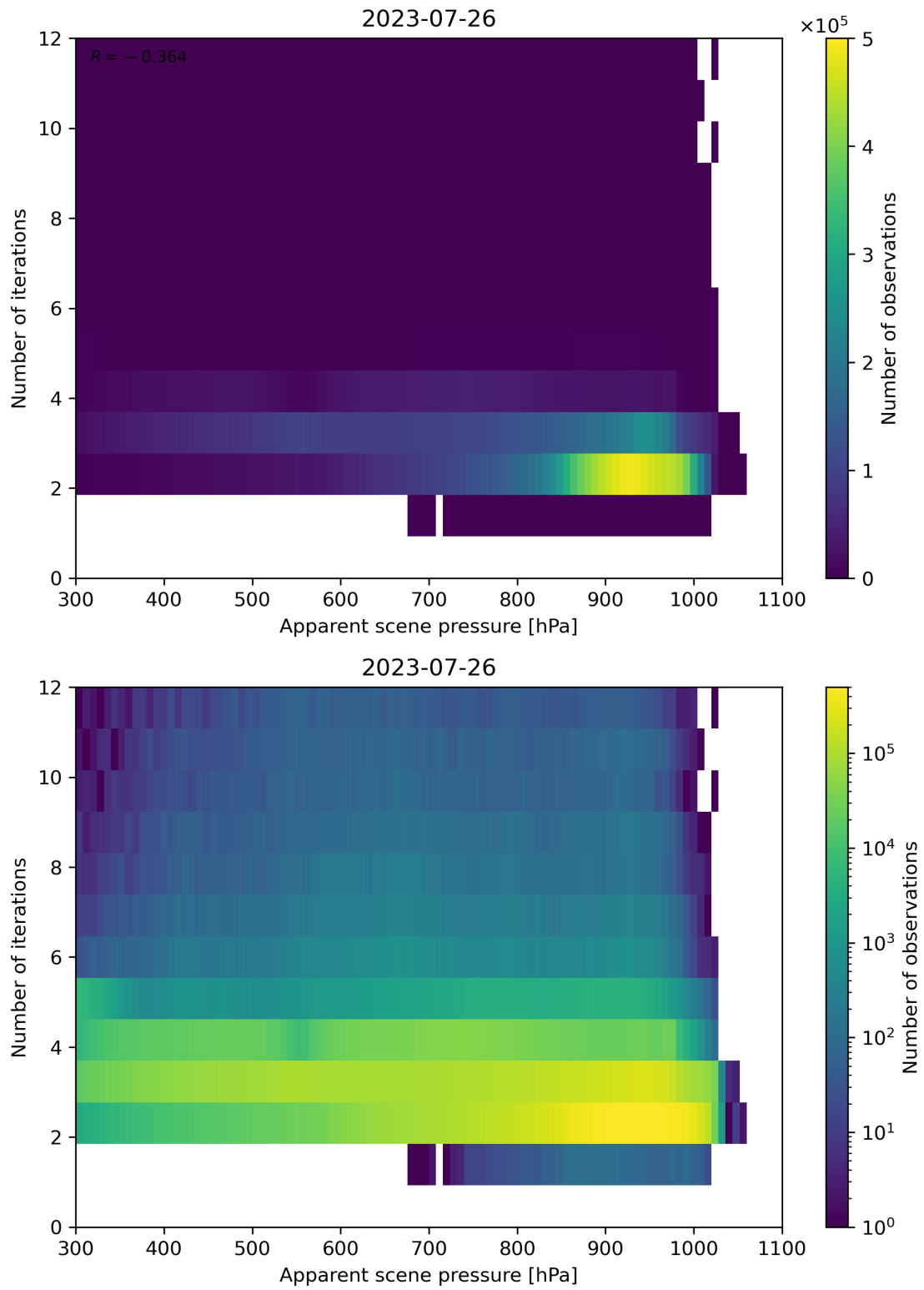
Figure 66: Scatter density plot of “Apparent scene pressure” against “Number of iterations” for 2023-07-25 to 2023-07-27.
