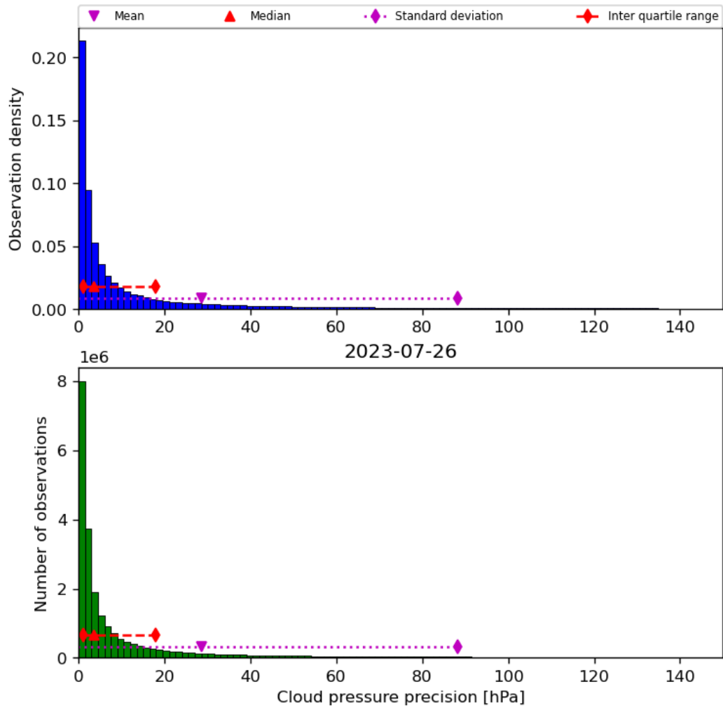
Figure 31: Histogram of “Cloud pressure precision” for 2023-07-25 to 2023-07-27
