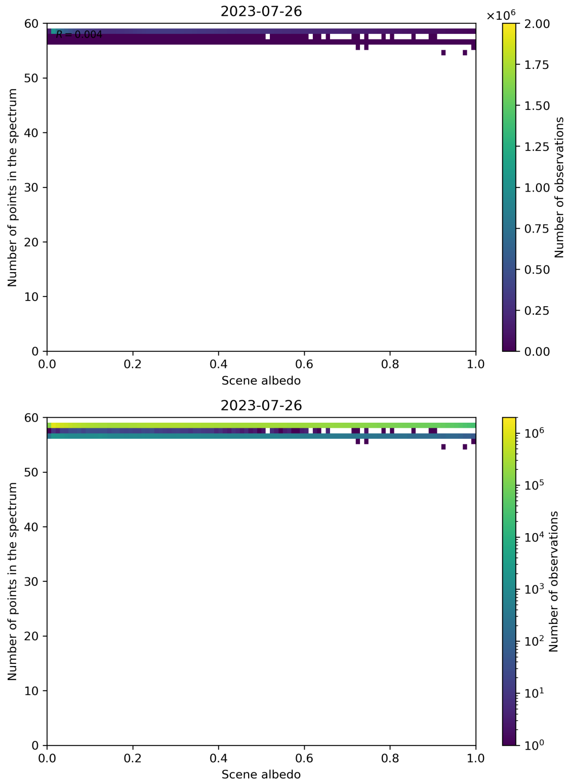
Figure 116: Scatter density plot of “Scene albedo” against “Number of points in the spectrum” for 2023-07-25 to 2023-07-27.
