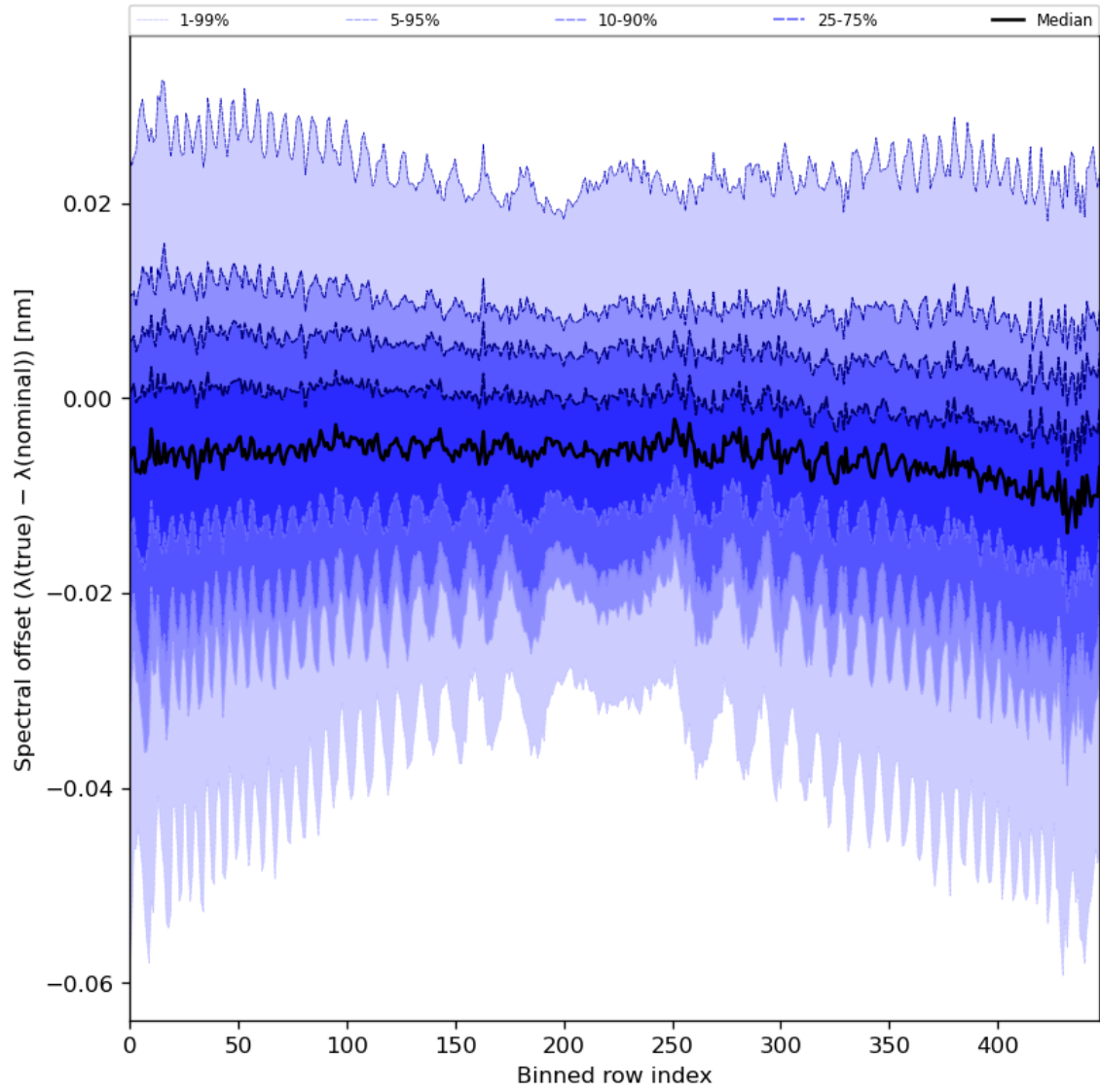
Figure 62: Along track statistics of “Spectral offset ( \lambda(\text{true}) - \lambda(\text{nominal}) )” for 2023-07-25 to 2023-07-27
