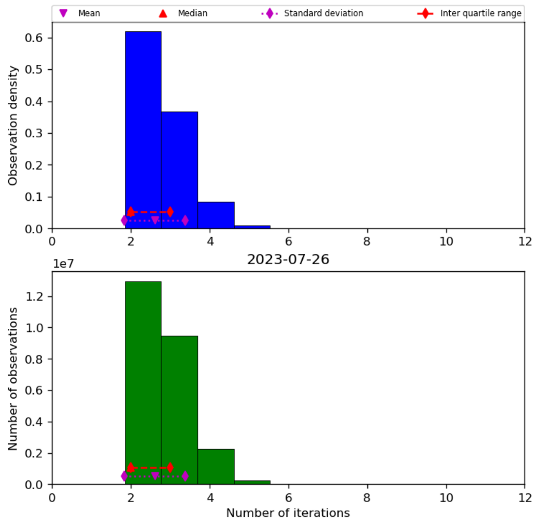
Figure 39: Histogram of “Number of iterations” for 2023-07-25 to 2023-07-27
