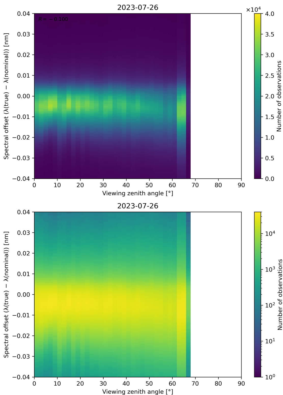
Figure 140: Scatter density plot of “Viewing zenith angle” against “Spectral offset ( \lambda(\text{true}) - \lambda(\text{nominal}) )” for 2023-07-25 to 2023-07-27.
