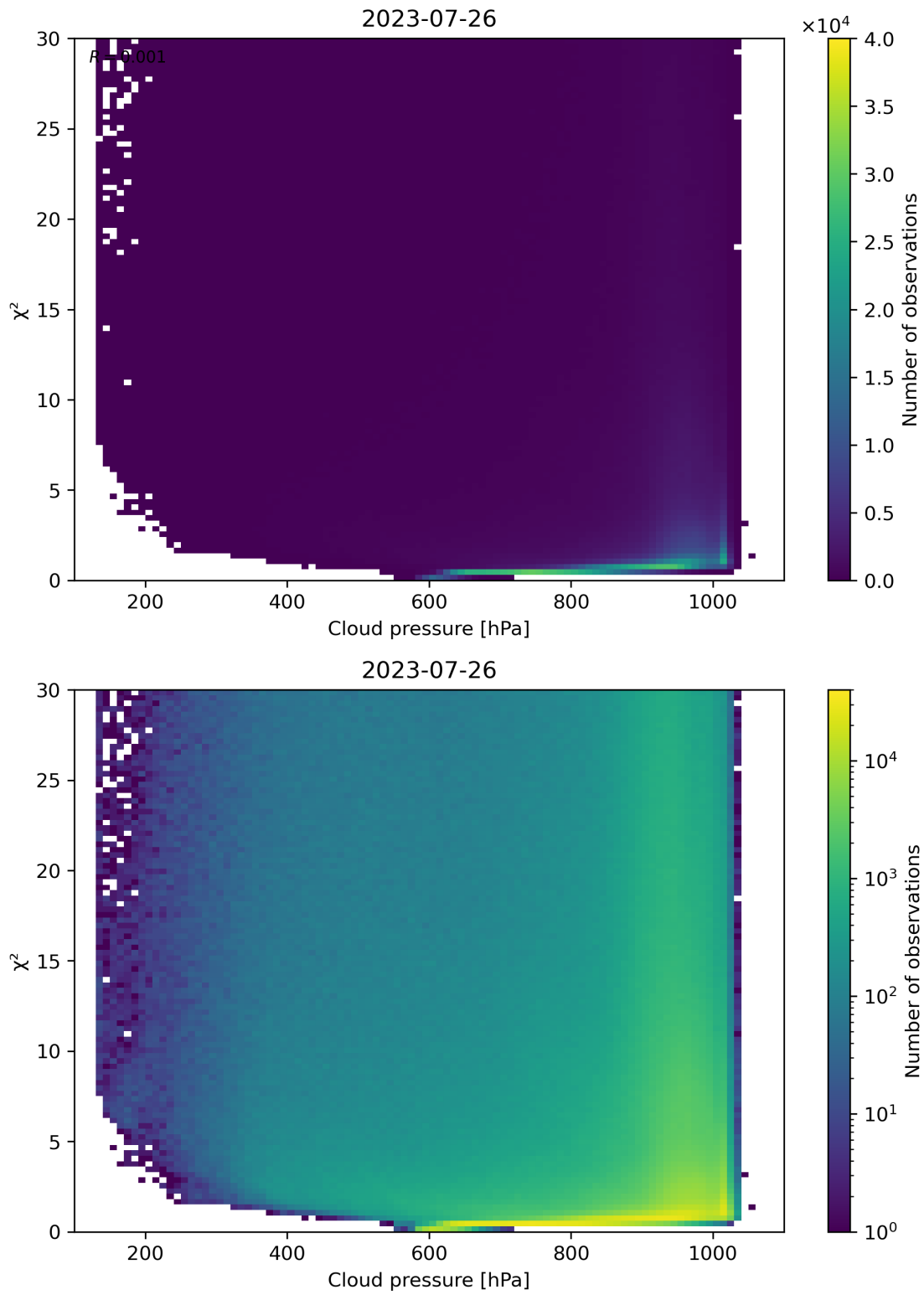
Figure 85: Scatter density plot of “Cloud pressure” against “ \chi^2 ” for 2023-07-25 to 2023-07-27.
