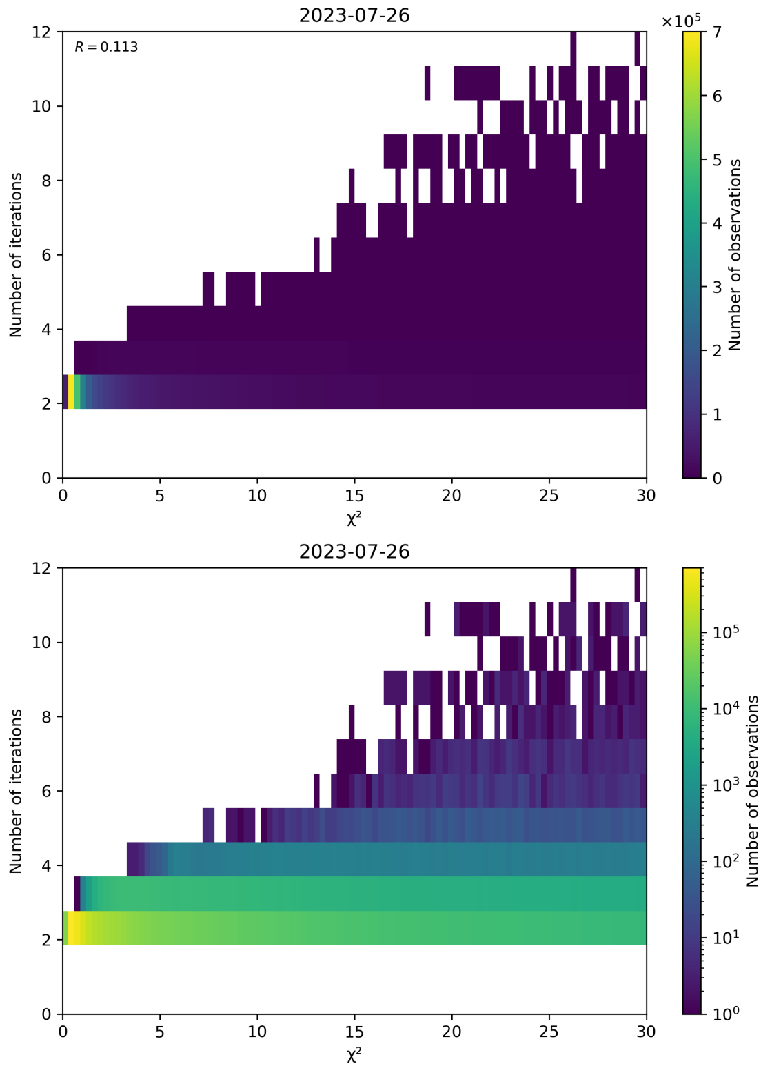
Figure 73: Scatter density plot of “ \chi^2 ” against “Number of iterations” for 2023-07-25 to 2023-07-27.
