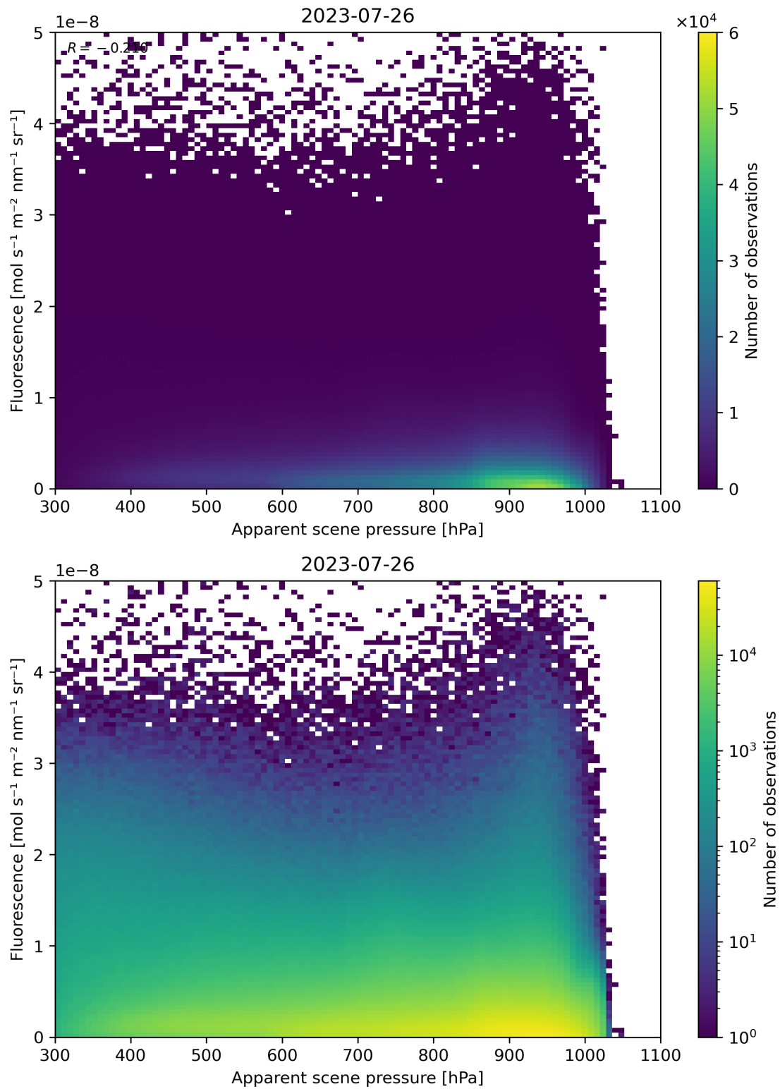
Figure 65: Scatter density plot of “Apparent scene pressure” against “Fluorescence” for 2023-07-25 to 2023-07-27.
