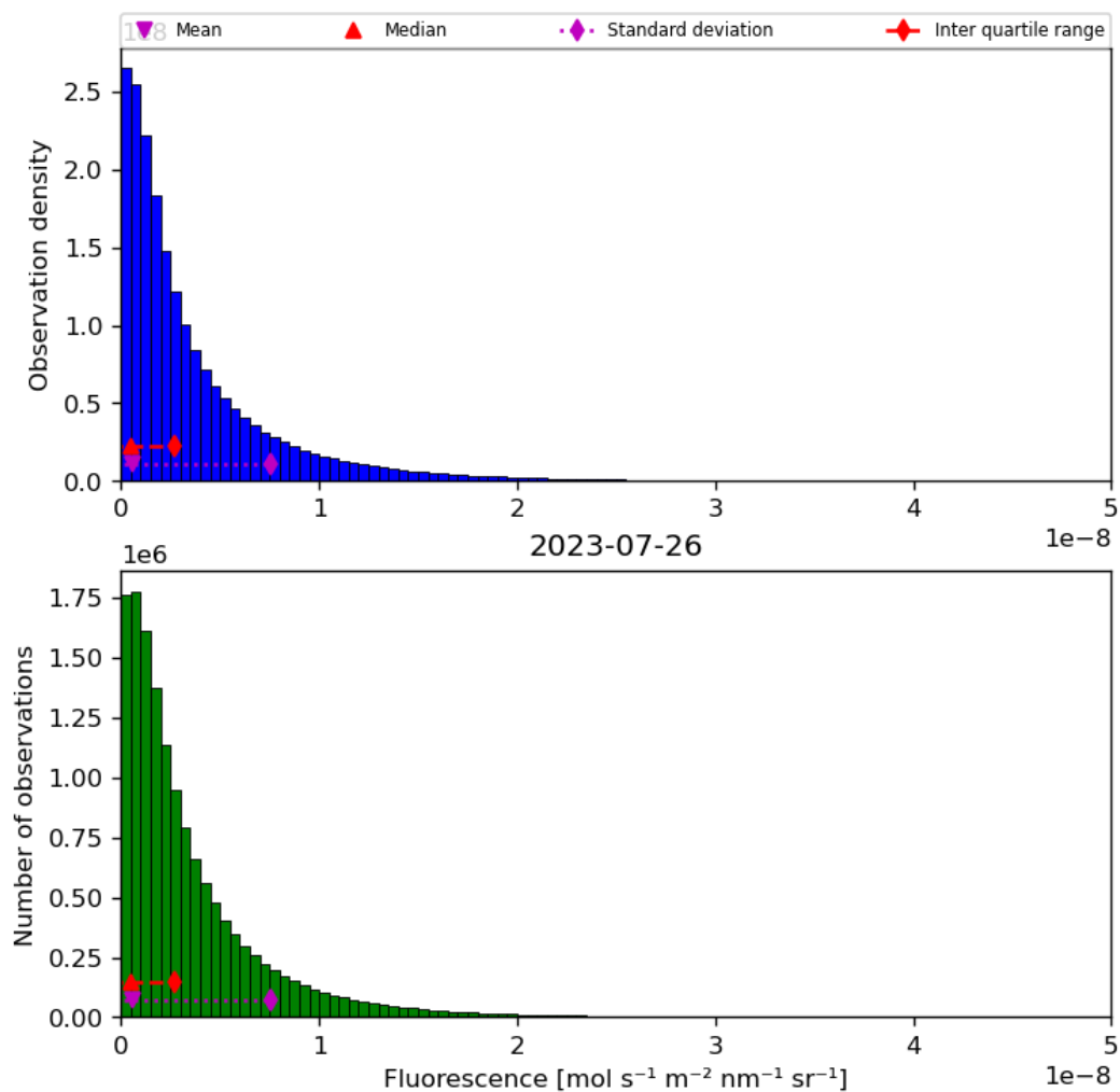
Figure 40: Histogram of “Fluorescence” for 2023-07-25 to 2023-07-27
