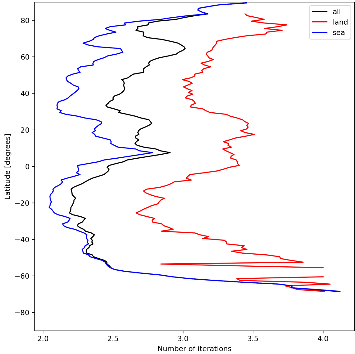
Figure 22: Zonal average of “Number of iterations” for 2023-07-25 to 2023-07-27.
