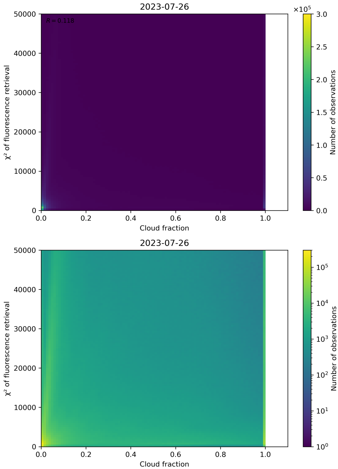
Figure 78: Scatter density plot of “Cloud fraction” against “ \chi^2 of fluorescence retrieval” for 2023-07-25 to 2023-07-27.
