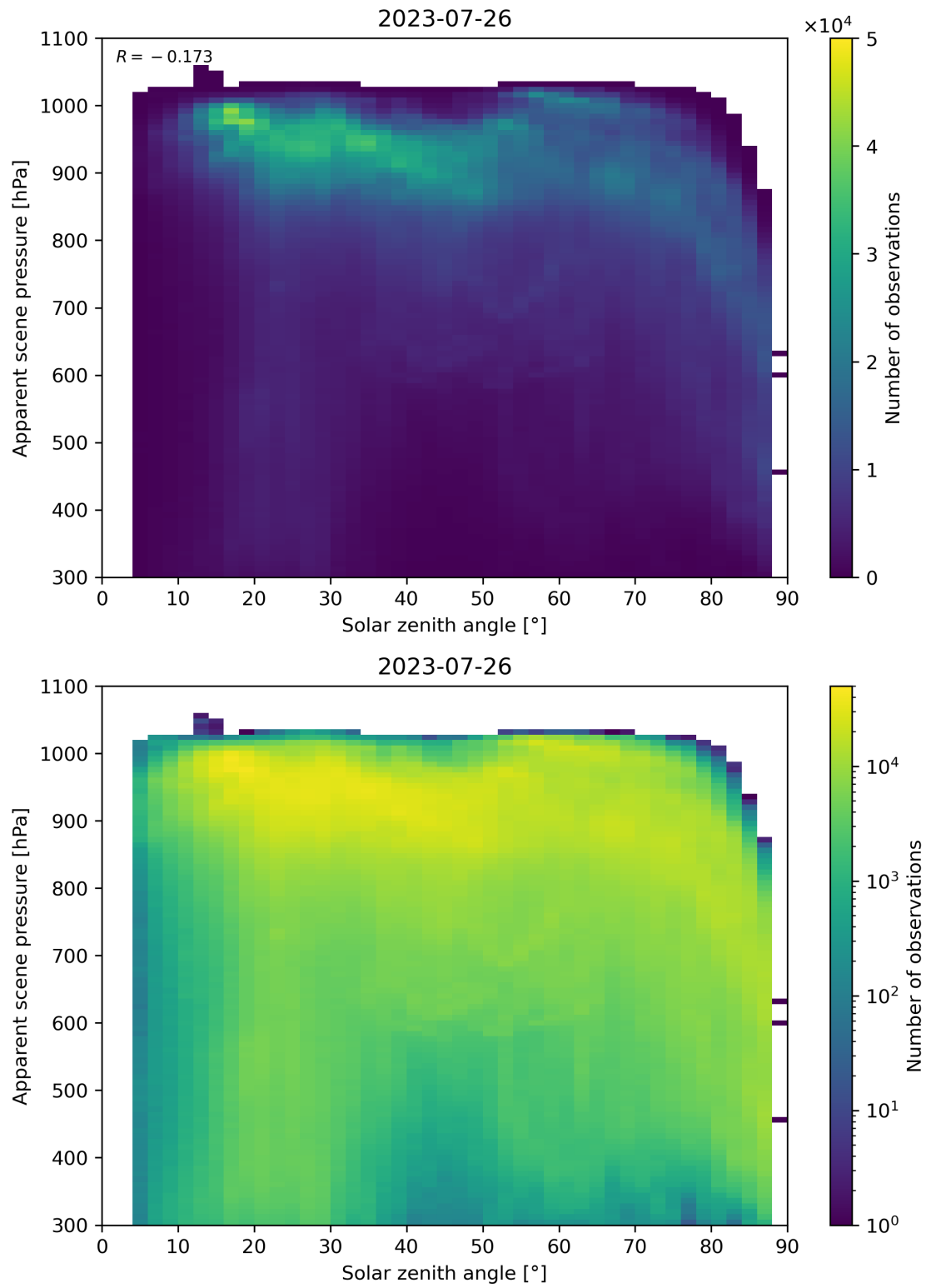
Figure 118: Scatter density plot of “Solar zenith angle” against “Apparent scene pressure” for 2023-07-25 to 2023-07-27.
