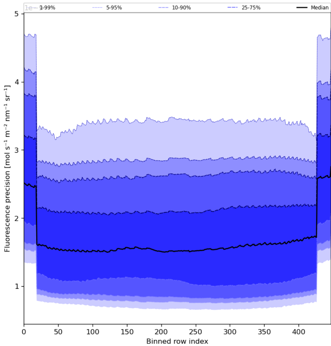
Figure 58: Along track statistics of “Fluorescence precision” for 2023-07-25 to 2023-07-27
