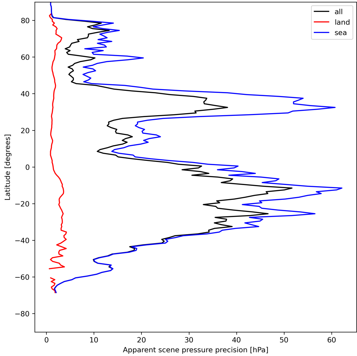
Figure 20: Zonal average of “Apparent scene pressure precision” for 2023-07-25 to 2023-07-27.
