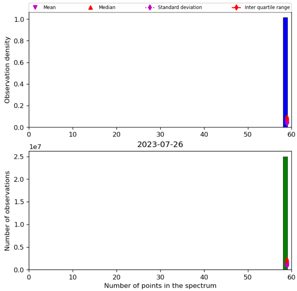
Figure 44: Histogram of “Number of points in the spectrum” for 2023-07-25 to 2023-07-27
