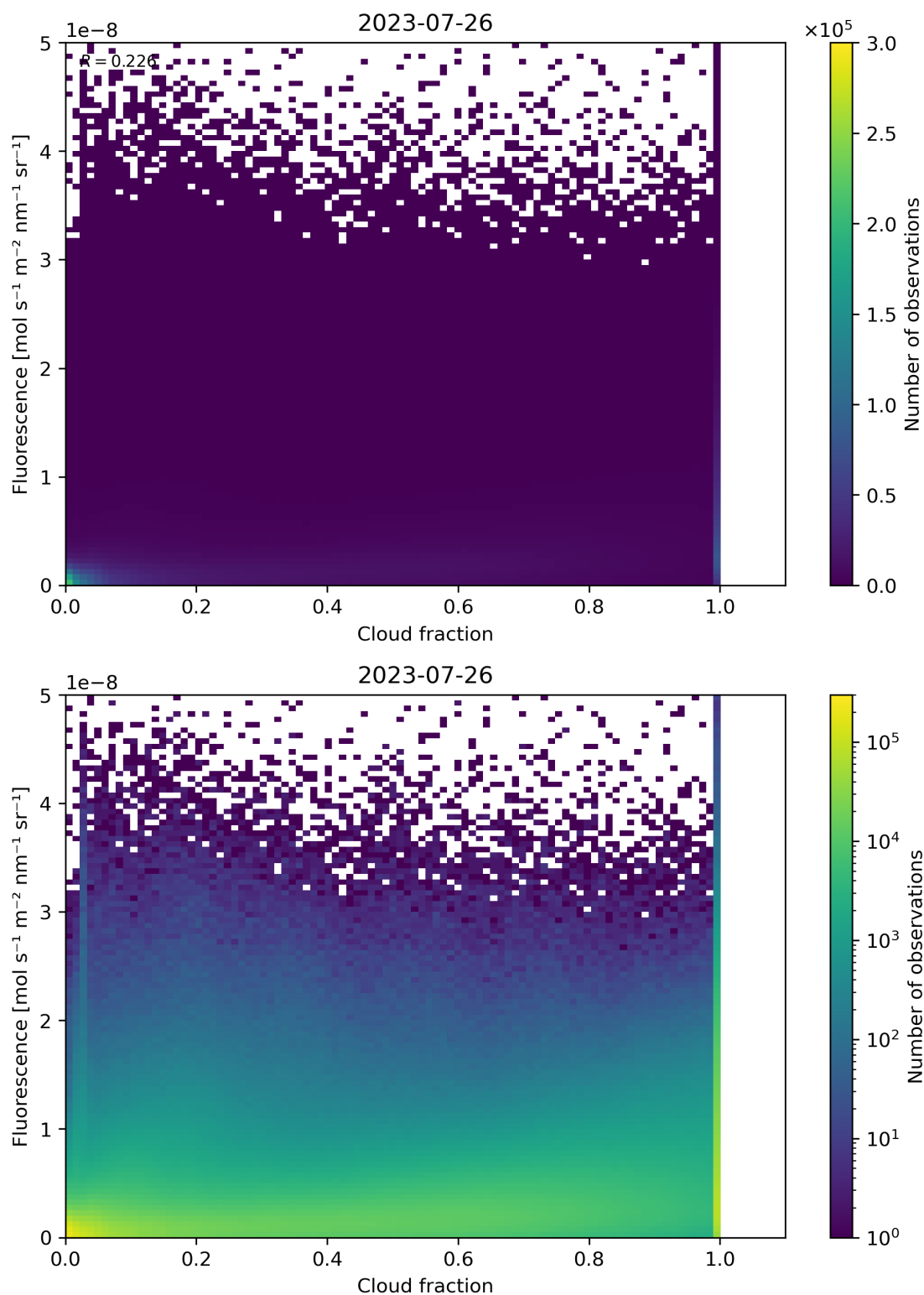
Figure 79: Scatter density plot of “Cloud fraction” against “Fluorescence” for 2023-07-25 to 2023-07-27.
