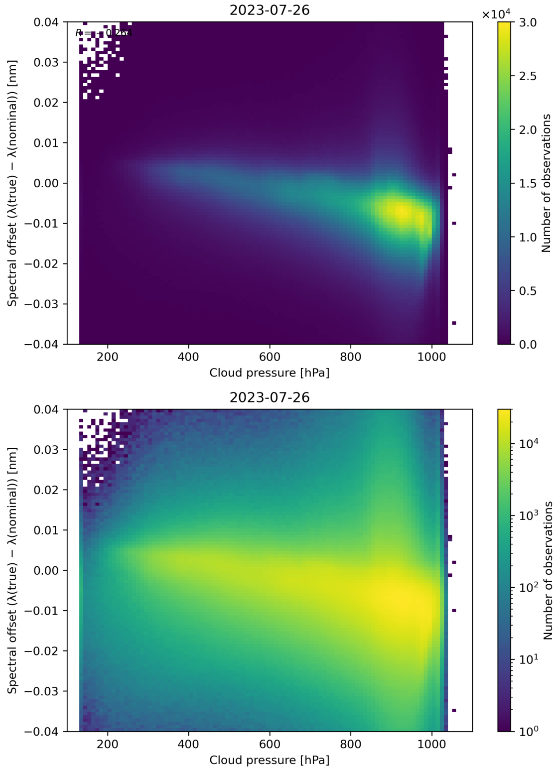
Figure 92: Scatter density plot of “Cloud pressure” against “Spectral offset ( \lambda(\text{true}) - \lambda(\text{nominal}) )” for 2023-07-25 to 2023-07-27.
