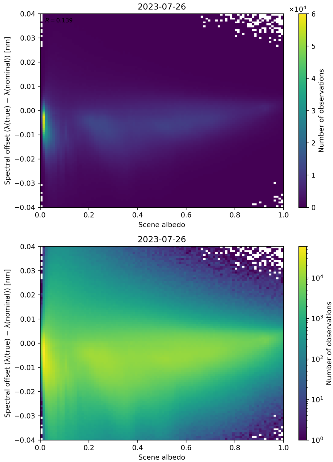
Figure 117: Scatter density plot of “Scene albedo” against “Spectral offset ( \lambda(\text{true}) - \lambda(\text{nominal}) )” for 2023-07-25 to 2023-07-27.
