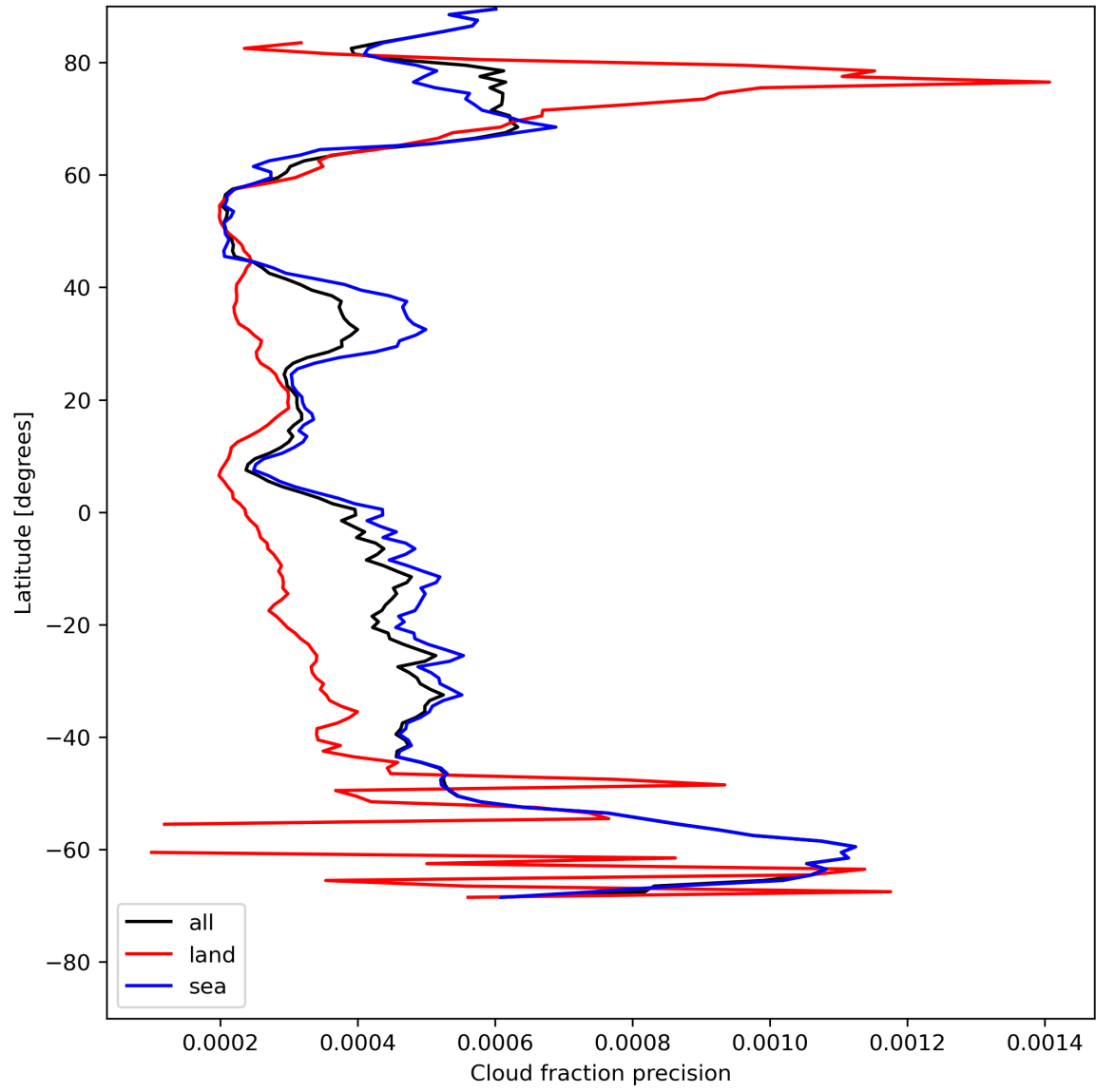
Figure 16: Zonal average of “Cloud fraction precision” for 2023-07-25 to 2023-07-27.
