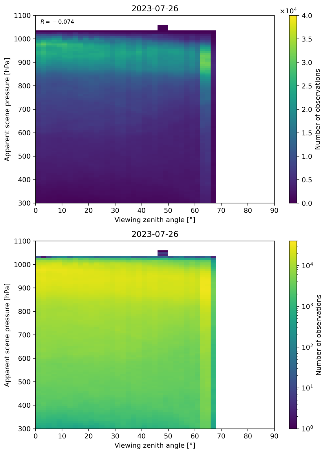
Figure 129: Scatter density plot of “Viewing zenith angle” against “Apparent scene pressure” for 2023-07-25 to 2023-07-27.
