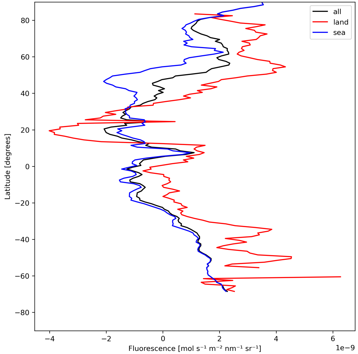
Figure 23: Zonal average of “Fluorescence” for 2023-07-25 to 2023-07-27.
