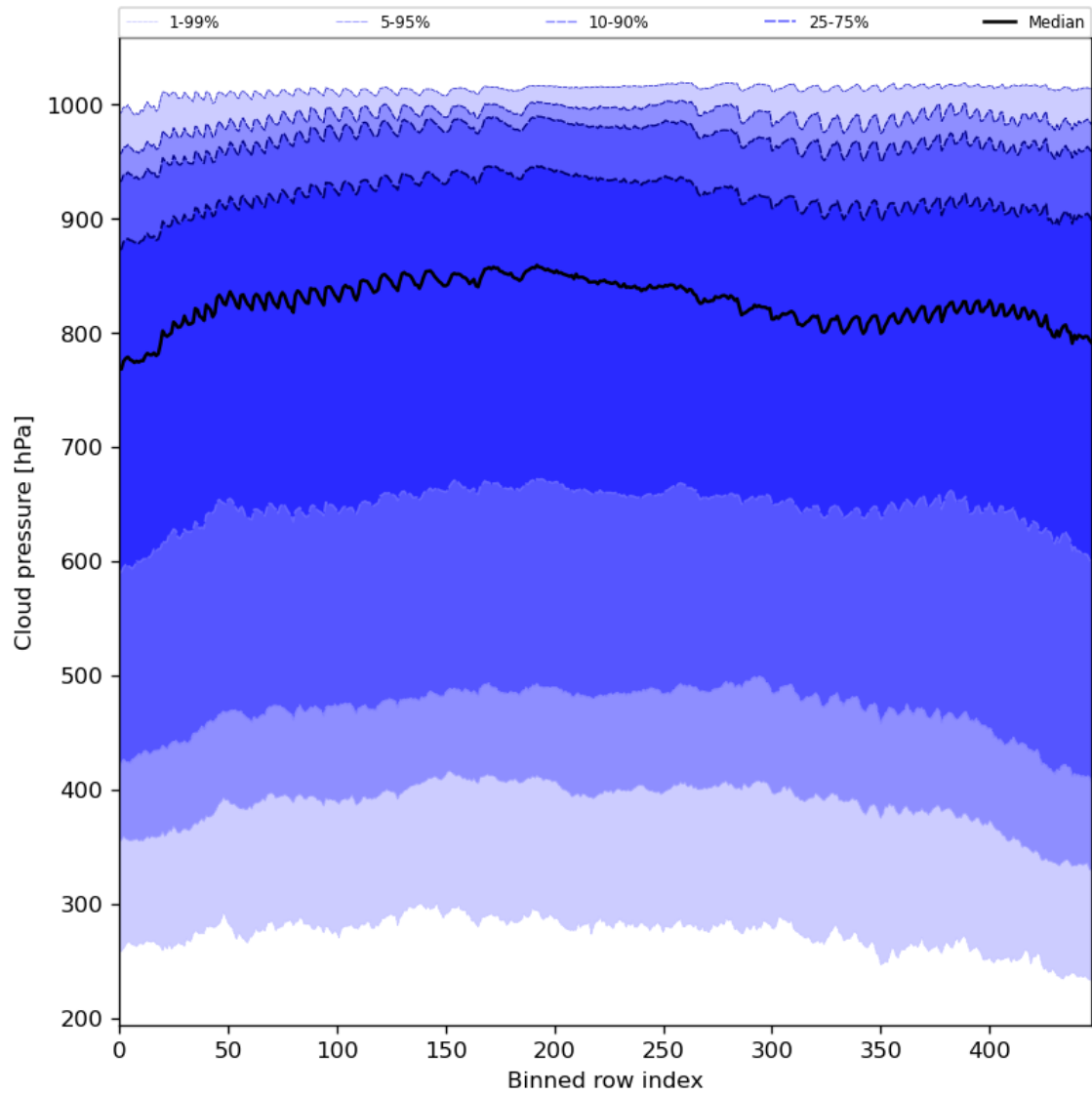
Figure 47: Along track statistics of “Cloud pressure” for 2023-07-25 to 2023-07-27
