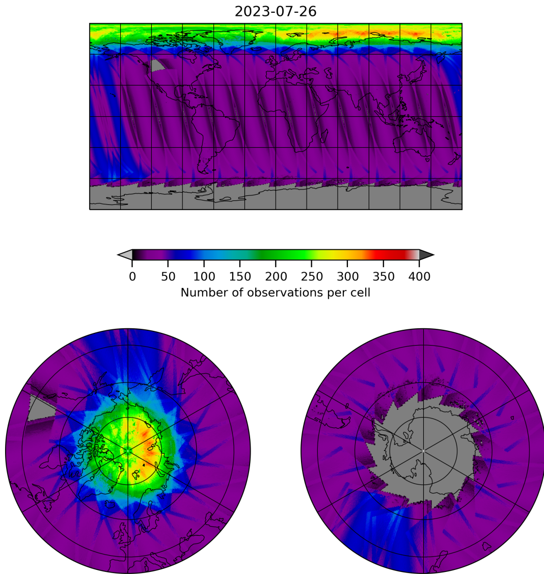
Figure 11: Map of the number of observations for 2023-07-25 to 2023-07-27
