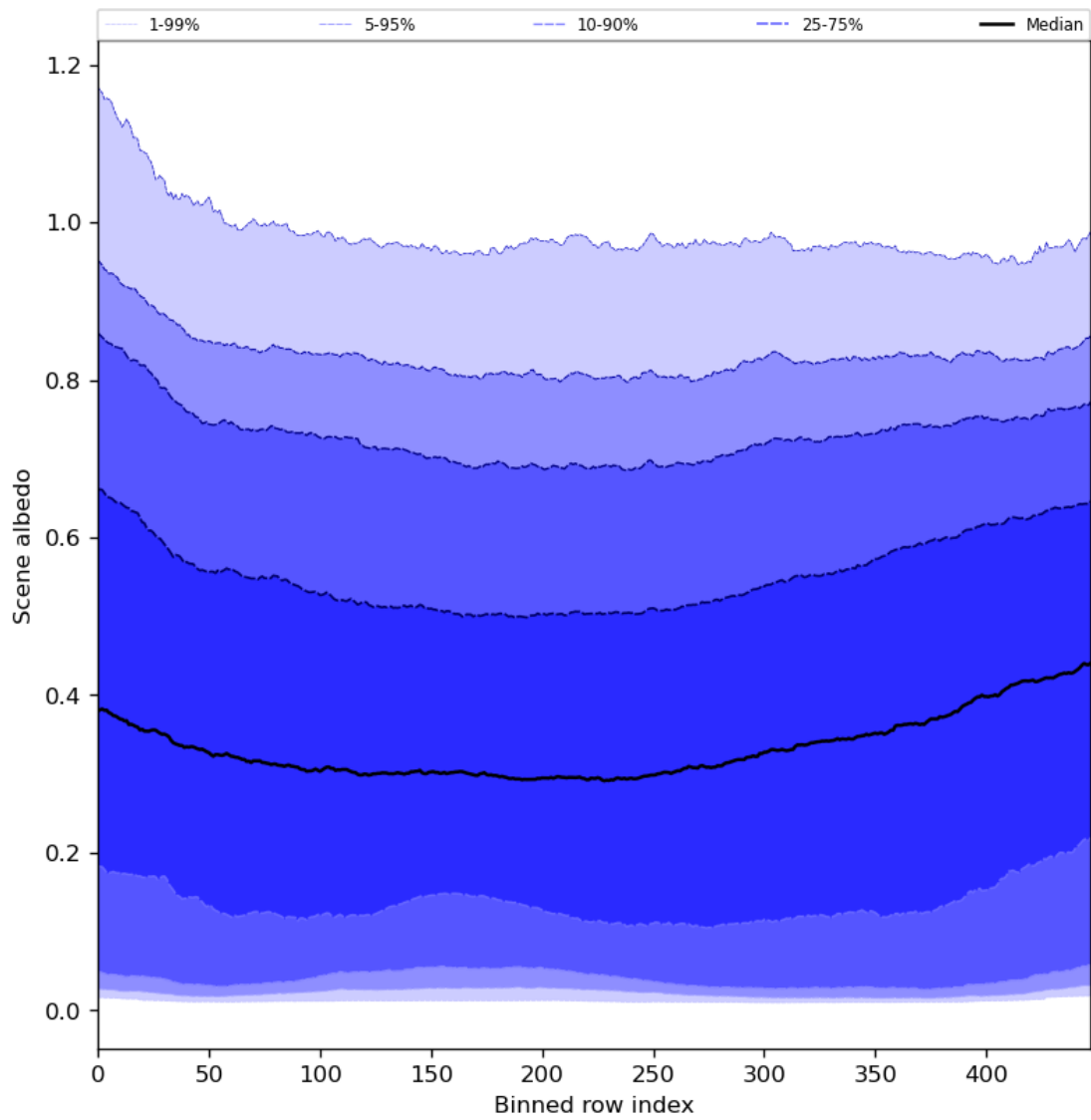
Figure 51: Along track statistics of “Scene albedo” for 2023-07-25 to 2023-07-27
