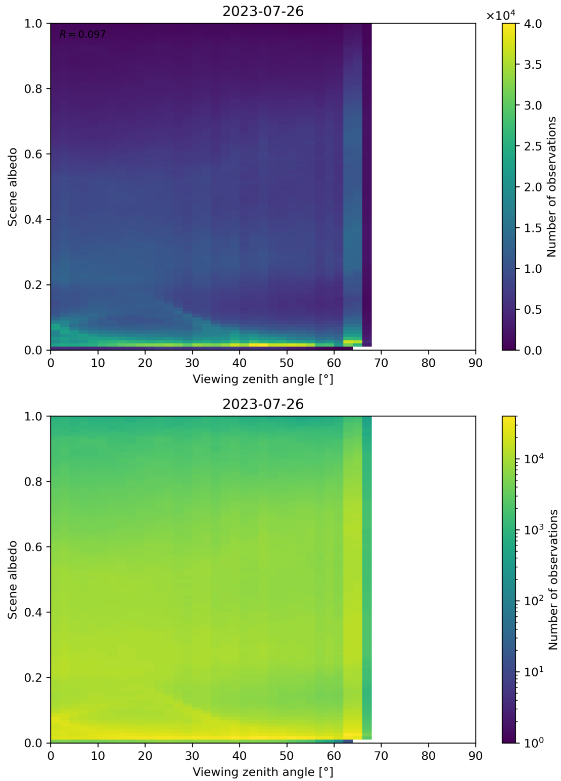
Figure 138: Scatter density plot of “Viewing zenith angle” against “Scene albedo” for 2023-07-25 to 2023-07-27.
