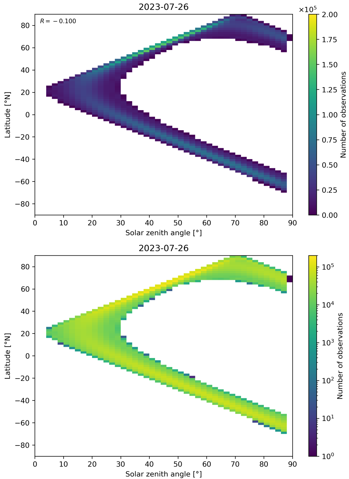
Figure 124: Scatter density plot of “Solar zenith angle” against “Latitude” for 2023-07-25 to 2023-07-27.
