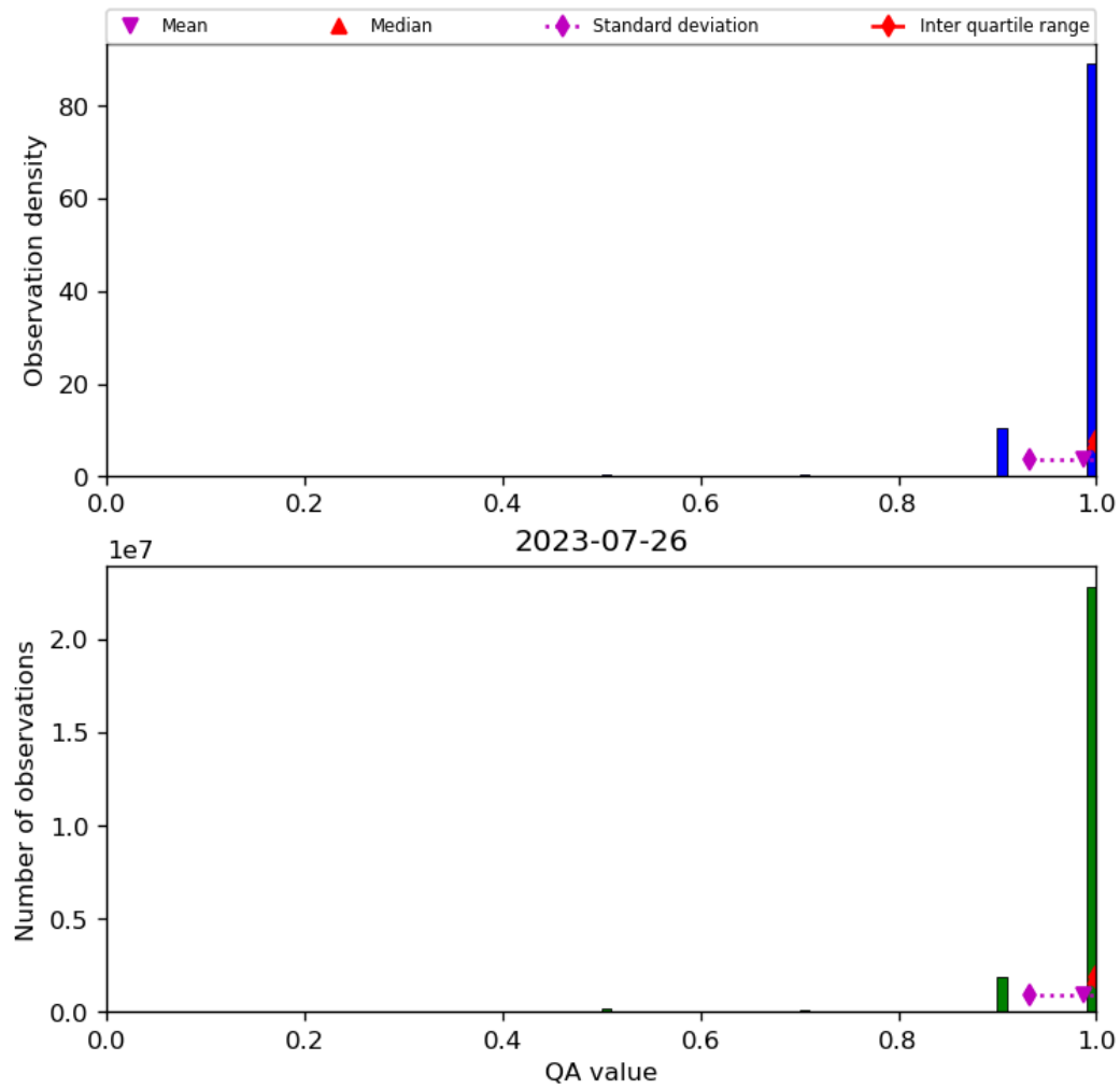
Figure 29: Histogram of “QA value” for 2023-07-25 to 2023-07-27
