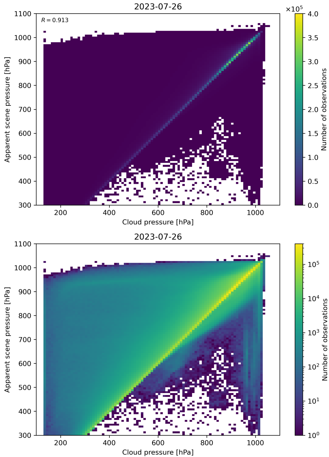
Figure 84: Scatter density plot of “Cloud pressure” against “Apparent scene pressure” for 2023-07-25 to 2023-07-27.
