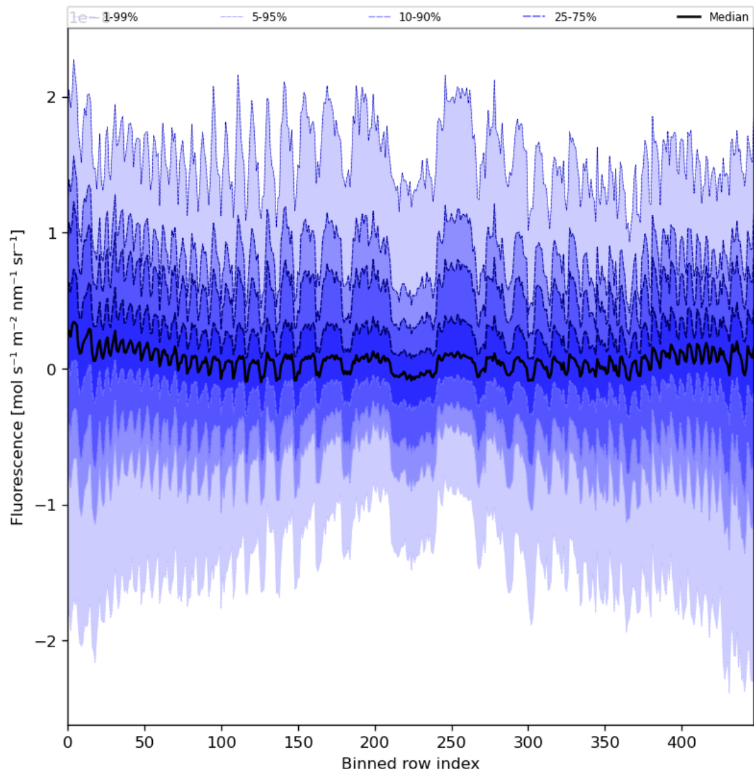
Figure 57: Along track statistics of “Fluorescence” for 2023-07-25 to 2023-07-27
