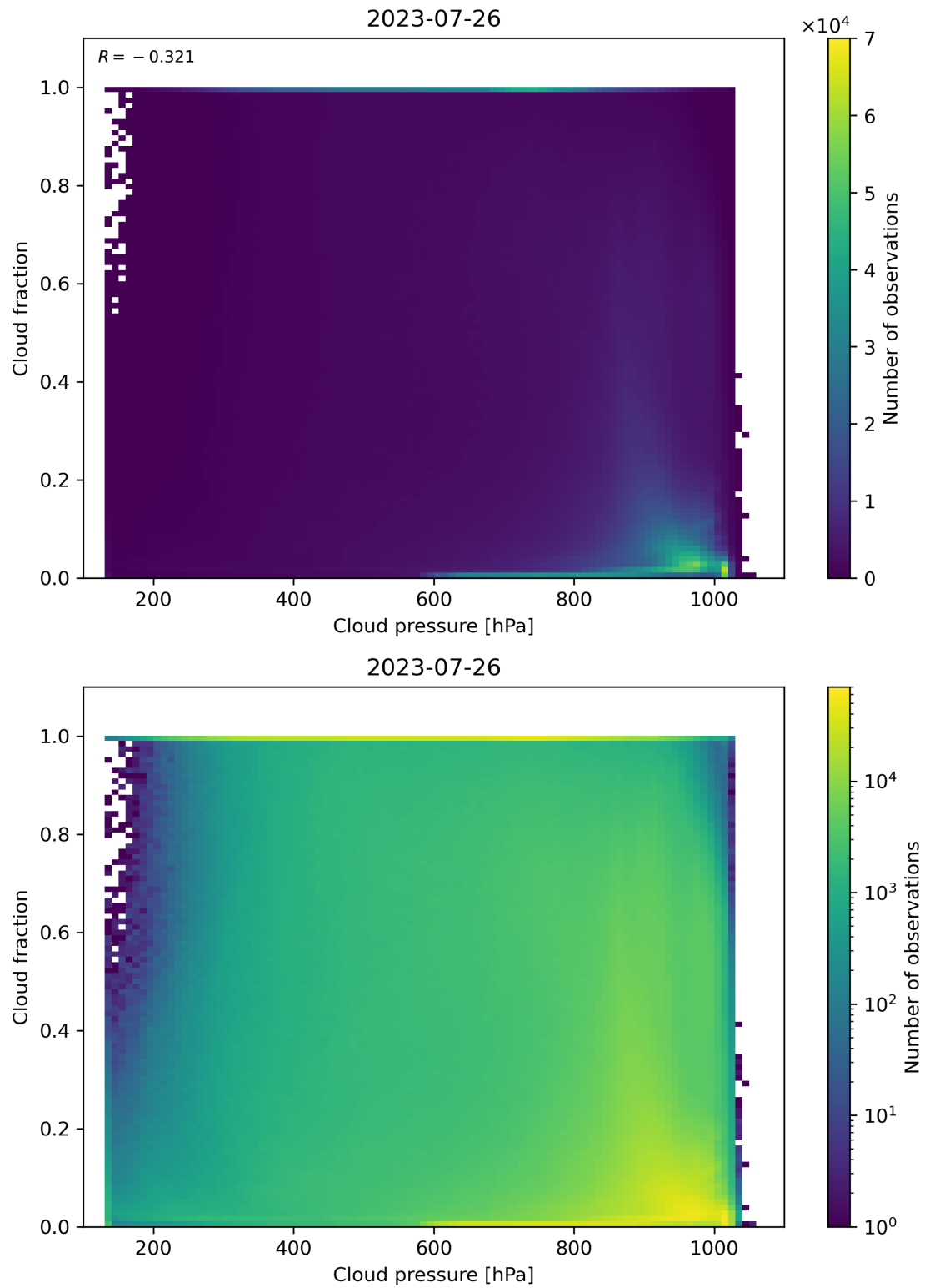
Figure 87: Scatter density plot of “Cloud pressure” against “Cloud fraction” for 2023-07-25 to 2023-07-27.
