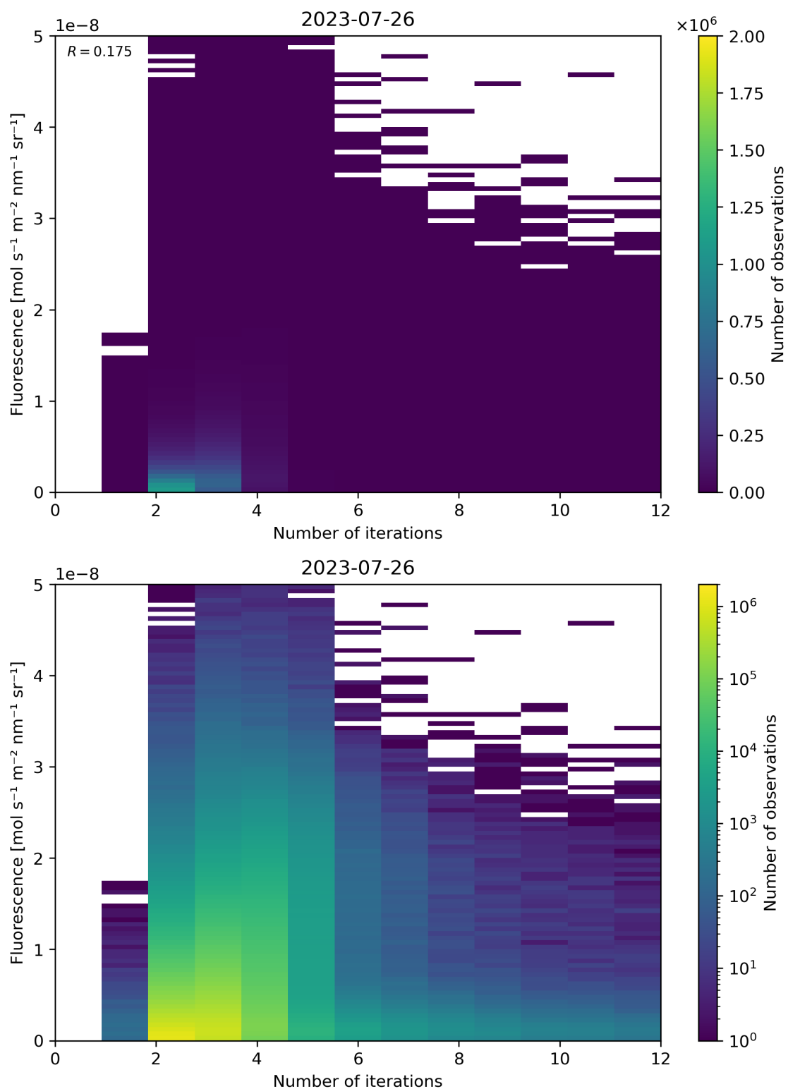
Figure 107: Scatter density plot of “Number of iterations” against “Fluorescence” for 2023-07-25 to 2023-07-27.
