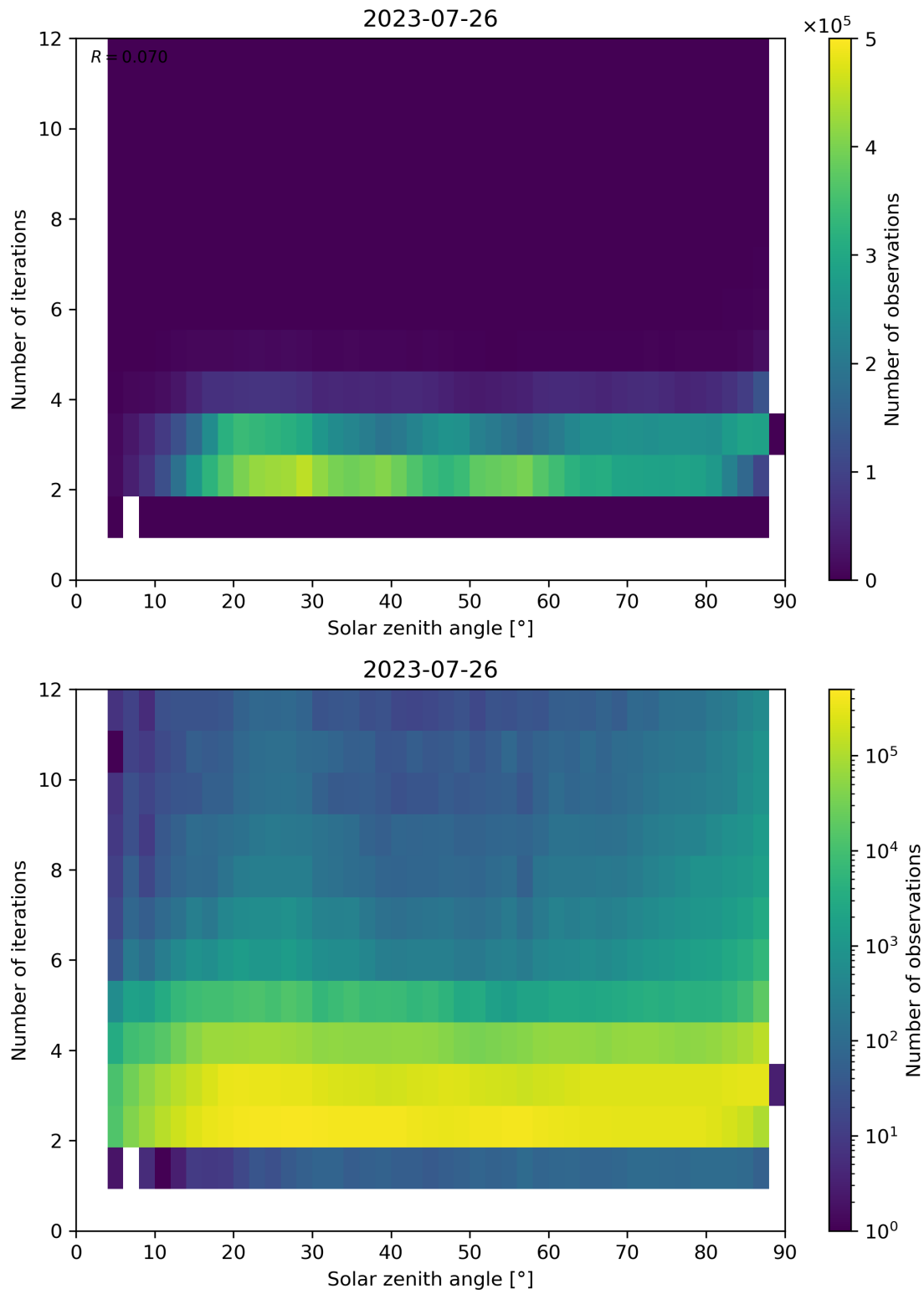
Figure 125: Scatter density plot of “Solar zenith angle” against “Number of iterations” for 2023-07-25 to 2023-07-27.
