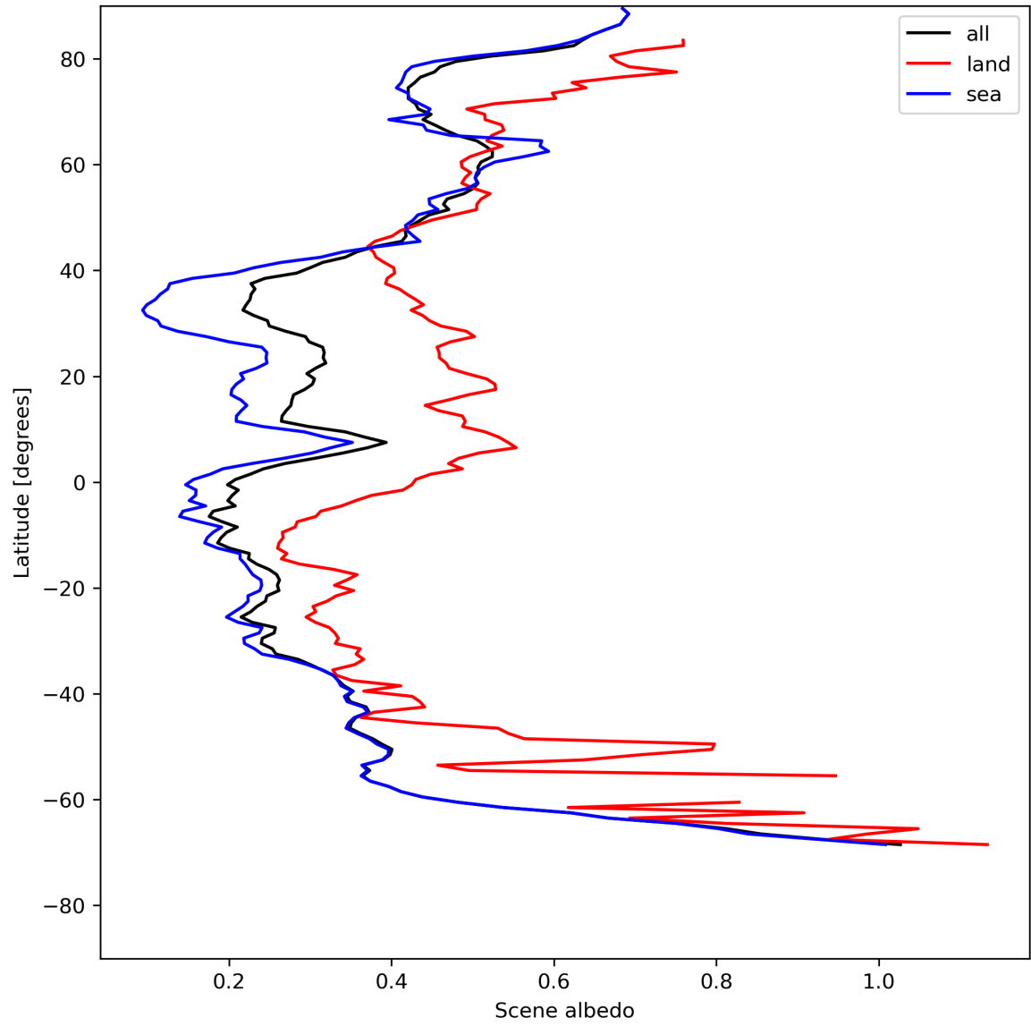
Figure 17: Zonal average of “Scene albedo” for 2023-07-25 to 2023-07-27.
