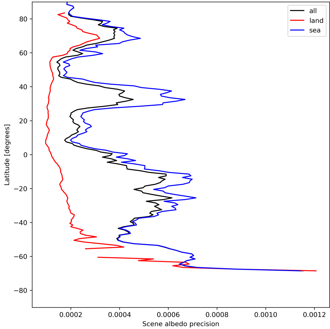
Figure 18: Zonal average of “Scene albedo precision” for 2023-07-25 to 2023-07-27.
