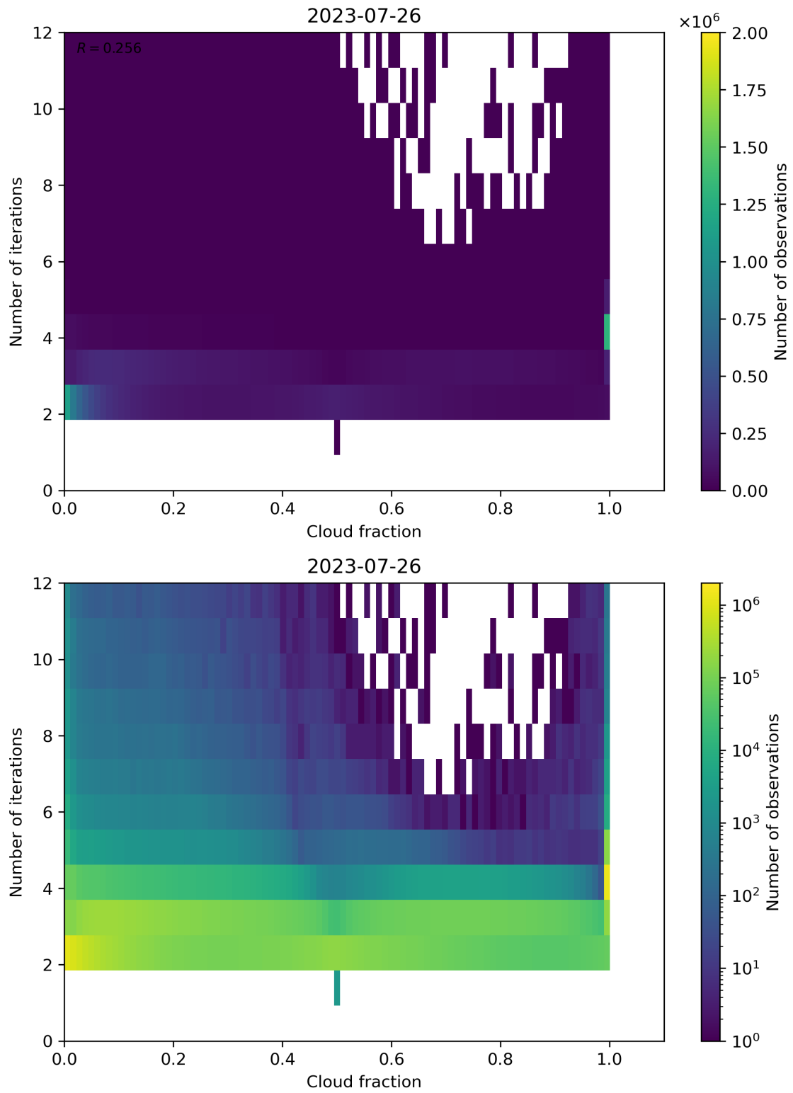
Figure 80: Scatter density plot of “Cloud fraction” against “Number of iterations” for 2023-07-25 to 2023-07-27.
