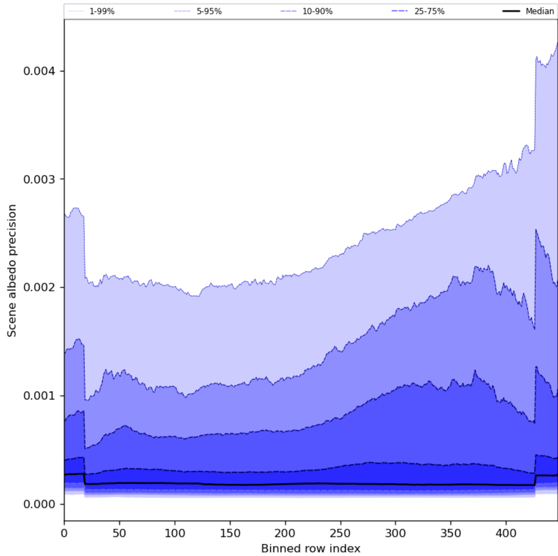
Figure 52: Along track statistics of “Scene albedo precision” for 2023-07-25 to 2023-07-27
