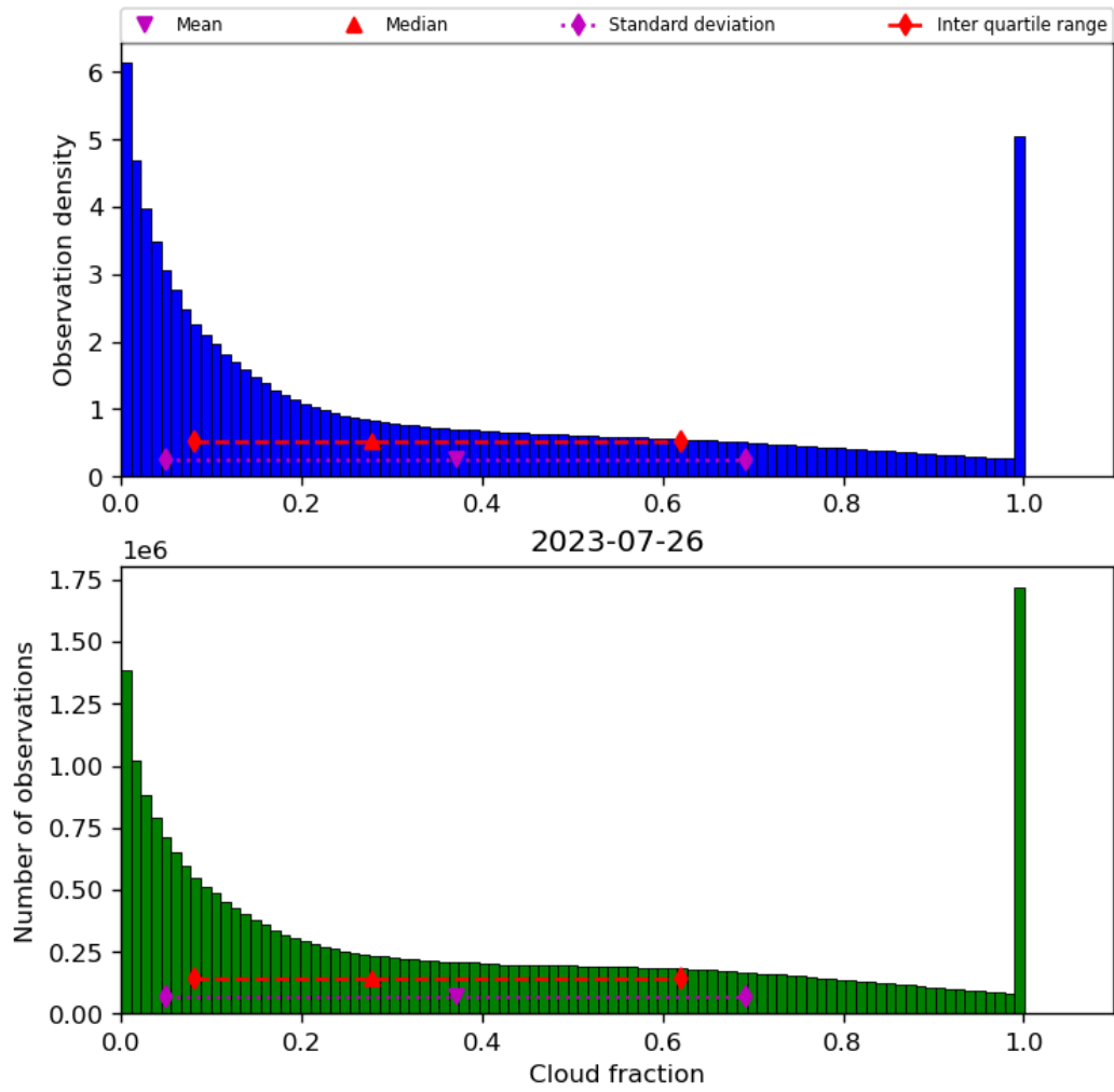
Figure 32: Histogram of “Cloud fraction” for 2023-07-25 to 2023-07-27
