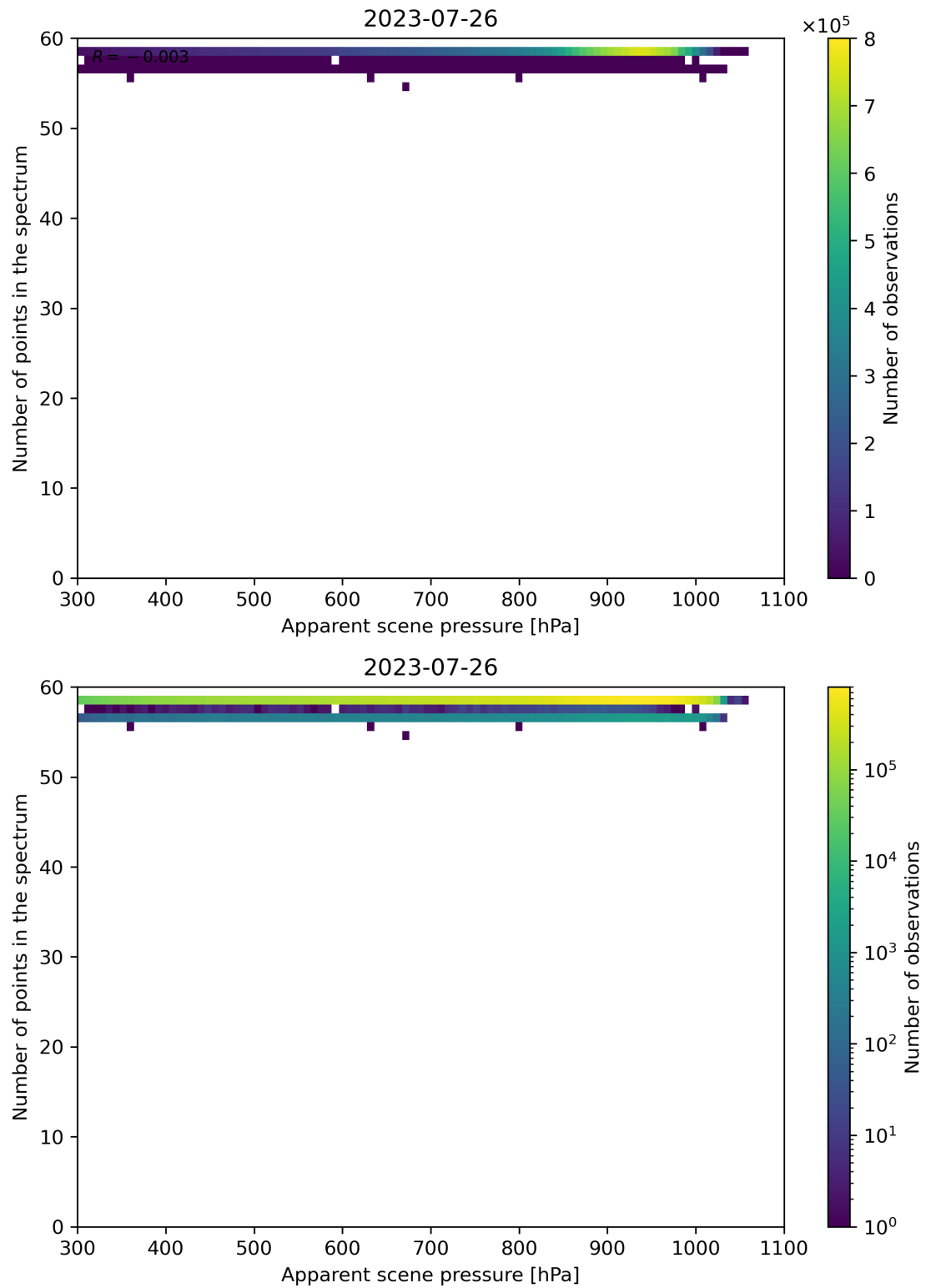
Figure 67: Scatter density plot of “Apparent scene pressure” against “Number of points in the spectrum” for 2023-07-25 to 2023-07-27.
