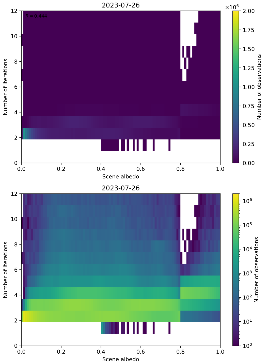
Figure 115: Scatter density plot of “Scene albedo” against “Number of iterations” for 2023-07-25 to 2023-07-27.
