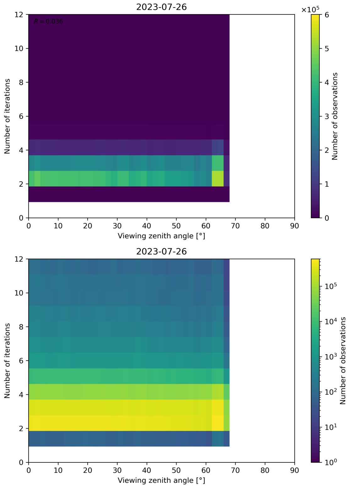
Figure 136: Scatter density plot of “Viewing zenith angle” against “Number of iterations” for 2023-07-25 to 2023-07-27.
