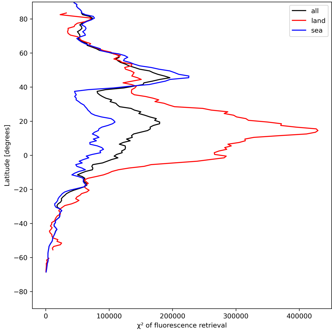
Figure 25: Zonal average of “ \chi^2 of fluorescence retrieval” for 2023-07-25 to 2023-07-27.
