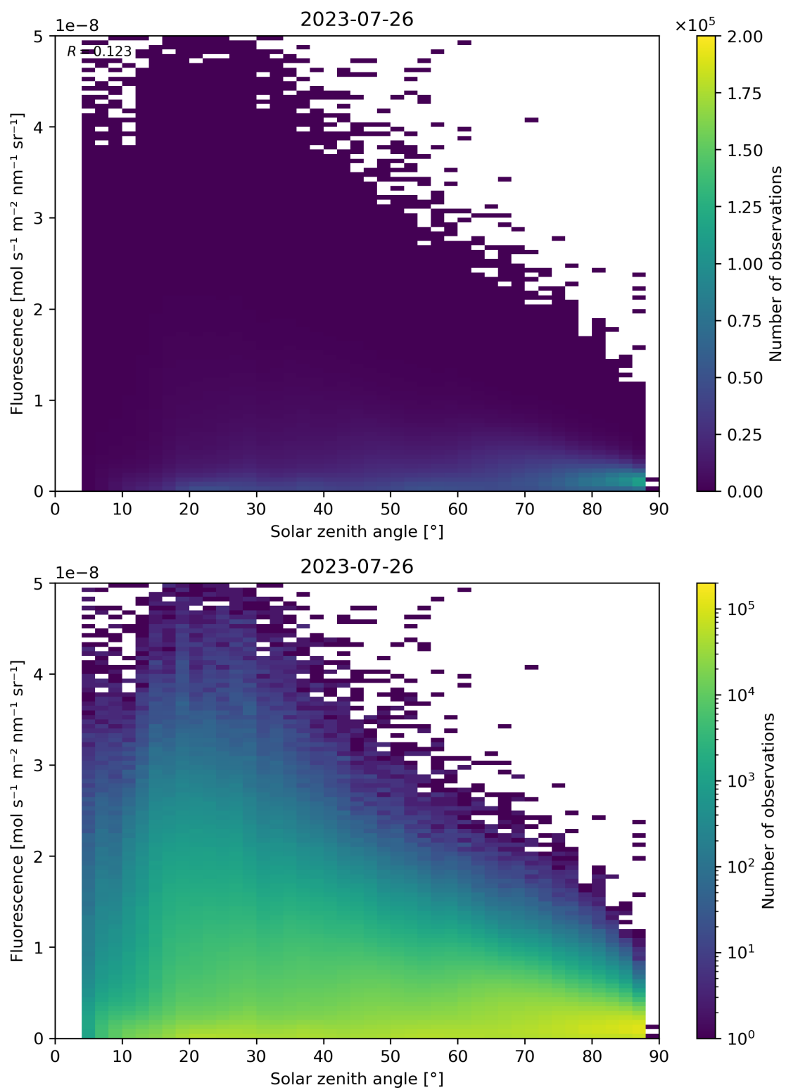
Figure 123: Scatter density plot of “Solar zenith angle” against “Fluorescence” for 2023-07-25 to 2023-07-27.
