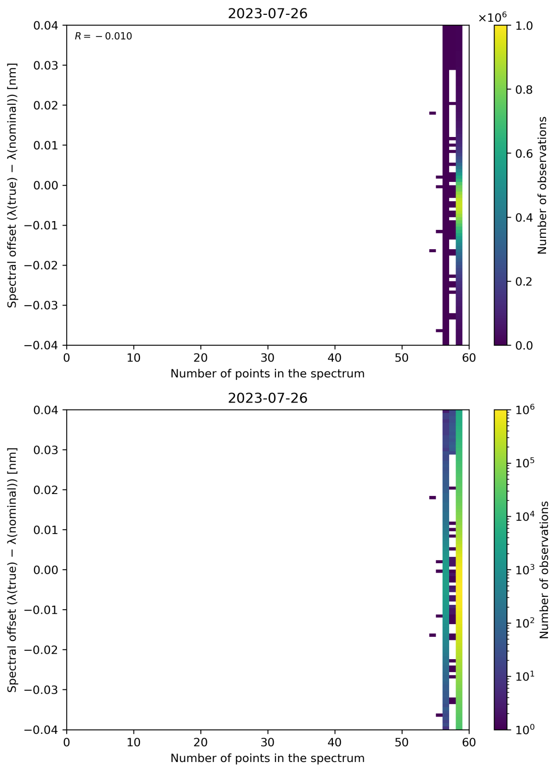
Figure 110: Scatter density plot of “Number of points in the spectrum” against “Spectral offset ( \lambda(\text{true}) - \lambda(\text{nominal}) )” for 2023-07-25 to 2023-07-27.
