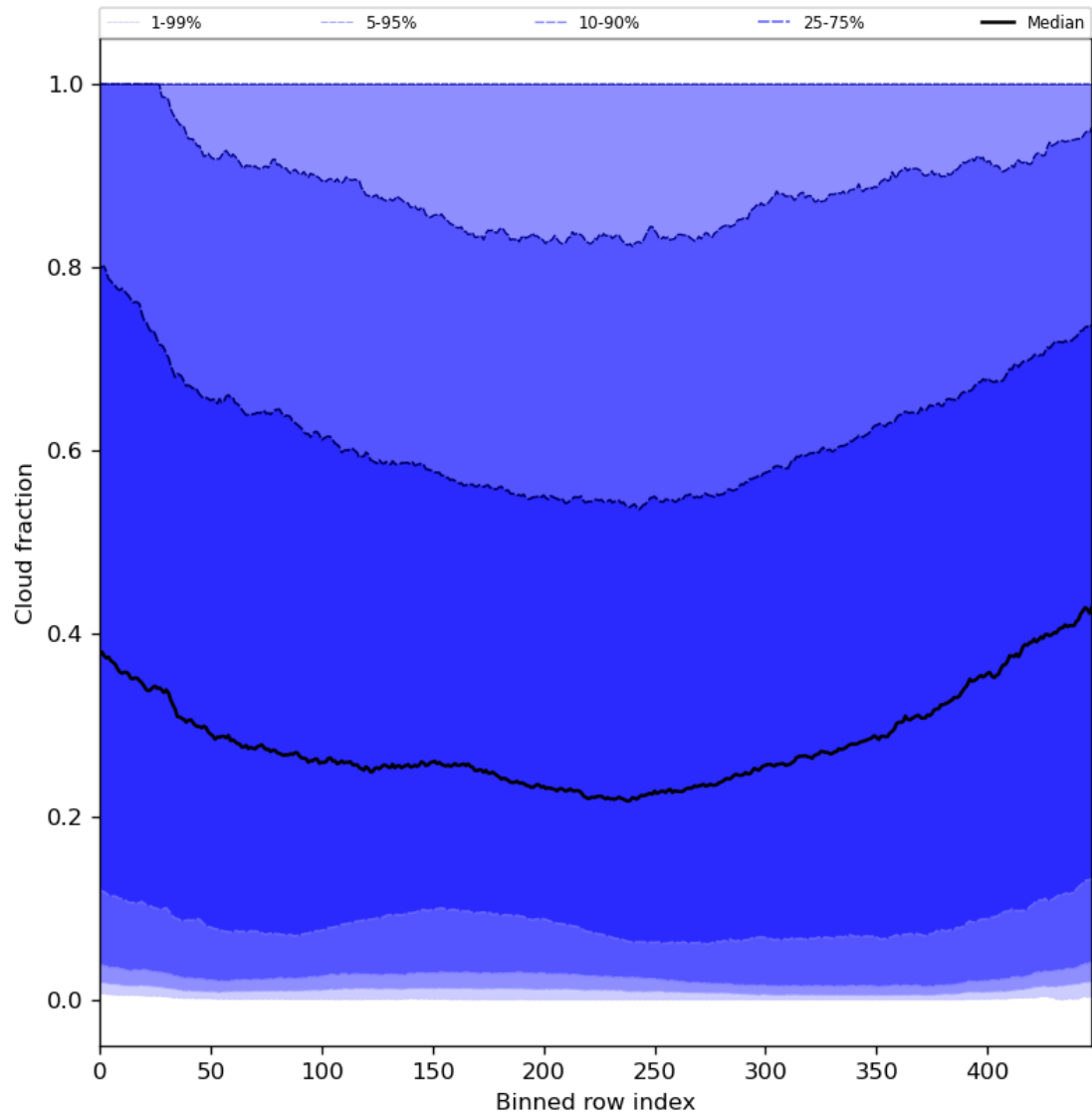
Figure 49: Along track statistics of “Cloud fraction” for 2023-07-25 to 2023-07-27
