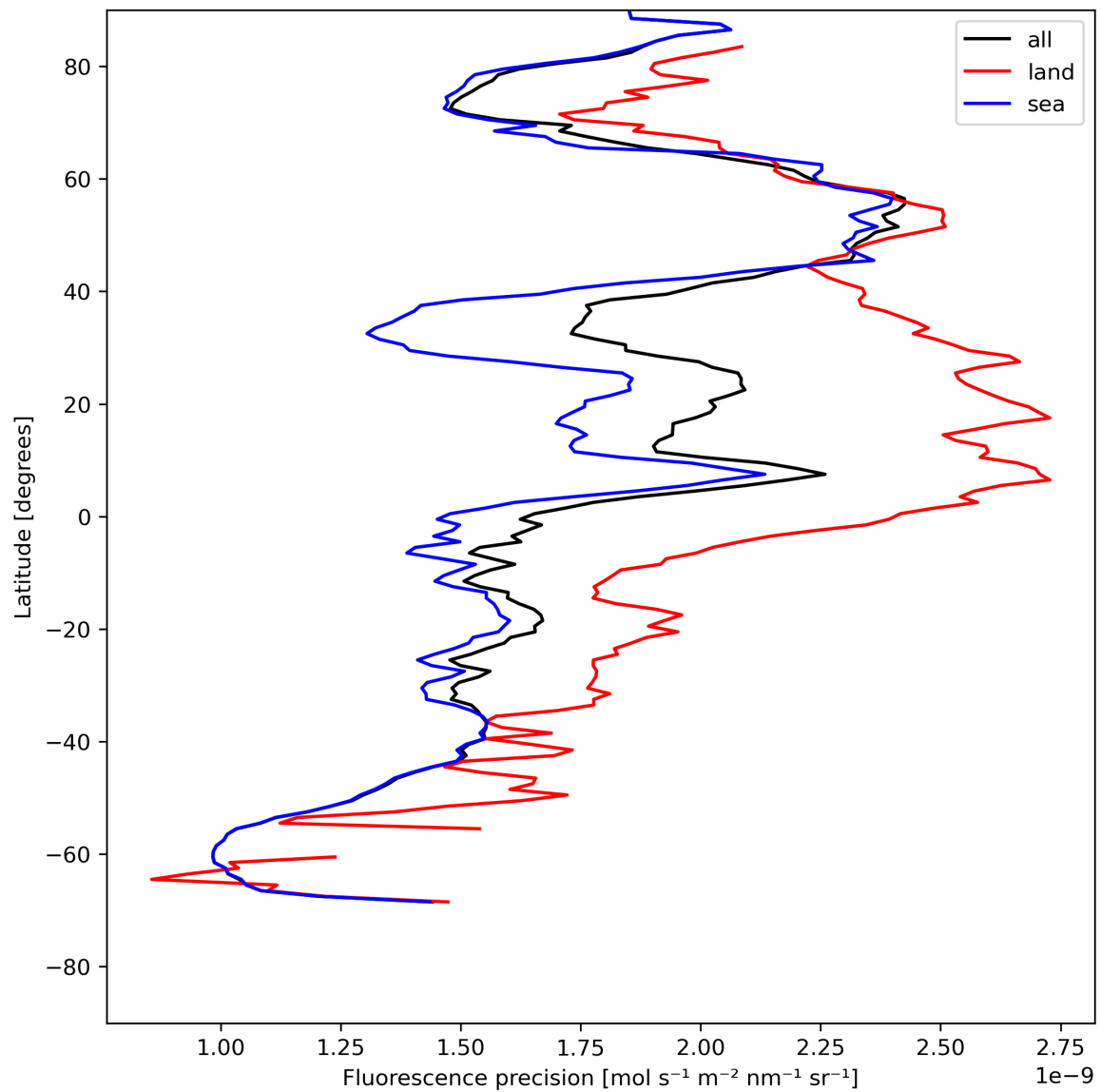
Figure 24: Zonal average of “Fluorescence precision” for 2023-07-25 to 2023-07-27.
