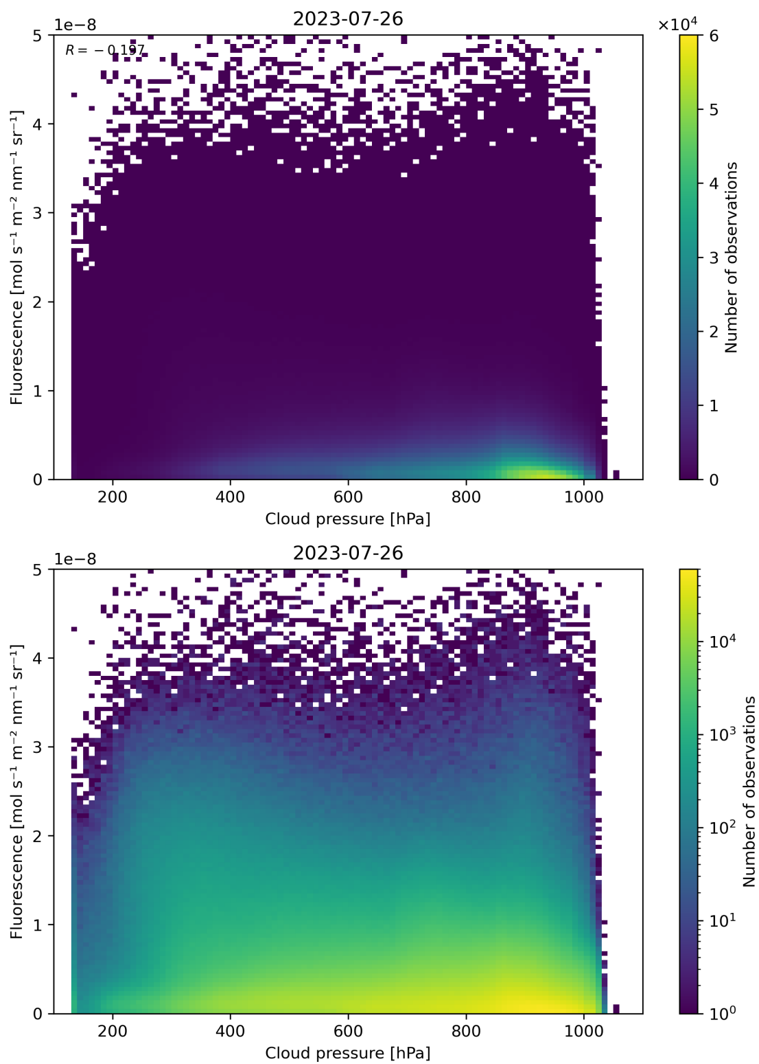
Figure 88: Scatter density plot of “Cloud pressure” against “Fluorescence” for 2023-07-25 to 2023-07-27.
