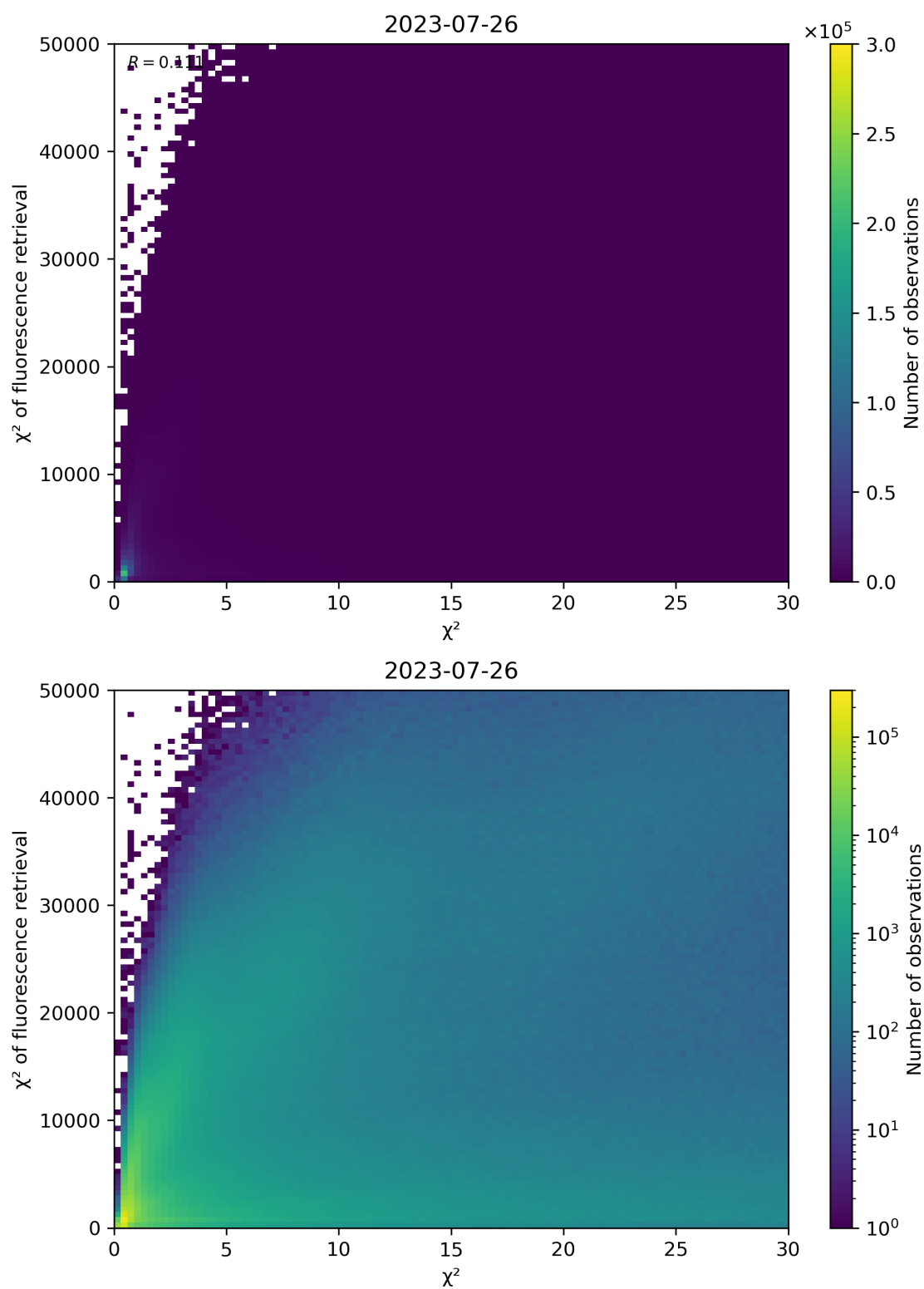
Figure 69: Scatter density plot of “ \chi^2 ” against “ \chi^2 of fluorescence retrieval” for 2023-07-25 to 2023-07-27.
