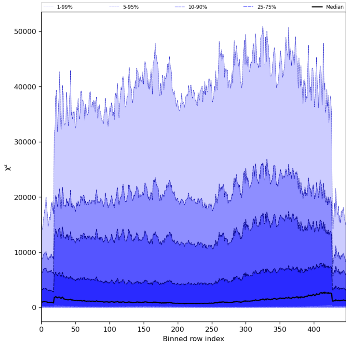
Figure 55: Along track statistics of “ \chi^2 ” for 2023-07-25 to 2023-07-27
