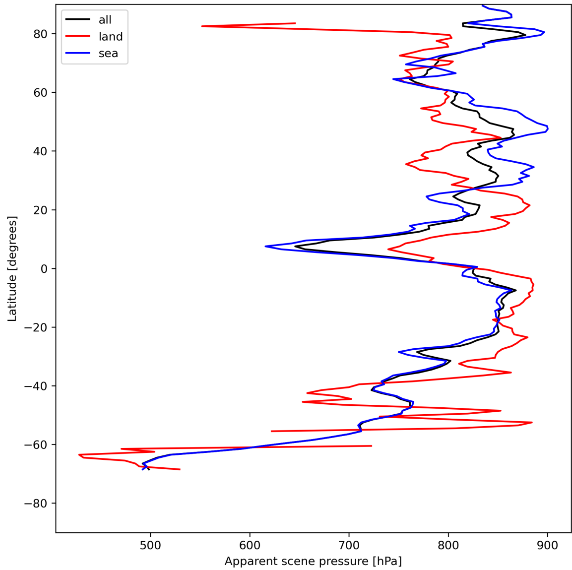
Figure 19: Zonal average of “Apparent scene pressure” for 2023-07-25 to 2023-07-27.
