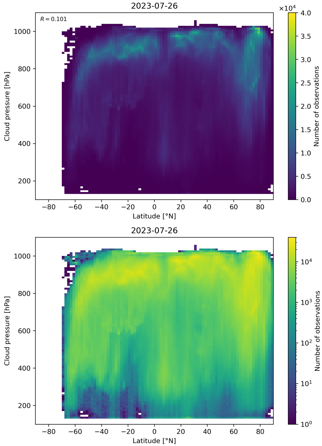
Figure 100: Scatter density plot of “Latitude” against “Cloud pressure” for 2023-07-25 to 2023-07-27.
