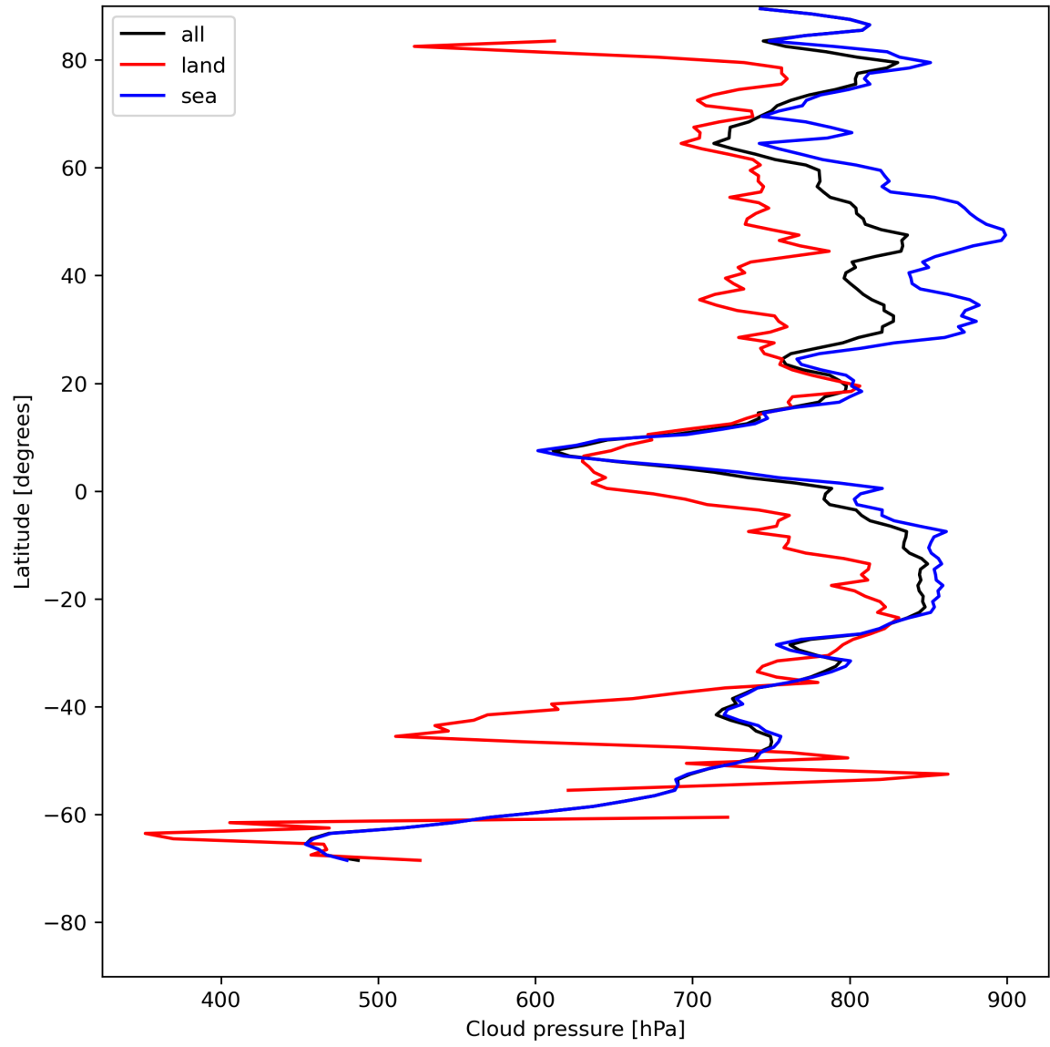
Figure 13: Zonal average of “Cloud pressure” for 2023-07-25 to 2023-07-27.
