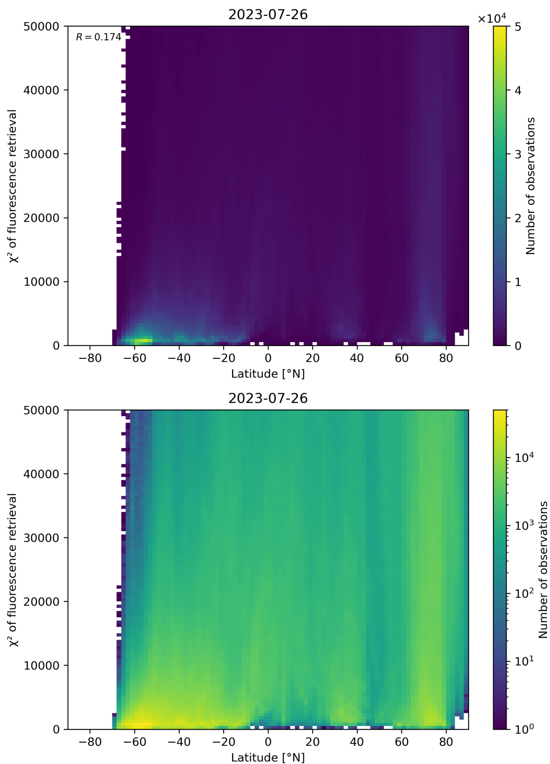
Figure 98: Scatter density plot of “Latitude” against “ \chi^2 of fluorescence retrieval” for 2023-07-25 to 2023-07-27.
