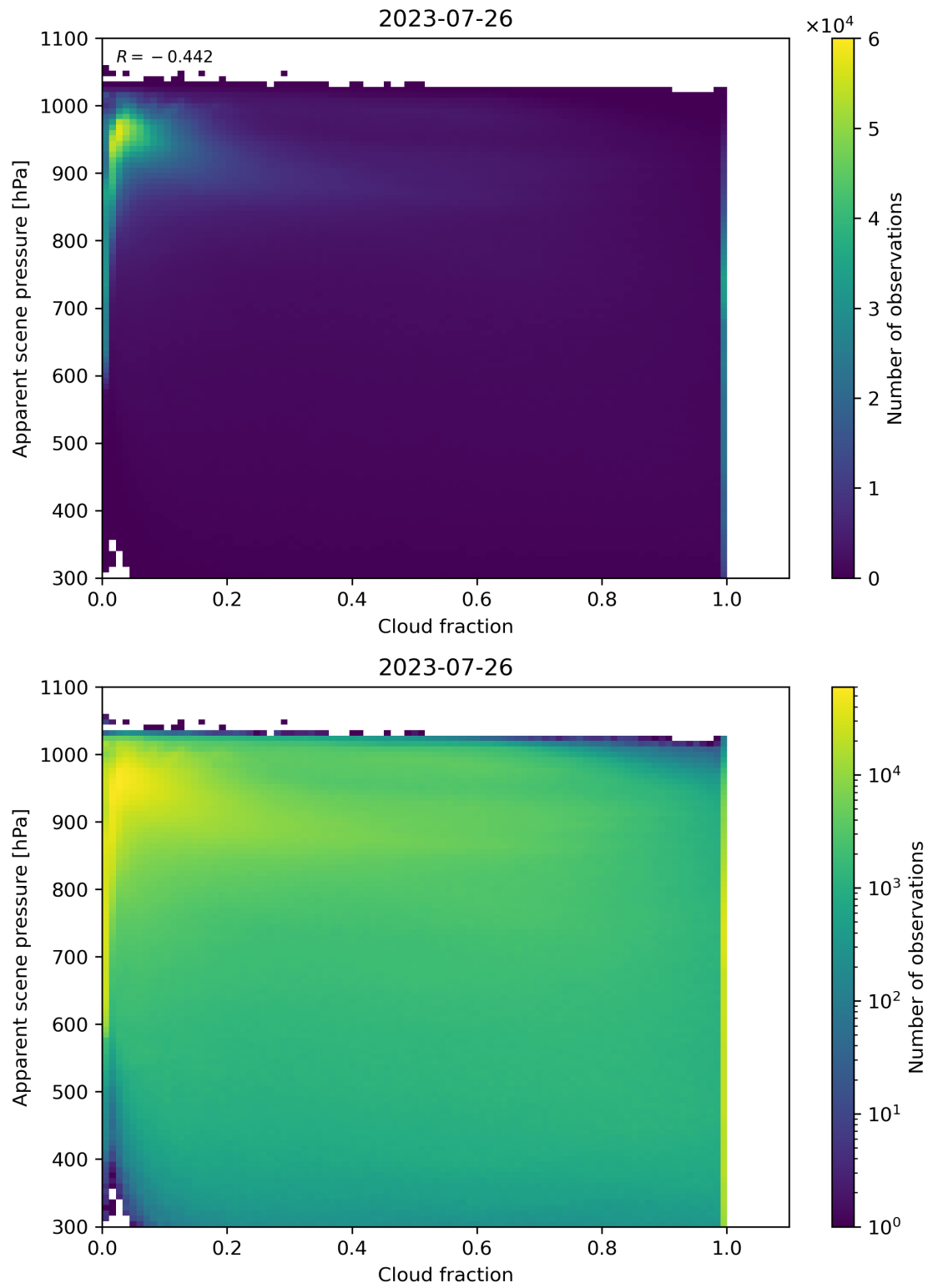
Figure 76: Scatter density plot of “Cloud fraction” against “Apparent scene pressure” for 2023-07-25 to 2023-07-27.
