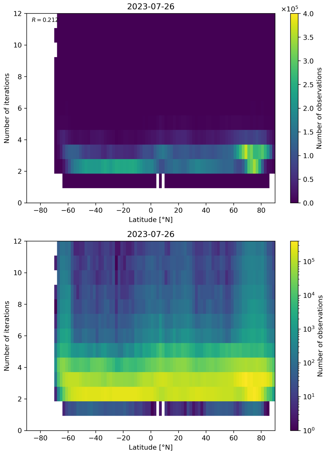
Figure 102: Scatter density plot of “Latitude” against “Number of iterations” for 2023-07-25 to 2023-07-27.
