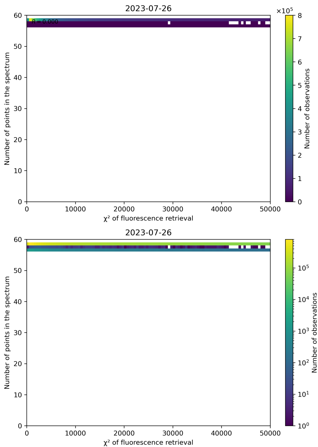
Figure 71: Scatter density plot of “ \chi^2 of fluorescence retrieval” against “Number of points in the spectrum” for 2023-07-25 to 2023-07-27.
