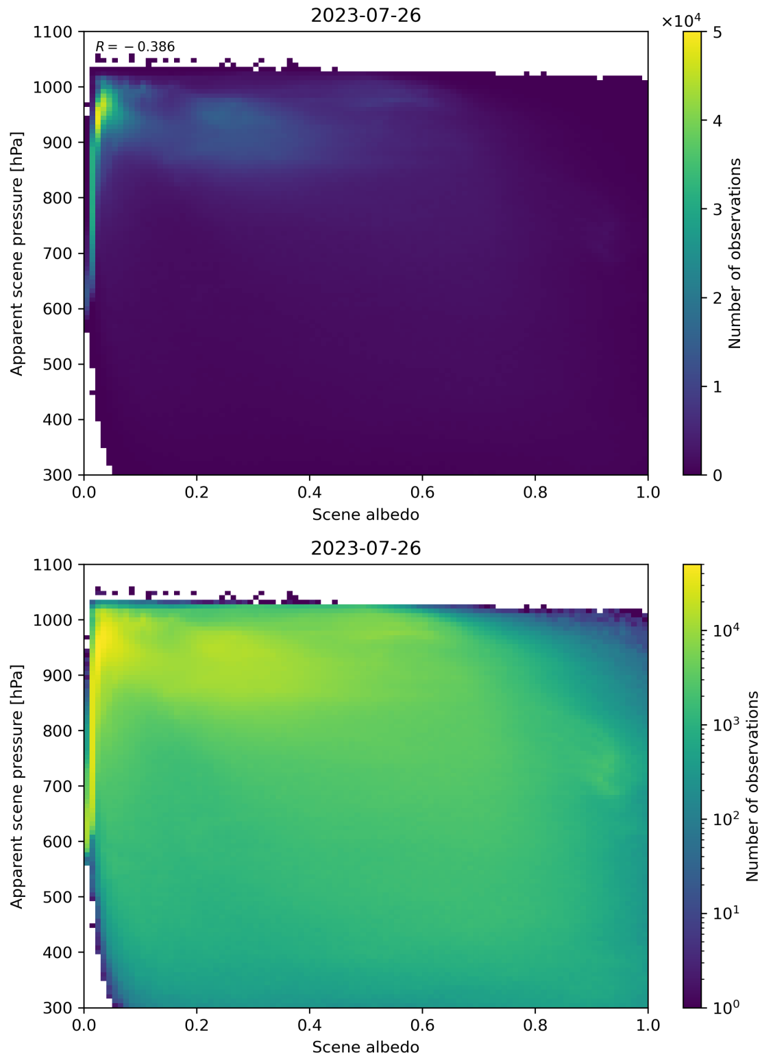
Figure 111: Scatter density plot of “Scene albedo” against “Apparent scene pressure” for 2023-07-25 to 2023-07-27.
