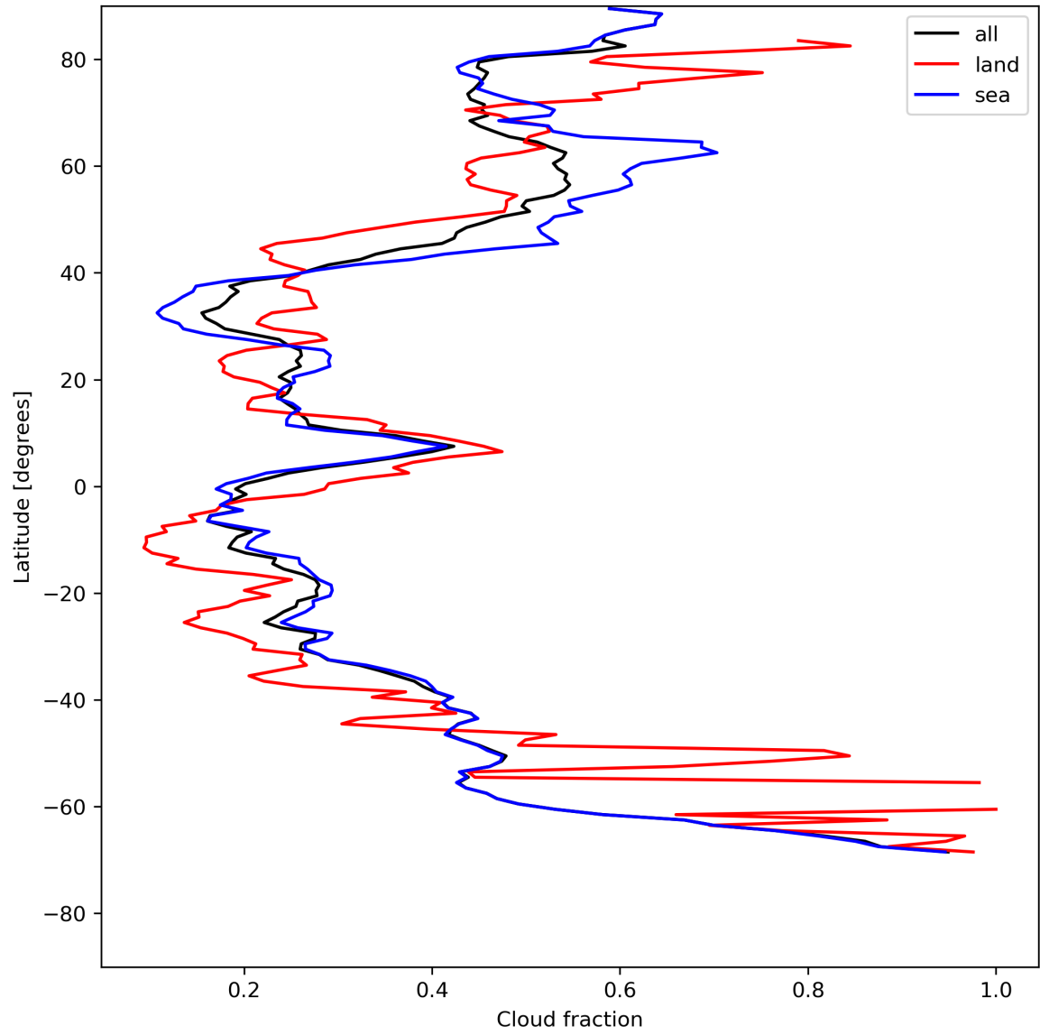
Figure 15: Zonal average of “Cloud fraction” for 2023-07-25 to 2023-07-27.
