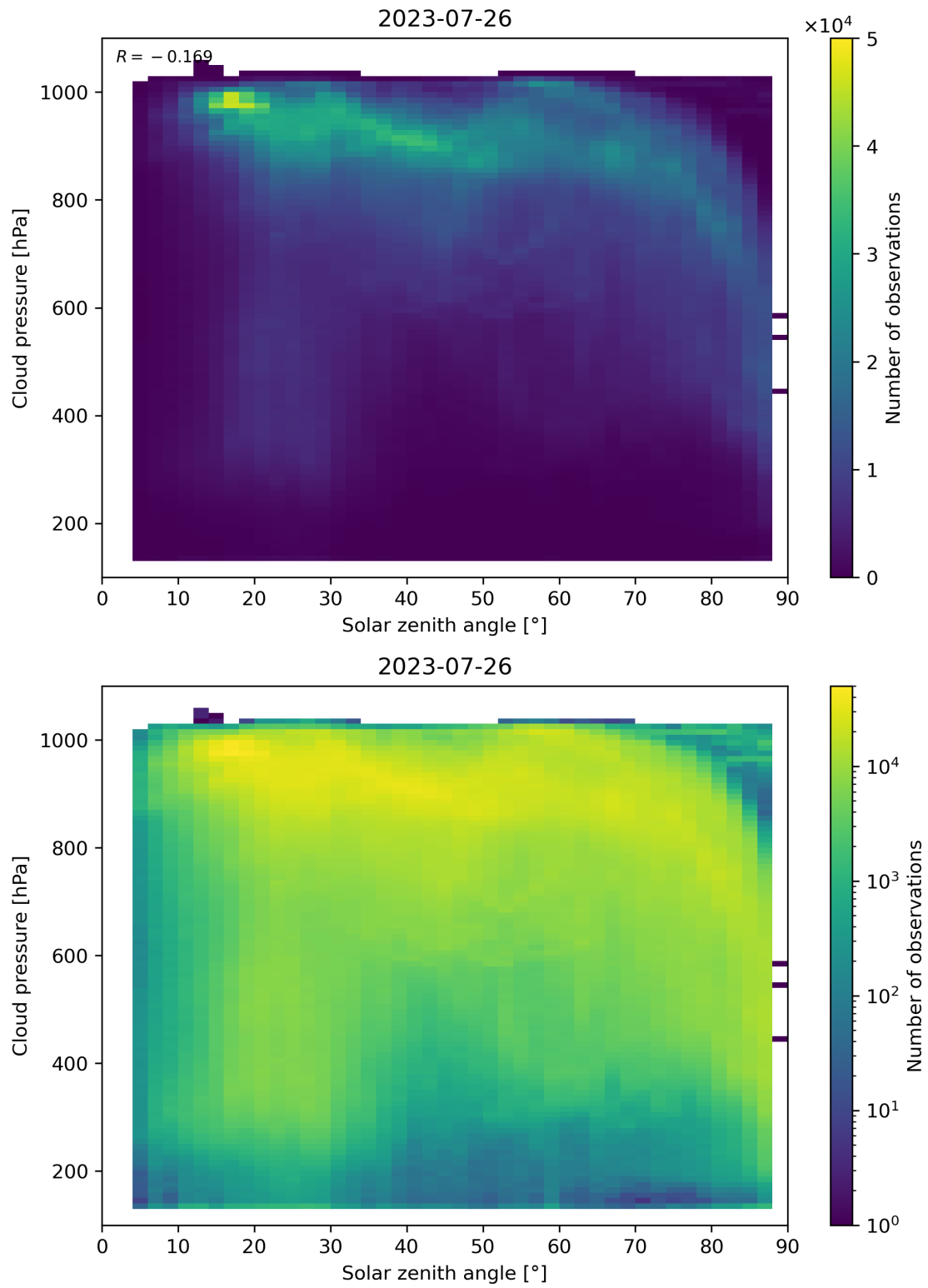
Figure 122: Scatter density plot of “Solar zenith angle” against “Cloud pressure” for 2023-07-25 to 2023-07-27.
