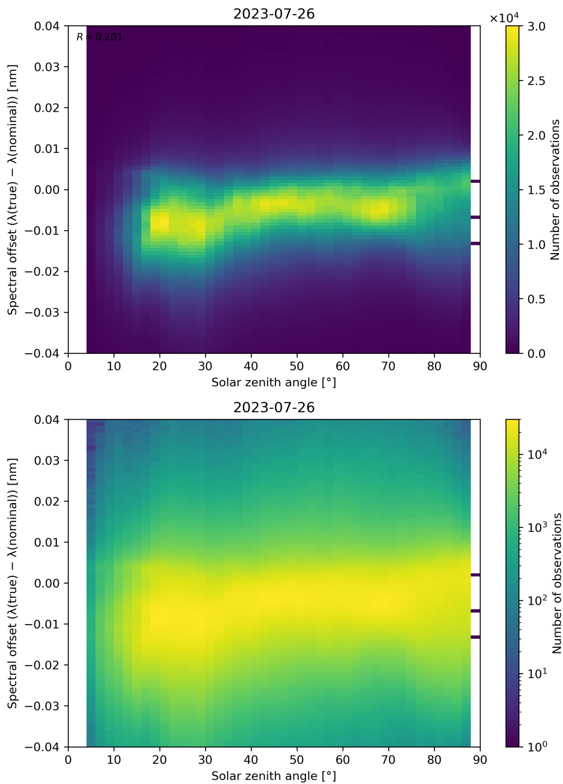
Figure 128: Scatter density plot of “Solar zenith angle” against “Spectral offset ( \lambda(\text{true}) - \lambda(\text{nominal}) )” for 2023-07-25 to 2023-07-27.
