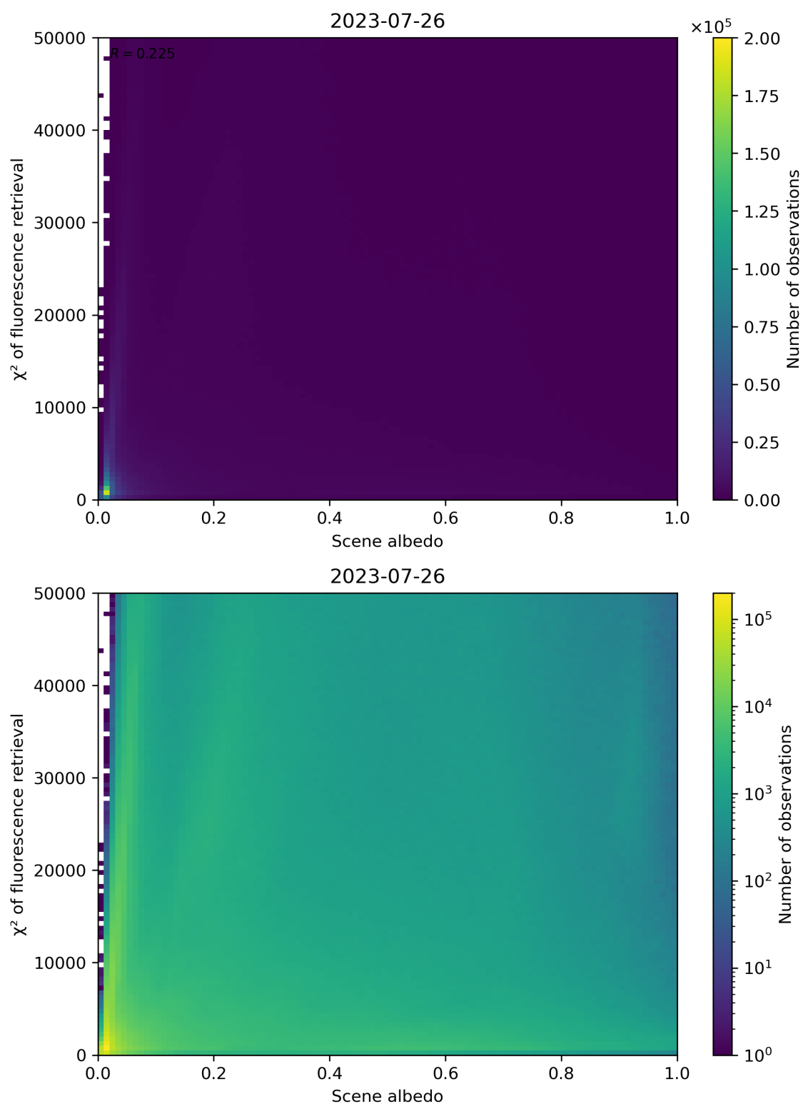
Figure 113: Scatter density plot of “Scene albedo” against “ \chi^2 of fluorescence retrieval” for 2023-07-25 to 2023-07-27.
