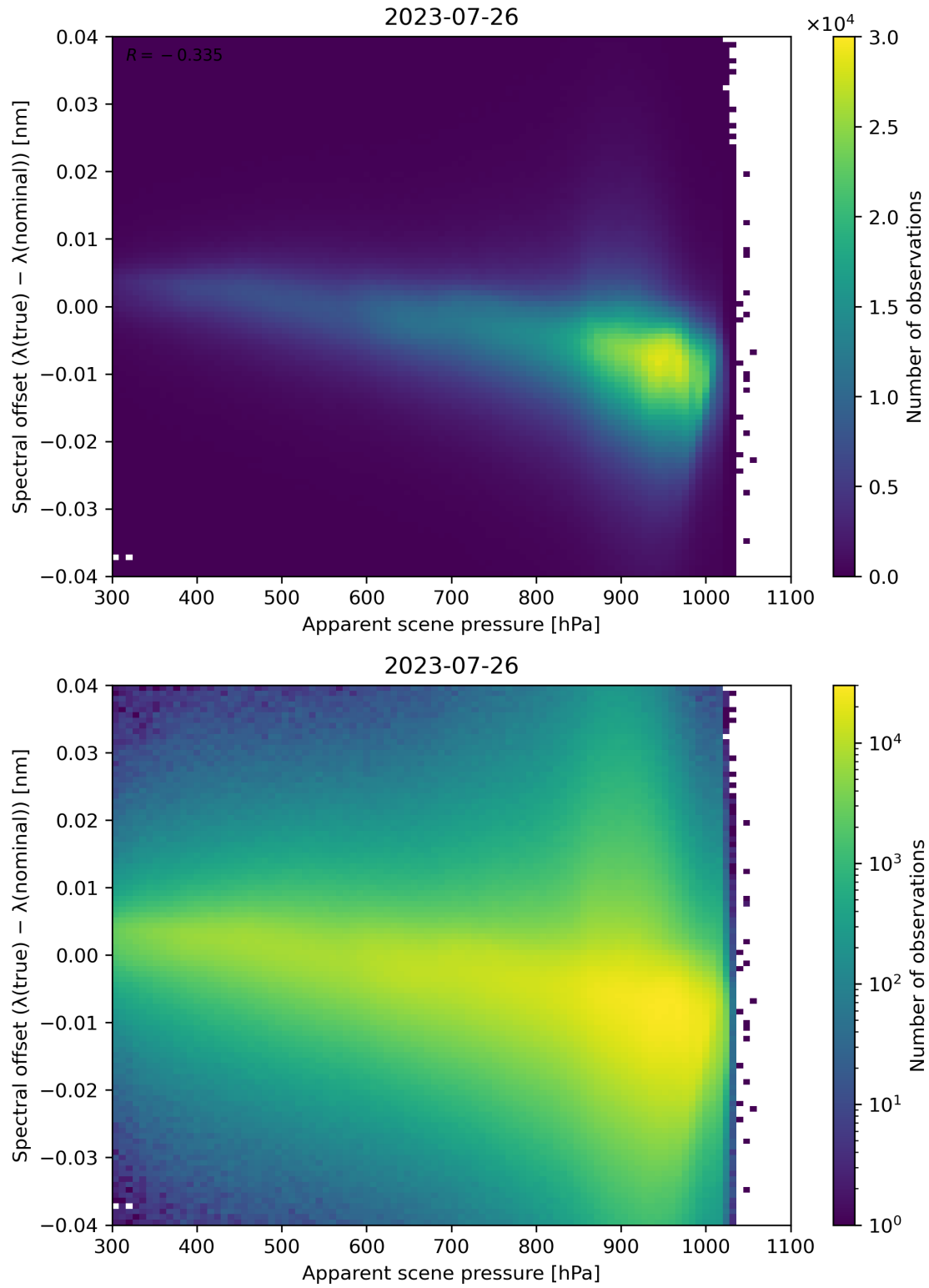
Figure 68: Scatter density plot of “Apparent scene pressure” against “Spectral offset ( \lambda(\text{true}) - \lambda(\text{nominal}) )” for 2023-07-25 to 2023-07-27.
