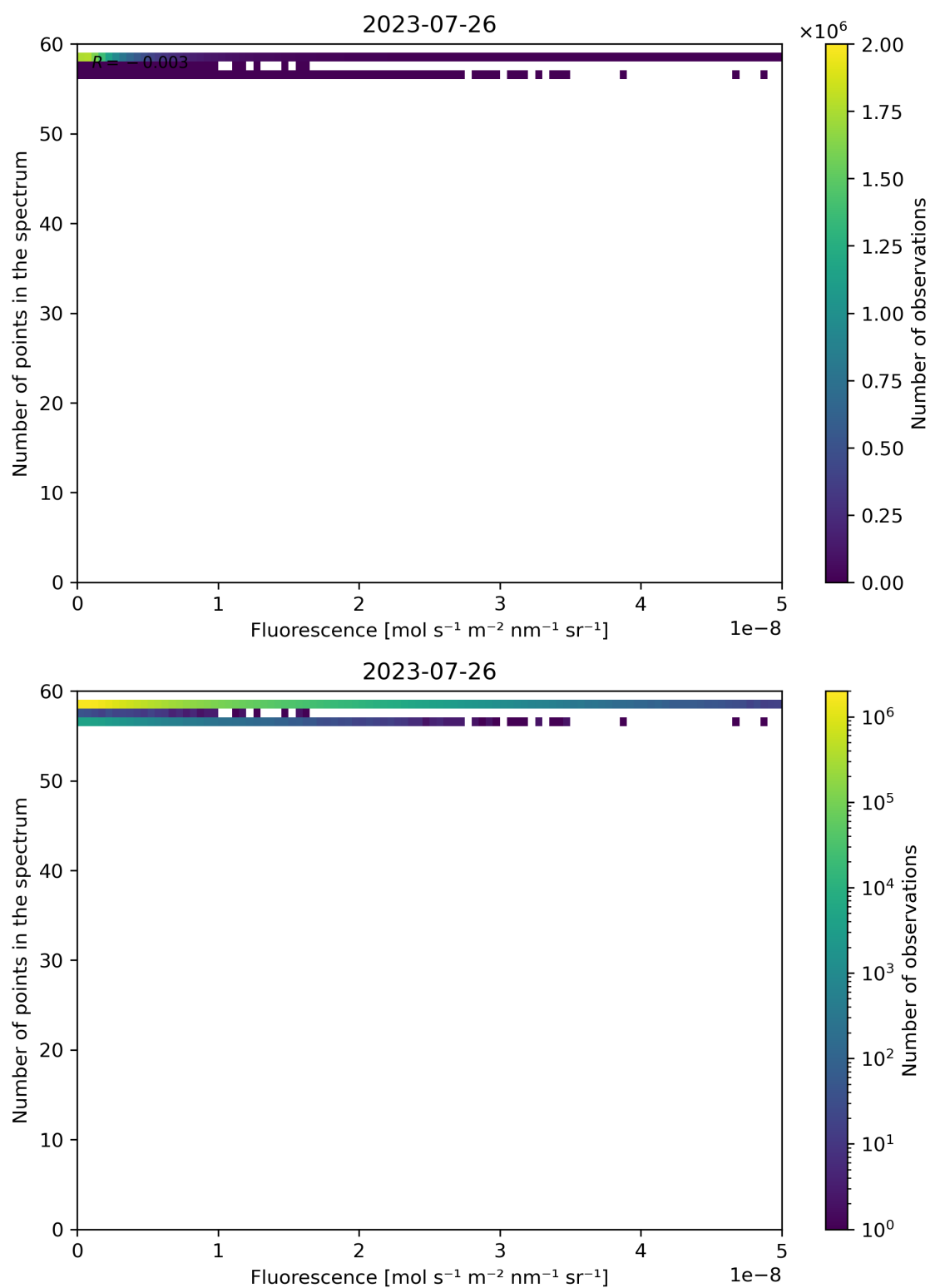
Figure 94: Scatter density plot of “Fluorescence” against “Number of points in the spectrum” for 2023-07-25 to 2023-07-27.
