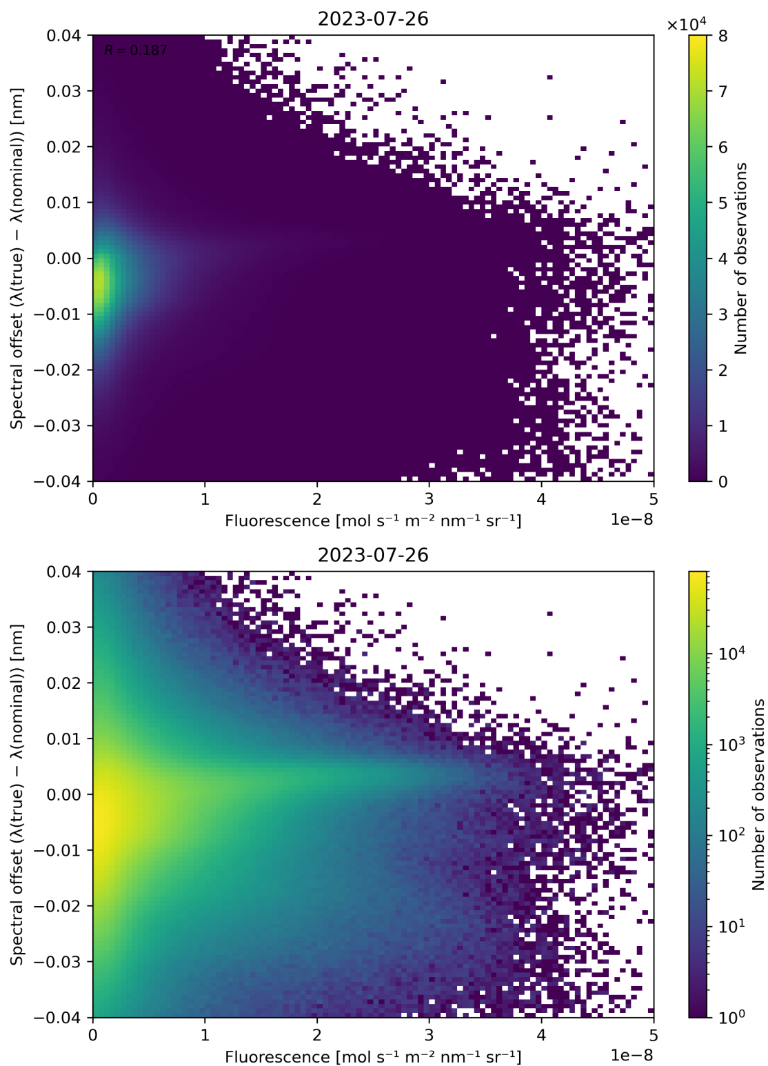
Figure 95: Scatter density plot of “Fluorescence” against “Spectral offset ( \lambda(\text{true}) - \lambda(\text{nominal}) )” for 2023-07-25 to 2023-07-27.
