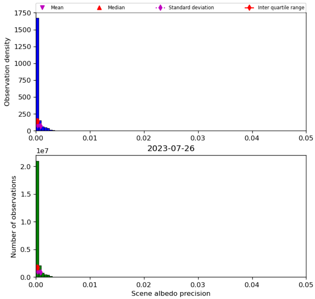
Figure 35: Histogram of “Scene albedo precision” for 2023-07-25 to 2023-07-27
