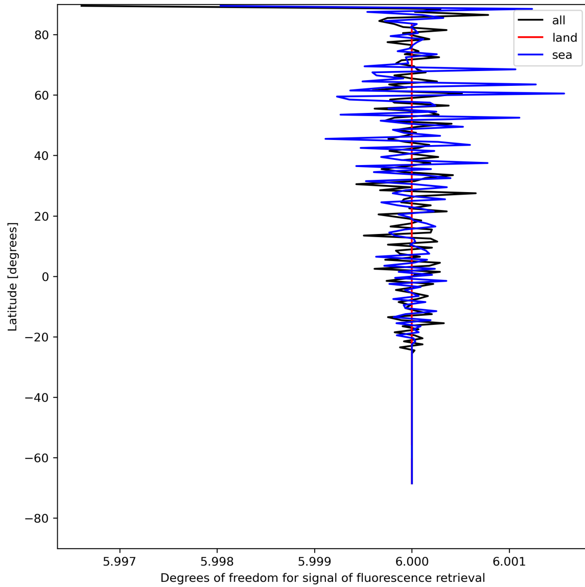
Figure 26: Zonal average of “Degrees of freedom for signal of fluorescence retrieval” for 2023-07-25 to 2023-07-27.
