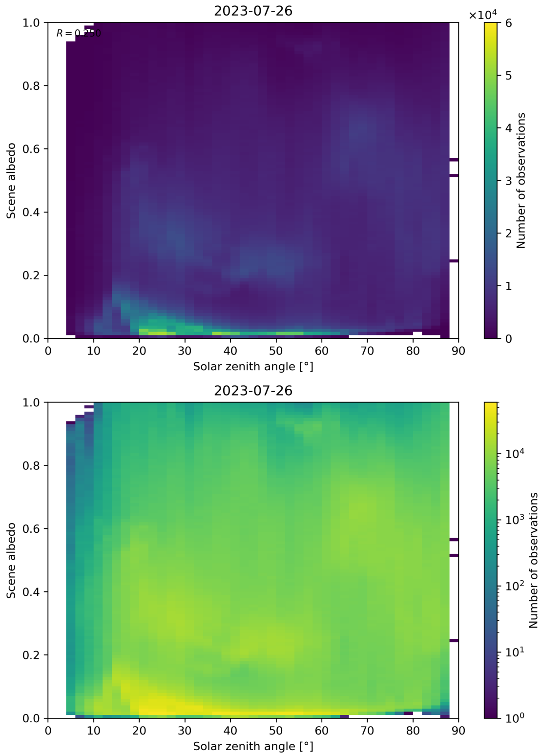
Figure 127: Scatter density plot of “Solar zenith angle” against “Scene albedo” for 2023-07-25 to 2023-07-27.
