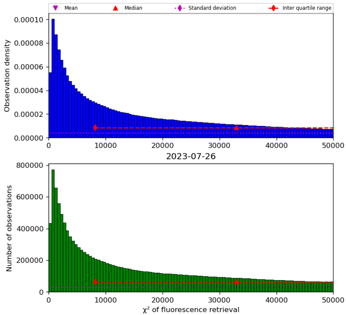
Figure 42: Histogram of “ \chi^2 of fluorescence retrieval” for 2023-07-25 to 2023-07-27
