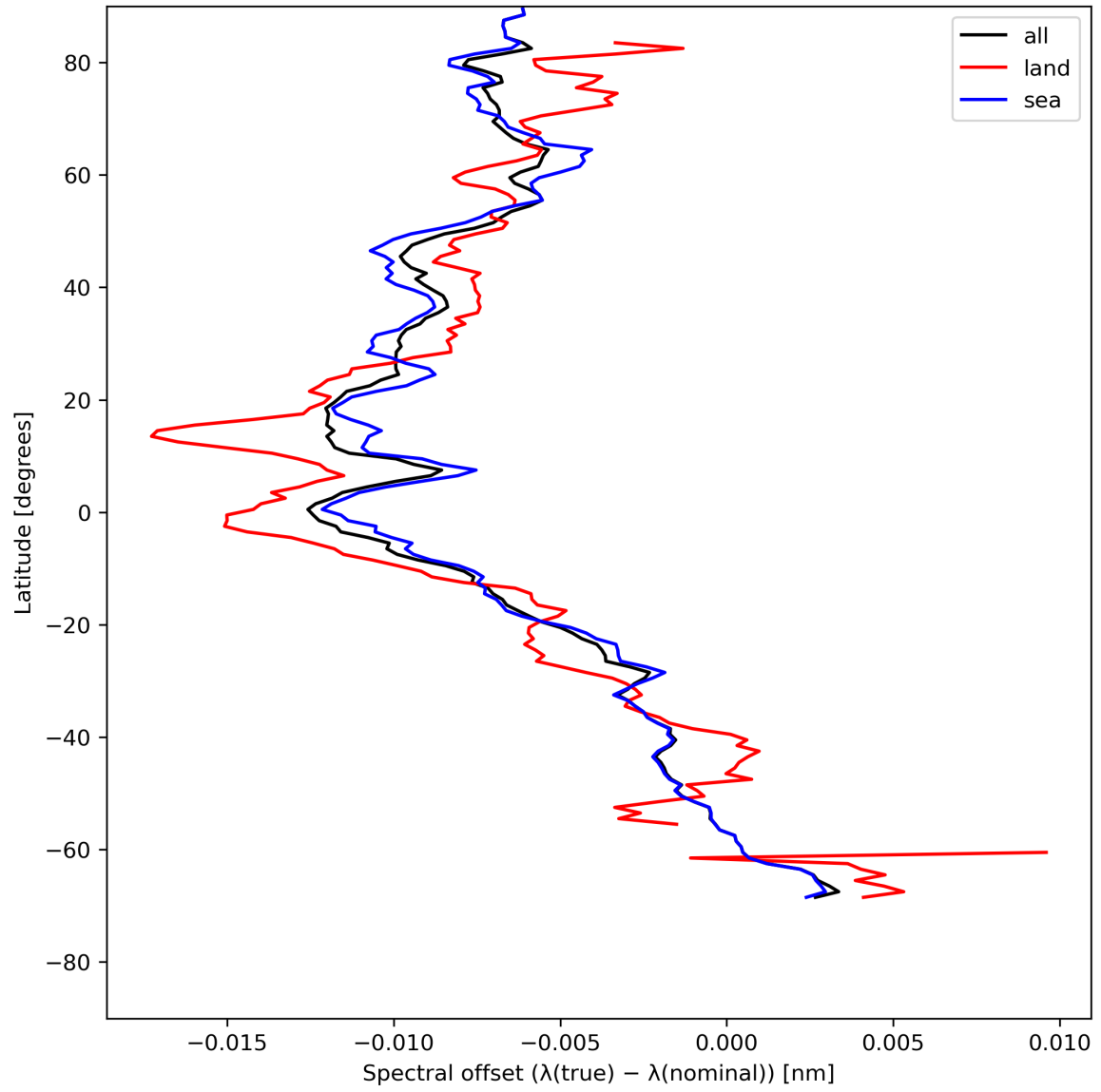
Figure 28: Zonal average of “Spectral offset ( \lambda(\text{true}) - \lambda(\text{nominal}) )” for 2023-07-25 to 2023-07-27.
