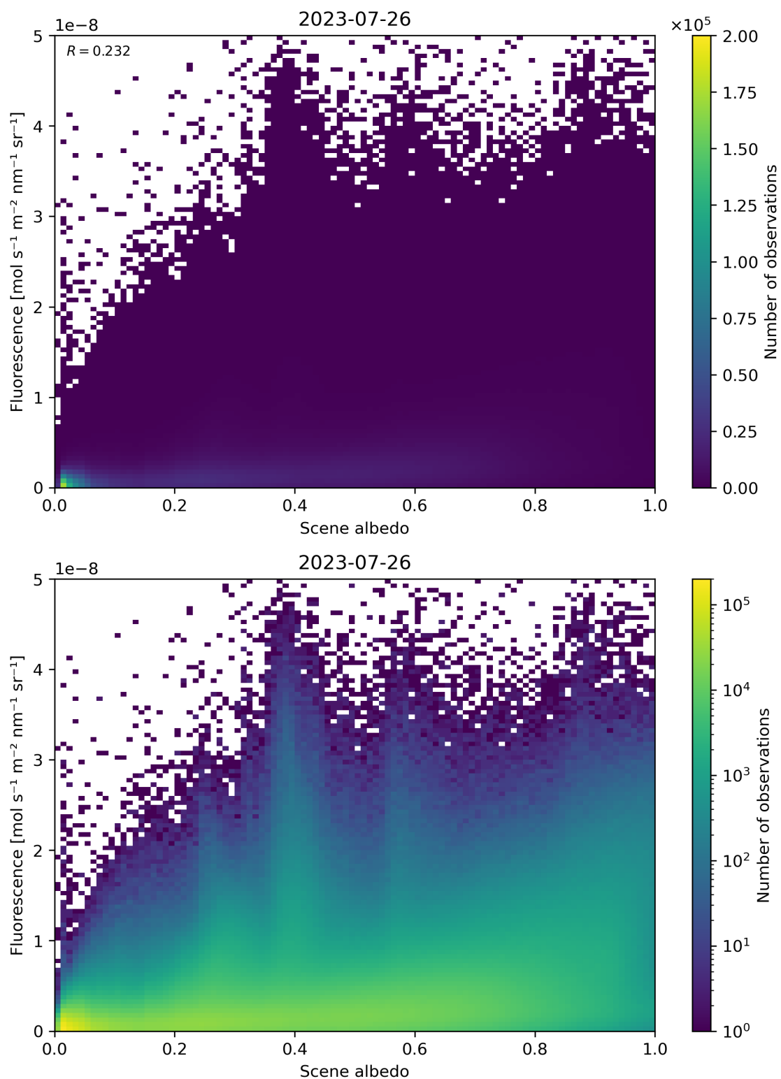
Figure 114: Scatter density plot of “Scene albedo” against “Fluorescence” for 2023-07-25 to 2023-07-27.
