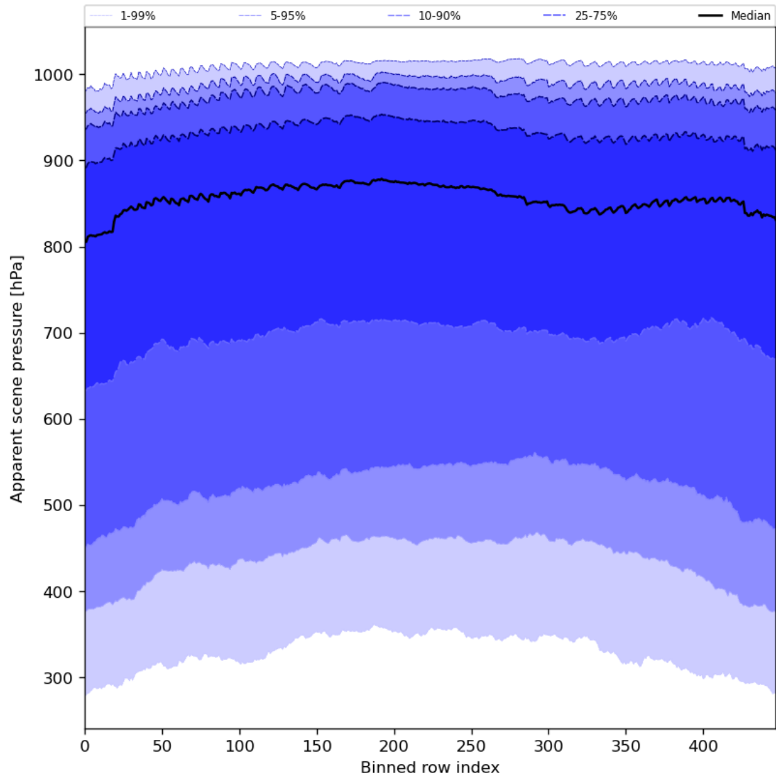
Figure 53: Along track statistics of “Apparent scene pressure” for 2023-07-25 to 2023-07-27
