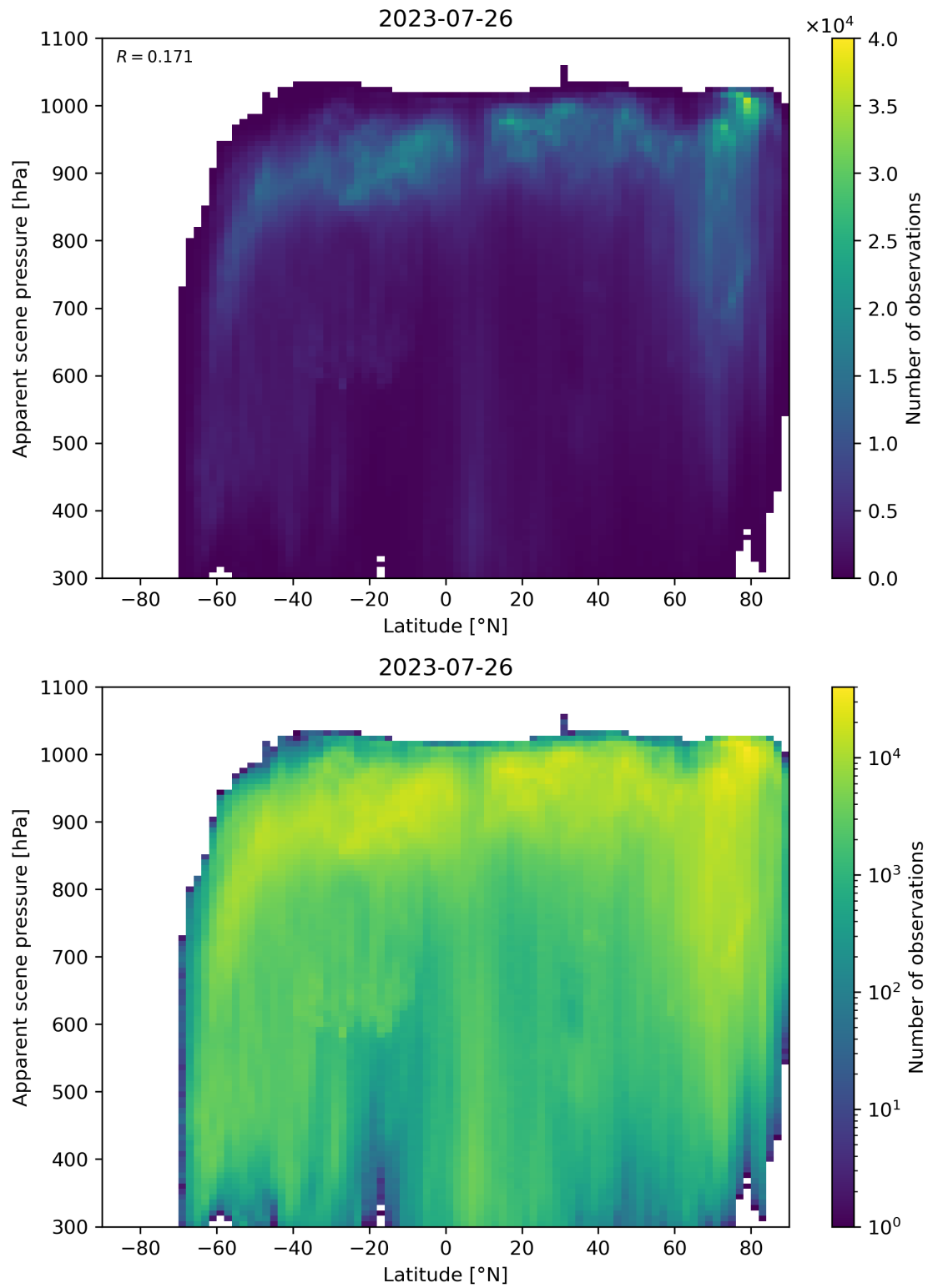
Figure 96: Scatter density plot of “Latitude” against “Apparent scene pressure” for 2023-07-25 to 2023-07-27.
