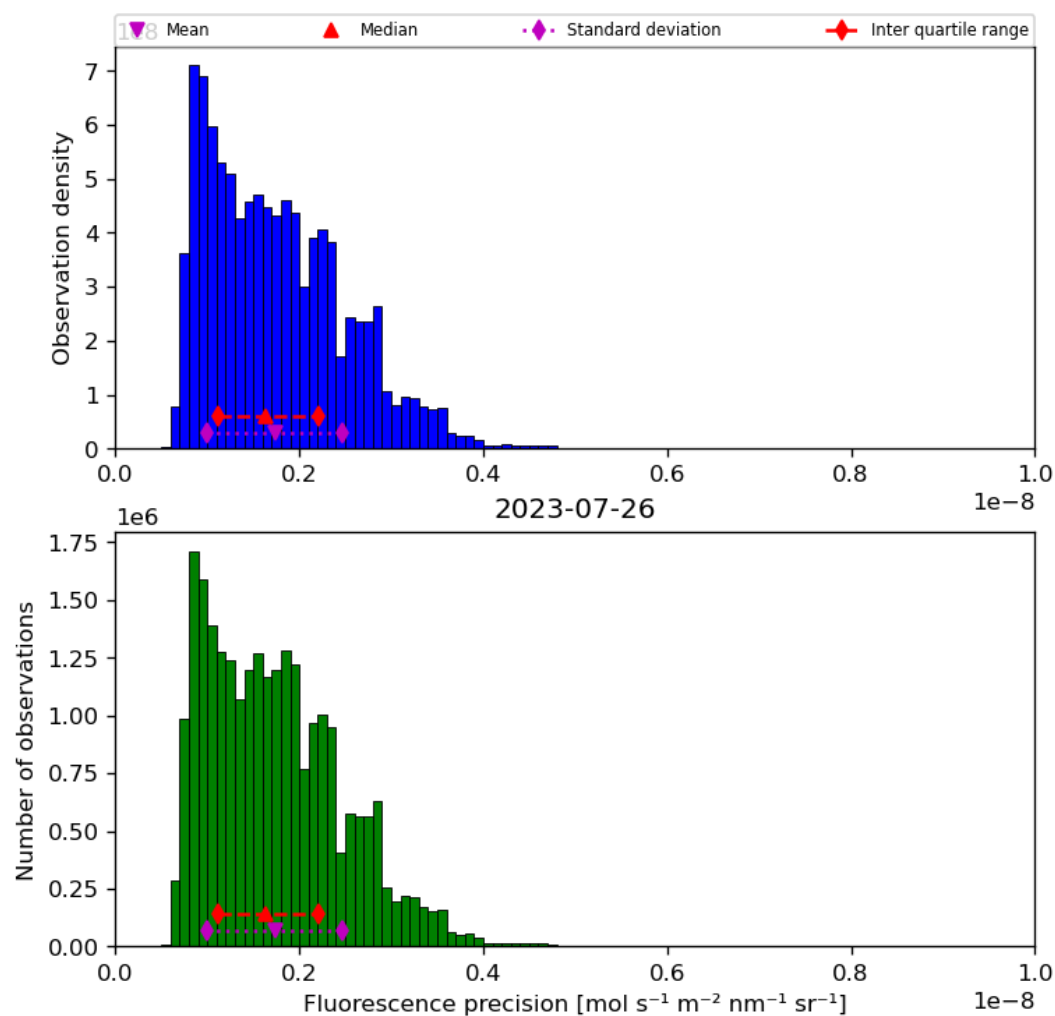
Figure 41: Histogram of “Fluorescence precision” for 2023-07-25 to 2023-07-27
