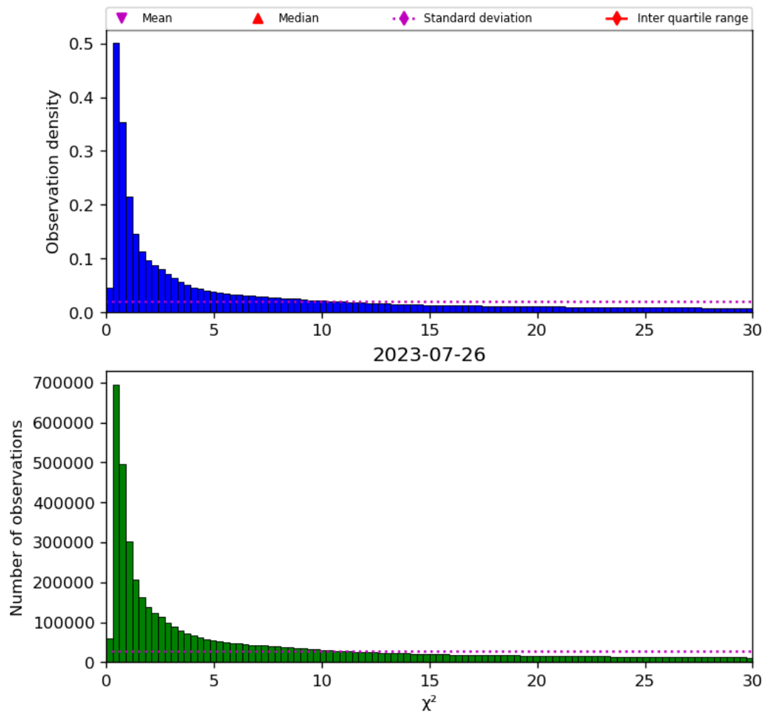
Figure 38: Histogram of " \chi^2 " for 2023-07-25 to 2023-07-27
