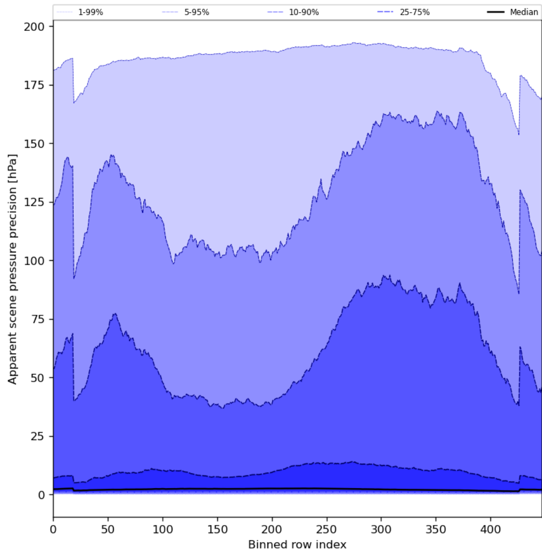
Figure 54: Along track statistics of “Apparent scene pressure precision” for 2023-07-25 to 2023-07-27
