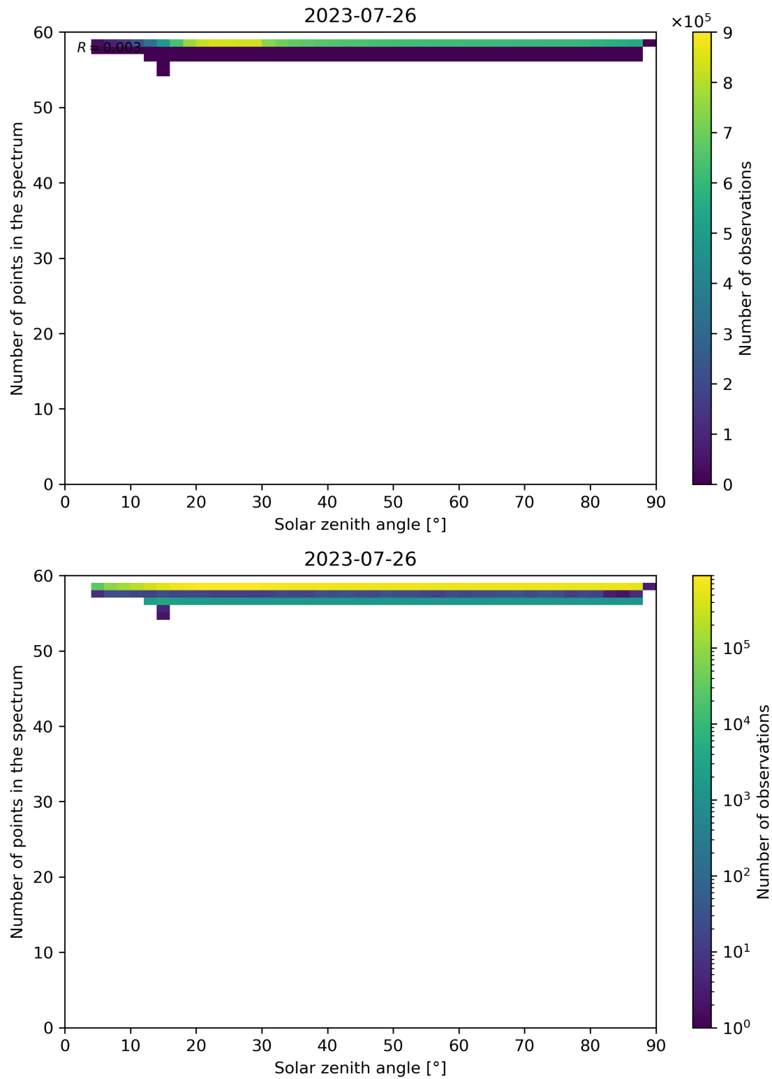
Figure 126: Scatter density plot of “Solar zenith angle” against “Number of points in the spectrum” for 2023-07-25 to 2023-07-27.
