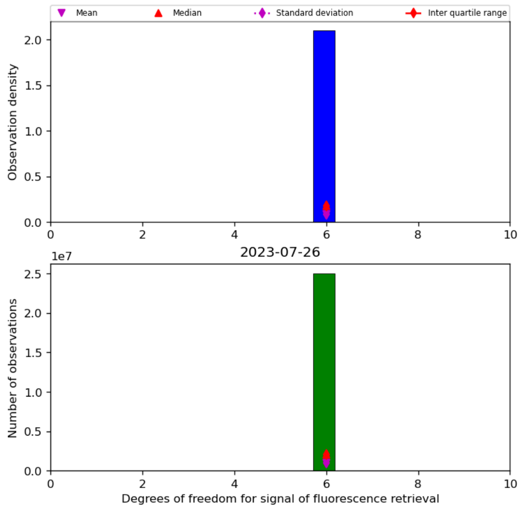
Figure 43: Histogram of “Degrees of freedom for signal of fluorescence retrieval” for 2023-07-25 to 2023-07-27
