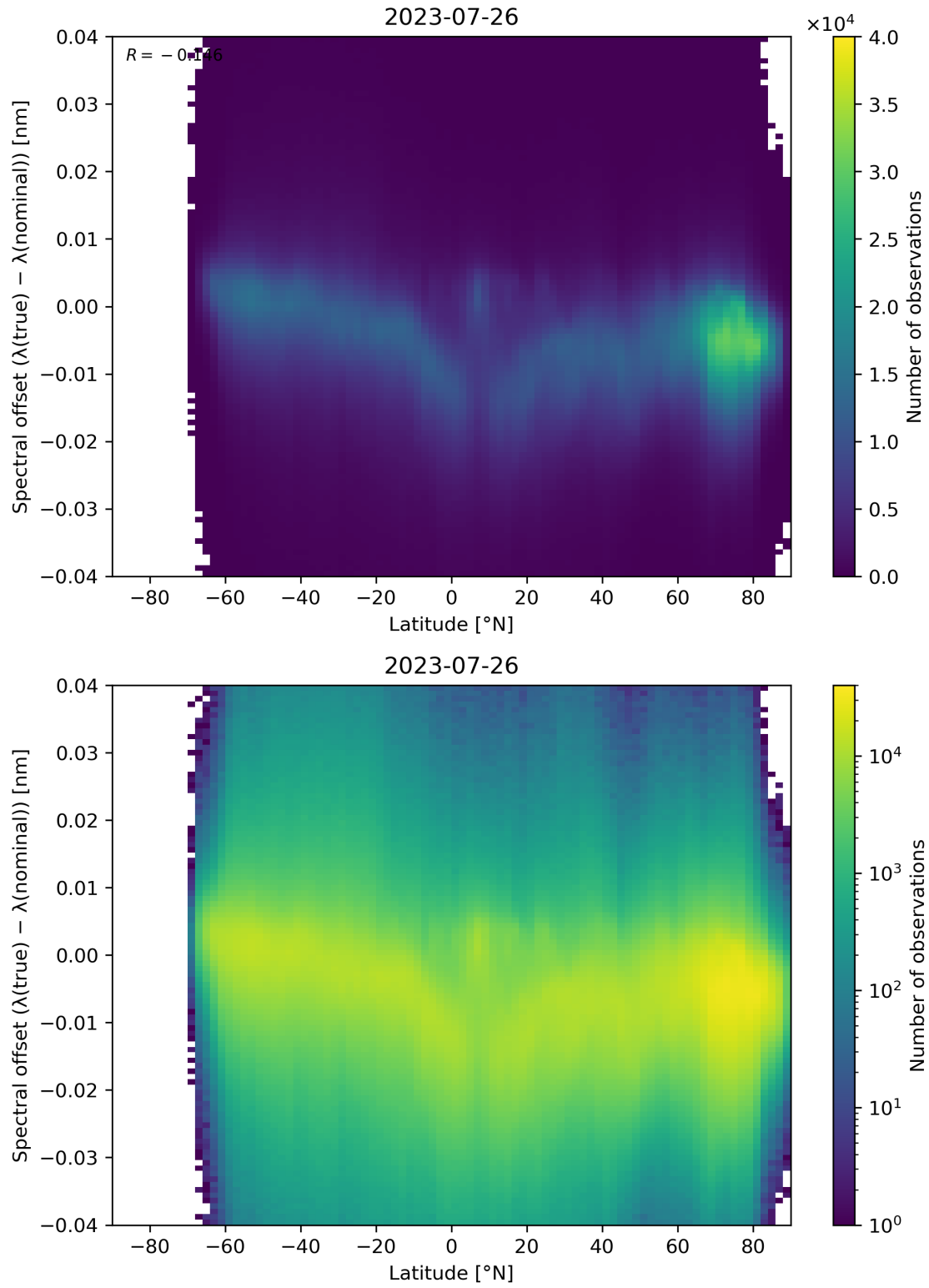
Figure 105: Scatter density plot of “Latitude” against “Spectral offset ( \lambda(\text{true}) - \lambda(\text{nominal}) )” for 2023-07-25 to 2023-07-27.
