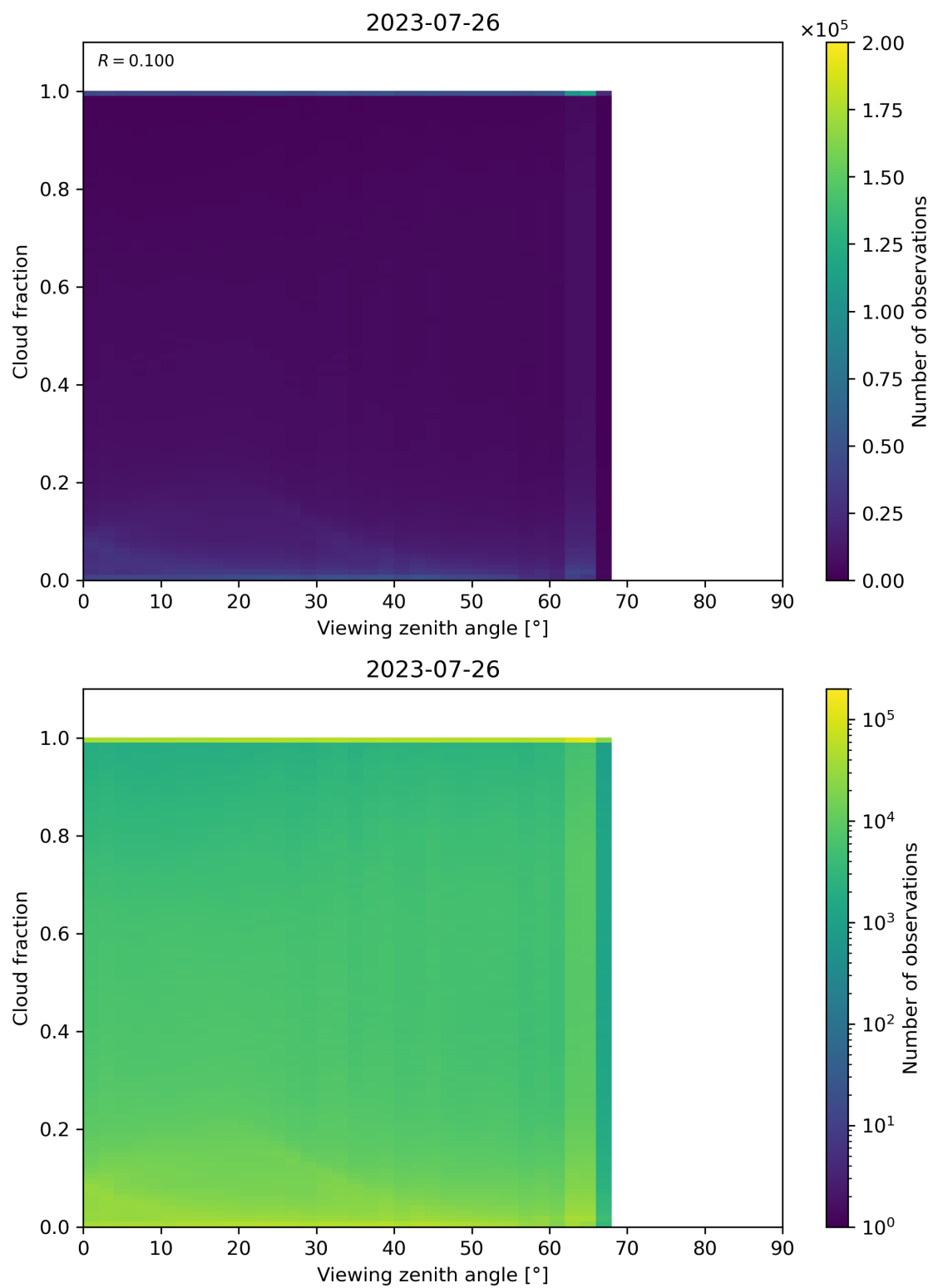
Figure 132: Scatter density plot of “Viewing zenith angle” against “Cloud fraction” for 2023-07-25 to 2023-07-27.
