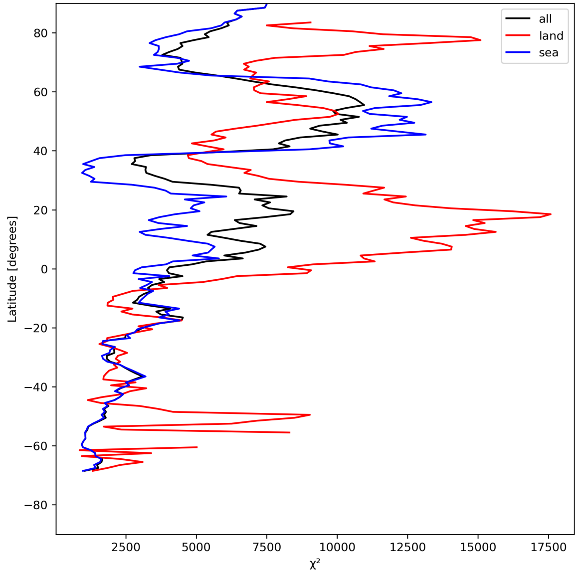
Figure 21: Zonal average of “ \chi^2 ” for 2023-07-25 to 2023-07-27.
