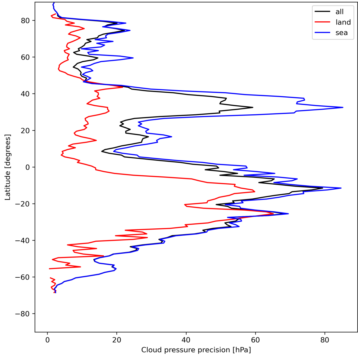
Figure 14: Zonal average of “Cloud pressure precision” for 2023-07-25 to 2023-07-27.
