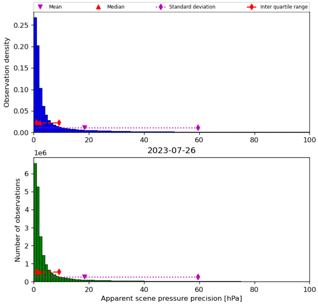
Figure 37: Histogram of “Apparent scene pressure precision” for 2023-07-25 to 2023-07-27
