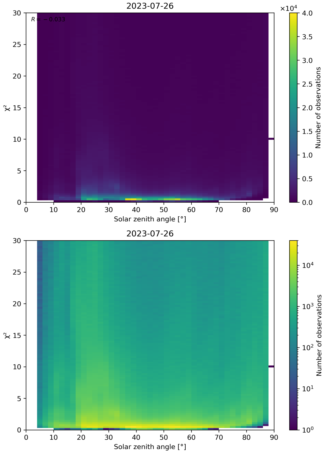
Figure 119: Scatter density plot of “Solar zenith angle” against “ \chi^2 ” for 2023-07-25 to 2023-07-27.
