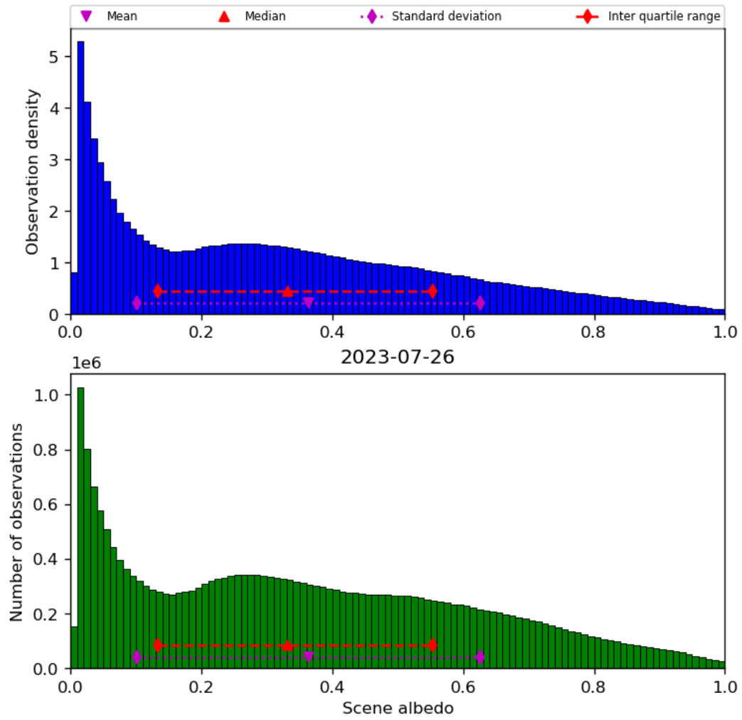
Figure 34: Histogram of “Scene albedo” for 2023-07-25 to 2023-07-27
