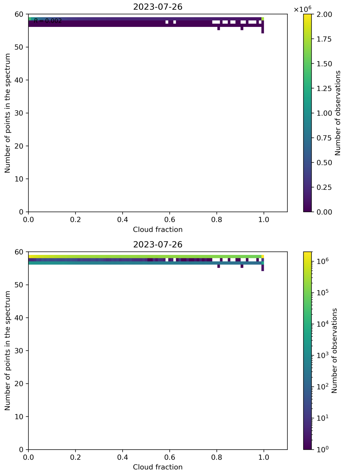
Figure 81: Scatter density plot of “Cloud fraction” against “Number of points in the spectrum” for 2023-07-25 to 2023-07-27.
