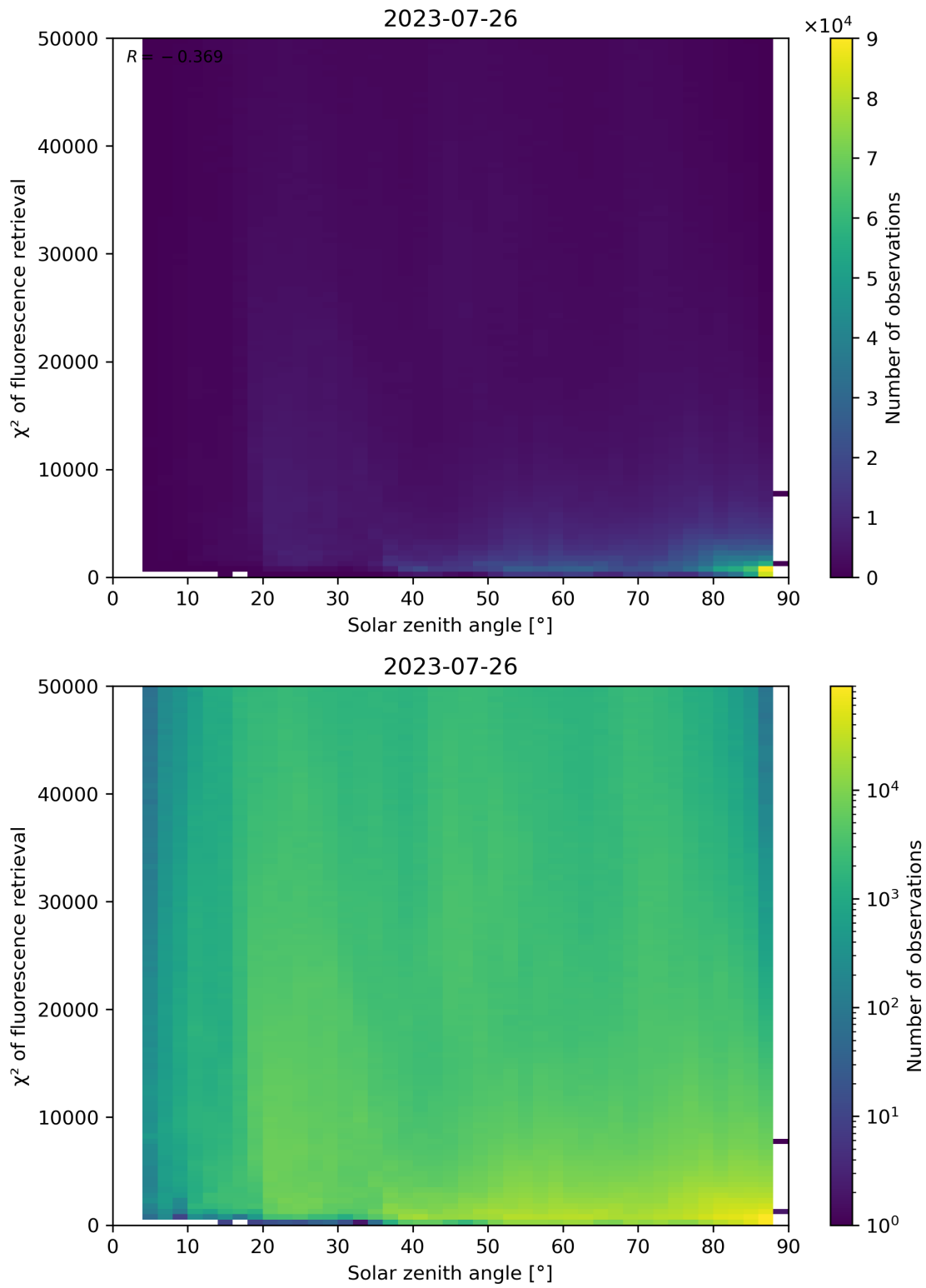
Figure 120: Scatter density plot of “Solar zenith angle” against “ \chi^2 of fluorescence retrieval” for 2023-07-25 to 2023-07-27.
