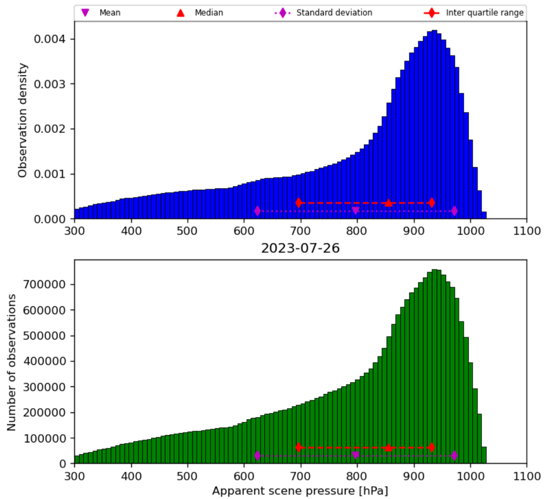
Figure 36: Histogram of “Apparent scene pressure” for 2023-07-25 to 2023-07-27
