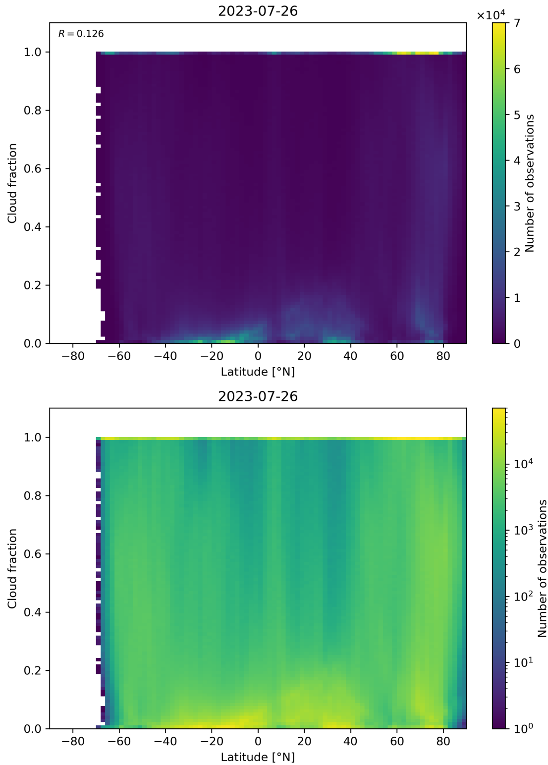
Figure 99: Scatter density plot of “Latitude” against “Cloud fraction” for 2023-07-25 to 2023-07-27.
