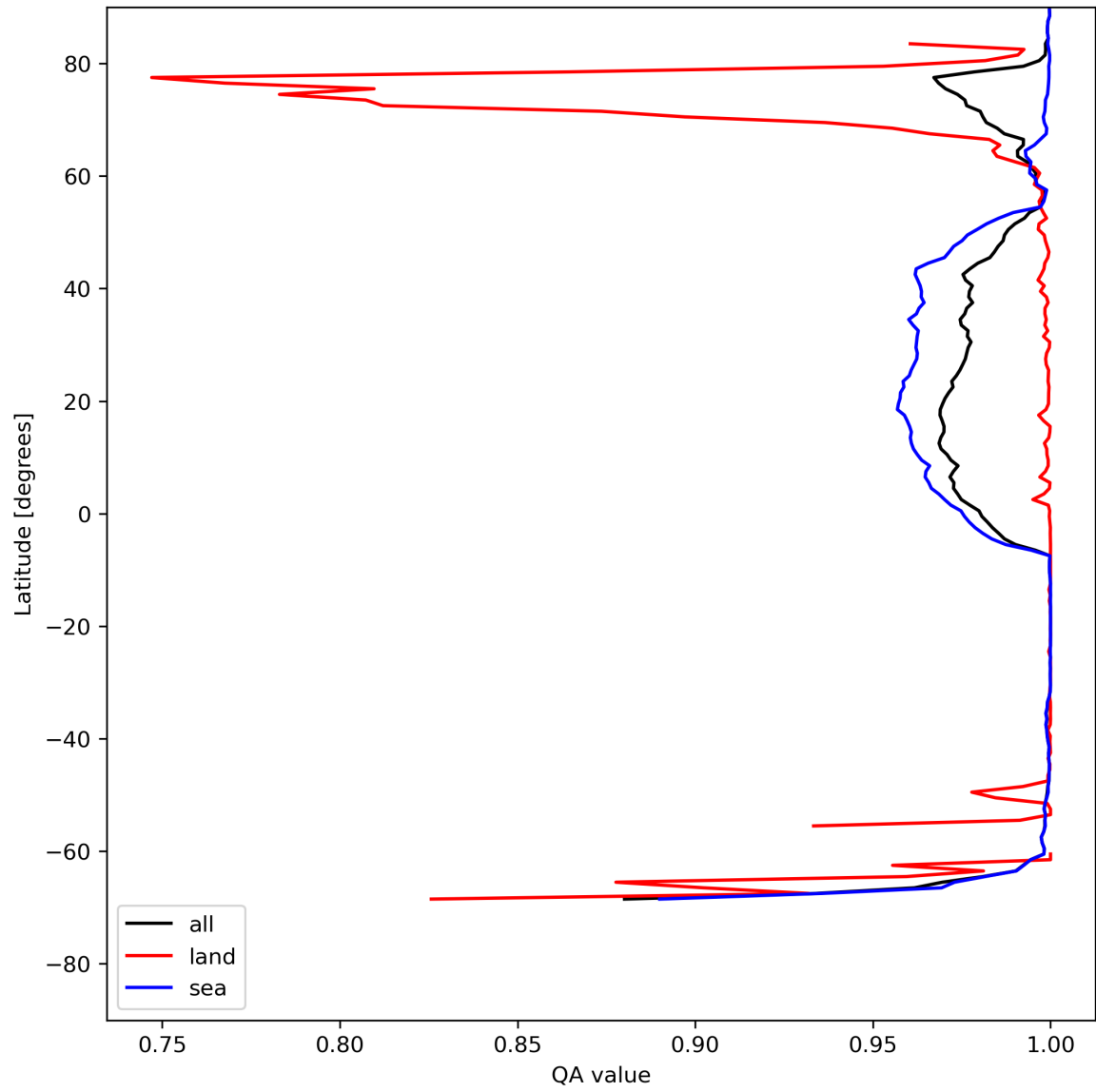
Figure 12: Zonal average of “QA value” for 2023-07-25 to 2023-07-27.
