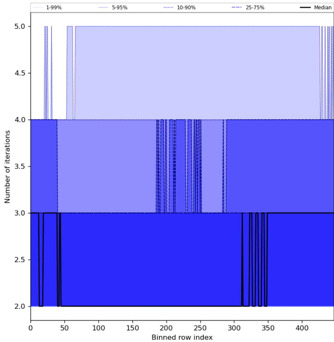
Figure 56: Along track statistics of “Number of iterations” for 2023-07-25 to 2023-07-27
