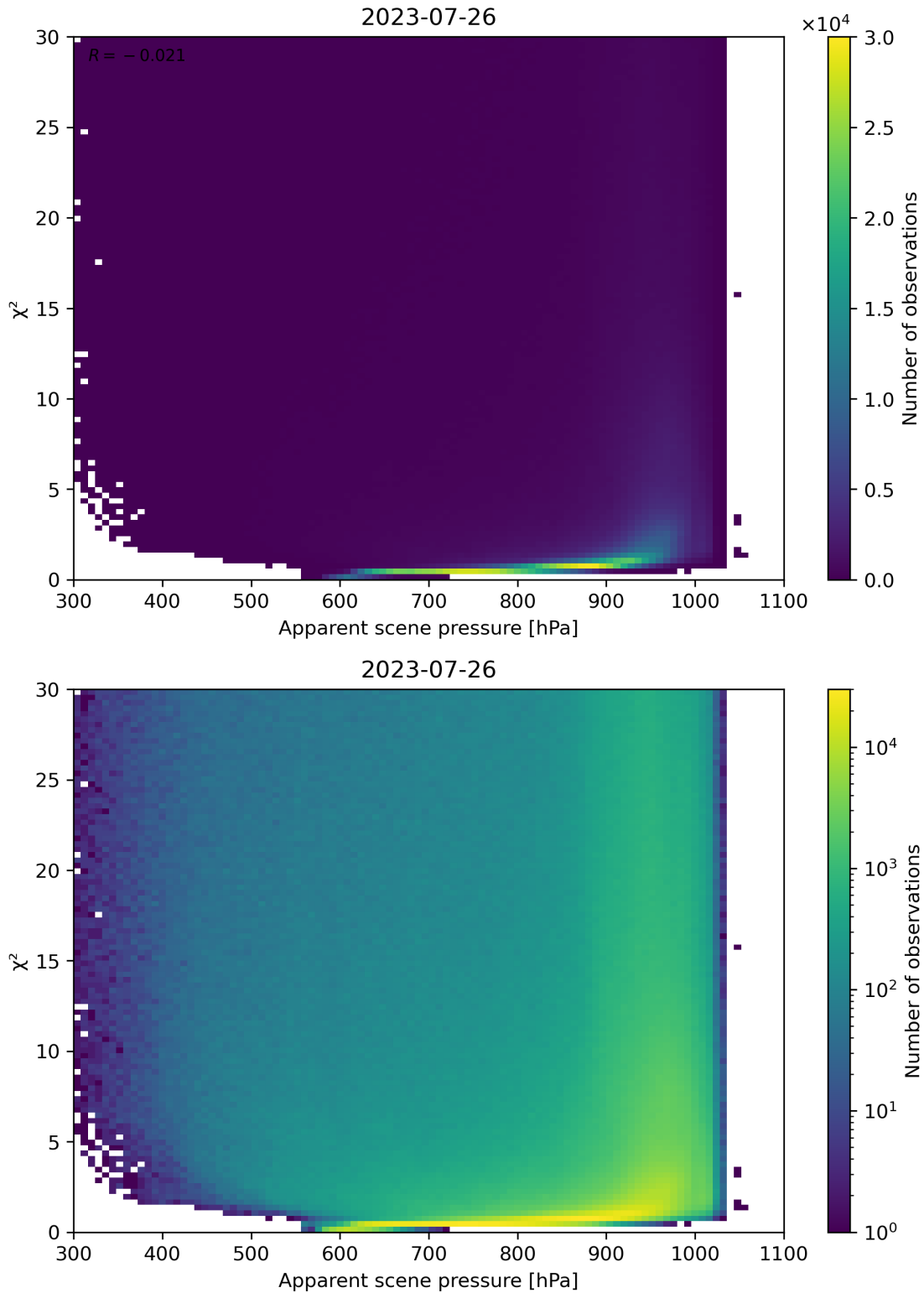
Figure 63: Scatter density plot of “Apparent scene pressure” against “ \chi^2 ” for 2023-07-25 to 2023-07-27.
