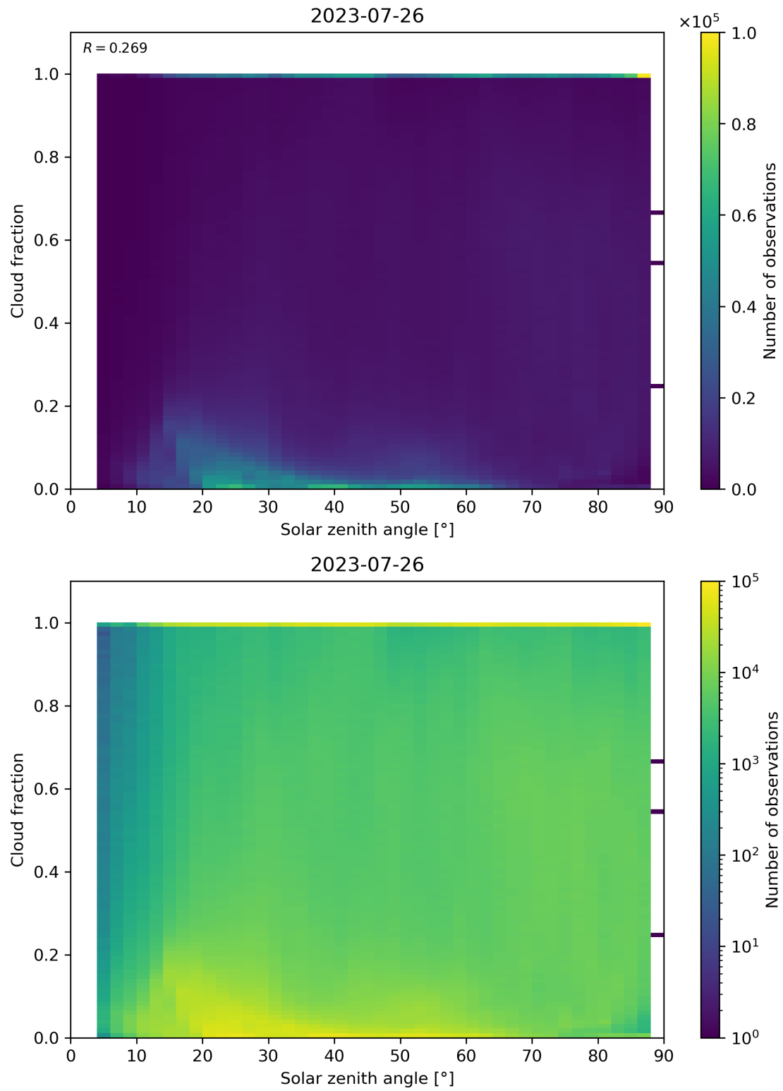
Figure 121: Scatter density plot of “Solar zenith angle” against “Cloud fraction” for 2023-07-25 to 2023-07-27.
