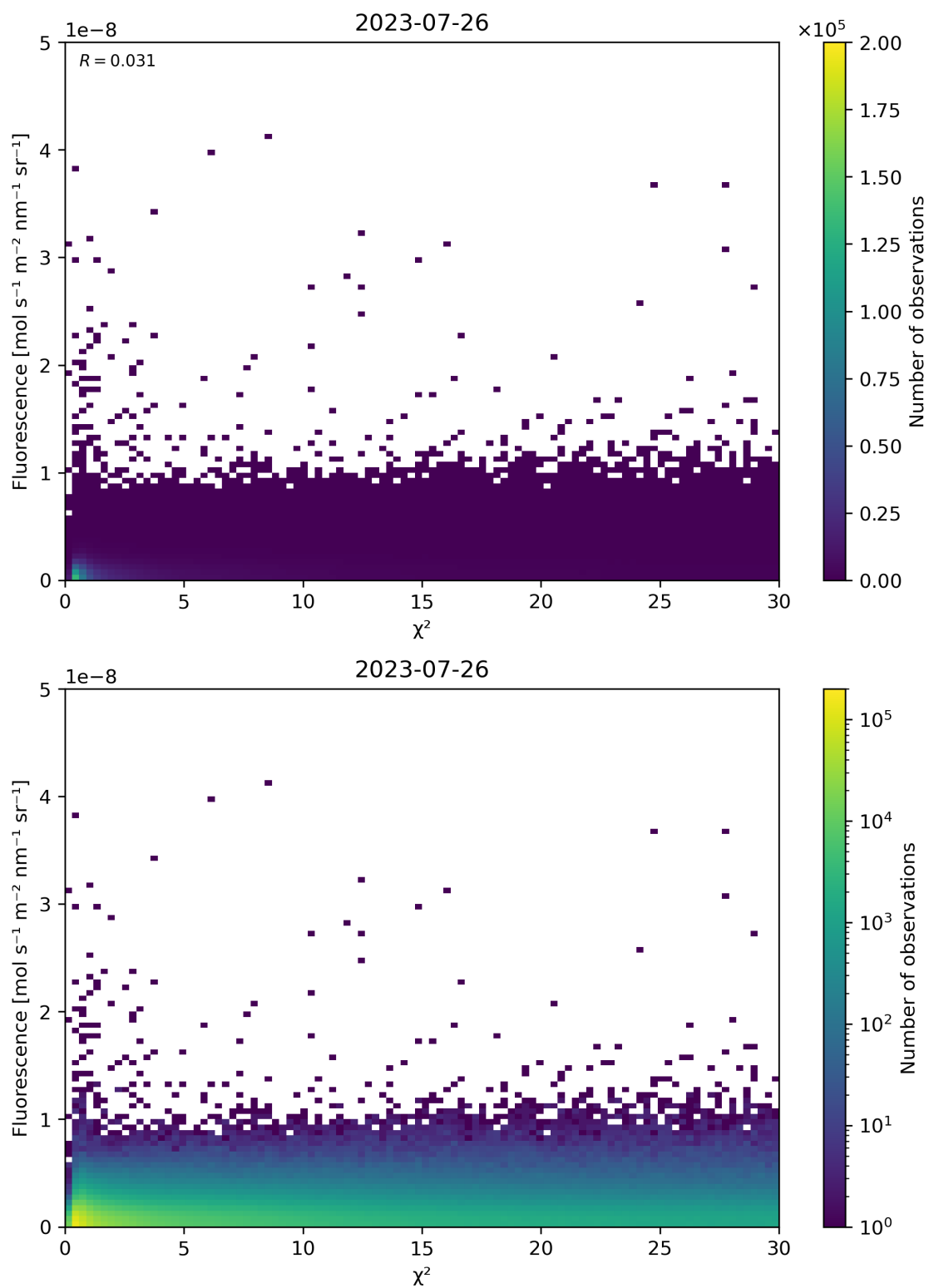
Figure 70: Scatter density plot of “ \chi^2 ” against “Fluorescence” for 2023-07-25 to 2023-07-27.
