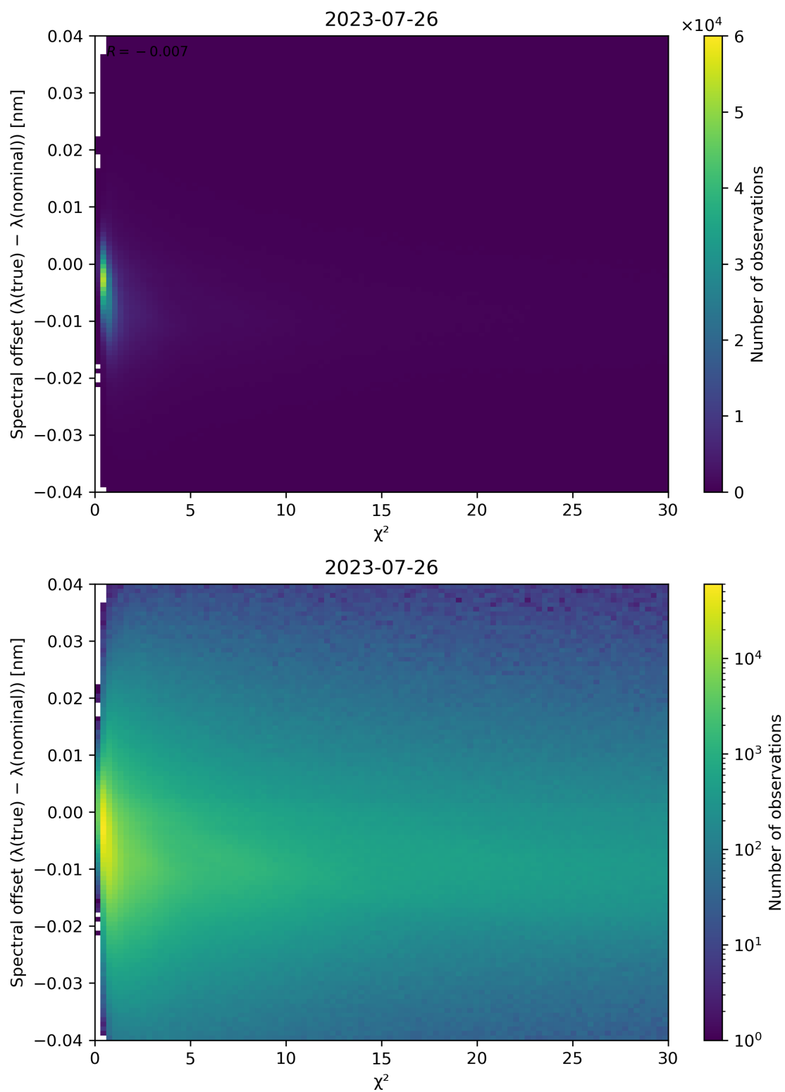
Figure 75: Scatter density plot of “ \chi^2 ” against “Spectral offset ( \lambda(\text{true}) - \lambda(\text{nominal}) )” for 2023-07-25 to 2023-07-27.
