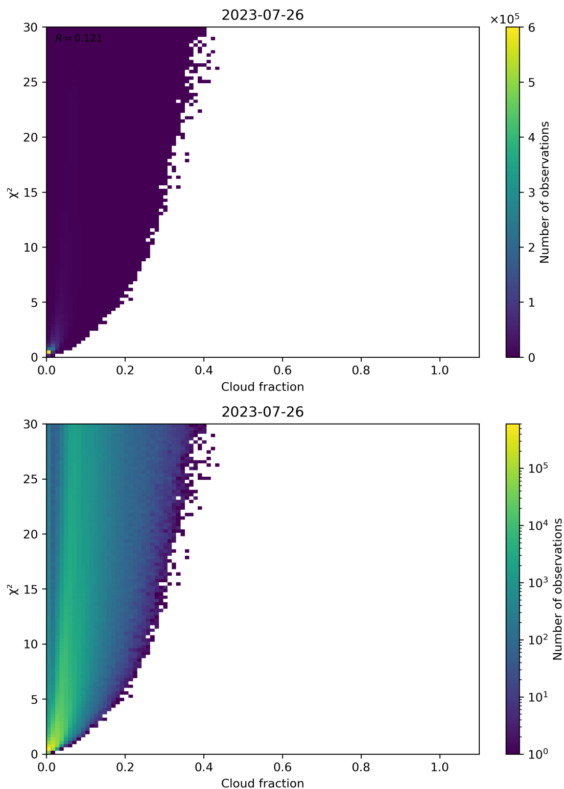
Figure 77: Scatter density plot of “Cloud fraction” against “ \chi^2 ” for 2023-07-25 to 2023-07-27.
