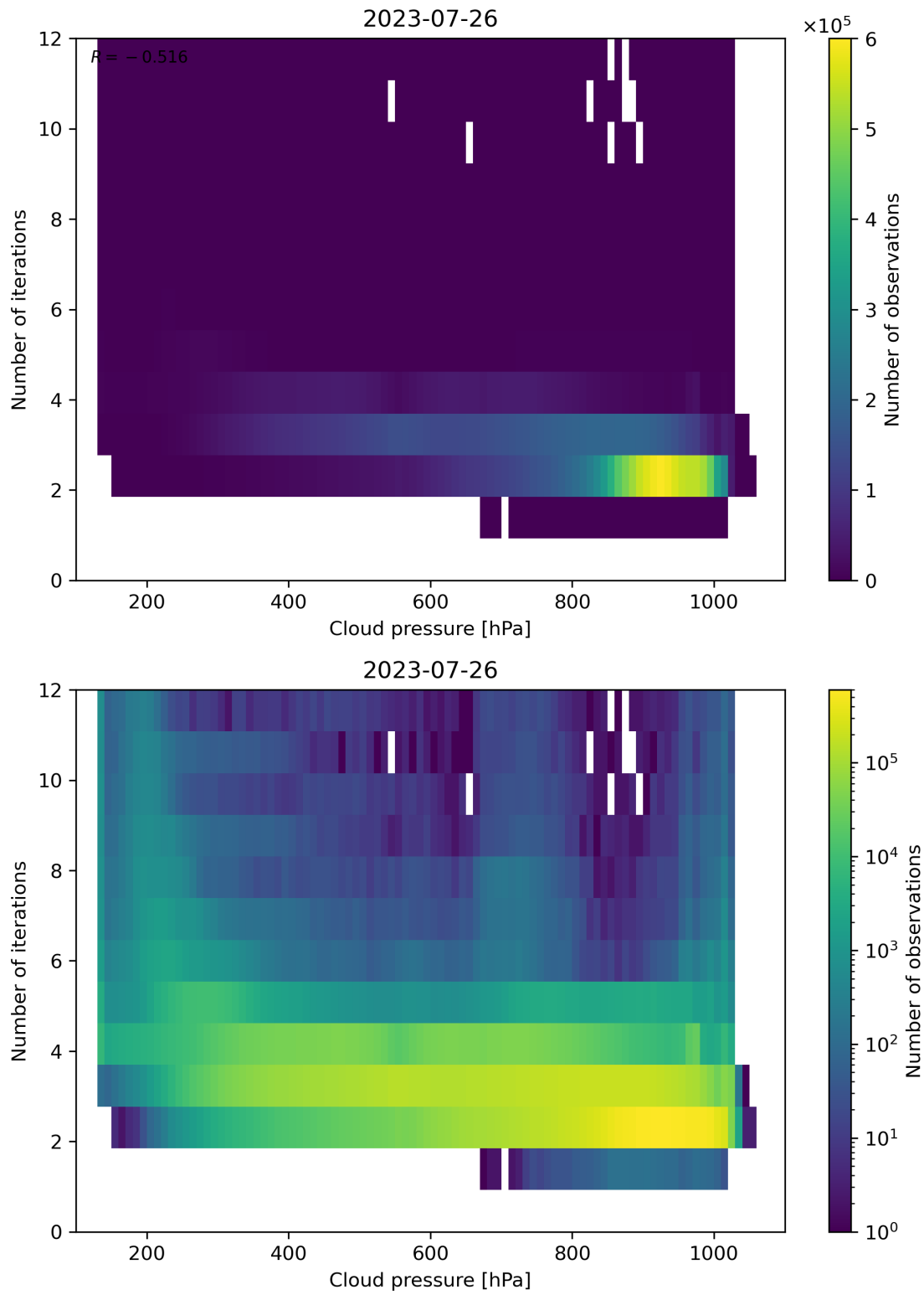
Figure 89: Scatter density plot of “Cloud pressure” against “Number of iterations” for 2023-07-25 to 2023-07-27.
