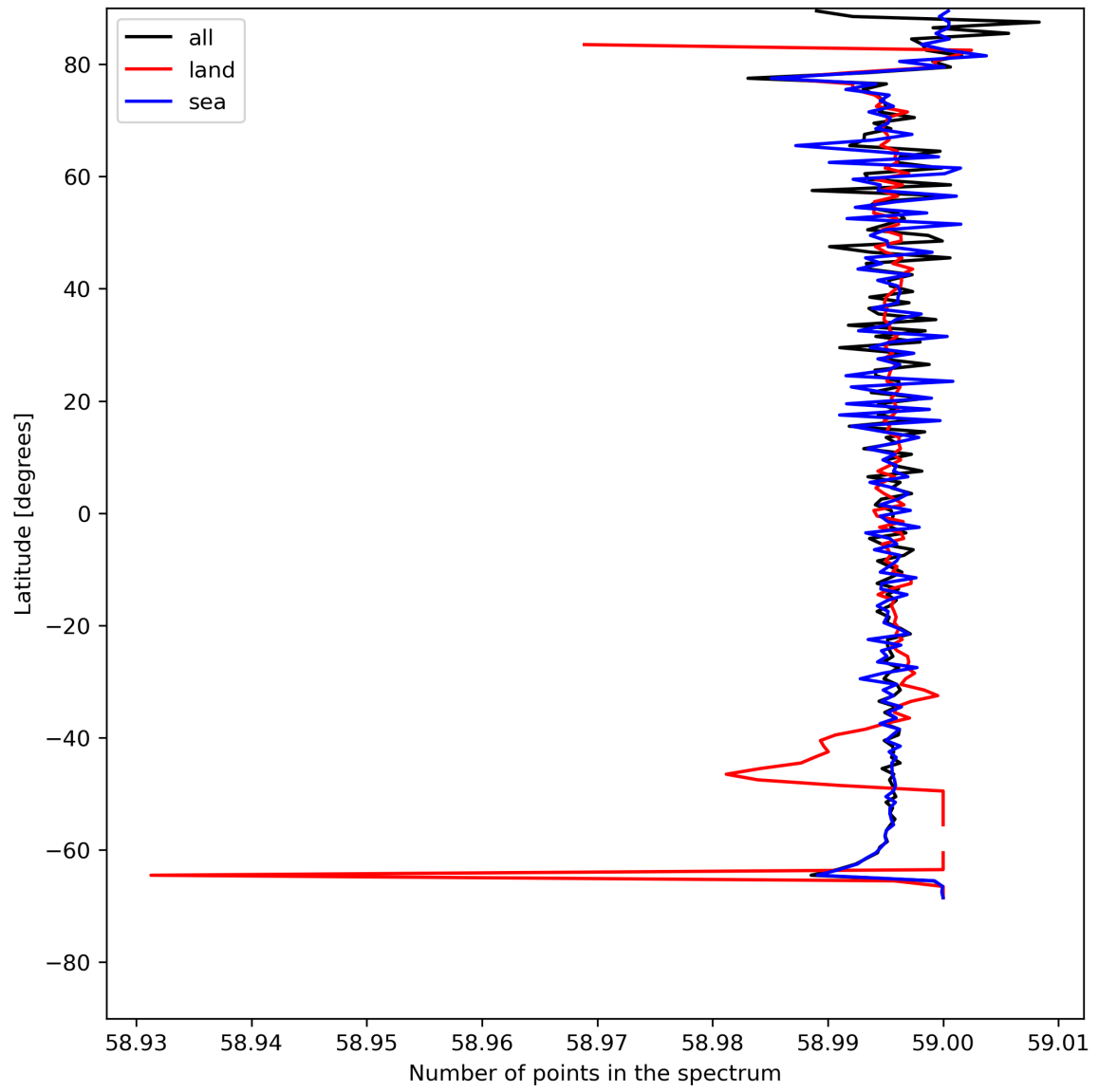
Figure 27: Zonal average of “Number of points in the spectrum” for 2023-07-25 to 2023-07-27.
