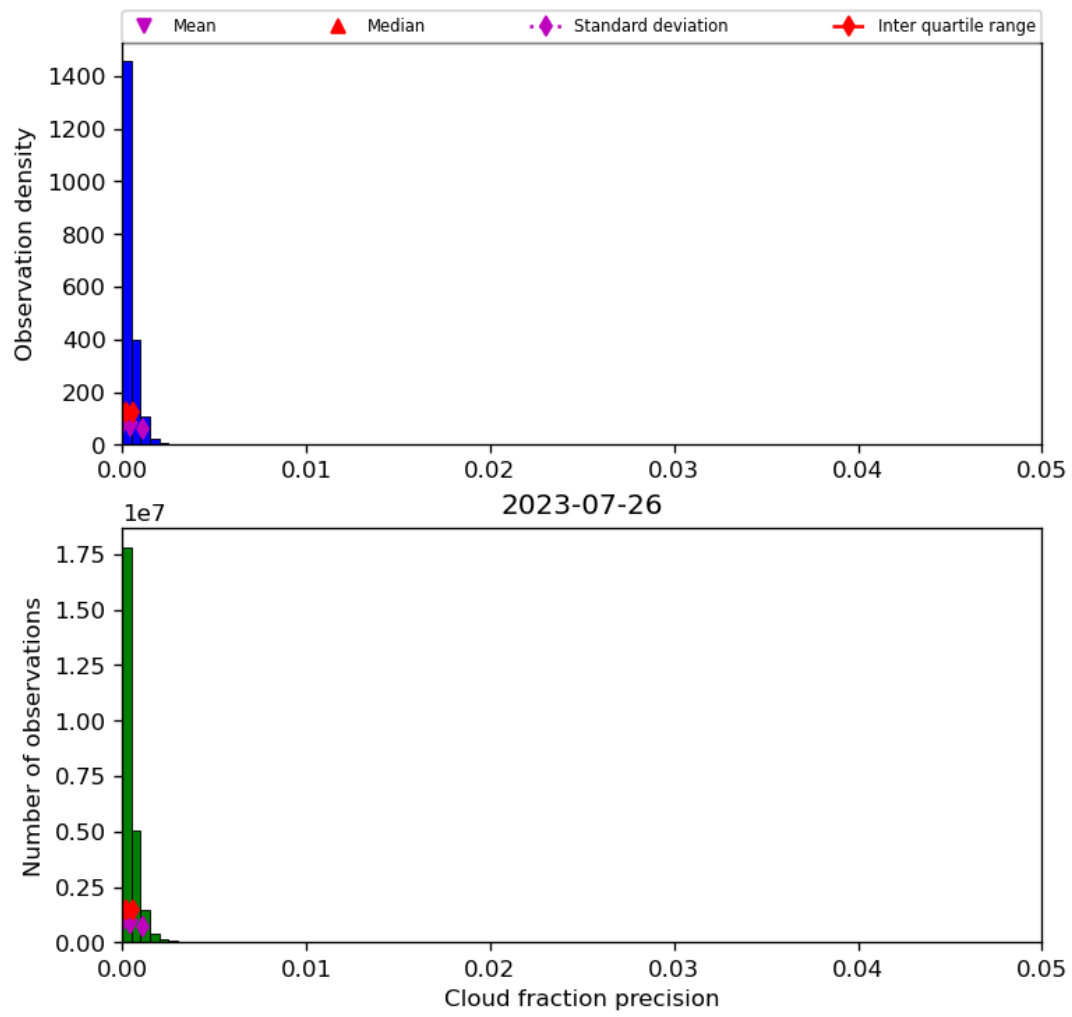
Figure 33: Histogram of “Cloud fraction precision” for 2023-07-25 to 2023-07-27
