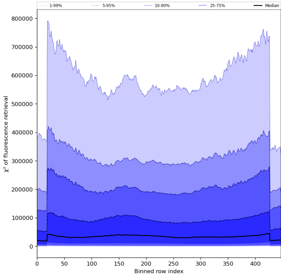
Figure 59: Along track statistics of “ \chi^2 of fluorescence retrieval” for 2023-07-25 to 2023-07-27
