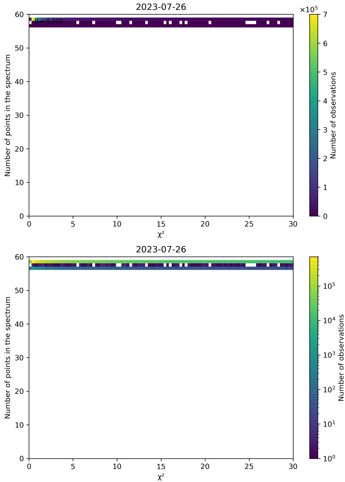
Figure 74: Scatter density plot of “ \chi^2 ” against “Number of points in the spectrum” for 2023-07-25 to 2023-07-27.
