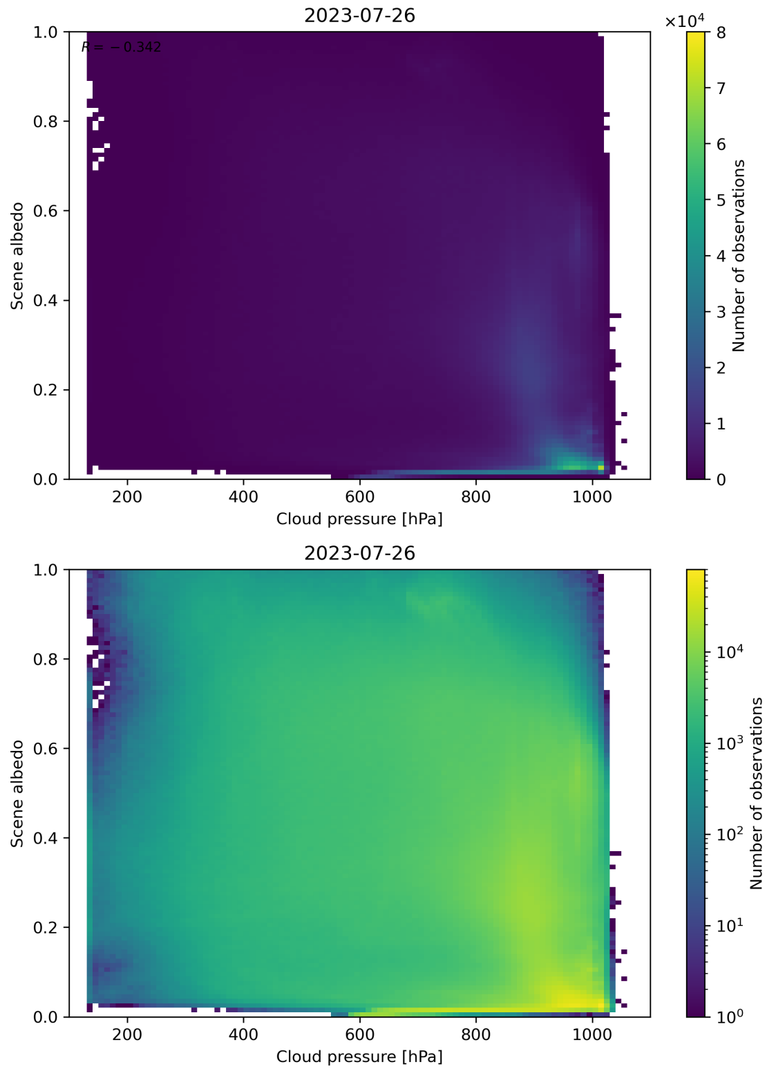
Figure 91: Scatter density plot of “Cloud pressure” against “Scene albedo” for 2023-07-25 to 2023-07-27.
