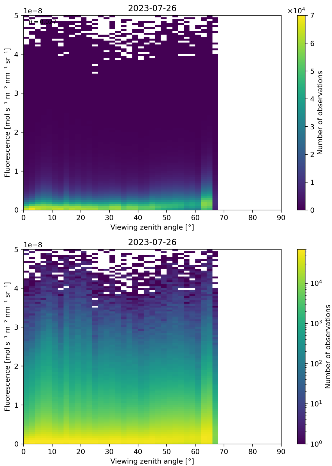
Figure 134: Scatter density plot of “Viewing zenith angle” against “Fluorescence” for 2023-07-25 to 2023-07-27.
