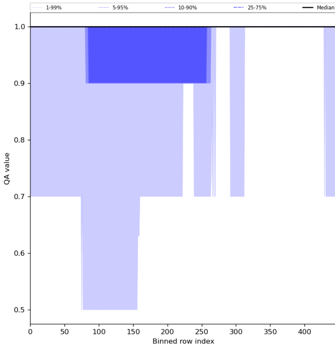
Figure 46: Along track statistics of “QA value” for 2023-07-25 to 2023-07-27
