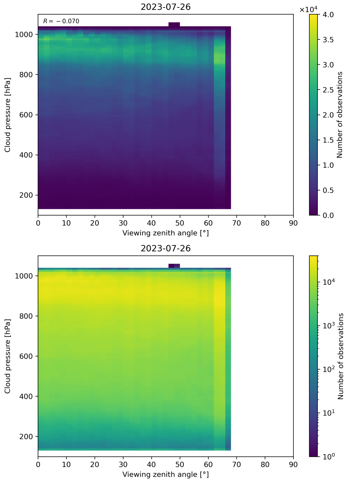
Figure 133: Scatter density plot of “Viewing zenith angle” against “Cloud pressure” for 2023-07-25 to 2023-07-27.
