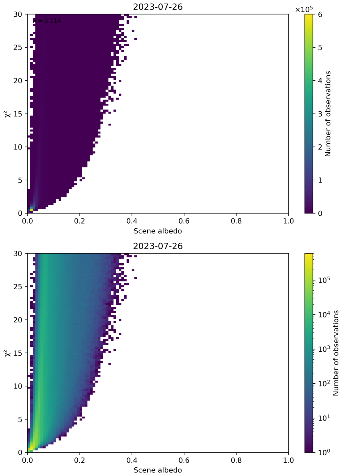
Figure 112: Scatter density plot of “Scene albedo” against “ \chi^2 ” for 2023-07-25 to 2023-07-27.
