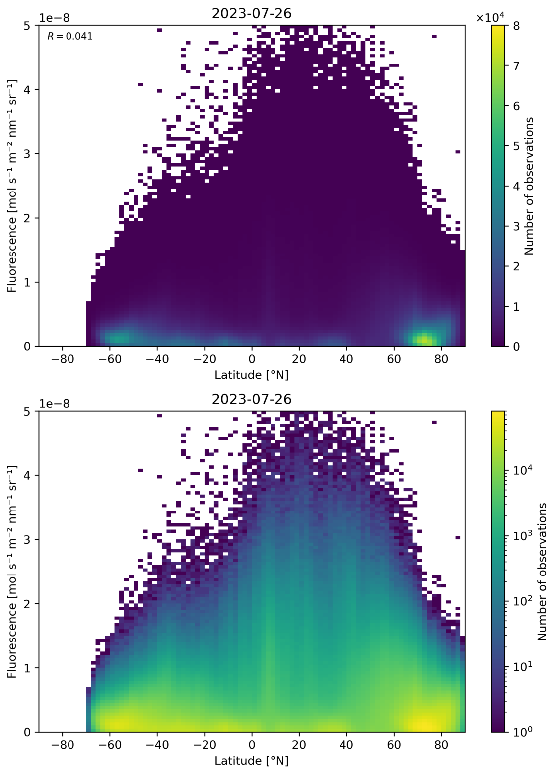
Figure 101: Scatter density plot of “Latitude” against “Fluorescence” for 2023-07-25 to 2023-07-27.
