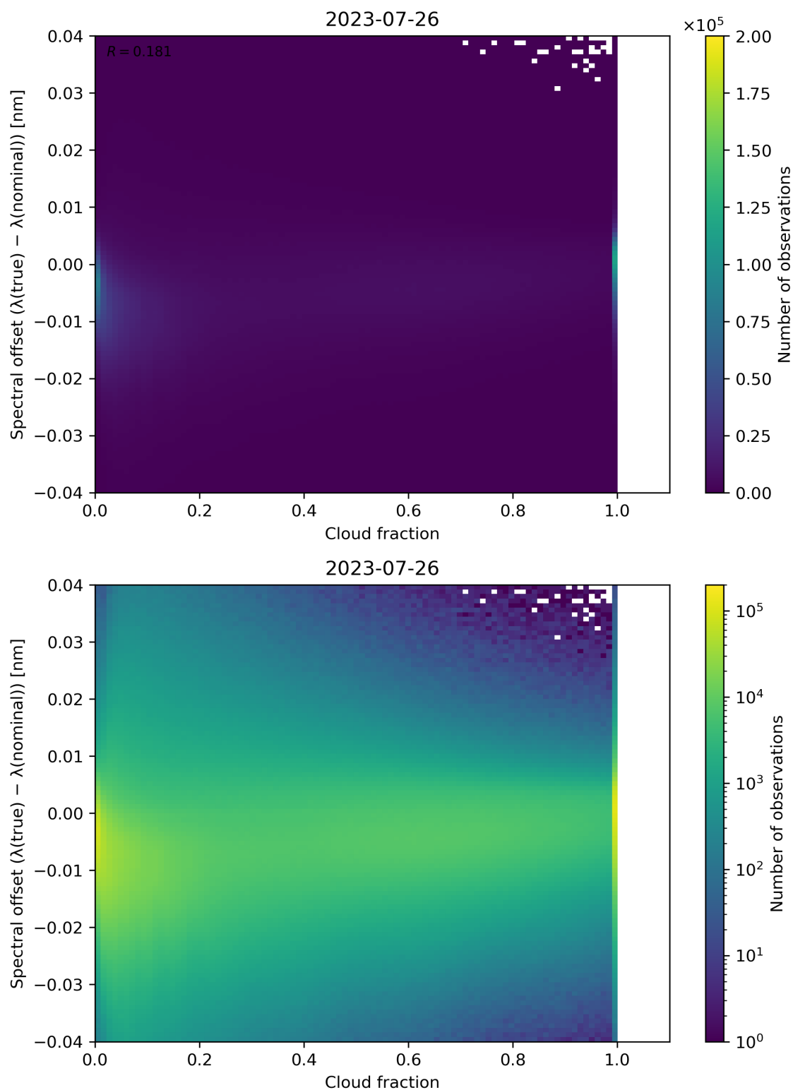
Figure 83: Scatter density plot of “Cloud fraction” against “Spectral offset ( \lambda(\text{true}) - \lambda(\text{nominal}) )” for 2023-07-25 to 2023-07-27.
