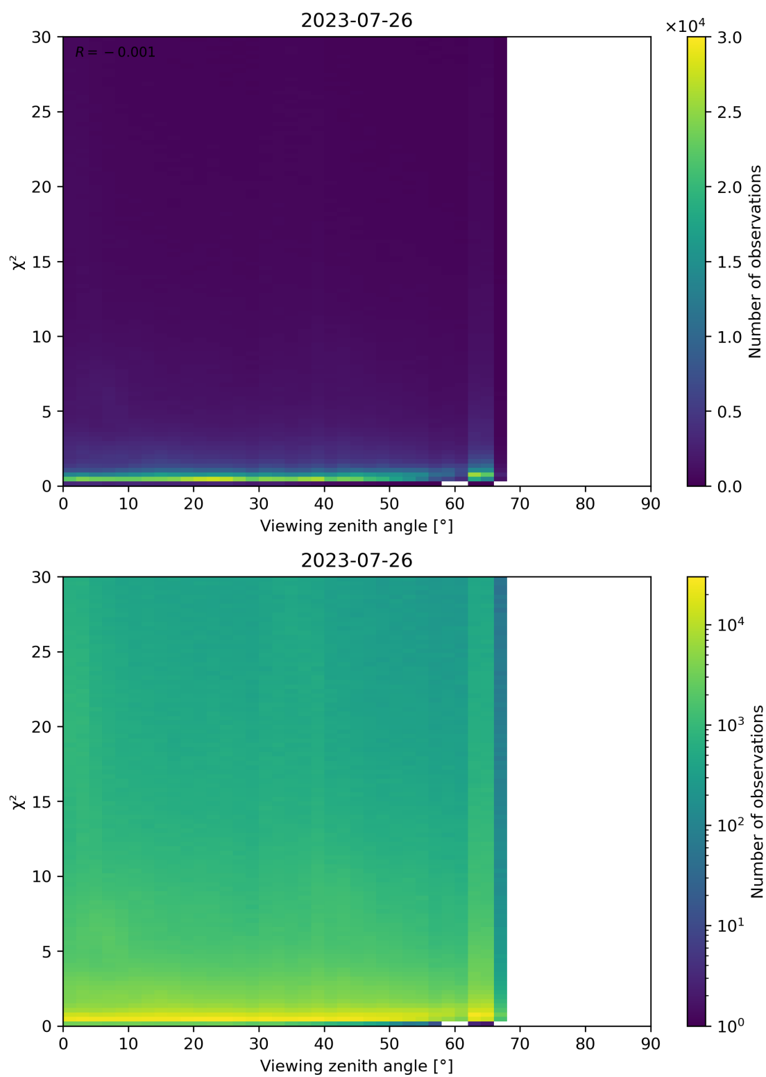
Figure 130: Scatter density plot of “Viewing zenith angle” against “ \chi^2 ” for 2023-07-25 to 2023-07-27.
