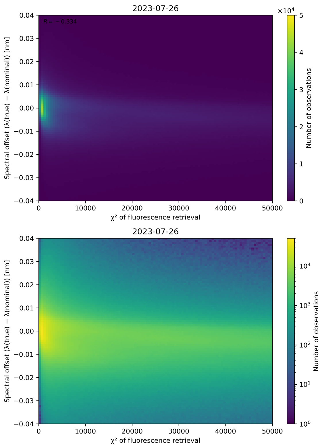
Figure 72: Scatter density plot of " \chi^2 of fluorescence retrieval" against "Spectral offset ( \lambda(\text{true}) - \lambda(\text{nominal})) " for 2023-07-25 to 2023-07-27.
