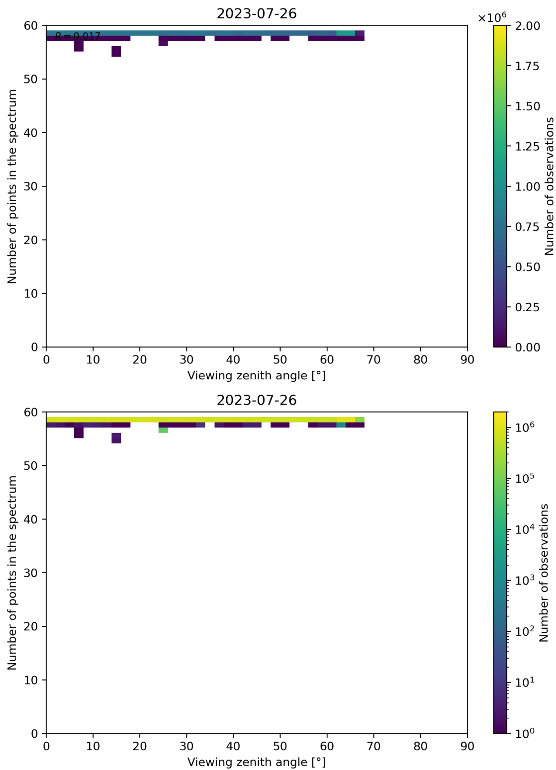
Figure 137: Scatter density plot of “Viewing zenith angle” against “Number of points in the spectrum” for 2023-07-25 to 2023-07-27.
