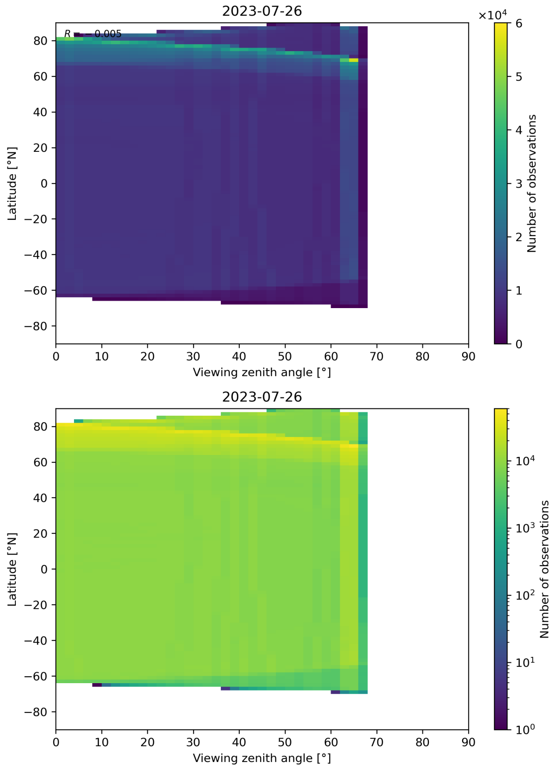
Figure 135: Scatter density plot of “Viewing zenith angle” against “Latitude” for 2023-07-25 to 2023-07-27.
