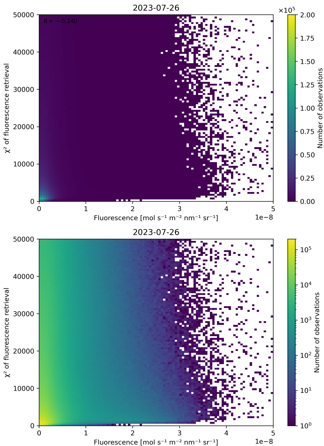
Figure 93: Scatter density plot of “Fluorescence” against “ \chi^2 of fluorescence retrieval” for 2023-07-25 to 2023-07-27.
