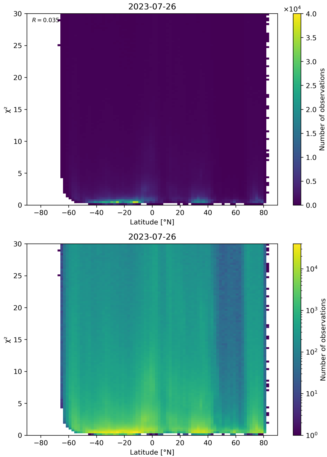
Figure 97: Scatter density plot of “Latitude” against “ \chi^2 ” for 2023-07-25 to 2023-07-27.
