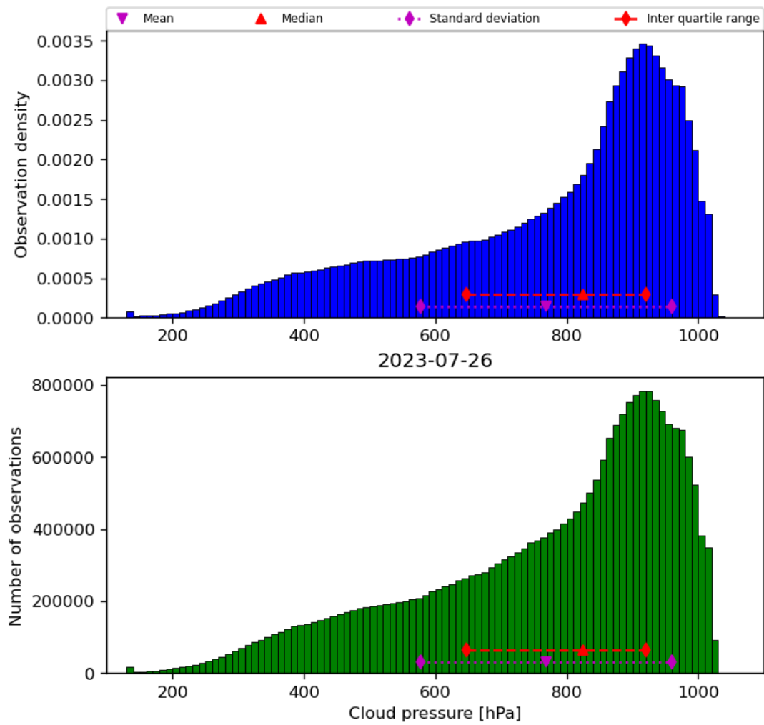
Figure 30: Histogram of “Cloud pressure” for 2023-07-25 to 2023-07-27
