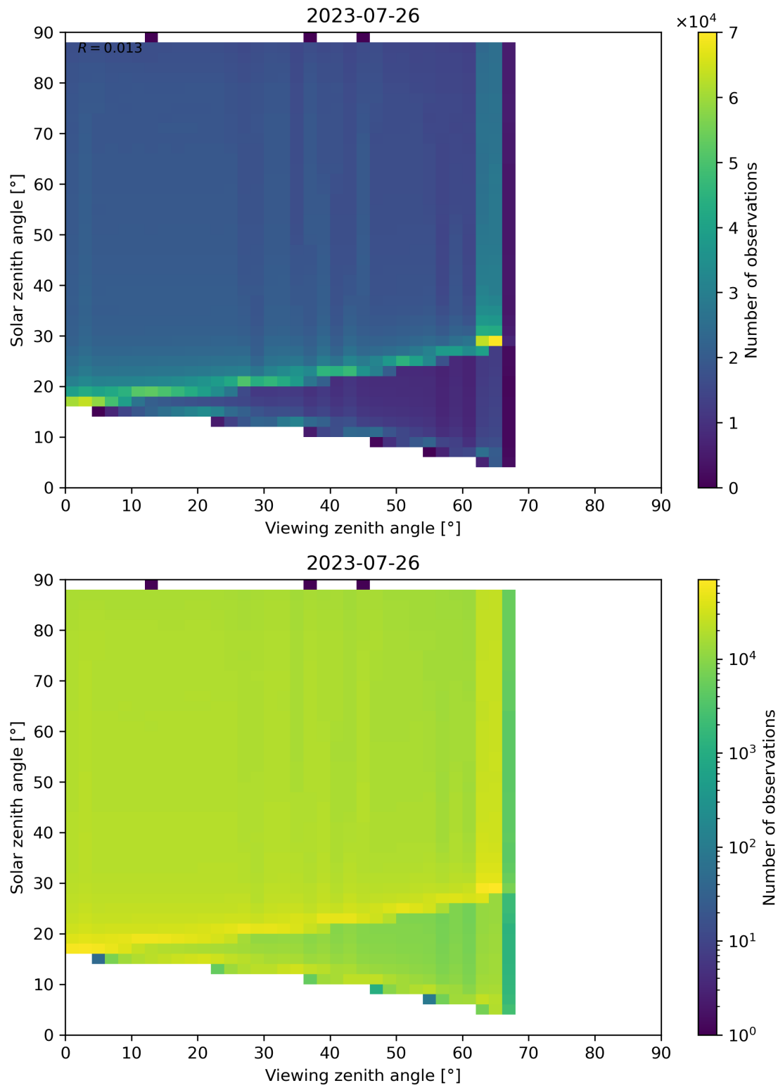
Figure 139: Scatter density plot of “Viewing zenith angle” against “Solar zenith angle” for 2023-07-25 to 2023-07-27.
