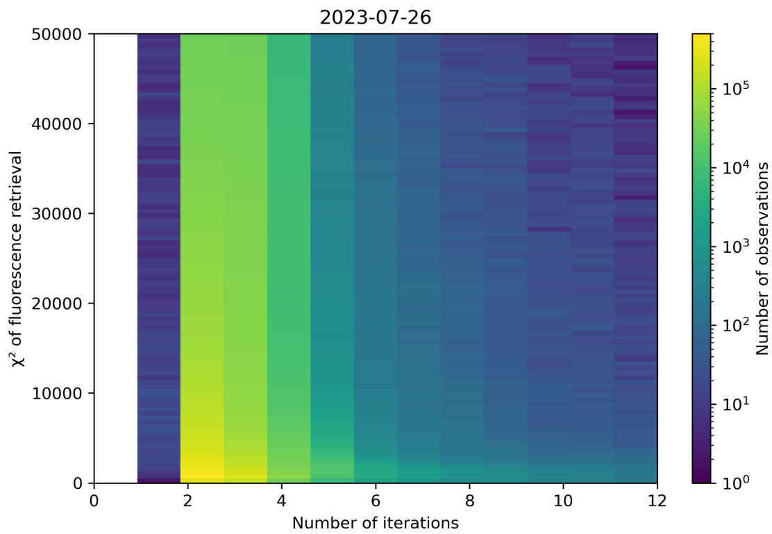
Figure 106: Scatter density plot of “Number of iterations” against “ \chi^2 of fluorescence retrieval” for 2023-07-25 to 2023-07-27.
