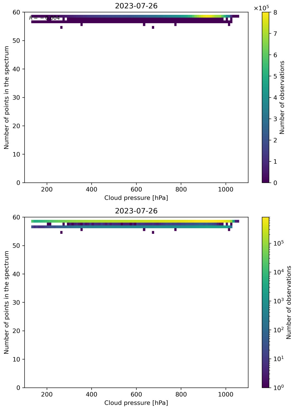
Figure 90: Scatter density plot of “Cloud pressure” against “Number of points in the spectrum” for 2023-07-25 to 2023-07-27.
