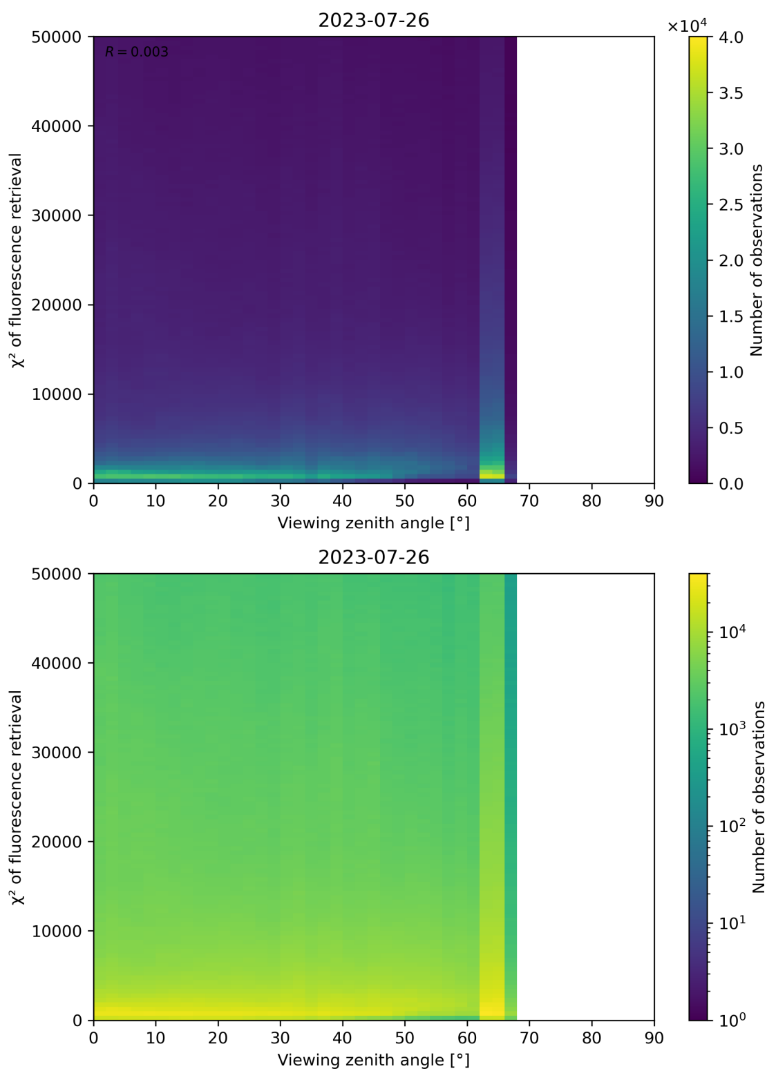
Figure 131: Scatter density plot of “Viewing zenith angle” against “ \chi^2 of fluorescence retrieval” for 2023-07-25 to 2023-07-27.
