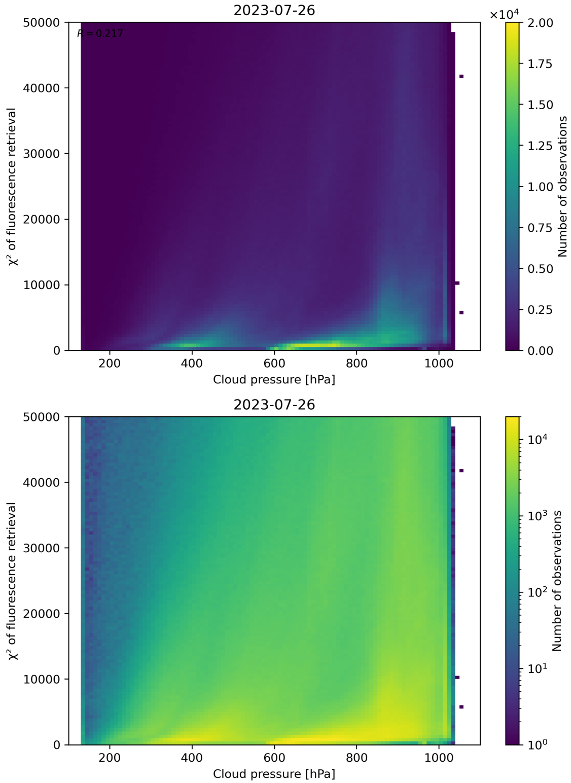
Figure 86: Scatter density plot of “Cloud pressure” against “ \chi^2 of fluorescence retrieval” for 2023-07-25 to 2023-07-27.
