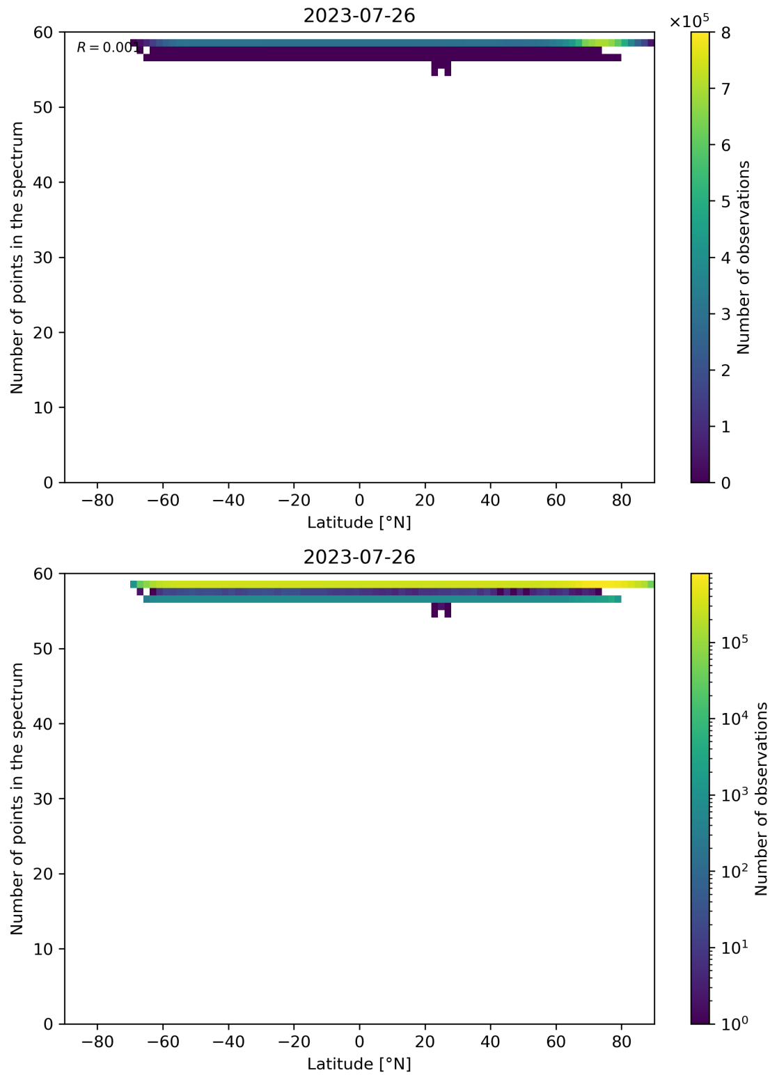
Figure 103: Scatter density plot of “Latitude” against “Number of points in the spectrum” for 2023-07-25 to 2023-07-27.
