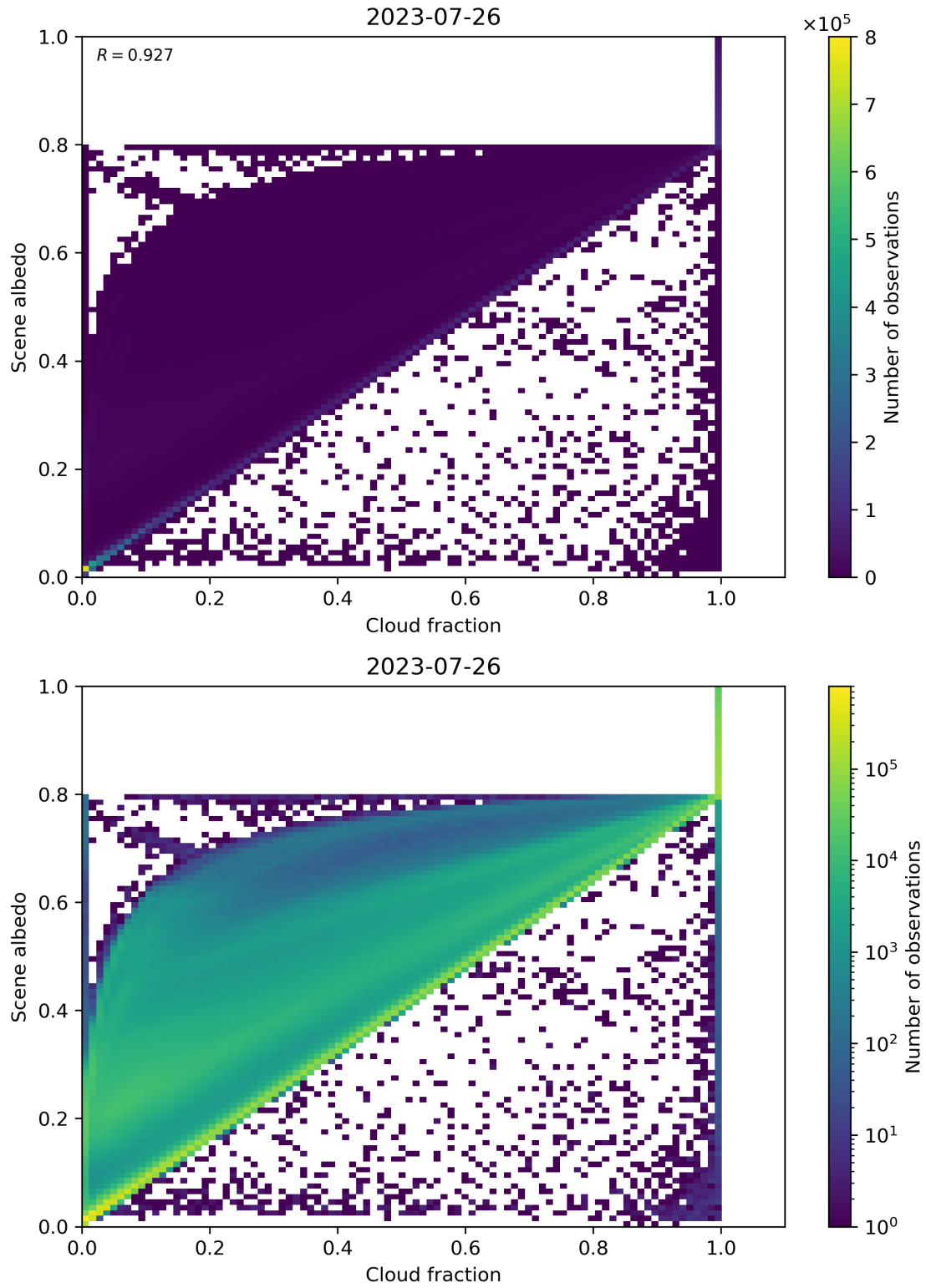
Figure 82: Scatter density plot of “Cloud fraction” against “Scene albedo” for 2023-07-25 to 2023-07-27.
