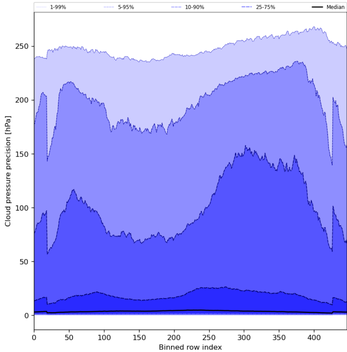
Figure 48: Along track statistics of “Cloud pressure precision” for 2023-07-25 to 2023-07-27
