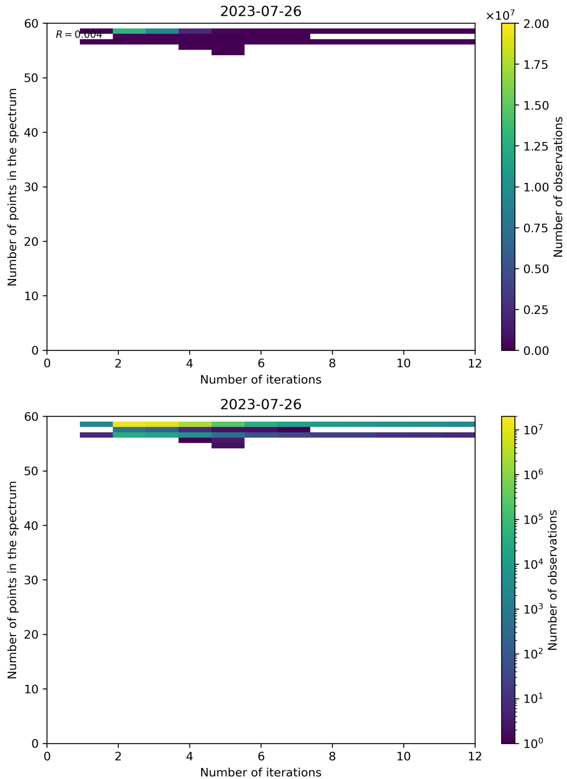
Figure 108: Scatter density plot of “Number of iterations” against “Number of points in the spectrum” for 2023-07-25 to 2023-07-27.
