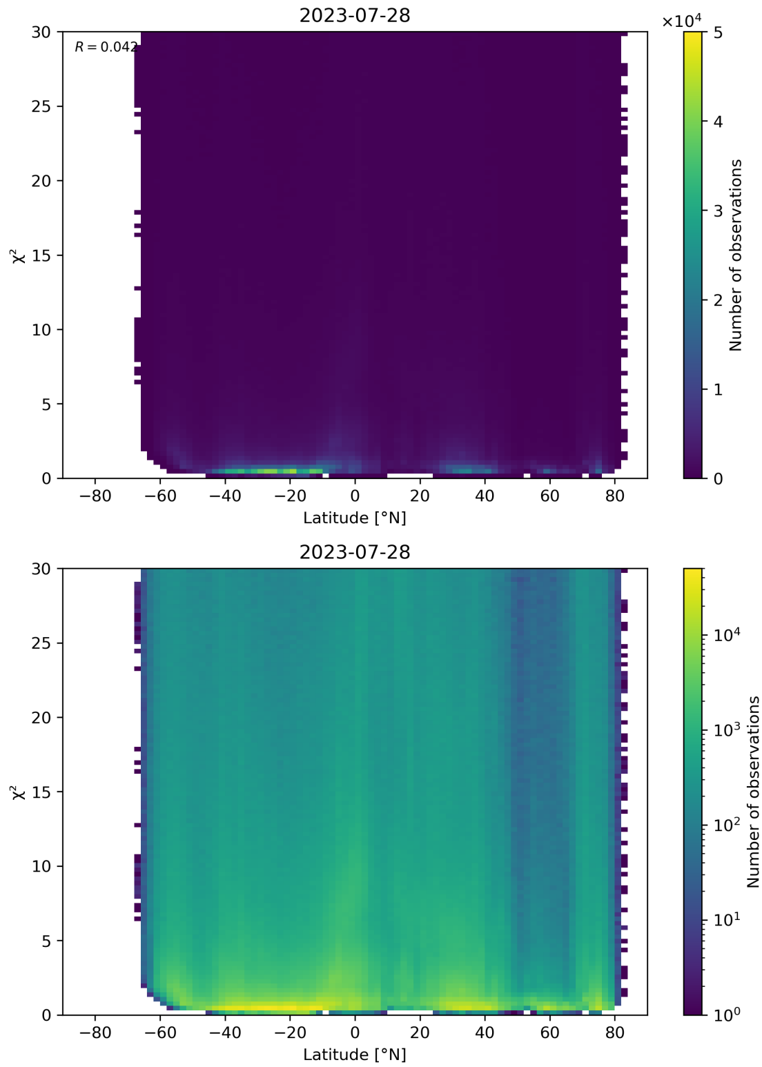
Figure 97: Scatter density plot of “Latitude” against “ \chi^2 ” for 2023-07-27 to 2023-07-29.
