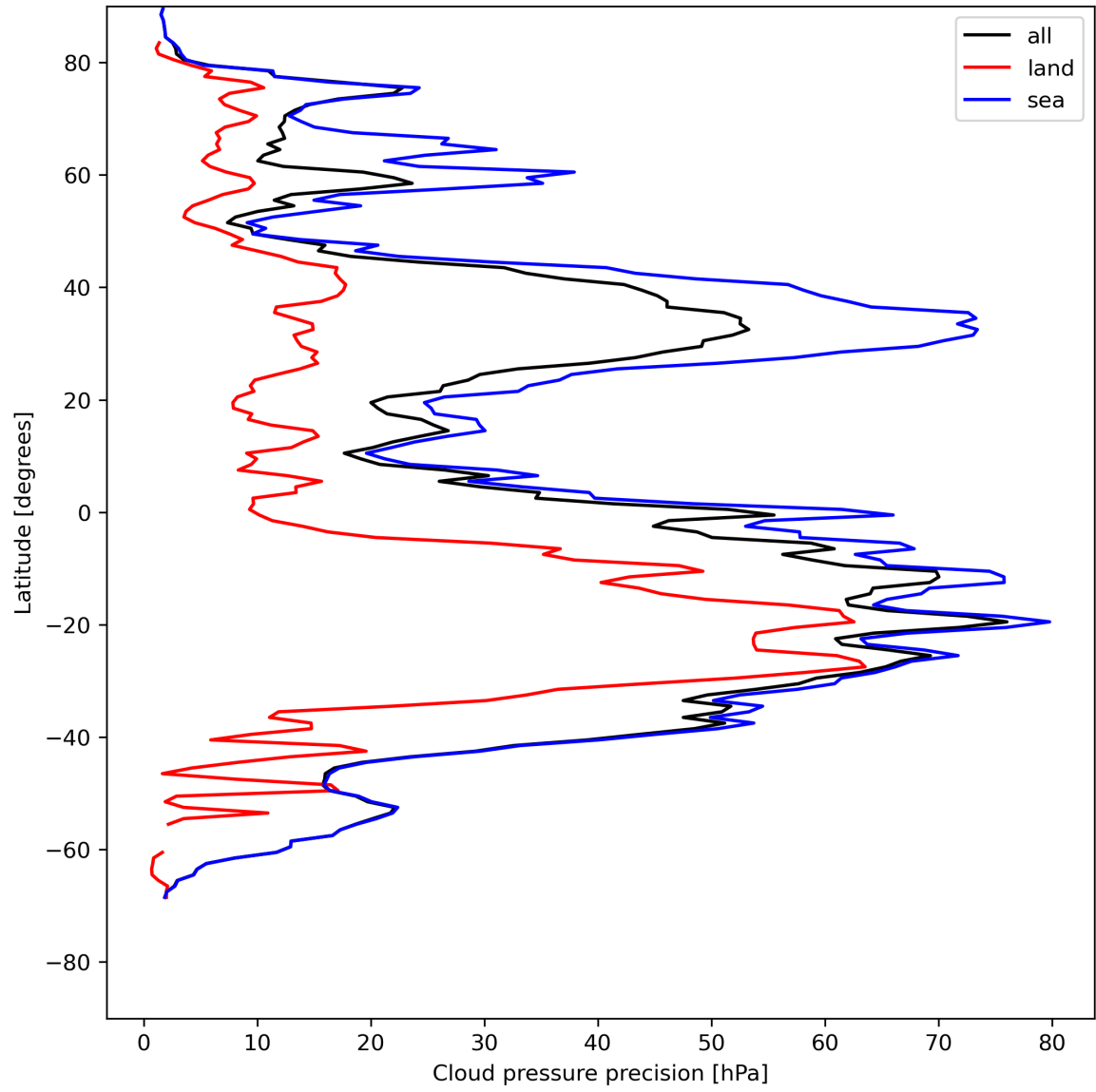
Figure 14: Zonal average of “Cloud pressure precision” for 2023-07-27 to 2023-07-29.
