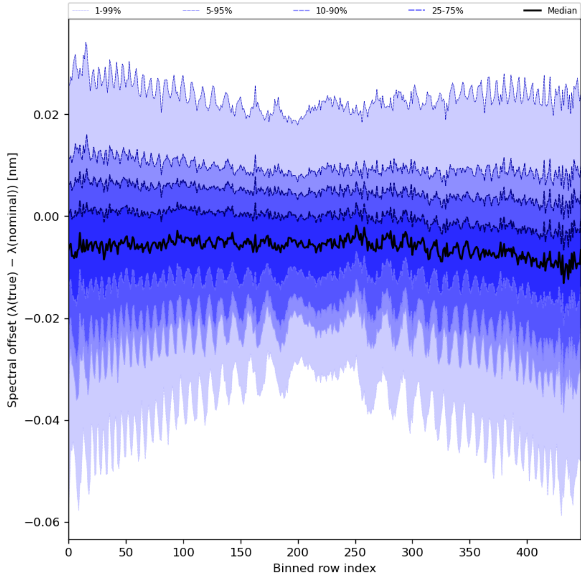
Figure 62: Along track statistics of “Spectral offset ( \lambda(\text{true}) - \lambda(\text{nominal}) )” for 2023-07-27 to 2023-07-29
