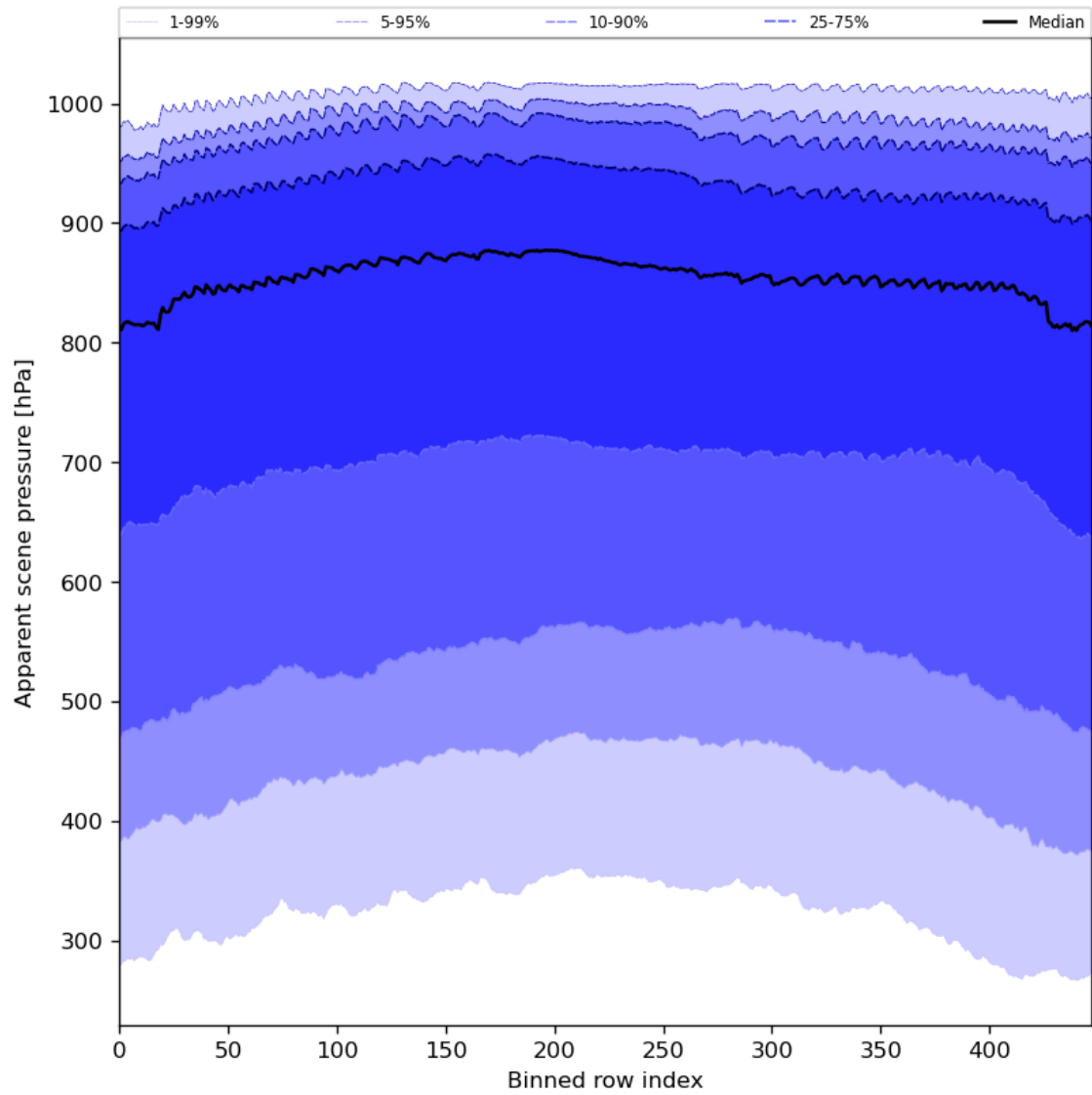
Figure 53: Along track statistics of “Apparent scene pressure” for 2023-07-27 to 2023-07-29
