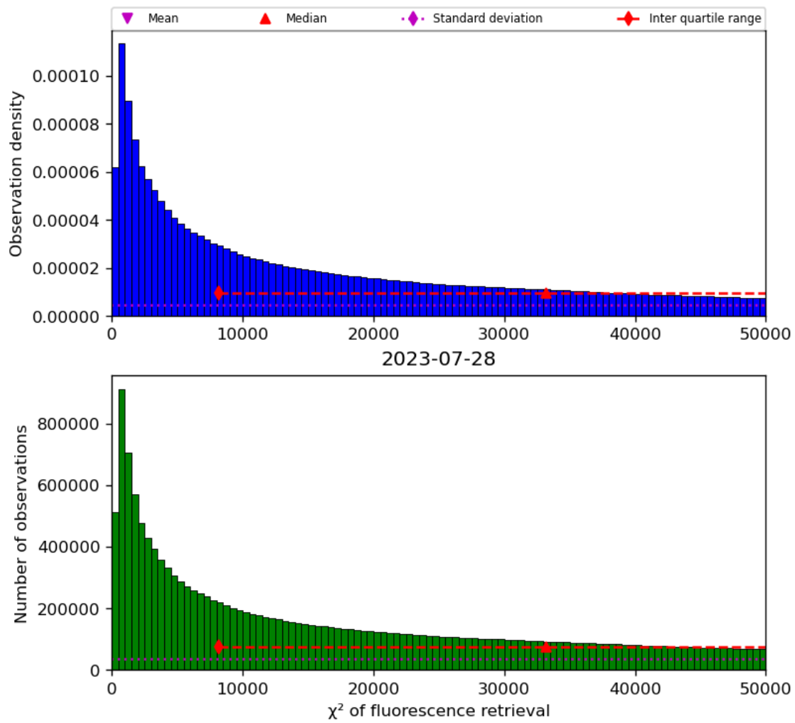
Figure 42: Histogram of “ \chi^2 of fluorescence retrieval” for 2023-07-27 to 2023-07-29
