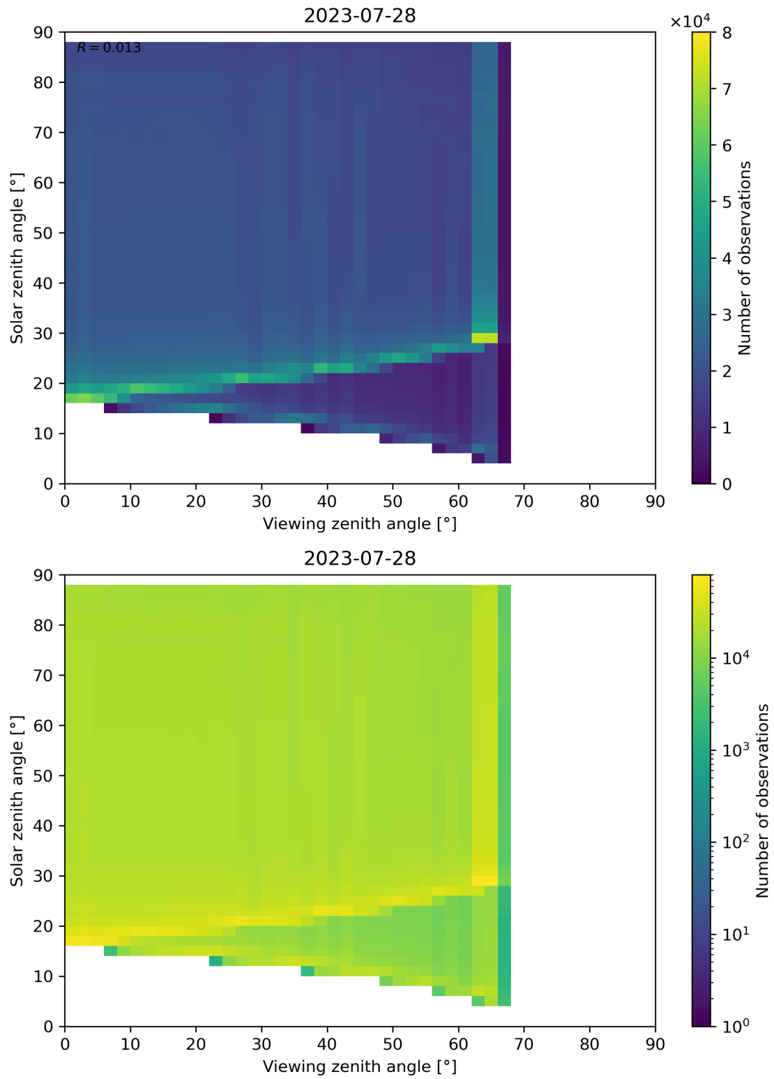
Figure 139: Scatter density plot of “Viewing zenith angle” against “Solar zenith angle” for 2023-07-27 to 2023-07-29.
