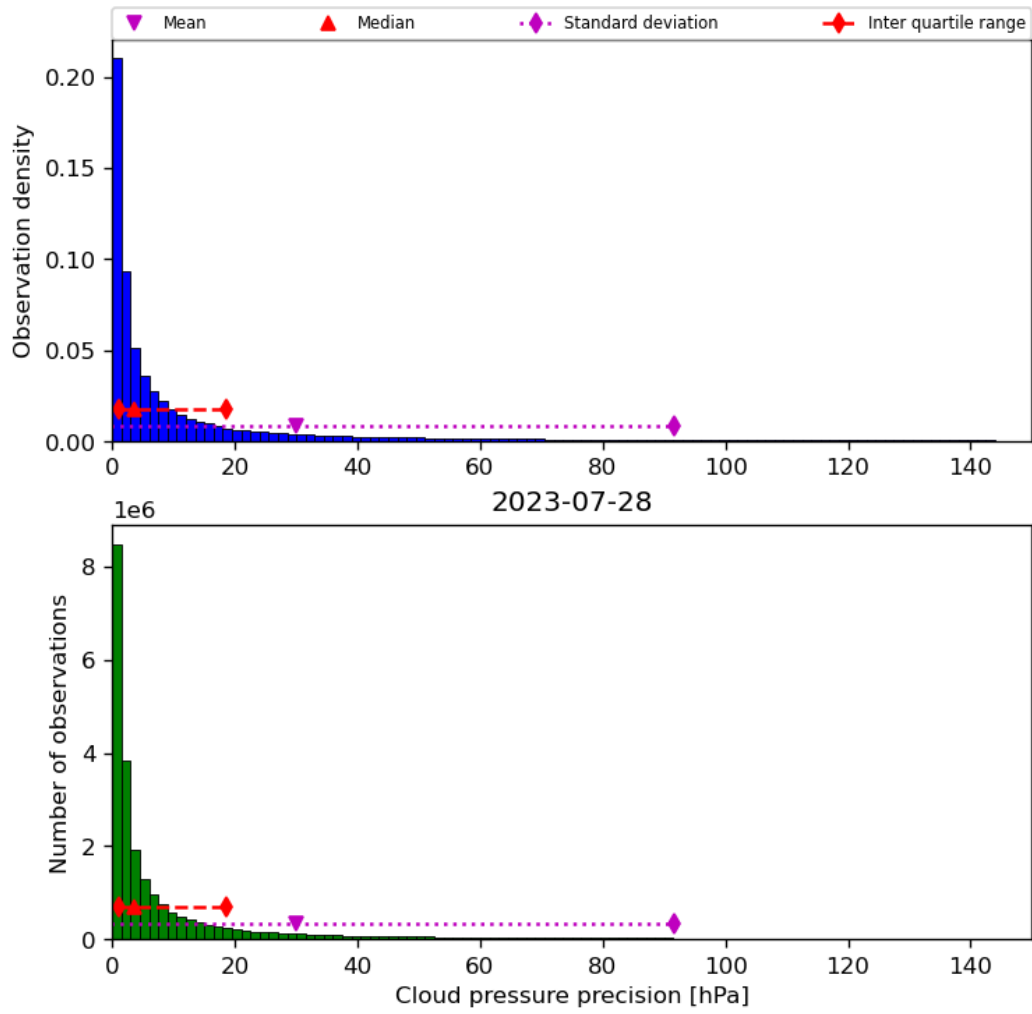
Figure 31: Histogram of “Cloud pressure precision” for 2023-07-27 to 2023-07-29
