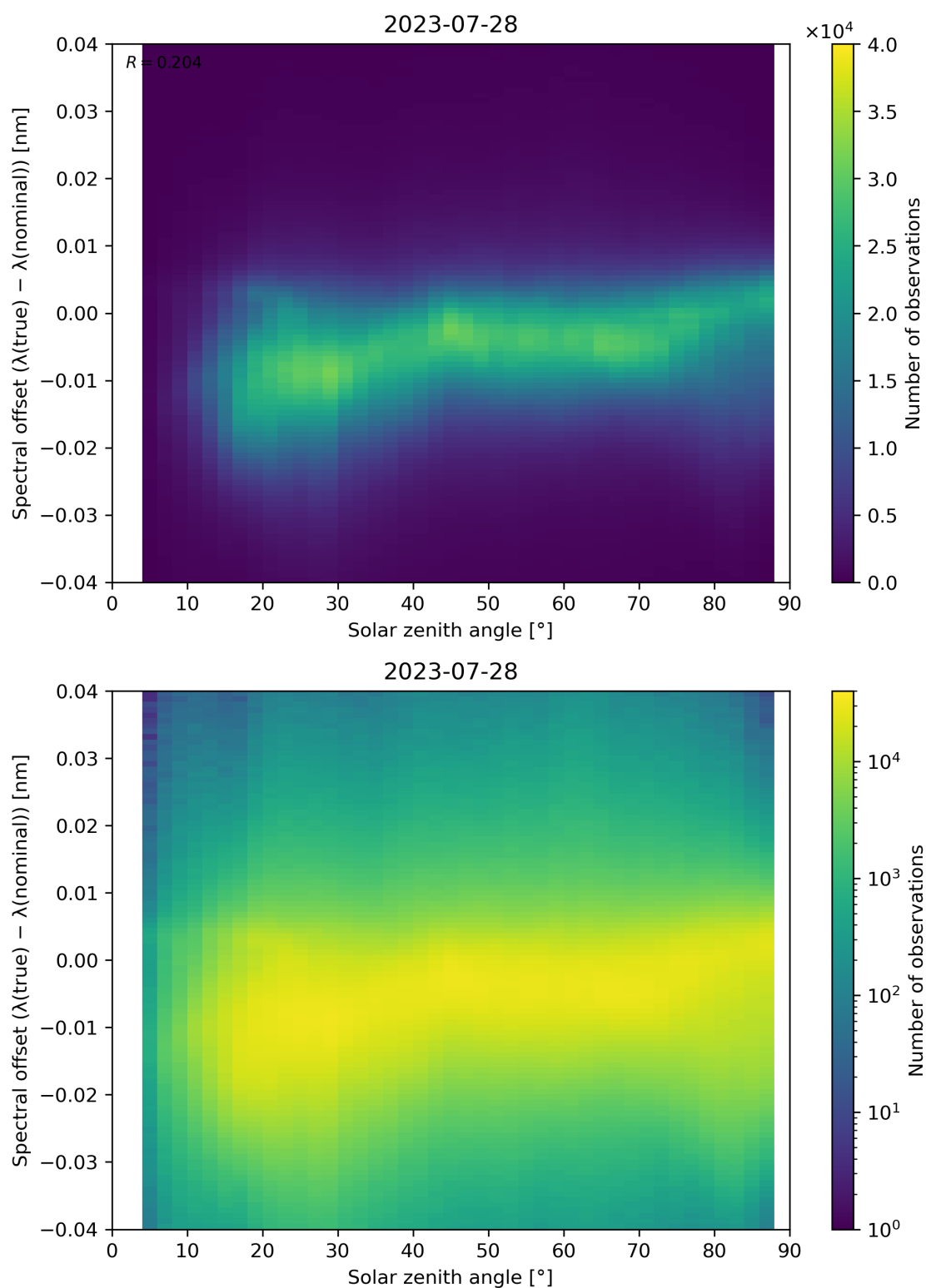
Figure 128: Scatter density plot of “Solar zenith angle” against “Spectral offset ( \lambda(\text{true}) - \lambda(\text{nominal}) )” for 2023-07-27 to 2023-07-29.
