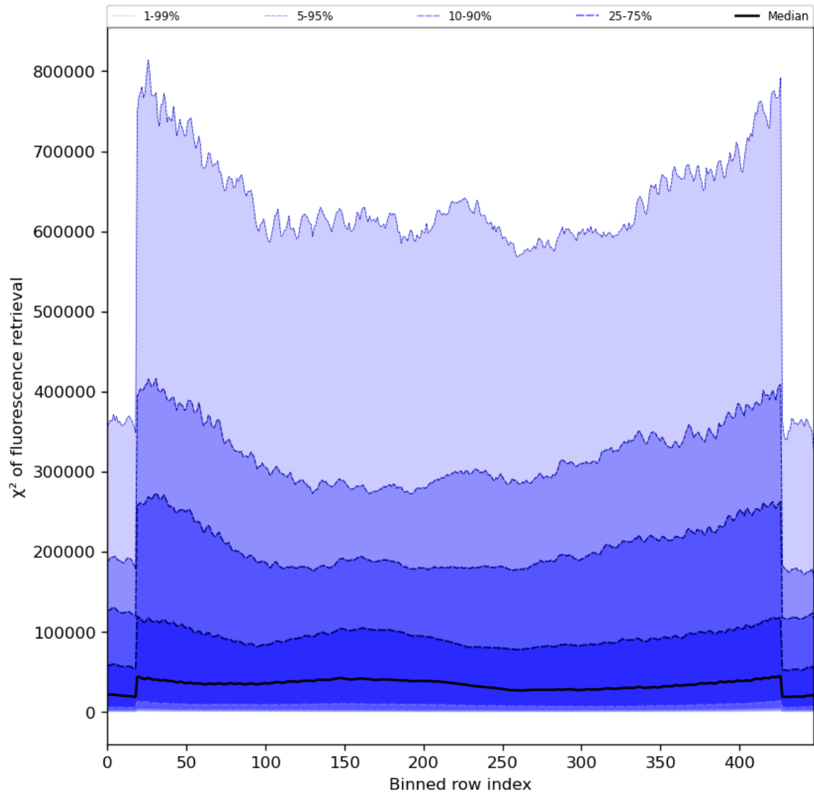
Figure 59: Along track statistics of “ \chi^2 of fluorescence retrieval” for 2023-07-27 to 2023-07-29
