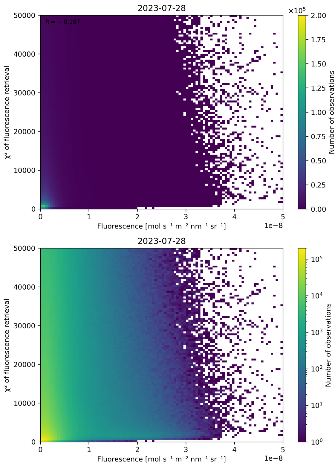
Figure 93: Scatter density plot of “Fluorescence” against “ \chi^2 of fluorescence retrieval” for 2023-07-27 to 2023-07-29.
