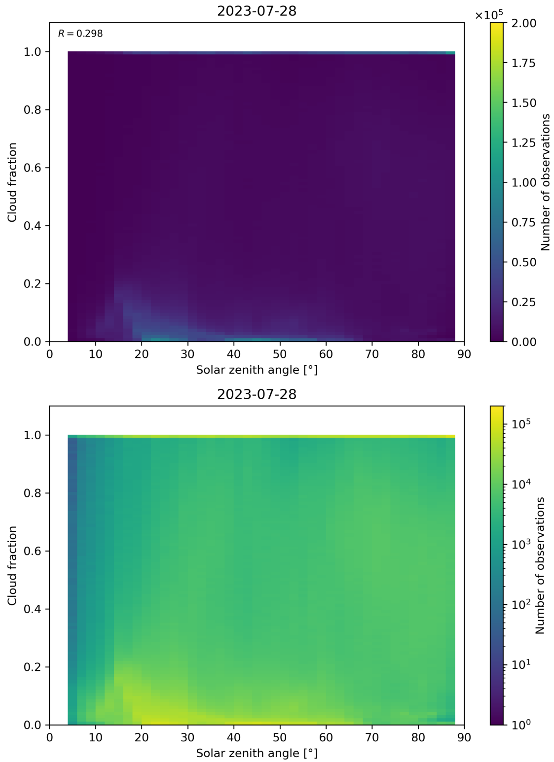
Figure 121: Scatter density plot of “Solar zenith angle” against “Cloud fraction” for 2023-07-27 to 2023-07-29.
