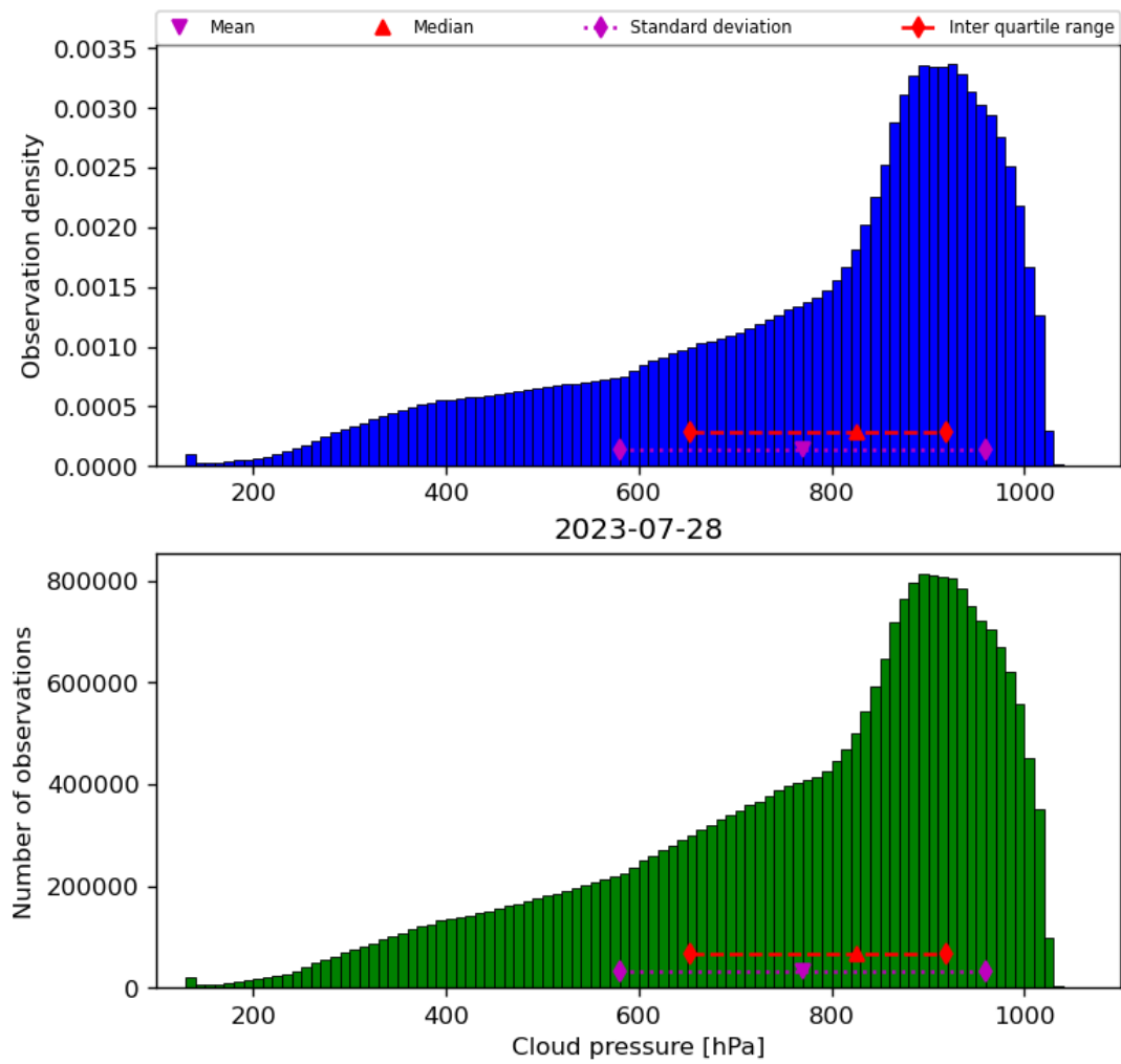
Figure 30: Histogram of “Cloud pressure” for 2023-07-27 to 2023-07-29
