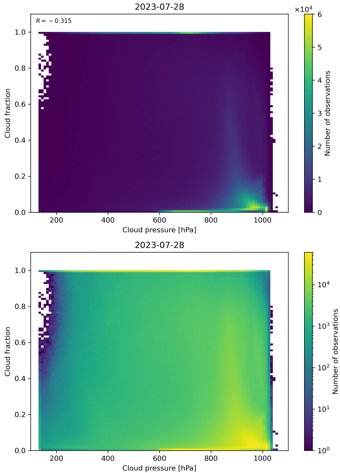
Figure 87: Scatter density plot of “Cloud pressure” against “Cloud fraction” for 2023-07-27 to 2023-07-29.
