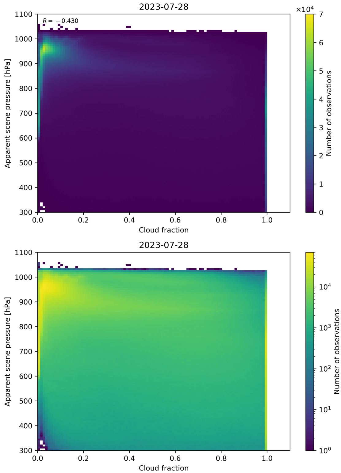
Figure 76: Scatter density plot of “Cloud fraction” against “Apparent scene pressure” for 2023-07-27 to 2023-07-29.
