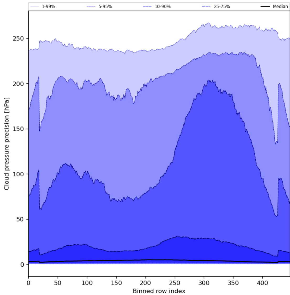
Figure 48: Along track statistics of “Cloud pressure precision” for 2023-07-27 to 2023-07-29
