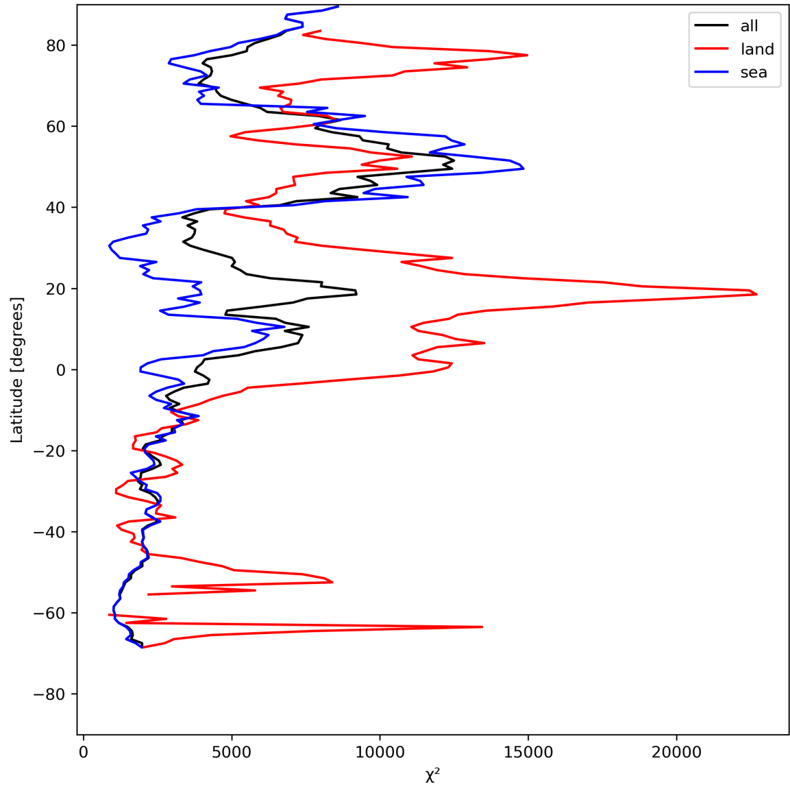
Figure 21: Zonal average of “ \chi^2 ” for 2023-07-27 to 2023-07-29.
