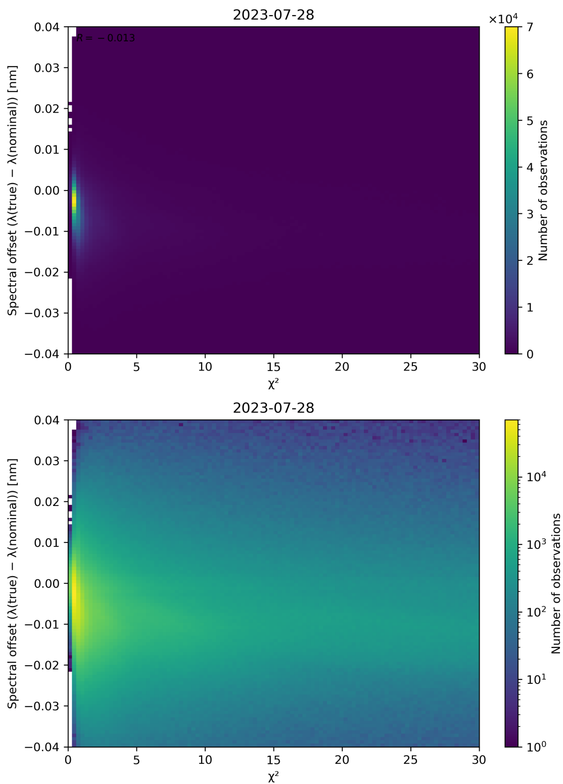
Figure 75: Scatter density plot of " \chi^2 " against "Spectral offset ( \lambda(\text{true}) - \lambda(\text{nominal}) )" for 2023-07-27 to 2023-07-29.
