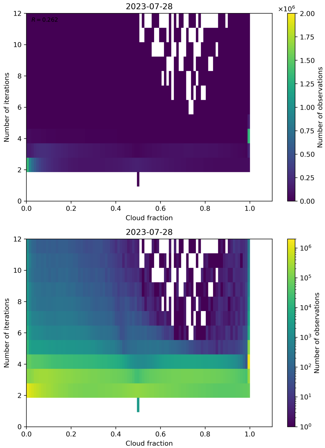
Figure 80: Scatter density plot of “Cloud fraction” against “Number of iterations” for 2023-07-27 to 2023-07-29.
