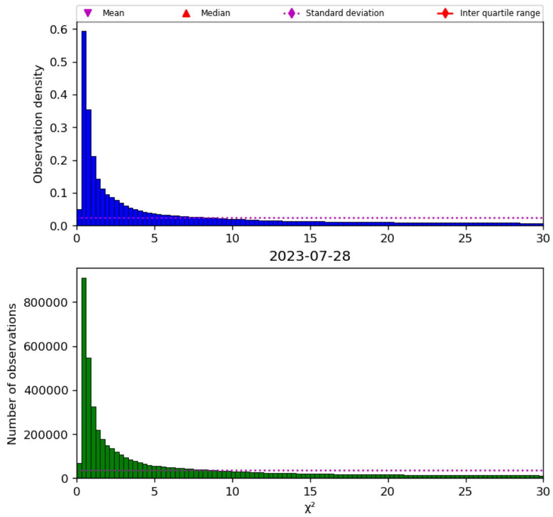
Figure 38: Histogram of “ \chi^2 ” for 2023-07-27 to 2023-07-29
