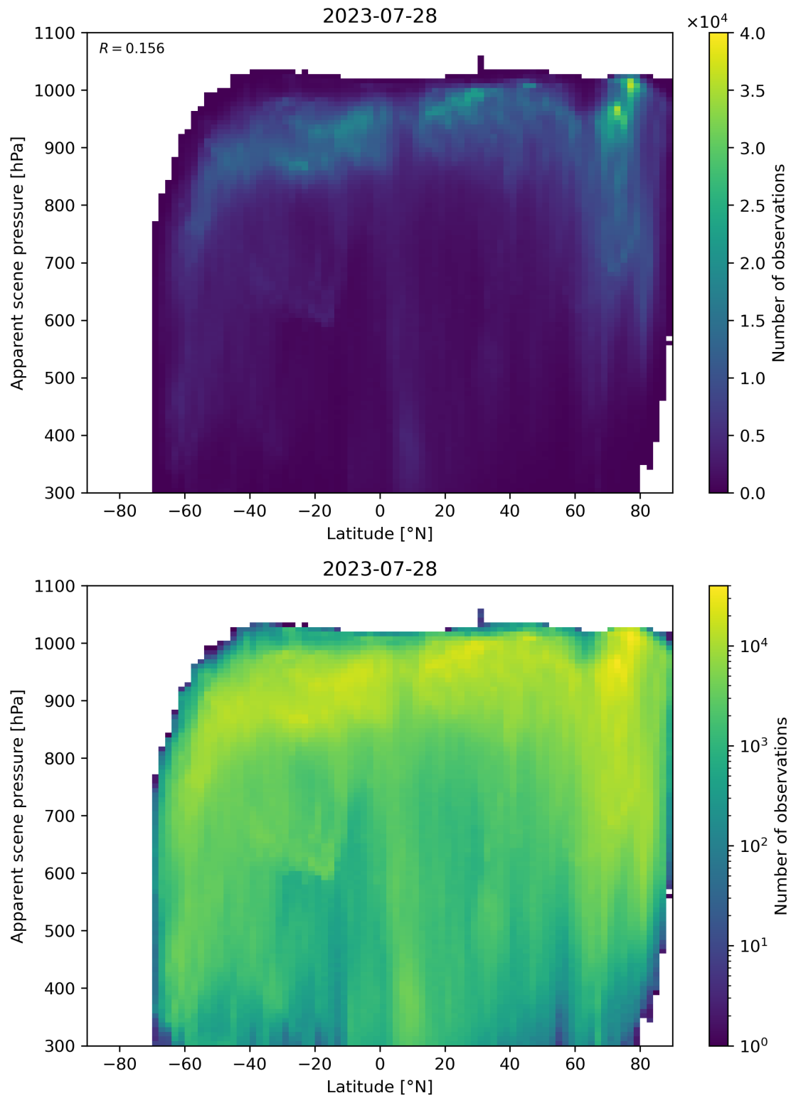
Figure 96: Scatter density plot of “Latitude” against “Apparent scene pressure” for 2023-07-27 to 2023-07-29.
