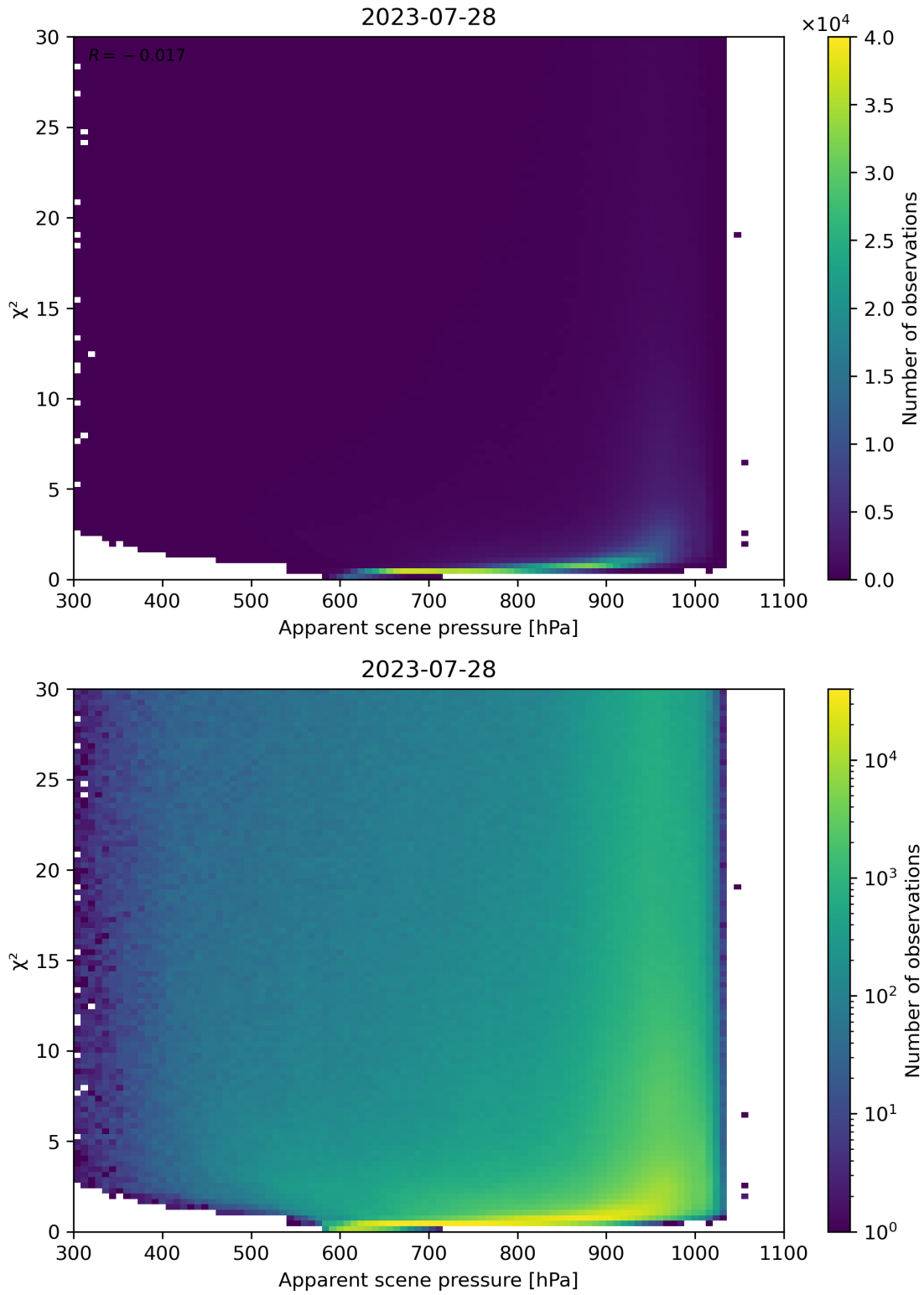
Figure 63: Scatter density plot of “Apparent scene pressure” against “ \chi^2 ” for 2023-07-27 to 2023-07-29.
