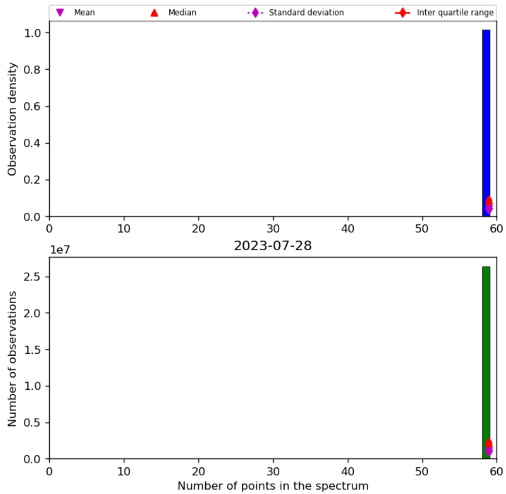
Figure 44: Histogram of “Number of points in the spectrum” for 2023-07-27 to 2023-07-29
