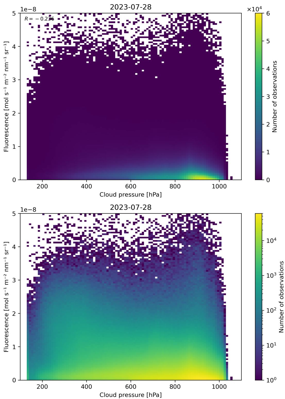
Figure 88: Scatter density plot of “Cloud pressure” against “Fluorescence” for 2023-07-27 to 2023-07-29.
