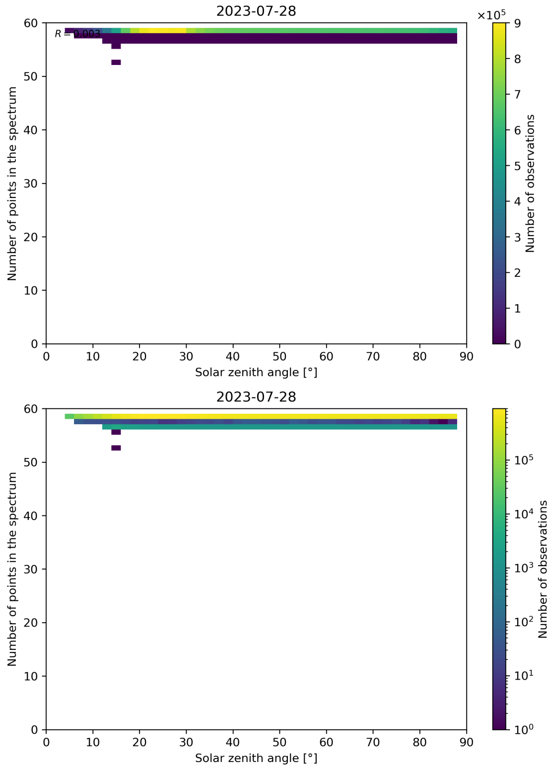
Figure 126: Scatter density plot of “Solar zenith angle” against “Number of points in the spectrum” for 2023-07-27 to 2023-07-29.
