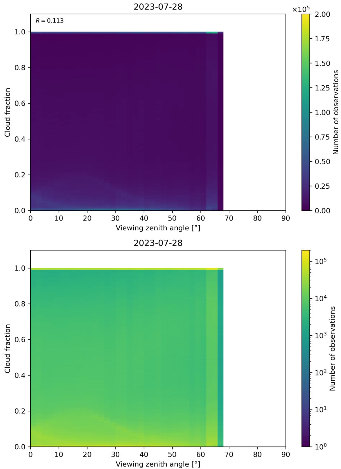
Figure 132: Scatter density plot of “Viewing zenith angle” against “Cloud fraction” for 2023-07-27 to 2023-07-29.
