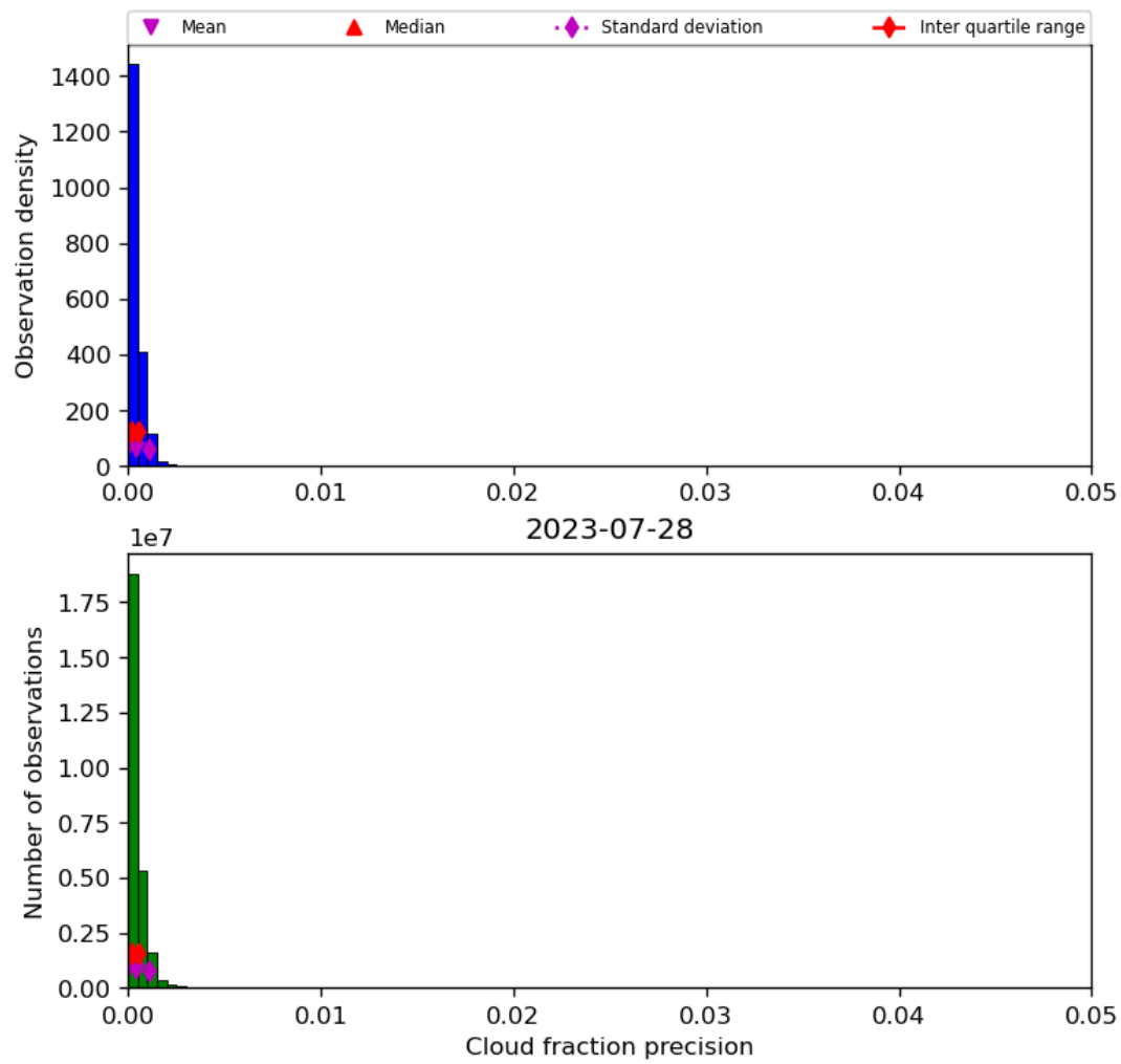
Figure 33: Histogram of “Cloud fraction precision” for 2023-07-27 to 2023-07-29
