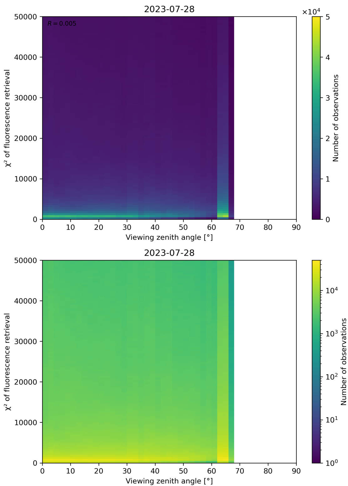
Figure 131: Scatter density plot of “Viewing zenith angle” against “ \chi^2 of fluorescence retrieval” for 2023-07-27 to 2023-07-29.
