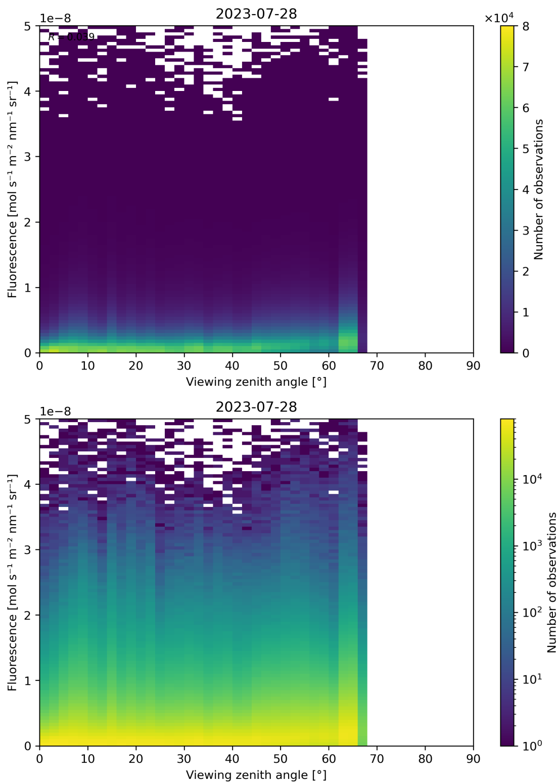
Figure 134: Scatter density plot of “Viewing zenith angle” against “Fluorescence” for 2023-07-27 to 2023-07-29.
