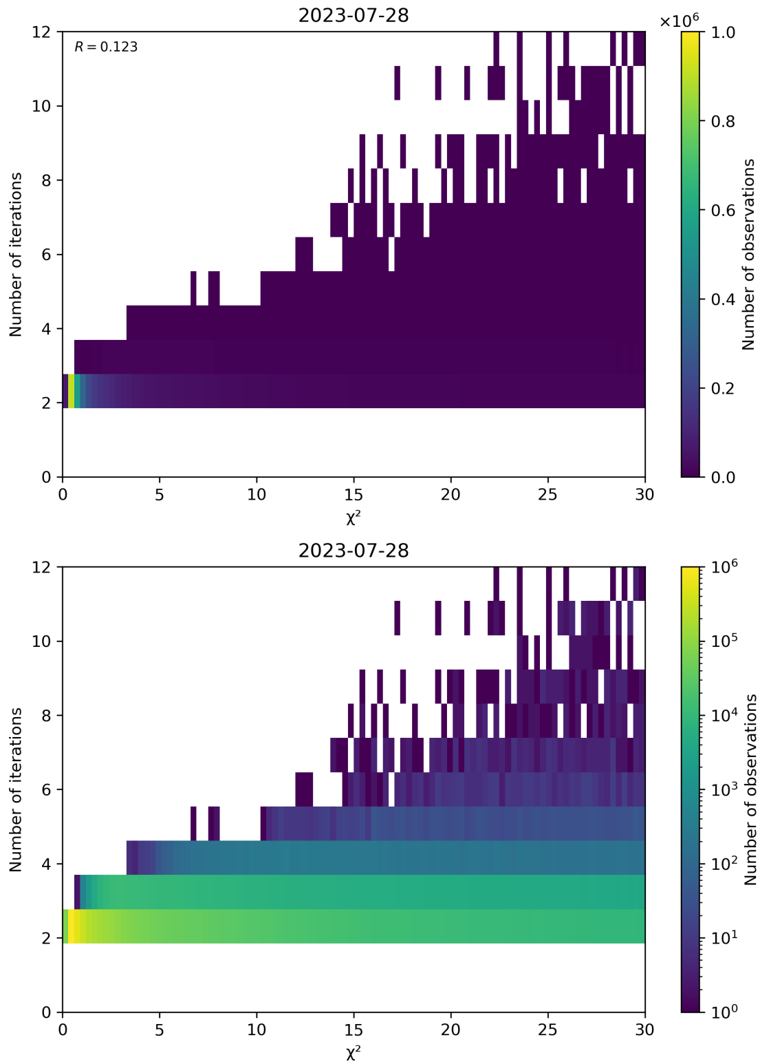
Figure 73: Scatter density plot of " \chi^2 " against "Number of iterations" for 2023-07-27 to 2023-07-29.
