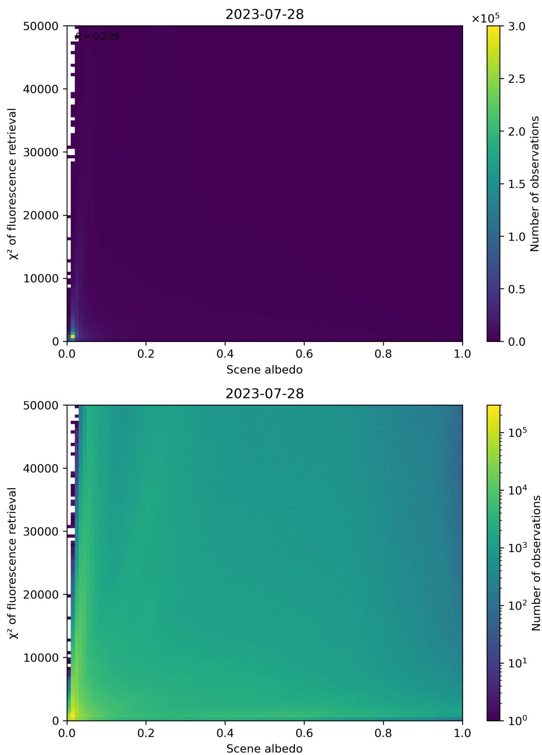
Figure 113: Scatter density plot of “Scene albedo” against “ \chi^2 of fluorescence retrieval” for 2023-07-27 to 2023-07-29.
