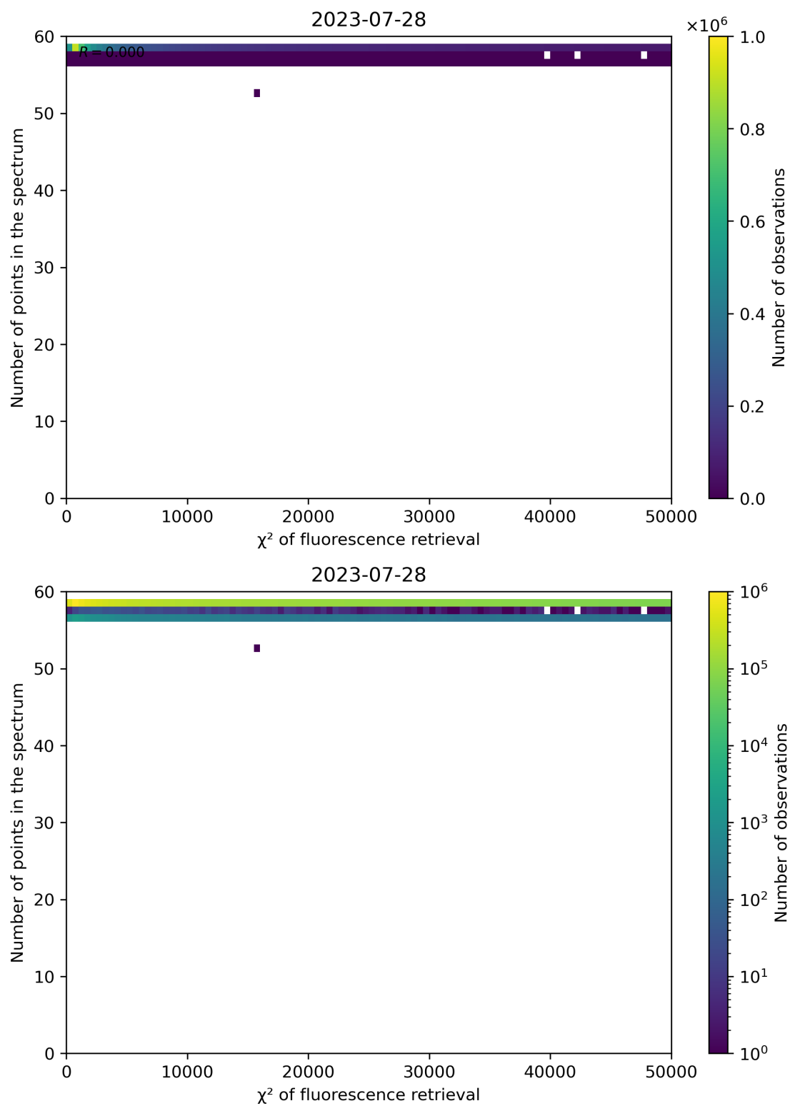
Figure 71: Scatter density plot of “ \chi^2 of fluorescence retrieval” against “Number of points in the spectrum” for 2023-07-27 to 2023-07-29.
