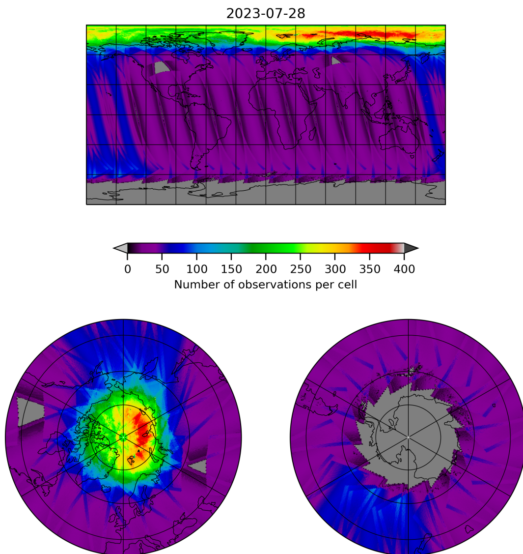
Figure 11: Map of the number of observations for 2023-07-27 to 2023-07-29
