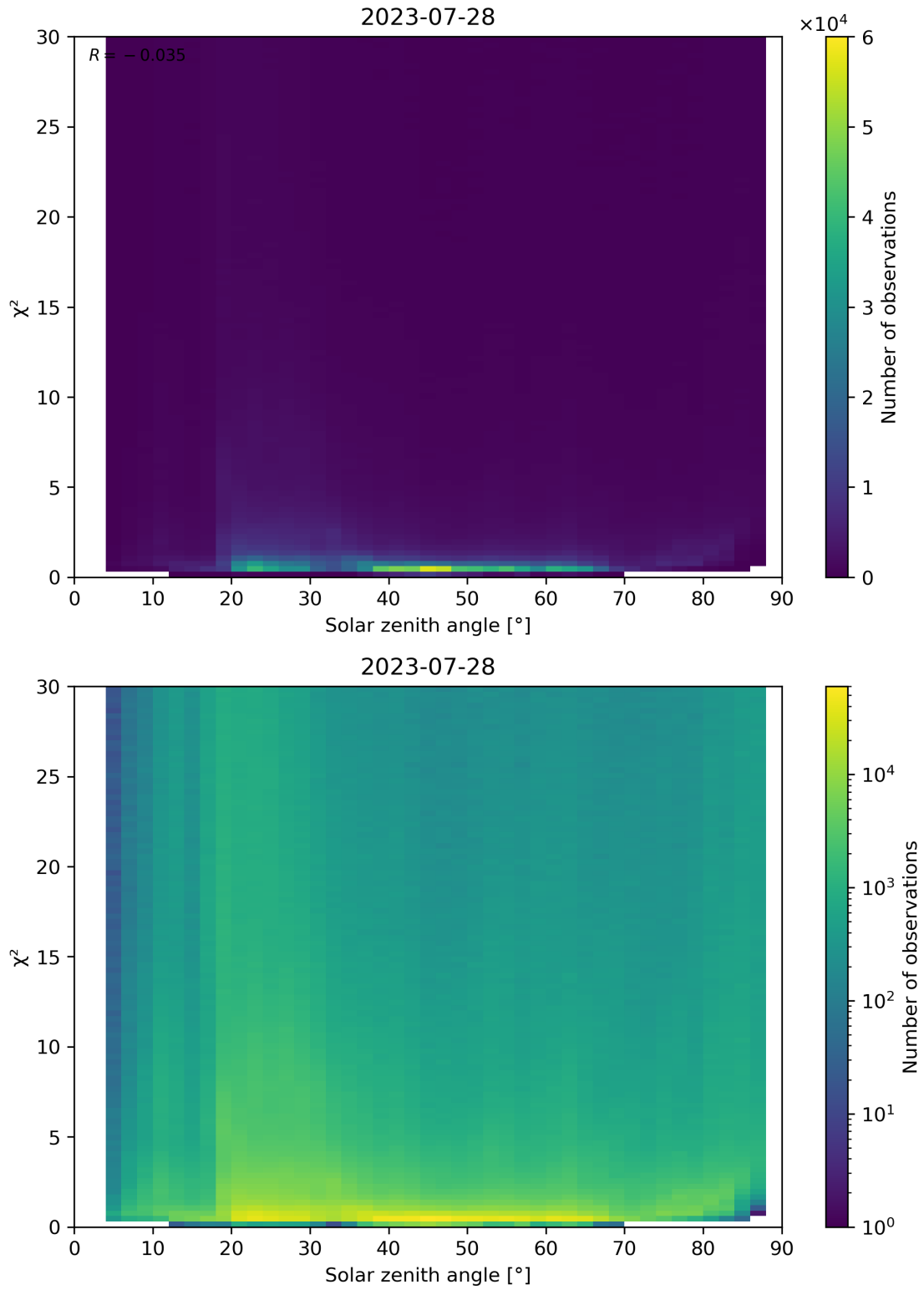
Figure 119: Scatter density plot of “Solar zenith angle” against “ \chi^2 ” for 2023-07-27 to 2023-07-29.
