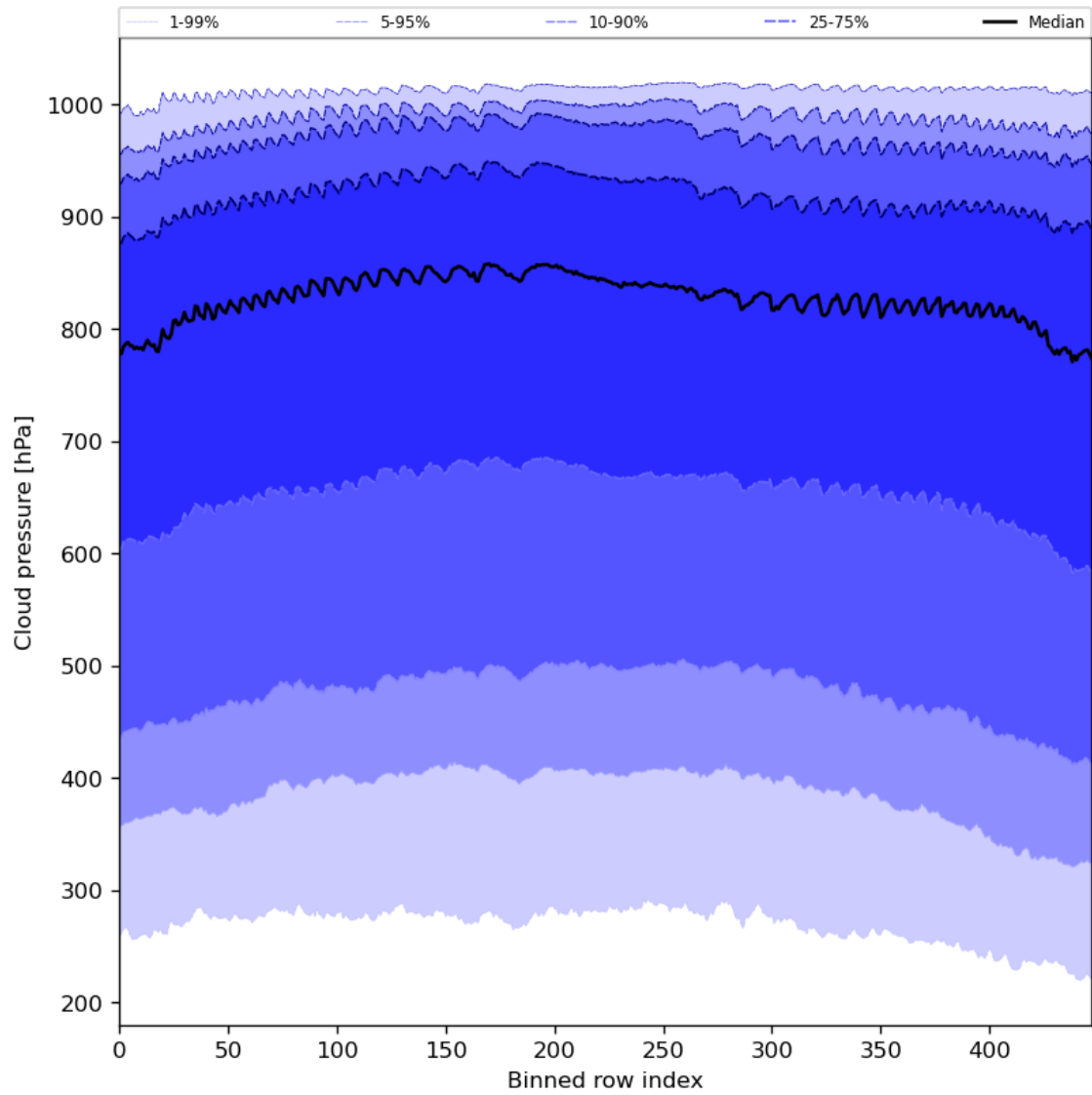
Figure 47: Along track statistics of “Cloud pressure” for 2023-07-27 to 2023-07-29
