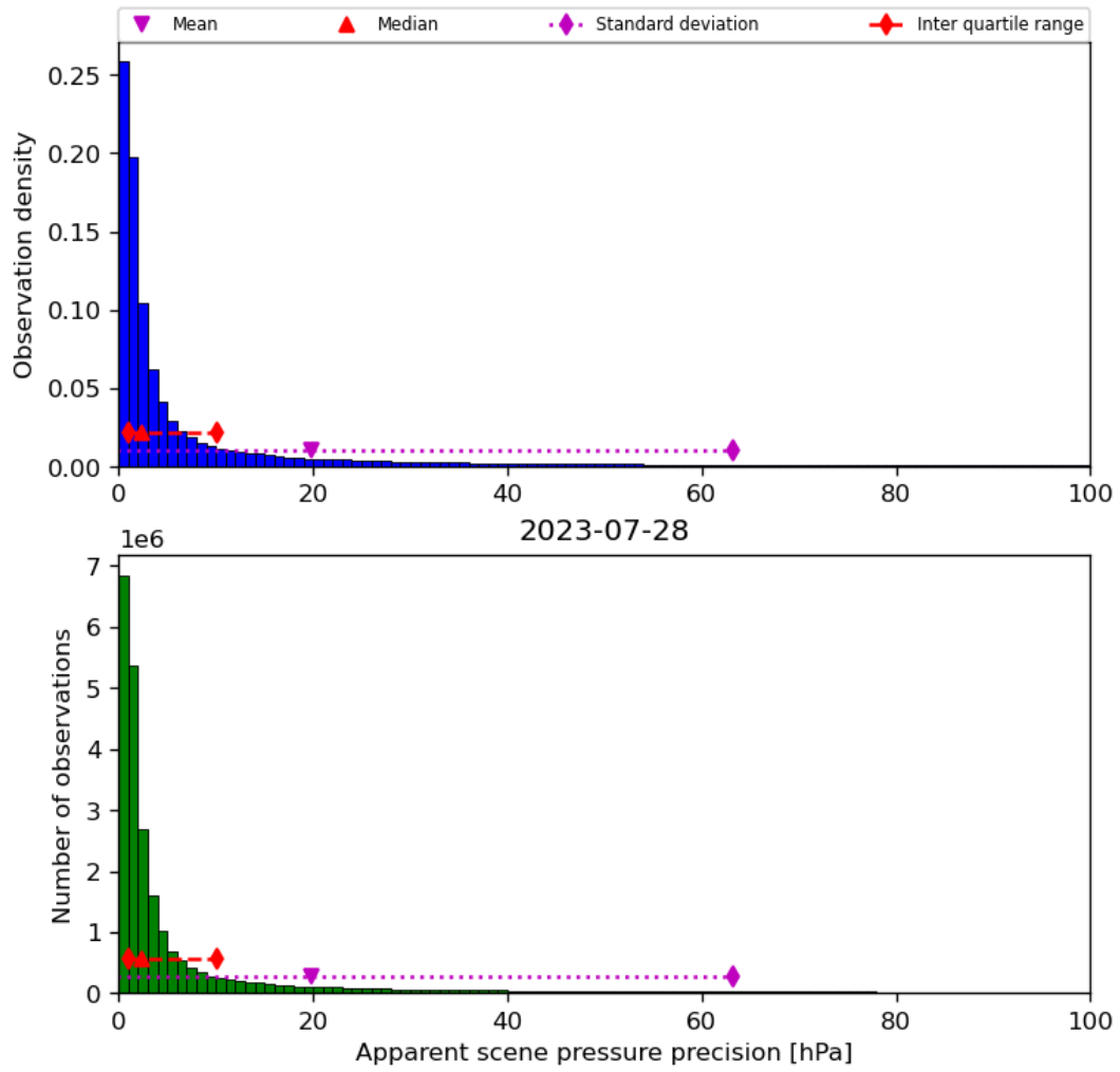
Figure 37: Histogram of “Apparent scene pressure precision” for 2023-07-27 to 2023-07-29
