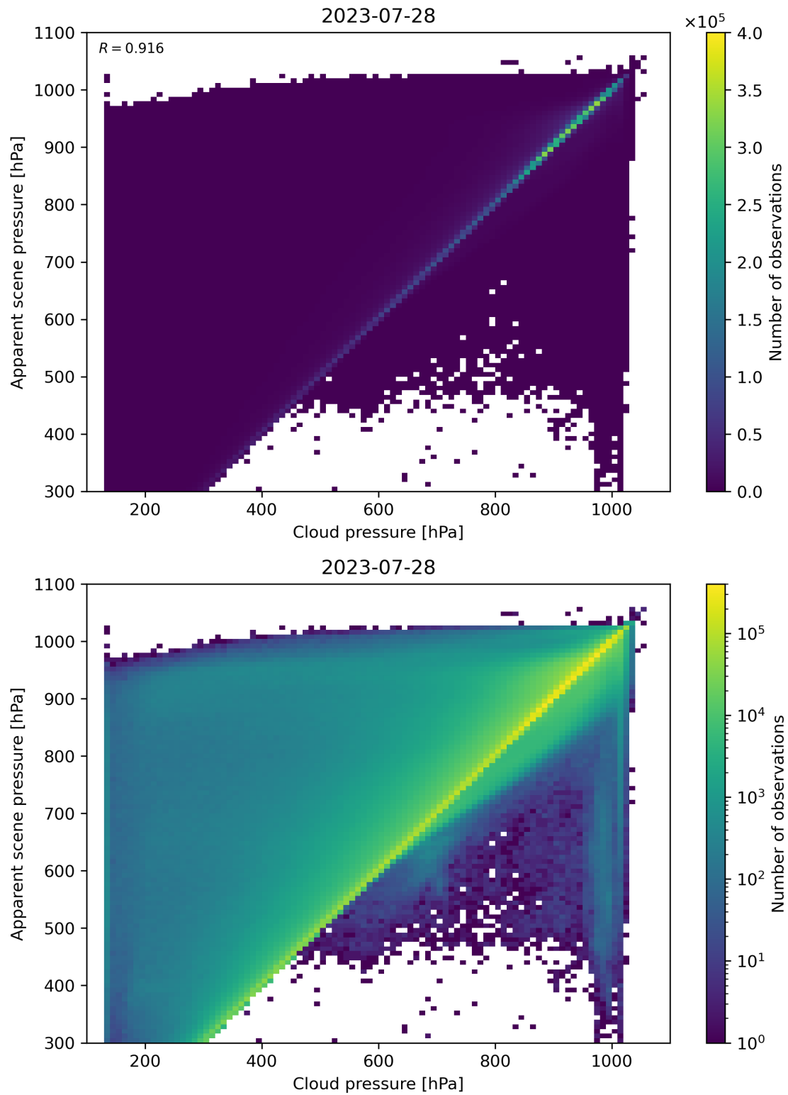
Figure 84: Scatter density plot of “Cloud pressure” against “Apparent scene pressure” for 2023-07-27 to 2023-07-29.
