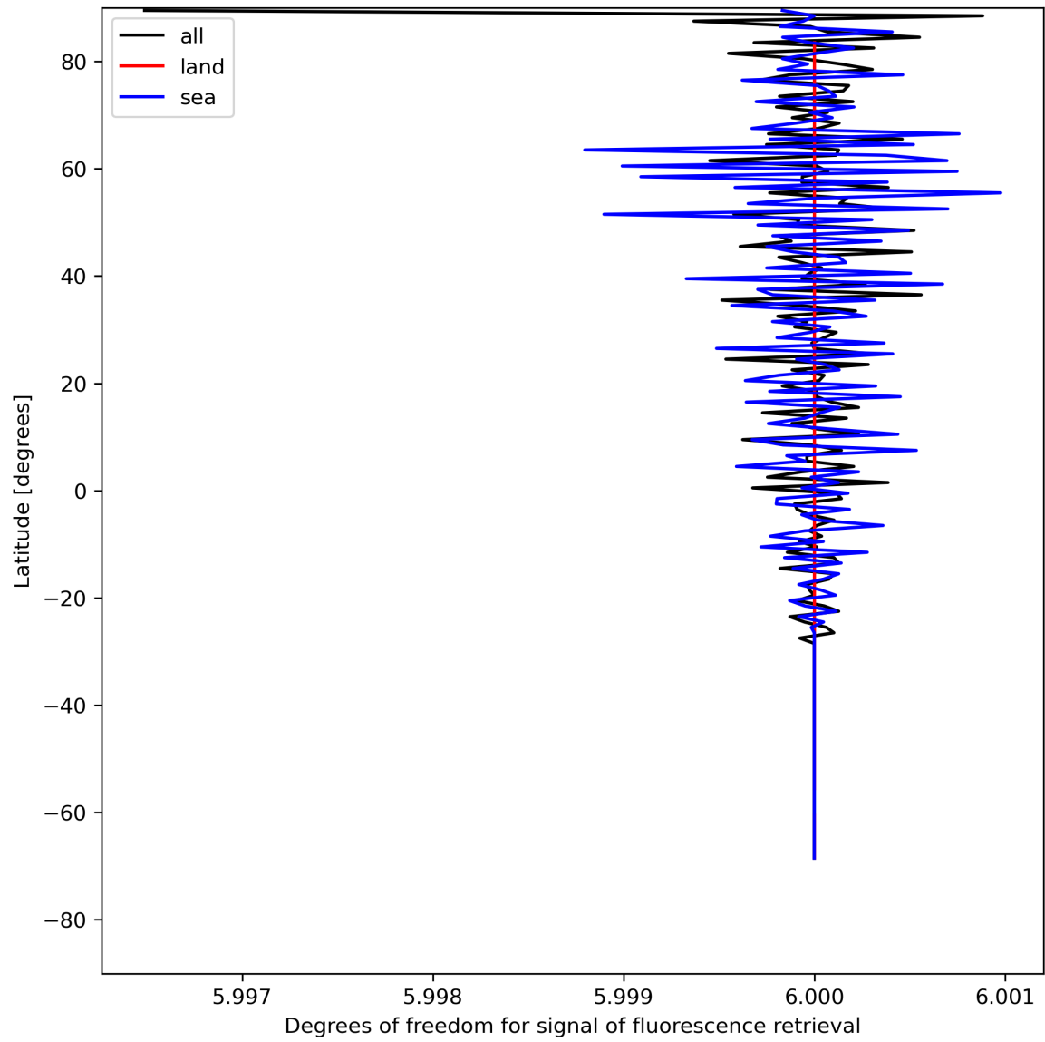
Figure 26: Zonal average of “Degrees of freedom for signal of fluorescence retrieval” for 2023-07-27 to 2023-07-29.
