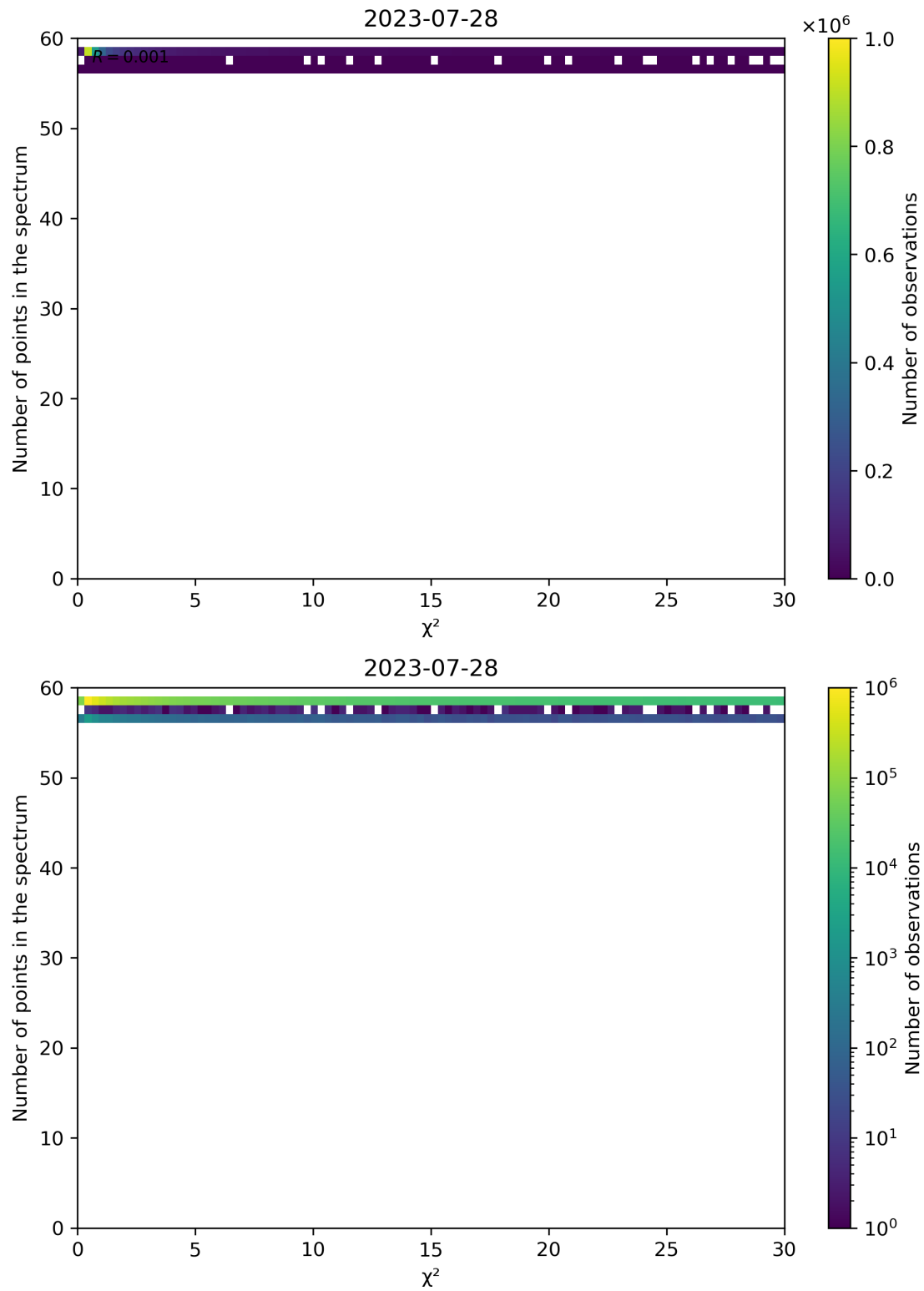
Figure 74: Scatter density plot of “ \chi^2 ” against “Number of points in the spectrum” for 2023-07-27 to 2023-07-29.
