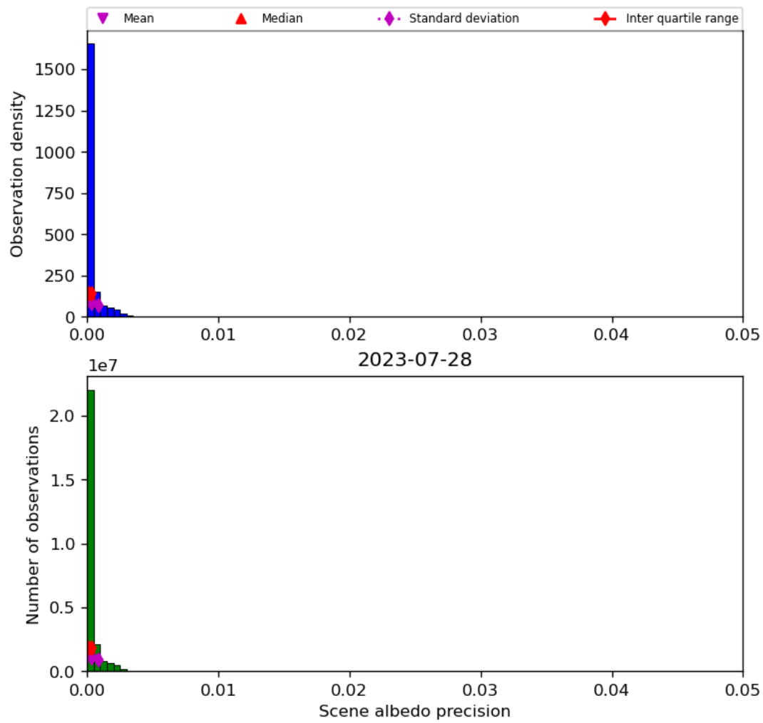
Figure 35: Histogram of “Scene albedo precision” for 2023-07-27 to 2023-07-29
