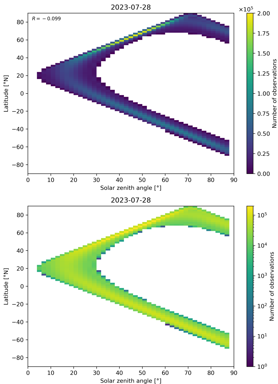
Figure 124: Scatter density plot of “Solar zenith angle” against “Latitude” for 2023-07-27 to 2023-07-29.
