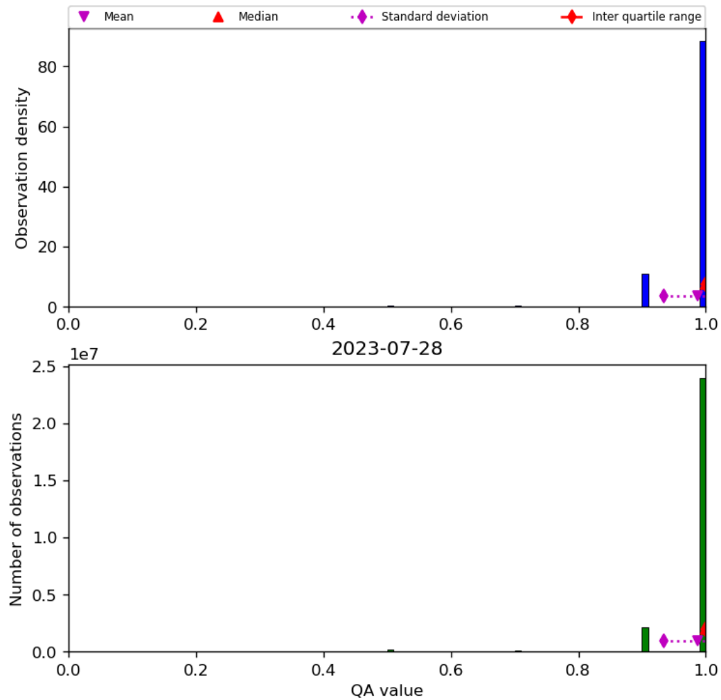
Figure 29: Histogram of “QA value” for 2023-07-27 to 2023-07-29
