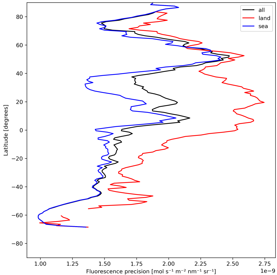
Figure 24: Zonal average of “Fluorescence precision” for 2023-07-27 to 2023-07-29.
