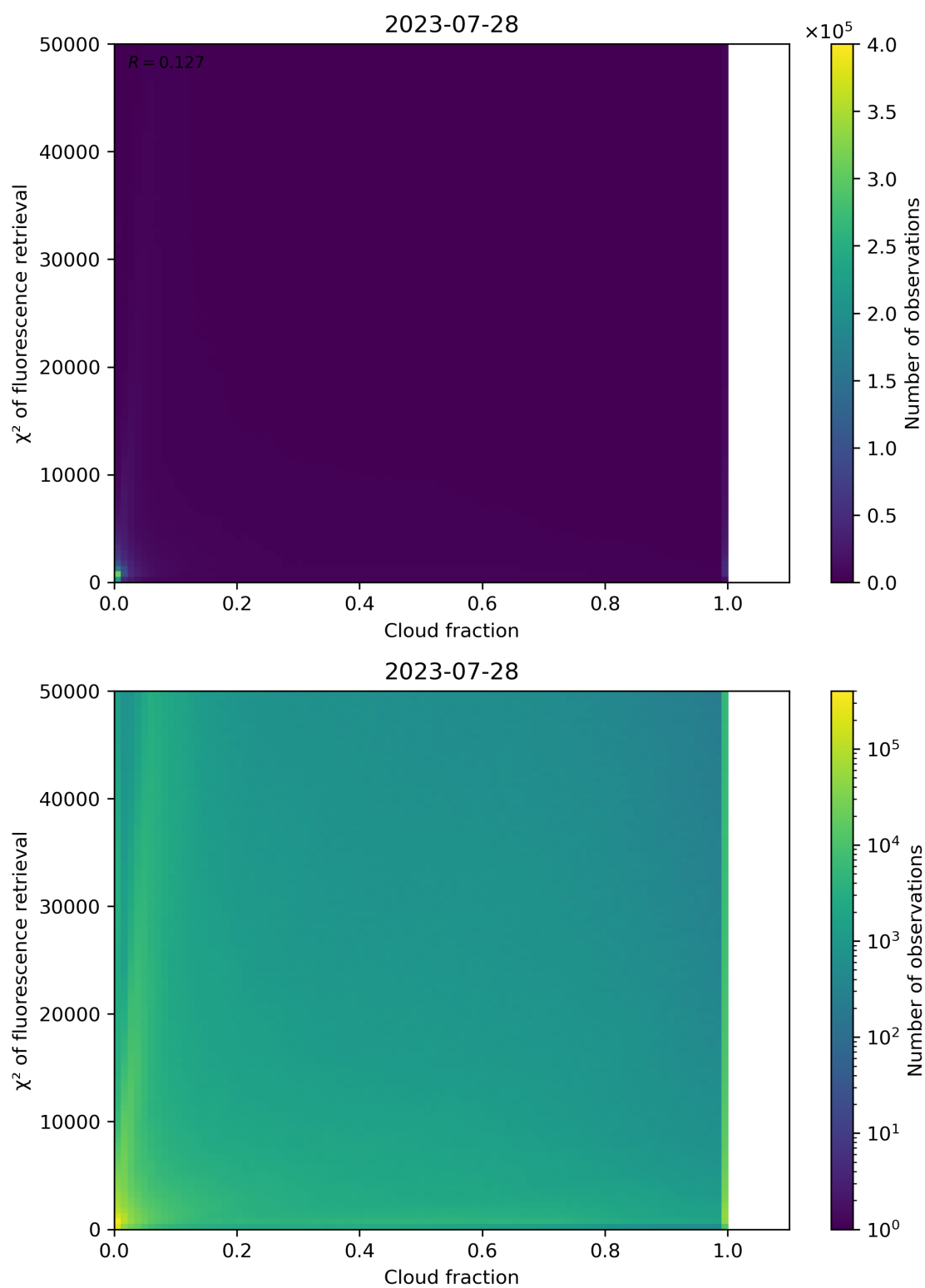
Figure 78: Scatter density plot of “Cloud fraction” against “ \chi^2 of fluorescence retrieval” for 2023-07-27 to 2023-07-29.
