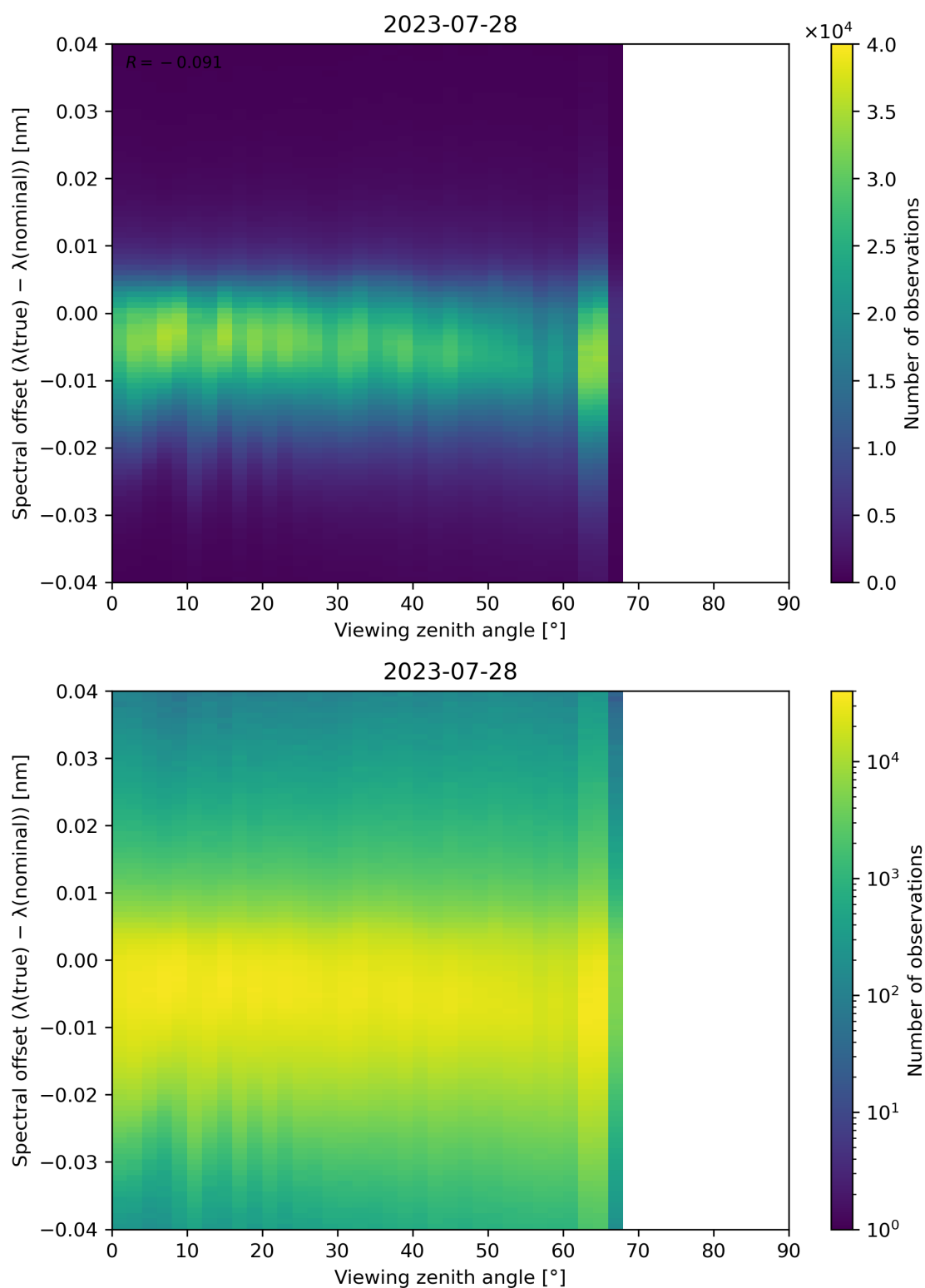
Figure 140: Scatter density plot of “Viewing zenith angle” against “Spectral offset ( \lambda(\text{true}) - \lambda(\text{nominal}) )” for 2023-07-27 to 2023-07-29.
