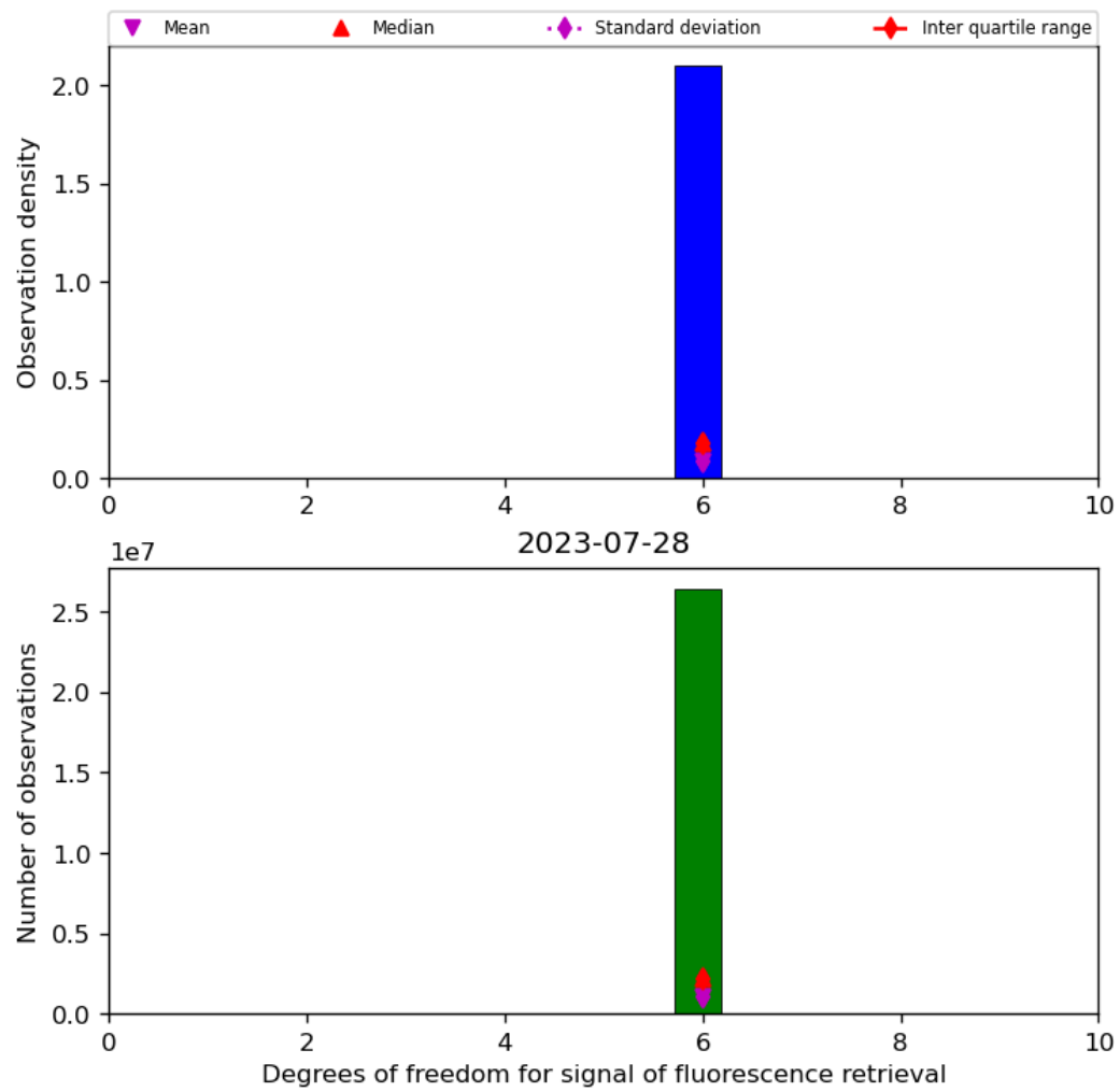
Figure 43: Histogram of “Degrees of freedom for signal of fluorescence retrieval” for 2023-07-27 to 2023-07-29
