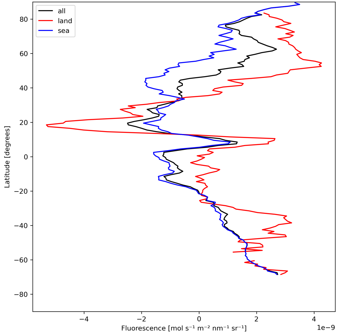
Figure 23: Zonal average of “Fluorescence” for 2023-07-27 to 2023-07-29.
