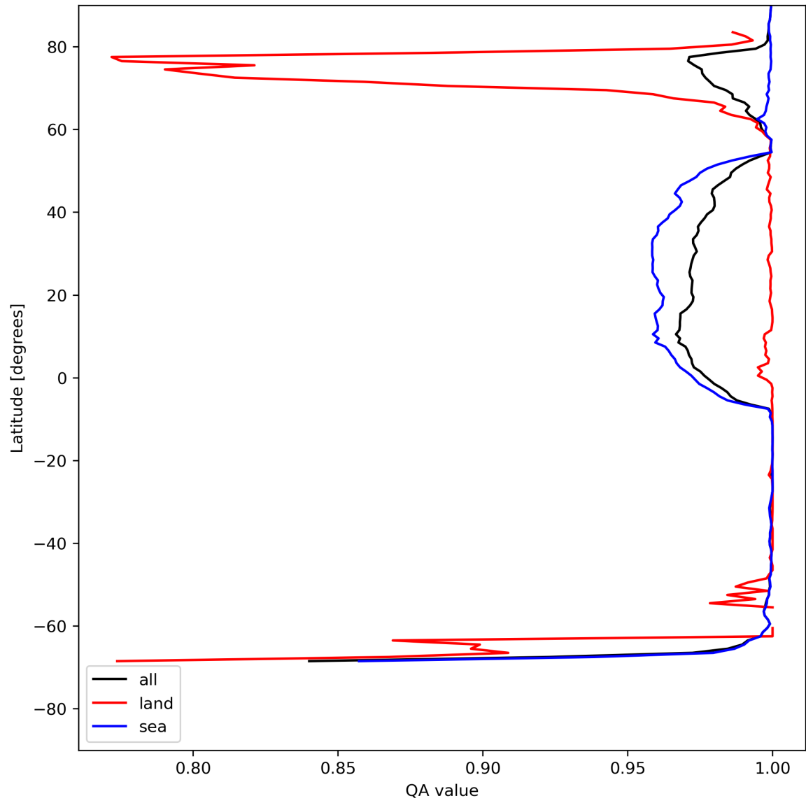
Figure 12: Zonal average of “QA value” for 2023-07-27 to 2023-07-29.
