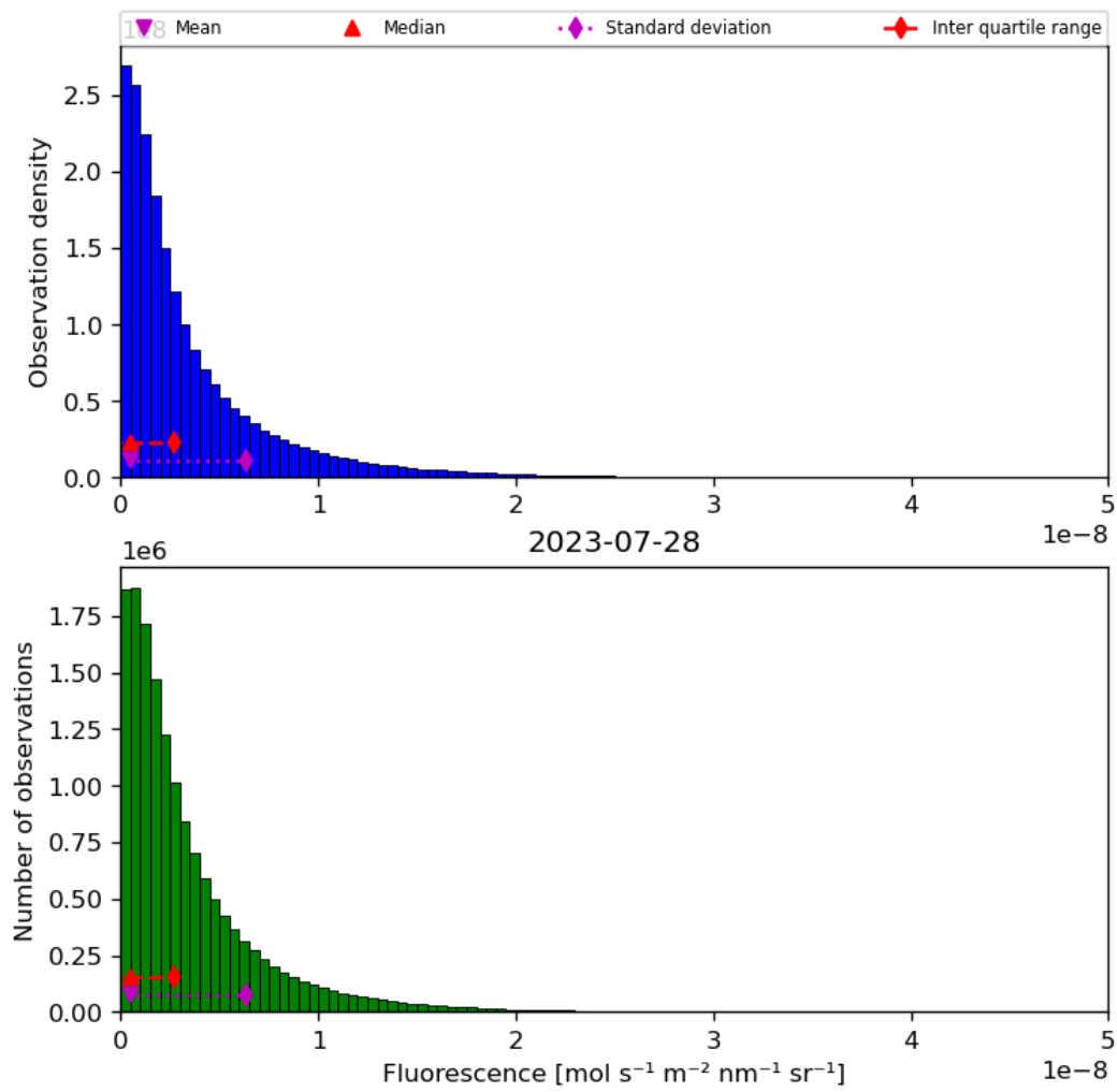
Figure 40: Histogram of “Fluorescence” for 2023-07-27 to 2023-07-29
