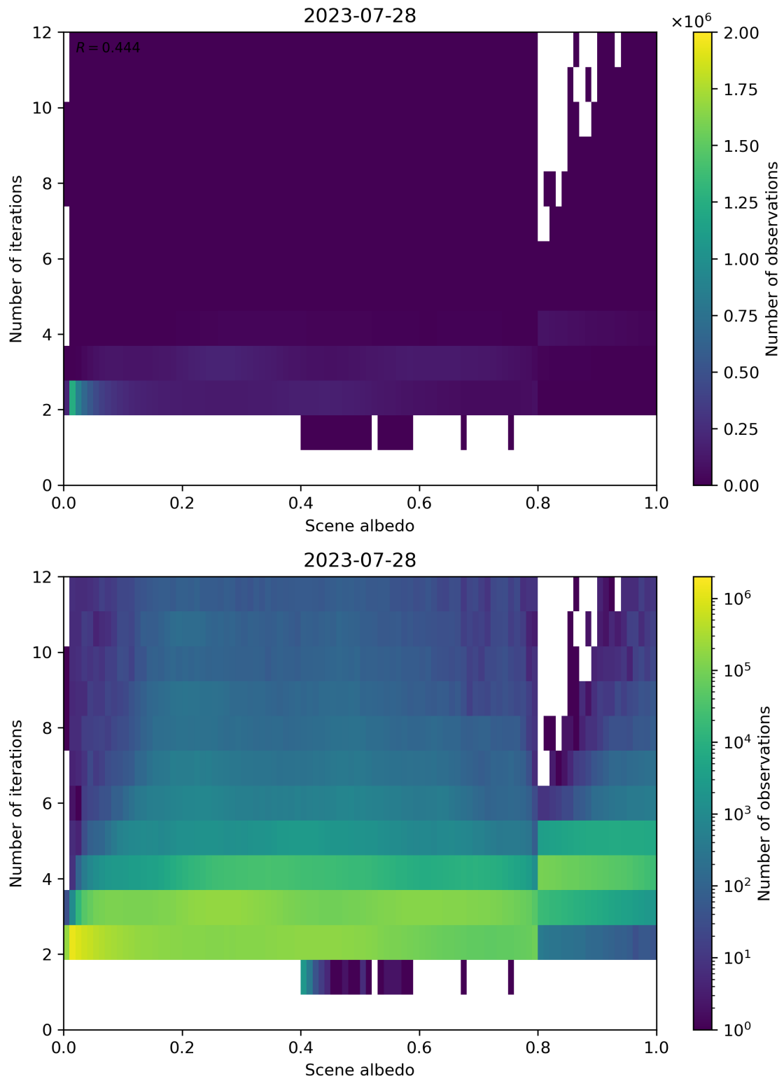
Figure 115: Scatter density plot of “Scene albedo” against “Number of iterations” for 2023-07-27 to 2023-07-29.
