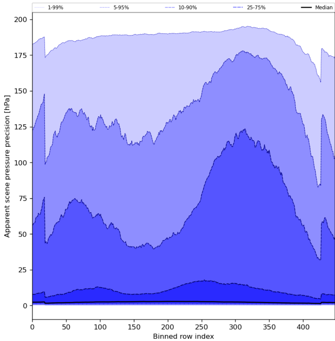
Figure 54: Along track statistics of “Apparent scene pressure precision” for 2023-07-27 to 2023-07-29
