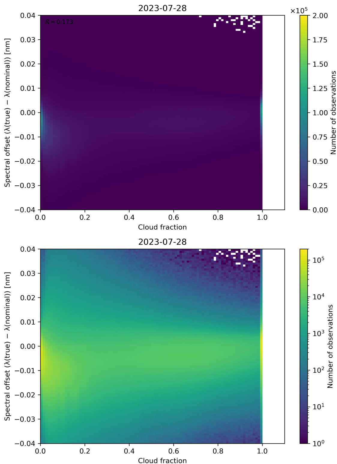
Figure 83: Scatter density plot of “Cloud fraction” against “Spectral offset ( \lambda(\text{true}) - \lambda(\text{nominal}) )” for 2023-07-27 to 2023-07-29.
