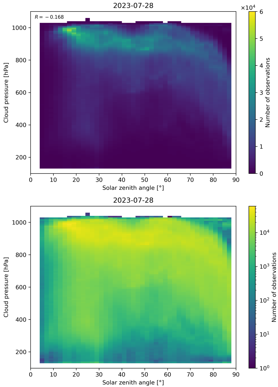
Figure 122: Scatter density plot of “Solar zenith angle” against “Cloud pressure” for 2023-07-27 to 2023-07-29.
