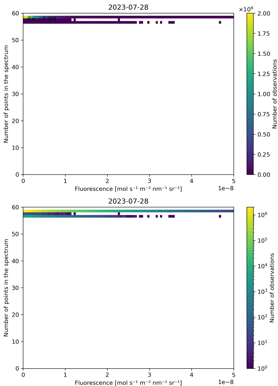
Figure 94: Scatter density plot of “Fluorescence” against “Number of points in the spectrum” for 2023-07-27 to 2023-07-29.
