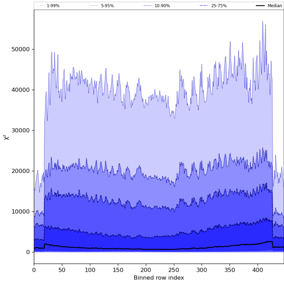
Figure 55: Along track statistics of “ \chi^2 ” for 2023-07-27 to 2023-07-29
