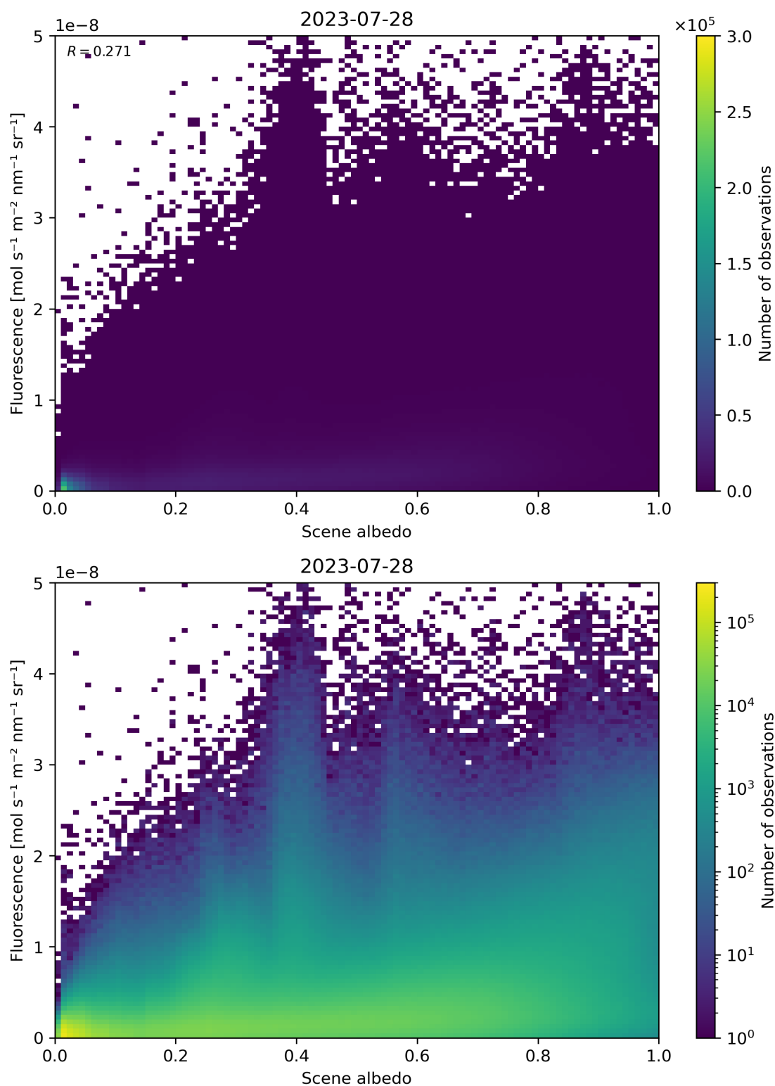
Figure 114: Scatter density plot of “Scene albedo” against “Fluorescence” for 2023-07-27 to 2023-07-29.
