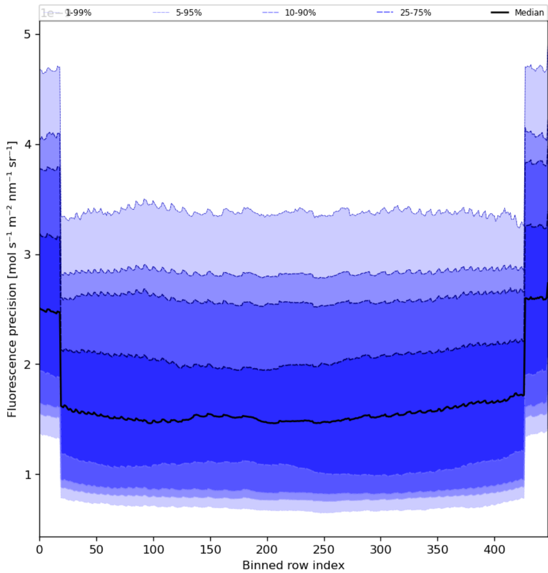
Figure 58: Along track statistics of “Fluorescence precision” for 2023-07-27 to 2023-07-29
