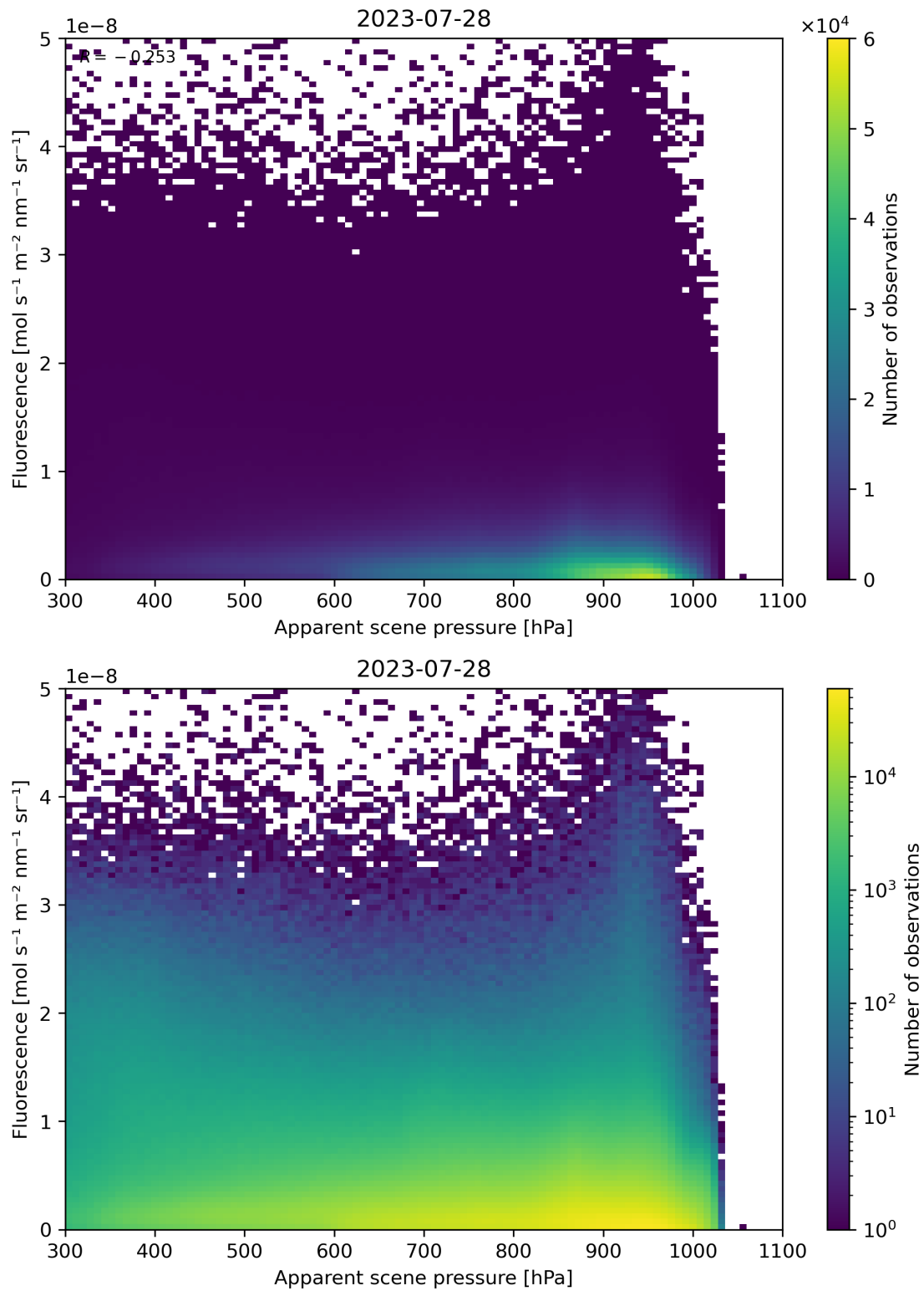
Figure 65: Scatter density plot of “Apparent scene pressure” against “Fluorescence” for 2023-07-27 to 2023-07-29.
