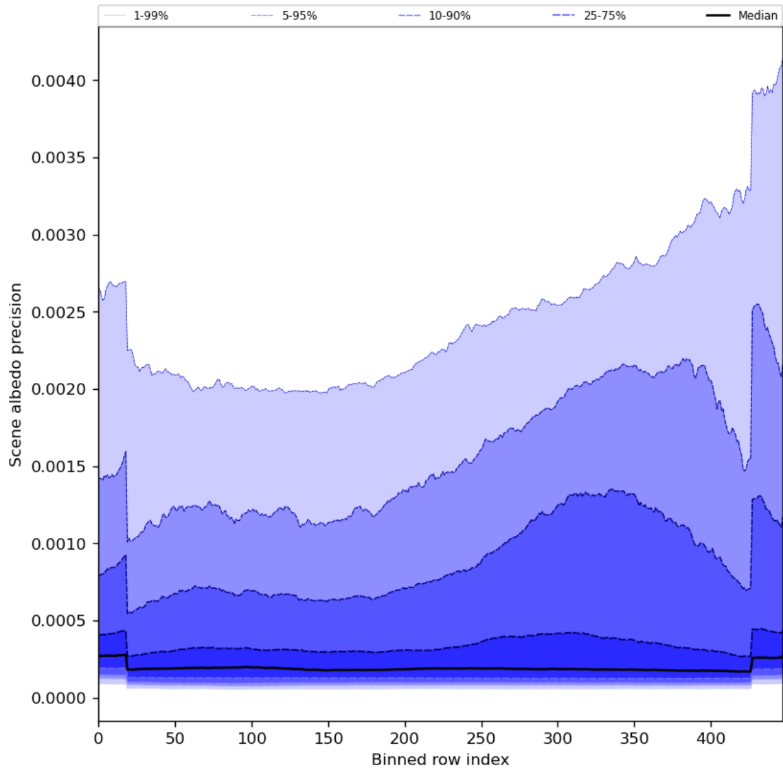
Figure 52: Along track statistics of “Scene albedo precision” for 2023-07-27 to 2023-07-29
