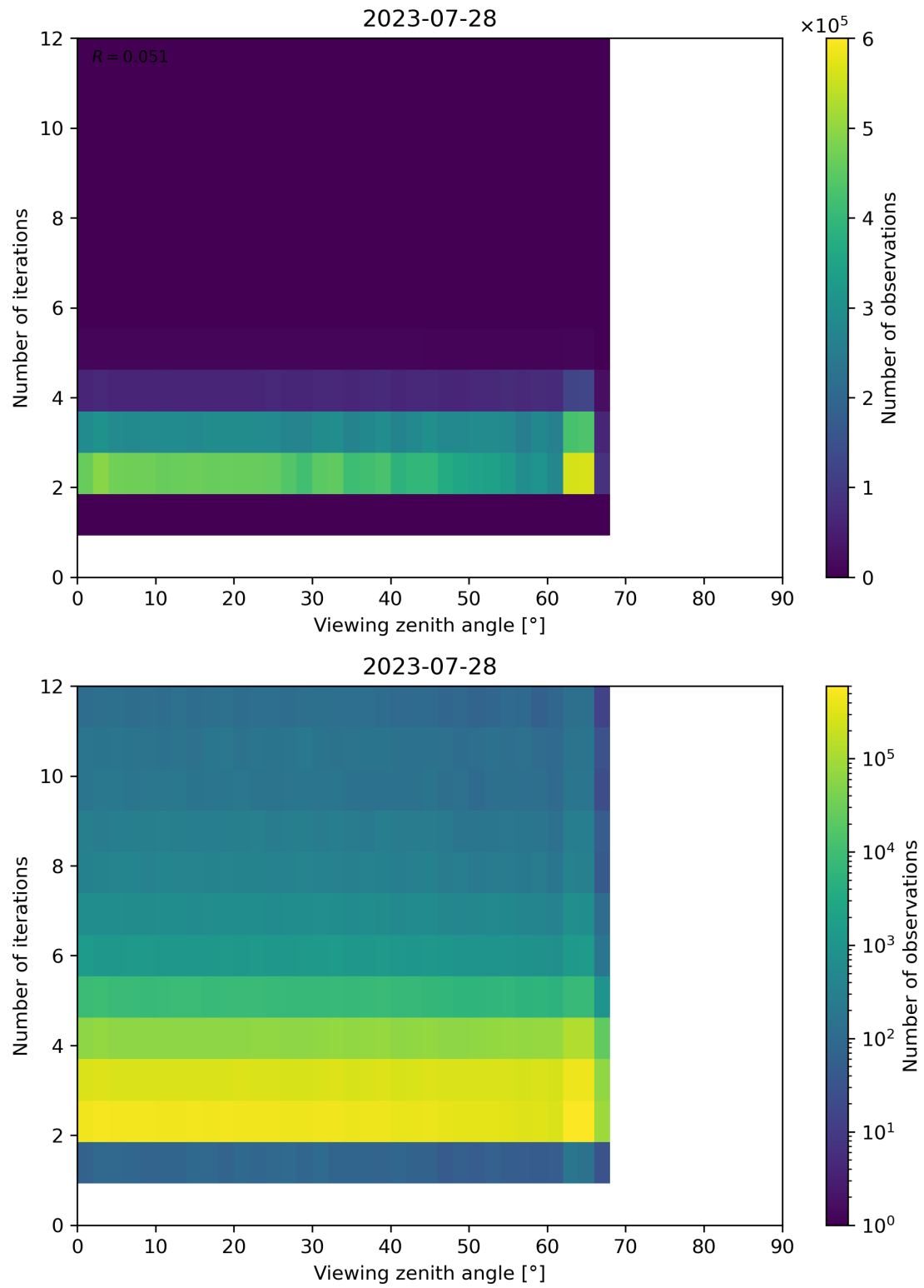
Figure 136: Scatter density plot of “Viewing zenith angle” against “Number of iterations” for 2023-07-27 to 2023-07-29.
