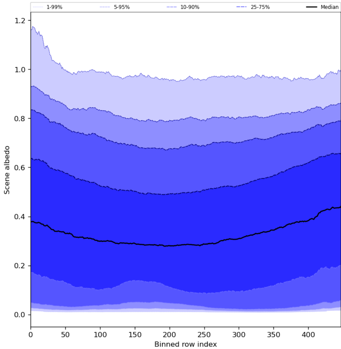
Figure 51: Along track statistics of “Scene albedo” for 2023-07-27 to 2023-07-29
