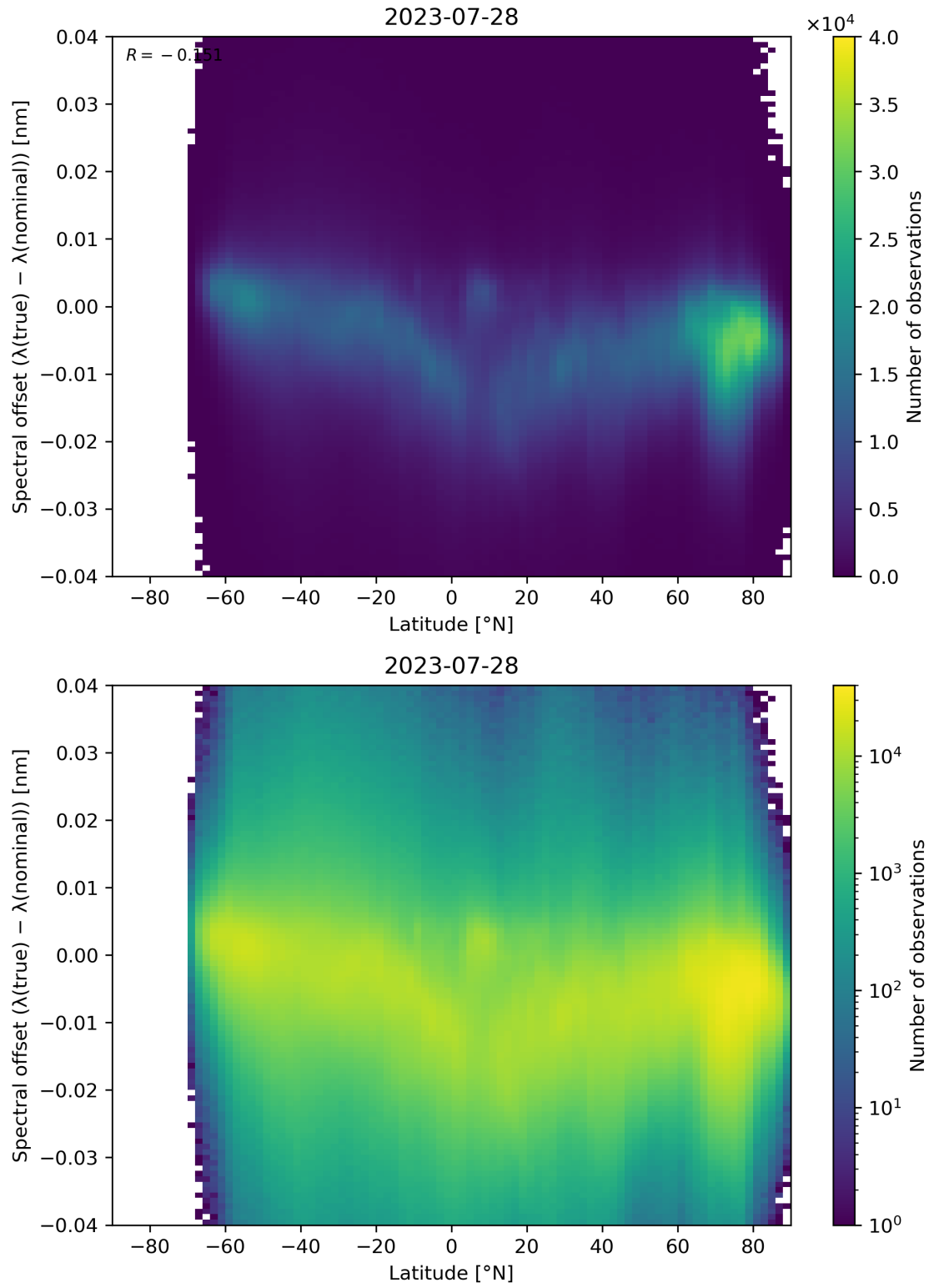
Figure 105: Scatter density plot of “Latitude” against “Spectral offset ( \lambda(\text{true}) - \lambda(\text{nominal}) )” for 2023-07-27 to 2023-07-29.
