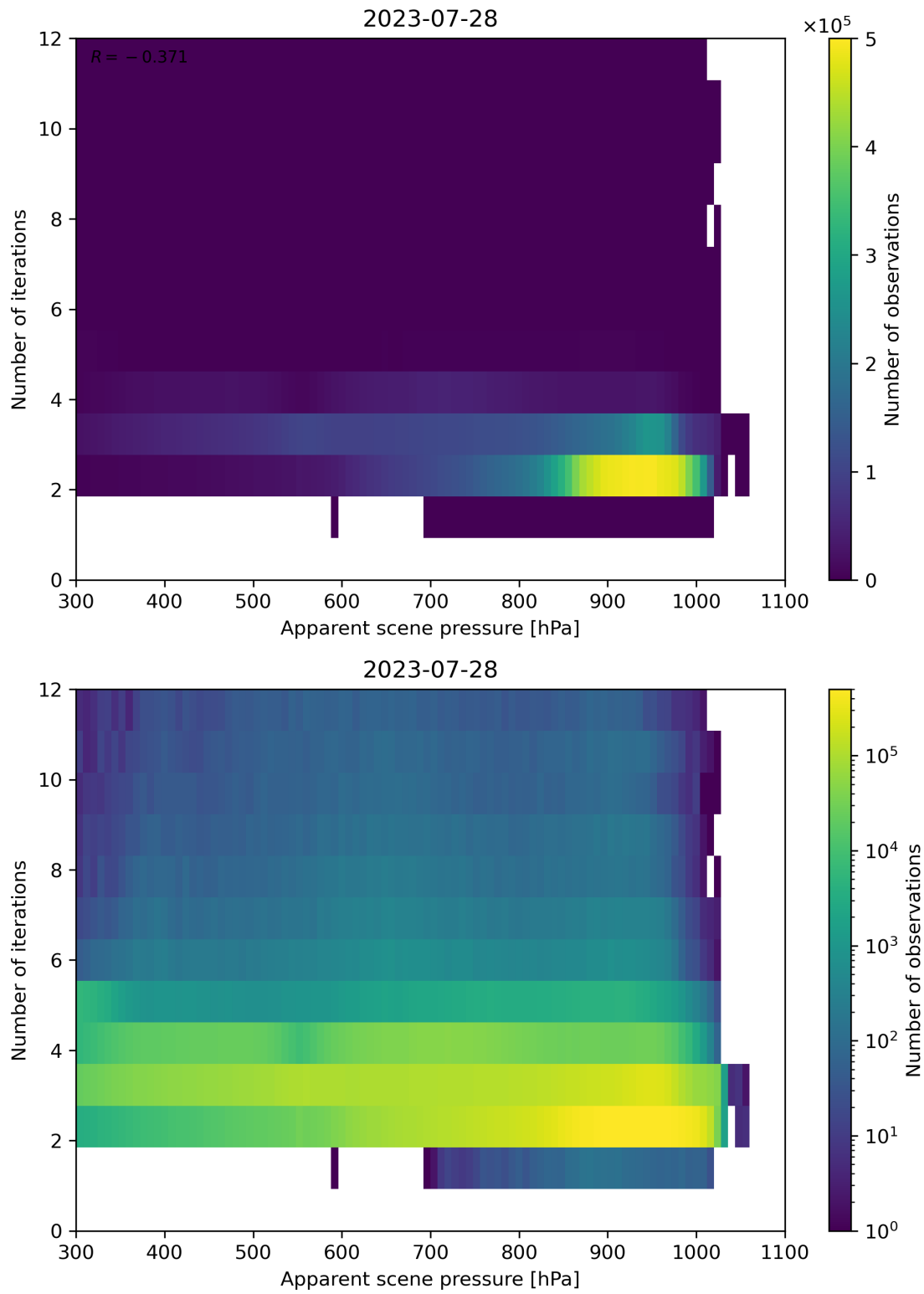
Figure 66: Scatter density plot of “Apparent scene pressure” against “Number of iterations” for 2023-07-27 to 2023-07-29.
