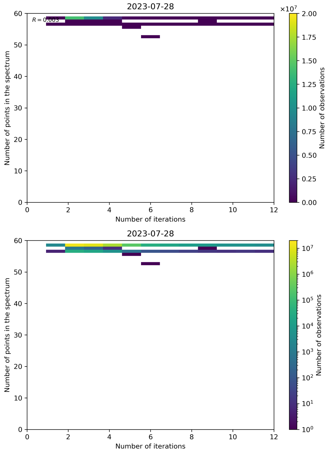
Figure 108: Scatter density plot of “Number of iterations” against “Number of points in the spectrum” for 2023-07-27 to 2023-07-29.
