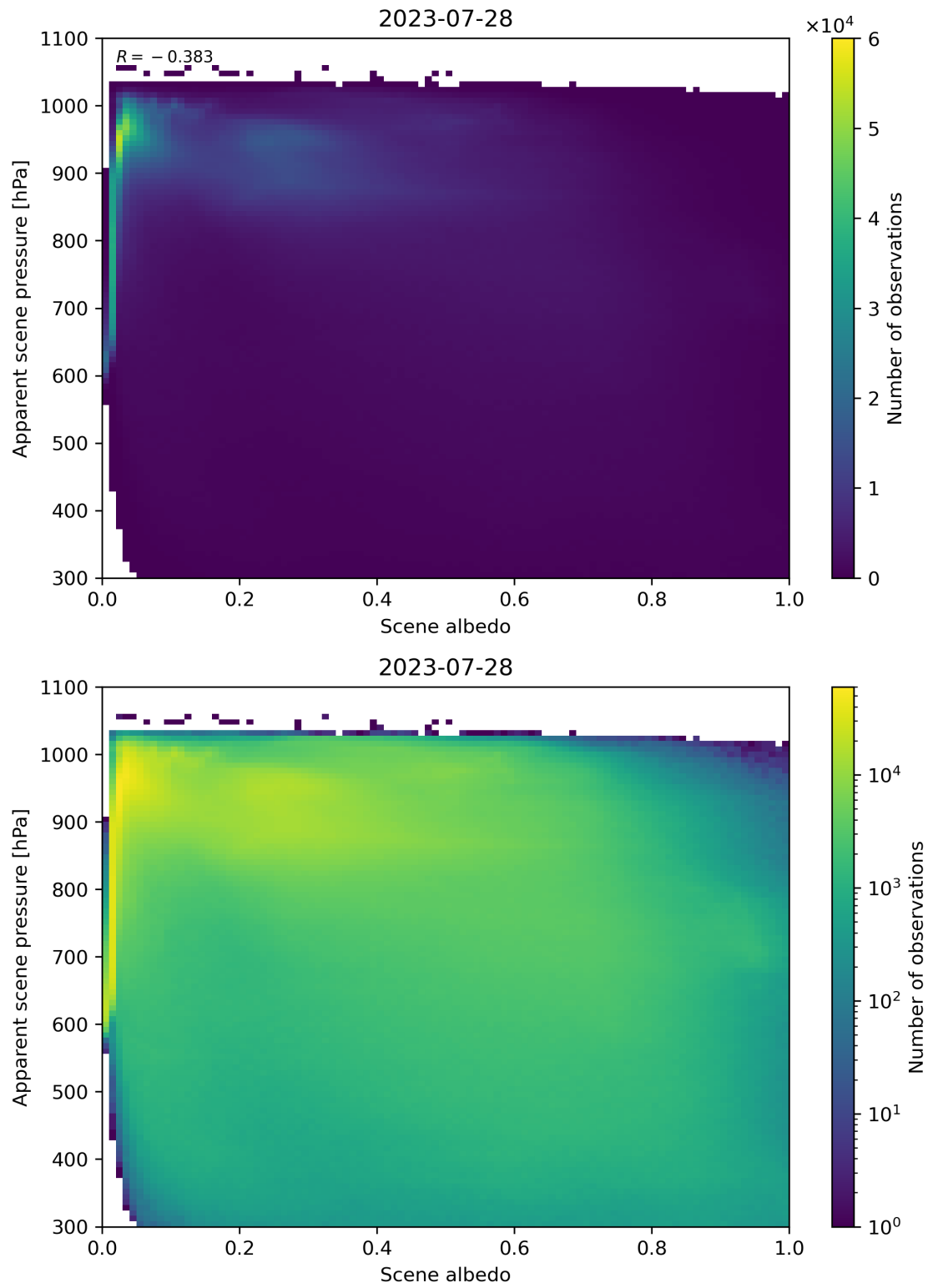
Figure 111: Scatter density plot of “Scene albedo” against “Apparent scene pressure” for 2023-07-27 to 2023-07-29.
