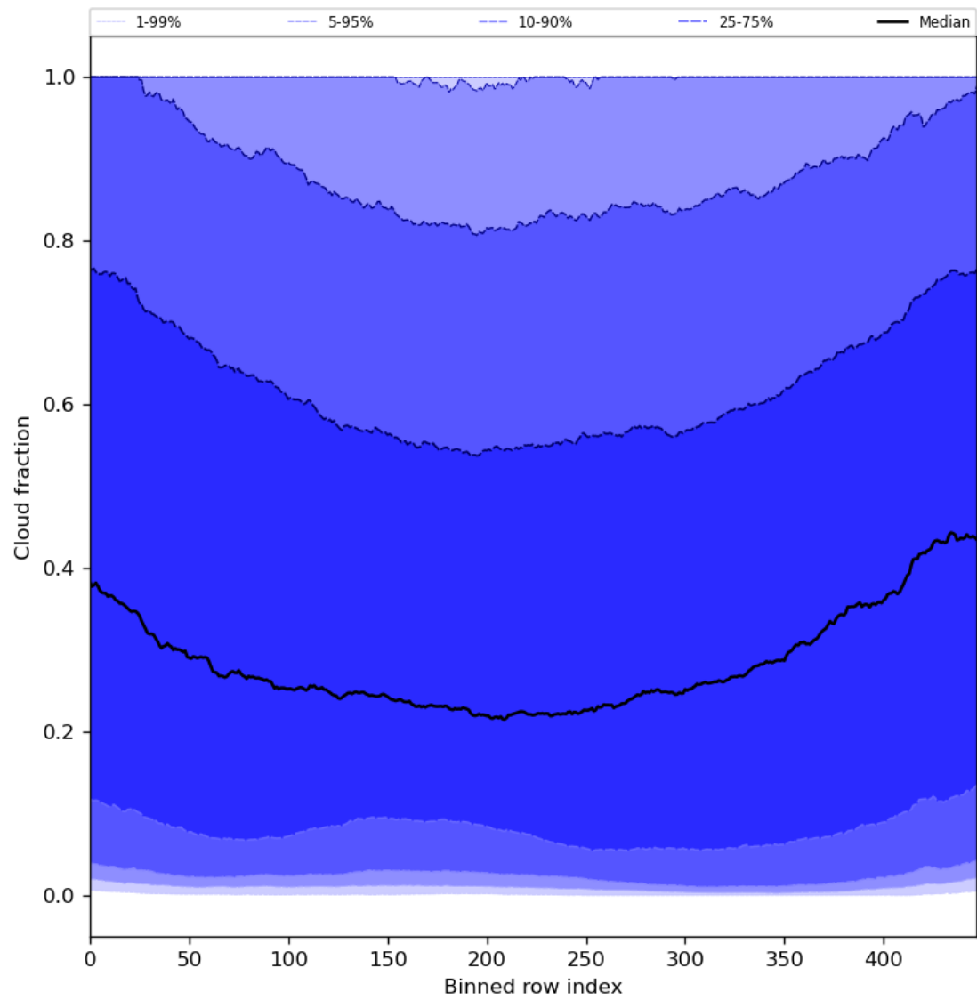
Figure 49: Along track statistics of “Cloud fraction” for 2023-07-27 to 2023-07-29
