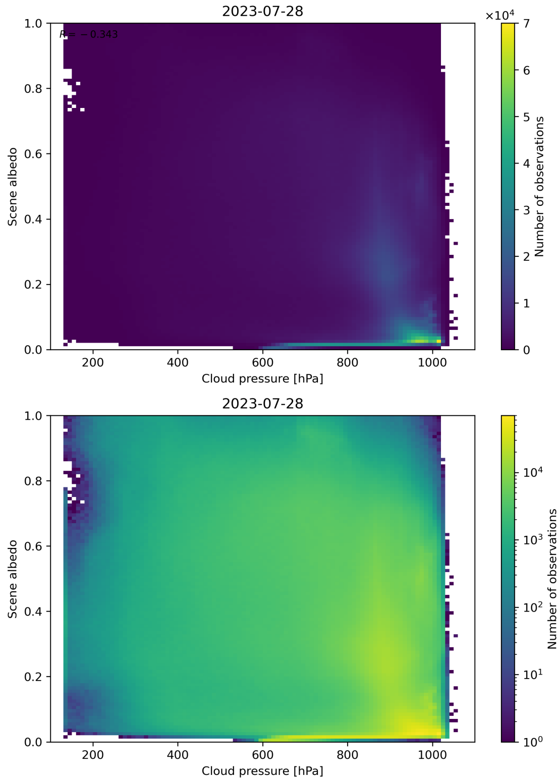
Figure 91: Scatter density plot of “Cloud pressure” against “Scene albedo” for 2023-07-27 to 2023-07-29.
