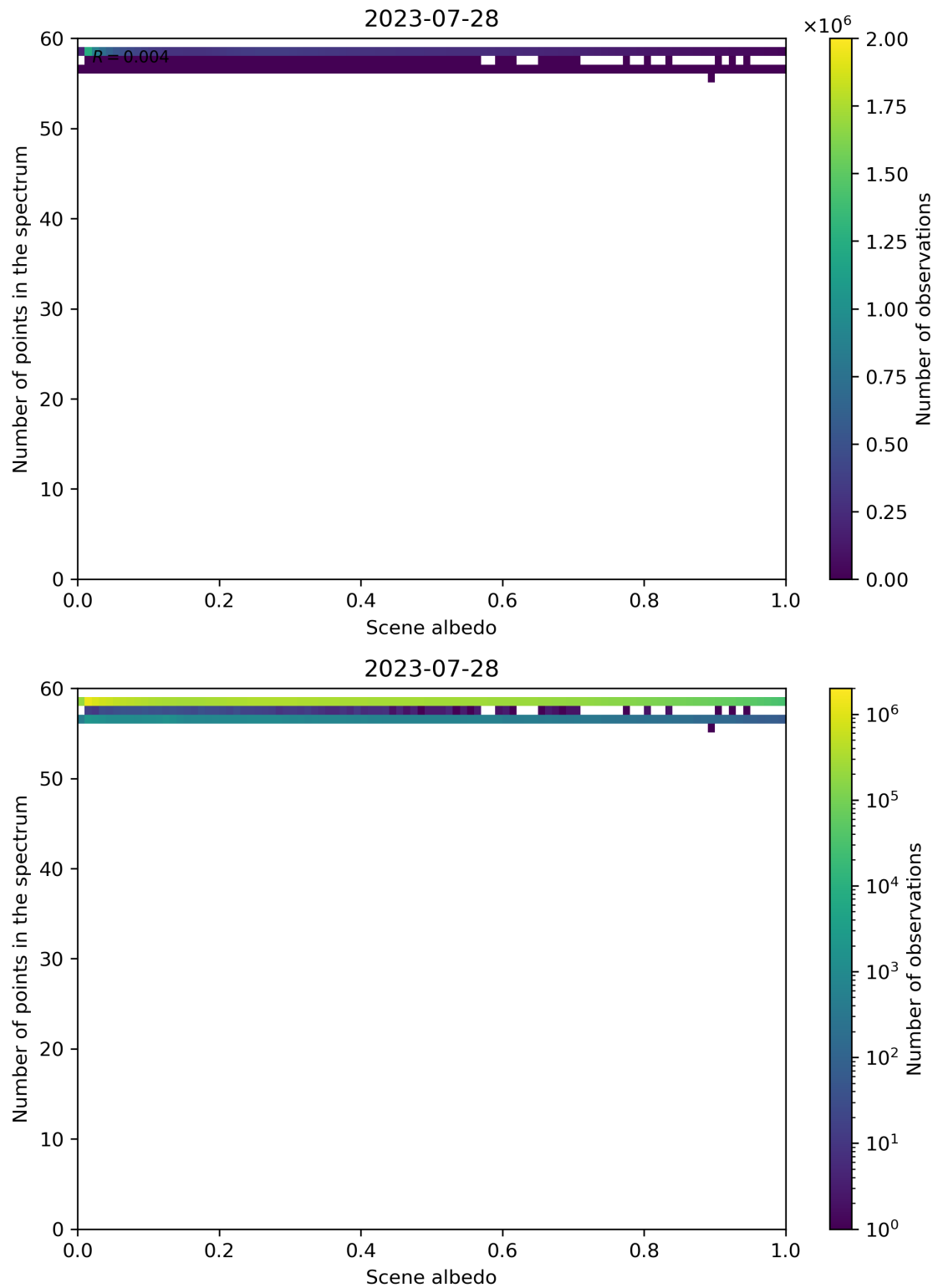
Figure 116: Scatter density plot of “Scene albedo” against “Number of points in the spectrum” for 2023-07-27 to 2023-07-29.
