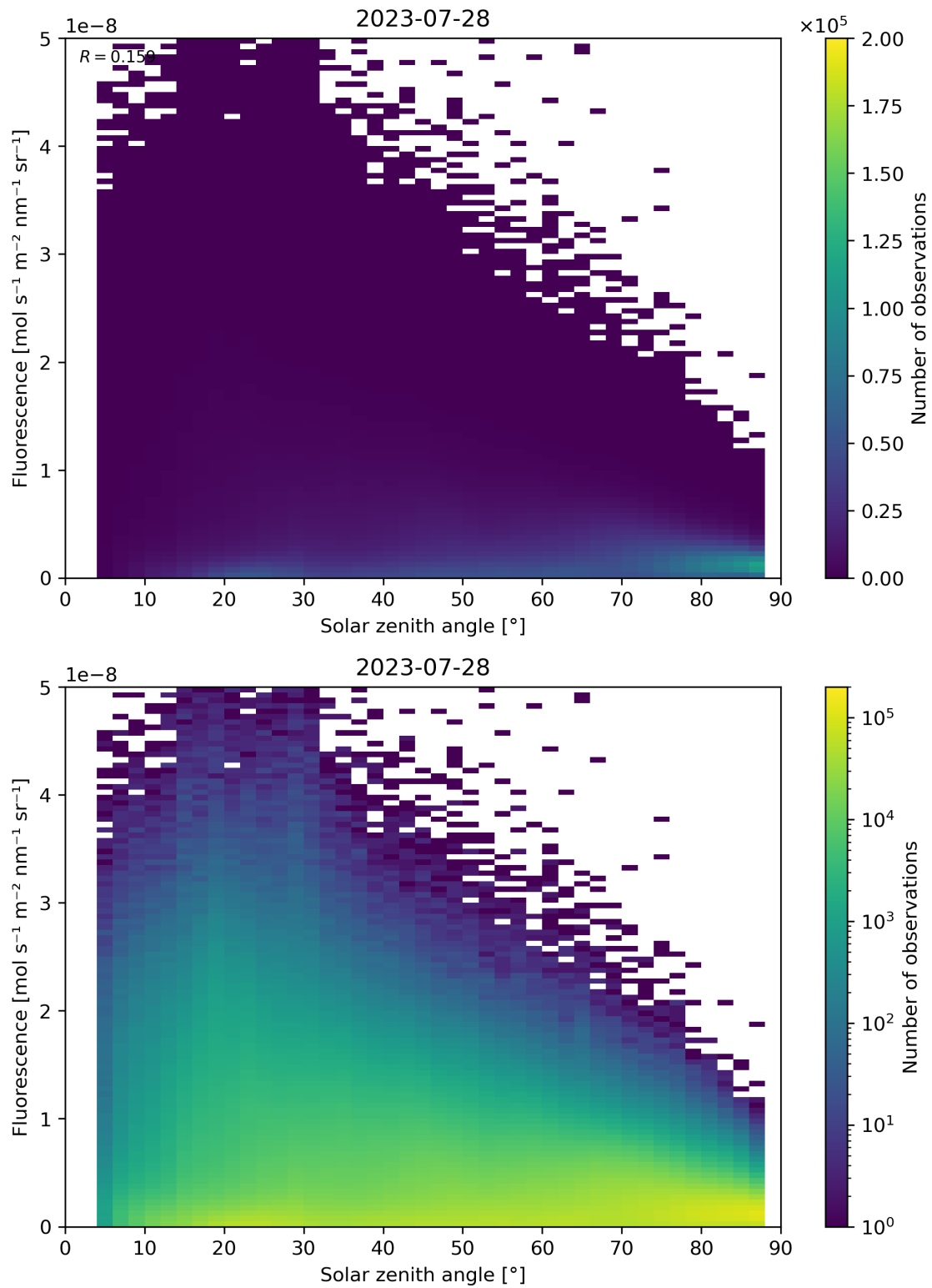
Figure 123: Scatter density plot of “Solar zenith angle” against “Fluorescence” for 2023-07-27 to 2023-07-29.
