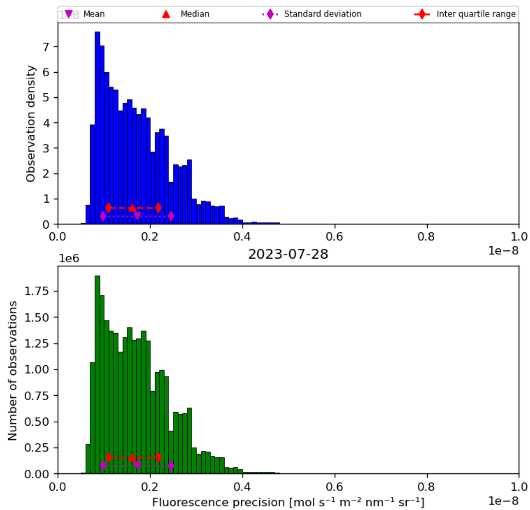
Figure 41: Histogram of “Fluorescence precision” for 2023-07-27 to 2023-07-29
