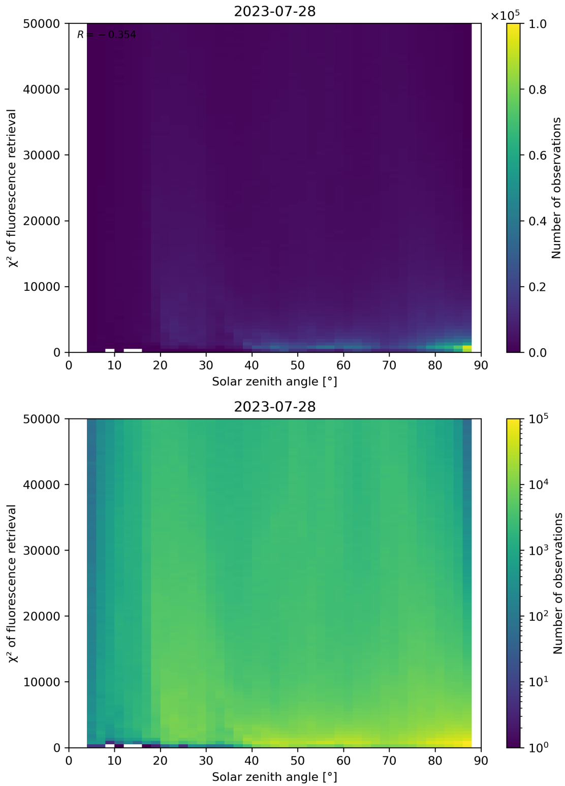
Figure 120: Scatter density plot of “Solar zenith angle” against “ \chi^2 of fluorescence retrieval” for 2023-07-27 to 2023-07-29.
