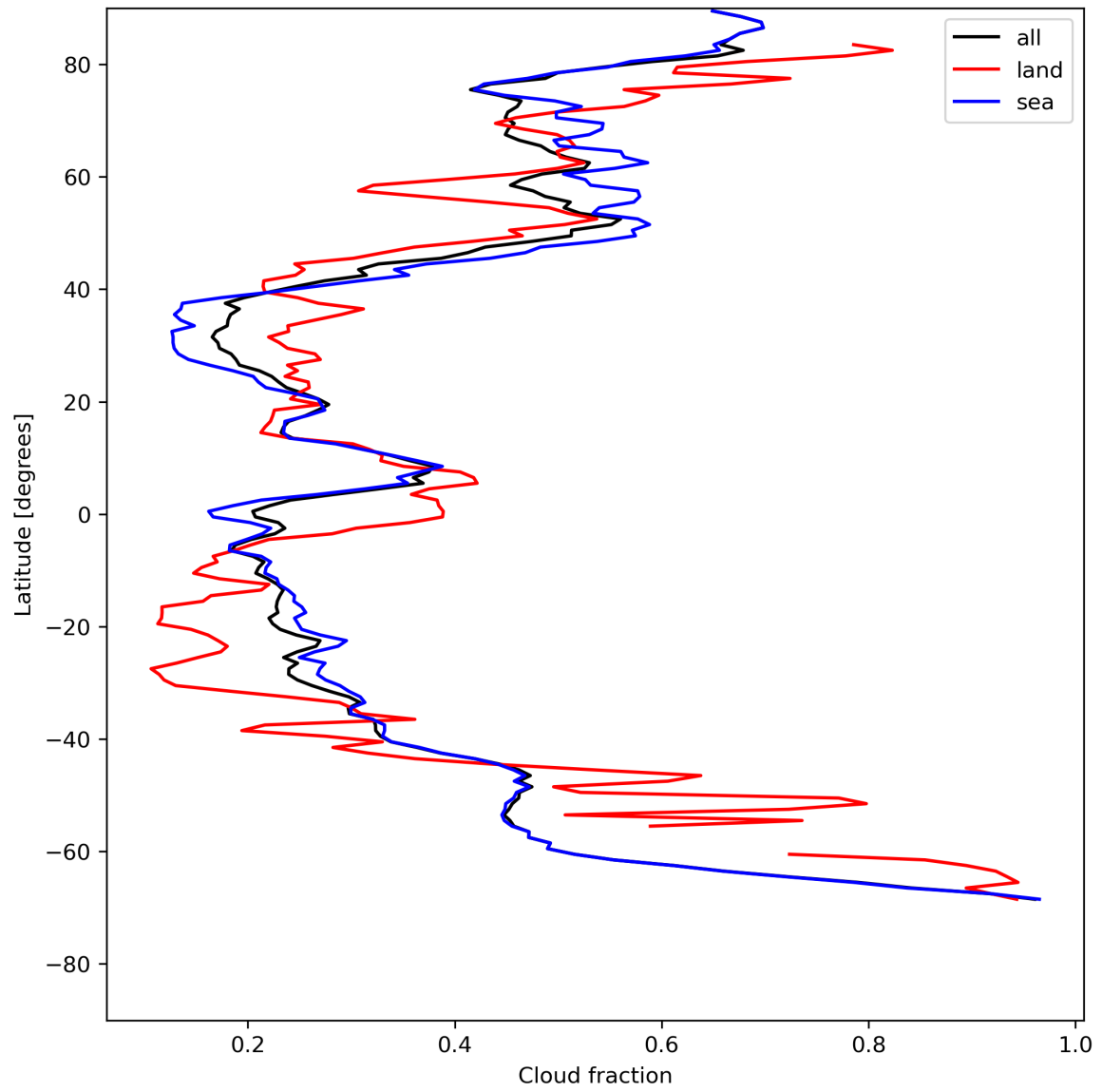
Figure 15: Zonal average of “Cloud fraction” for 2023-07-27 to 2023-07-29.
