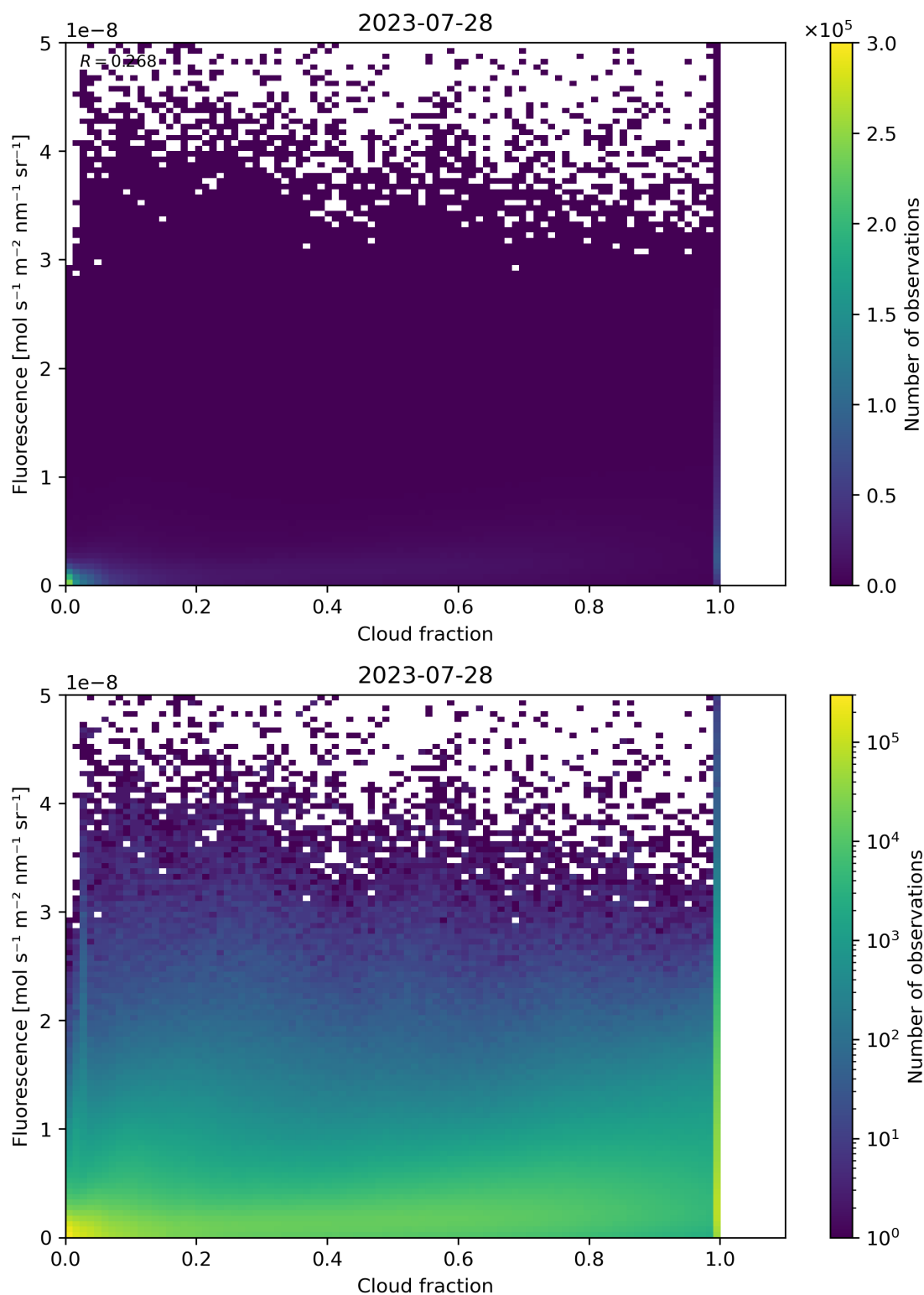
Figure 79: Scatter density plot of “Cloud fraction” against “Fluorescence” for 2023-07-27 to 2023-07-29.
