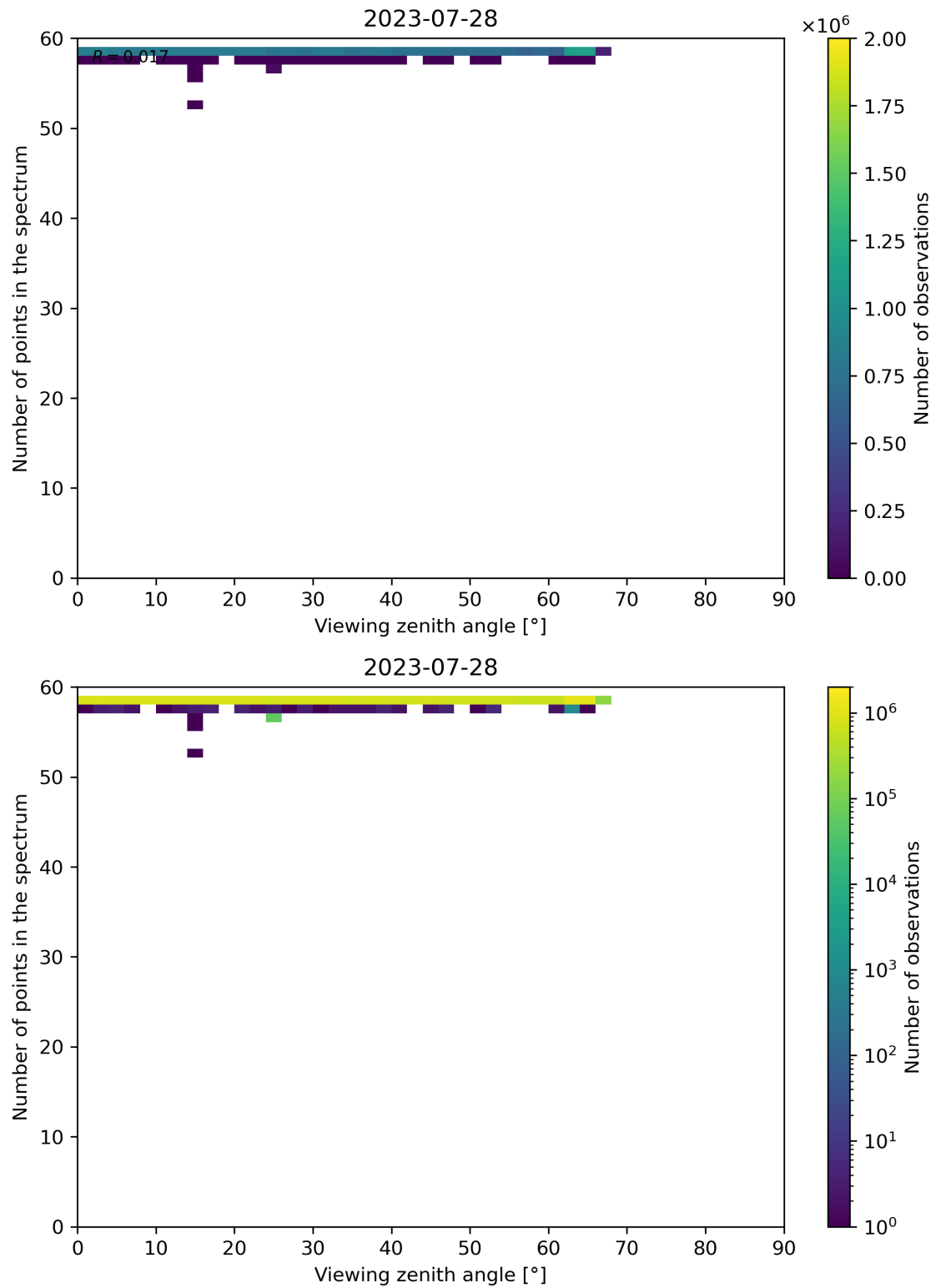
Figure 137: Scatter density plot of “Viewing zenith angle” against “Number of points in the spectrum” for 2023-07-27 to 2023-07-29.
