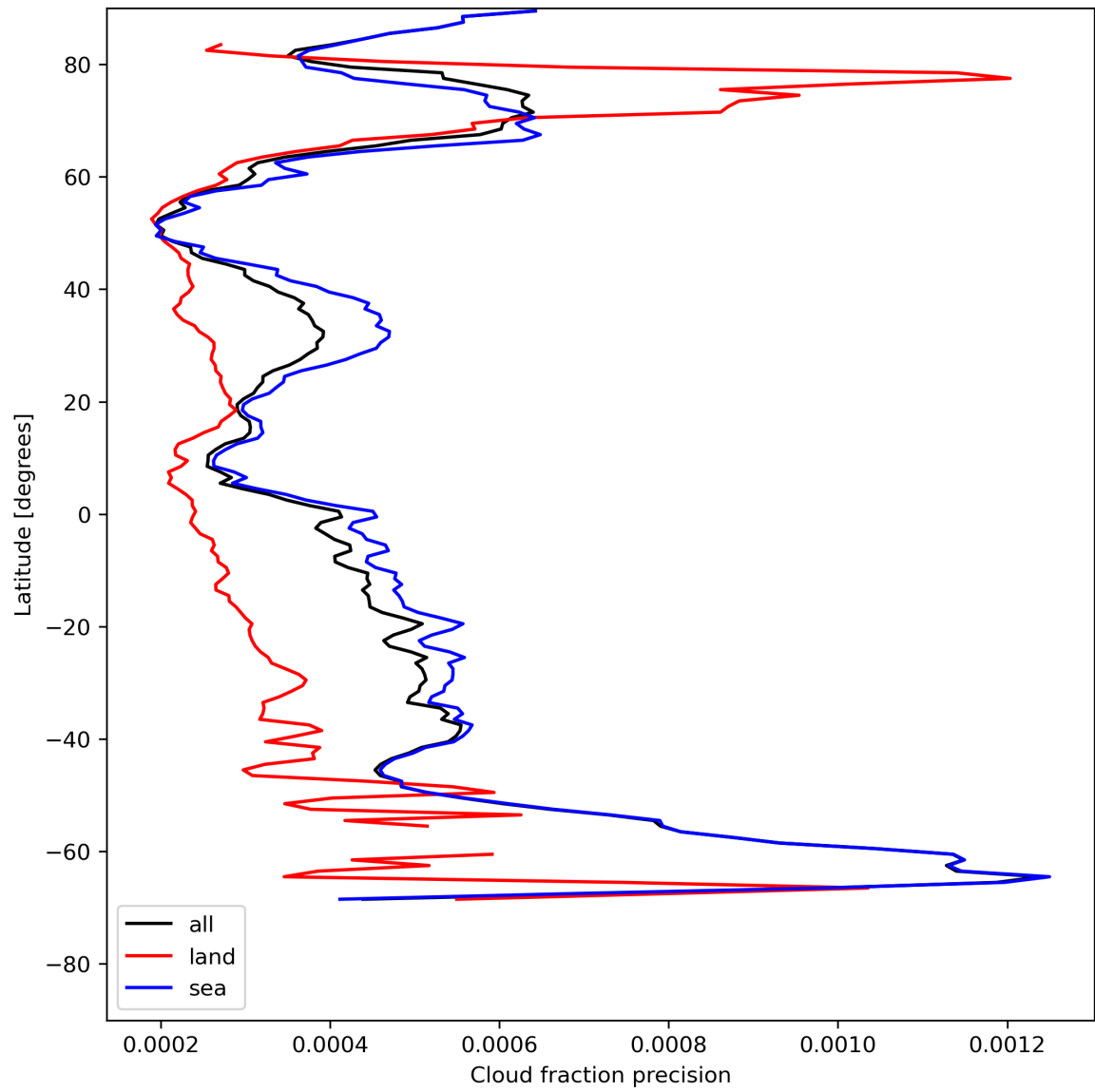
Figure 16: Zonal average of “Cloud fraction precision” for 2023-07-27 to 2023-07-29.
