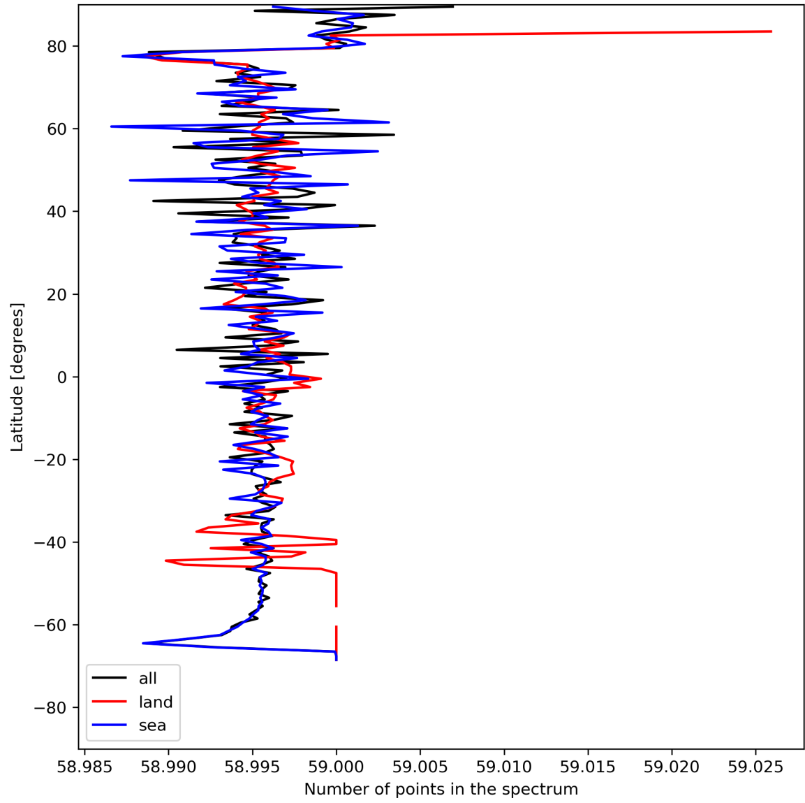
Figure 27: Zonal average of “Number of points in the spectrum” for 2023-07-27 to 2023-07-29.
