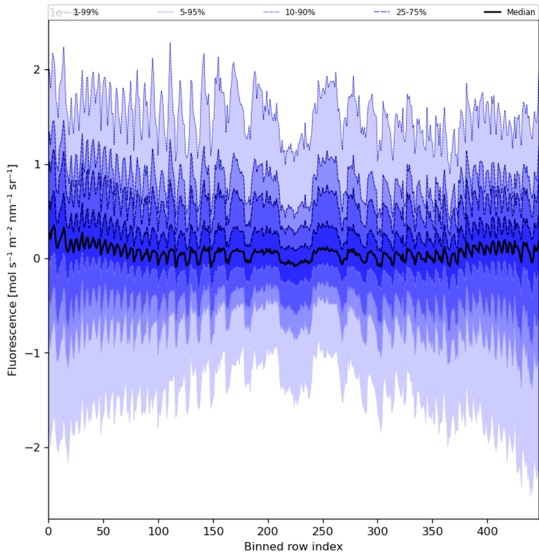
Figure 57: Along track statistics of “Fluorescence” for 2023-07-27 to 2023-07-29
