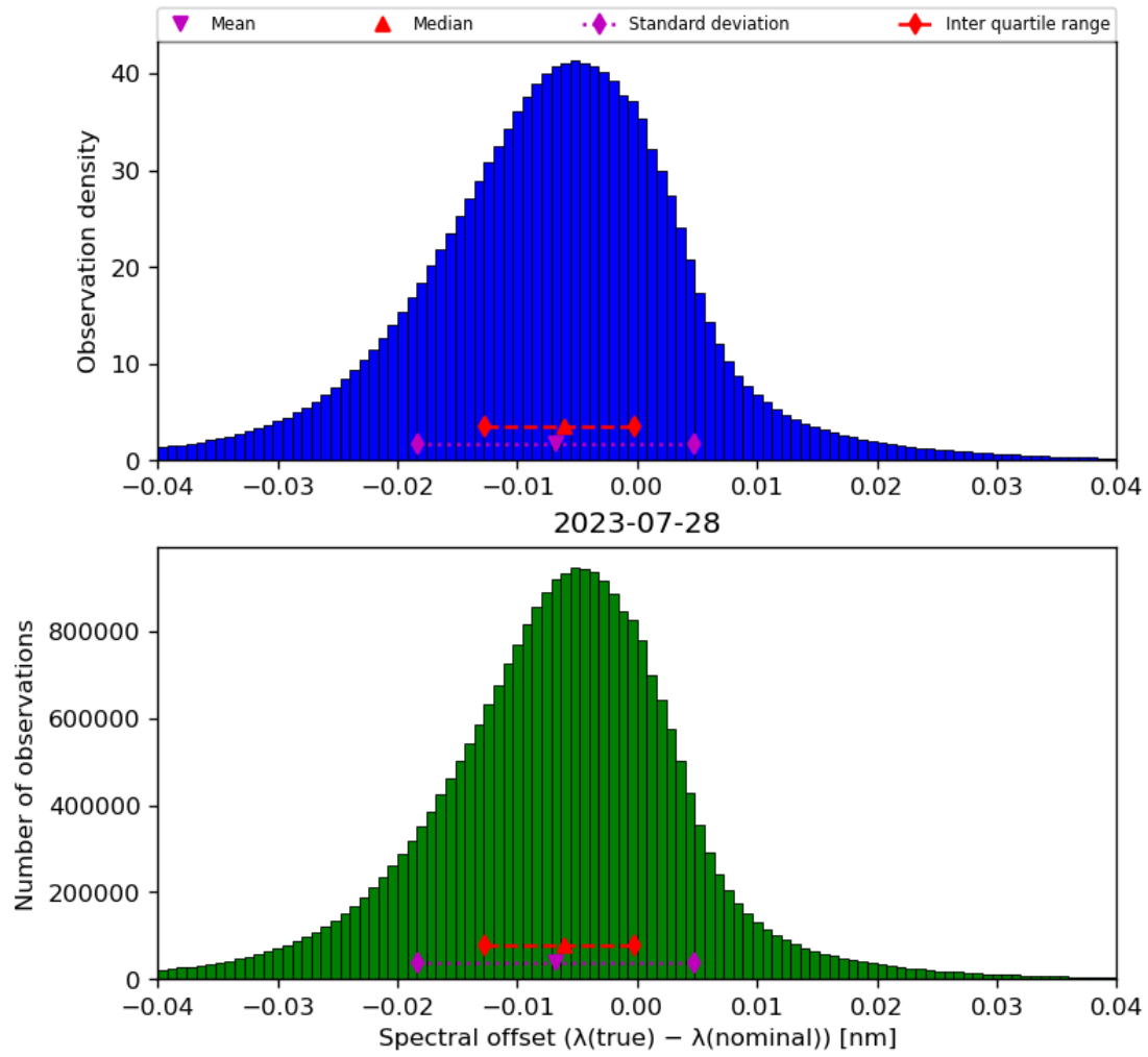
Figure 45: Histogram of “Spectral offset ( \lambda(\text{true}) - \lambda(\text{nominal}) )” for 2023-07-27 to 2023-07-29
