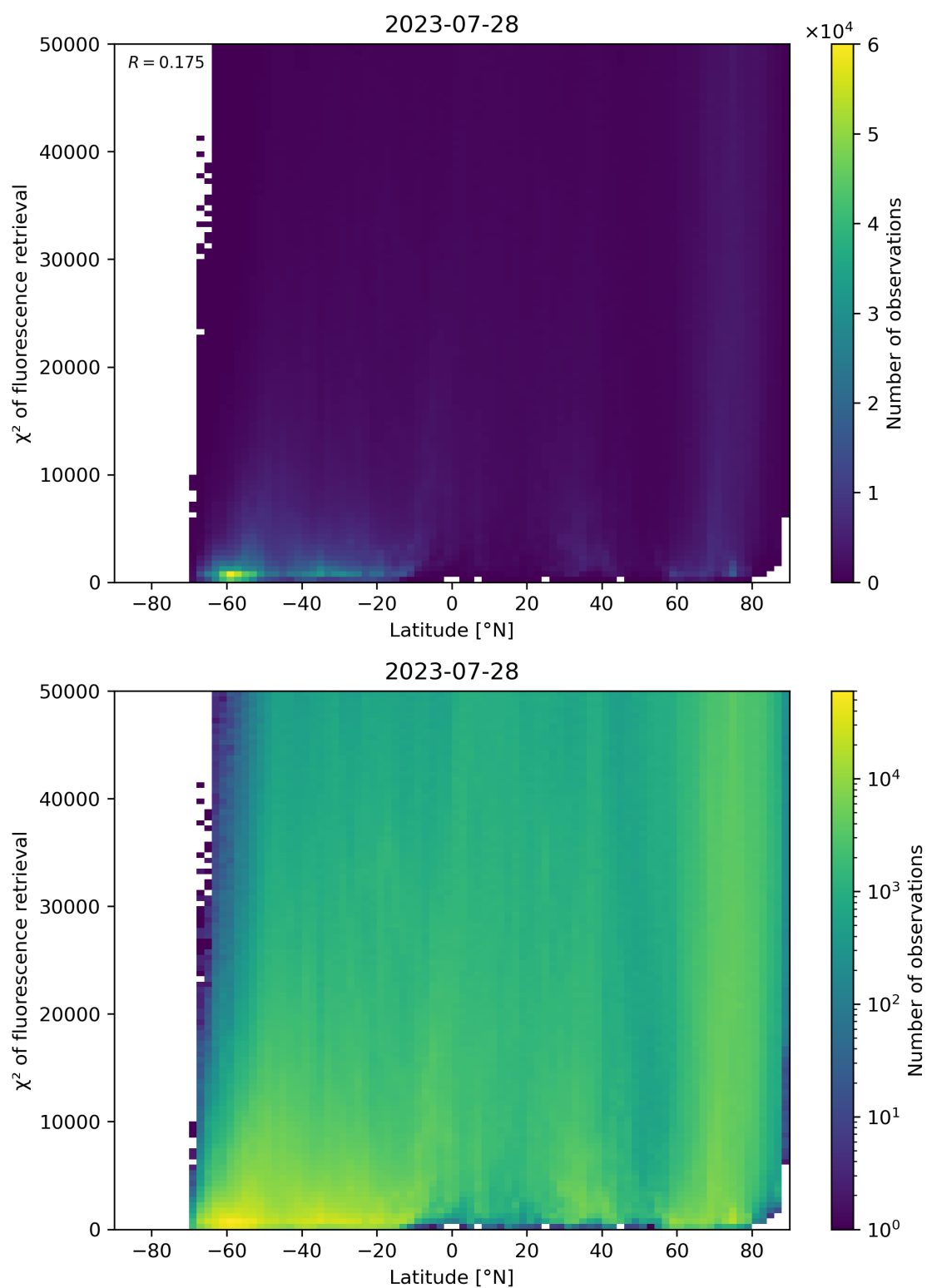
Figure 98: Scatter density plot of “Latitude” against “ \chi^2 of fluorescence retrieval” for 2023-07-27 to 2023-07-29.
