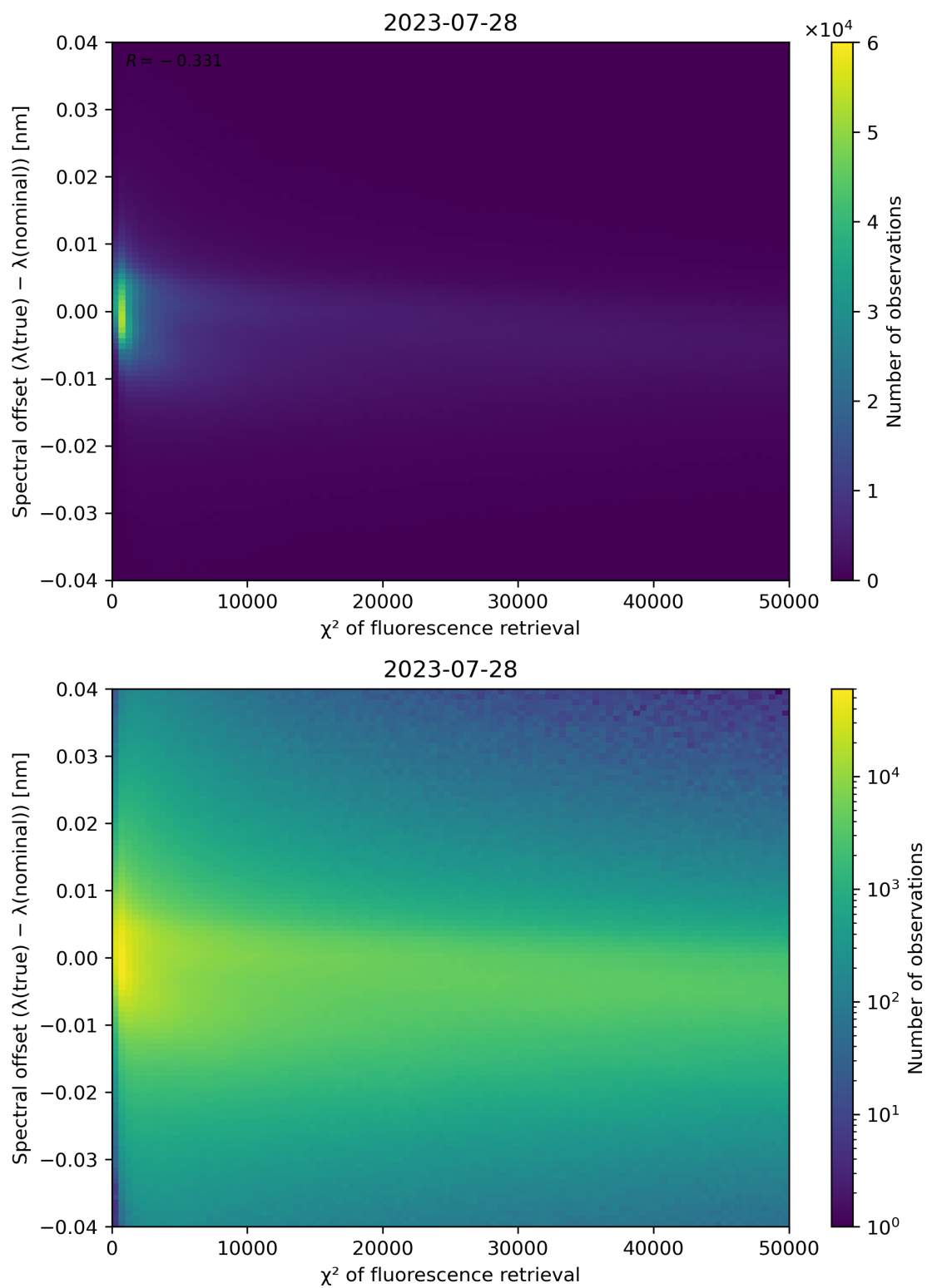
Figure 72: Scatter density plot of " \chi^2 of fluorescence retrieval" against "Spectral offset ( \lambda(\text{true}) - \lambda(\text{nominal}) )" for 2023-07-27 to 2023-07-29.
