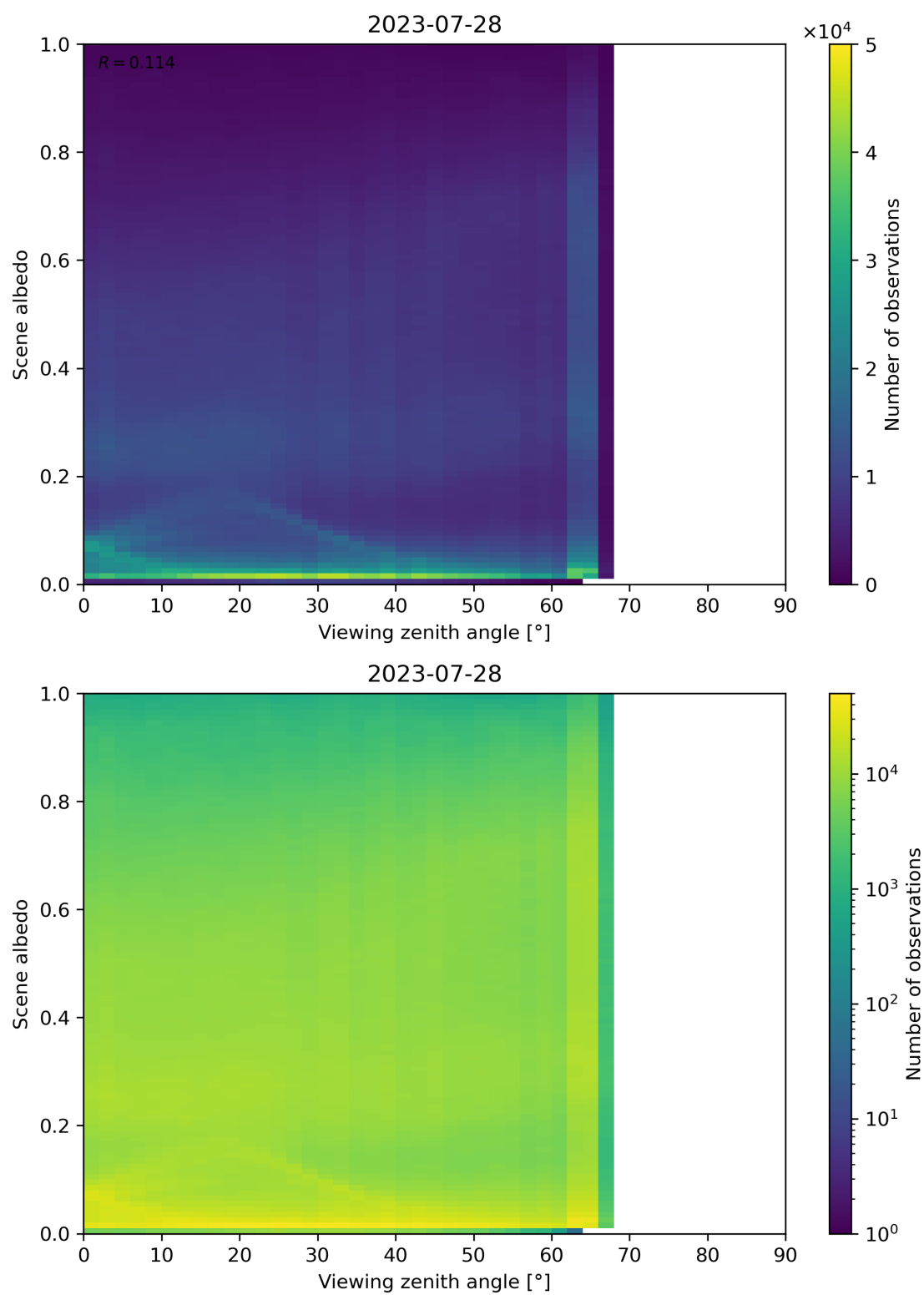
Figure 138: Scatter density plot of “Viewing zenith angle” against “Scene albedo” for 2023-07-27 to 2023-07-29.
