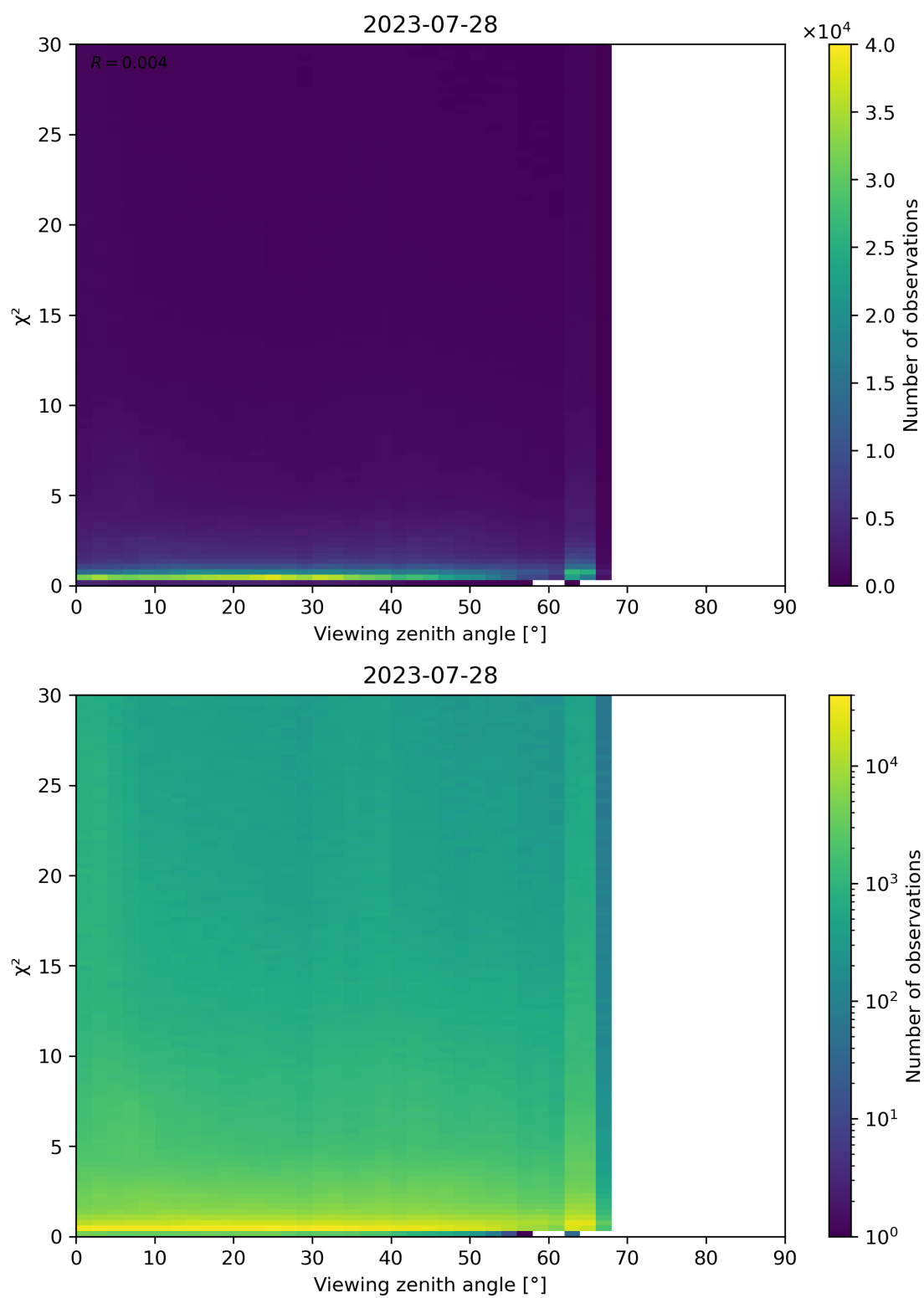
Figure 130: Scatter density plot of “Viewing zenith angle” against “ \chi^2 ” for 2023-07-27 to 2023-07-29.
