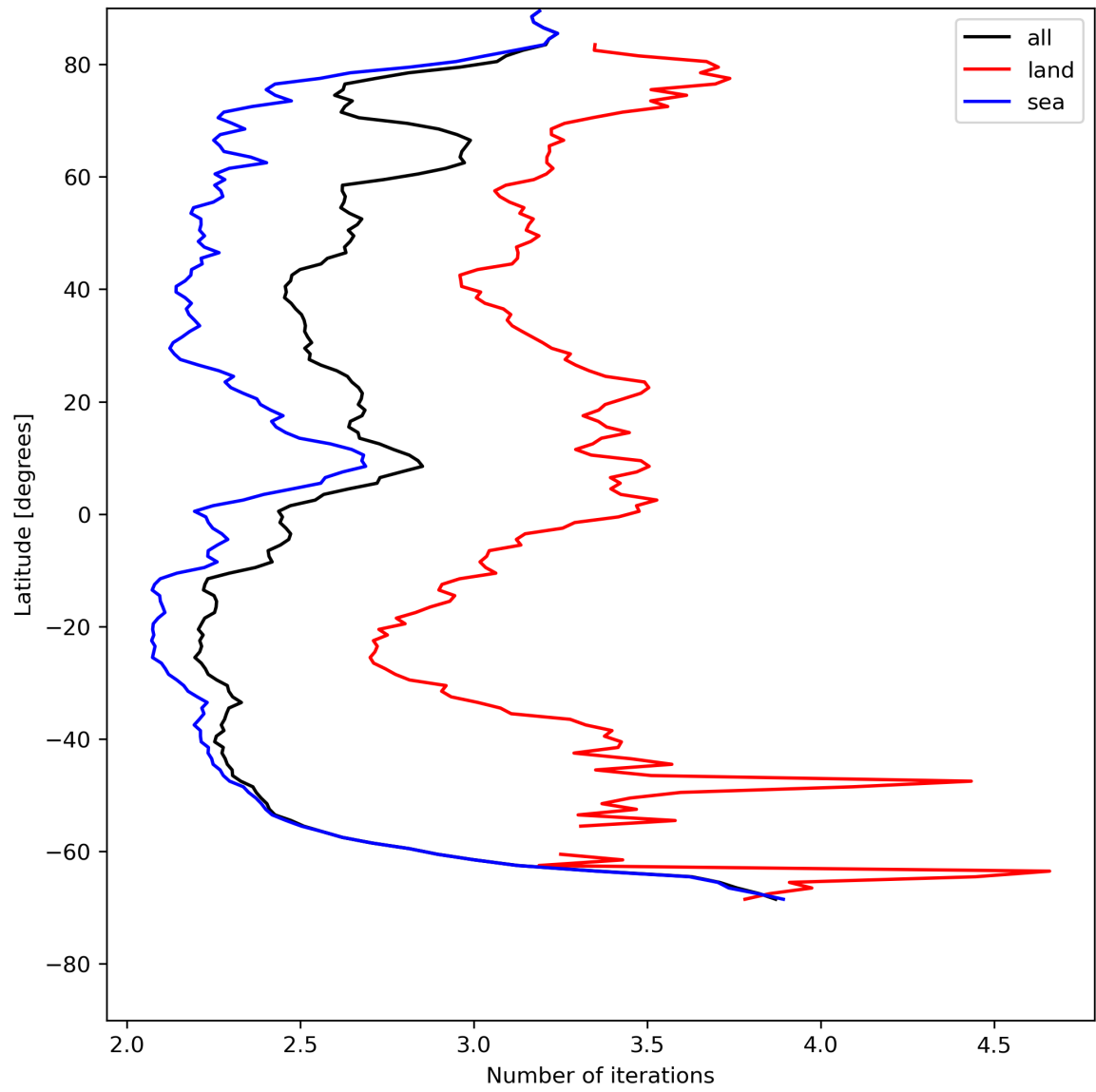
Figure 22: Zonal average of “Number of iterations” for 2023-07-27 to 2023-07-29.
