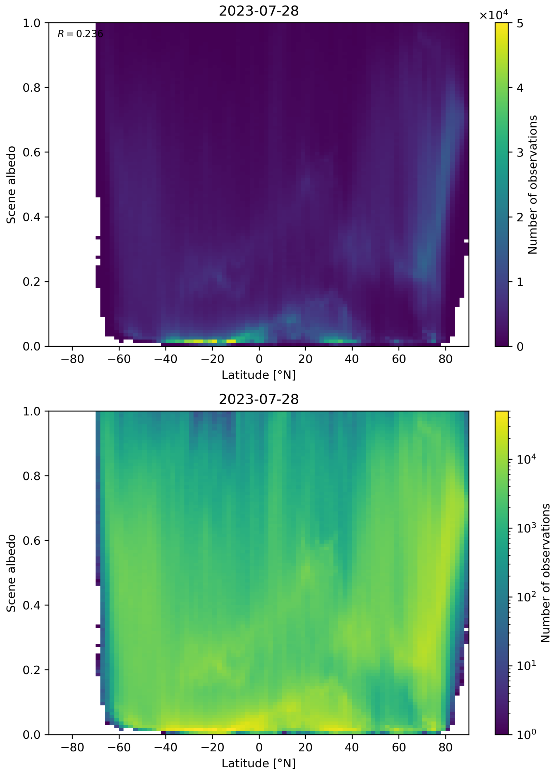
Figure 104: Scatter density plot of “Latitude” against “Scene albedo” for 2023-07-27 to 2023-07-29.
