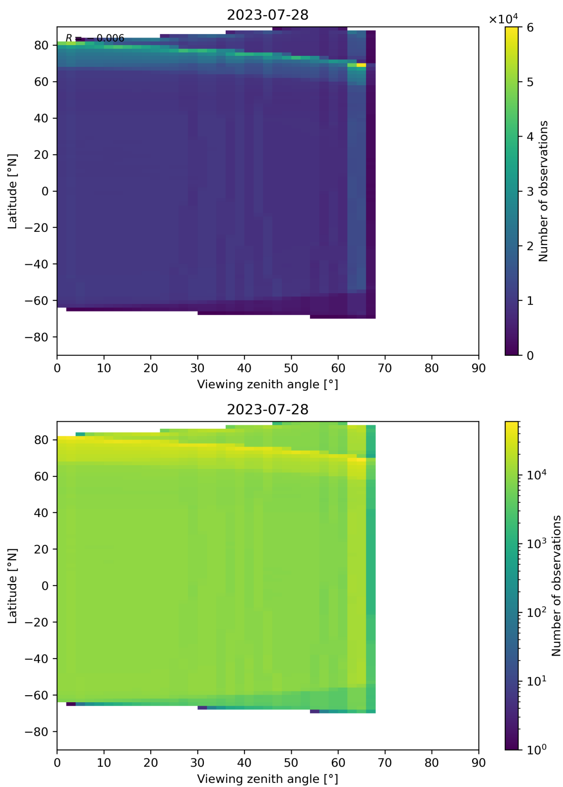
Figure 135: Scatter density plot of “Viewing zenith angle” against “Latitude” for 2023-07-27 to 2023-07-29.
