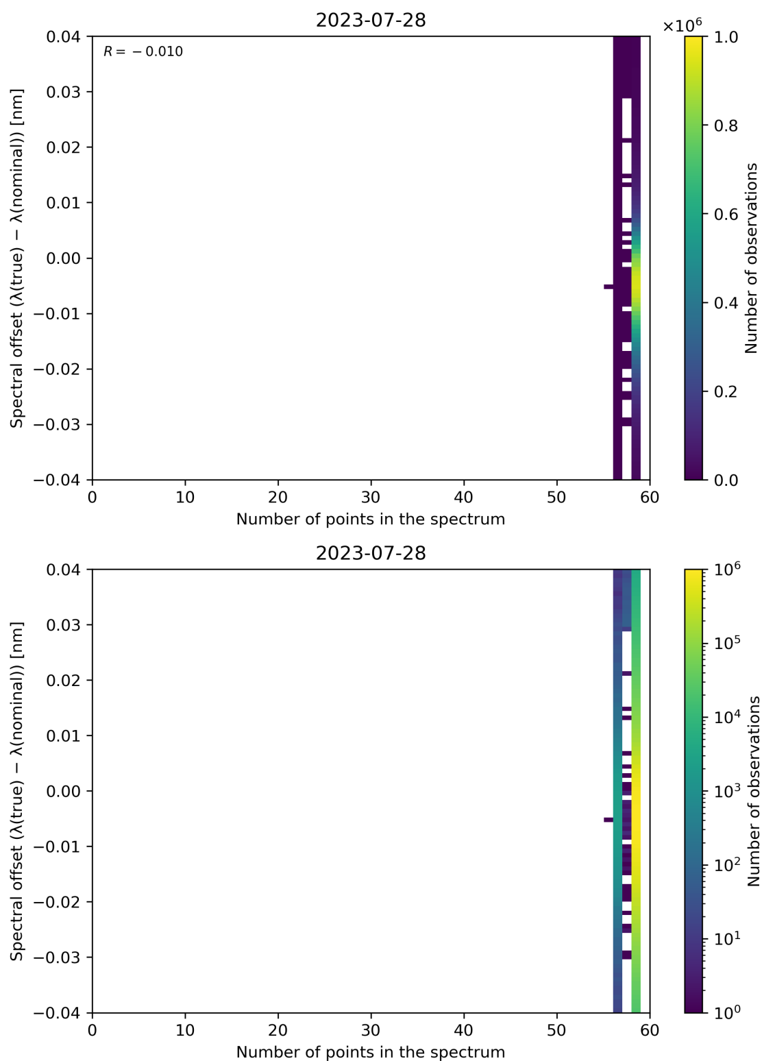
Figure 110: Scatter density plot of “Number of points in the spectrum” against “Spectral offset ( \lambda(\text{true}) - \lambda(\text{nominal}) )” for 2023-07-27 to 2023-07-29.
