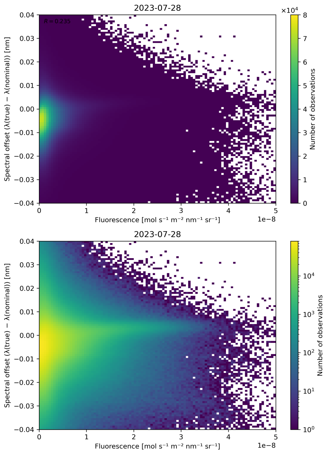
Figure 95: Scatter density plot of “Fluorescence” against “Spectral offset ( \lambda(\text{true}) - \lambda(\text{nominal}) )” for 2023-07-27 to 2023-07-29.
