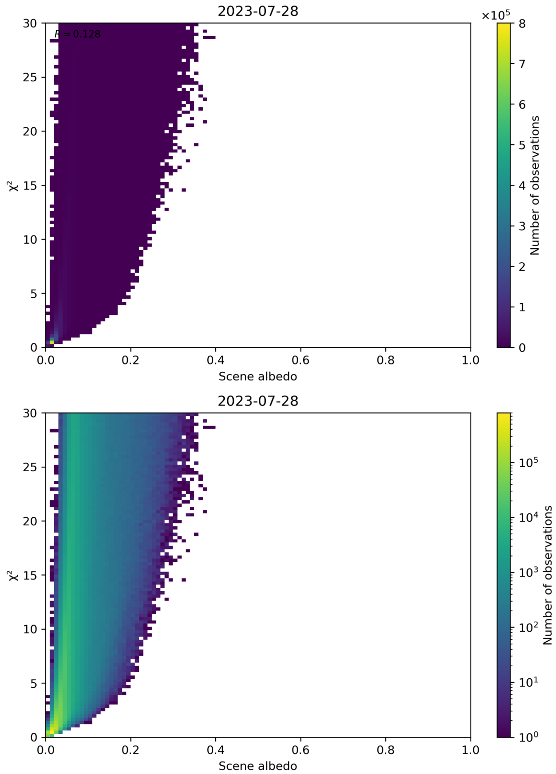
Figure 112: Scatter density plot of “Scene albedo” against “ \chi^2 ” for 2023-07-27 to 2023-07-29.
