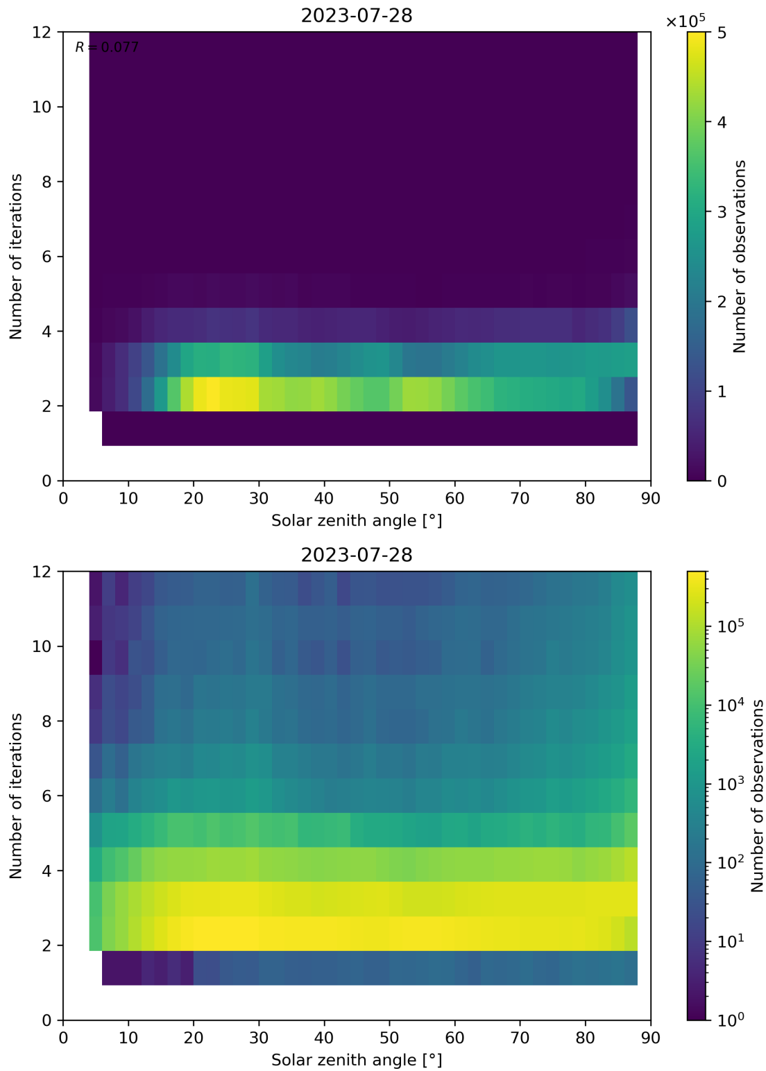
Figure 125: Scatter density plot of “Solar zenith angle” against “Number of iterations” for 2023-07-27 to 2023-07-29.
