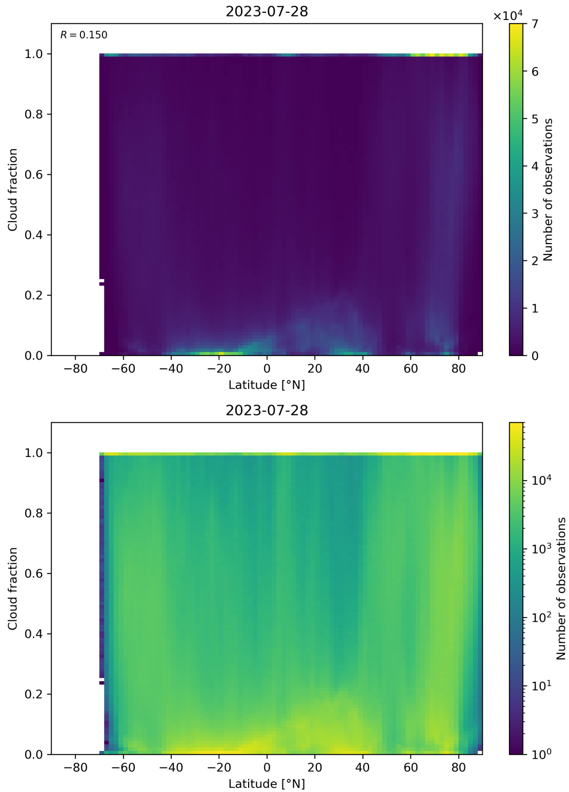
Figure 99: Scatter density plot of “Latitude” against “Cloud fraction” for 2023-07-27 to 2023-07-29.
