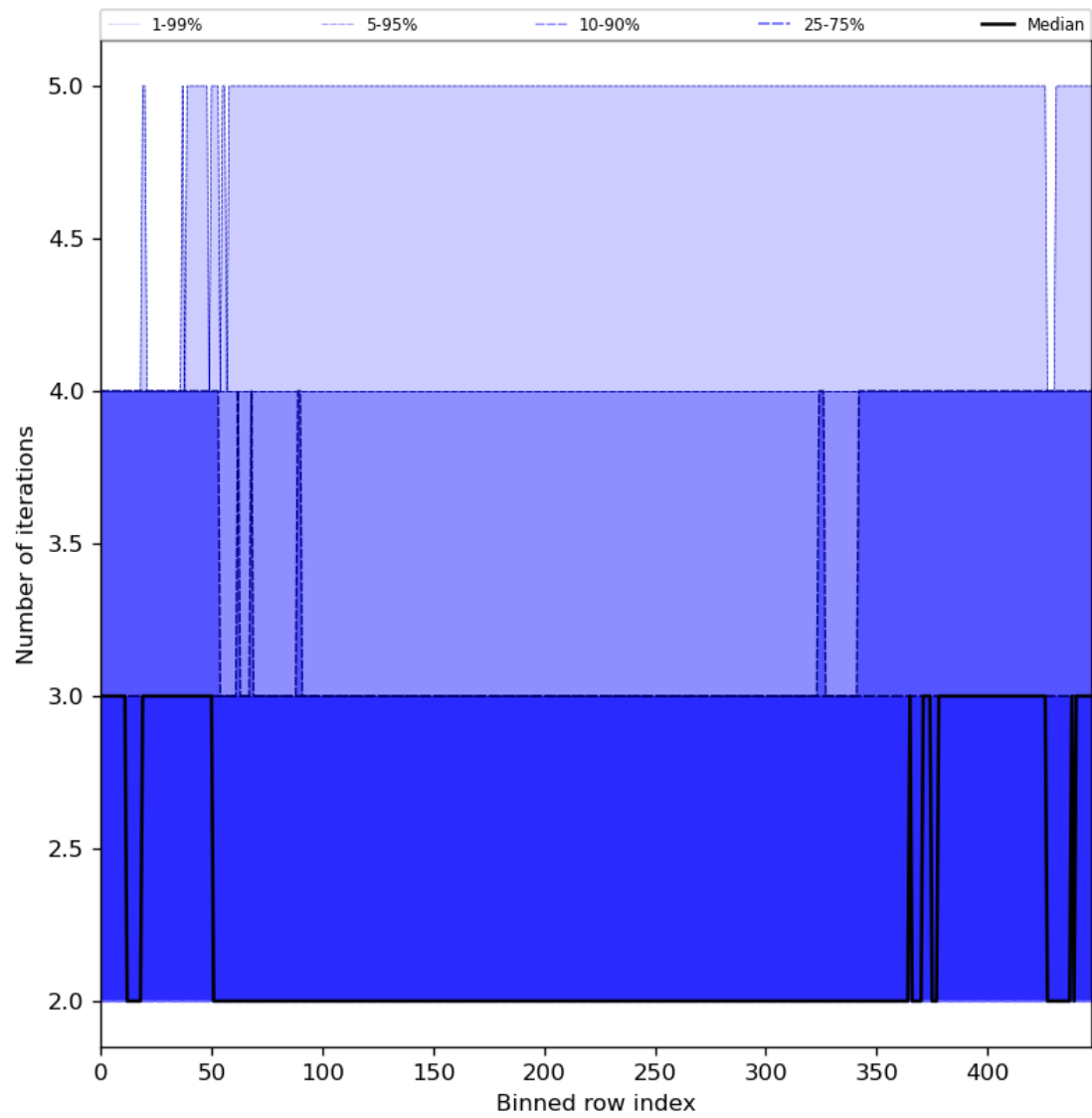
Figure 56: Along track statistics of “Number of iterations” for 2023-07-27 to 2023-07-29
