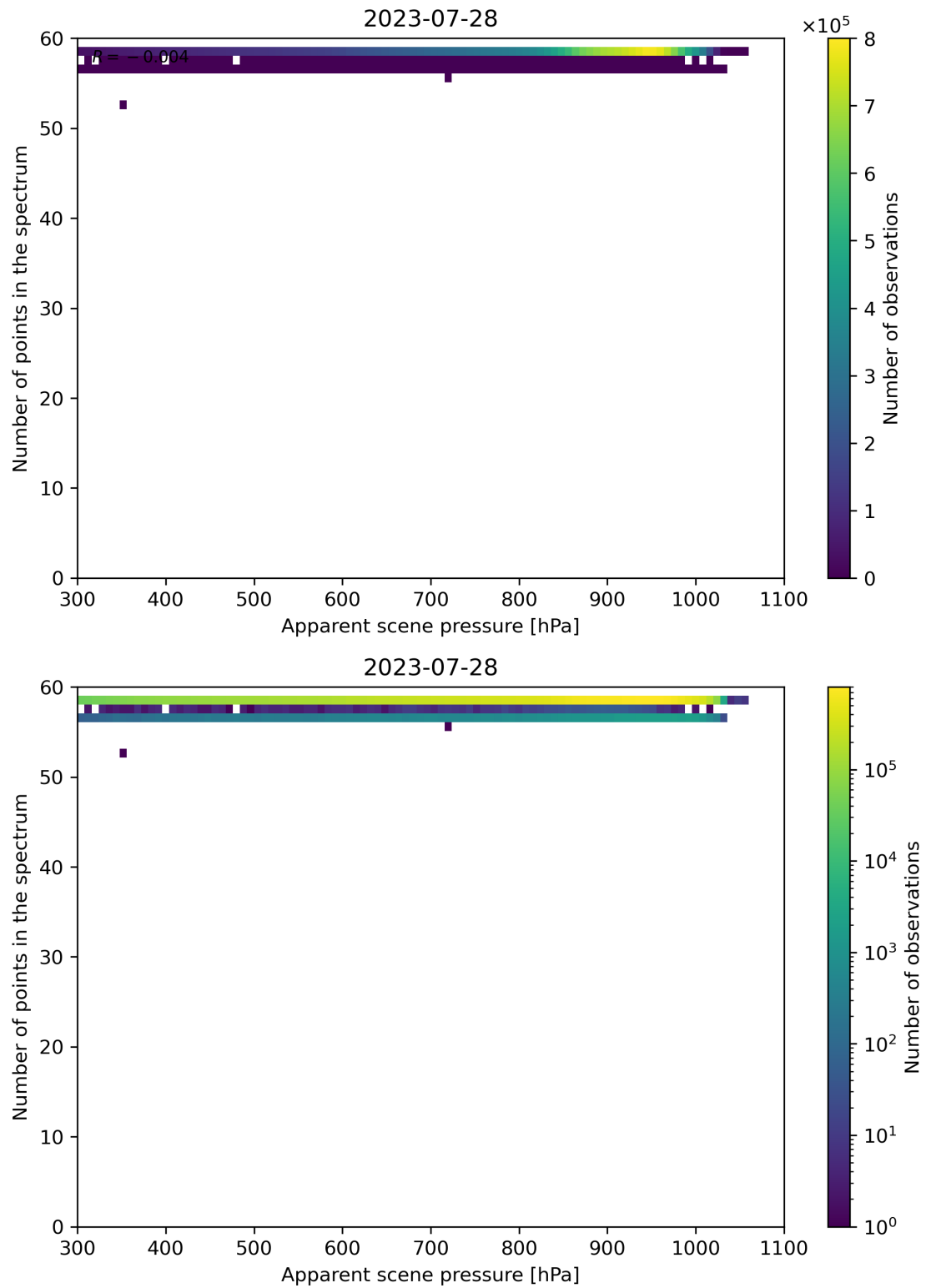
Figure 67: Scatter density plot of “Apparent scene pressure” against “Number of points in the spectrum” for 2023-07-27 to 2023-07-29.
