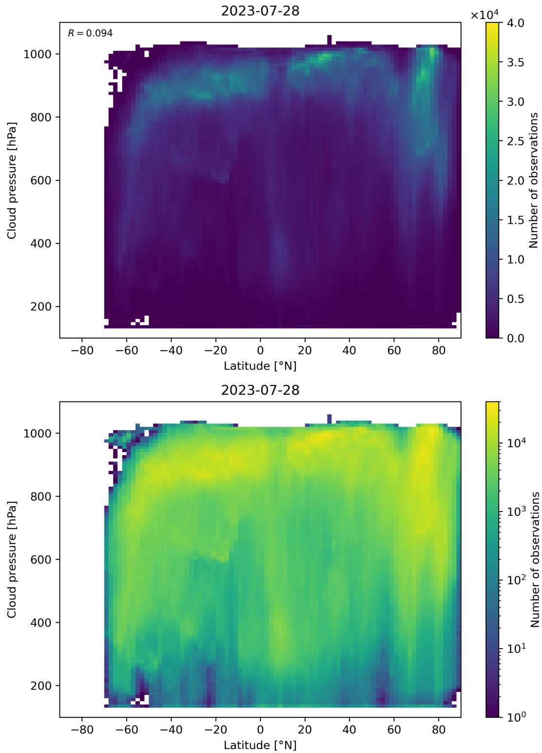
Figure 100: Scatter density plot of “Latitude” against “Cloud pressure” for 2023-07-27 to 2023-07-29.
