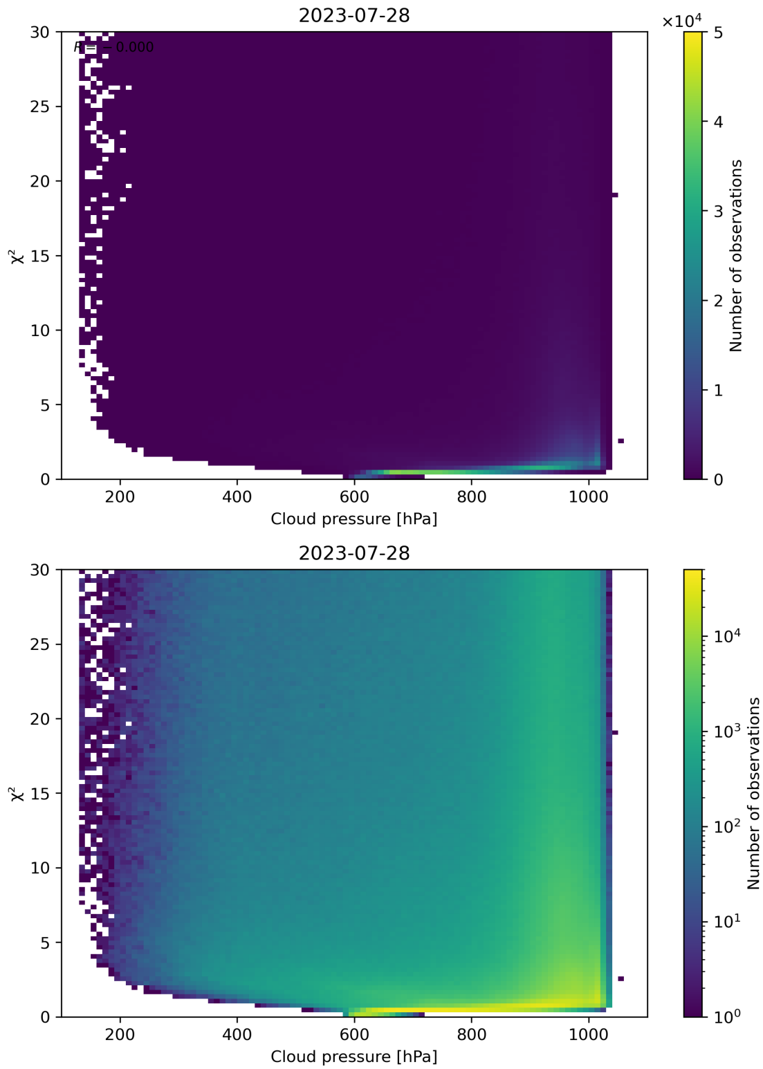
Figure 85: Scatter density plot of “Cloud pressure” against “ \chi^2 ” for 2023-07-27 to 2023-07-29.
