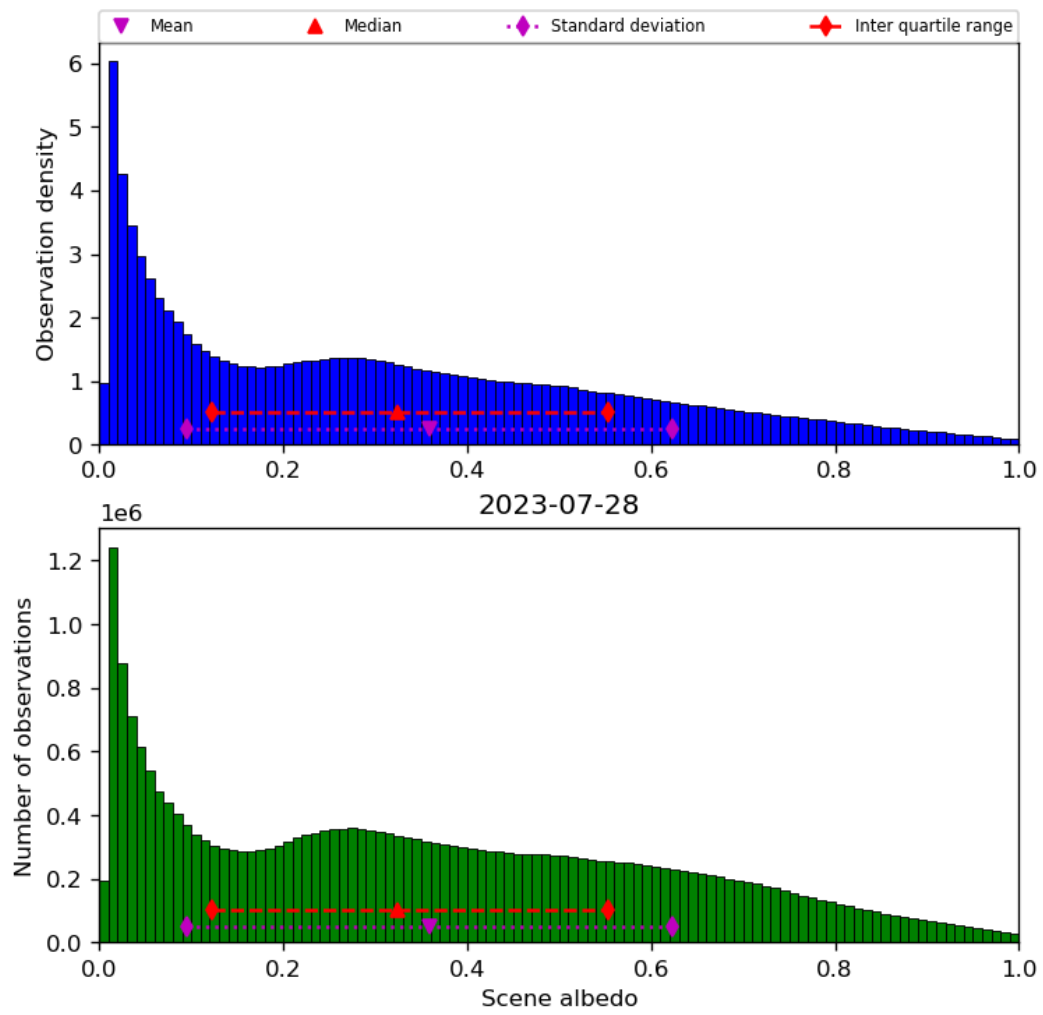
Figure 34: Histogram of "Scene albedo" for 2023-07-27 to 2023-07-29
