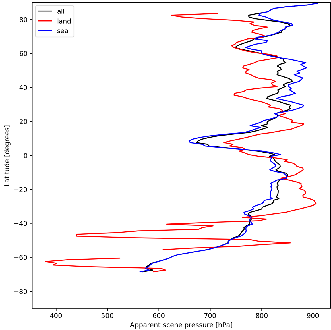
Figure 19: Zonal average of “Apparent scene pressure” for 2023-07-27 to 2023-07-29.
