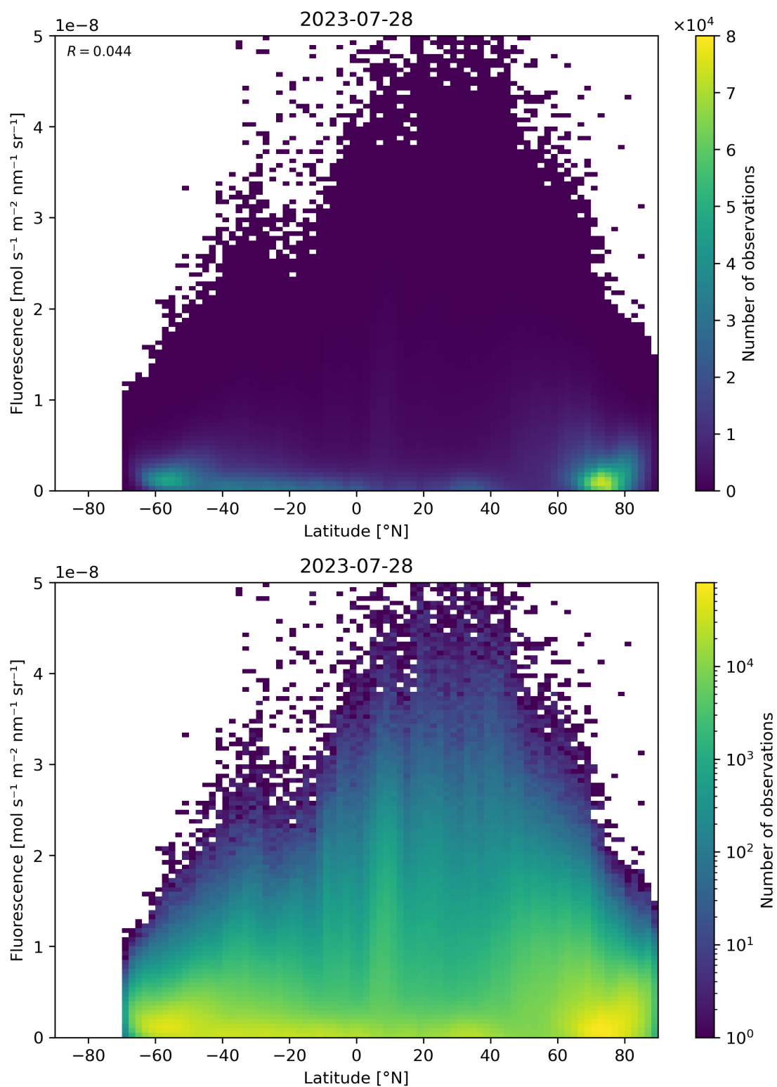
Figure 101: Scatter density plot of “Latitude” against “Fluorescence” for 2023-07-27 to 2023-07-29.
