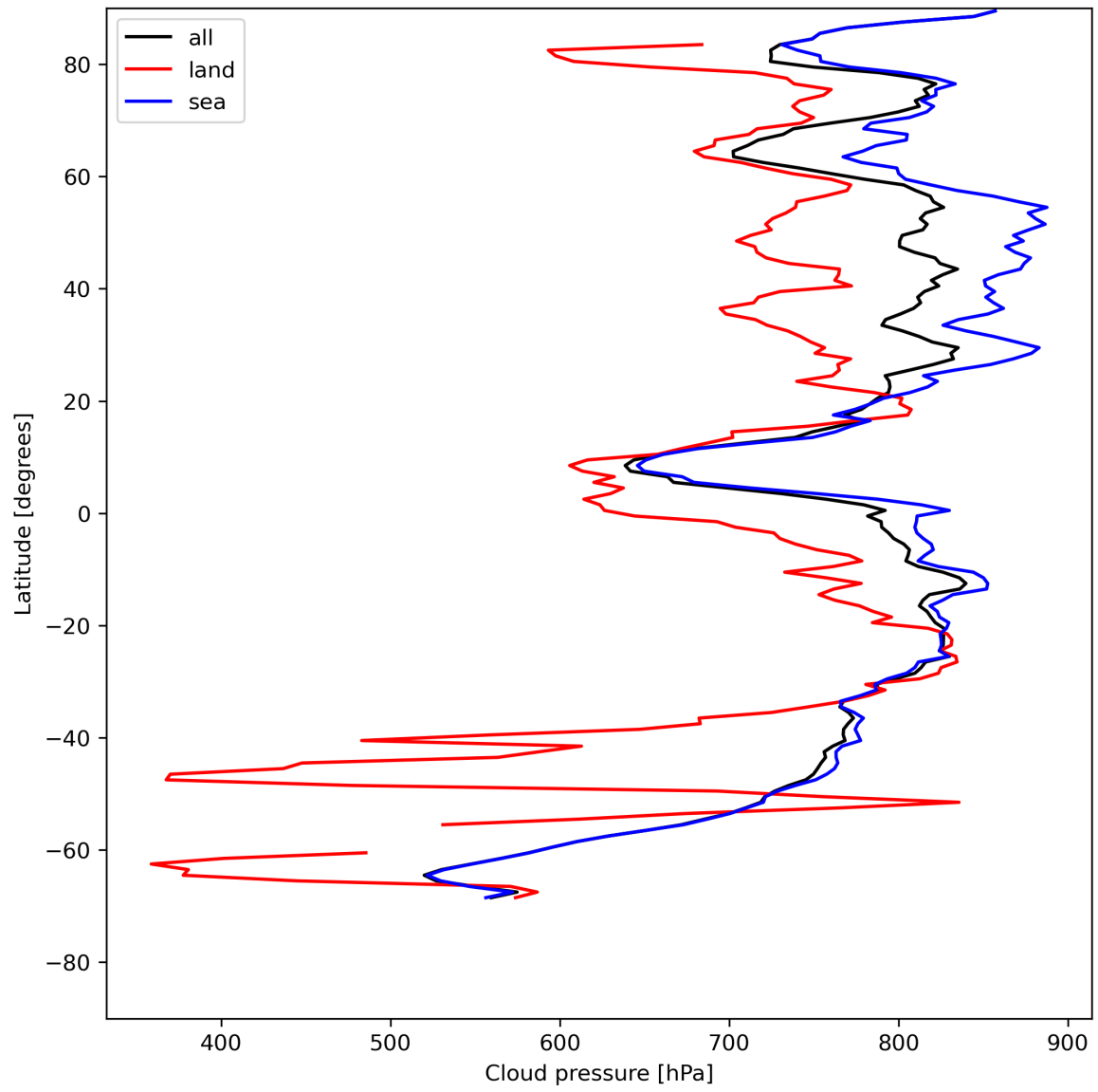
Figure 13: Zonal average of “Cloud pressure” for 2023-07-27 to 2023-07-29.
