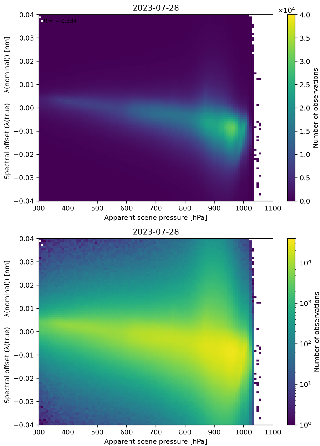
Figure 68: Scatter density plot of “Apparent scene pressure” against “Spectral offset ( \lambda(\text{true}) - \lambda(\text{nominal}) )” for 2023-07-27 to 2023-07-29.
