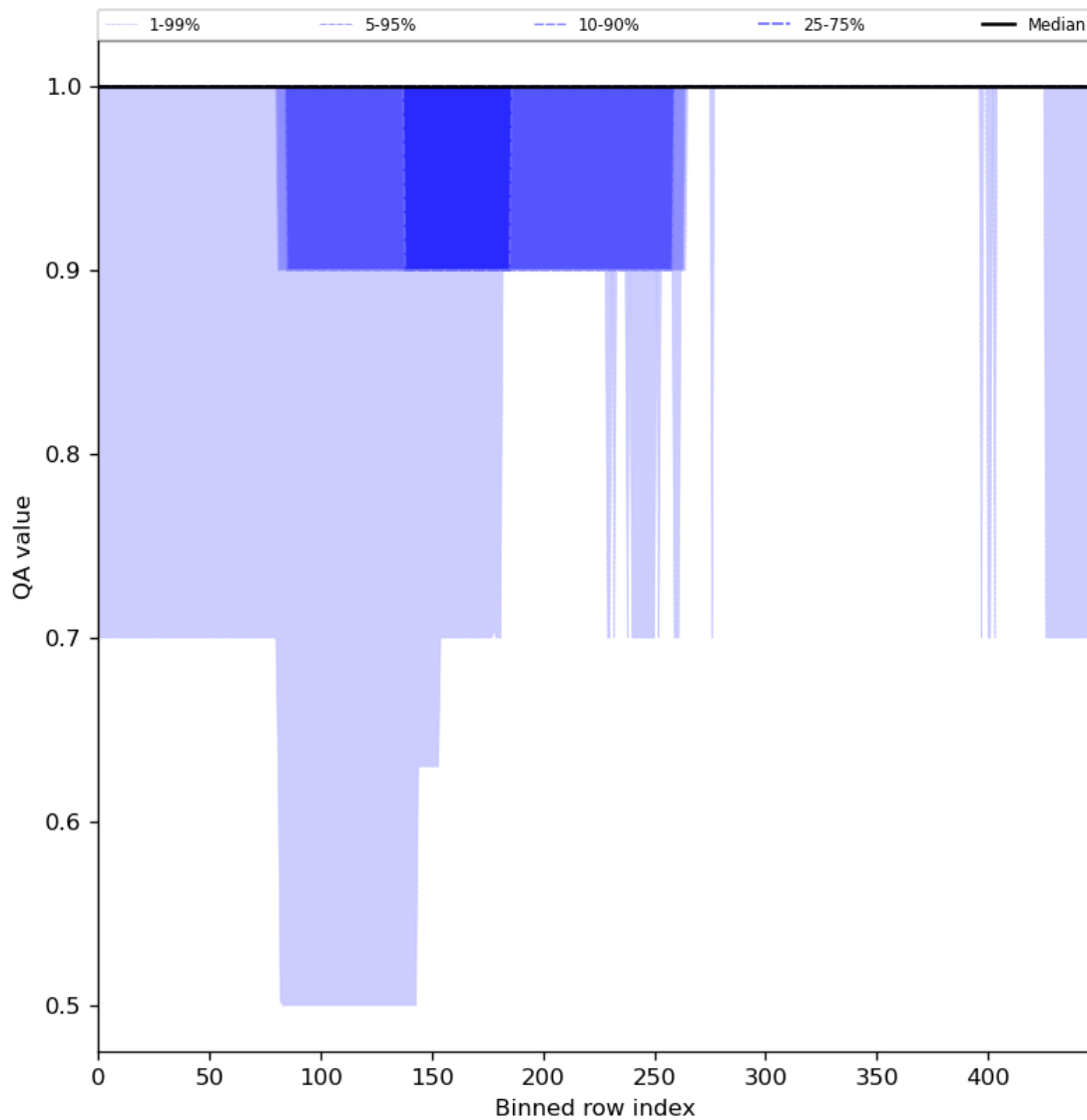
Figure 46: Along track statistics of “QA value” for 2023-07-27 to 2023-07-29
