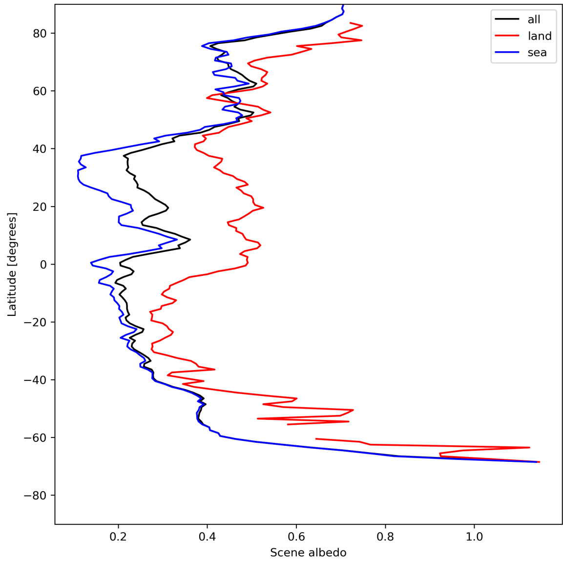
Figure 17: Zonal average of “Scene albedo” for 2023-07-27 to 2023-07-29.
