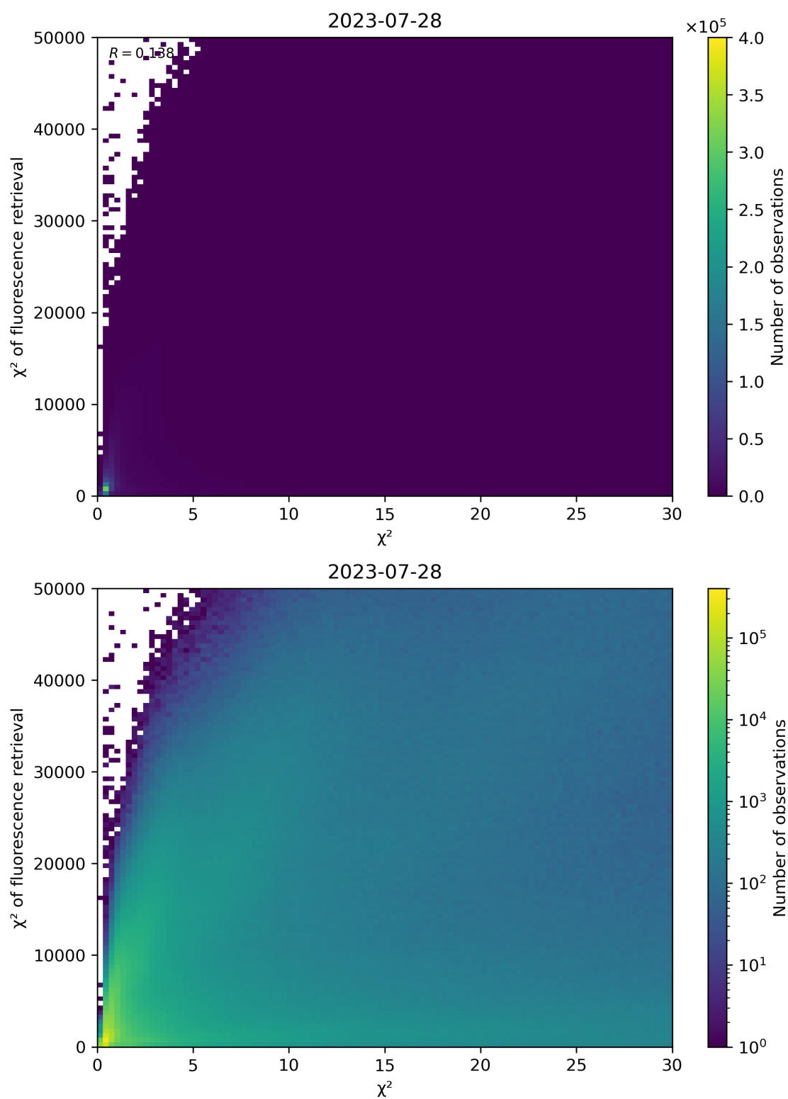
Figure 69: Scatter density plot of “ \chi^2 ” against “ \chi^2 of fluorescence retrieval” for 2023-07-27 to 2023-07-29.
