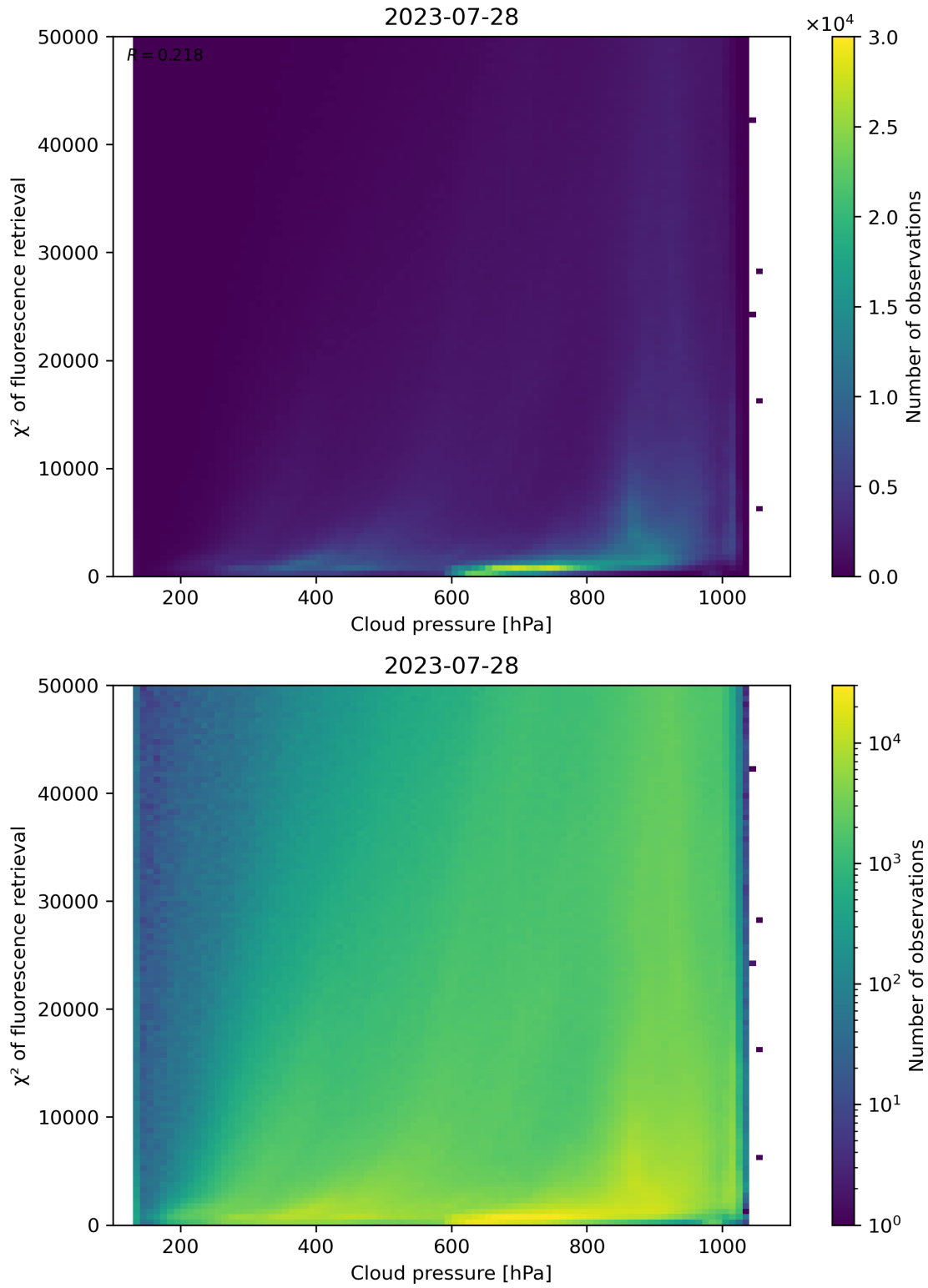
Figure 86: Scatter density plot of “Cloud pressure” against “ \chi^2 of fluorescence retrieval” for 2023-07-27 to 2023-07-29.
