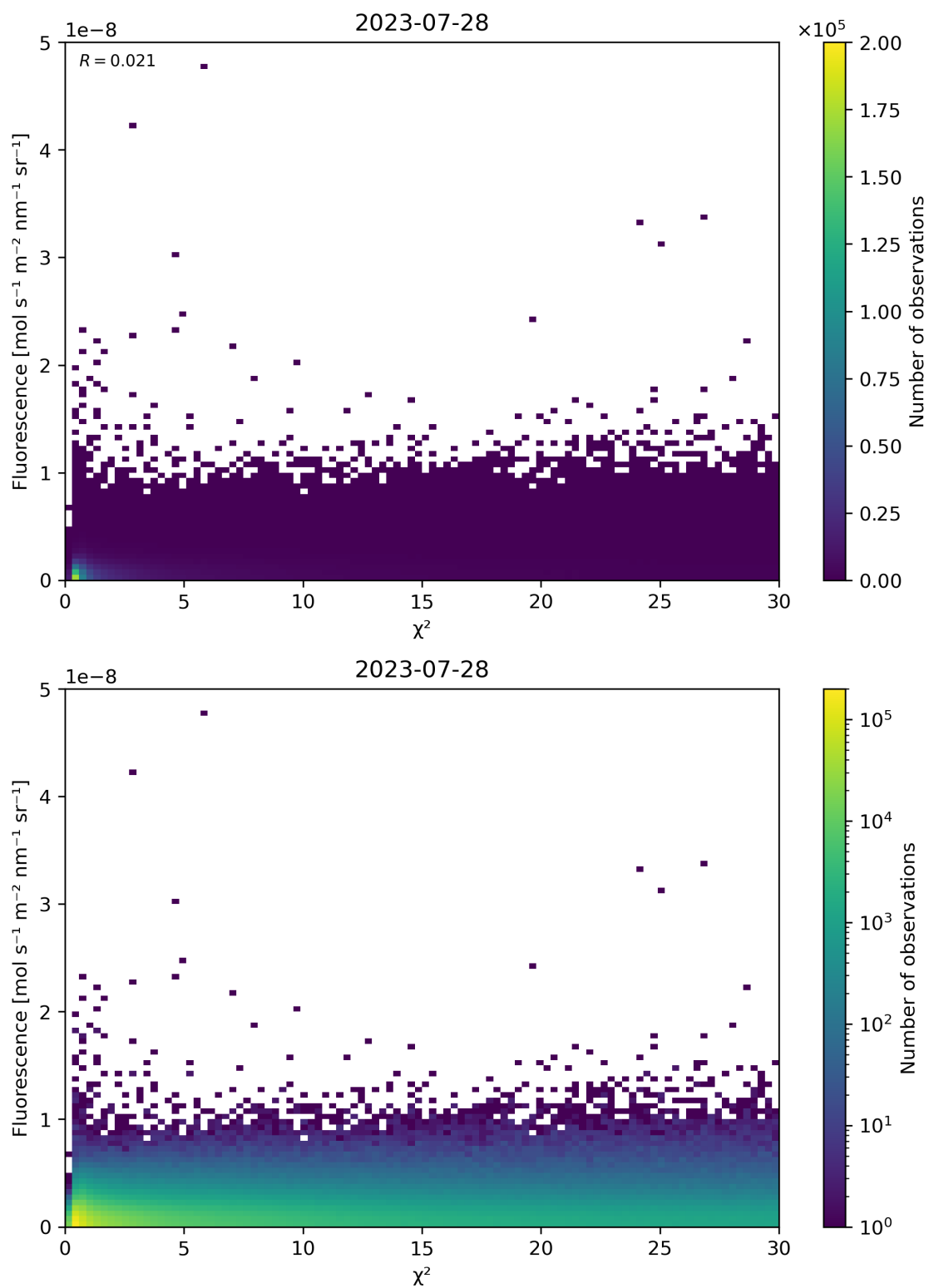
Figure 70: Scatter density plot of “ \chi^2 ” against “Fluorescence” for 2023-07-27 to 2023-07-29.
