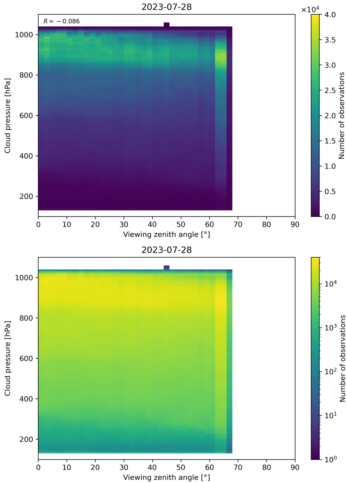
Figure 133: Scatter density plot of “Viewing zenith angle” against “Cloud pressure” for 2023-07-27 to 2023-07-29.
