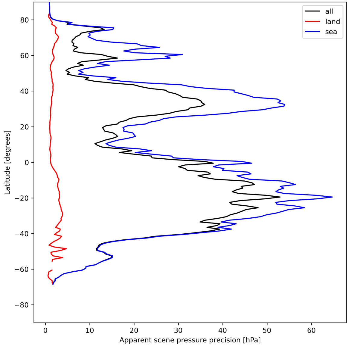
Figure 20: Zonal average of “Apparent scene pressure precision” for 2023-07-27 to 2023-07-29.
