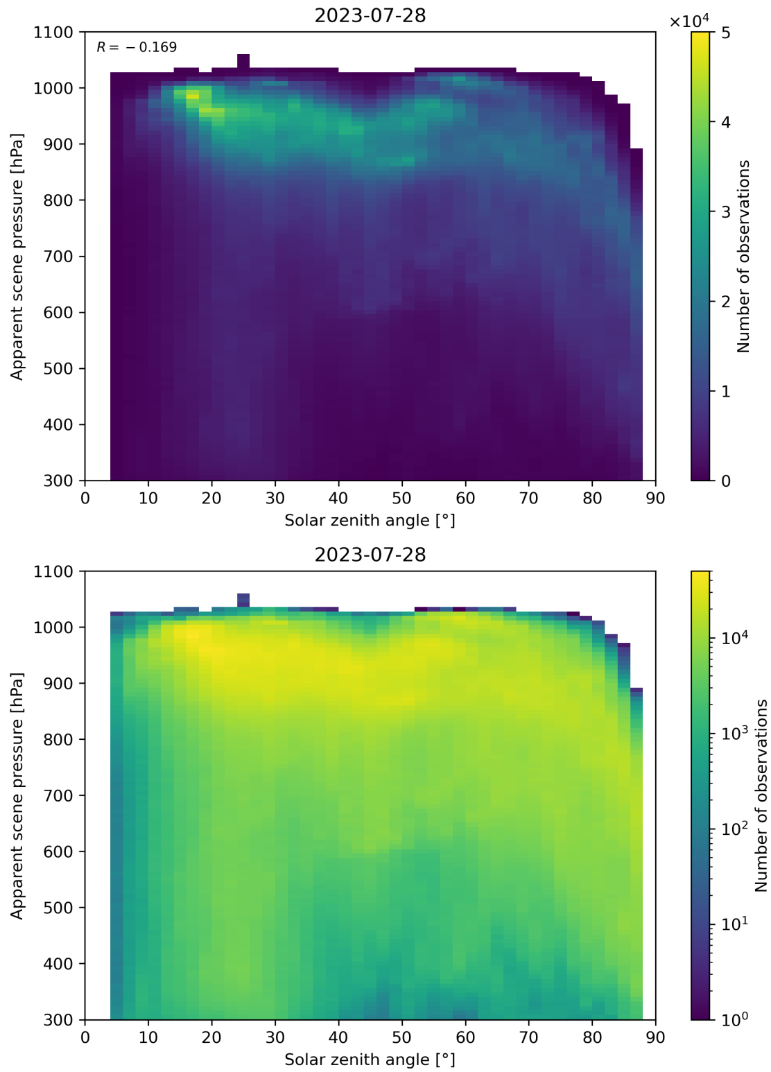
Figure 118: Scatter density plot of “Solar zenith angle” against “Apparent scene pressure” for 2023-07-27 to 2023-07-29.
