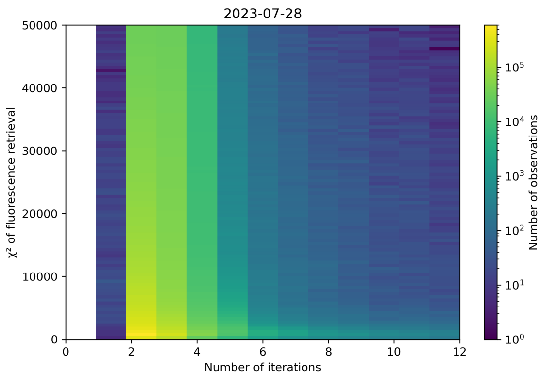
Figure 106: Scatter density plot of “Number of iterations” against “ \chi^2 of fluorescence retrieval” for 2023-07-27 to 2023-07-29.
