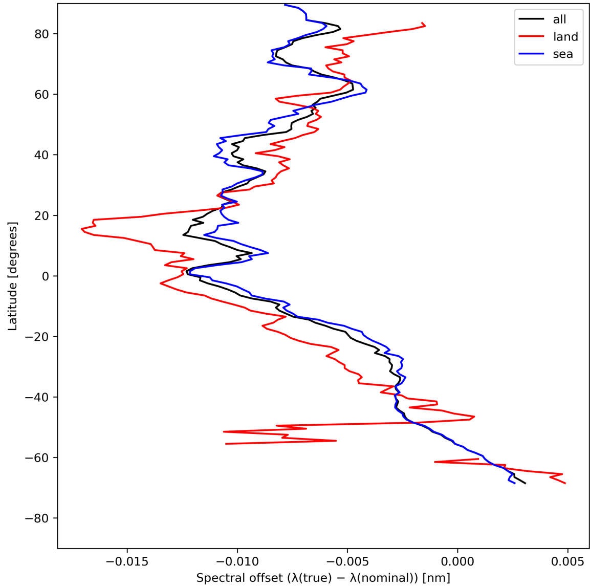
Figure 28: Zonal average of “Spectral offset ( \lambda(\text{true}) - \lambda(\text{nominal}) )” for 2023-07-27 to 2023-07-29.
