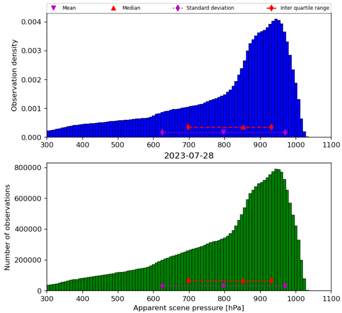
Figure 36: Histogram of “Apparent scene pressure” for 2023-07-27 to 2023-07-29
