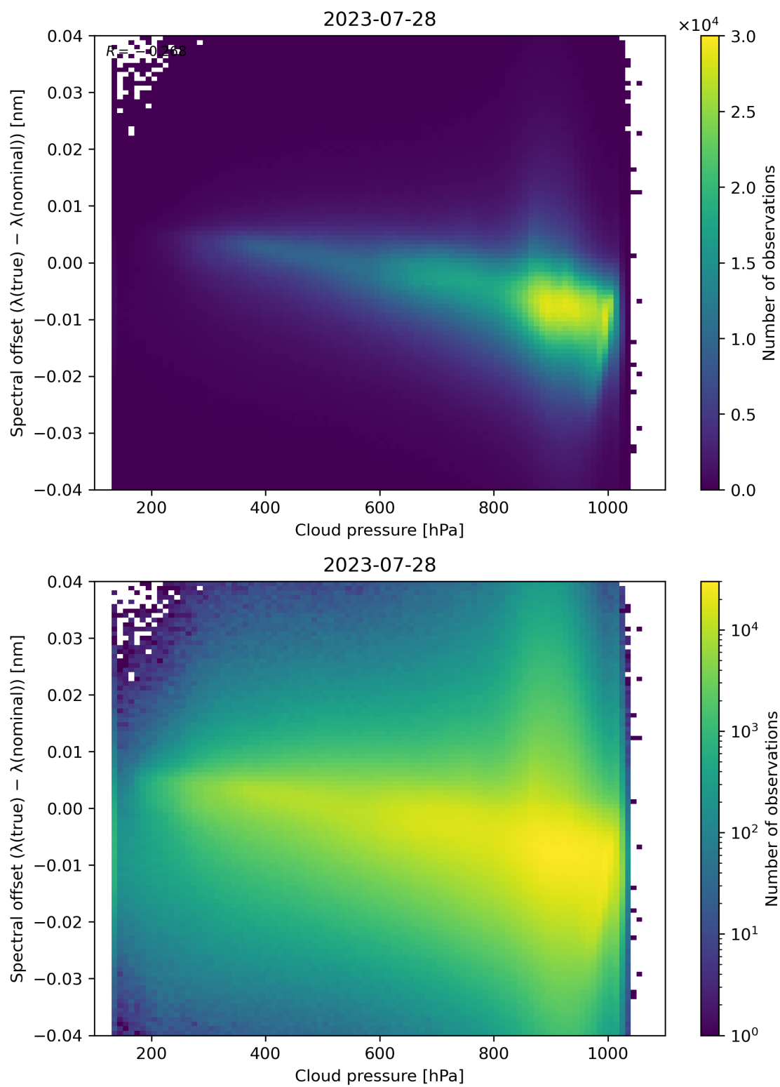
Figure 92: Scatter density plot of “Cloud pressure” against “Spectral offset ( \lambda(\text{true}) - \lambda(\text{nominal}) )” for 2023-07-27 to 2023-07-29.
