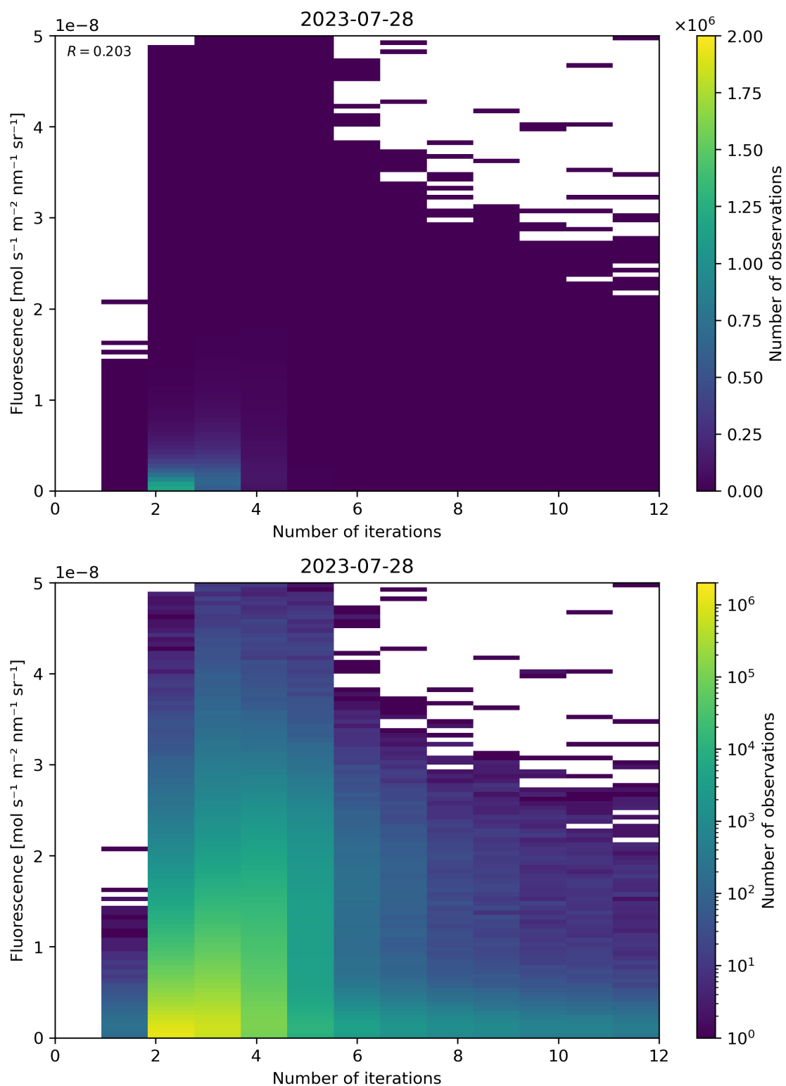
Figure 107: Scatter density plot of “Number of iterations” against “Fluorescence” for 2023-07-27 to 2023-07-29.
