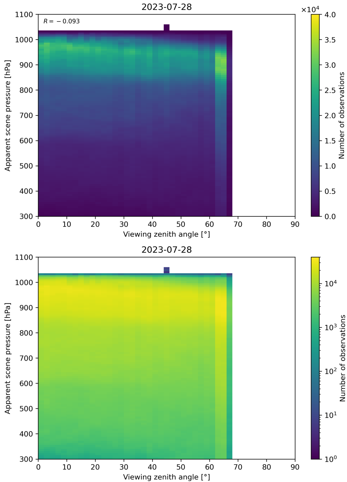
Figure 129: Scatter density plot of “Viewing zenith angle” against “Apparent scene pressure” for 2023-07-27 to 2023-07-29.
