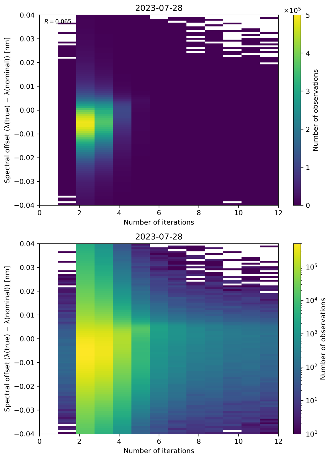
Figure 109: Scatter density plot of “Number of iterations” against “Spectral offset ( \lambda(\text{true}) - \lambda(\text{nominal}) )” for 2023-07-27 to 2023-07-29.
