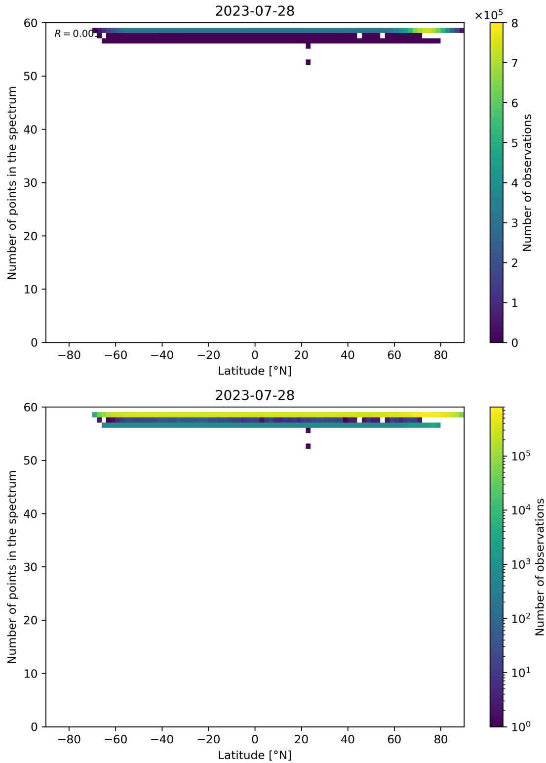
Figure 103: Scatter density plot of “Latitude” against “Number of points in the spectrum” for 2023-07-27 to 2023-07-29.
