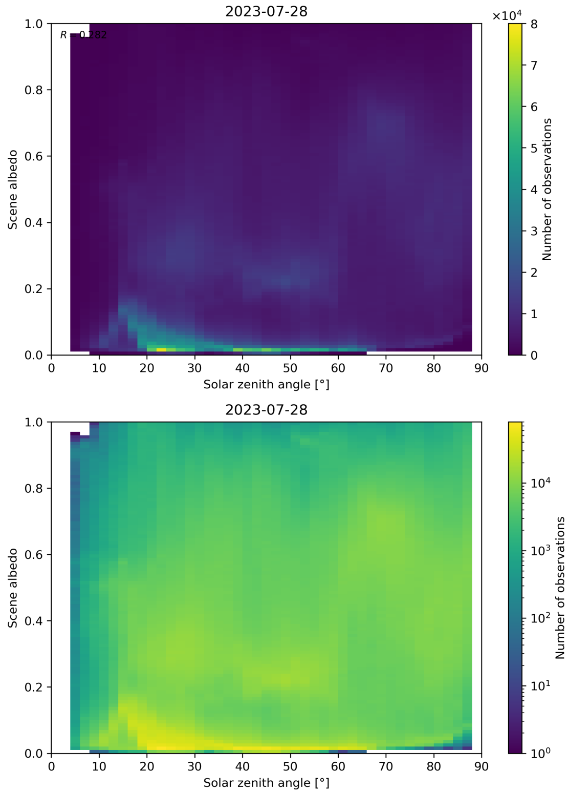
Figure 127: Scatter density plot of “Solar zenith angle” against “Scene albedo” for 2023-07-27 to 2023-07-29.
