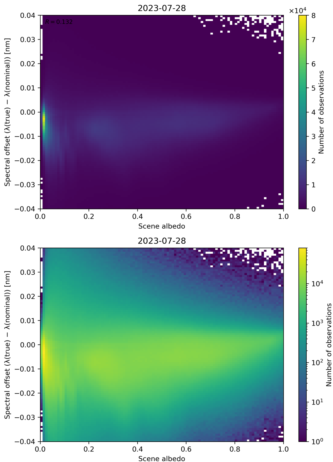
Figure 117: Scatter density plot of “Scene albedo” against “Spectral offset ( \lambda(\text{true}) - \lambda(\text{nominal}) )” for 2023-07-27 to 2023-07-29.
