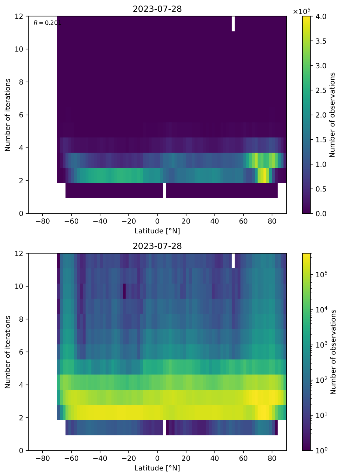
Figure 102: Scatter density plot of “Latitude” against “Number of iterations” for 2023-07-27 to 2023-07-29.
