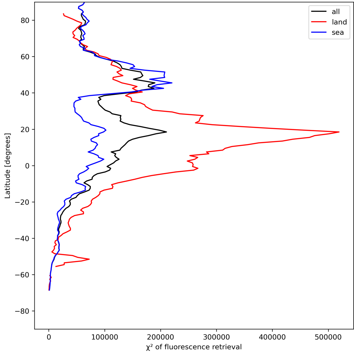
Figure 25: Zonal average of “ \chi^2 of fluorescence retrieval” for 2023-07-27 to 2023-07-29.
