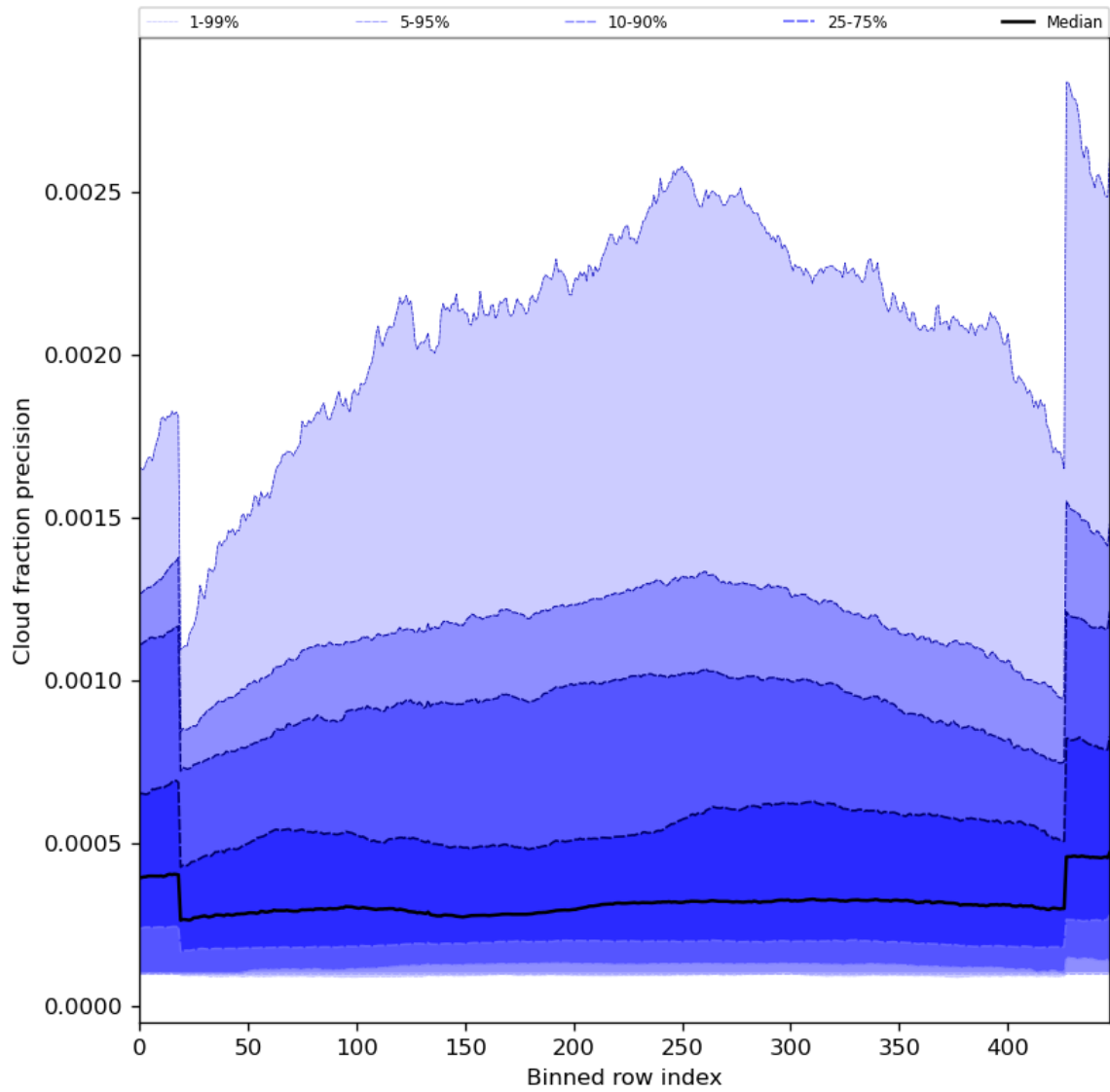
Figure 50: Along track statistics of “Cloud fraction precision” for 2023-07-27 to 2023-07-29
