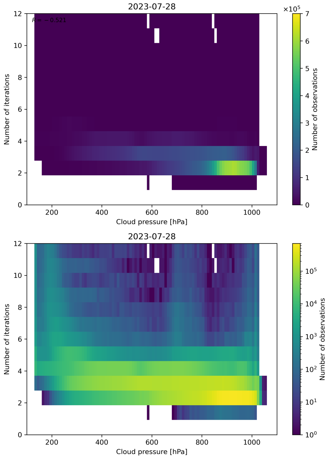
Figure 89: Scatter density plot of “Cloud pressure” against “Number of iterations” for 2023-07-27 to 2023-07-29.
