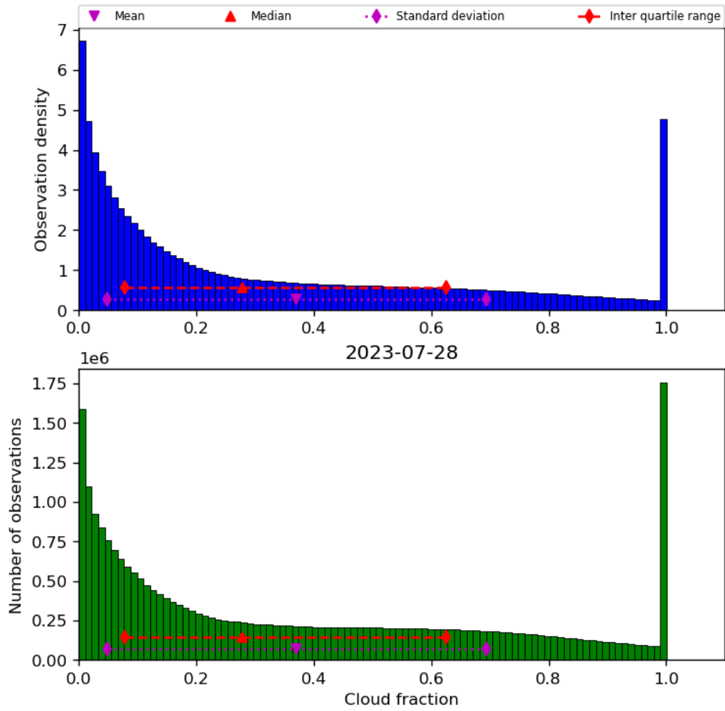
Figure 32: Histogram of “Cloud fraction” for 2023-07-27 to 2023-07-29
