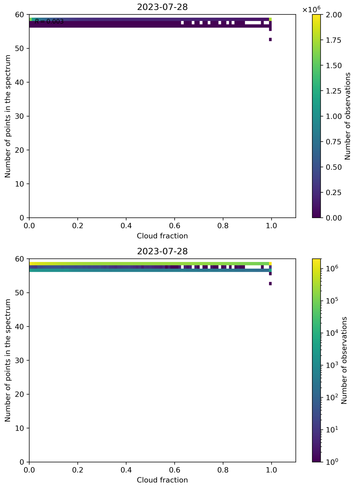
Figure 81: Scatter density plot of “Cloud fraction” against “Number of points in the spectrum” for 2023-07-27 to 2023-07-29.
