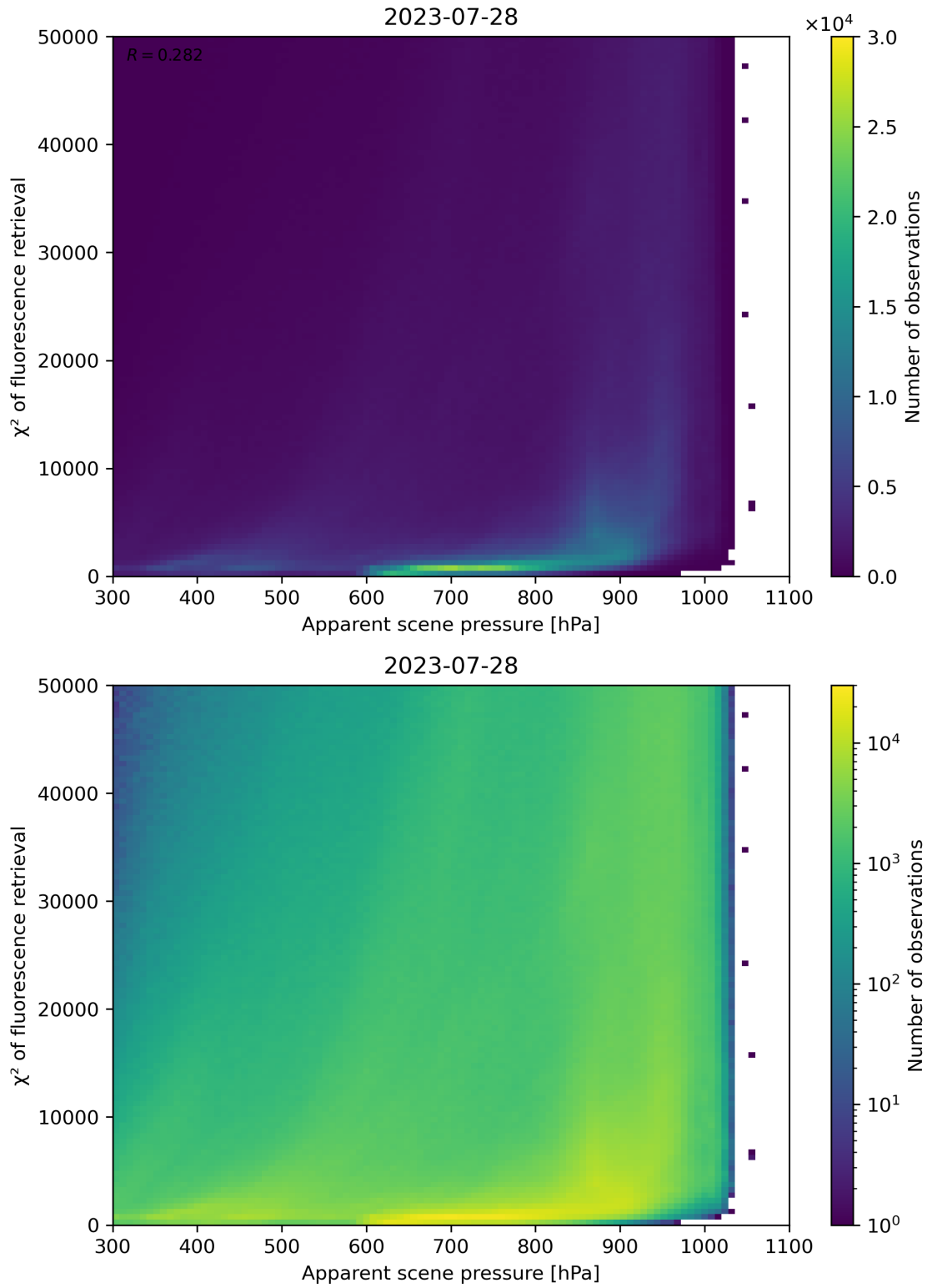
Figure 64: Scatter density plot of “Apparent scene pressure” against “ \chi^2 of fluorescence retrieval” for 2023-07-27 to 2023-07-29.
