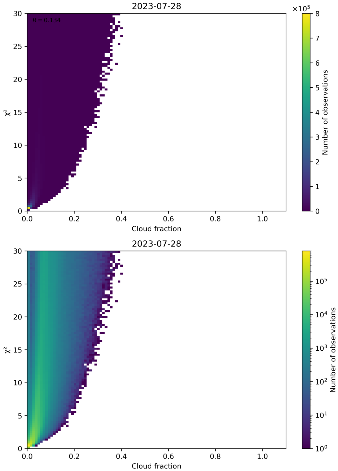
Figure 77: Scatter density plot of “Cloud fraction” against “ \chi^2 ” for 2023-07-27 to 2023-07-29.
