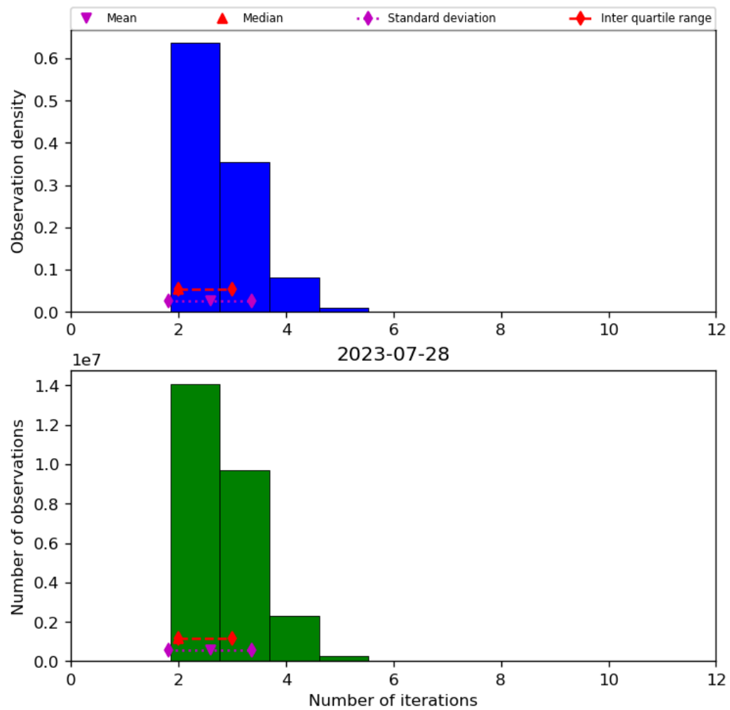
Figure 39: Histogram of “Number of iterations” for 2023-07-27 to 2023-07-29
