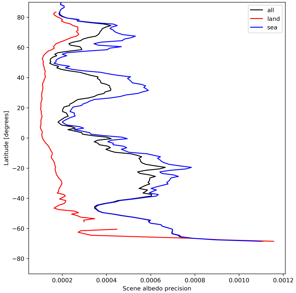
Figure 18: Zonal average of “Scene albedo precision” for 2023-07-27 to 2023-07-29.
