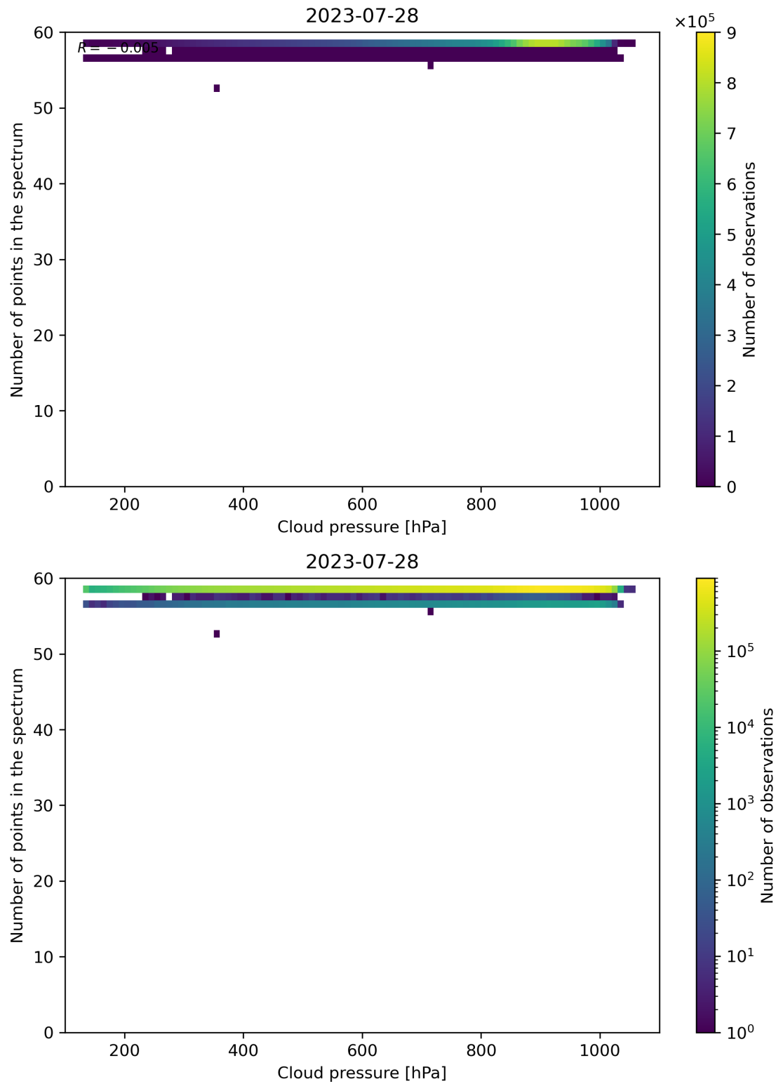
Figure 90: Scatter density plot of “Cloud pressure” against “Number of points in the spectrum” for 2023-07-27 to 2023-07-29.
