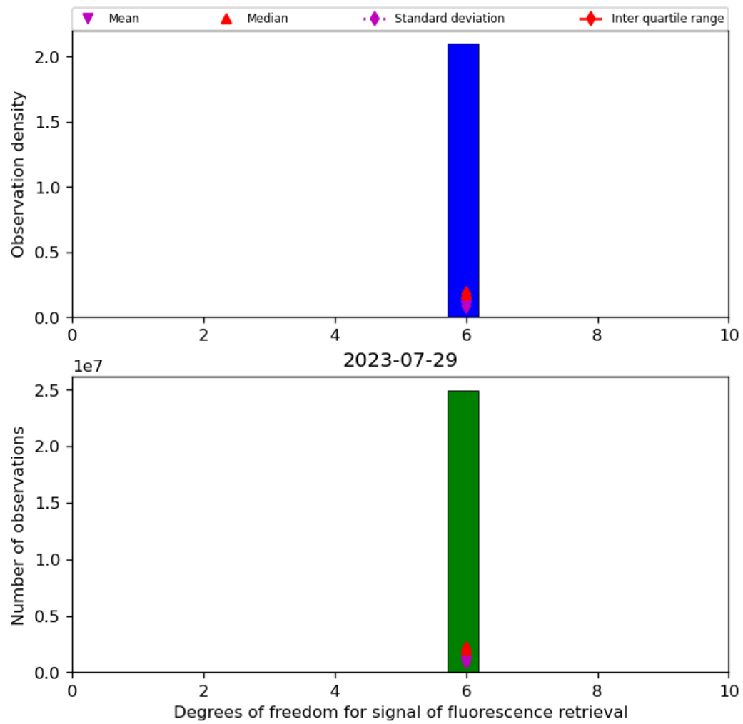
Figure 43: Histogram of “Degrees of freedom for signal of fluorescence retrieval” for 2023-07-29 to 2023-07-30
