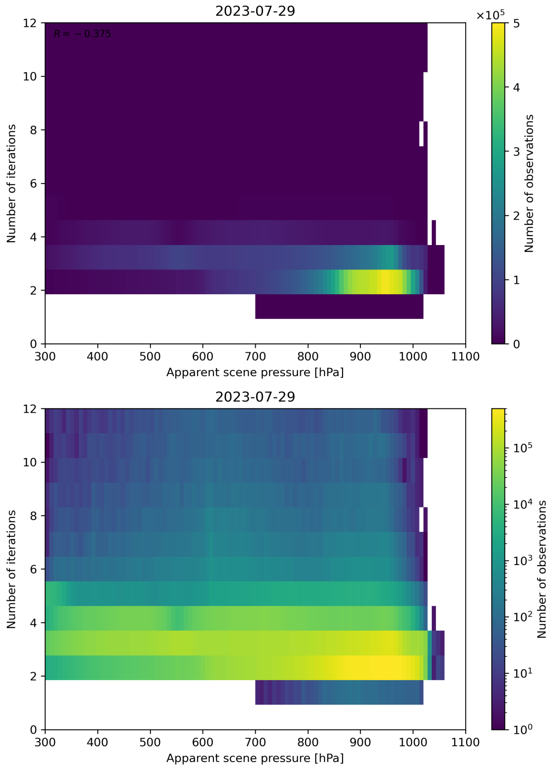
Figure 66: Scatter density plot of “Apparent scene pressure” against “Number of iterations” for 2023-07-29 to 2023-07-30.
