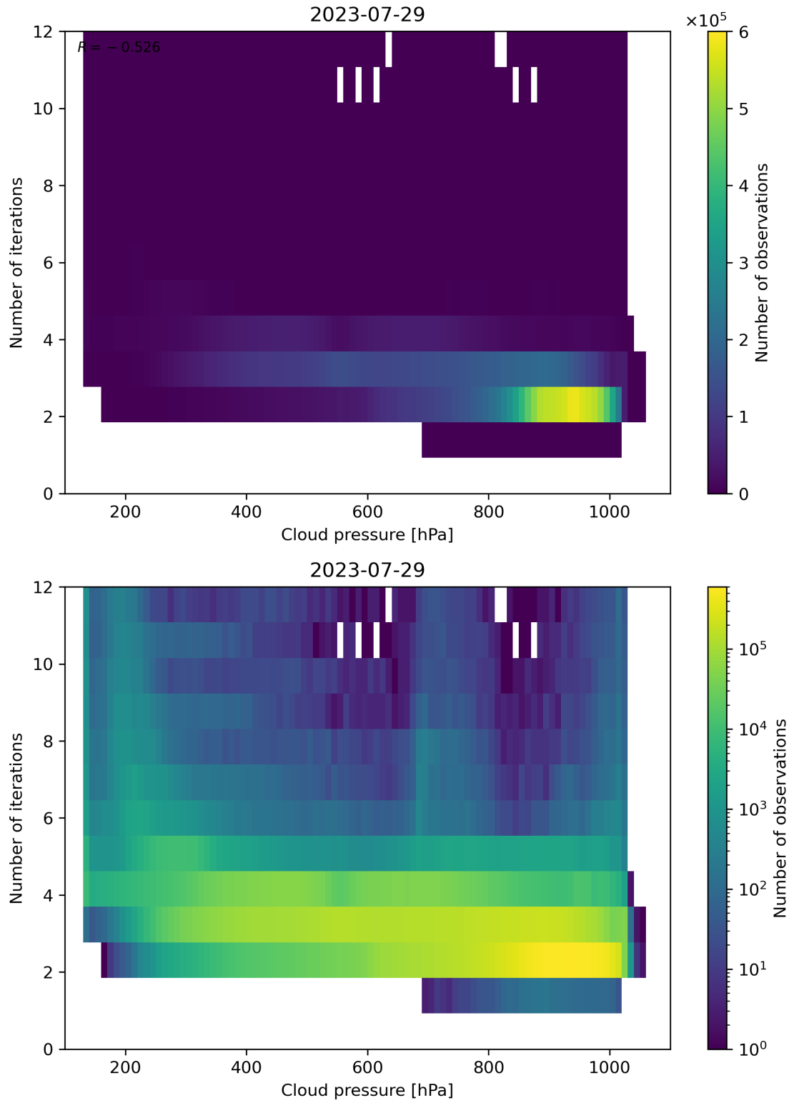
Figure 89: Scatter density plot of “Cloud pressure” against “Number of iterations” for 2023-07-29 to 2023-07-30.
