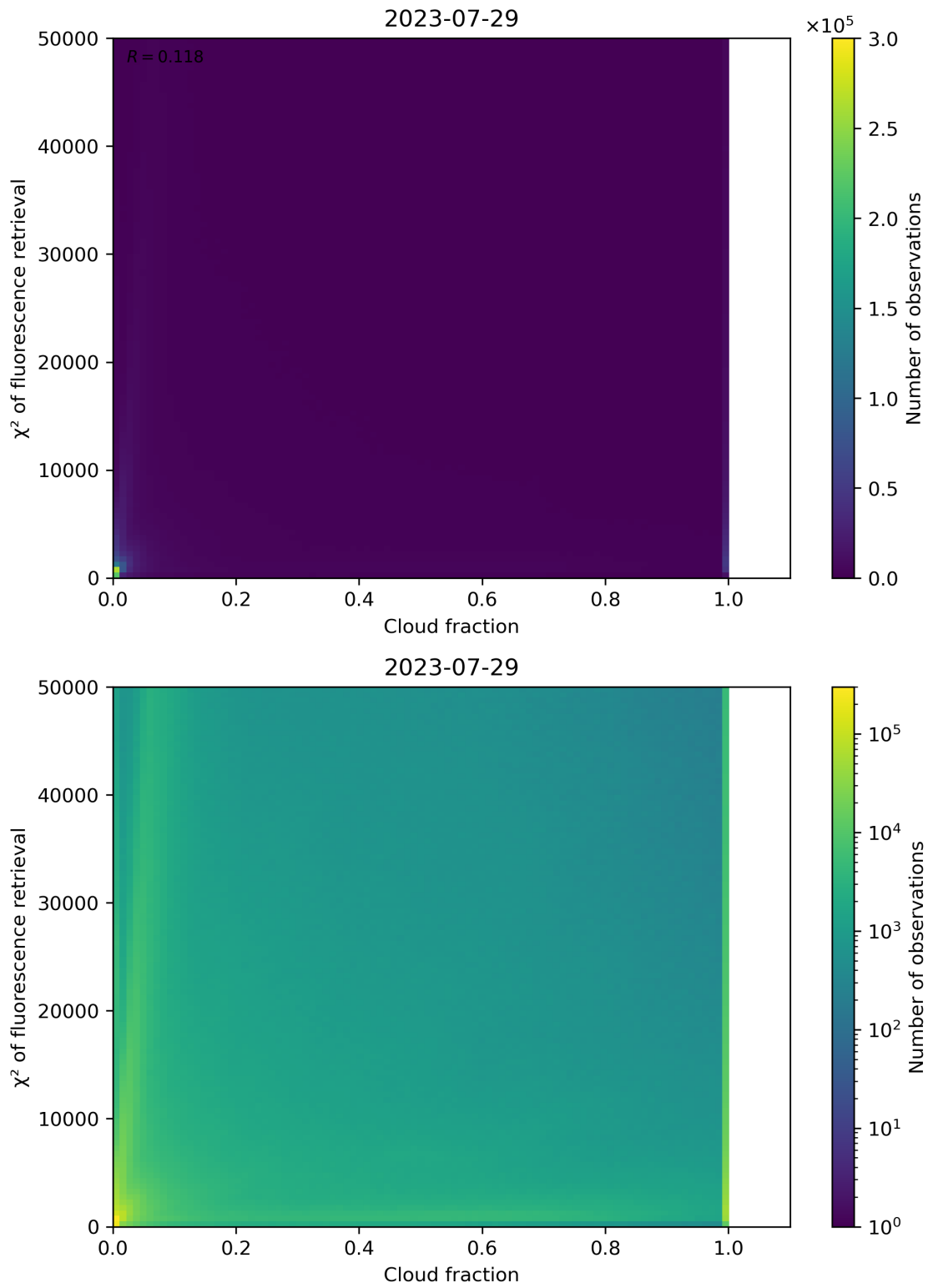
Figure 78: Scatter density plot of “Cloud fraction” against “ \chi^2 of fluorescence retrieval” for 2023-07-29 to 2023-07-30.
