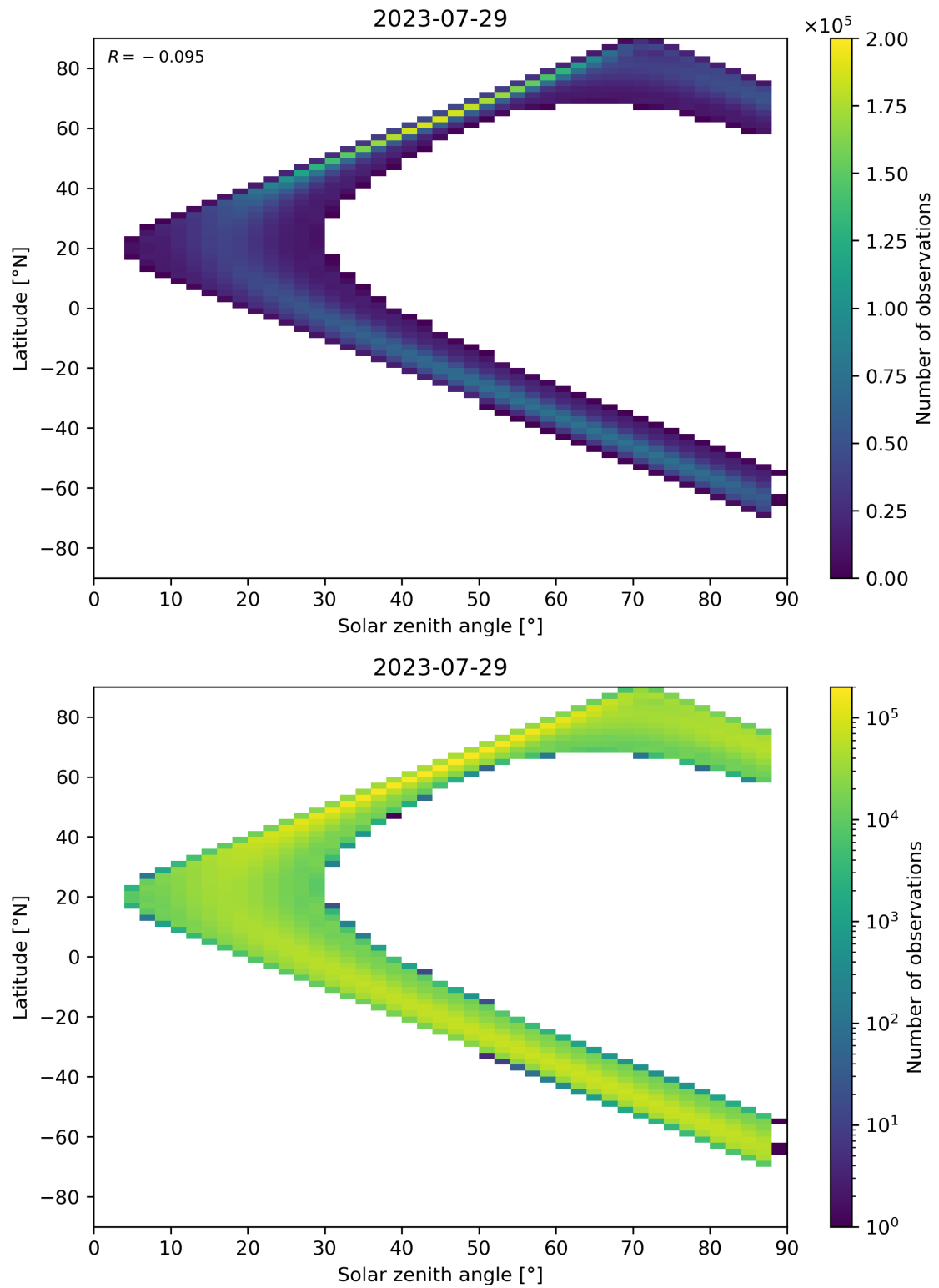
Figure 124: Scatter density plot of “Solar zenith angle” against “Latitude” for 2023-07-29 to 2023-07-30.
