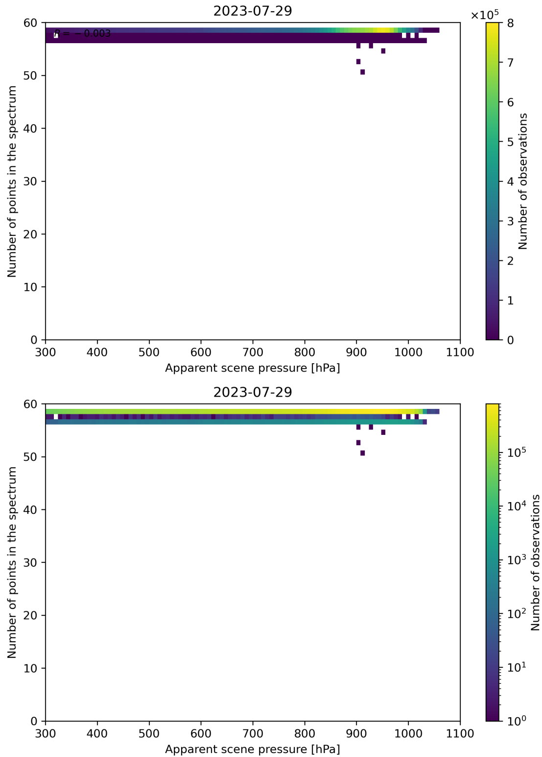
Figure 67: Scatter density plot of “Apparent scene pressure” against “Number of points in the spectrum” for 2023-07-29 to 2023-07-30.
