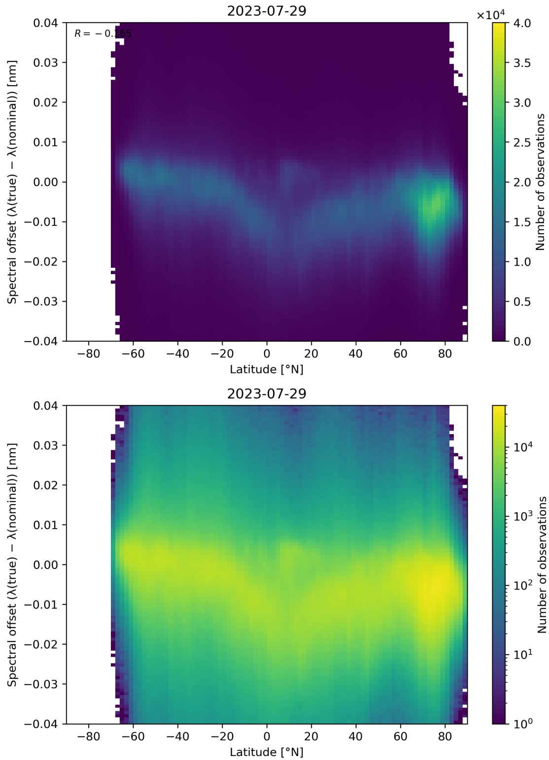
Figure 105: Scatter density plot of “Latitude” against “Spectral offset ( \lambda(\text{true}) - \lambda(\text{nominal}) )” for 2023-07-29 to 2023-07-30.
