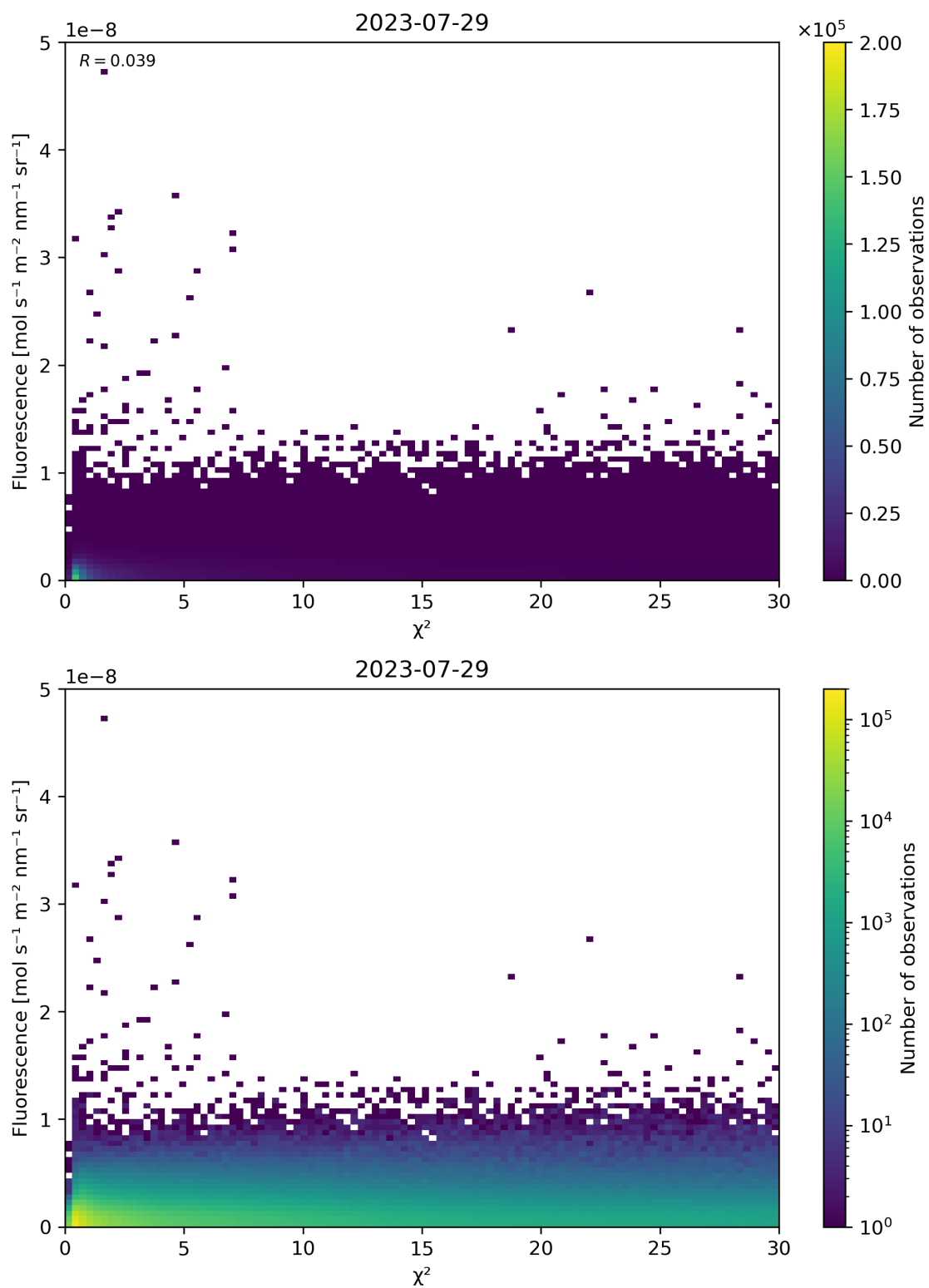
Figure 70: Scatter density plot of “ \chi^2 ” against “Fluorescence” for 2023-07-29 to 2023-07-30.
