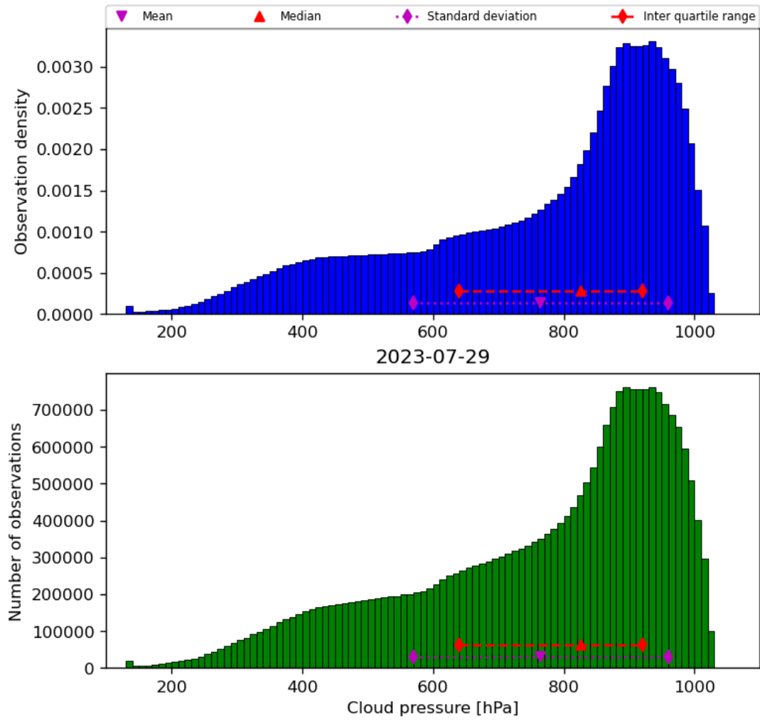
Figure 30: Histogram of “Cloud pressure” for 2023-07-29 to 2023-07-30
