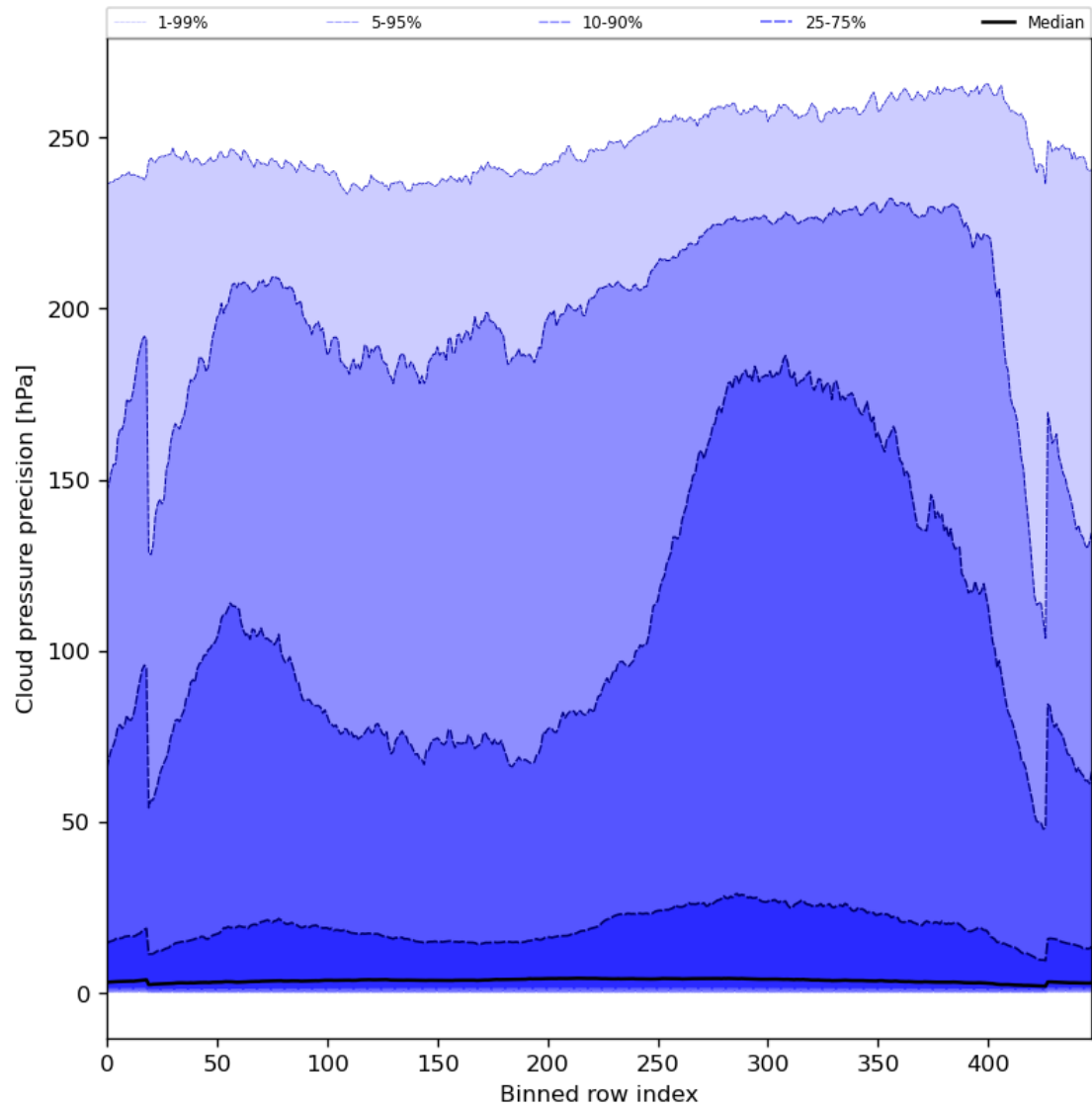
Figure 48: Along track statistics of “Cloud pressure precision” for 2023-07-29 to 2023-07-30
