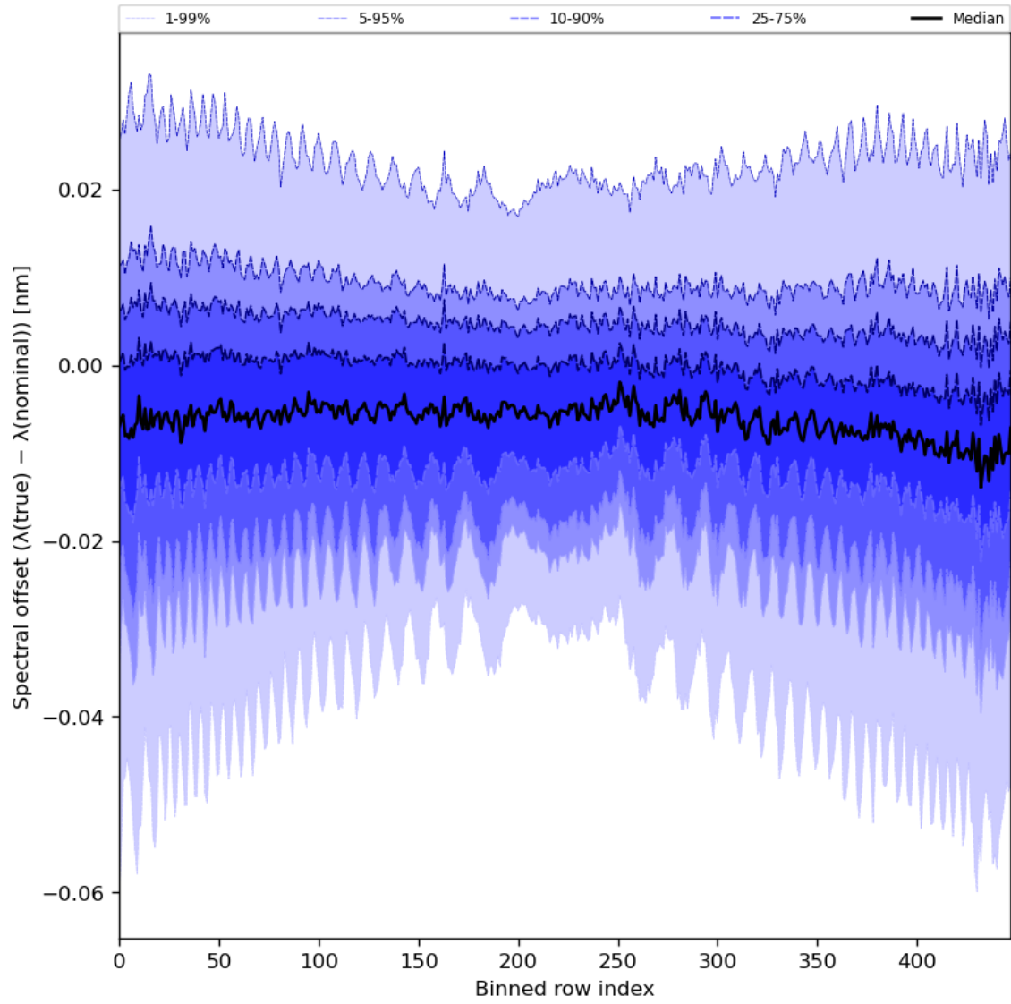
Figure 62: Along track statistics of “Spectral offset ( \lambda(\text{true}) - \lambda(\text{nominal}) )” for 2023-07-29 to 2023-07-30
