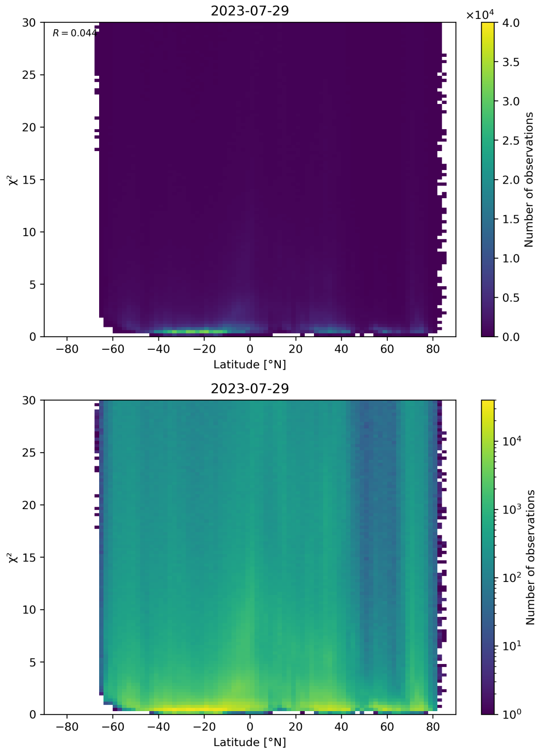
Figure 97: Scatter density plot of “Latitude” against “ \chi^2 ” for 2023-07-29 to 2023-07-30.
