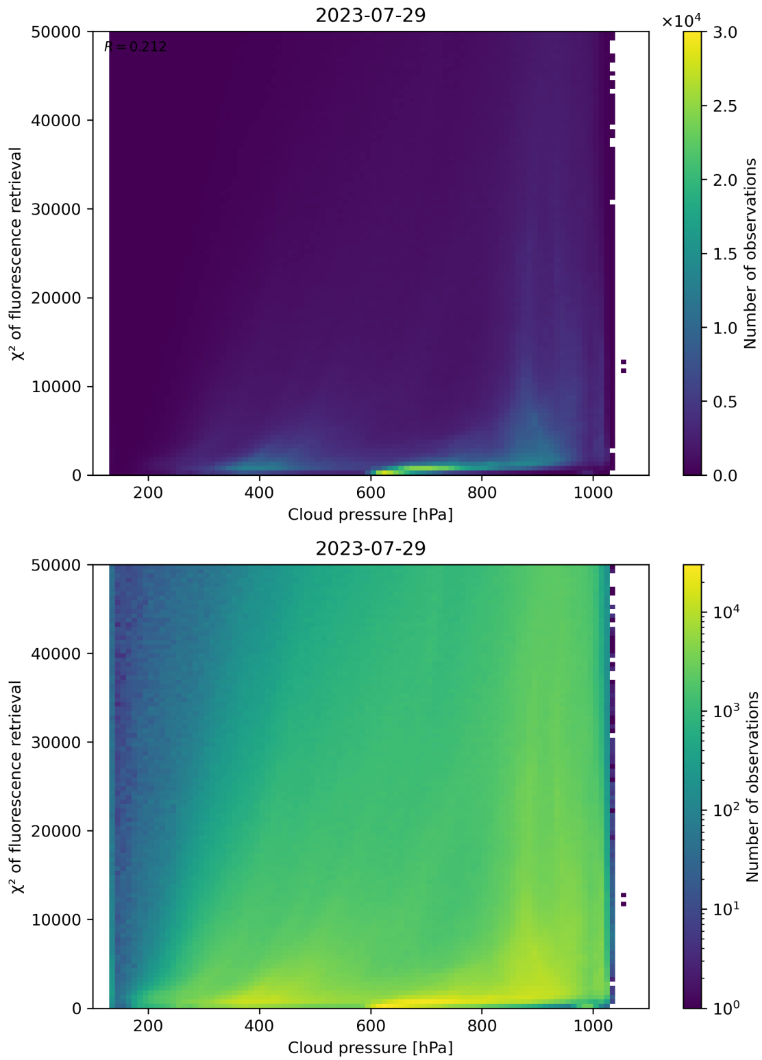
Figure 86: Scatter density plot of “Cloud pressure” against “ \chi^2 of fluorescence retrieval” for 2023-07-29 to 2023-07-30.
