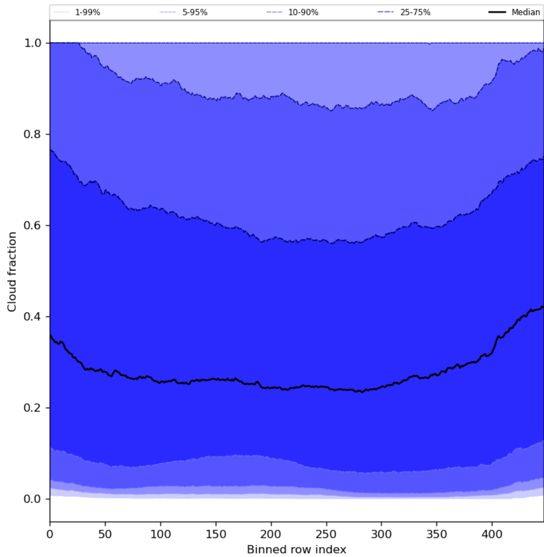
Figure 49: Along track statistics of “Cloud fraction” for 2023-07-29 to 2023-07-30
