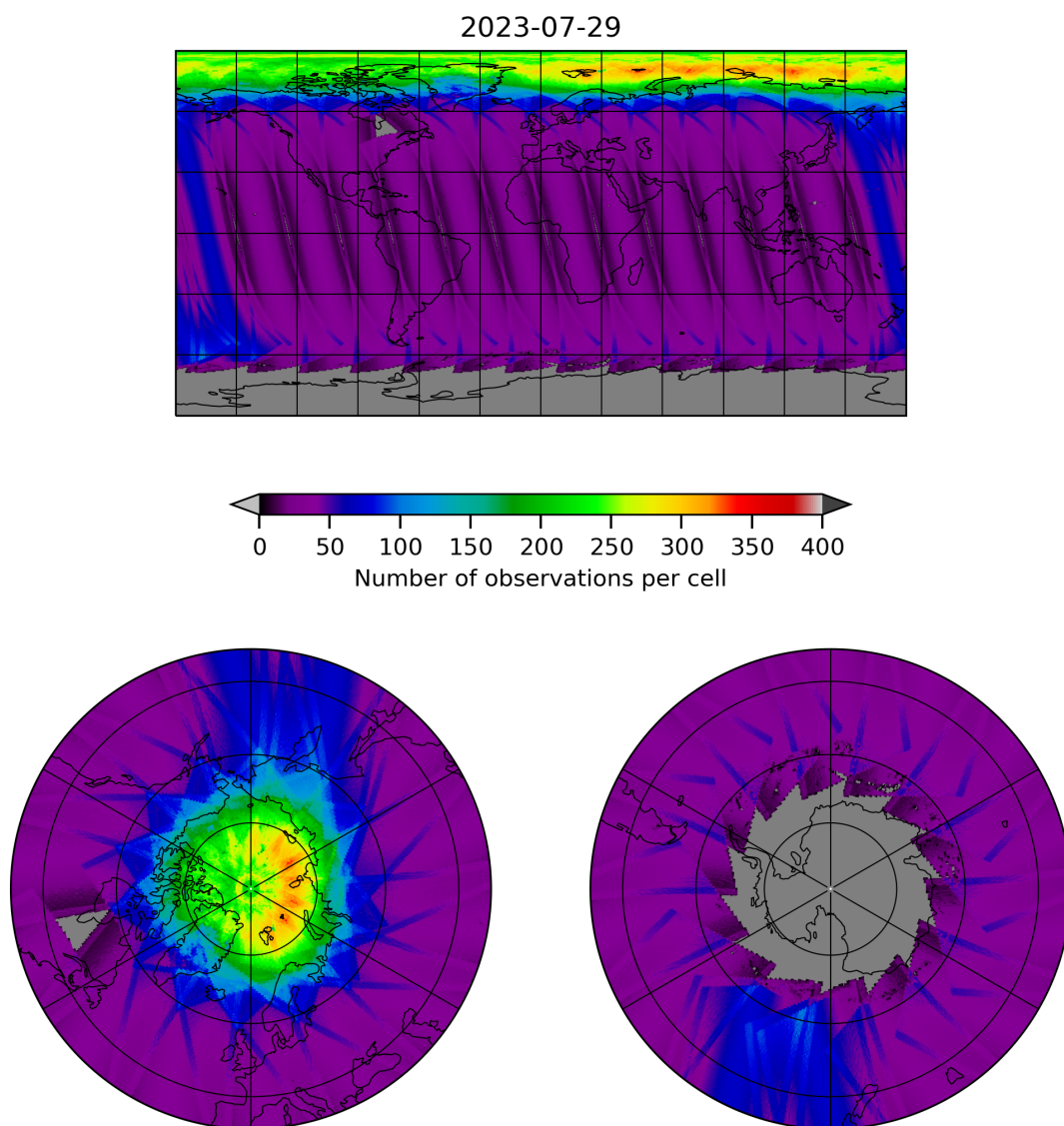
Figure 11: Map of the number of observations for 2023-07-29 to 2023-07-30
