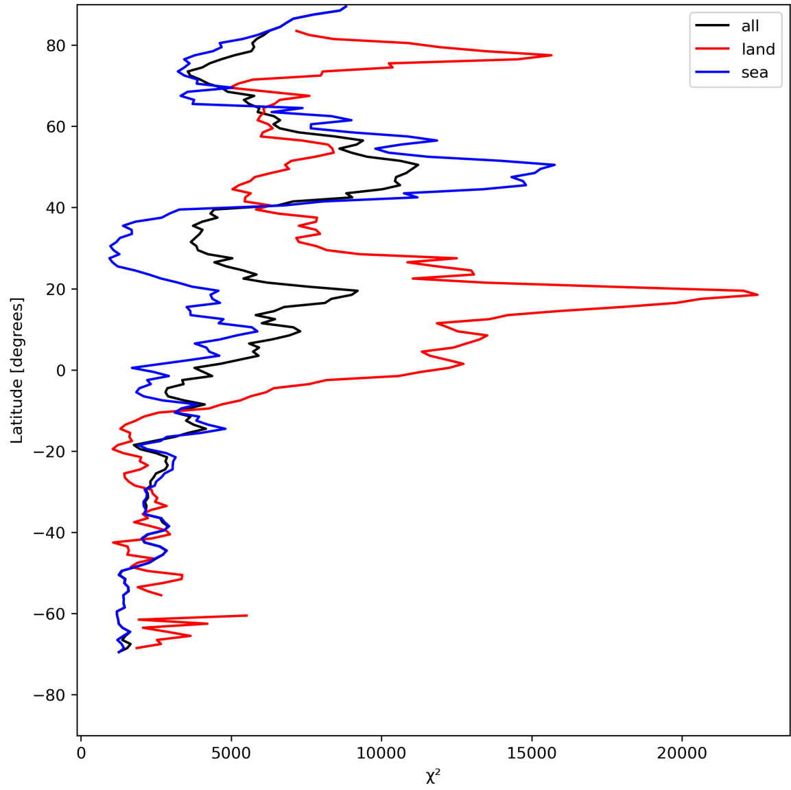
Figure 21: Zonal average of “ \chi^2 ” for 2023-07-29 to 2023-07-30.
