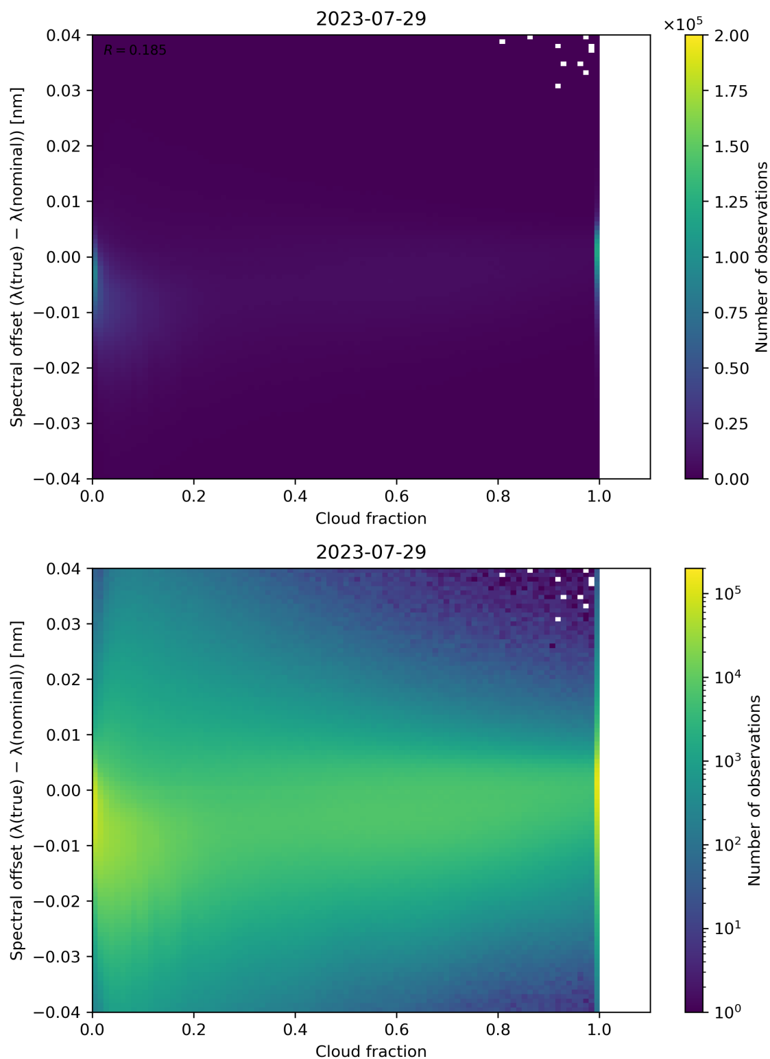
Figure 83: Scatter density plot of “Cloud fraction” against “Spectral offset ( \lambda(\text{true}) - \lambda(\text{nominal}) )” for 2023-07-29 to 2023-07-30.
