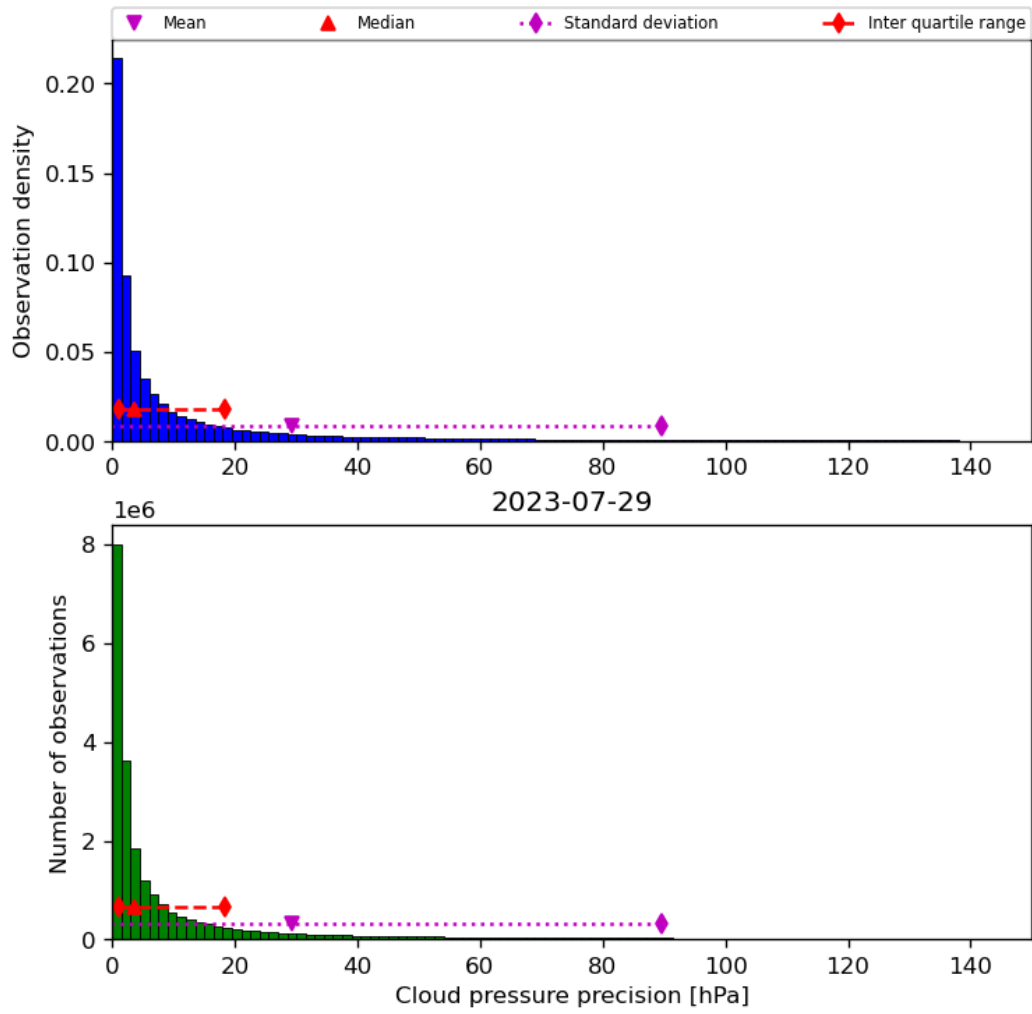
Figure 31: Histogram of “Cloud pressure precision” for 2023-07-29 to 2023-07-30
