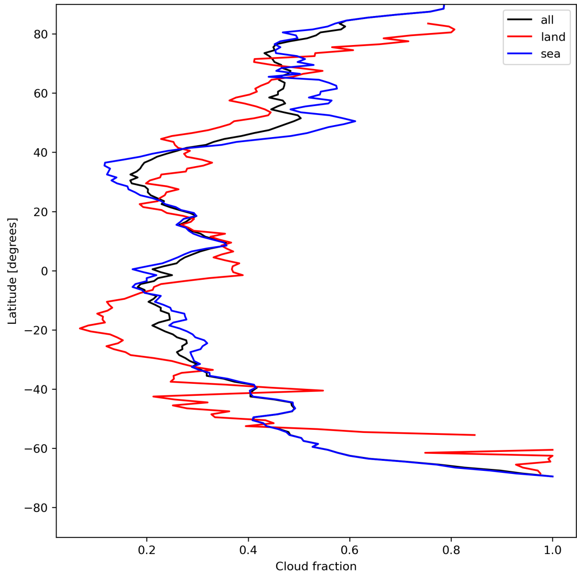
Figure 15: Zonal average of “Cloud fraction” for 2023-07-29 to 2023-07-30.
