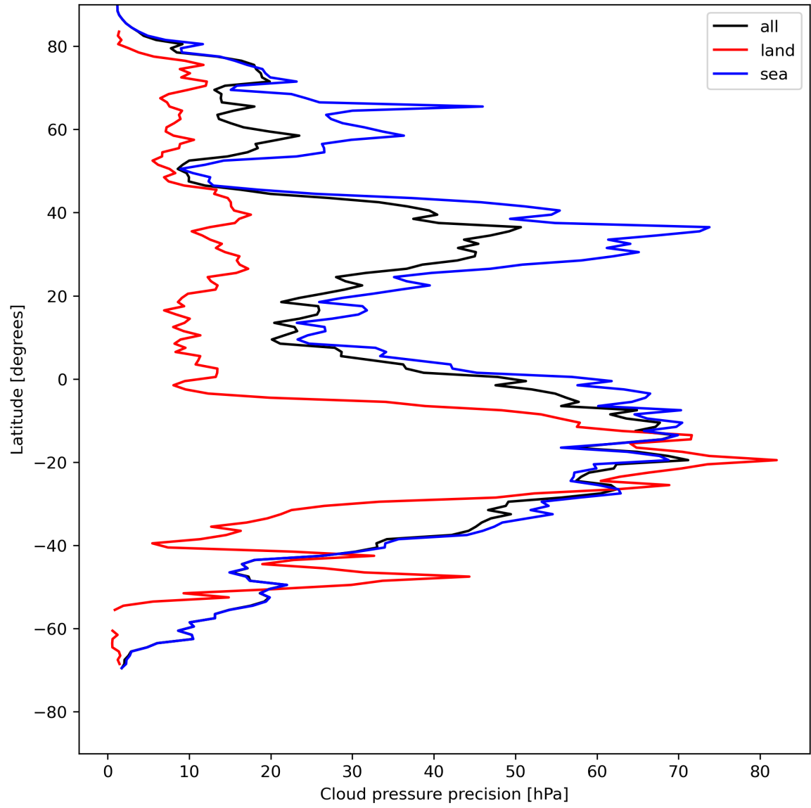
Figure 14: Zonal average of “Cloud pressure precision” for 2023-07-29 to 2023-07-30.
