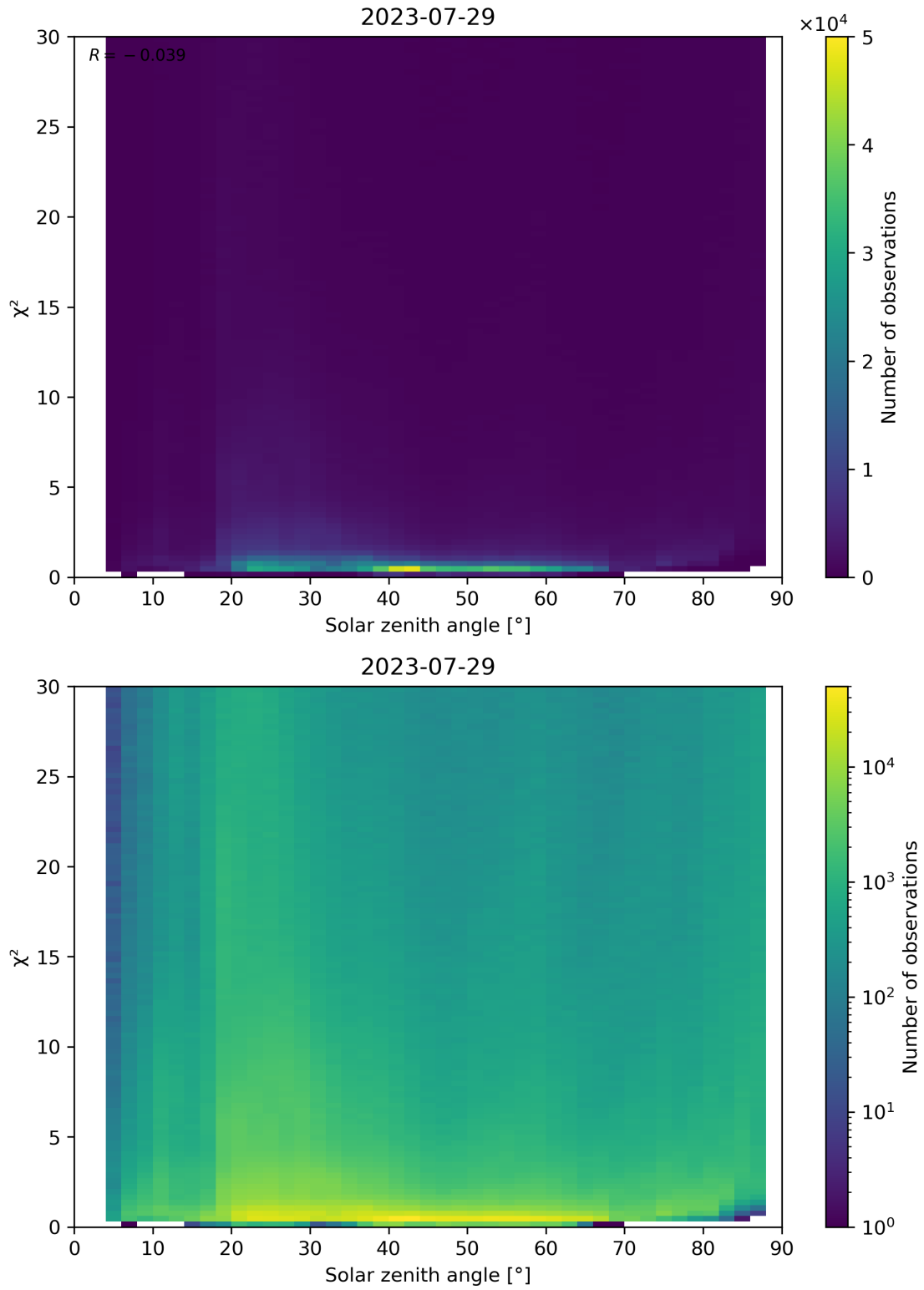
Figure 119: Scatter density plot of “Solar zenith angle” against “ \chi^2 ” for 2023-07-29 to 2023-07-30.
