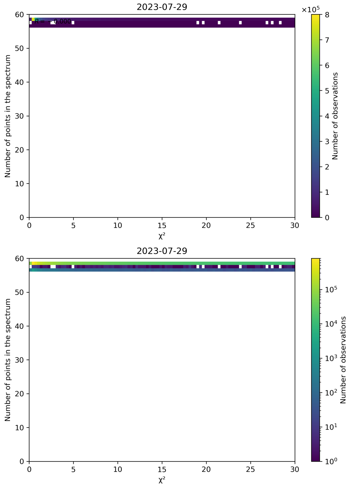
Figure 74: Scatter density plot of “ \chi^2 ” against “Number of points in the spectrum” for 2023-07-29 to 2023-07-30.
