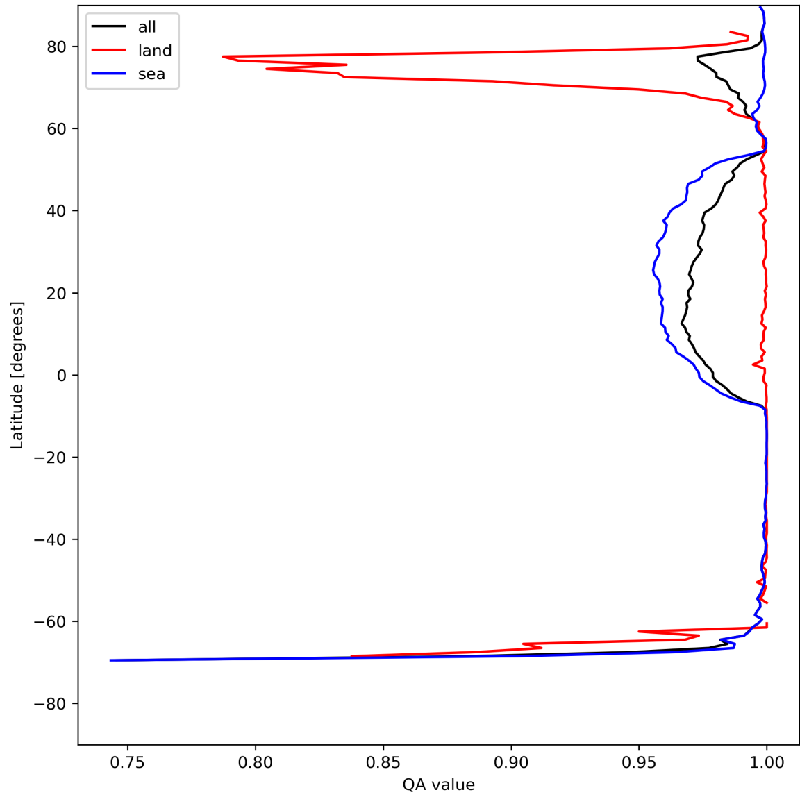
Figure 12: Zonal average of “QA value” for 2023-07-29 to 2023-07-30.
