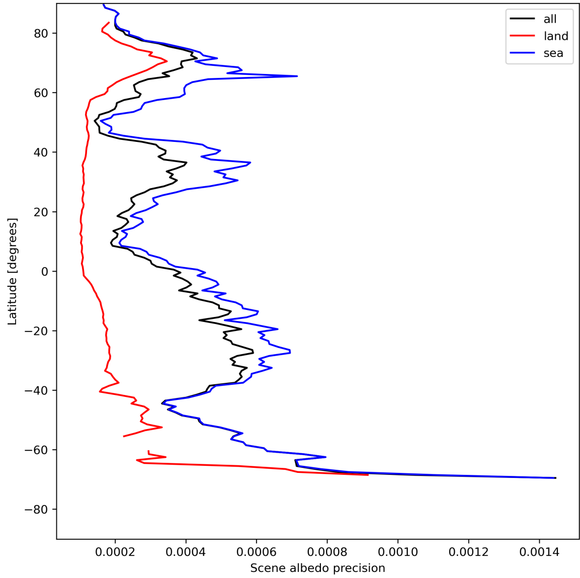
Figure 18: Zonal average of “Scene albedo precision” for 2023-07-29 to 2023-07-30.
