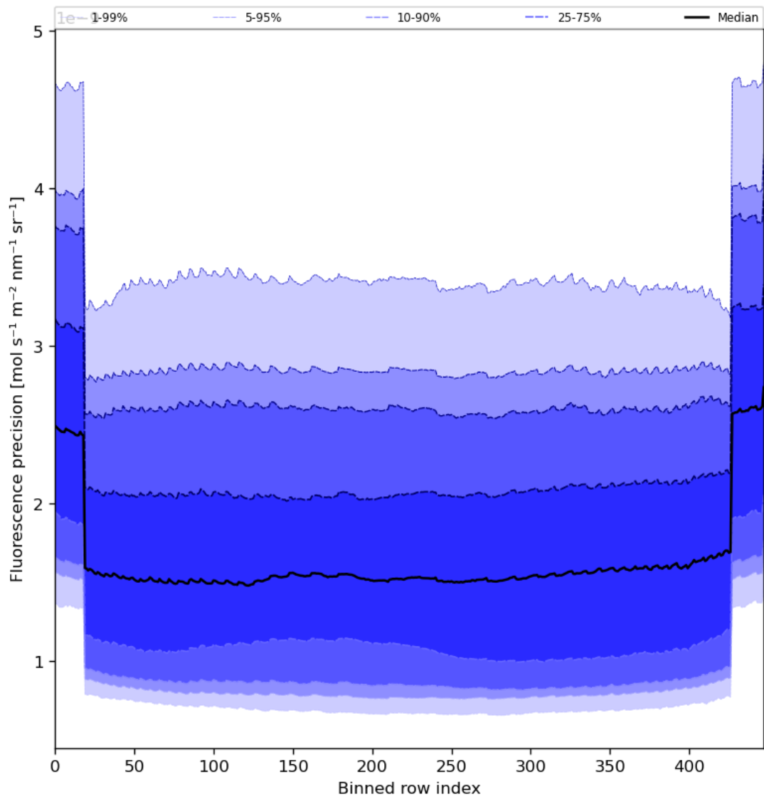
Figure 58: Along track statistics of “Fluorescence precision” for 2023-07-29 to 2023-07-30
