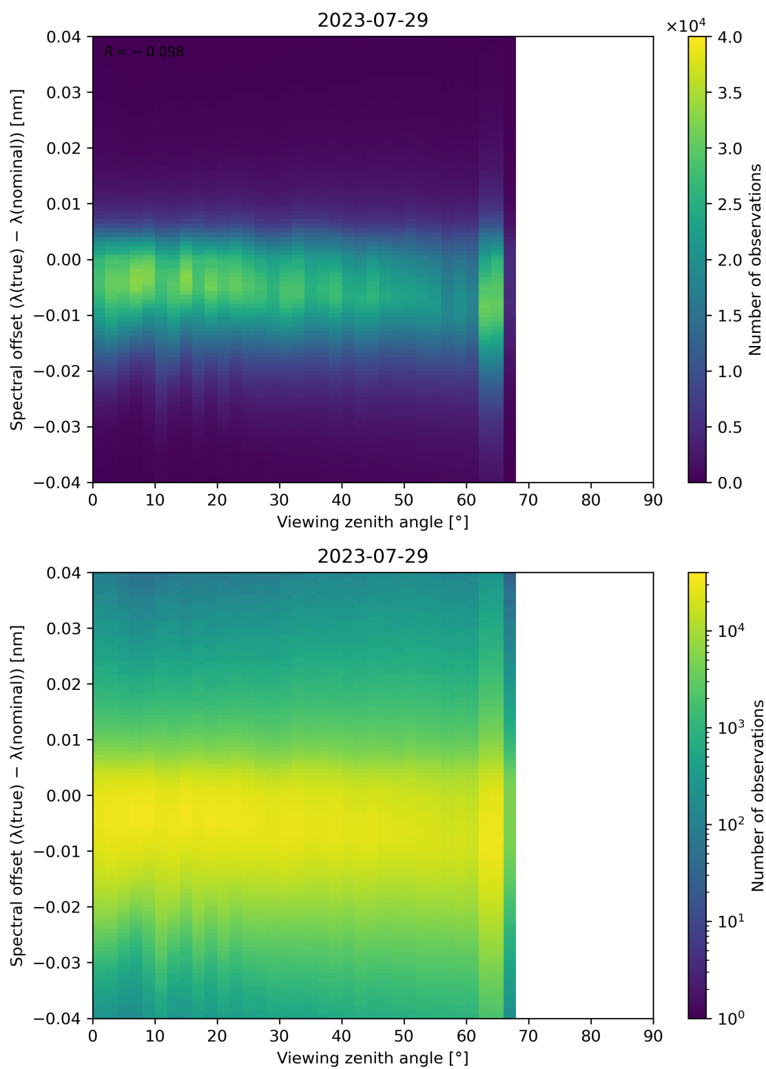
Figure 140: Scatter density plot of “Viewing zenith angle” against “Spectral offset ( \lambda(\text{true}) - \lambda(\text{nominal}) )” for 2023-07-29 to 2023-07-30.
