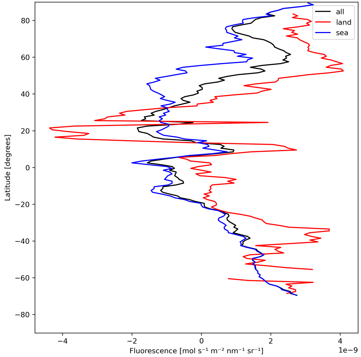
Figure 23: Zonal average of “Fluorescence” for 2023-07-29 to 2023-07-30.
