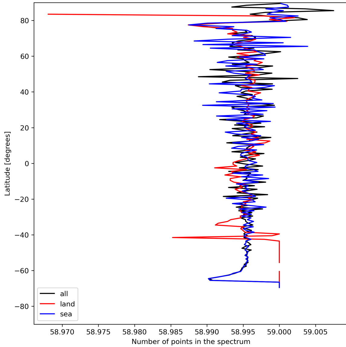
Figure 27: Zonal average of “Number of points in the spectrum” for 2023-07-29 to 2023-07-30.
