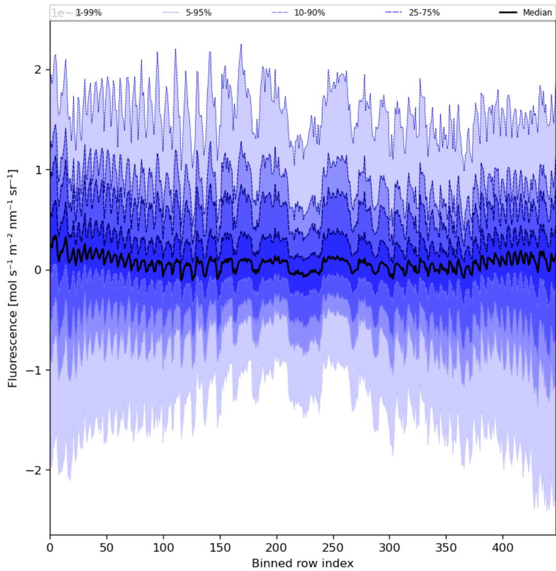
Figure 57: Along track statistics of “Fluorescence” for 2023-07-29 to 2023-07-30
