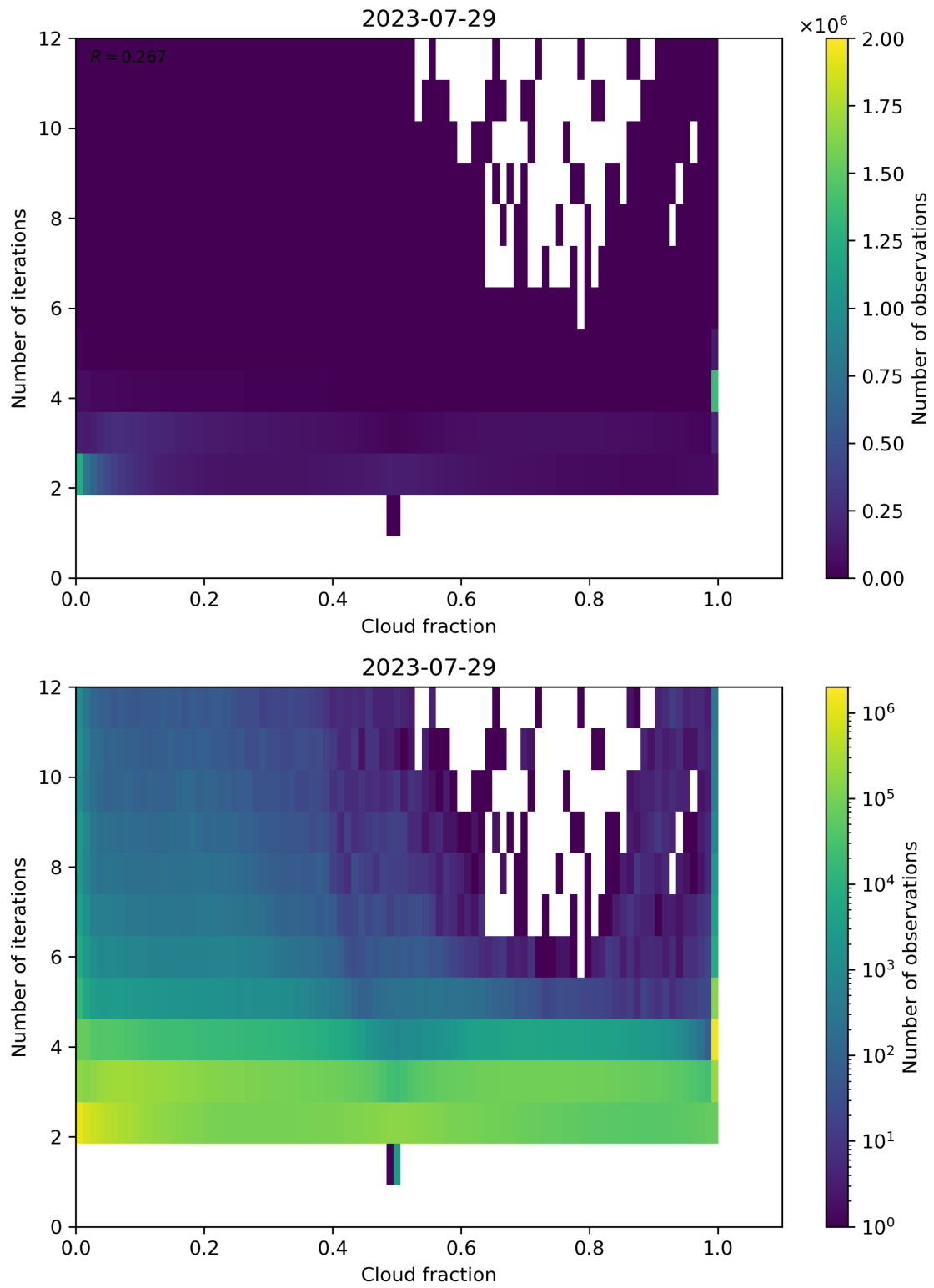
Figure 80: Scatter density plot of “Cloud fraction” against “Number of iterations” for 2023-07-29 to 2023-07-30.
