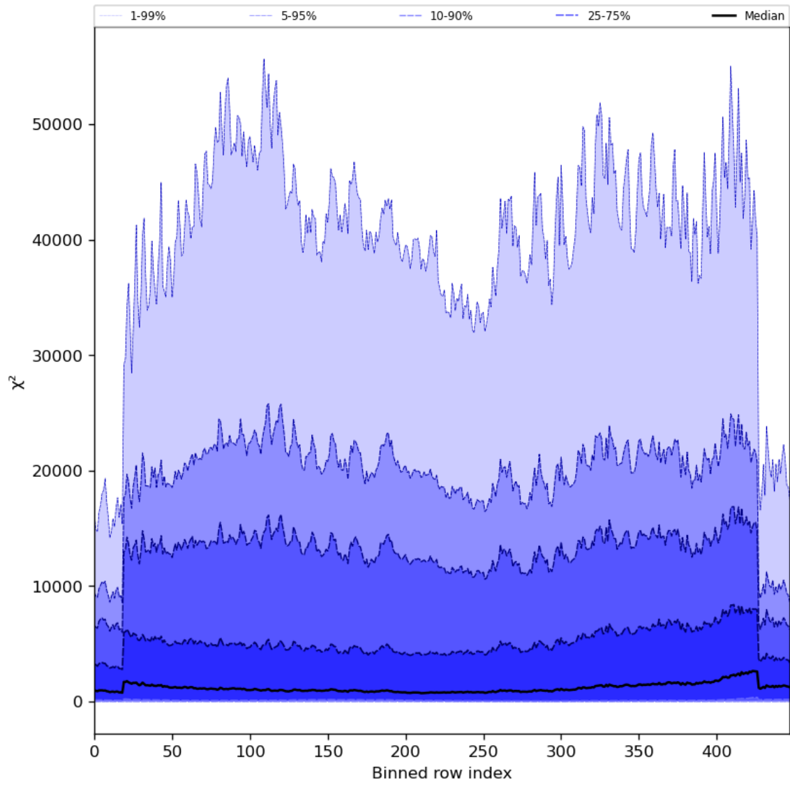
Figure 55: Along track statistics of “ \chi^2 ” for 2023-07-29 to 2023-07-30
