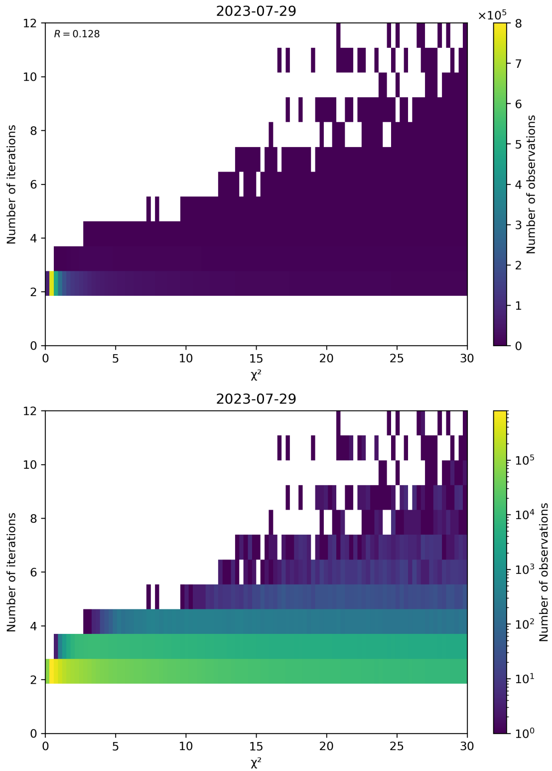
Figure 73: Scatter density plot of “ \chi^2 ” against “Number of iterations” for 2023-07-29 to 2023-07-30.
