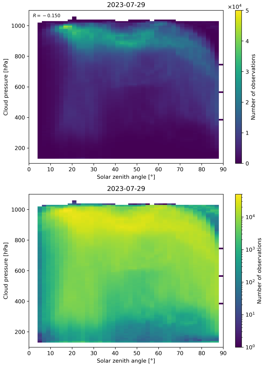
Figure 122: Scatter density plot of “Solar zenith angle” against “Cloud pressure” for 2023-07-29 to 2023-07-30.
