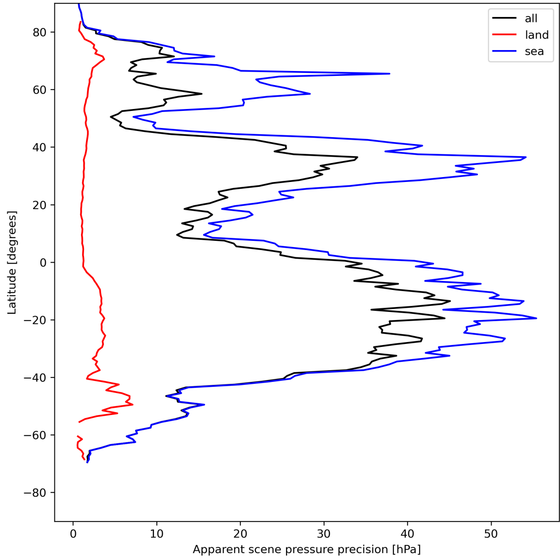
Figure 20: Zonal average of “Apparent scene pressure precision” for 2023-07-29 to 2023-07-30.
