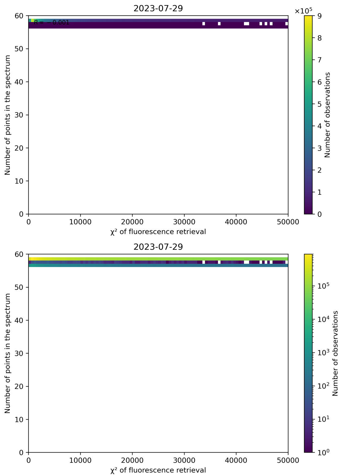
Figure 71: Scatter density plot of “ \chi^2 of fluorescence retrieval” against “Number of points in the spectrum” for 2023-07-29 to 2023-07-30.
