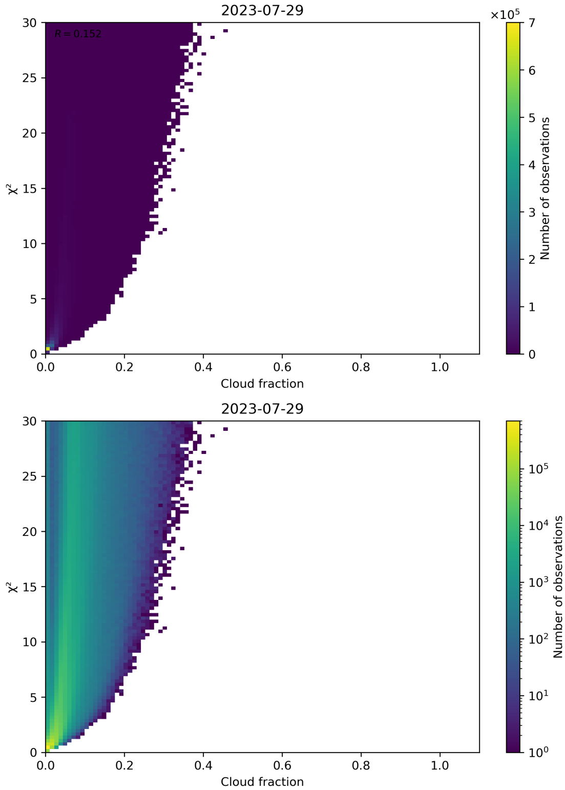
Figure 77: Scatter density plot of “Cloud fraction” against “ \chi^2 ” for 2023-07-29 to 2023-07-30.
