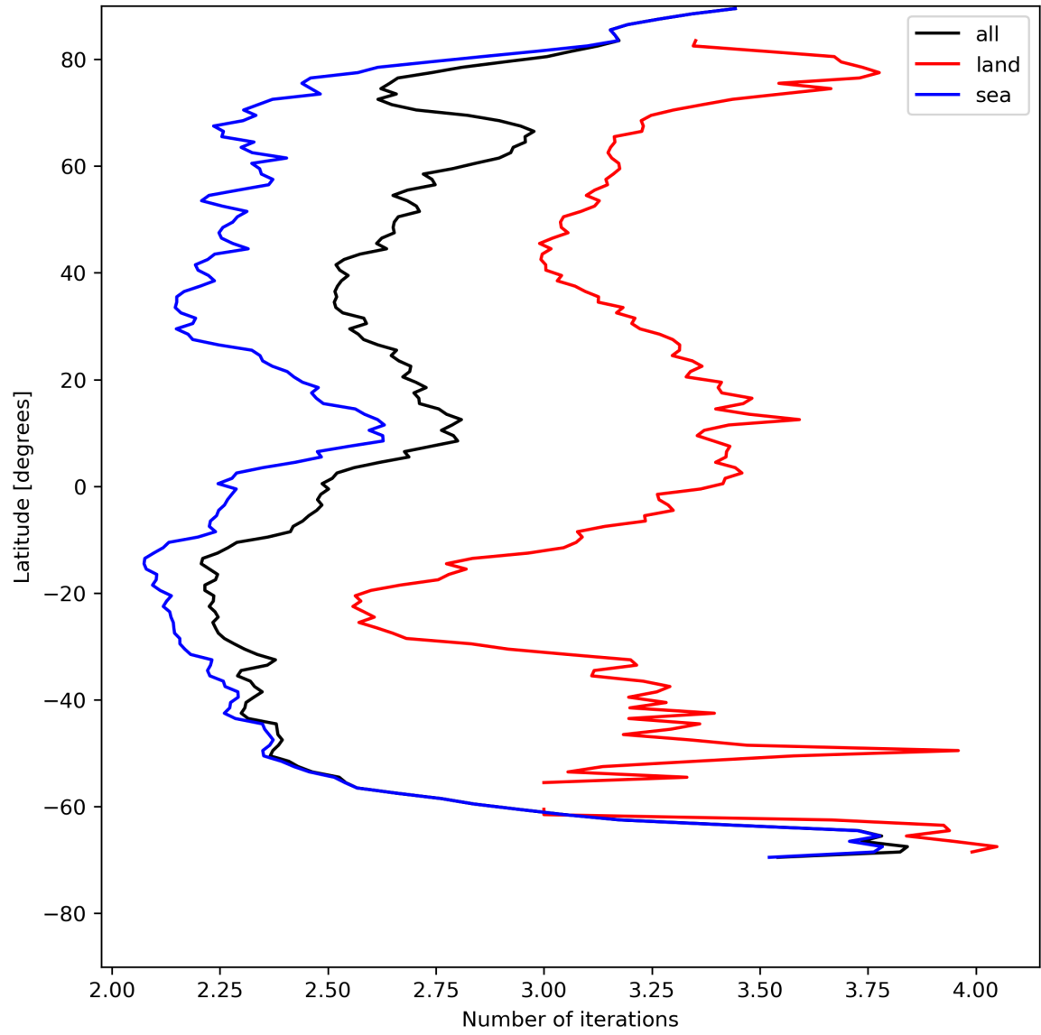
Figure 22: Zonal average of “Number of iterations” for 2023-07-29 to 2023-07-30.
