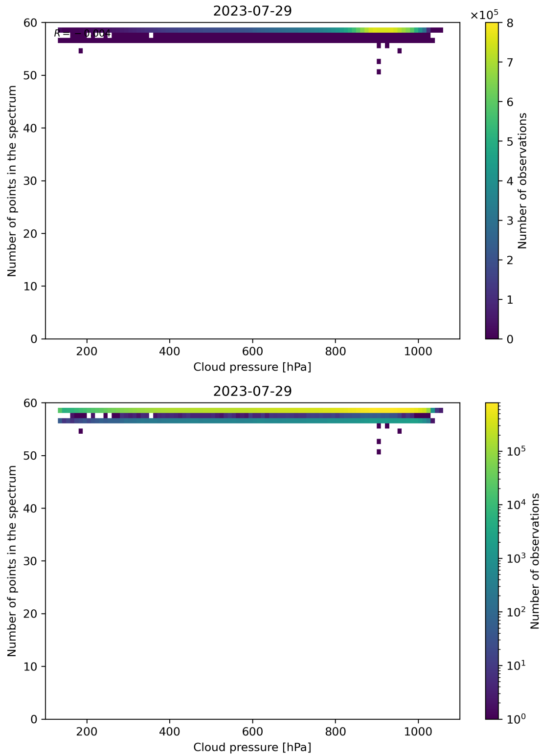
Figure 90: Scatter density plot of “Cloud pressure” against “Number of points in the spectrum” for 2023-07-29 to 2023-07-30.
