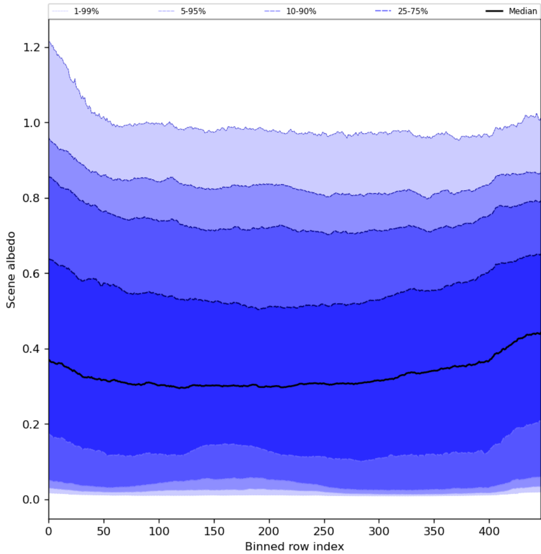
Figure 51: Along track statistics of “Scene albedo” for 2023-07-29 to 2023-07-30
