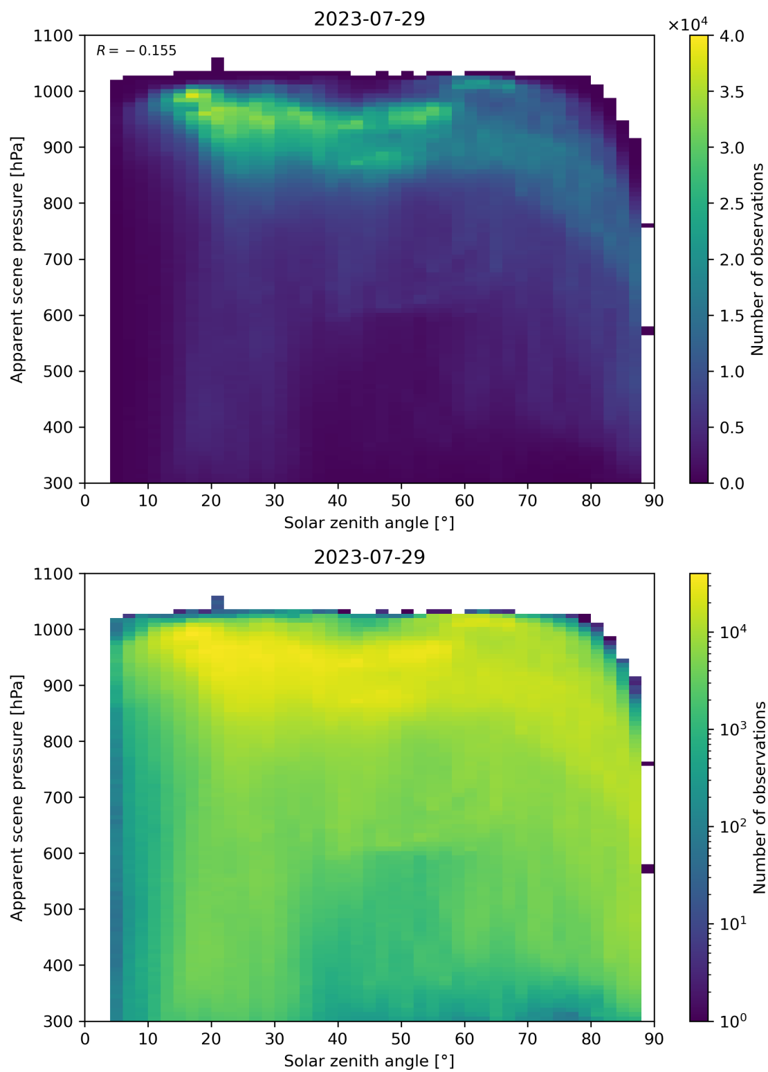
Figure 118: Scatter density plot of “Solar zenith angle” against “Apparent scene pressure” for 2023-07-29 to 2023-07-30.
