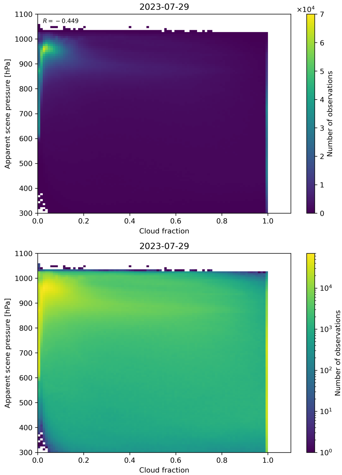
Figure 76: Scatter density plot of “Cloud fraction” against “Apparent scene pressure” for 2023-07-29 to 2023-07-30.
