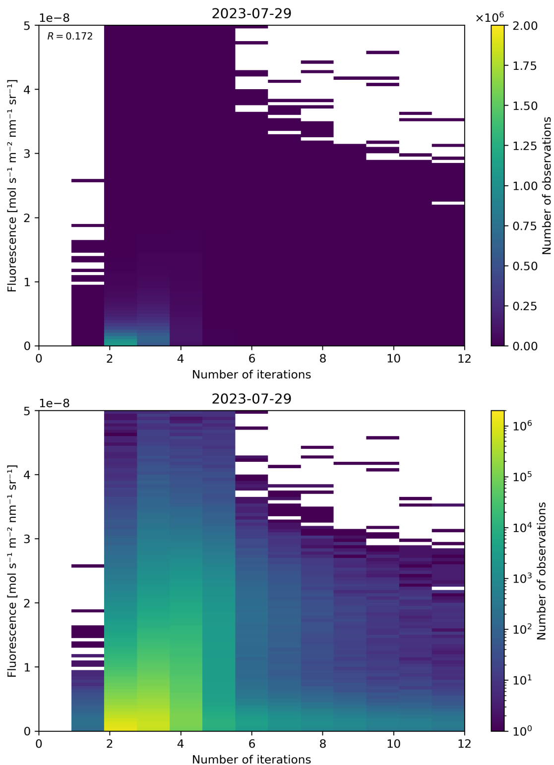
Figure 107: Scatter density plot of “Number of iterations” against “Fluorescence” for 2023-07-29 to 2023-07-30.
