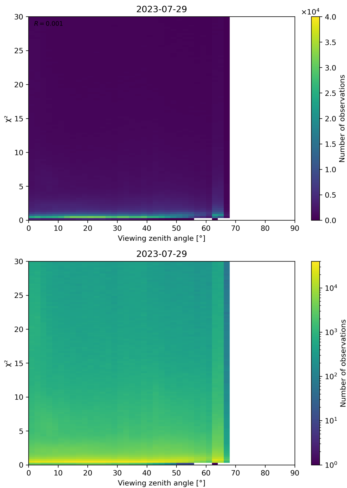
Figure 130: Scatter density plot of “Viewing zenith angle” against “ \chi^2 ” for 2023-07-29 to 2023-07-30.
