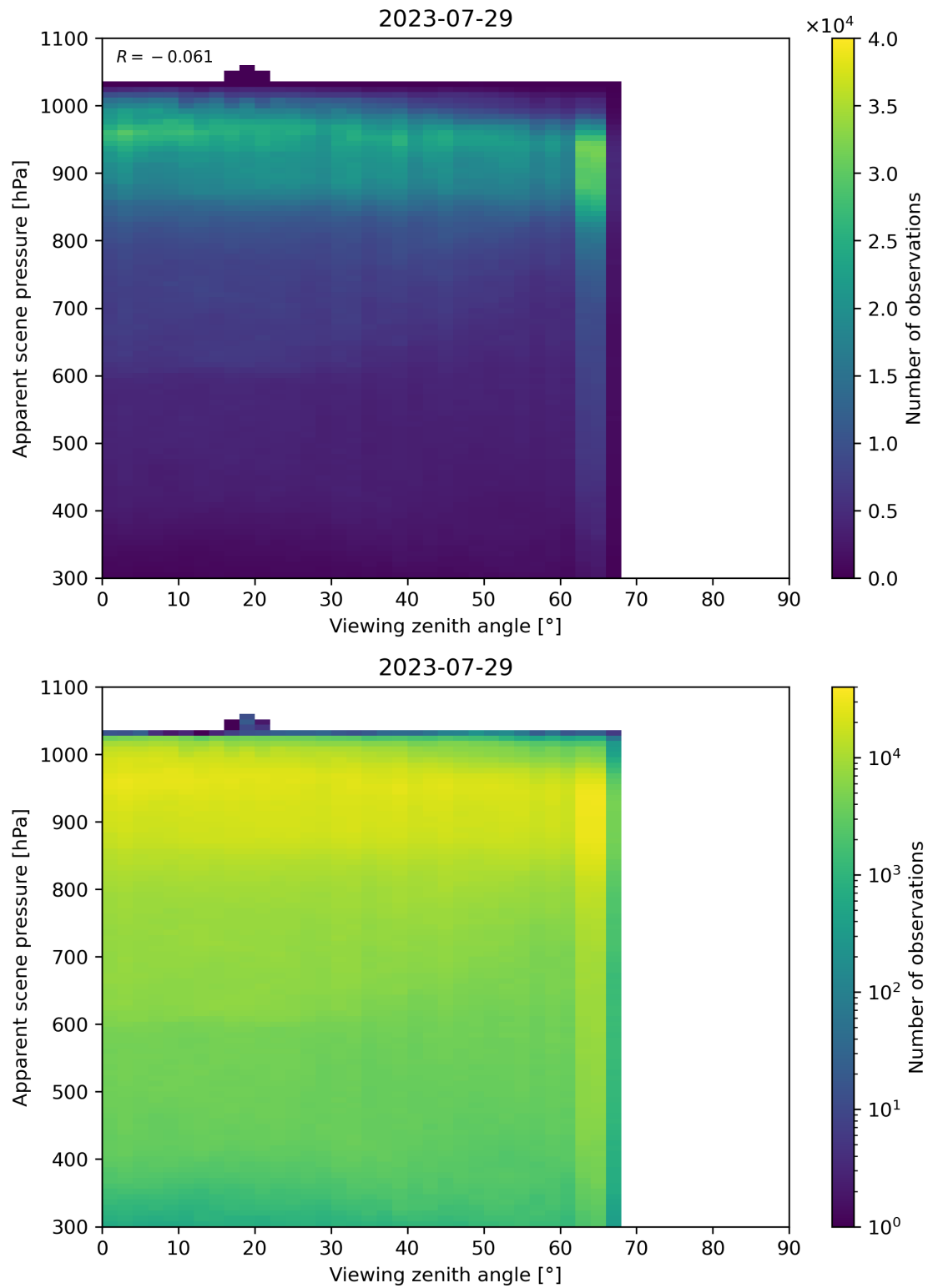
Figure 129: Scatter density plot of “Viewing zenith angle” against “Apparent scene pressure” for 2023-07-29 to 2023-07-30.
