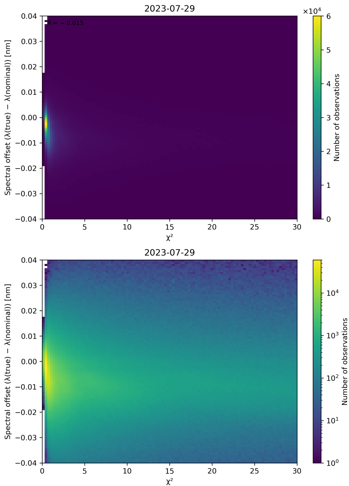
Figure 75: Scatter density plot of “ \chi^2 ” against “Spectral offset ( \lambda(\text{true}) - \lambda(\text{nominal}) )” for 2023-07-29 to 2023-07-30.
