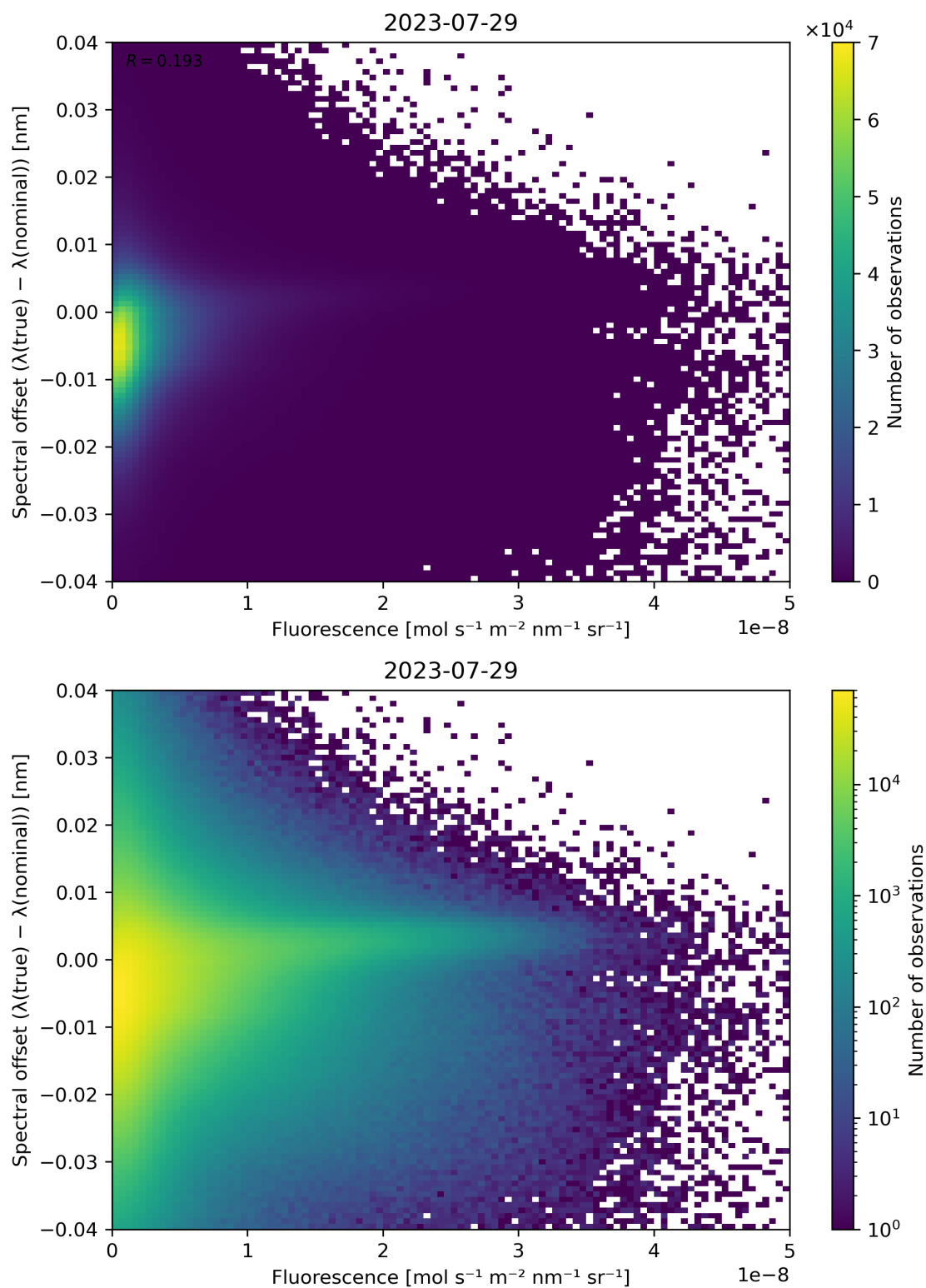
Figure 95: Scatter density plot of “Fluorescence” against “Spectral offset ( \lambda(\text{true}) - \lambda(\text{nominal}) )” for 2023-07-29 to 2023-07-30.
