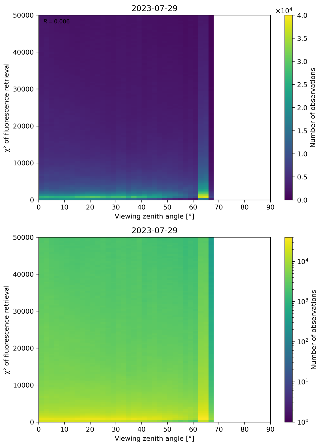
Figure 131: Scatter density plot of “Viewing zenith angle” against “ \chi^2 of fluorescence retrieval” for 2023-07-29 to 2023-07-30.
