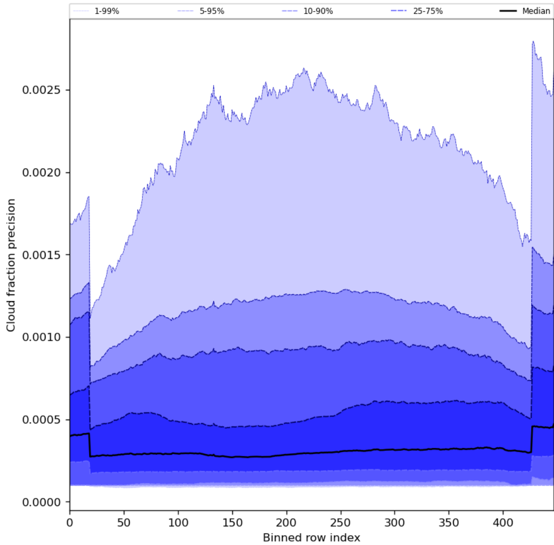
Figure 50: Along track statistics of “Cloud fraction precision” for 2023-07-29 to 2023-07-30
