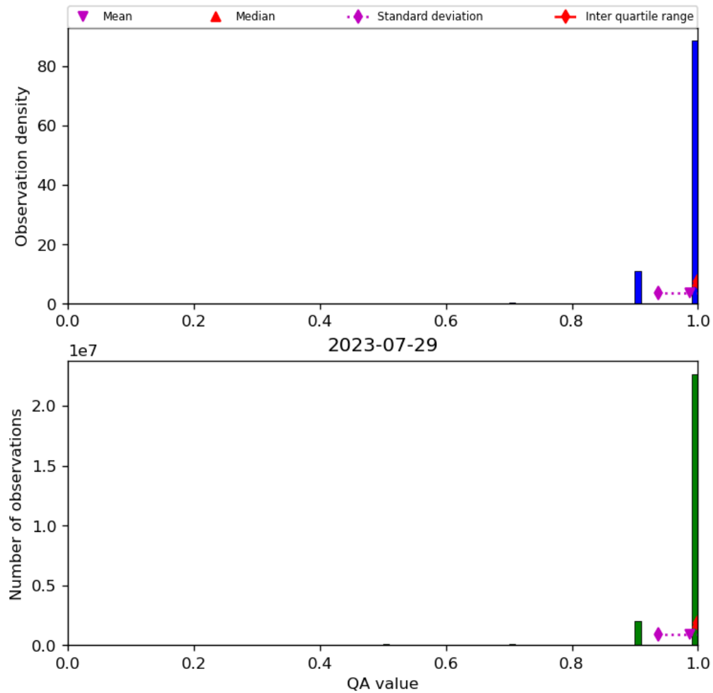
Figure 29: Histogram of “QA value” for 2023-07-29 to 2023-07-30
