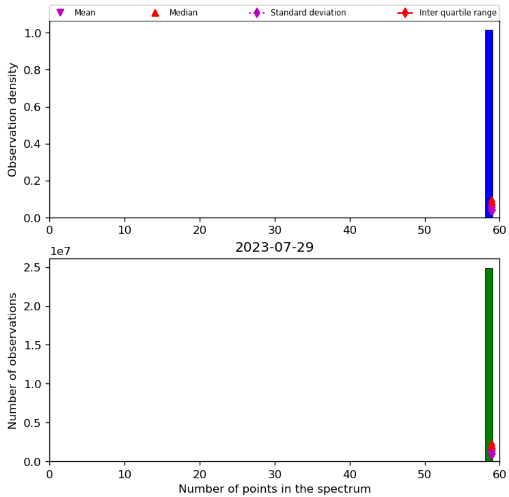
Figure 44: Histogram of “Number of points in the spectrum” for 2023-07-29 to 2023-07-30
