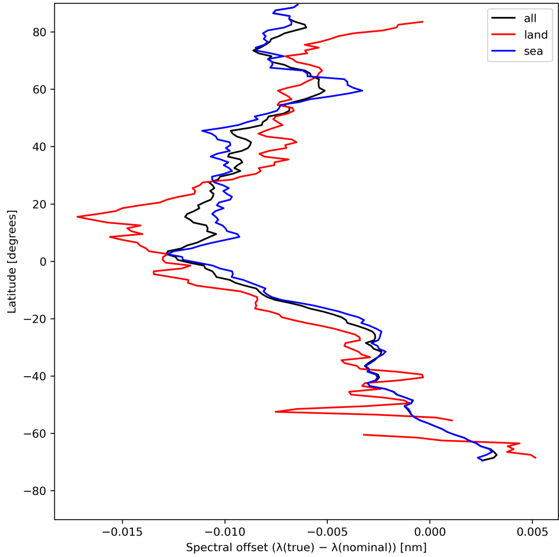
Figure 28: Zonal average of “Spectral offset ( \lambda(\text{true}) - \lambda(\text{nominal}) )” for 2023-07-29 to 2023-07-30.
