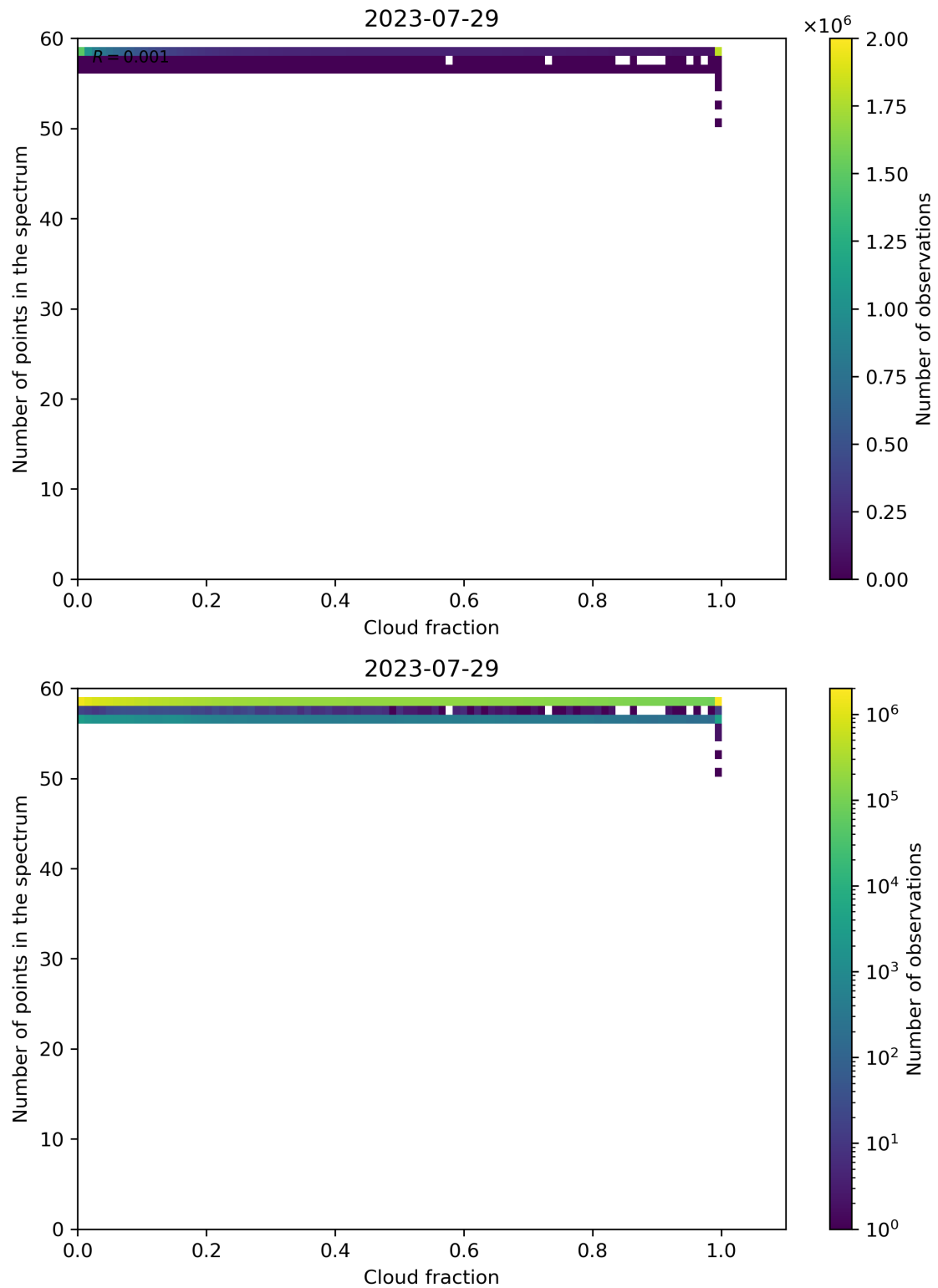
Figure 81: Scatter density plot of “Cloud fraction” against “Number of points in the spectrum” for 2023-07-29 to 2023-07-30.
