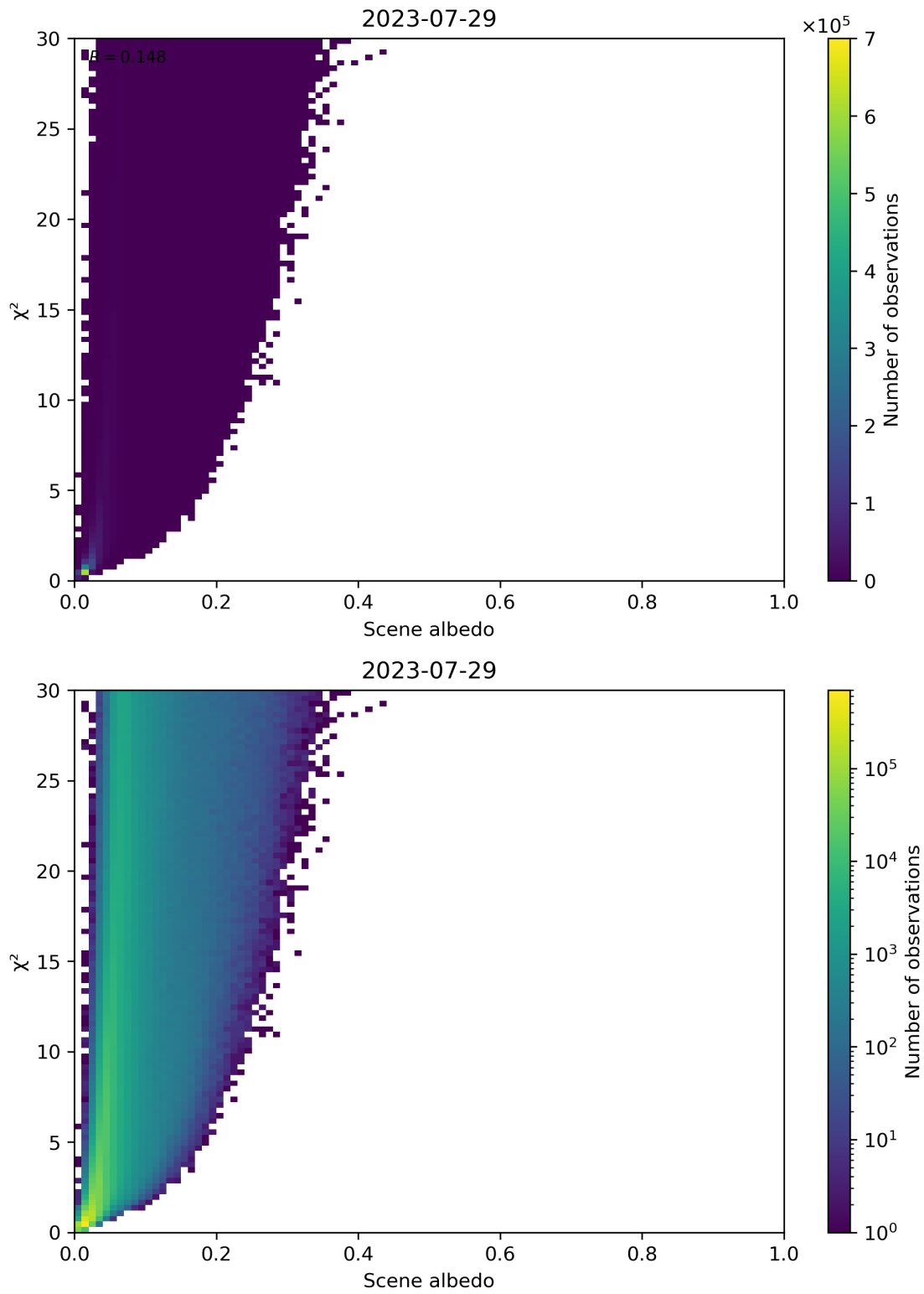
Figure 112: Scatter density plot of “Scene albedo” against “ \chi^2 ” for 2023-07-29 to 2023-07-30.
