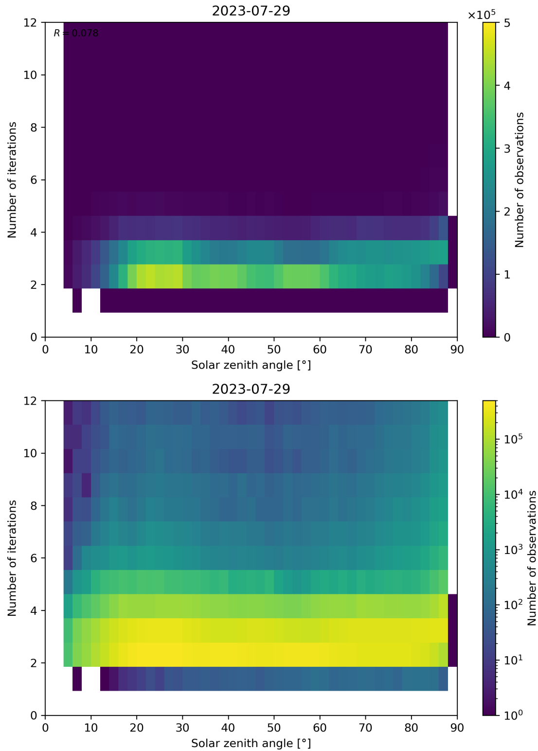
Figure 125: Scatter density plot of “Solar zenith angle” against “Number of iterations” for 2023-07-29 to 2023-07-30.
