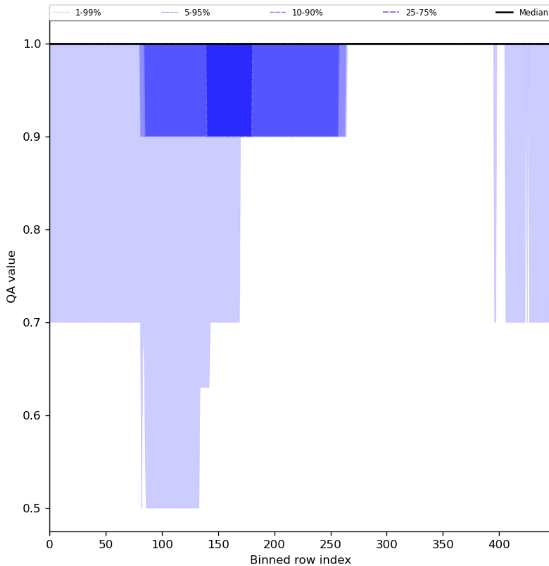
Figure 46: Along track statistics of “QA value” for 2023-07-29 to 2023-07-30
