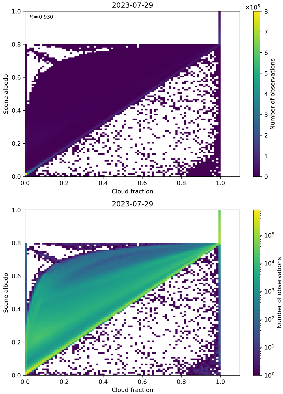
Figure 82: Scatter density plot of “Cloud fraction” against “Scene albedo” for 2023-07-29 to 2023-07-30.
