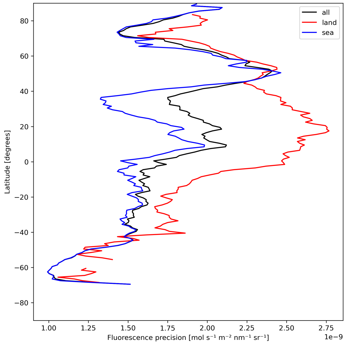
Figure 24: Zonal average of “Fluorescence precision” for 2023-07-29 to 2023-07-30.
