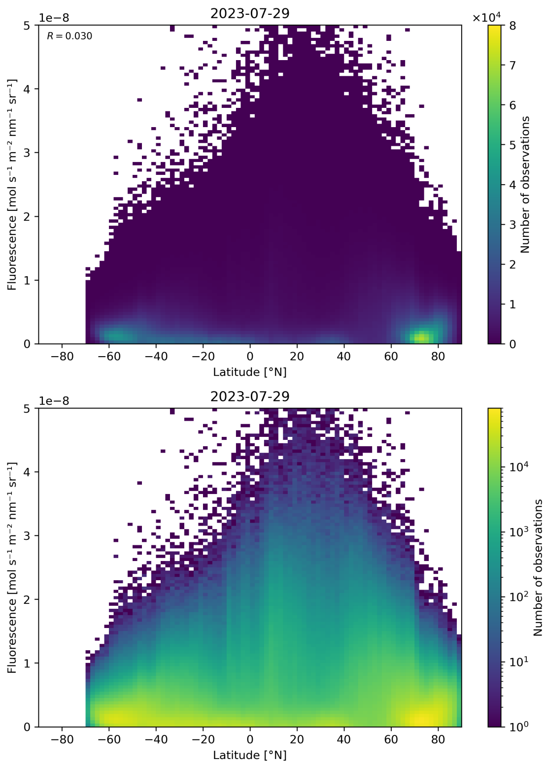
Figure 101: Scatter density plot of “Latitude” against “Fluorescence” for 2023-07-29 to 2023-07-30.
