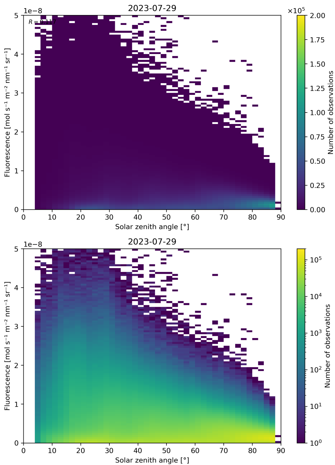
Figure 123: Scatter density plot of “Solar zenith angle” against “Fluorescence” for 2023-07-29 to 2023-07-30.
