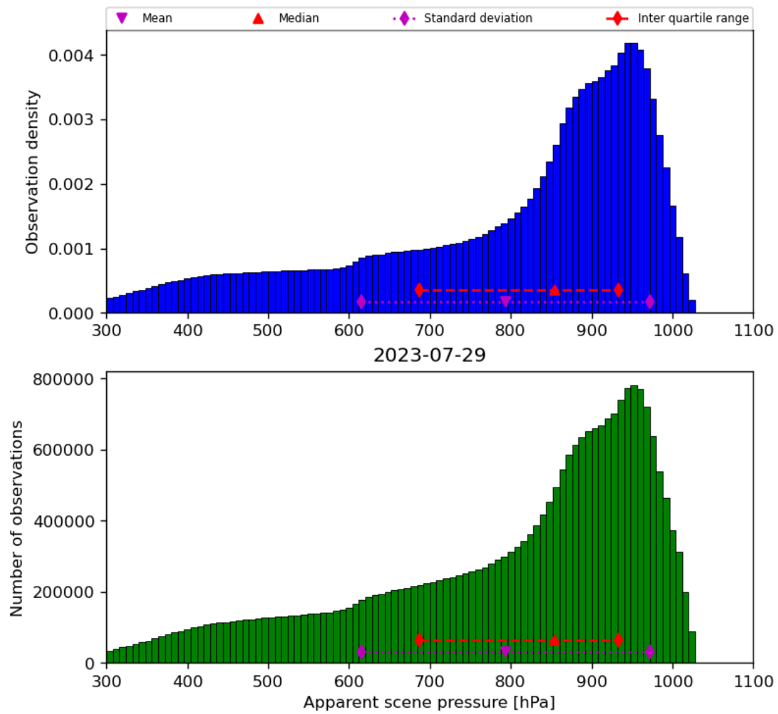
Figure 36: Histogram of “Apparent scene pressure” for 2023-07-29 to 2023-07-30
