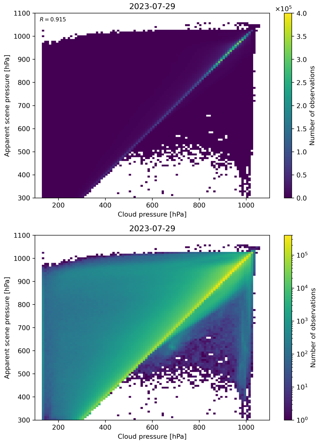
Figure 84: Scatter density plot of “Cloud pressure” against “Apparent scene pressure” for 2023-07-29 to 2023-07-30.
