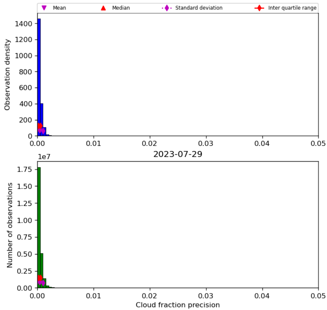
Figure 33: Histogram of “Cloud fraction precision” for 2023-07-29 to 2023-07-30
