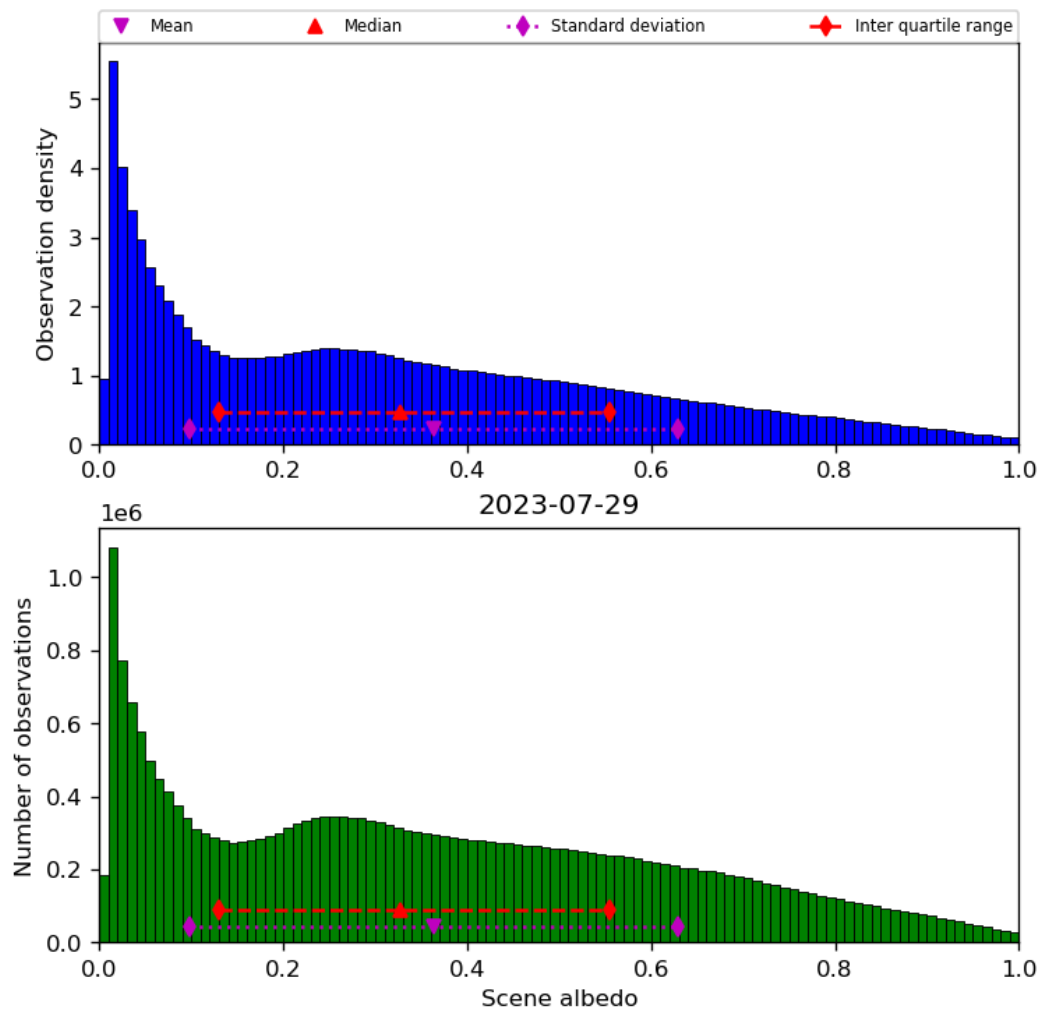
Figure 34: Histogram of “Scene albedo” for 2023-07-29 to 2023-07-30
