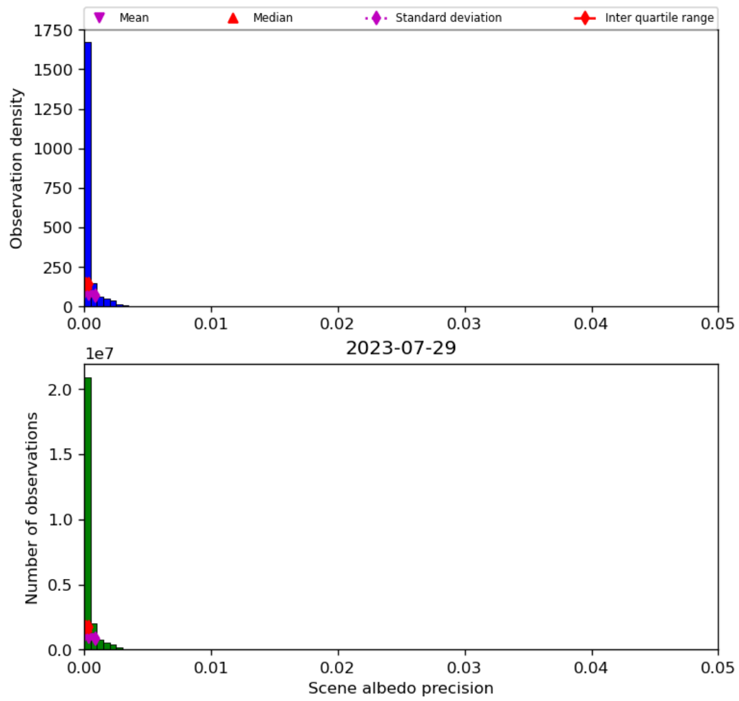
Figure 35: Histogram of “Scene albedo precision” for 2023-07-29 to 2023-07-30
