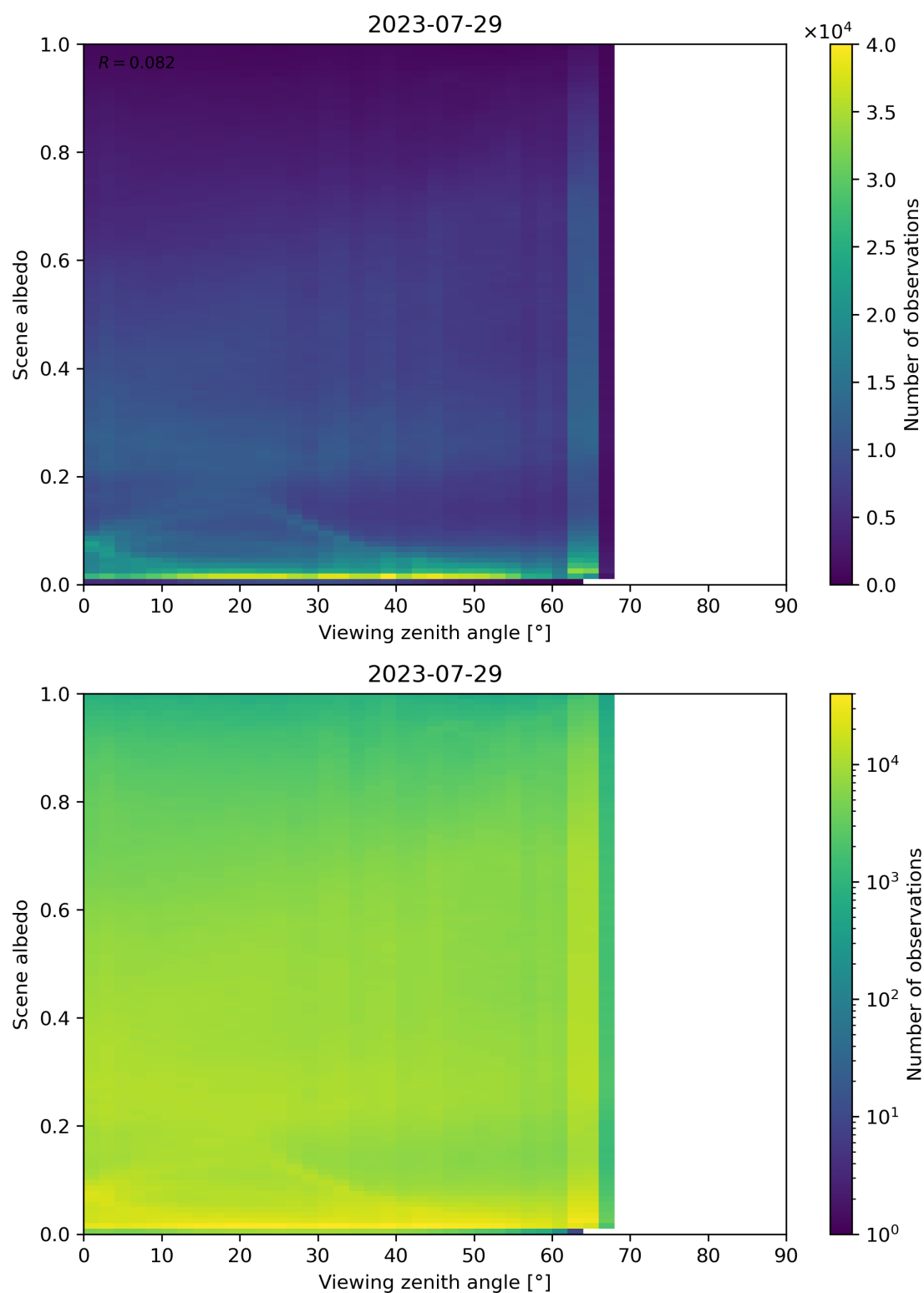
Figure 138: Scatter density plot of “Viewing zenith angle” against “Scene albedo” for 2023-07-29 to 2023-07-30.
