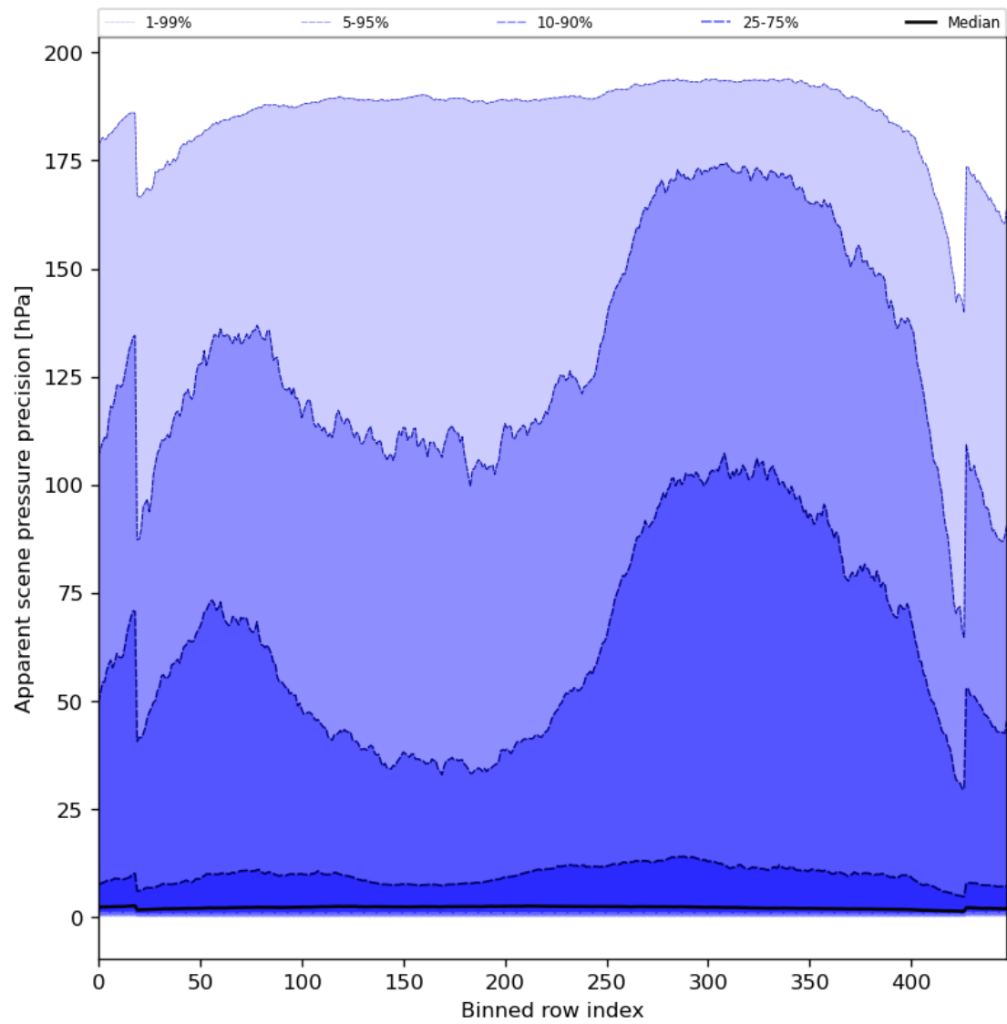
Figure 54: Along track statistics of “Apparent scene pressure precision” for 2023-07-29 to 2023-07-30
