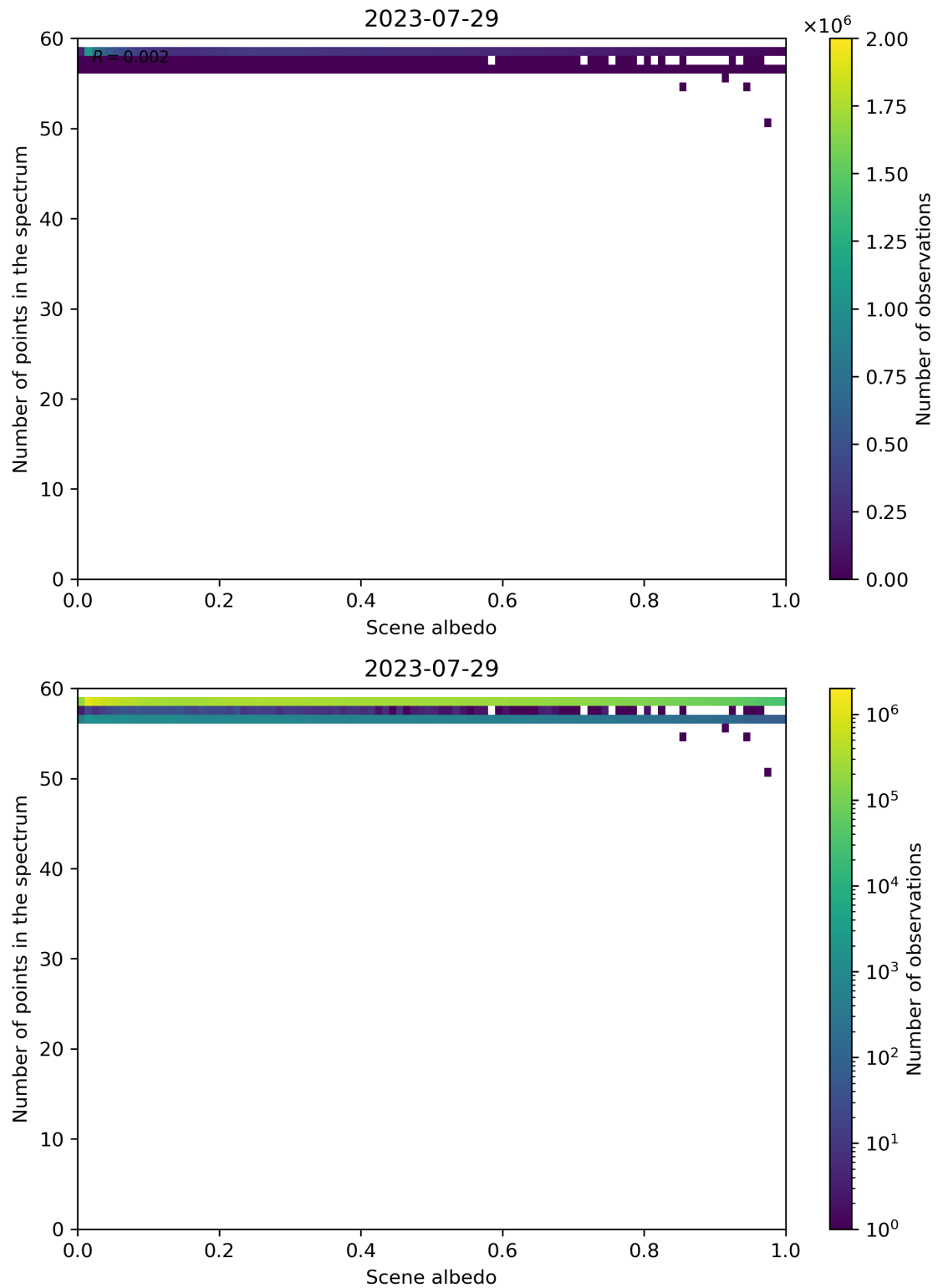
Figure 116: Scatter density plot of “Scene albedo” against “Number of points in the spectrum” for 2023-07-29 to 2023-07-30.
