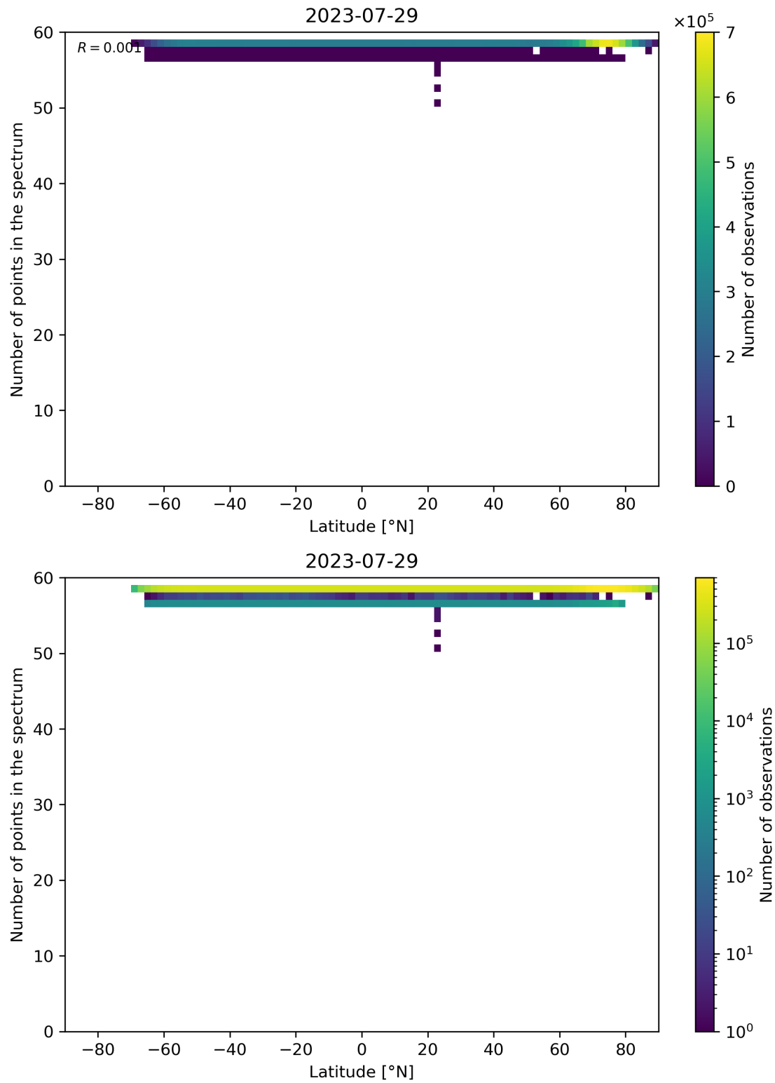
Figure 103: Scatter density plot of “Latitude” against “Number of points in the spectrum” for 2023-07-29 to 2023-07-30.
