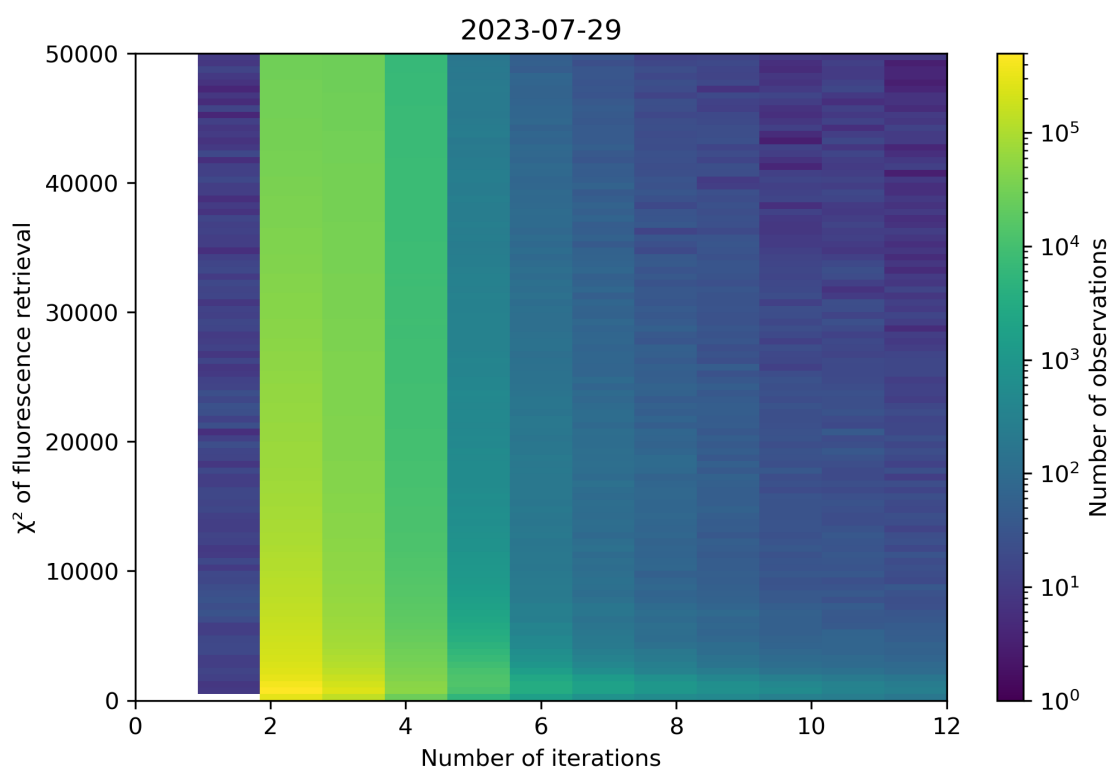
Figure 106: Scatter density plot of “Number of iterations” against “ \chi^2 of fluorescence retrieval” for 2023-07-29 to 2023-07-30.
