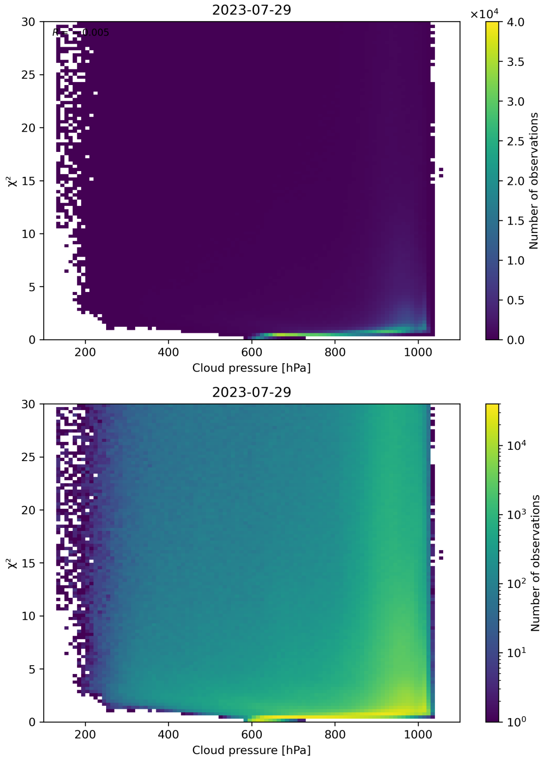
Figure 85: Scatter density plot of “Cloud pressure” against “ \chi^2 ” for 2023-07-29 to 2023-07-30.
