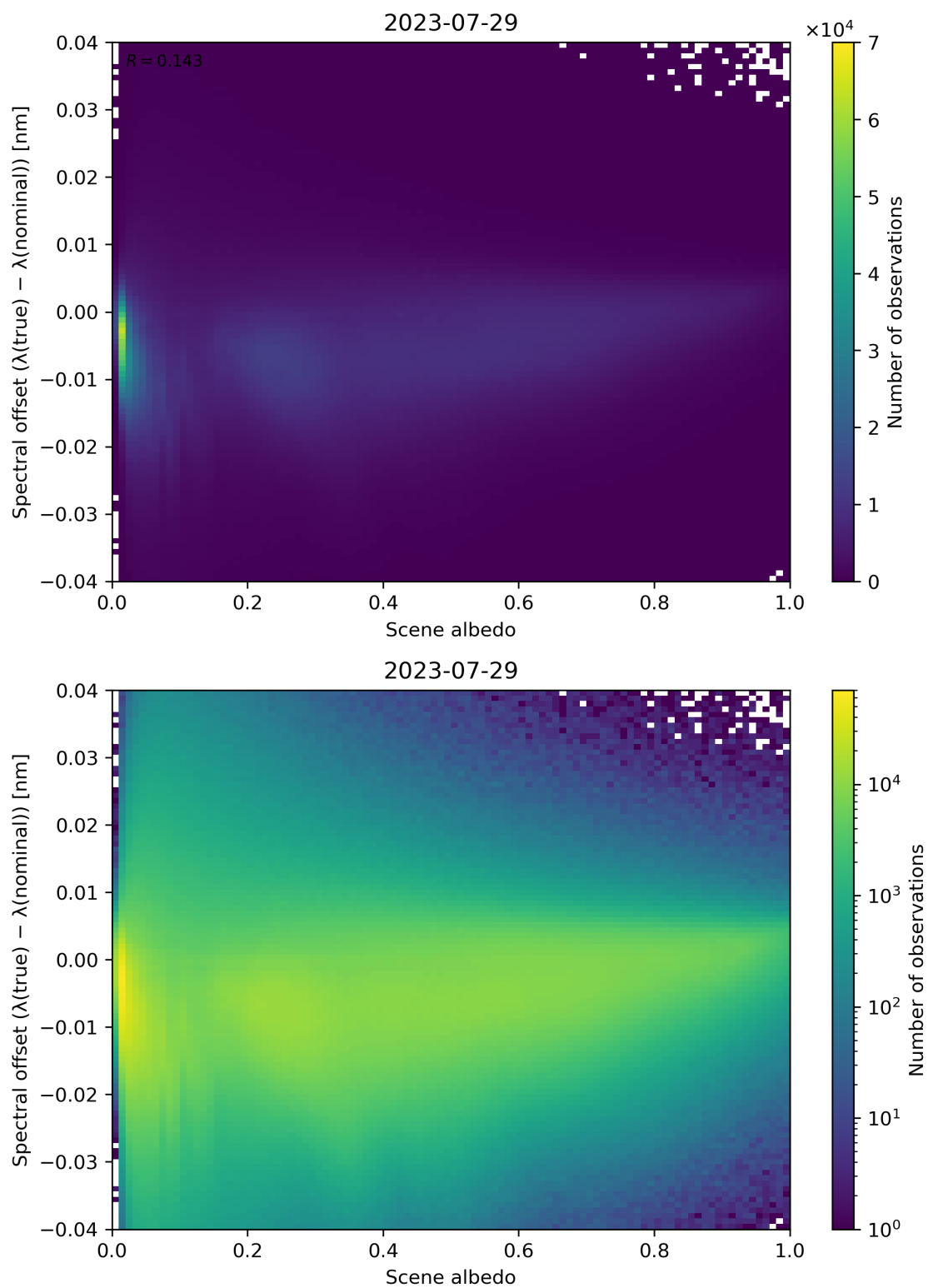
Figure 117: Scatter density plot of “Scene albedo” against “Spectral offset ( \lambda(\text{true}) - \lambda(\text{nominal}) )” for 2023-07-29 to 2023-07-30.
