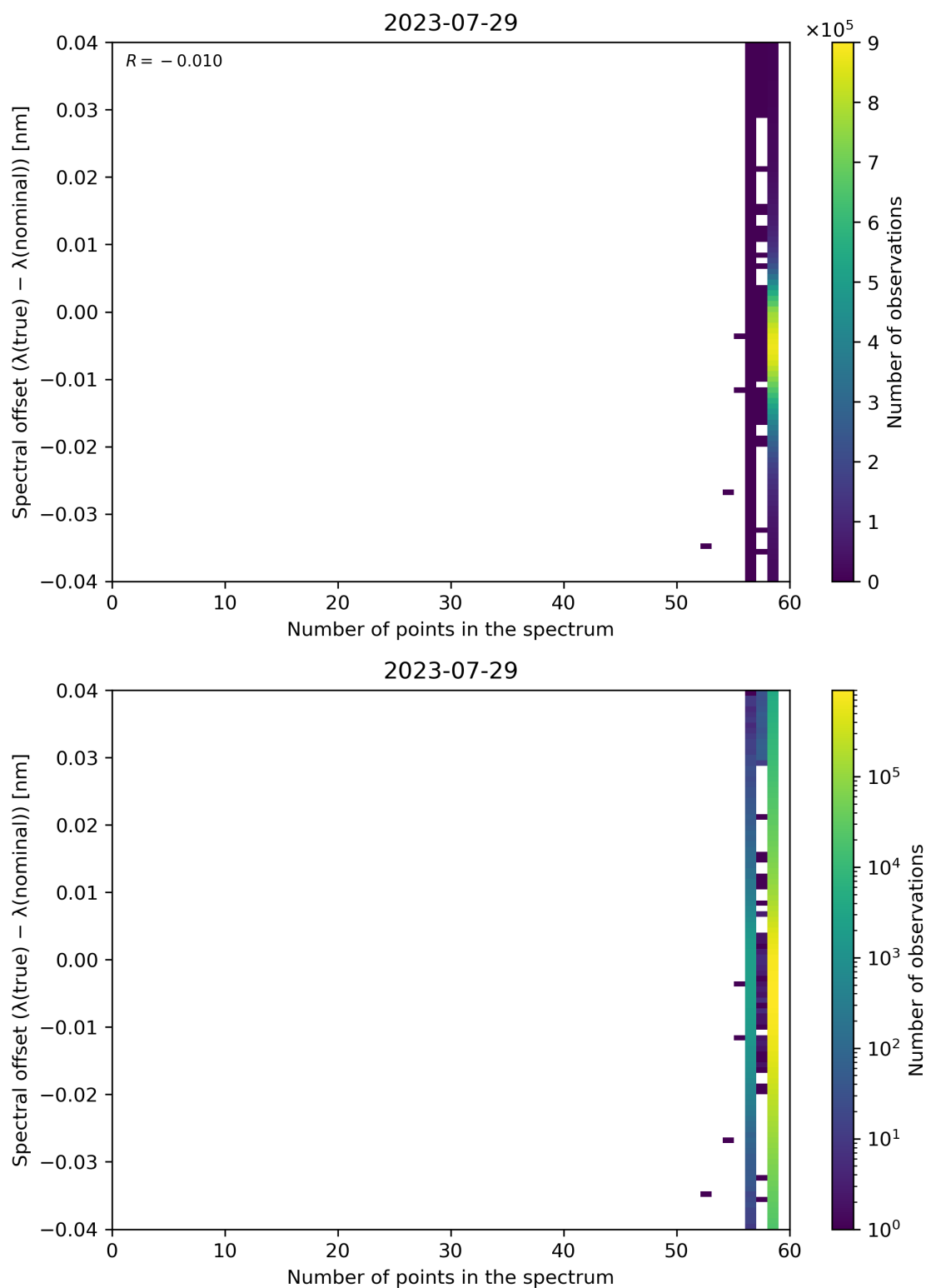
Figure 110: Scatter density plot of “Number of points in the spectrum” against “Spectral offset ( \lambda(\text{true}) - \lambda(\text{nominal}) )” for 2023-07-29 to 2023-07-30.
