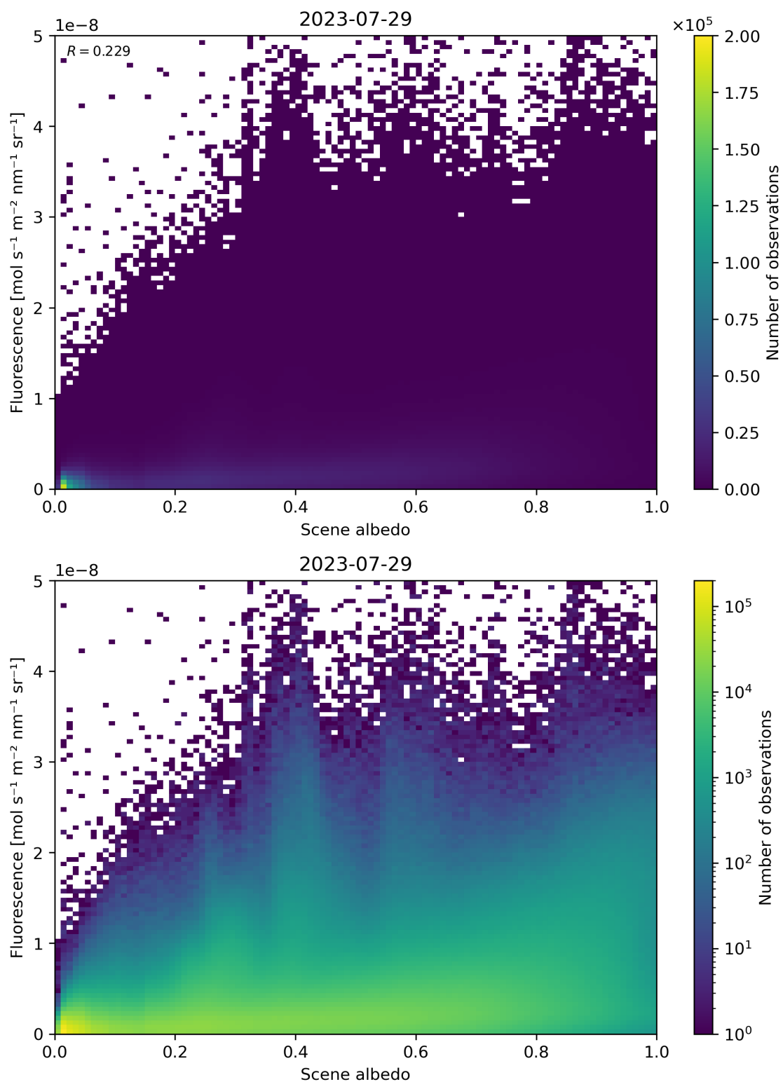
Figure 114: Scatter density plot of “Scene albedo” against “Fluorescence” for 2023-07-29 to 2023-07-30.
