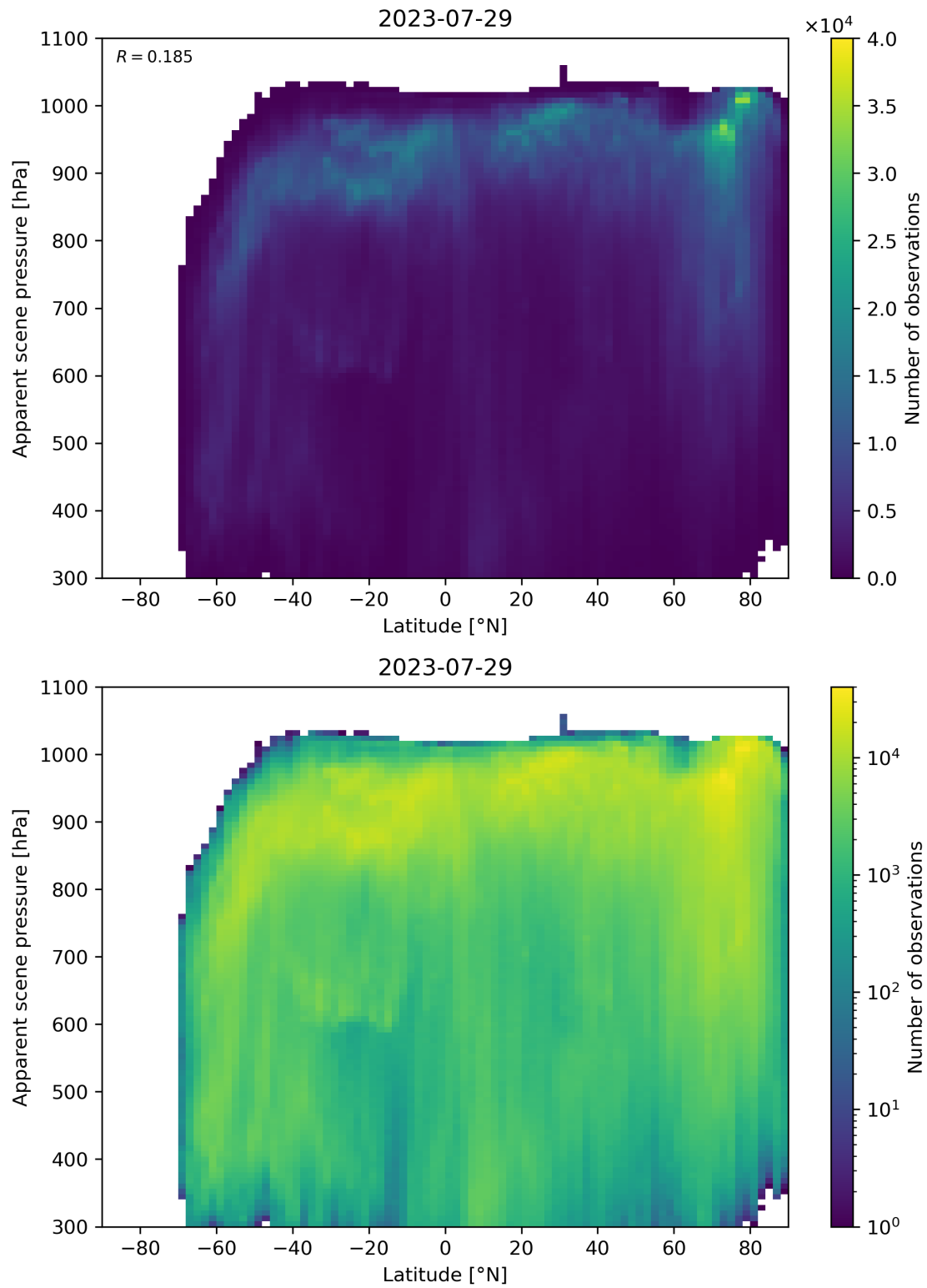
Figure 96: Scatter density plot of “Latitude” against “Apparent scene pressure” for 2023-07-29 to 2023-07-30.
