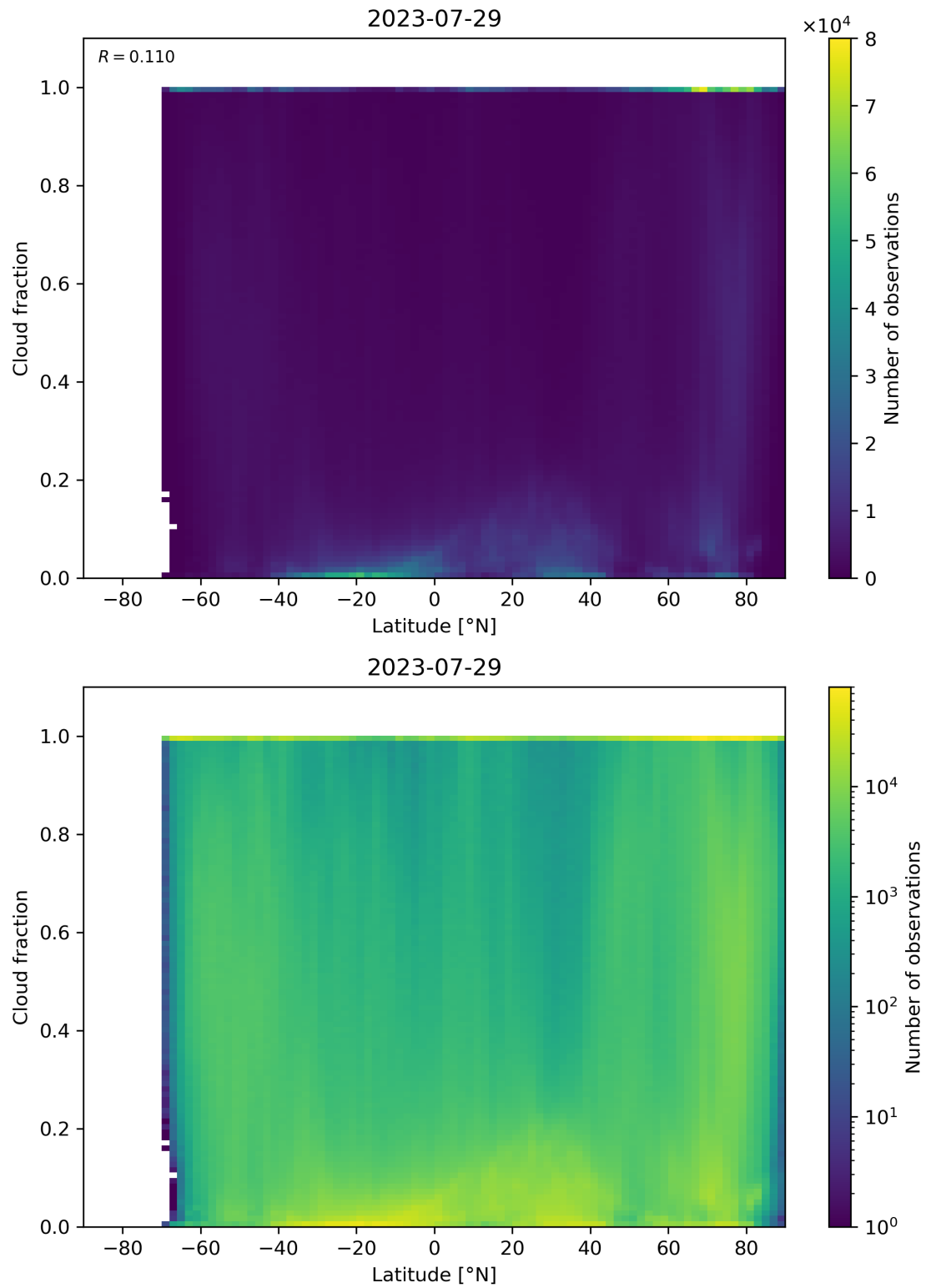
Figure 99: Scatter density plot of “Latitude” against “Cloud fraction” for 2023-07-29 to 2023-07-30.
