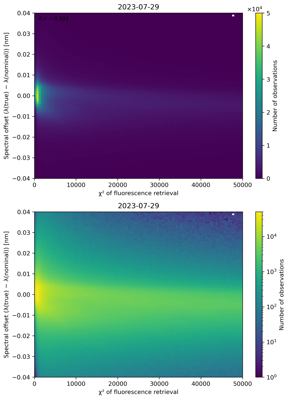
Figure 72: Scatter density plot of " \chi^2 of fluorescence retrieval" against "Spectral offset ( \lambda(\text{true}) - \lambda(\text{nominal}) )" for 2023-07-29 to 2023-07-30.
