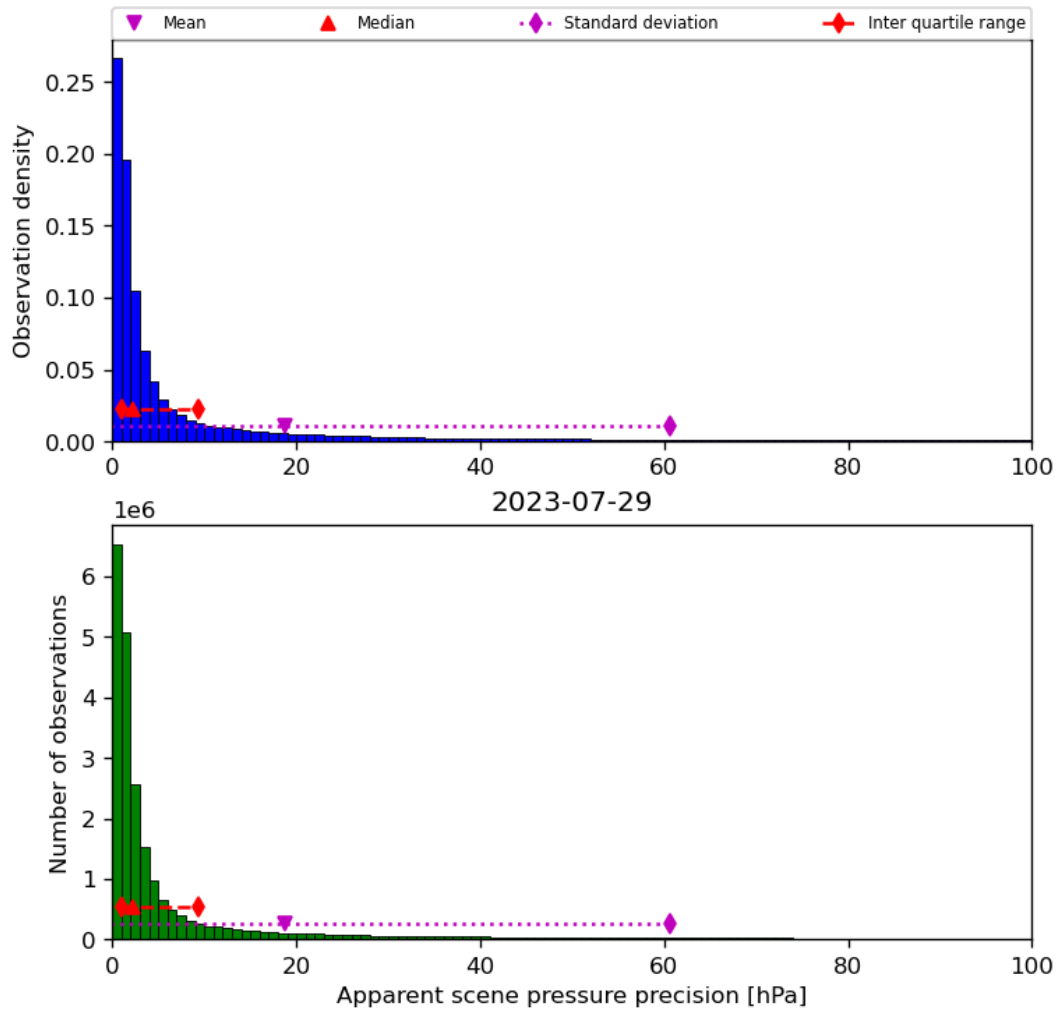
Figure 37: Histogram of “Apparent scene pressure precision” for 2023-07-29 to 2023-07-30
