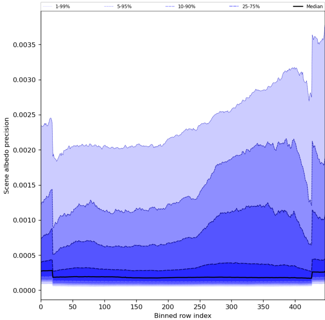
Figure 52: Along track statistics of “Scene albedo precision” for 2023-07-29 to 2023-07-30
