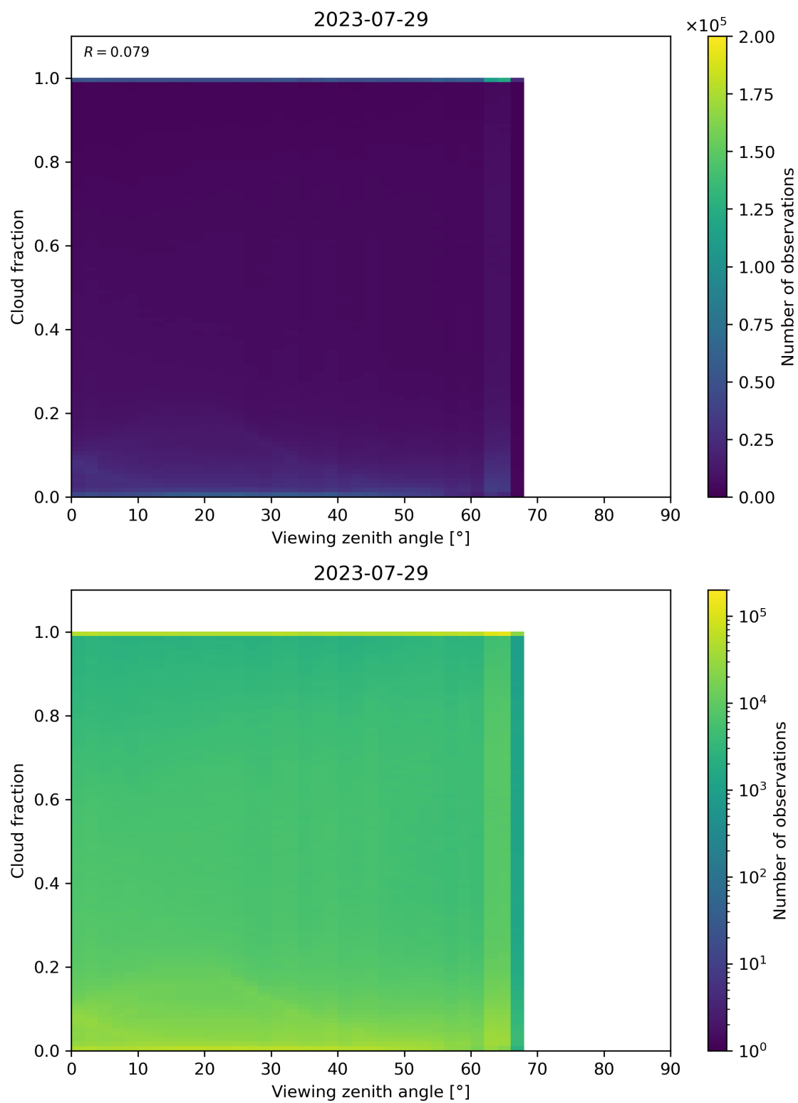
Figure 132: Scatter density plot of “Viewing zenith angle” against “Cloud fraction” for 2023-07-29 to 2023-07-30.
