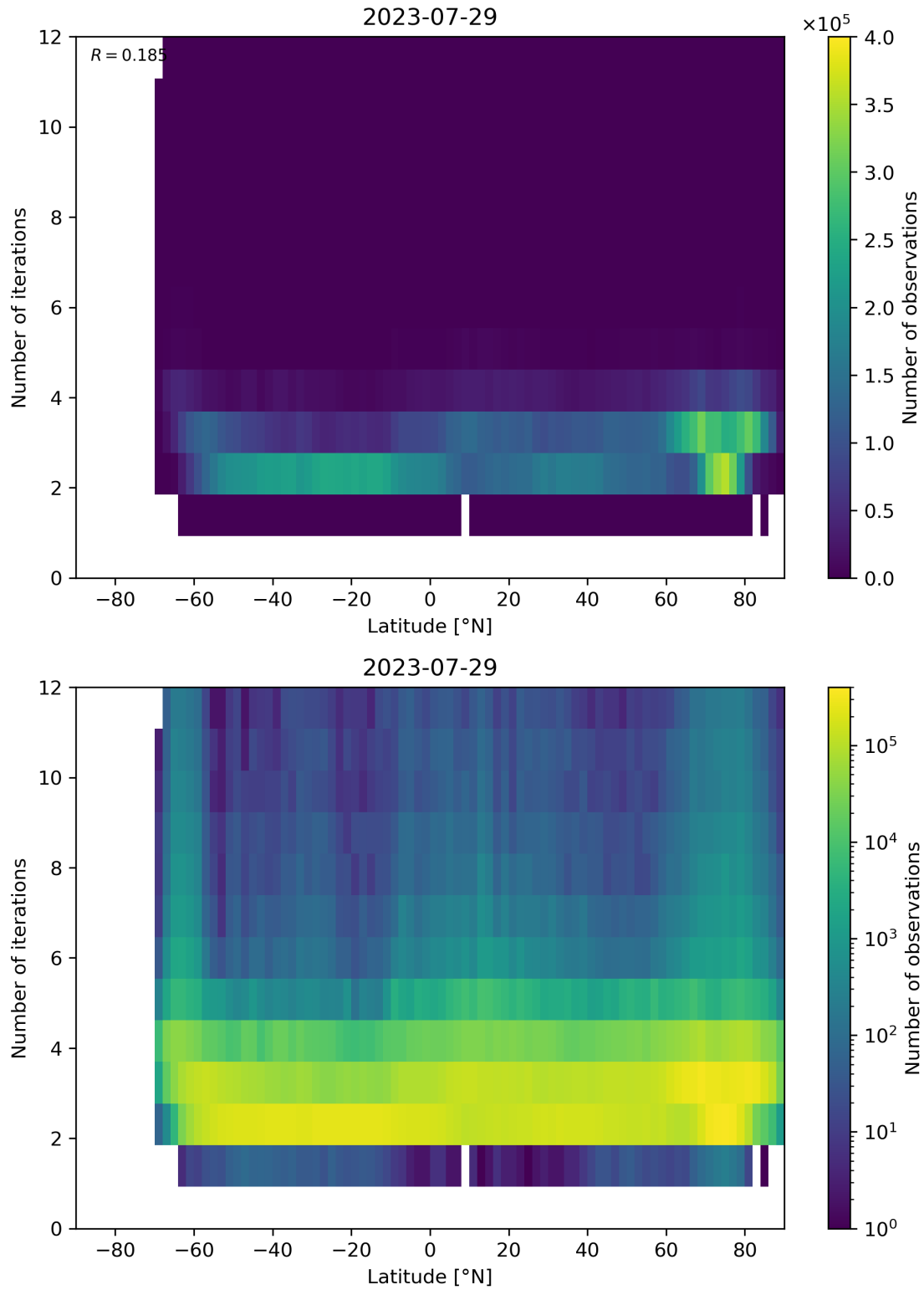
Figure 102: Scatter density plot of “Latitude” against “Number of iterations” for 2023-07-29 to 2023-07-30.
