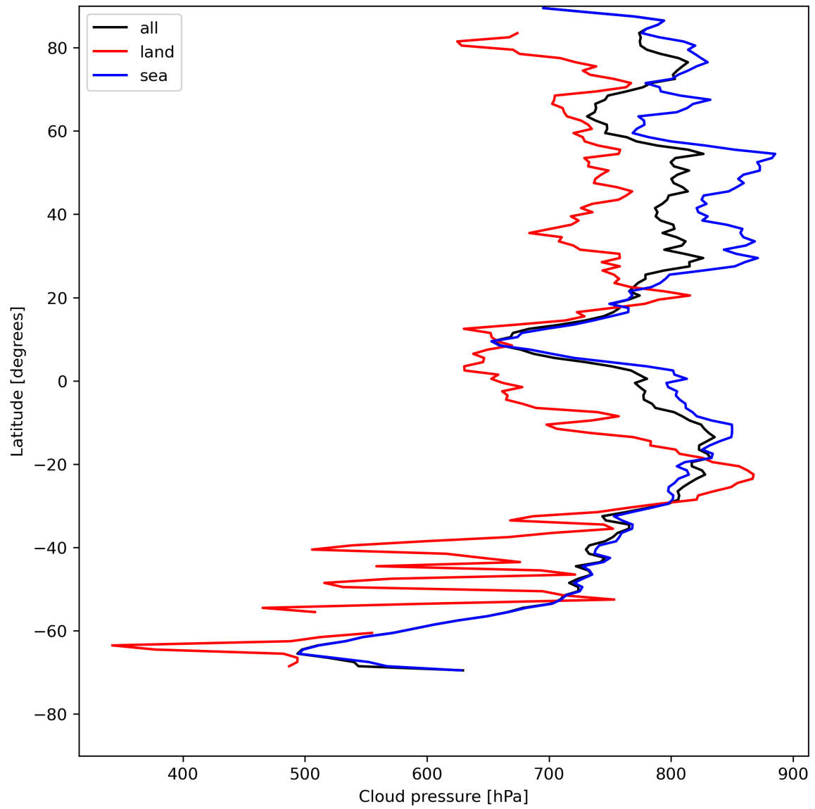
Figure 13: Zonal average of “Cloud pressure” for 2023-07-29 to 2023-07-30.
