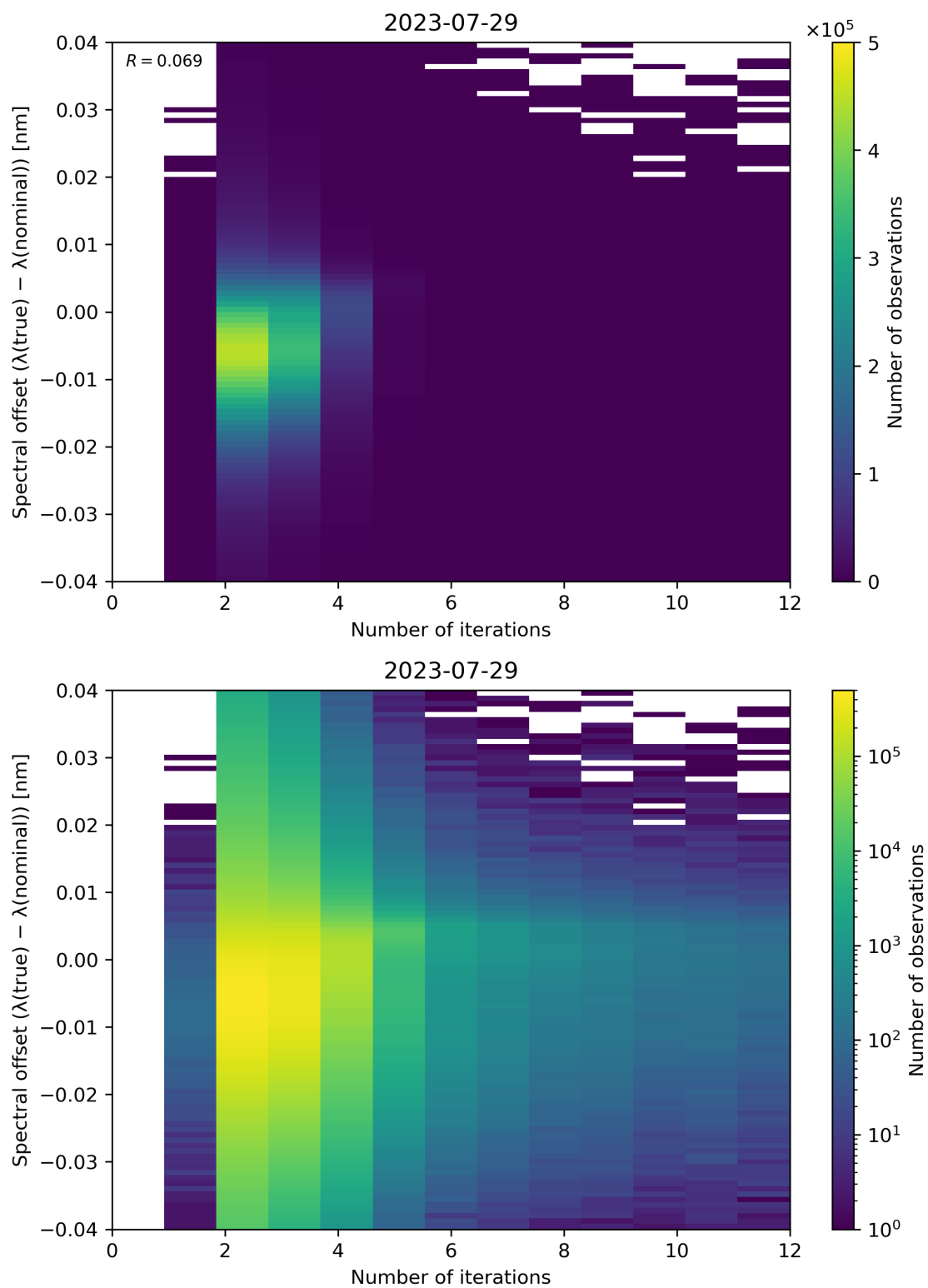
Figure 109: Scatter density plot of “Number of iterations” against “Spectral offset ( \lambda(\text{true}) - \lambda(\text{nominal}) )” for 2023-07-29 to 2023-07-30.
