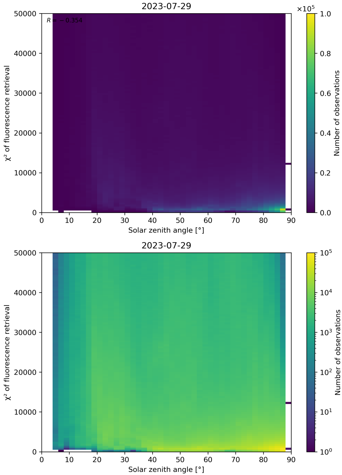
Figure 120: Scatter density plot of “Solar zenith angle” against “ \chi^2 of fluorescence retrieval” for 2023-07-29 to 2023-07-30.
