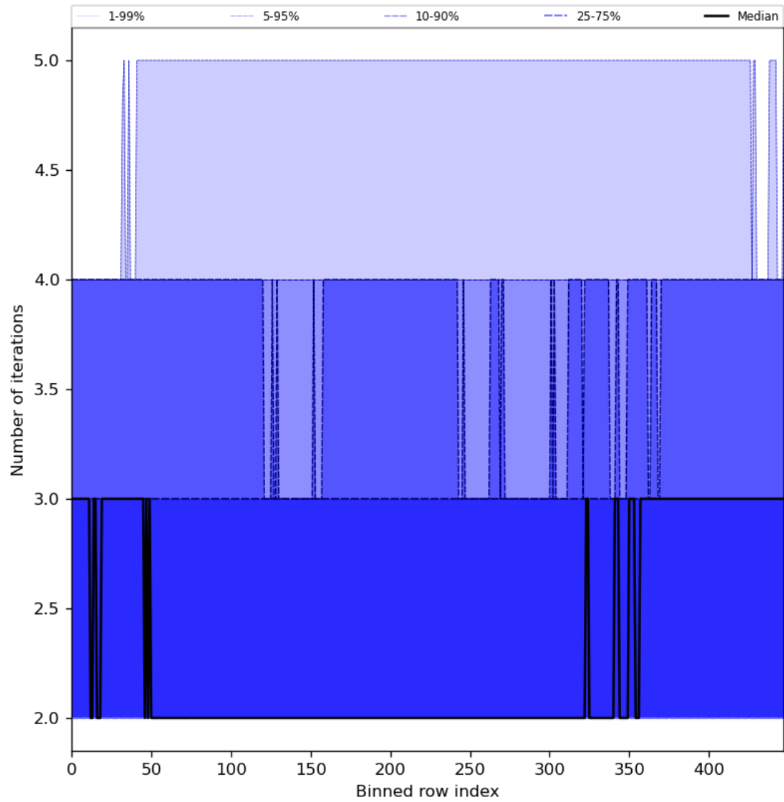
Figure 56: Along track statistics of “Number of iterations” for 2023-07-29 to 2023-07-30
