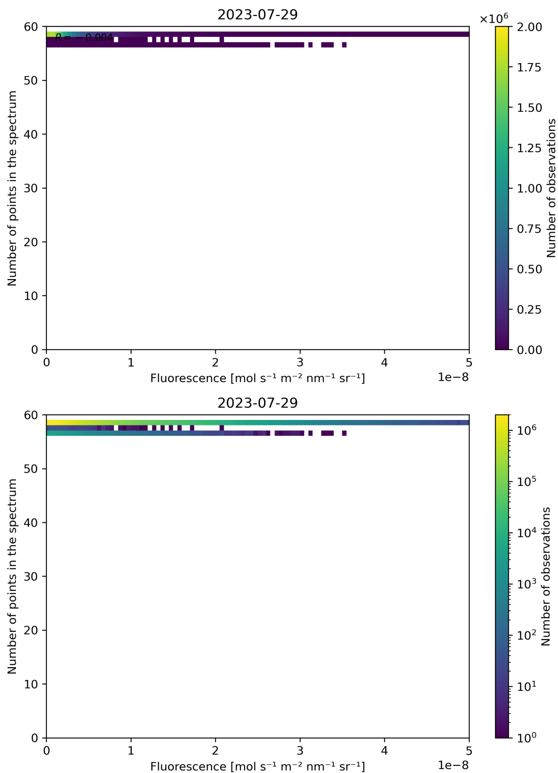
Figure 94: Scatter density plot of “Fluorescence” against “Number of points in the spectrum” for 2023-07-29 to 2023-07-30.
