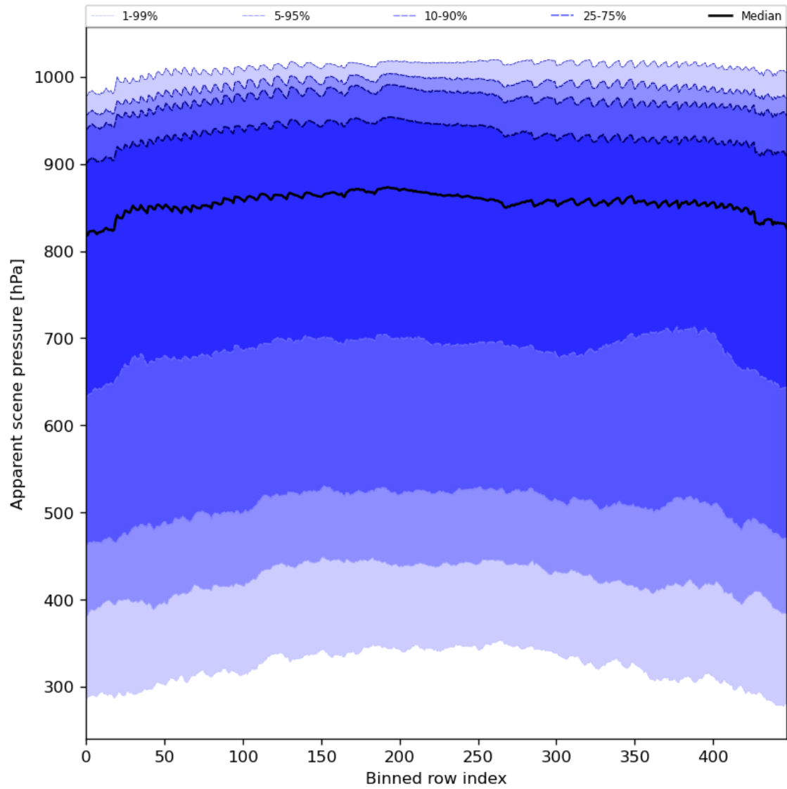
Figure 53: Along track statistics of “Apparent scene pressure” for 2023-07-29 to 2023-07-30
