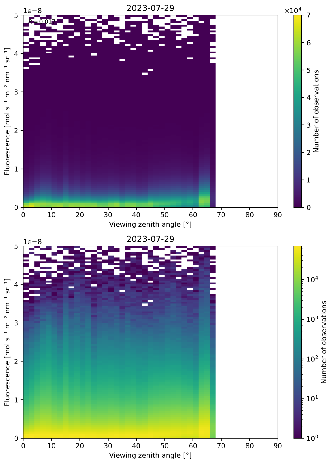
Figure 134: Scatter density plot of “Viewing zenith angle” against “Fluorescence” for 2023-07-29 to 2023-07-30.
