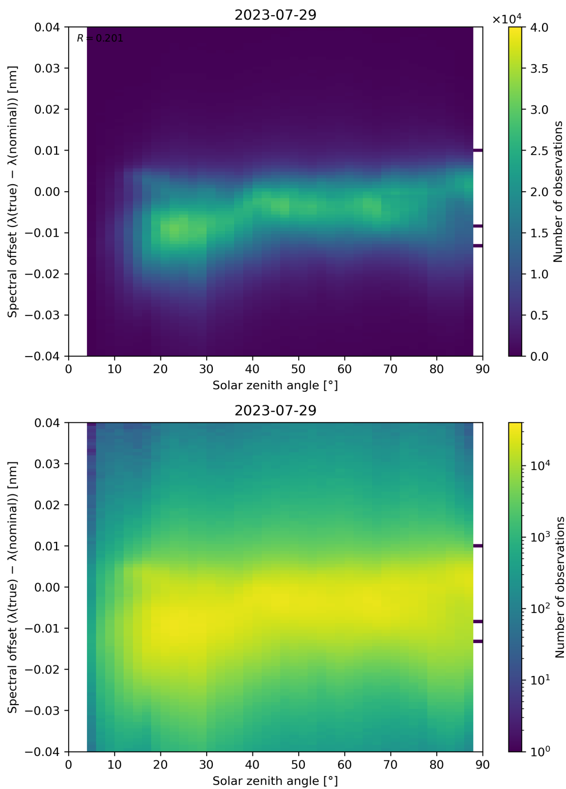
Figure 128: Scatter density plot of “Solar zenith angle” against “Spectral offset ( \lambda(\text{true}) - \lambda(\text{nominal}) )” for 2023-07-29 to 2023-07-30.
