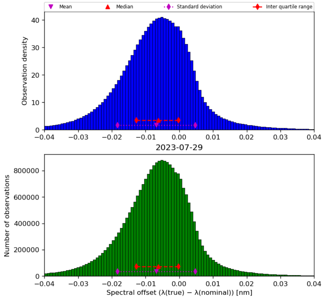
Figure 45: Histogram of “Spectral offset ( \lambda(\text{true}) - \lambda(\text{nominal}) )” for 2023-07-29 to 2023-07-30
