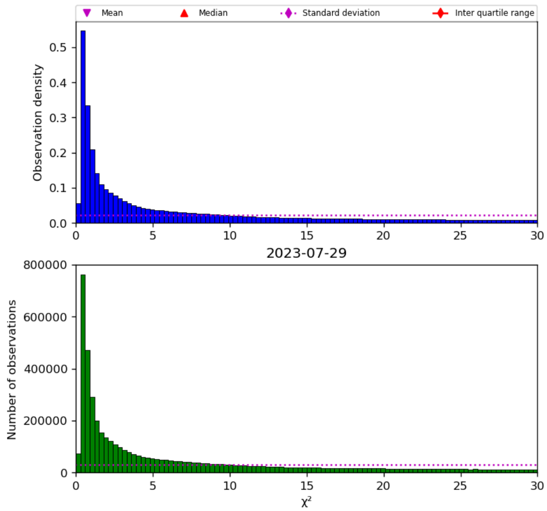
Figure 38: Histogram of “ \chi^2 ” for 2023-07-29 to 2023-07-30
