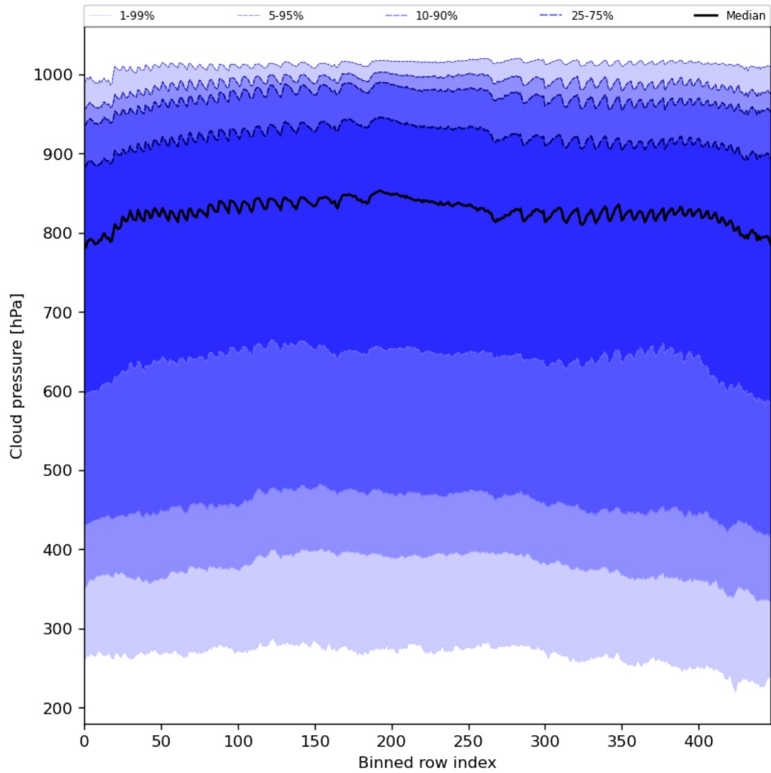
Figure 47: Along track statistics of “Cloud pressure” for 2023-07-29 to 2023-07-30
