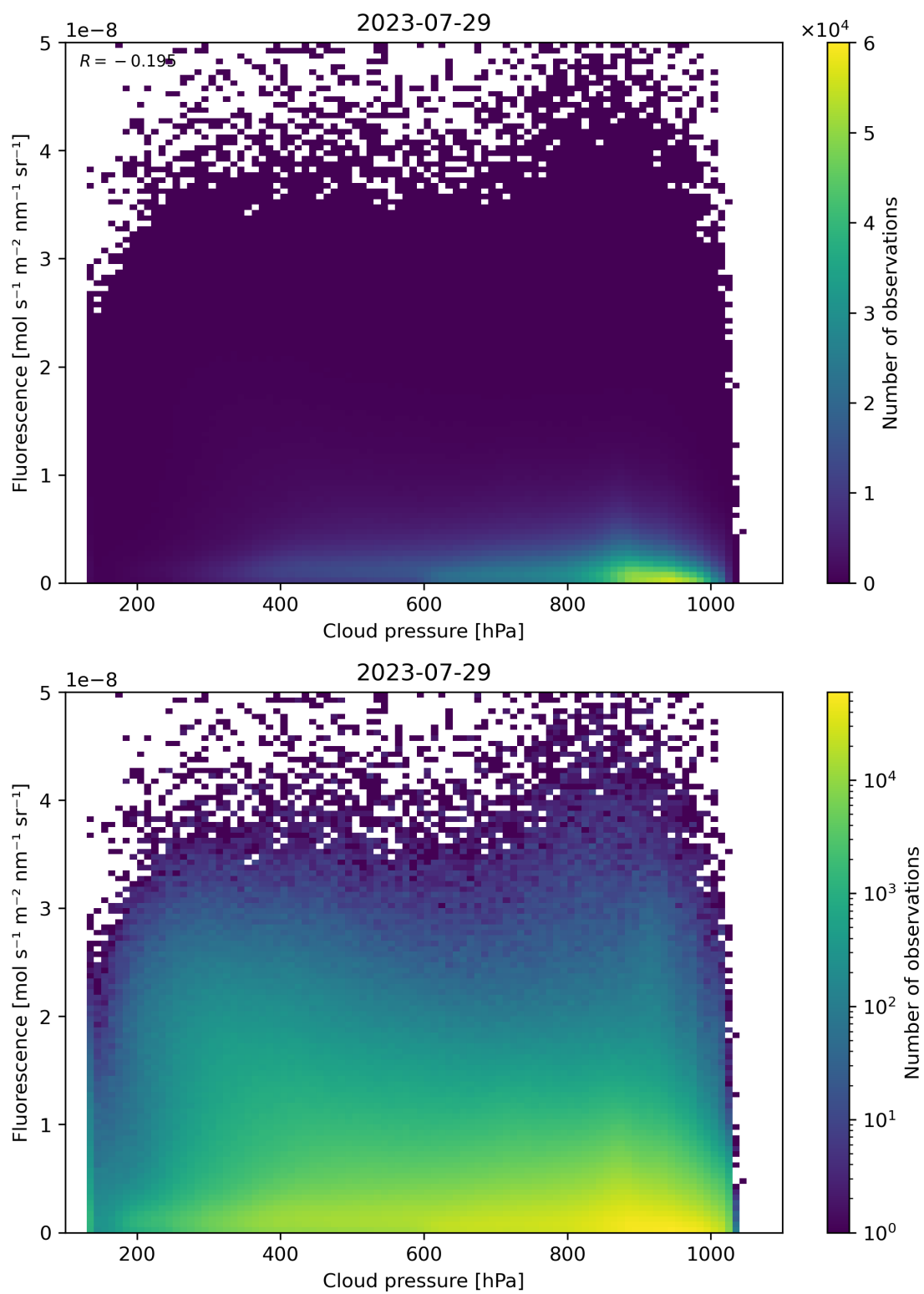
Figure 88: Scatter density plot of “Cloud pressure” against “Fluorescence” for 2023-07-29 to 2023-07-30.
