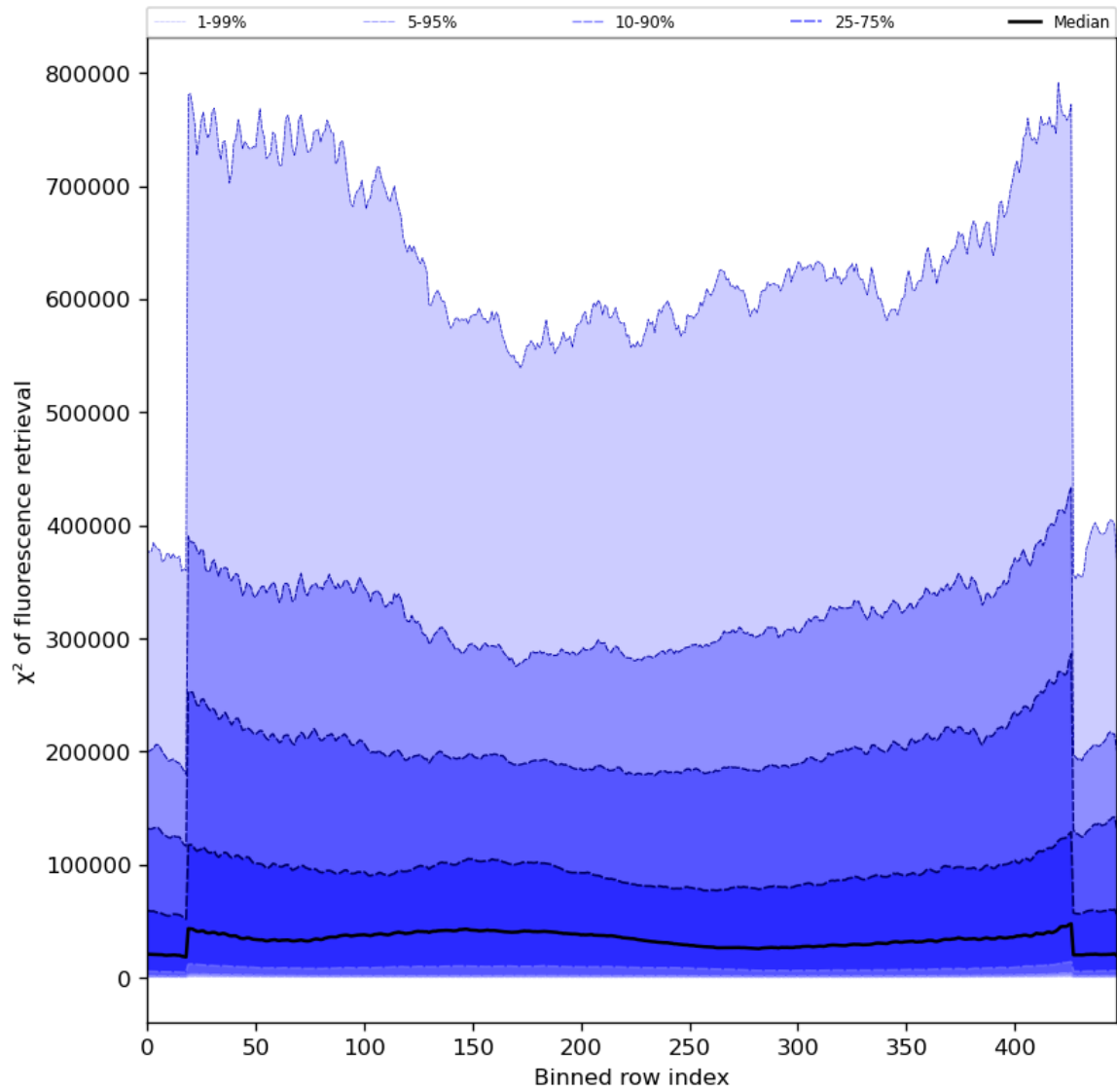
Figure 59: Along track statistics of “ \chi^2 of fluorescence retrieval” for 2023-07-29 to 2023-07-30
