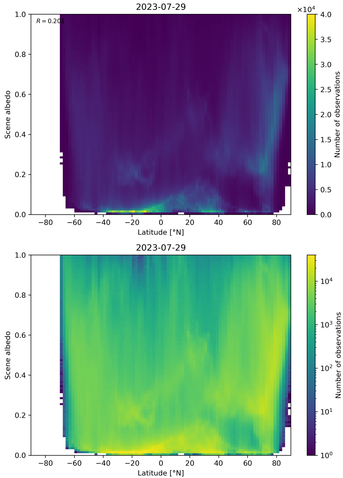
Figure 104: Scatter density plot of “Latitude” against “Scene albedo” for 2023-07-29 to 2023-07-30.
