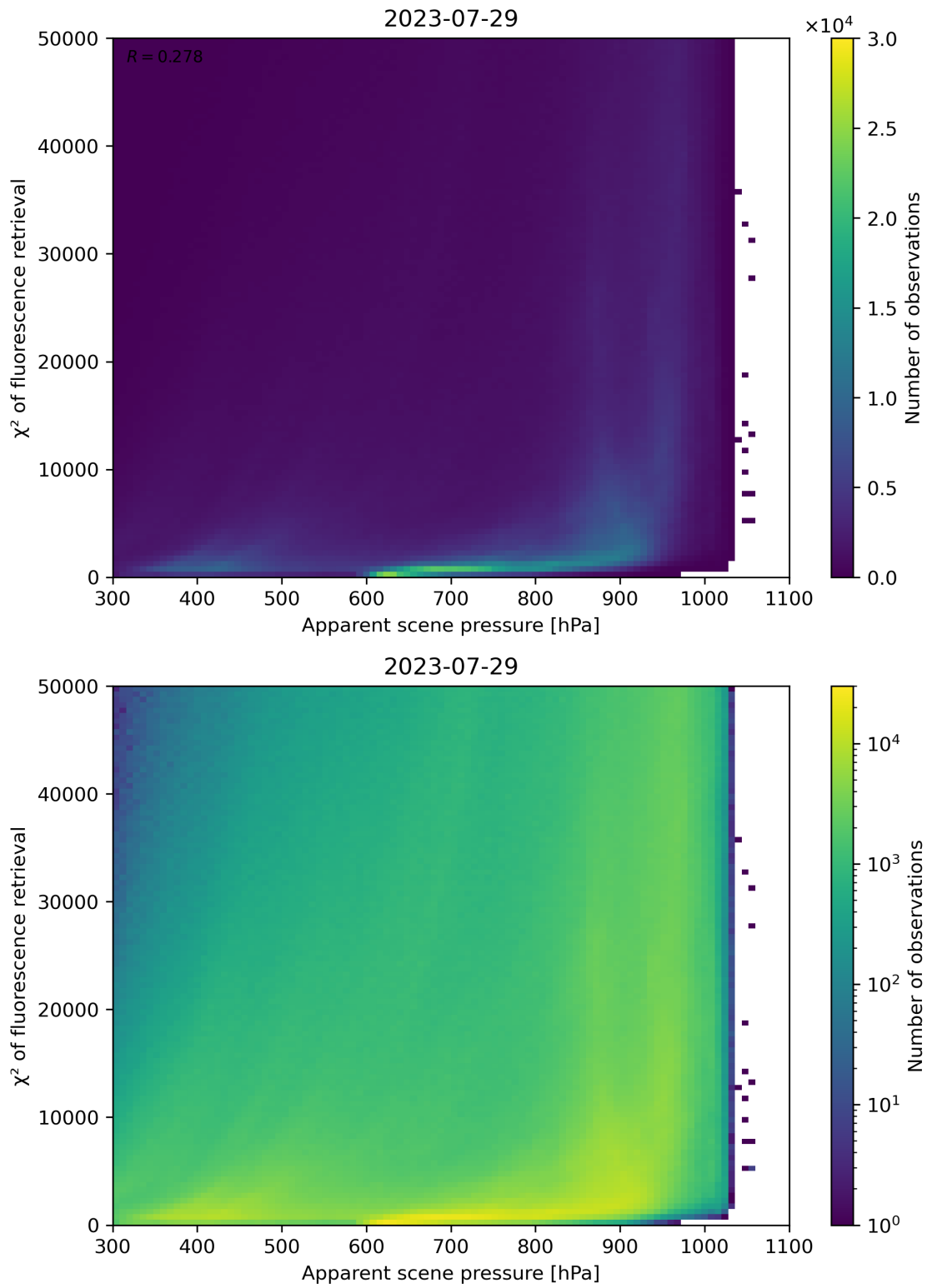
Figure 64: Scatter density plot of “Apparent scene pressure” against “ \chi^2 of fluorescence retrieval” for 2023-07-29 to 2023-07-30.
