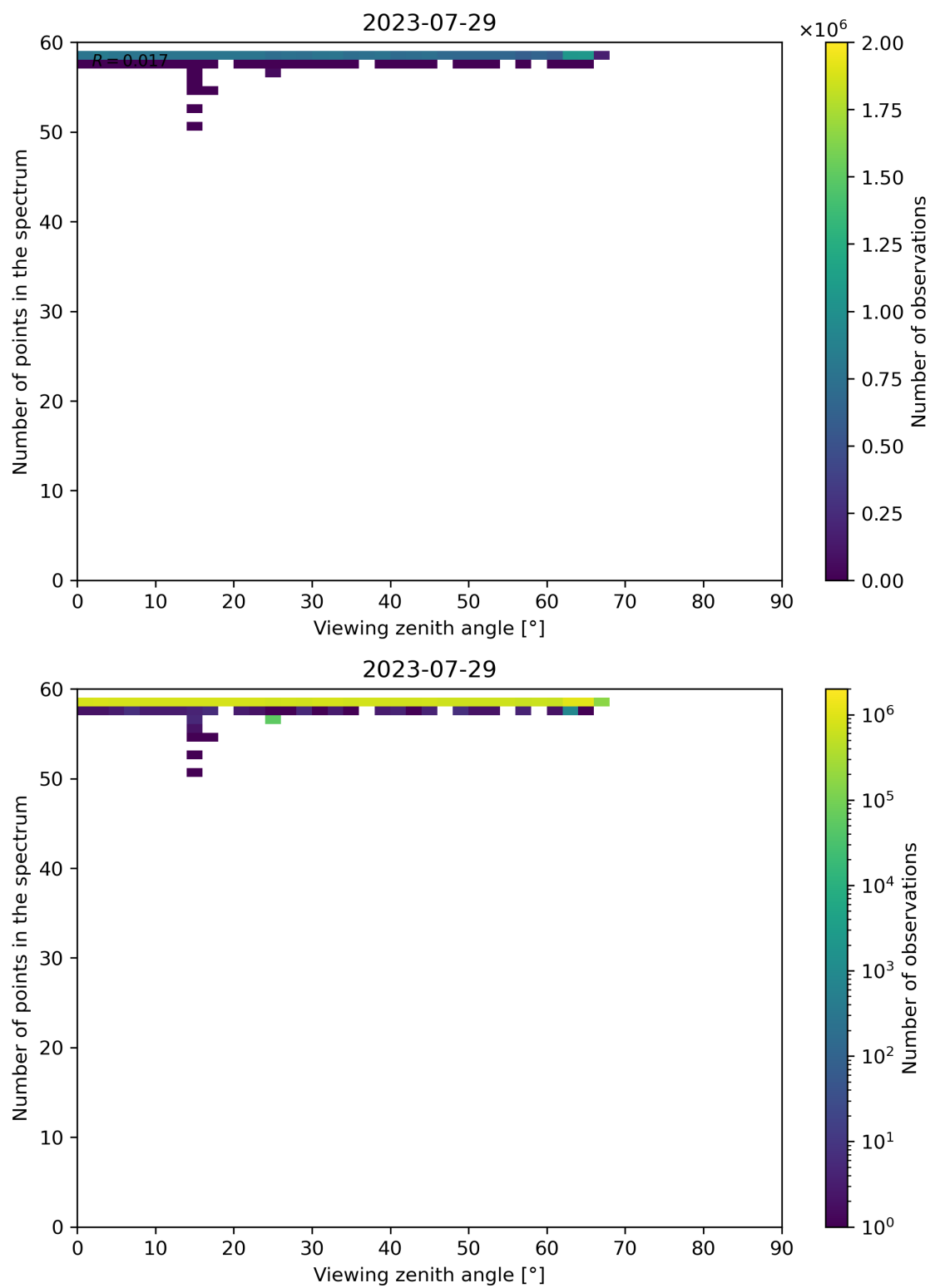
Figure 137: Scatter density plot of “Viewing zenith angle” against “Number of points in the spectrum” for 2023-07-29 to 2023-07-30.
