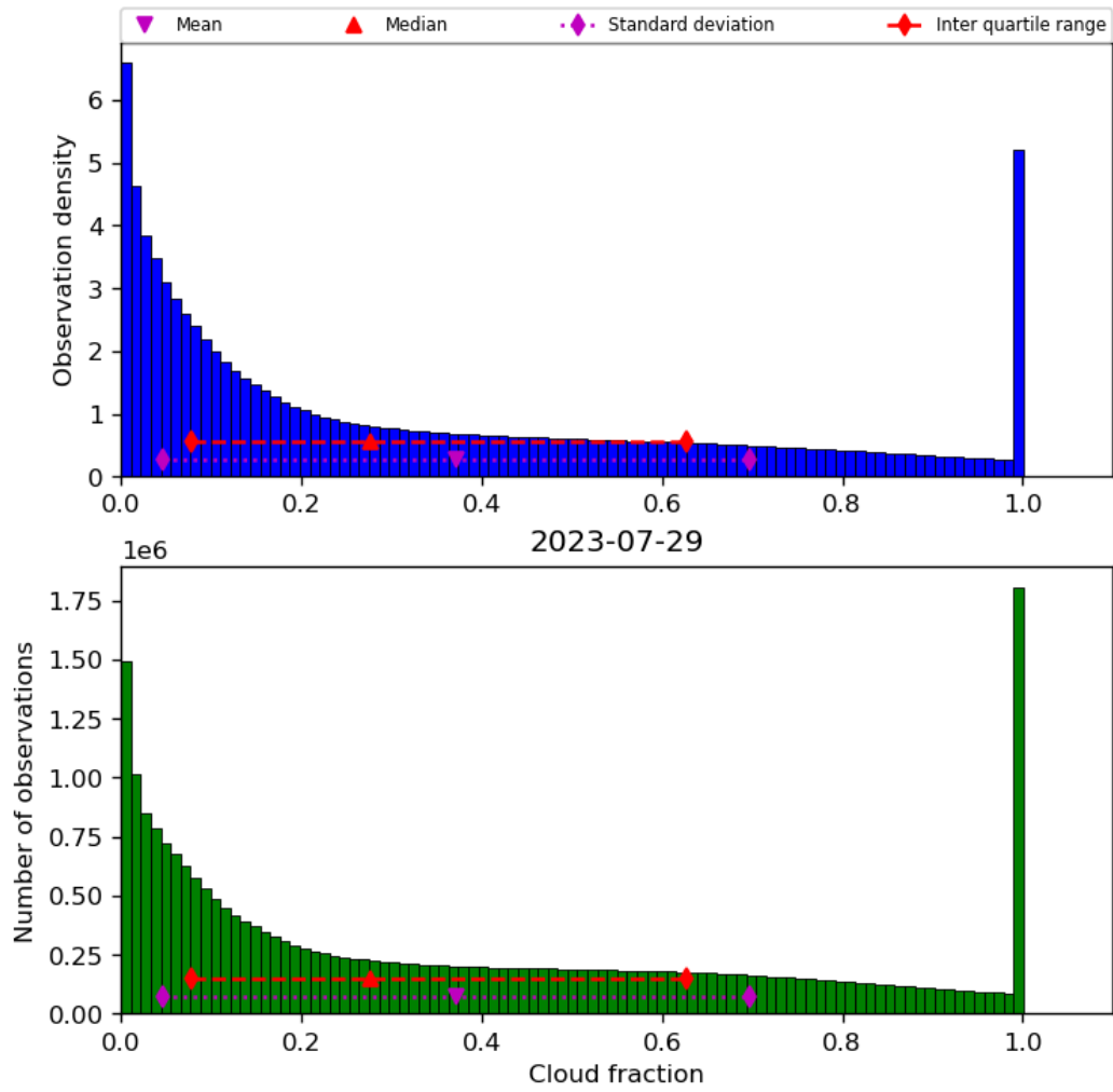
Figure 32: Histogram of “Cloud fraction” for 2023-07-29 to 2023-07-30
