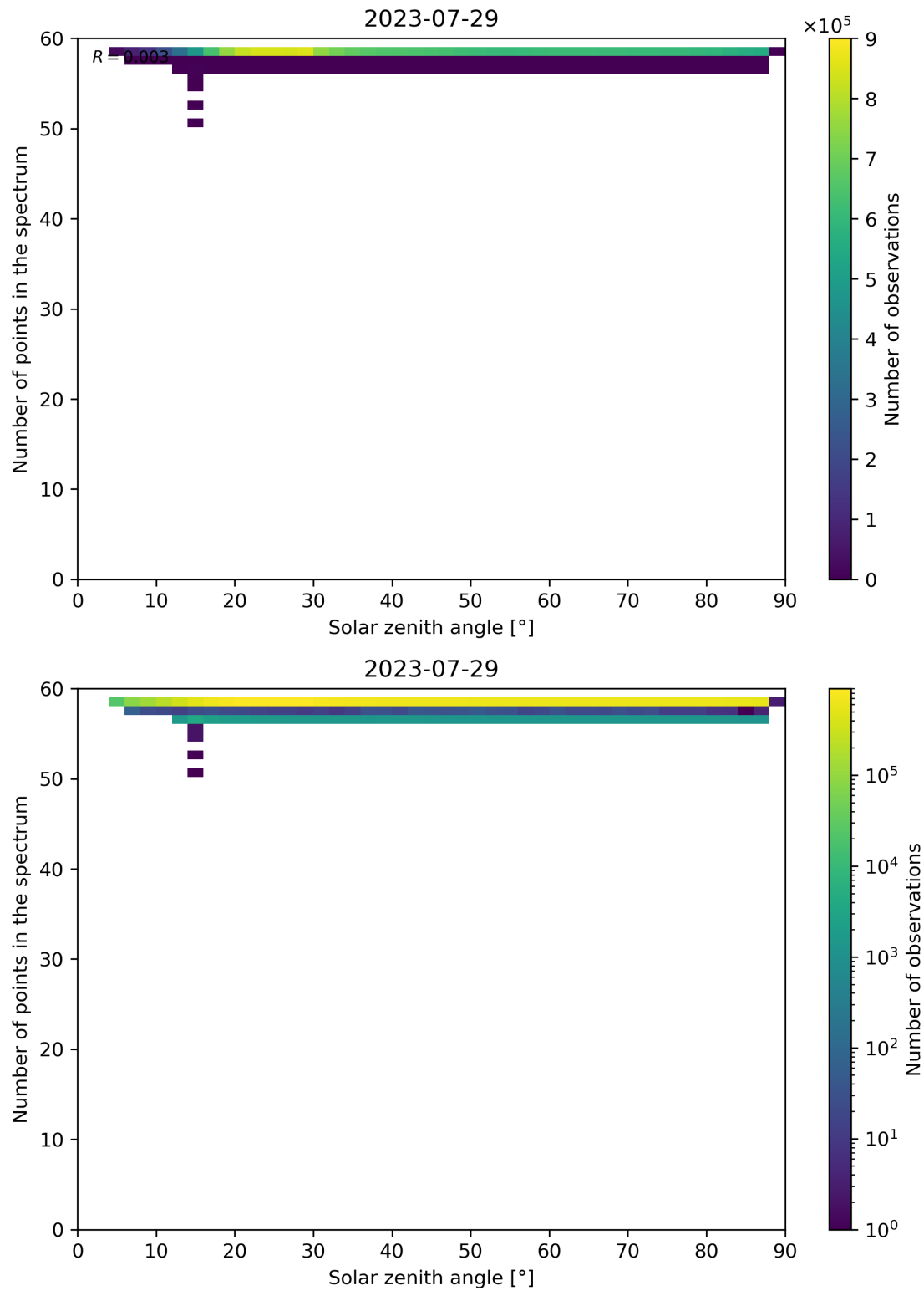
Figure 126: Scatter density plot of “Solar zenith angle” against “Number of points in the spectrum” for 2023-07-29 to 2023-07-30.
