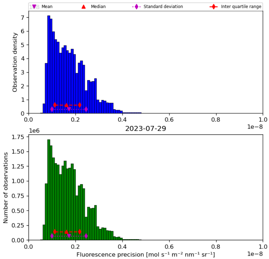
Figure 41: Histogram of “Fluorescence precision” for 2023-07-29 to 2023-07-30
