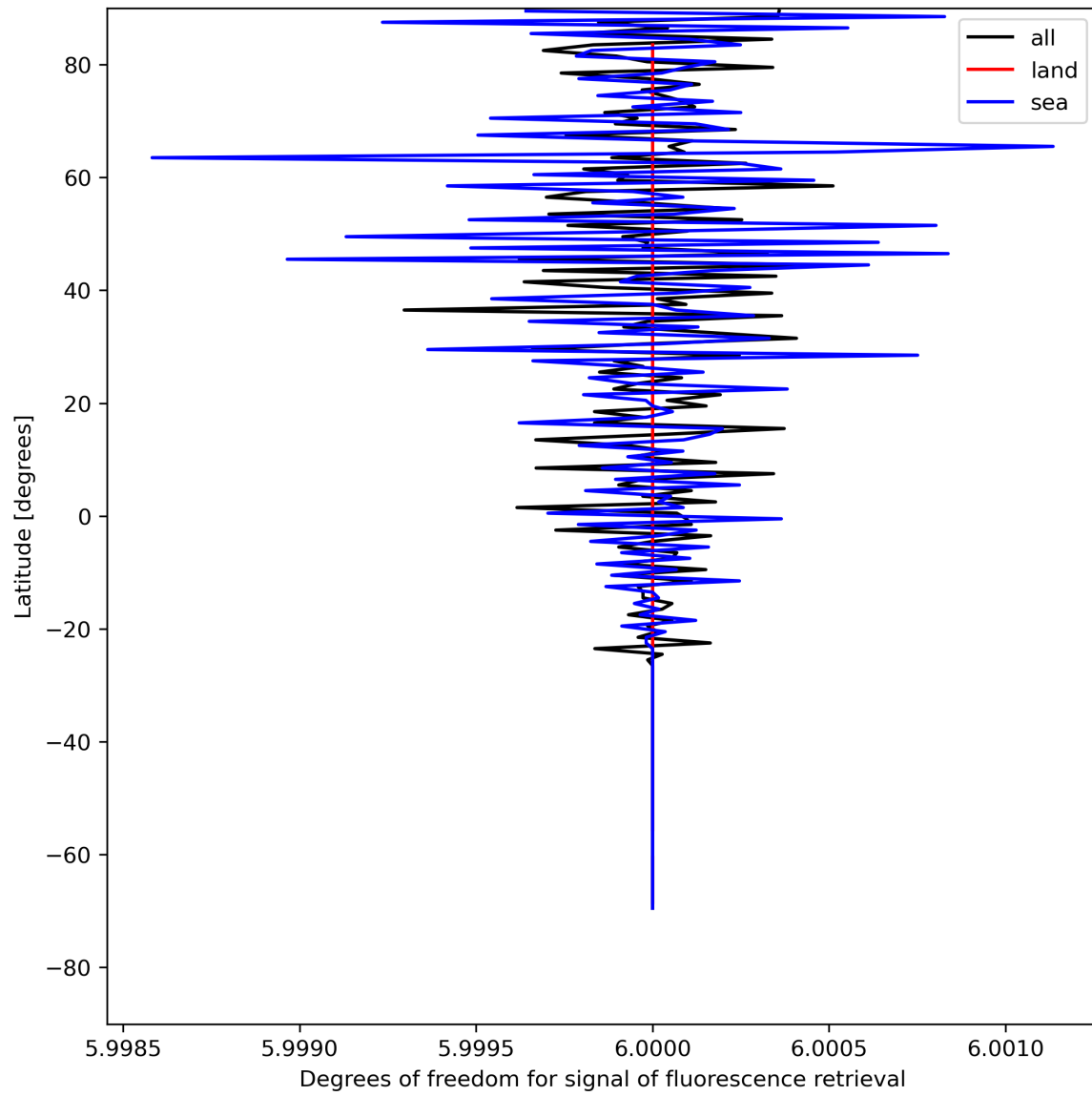
Figure 26: Zonal average of “Degrees of freedom for signal of fluorescence retrieval” for 2023-07-29 to 2023-07-30.
