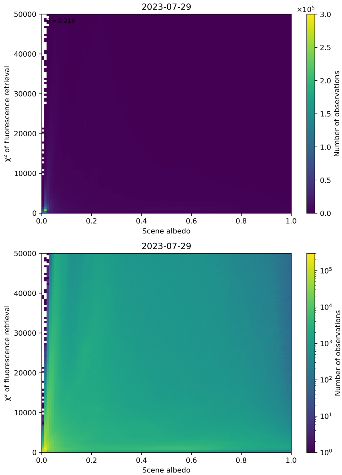
Figure 113: Scatter density plot of “Scene albedo” against “ \chi^2 of fluorescence retrieval” for 2023-07-29 to 2023-07-30.
