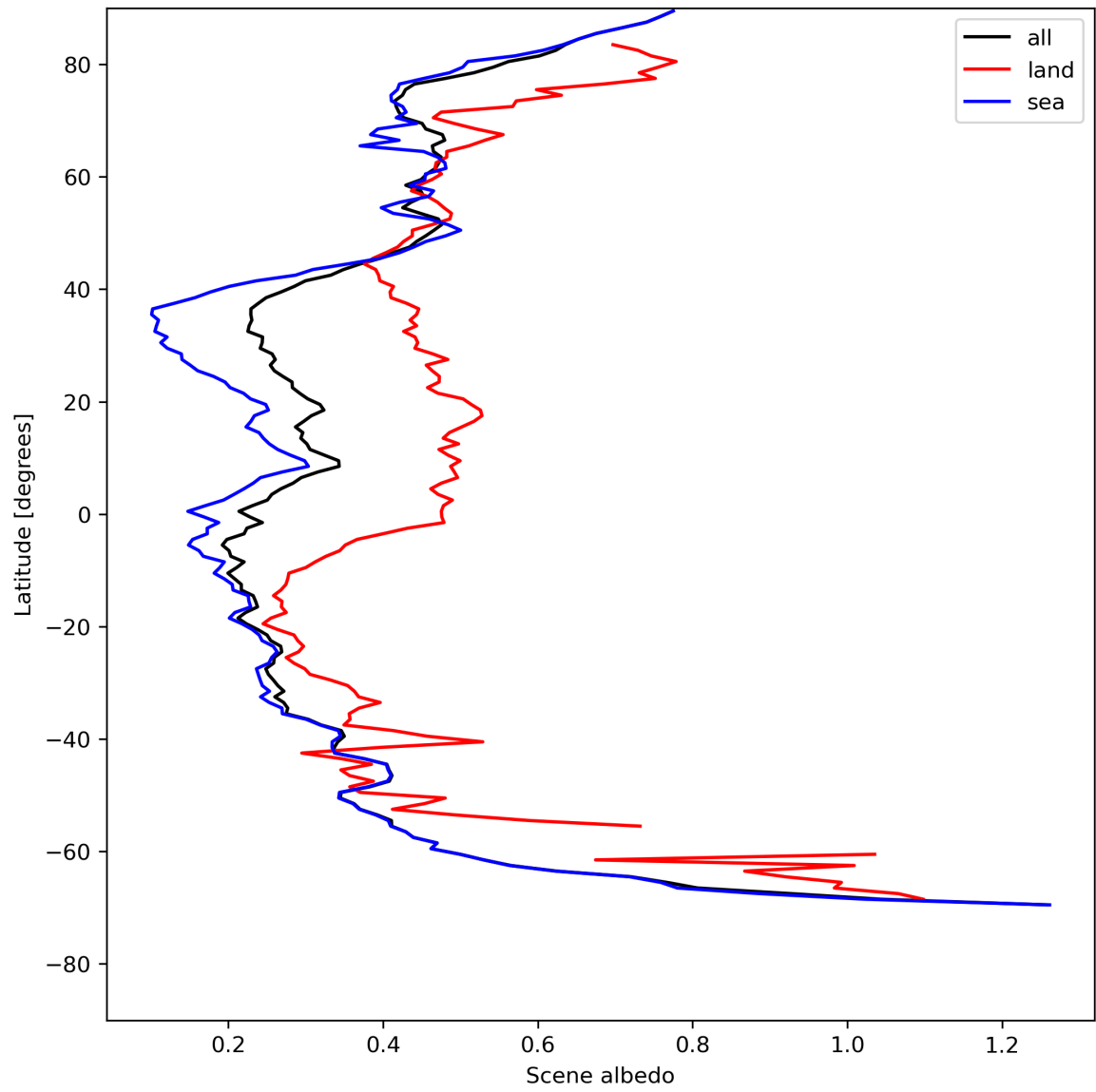
Figure 17: Zonal average of “Scene albedo” for 2023-07-29 to 2023-07-30.
