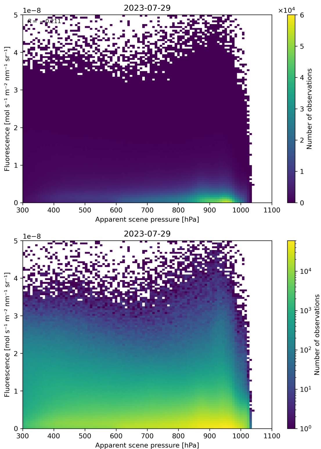
Figure 65: Scatter density plot of “Apparent scene pressure” against “Fluorescence” for 2023-07-29 to 2023-07-30.
