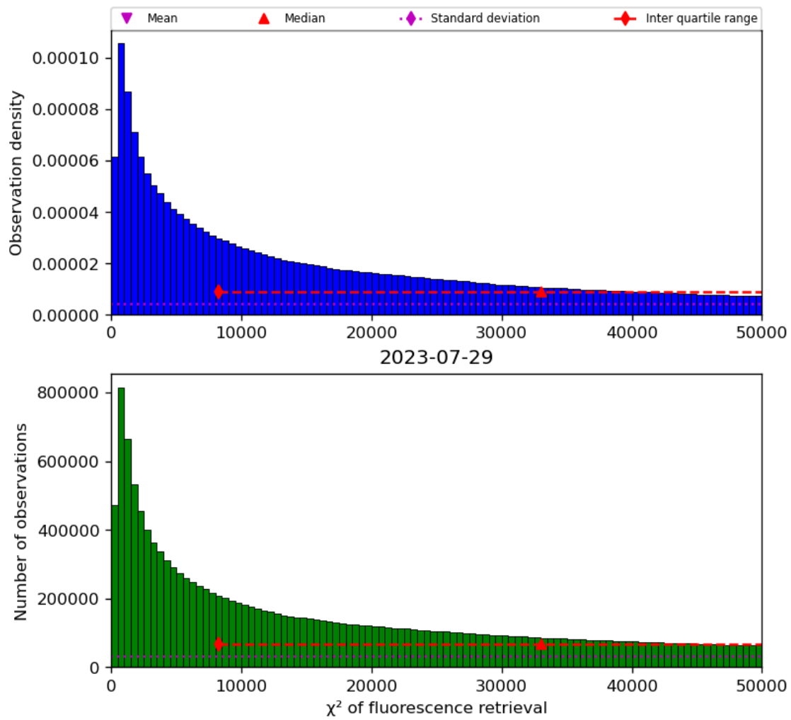
Figure 42: Histogram of “ \chi^2 of fluorescence retrieval” for 2023-07-29 to 2023-07-30
