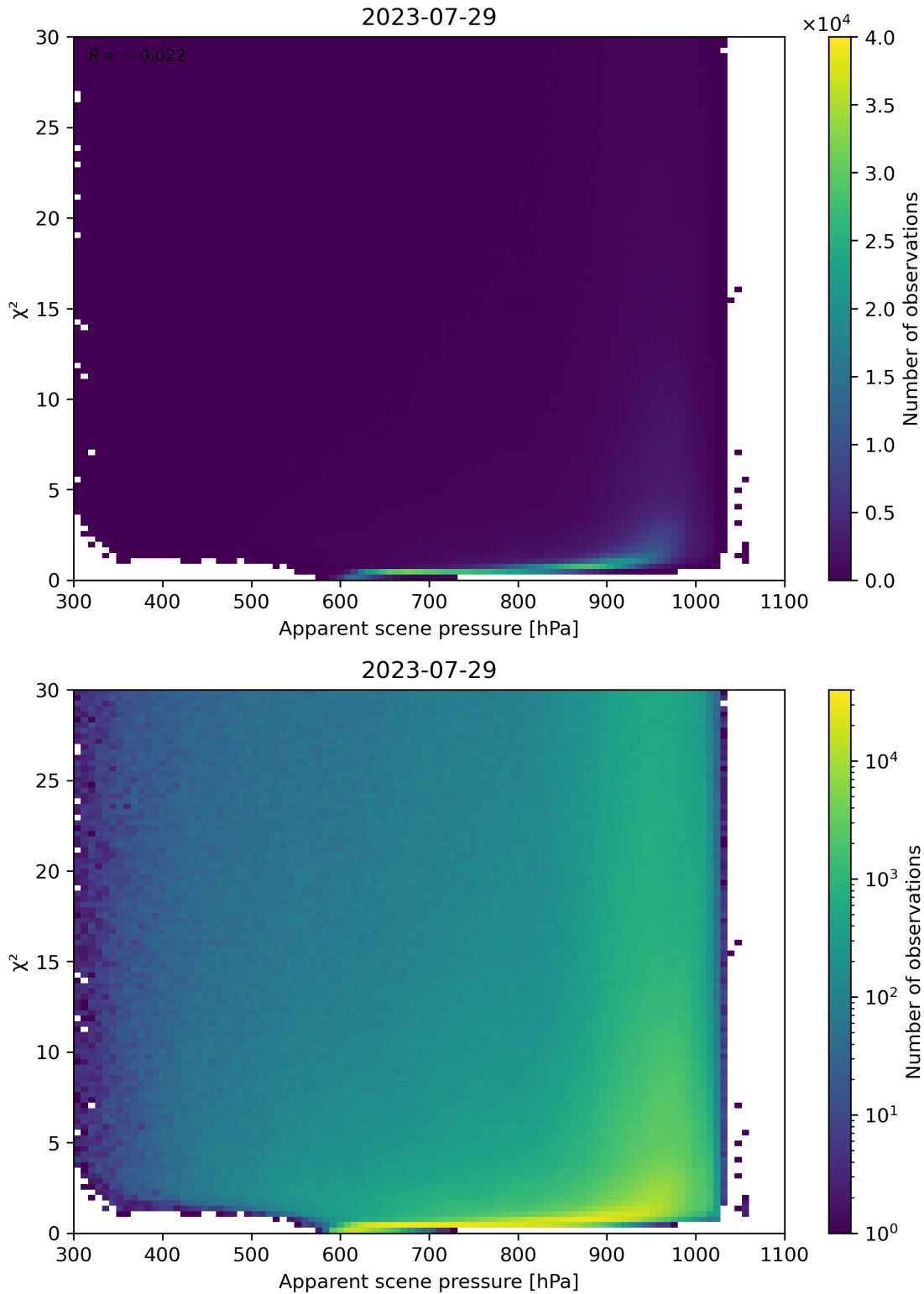
Figure 63: Scatter density plot of “Apparent scene pressure” against “ \chi^2 ” for 2023-07-29 to 2023-07-30.
