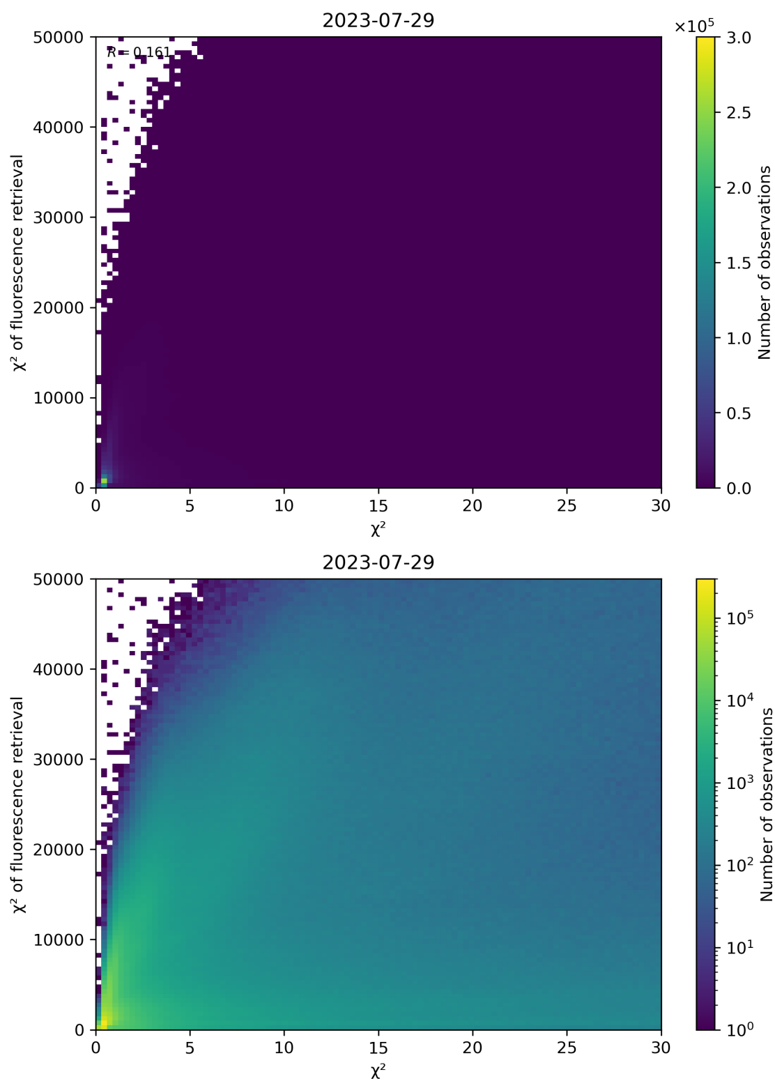
Figure 69: Scatter density plot of “ \chi^2 ” against “ \chi^2 of fluorescence retrieval” for 2023-07-29 to 2023-07-30.
