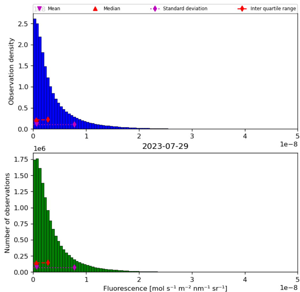
Figure 40: Histogram of “Fluorescence” for 2023-07-29 to 2023-07-30
