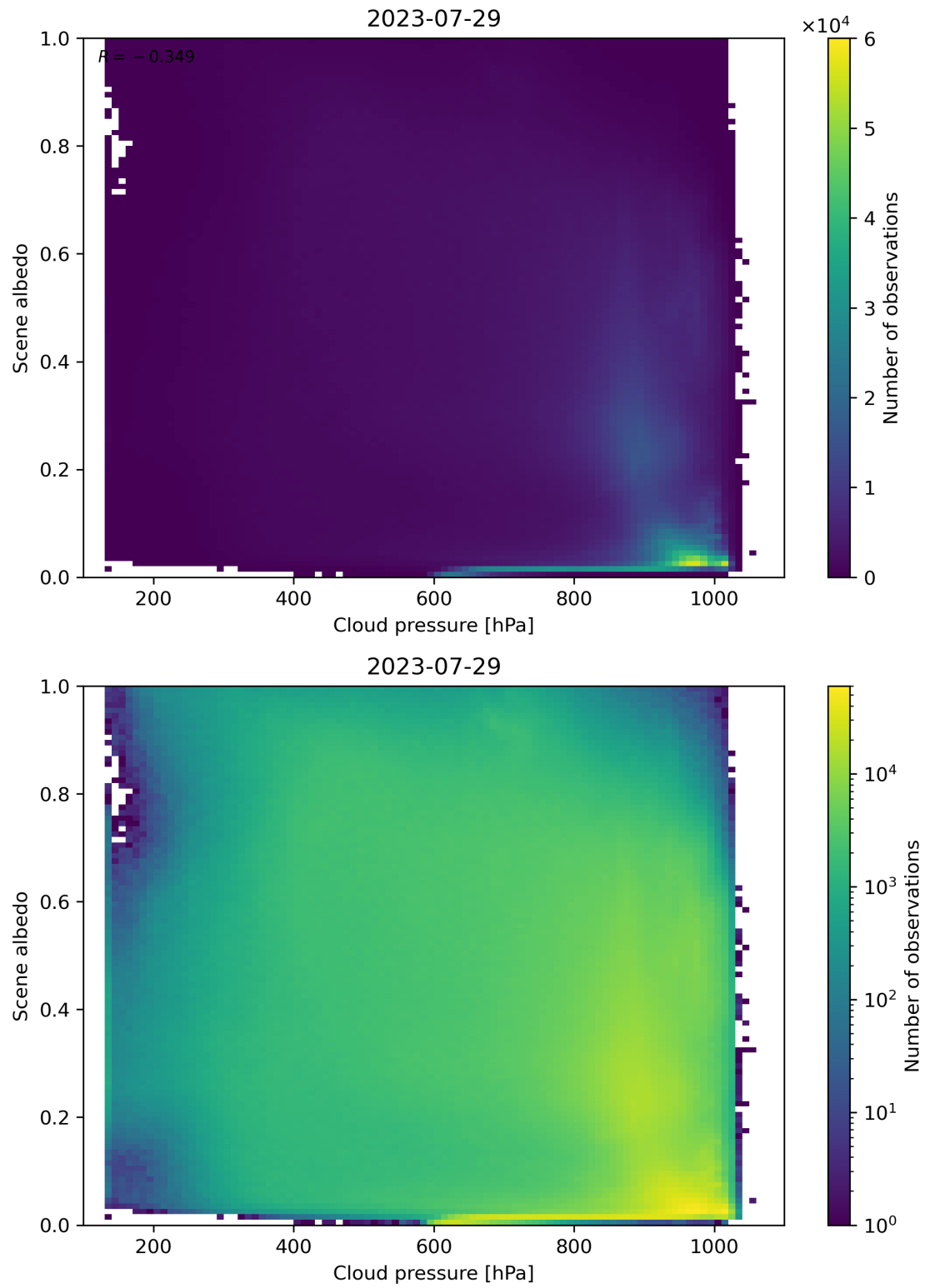
Figure 91: Scatter density plot of “Cloud pressure” against “Scene albedo” for 2023-07-29 to 2023-07-30.
