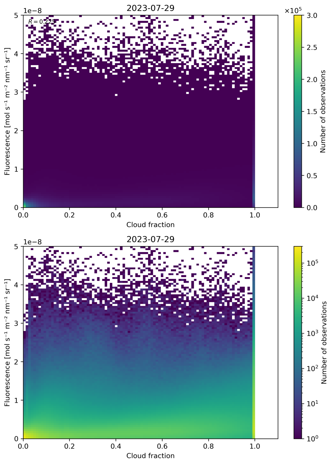
Figure 79: Scatter density plot of “Cloud fraction” against “Fluorescence” for 2023-07-29 to 2023-07-30.
