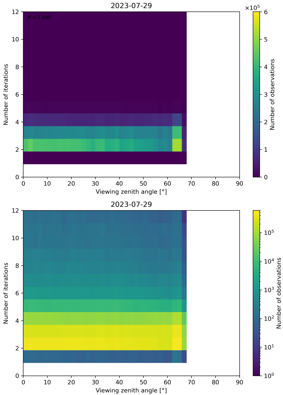
Figure 136: Scatter density plot of “Viewing zenith angle” against “Number of iterations” for 2023-07-29 to 2023-07-30.
