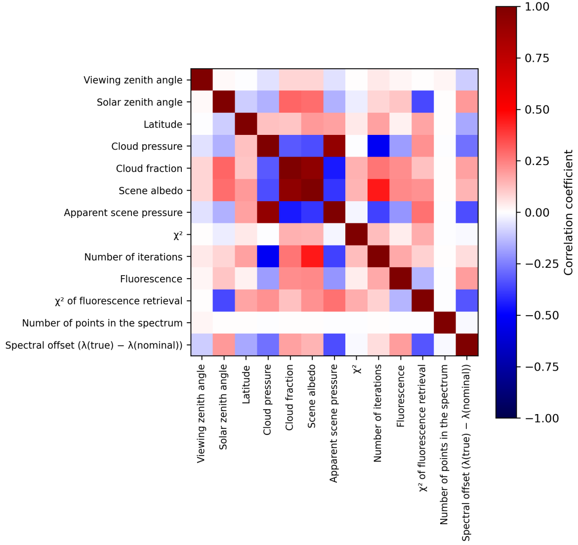
Figure 2: Map of correlation matrix for 2023-07-29 to 2023-07-30.
