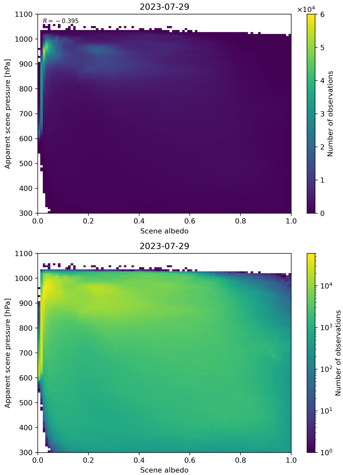
Figure 111: Scatter density plot of “Scene albedo” against “Apparent scene pressure” for 2023-07-29 to 2023-07-30.
