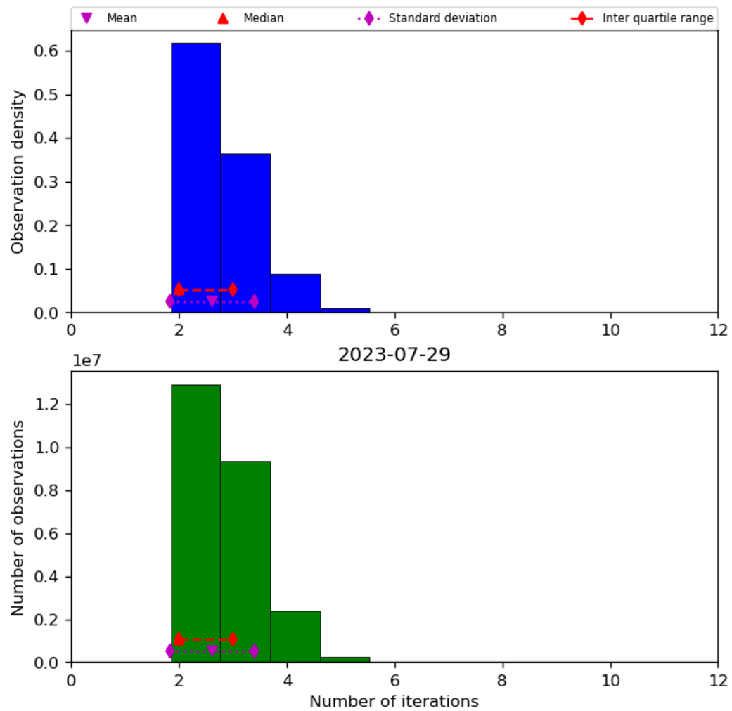
Figure 39: Histogram of “Number of iterations” for 2023-07-29 to 2023-07-30
