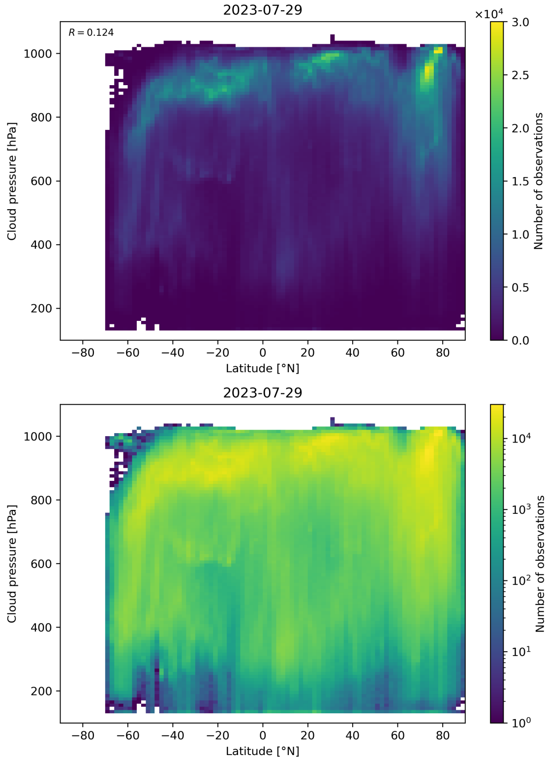
Figure 100: Scatter density plot of “Latitude” against “Cloud pressure” for 2023-07-29 to 2023-07-30.
