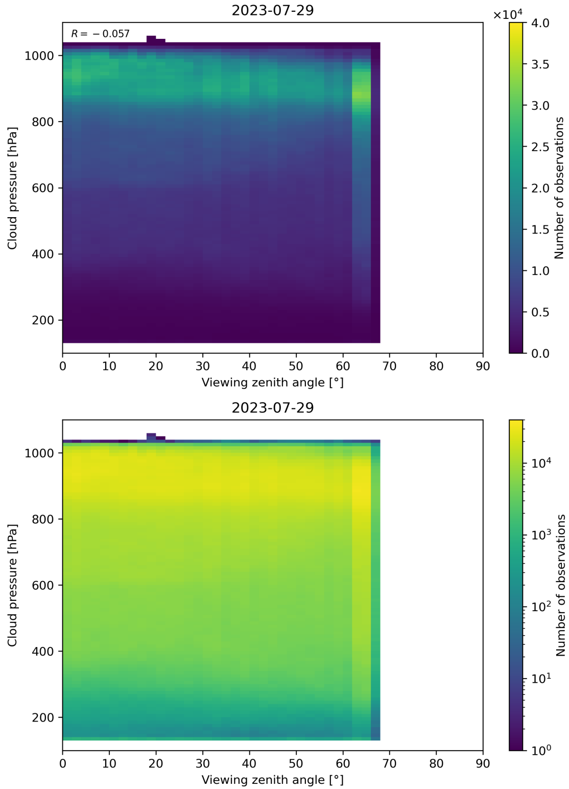
Figure 133: Scatter density plot of “Viewing zenith angle” against “Cloud pressure” for 2023-07-29 to 2023-07-30.
