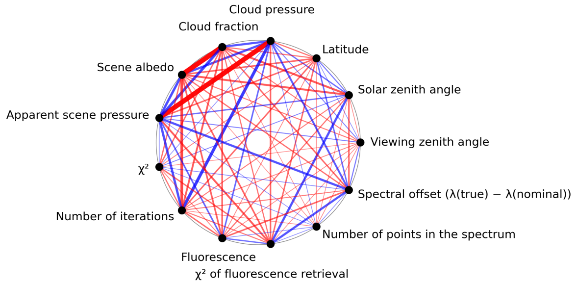
Figure 1: Map of correlation graph for 2023-07-29 to 2023-07-30.
