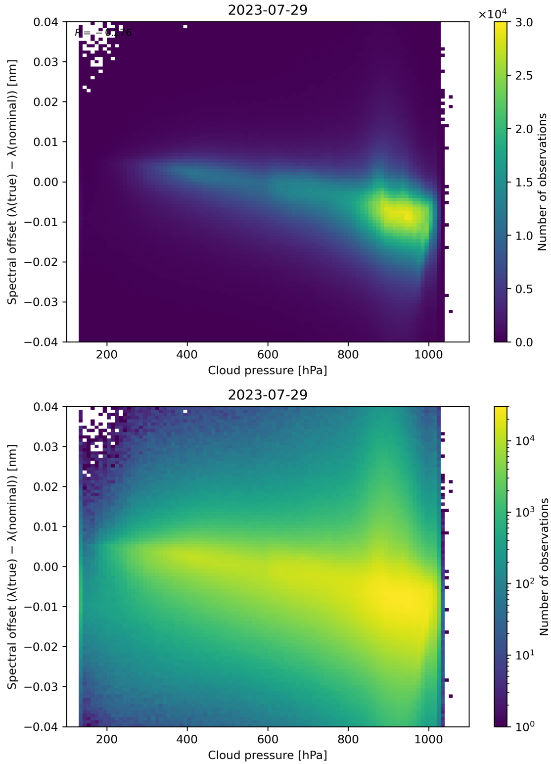
Figure 92: Scatter density plot of “Cloud pressure” against “Spectral offset ( \lambda(\text{true}) - \lambda(\text{nominal}) )” for 2023-07-29 to 2023-07-30.
