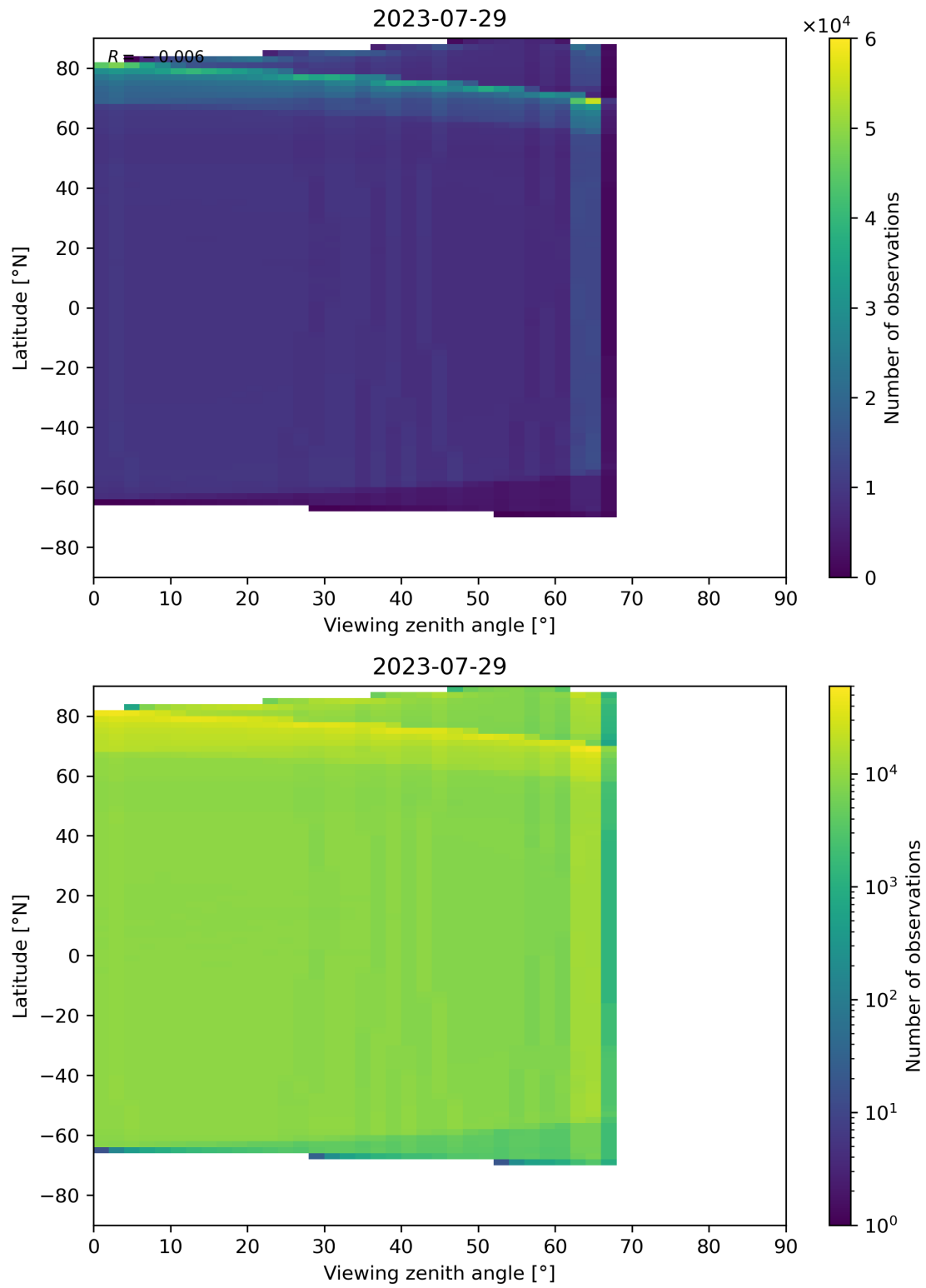
Figure 135: Scatter density plot of “Viewing zenith angle” against “Latitude” for 2023-07-29 to 2023-07-30.
