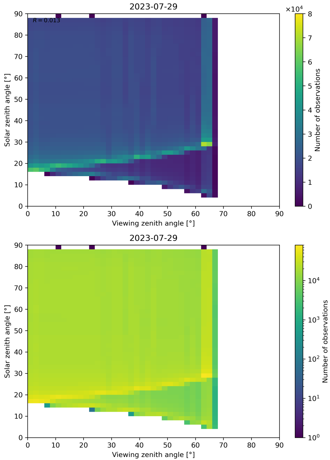
Figure 139: Scatter density plot of “Viewing zenith angle” against “Solar zenith angle” for 2023-07-29 to 2023-07-30.
