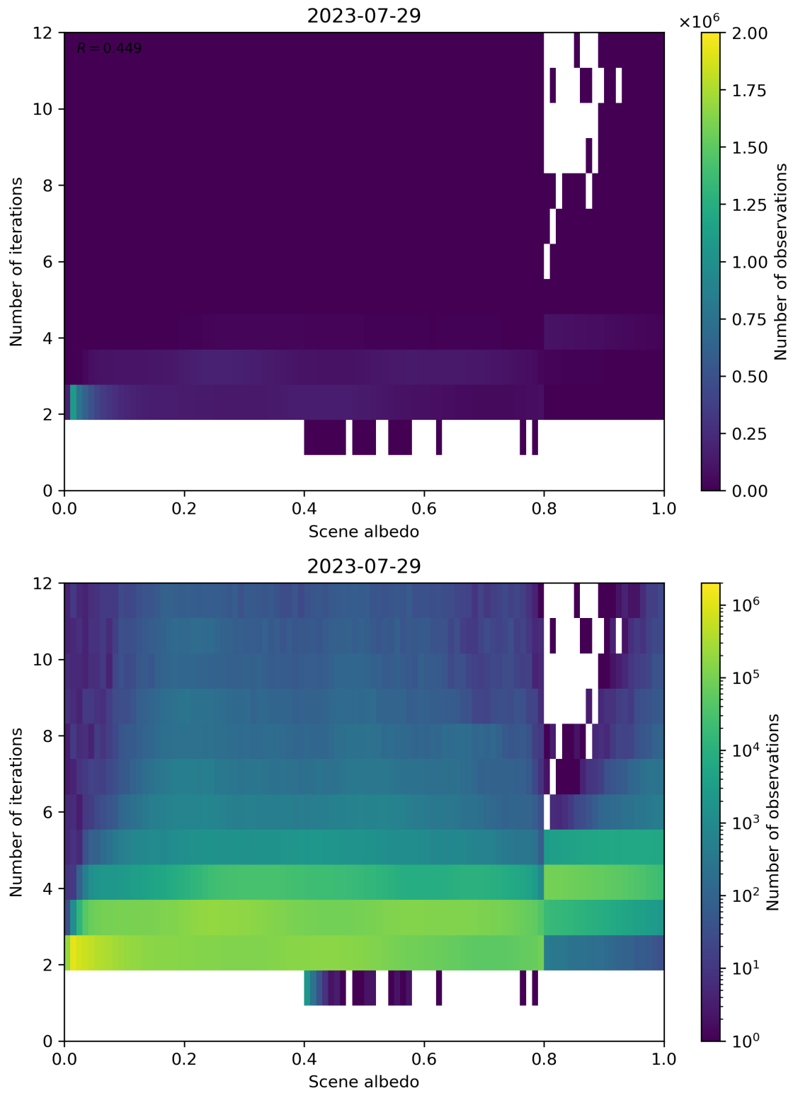
Figure 115: Scatter density plot of “Scene albedo” against “Number of iterations” for 2023-07-29 to 2023-07-30.
