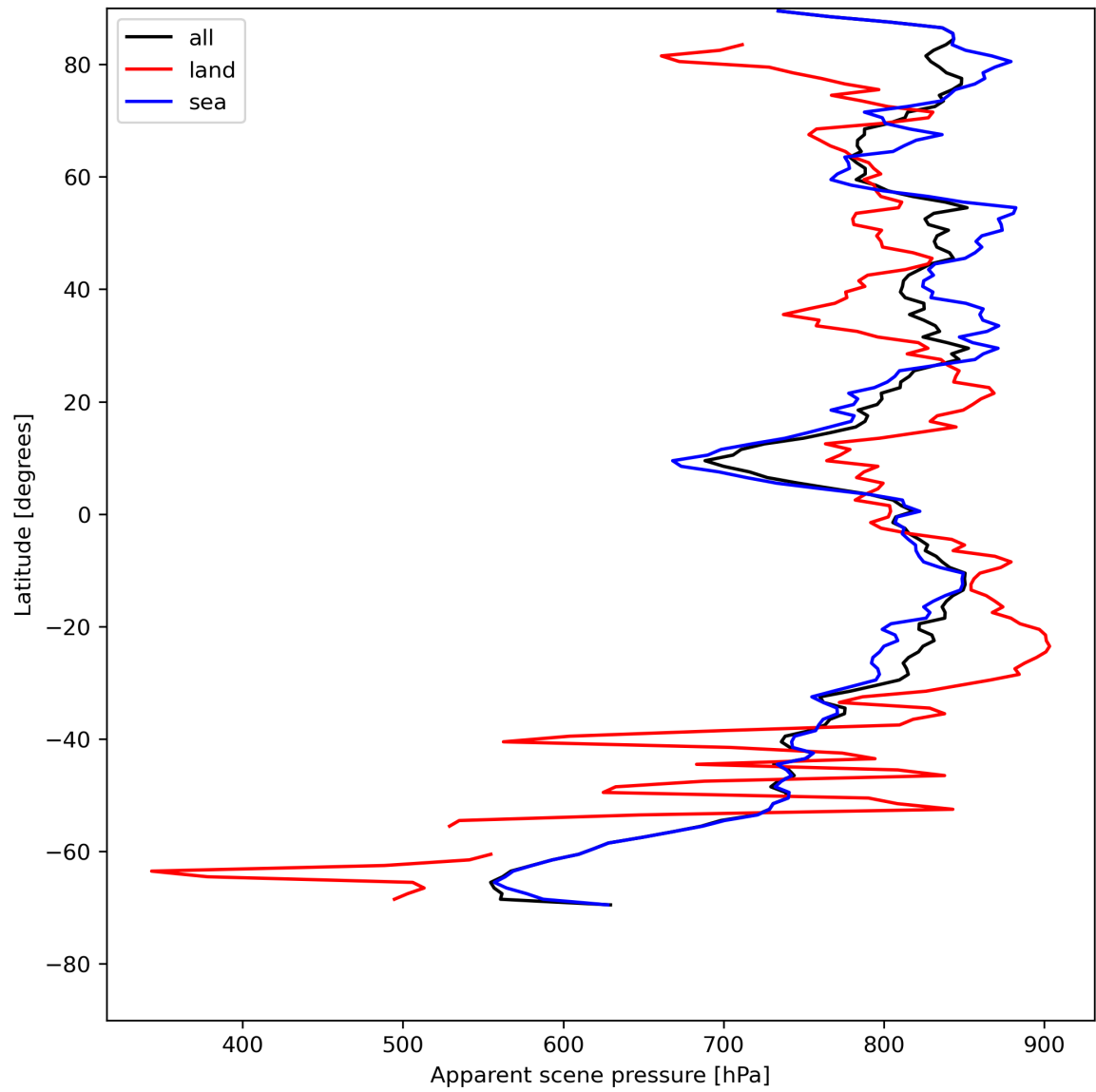
Figure 19: Zonal average of “Apparent scene pressure” for 2023-07-29 to 2023-07-30.
