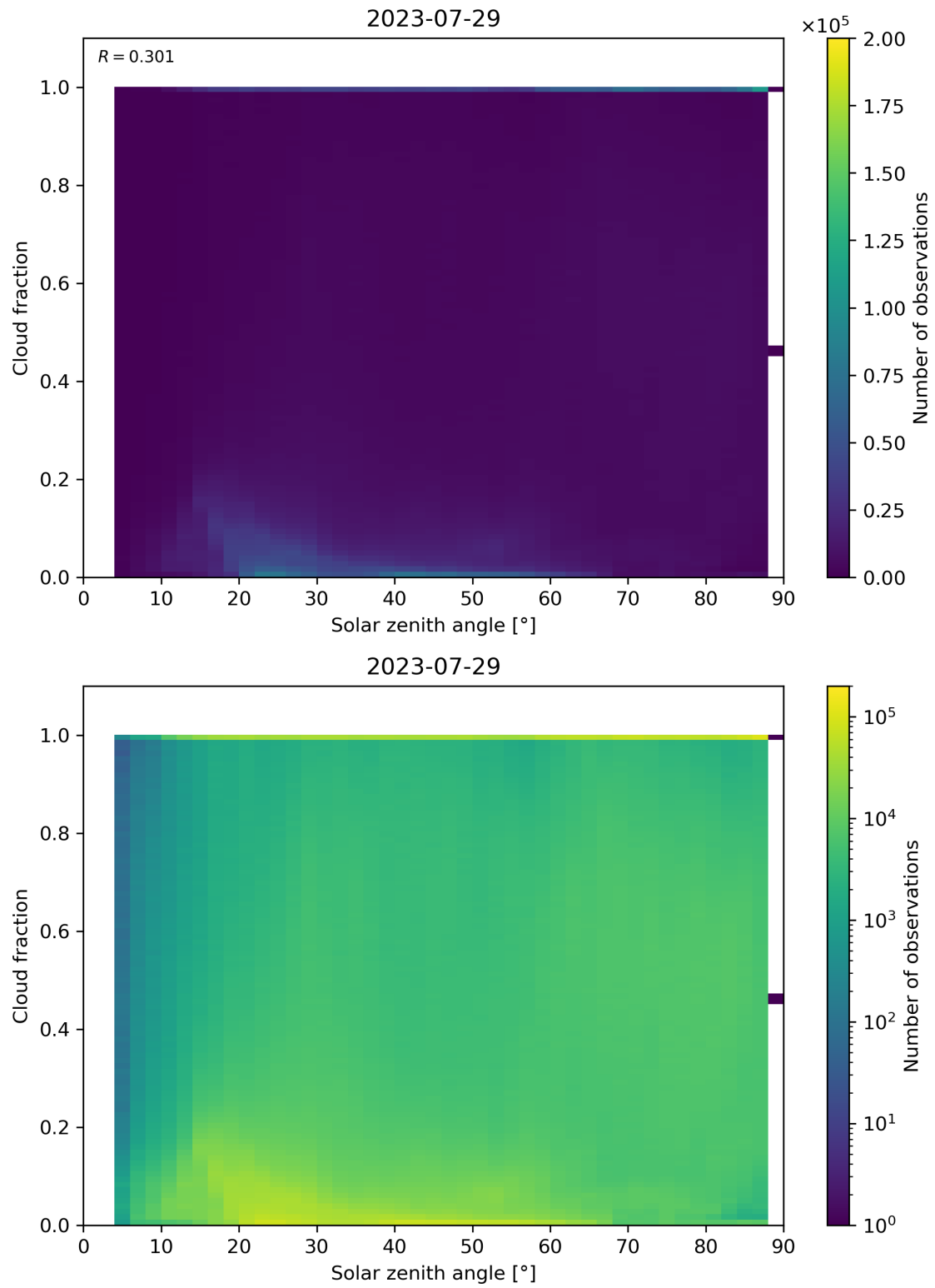
Figure 121: Scatter density plot of “Solar zenith angle” against “Cloud fraction” for 2023-07-29 to 2023-07-30.
