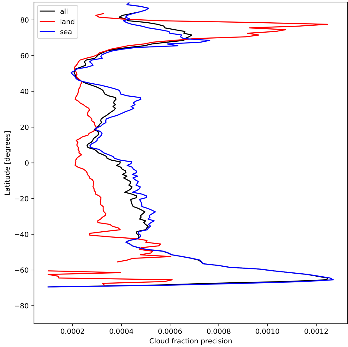
Figure 16: Zonal average of “Cloud fraction precision” for 2023-07-29 to 2023-07-30.
