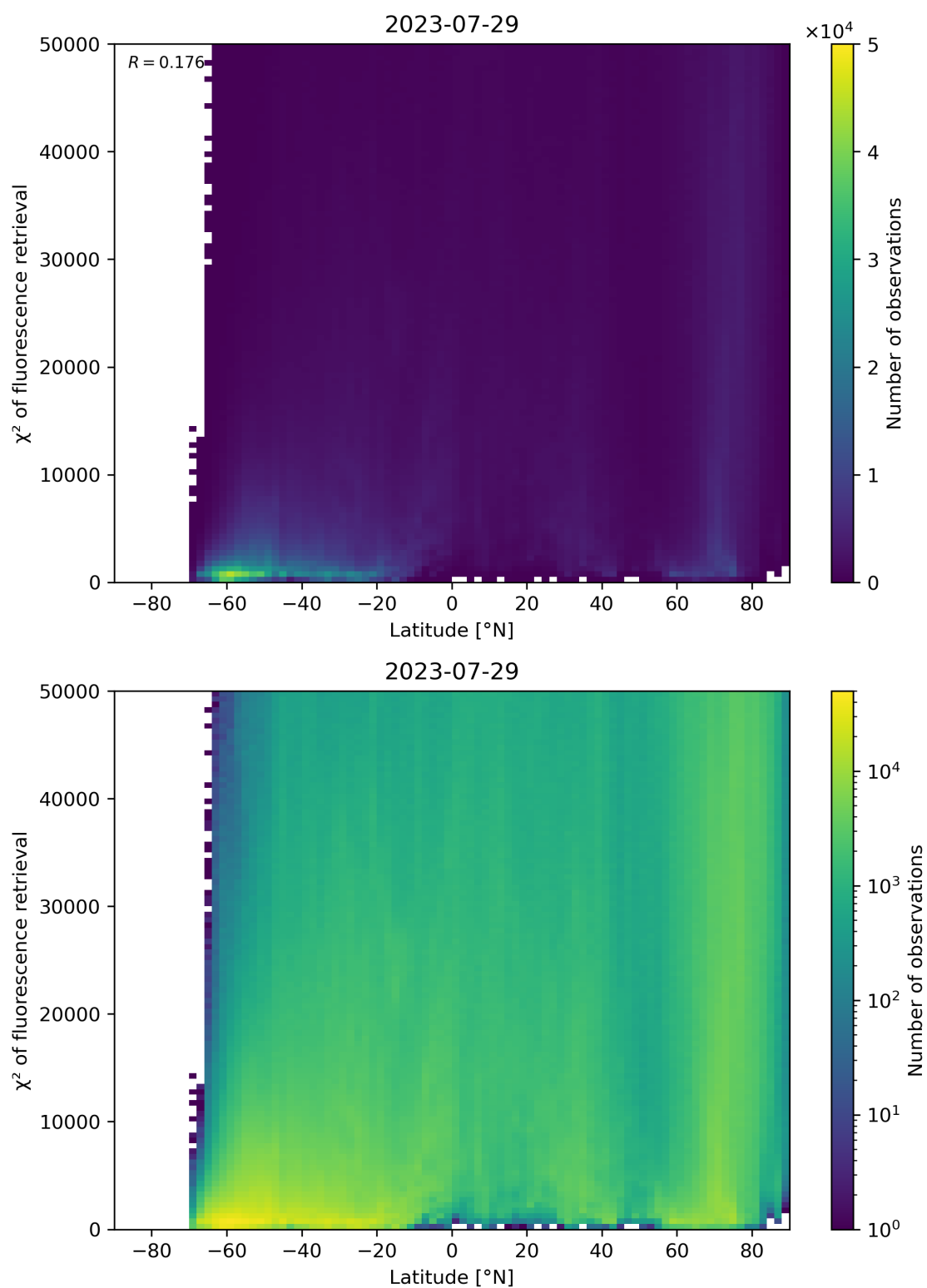
Figure 98: Scatter density plot of “Latitude” against “ \chi^2 of fluorescence retrieval” for 2023-07-29 to 2023-07-30.
