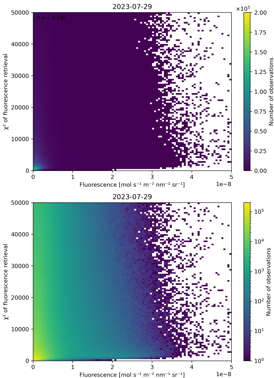
Figure 93: Scatter density plot of “Fluorescence” against “ \chi^2 of fluorescence retrieval” for 2023-07-29 to 2023-07-30.
