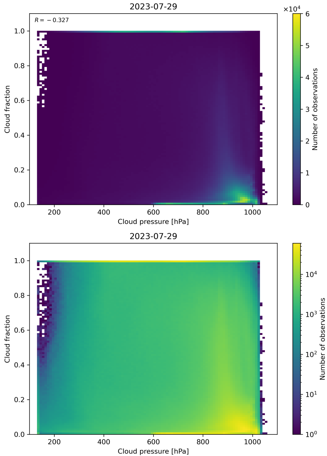
Figure 87: Scatter density plot of “Cloud pressure” against “Cloud fraction” for 2023-07-29 to 2023-07-30.
