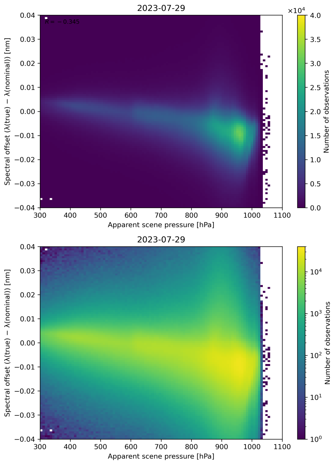
Figure 68: Scatter density plot of “Apparent scene pressure” against “Spectral offset ( \lambda(\text{true}) - \lambda(\text{nominal}) )” for 2023-07-29 to 2023-07-30.
