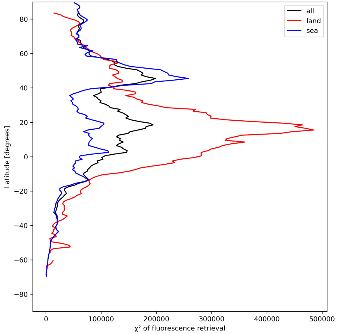
Figure 25: Zonal average of “ \chi^2 of fluorescence retrieval” for 2023-07-29 to 2023-07-30.
