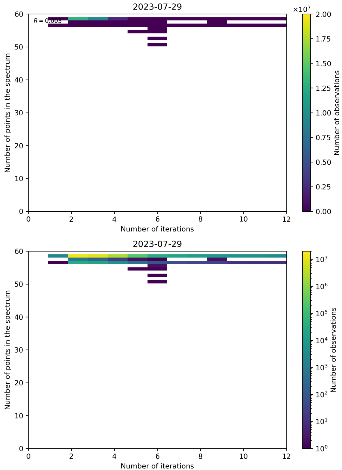
Figure 108: Scatter density plot of “Number of iterations” against “Number of points in the spectrum” for 2023-07-29 to 2023-07-30.
