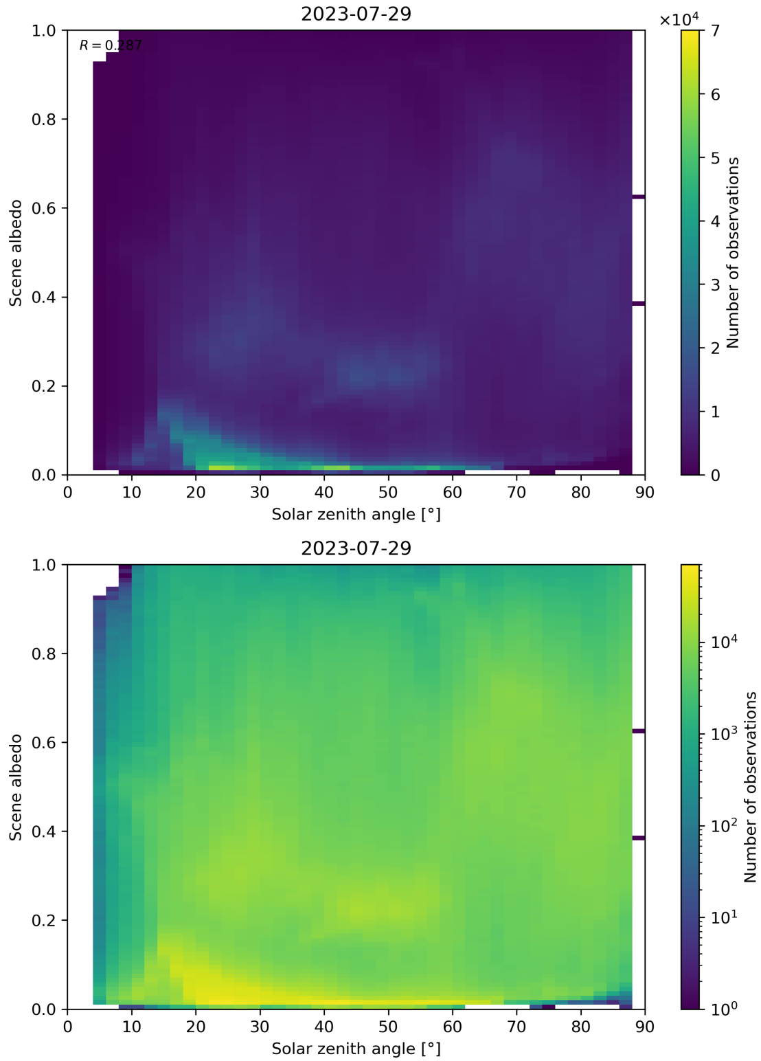
Figure 127: Scatter density plot of “Solar zenith angle” against “Scene albedo” for 2023-07-29 to 2023-07-30.
