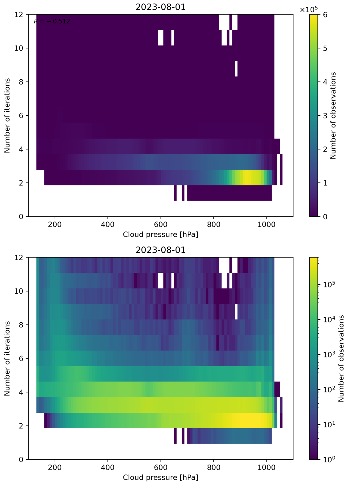
Figure 89: Scatter density plot of “Cloud pressure” against “Number of iterations” for 2023-07-31 to 2023-08-02.
