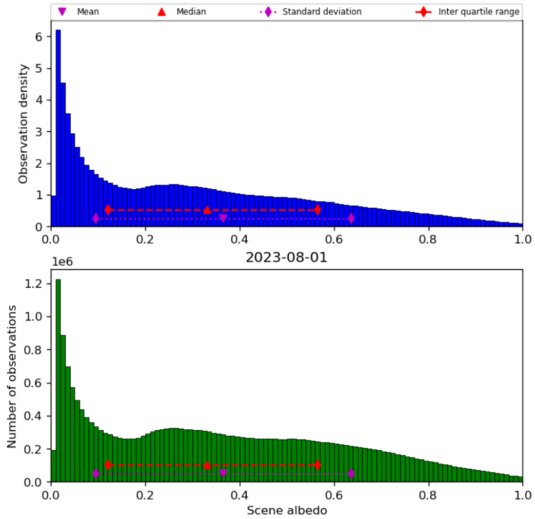
Figure 34: Histogram of “Scene albedo” for 2023-07-31 to 2023-08-02
