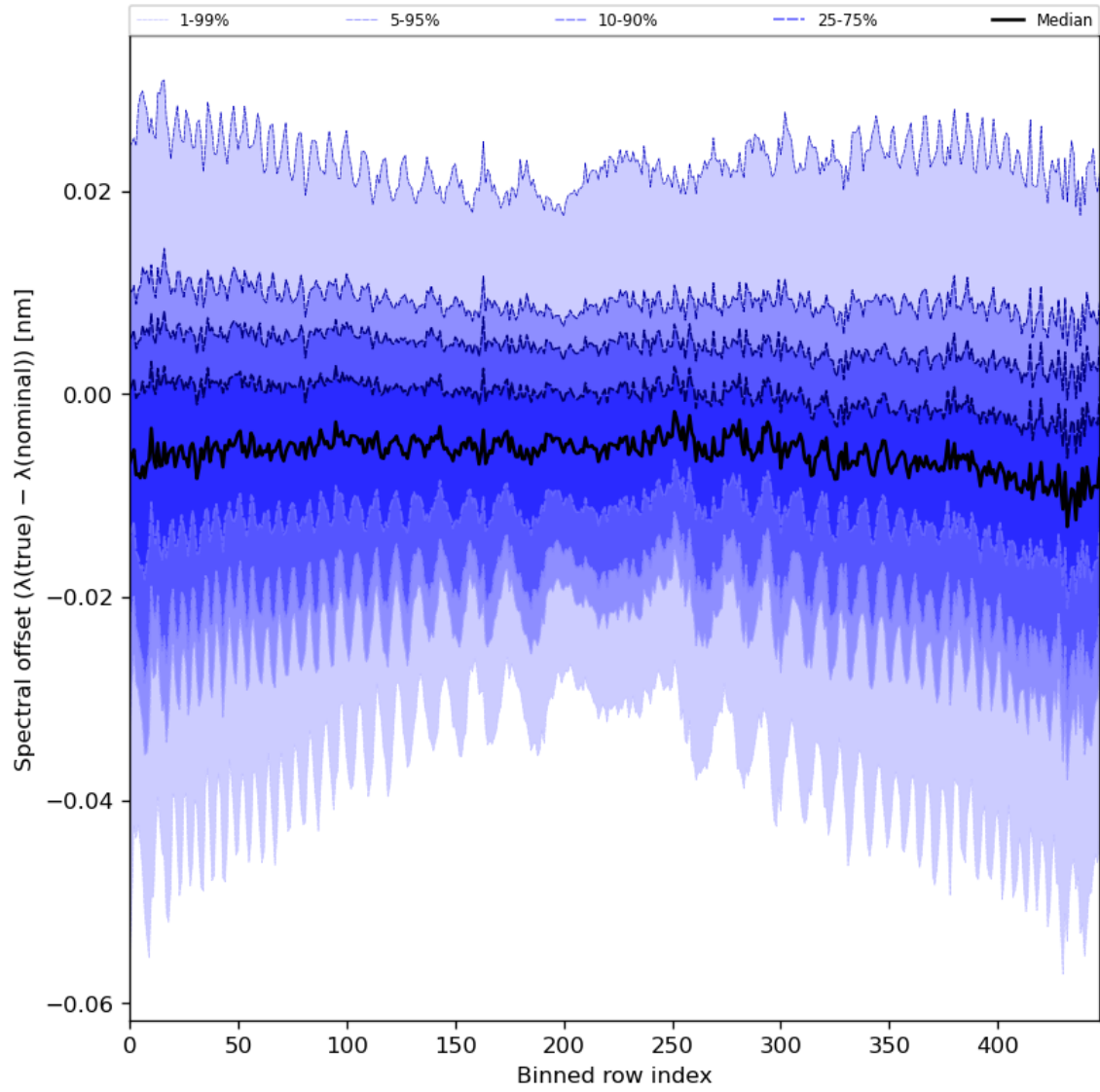
Figure 62: Along track statistics of “Spectral offset ( \lambda(\text{true}) - \lambda(\text{nominal}) )” for 2023-07-31 to 2023-08-02
