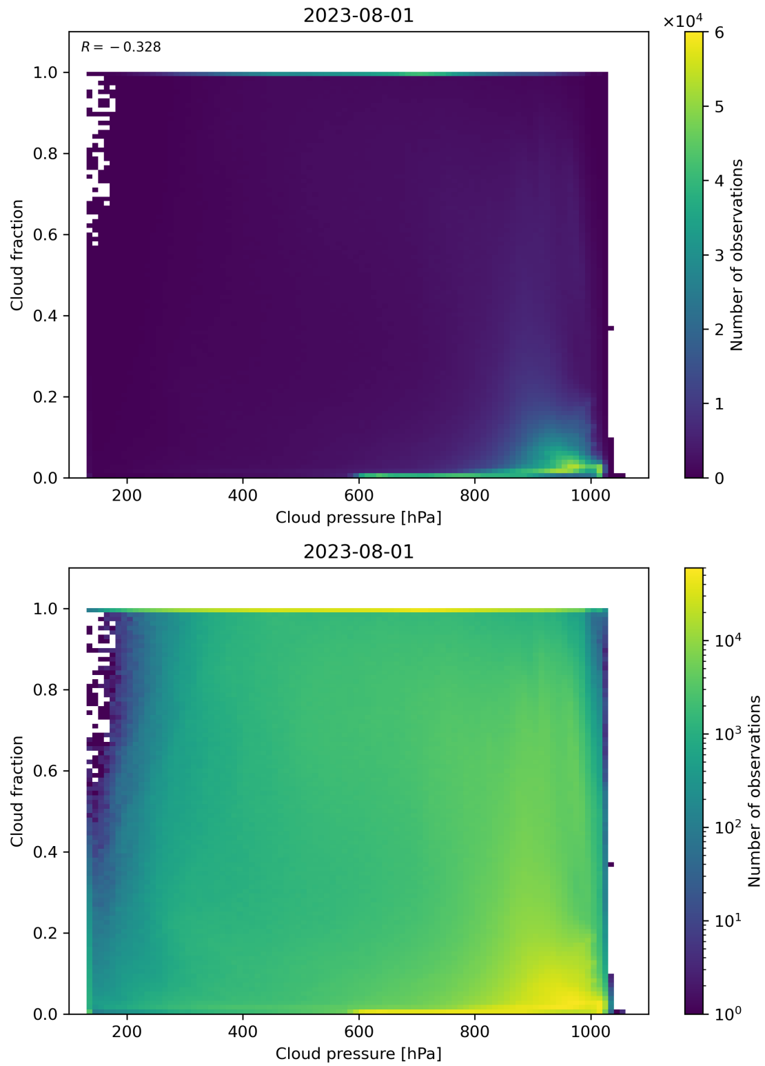
Figure 87: Scatter density plot of “Cloud pressure” against “Cloud fraction” for 2023-07-31 to 2023-08-02.
