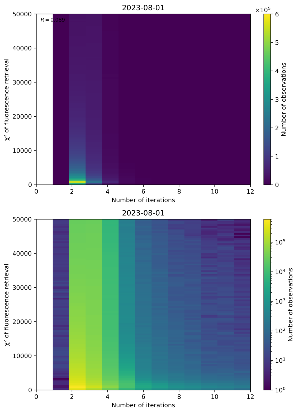
Figure 106: Scatter density plot of “Number of iterations” against “ \chi^2 of fluorescence retrieval” for 2023-07-31 to 2023-08-02.
