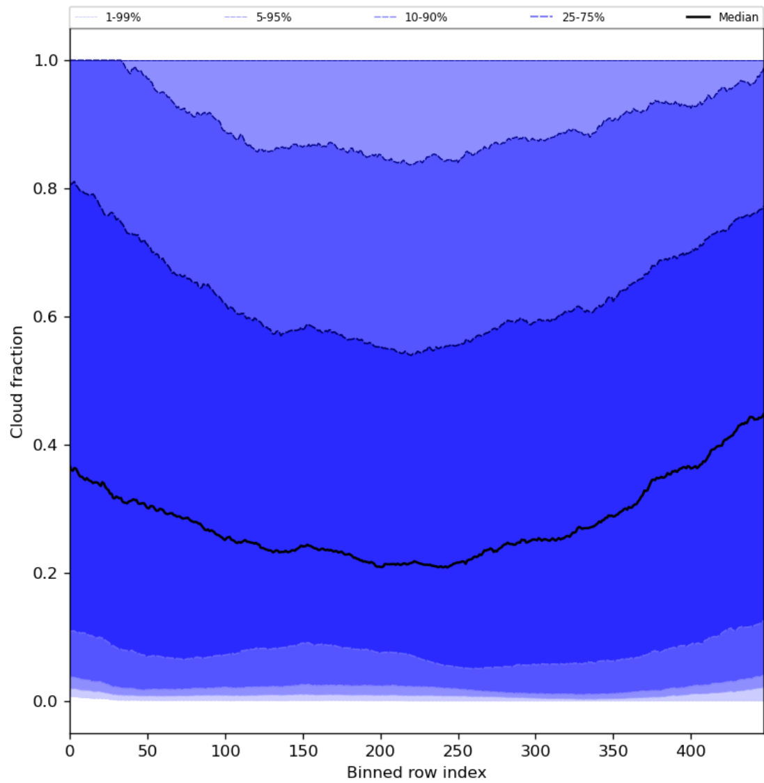
Figure 49: Along track statistics of “Cloud fraction” for 2023-07-31 to 2023-08-02
