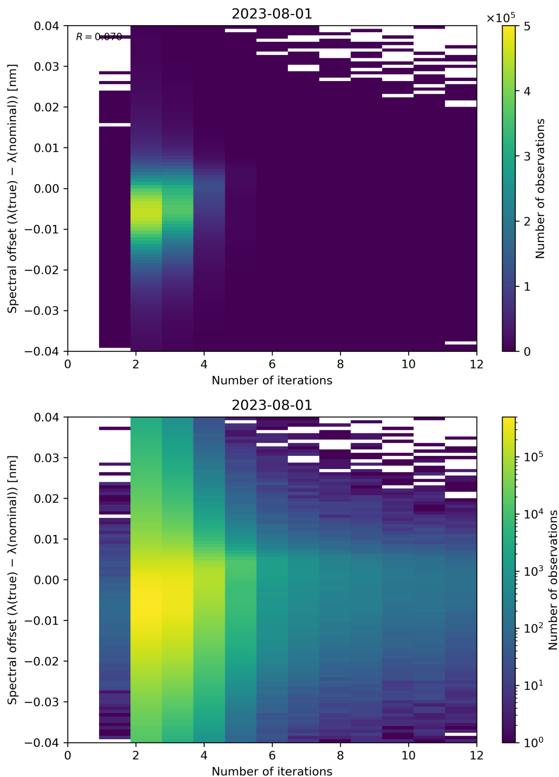
Figure 109: Scatter density plot of “Number of iterations” against “Spectral offset ( \lambda(\text{true}) - \lambda(\text{nominal}) )” for 2023-07-31 to 2023-08-02.
