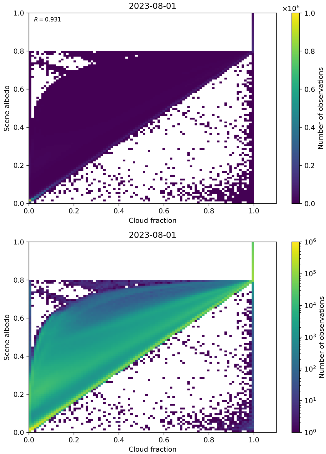
Figure 82: Scatter density plot of “Cloud fraction” against “Scene albedo” for 2023-07-31 to 2023-08-02.
