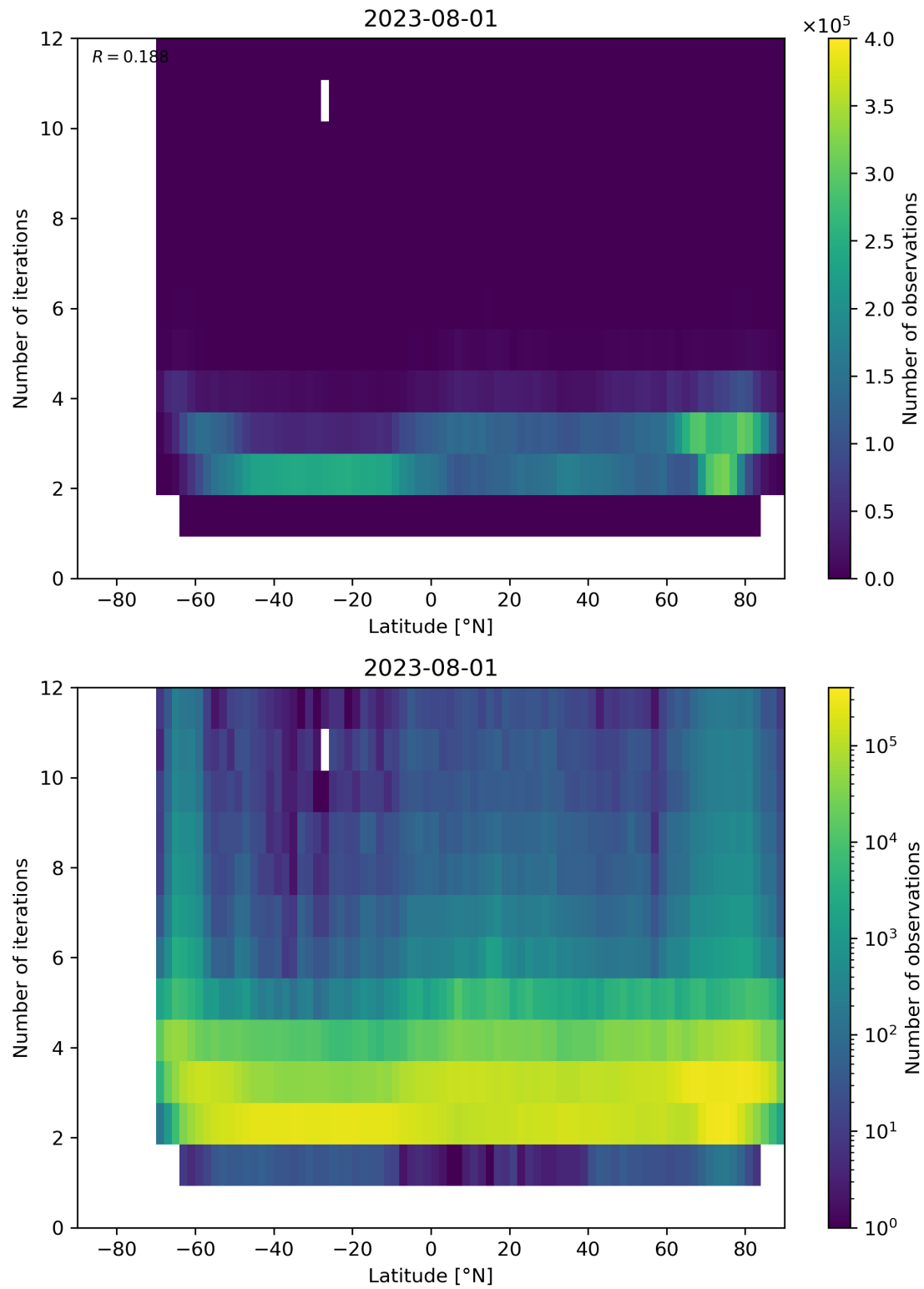
Figure 102: Scatter density plot of “Latitude” against “Number of iterations” for 2023-07-31 to 2023-08-02.
