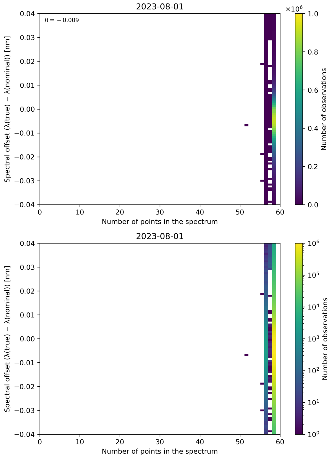
Figure 110: Scatter density plot of “Number of points in the spectrum” against “Spectral offset ( \lambda(\text{true}) - \lambda(\text{nominal}) )” for 2023-07-31 to 2023-08-02.
