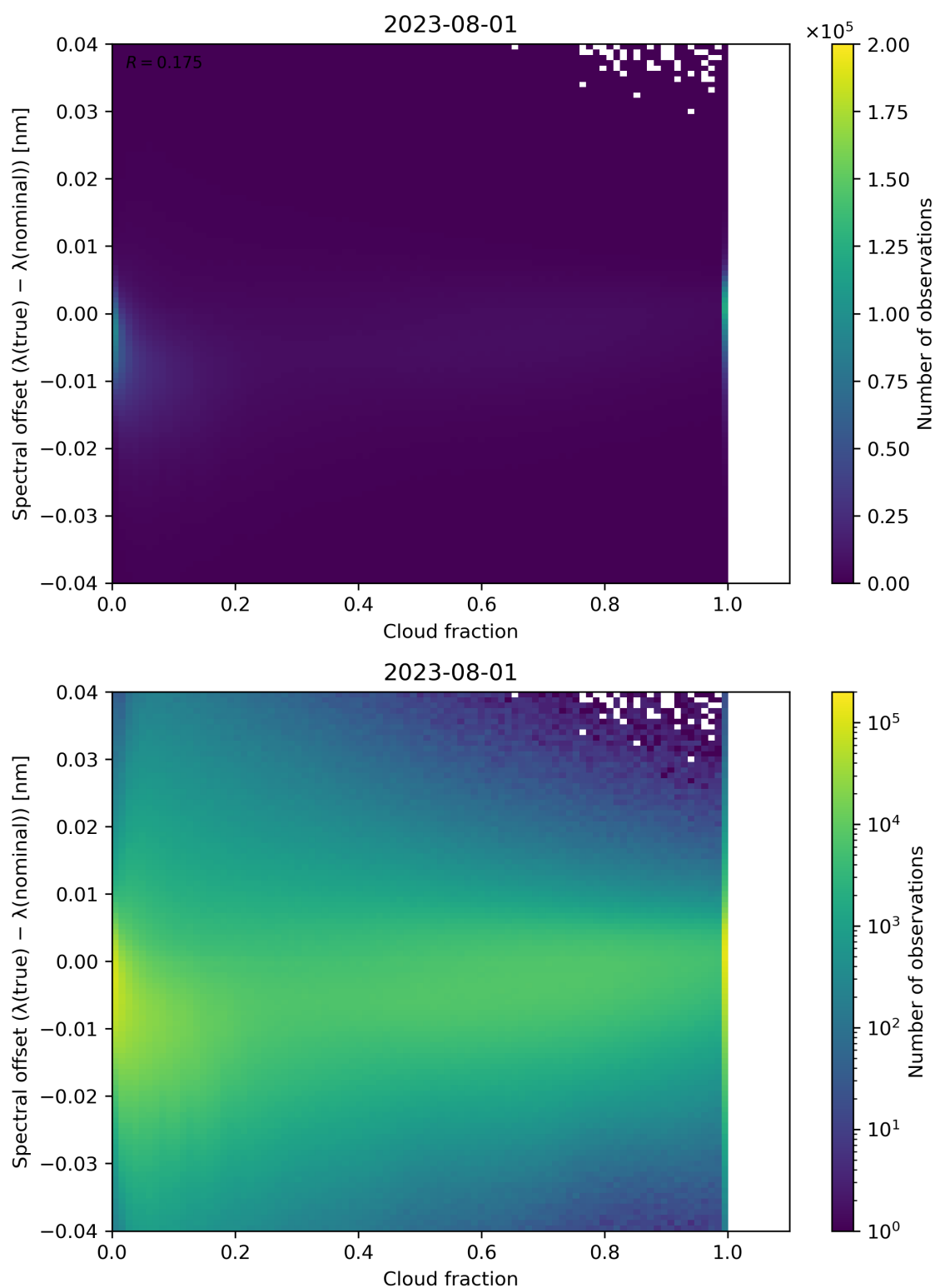
Figure 83: Scatter density plot of “Cloud fraction” against “Spectral offset ( \lambda(\text{true}) - \lambda(\text{nominal}) )” for 2023-07-31 to 2023-08-02.
