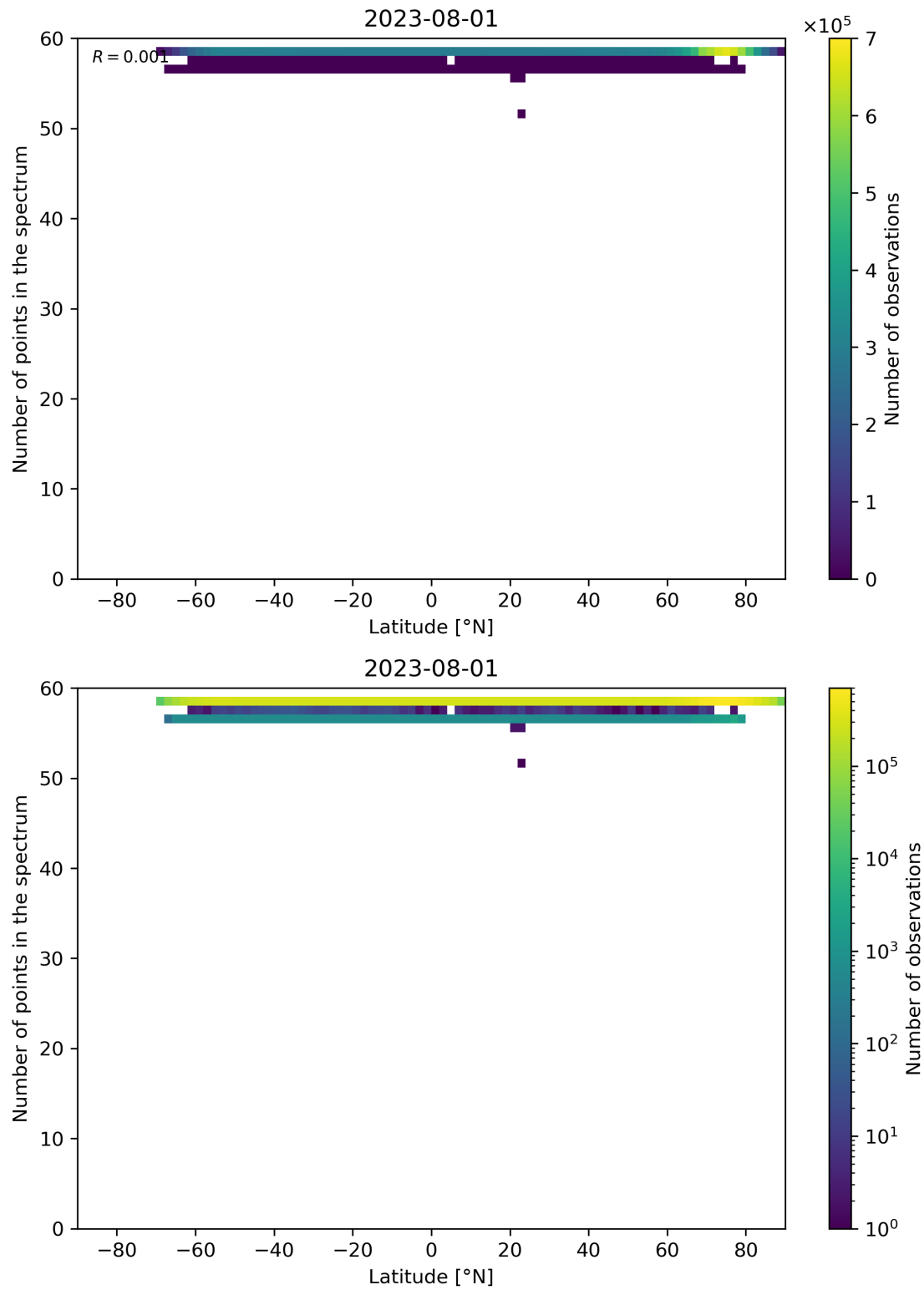
Figure 103: Scatter density plot of “Latitude” against “Number of points in the spectrum” for 2023-07-31 to 2023-08-02.
