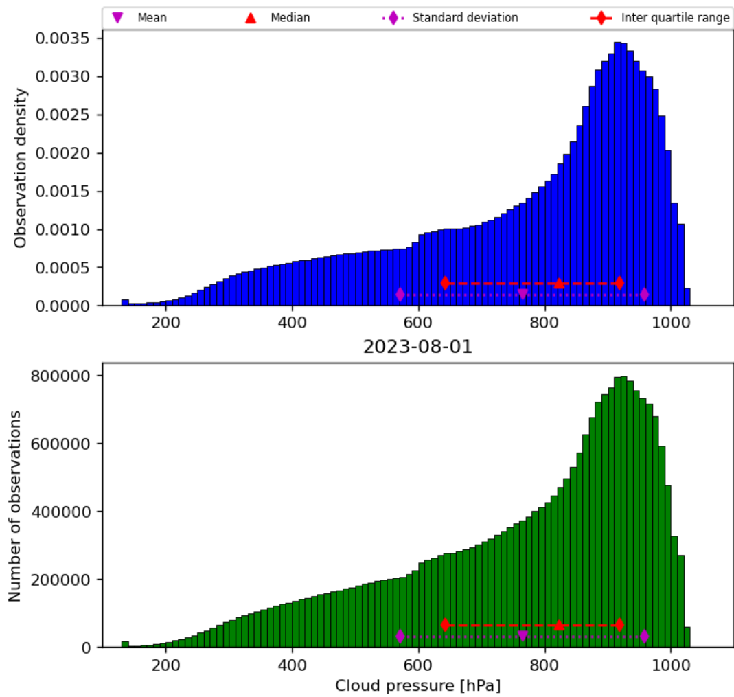
Figure 30: Histogram of “Cloud pressure” for 2023-07-31 to 2023-08-02
