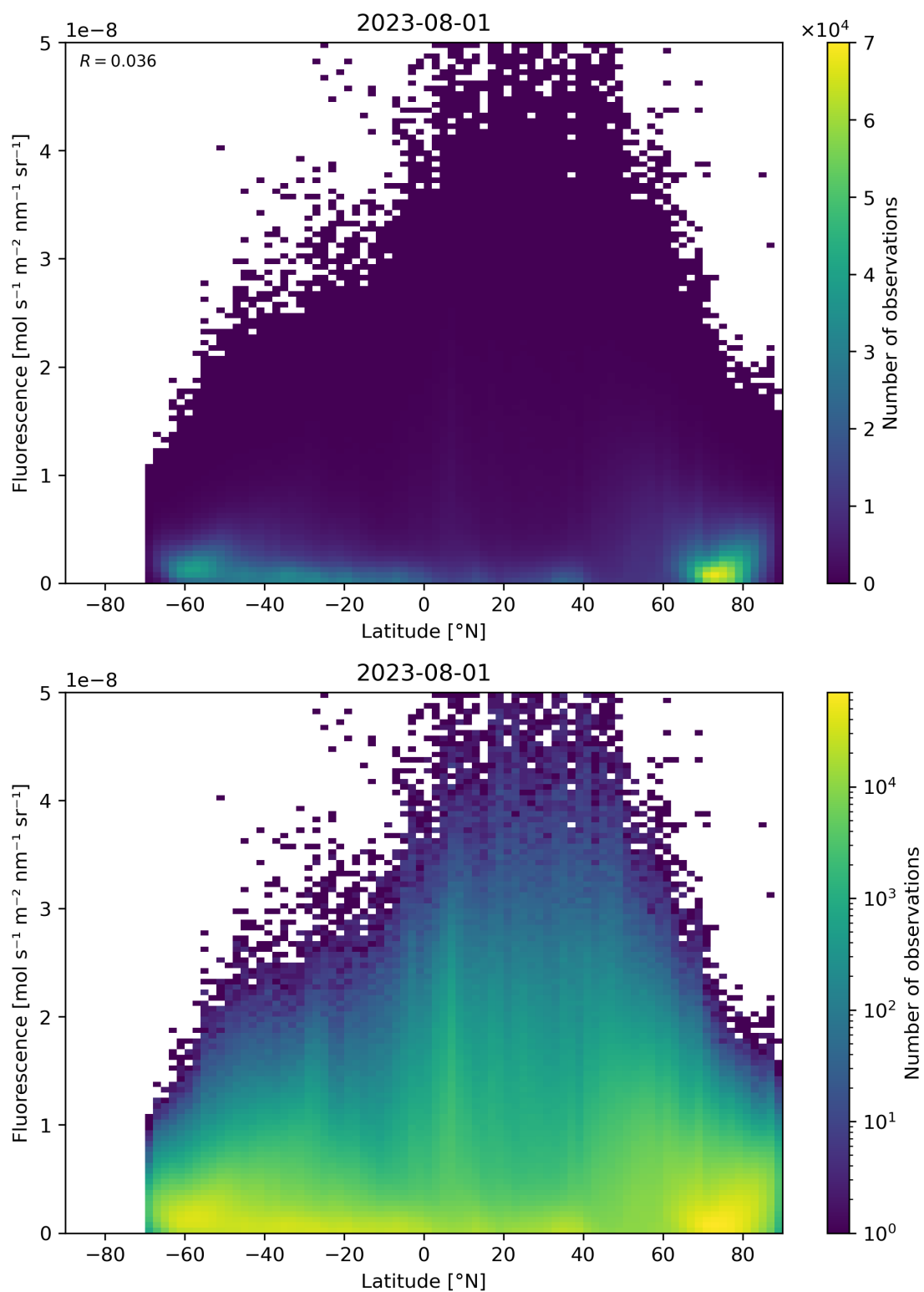
Figure 101: Scatter density plot of “Latitude” against “Fluorescence” for 2023-07-31 to 2023-08-02.
