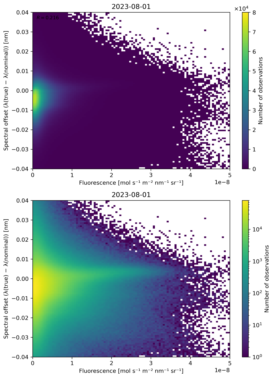
Figure 95: Scatter density plot of “Fluorescence” against “Spectral offset ( \lambda(\text{true}) - \lambda(\text{nominal}) )” for 2023-07-31 to 2023-08-02.
