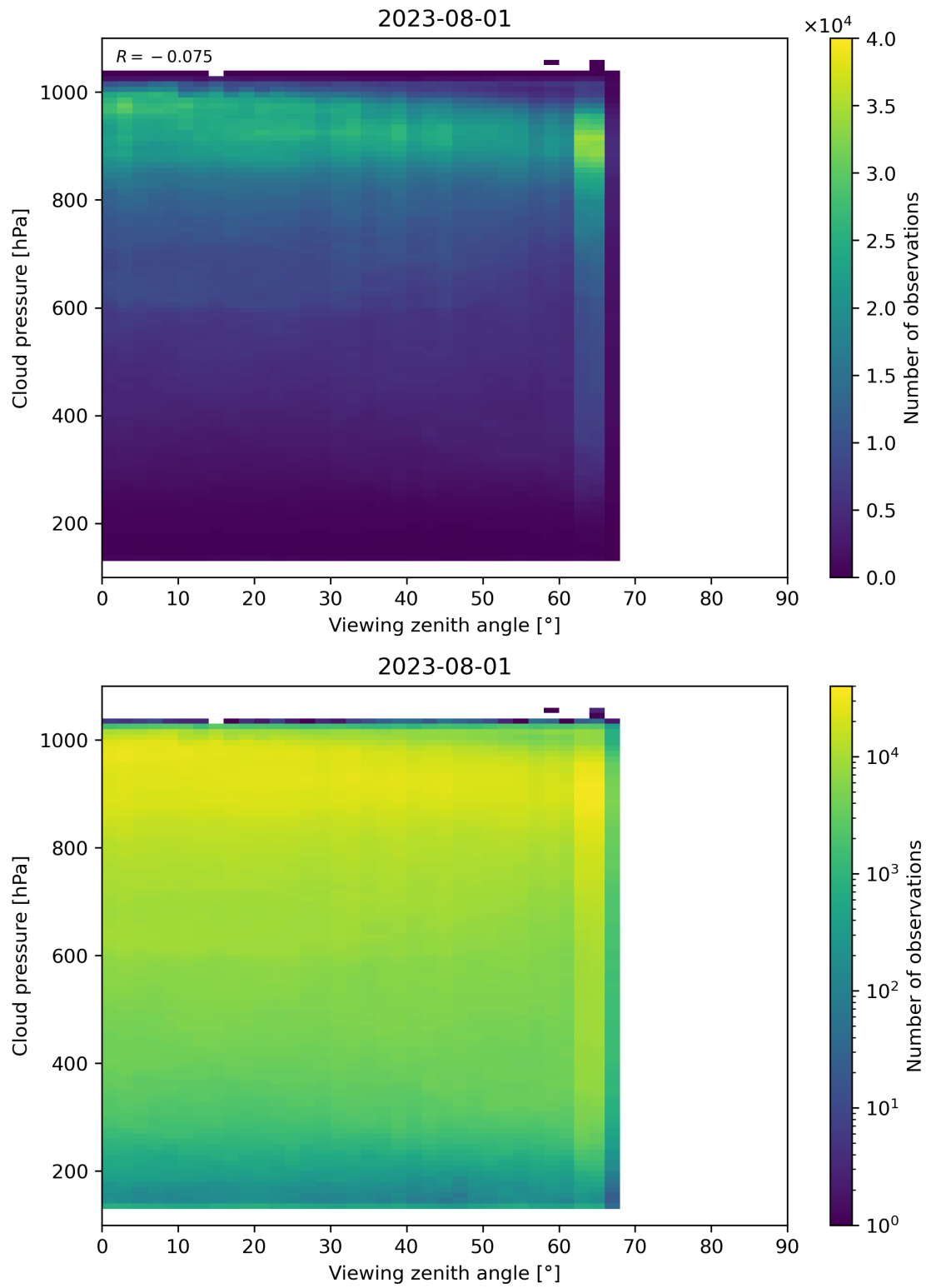
Figure 133: Scatter density plot of “Viewing zenith angle” against “Cloud pressure” for 2023-07-31 to 2023-08-02.
