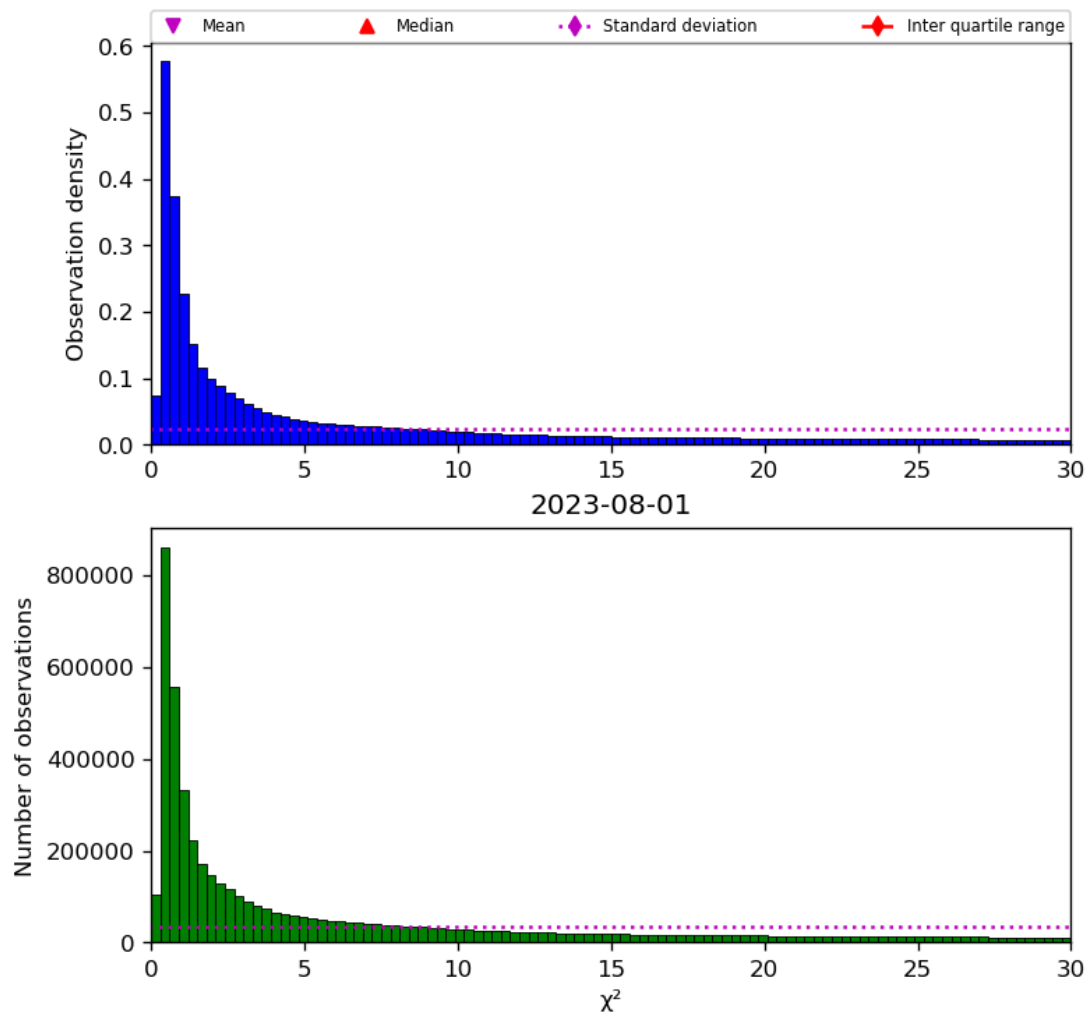
Figure 38: Histogram of “ \chi^2 ” for 2023-07-31 to 2023-08-02
