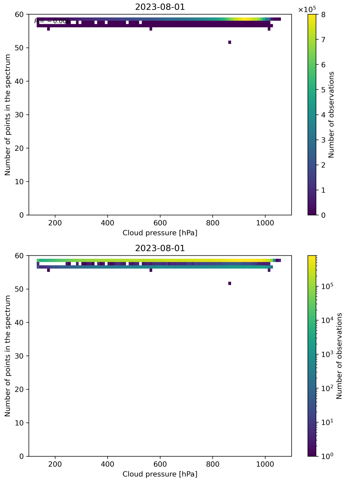
Figure 90: Scatter density plot of “Cloud pressure” against “Number of points in the spectrum” for 2023-07-31 to 2023-08-02.
