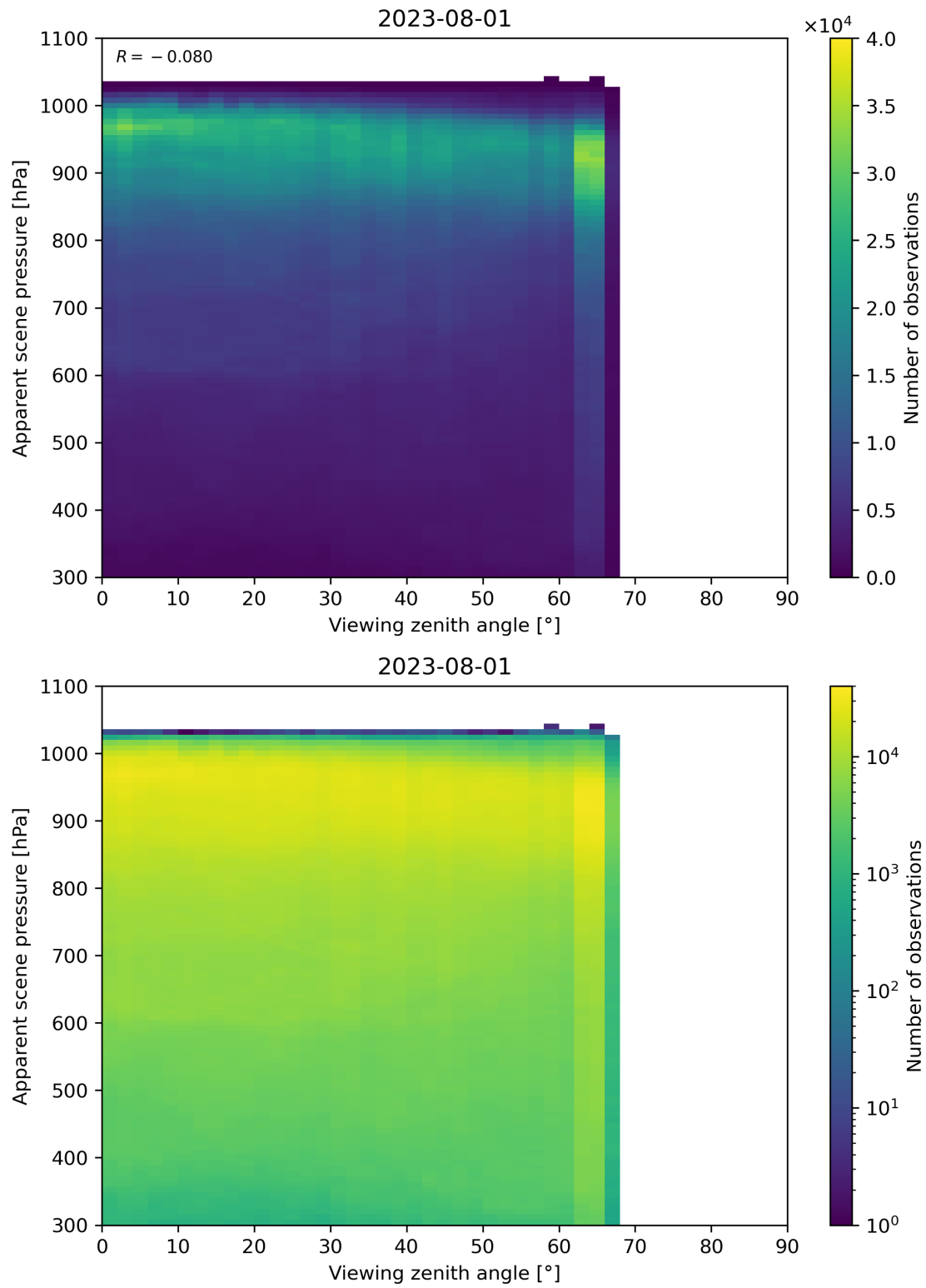
Figure 129: Scatter density plot of “Viewing zenith angle” against “Apparent scene pressure” for 2023-07-31 to 2023-08-02.
