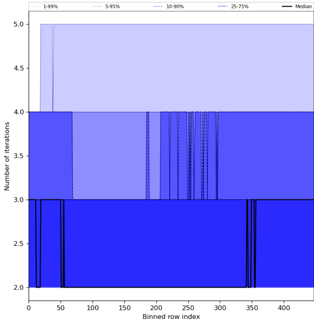
Figure 56: Along track statistics of “Number of iterations” for 2023-07-31 to 2023-08-02
