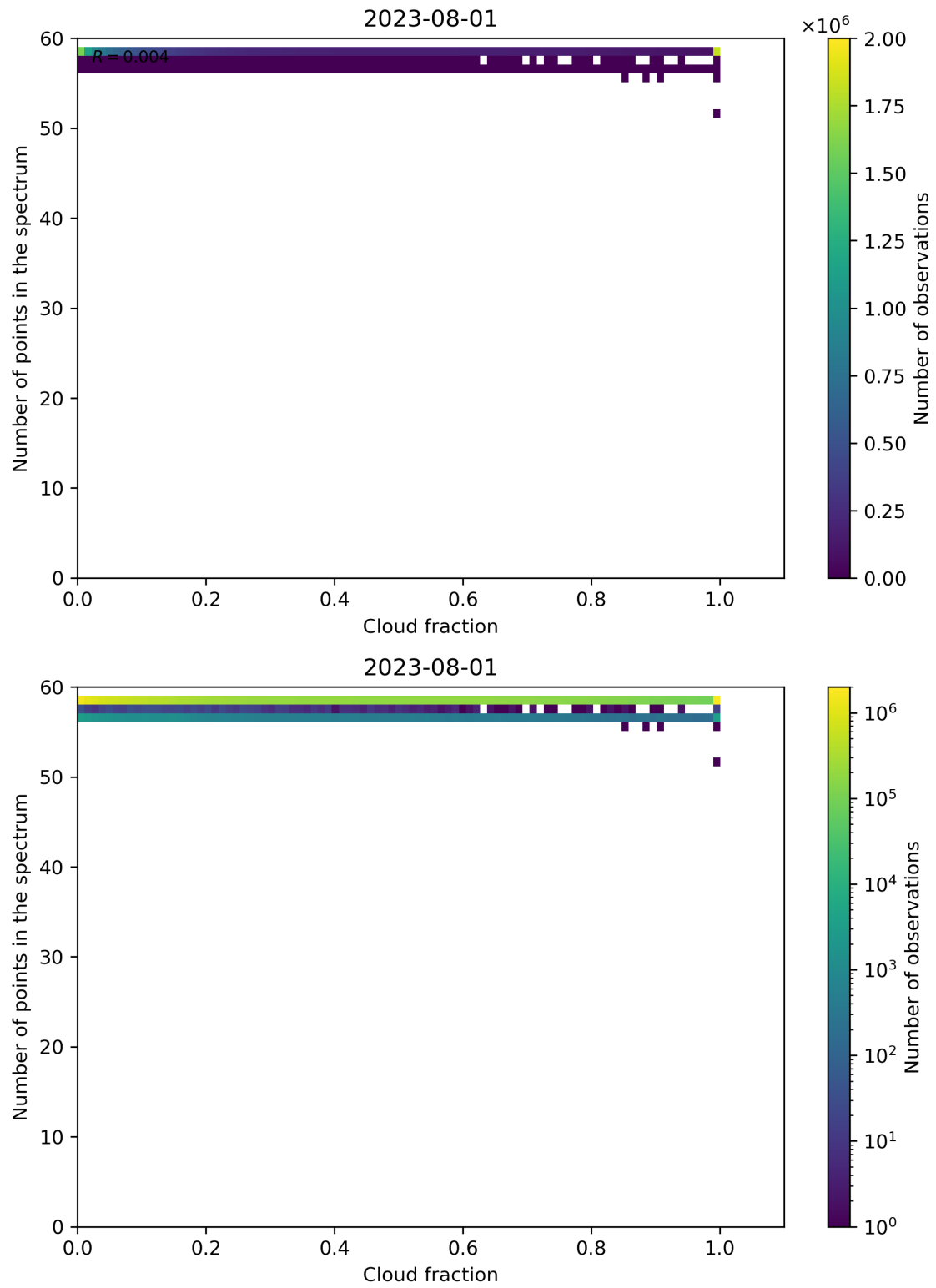
Figure 81: Scatter density plot of “Cloud fraction” against “Number of points in the spectrum” for 2023-07-31 to 2023-08-02.
