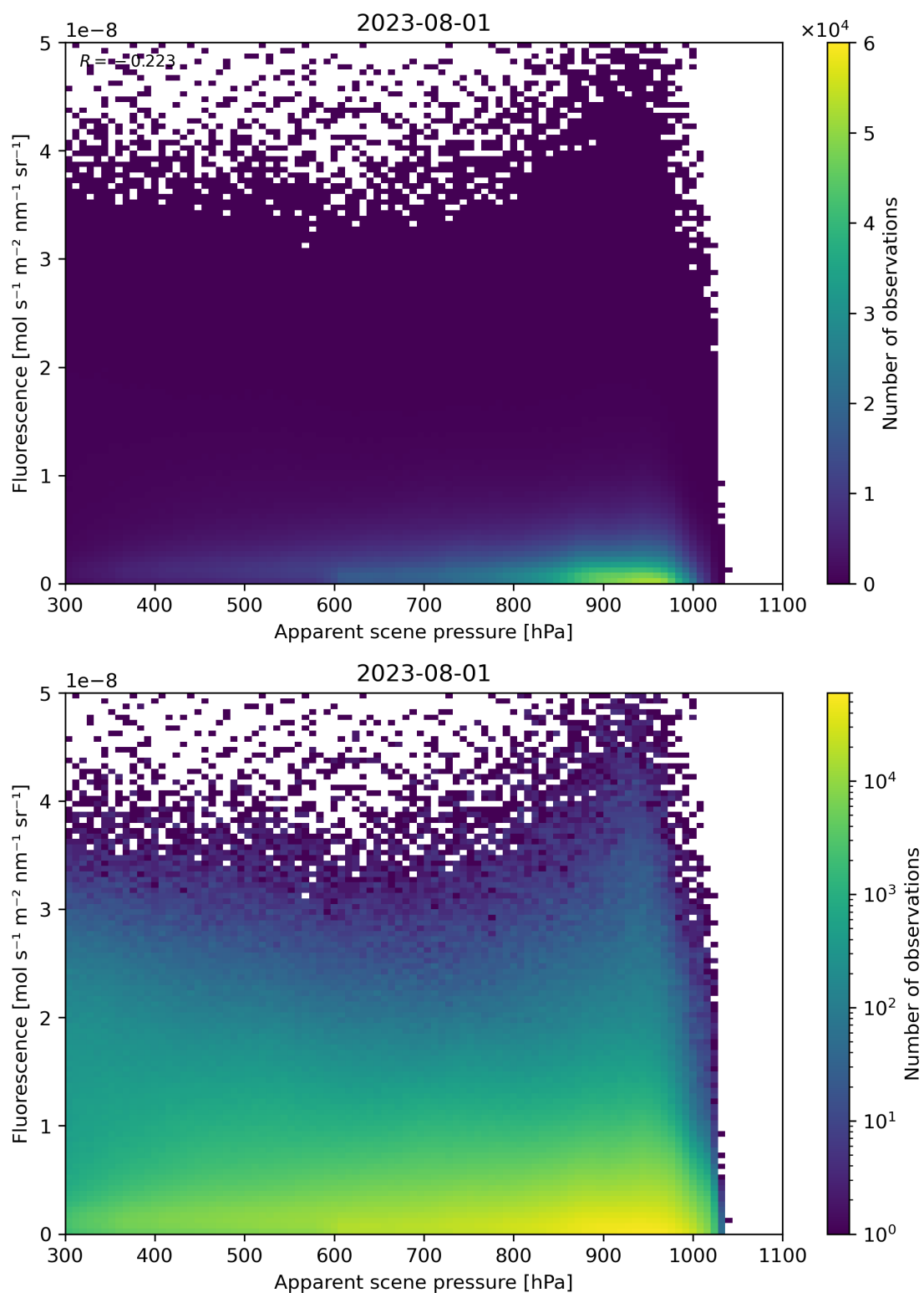
Figure 65: Scatter density plot of “Apparent scene pressure” against “Fluorescence” for 2023-07-31 to 2023-08-02.
