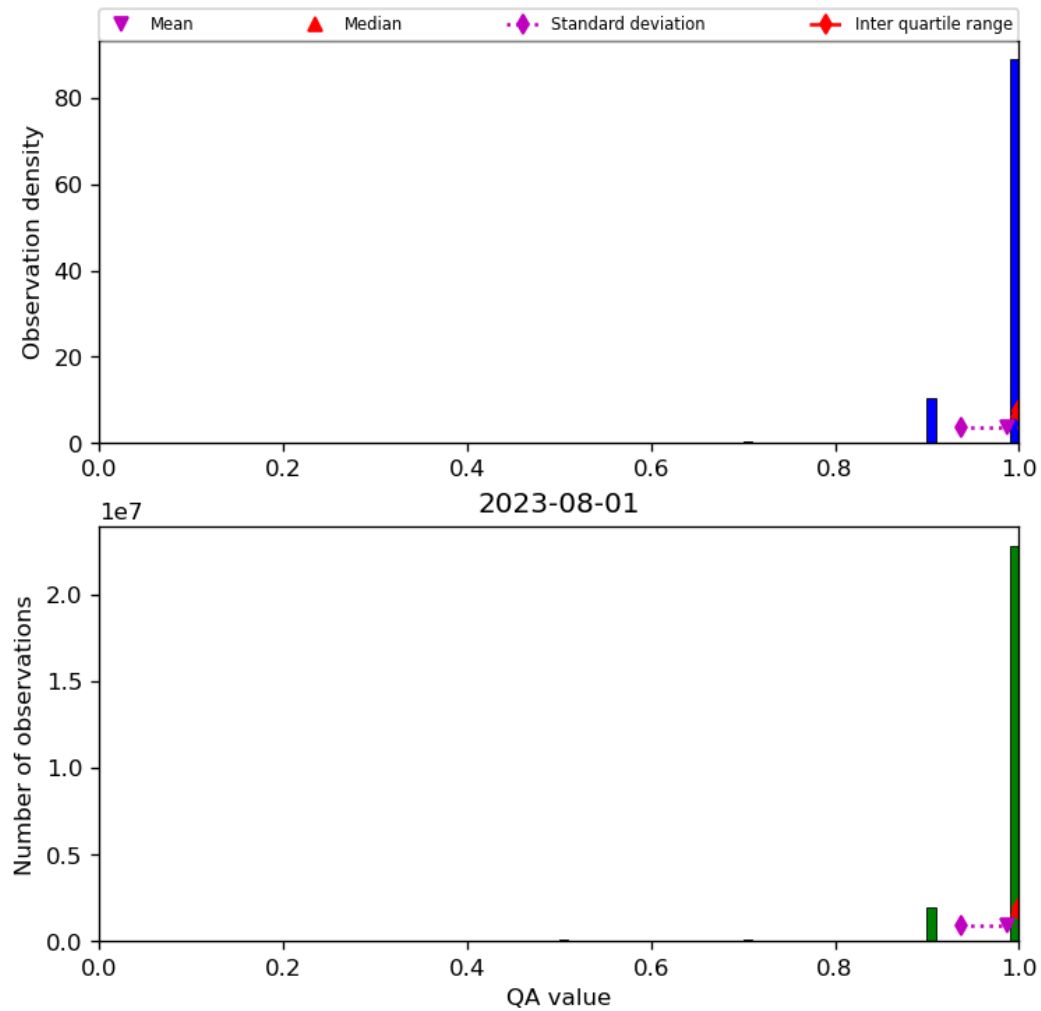
Figure 29: Histogram of “QA value” for 2023-07-31 to 2023-08-02
