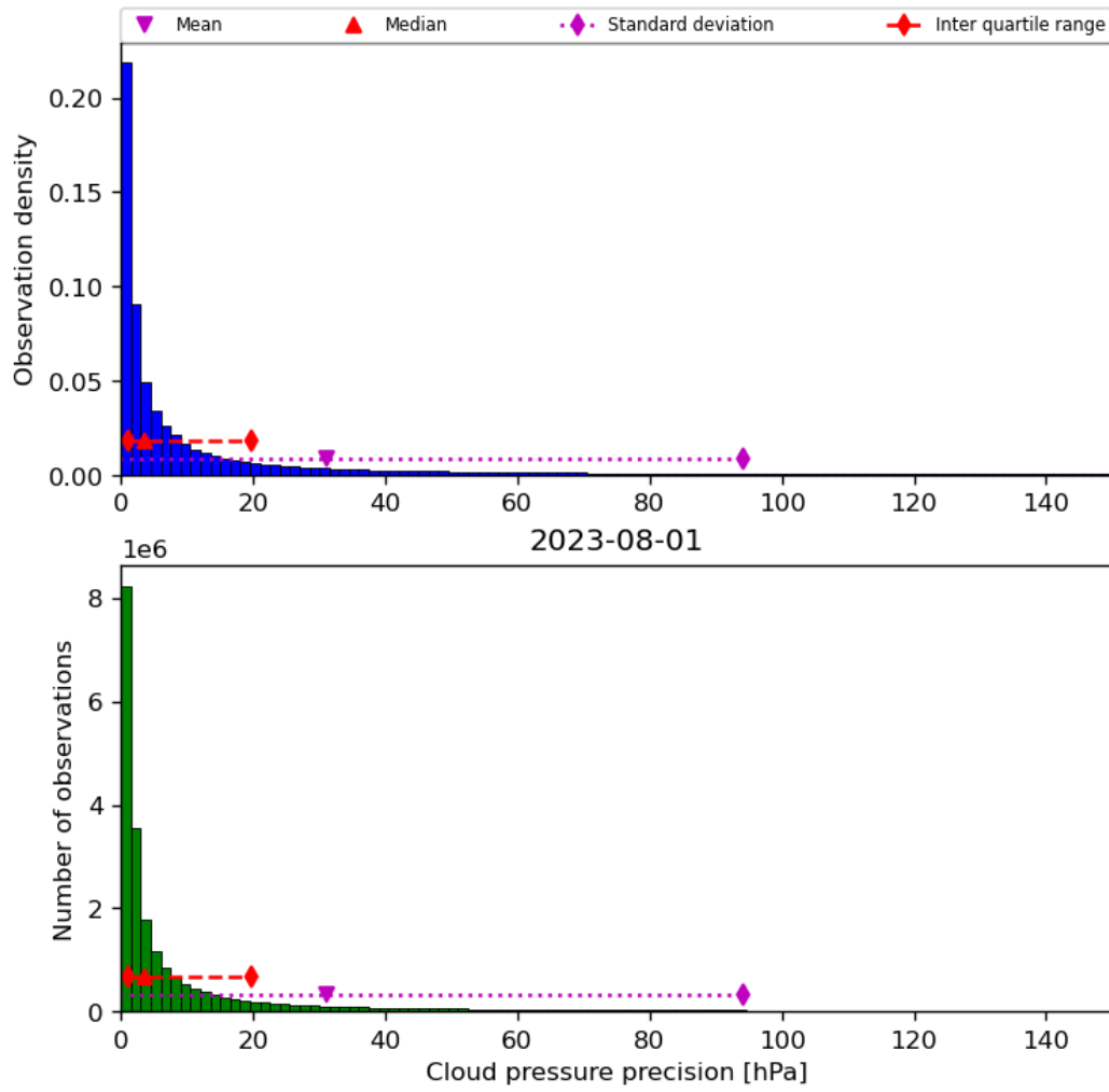
Figure 31: Histogram of “Cloud pressure precision” for 2023-07-31 to 2023-08-02
