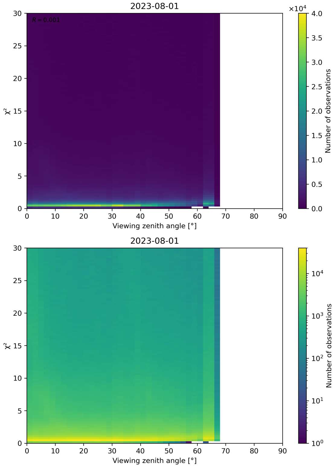
Figure 130: Scatter density plot of “Viewing zenith angle” against “ \chi^2 ” for 2023-07-31 to 2023-08-02.
