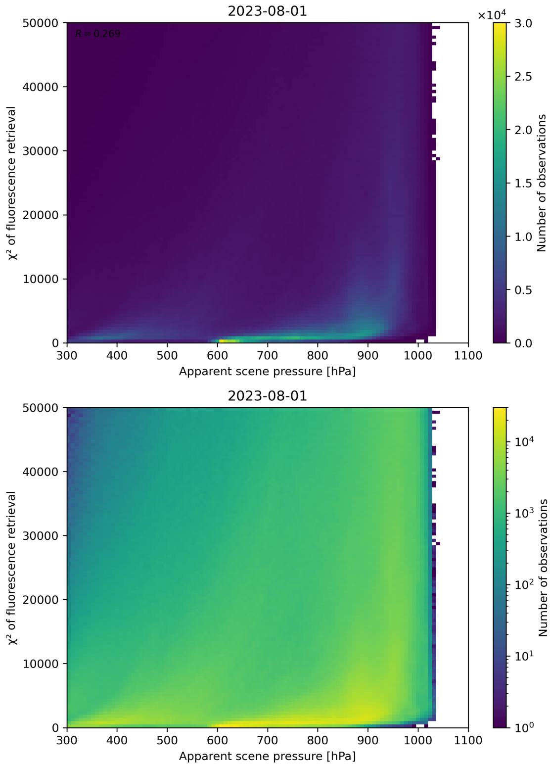
Figure 64: Scatter density plot of “Apparent scene pressure” against “ \chi^2 of fluorescence retrieval” for 2023-07-31 to 2023-08-02.
