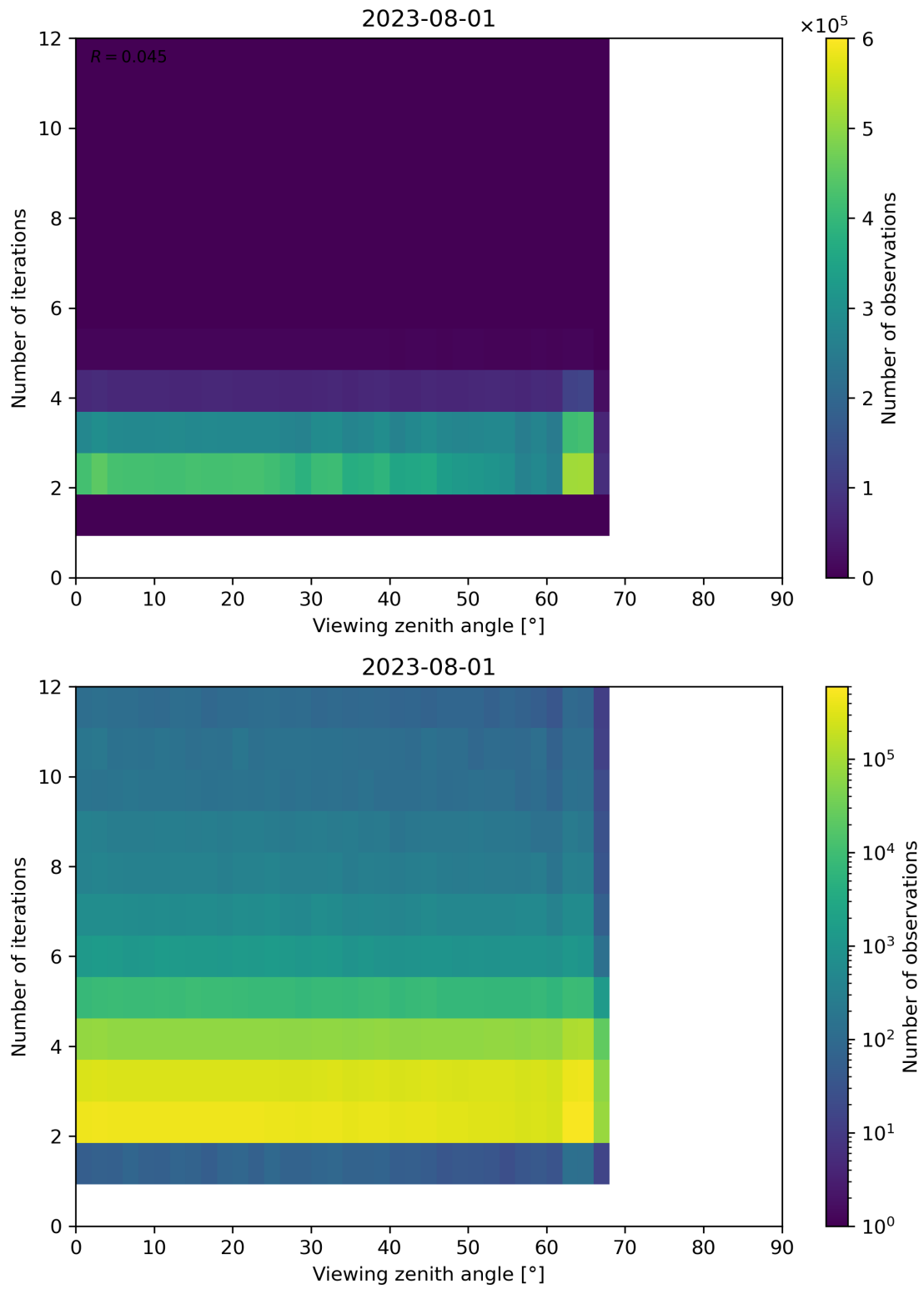
Figure 136: Scatter density plot of “Viewing zenith angle” against “Number of iterations” for 2023-07-31 to 2023-08-02.
