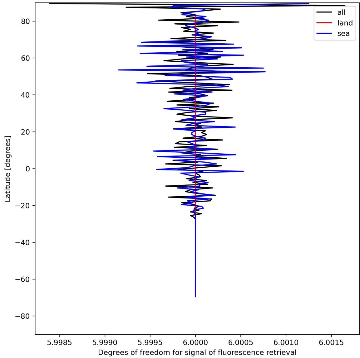
Figure 26: Zonal average of “Degrees of freedom for signal of fluorescence retrieval” for 2023-07-31 to 2023-08-02.
