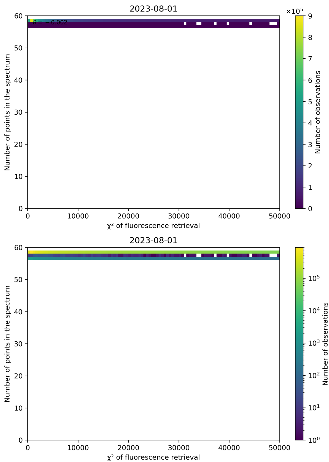
Figure 71: Scatter density plot of " \chi^2 of fluorescence retrieval" against "Number of points in the spectrum" for 2023-07-31 to 2023-08-02.
