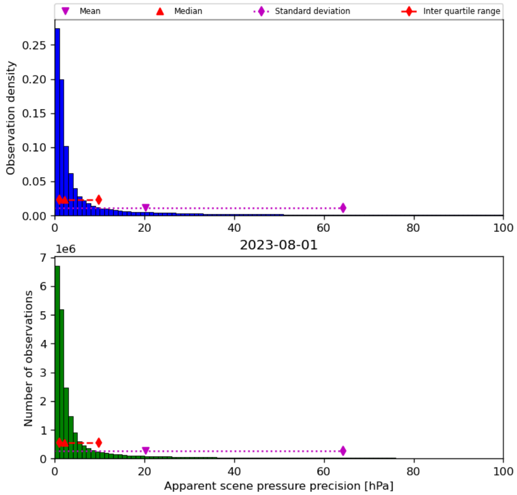
Figure 37: Histogram of “Apparent scene pressure precision” for 2023-07-31 to 2023-08-02
