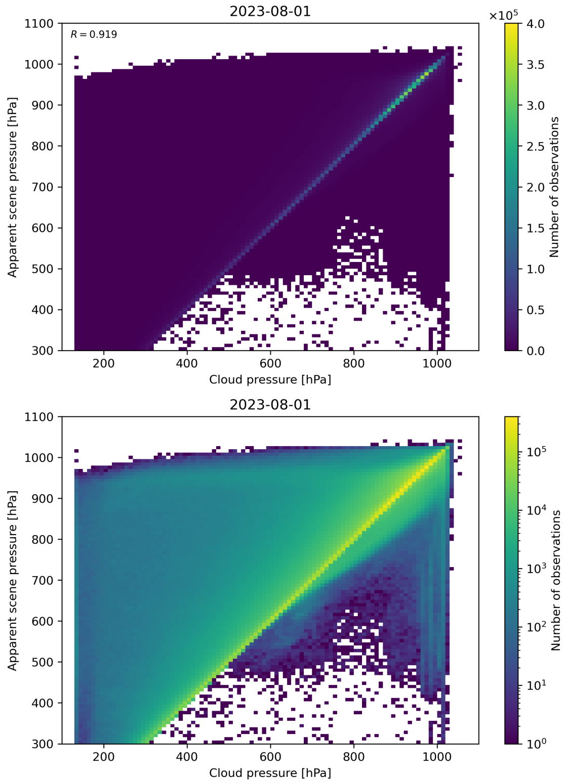
Figure 84: Scatter density plot of “Cloud pressure” against “Apparent scene pressure” for 2023-07-31 to 2023-08-02.
