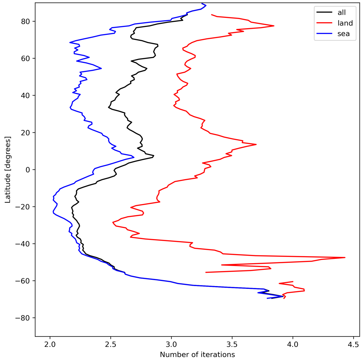
Figure 22: Zonal average of “Number of iterations” for 2023-07-31 to 2023-08-02.
