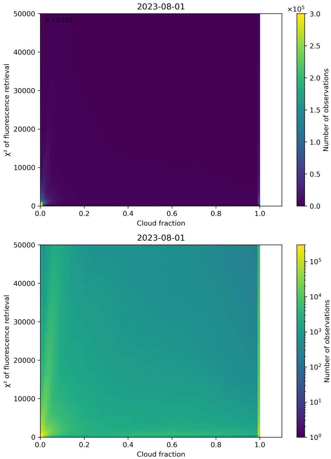
Figure 78: Scatter density plot of “Cloud fraction” against “ \chi^2 of fluorescence retrieval” for 2023-07-31 to 2023-08-02.
