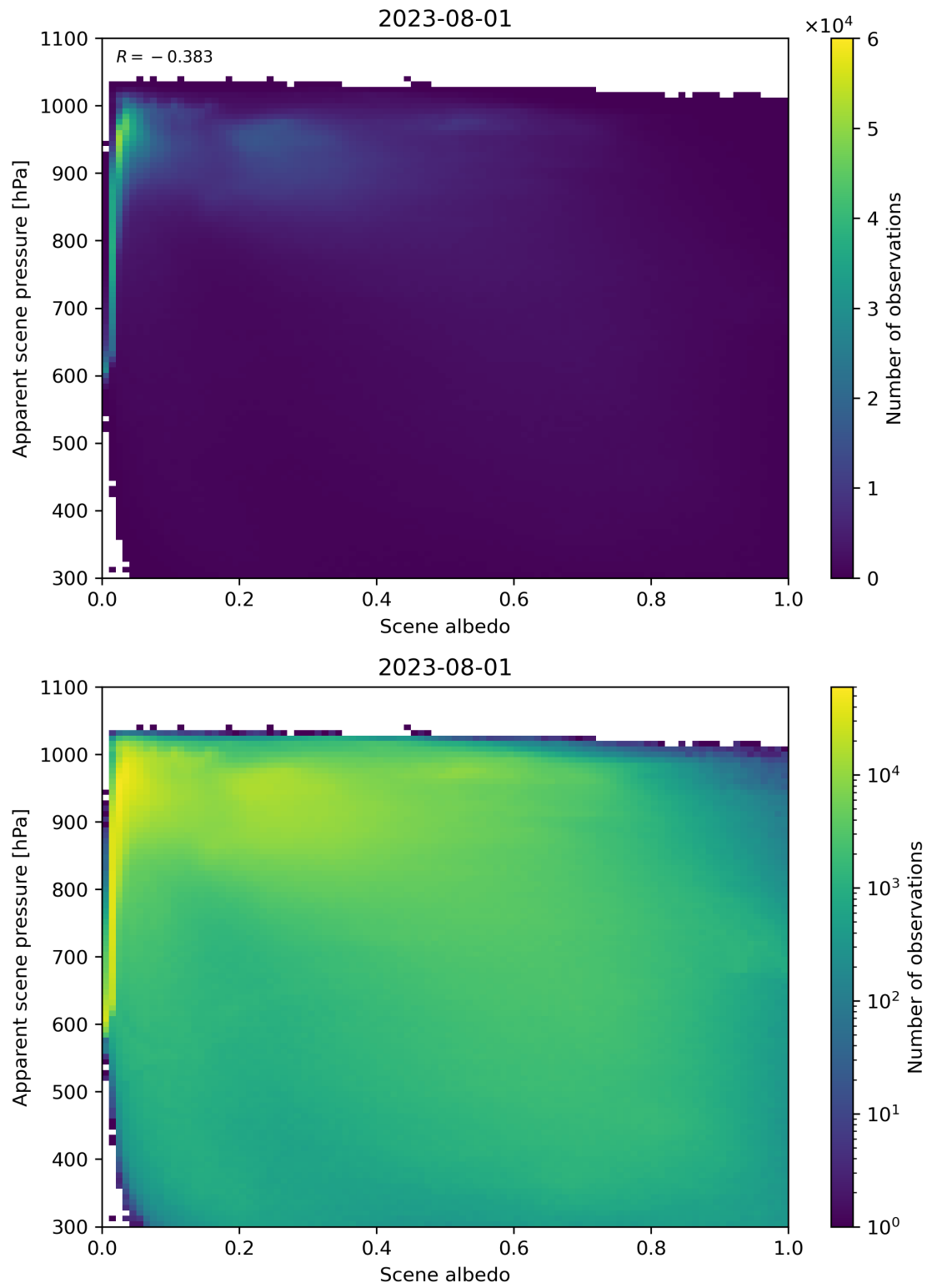
Figure 111: Scatter density plot of “Scene albedo” against “Apparent scene pressure” for 2023-07-31 to 2023-08-02.
