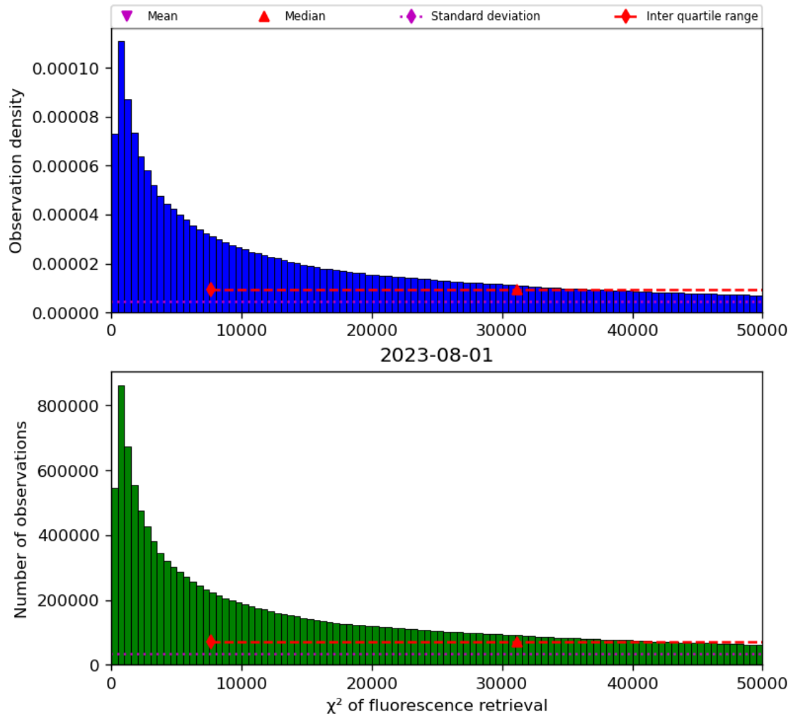
Figure 42: Histogram of “ \chi^2 of fluorescence retrieval” for 2023-07-31 to 2023-08-02
