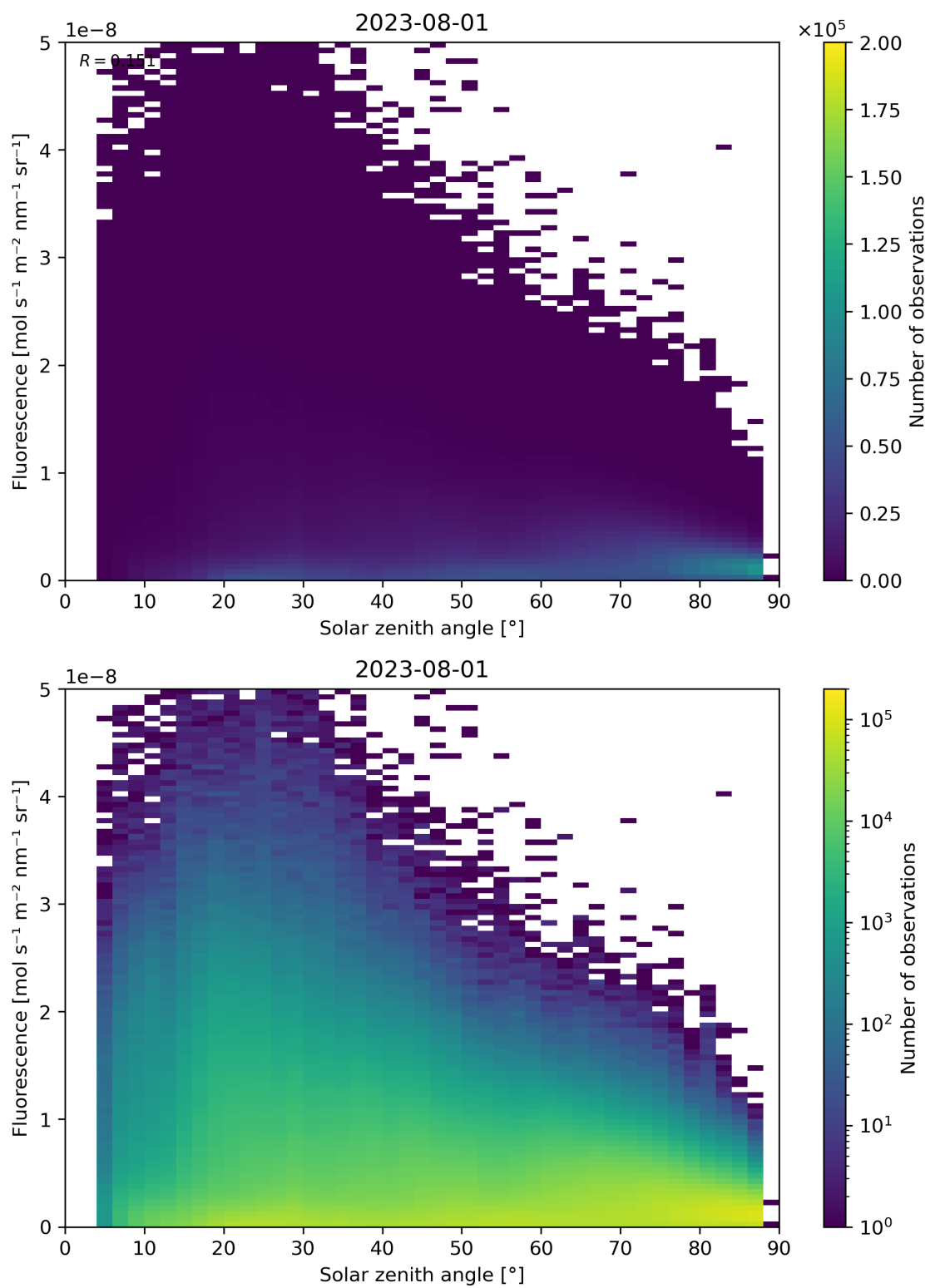
Figure 123: Scatter density plot of “Solar zenith angle” against “Fluorescence” for 2023-07-31 to 2023-08-02.
