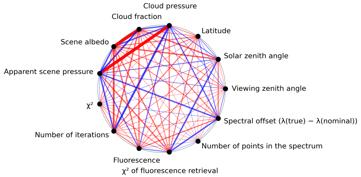
Figure 1: Map of correlation graph for 2023-07-31 to 2023-08-02.
