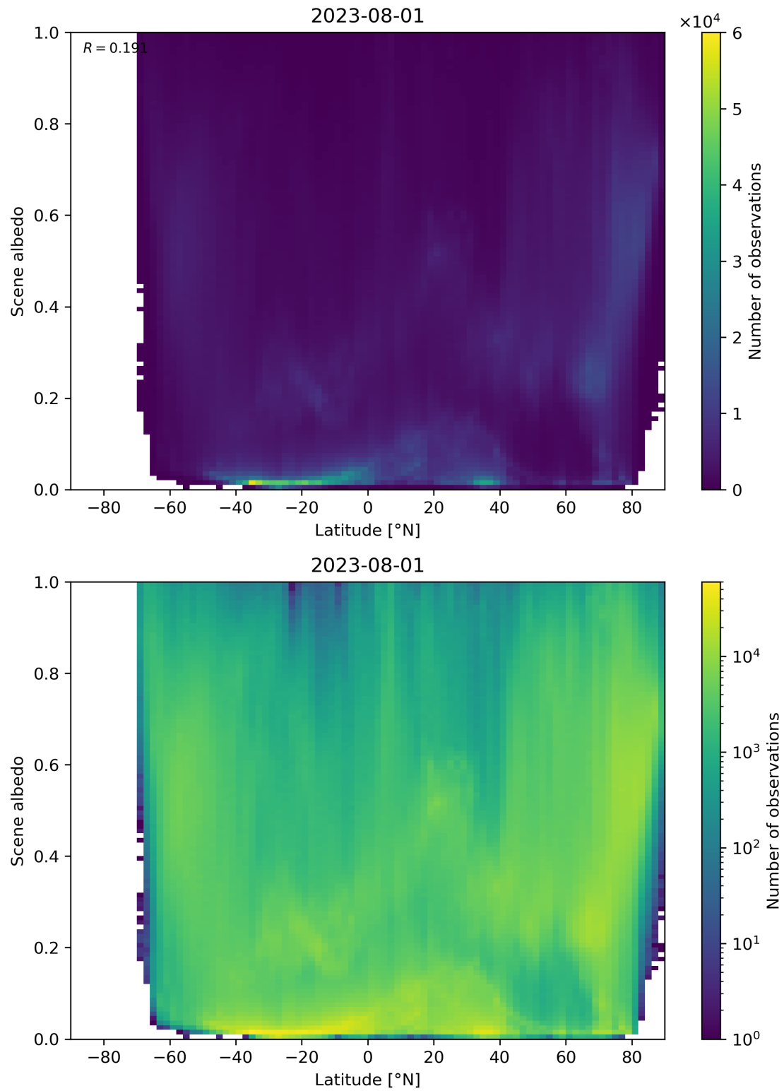
Figure 104: Scatter density plot of “Latitude” against “Scene albedo” for 2023-07-31 to 2023-08-02.
