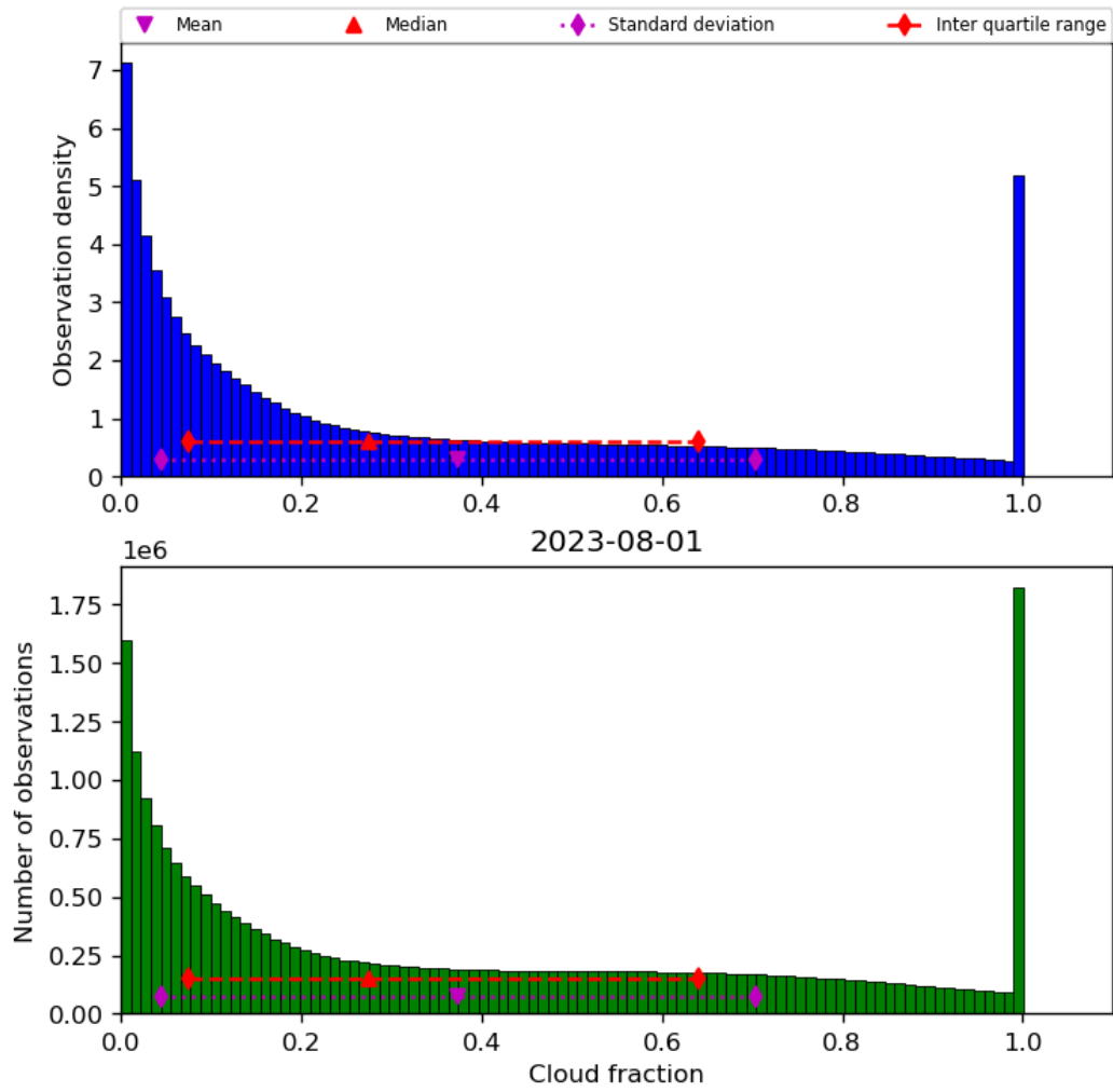
Figure 32: Histogram of “Cloud fraction” for 2023-07-31 to 2023-08-02
