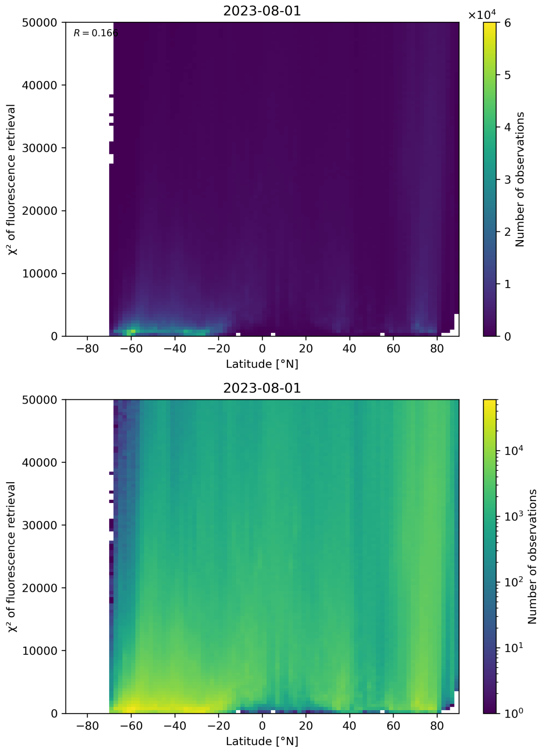
Figure 98: Scatter density plot of “Latitude” against “ \chi^2 of fluorescence retrieval” for 2023-07-31 to 2023-08-02.
