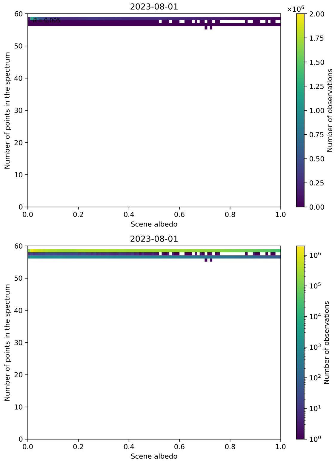
Figure 116: Scatter density plot of “Scene albedo” against “Number of points in the spectrum” for 2023-07-31 to 2023-08-02.
