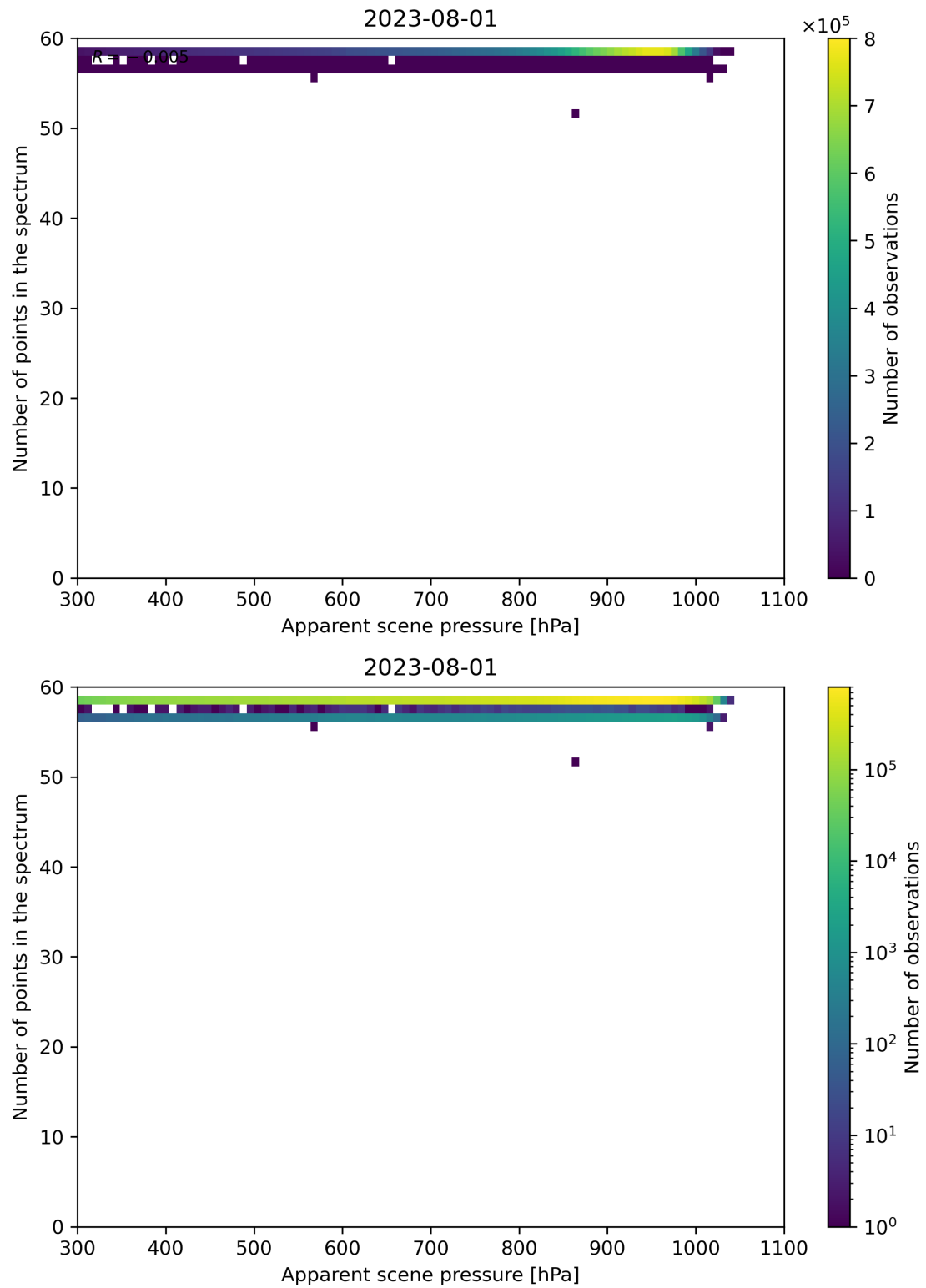
Figure 67: Scatter density plot of “Apparent scene pressure” against “Number of points in the spectrum” for 2023-07-31 to 2023-08-02.
