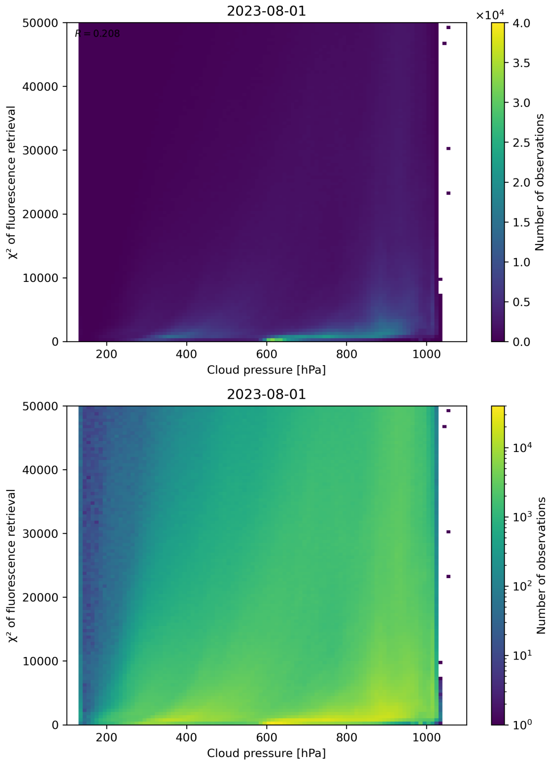
Figure 86: Scatter density plot of “Cloud pressure” against “ \chi^2 of fluorescence retrieval” for 2023-07-31 to 2023-08-02.
