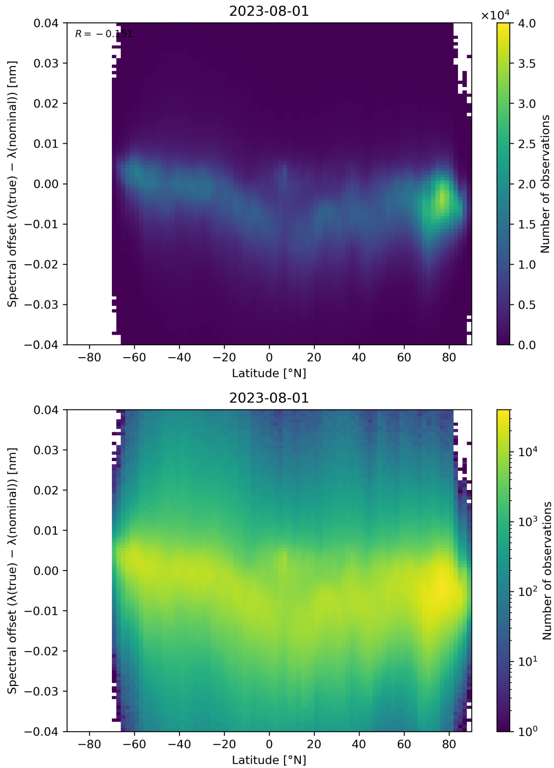
Figure 105: Scatter density plot of “Latitude” against “Spectral offset ( \lambda(\text{true}) - \lambda(\text{nominal}) )” for 2023-07-31 to 2023-08-02.
