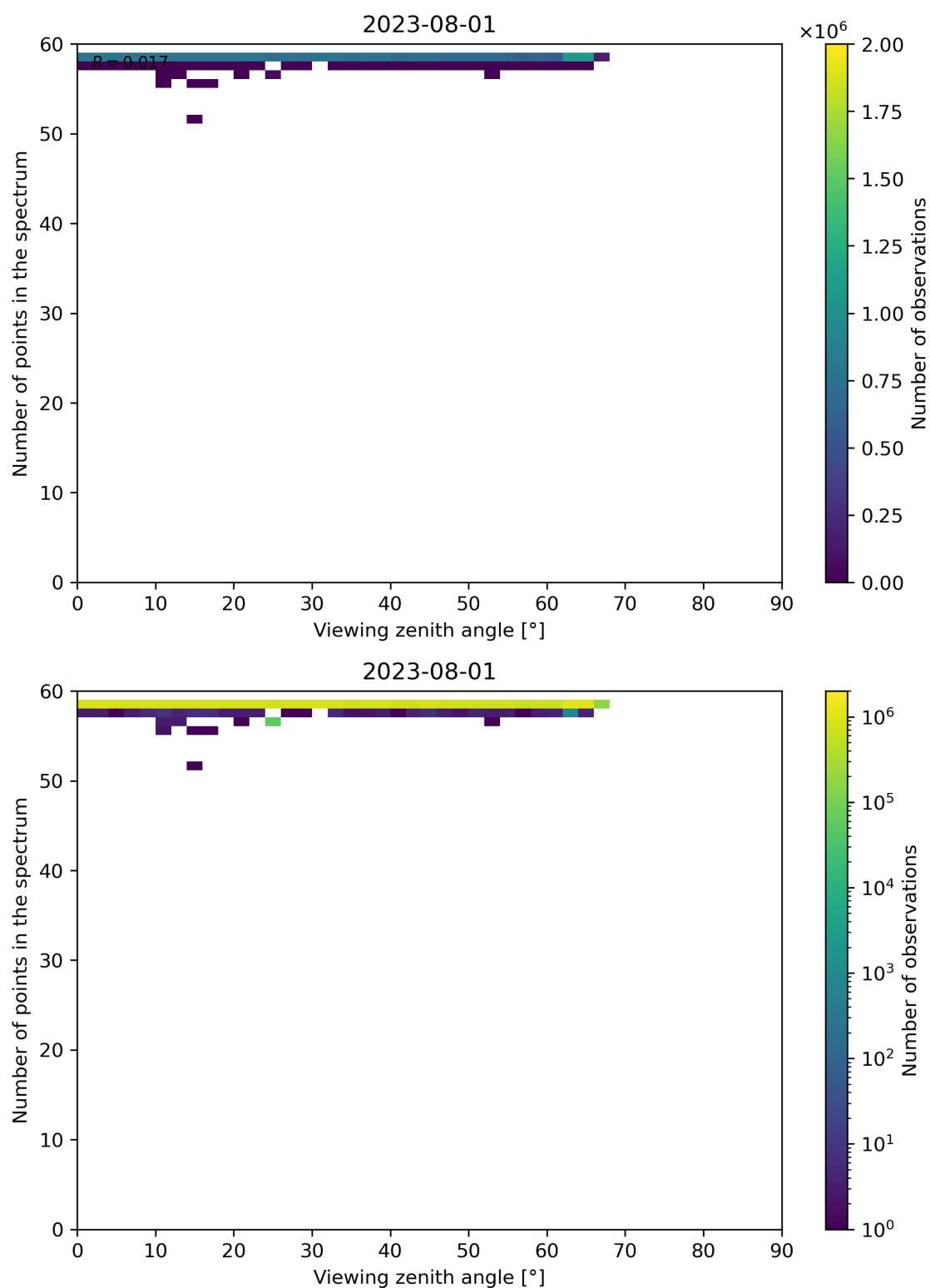
Figure 137: Scatter density plot of “Viewing zenith angle” against “Number of points in the spectrum” for 2023-07-31 to 2023-08-02.
