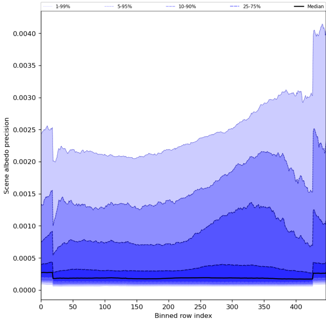
Figure 52: Along track statistics of “Scene albedo precision” for 2023-07-31 to 2023-08-02
