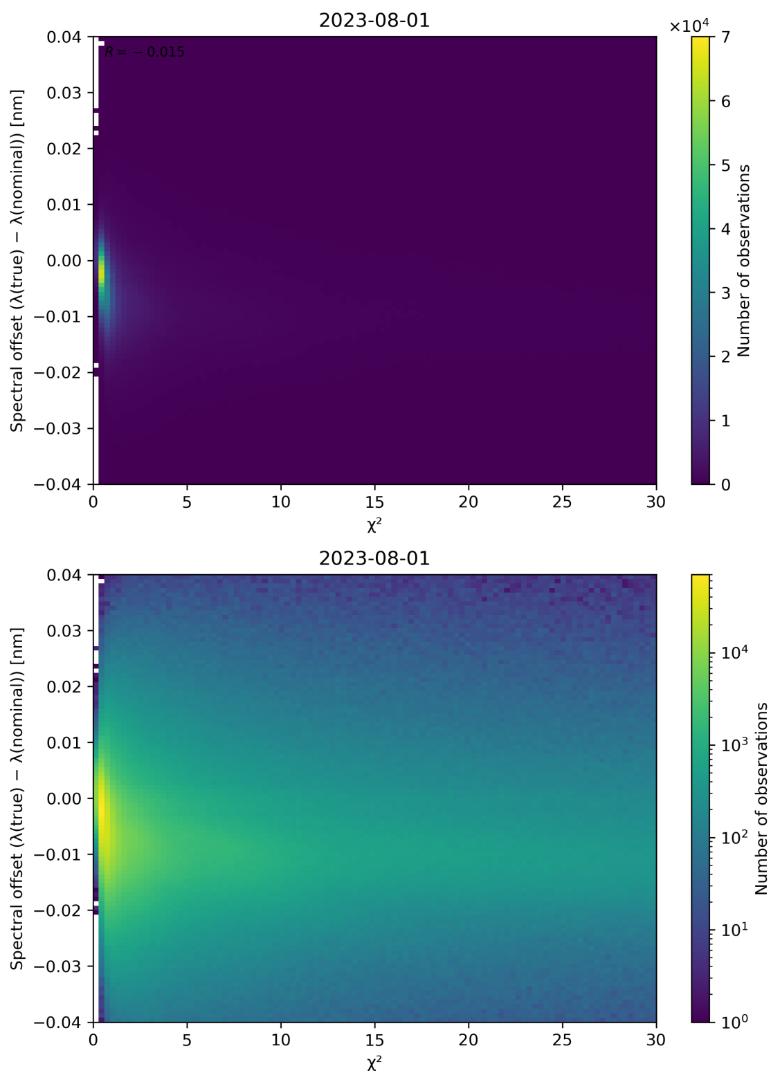
Figure 75: Scatter density plot of “ \chi^2 ” against “Spectral offset ( \lambda(\text{true}) - \lambda(\text{nominal}) )” for 2023-07-31 to 2023-08-02.
