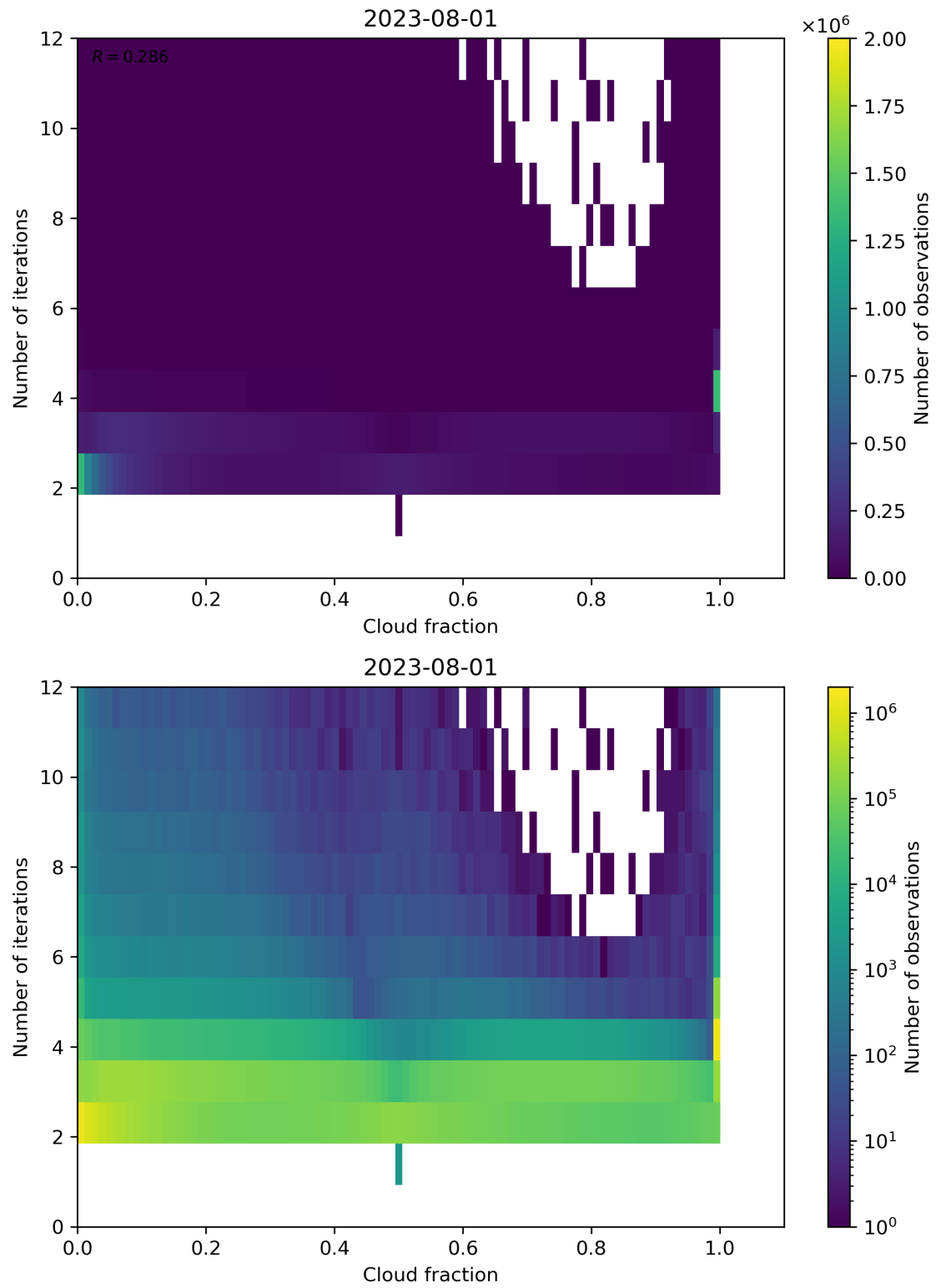
Figure 80: Scatter density plot of “Cloud fraction” against “Number of iterations” for 2023-07-31 to 2023-08-02.
