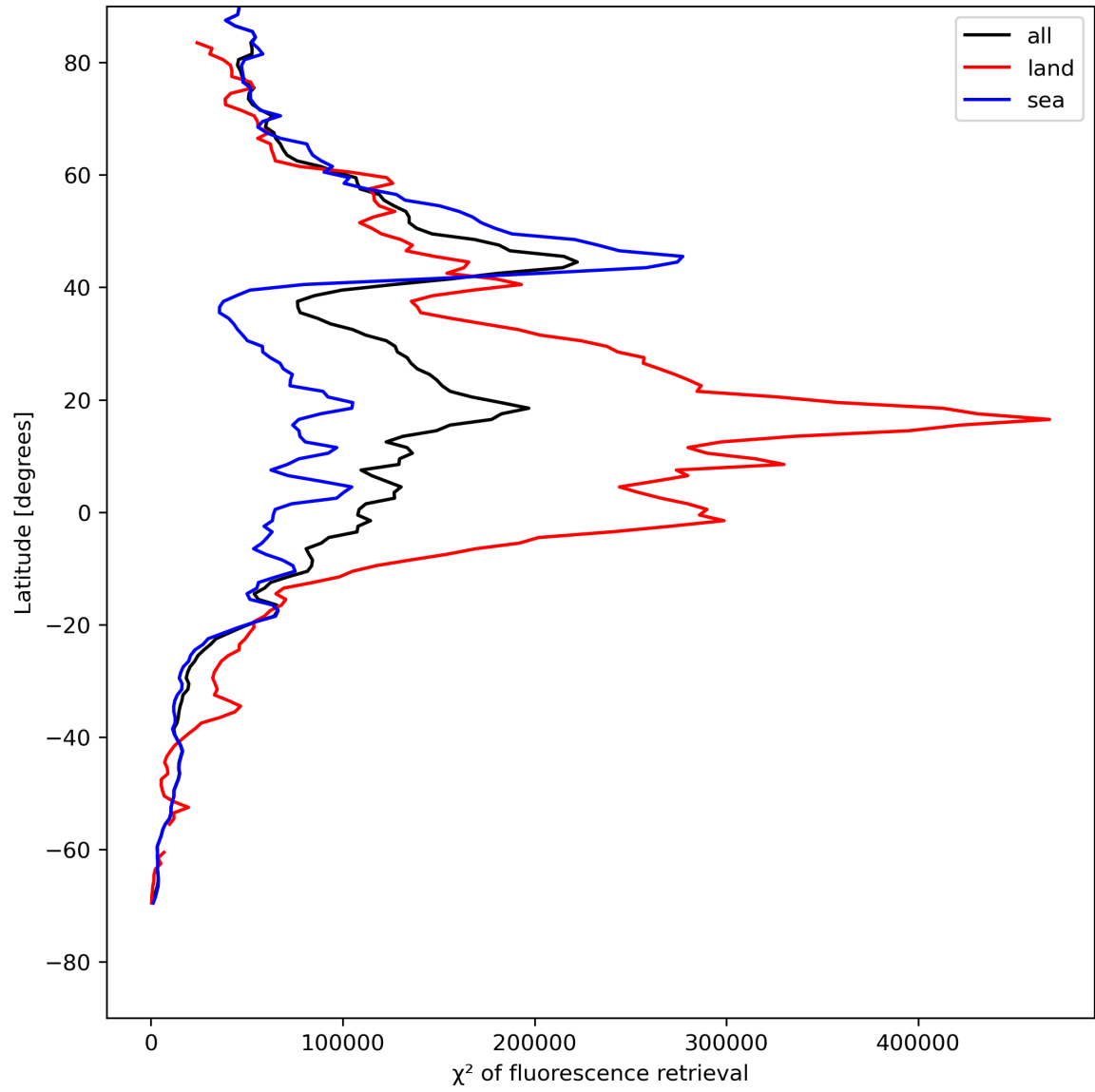
Figure 25: Zonal average of “ \chi^2 of fluorescence retrieval” for 2023-07-31 to 2023-08-02.
