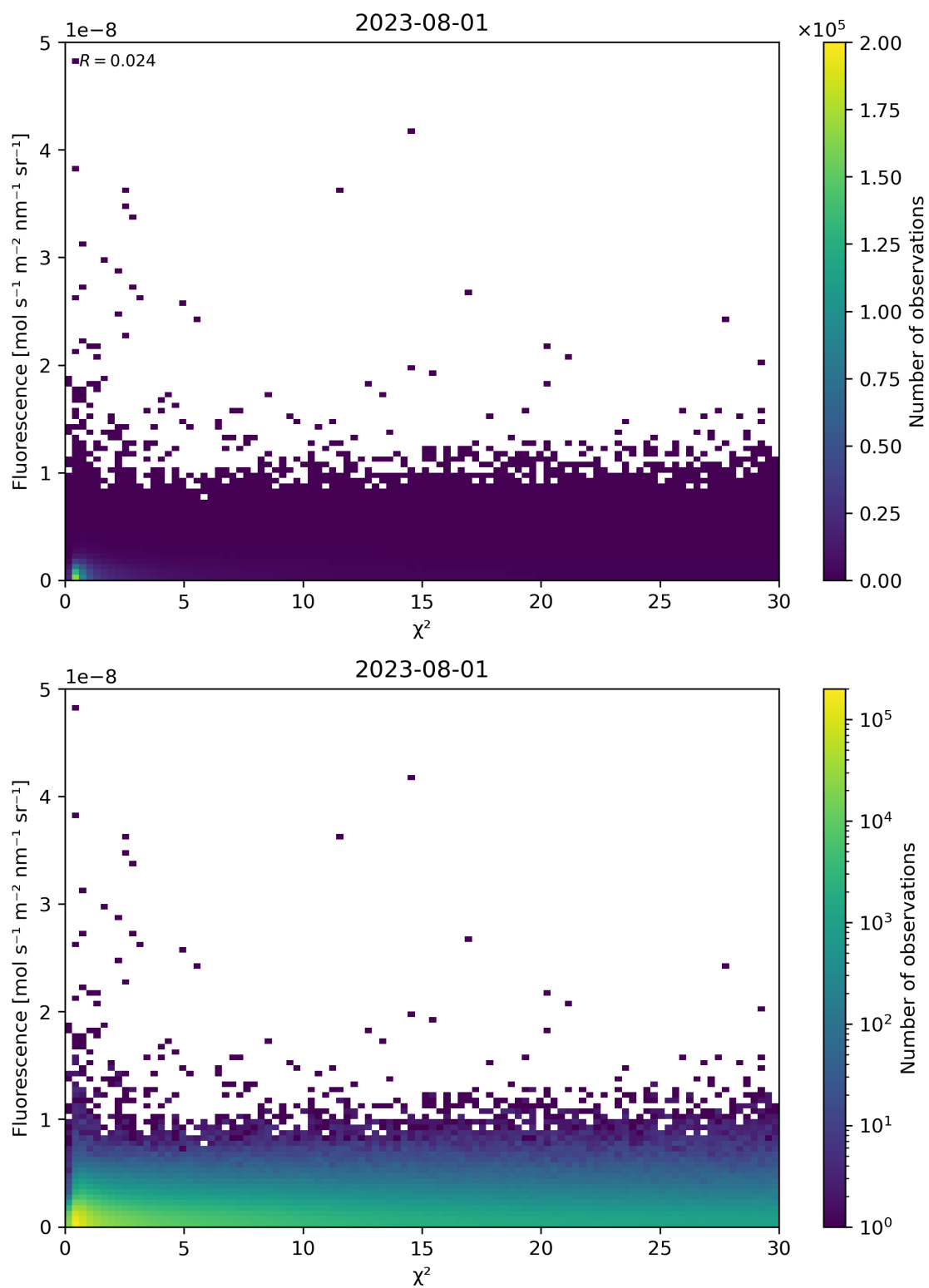
Figure 70: Scatter density plot of “ \chi^2 ” against “Fluorescence” for 2023-07-31 to 2023-08-02.
