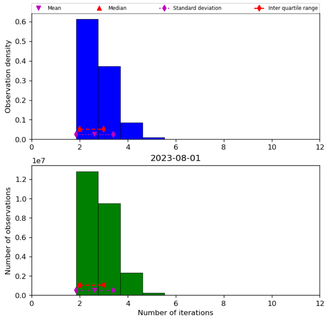
Figure 39: Histogram of “Number of iterations” for 2023-07-31 to 2023-08-02
