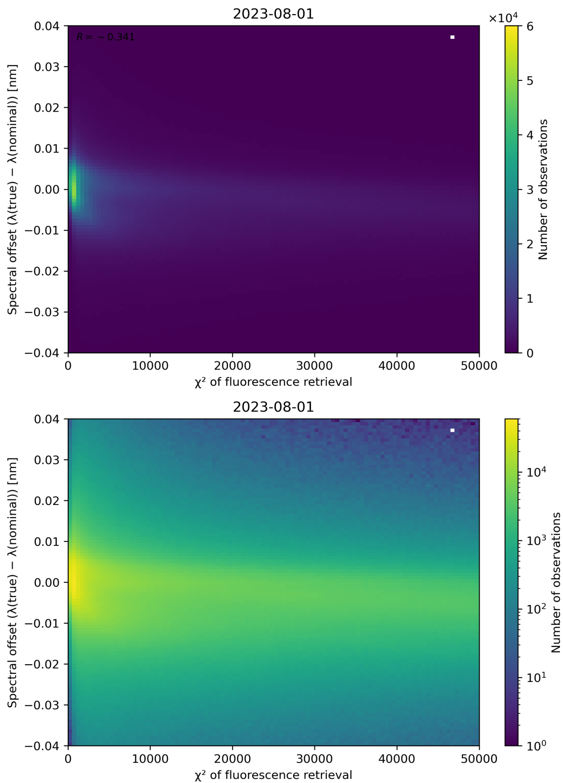
Figure 72: Scatter density plot of " \chi^2 of fluorescence retrieval" against "Spectral offset ( \lambda(\text{true}) - \lambda(\text{nominal})) " for 2023-07-31 to 2023-08-02.
