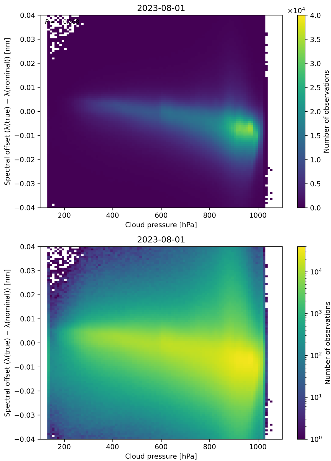
Figure 92: Scatter density plot of “Cloud pressure” against “Spectral offset ( \lambda(\text{true}) - \lambda(\text{nominal}) )” for 2023-07-31 to 2023-08-02.
