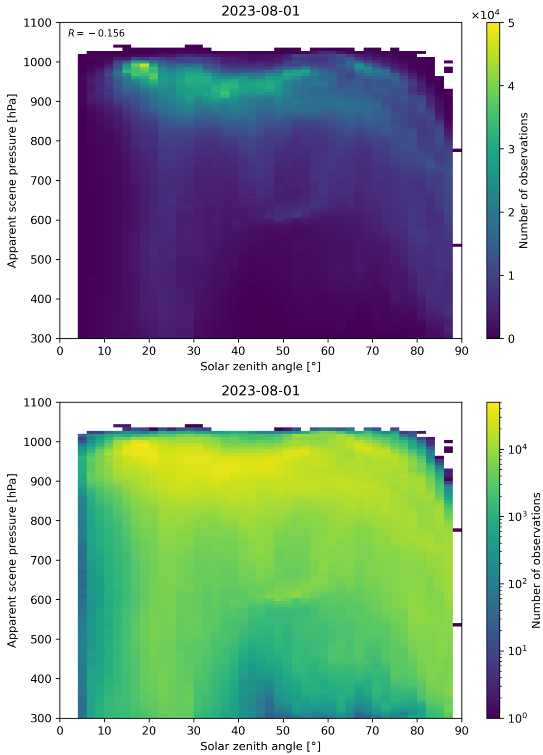
Figure 118: Scatter density plot of “Solar zenith angle” against “Apparent scene pressure” for 2023-07-31 to 2023-08-02.
