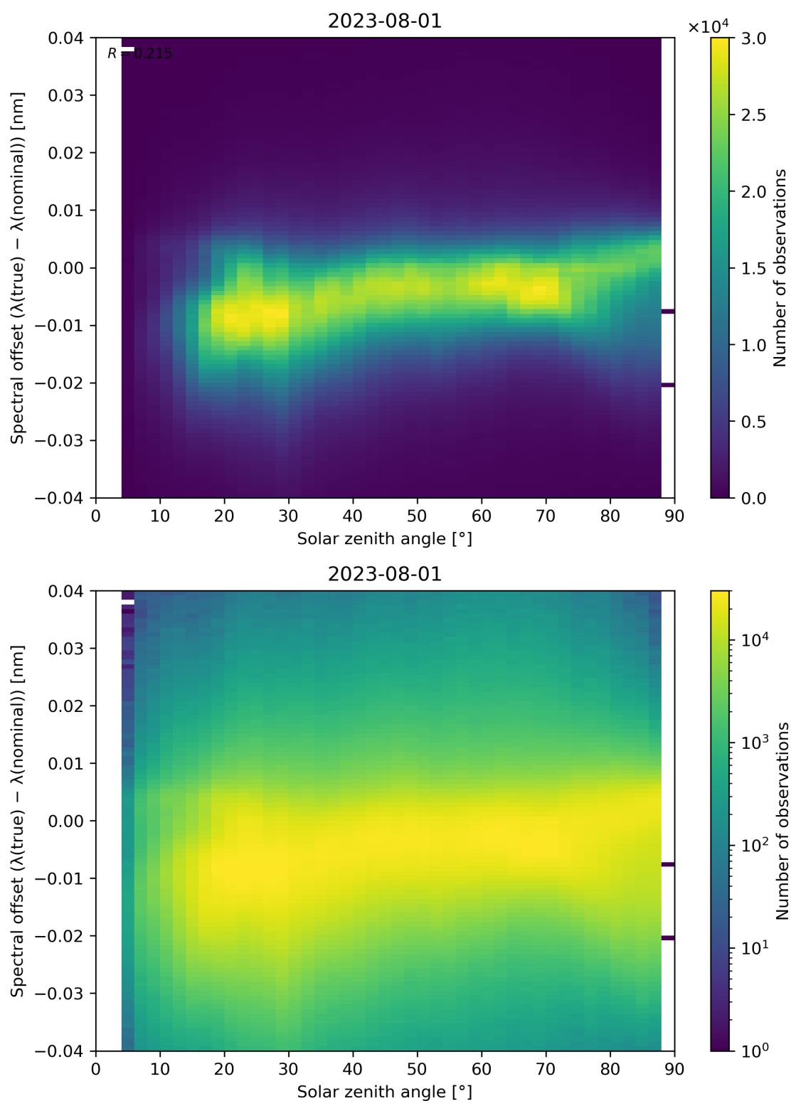
Figure 128: Scatter density plot of “Solar zenith angle” against “Spectral offset ( \lambda(\text{true}) - \lambda(\text{nominal}) )” for 2023-07-31 to 2023-08-02.
