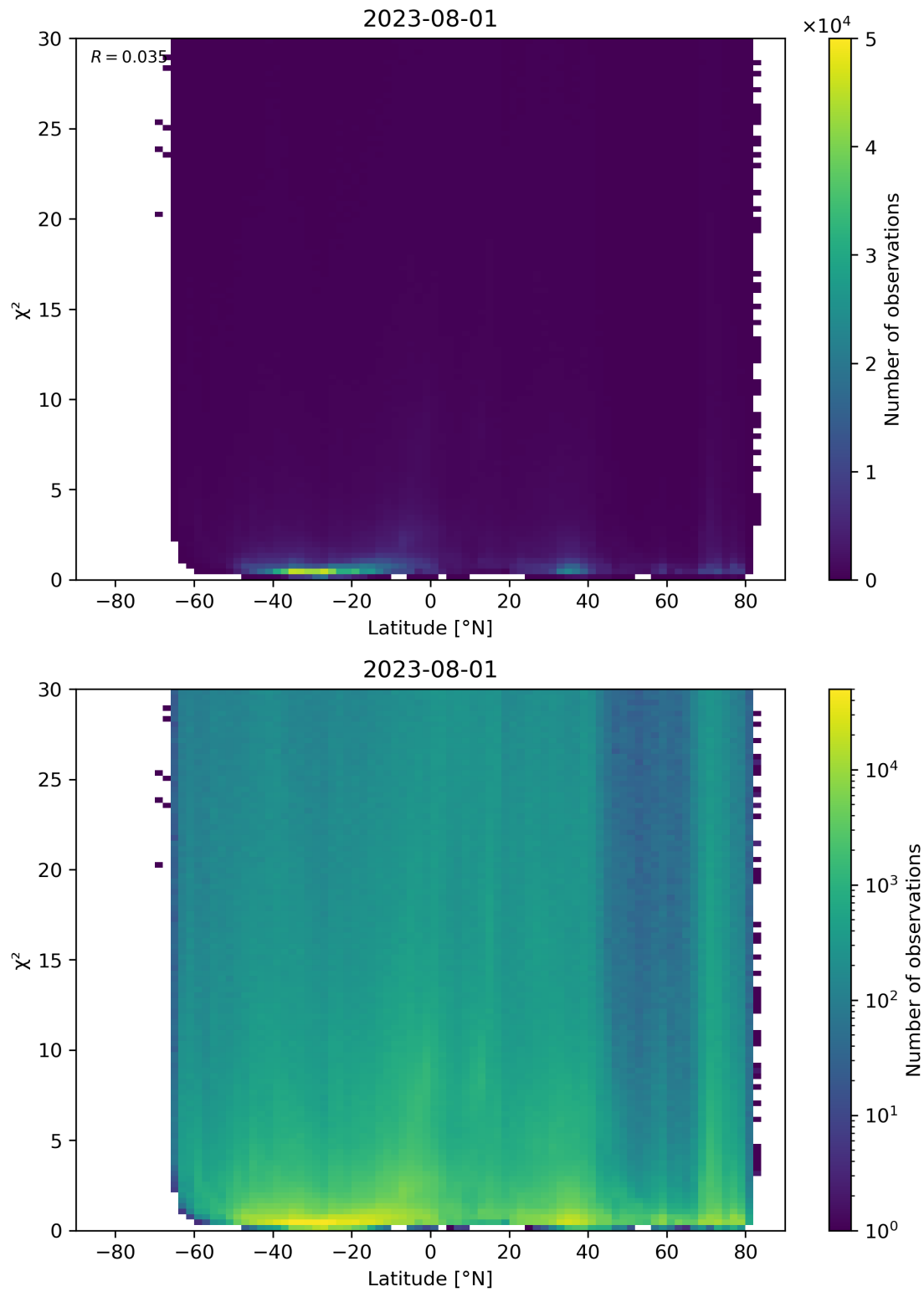
Figure 97: Scatter density plot of “Latitude” against “ \chi^2 ” for 2023-07-31 to 2023-08-02.
