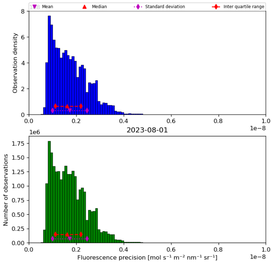
Figure 41: Histogram of “Fluorescence precision” for 2023-07-31 to 2023-08-02
