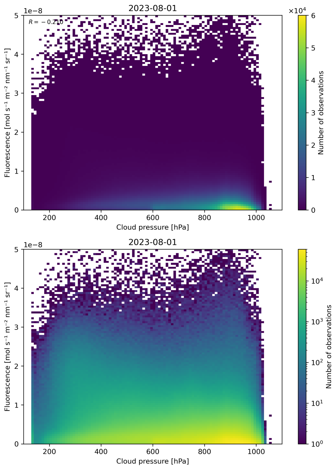
Figure 88: Scatter density plot of “Cloud pressure” against “Fluorescence” for 2023-07-31 to 2023-08-02.
