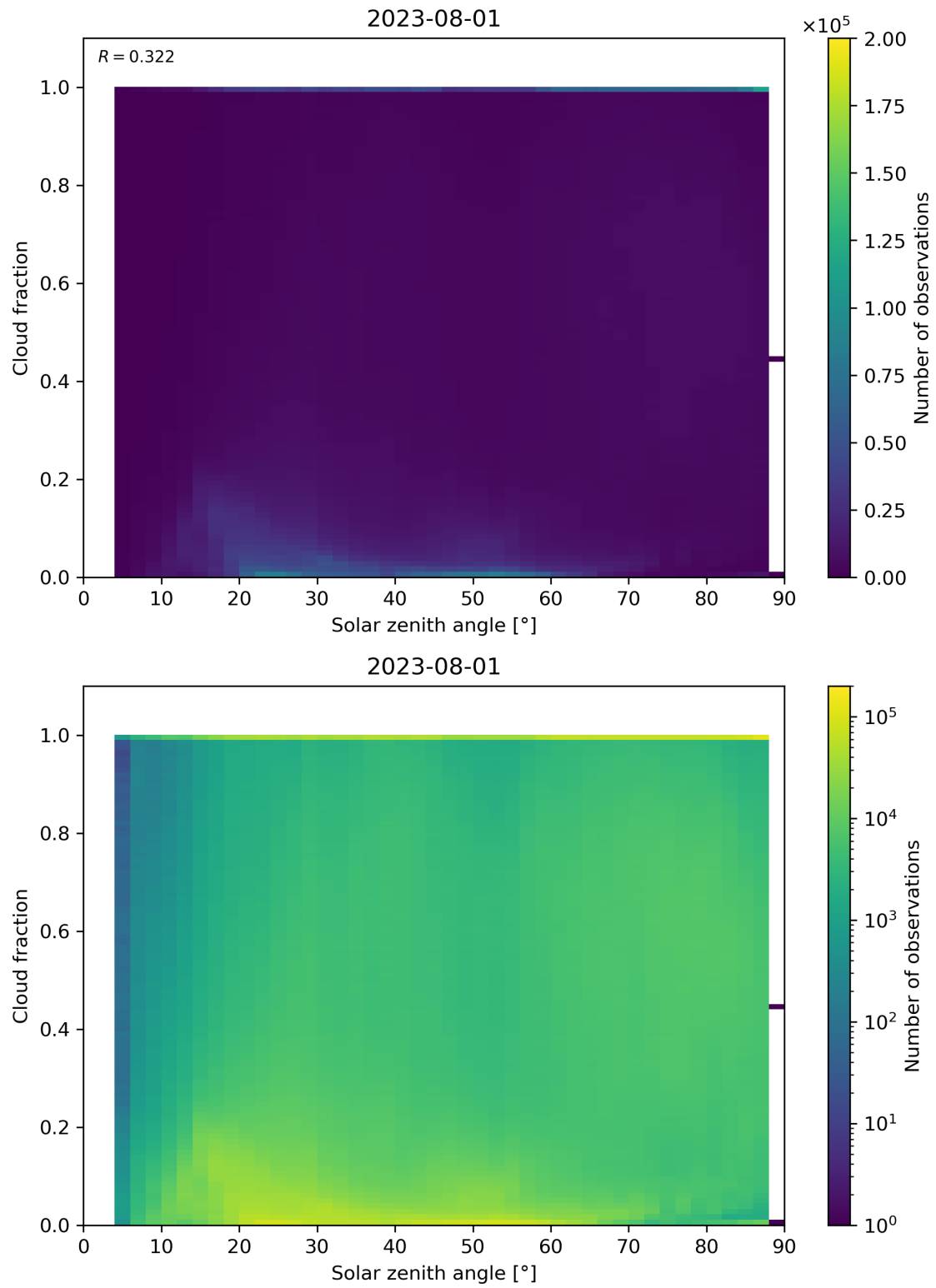
Figure 121: Scatter density plot of “Solar zenith angle” against “Cloud fraction” for 2023-07-31 to 2023-08-02.
