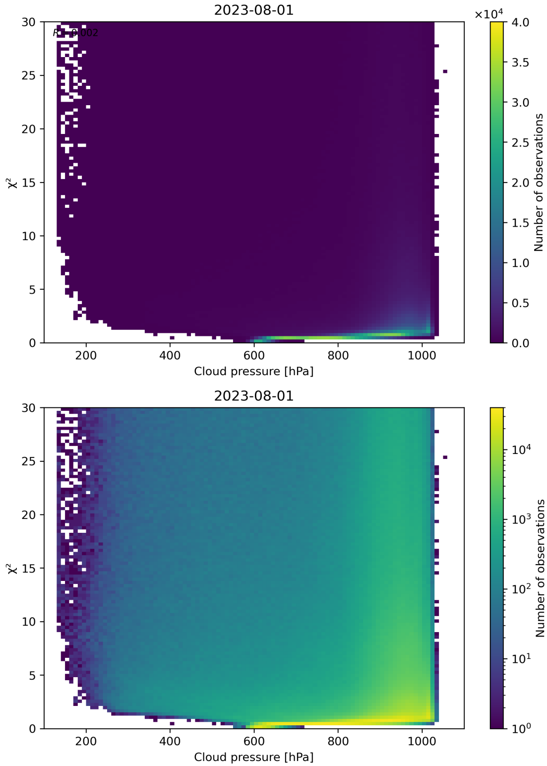
Figure 85: Scatter density plot of “Cloud pressure” against “ \chi^2 ” for 2023-07-31 to 2023-08-02.
