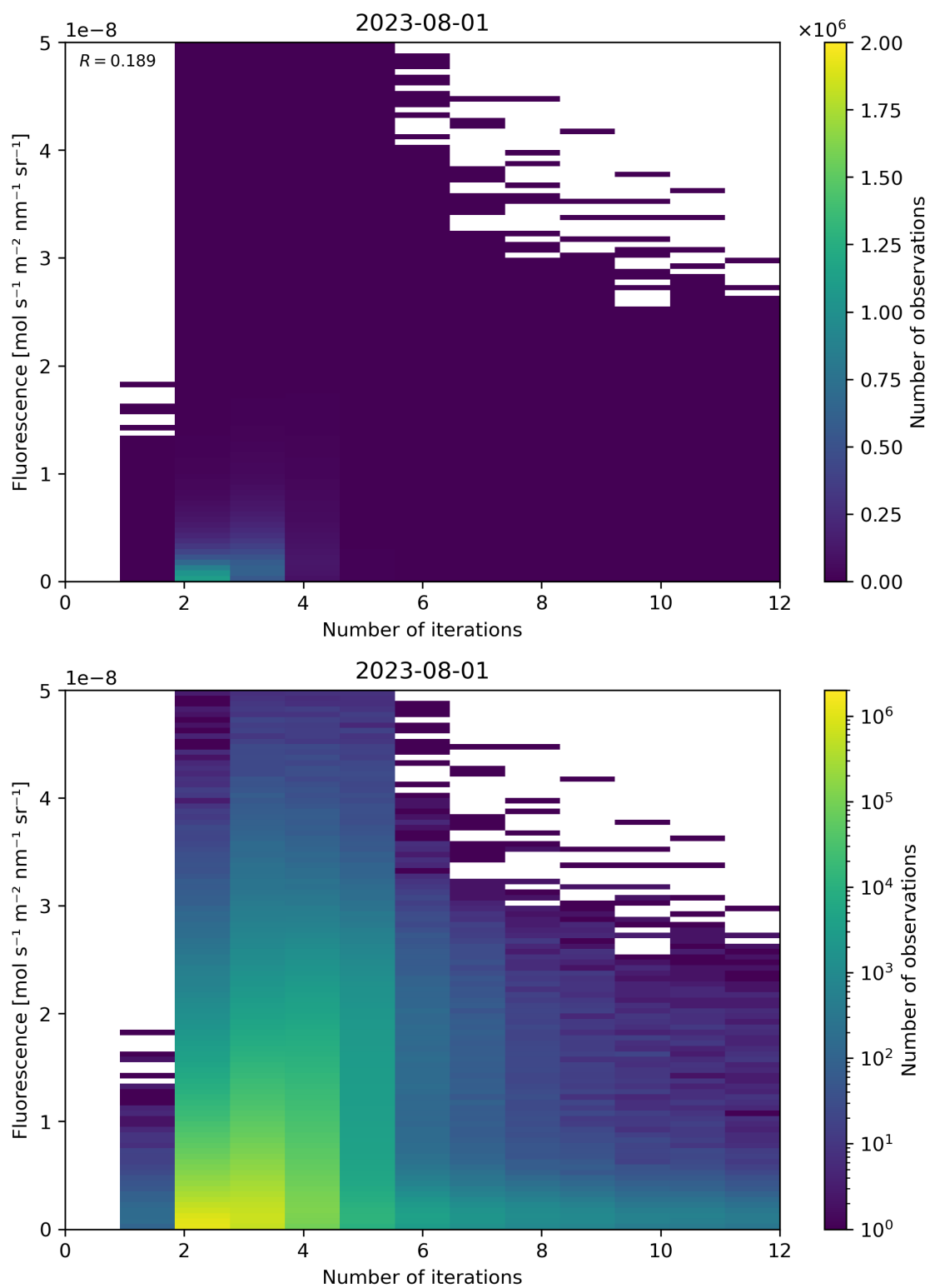
Figure 107: Scatter density plot of “Number of iterations” against “Fluorescence” for 2023-07-31 to 2023-08-02.
