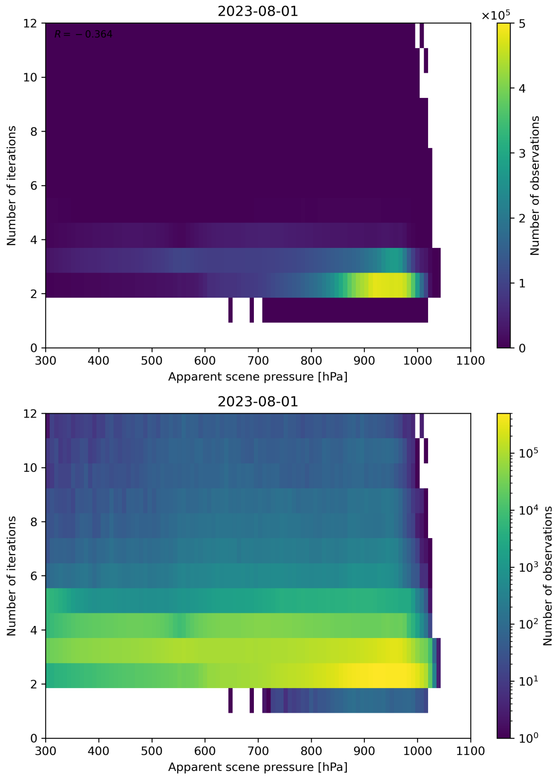
Figure 66: Scatter density plot of “Apparent scene pressure” against “Number of iterations” for 2023-07-31 to 2023-08-02.
