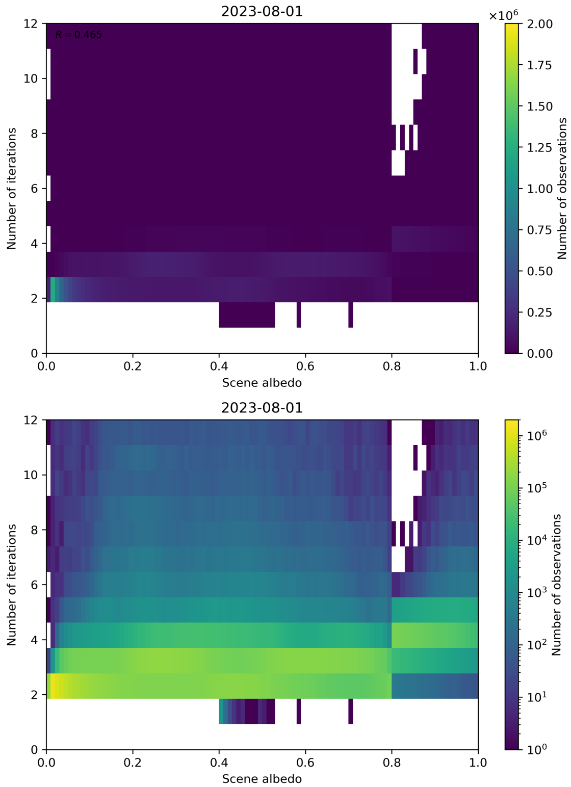
Figure 115: Scatter density plot of “Scene albedo” against “Number of iterations” for 2023-07-31 to 2023-08-02.
