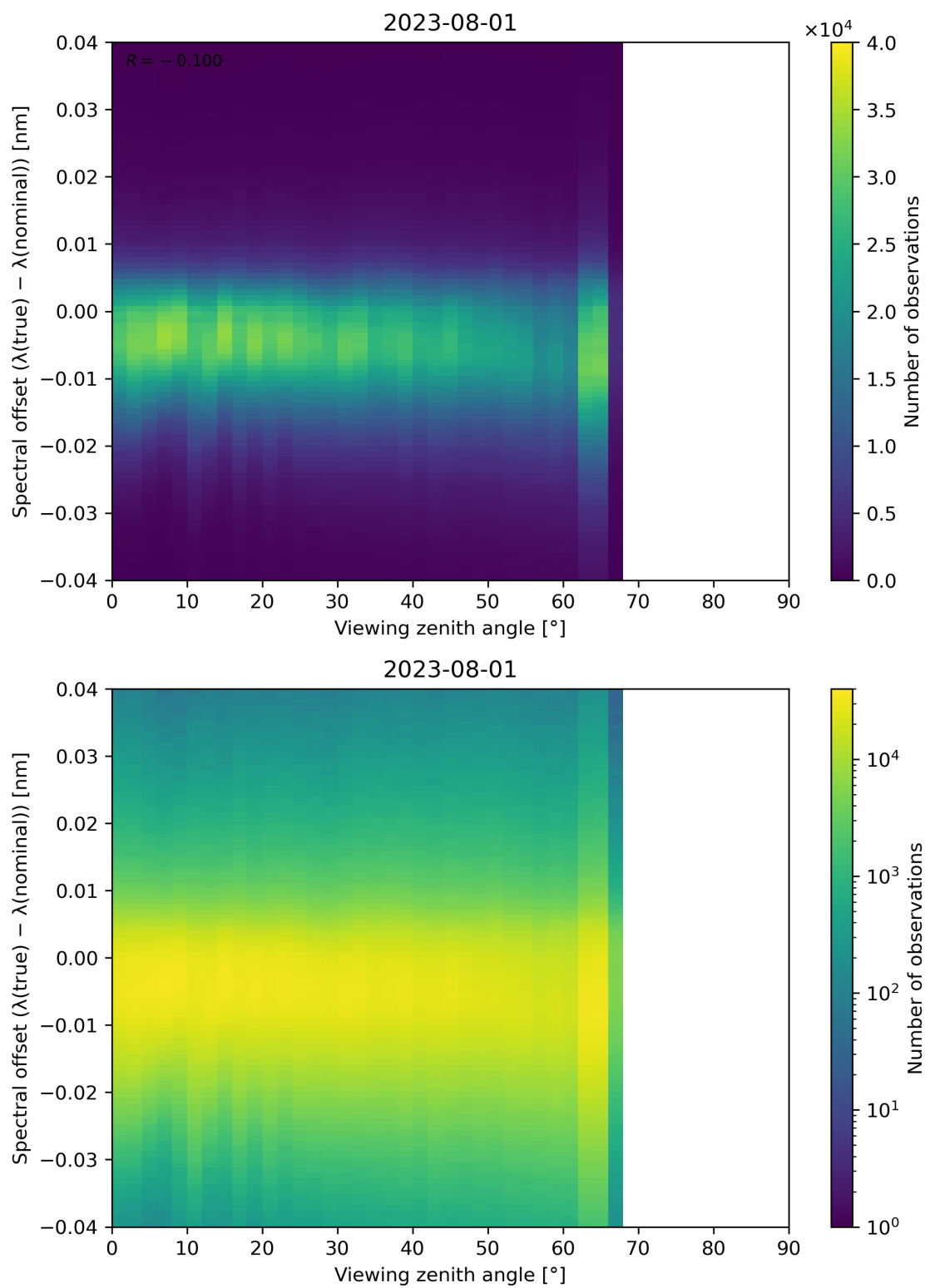
Figure 140: Scatter density plot of “Viewing zenith angle” against “Spectral offset ( \lambda(\text{true}) - \lambda(\text{nominal}) )” for 2023-07-31 to 2023-08-02.
