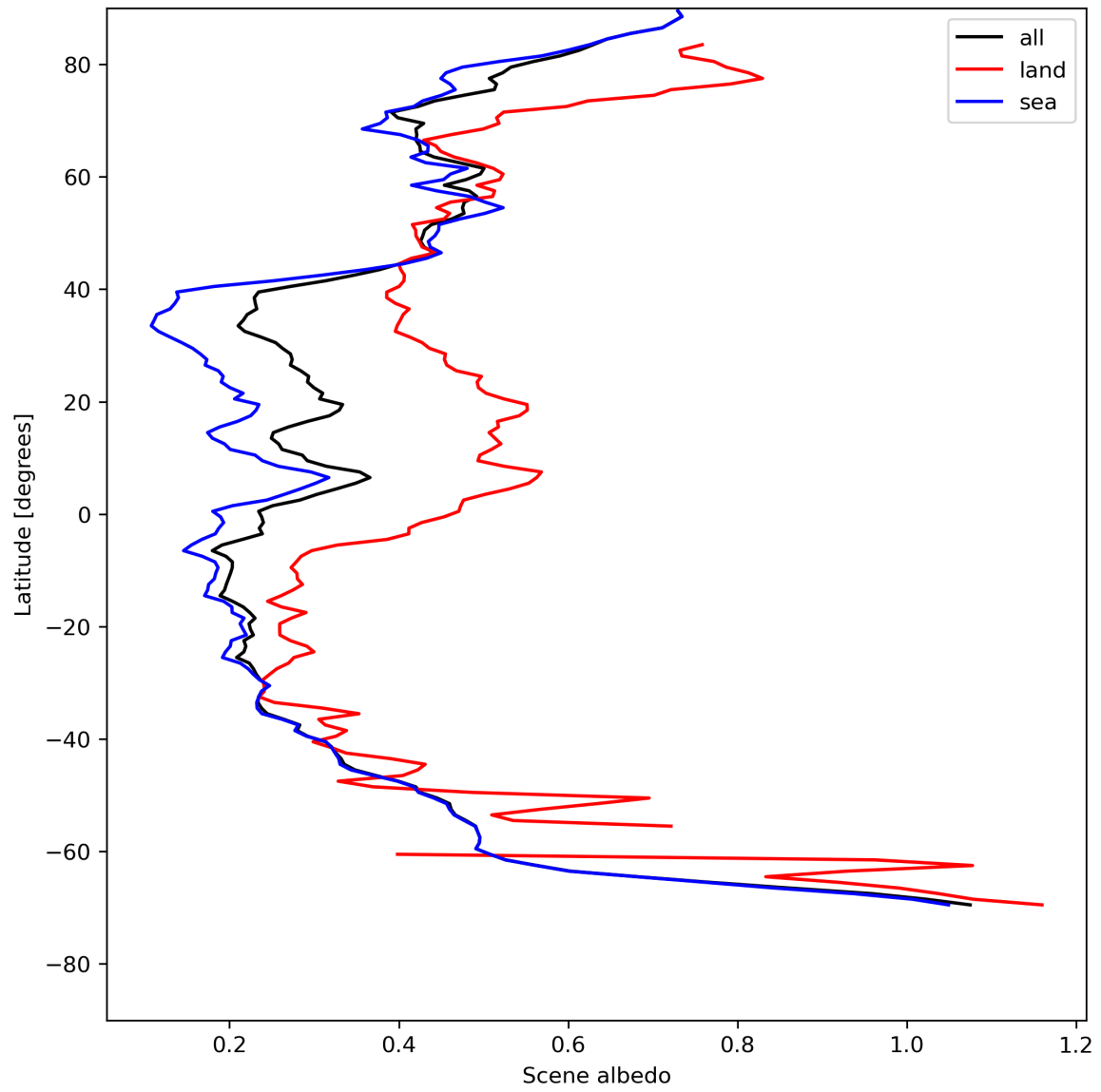
Figure 17: Zonal average of “Scene albedo” for 2023-07-31 to 2023-08-02.
