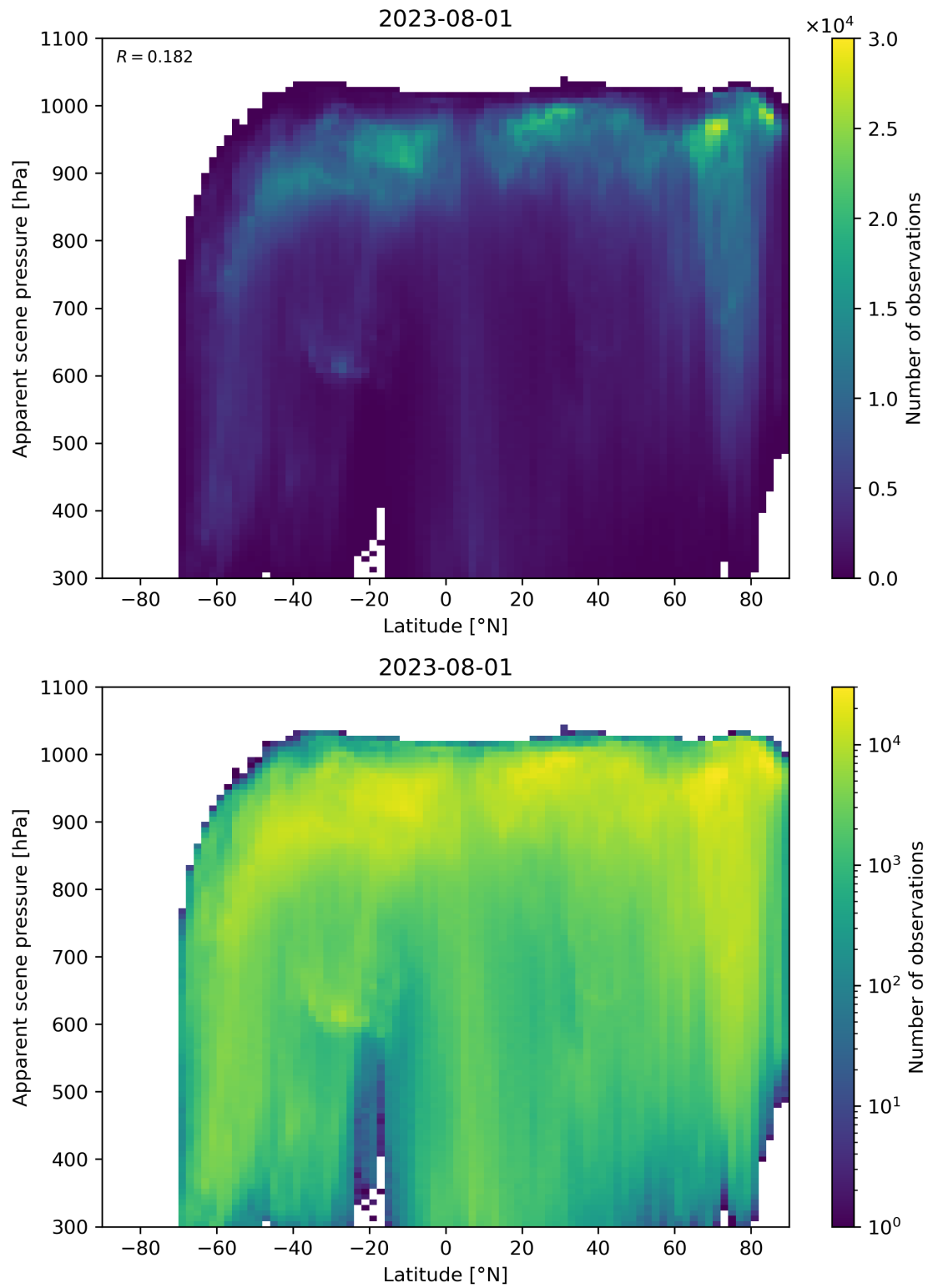
Figure 96: Scatter density plot of “Latitude” against “Apparent scene pressure” for 2023-07-31 to 2023-08-02.
