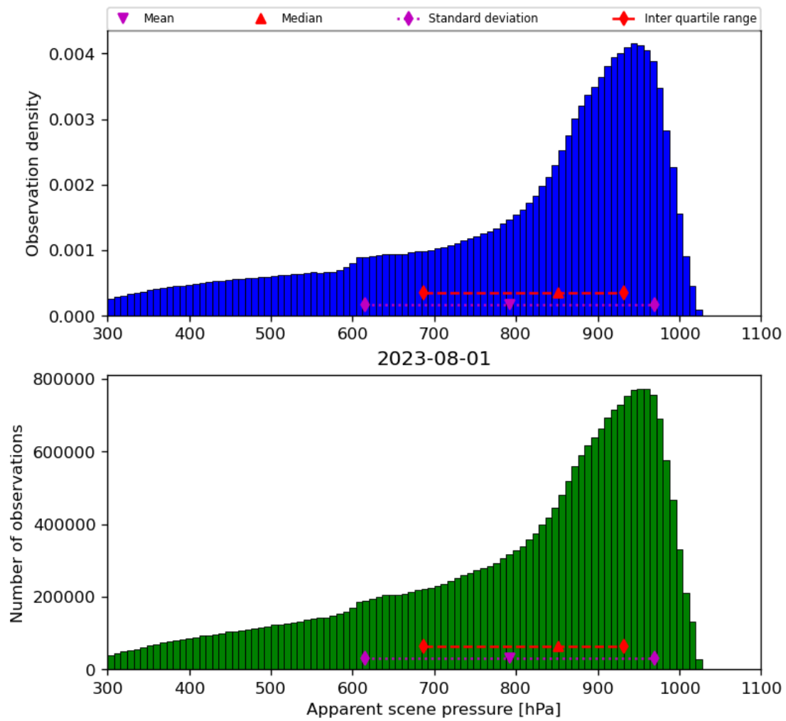
Figure 36: Histogram of “Apparent scene pressure” for 2023-07-31 to 2023-08-02
