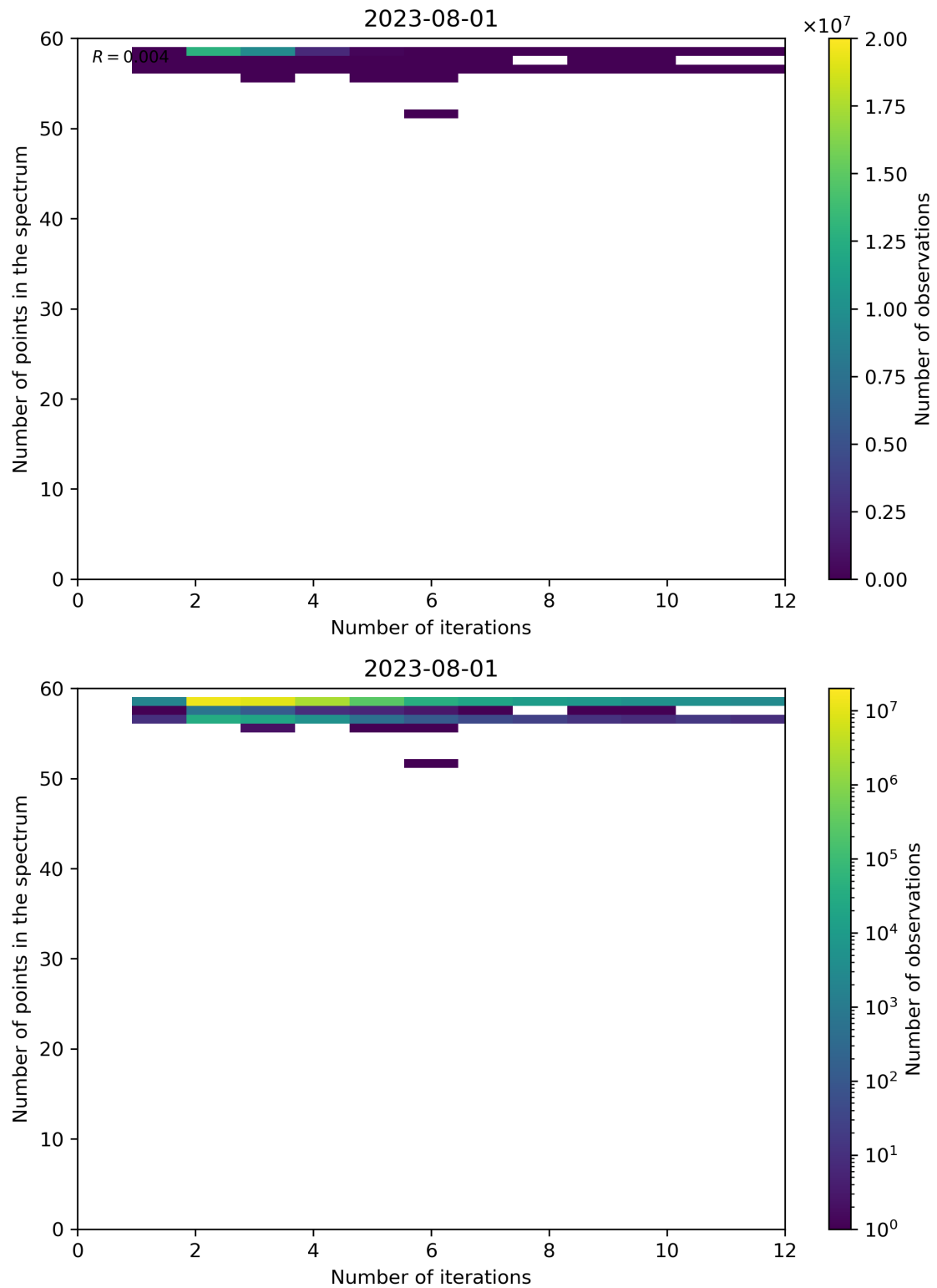
Figure 108: Scatter density plot of “Number of iterations” against “Number of points in the spectrum” for 2023-07-31 to 2023-08-02.
