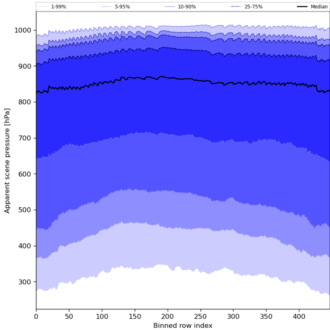
Figure 53: Along track statistics of “Apparent scene pressure” for 2023-07-31 to 2023-08-02
