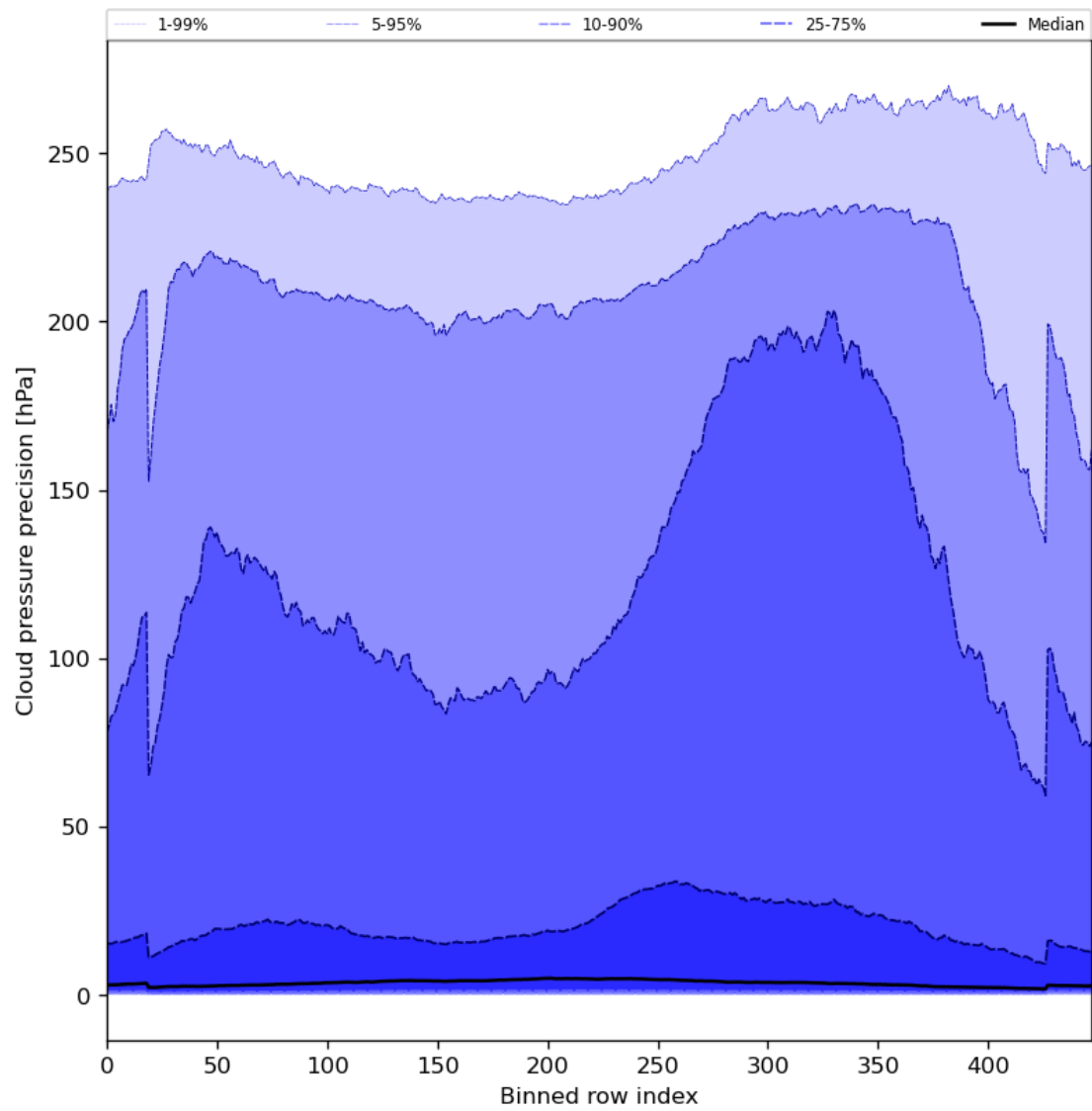
Figure 48: Along track statistics of “Cloud pressure precision” for 2023-07-31 to 2023-08-02
