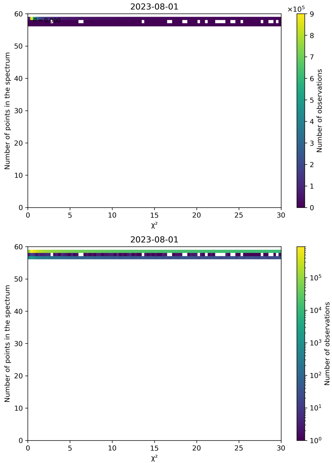
Figure 74: Scatter density plot of “ \chi^2 ” against “Number of points in the spectrum” for 2023-07-31 to 2023-08-02.
