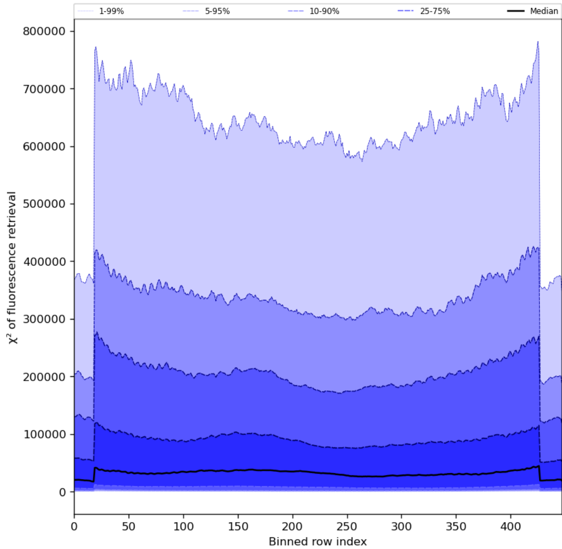
Figure 59: Along track statistics of “ \chi^2 of fluorescence retrieval” for 2023-07-31 to 2023-08-02
