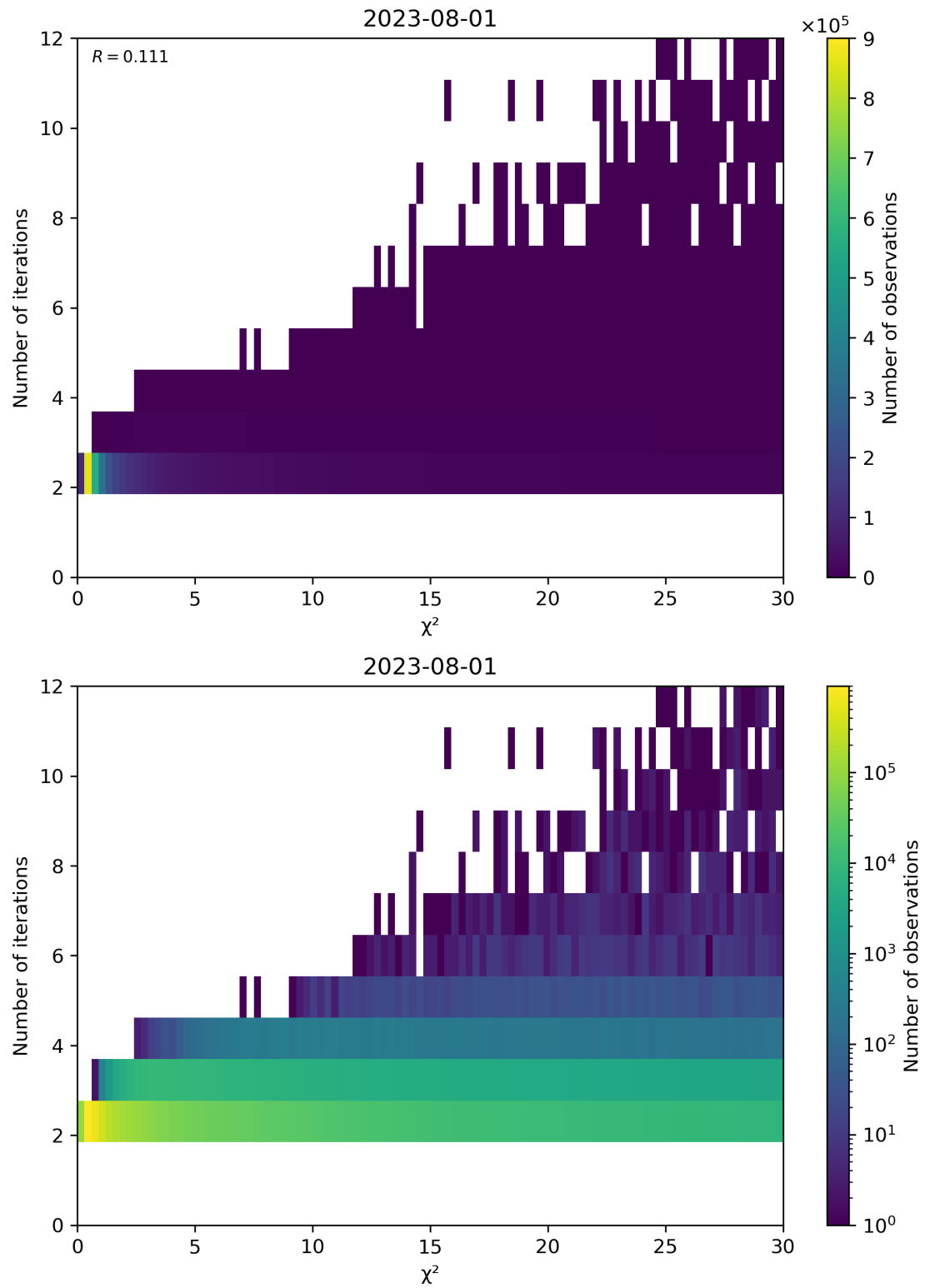
Figure 73: Scatter density plot of “ \chi^2 ” against “Number of iterations” for 2023-07-31 to 2023-08-02.
