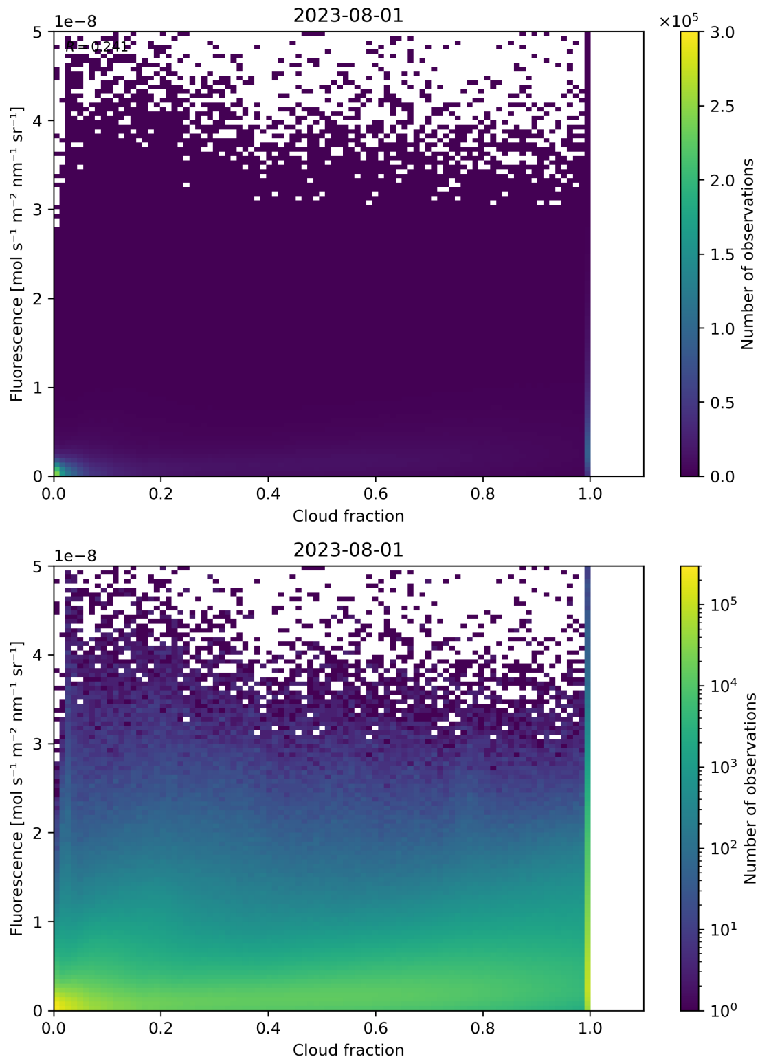
Figure 79: Scatter density plot of “Cloud fraction” against “Fluorescence” for 2023-07-31 to 2023-08-02.
