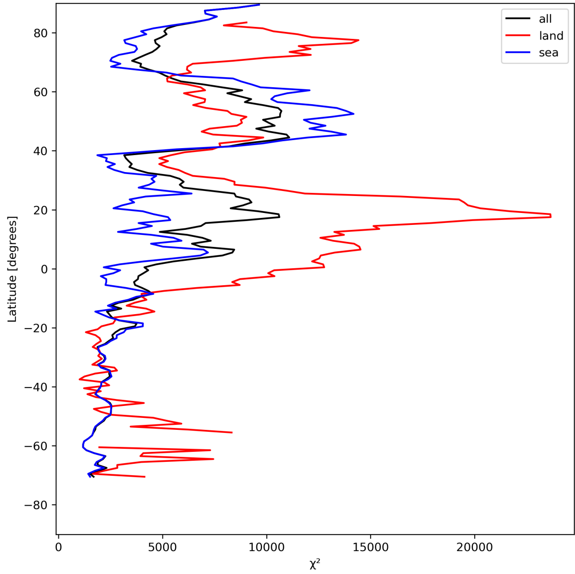
Figure 21: Zonal average of “ \chi^2 ” for 2023-08-01 to 2023-08-03.
