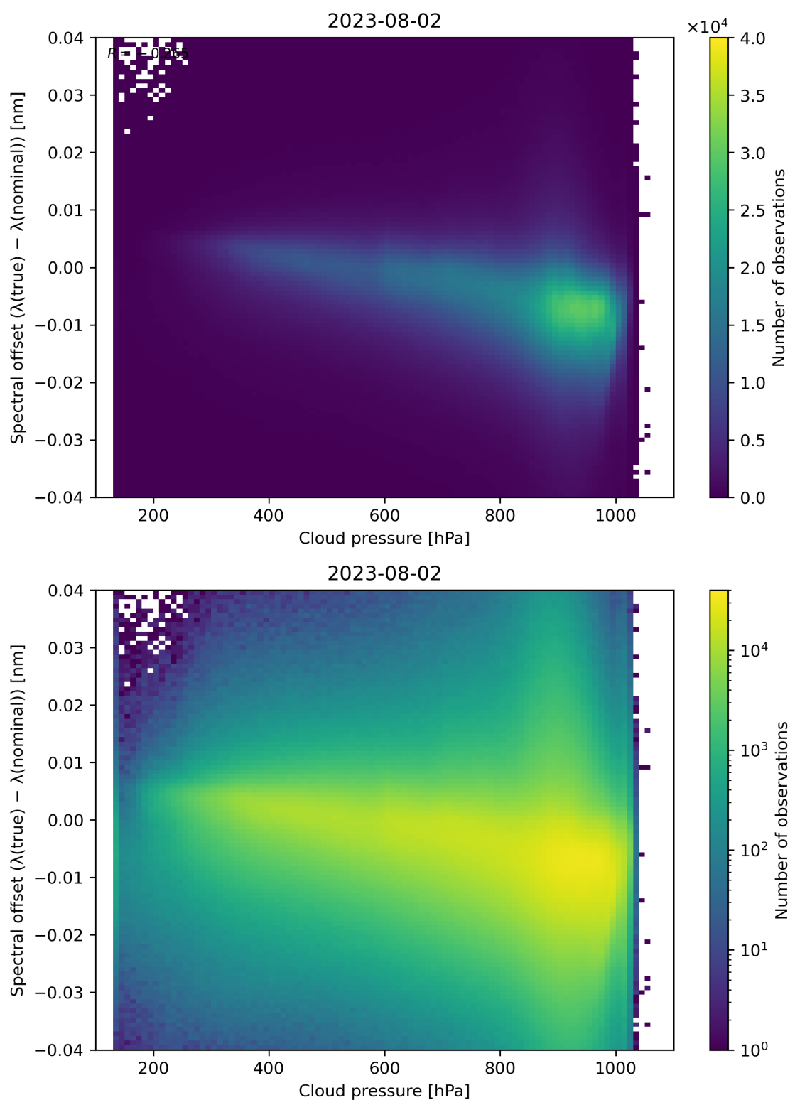
Figure 92: Scatter density plot of “Cloud pressure” against “Spectral offset ( \lambda(\text{true}) - \lambda(\text{nominal}) )” for 2023-08-01 to 2023-08-03.
