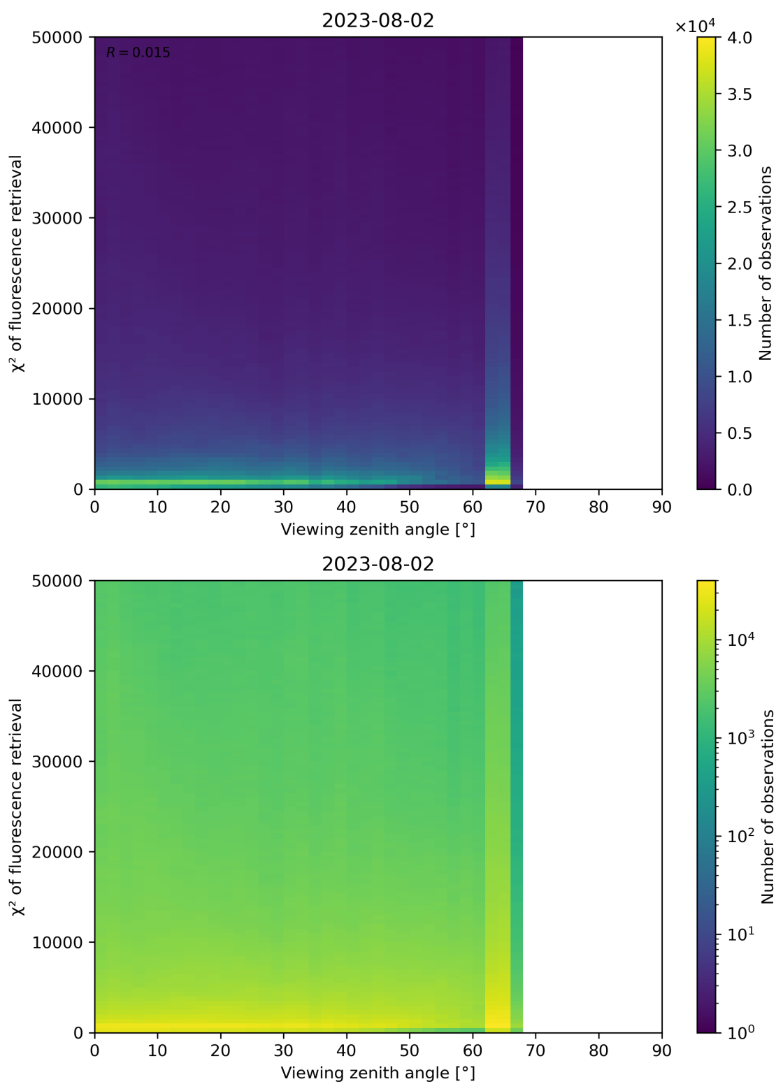
Figure 131: Scatter density plot of “Viewing zenith angle” against “ \chi^2 of fluorescence retrieval” for 2023-08-01 to 2023-08-03.
