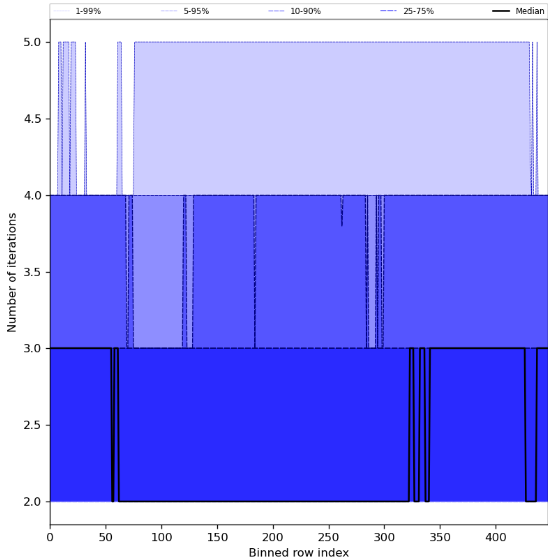
Figure 56: Along track statistics of “Number of iterations” for 2023-08-01 to 2023-08-03
