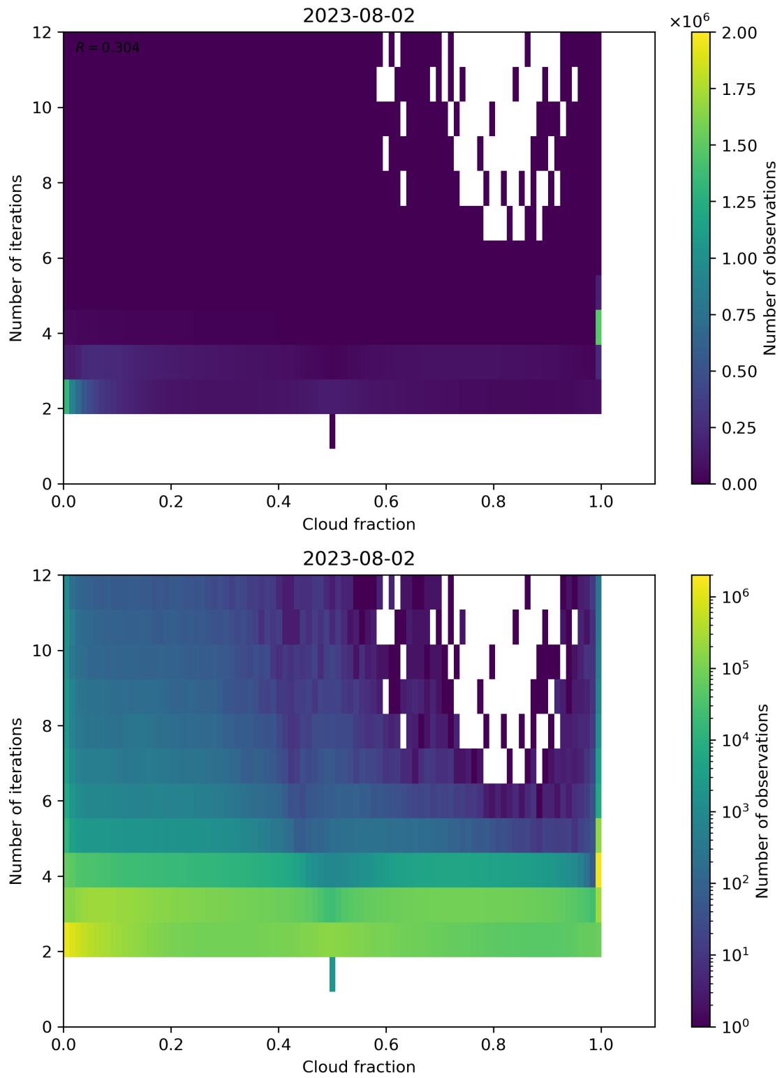
Figure 80: Scatter density plot of “Cloud fraction” against “Number of iterations” for 2023-08-01 to 2023-08-03.
