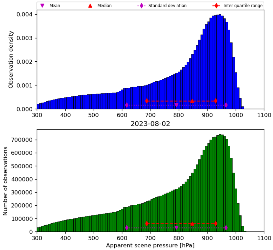
Figure 36: Histogram of “Apparent scene pressure” for 2023-08-01 to 2023-08-03
