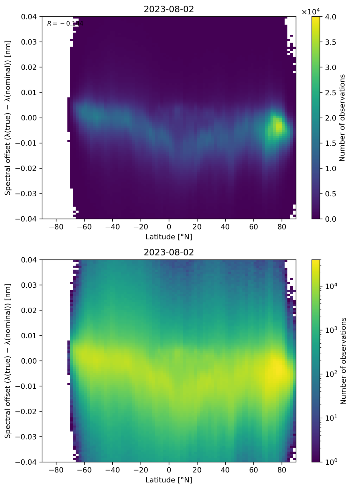
Figure 105: Scatter density plot of “Latitude” against “Spectral offset ( \lambda(\text{true}) - \lambda(\text{nominal}) )” for 2023-08-01 to 2023-08-03.
