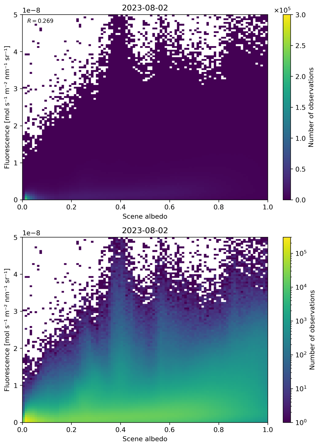
Figure 114: Scatter density plot of “Scene albedo” against “Fluorescence” for 2023-08-01 to 2023-08-03.
