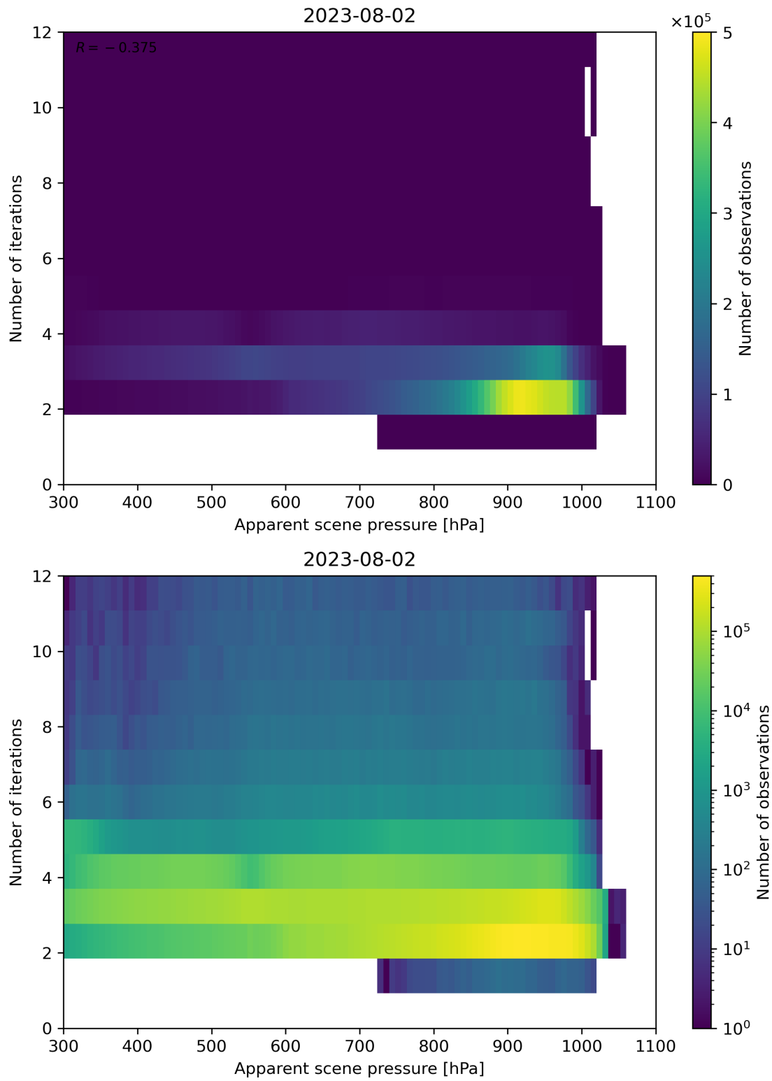
Figure 66: Scatter density plot of “Apparent scene pressure” against “Number of iterations” for 2023-08-01 to 2023-08-03.
