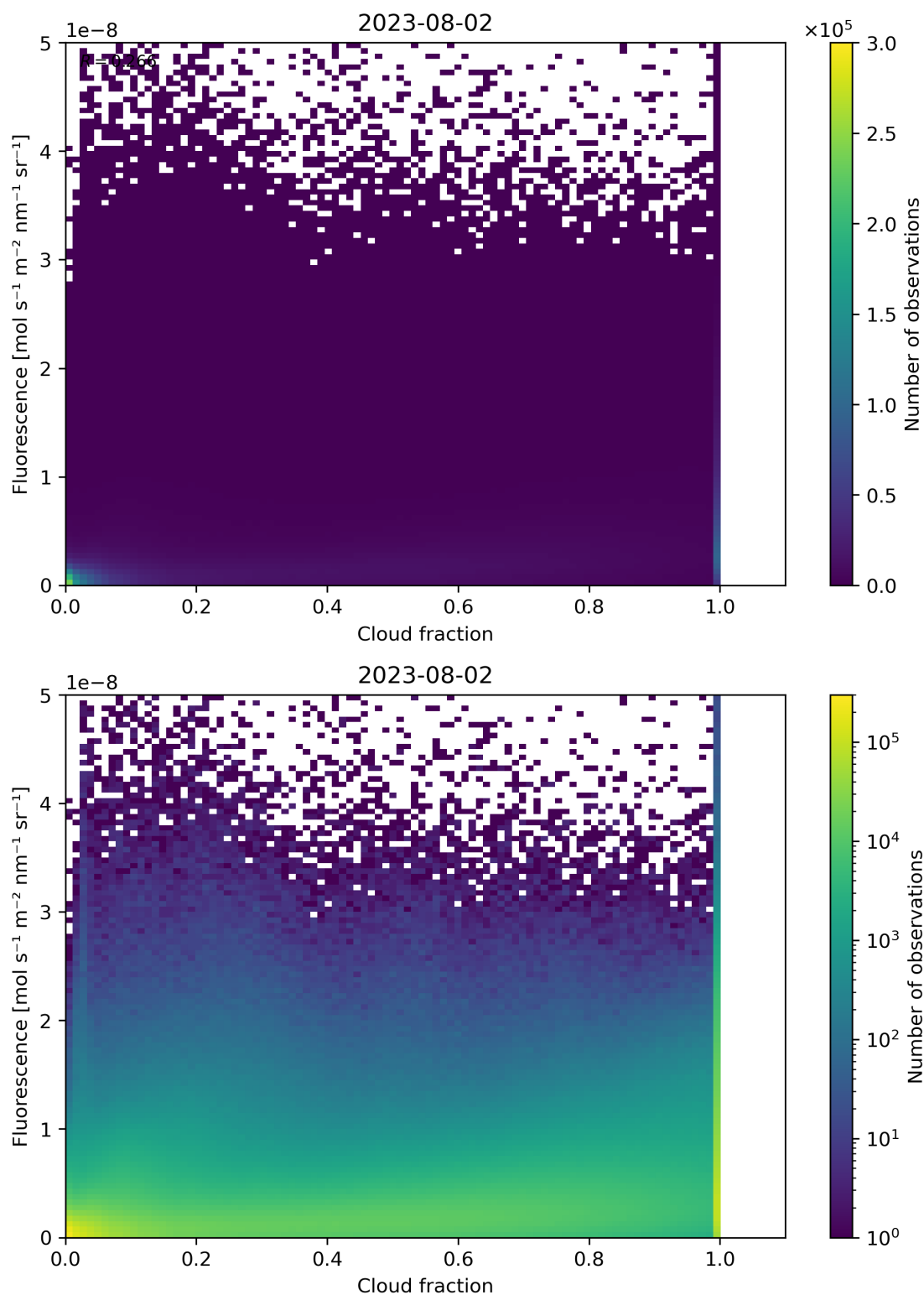
Figure 79: Scatter density plot of “Cloud fraction” against “Fluorescence” for 2023-08-01 to 2023-08-03.
