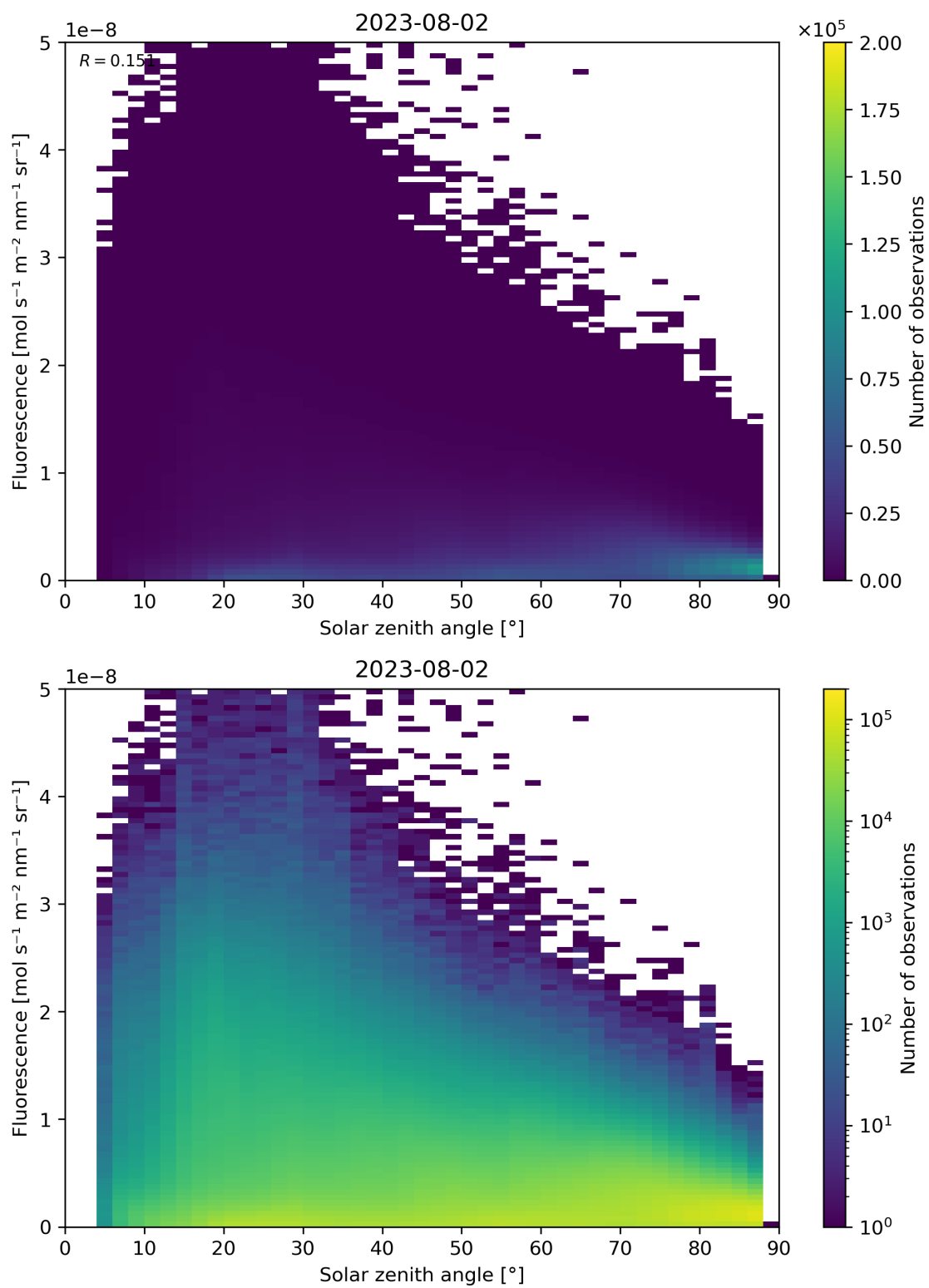
Figure 123: Scatter density plot of “Solar zenith angle” against “Fluorescence” for 2023-08-01 to 2023-08-03.
