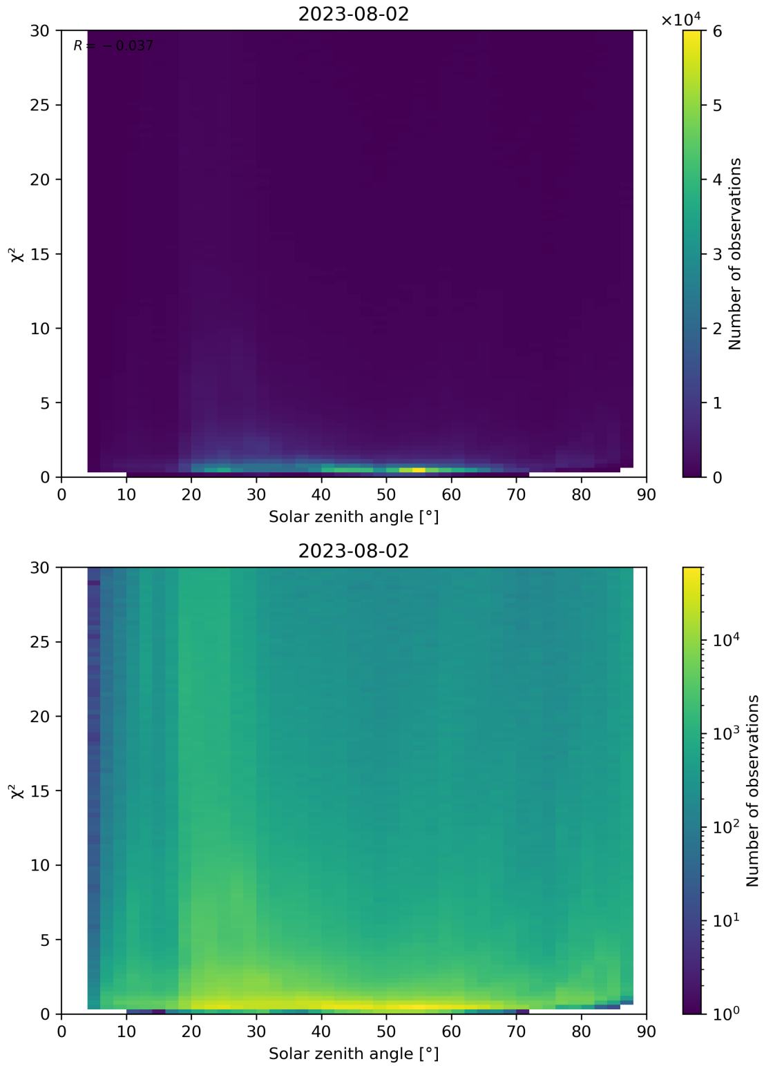
Figure 119: Scatter density plot of “Solar zenith angle” against “ \chi^2 ” for 2023-08-01 to 2023-08-03.
