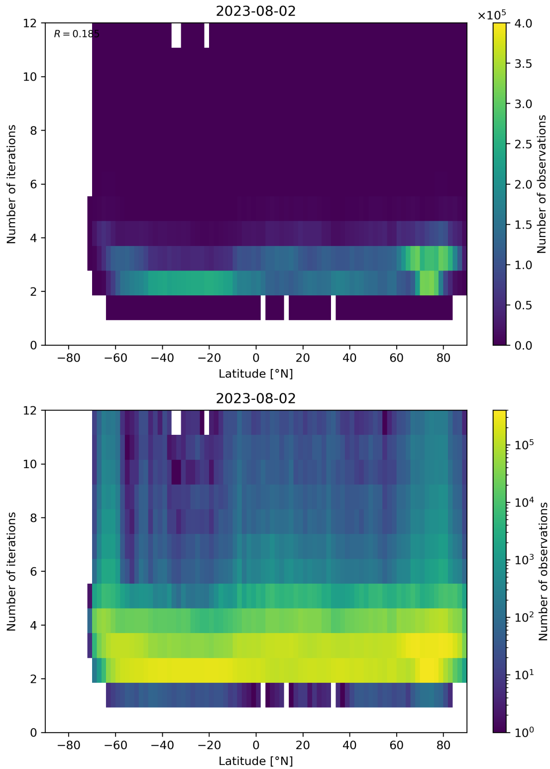
Figure 102: Scatter density plot of “Latitude” against “Number of iterations” for 2023-08-01 to 2023-08-03.
