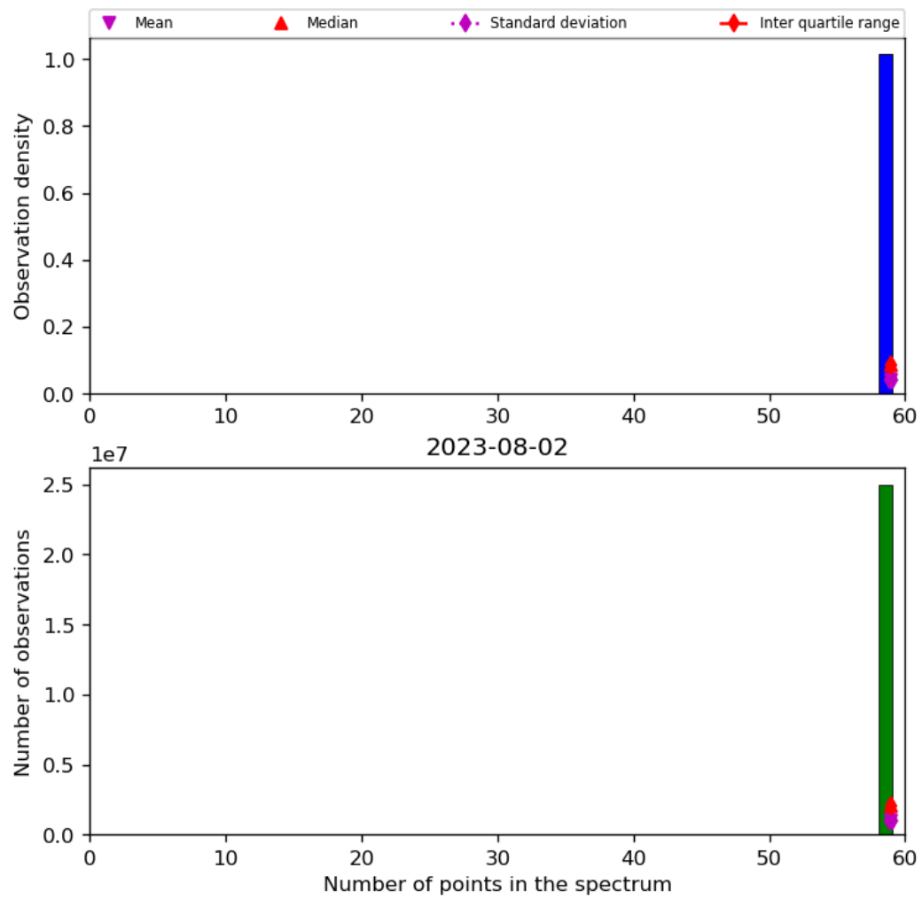
Figure 44: Histogram of “Number of points in the spectrum” for 2023-08-01 to 2023-08-03
