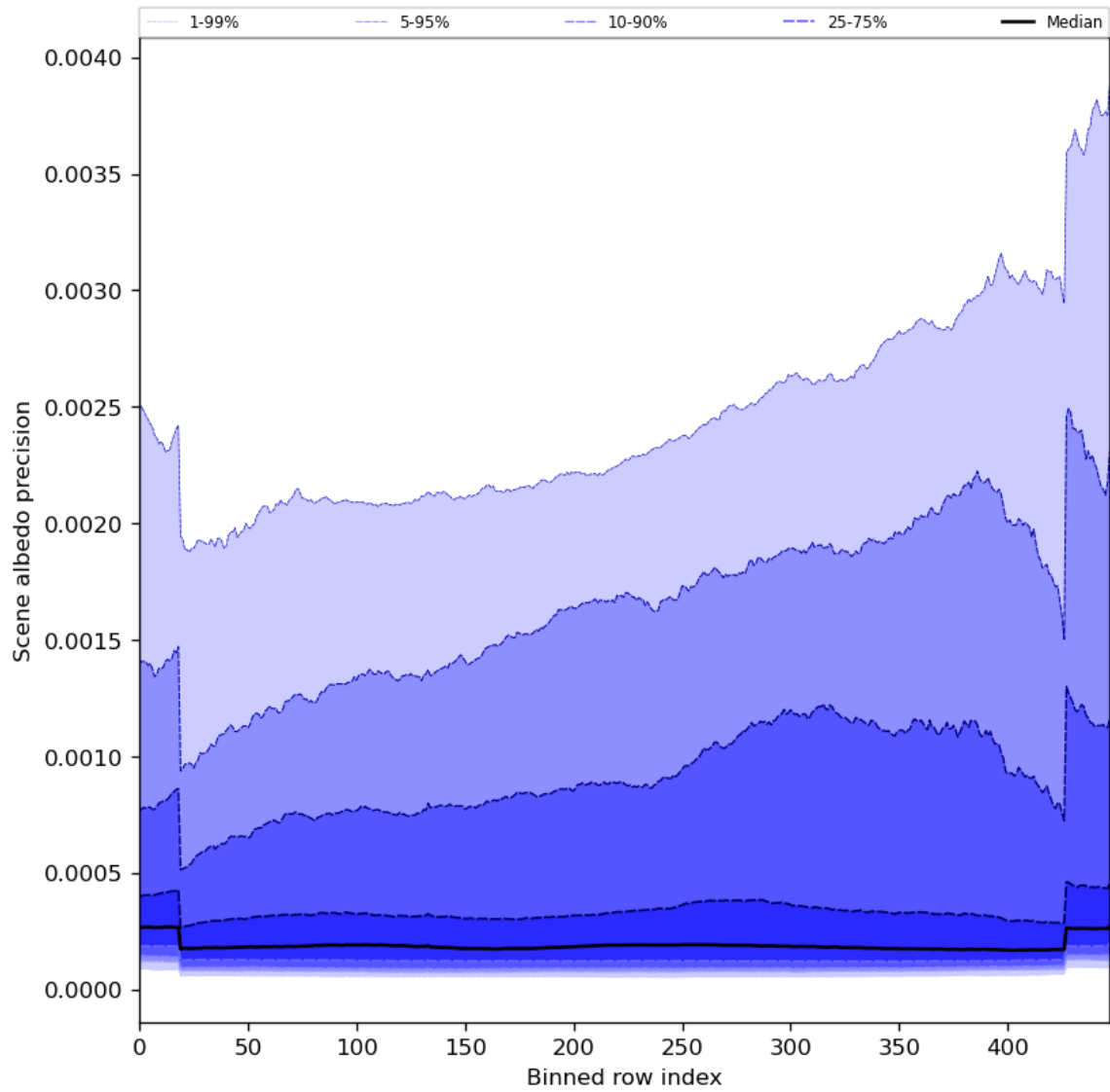
Figure 52: Along track statistics of “Scene albedo precision” for 2023-08-01 to 2023-08-03
