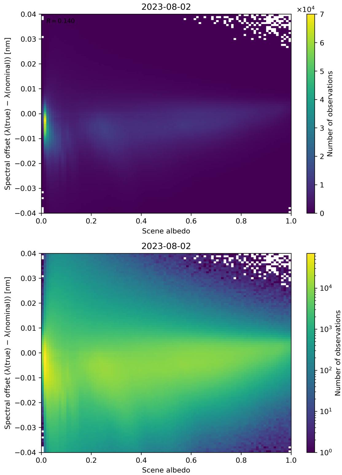
Figure 117: Scatter density plot of “Scene albedo” against “Spectral offset ( \lambda(\text{true}) - \lambda(\text{nominal}) )” for 2023-08-01 to 2023-08-03.
