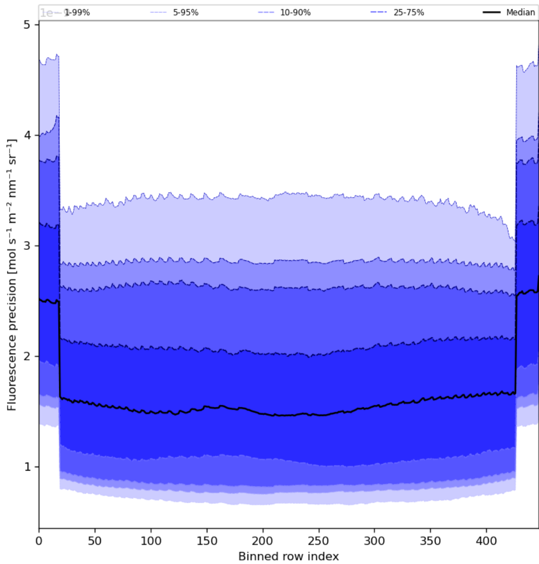
Figure 58: Along track statistics of “Fluorescence precision” for 2023-08-01 to 2023-08-03
