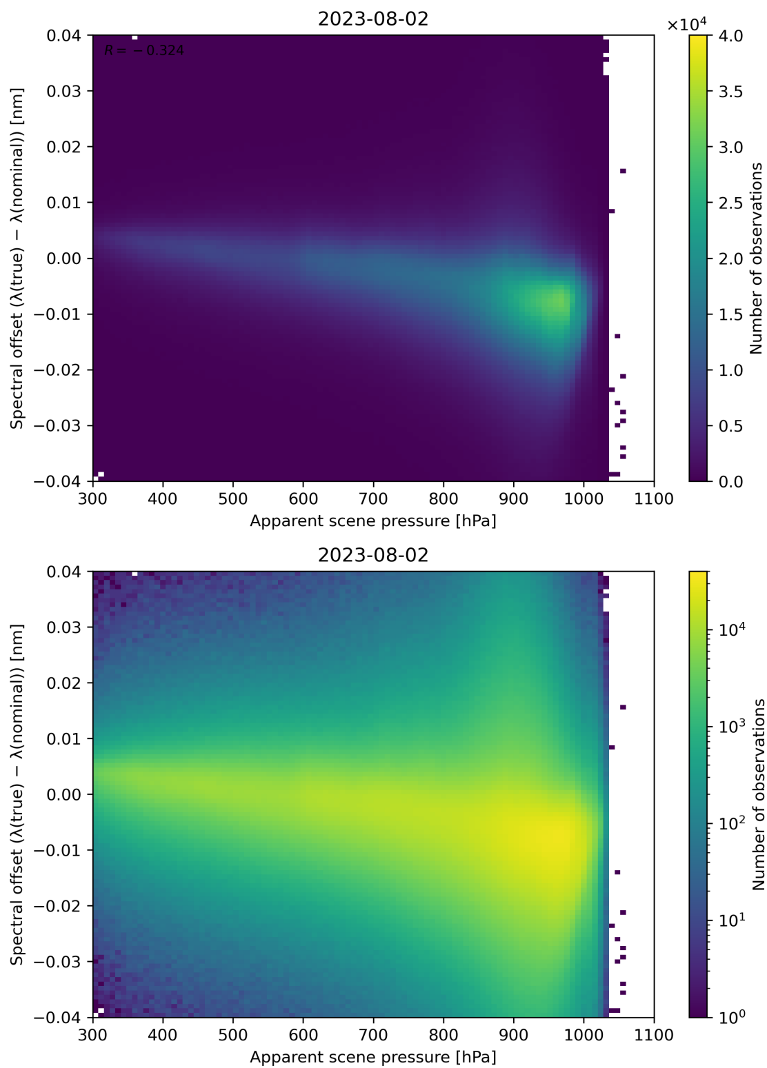
Figure 68: Scatter density plot of “Apparent scene pressure” against “Spectral offset ( \lambda(\text{true}) - \lambda(\text{nominal}) )” for 2023-08-01 to 2023-08-03.
