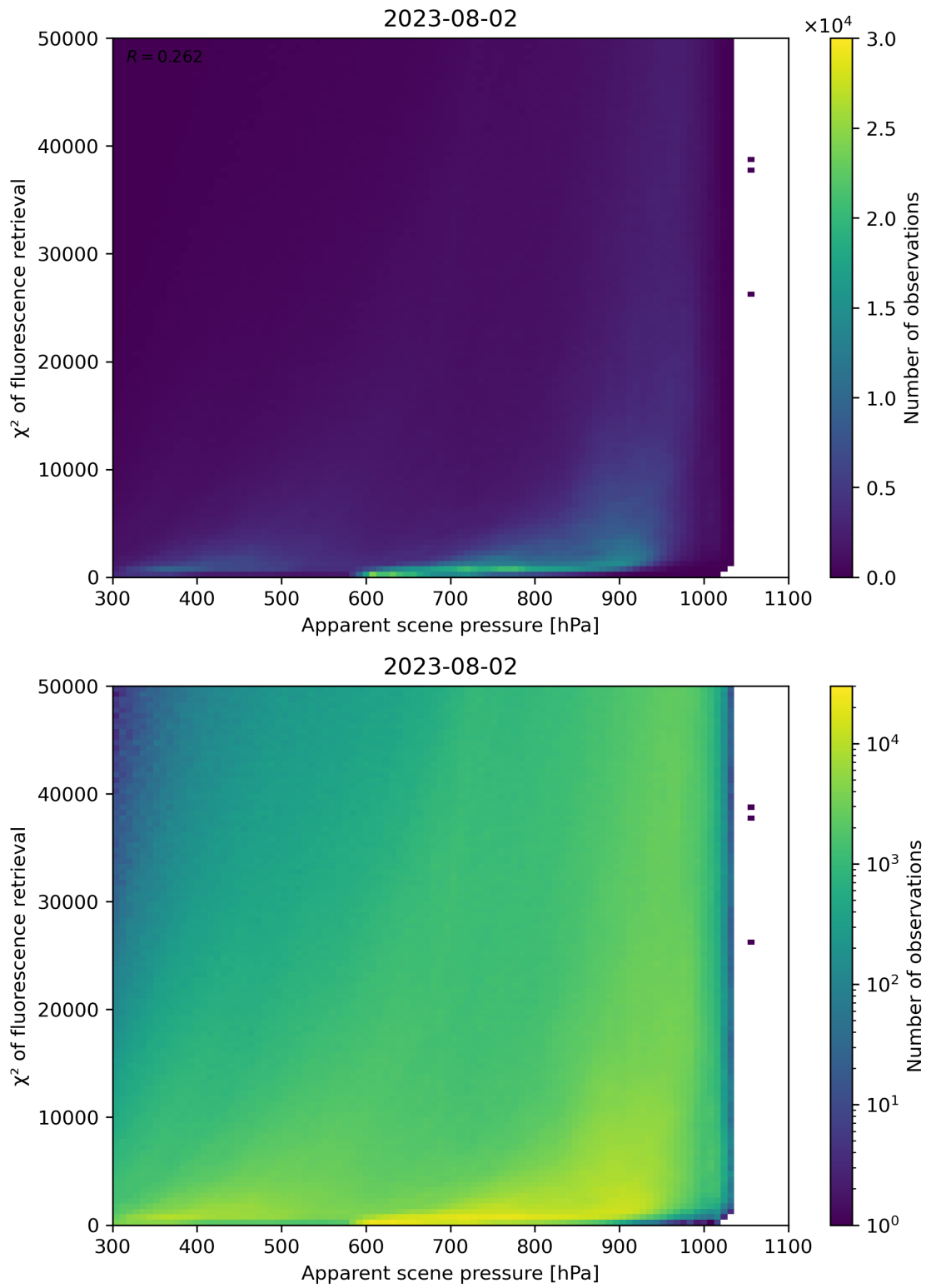
Figure 64: Scatter density plot of “Apparent scene pressure” against “ \chi^2 of fluorescence retrieval” for 2023-08-01 to 2023-08-03.
