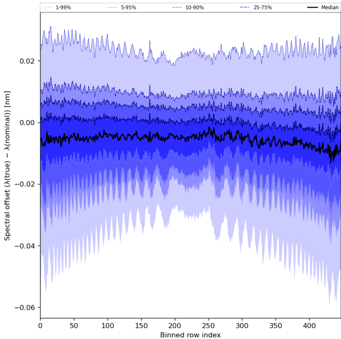
Figure 62: Along track statistics of “Spectral offset ( \lambda(\text{true}) - \lambda(\text{nominal}) )” for 2023-08-01 to 2023-08-03
