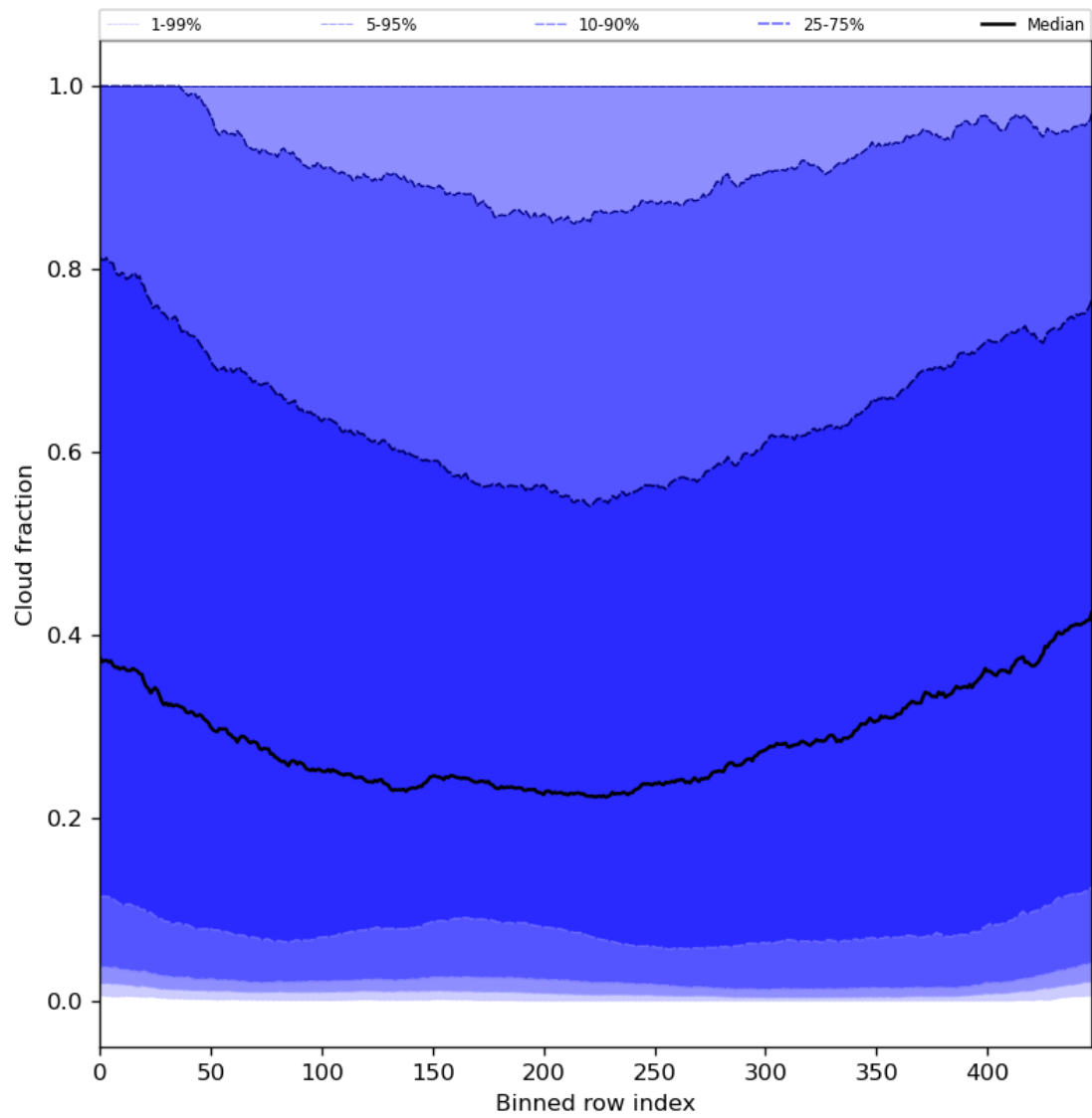
Figure 49: Along track statistics of “Cloud fraction” for 2023-08-01 to 2023-08-03
