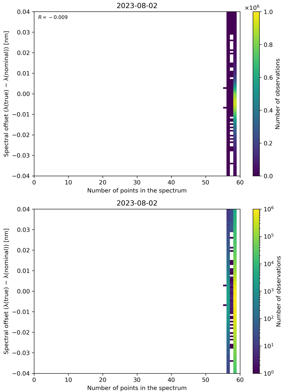
Figure 110: Scatter density plot of “Number of points in the spectrum” against “Spectral offset ( \lambda(\text{true}) - \lambda(\text{nominal}) )” for 2023-08-01 to 2023-08-03.
