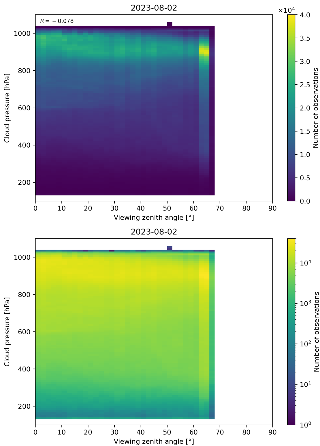
Figure 133: Scatter density plot of “Viewing zenith angle” against “Cloud pressure” for 2023-08-01 to 2023-08-03.
