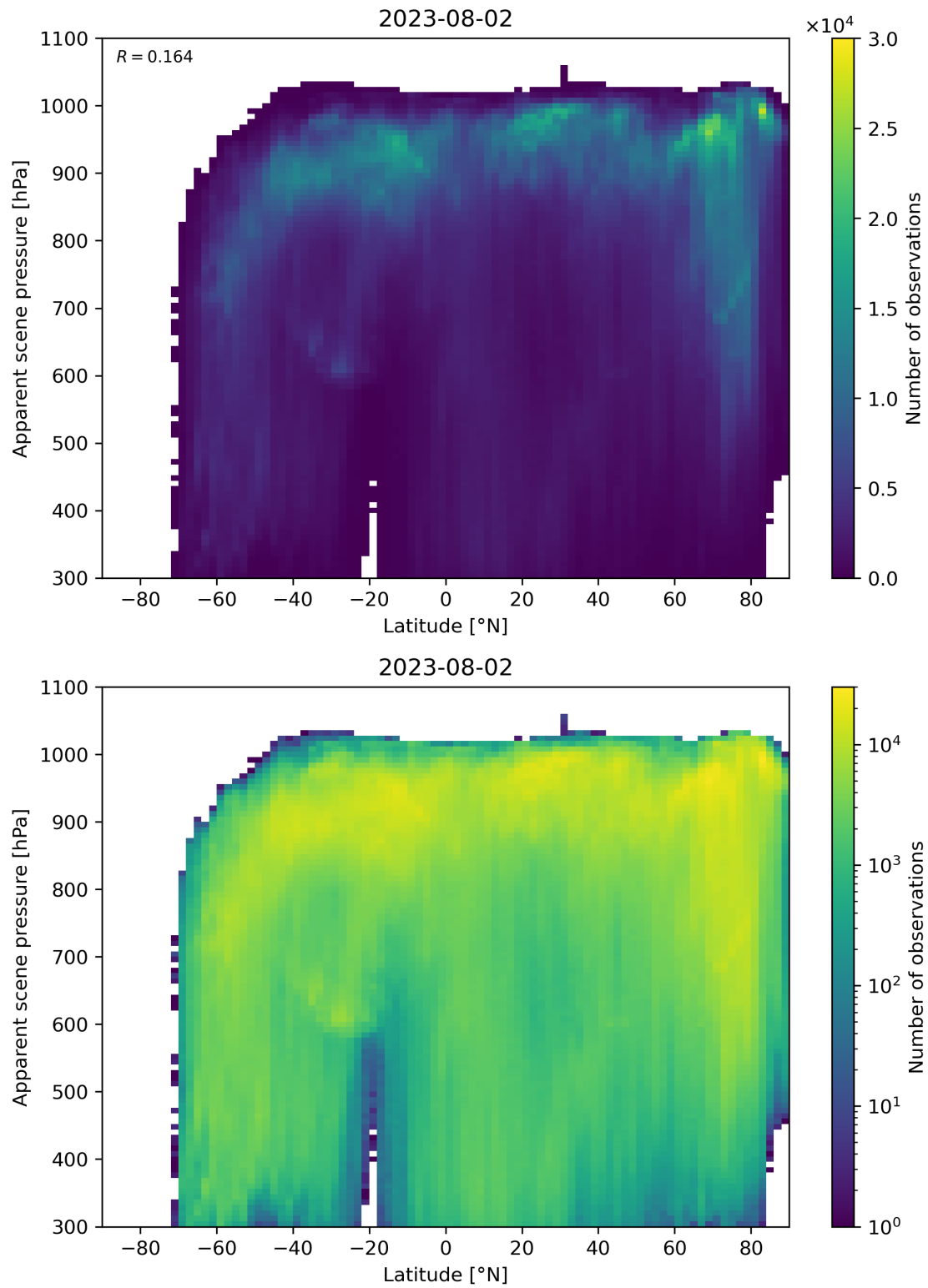
Figure 96: Scatter density plot of “Latitude” against “Apparent scene pressure” for 2023-08-01 to 2023-08-03.
