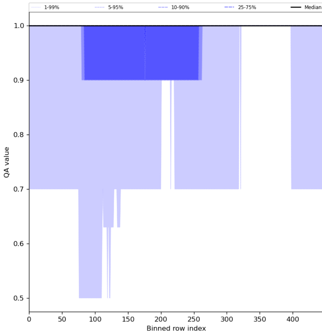
Figure 46: Along track statistics of “QA value” for 2023-08-01 to 2023-08-03
