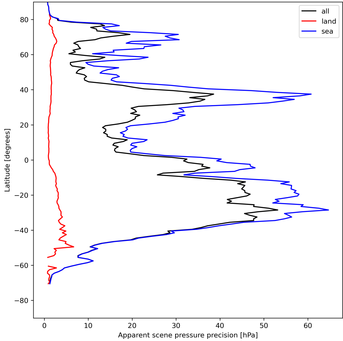
Figure 20: Zonal average of “Apparent scene pressure precision” for 2023-08-01 to 2023-08-03.
