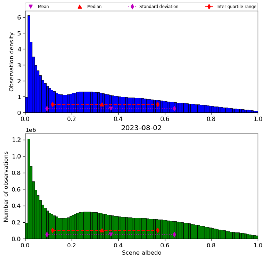
Figure 34: Histogram of “Scene albedo” for 2023-08-01 to 2023-08-03
