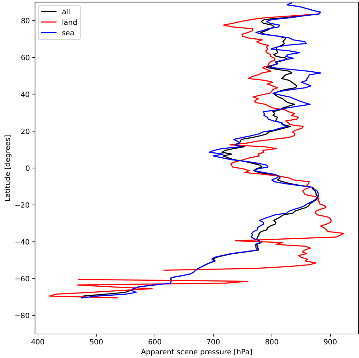
Figure 19: Zonal average of “Apparent scene pressure” for 2023-08-01 to 2023-08-03.
