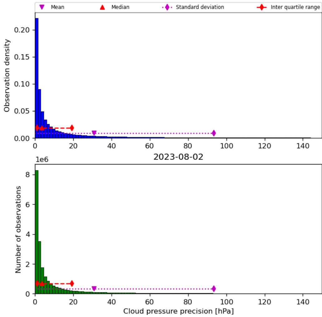
Figure 31: Histogram of “Cloud pressure precision” for 2023-08-01 to 2023-08-03
