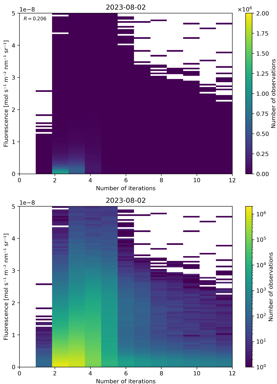
Figure 107: Scatter density plot of "Number of iterations" against "Fluorescence" for 2023-08-01 to 2023-08-03.
