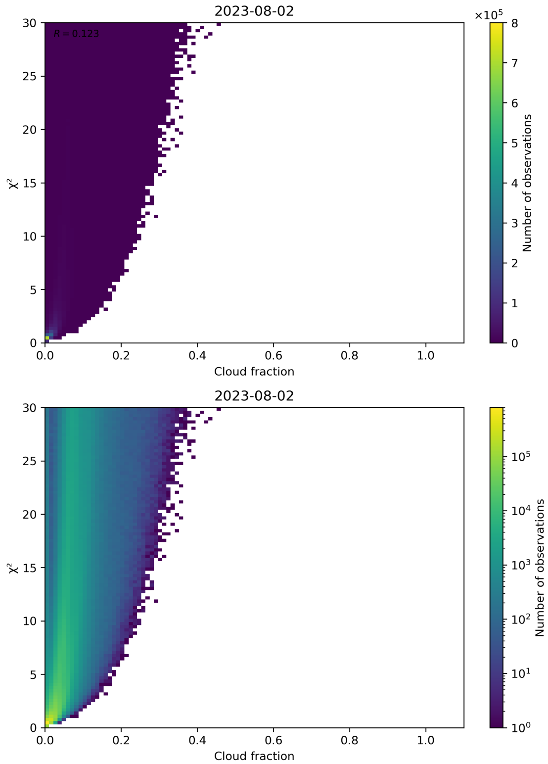
Figure 77: Scatter density plot of “Cloud fraction” against “ \chi^2 ” for 2023-08-01 to 2023-08-03.
