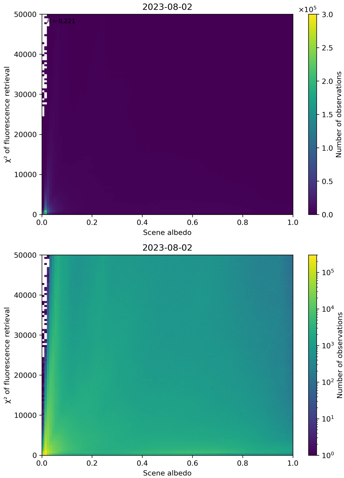
Figure 113: Scatter density plot of “Scene albedo” against “ \chi^2 of fluorescence retrieval” for 2023-08-01 to 2023-08-03.
