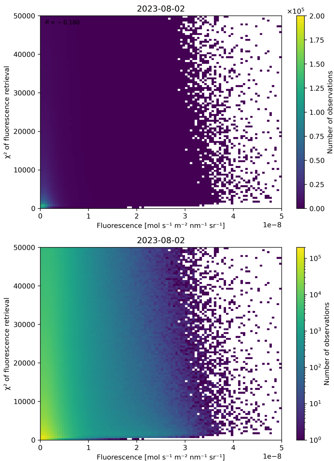
Figure 93: Scatter density plot of “Fluorescence” against “ \chi^2 of fluorescence retrieval” for 2023-08-01 to 2023-08-03.
