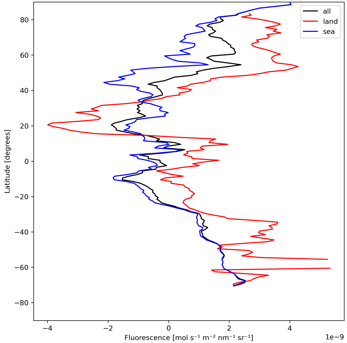
Figure 23: Zonal average of “Fluorescence” for 2023-08-01 to 2023-08-03.
