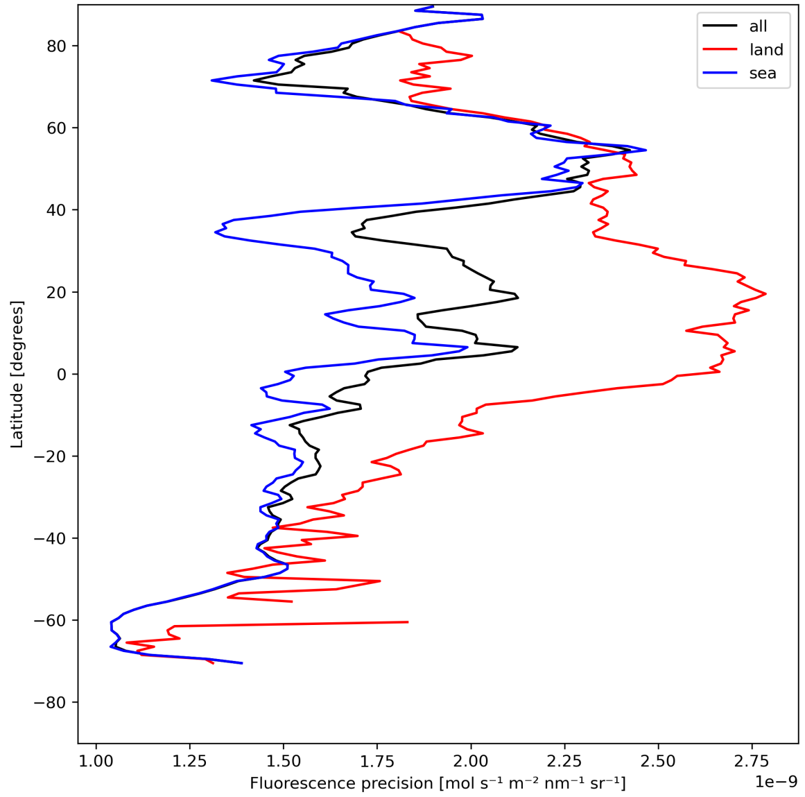
Figure 24: Zonal average of “Fluorescence precision” for 2023-08-01 to 2023-08-03.
