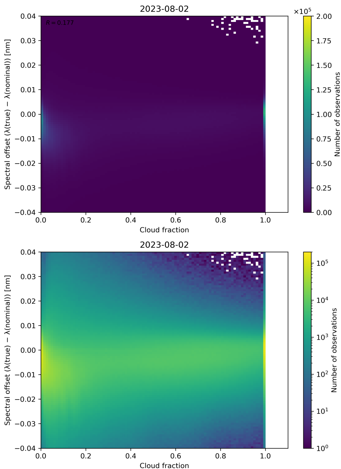
Figure 83: Scatter density plot of “Cloud fraction” against “Spectral offset ( \lambda(\text{true}) - \lambda(\text{nominal}) )” for 2023-08-01 to 2023-08-03.
