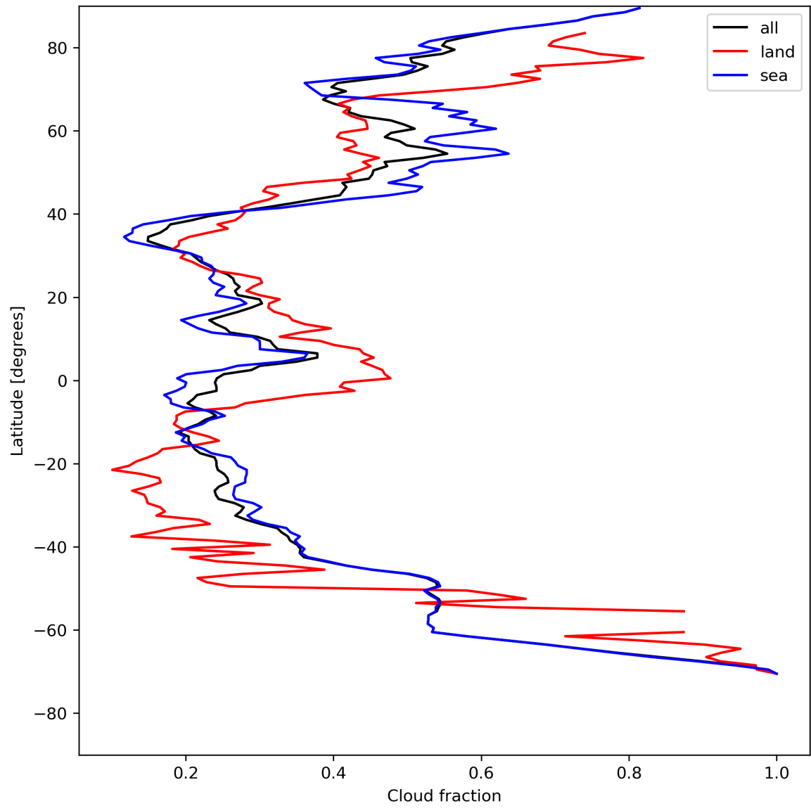
Figure 15: Zonal average of “Cloud fraction” for 2023-08-01 to 2023-08-03.
