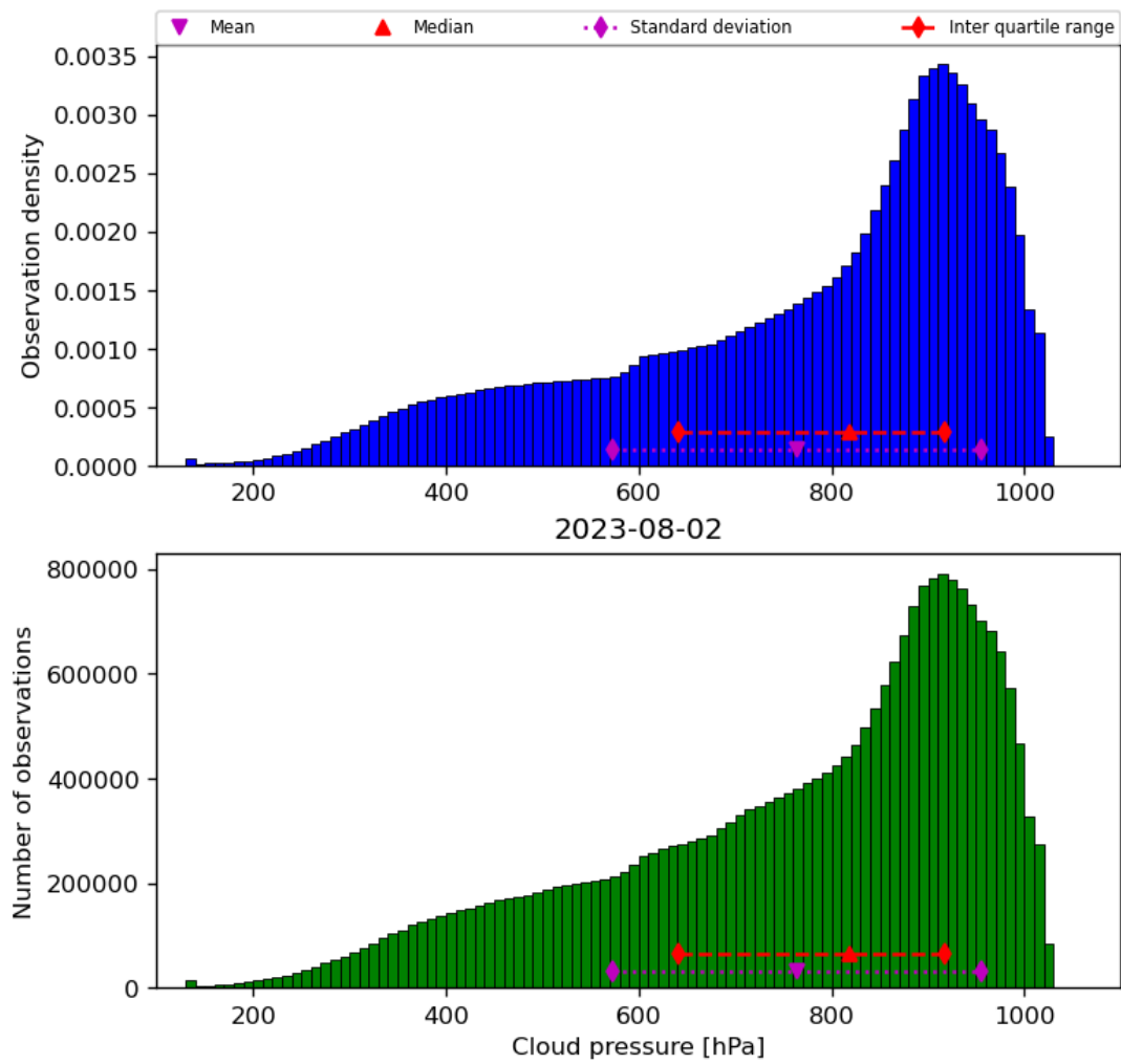
Figure 30: Histogram of “Cloud pressure” for 2023-08-01 to 2023-08-03
