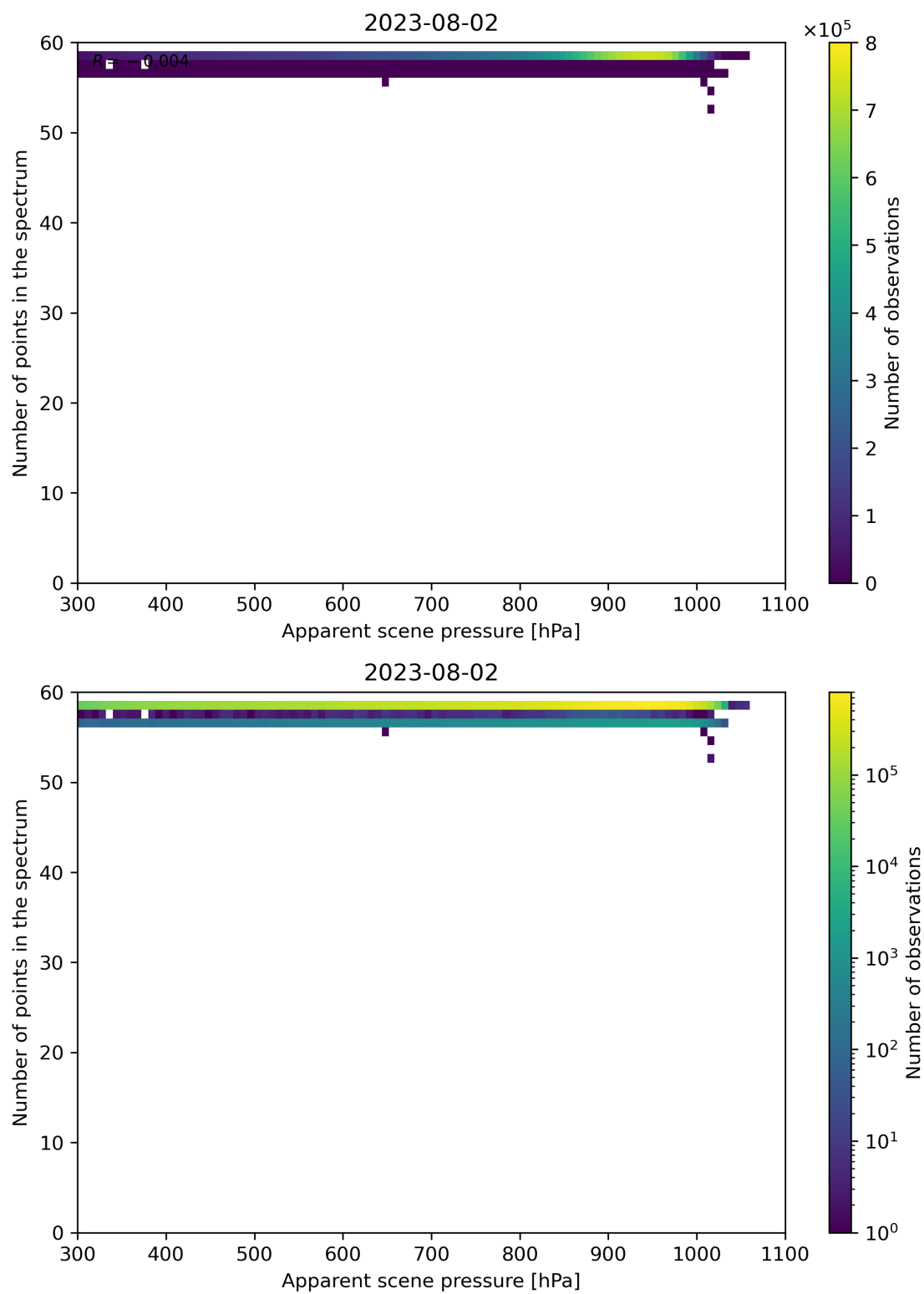
Figure 67: Scatter density plot of “Apparent scene pressure” against “Number of points in the spectrum” for 2023-08-01 to 2023-08-03.
