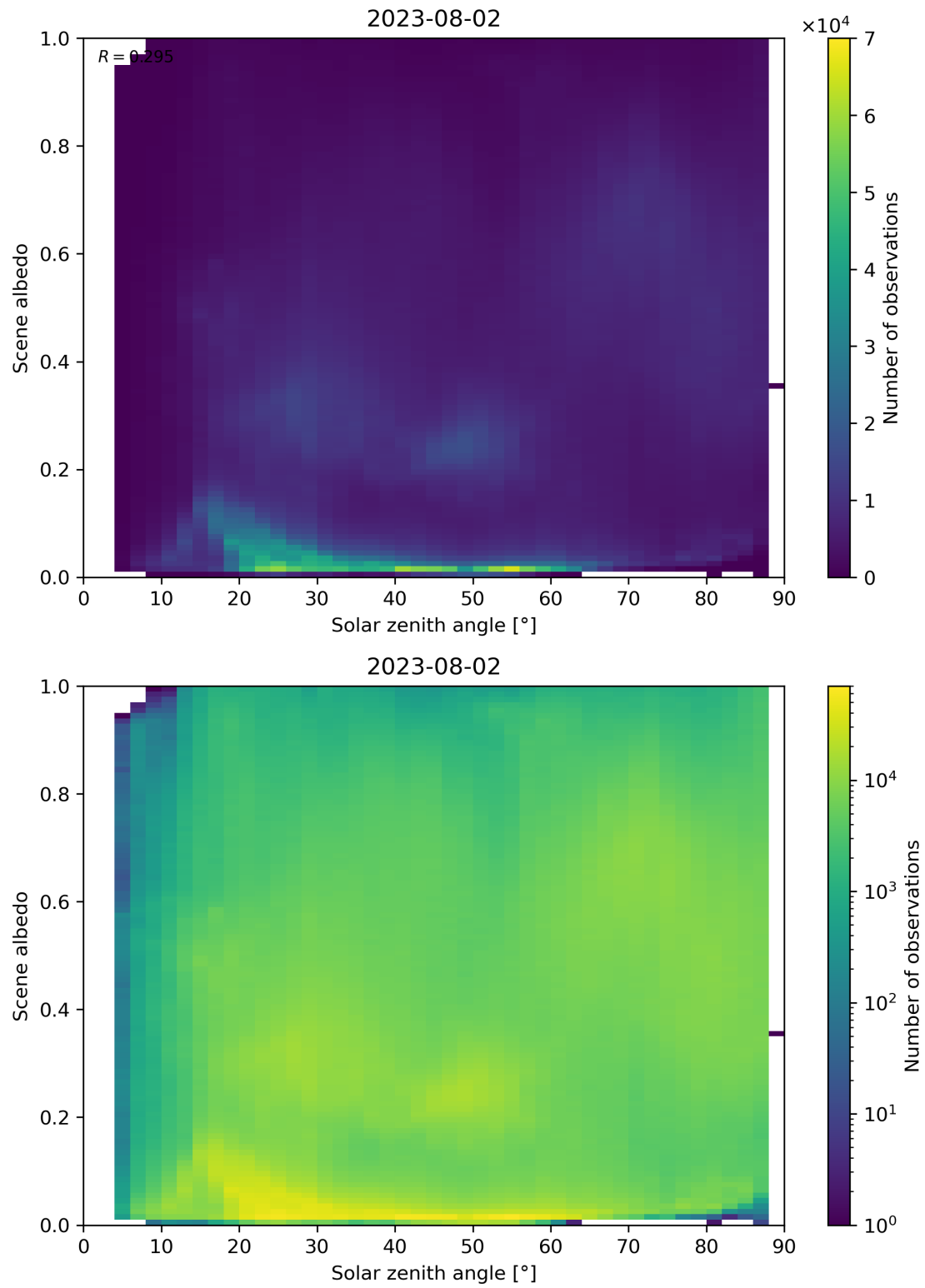
Figure 127: Scatter density plot of “Solar zenith angle” against “Scene albedo” for 2023-08-01 to 2023-08-03.
