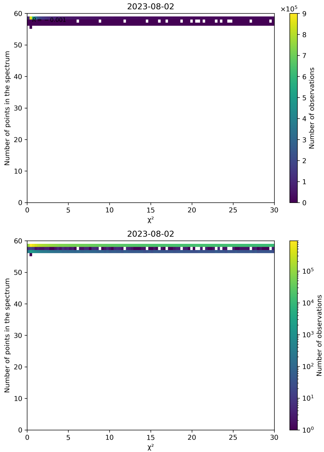
Figure 74: Scatter density plot of " \chi^2 " against "Number of points in the spectrum" for 2023-08-01 to 2023-08-03.
