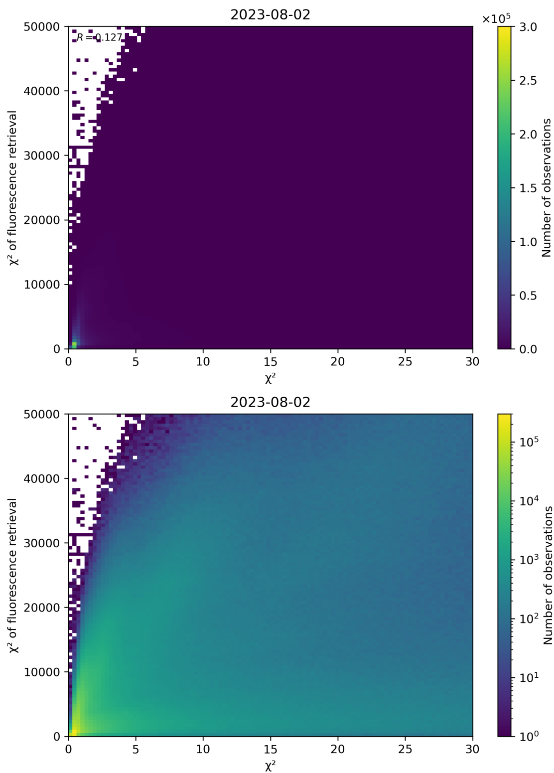
Figure 69: Scatter density plot of “ \chi^2 ” against “ \chi^2 of fluorescence retrieval” for 2023-08-01 to 2023-08-03.
