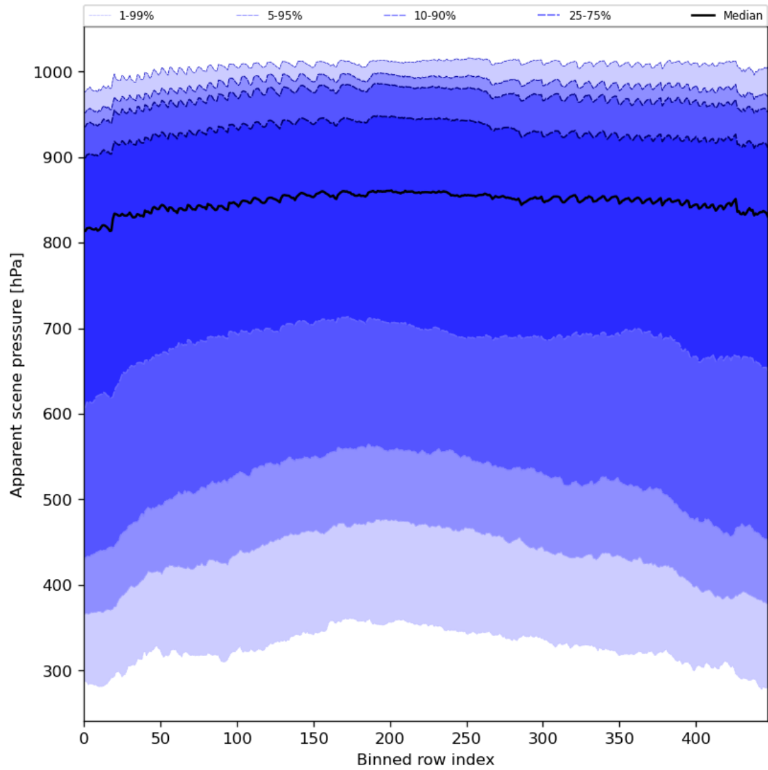
Figure 53: Along track statistics of “Apparent scene pressure” for 2023-08-01 to 2023-08-03
