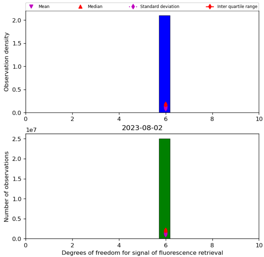
Figure 43: Histogram of “Degrees of freedom for signal of fluorescence retrieval” for 2023-08-01 to 2023-08-03
