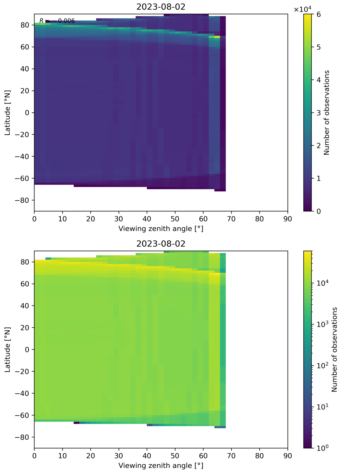
Figure 135: Scatter density plot of “Viewing zenith angle” against “Latitude” for 2023-08-01 to 2023-08-03.
