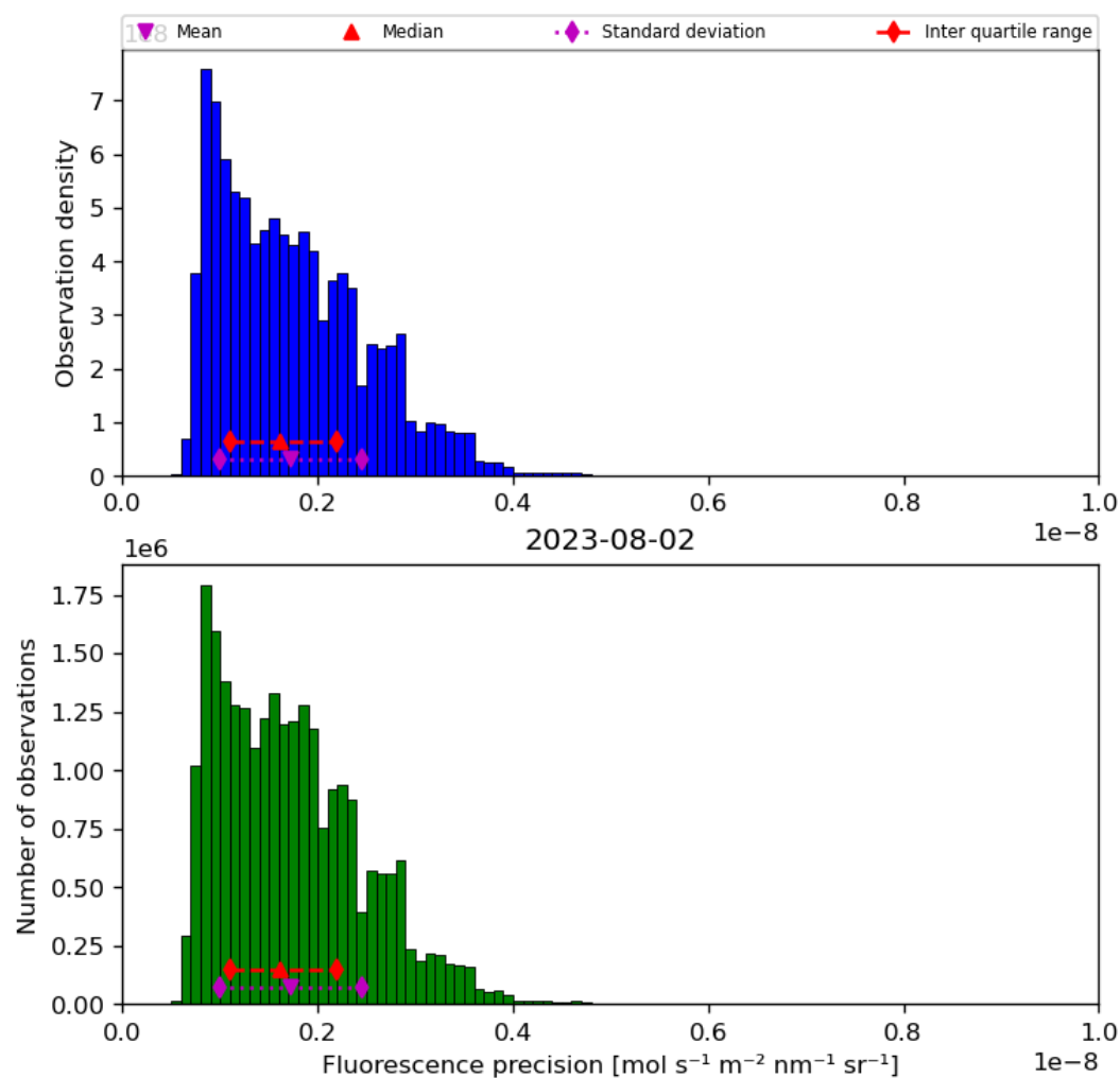
Figure 41: Histogram of “Fluorescence precision” for 2023-08-01 to 2023-08-03
