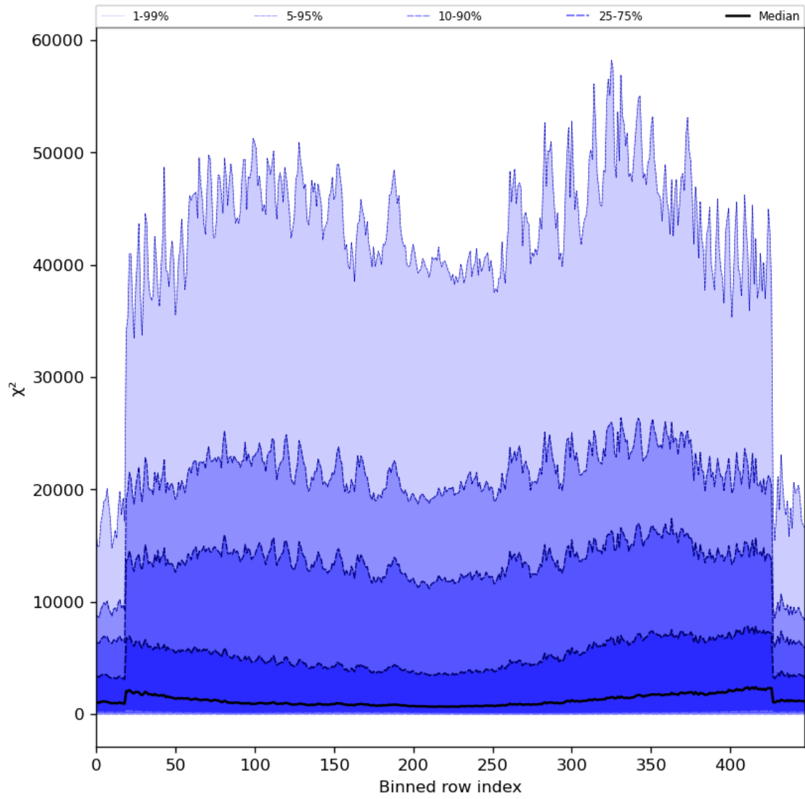
Figure 55: Along track statistics of “ \chi^2 ” for 2023-08-01 to 2023-08-03
