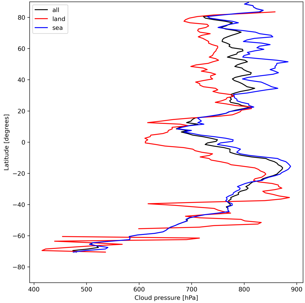
Figure 13: Zonal average of “Cloud pressure” for 2023-08-01 to 2023-08-03.
