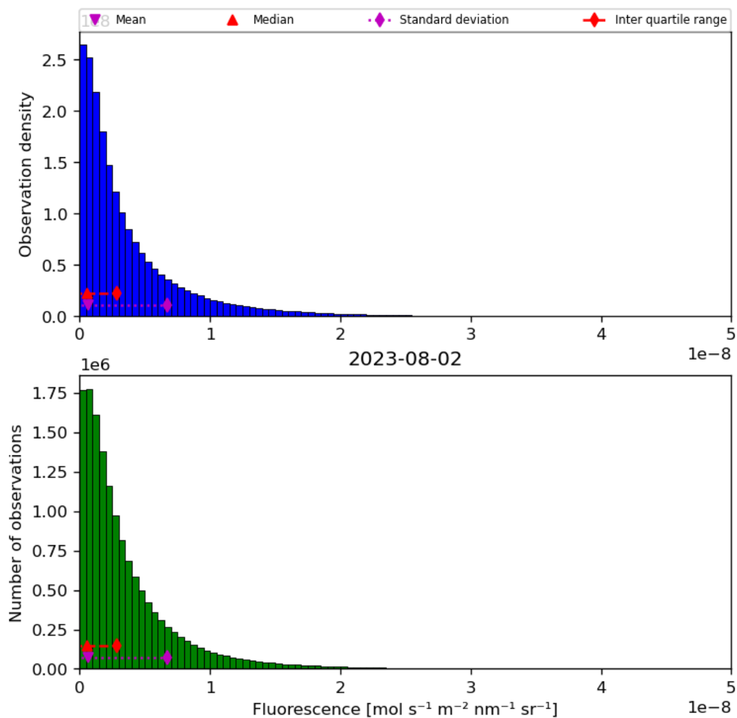
Figure 40: Histogram of “Fluorescence” for 2023-08-01 to 2023-08-03
