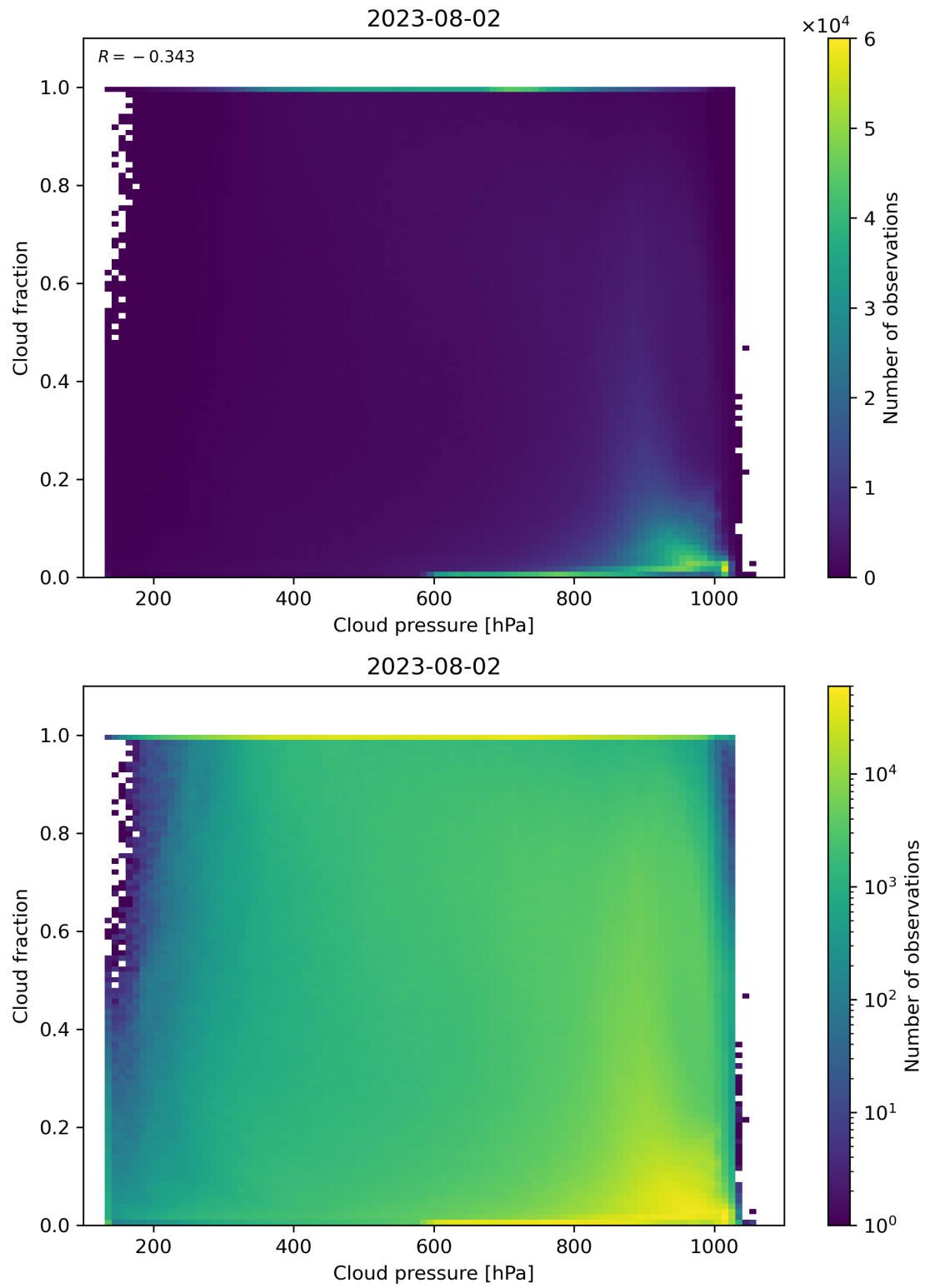
Figure 87: Scatter density plot of “Cloud pressure” against “Cloud fraction” for 2023-08-01 to 2023-08-03.
