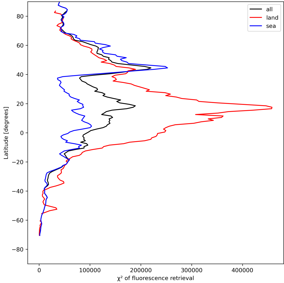
Figure 25: Zonal average of “ \chi^2 of fluorescence retrieval” for 2023-08-01 to 2023-08-03.
