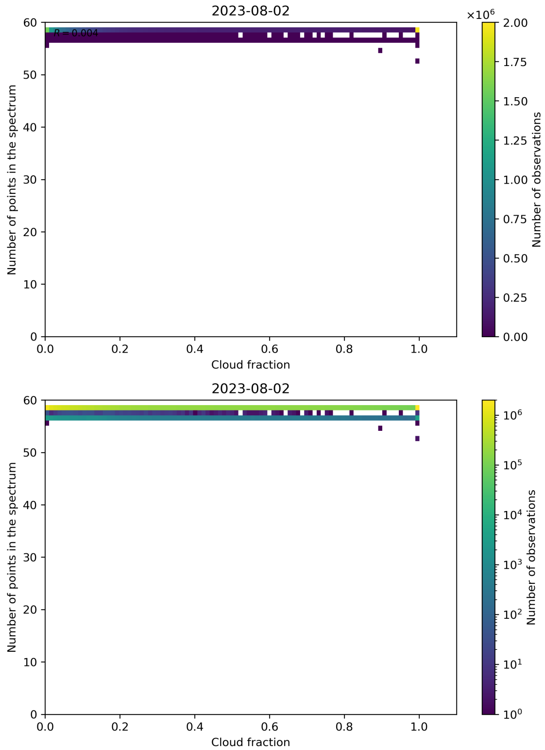
Figure 81: Scatter density plot of “Cloud fraction” against “Number of points in the spectrum” for 2023-08-01 to 2023-08-03.
