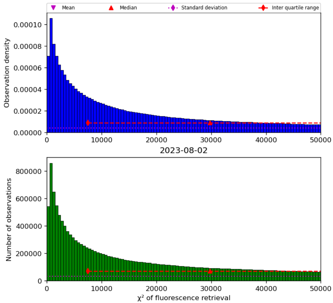
Figure 42: Histogram of “ \chi^2 of fluorescence retrieval” for 2023-08-01 to 2023-08-03
