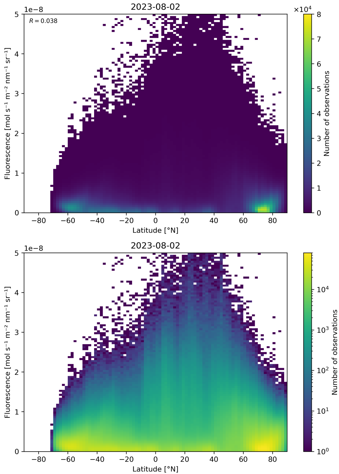
Figure 101: Scatter density plot of “Latitude” against “Fluorescence” for 2023-08-01 to 2023-08-03.
