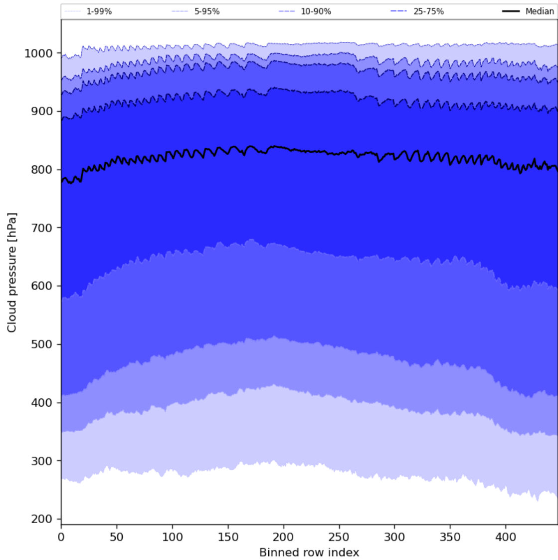
Figure 47: Along track statistics of “Cloud pressure” for 2023-08-01 to 2023-08-03
