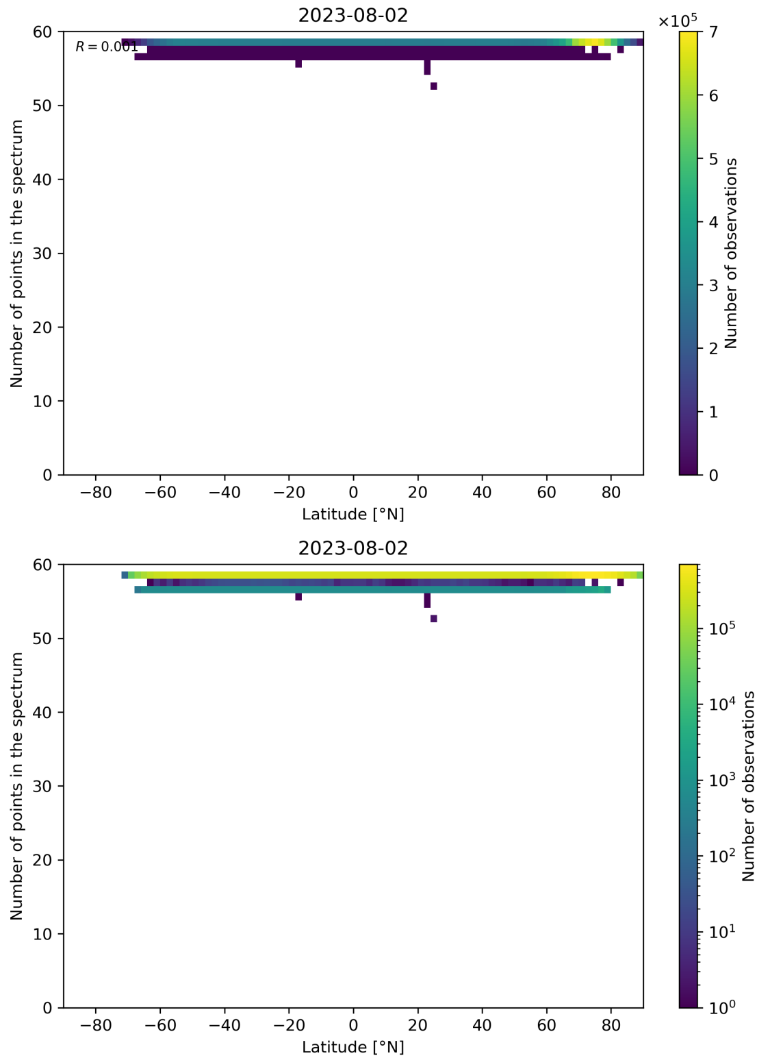
Figure 103: Scatter density plot of “Latitude” against “Number of points in the spectrum” for 2023-08-01 to 2023-08-03.
