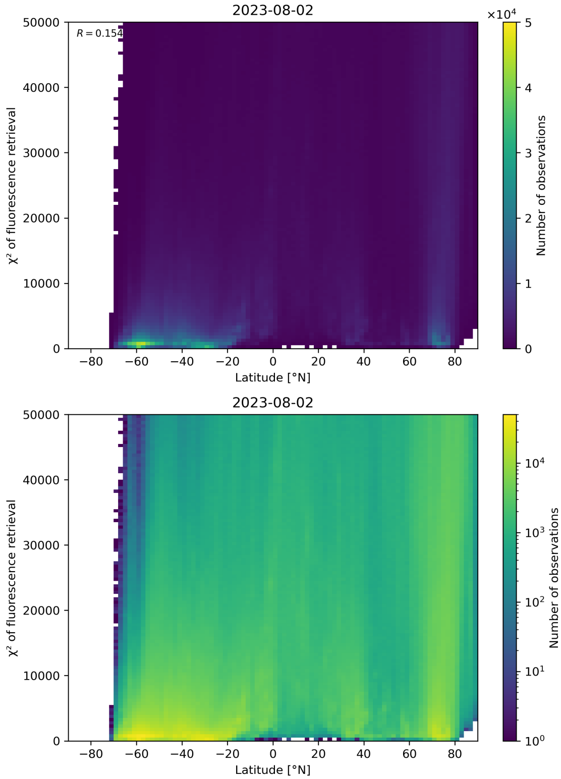
Figure 98: Scatter density plot of “Latitude” against “ \chi^2 of fluorescence retrieval” for 2023-08-01 to 2023-08-03.
