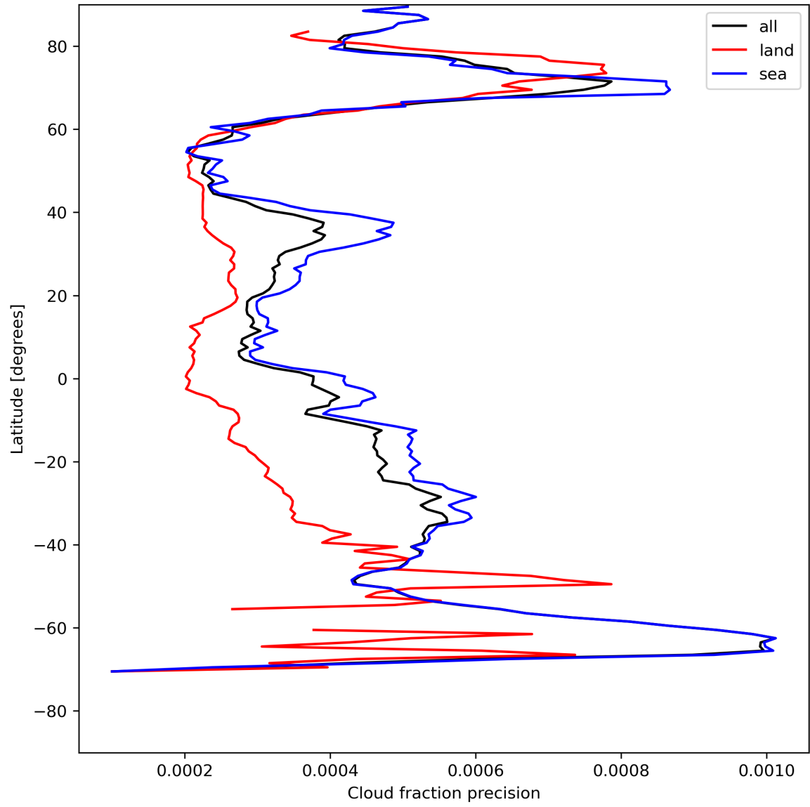
Figure 16: Zonal average of “Cloud fraction precision” for 2023-08-01 to 2023-08-03.
