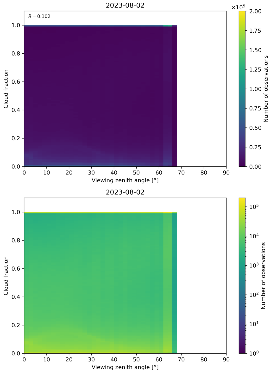
Figure 132: Scatter density plot of “Viewing zenith angle” against “Cloud fraction” for 2023-08-01 to 2023-08-03.
