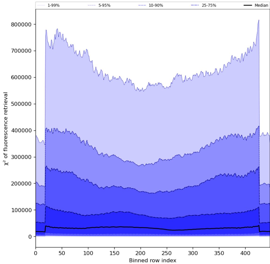
Figure 59: Along track statistics of “ \chi^2 of fluorescence retrieval” for 2023-08-01 to 2023-08-03
