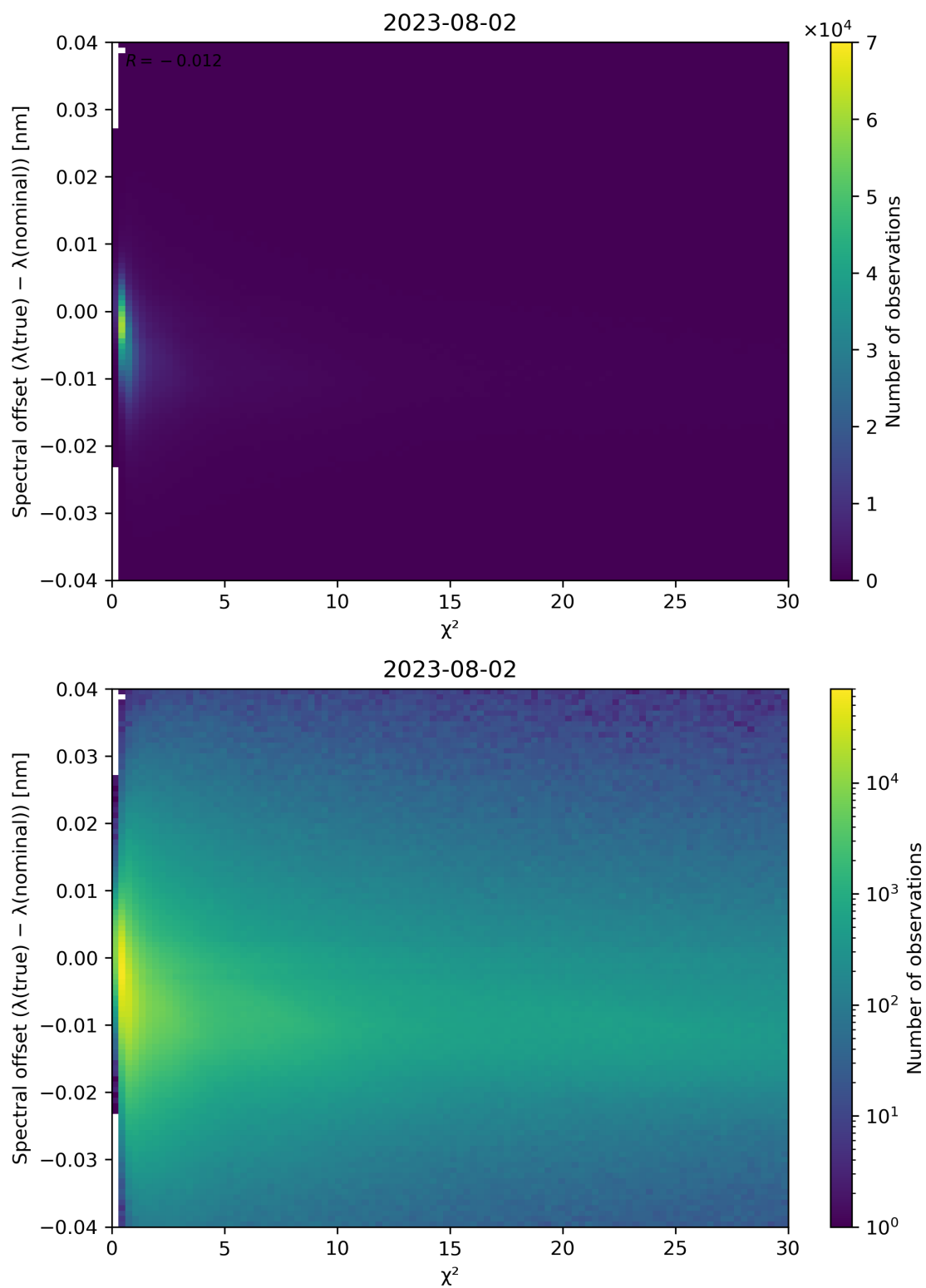
Figure 75: Scatter density plot of “ \chi^2 ” against “Spectral offset ( \lambda(\text{true}) - \lambda(\text{nominal}) )” for 2023-08-01 to 2023-08-03.
