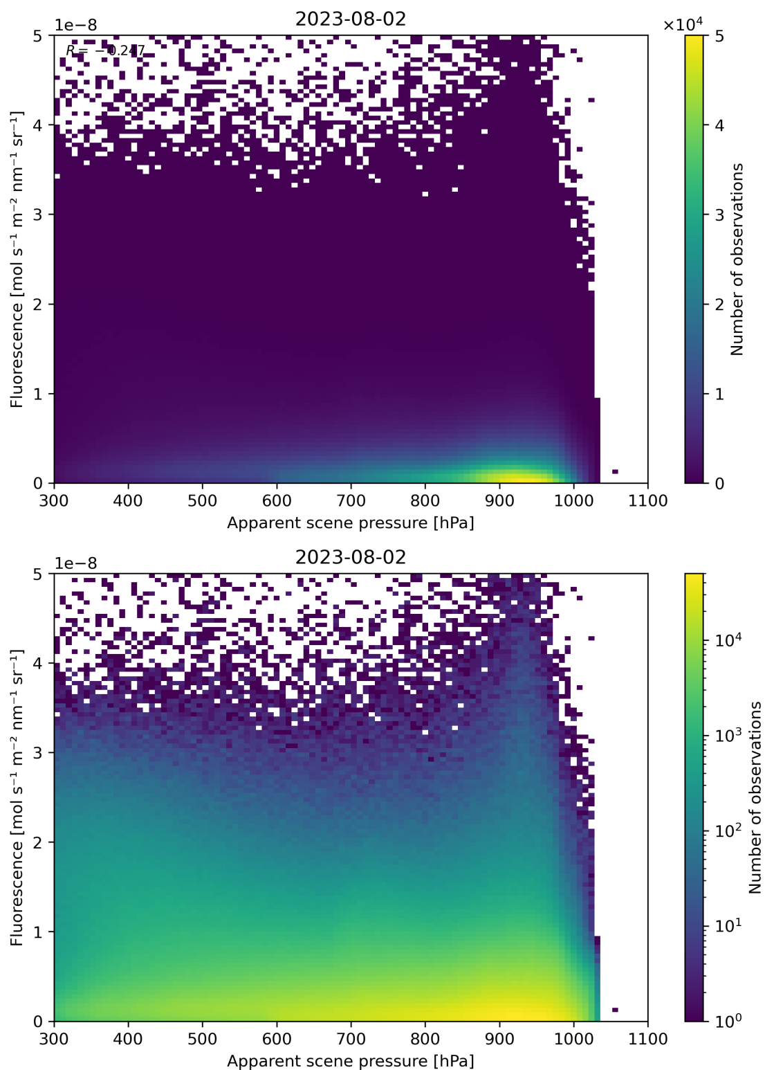
Figure 65: Scatter density plot of “Apparent scene pressure” against “Fluorescence” for 2023-08-01 to 2023-08-03.
