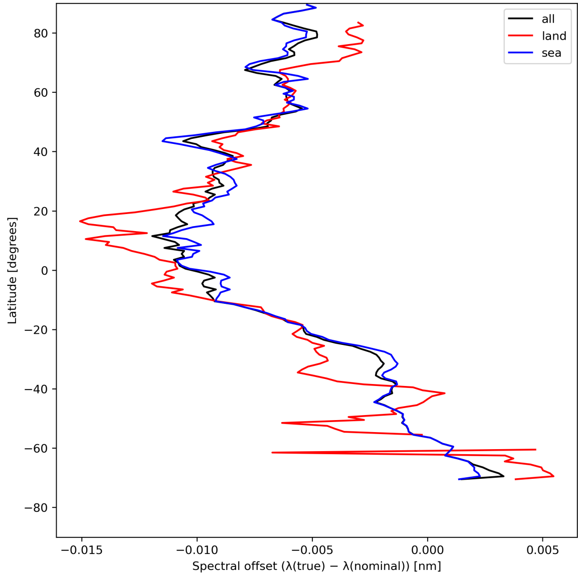
Figure 28: Zonal average of “Spectral offset ( \lambda(\text{true}) - \lambda(\text{nominal}) )” for 2023-08-01 to 2023-08-03.
