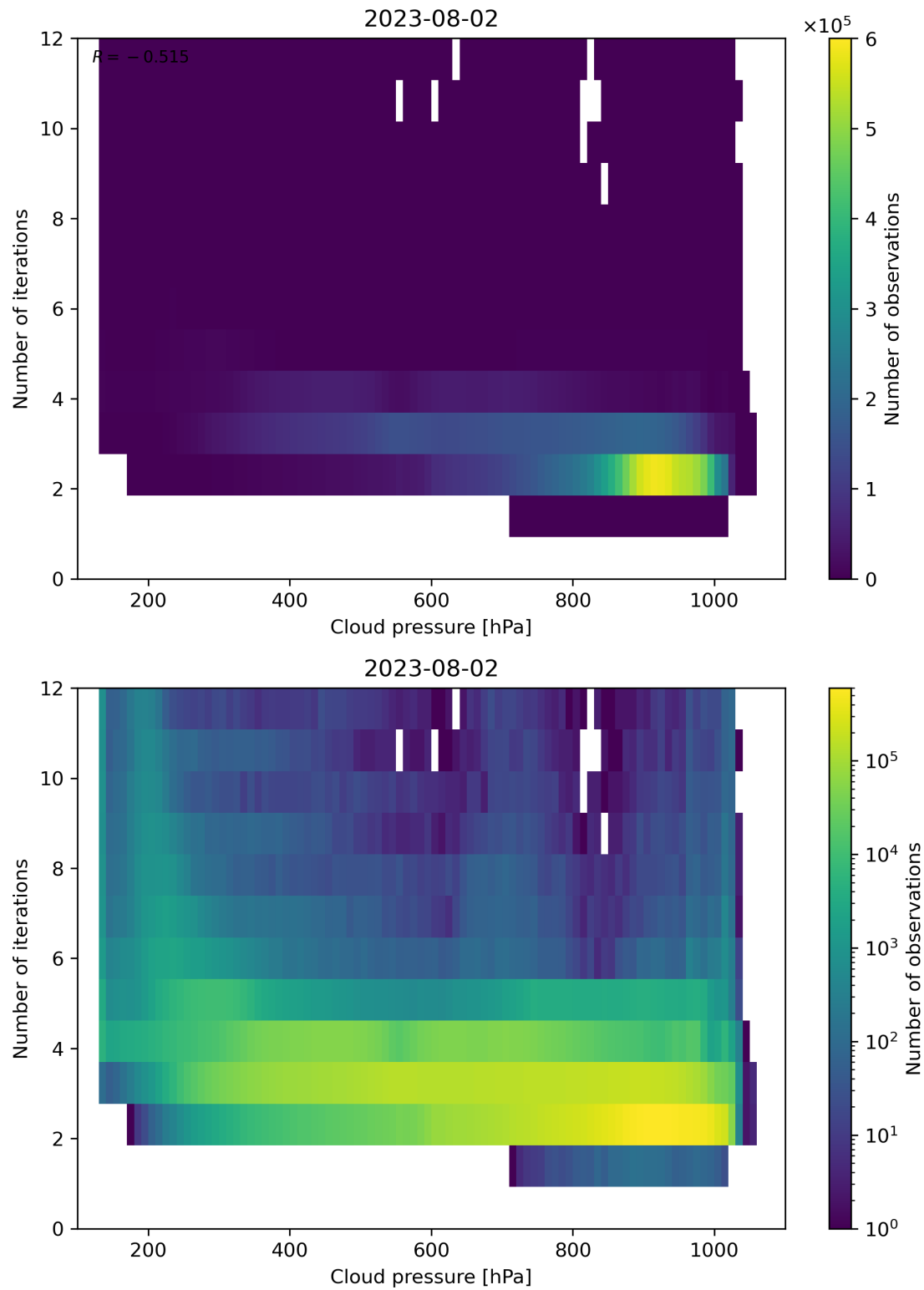
Figure 89: Scatter density plot of “Cloud pressure” against “Number of iterations” for 2023-08-01 to 2023-08-03.
