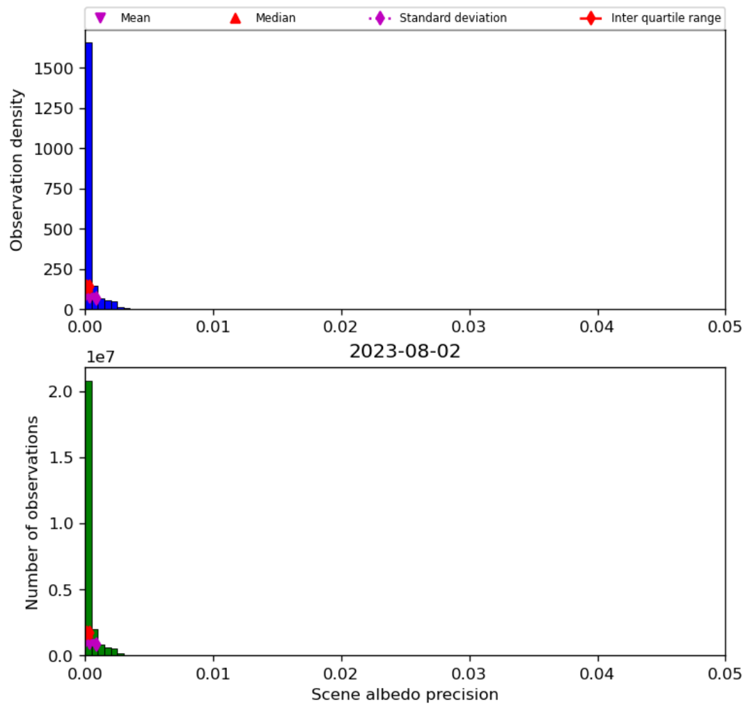
Figure 35: Histogram of “Scene albedo precision” for 2023-08-01 to 2023-08-03
