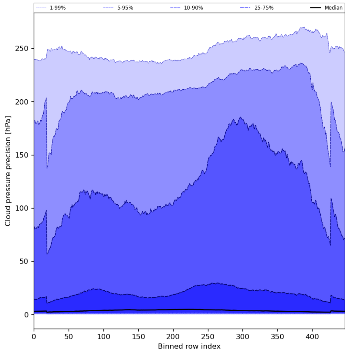
Figure 48: Along track statistics of “Cloud pressure precision” for 2023-08-01 to 2023-08-03
