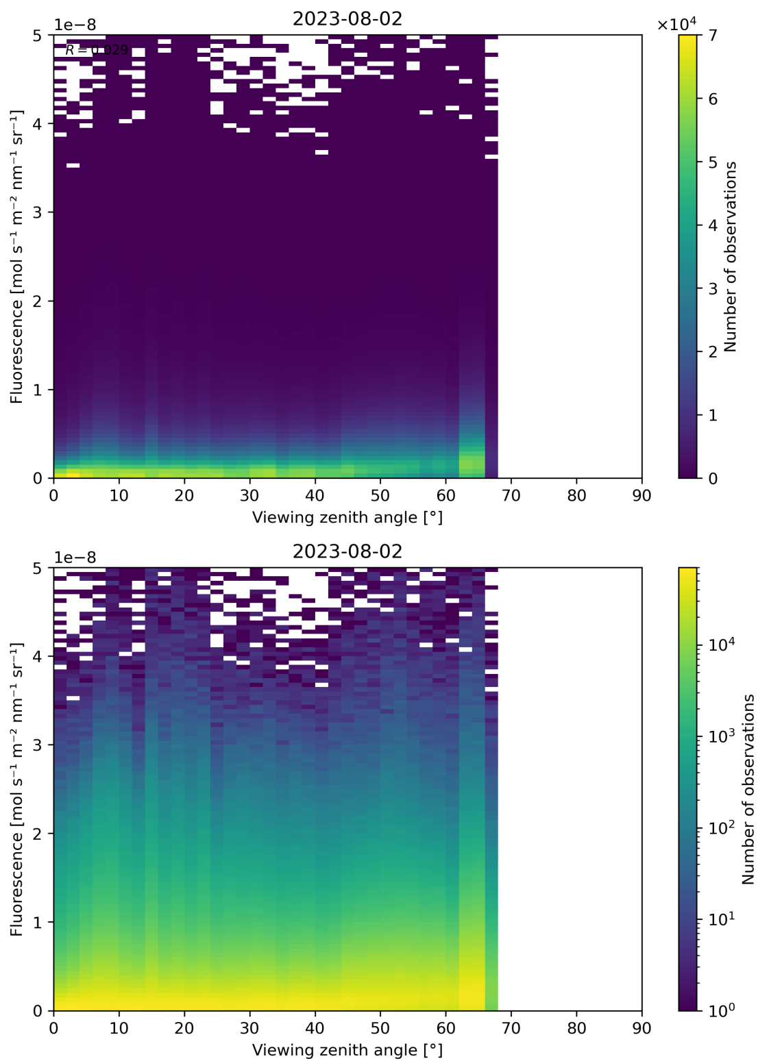
Figure 134: Scatter density plot of “Viewing zenith angle” against “Fluorescence” for 2023-08-01 to 2023-08-03.
