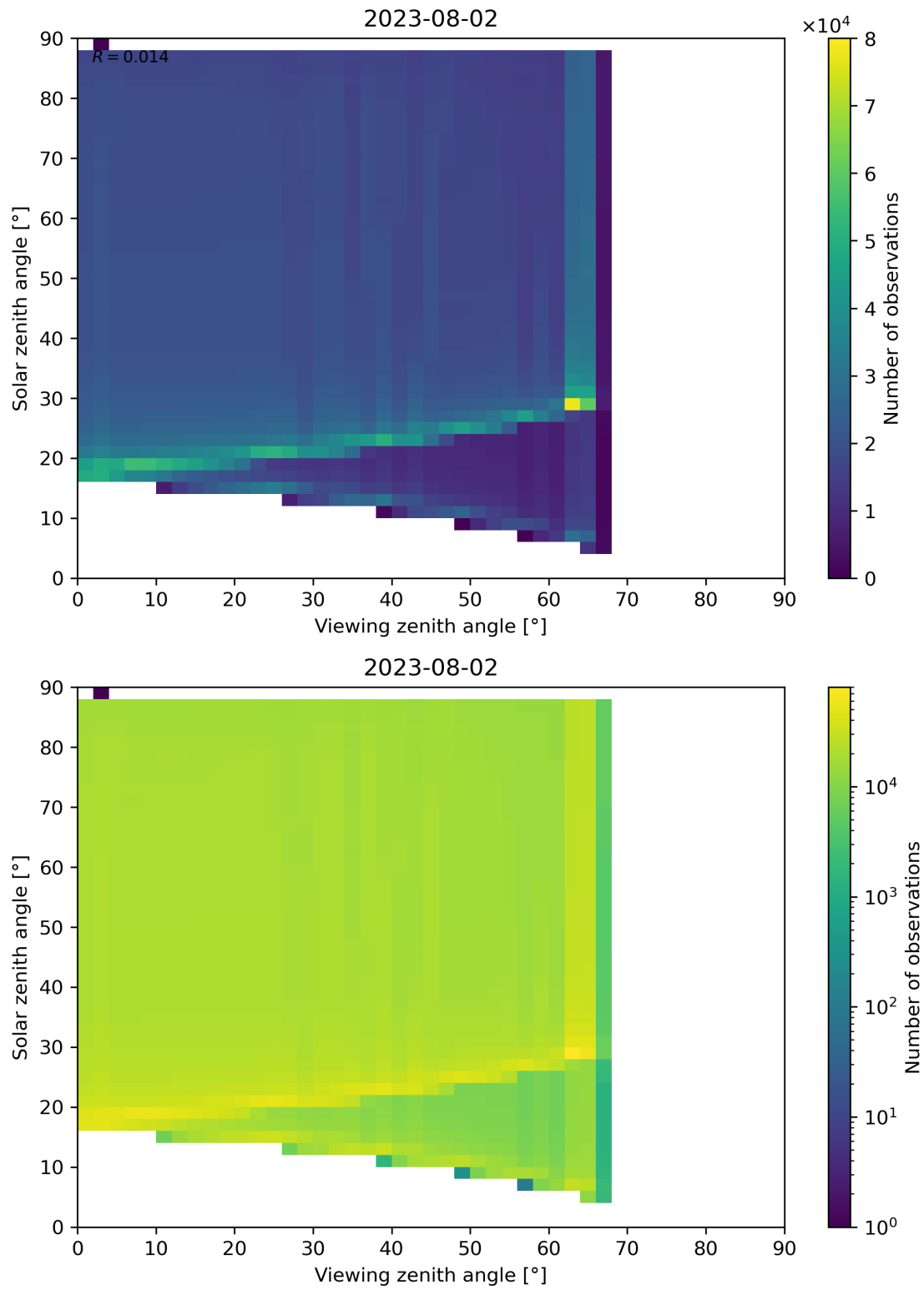
Figure 139: Scatter density plot of “Viewing zenith angle” against “Solar zenith angle” for 2023-08-01 to 2023-08-03.
