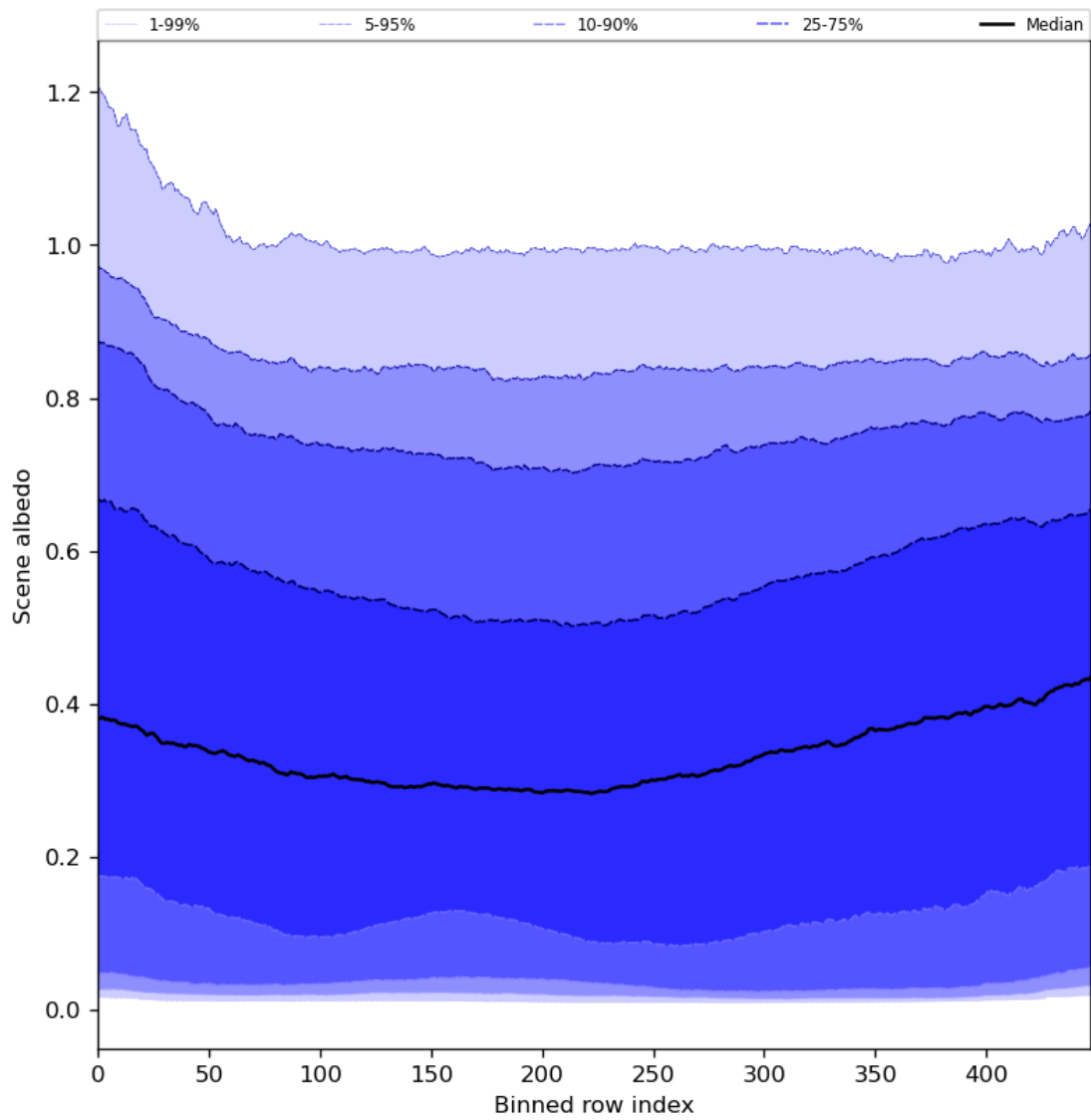
Figure 51: Along track statistics of “Scene albedo” for 2023-08-01 to 2023-08-03
