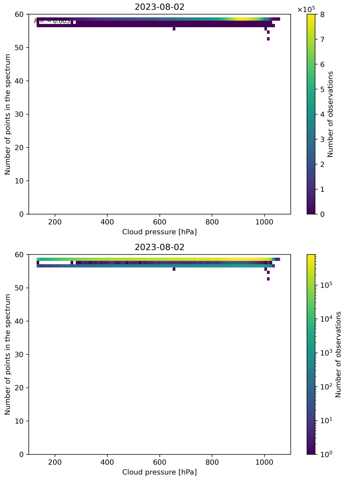
Figure 90: Scatter density plot of “Cloud pressure” against “Number of points in the spectrum” for 2023-08-01 to 2023-08-03.
