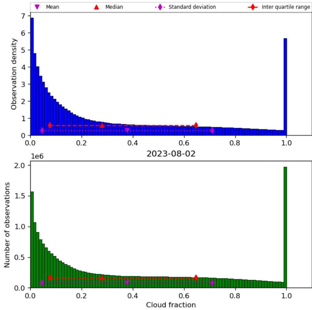
Figure 32: Histogram of “Cloud fraction” for 2023-08-01 to 2023-08-03
