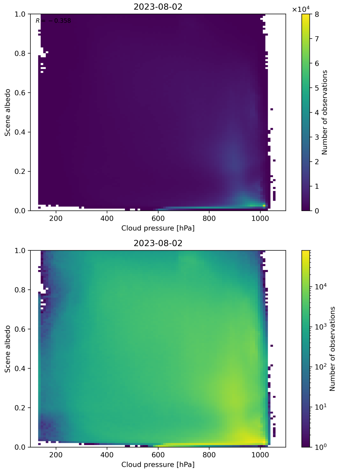
Figure 91: Scatter density plot of “Cloud pressure” against “Scene albedo” for 2023-08-01 to 2023-08-03.
