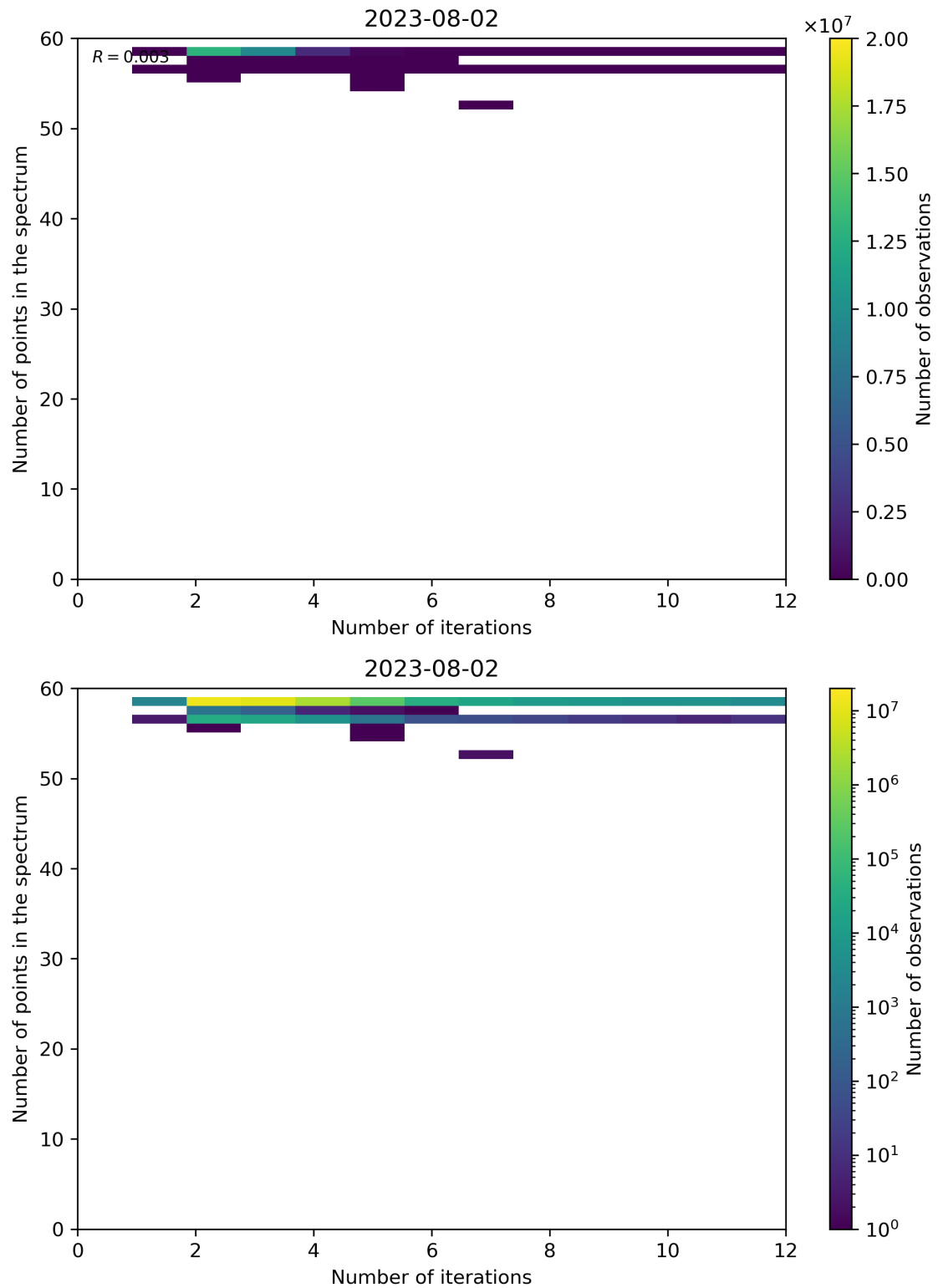
Figure 108: Scatter density plot of “Number of iterations” against “Number of points in the spectrum” for 2023-08-01 to 2023-08-03.
