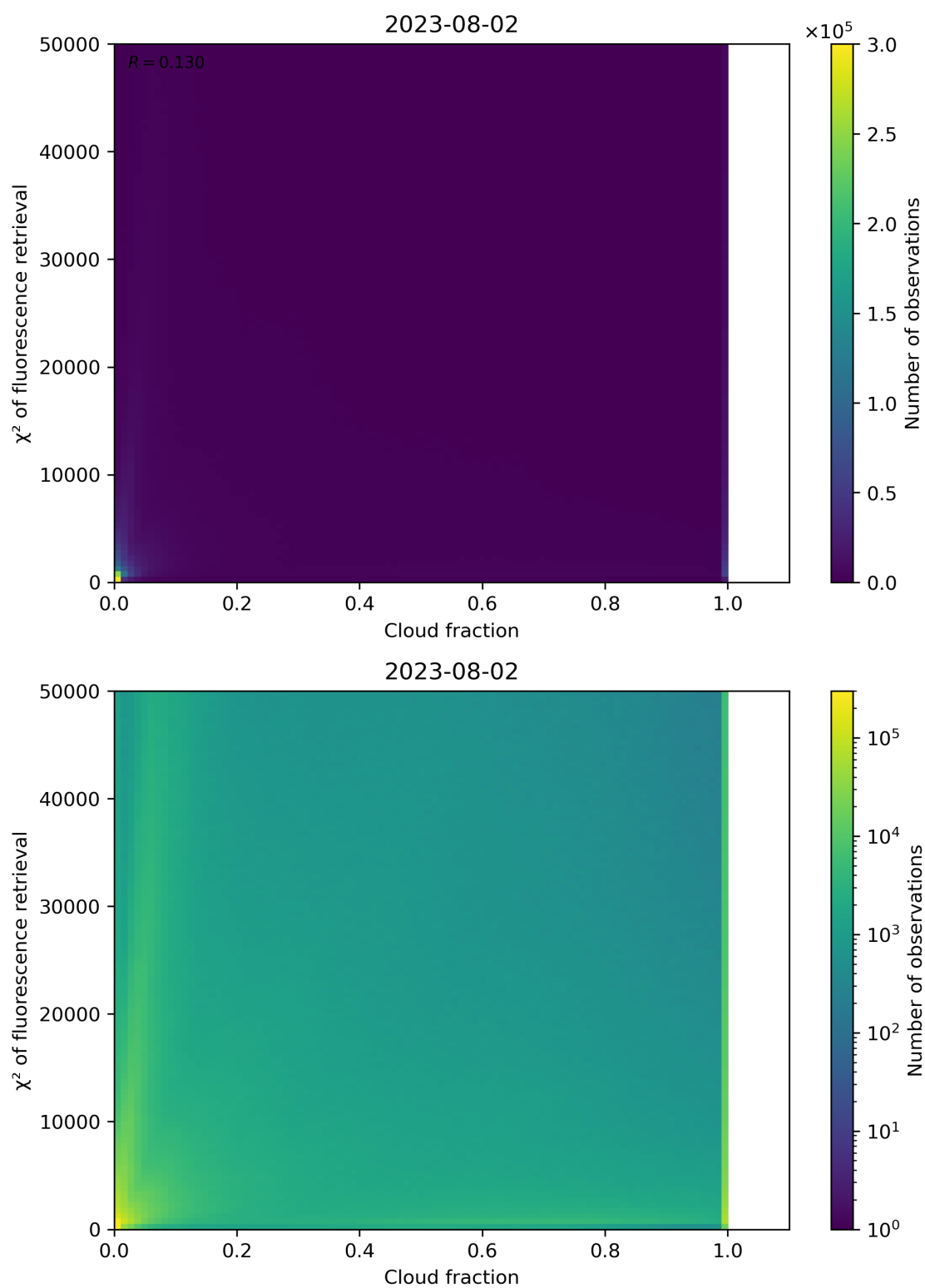
Figure 78: Scatter density plot of “Cloud fraction” against “ \chi^2 of fluorescence retrieval” for 2023-08-01 to 2023-08-03.
