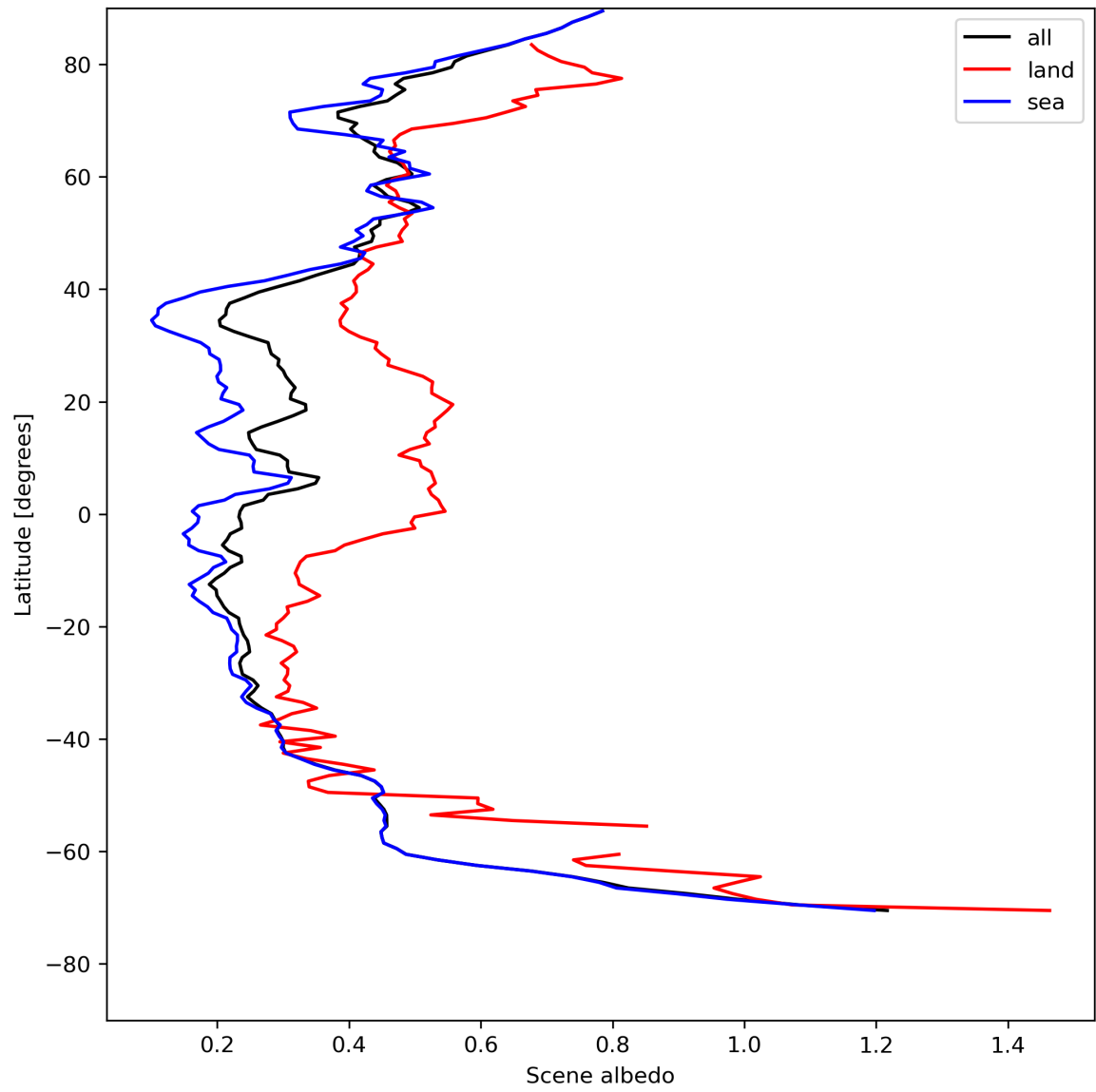
Figure 17: Zonal average of “Scene albedo” for 2023-08-01 to 2023-08-03.
