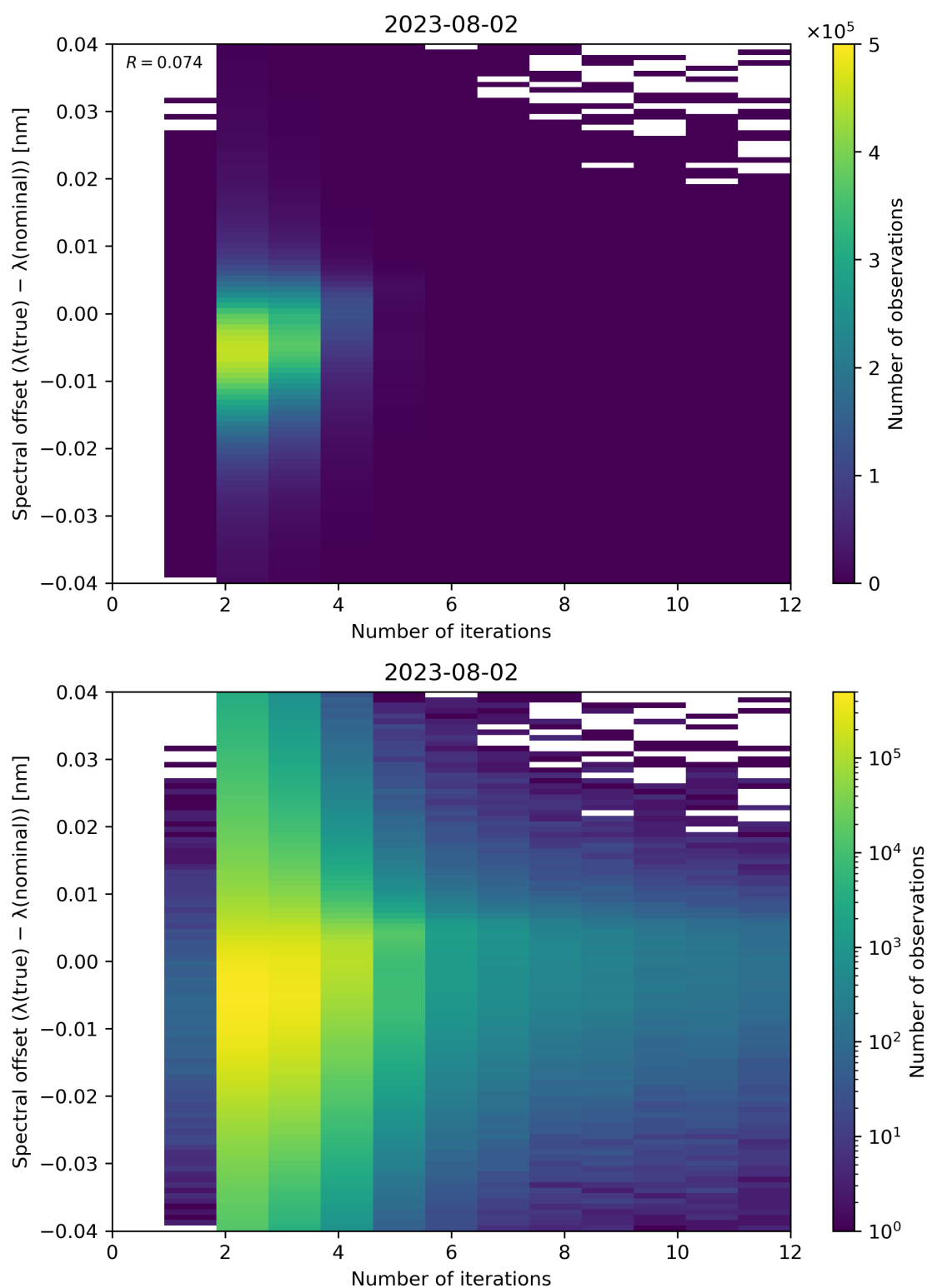
Figure 109: Scatter density plot of “Number of iterations” against “Spectral offset ( \lambda(\text{true}) - \lambda(\text{nominal}) )” for 2023-08-01 to 2023-08-03.
