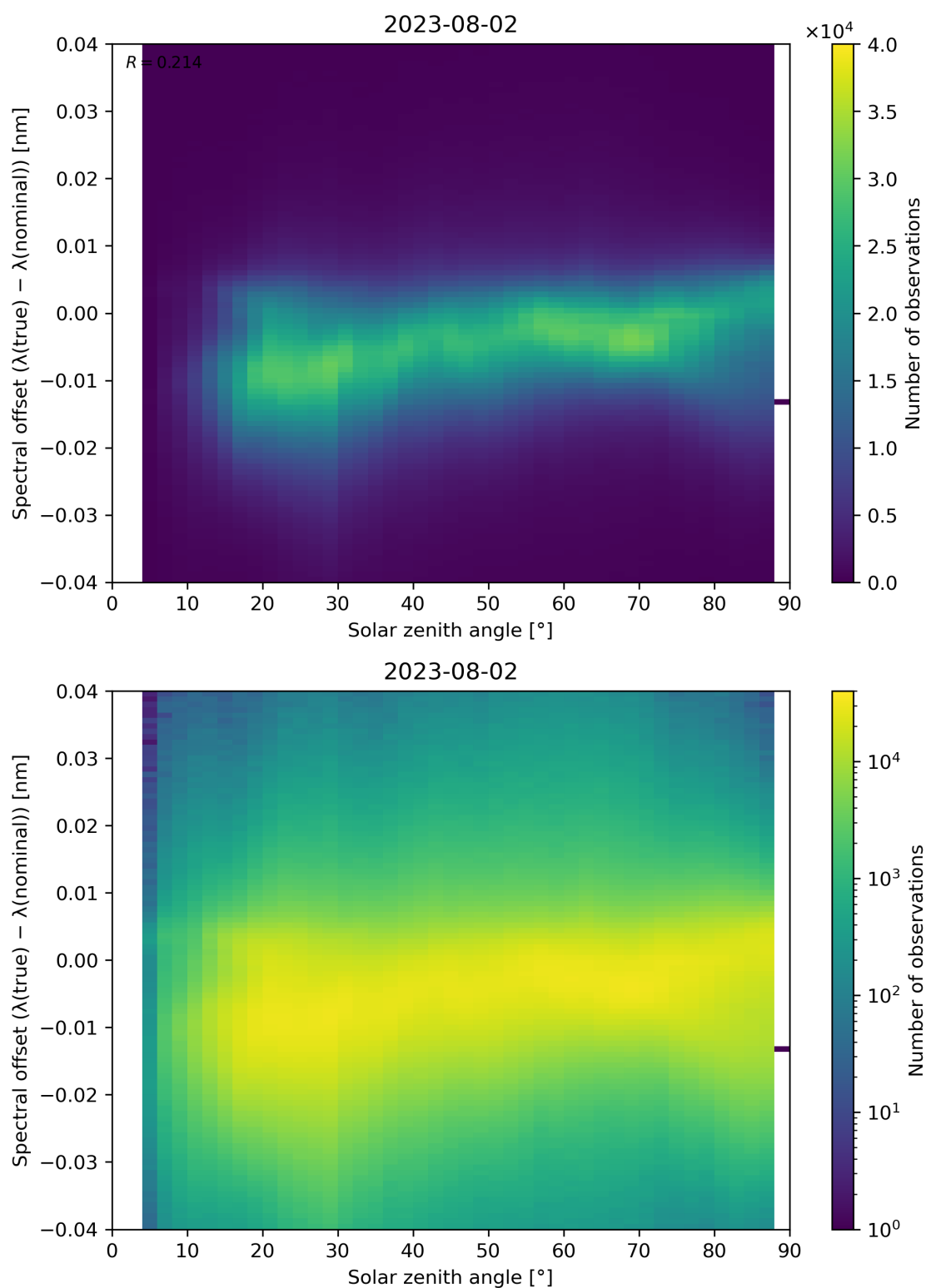
Figure 128: Scatter density plot of “Solar zenith angle” against “Spectral offset ( \lambda(\text{true}) - \lambda(\text{nominal}) )” for 2023-08-01 to 2023-08-03.
