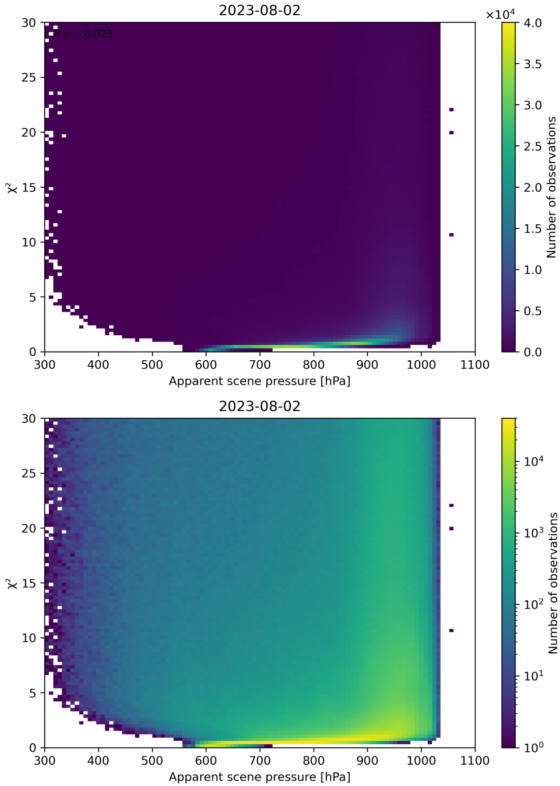
Figure 63: Scatter density plot of “Apparent scene pressure” against “ \chi^2 ” for 2023-08-01 to 2023-08-03.
