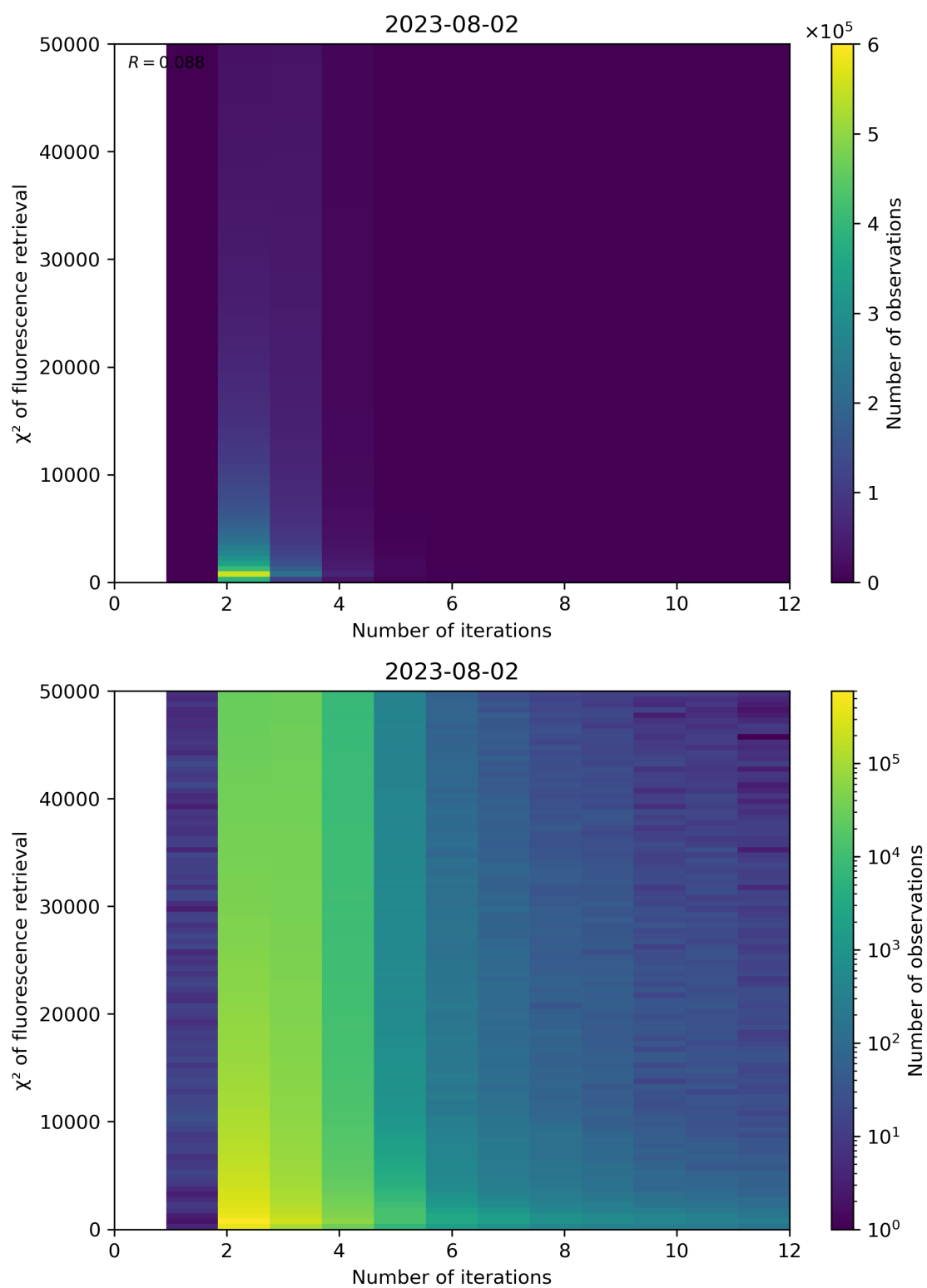
Figure 106: Scatter density plot of “Number of iterations” against “ \chi^2 of fluorescence retrieval” for 2023-08-01 to 2023-08-03.
