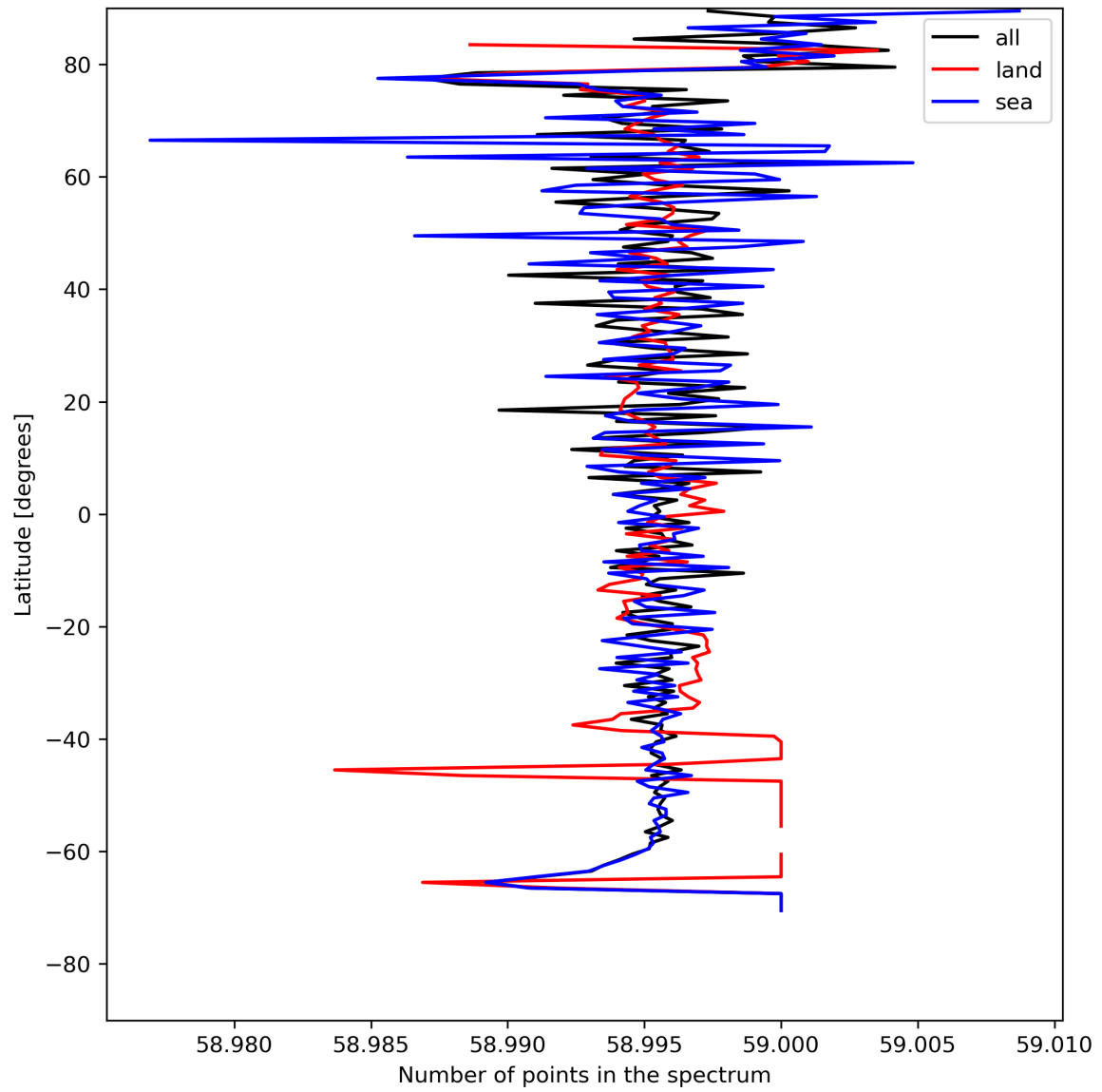
Figure 27: Zonal average of “Number of points in the spectrum” for 2023-08-01 to 2023-08-03.
