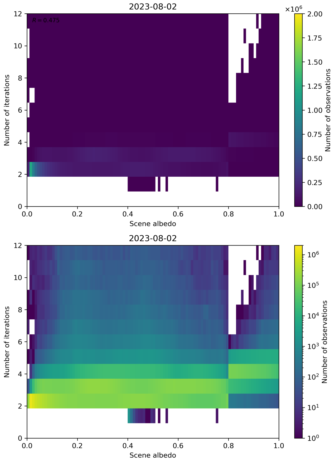
Figure 115: Scatter density plot of “Scene albedo” against “Number of iterations” for 2023-08-01 to 2023-08-03.
