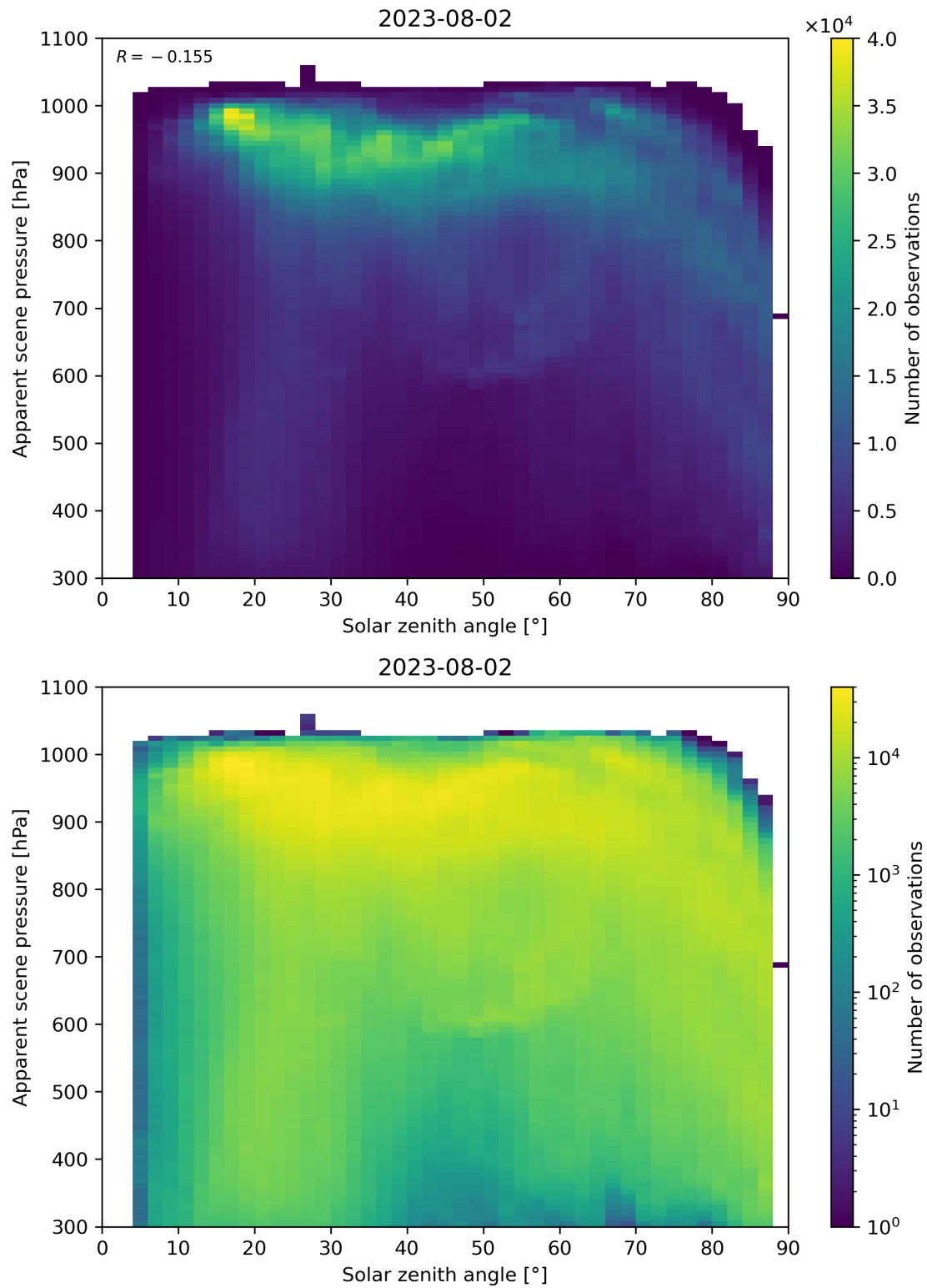
Figure 118: Scatter density plot of “Solar zenith angle” against “Apparent scene pressure” for 2023-08-01 to 2023-08-03.
