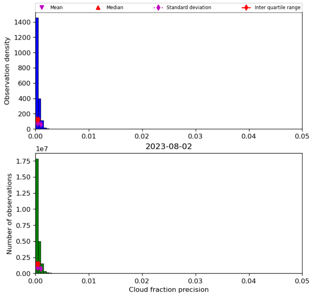
Figure 33: Histogram of “Cloud fraction precision” for 2023-08-01 to 2023-08-03
