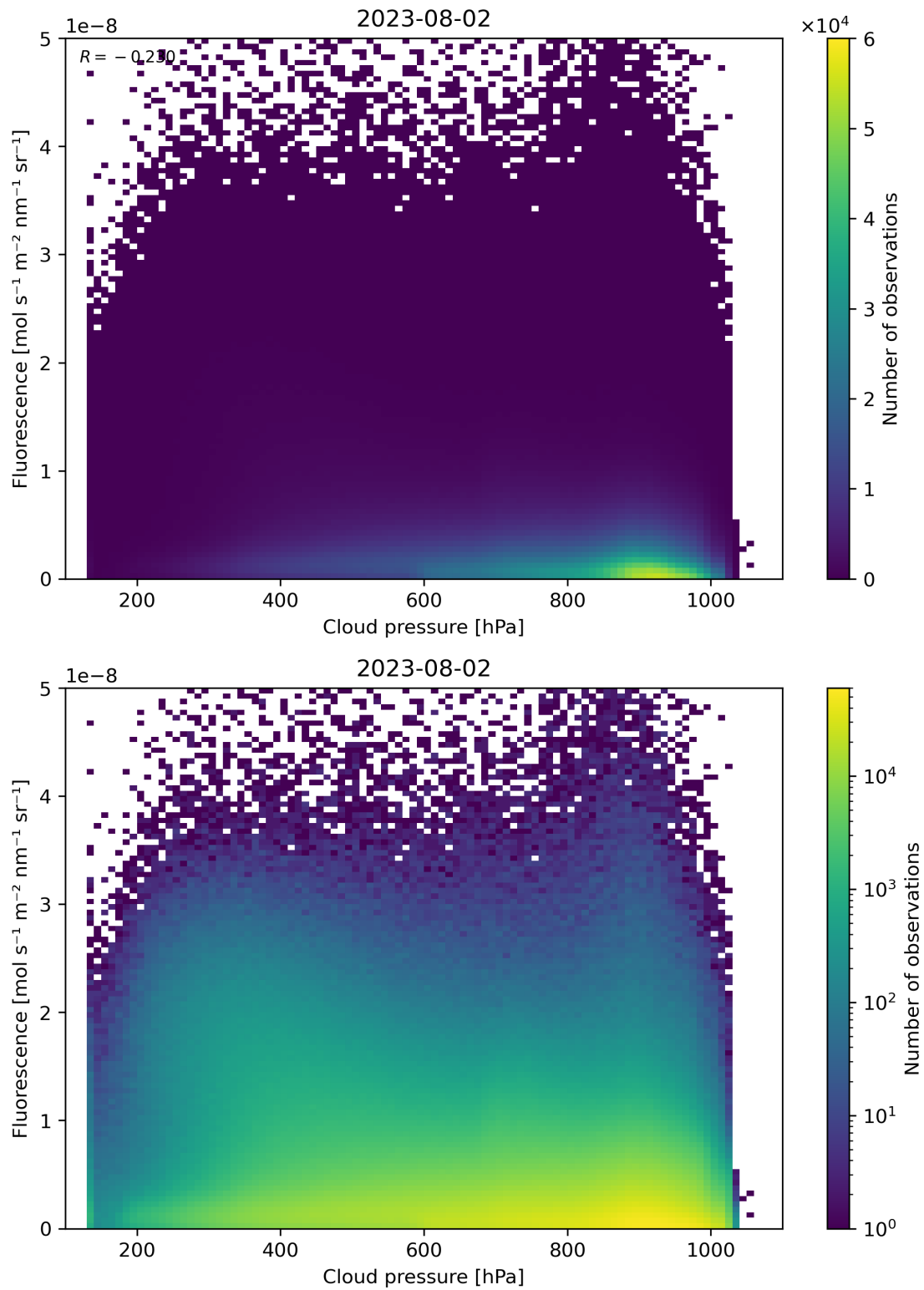
Figure 88: Scatter density plot of “Cloud pressure” against “Fluorescence” for 2023-08-01 to 2023-08-03.
