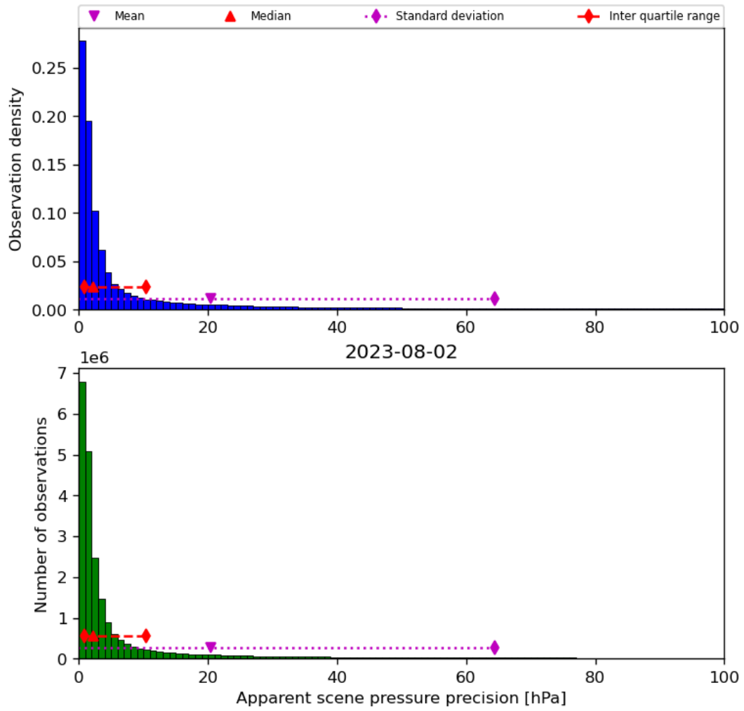
Figure 37: Histogram of “Apparent scene pressure precision” for 2023-08-01 to 2023-08-03
