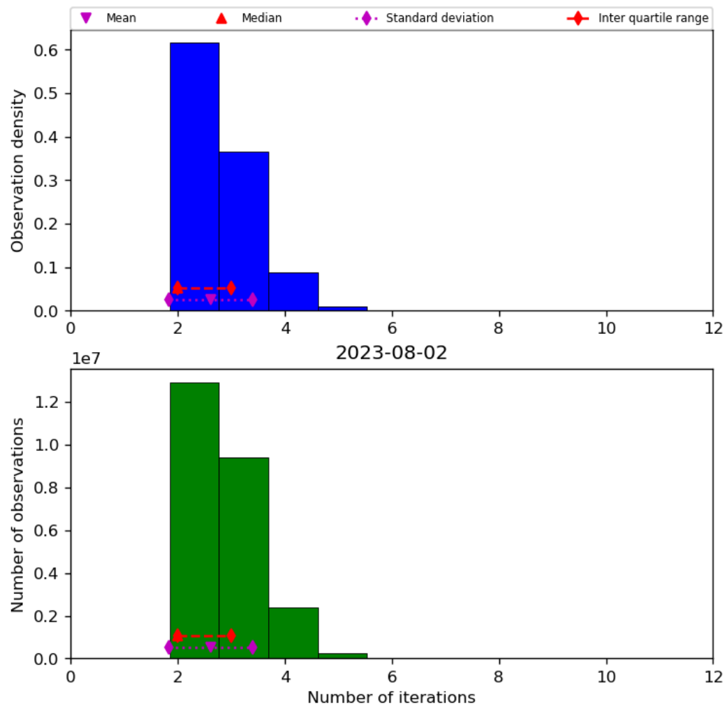
Figure 39: Histogram of “Number of iterations” for 2023-08-01 to 2023-08-03
