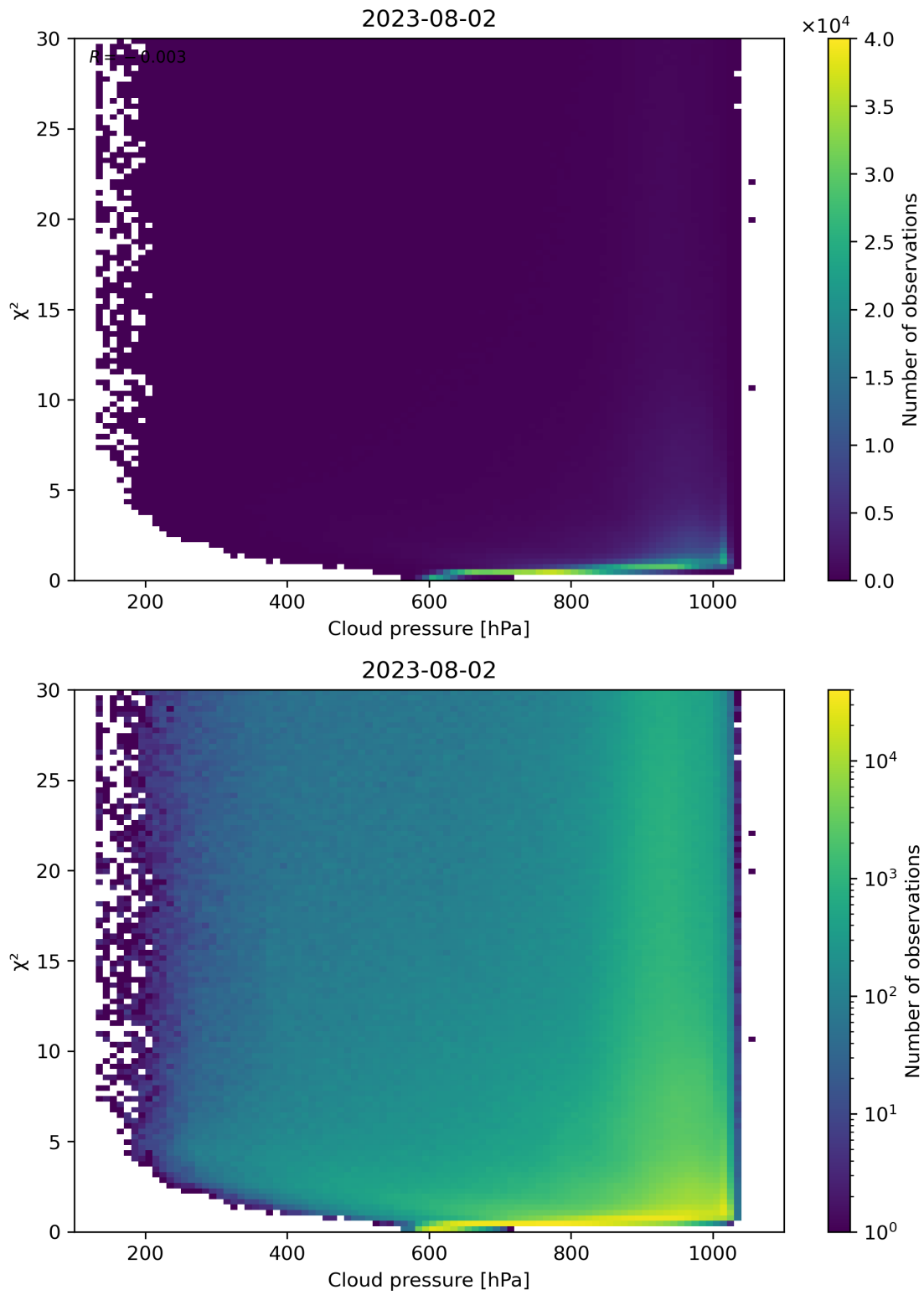
Figure 85: Scatter density plot of “Cloud pressure” against “ \chi^2 ” for 2023-08-01 to 2023-08-03.
