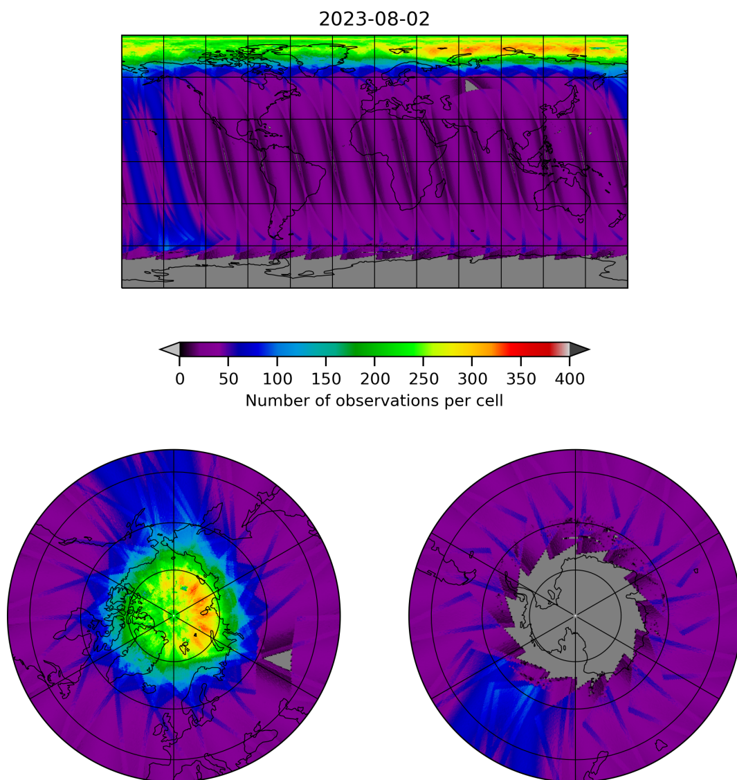
Figure 11: Map of the number of observations for 2023-08-01 to 2023-08-03
