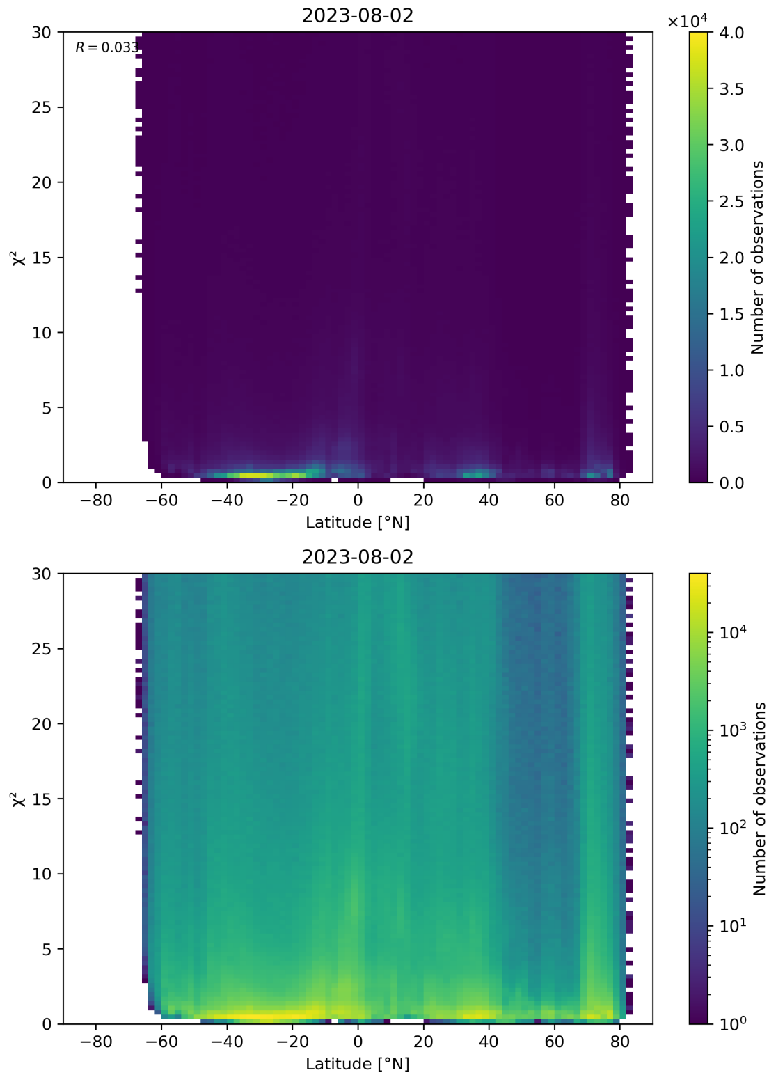
Figure 97: Scatter density plot of “Latitude” against “ \chi^2 ” for 2023-08-01 to 2023-08-03.
