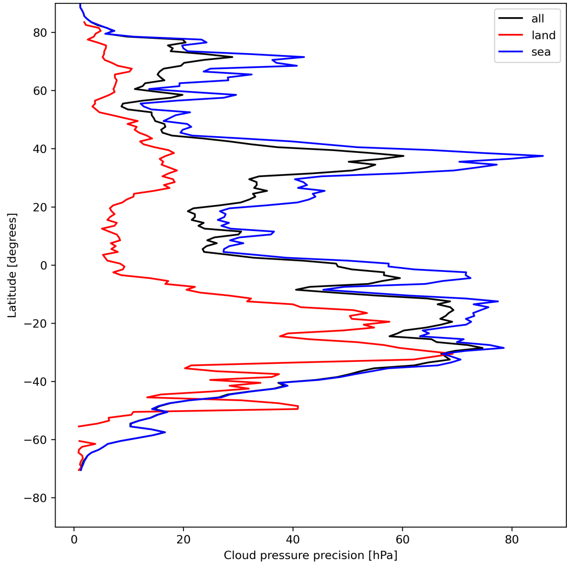
Figure 14: Zonal average of “Cloud pressure precision” for 2023-08-01 to 2023-08-03.
