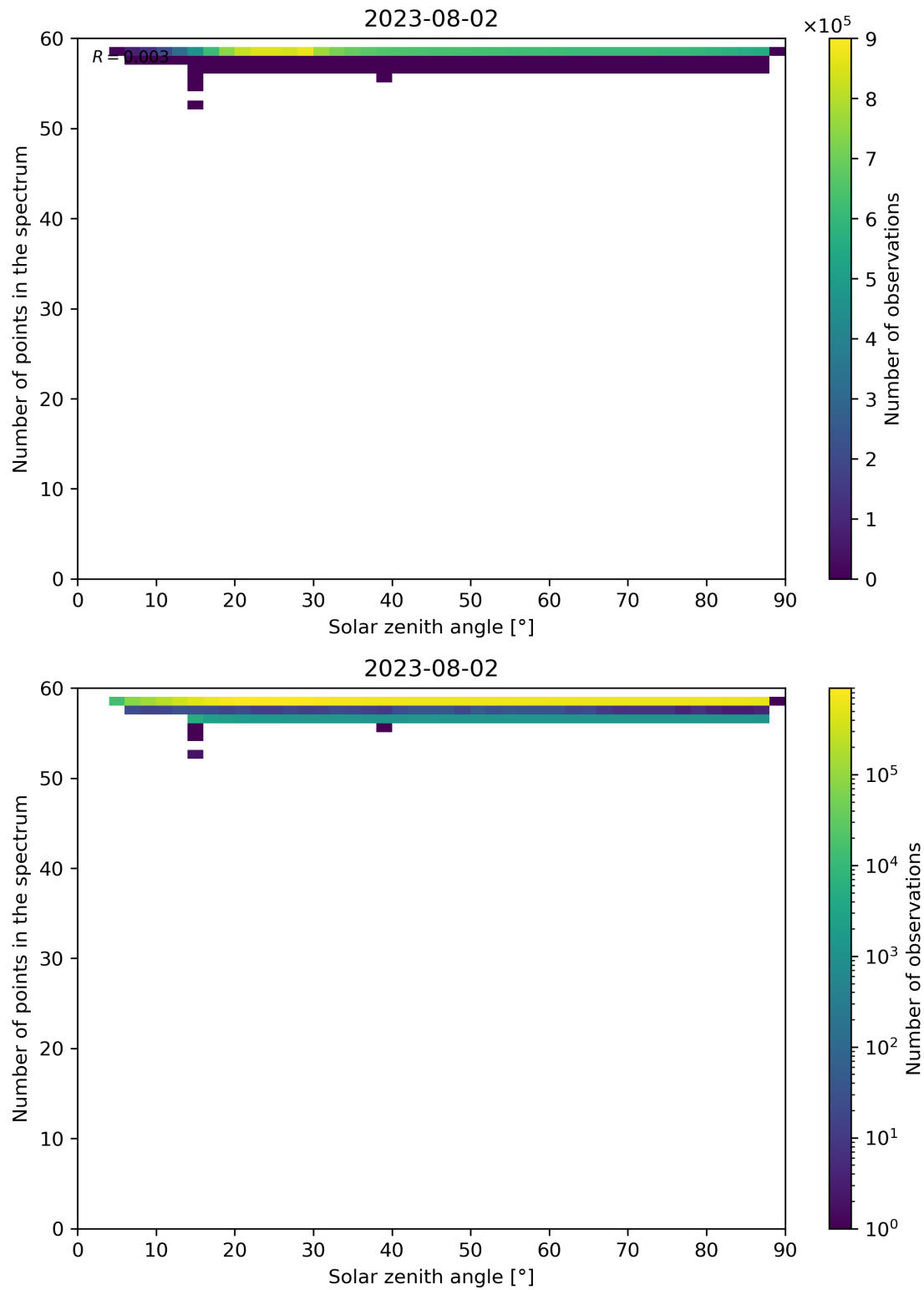
Figure 126: Scatter density plot of “Solar zenith angle” against “Number of points in the spectrum” for 2023-08-01 to 2023-08-03.
