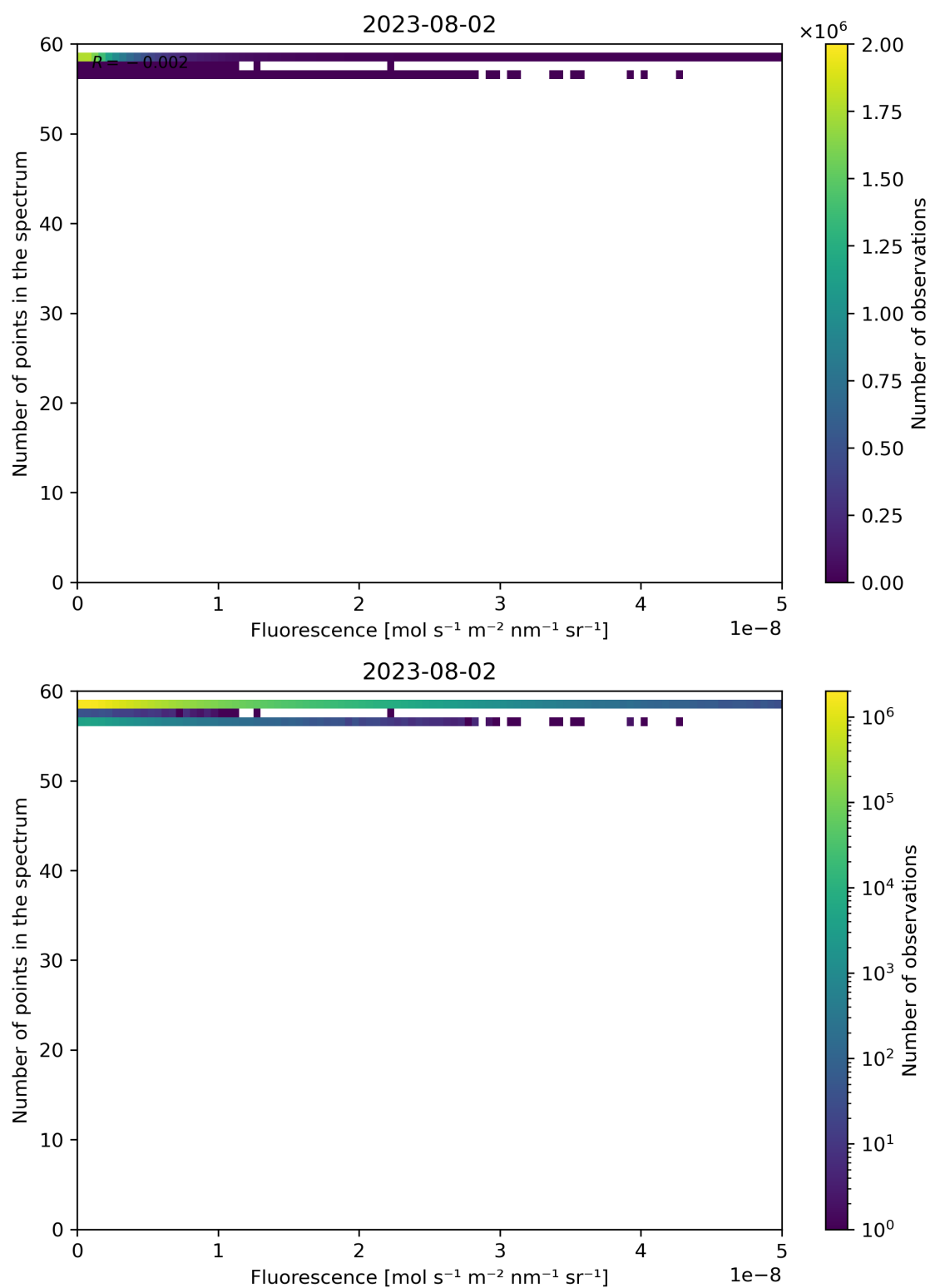
Figure 94: Scatter density plot of “Fluorescence” against “Number of points in the spectrum” for 2023-08-01 to 2023-08-03.
