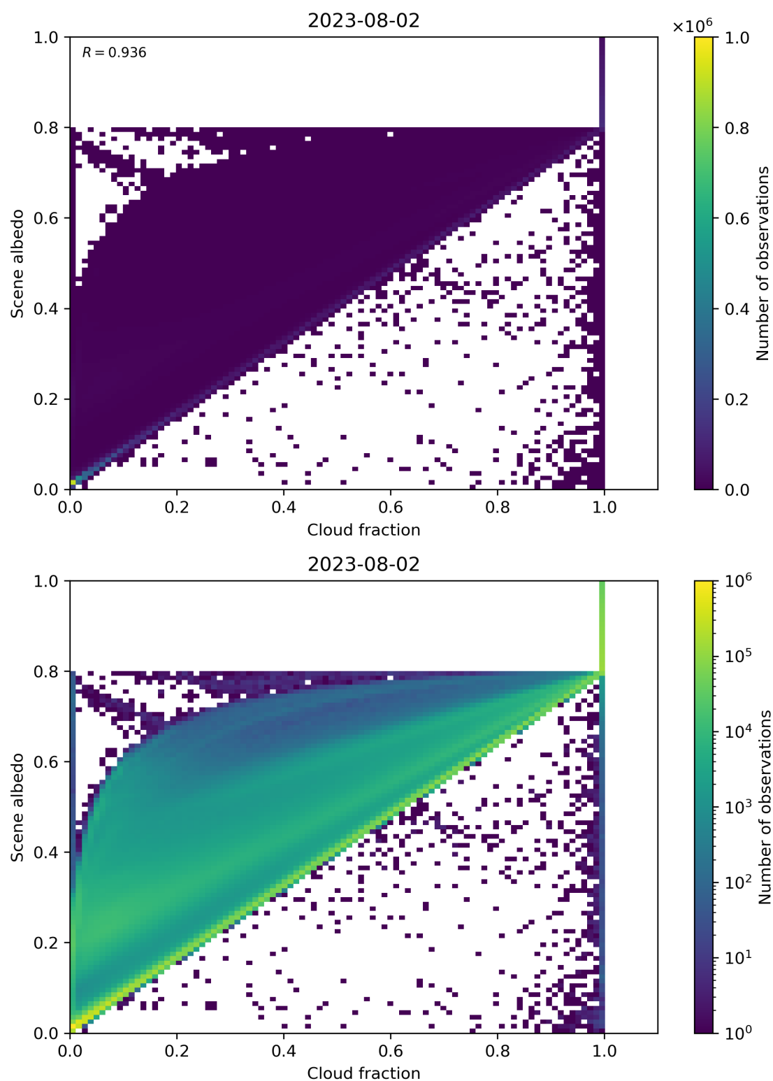
Figure 82: Scatter density plot of “Cloud fraction” against “Scene albedo” for 2023-08-01 to 2023-08-03.
