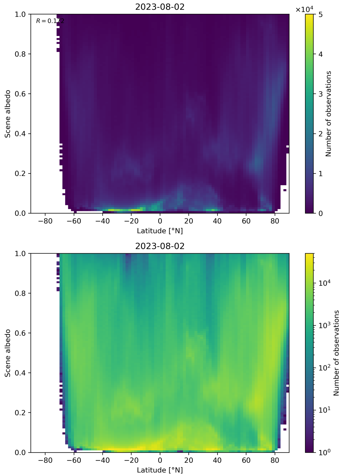
Figure 104: Scatter density plot of “Latitude” against “Scene albedo” for 2023-08-01 to 2023-08-03.
