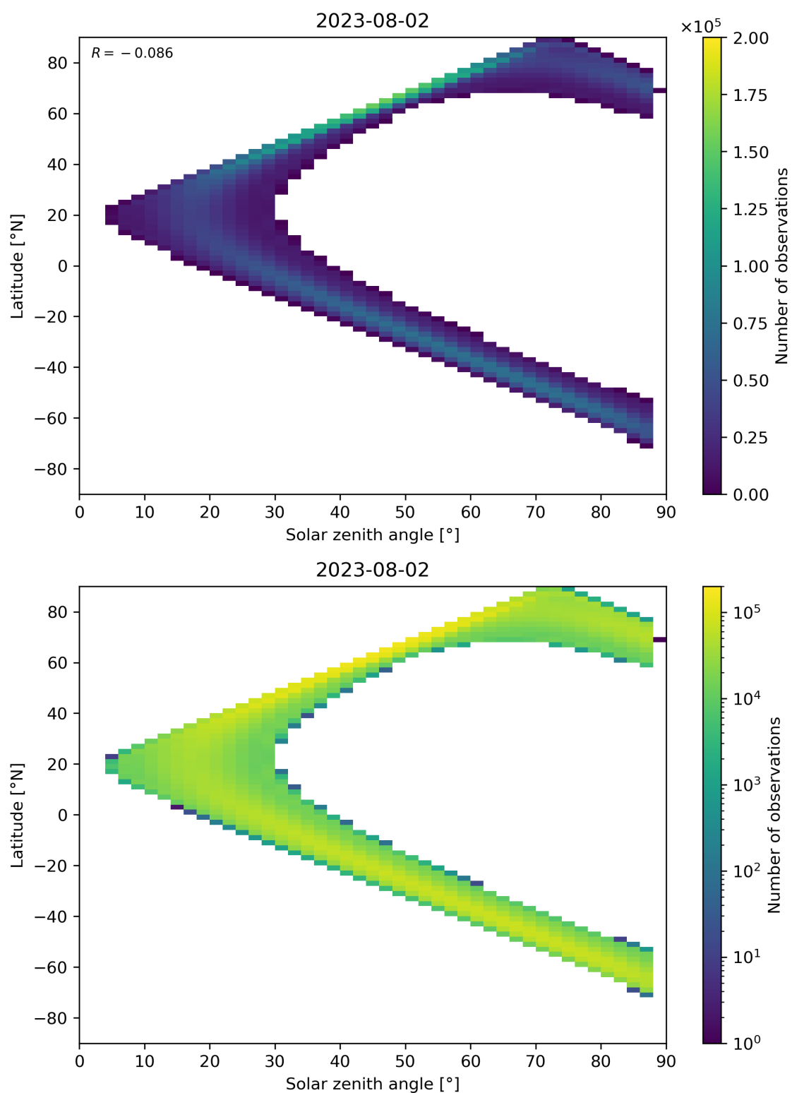
Figure 124: Scatter density plot of “Solar zenith angle” against “Latitude” for 2023-08-01 to 2023-08-03.
