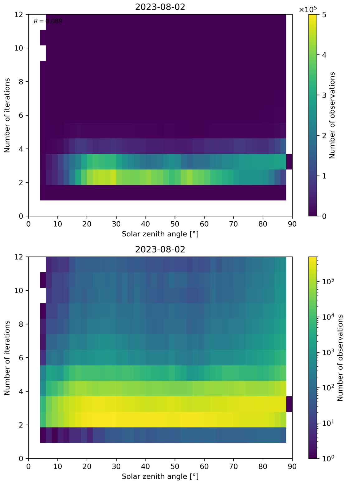
Figure 125: Scatter density plot of “Solar zenith angle” against “Number of iterations” for 2023-08-01 to 2023-08-03.
