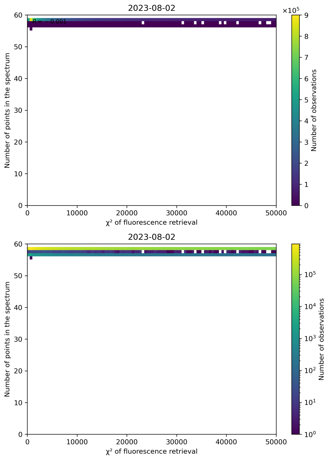
Figure 71: Scatter density plot of " \chi^2 of fluorescence retrieval" against "Number of points in the spectrum" for 2023-08-01 to 2023-08-03.
