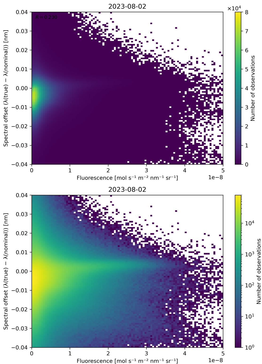
Figure 95: Scatter density plot of “Fluorescence” against “Spectral offset ( \lambda(\text{true}) - \lambda(\text{nominal}) )” for 2023-08-01 to 2023-08-03.
