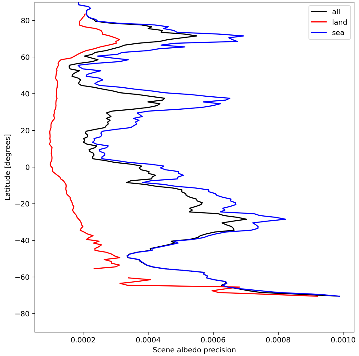
Figure 18: Zonal average of “Scene albedo precision” for 2023-08-01 to 2023-08-03.
