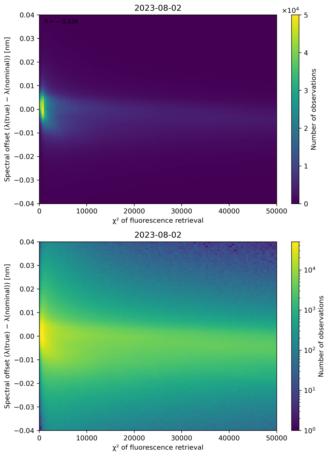
Figure 72: Scatter density plot of “ \chi^2 of fluorescence retrieval” against “Spectral offset ( \lambda(\text{true}) - \lambda(\text{nominal}) )” for 2023-08-01 to 2023-08-03.
