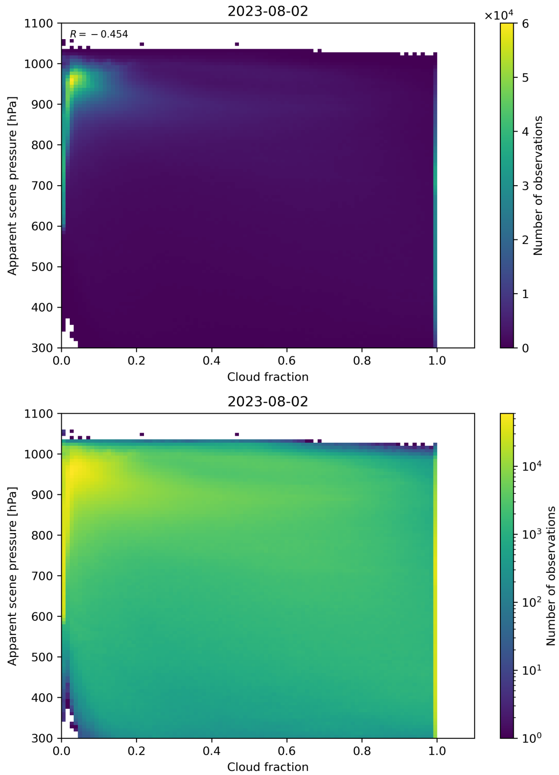
Figure 76: Scatter density plot of “Cloud fraction” against “Apparent scene pressure” for 2023-08-01 to 2023-08-03.
