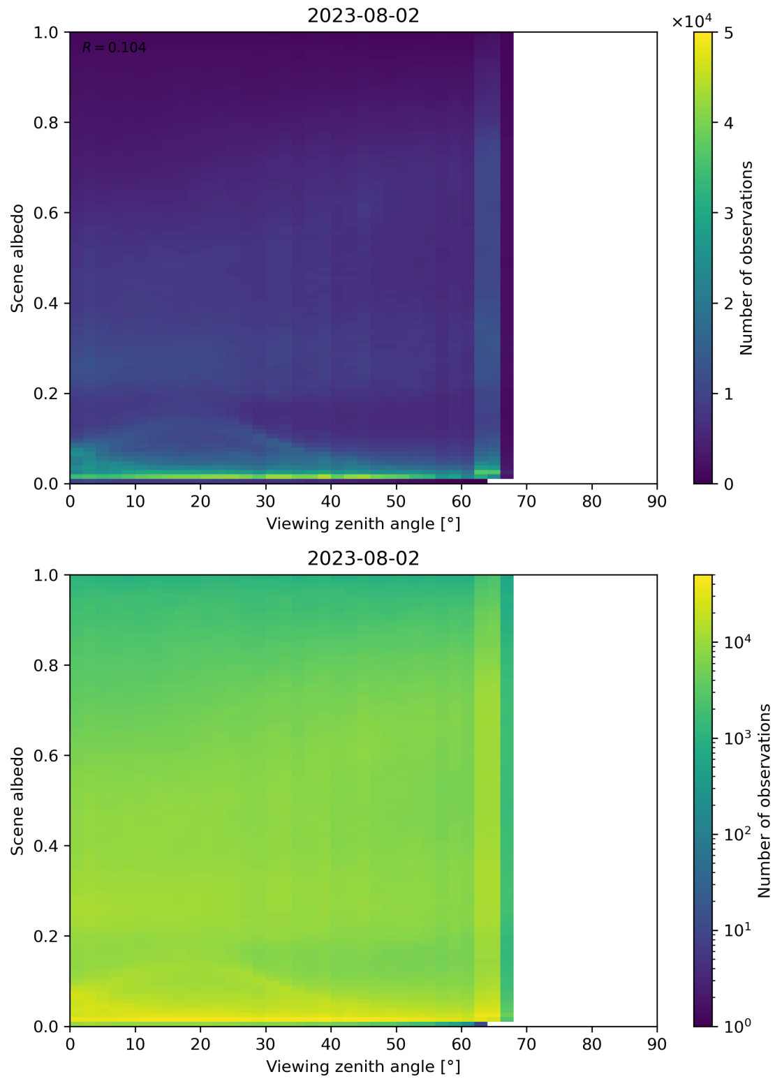
Figure 138: Scatter density plot of “Viewing zenith angle” against “Scene albedo” for 2023-08-01 to 2023-08-03.
