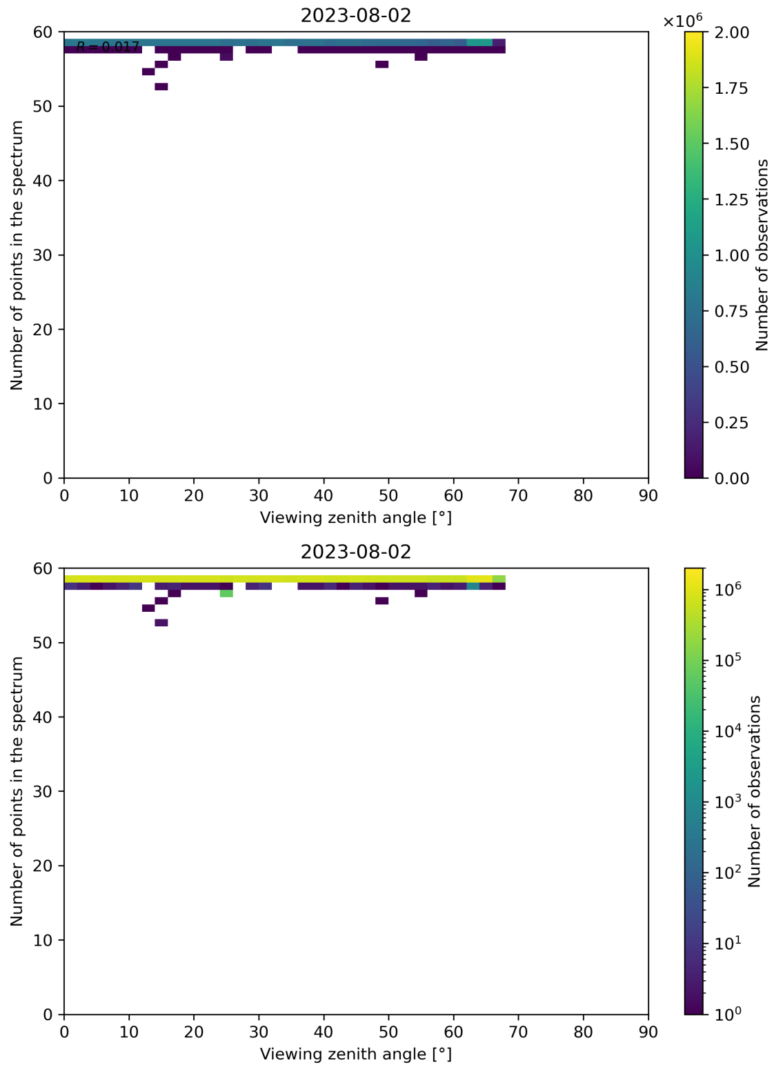
Figure 137: Scatter density plot of “Viewing zenith angle” against “Number of points in the spectrum” for 2023-08-01 to 2023-08-03.
