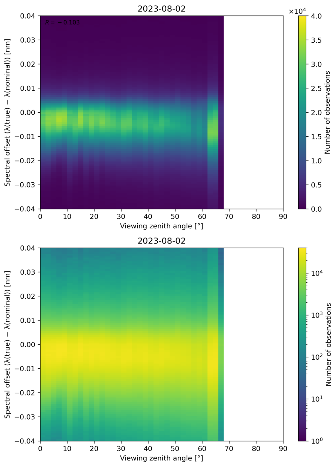
Figure 140: Scatter density plot of “Viewing zenith angle” against “Spectral offset ( \lambda(\text{true}) - \lambda(\text{nominal}) )” for 2023-08-01 to 2023-08-03.
