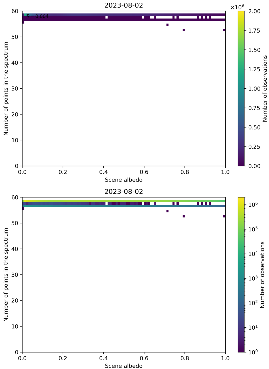
Figure 116: Scatter density plot of “Scene albedo” against “Number of points in the spectrum” for 2023-08-01 to 2023-08-03.
