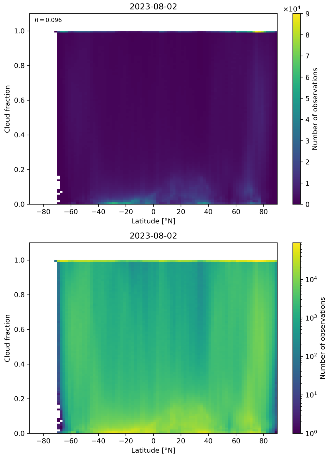
Figure 99: Scatter density plot of “Latitude” against “Cloud fraction” for 2023-08-01 to 2023-08-03.
