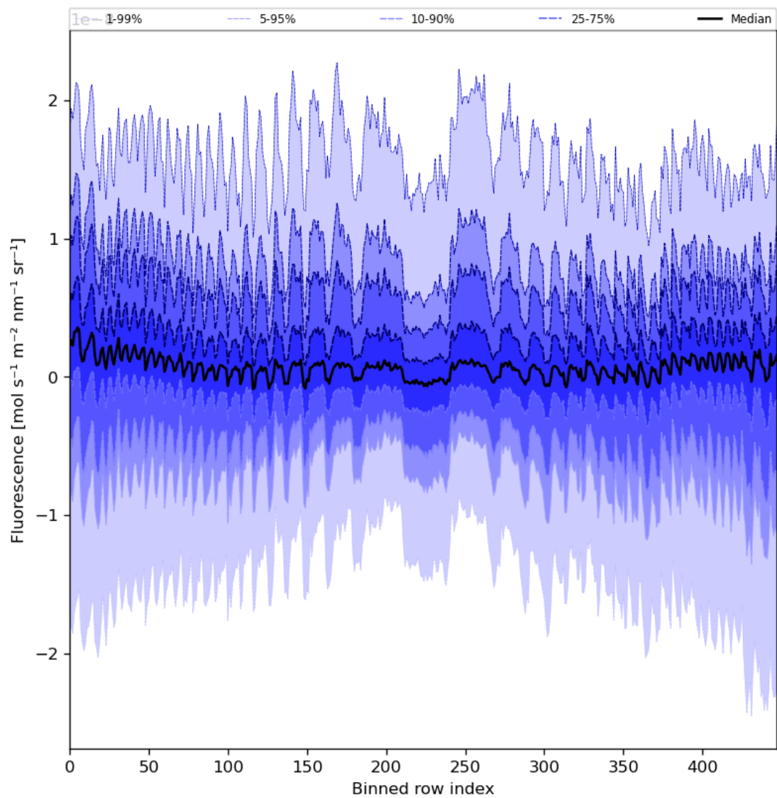
Figure 57: Along track statistics of "Fluorescence" for 2023-08-01 to 2023-08-03
