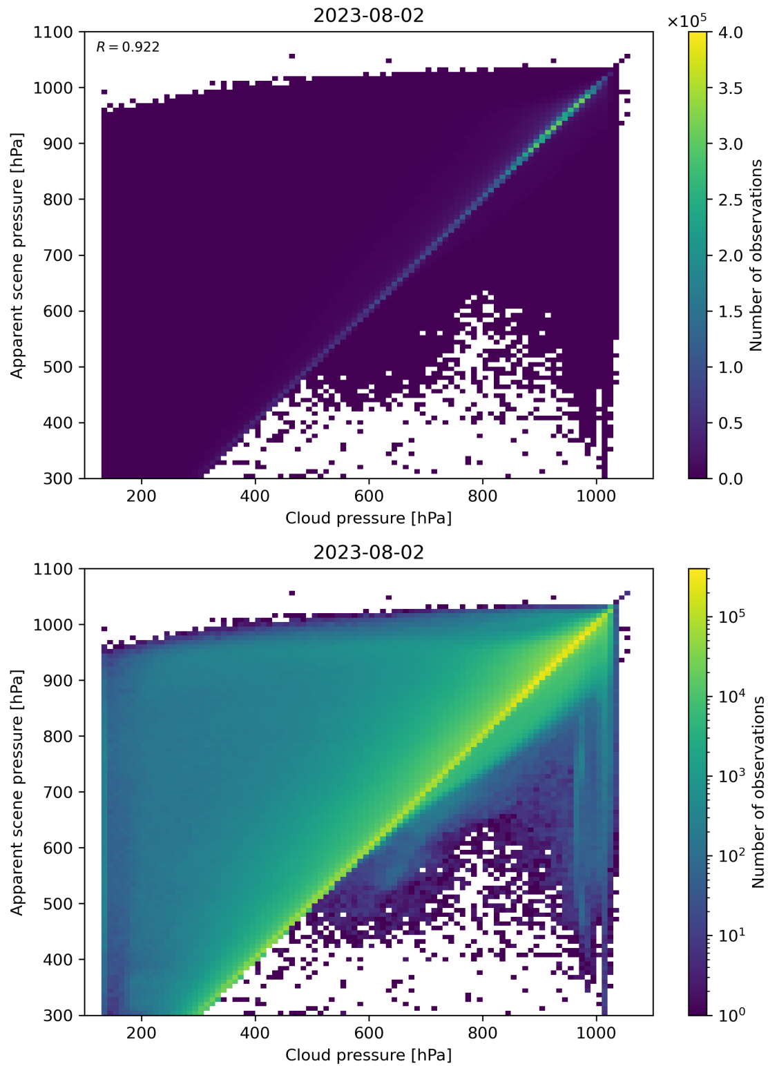
Figure 84: Scatter density plot of “Cloud pressure” against “Apparent scene pressure” for 2023-08-01 to 2023-08-03.
