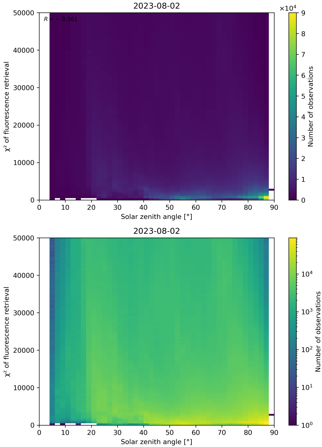
Figure 120: Scatter density plot of “Solar zenith angle” against “ \chi^2 of fluorescence retrieval” for 2023-08-01 to 2023-08-03.
