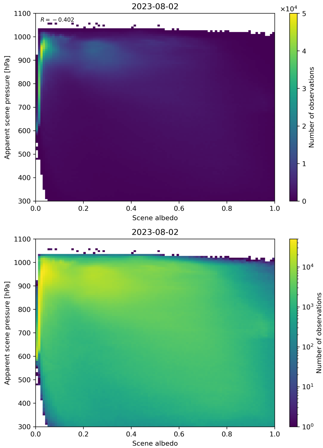
Figure 111: Scatter density plot of “Scene albedo” against “Apparent scene pressure” for 2023-08-01 to 2023-08-03.
