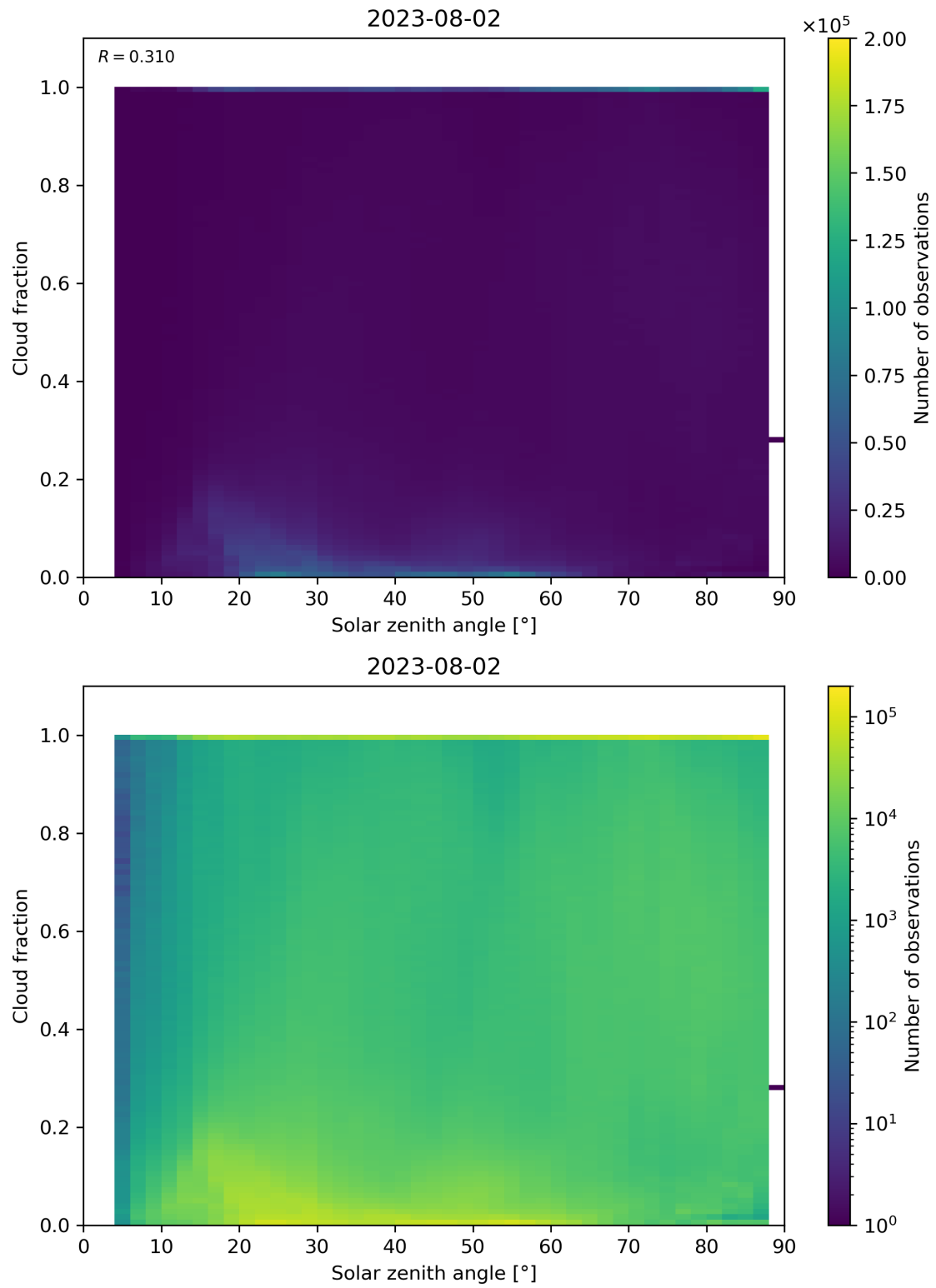
Figure 121: Scatter density plot of “Solar zenith angle” against “Cloud fraction” for 2023-08-01 to 2023-08-03.
