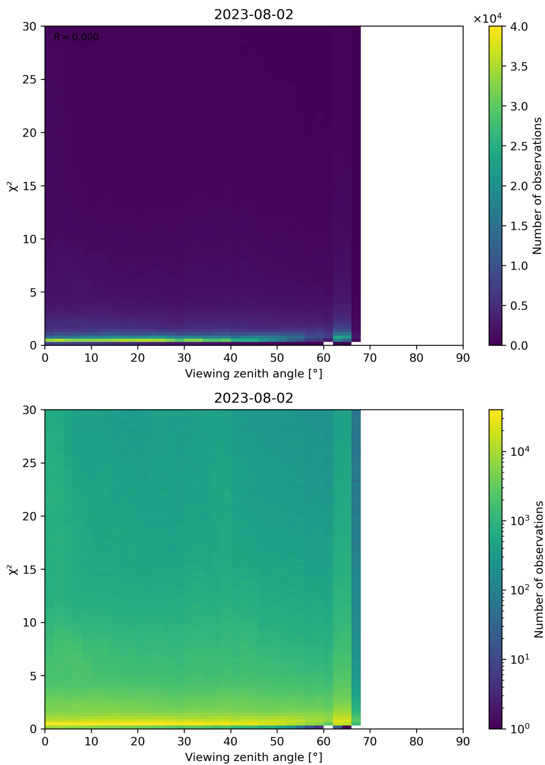
Figure 130: Scatter density plot of “Viewing zenith angle” against “ \chi^2 ” for 2023-08-01 to 2023-08-03.
