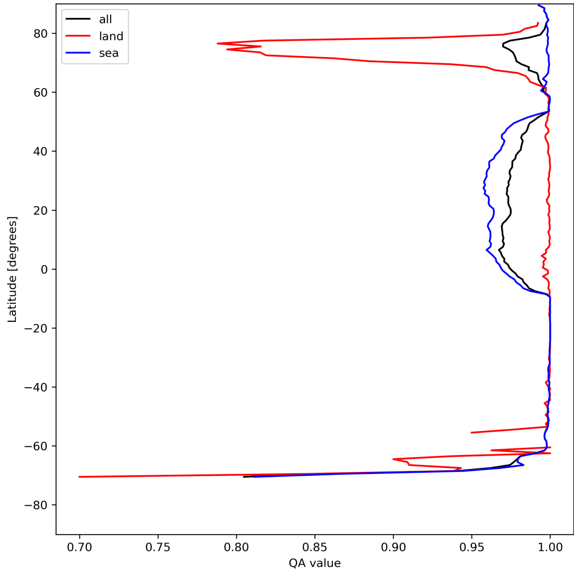
Figure 12: Zonal average of “QA value” for 2023-08-01 to 2023-08-03.
