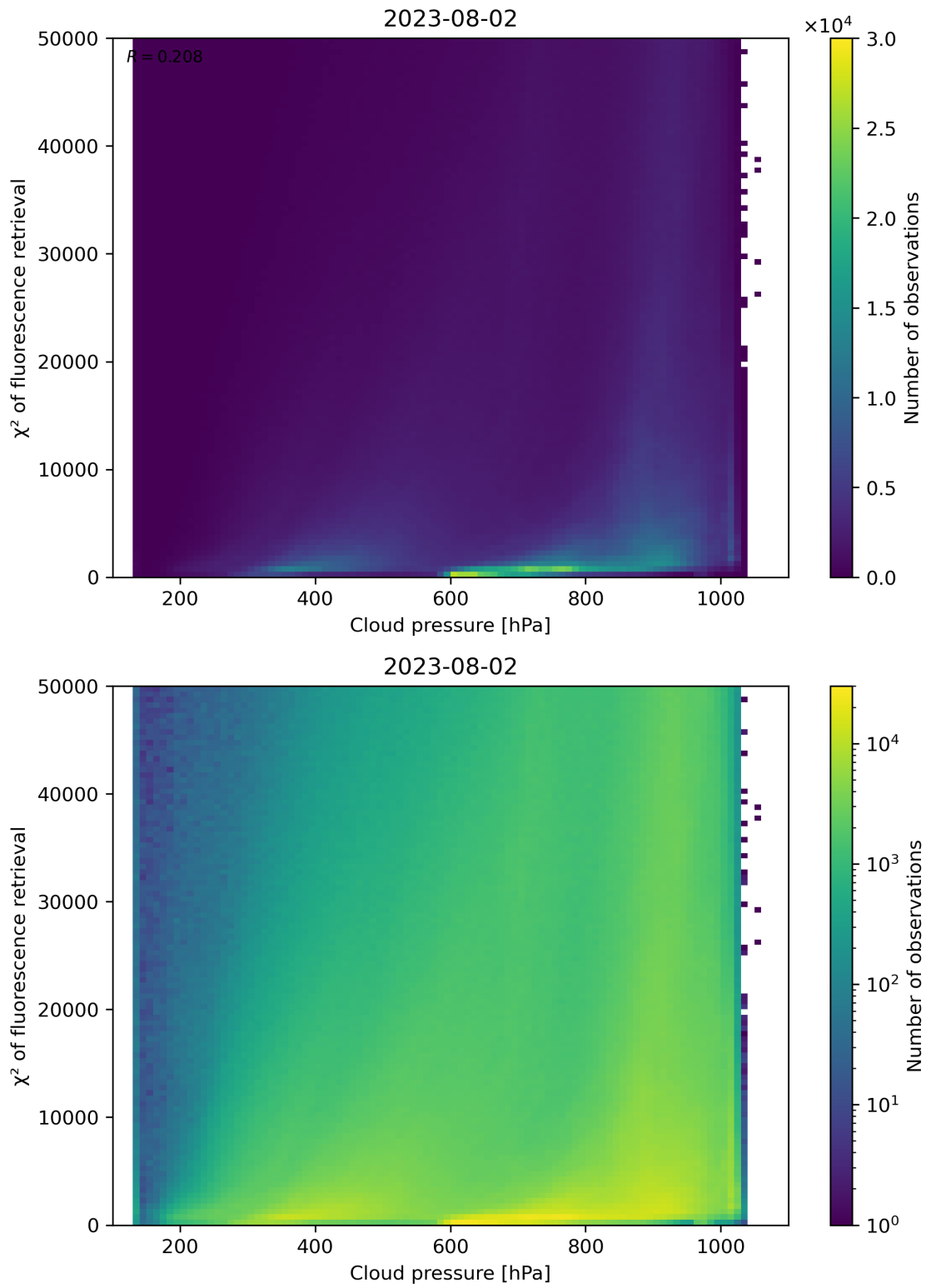
Figure 86: Scatter density plot of “Cloud pressure” against “ \chi^2 of fluorescence retrieval” for 2023-08-01 to 2023-08-03.
