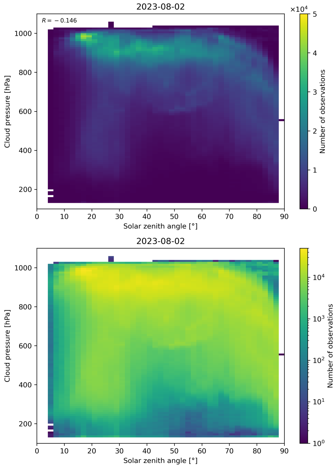
Figure 122: Scatter density plot of “Solar zenith angle” against “Cloud pressure” for 2023-08-01 to 2023-08-03.
