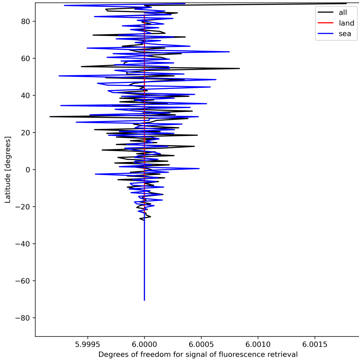
Figure 26: Zonal average of “Degrees of freedom for signal of fluorescence retrieval” for 2023-08-01 to 2023-08-03.
