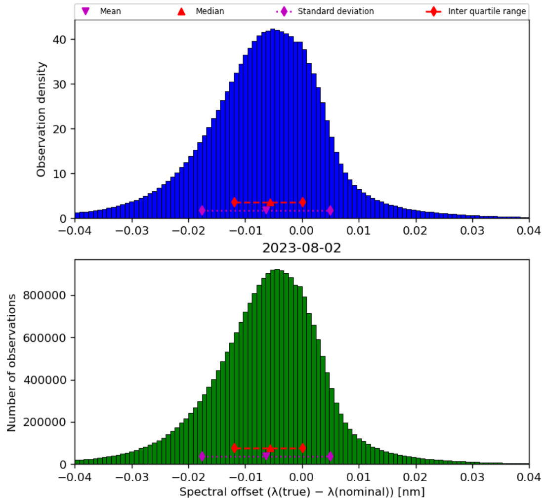
Figure 45: Histogram of “Spectral offset ( \lambda(\text{true}) - \lambda(\text{nominal}) )” for 2023-08-01 to 2023-08-03
