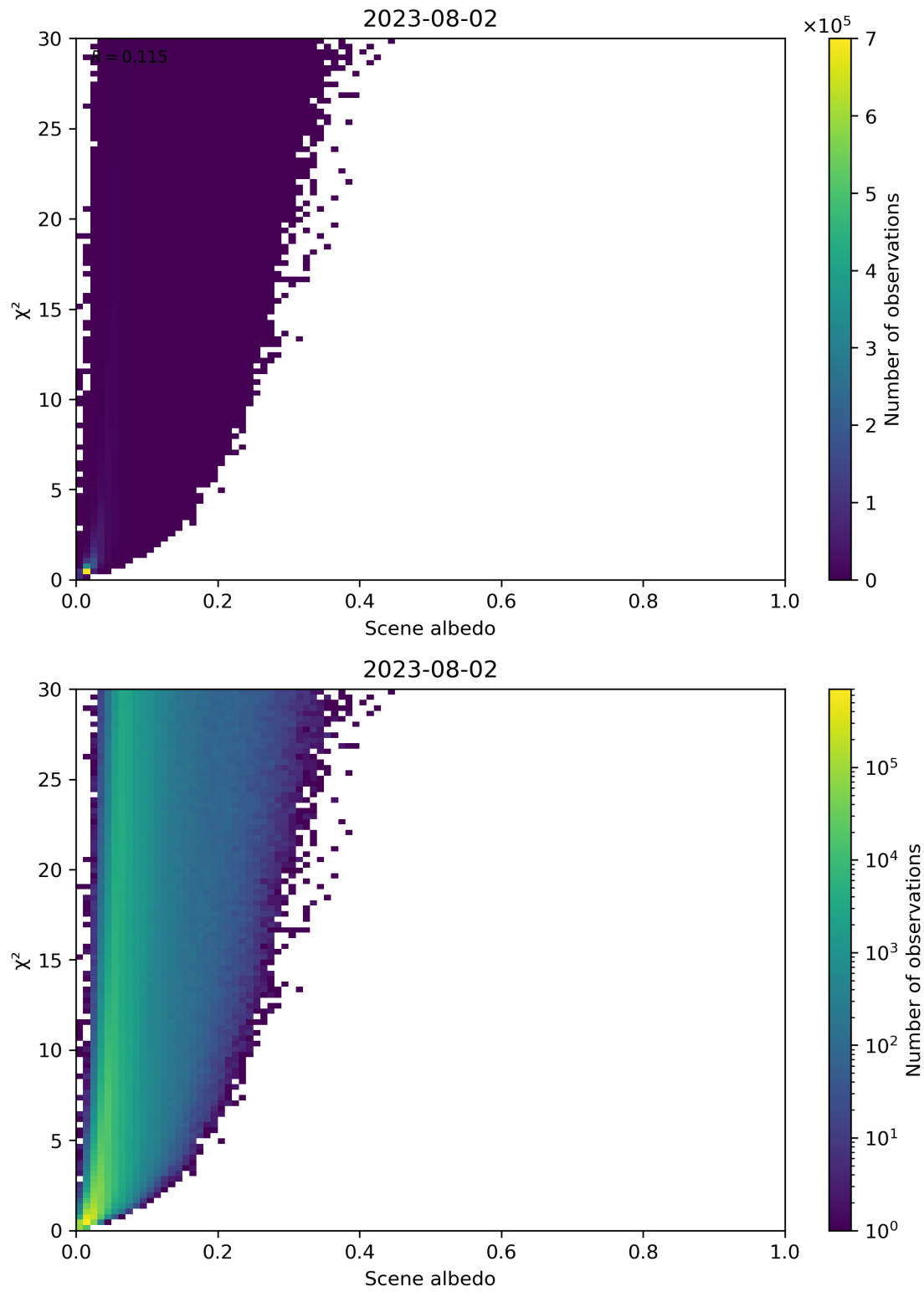
Figure 112: Scatter density plot of “Scene albedo” against “ \chi^2 ” for 2023-08-01 to 2023-08-03.
