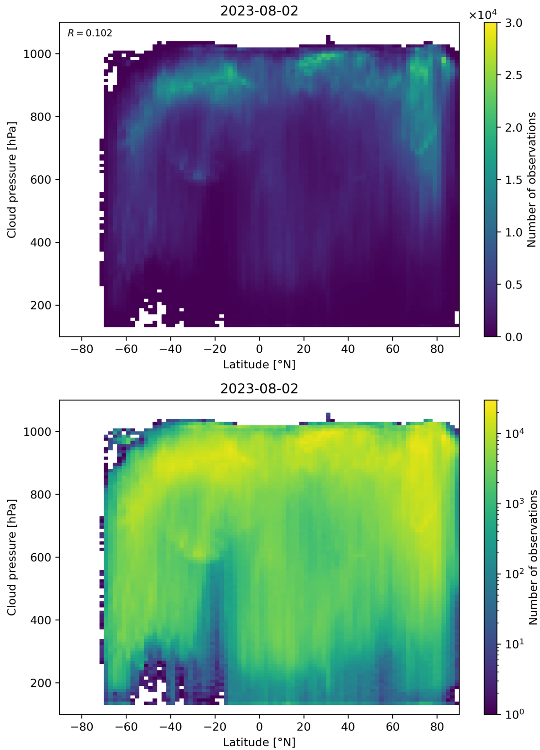
Figure 100: Scatter density plot of “Latitude” against “Cloud pressure” for 2023-08-01 to 2023-08-03.
