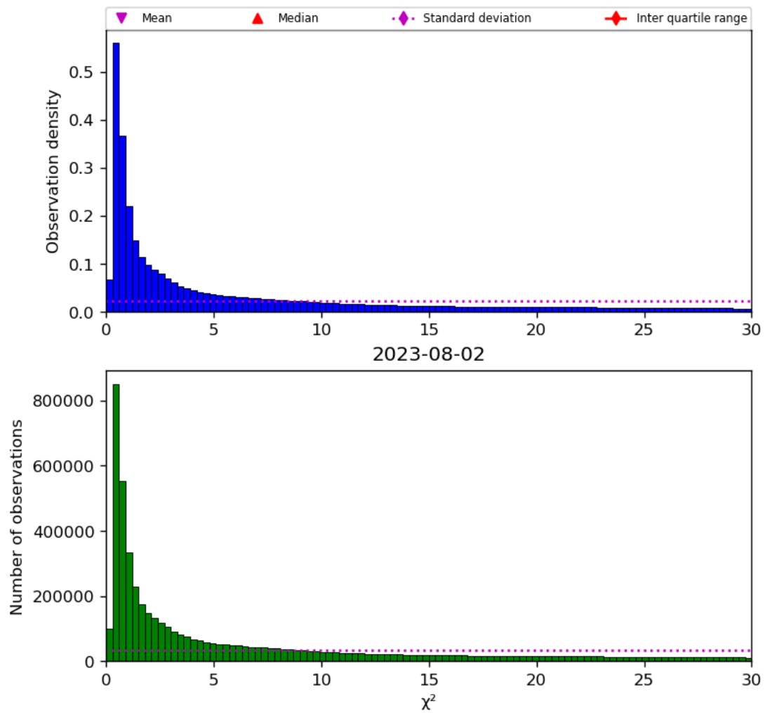
Figure 38: Histogram of “ \chi^2 ” for 2023-08-01 to 2023-08-03
