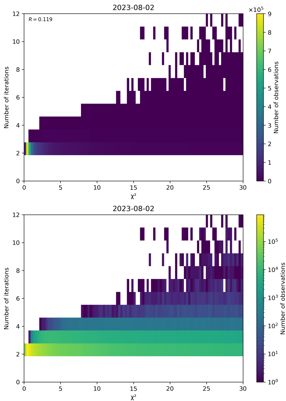
Figure 73: Scatter density plot of " \chi^2 " against "Number of iterations" for 2023-08-01 to 2023-08-03.
