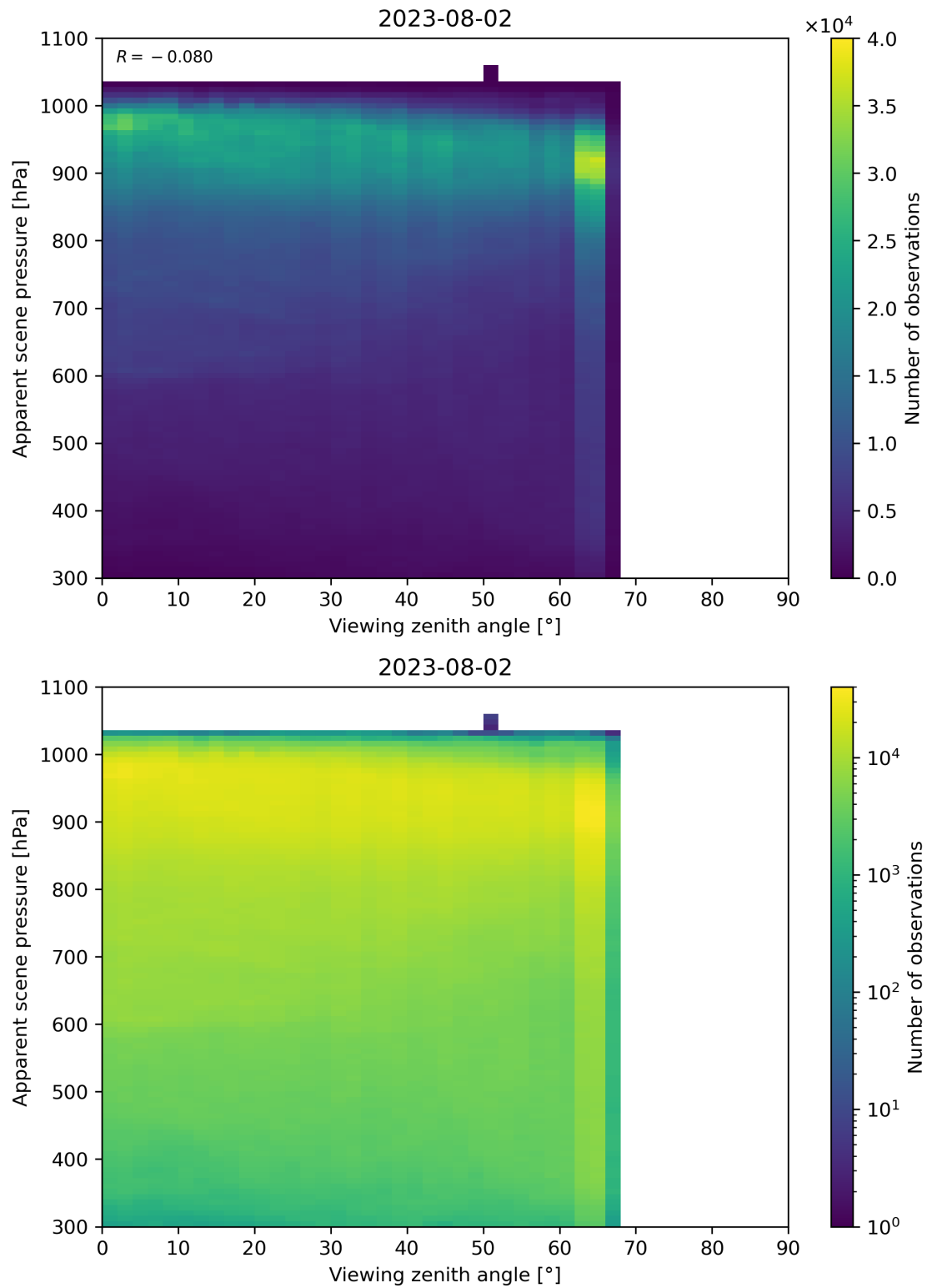
Figure 129: Scatter density plot of “Viewing zenith angle” against “Apparent scene pressure” for 2023-08-01 to 2023-08-03.
