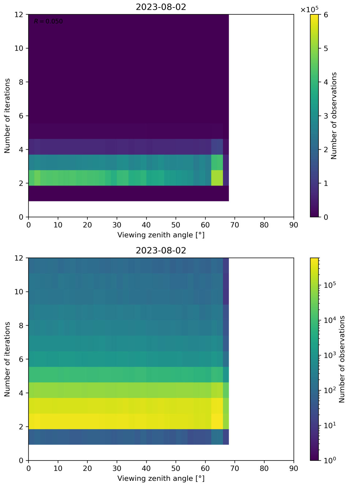
Figure 136: Scatter density plot of “Viewing zenith angle” against “Number of iterations” for 2023-08-01 to 2023-08-03.
