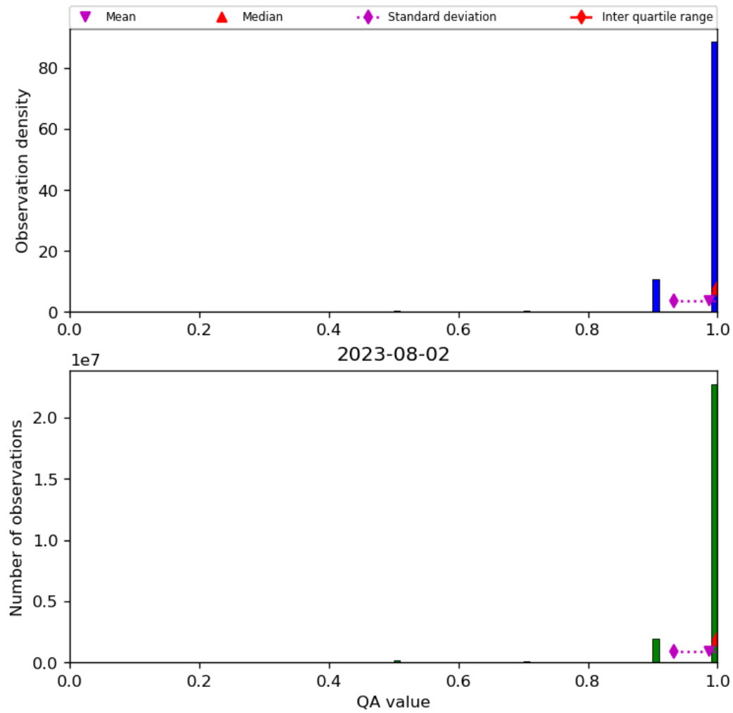
Figure 29: Histogram of “QA value” for 2023-08-01 to 2023-08-03
