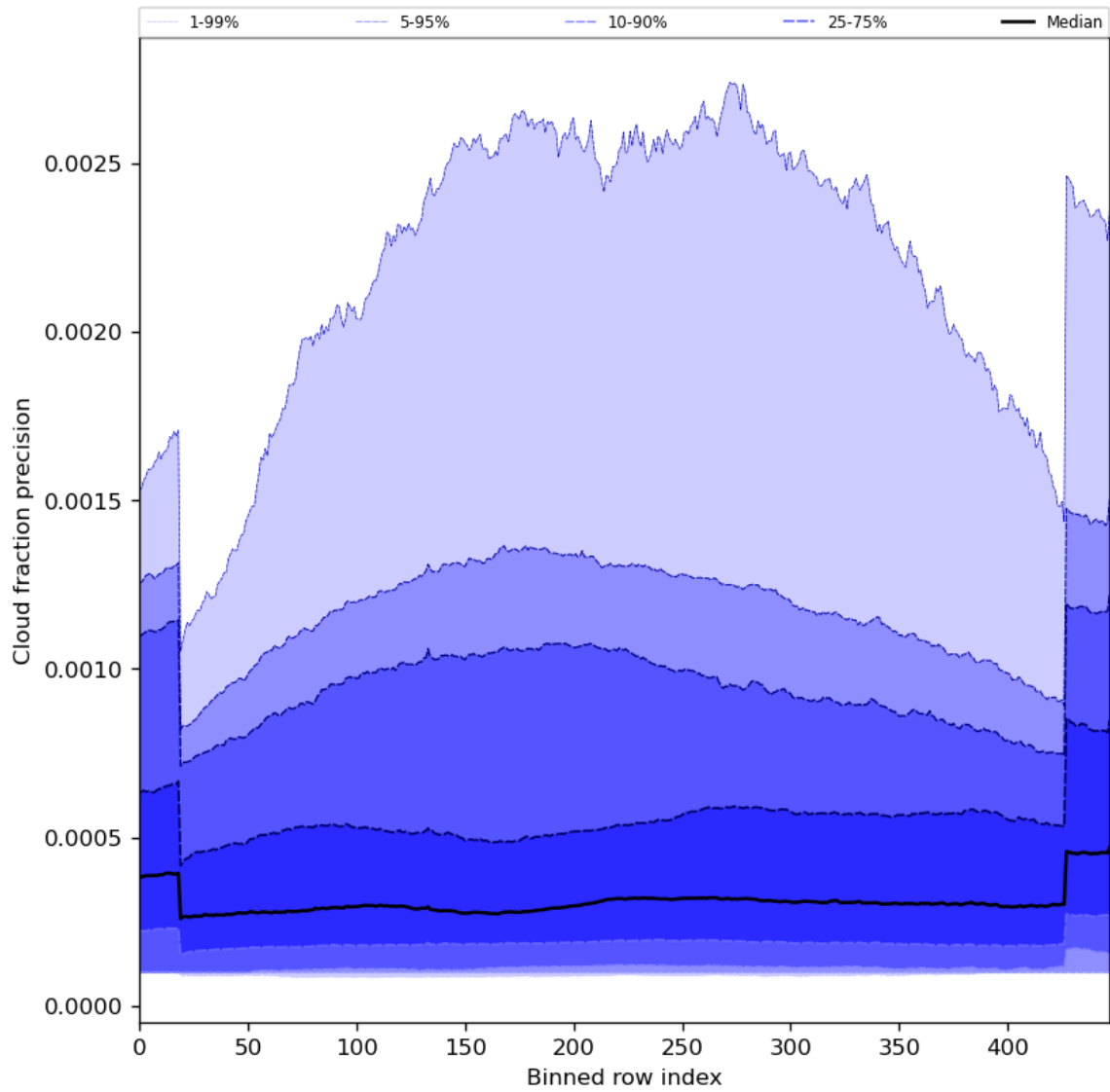
Figure 50: Along track statistics of “Cloud fraction precision” for 2023-08-01 to 2023-08-03
