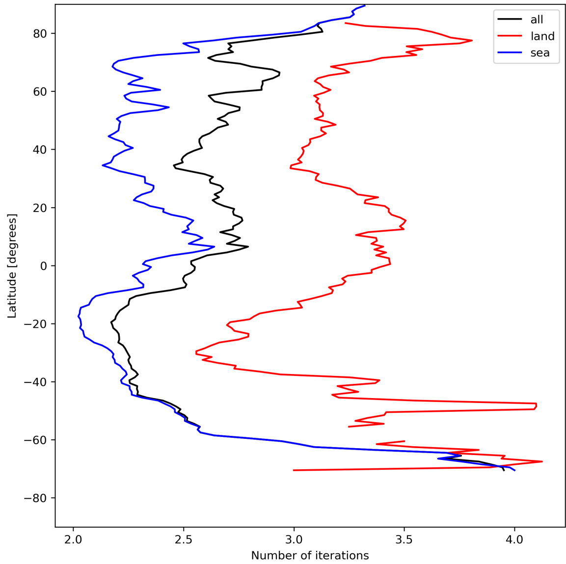
Figure 22: Zonal average of “Number of iterations” for 2023-08-01 to 2023-08-03.
