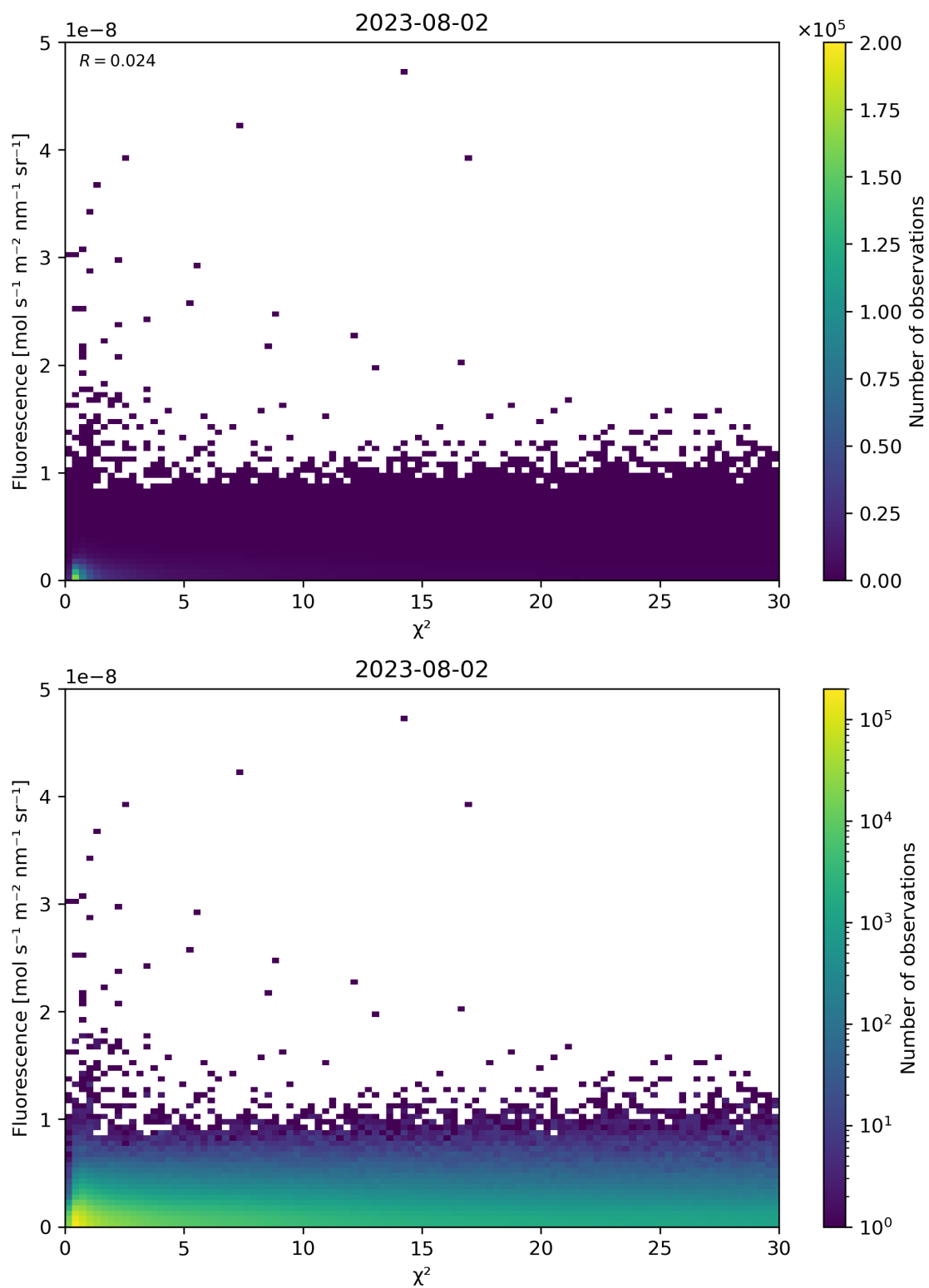
Figure 70: Scatter density plot of “ \chi^2 ” against “Fluorescence” for 2023-08-01 to 2023-08-03.
