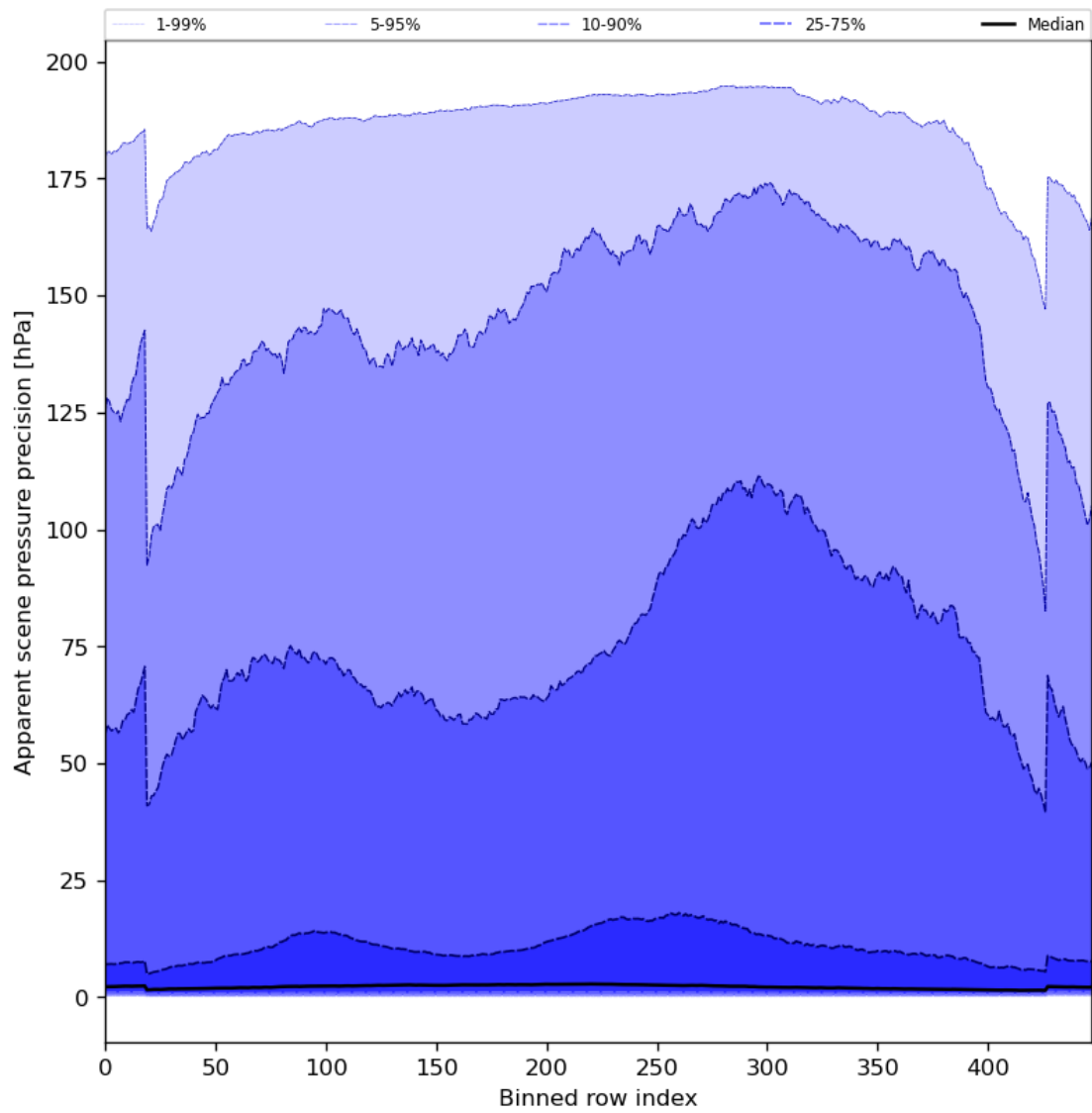
Figure 54: Along track statistics of “Apparent scene pressure precision” for 2023-08-01 to 2023-08-03
