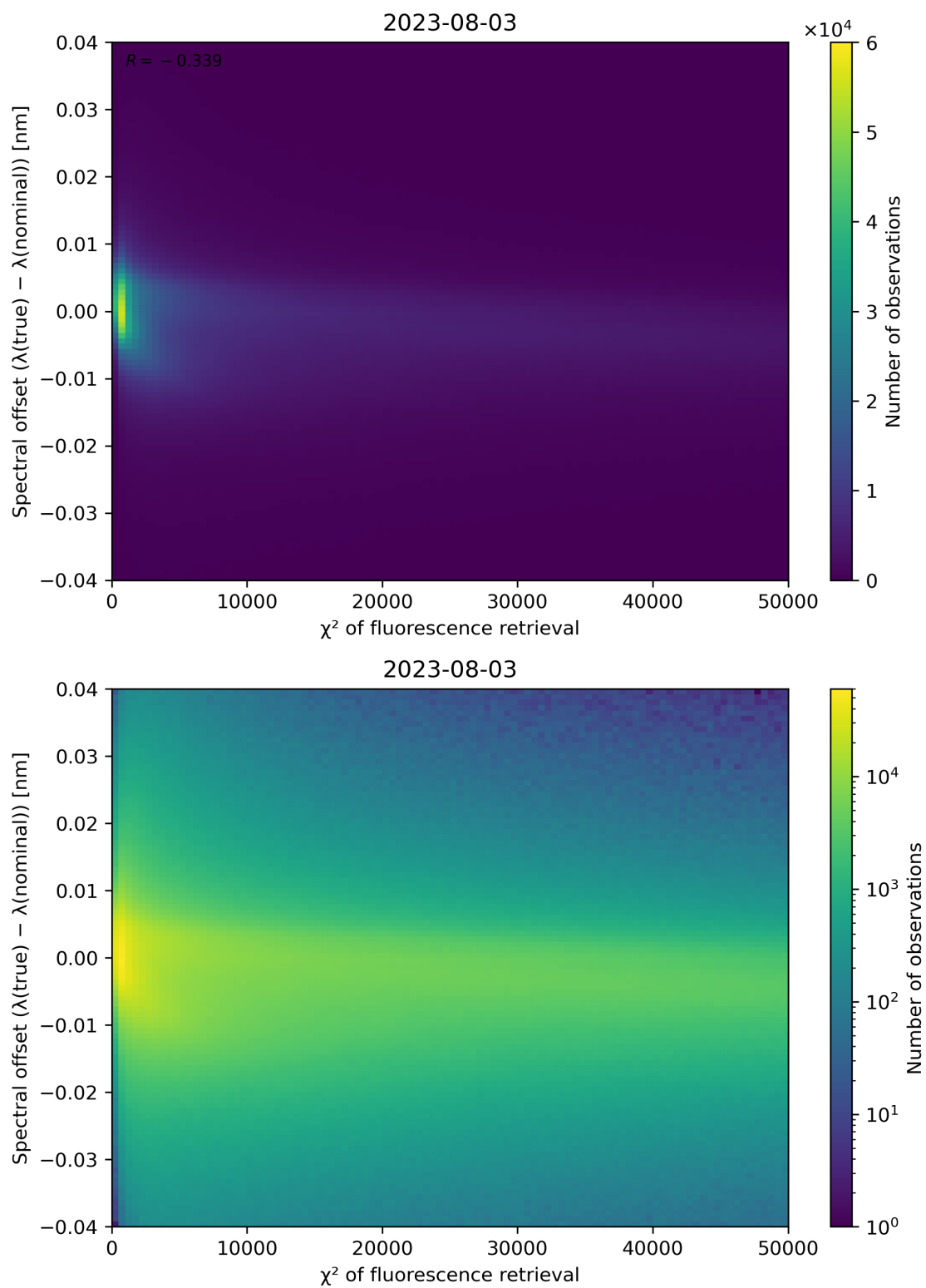
Figure 72: Scatter density plot of " \chi^2 of fluorescence retrieval" against "Spectral offset ( \lambda(\text{true}) - \lambda(\text{nominal})) " for 2023-08-02 to 2023-08-04.
