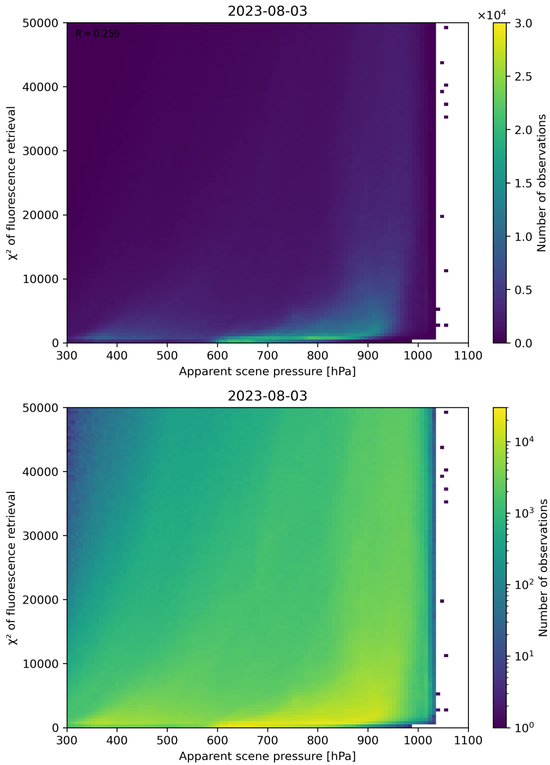
Figure 64: Scatter density plot of “Apparent scene pressure” against “ \chi^2 of fluorescence retrieval” for 2023-08-02 to 2023-08-04.
