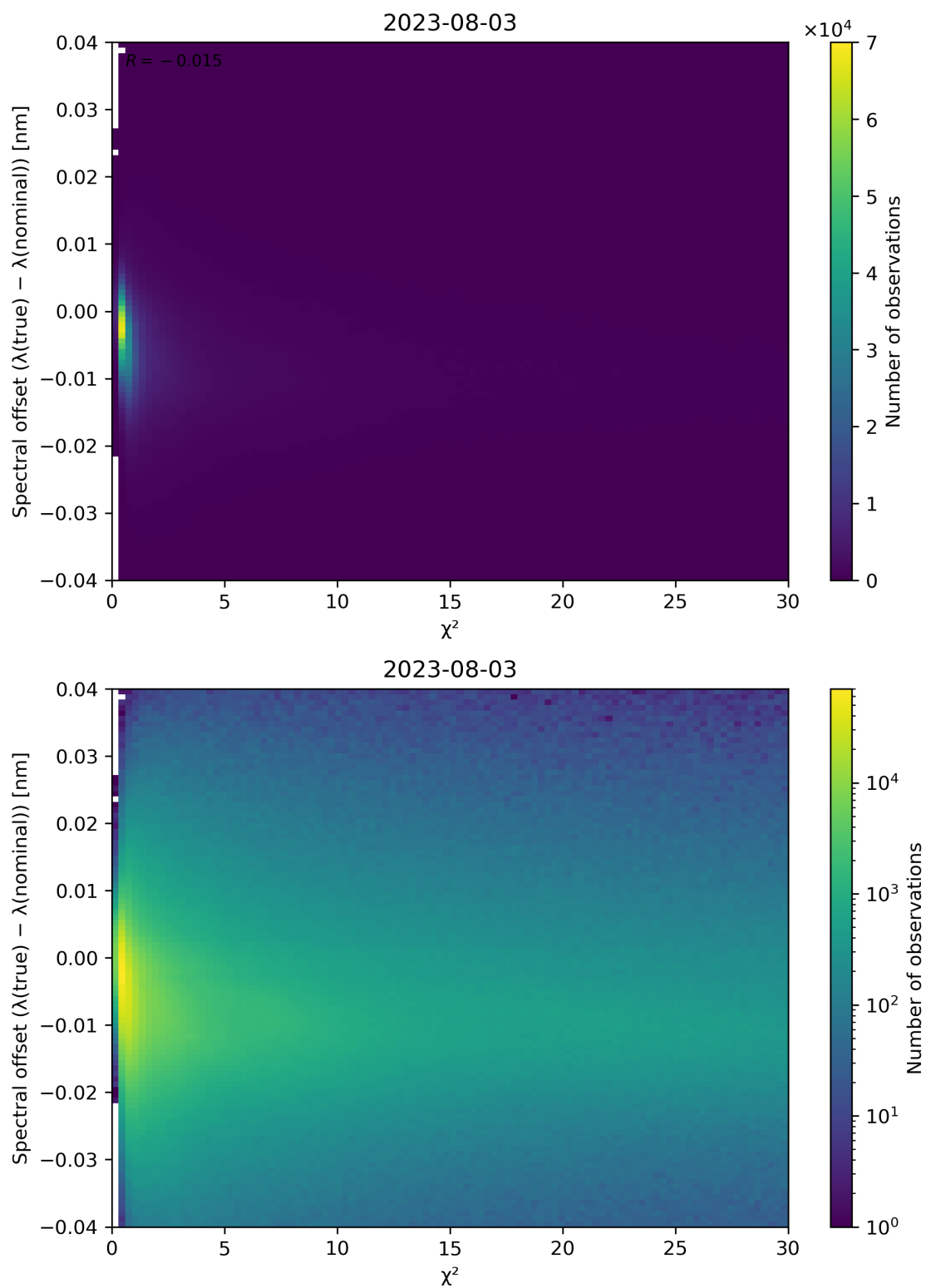
Figure 75: Scatter density plot of “ \chi^2 ” against “Spectral offset ( \lambda(\text{true}) - \lambda(\text{nominal}) )” for 2023-08-02 to 2023-08-04.
