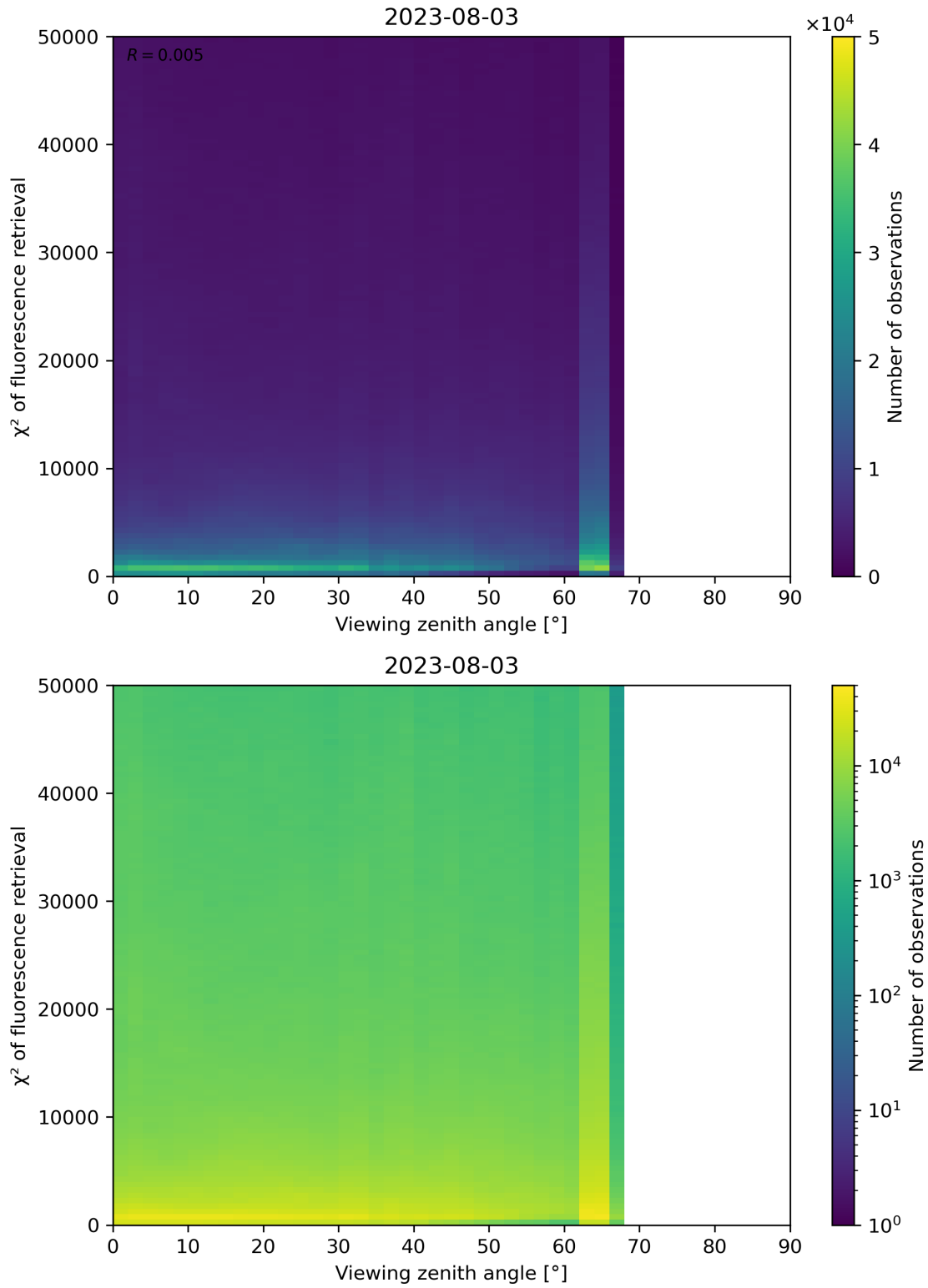
Figure 131: Scatter density plot of “Viewing zenith angle” against “ \chi^2 of fluorescence retrieval” for 2023-08-02 to 2023-08-04.
