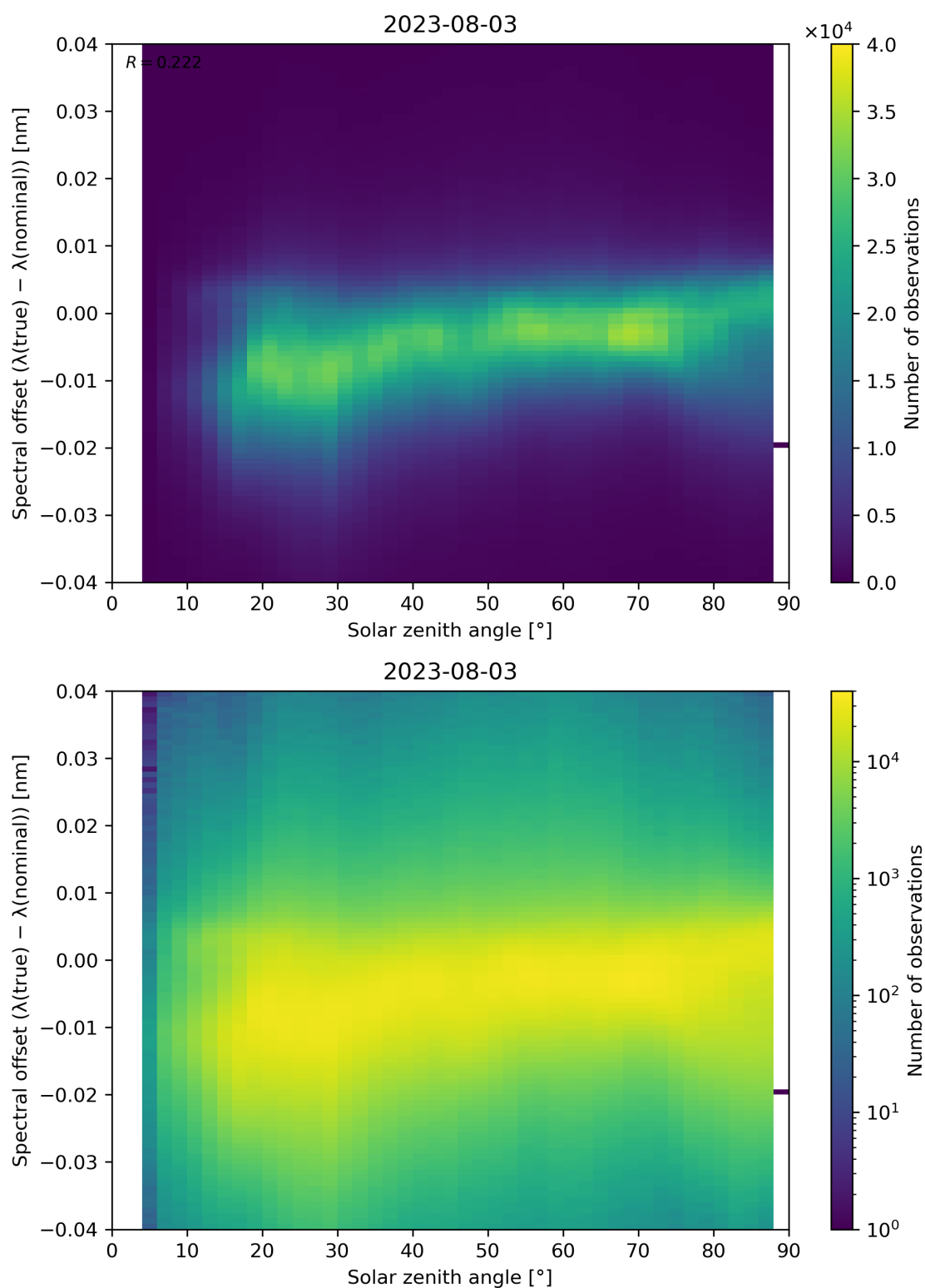
Figure 128: Scatter density plot of “Solar zenith angle” against “Spectral offset ( \lambda(\text{true}) - \lambda(\text{nominal}) )” for 2023-08-02 to 2023-08-04.
