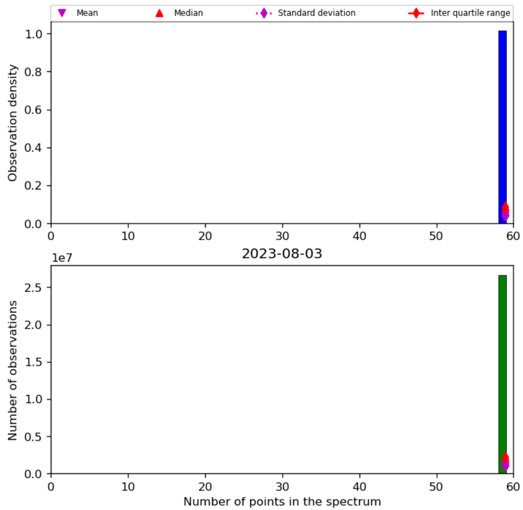
Figure 44: Histogram of “Number of points in the spectrum” for 2023-08-02 to 2023-08-04
