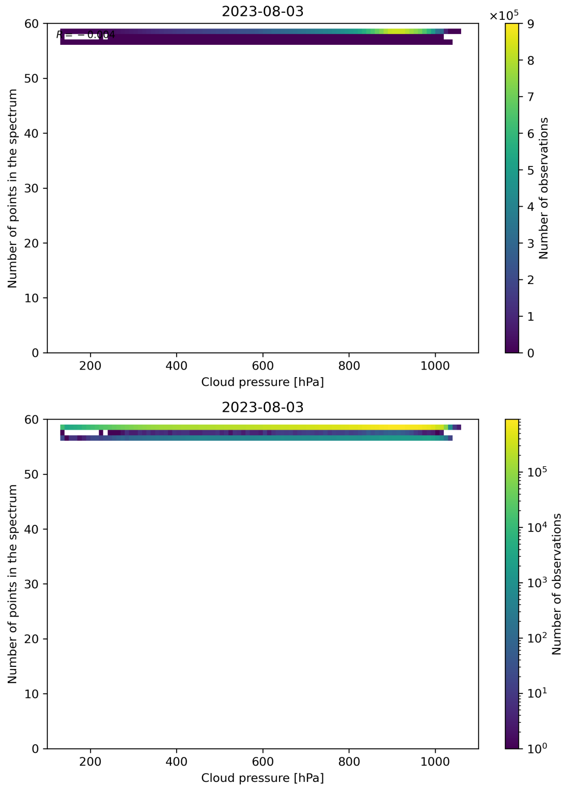
Figure 90: Scatter density plot of “Cloud pressure” against “Number of points in the spectrum” for 2023-08-02 to 2023-08-04.
