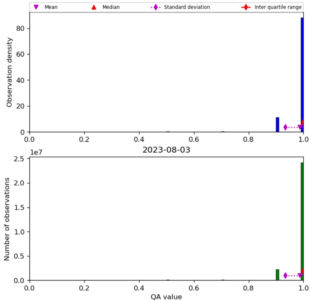
Figure 29: Histogram of “QA value” for 2023-08-02 to 2023-08-04
