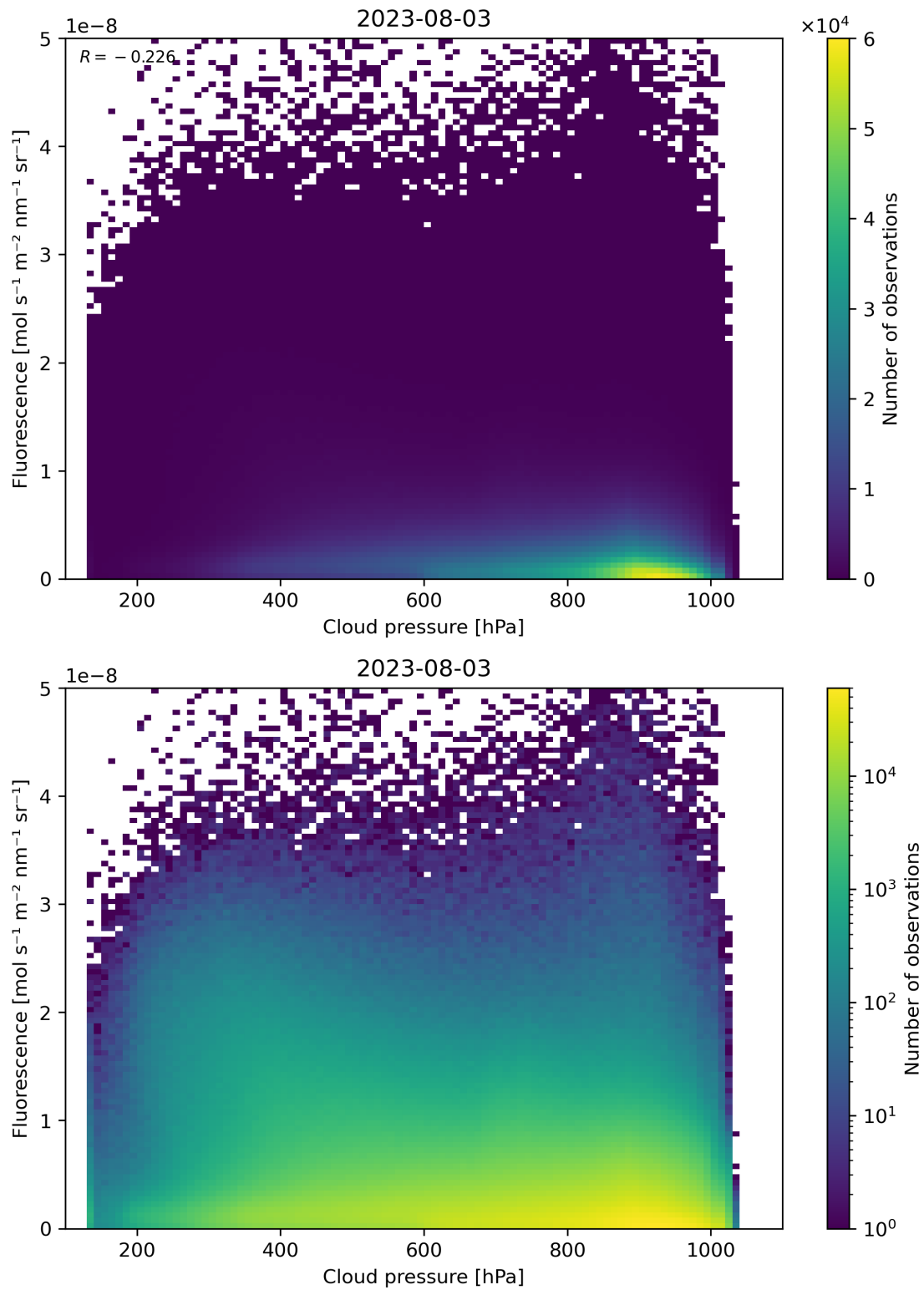
Figure 88: Scatter density plot of “Cloud pressure” against “Fluorescence” for 2023-08-02 to 2023-08-04.
