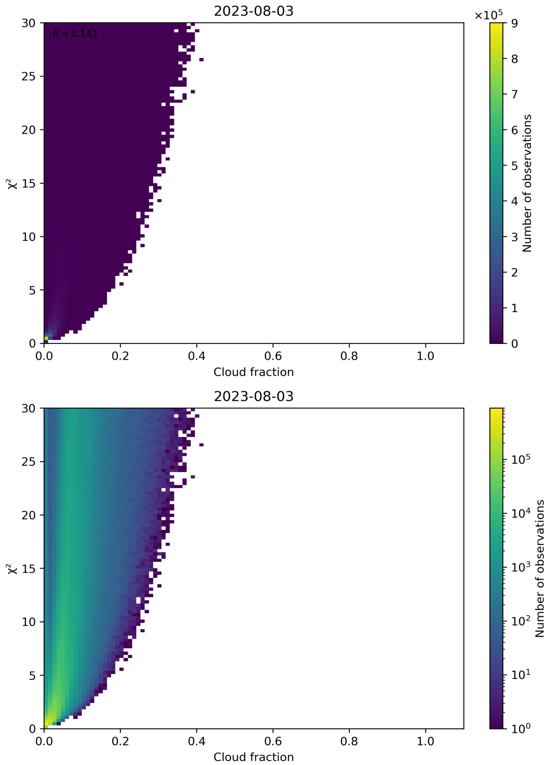
Figure 77: Scatter density plot of “Cloud fraction” against “ \chi^2 ” for 2023-08-02 to 2023-08-04.
