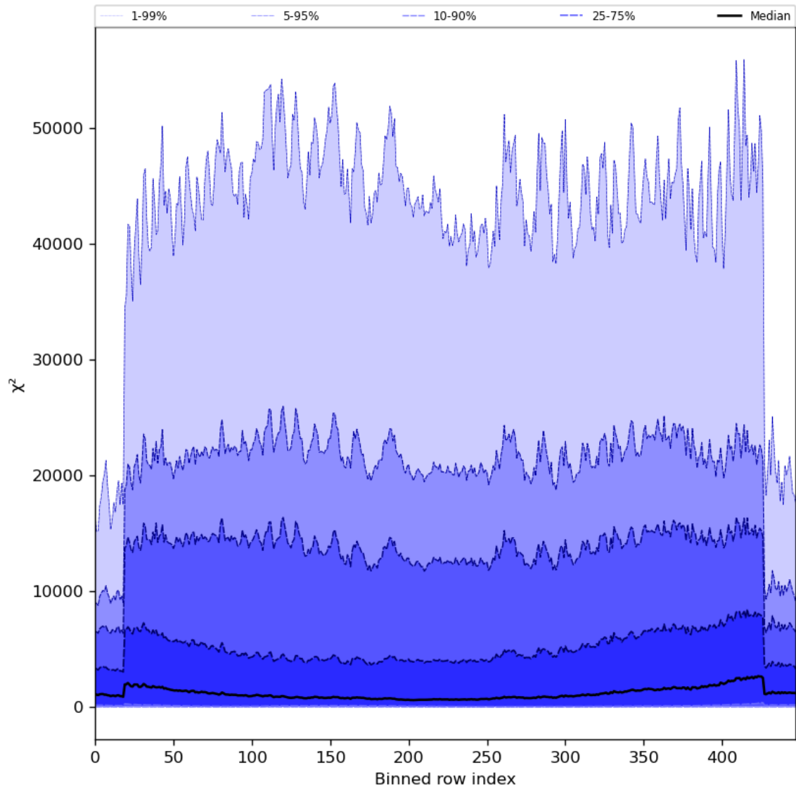
Figure 55: Along track statistics of “ \chi^2 ” for 2023-08-02 to 2023-08-04
