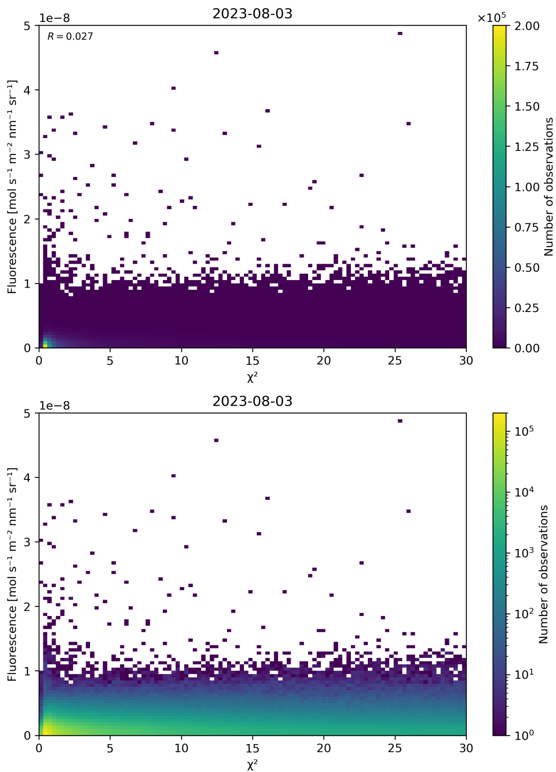
Figure 70: Scatter density plot of “ \chi^2 ” against “Fluorescence” for 2023-08-02 to 2023-08-04.
