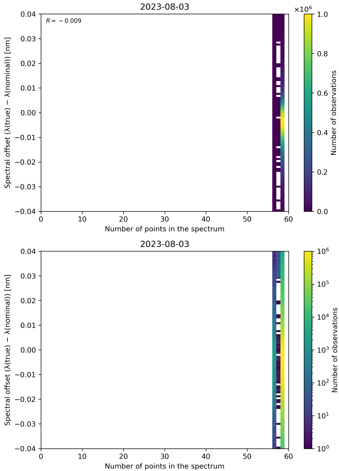
Figure 110: Scatter density plot of “Number of points in the spectrum” against “Spectral offset ( \lambda(\text{true}) - \lambda(\text{nominal}) )” for 2023-08-02 to 2023-08-04.
