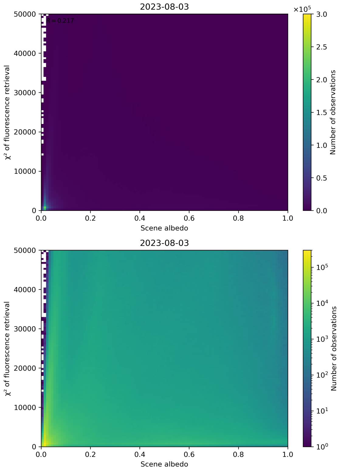
Figure 113: Scatter density plot of “Scene albedo” against “ \chi^2 of fluorescence retrieval” for 2023-08-02 to 2023-08-04.
