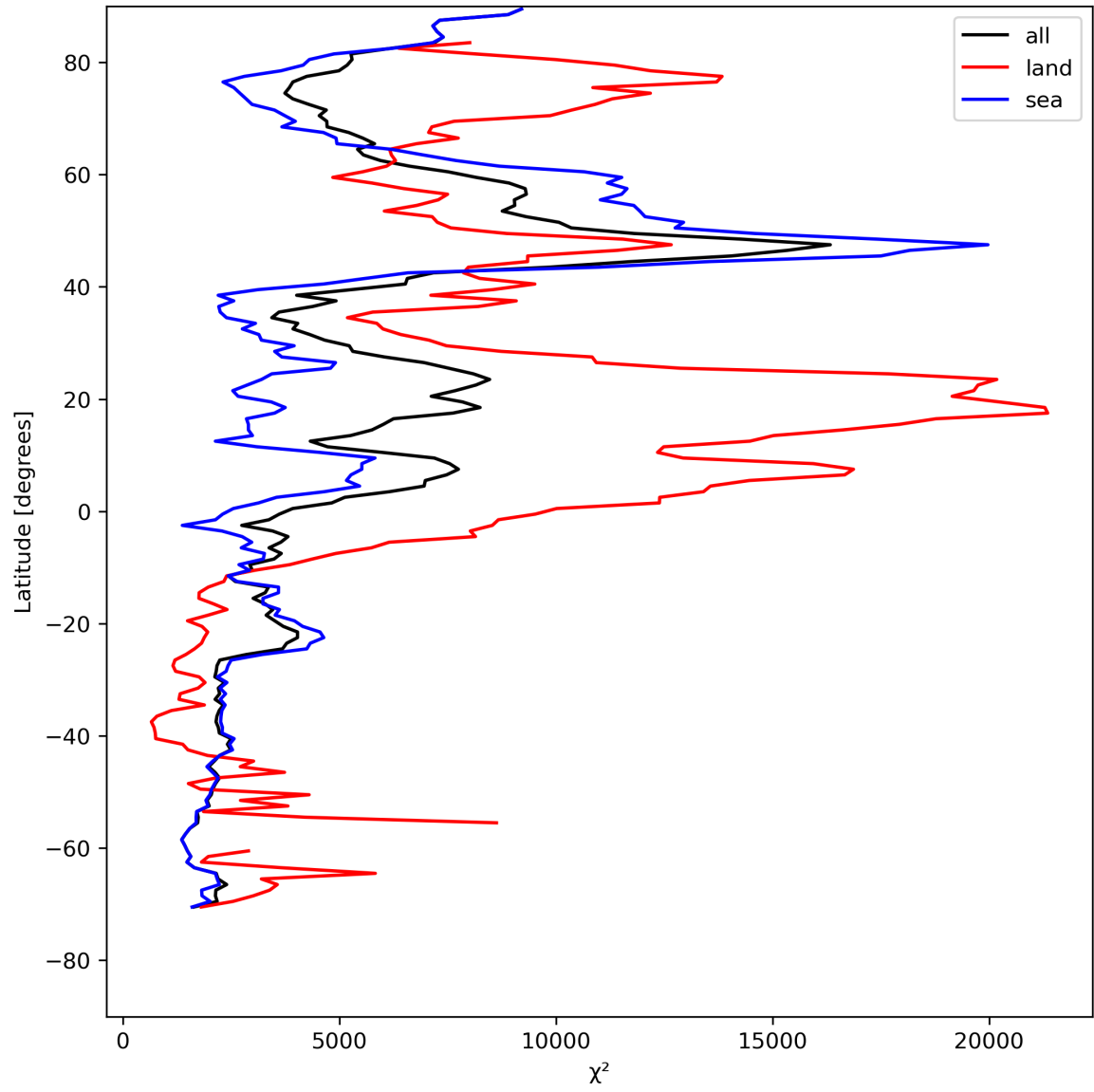
Figure 21: Zonal average of “ \chi^2 ” for 2023-08-02 to 2023-08-04.
