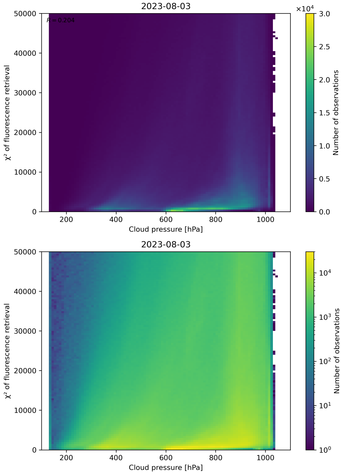
Figure 86: Scatter density plot of “Cloud pressure” against “ \chi^2 of fluorescence retrieval” for 2023-08-02 to 2023-08-04.
