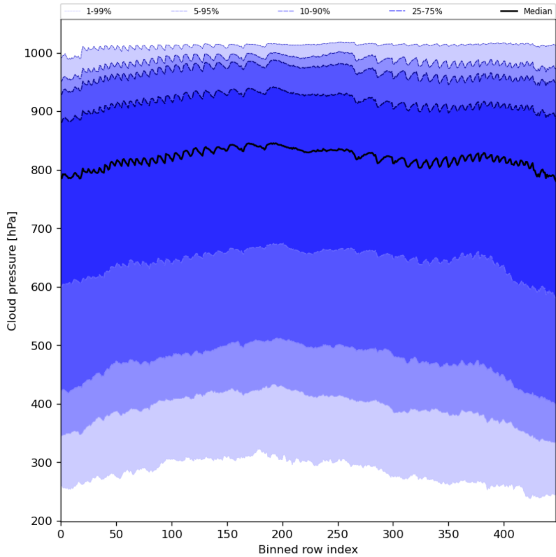
Figure 47: Along track statistics of “Cloud pressure” for 2023-08-02 to 2023-08-04
