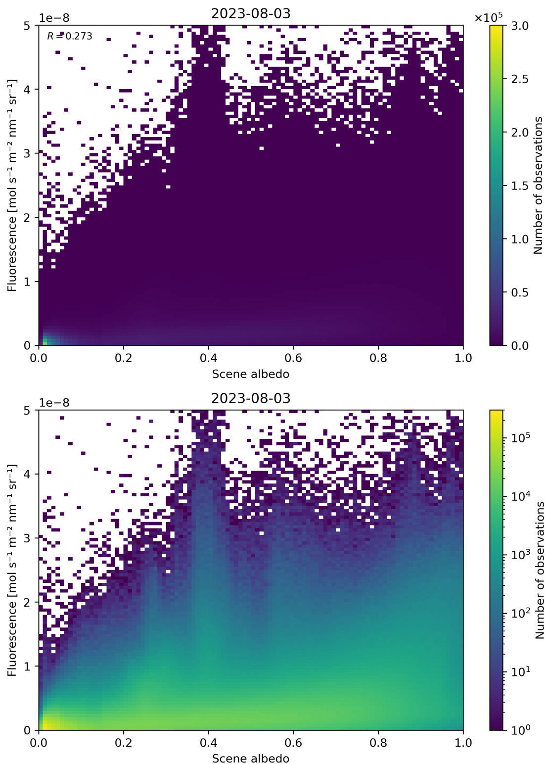
Figure 114: Scatter density plot of “Scene albedo” against “Fluorescence” for 2023-08-02 to 2023-08-04.
