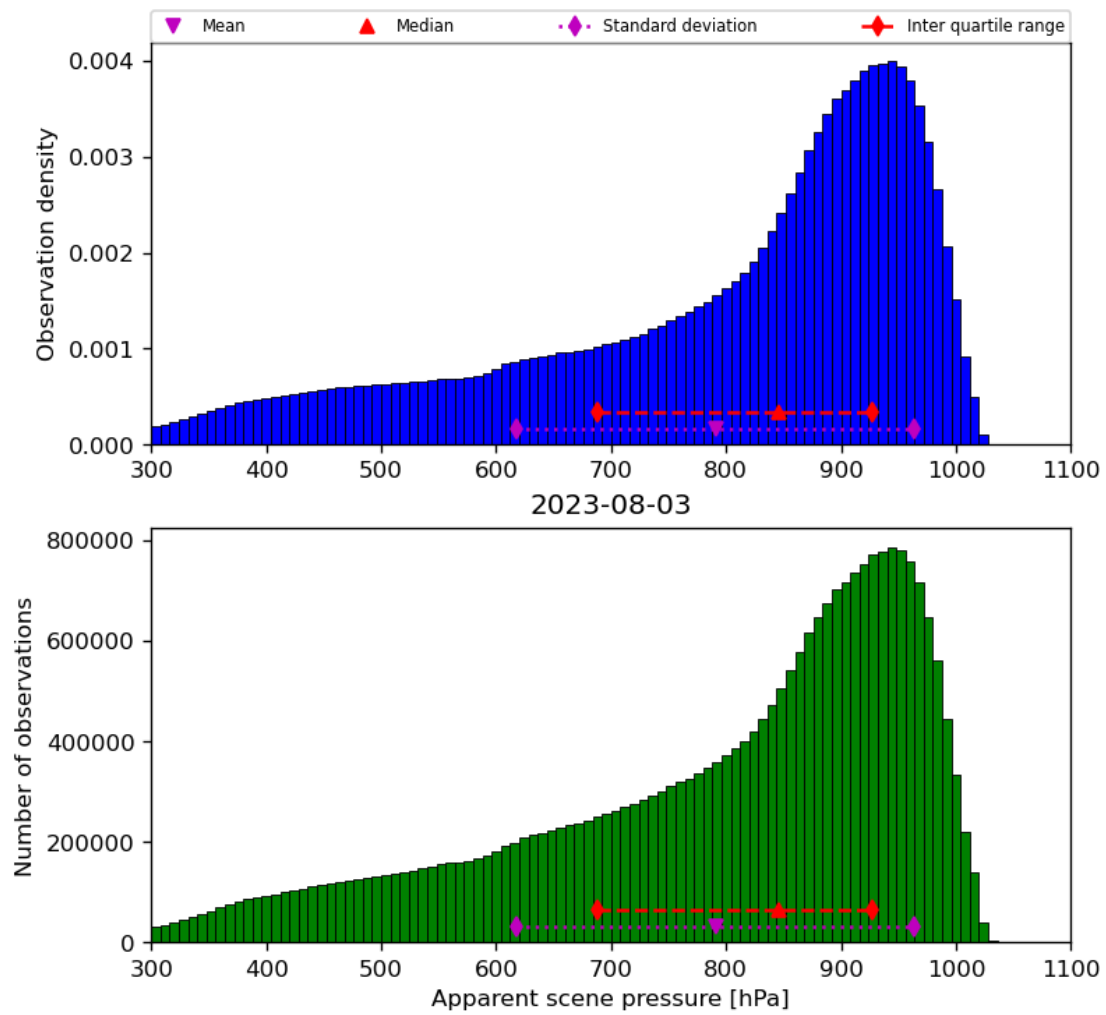
Figure 36: Histogram of “Apparent scene pressure” for 2023-08-02 to 2023-08-04
