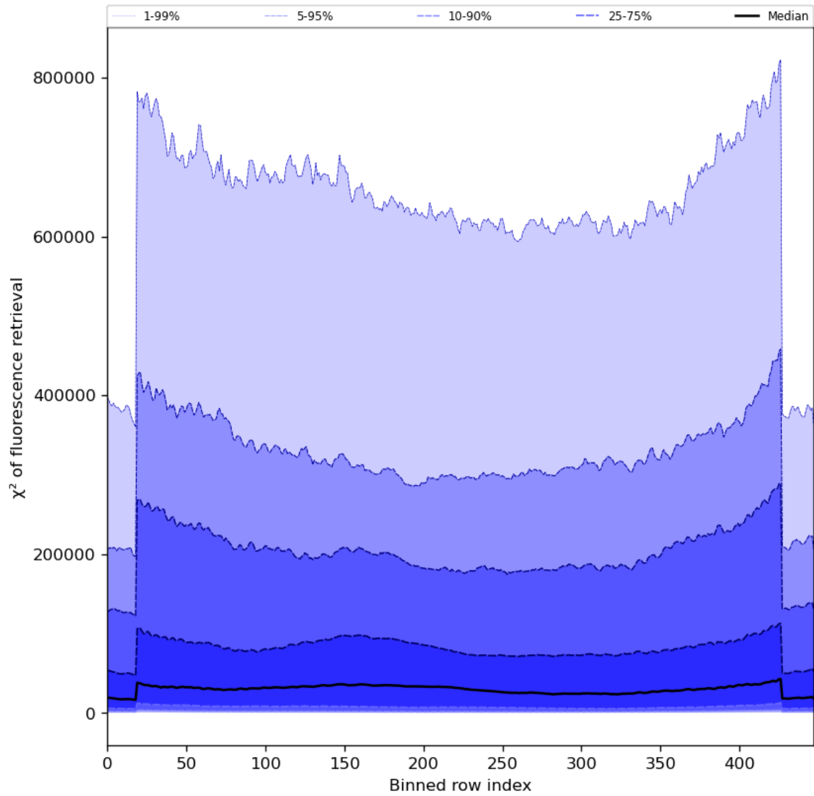
Figure 59: Along track statistics of “ \chi^2 of fluorescence retrieval” for 2023-08-02 to 2023-08-04
