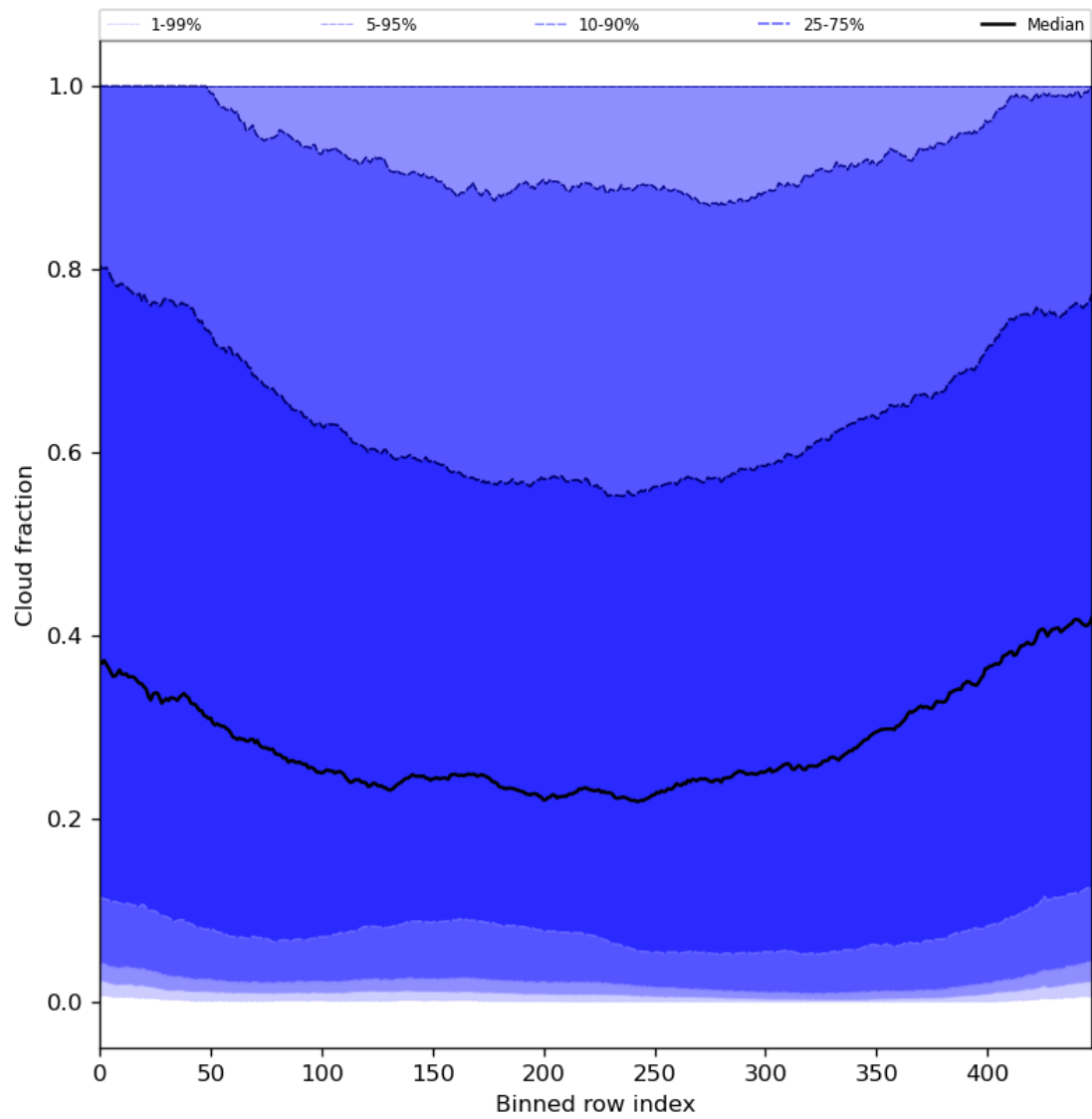
Figure 49: Along track statistics of “Cloud fraction” for 2023-08-02 to 2023-08-04
