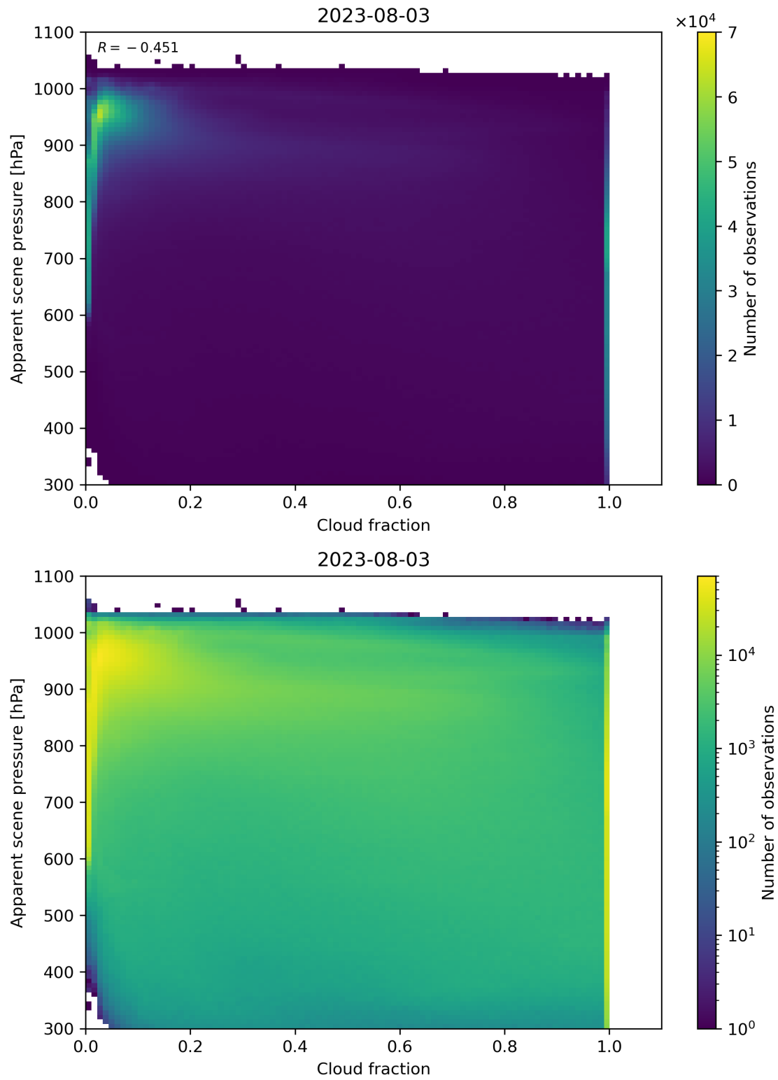
Figure 76: Scatter density plot of “Cloud fraction” against “Apparent scene pressure” for 2023-08-02 to 2023-08-04.
