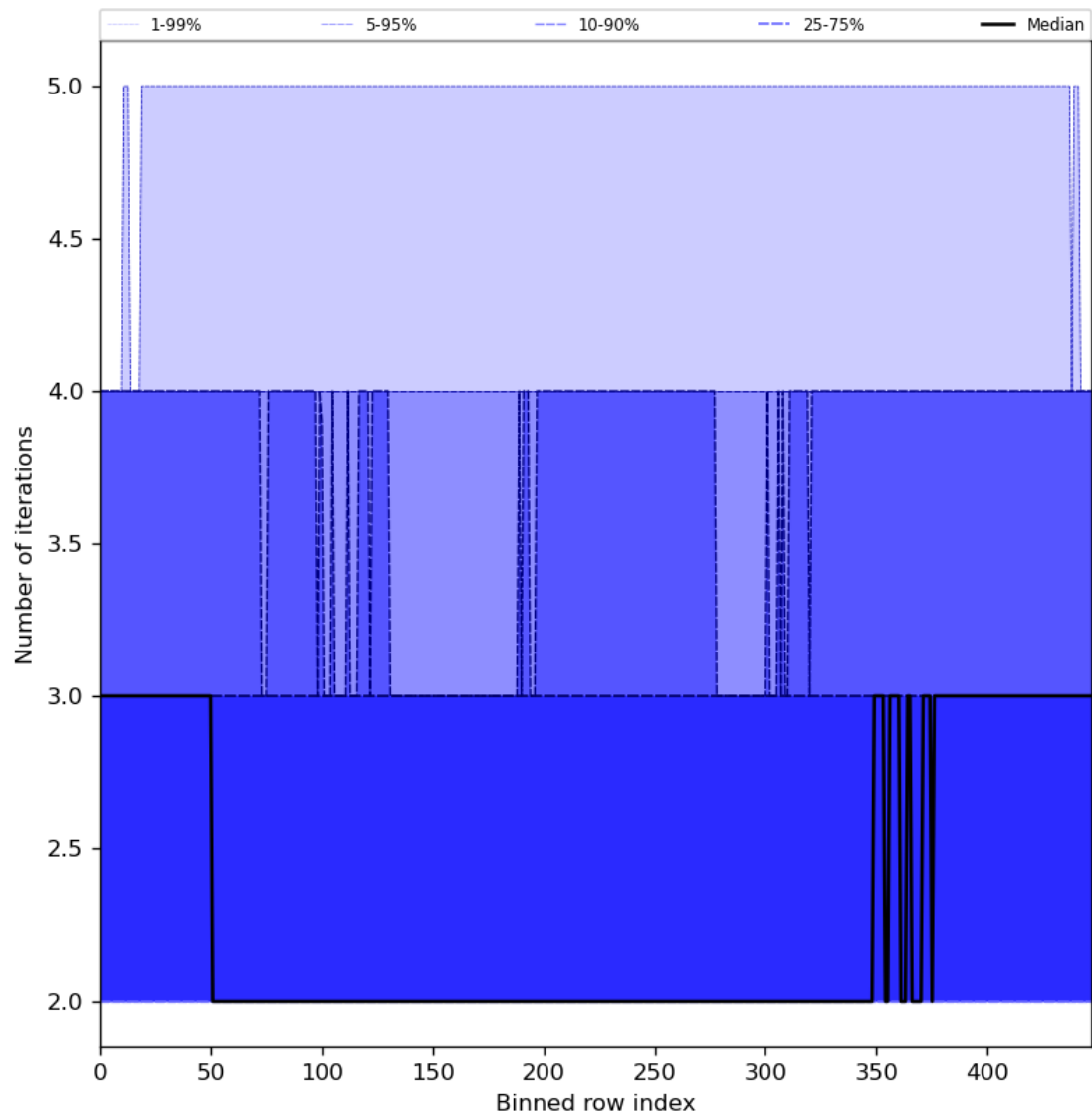
Figure 56: Along track statistics of “Number of iterations” for 2023-08-02 to 2023-08-04
