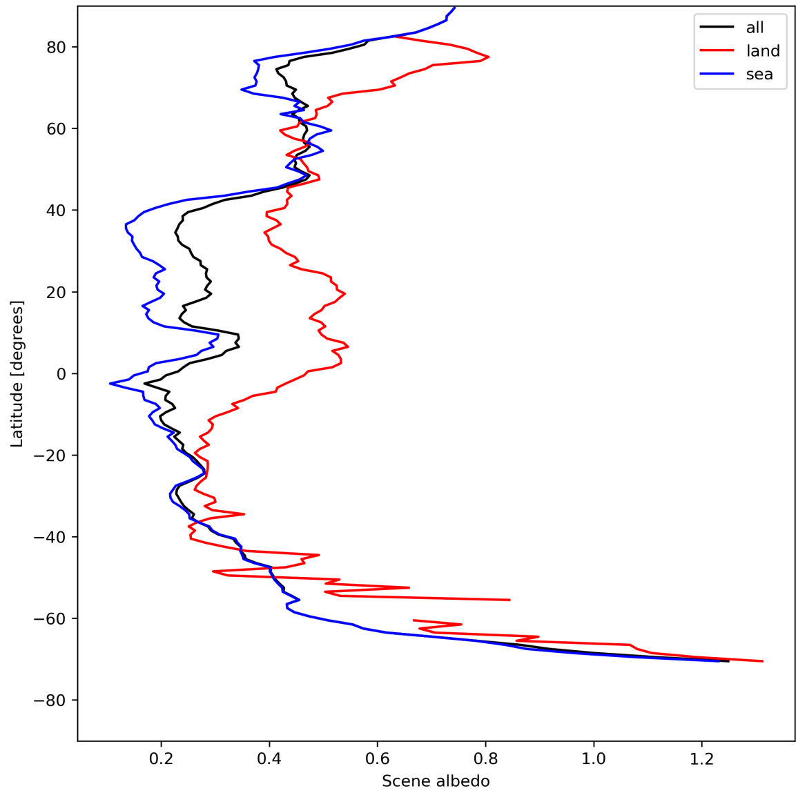
Figure 17: Zonal average of “Scene albedo” for 2023-08-02 to 2023-08-04.
