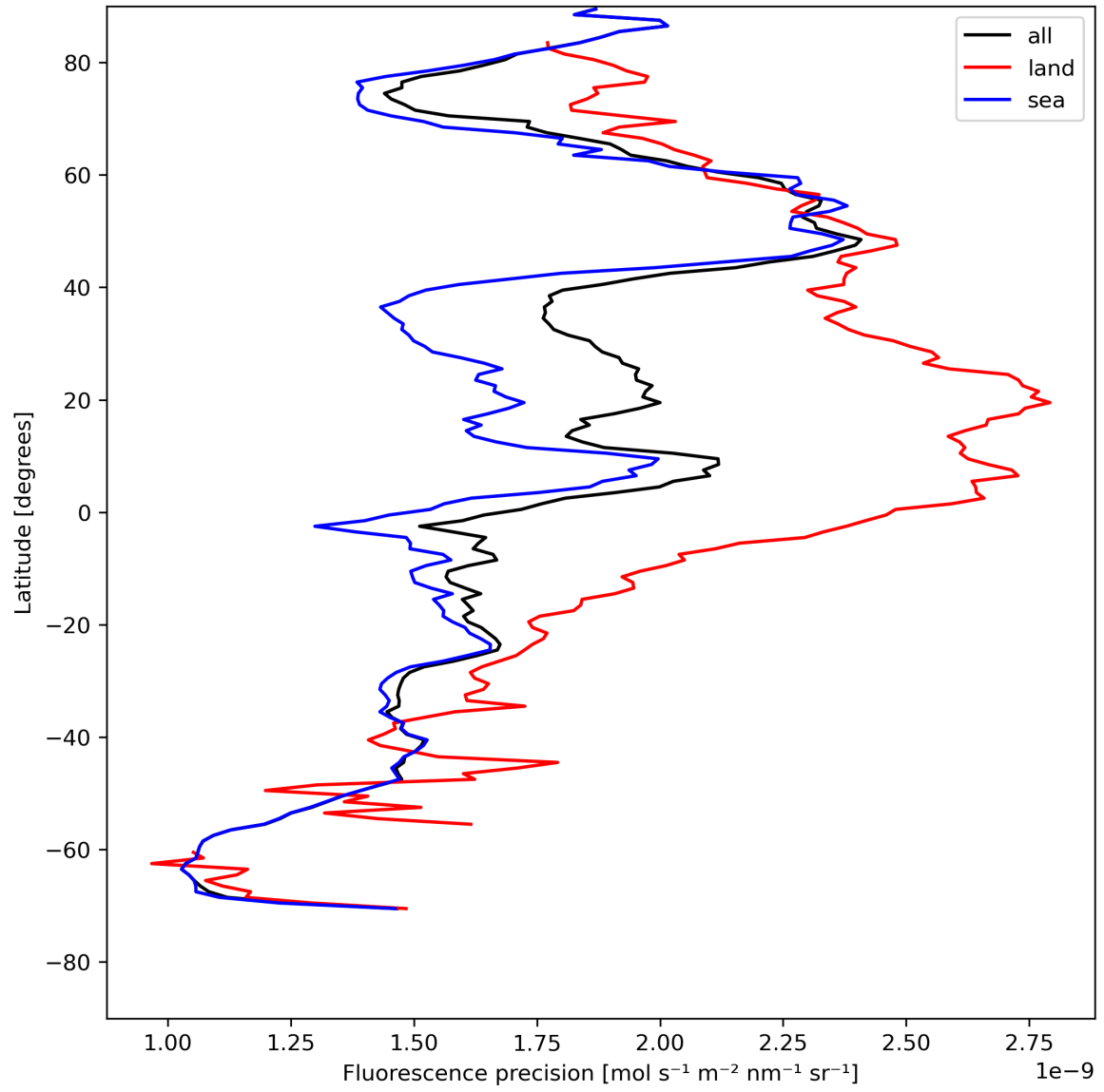
Figure 24: Zonal average of “Fluorescence precision” for 2023-08-02 to 2023-08-04.
