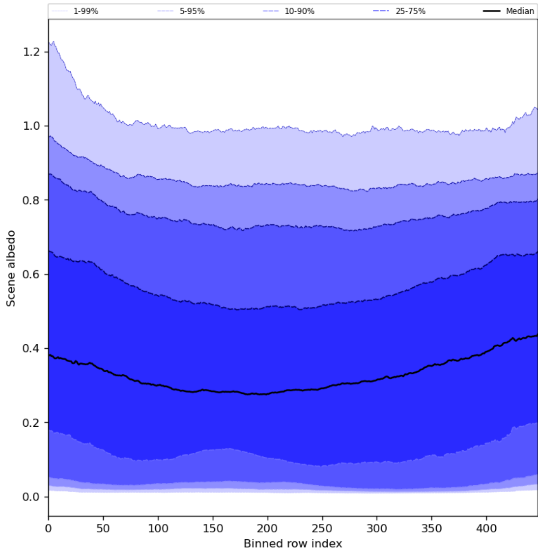
Figure 51: Along track statistics of “Scene albedo” for 2023-08-02 to 2023-08-04
