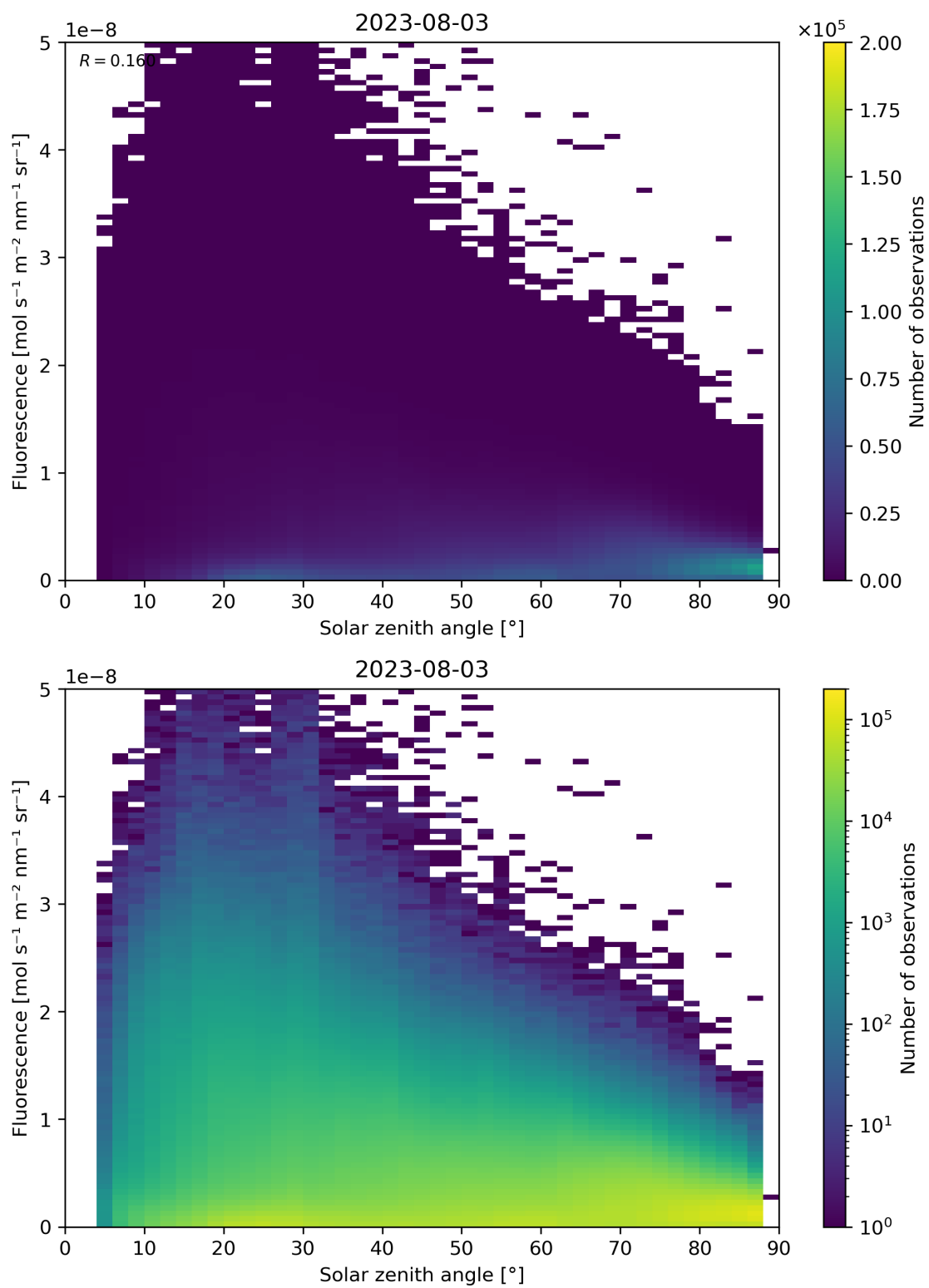
Figure 123: Scatter density plot of “Solar zenith angle” against “Fluorescence” for 2023-08-02 to 2023-08-04.
