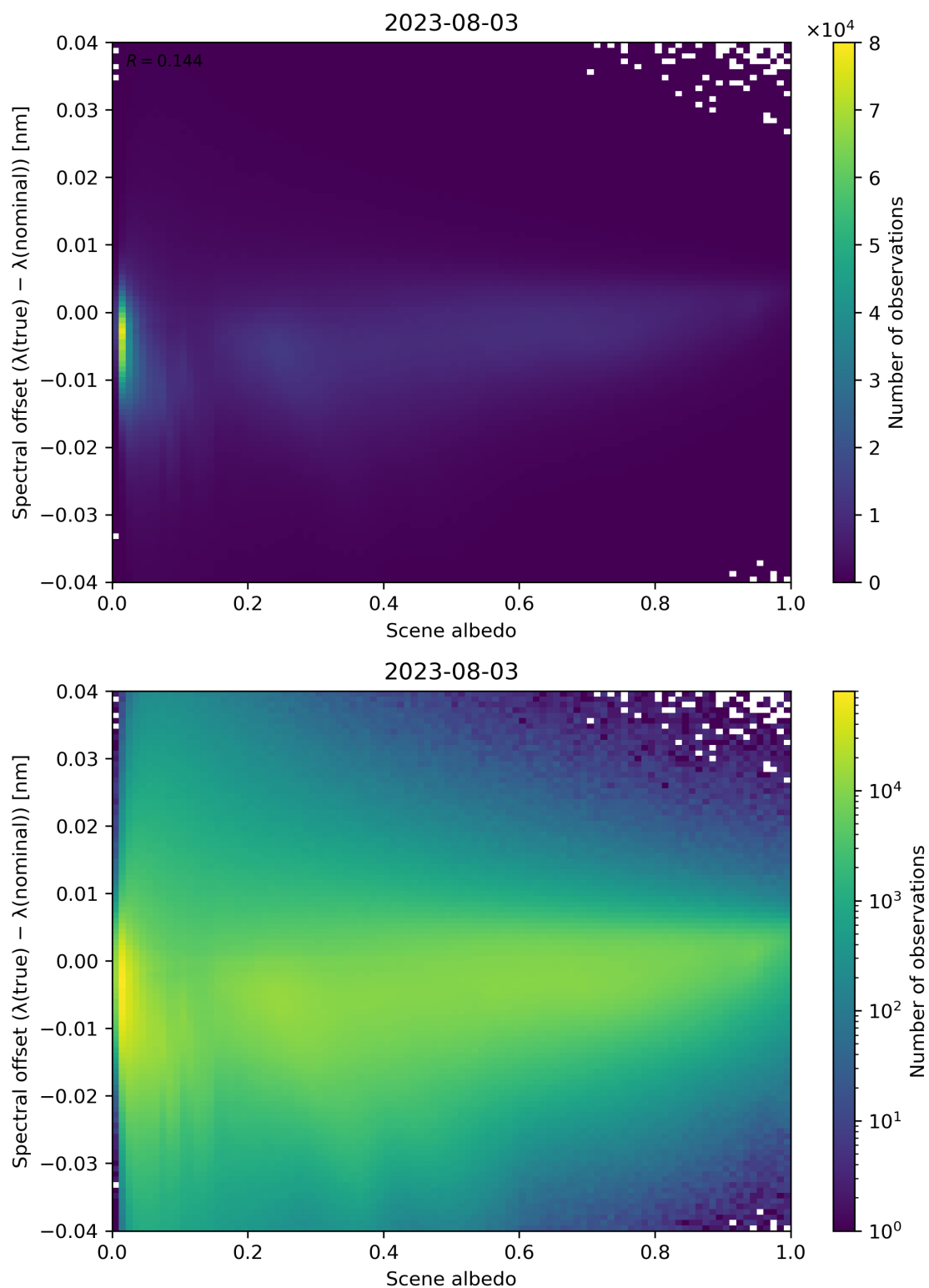
Figure 117: Scatter density plot of “Scene albedo” against “Spectral offset ( \lambda(\text{true}) - \lambda(\text{nominal}) )” for 2023-08-02 to 2023-08-04.
