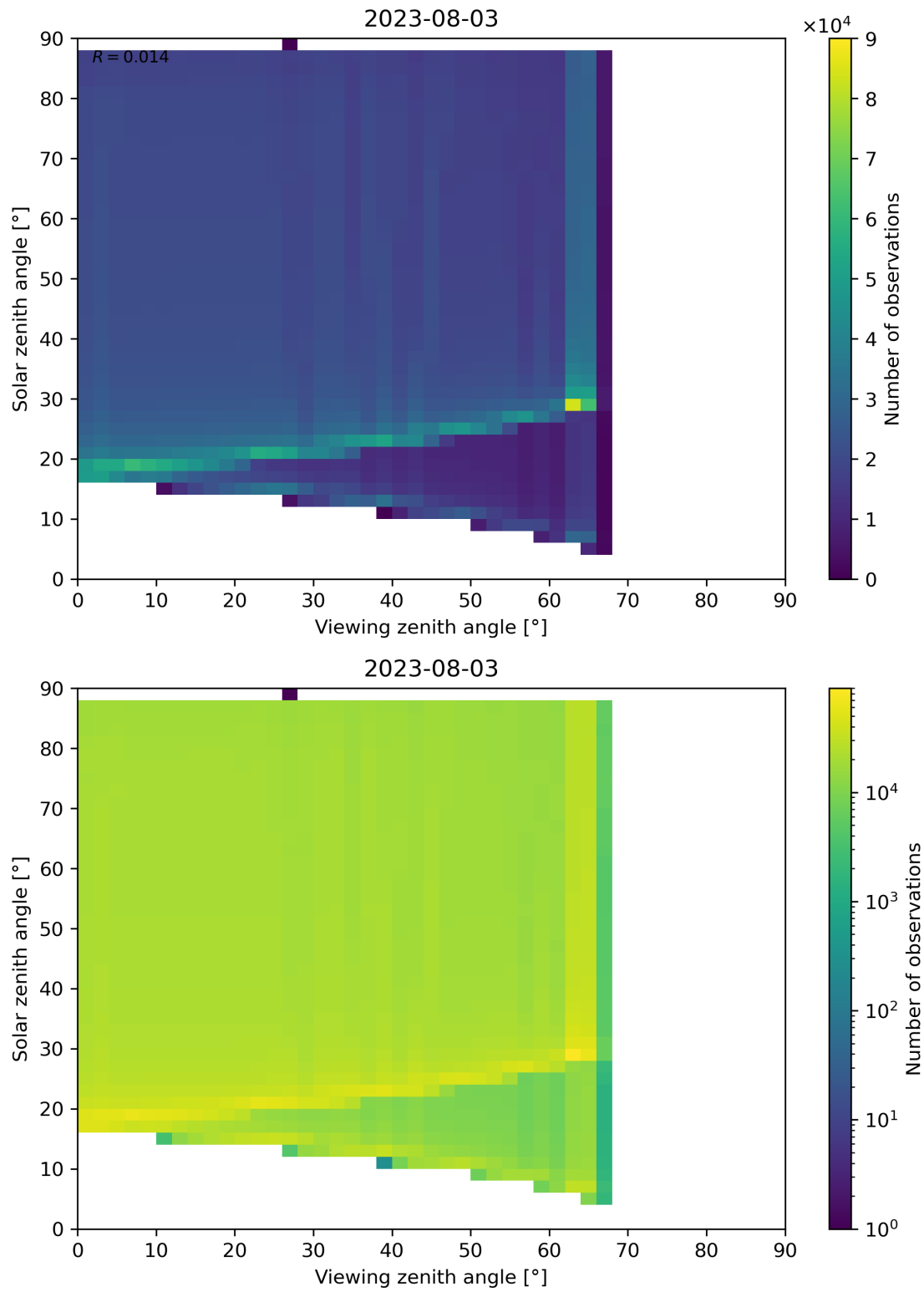
Figure 139: Scatter density plot of “Viewing zenith angle” against “Solar zenith angle” for 2023-08-02 to 2023-08-04.
