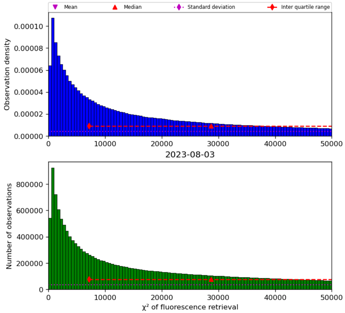
Figure 42: Histogram of “ \chi^2 of fluorescence retrieval” for 2023-08-02 to 2023-08-04
