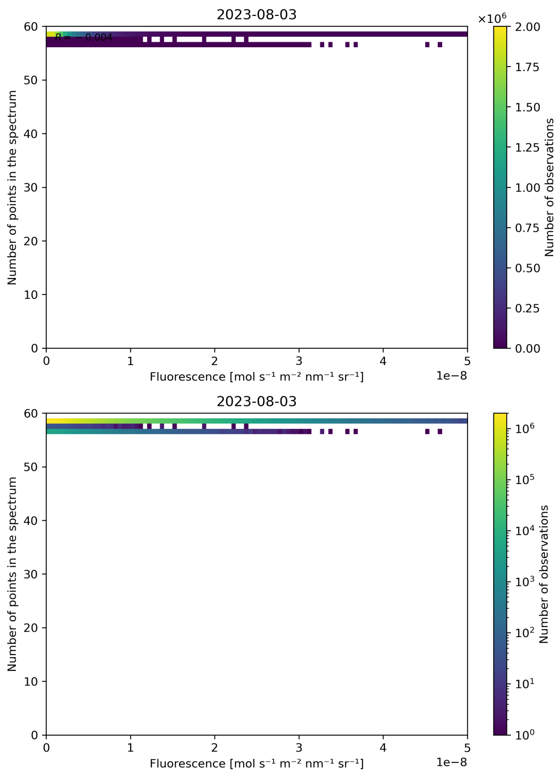
Figure 94: Scatter density plot of “Fluorescence” against “Number of points in the spectrum” for 2023-08-02 to 2023-08-04.
