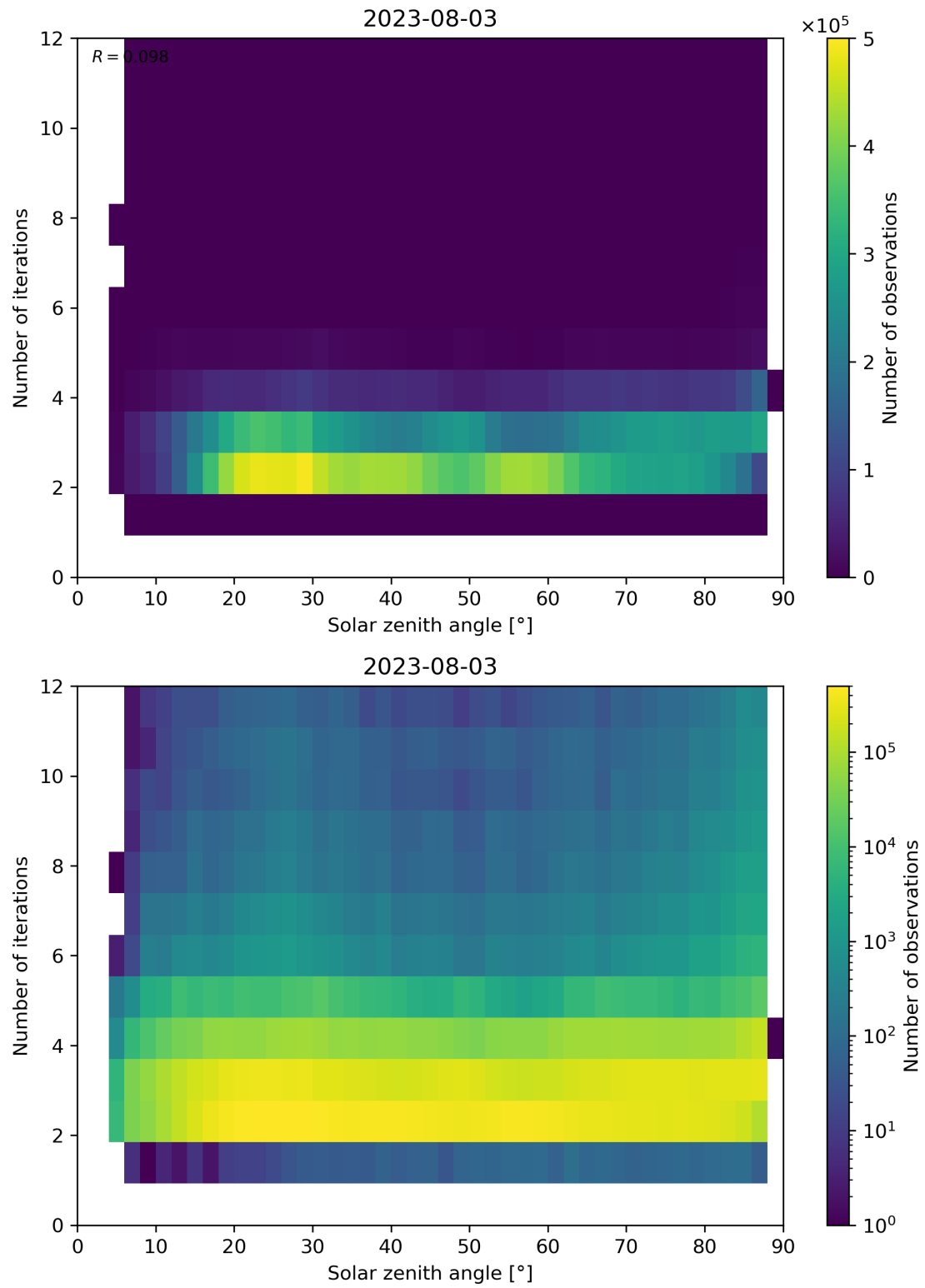
Figure 125: Scatter density plot of “Solar zenith angle” against “Number of iterations” for 2023-08-02 to 2023-08-04.
