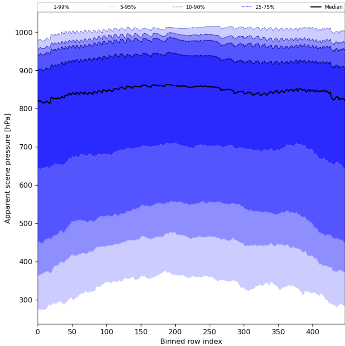
Figure 53: Along track statistics of “Apparent scene pressure” for 2023-08-02 to 2023-08-04
