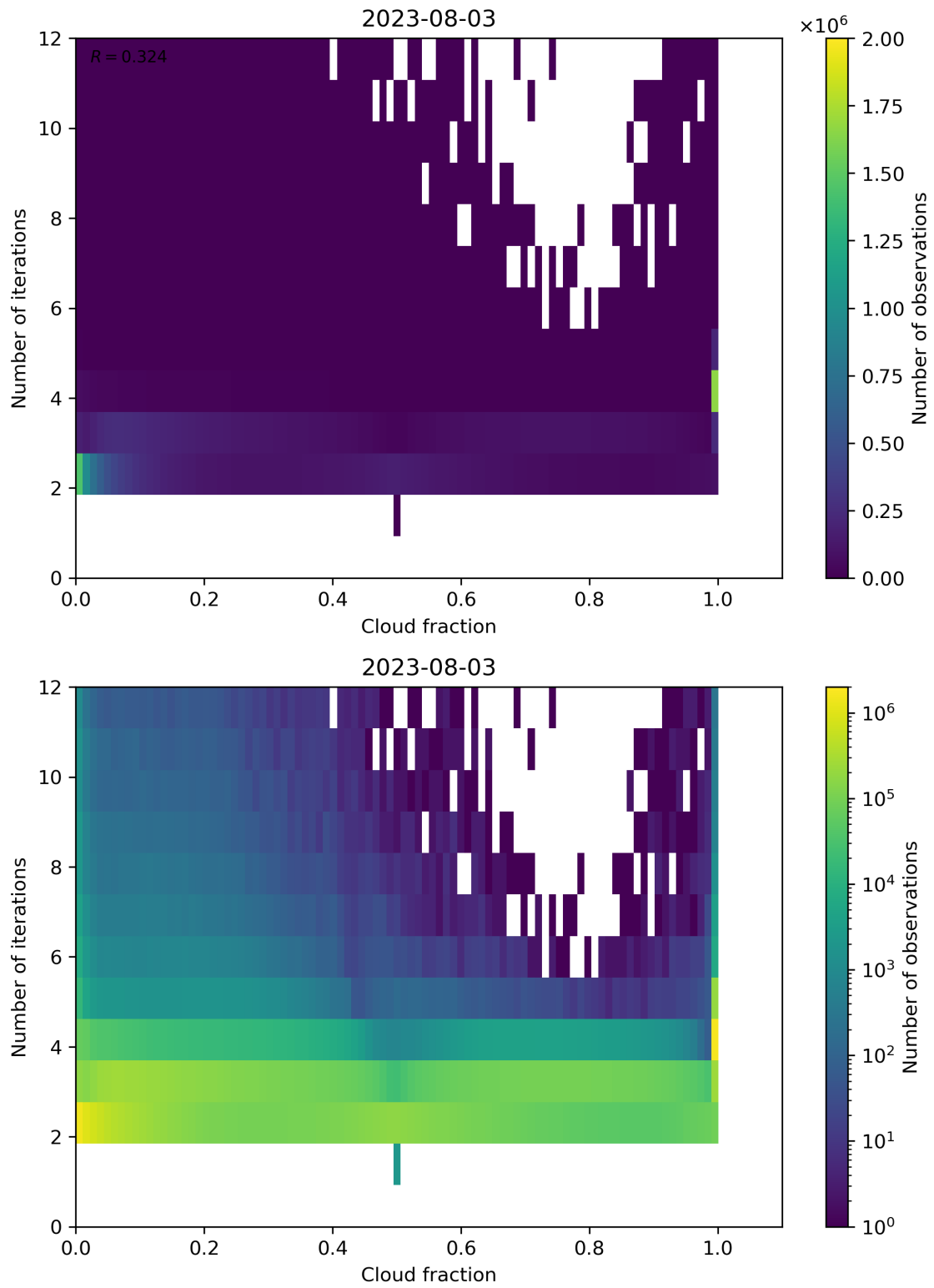
Figure 80: Scatter density plot of “Cloud fraction” against “Number of iterations” for 2023-08-02 to 2023-08-04.
