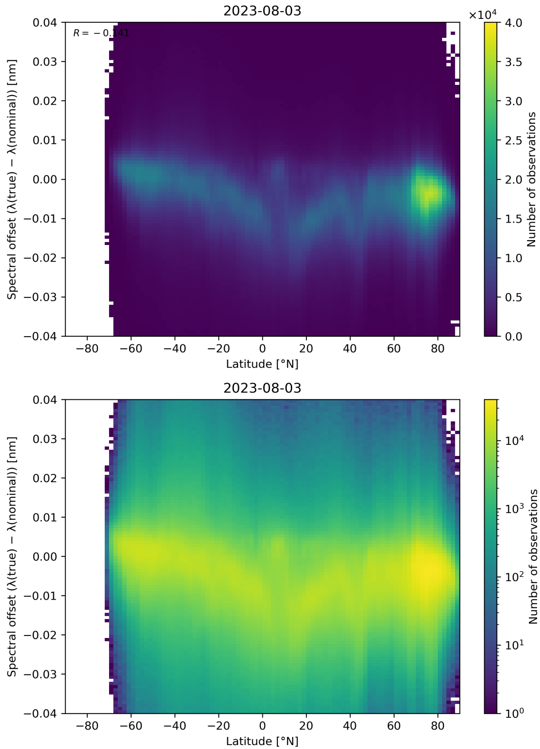
Figure 105: Scatter density plot of “Latitude” against “Spectral offset ( \lambda(\text{true}) - \lambda(\text{nominal}) )” for 2023-08-02 to 2023-08-04.
