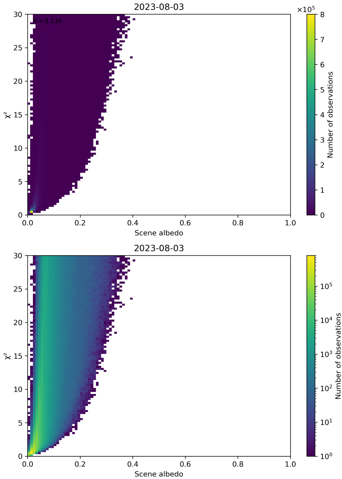
Figure 112: Scatter density plot of “Scene albedo” against “ \chi^2 ” for 2023-08-02 to 2023-08-04.
