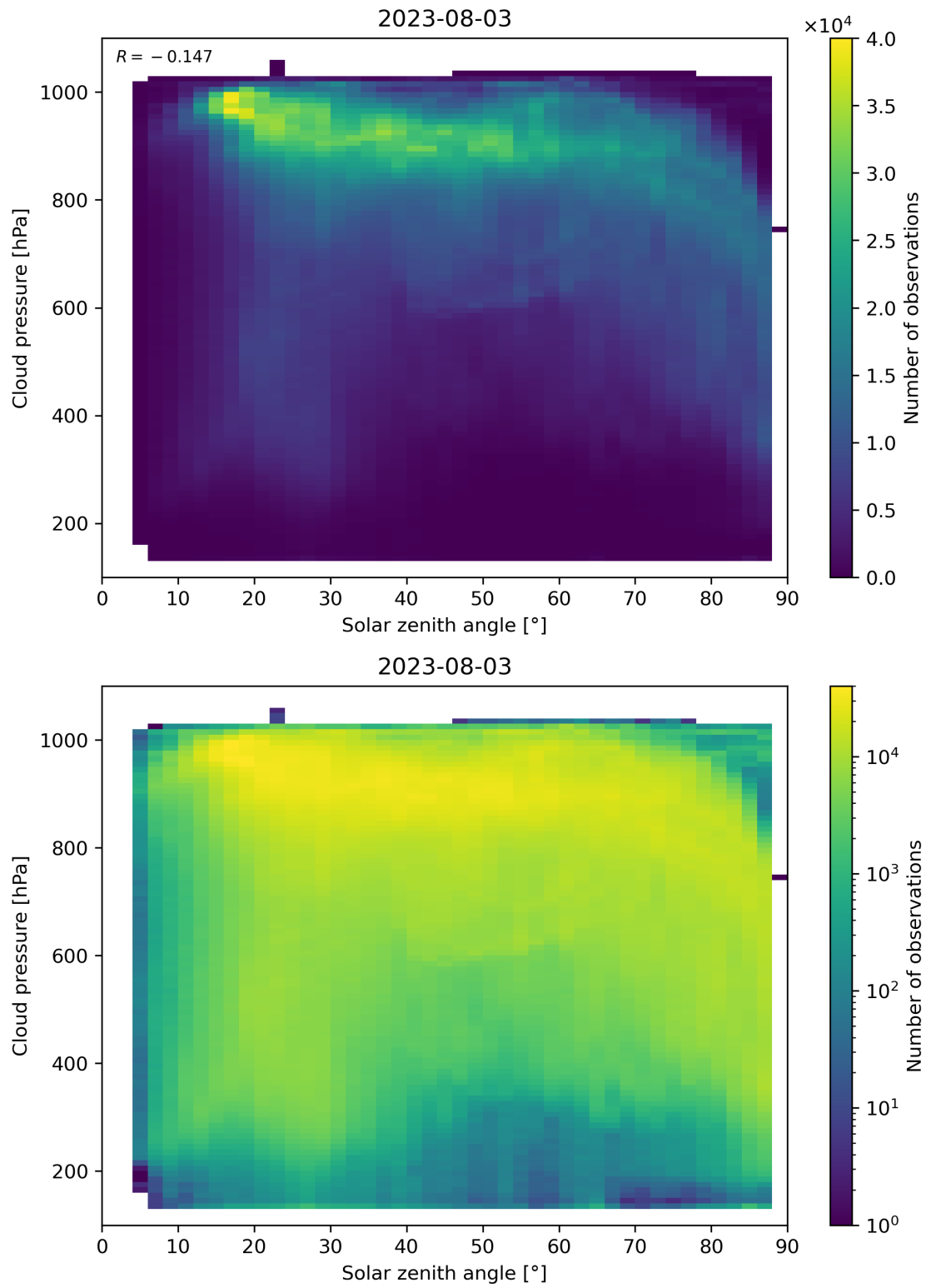
Figure 122: Scatter density plot of “Solar zenith angle” against “Cloud pressure” for 2023-08-02 to 2023-08-04.
