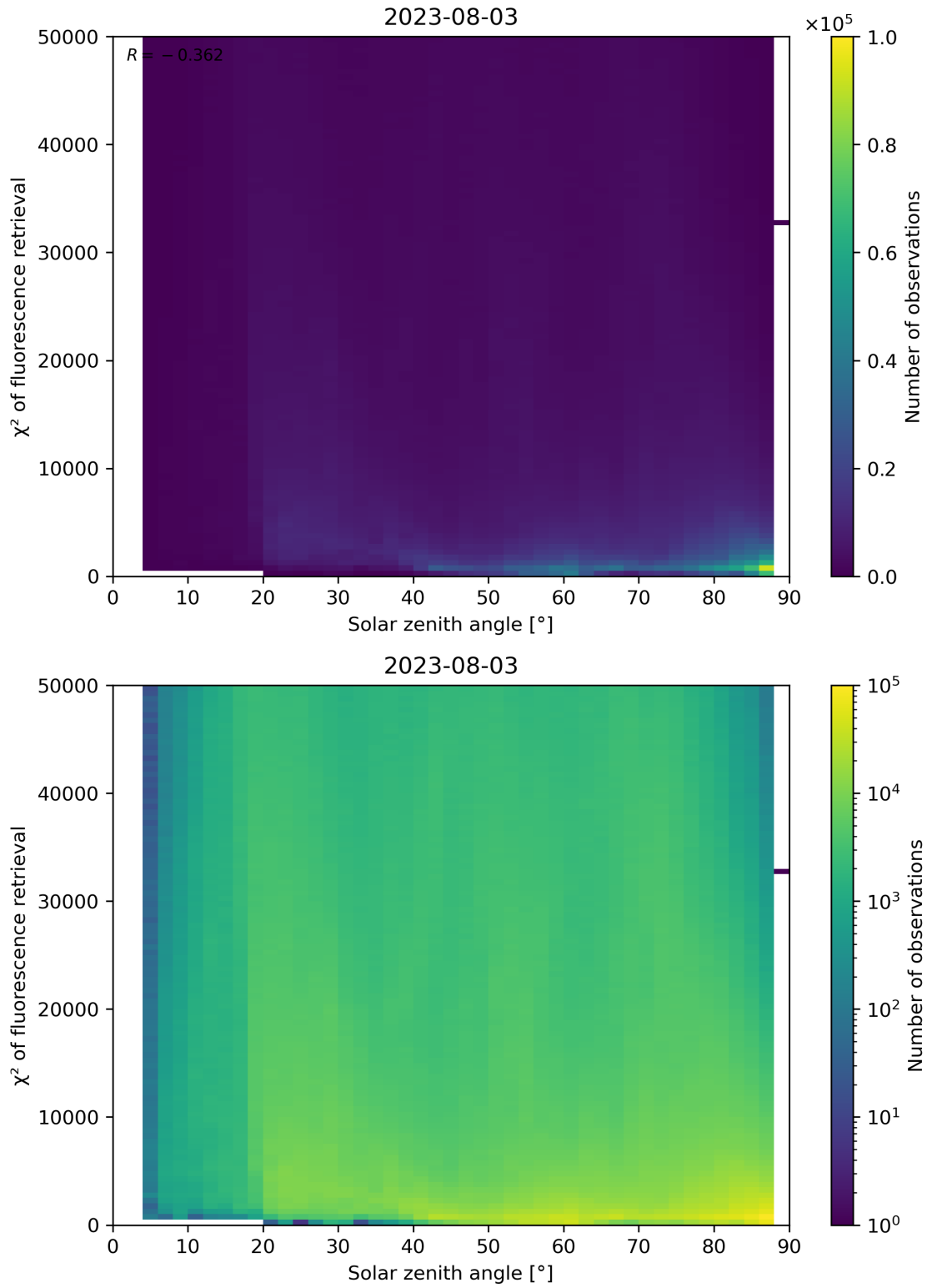
Figure 120: Scatter density plot of “Solar zenith angle” against “ \chi^2 of fluorescence retrieval” for 2023-08-02 to 2023-08-04.
