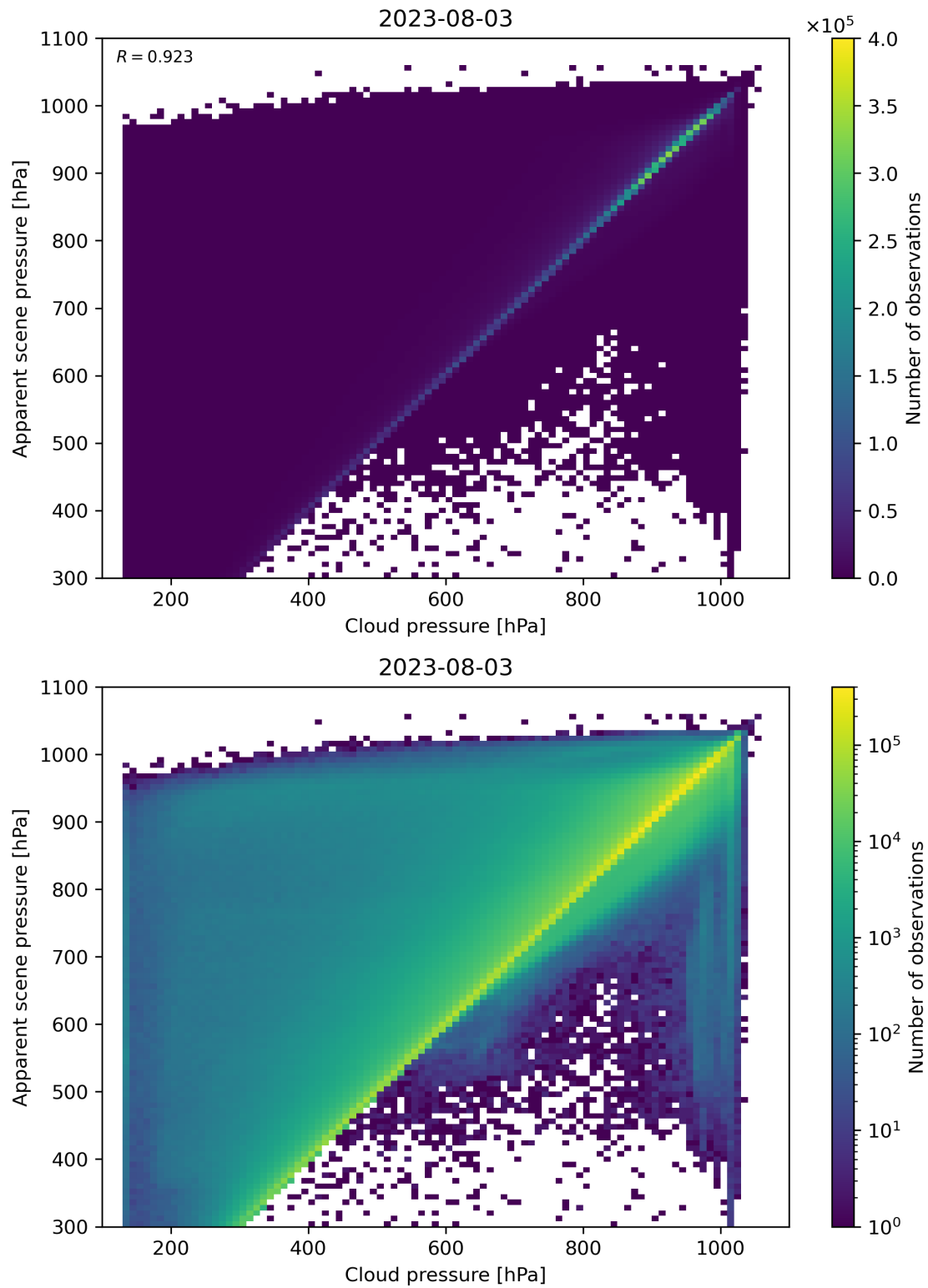
Figure 84: Scatter density plot of “Cloud pressure” against “Apparent scene pressure” for 2023-08-02 to 2023-08-04.
