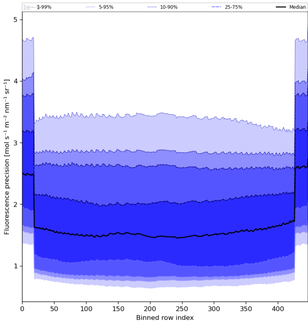
Figure 58: Along track statistics of “Fluorescence precision” for 2023-08-02 to 2023-08-04
