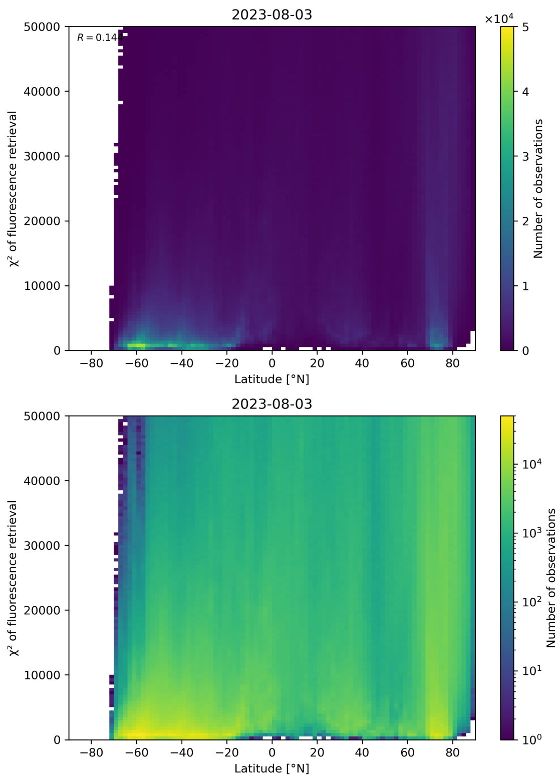
Figure 98: Scatter density plot of “Latitude” against “ \chi^2 of fluorescence retrieval” for 2023-08-02 to 2023-08-04.
