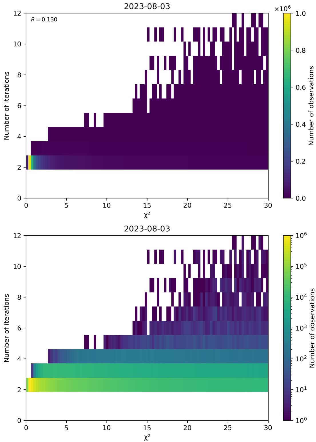
Figure 73: Scatter density plot of “ \chi^2 ” against “Number of iterations” for 2023-08-02 to 2023-08-04.
