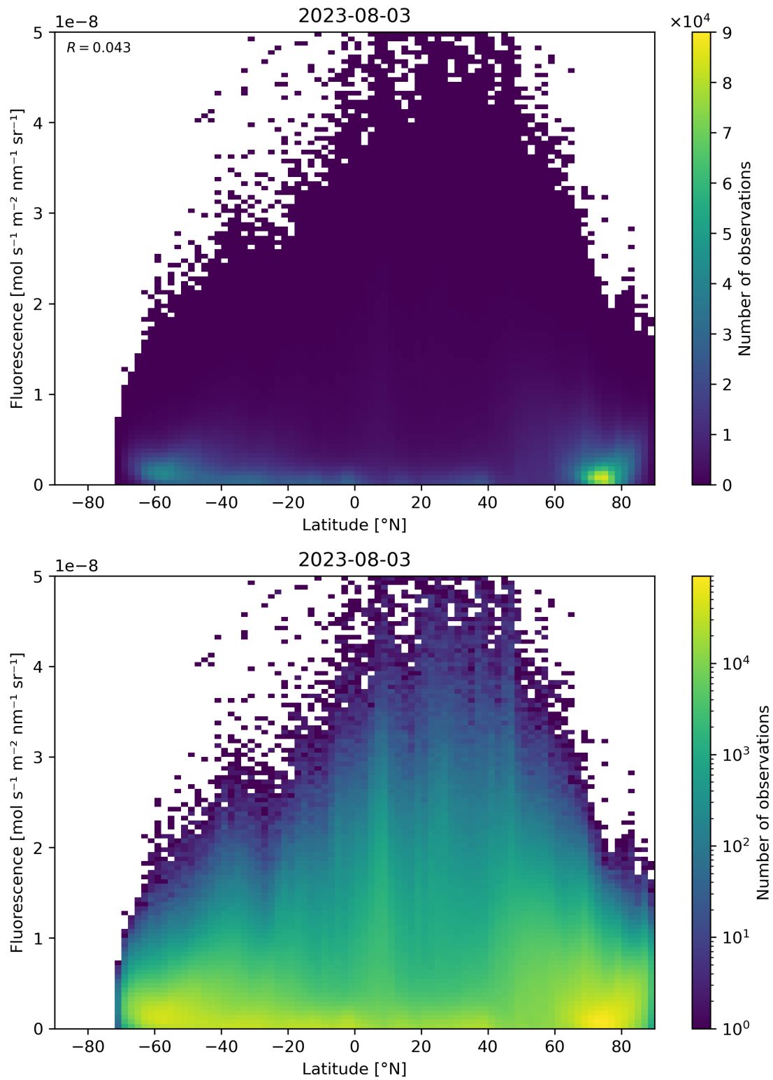
Figure 101: Scatter density plot of “Latitude” against “Fluorescence” for 2023-08-02 to 2023-08-04.
