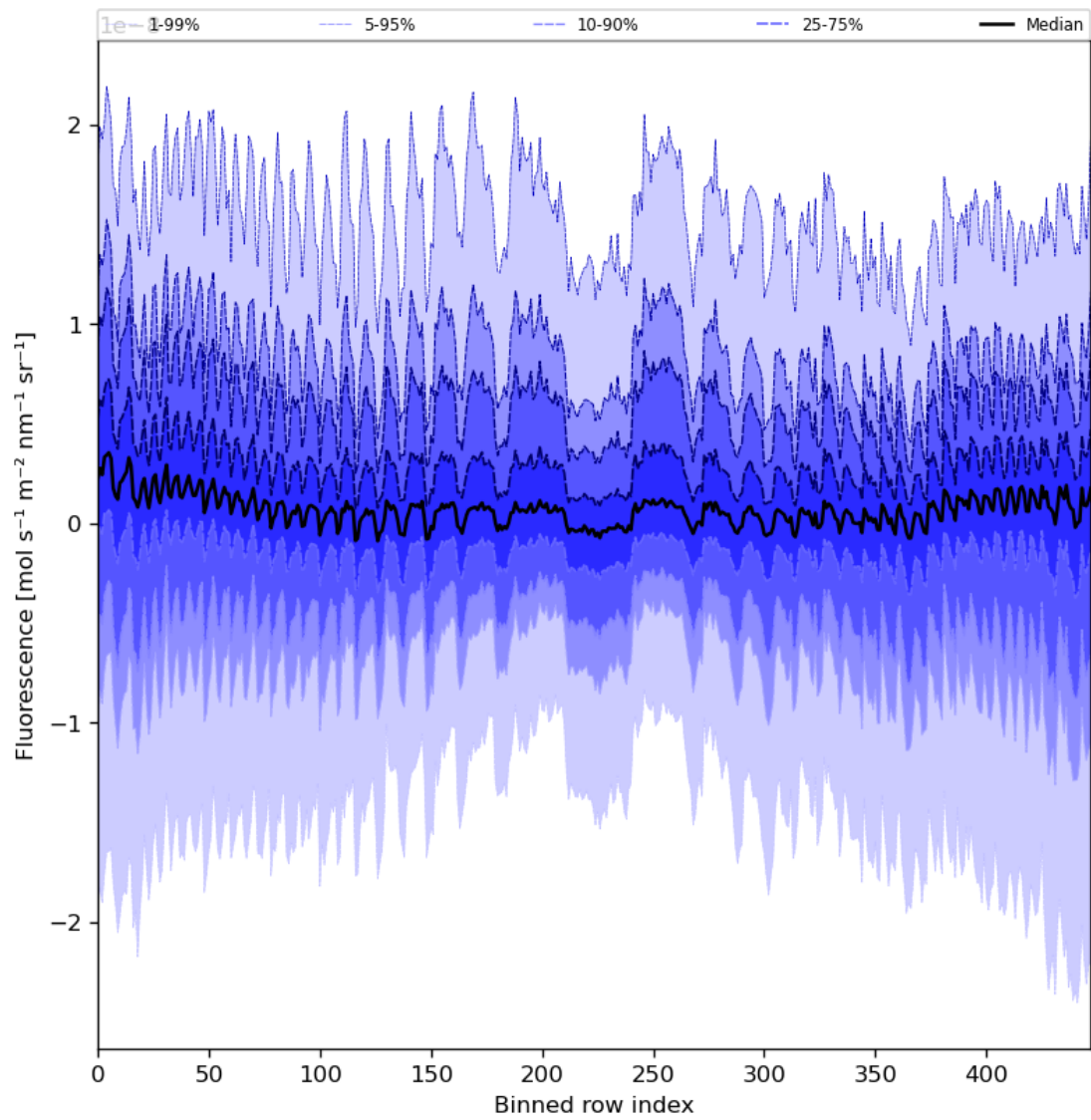
Figure 57: Along track statistics of “Fluorescence” for 2023-08-02 to 2023-08-04
