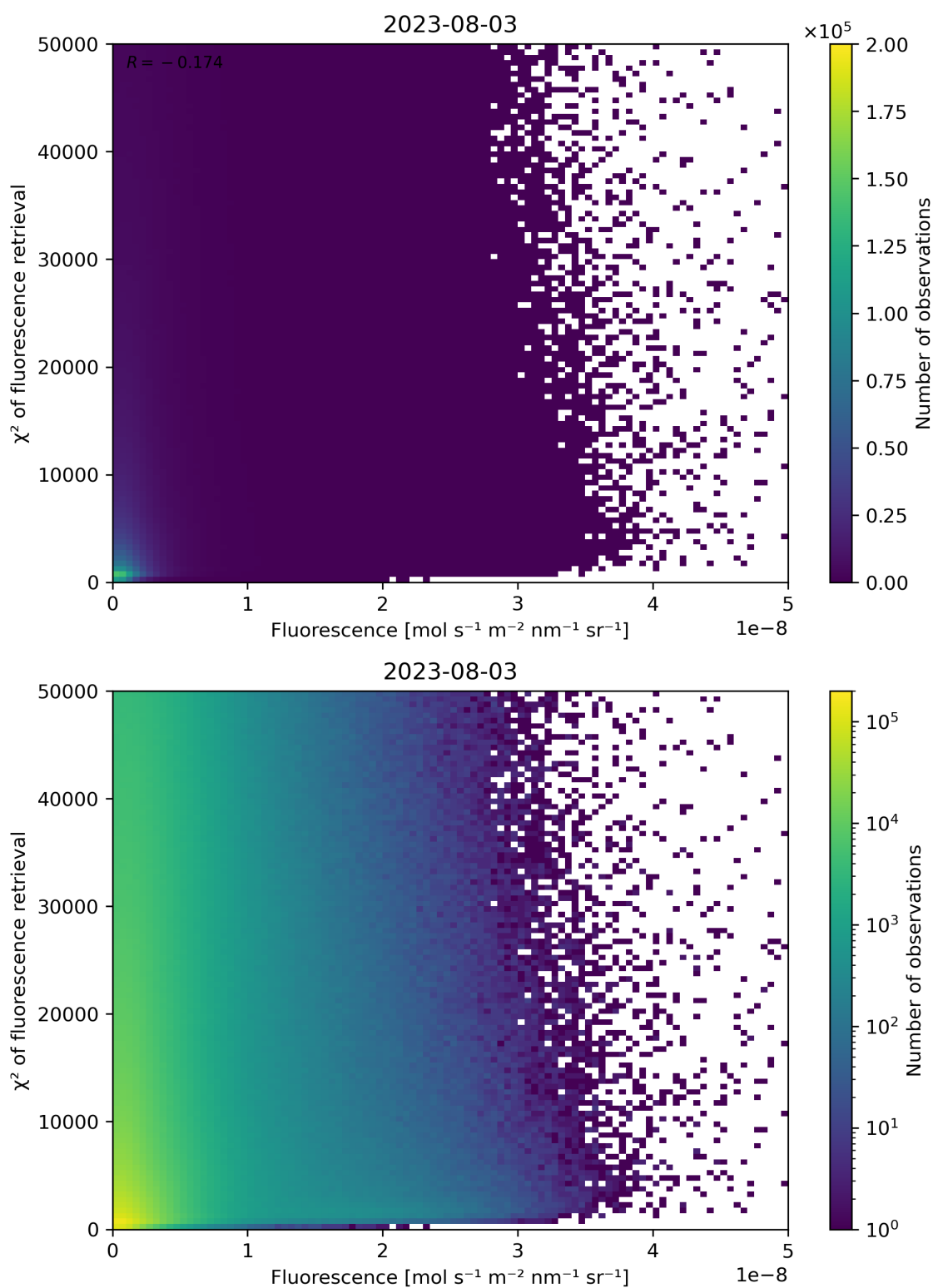
Figure 93: Scatter density plot of “Fluorescence” against “ \chi^2 of fluorescence retrieval” for 2023-08-02 to 2023-08-04.
