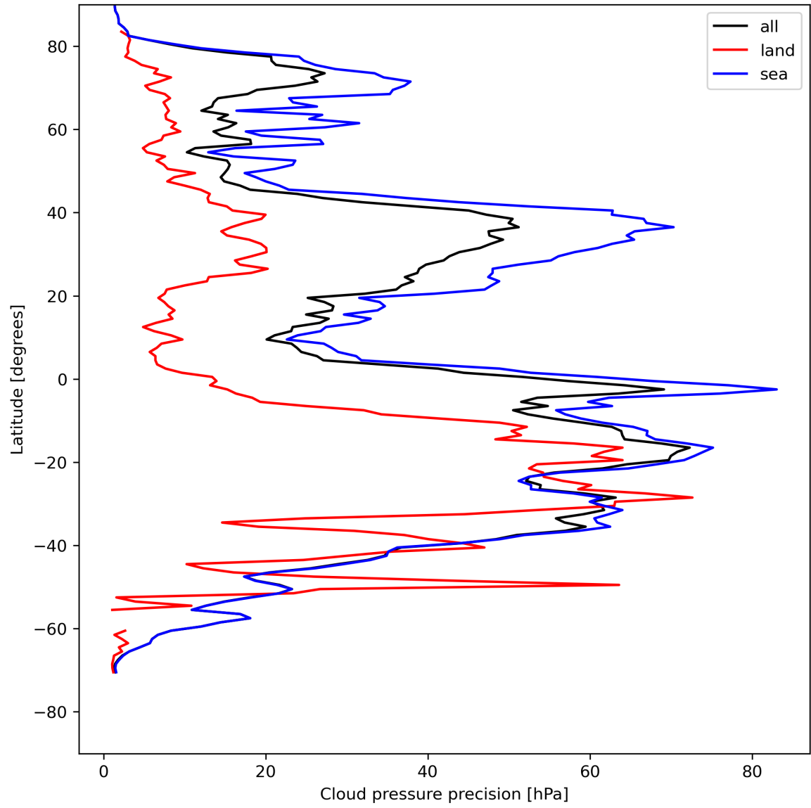
Figure 14: Zonal average of “Cloud pressure precision” for 2023-08-02 to 2023-08-04.
