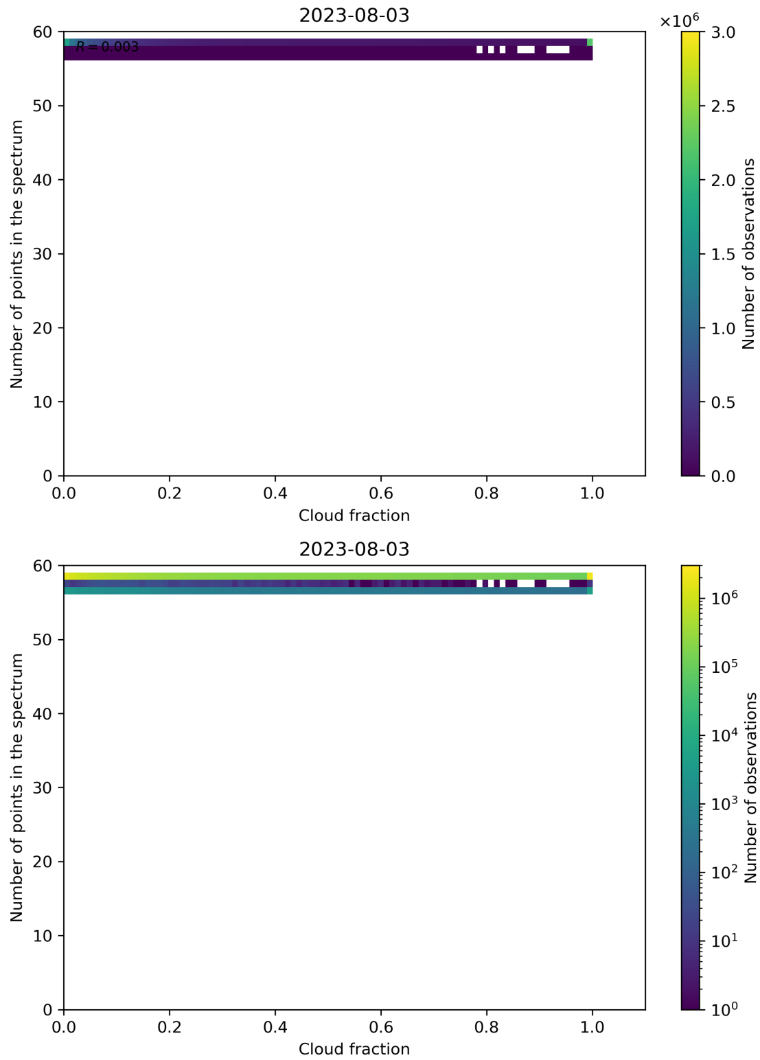
Figure 81: Scatter density plot of “Cloud fraction” against “Number of points in the spectrum” for 2023-08-02 to 2023-08-04.
