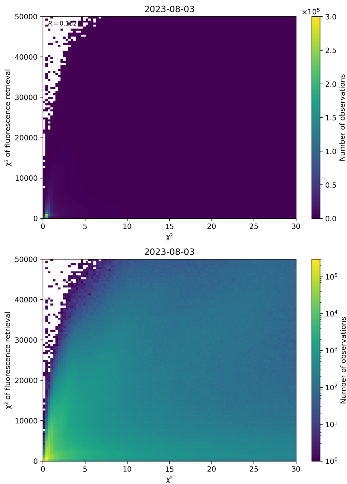
Figure 69: Scatter density plot of “ \chi^2 ” against “ \chi^2 of fluorescence retrieval” for 2023-08-02 to 2023-08-04.
