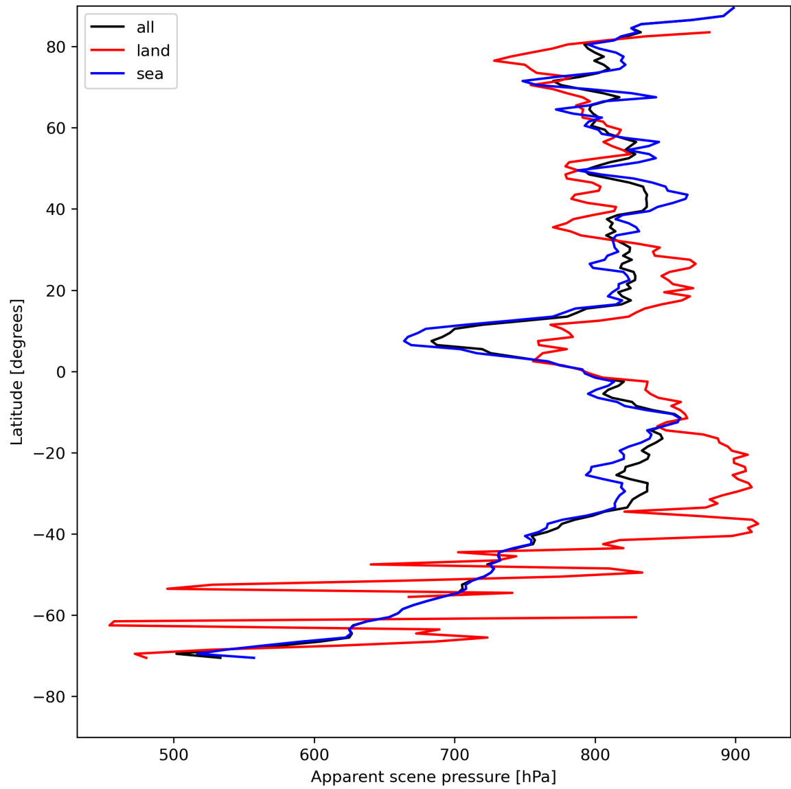
Figure 19: Zonal average of “Apparent scene pressure” for 2023-08-02 to 2023-08-04.
