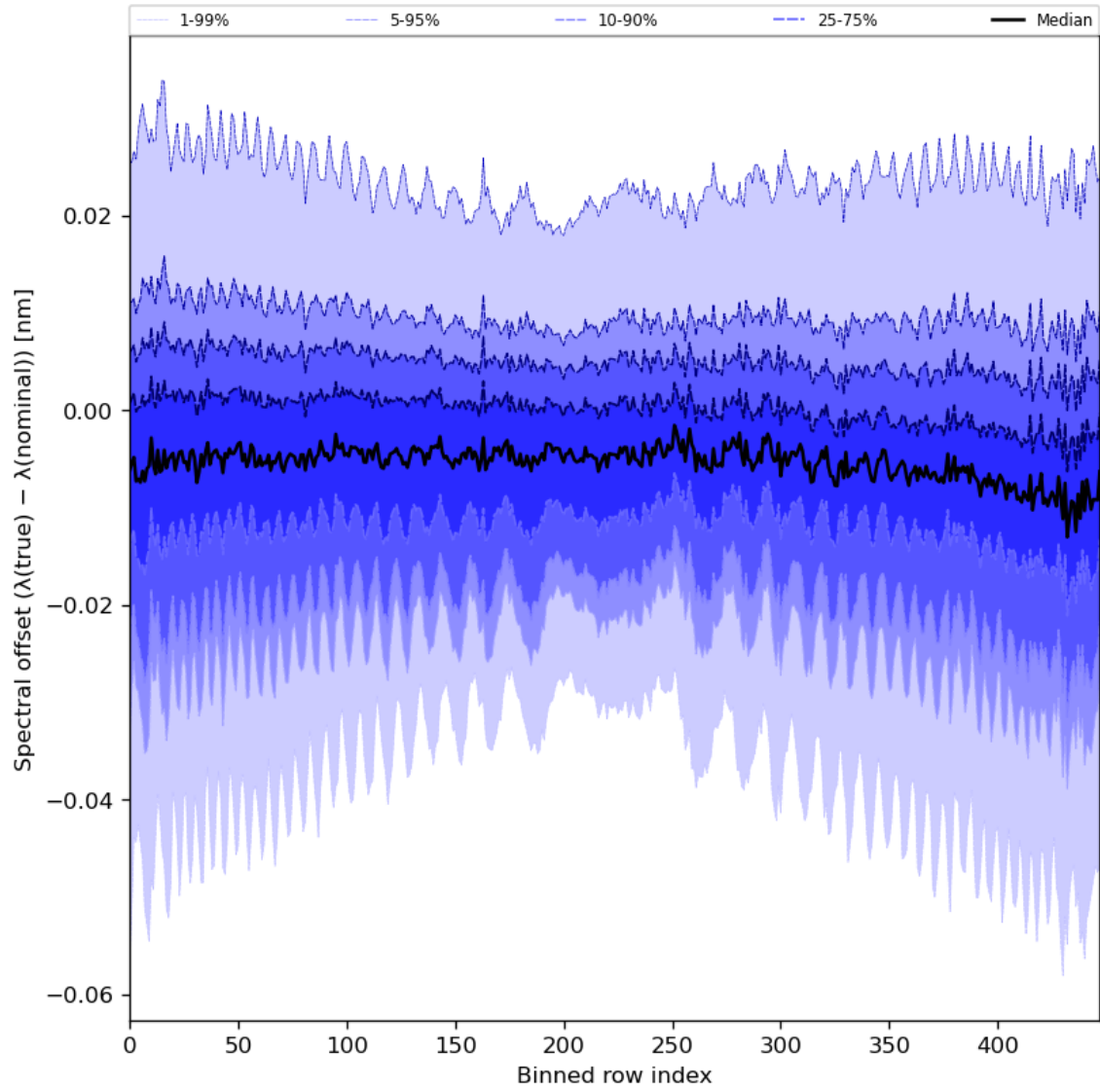
Figure 62: Along track statistics of “Spectral offset ( \lambda(\text{true}) - \lambda(\text{nominal}) )” for 2023-08-02 to 2023-08-04
