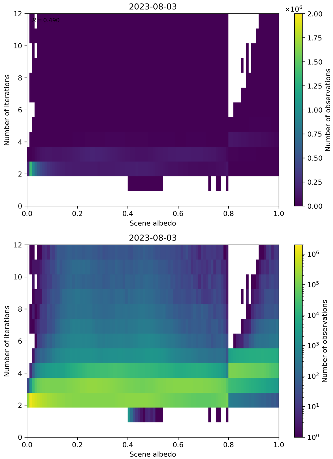
Figure 115: Scatter density plot of “Scene albedo” against “Number of iterations” for 2023-08-02 to 2023-08-04.
