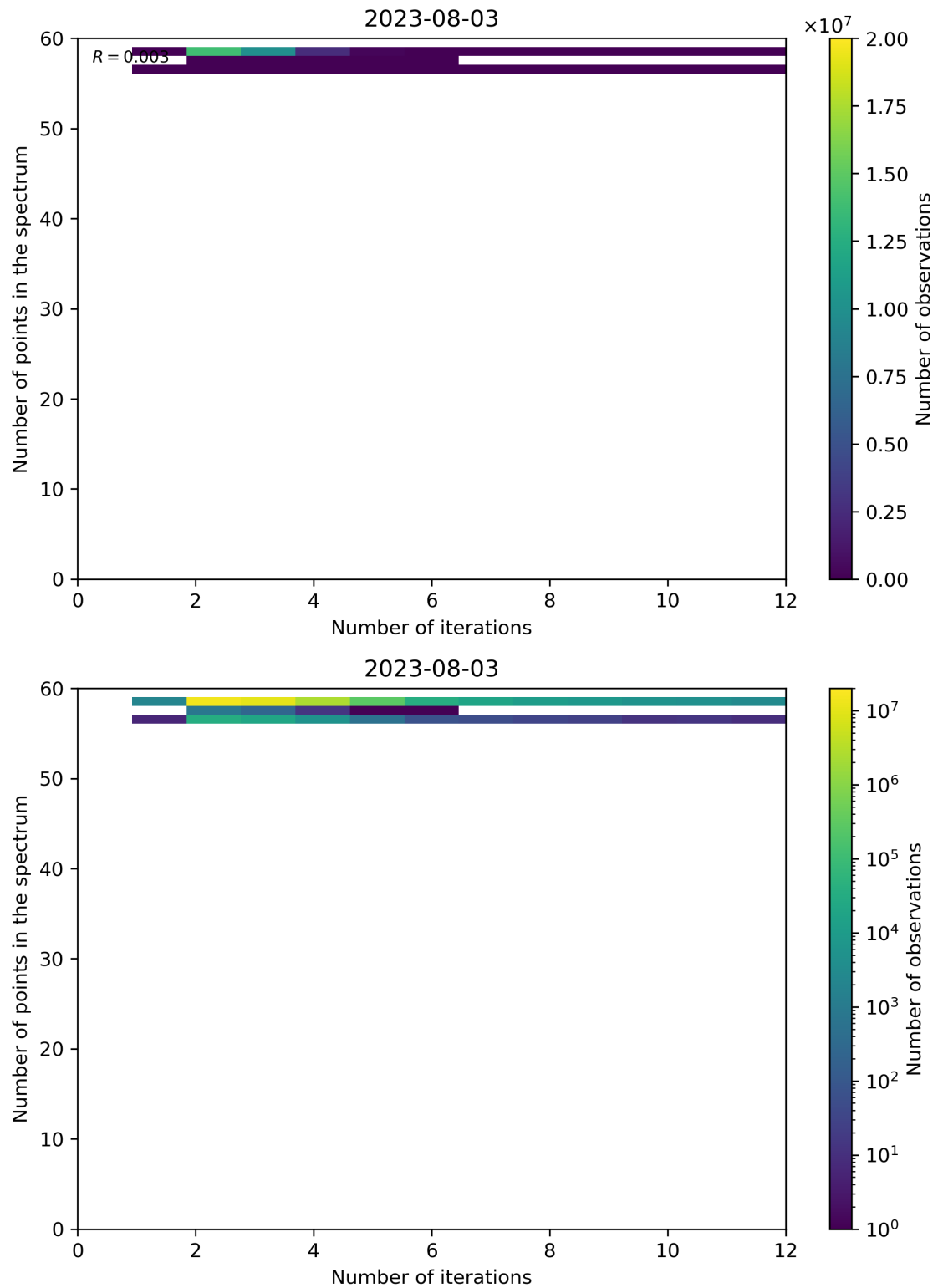
Figure 108: Scatter density plot of “Number of iterations” against “Number of points in the spectrum” for 2023-08-02 to 2023-08-04.
