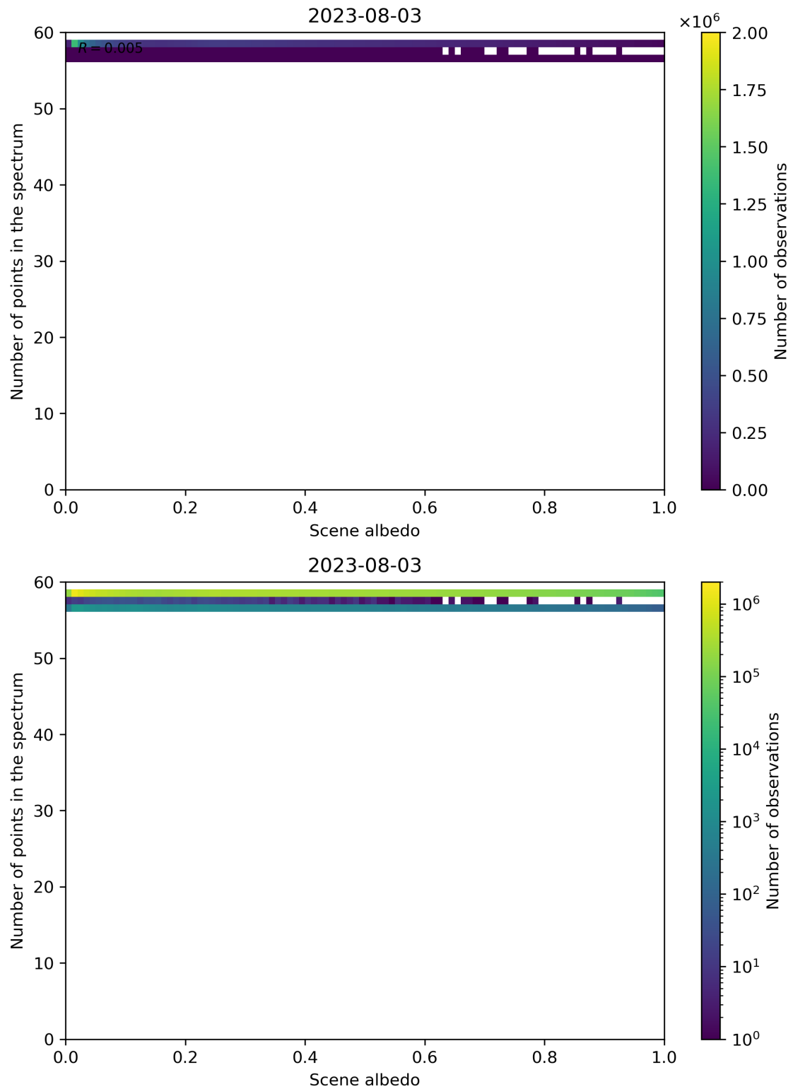
Figure 116: Scatter density plot of “Scene albedo” against “Number of points in the spectrum” for 2023-08-02 to 2023-08-04.
