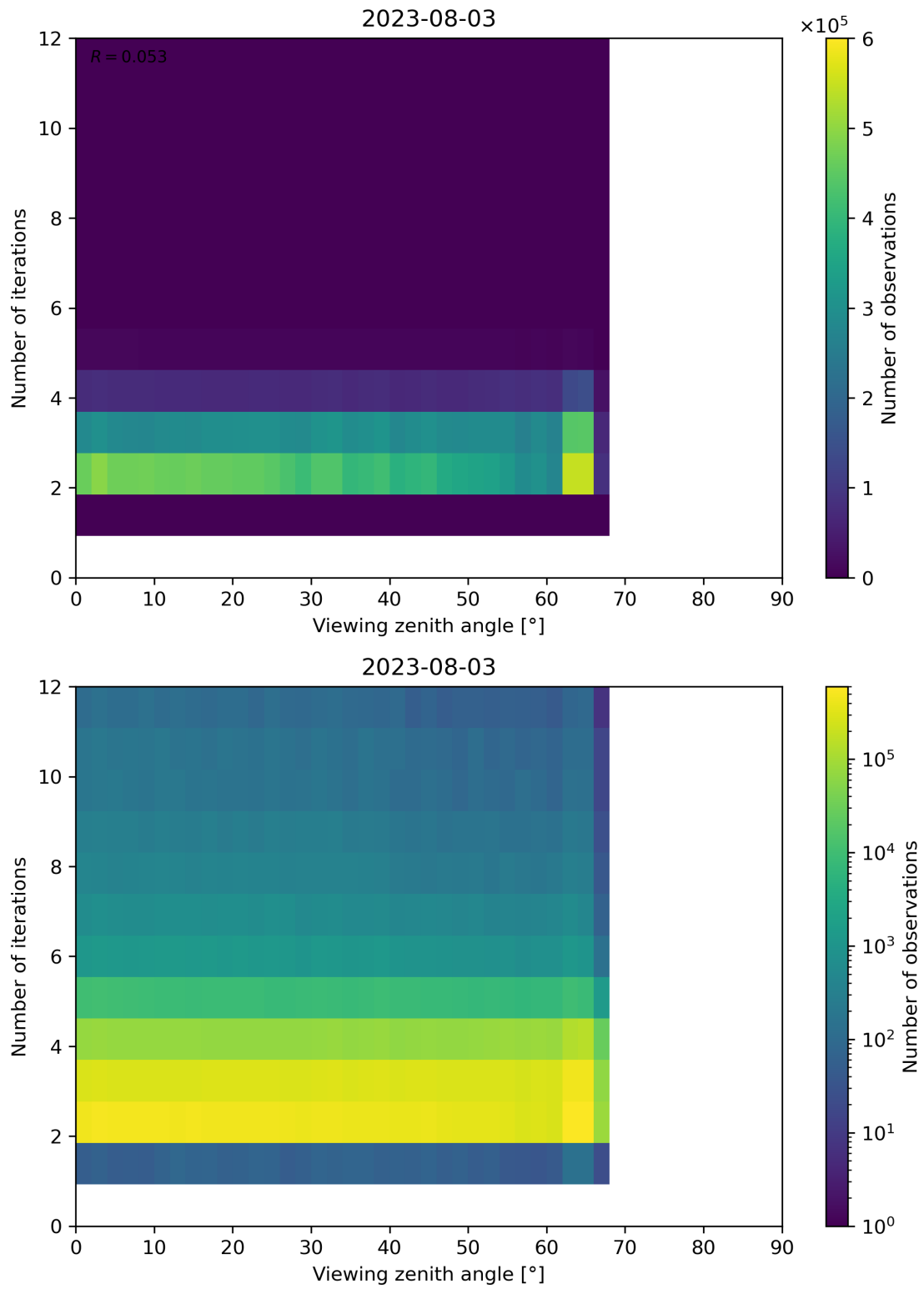
Figure 136: Scatter density plot of “Viewing zenith angle” against “Number of iterations” for 2023-08-02 to 2023-08-04.
