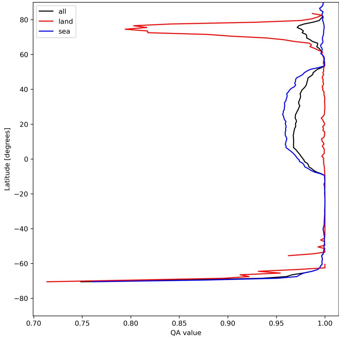
Figure 12: Zonal average of “QA value” for 2023-08-02 to 2023-08-04.
