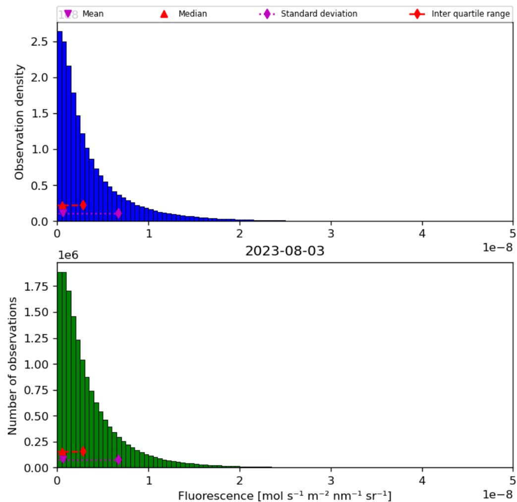
Figure 40: Histogram of “Fluorescence” for 2023-08-02 to 2023-08-04
