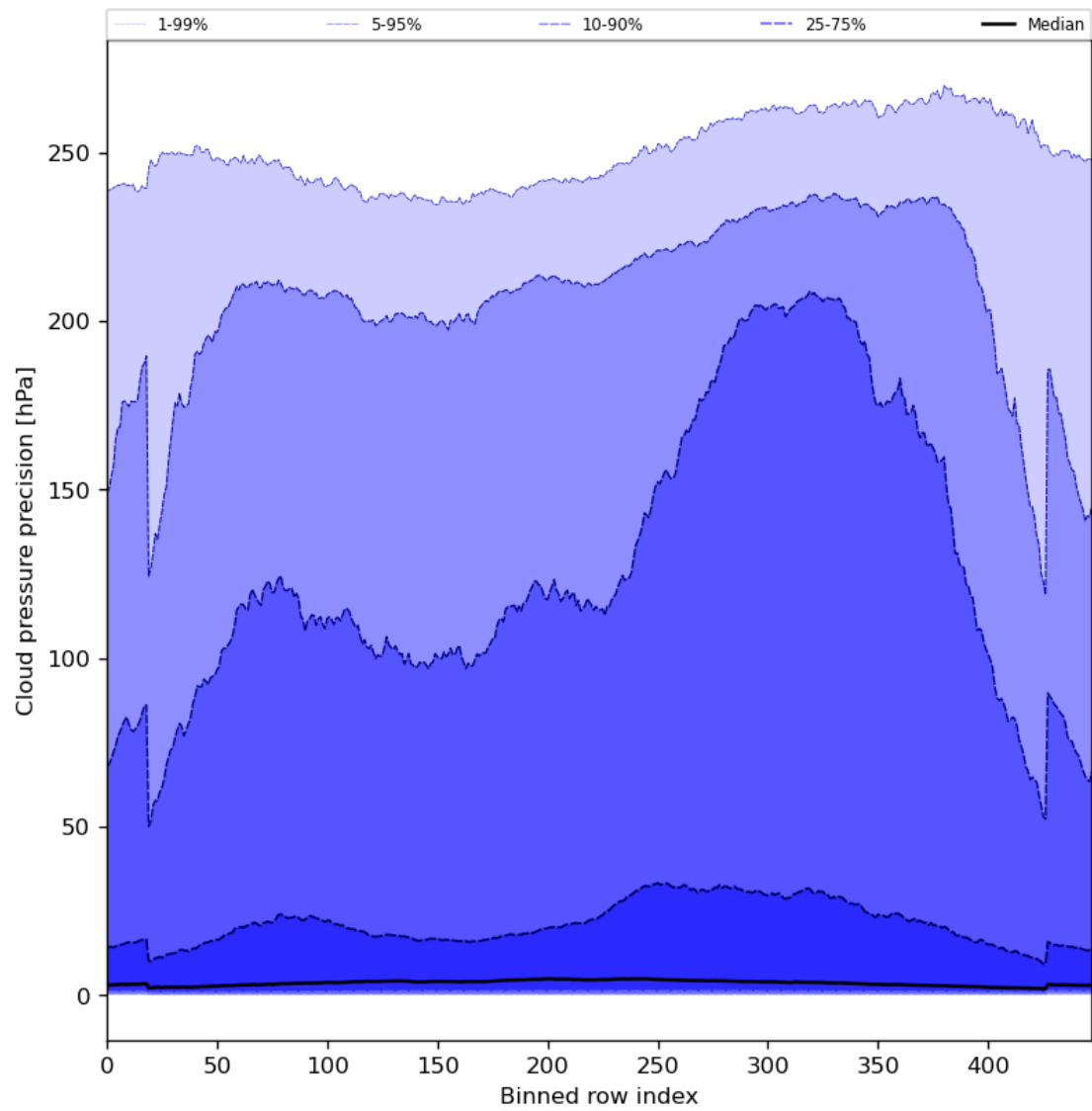
Figure 48: Along track statistics of “Cloud pressure precision” for 2023-08-02 to 2023-08-04
