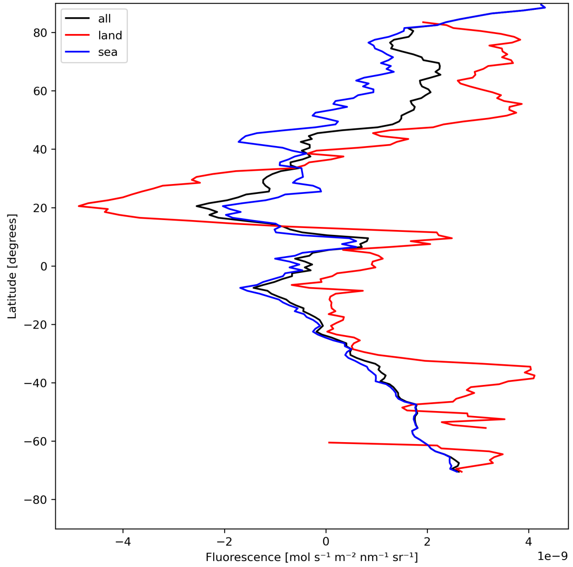
Figure 23: Zonal average of “Fluorescence” for 2023-08-02 to 2023-08-04.
