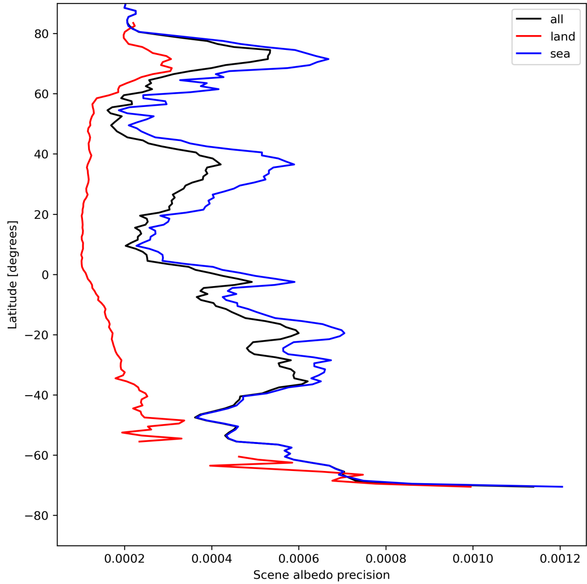
Figure 18: Zonal average of “Scene albedo precision” for 2023-08-02 to 2023-08-04.
