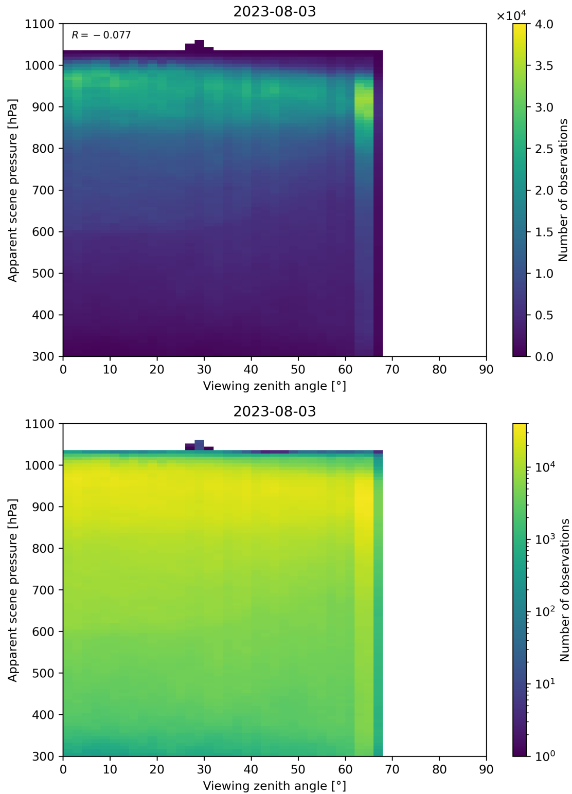
Figure 129: Scatter density plot of “Viewing zenith angle” against “Apparent scene pressure” for 2023-08-02 to 2023-08-04.
