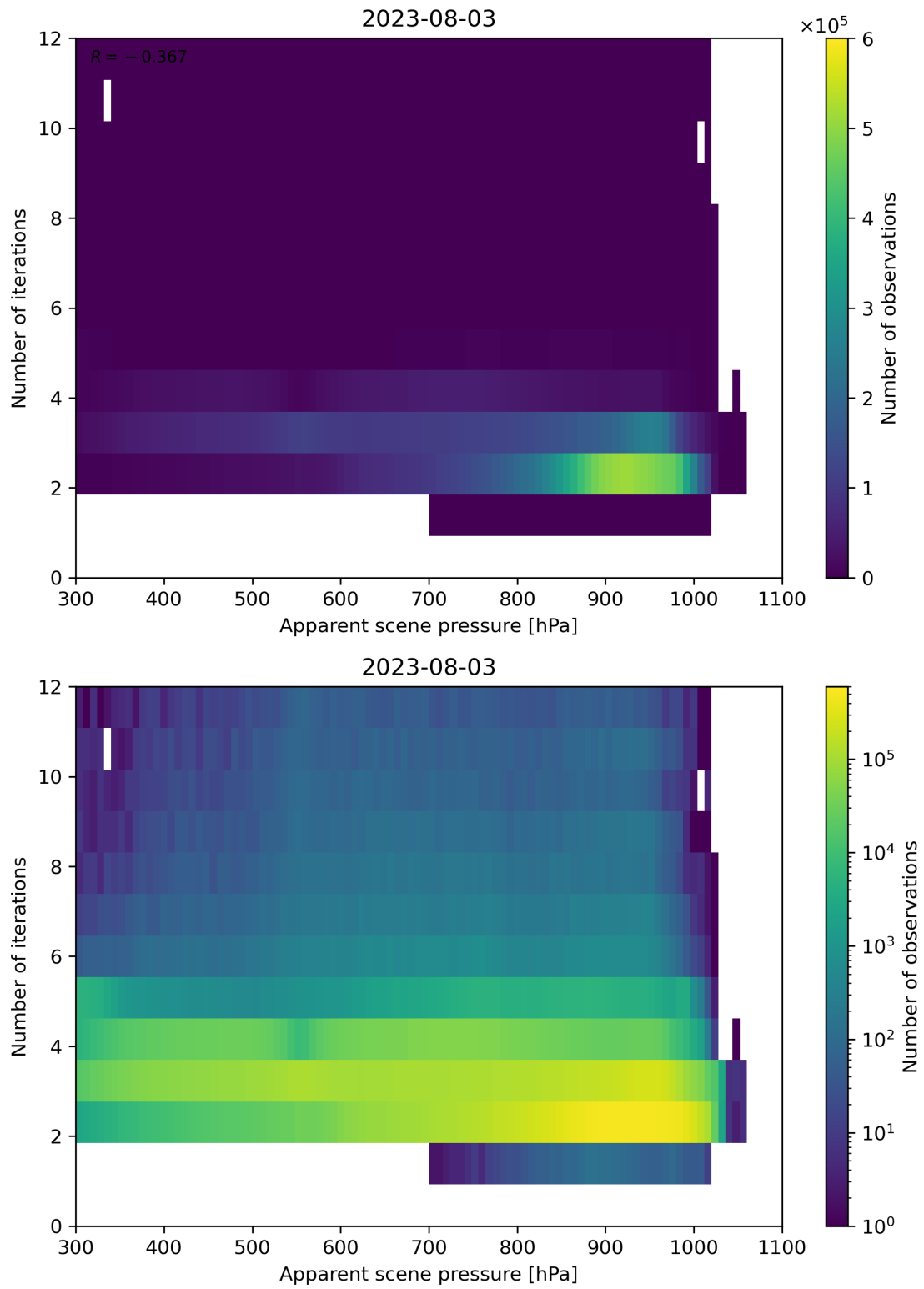
Figure 66: Scatter density plot of “Apparent scene pressure” against “Number of iterations” for 2023-08-02 to 2023-08-04.
