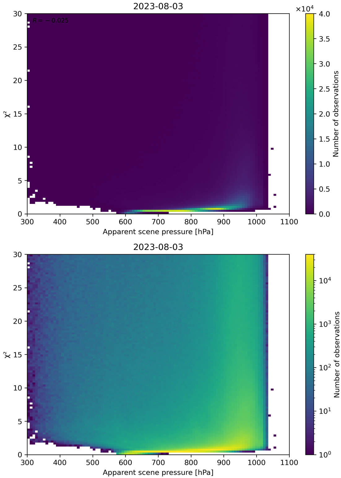
Figure 63: Scatter density plot of “Apparent scene pressure” against “ \chi^2 ” for 2023-08-02 to 2023-08-04.
