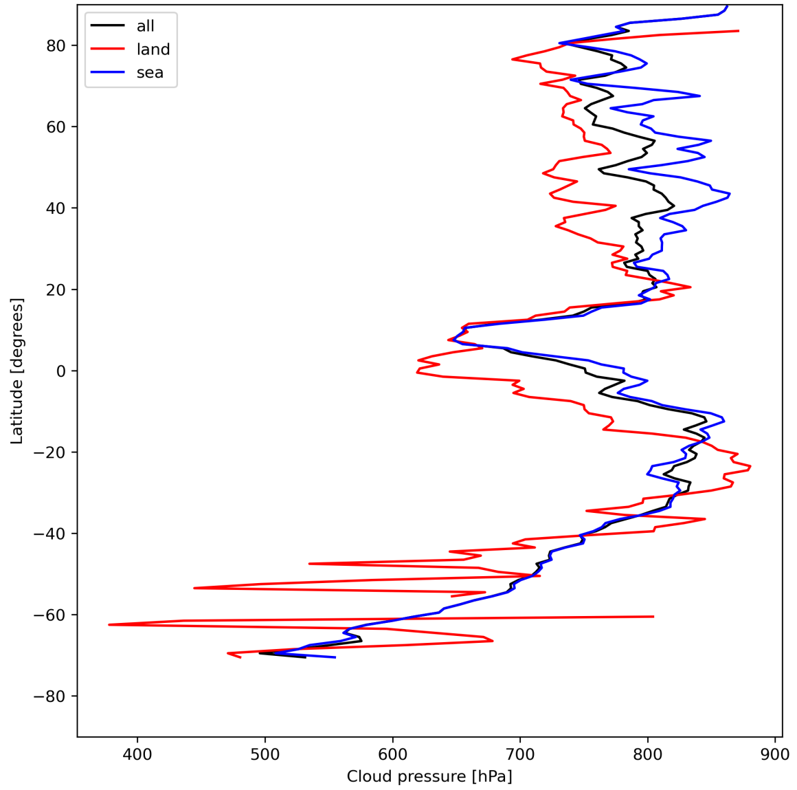
Figure 13: Zonal average of “Cloud pressure” for 2023-08-02 to 2023-08-04.
