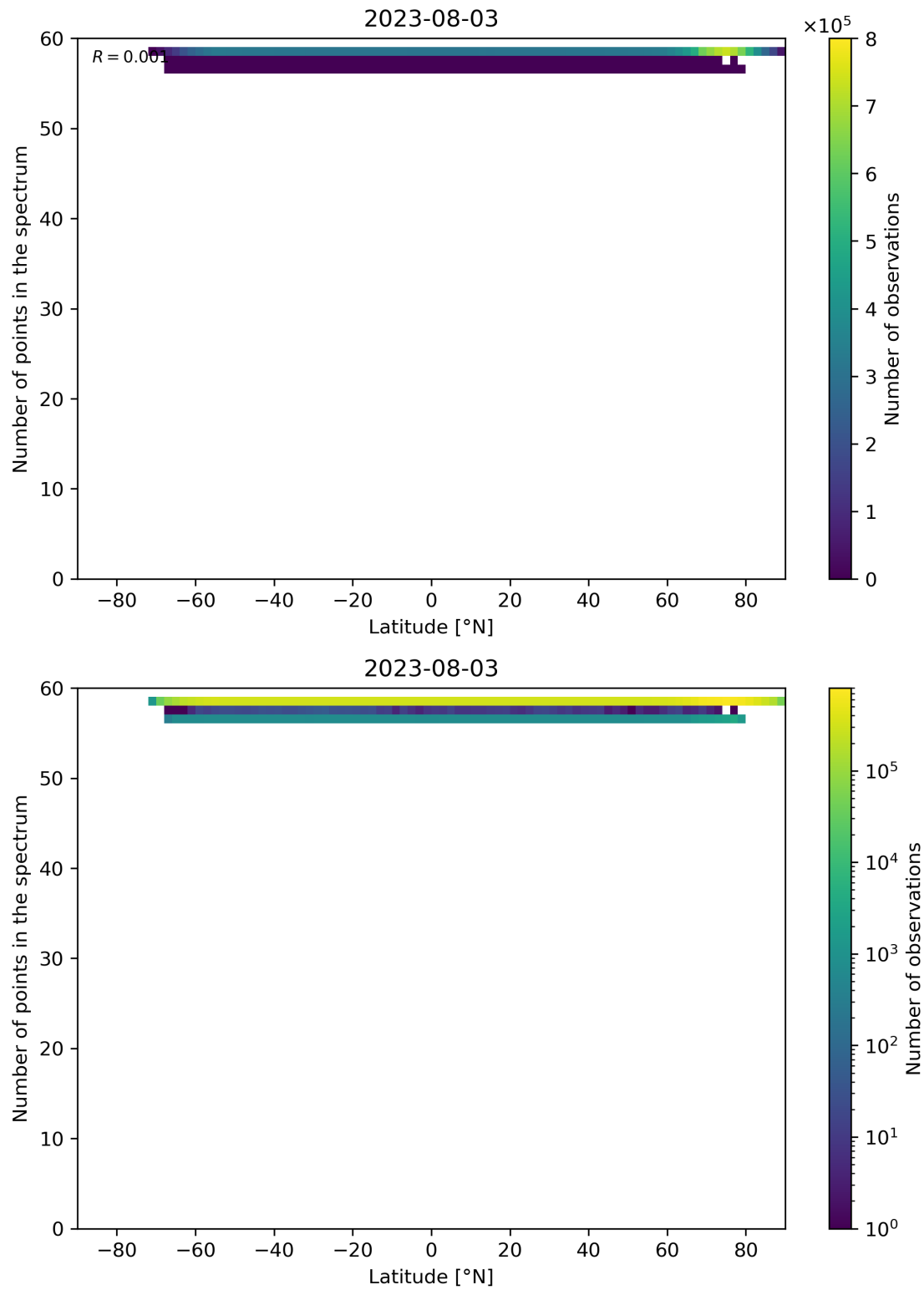
Figure 103: Scatter density plot of “Latitude” against “Number of points in the spectrum” for 2023-08-02 to 2023-08-04.
