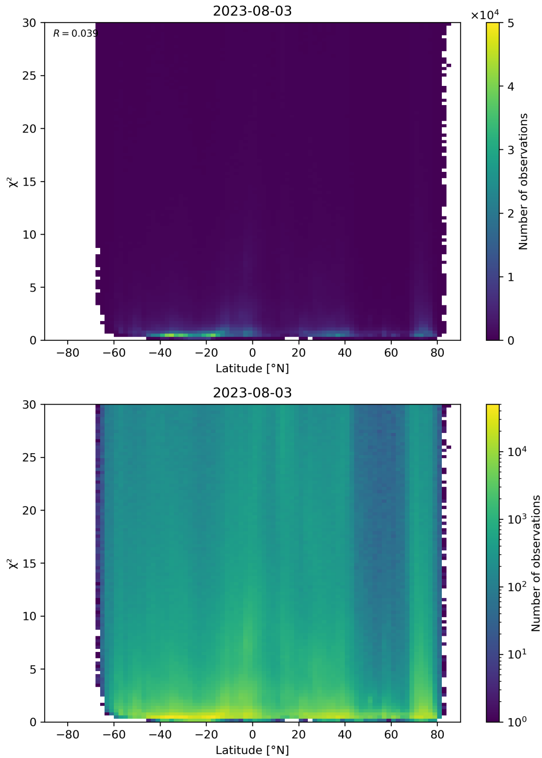
Figure 97: Scatter density plot of “Latitude” against “ \chi^2 ” for 2023-08-02 to 2023-08-04.
