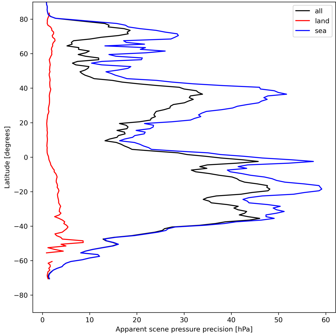
Figure 20: Zonal average of “Apparent scene pressure precision” for 2023-08-02 to 2023-08-04.
