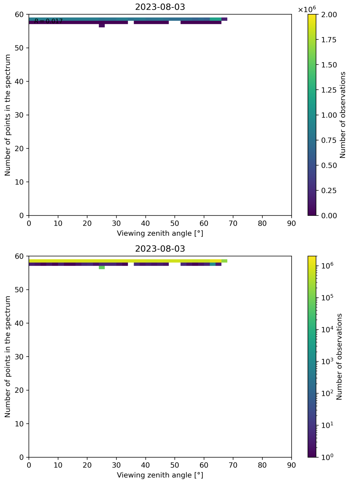
Figure 137: Scatter density plot of “Viewing zenith angle” against “Number of points in the spectrum” for 2023-08-02 to 2023-08-04.
