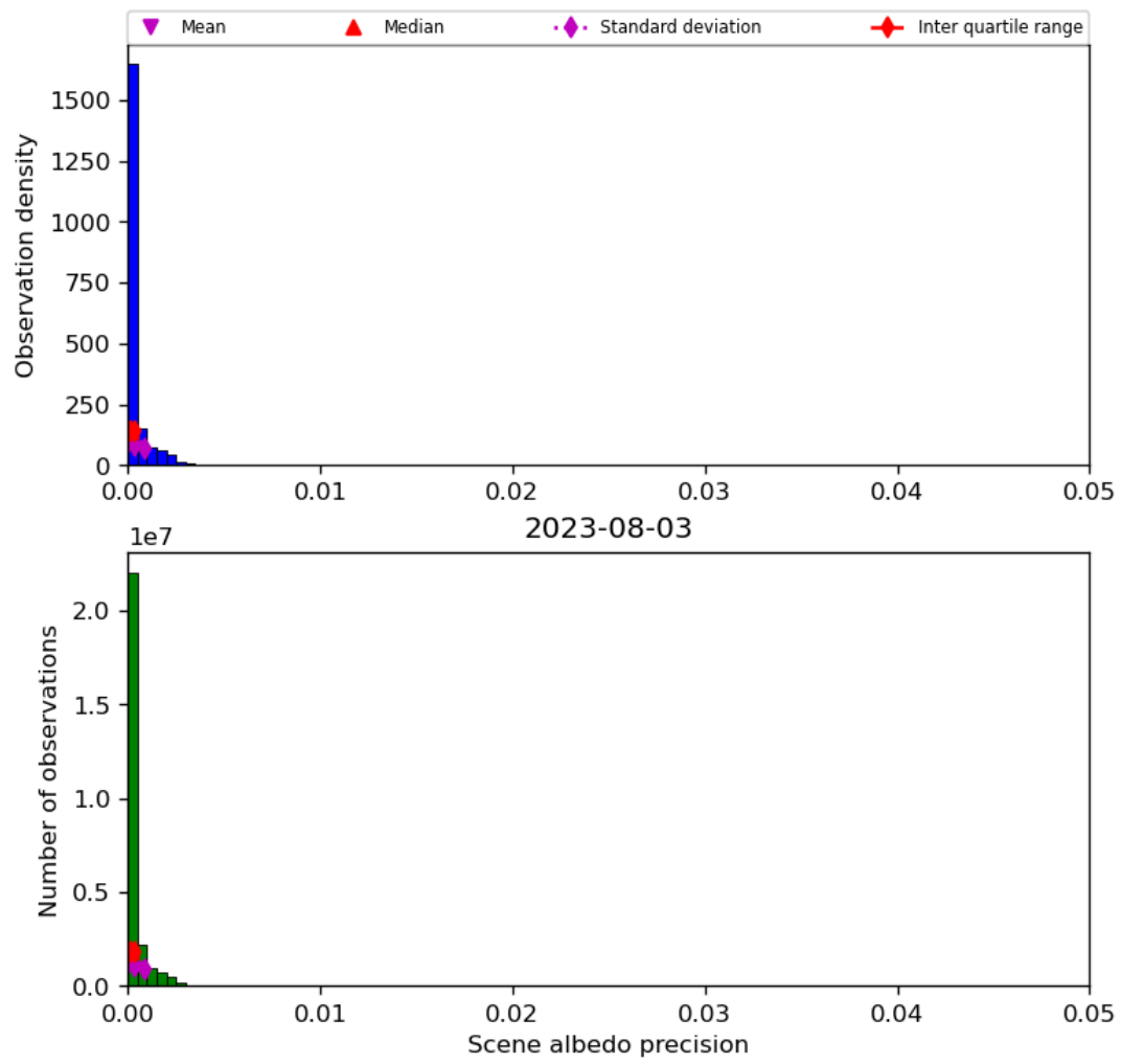
Figure 35: Histogram of “Scene albedo precision” for 2023-08-02 to 2023-08-04
