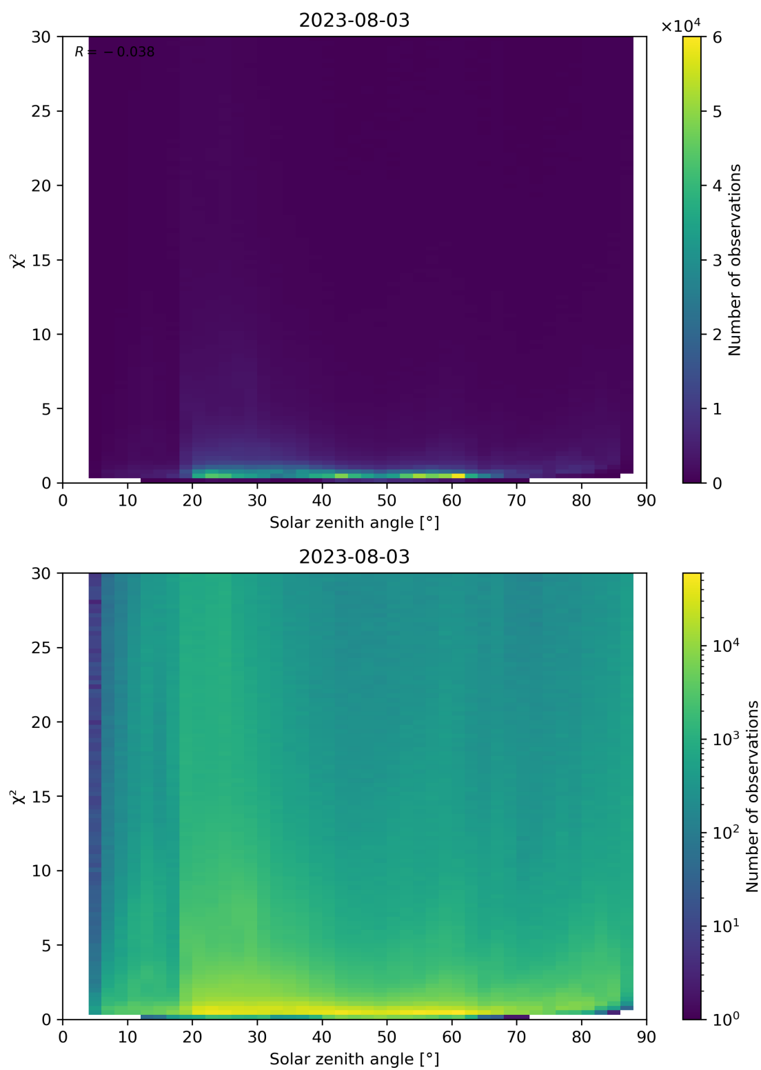
Figure 119: Scatter density plot of “Solar zenith angle” against “ \chi^2 ” for 2023-08-02 to 2023-08-04.
