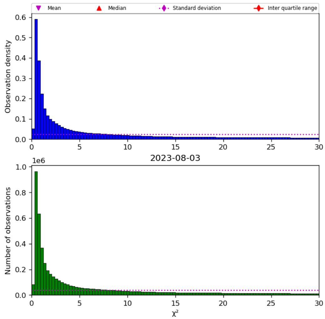
Figure 38: Histogram of “ \chi^2 ” for 2023-08-02 to 2023-08-04
