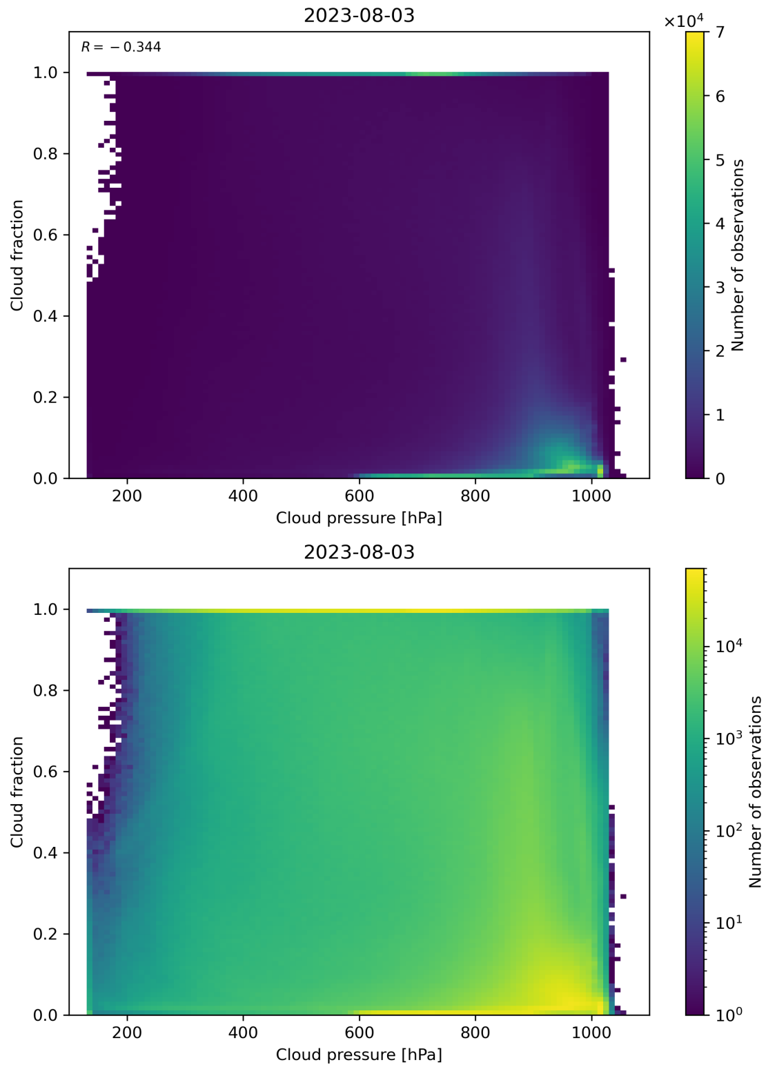
Figure 87: Scatter density plot of “Cloud pressure” against “Cloud fraction” for 2023-08-02 to 2023-08-04.
