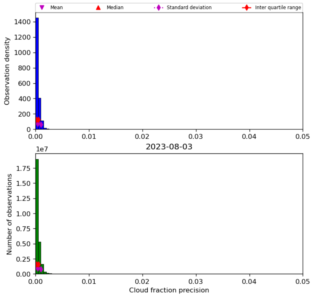
Figure 33: Histogram of “Cloud fraction precision” for 2023-08-02 to 2023-08-04
