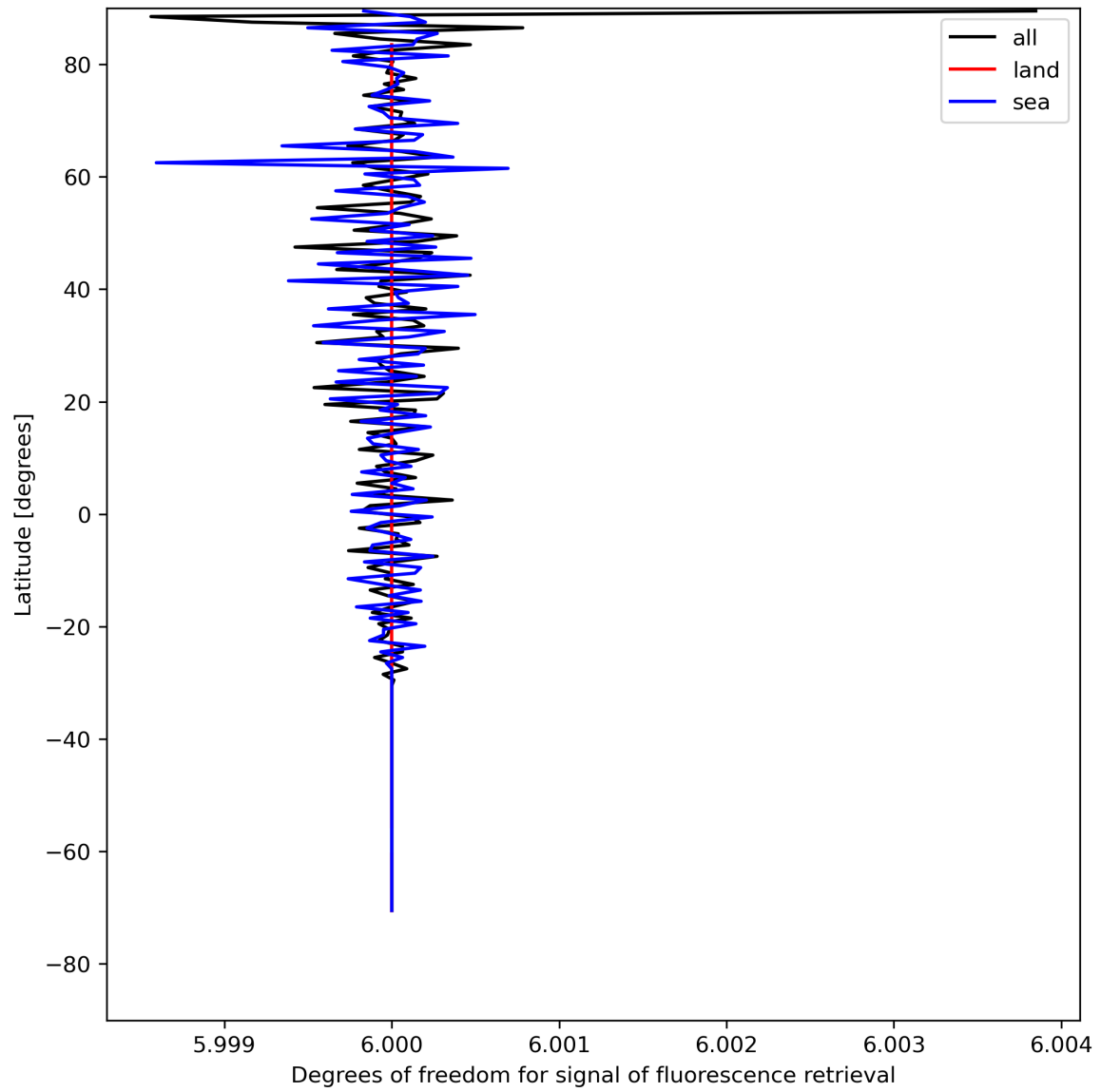
Figure 26: Zonal average of “Degrees of freedom for signal of fluorescence retrieval” for 2023-08-02 to 2023-08-04.
