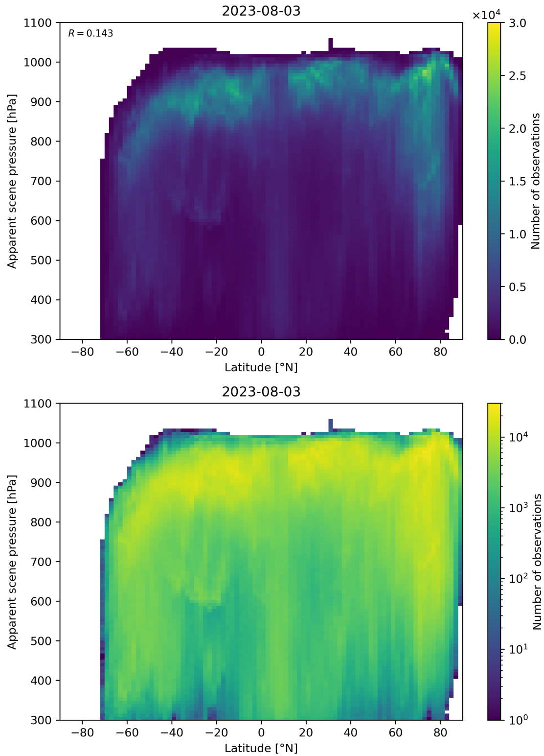
Figure 96: Scatter density plot of “Latitude” against “Apparent scene pressure” for 2023-08-02 to 2023-08-04.
