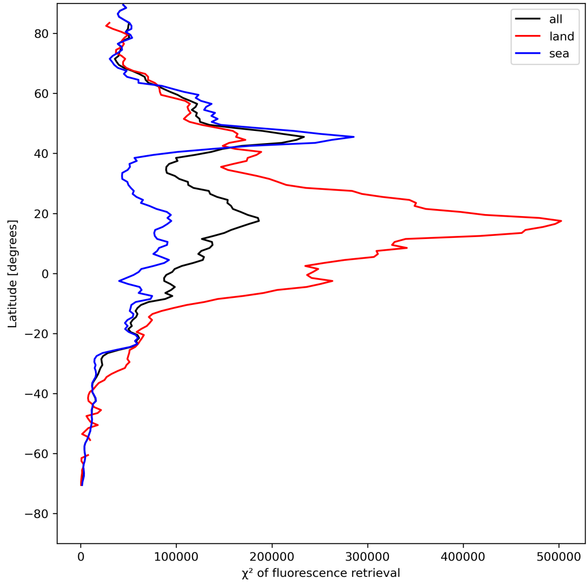
Figure 25: Zonal average of “ \chi^2 of fluorescence retrieval” for 2023-08-02 to 2023-08-04.
