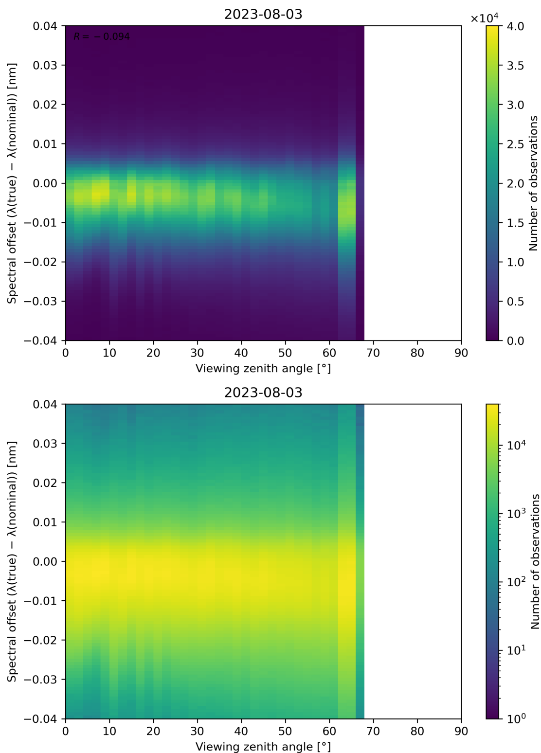
Figure 140: Scatter density plot of “Viewing zenith angle” against “Spectral offset ( \lambda(\text{true}) - \lambda(\text{nominal}) )” for 2023-08-02 to 2023-08-04.
