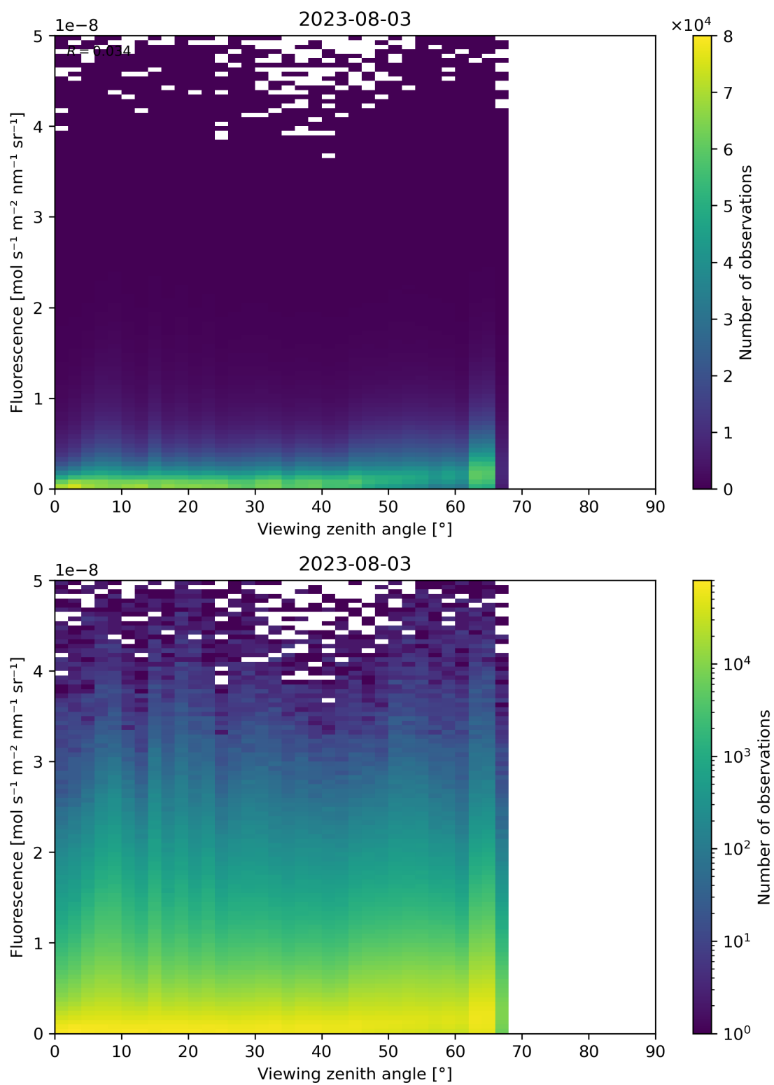
Figure 134: Scatter density plot of “Viewing zenith angle” against “Fluorescence” for 2023-08-02 to 2023-08-04.
