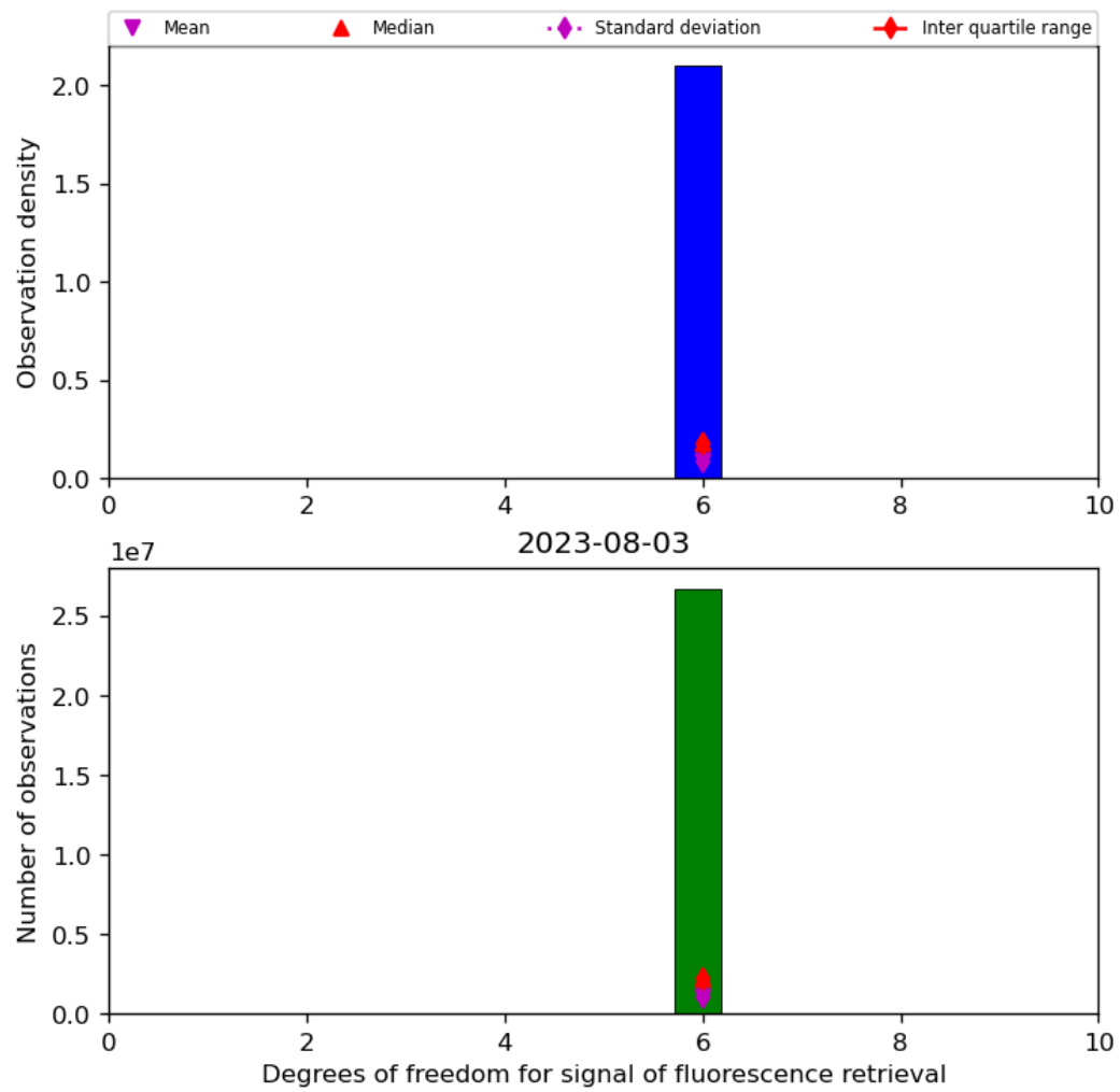
Figure 43: Histogram of “Degrees of freedom for signal of fluorescence retrieval” for 2023-08-02 to 2023-08-04
