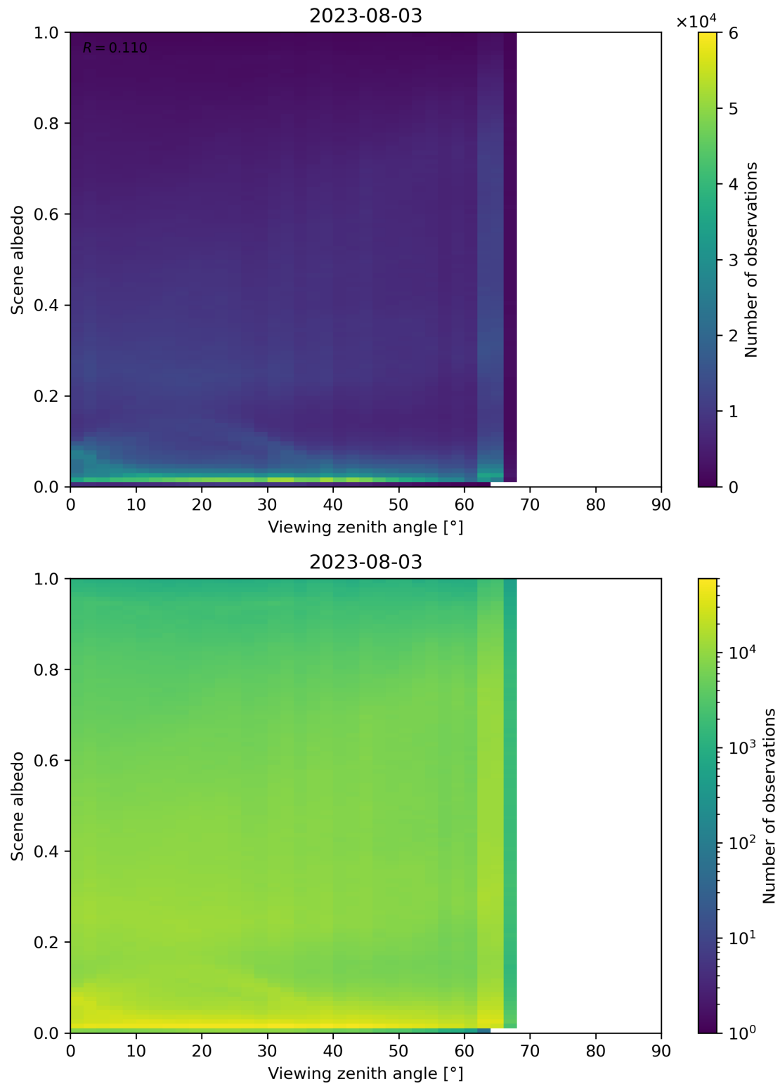
Figure 138: Scatter density plot of “Viewing zenith angle” against “Scene albedo” for 2023-08-02 to 2023-08-04.
