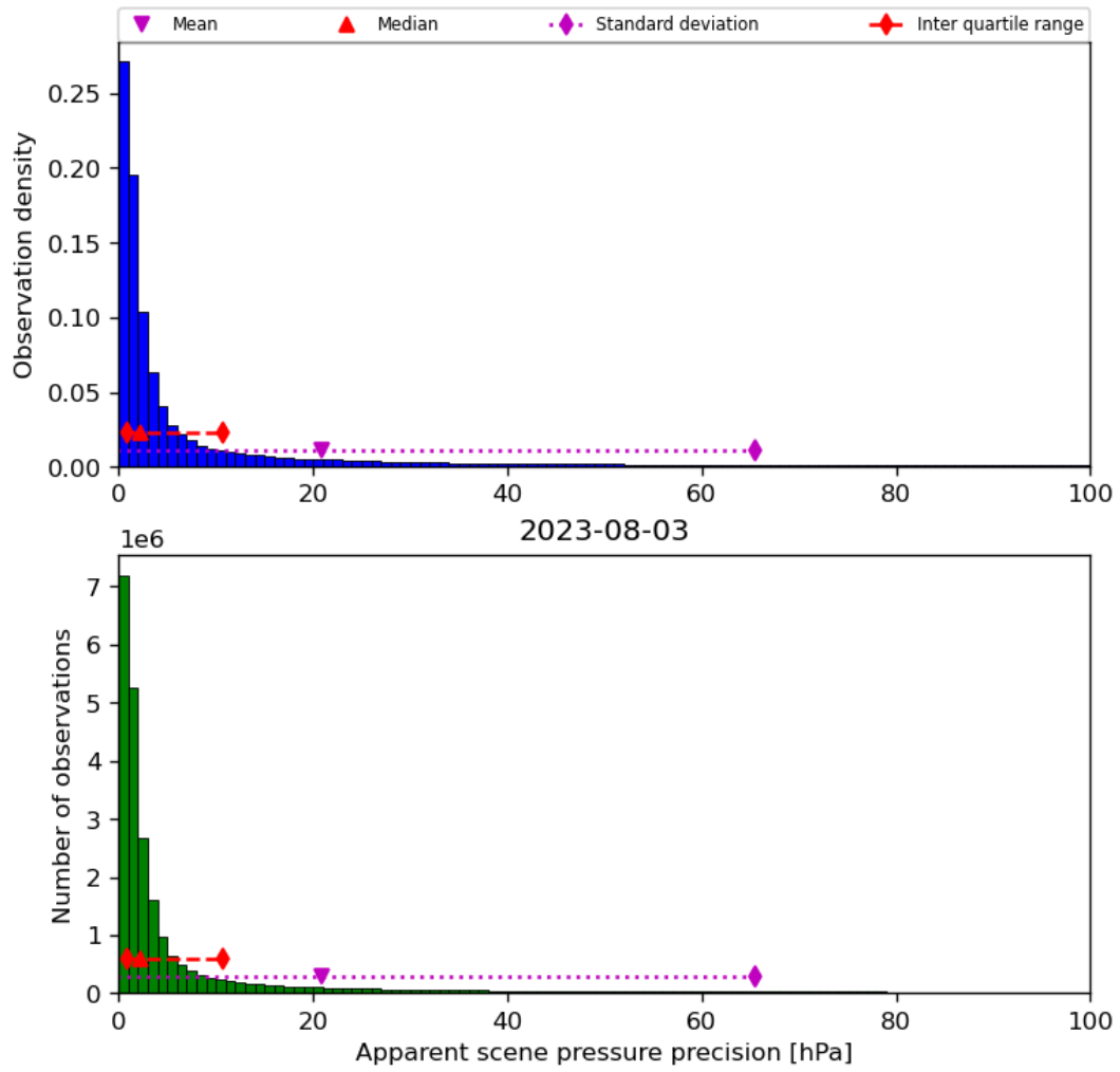
Figure 37: Histogram of “Apparent scene pressure precision” for 2023-08-02 to 2023-08-04
