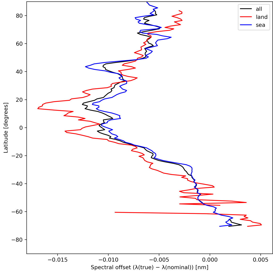
Figure 28: Zonal average of “Spectral offset ( \lambda(\text{true}) - \lambda(\text{nominal}) )” for 2023-08-02 to 2023-08-04.
