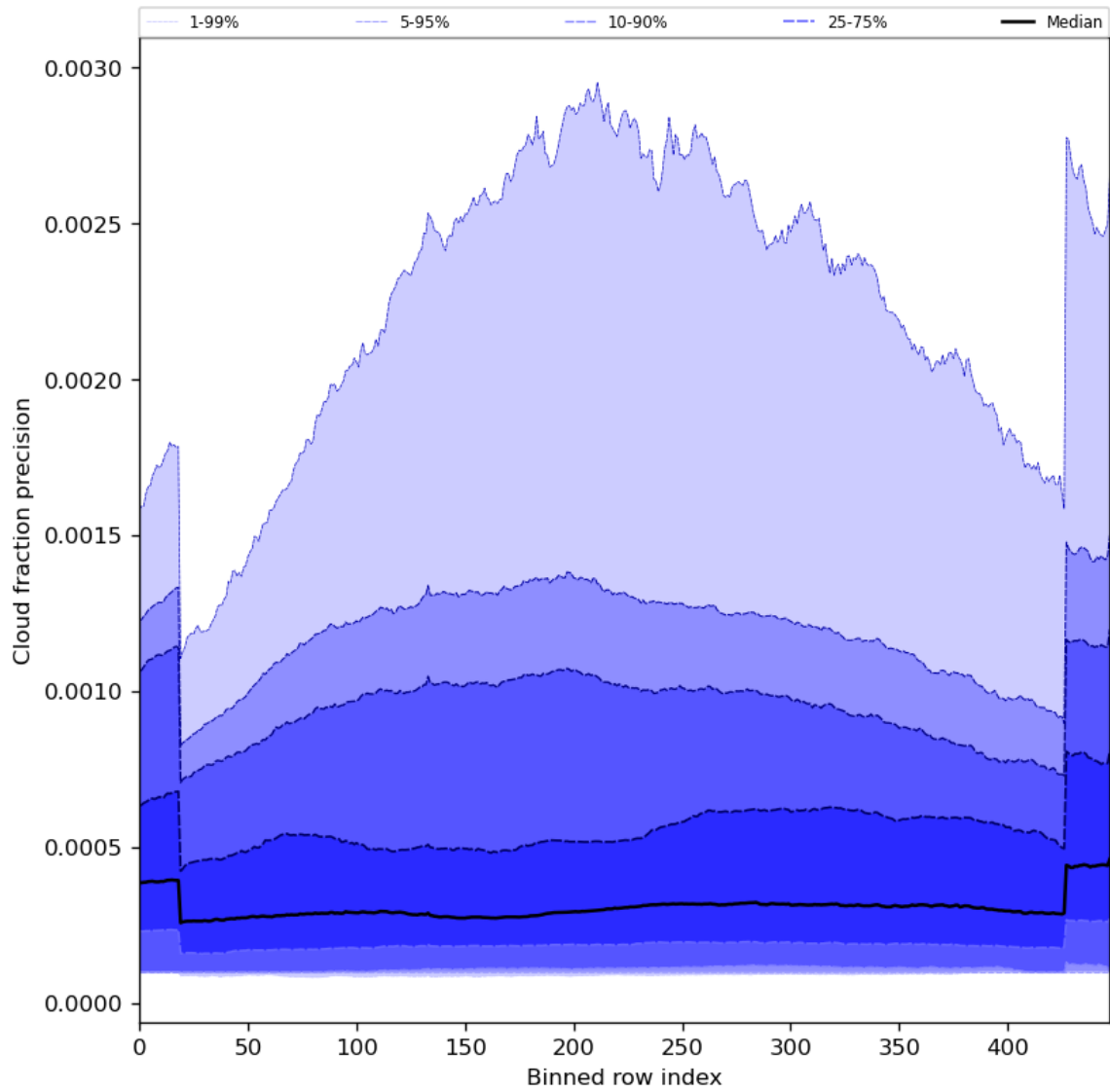
Figure 50: Along track statistics of “Cloud fraction precision” for 2023-08-02 to 2023-08-04
