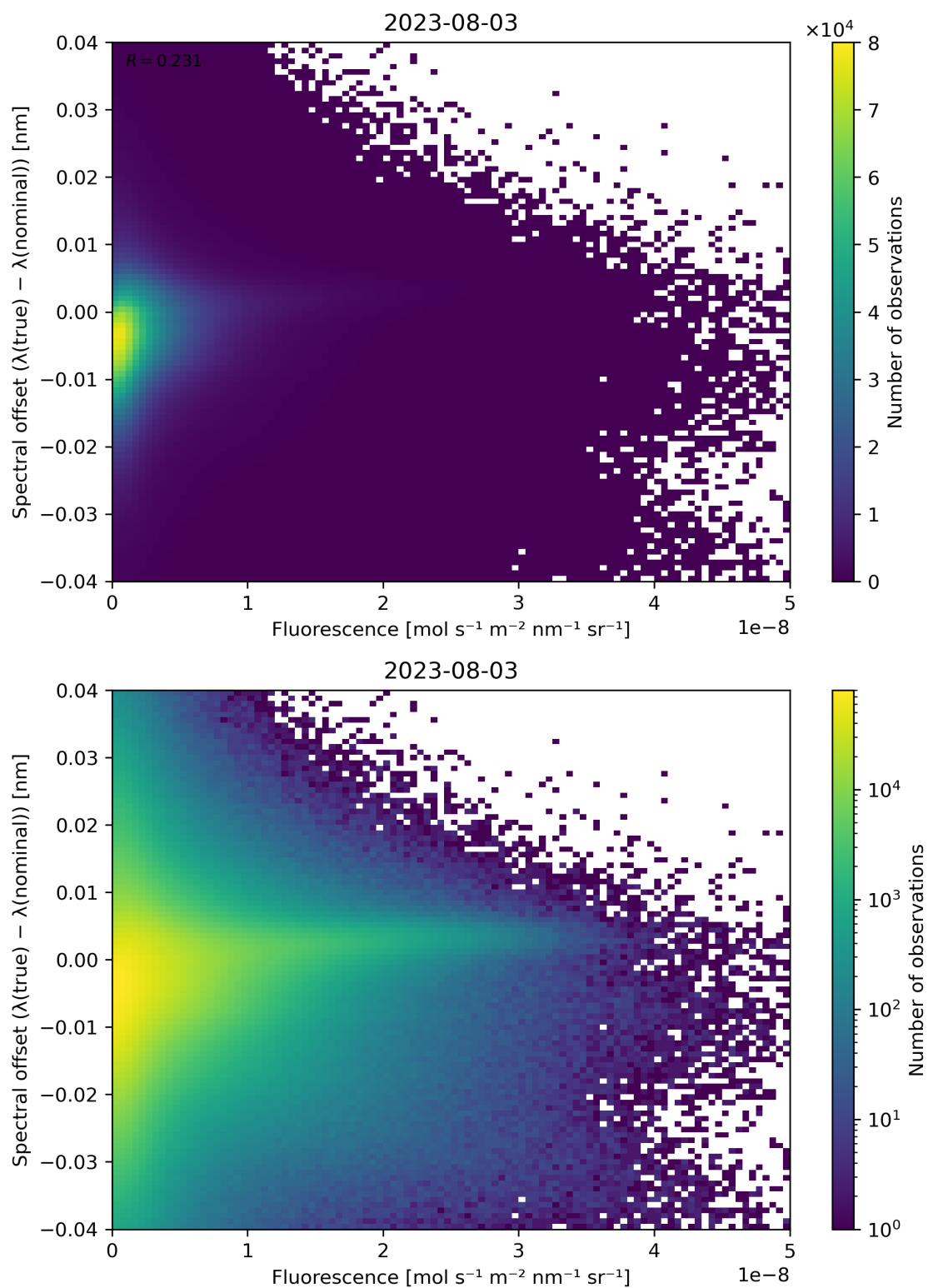
Figure 95: Scatter density plot of “Fluorescence” against “Spectral offset ( \lambda(\text{true}) - \lambda(\text{nominal}) )” for 2023-08-02 to 2023-08-04.
