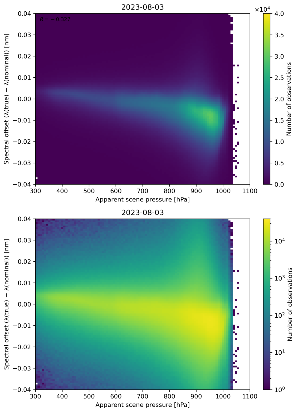
Figure 68: Scatter density plot of “Apparent scene pressure” against “Spectral offset ( \lambda(\text{true}) - \lambda(\text{nominal}) )” for 2023-08-02 to 2023-08-04.
