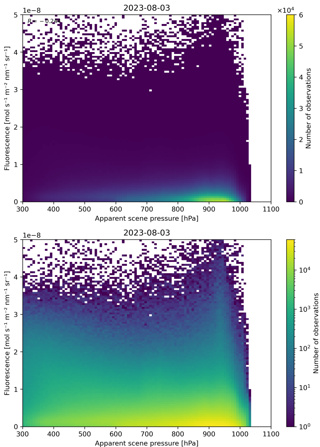
Figure 65: Scatter density plot of “Apparent scene pressure” against “Fluorescence” for 2023-08-02 to 2023-08-04.
