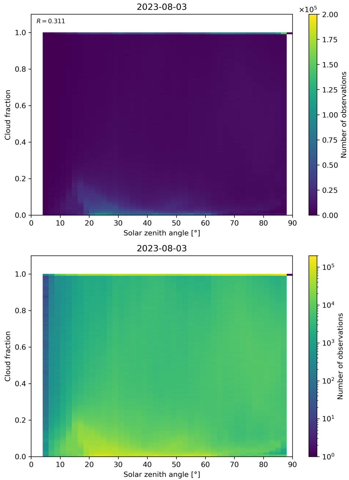
Figure 121: Scatter density plot of “Solar zenith angle” against “Cloud fraction” for 2023-08-02 to 2023-08-04.
