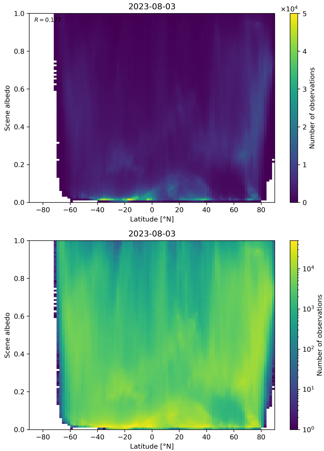
Figure 104: Scatter density plot of “Latitude” against “Scene albedo” for 2023-08-02 to 2023-08-04.
