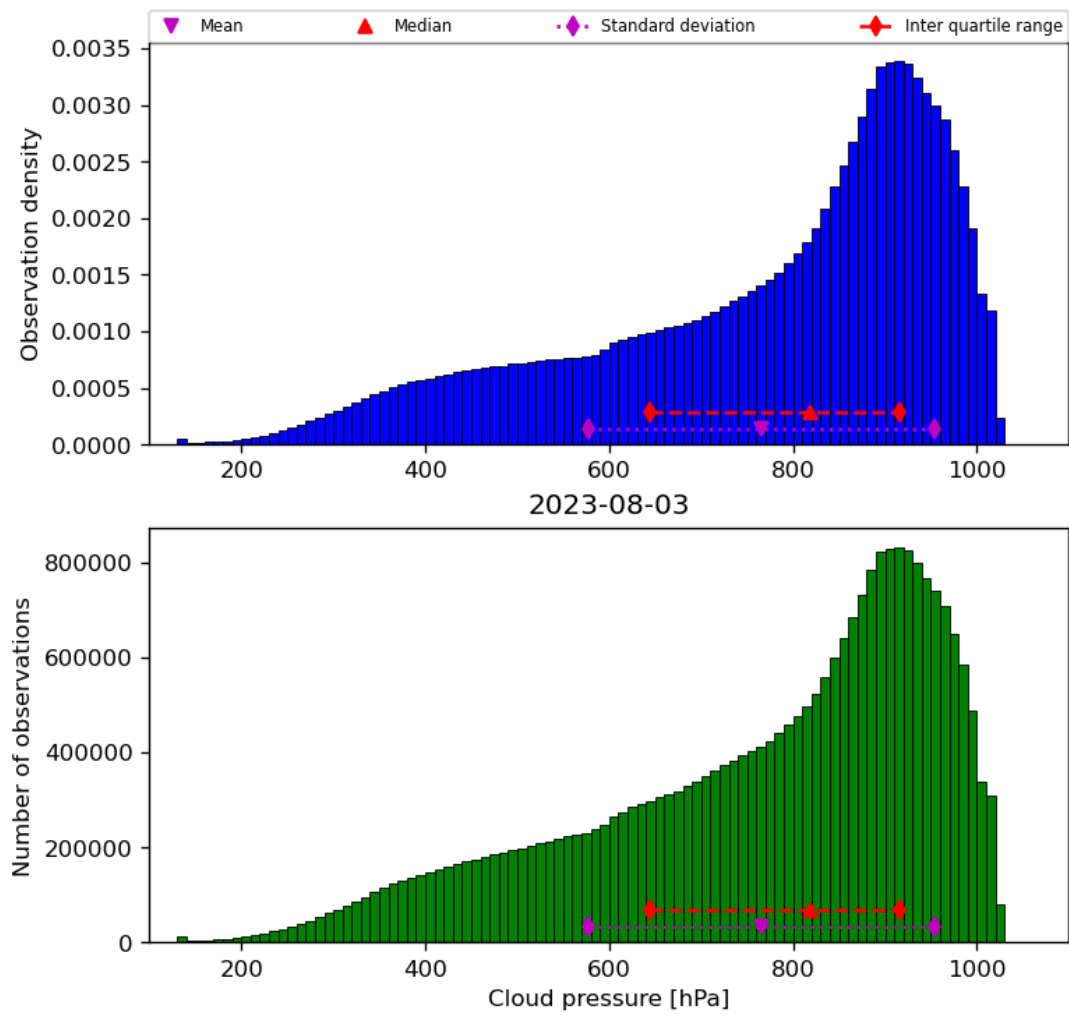
Figure 30: Histogram of “Cloud pressure” for 2023-08-02 to 2023-08-04
