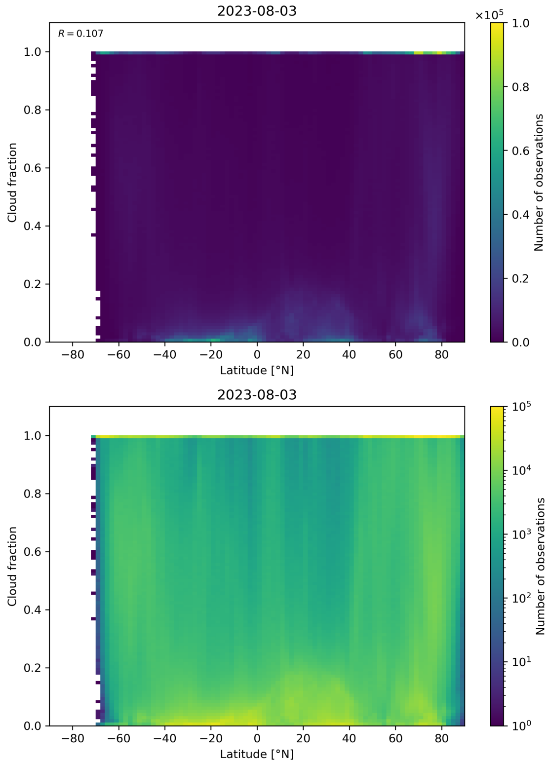
Figure 99: Scatter density plot of “Latitude” against “Cloud fraction” for 2023-08-02 to 2023-08-04.
