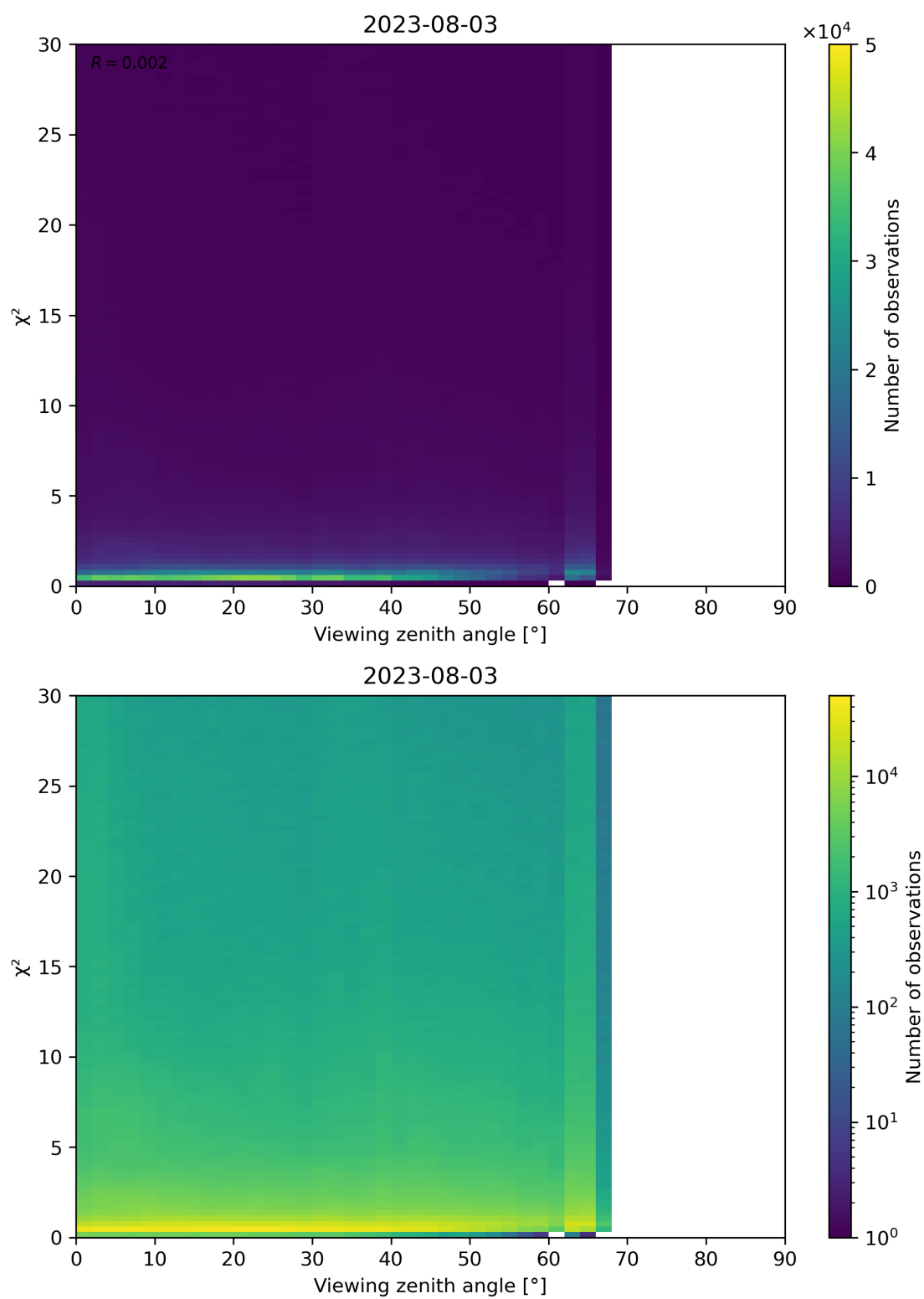
Figure 130: Scatter density plot of “Viewing zenith angle” against “ \chi^2 ” for 2023-08-02 to 2023-08-04.
