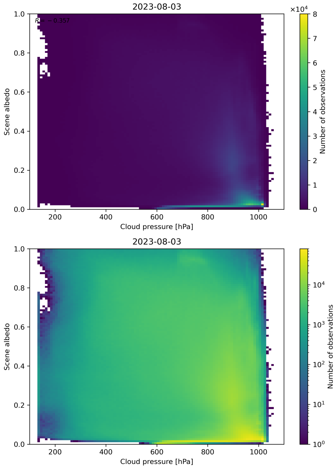
Figure 91: Scatter density plot of “Cloud pressure” against “Scene albedo” for 2023-08-02 to 2023-08-04.
