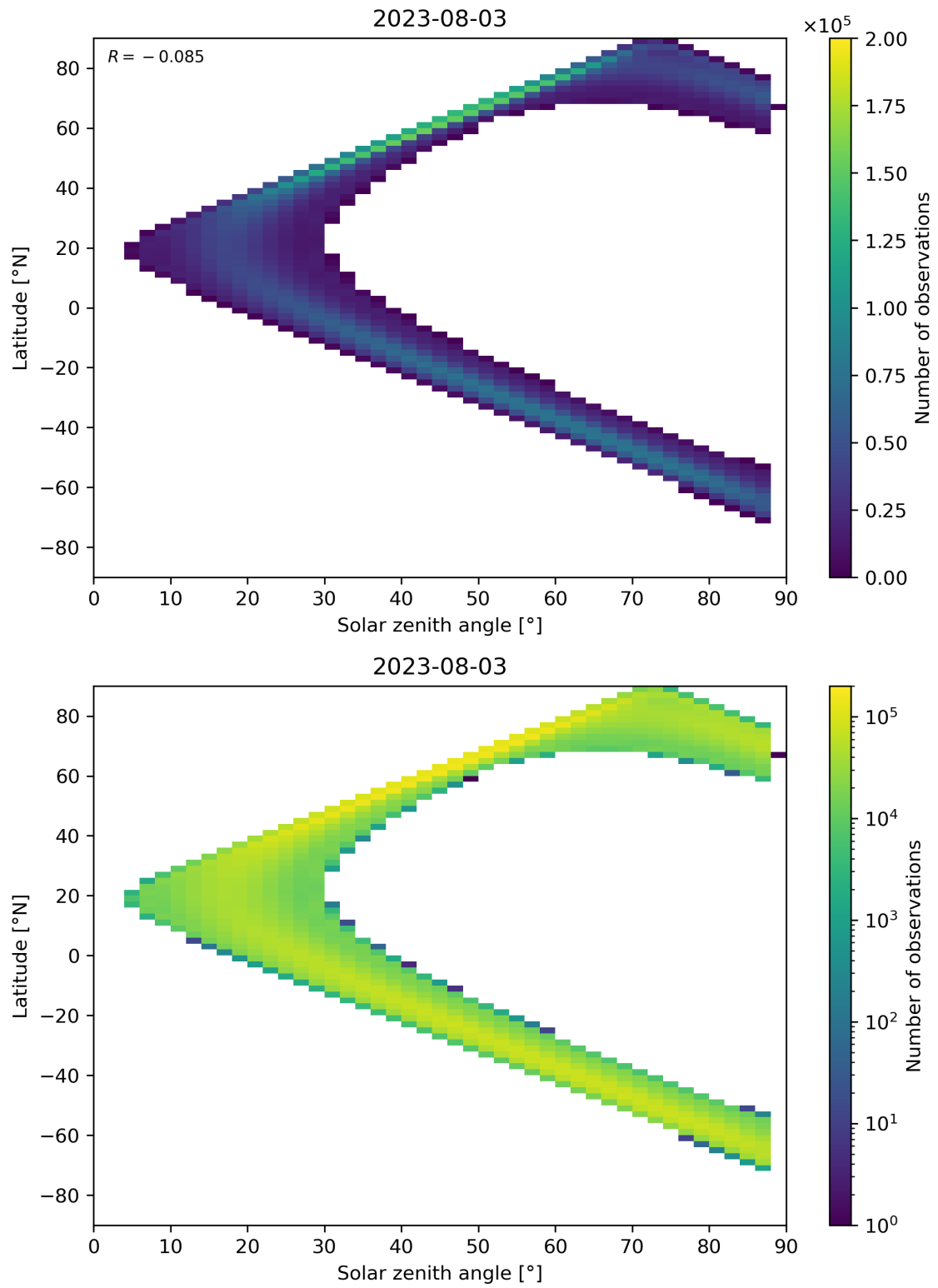
Figure 124: Scatter density plot of “Solar zenith angle” against “Latitude” for 2023-08-02 to 2023-08-04.
