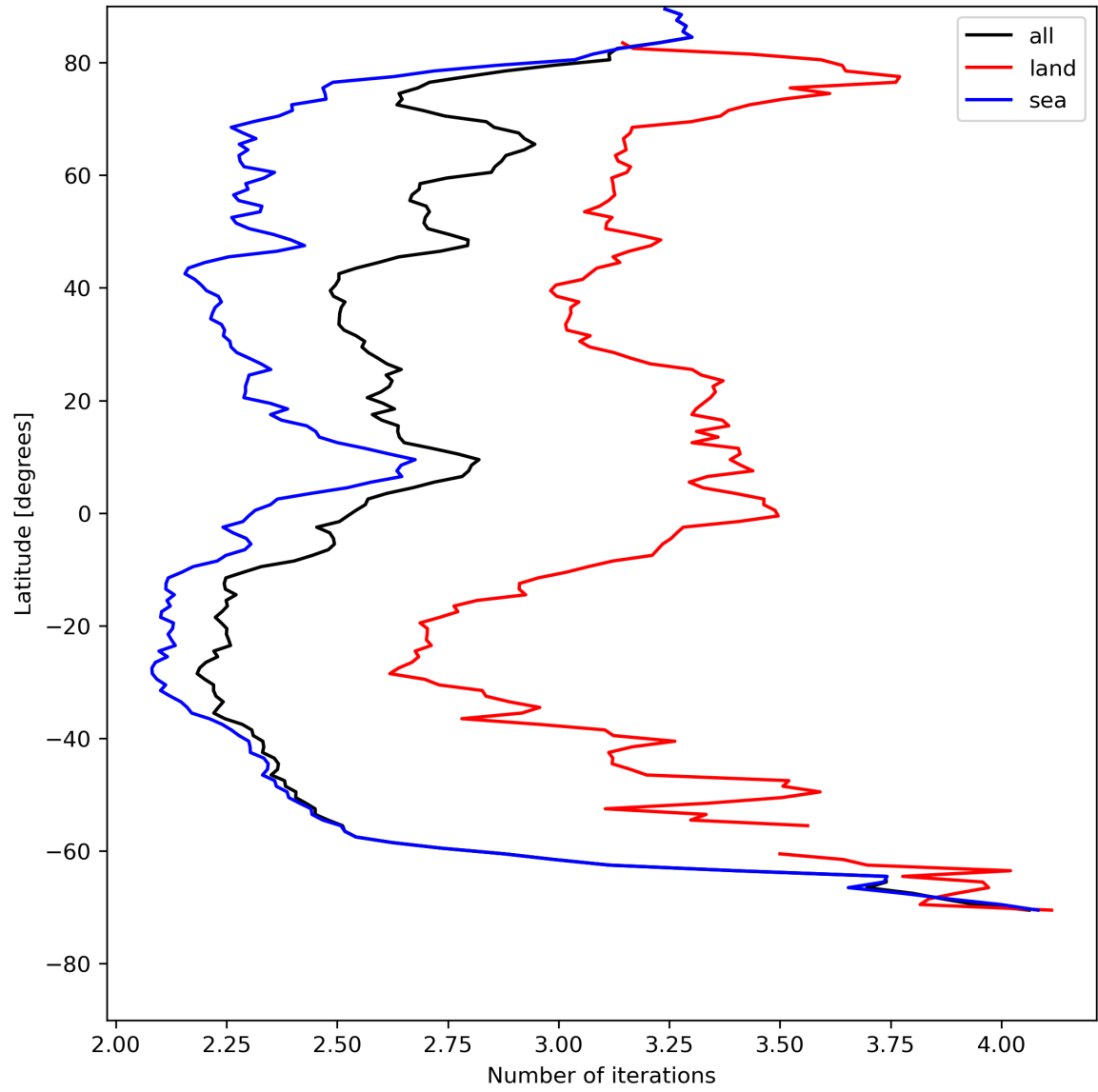
Figure 22: Zonal average of “Number of iterations” for 2023-08-02 to 2023-08-04.
