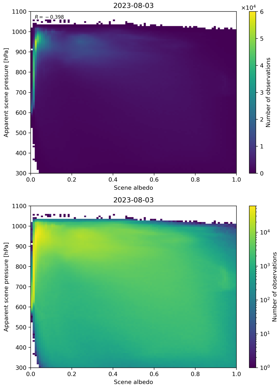
Figure 111: Scatter density plot of “Scene albedo” against “Apparent scene pressure” for 2023-08-02 to 2023-08-04.
