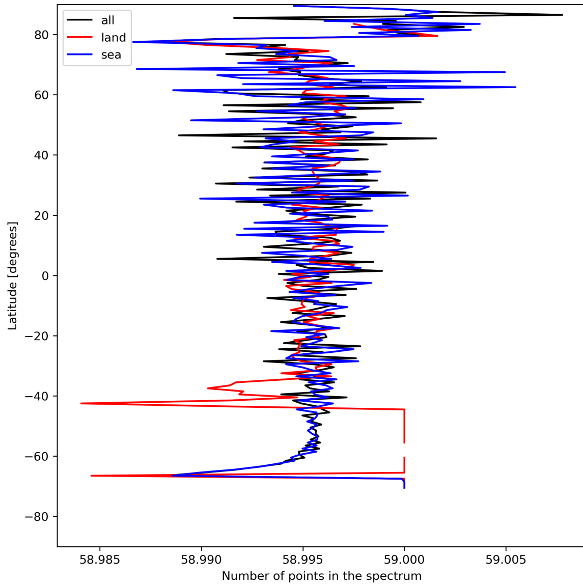
Figure 27: Zonal average of “Number of points in the spectrum” for 2023-08-02 to 2023-08-04.
