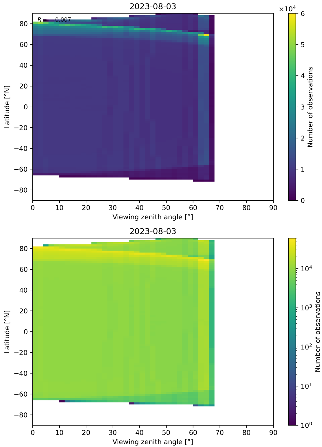
Figure 135: Scatter density plot of “Viewing zenith angle” against “Latitude” for 2023-08-02 to 2023-08-04.
