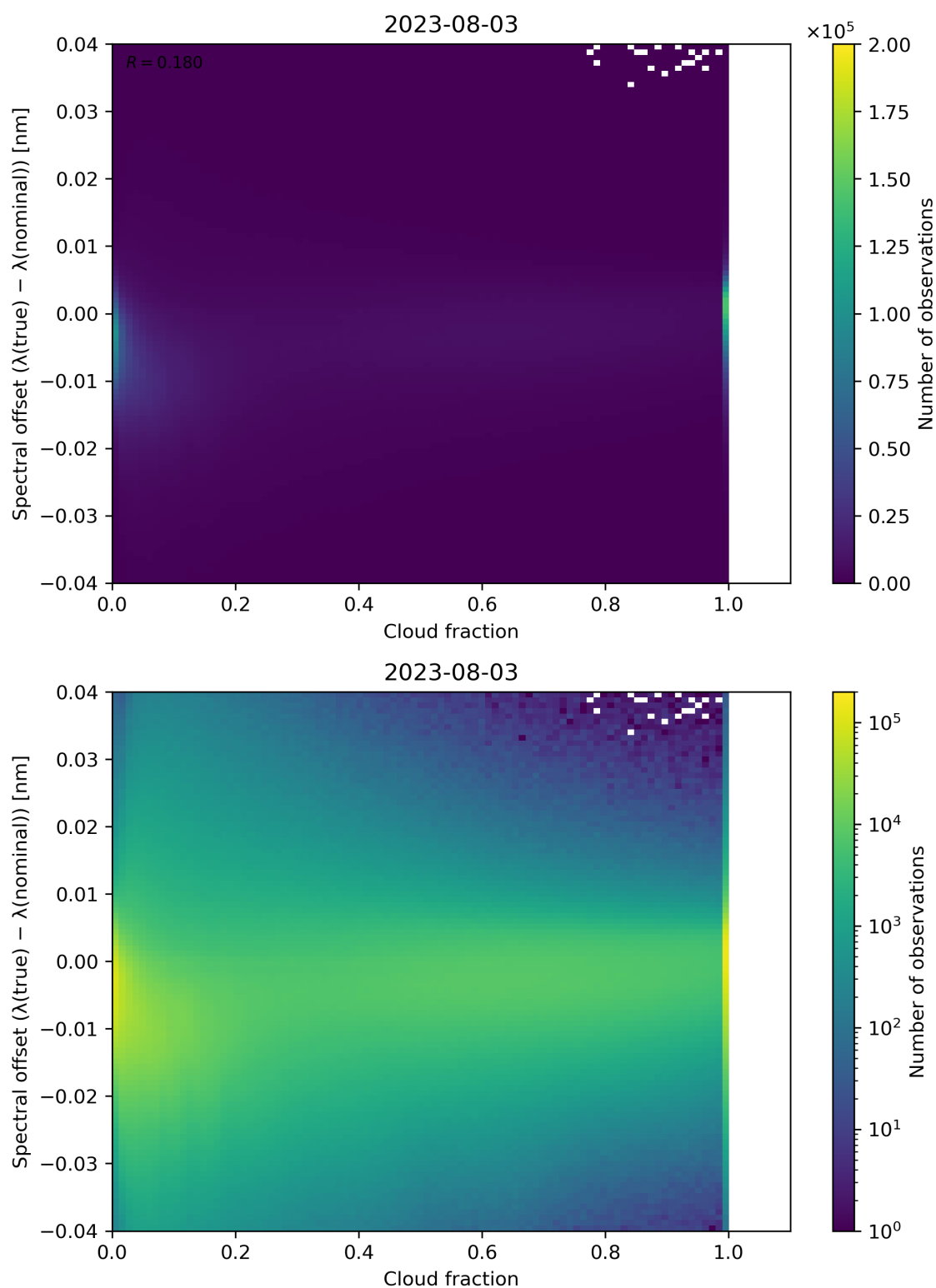
Figure 83: Scatter density plot of “Cloud fraction” against “Spectral offset ( \lambda(\text{true}) - \lambda(\text{nominal}) )” for 2023-08-02 to 2023-08-04.
