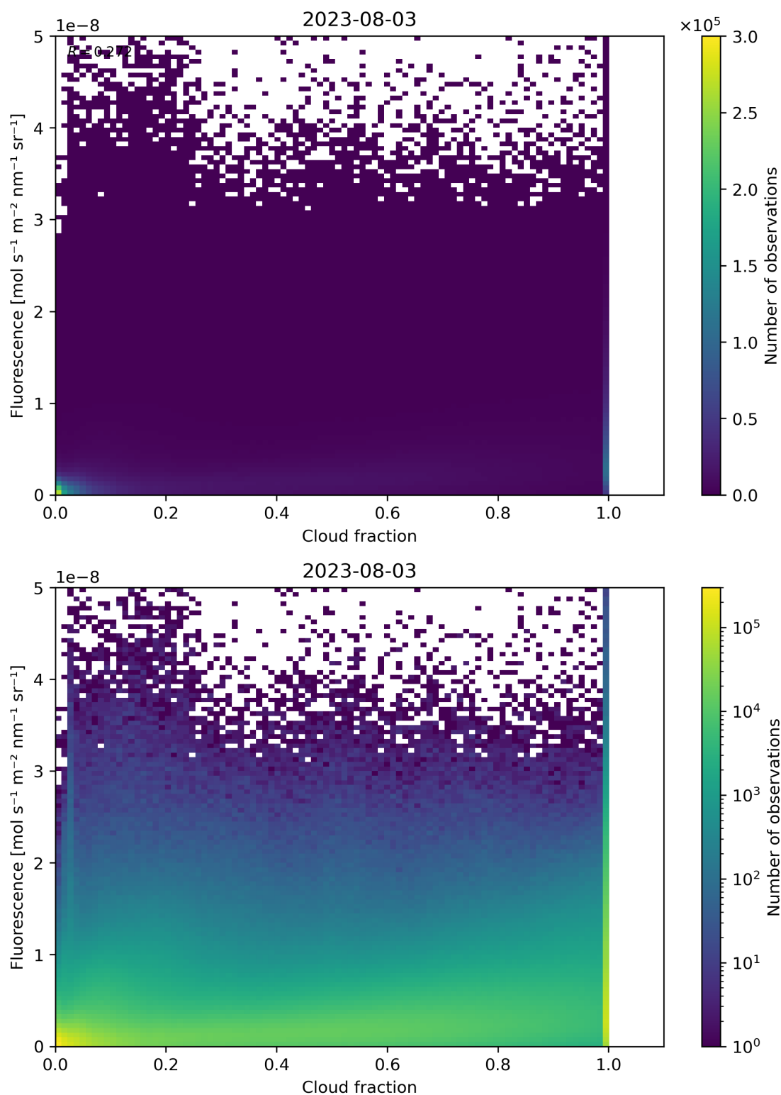
Figure 79: Scatter density plot of “Cloud fraction” against “Fluorescence” for 2023-08-02 to 2023-08-04.
