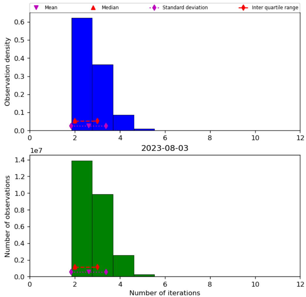
Figure 39: Histogram of “Number of iterations” for 2023-08-02 to 2023-08-04
