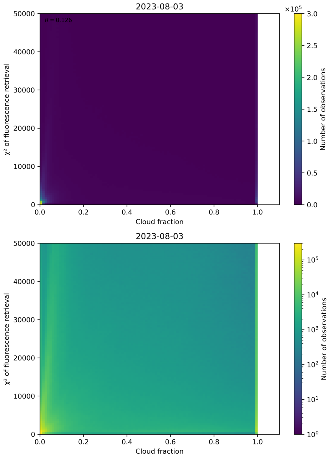
Figure 78: Scatter density plot of “Cloud fraction” against “ \chi^2 of fluorescence retrieval” for 2023-08-02 to 2023-08-04.
