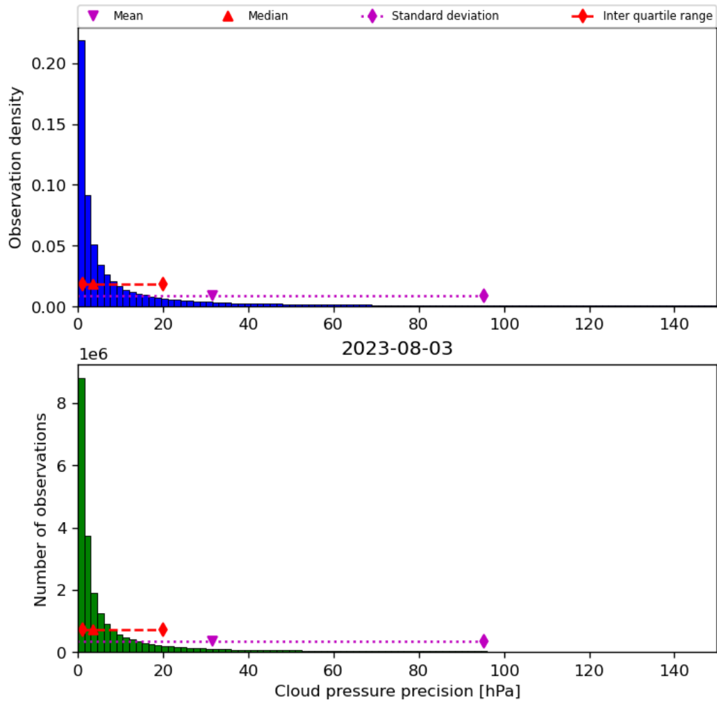
Figure 31: Histogram of “Cloud pressure precision” for 2023-08-02 to 2023-08-04
