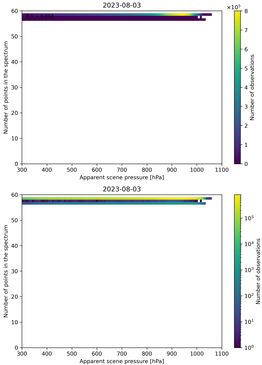
Figure 67: Scatter density plot of “Apparent scene pressure” against “Number of points in the spectrum” for 2023-08-02 to 2023-08-04.
