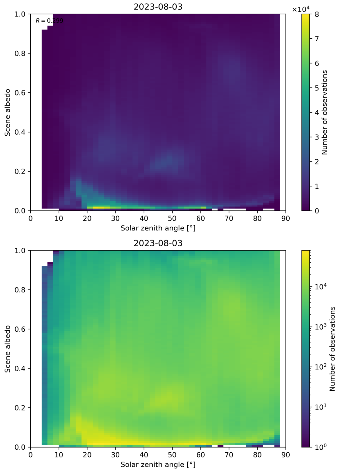
Figure 127: Scatter density plot of “Solar zenith angle” against “Scene albedo” for 2023-08-02 to 2023-08-04.
