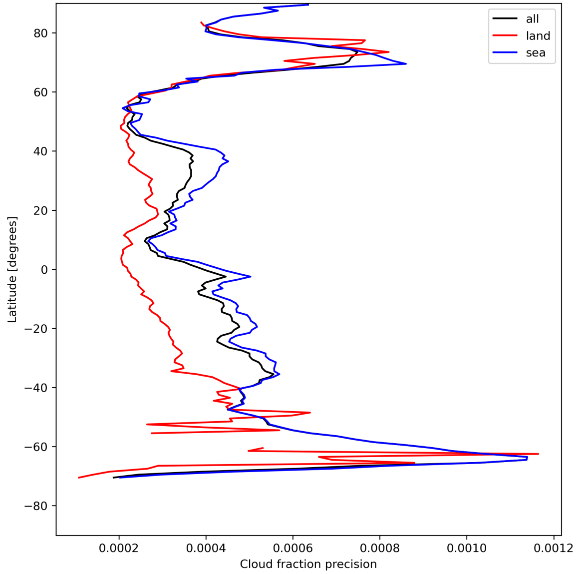
Figure 16: Zonal average of “Cloud fraction precision” for 2023-08-02 to 2023-08-04.
