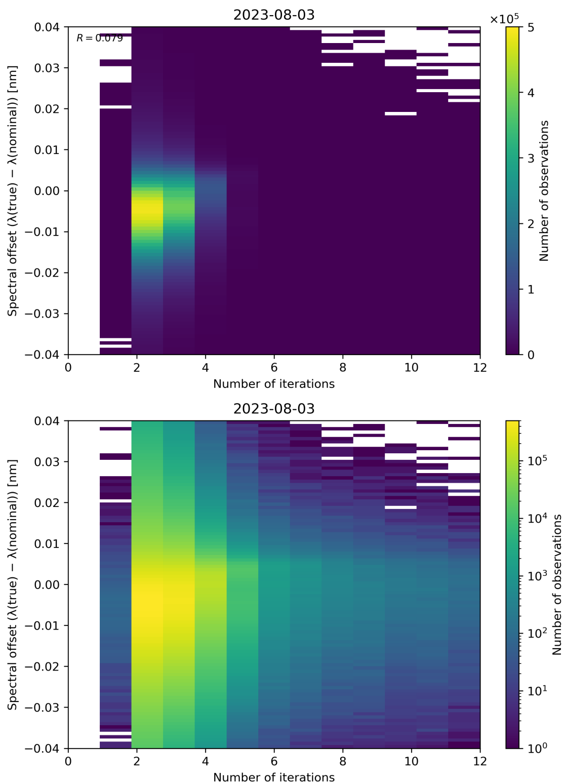
Figure 109: Scatter density plot of “Number of iterations” against “Spectral offset ( \lambda(\text{true}) - \lambda(\text{nominal}) )” for 2023-08-02 to 2023-08-04.
