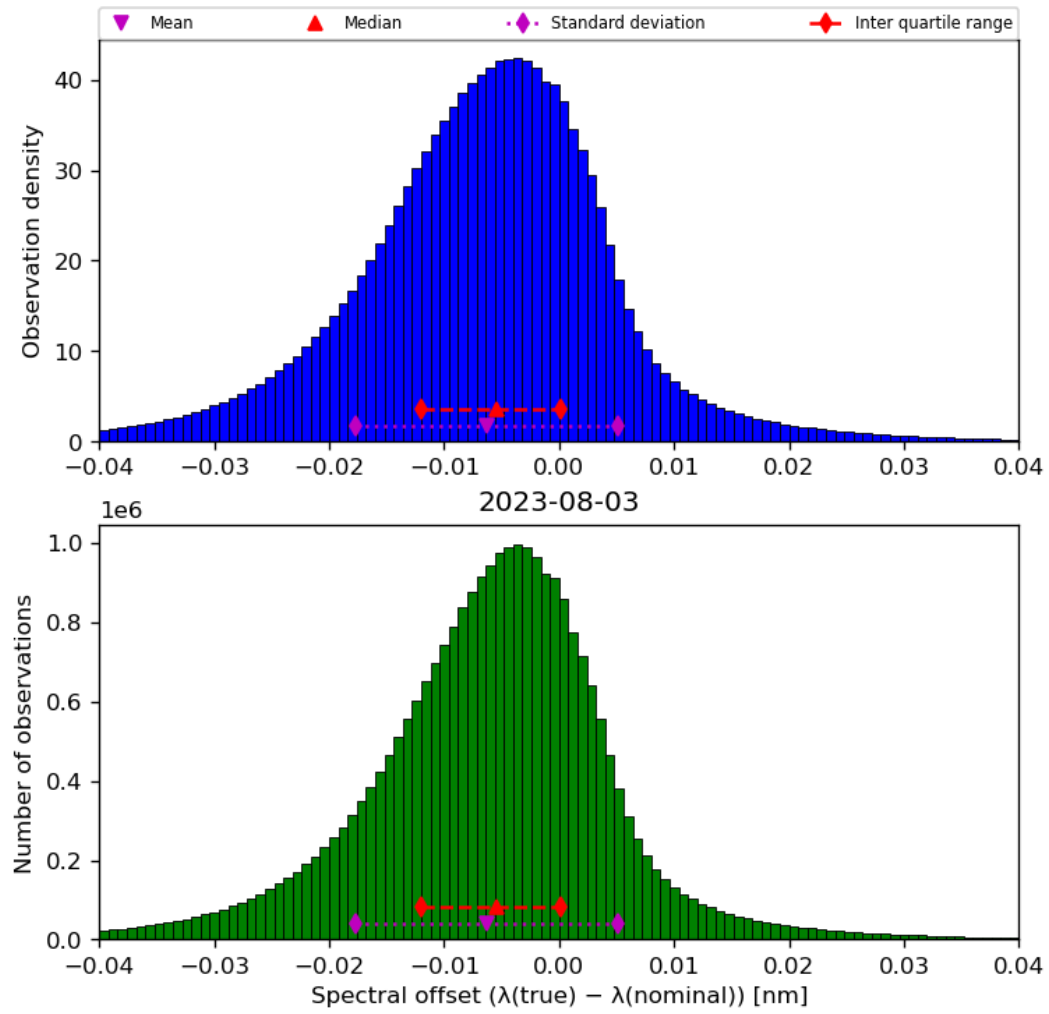
Figure 45: Histogram of “Spectral offset ( \lambda(\text{true}) - \lambda(\text{nominal}) )” for 2023-08-02 to 2023-08-04
