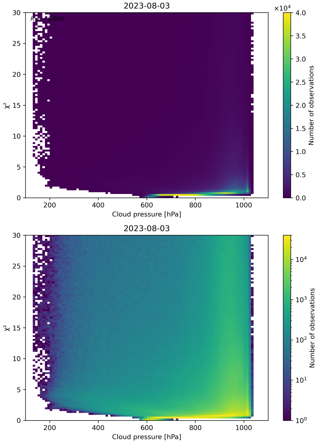
Figure 85: Scatter density plot of “Cloud pressure” against “ \chi^2 ” for 2023-08-02 to 2023-08-04.
