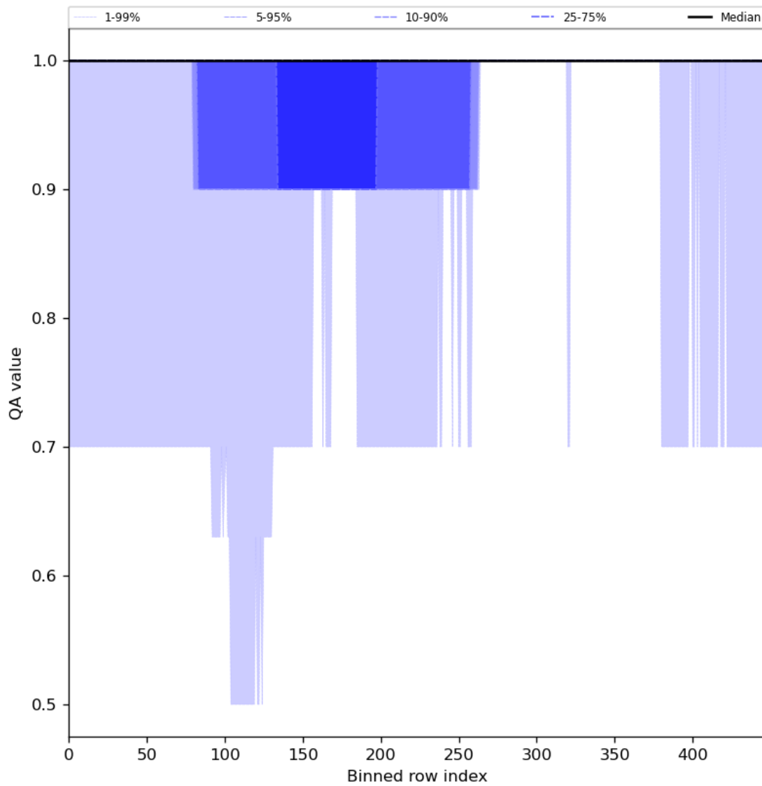
Figure 46: Along track statistics of “QA value” for 2023-08-02 to 2023-08-04
