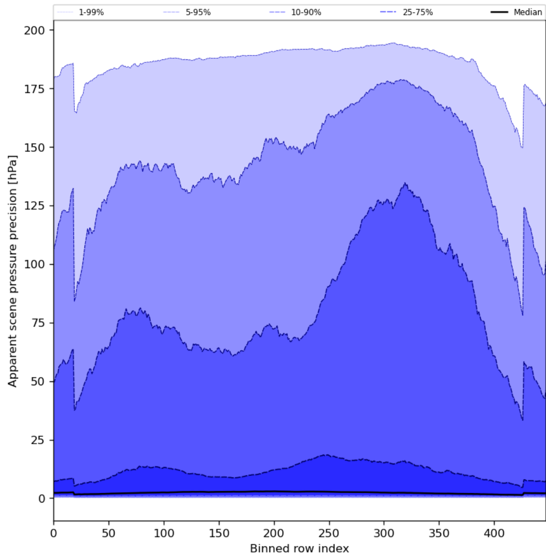
Figure 54: Along track statistics of “Apparent scene pressure precision” for 2023-08-02 to 2023-08-04
