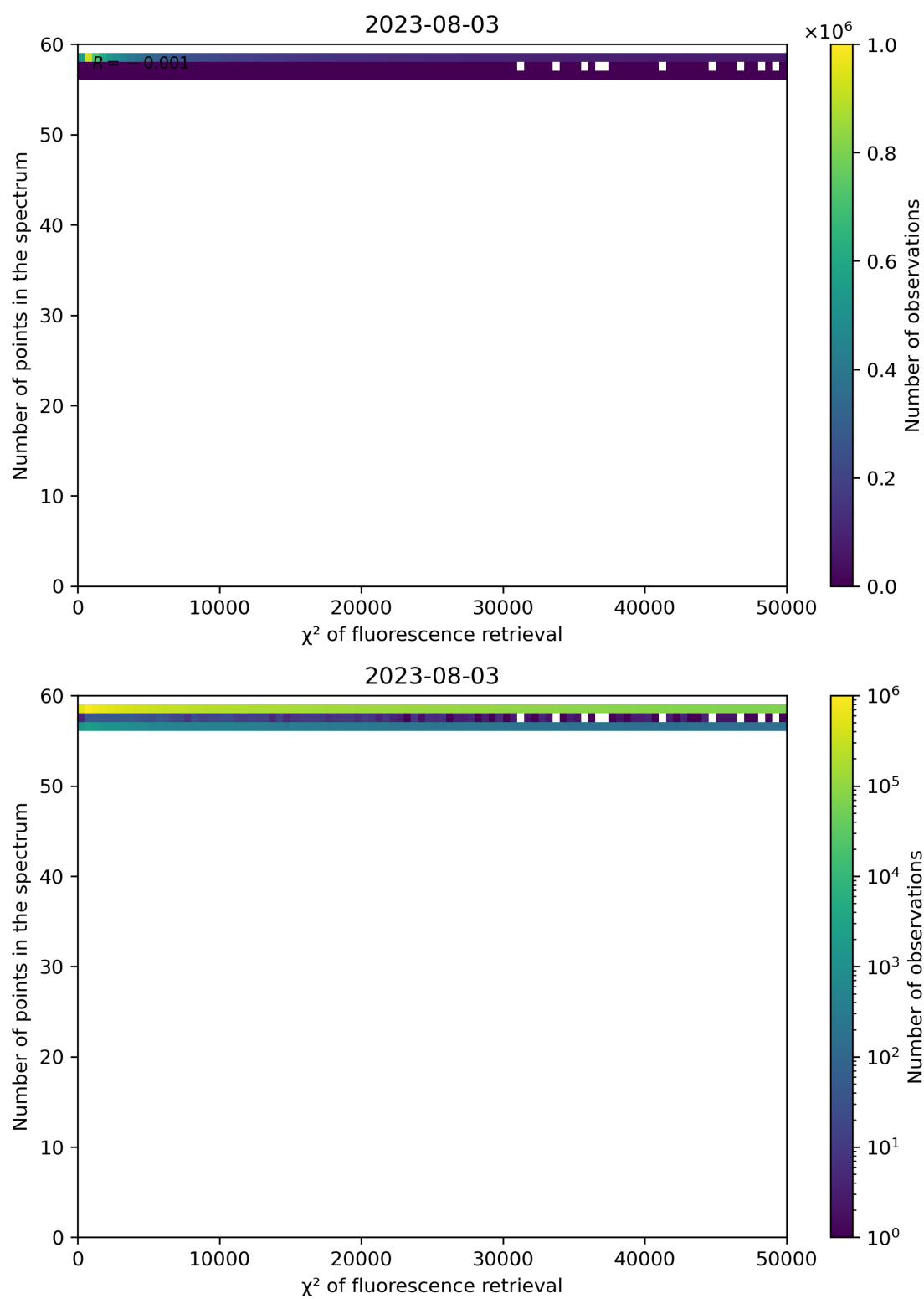
Figure 71: Scatter density plot of " \chi^2 of fluorescence retrieval" against "Number of points in the spectrum" for 2023-08-02 to 2023-08-04.
