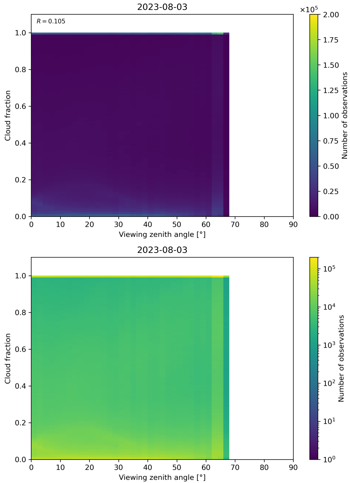
Figure 132: Scatter density plot of “Viewing zenith angle” against “Cloud fraction” for 2023-08-02 to 2023-08-04.
