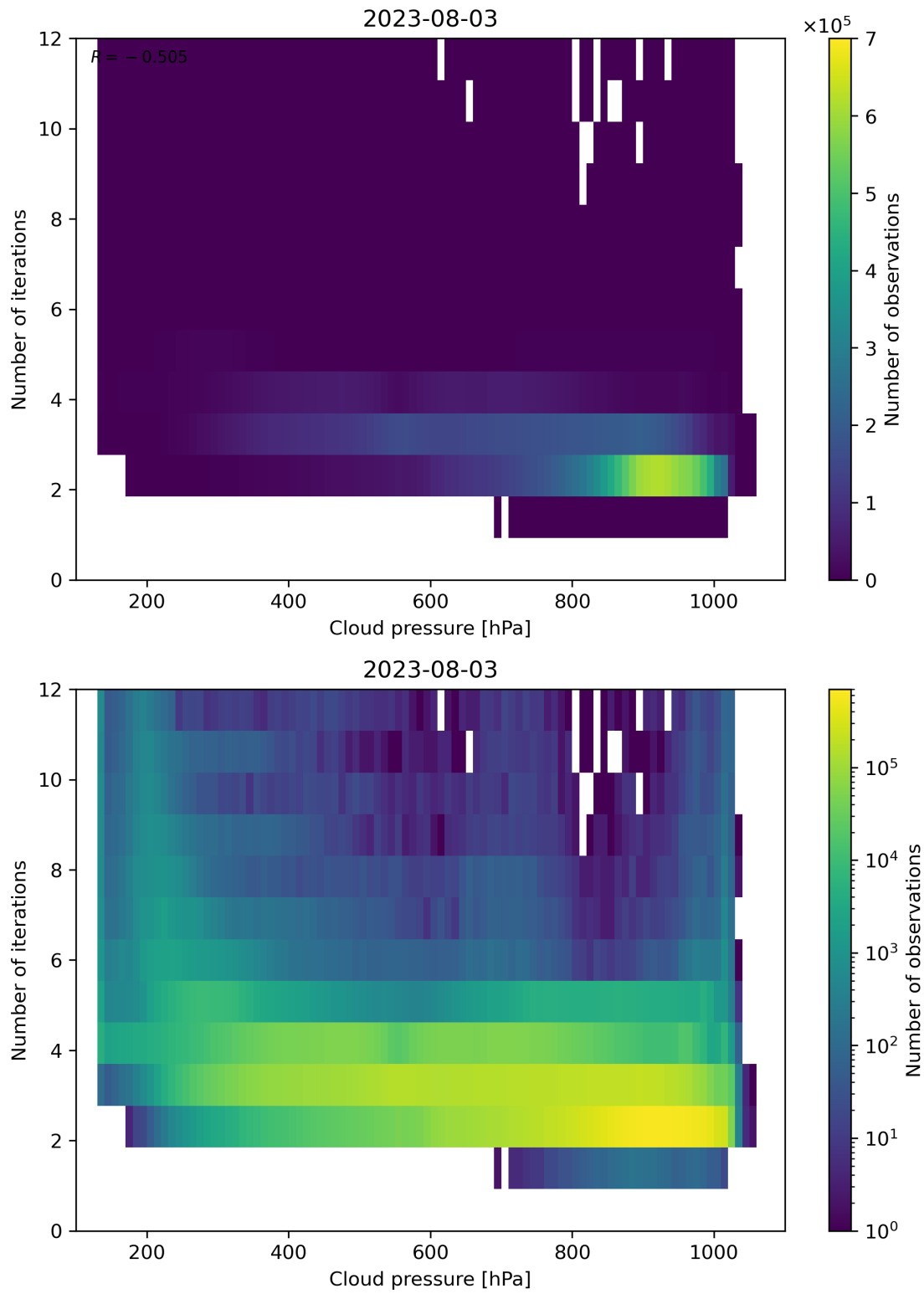
Figure 89: Scatter density plot of “Cloud pressure” against “Number of iterations” for 2023-08-02 to 2023-08-04.
