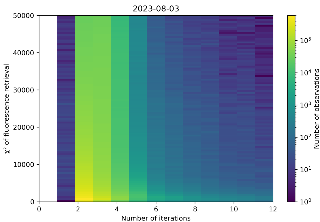
Figure 106: Scatter density plot of “Number of iterations” against “ \chi^2 of fluorescence retrieval” for 2023-08-02 to 2023-08-04.
