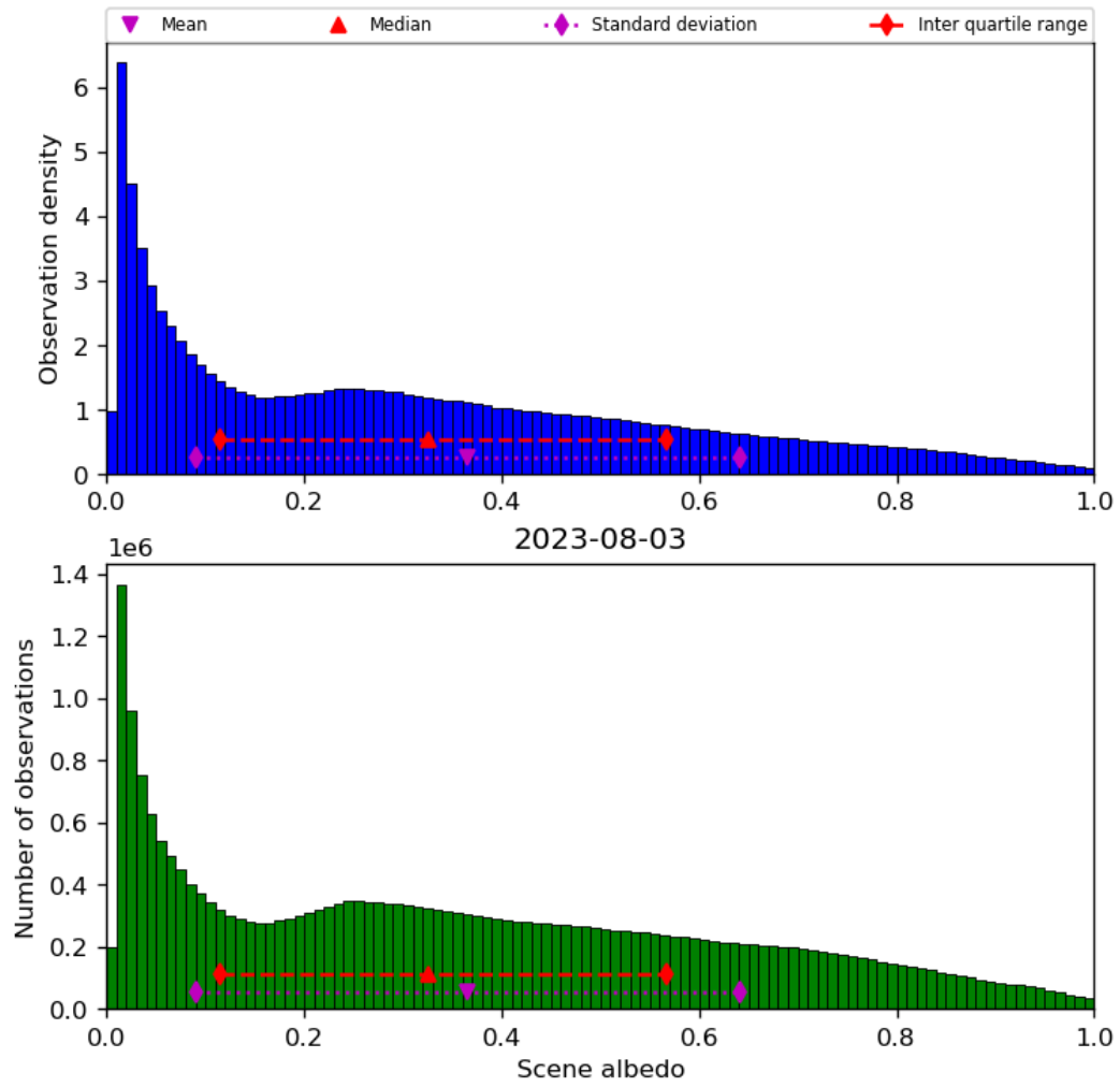
Figure 34: Histogram of “Scene albedo” for 2023-08-02 to 2023-08-04
