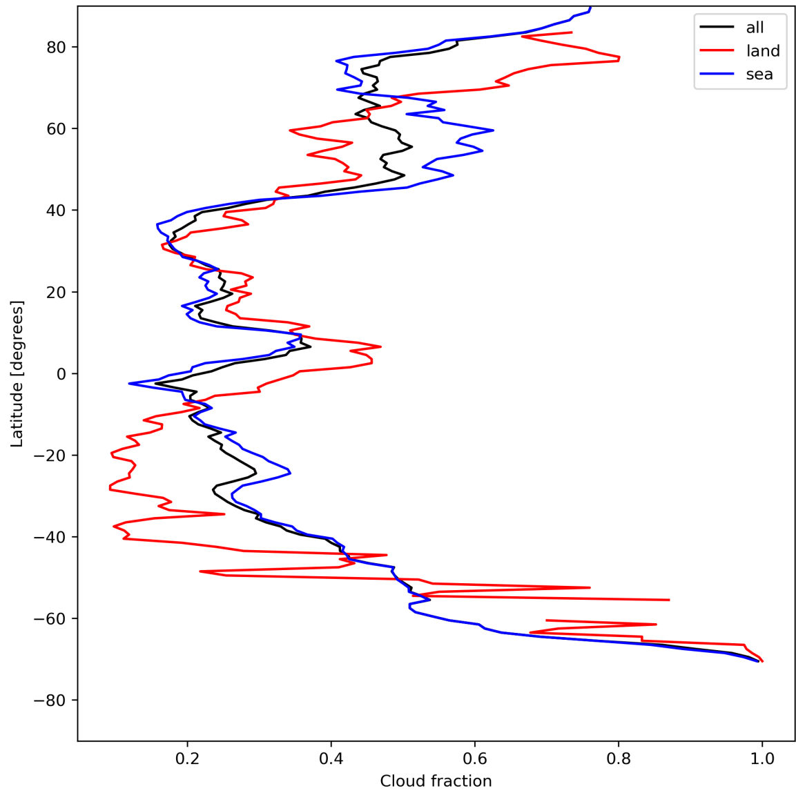
Figure 15: Zonal average of “Cloud fraction” for 2023-08-02 to 2023-08-04.
