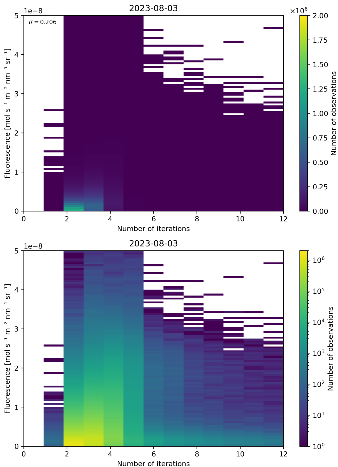
Figure 107: Scatter density plot of “Number of iterations” against “Fluorescence” for 2023-08-02 to 2023-08-04.
