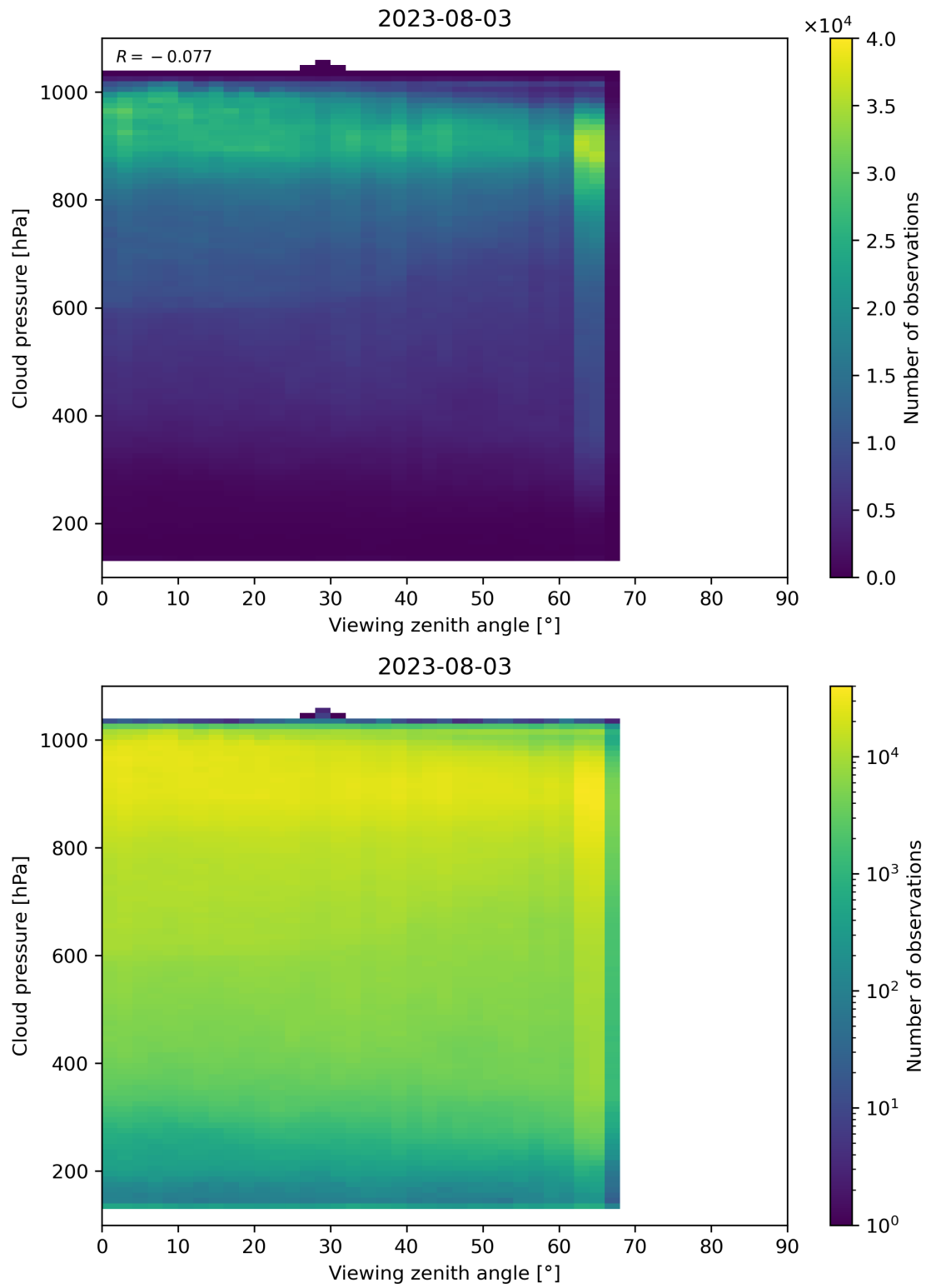
Figure 133: Scatter density plot of “Viewing zenith angle” against “Cloud pressure” for 2023-08-02 to 2023-08-04.
