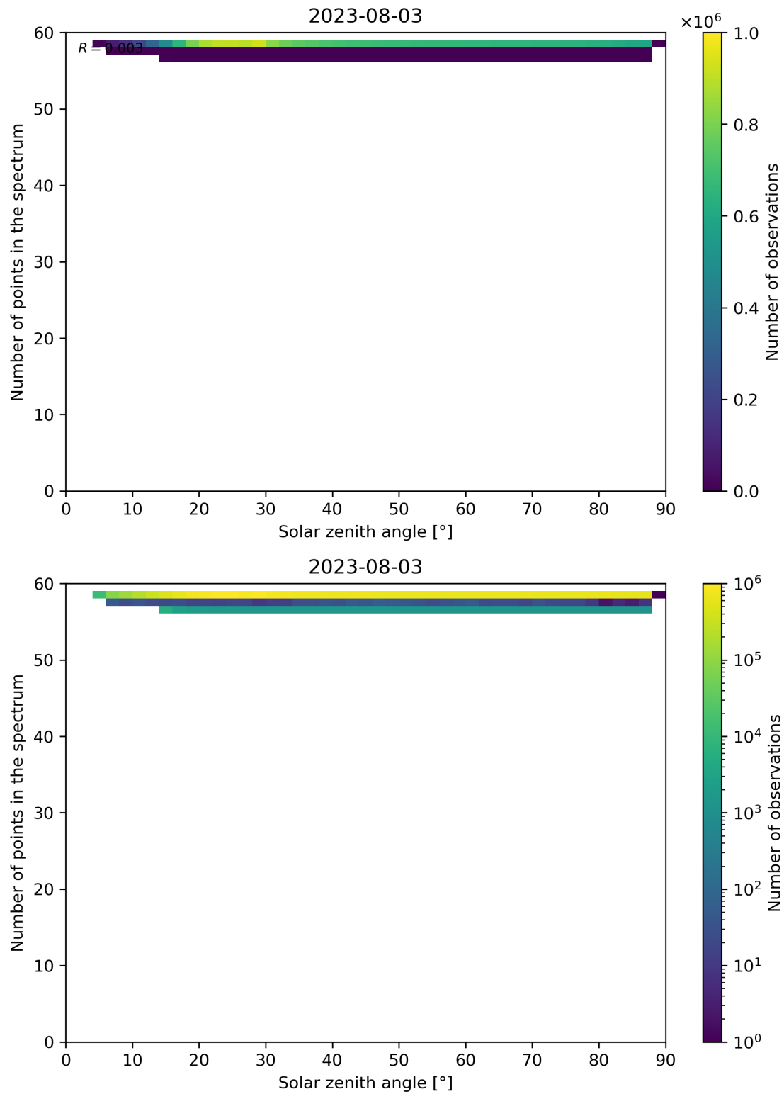
Figure 126: Scatter density plot of “Solar zenith angle” against “Number of points in the spectrum” for 2023-08-02 to 2023-08-04.
