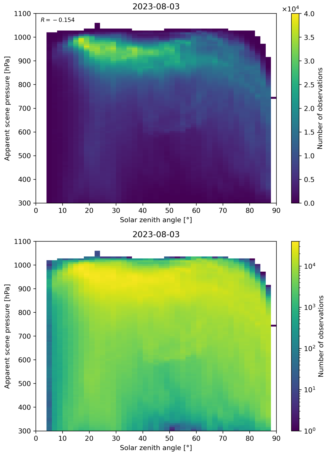
Figure 118: Scatter density plot of “Solar zenith angle” against “Apparent scene pressure” for 2023-08-02 to 2023-08-04.
