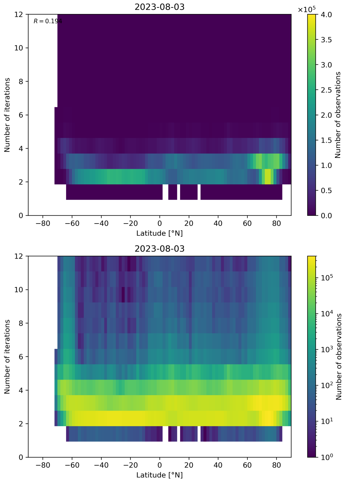
Figure 102: Scatter density plot of “Latitude” against “Number of iterations” for 2023-08-02 to 2023-08-04.
