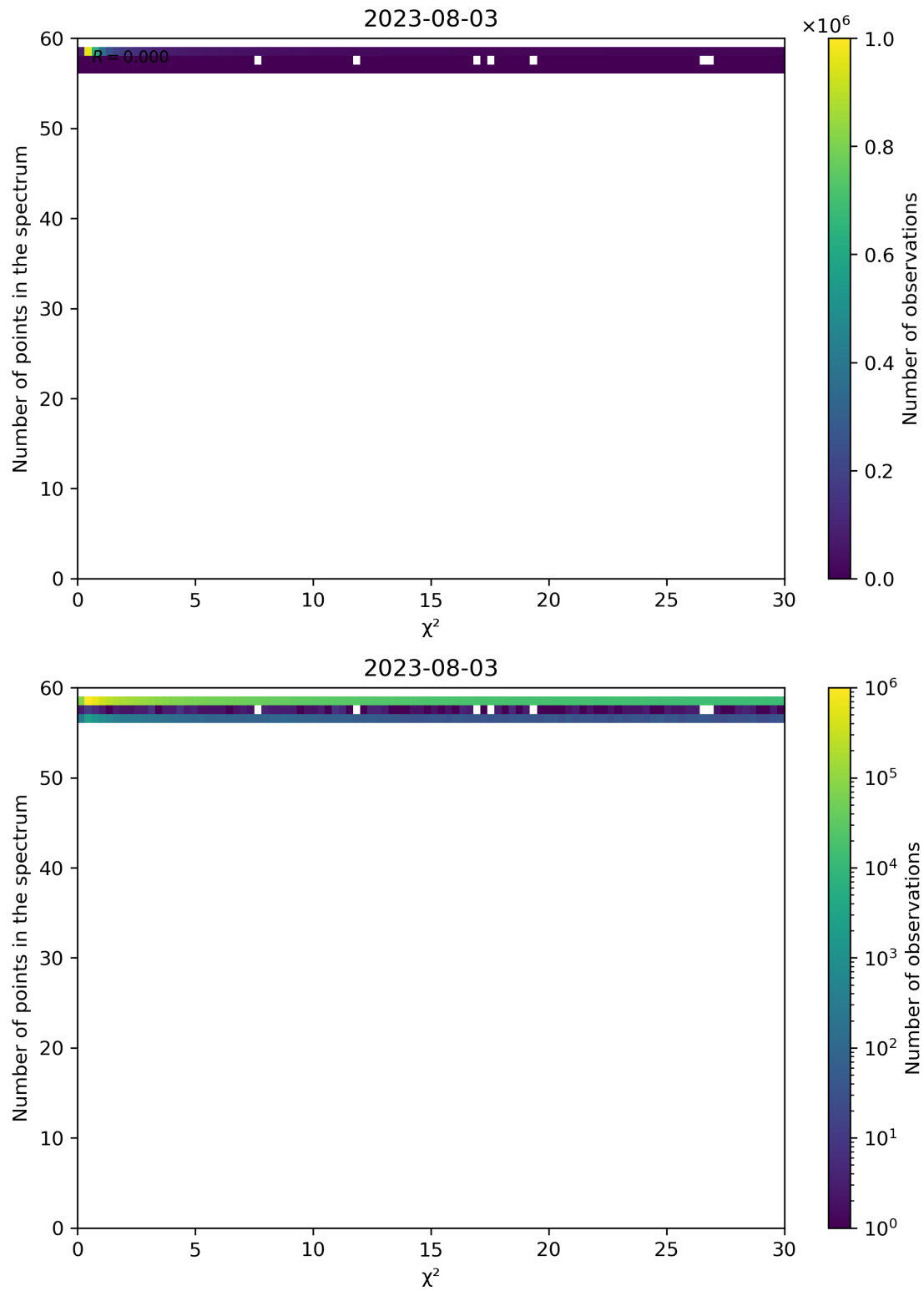
Figure 74: Scatter density plot of " \chi^2 " against "Number of points in the spectrum" for 2023-08-02 to 2023-08-04.
