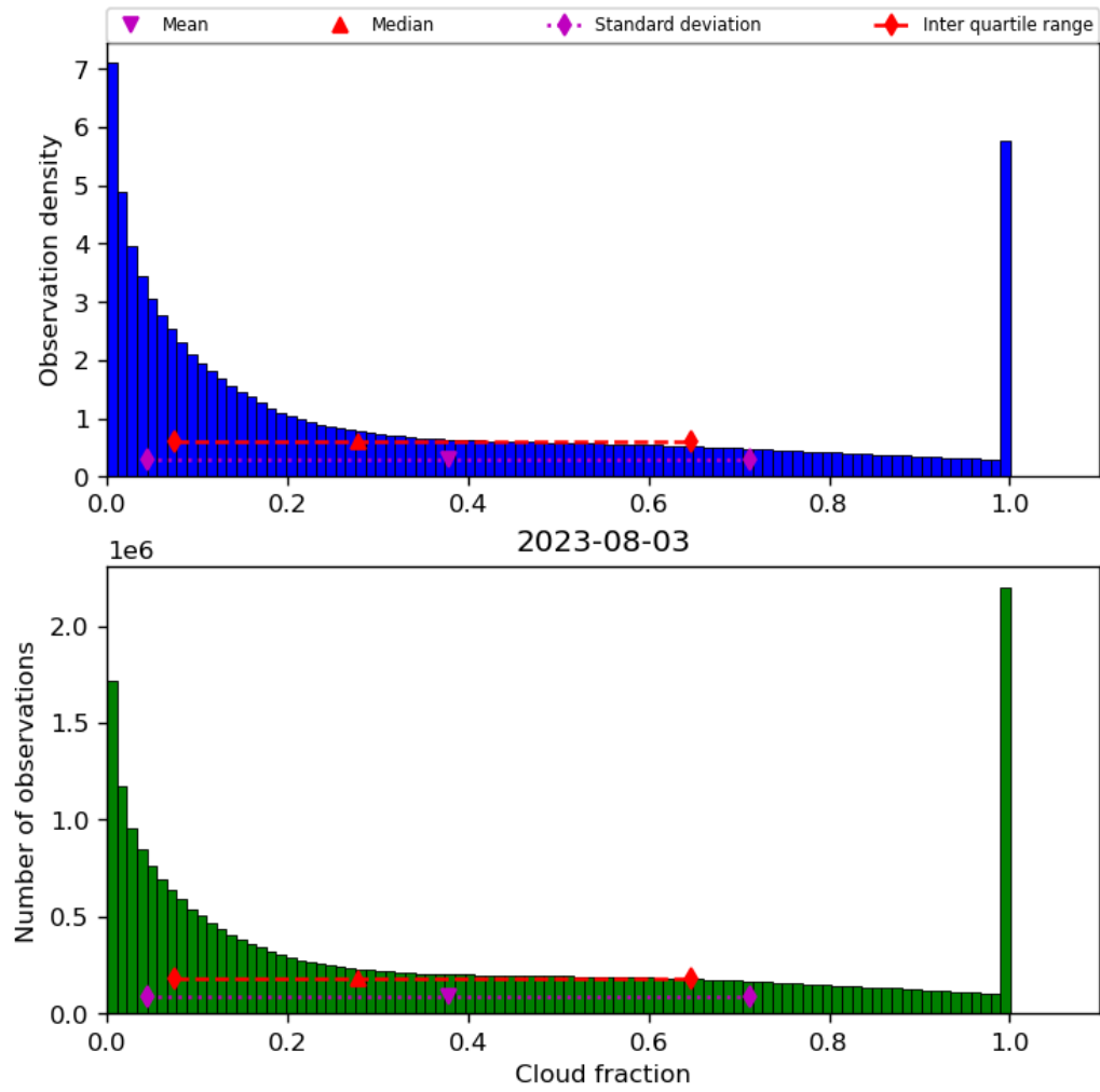
Figure 32: Histogram of “Cloud fraction” for 2023-08-02 to 2023-08-04
