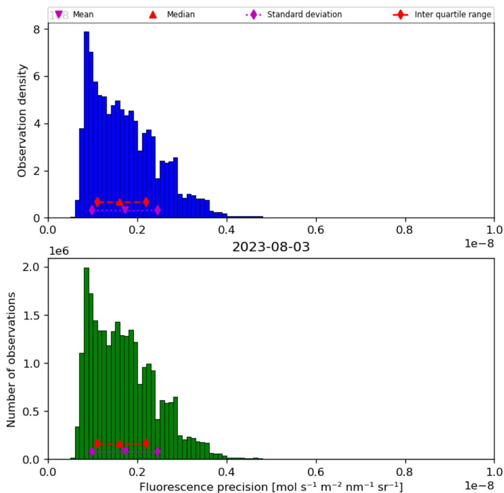
Figure 41: Histogram of “Fluorescence precision” for 2023-08-02 to 2023-08-04
