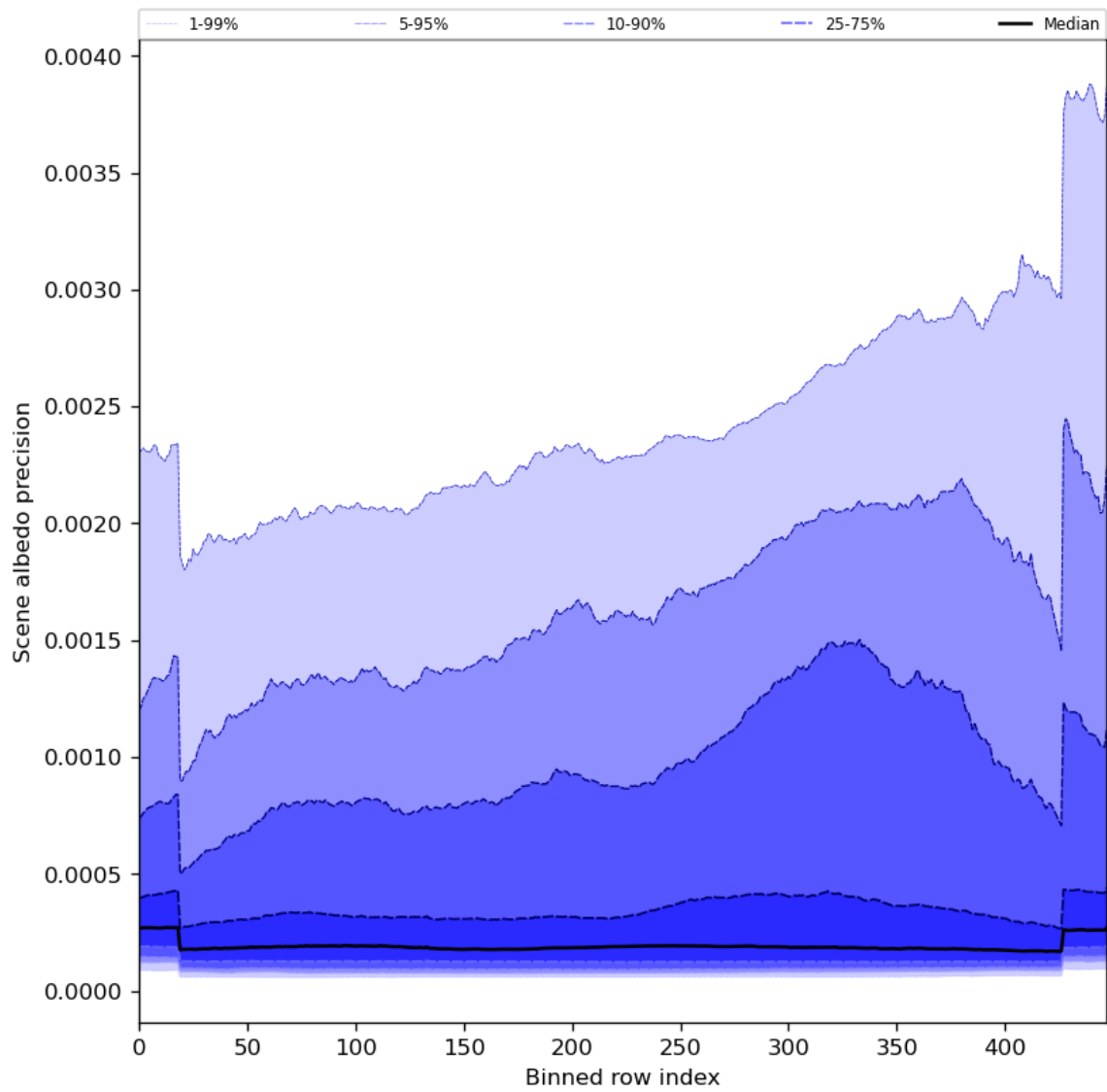
Figure 52: Along track statistics of “Scene albedo precision” for 2023-08-02 to 2023-08-04
