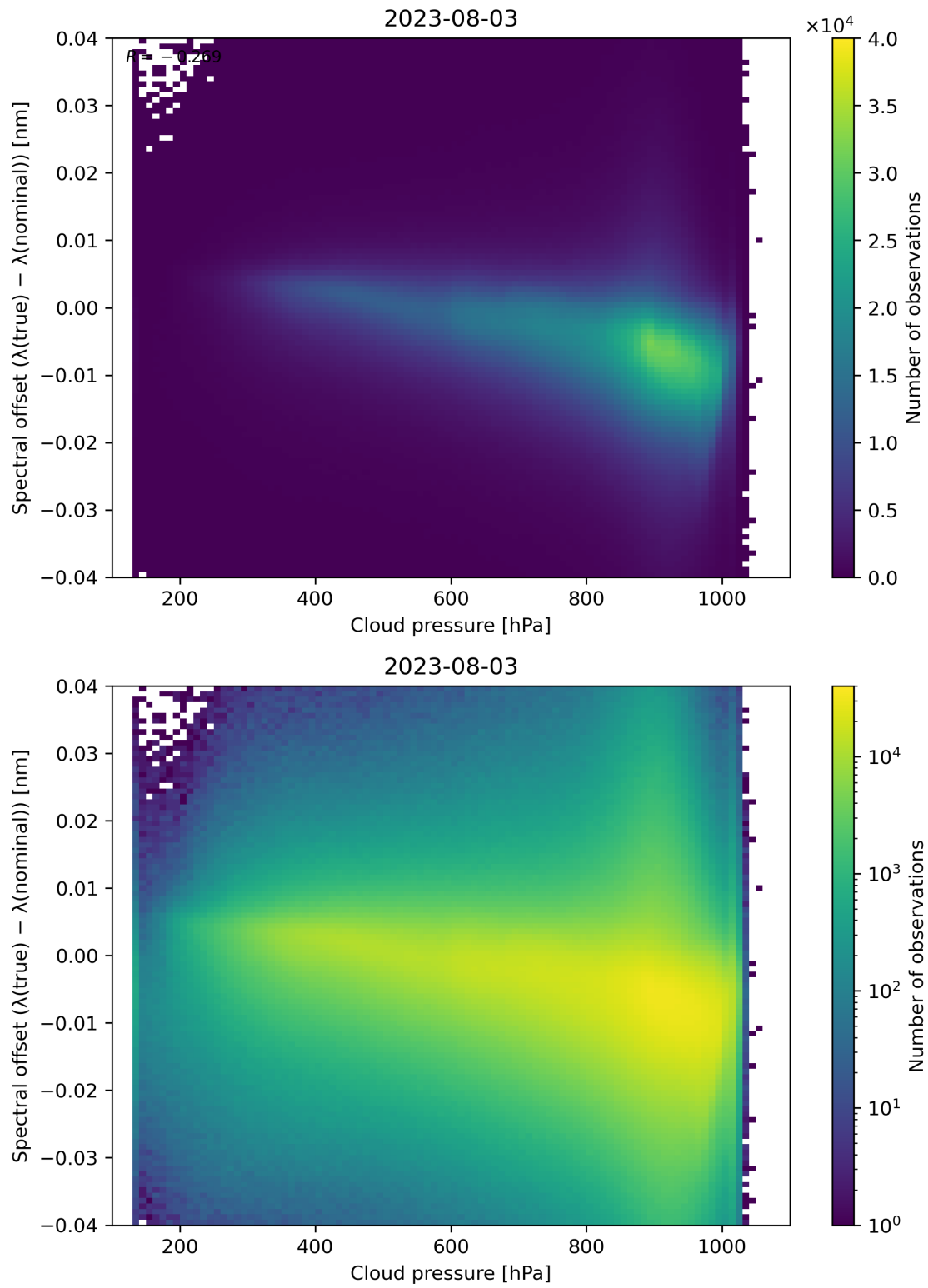
Figure 92: Scatter density plot of “Cloud pressure” against “Spectral offset ( \lambda(\text{true}) - \lambda(\text{nominal}) )” for 2023-08-02 to 2023-08-04.
