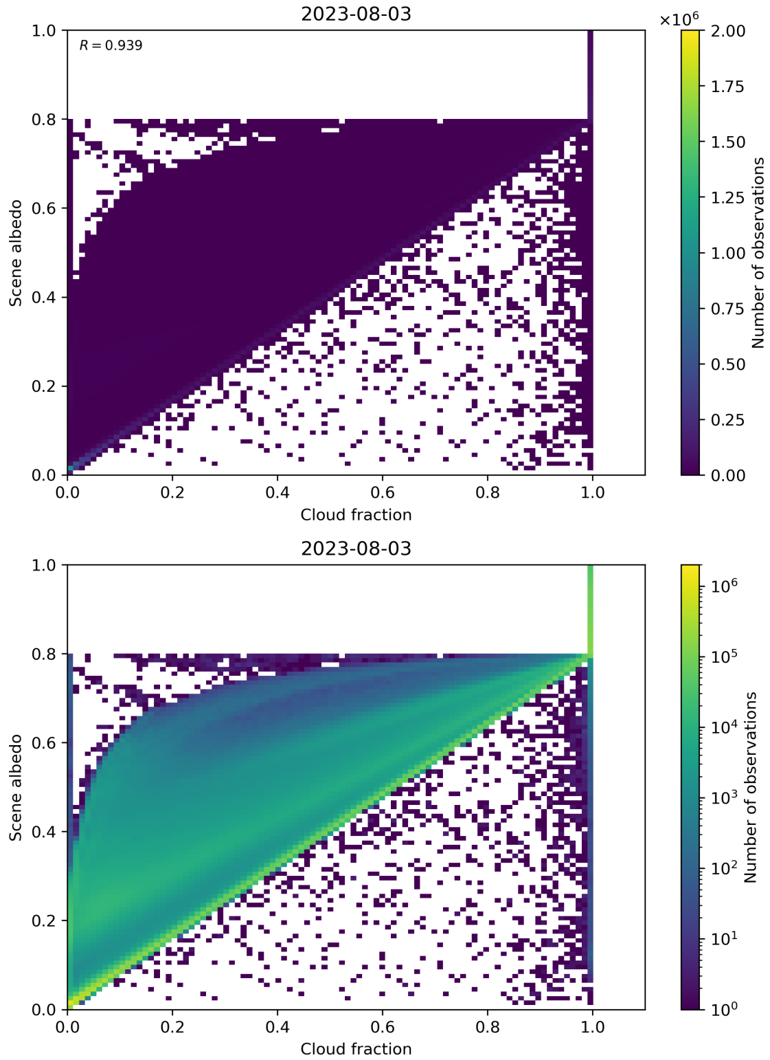
Figure 82: Scatter density plot of “Cloud fraction” against “Scene albedo” for 2023-08-02 to 2023-08-04.
