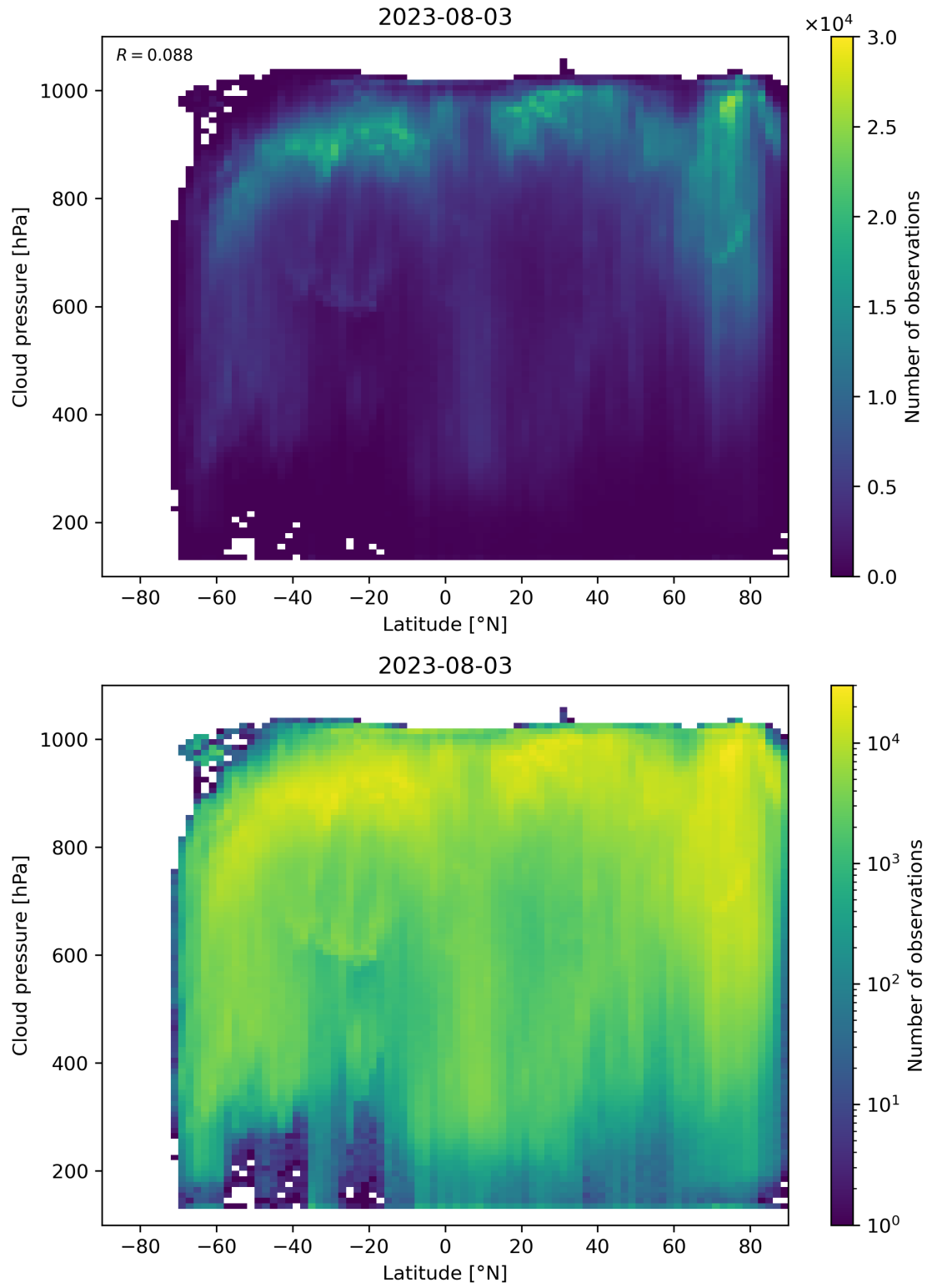
Figure 100: Scatter density plot of “Latitude” against “Cloud pressure” for 2023-08-02 to 2023-08-04.
