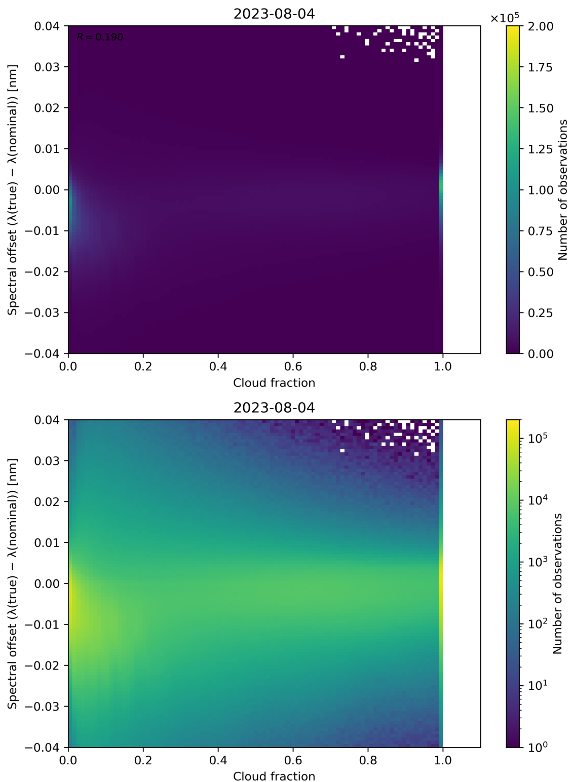
Figure 83: Scatter density plot of “Cloud fraction” against “Spectral offset ( \lambda(\text{true}) - \lambda(\text{nominal}) )” for 2023-08-04 to 2023-08-05.
