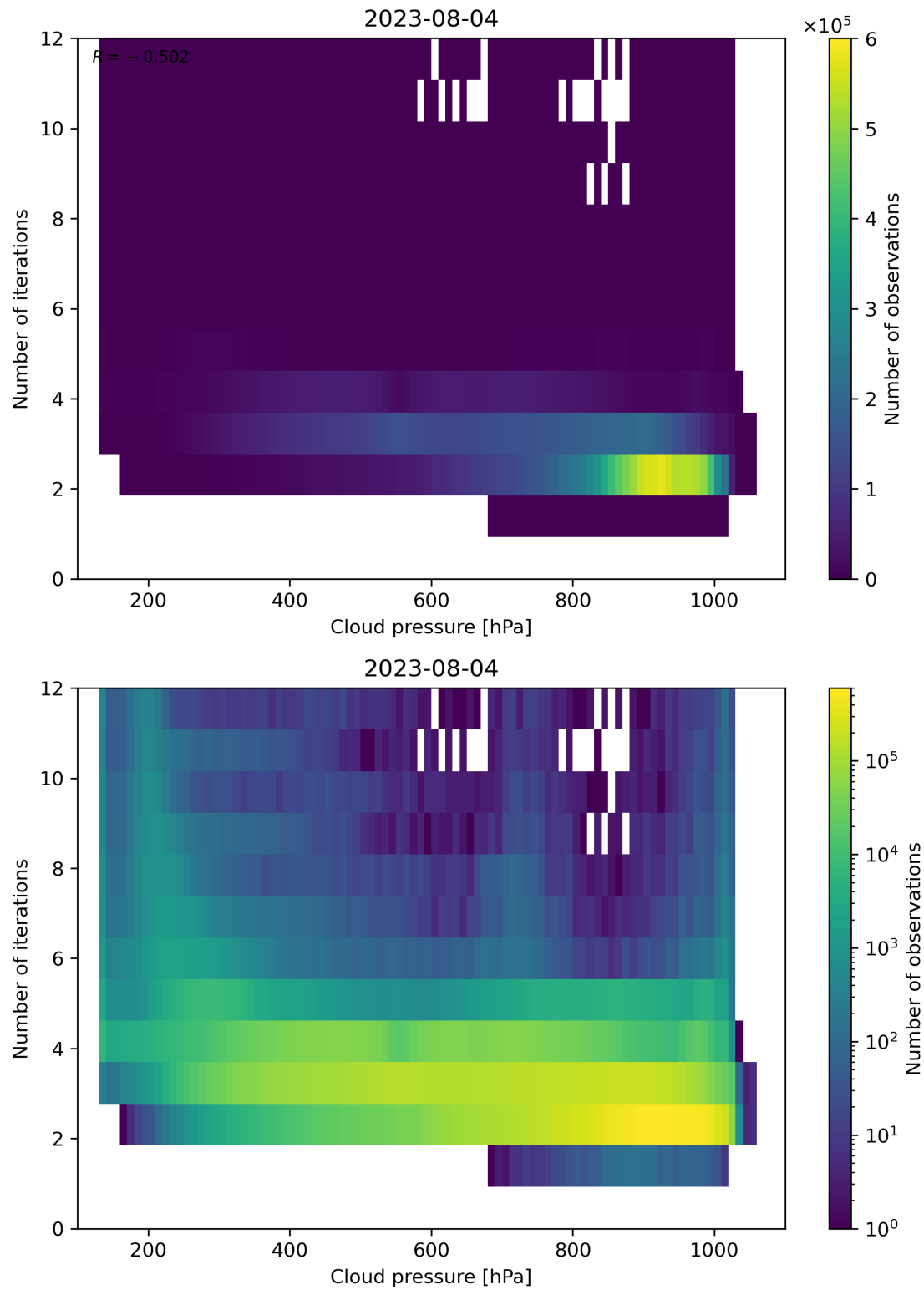
Figure 89: Scatter density plot of “Cloud pressure” against “Number of iterations” for 2023-08-04 to 2023-08-05.
