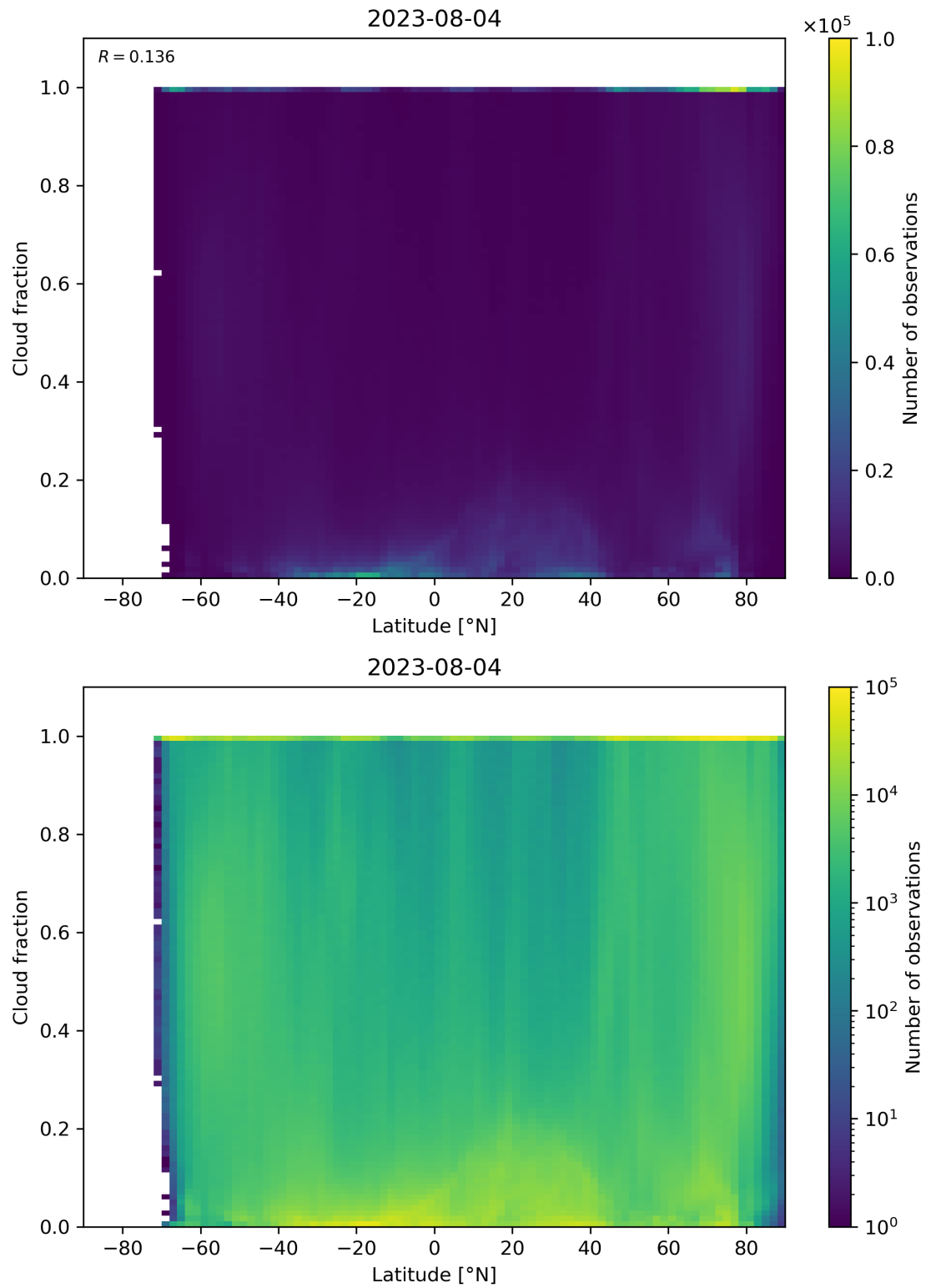
Figure 99: Scatter density plot of “Latitude” against “Cloud fraction” for 2023-08-04 to 2023-08-05.
