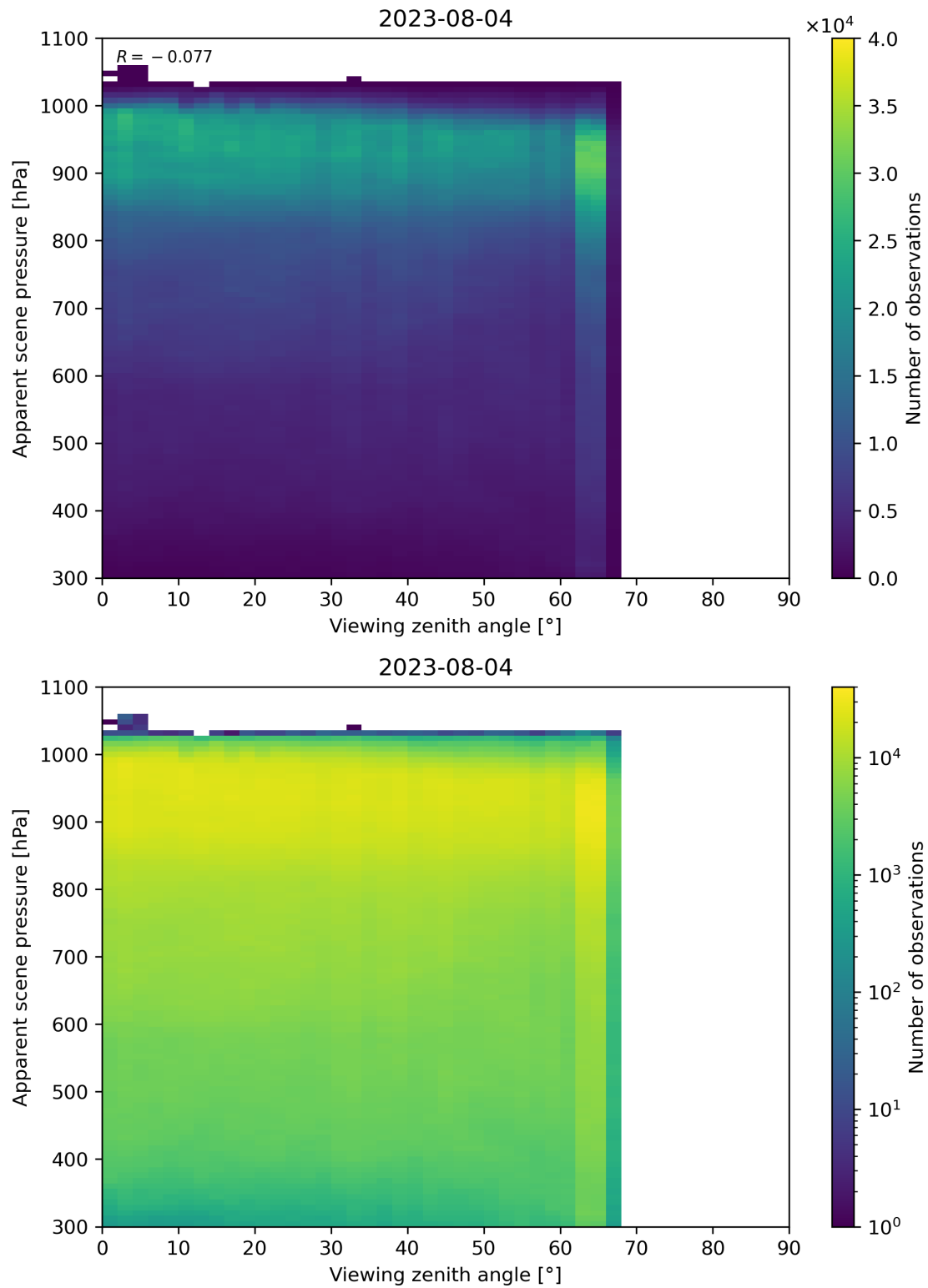
Figure 129: Scatter density plot of “Viewing zenith angle” against “Apparent scene pressure” for 2023-08-04 to 2023-08-05.
