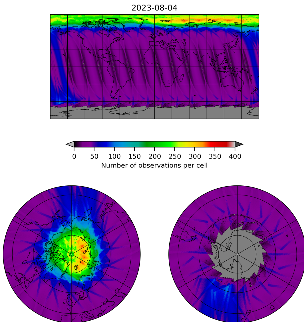
Figure 11: Map of the number of observations for 2023-08-04 to 2023-08-05
