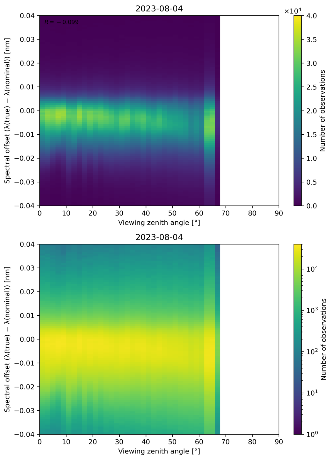
Figure 140: Scatter density plot of “Viewing zenith angle” against “Spectral offset ( \lambda(\text{true}) - \lambda(\text{nominal}) )” for 2023-08-04 to 2023-08-05.
