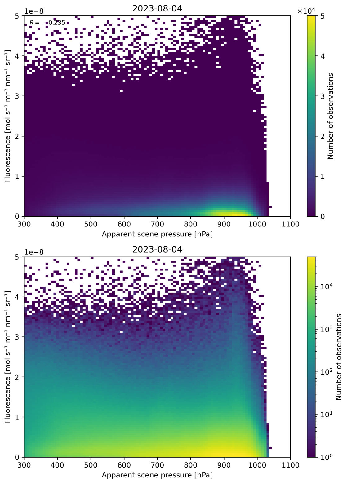
Figure 65: Scatter density plot of “Apparent scene pressure” against “Fluorescence” for 2023-08-04 to 2023-08-05.
