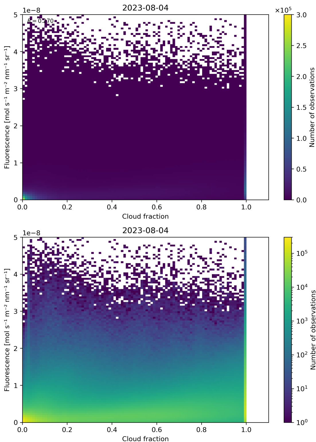
Figure 79: Scatter density plot of “Cloud fraction” against “Fluorescence” for 2023-08-04 to 2023-08-05.
