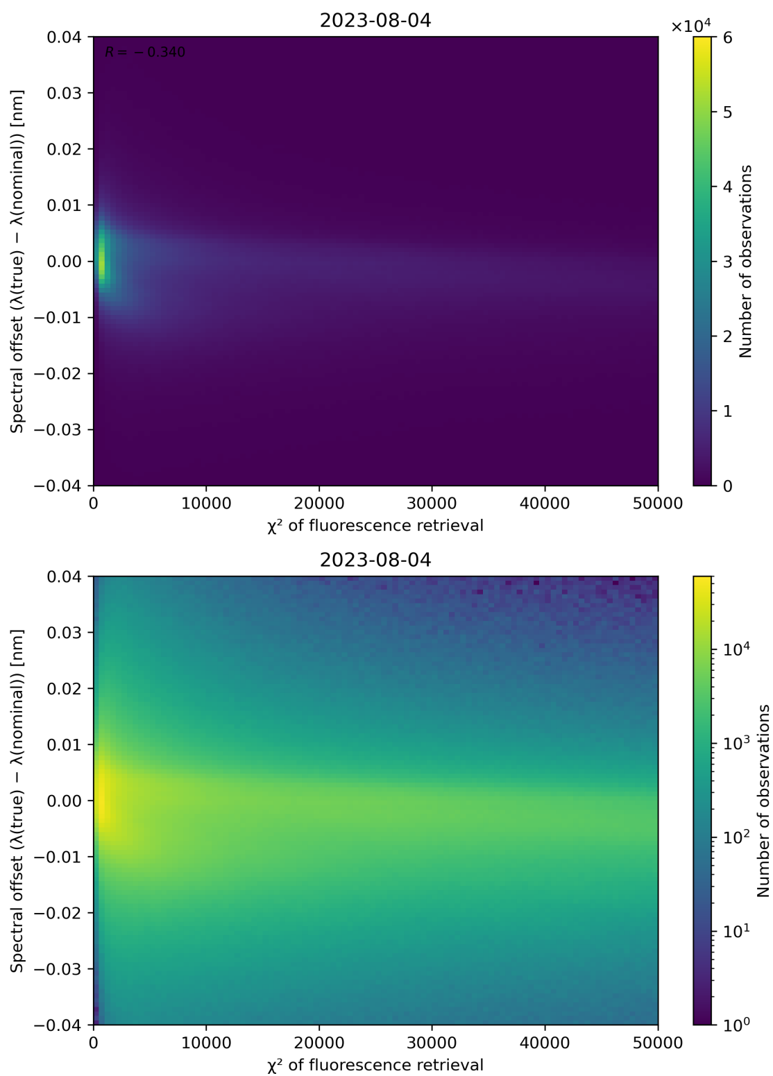
Figure 72: Scatter density plot of " \chi^2 of fluorescence retrieval" against "Spectral offset ( \lambda(\text{true}) - \lambda(\text{nominal})) " for 2023-08-04 to 2023-08-05.
