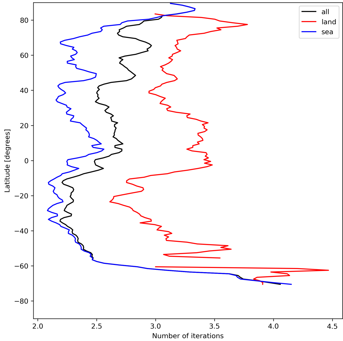
Figure 22: Zonal average of “Number of iterations” for 2023-08-04 to 2023-08-05.
