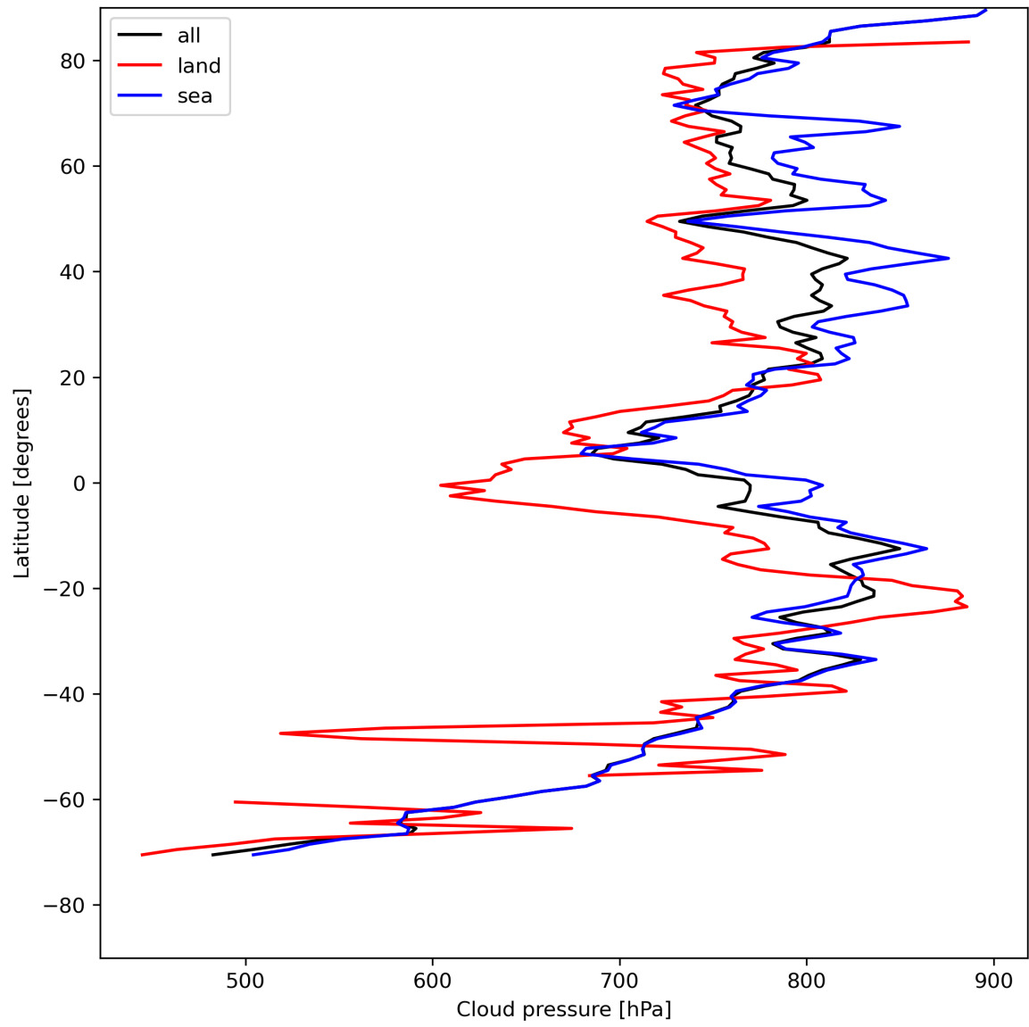
Figure 13: Zonal average of “Cloud pressure” for 2023-08-04 to 2023-08-05.
