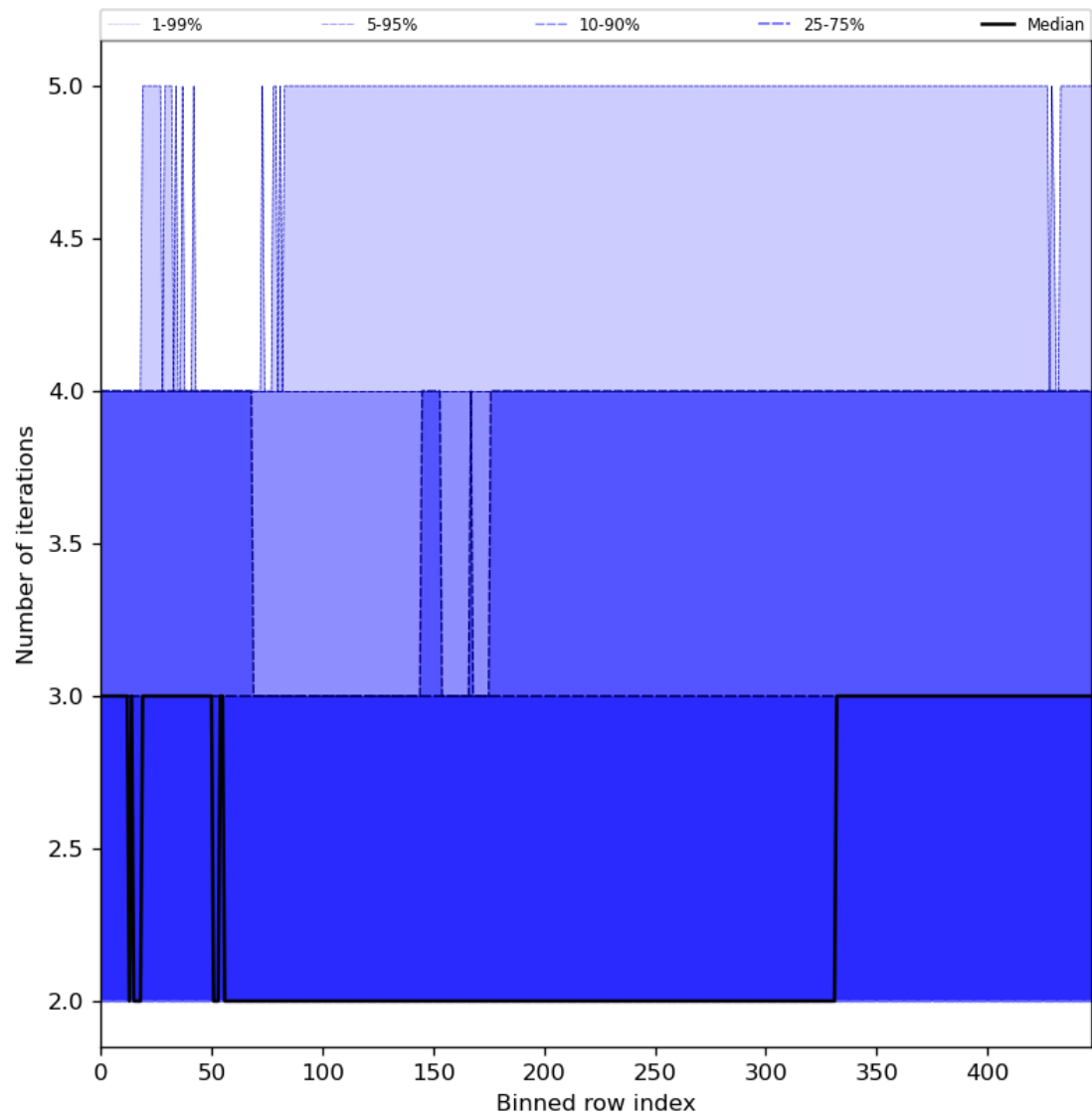
Figure 56: Along track statistics of “Number of iterations” for 2023-08-04 to 2023-08-05
