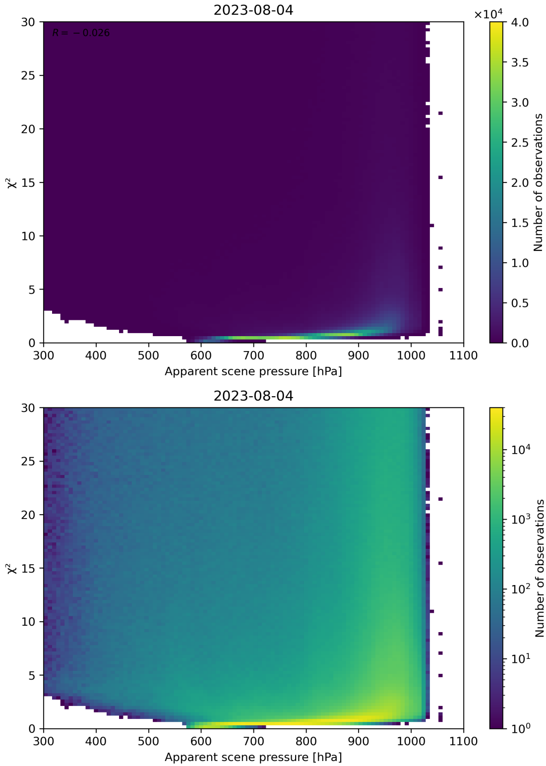
Figure 63: Scatter density plot of “Apparent scene pressure” against “ \chi^2 ” for 2023-08-04 to 2023-08-05.
