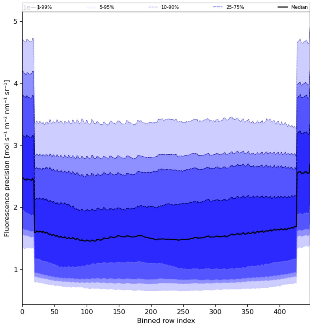
Figure 58: Along track statistics of “Fluorescence precision” for 2023-08-04 to 2023-08-05
