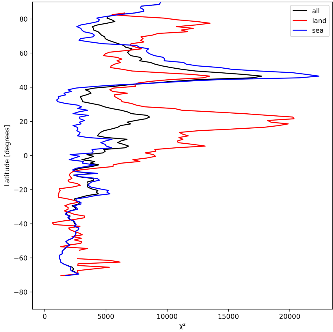
Figure 21: Zonal average of “ \chi^2 ” for 2023-08-04 to 2023-08-05.
