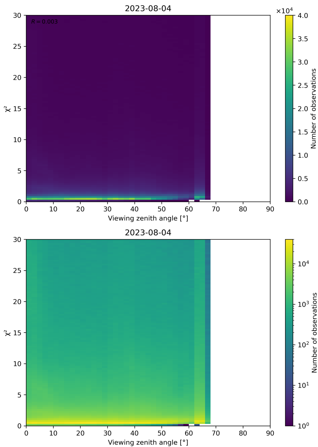
Figure 130: Scatter density plot of “Viewing zenith angle” against “ \chi^2 ” for 2023-08-04 to 2023-08-05.
