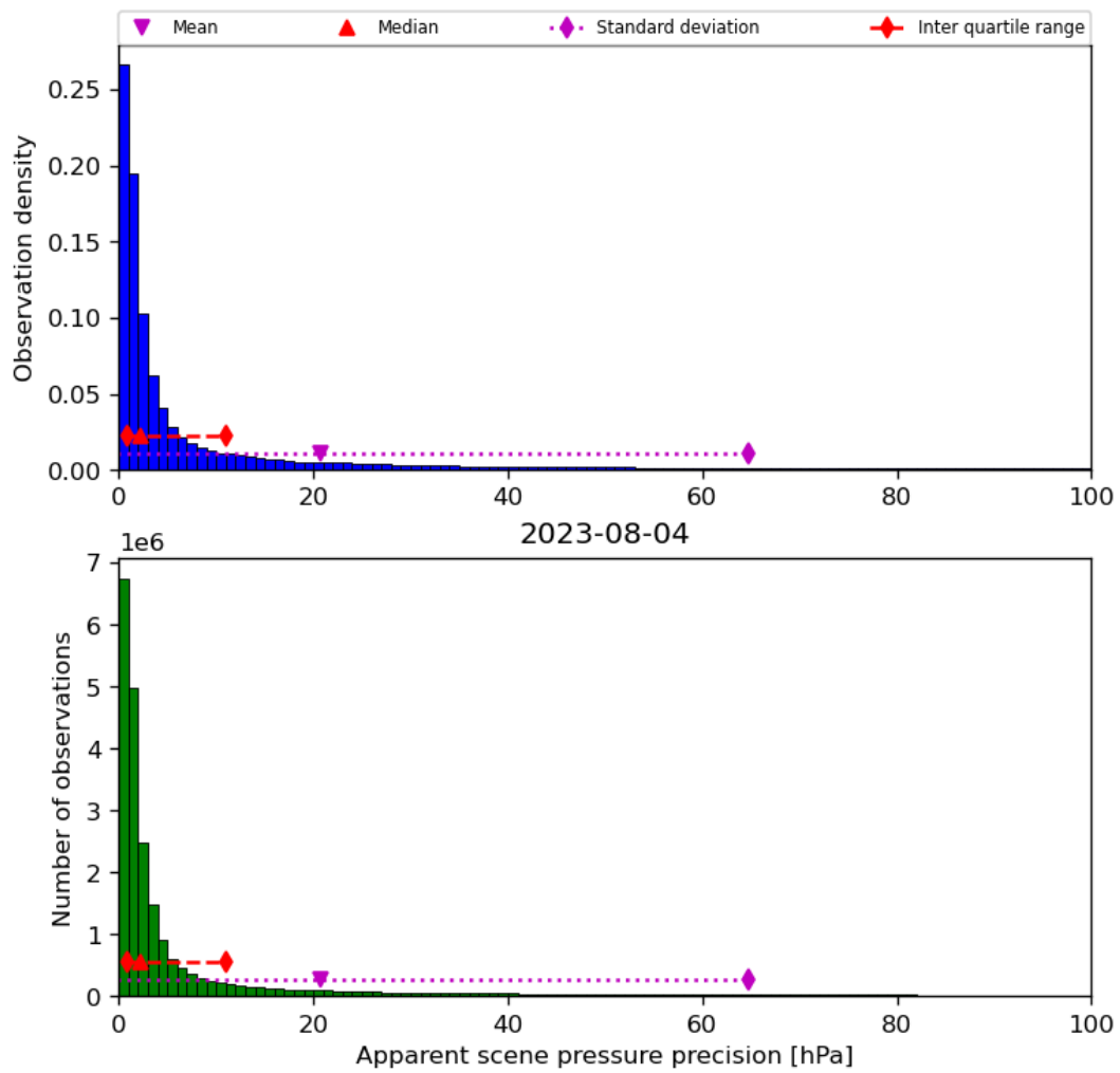
Figure 37: Histogram of “Apparent scene pressure precision” for 2023-08-04 to 2023-08-05
