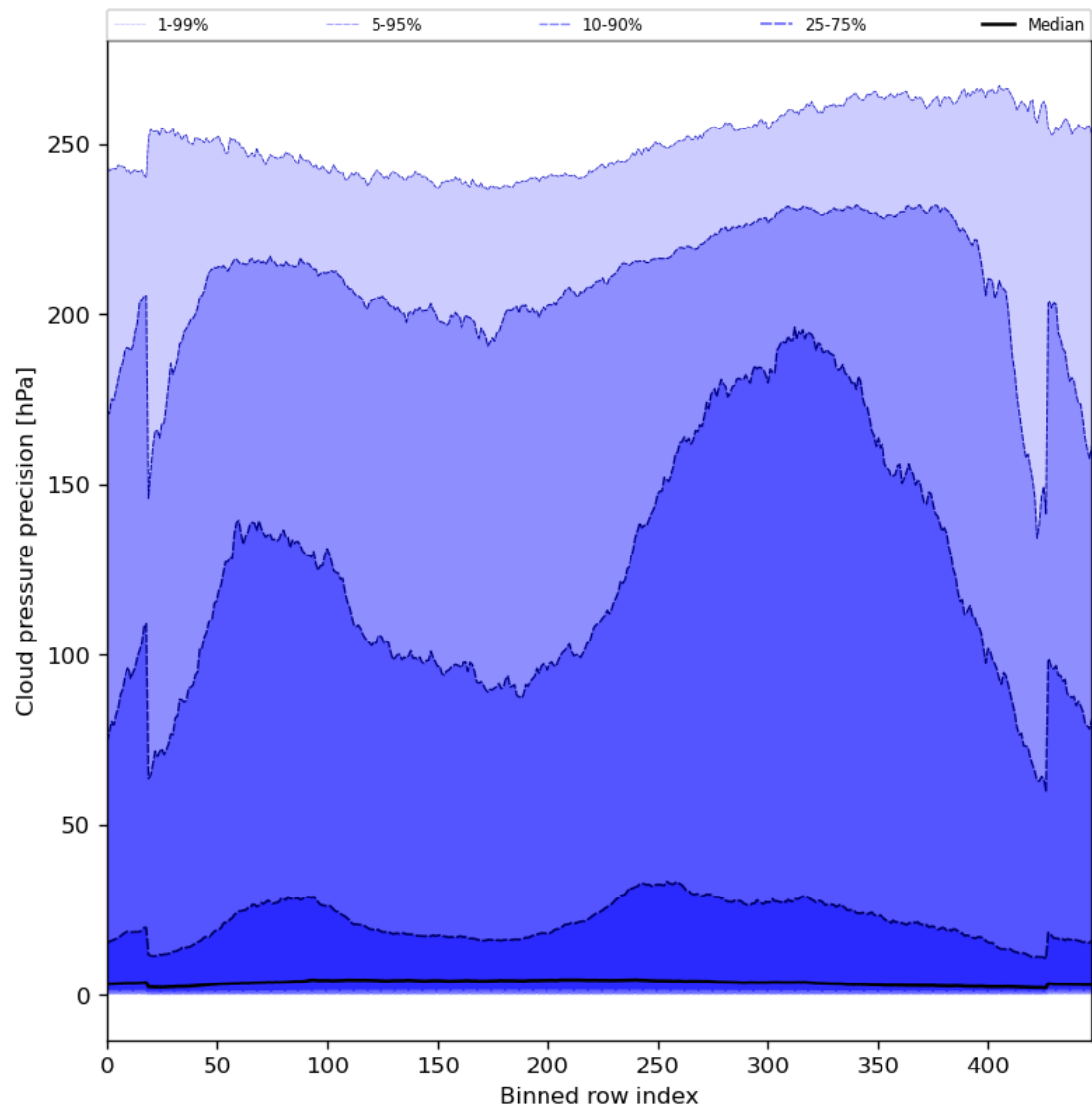
Figure 48: Along track statistics of “Cloud pressure precision” for 2023-08-04 to 2023-08-05
