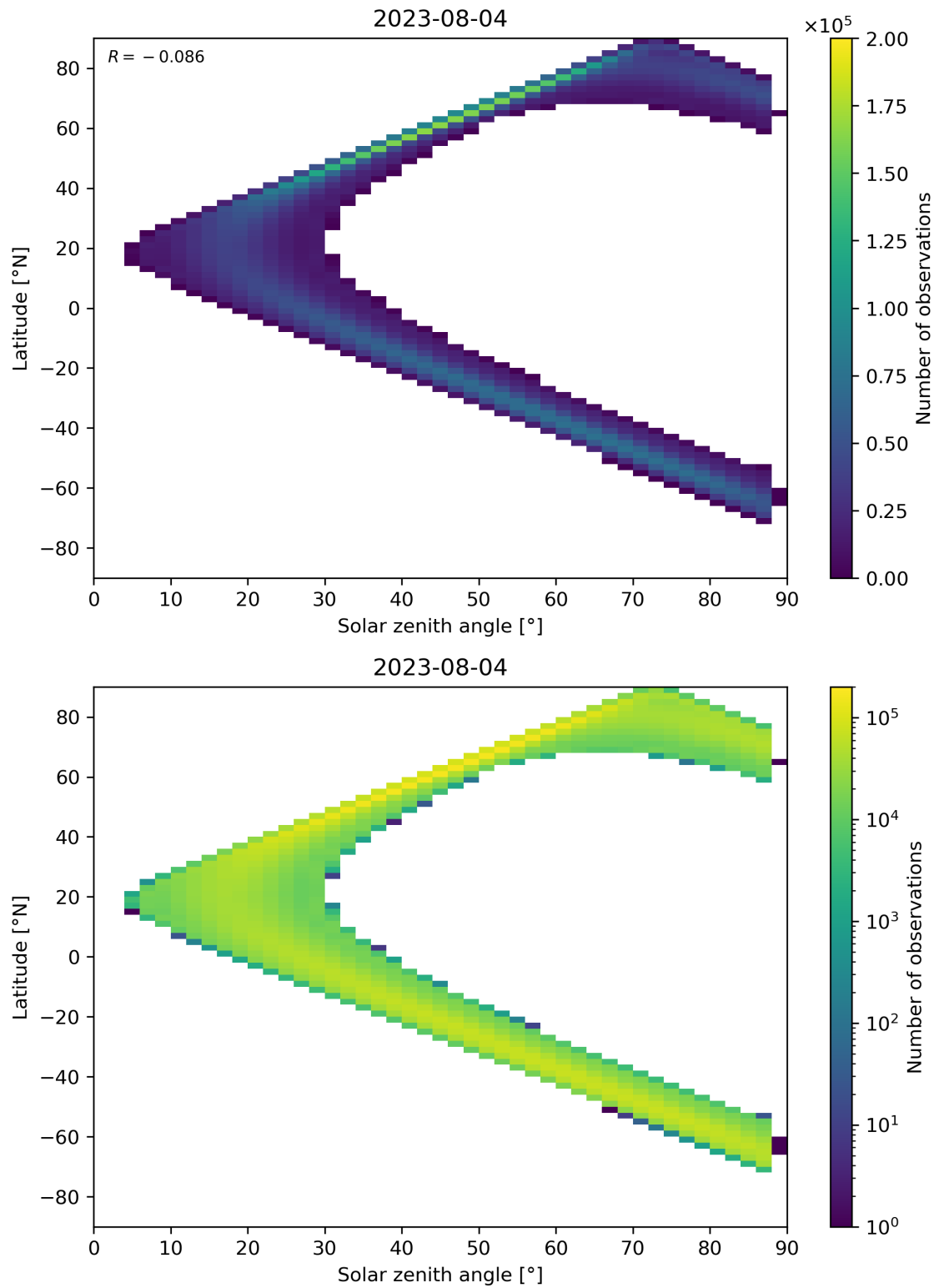
Figure 124: Scatter density plot of “Solar zenith angle” against “Latitude” for 2023-08-04 to 2023-08-05.
