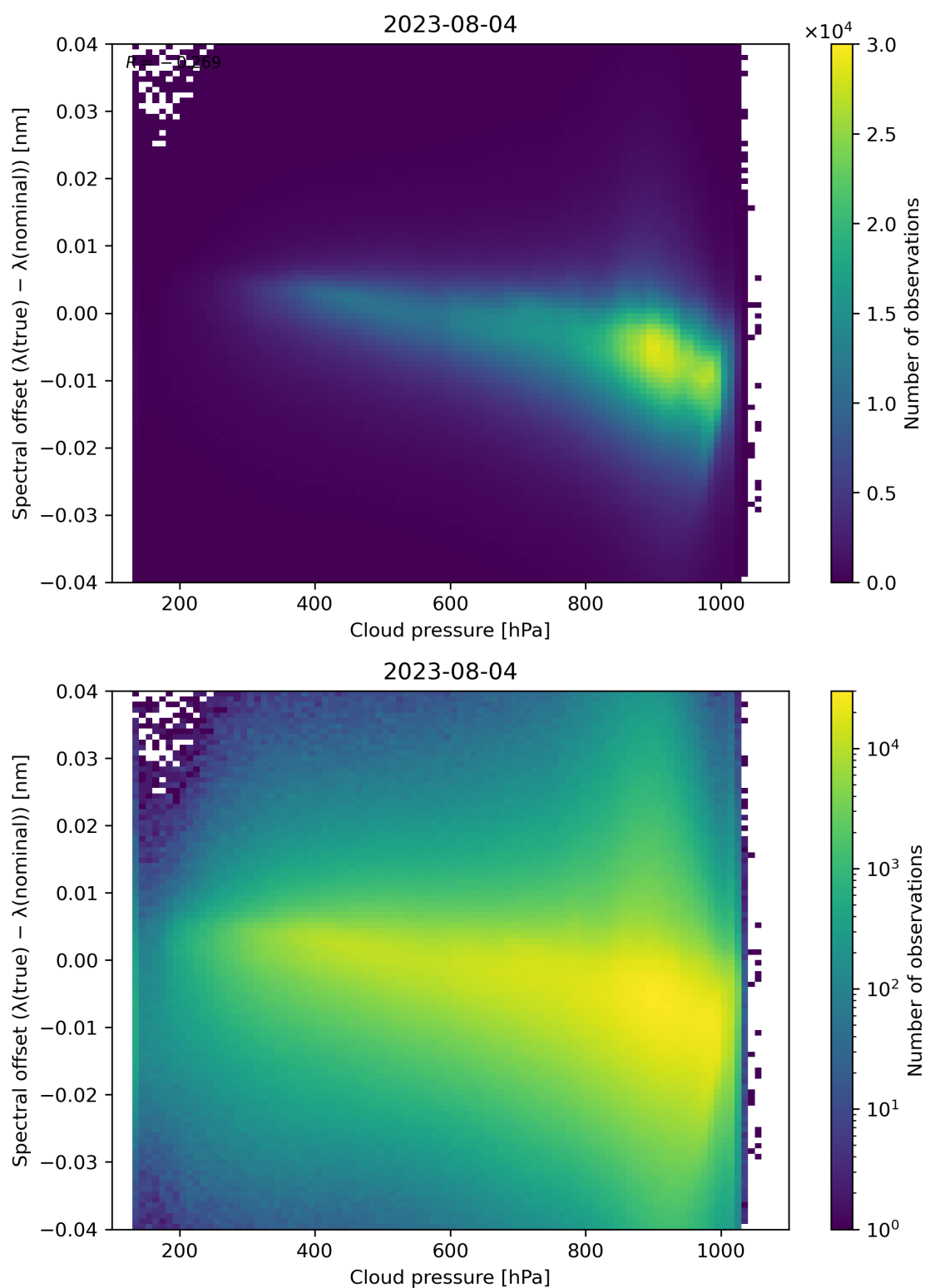
Figure 92: Scatter density plot of “Cloud pressure” against “Spectral offset ( \lambda(\text{true}) - \lambda(\text{nominal}) )” for 2023-08-04 to 2023-08-05.
