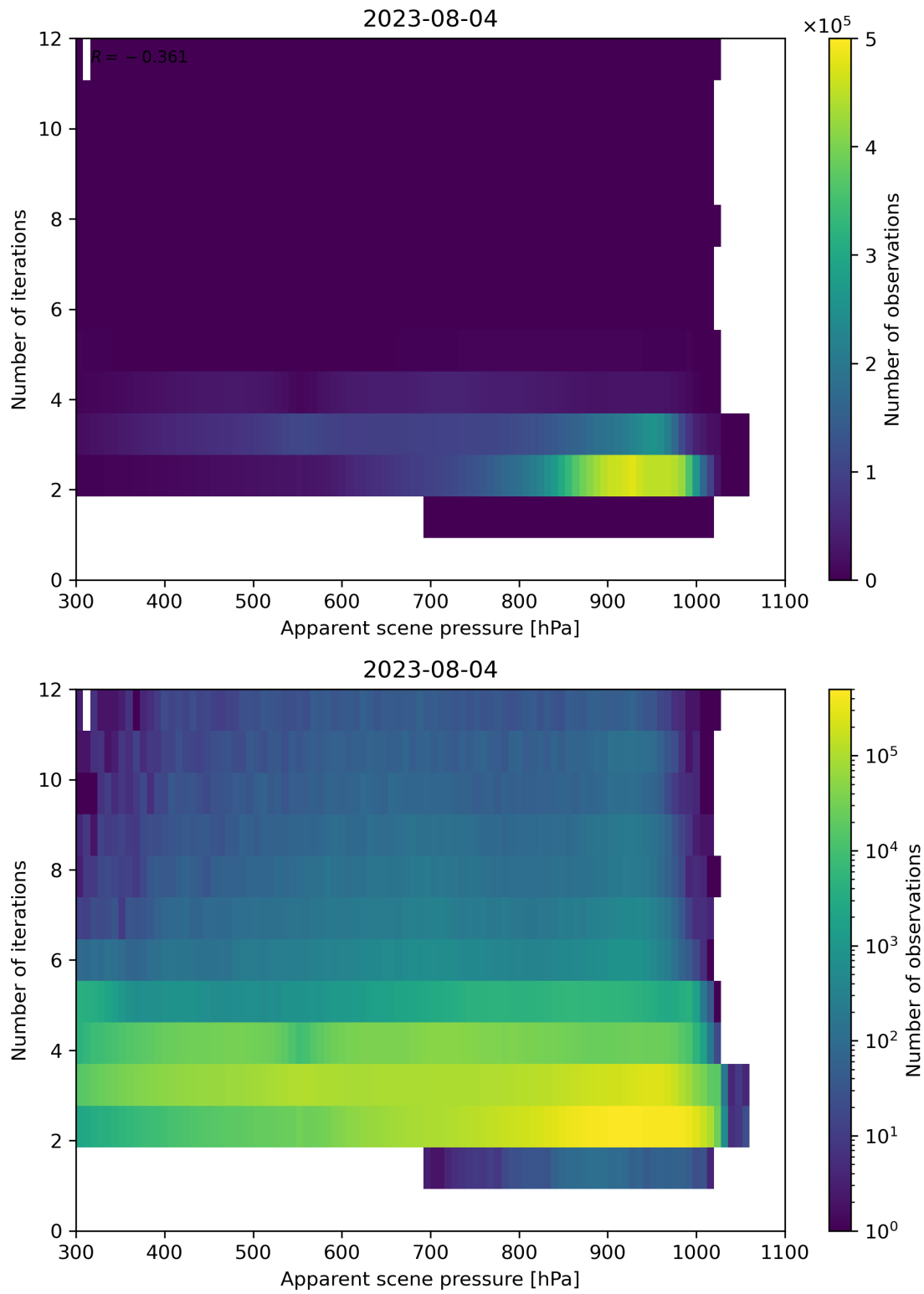
Figure 66: Scatter density plot of “Apparent scene pressure” against “Number of iterations” for 2023-08-04 to 2023-08-05.
