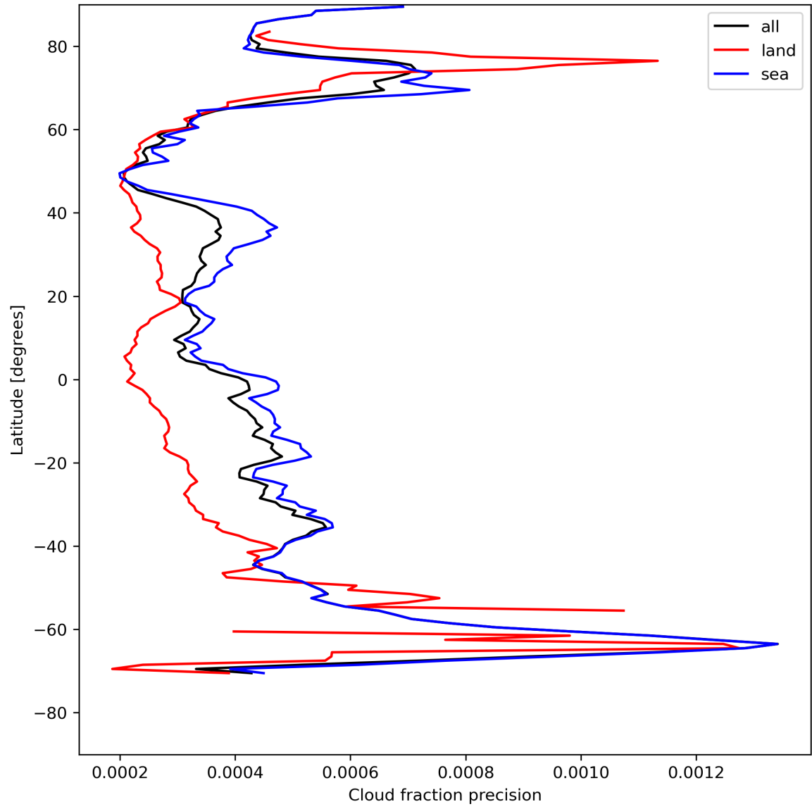
Figure 16: Zonal average of “Cloud fraction precision” for 2023-08-04 to 2023-08-05.
