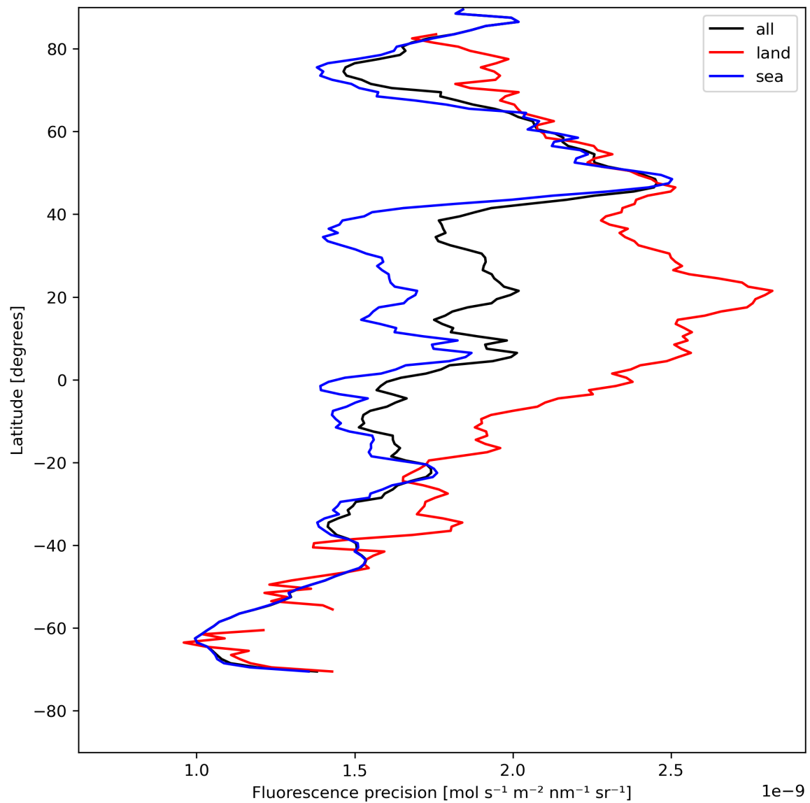
Figure 24: Zonal average of “Fluorescence precision” for 2023-08-04 to 2023-08-05.
