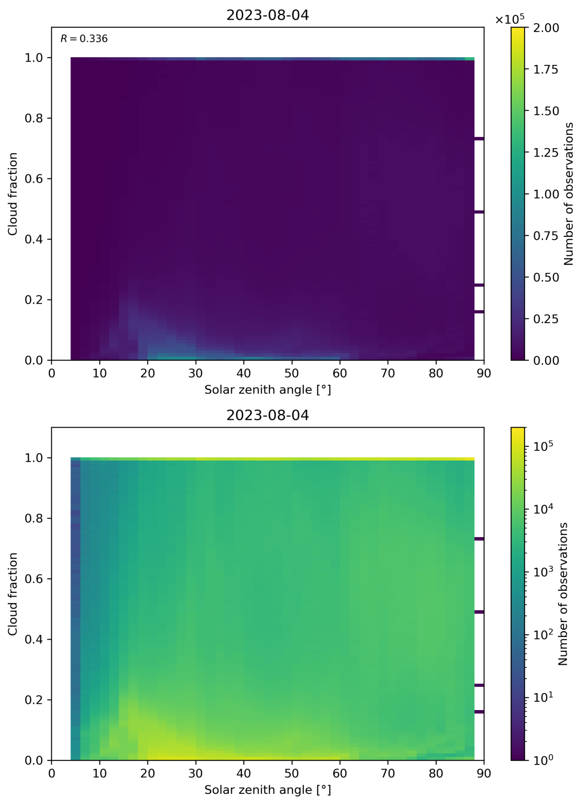
Figure 121: Scatter density plot of “Solar zenith angle” against “Cloud fraction” for 2023-08-04 to 2023-08-05.
