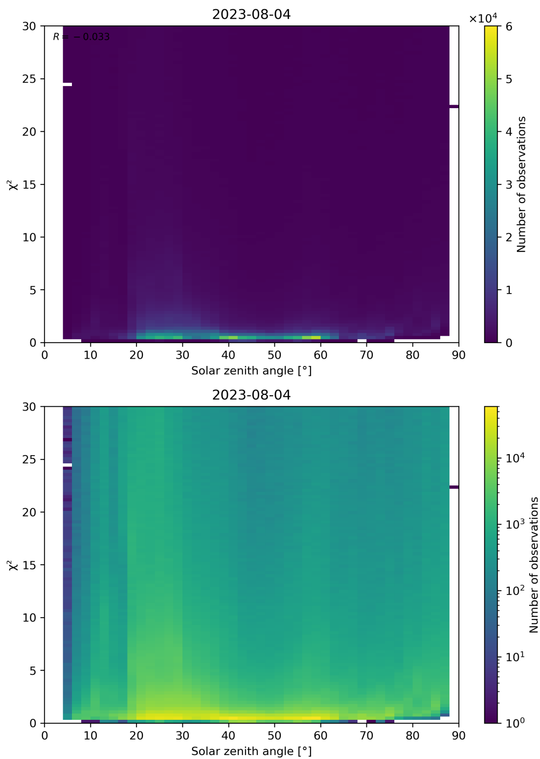
Figure 119: Scatter density plot of “Solar zenith angle” against “ \chi^2 ” for 2023-08-04 to 2023-08-05.
