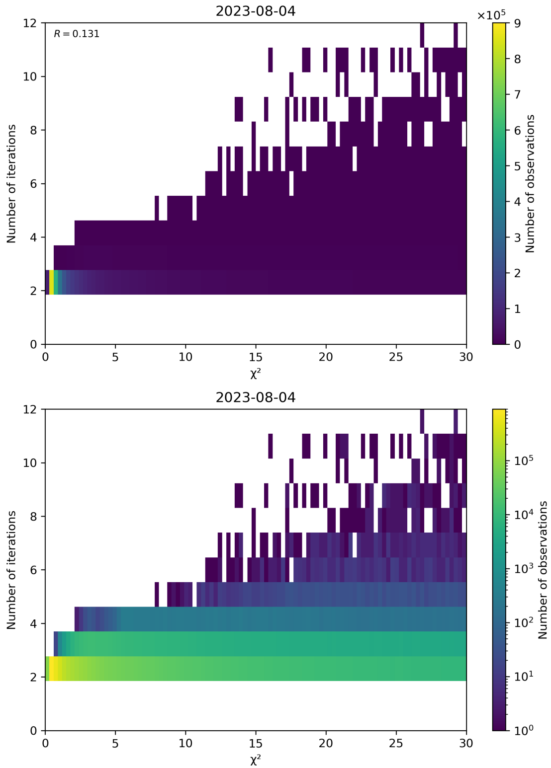
Figure 73: Scatter density plot of “ \chi^2 ” against “Number of iterations” for 2023-08-04 to 2023-08-05.
