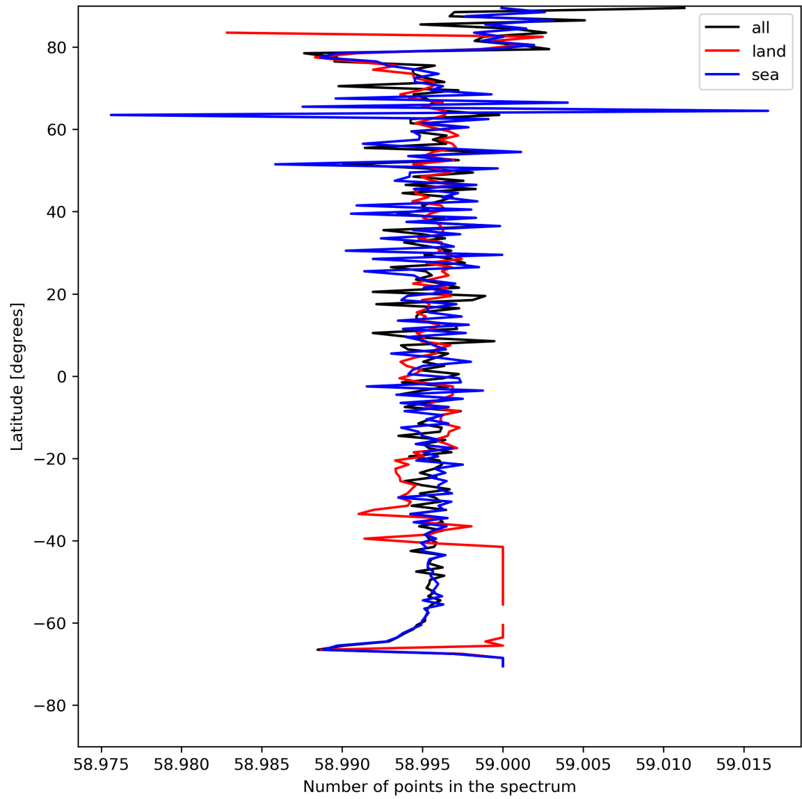
Figure 27: Zonal average of “Number of points in the spectrum” for 2023-08-04 to 2023-08-05.
