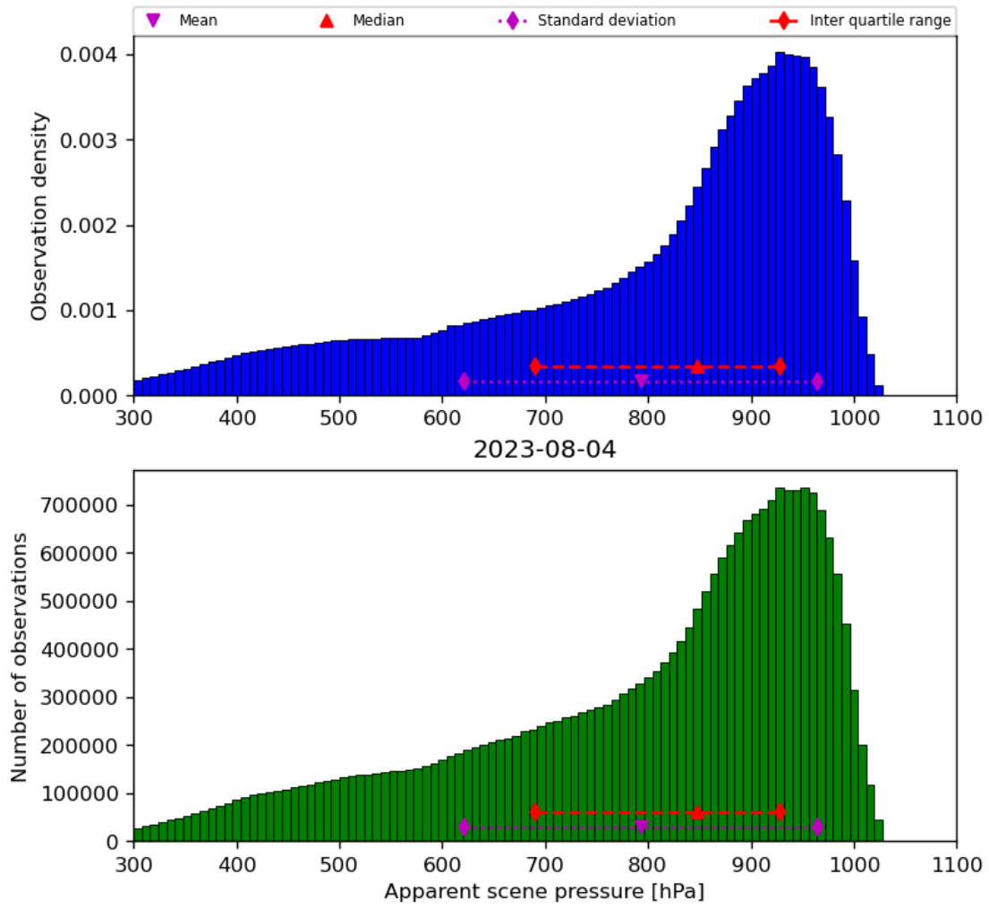
Figure 36: Histogram of "Apparent scene pressure" for 2023-08-04 to 2023-08-05
