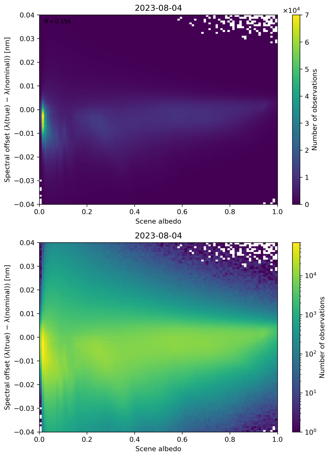
Figure 117: Scatter density plot of “Scene albedo” against “Spectral offset ( \lambda(\text{true}) - \lambda(\text{nominal}) )” for 2023-08-04 to 2023-08-05.
