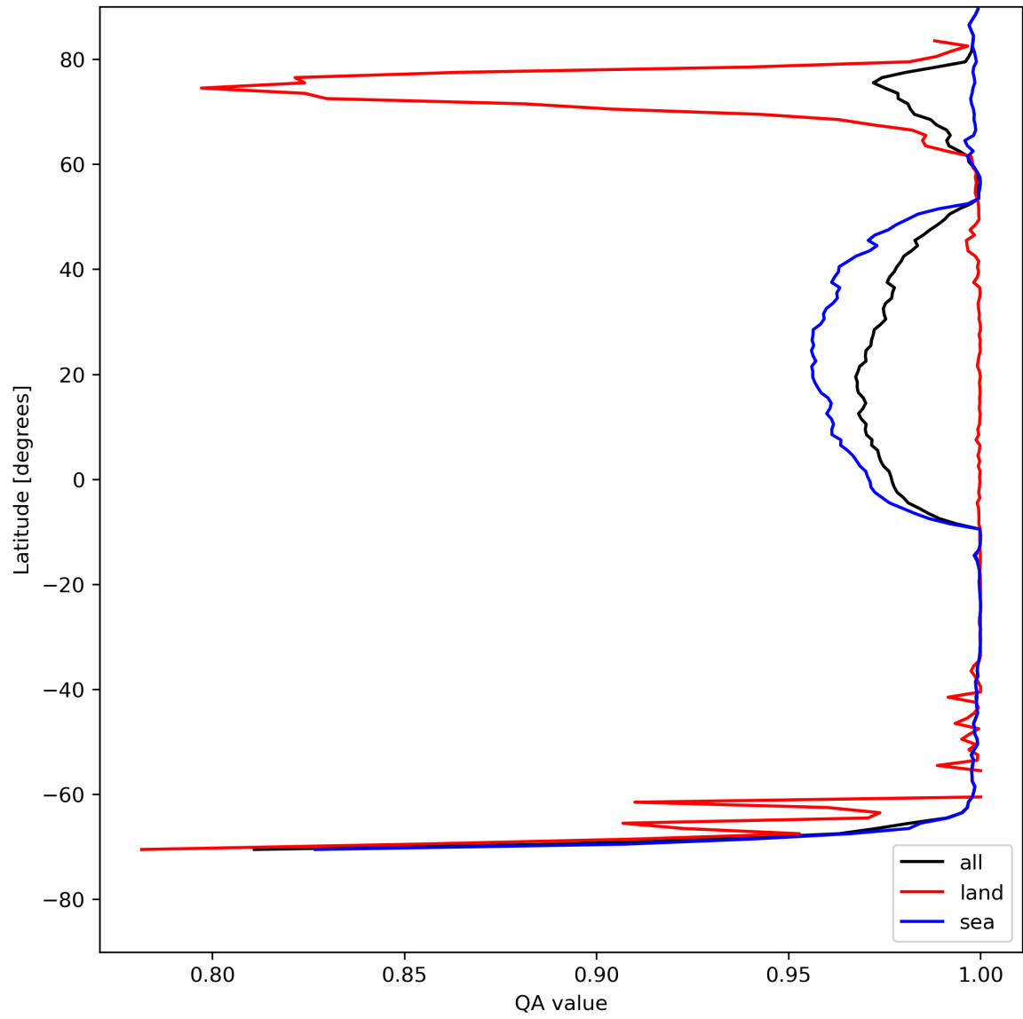
Figure 12: Zonal average of “QA value” for 2023-08-04 to 2023-08-05.
