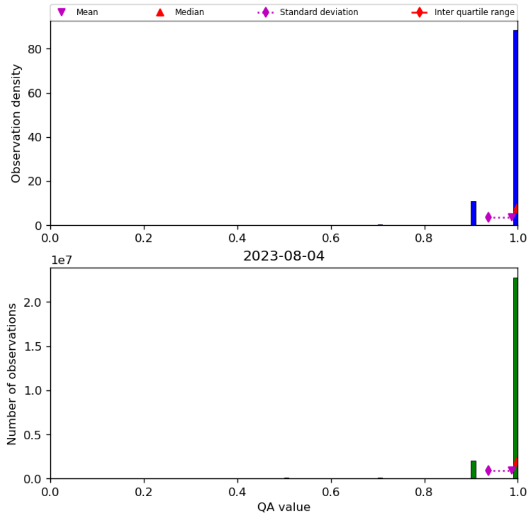
Figure 29: Histogram of “QA value” for 2023-08-04 to 2023-08-05
