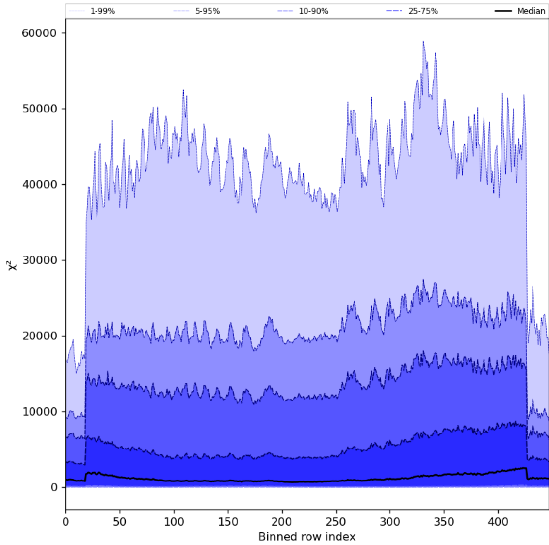
Figure 55: Along track statistics of “ \chi^2 ” for 2023-08-04 to 2023-08-05
