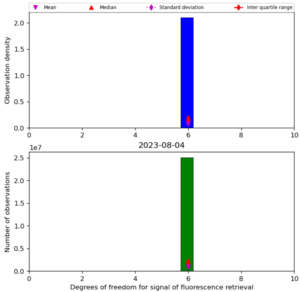
Figure 43: Histogram of “Degrees of freedom for signal of fluorescence retrieval” for 2023-08-04 to 2023-08-05
