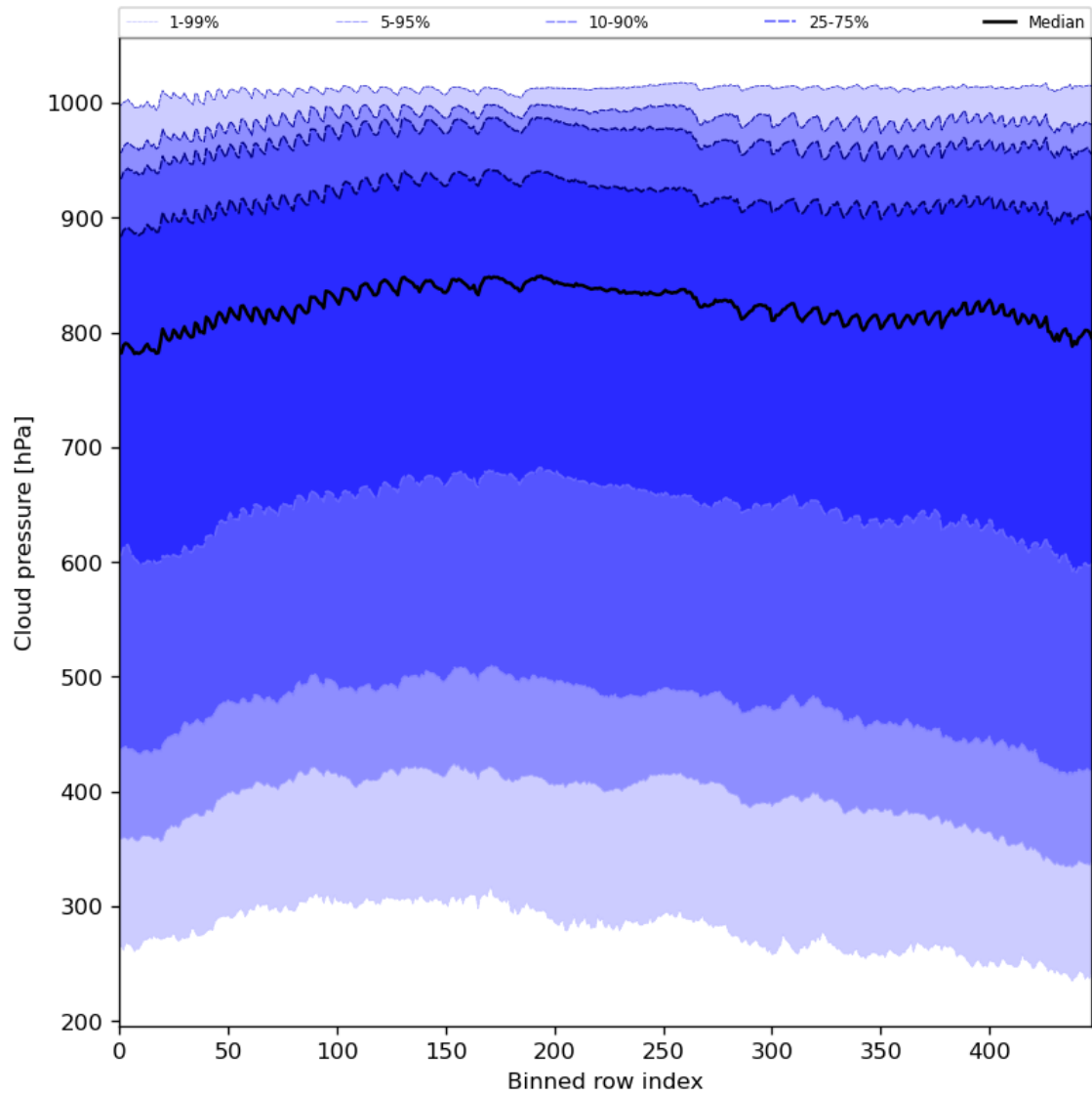
Figure 47: Along track statistics of “Cloud pressure” for 2023-08-04 to 2023-08-05
