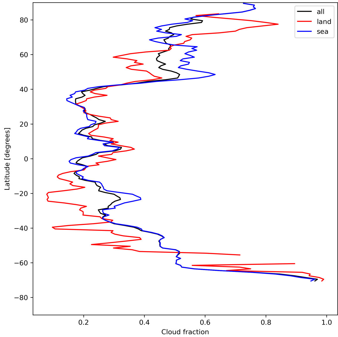
Figure 15: Zonal average of “Cloud fraction” for 2023-08-04 to 2023-08-05.
