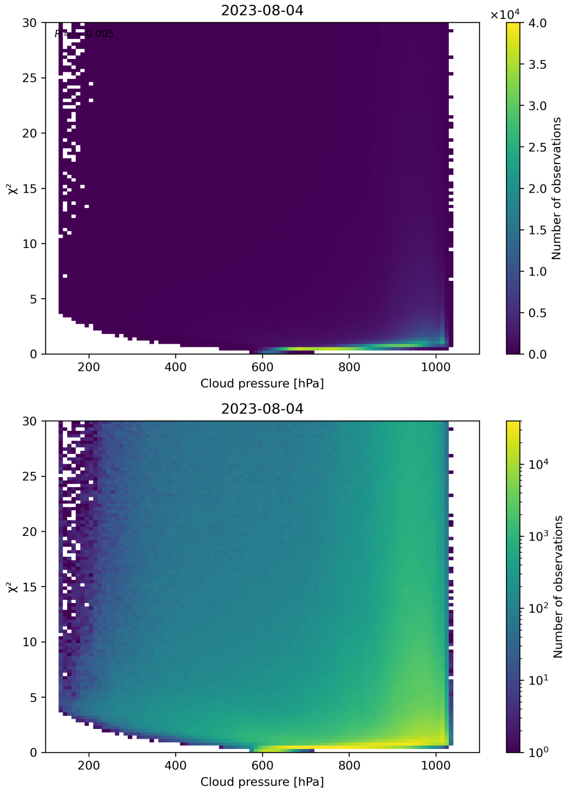
Figure 85: Scatter density plot of “Cloud pressure” against “ \chi^2 ” for 2023-08-04 to 2023-08-05.
