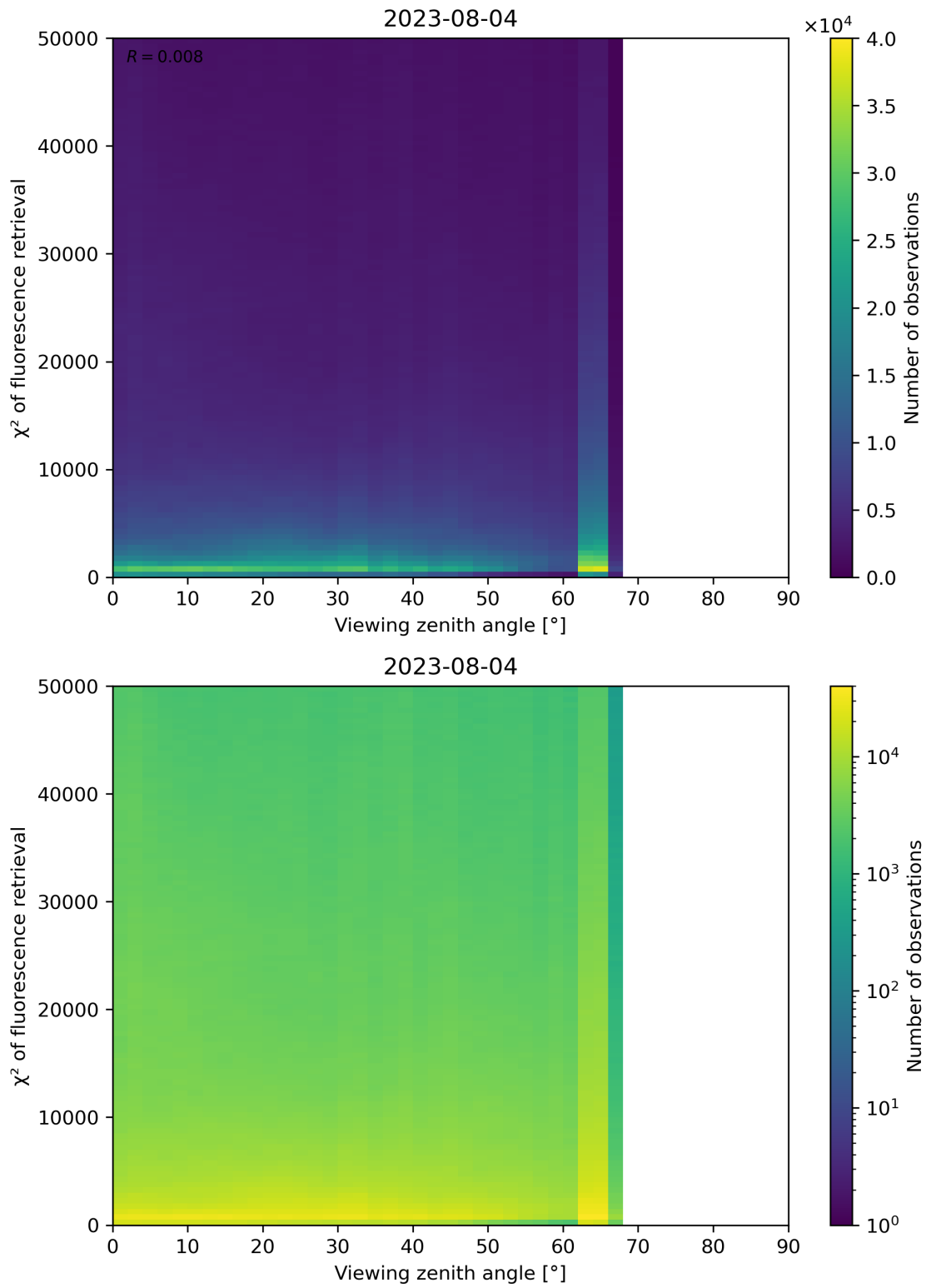
Figure 131: Scatter density plot of “Viewing zenith angle” against “ \chi^2 of fluorescence retrieval” for 2023-08-04 to 2023-08-05.
