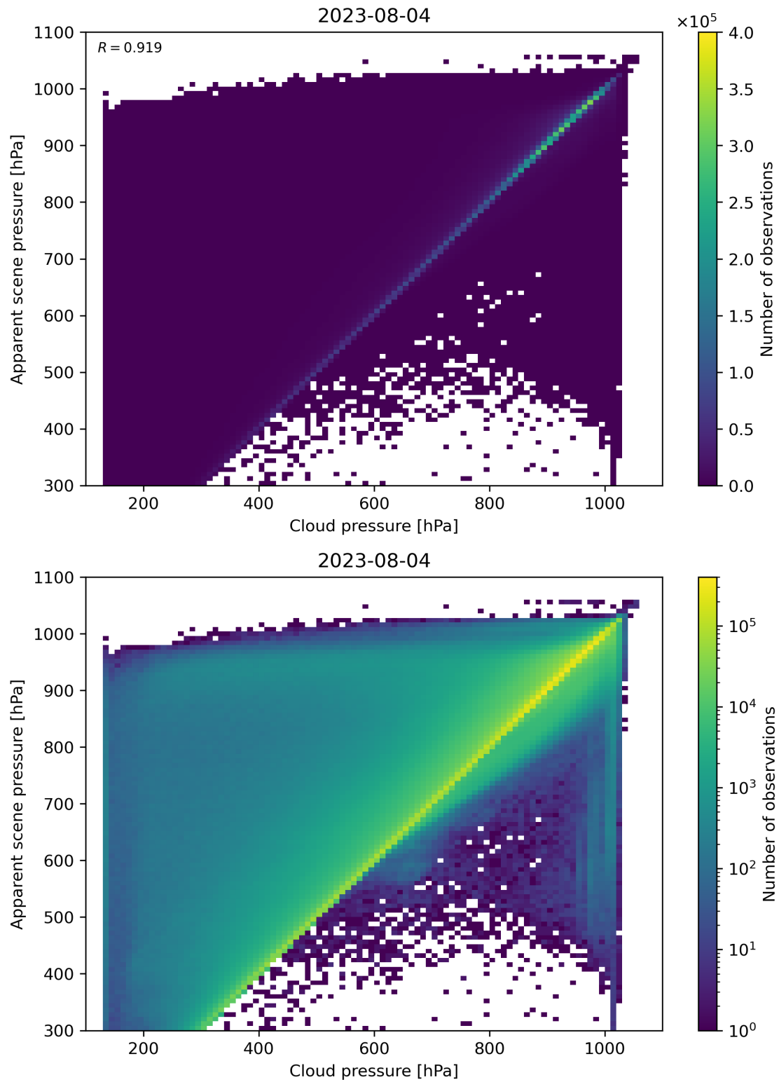
Figure 84: Scatter density plot of “Cloud pressure” against “Apparent scene pressure” for 2023-08-04 to 2023-08-05.
