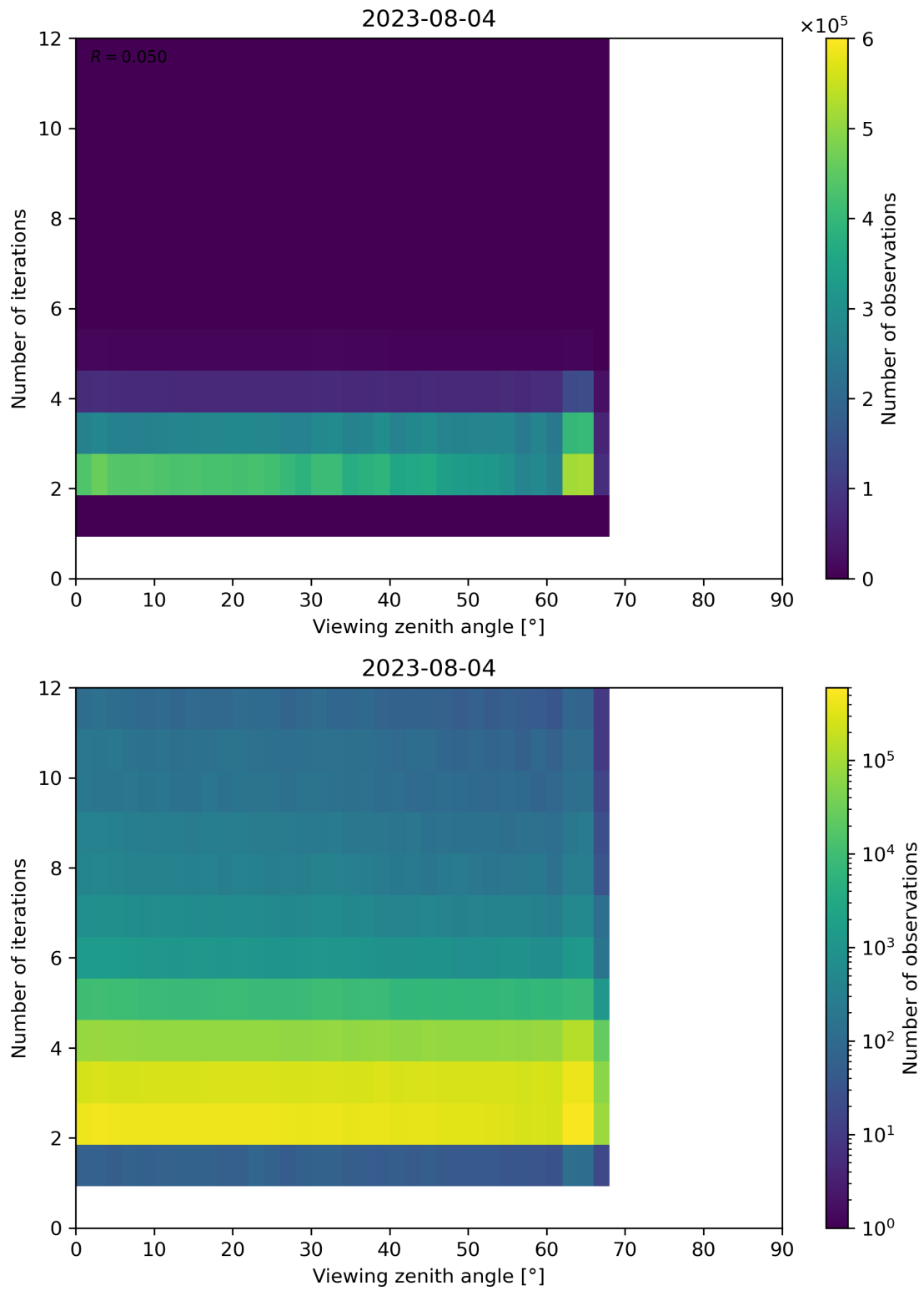
Figure 136: Scatter density plot of “Viewing zenith angle” against “Number of iterations” for 2023-08-04 to 2023-08-05.
