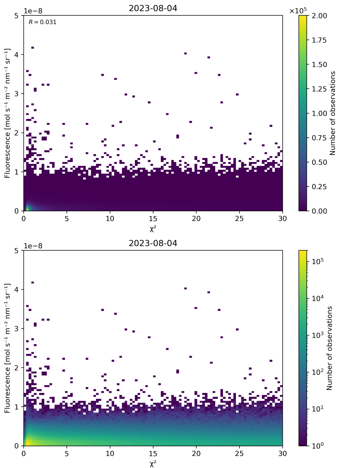
Figure 70: Scatter density plot of “ \chi^2 ” against “Fluorescence” for 2023-08-04 to 2023-08-05.
