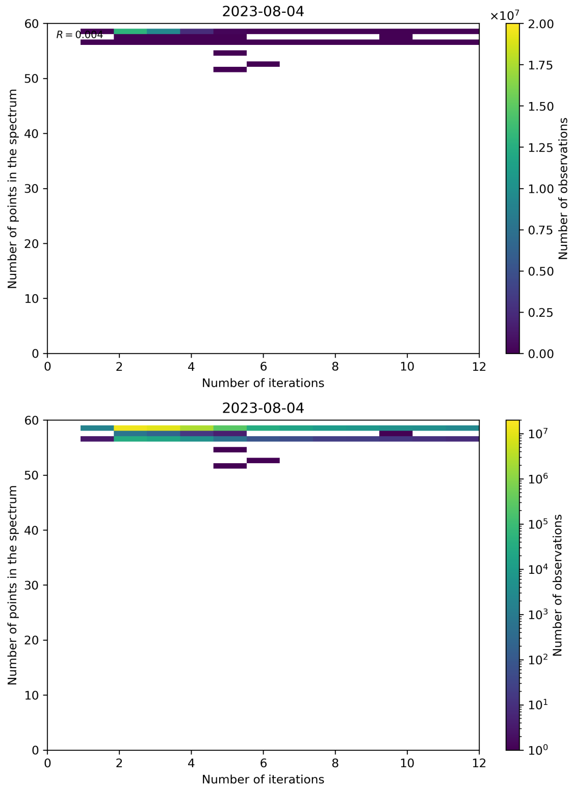
Figure 108: Scatter density plot of “Number of iterations” against “Number of points in the spectrum” for 2023-08-04 to 2023-08-05.
