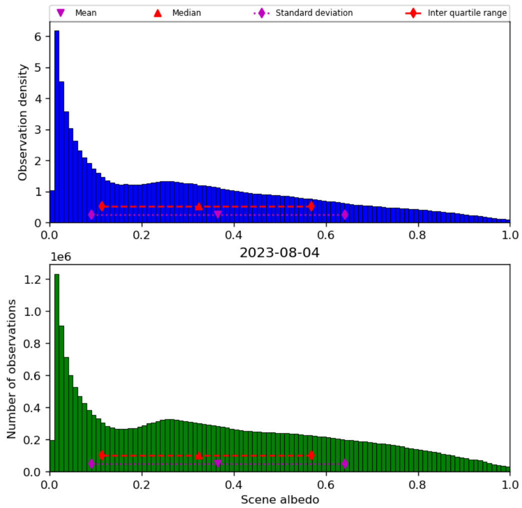
Figure 34: Histogram of “Scene albedo” for 2023-08-04 to 2023-08-05
