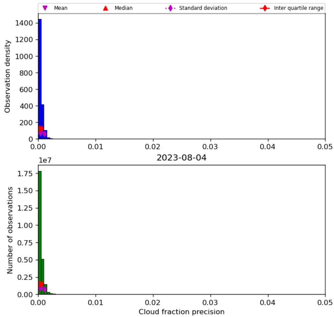
Figure 33: Histogram of “Cloud fraction precision” for 2023-08-04 to 2023-08-05
