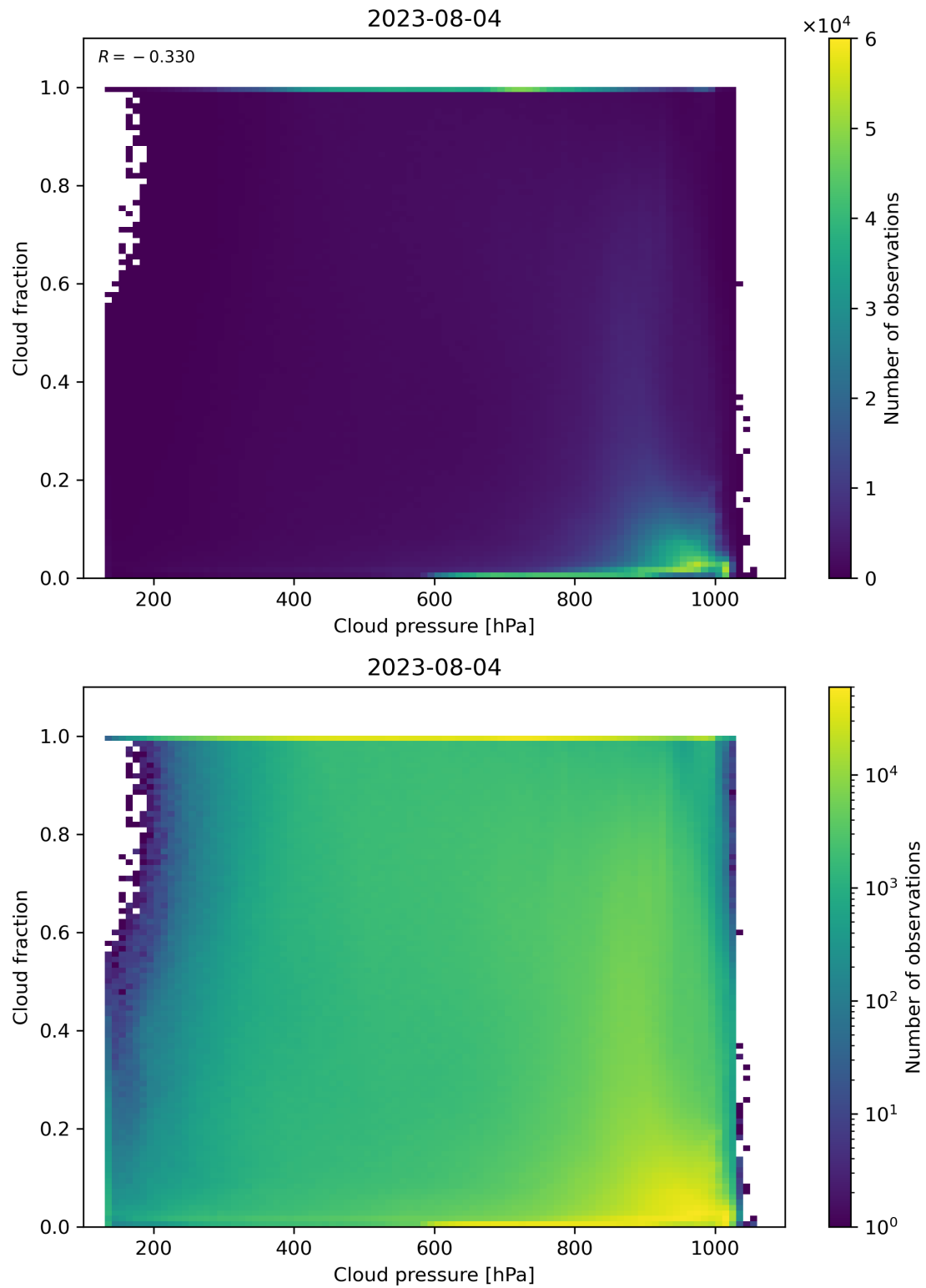
Figure 87: Scatter density plot of “Cloud pressure” against “Cloud fraction” for 2023-08-04 to 2023-08-05.
