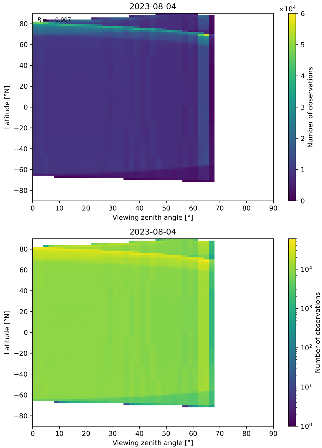
Figure 135: Scatter density plot of “Viewing zenith angle” against “Latitude” for 2023-08-04 to 2023-08-05.
