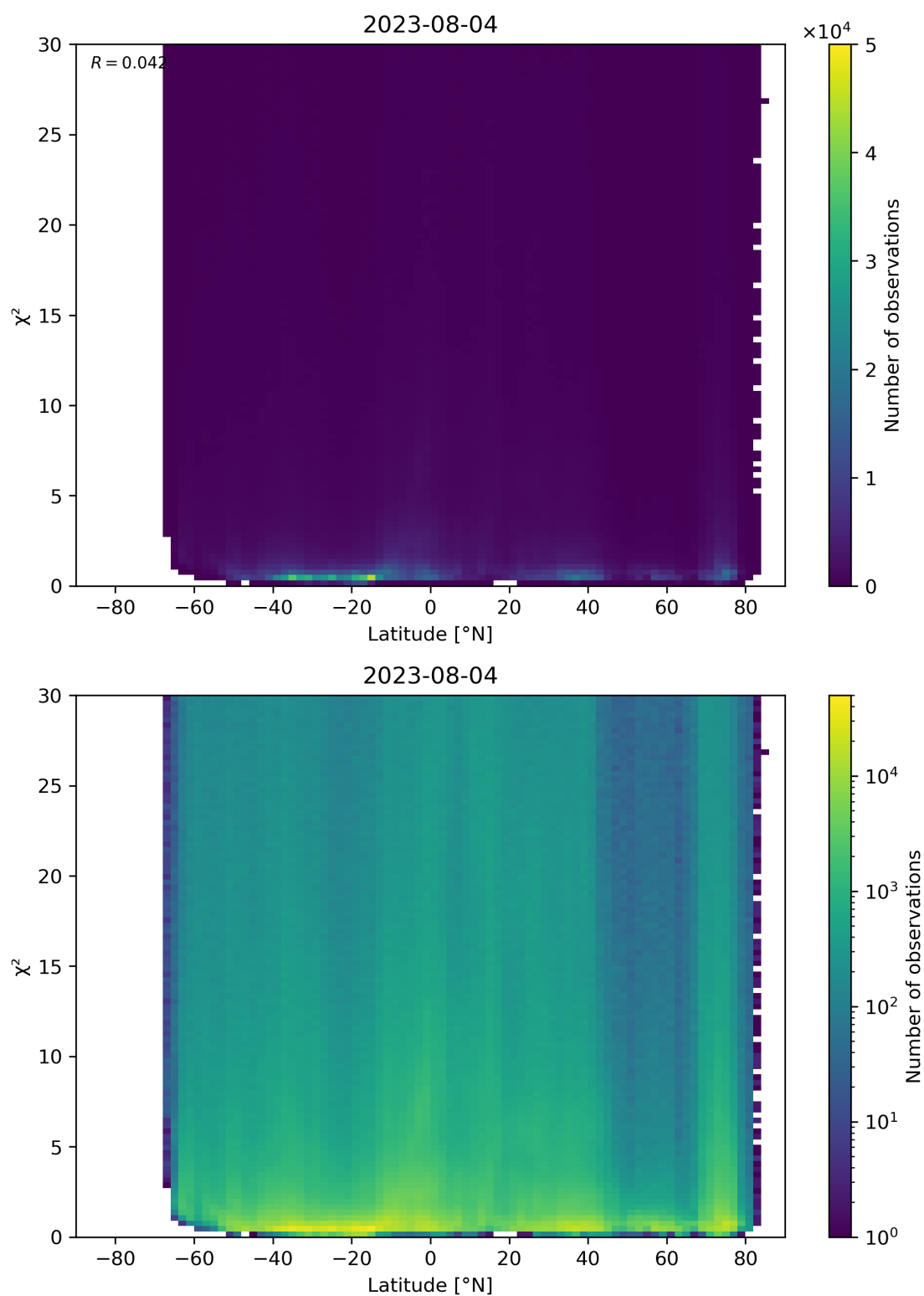
Figure 97: Scatter density plot of “Latitude” against “ \chi^2 ” for 2023-08-04 to 2023-08-05.
