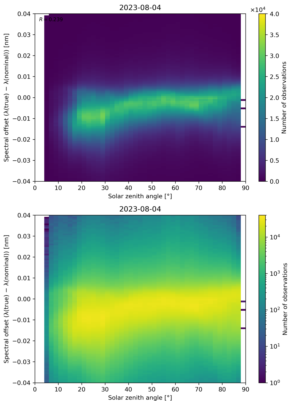
Figure 128: Scatter density plot of “Solar zenith angle” against “Spectral offset ( \lambda(\text{true}) - \lambda(\text{nominal}) )” for 2023-08-04 to 2023-08-05.
