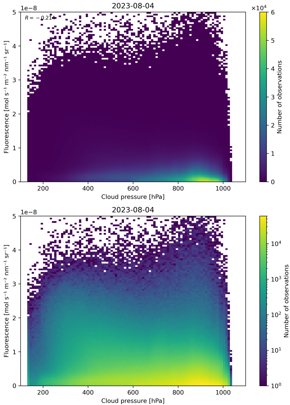
Figure 88: Scatter density plot of “Cloud pressure” against “Fluorescence” for 2023-08-04 to 2023-08-05.
