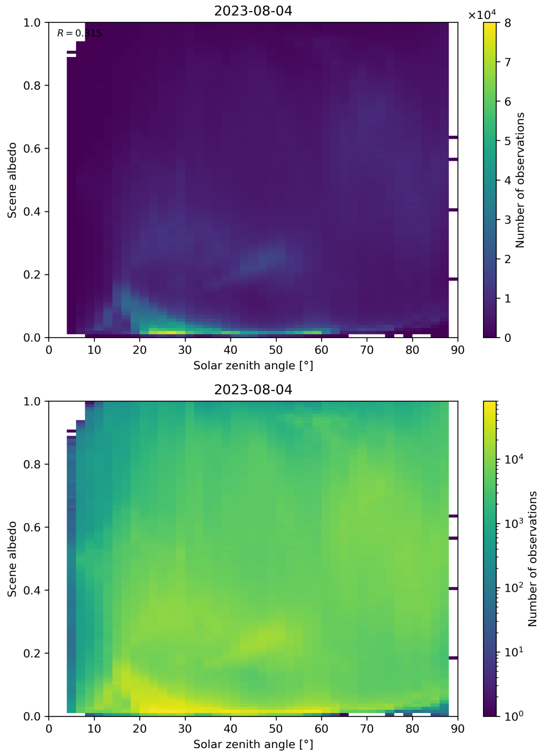
Figure 127: Scatter density plot of “Solar zenith angle” against “Scene albedo” for 2023-08-04 to 2023-08-05.
