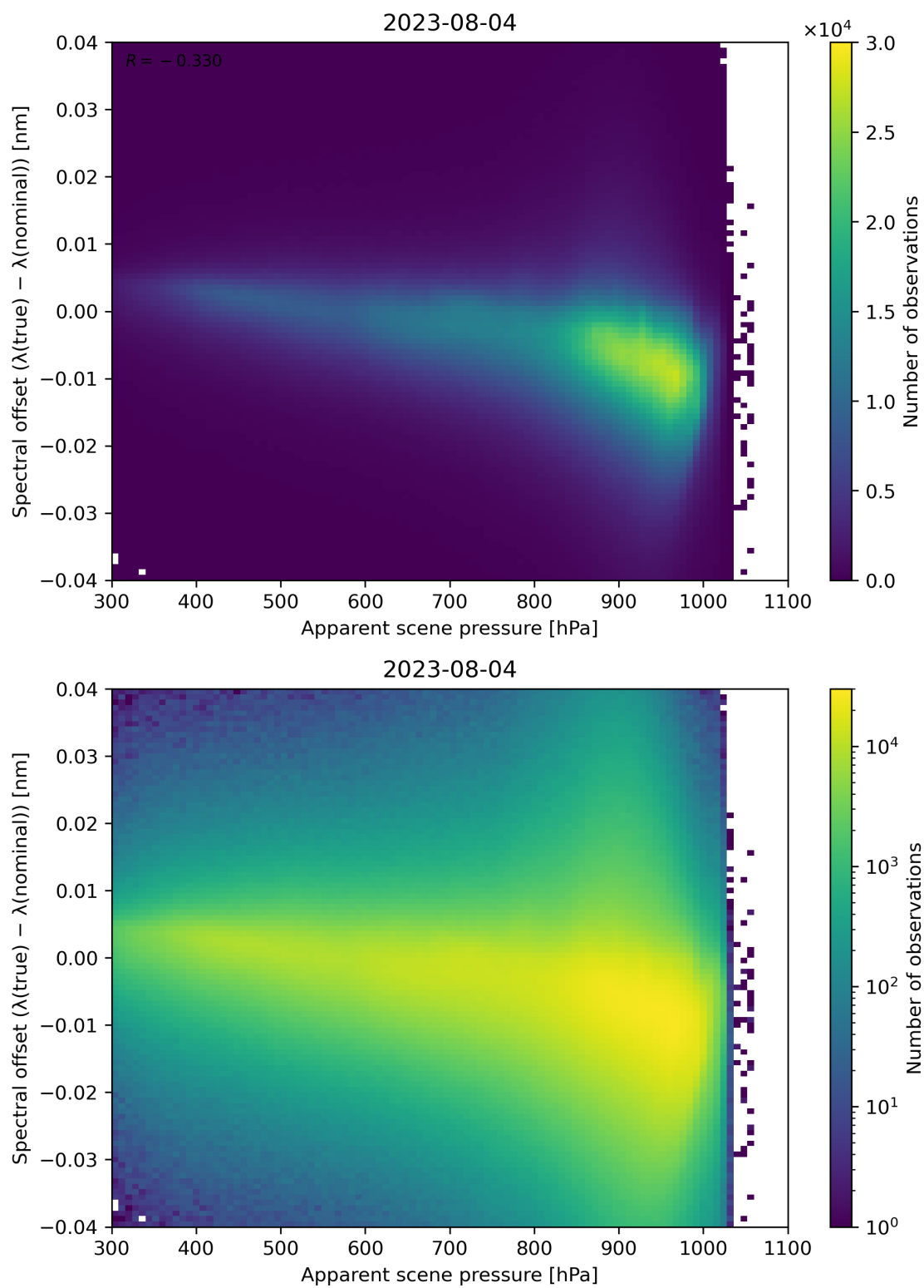
Figure 68: Scatter density plot of “Apparent scene pressure” against “Spectral offset ( \lambda(\text{true}) - \lambda(\text{nominal}) )” for 2023-08-04 to 2023-08-05.
