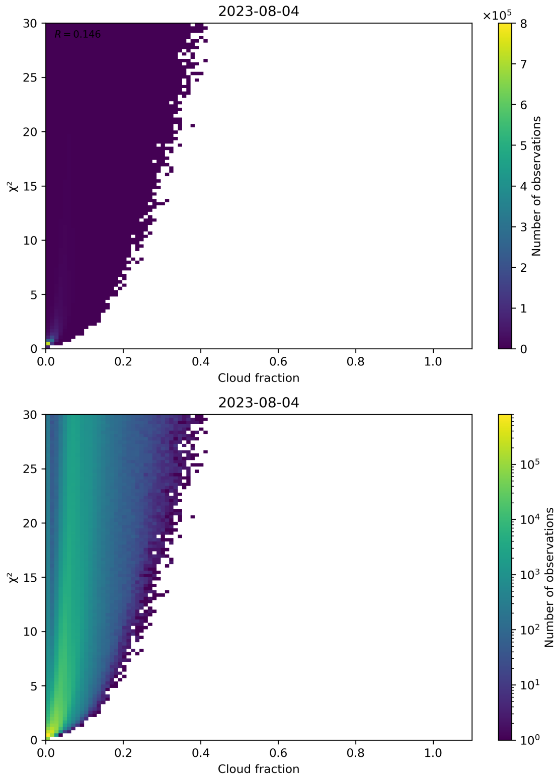
Figure 77: Scatter density plot of “Cloud fraction” against “ \chi^2 ” for 2023-08-04 to 2023-08-05.
