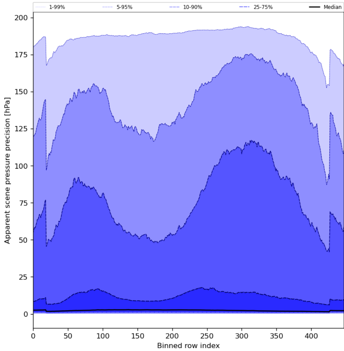
Figure 54: Along track statistics of “Apparent scene pressure precision” for 2023-08-04 to 2023-08-05
