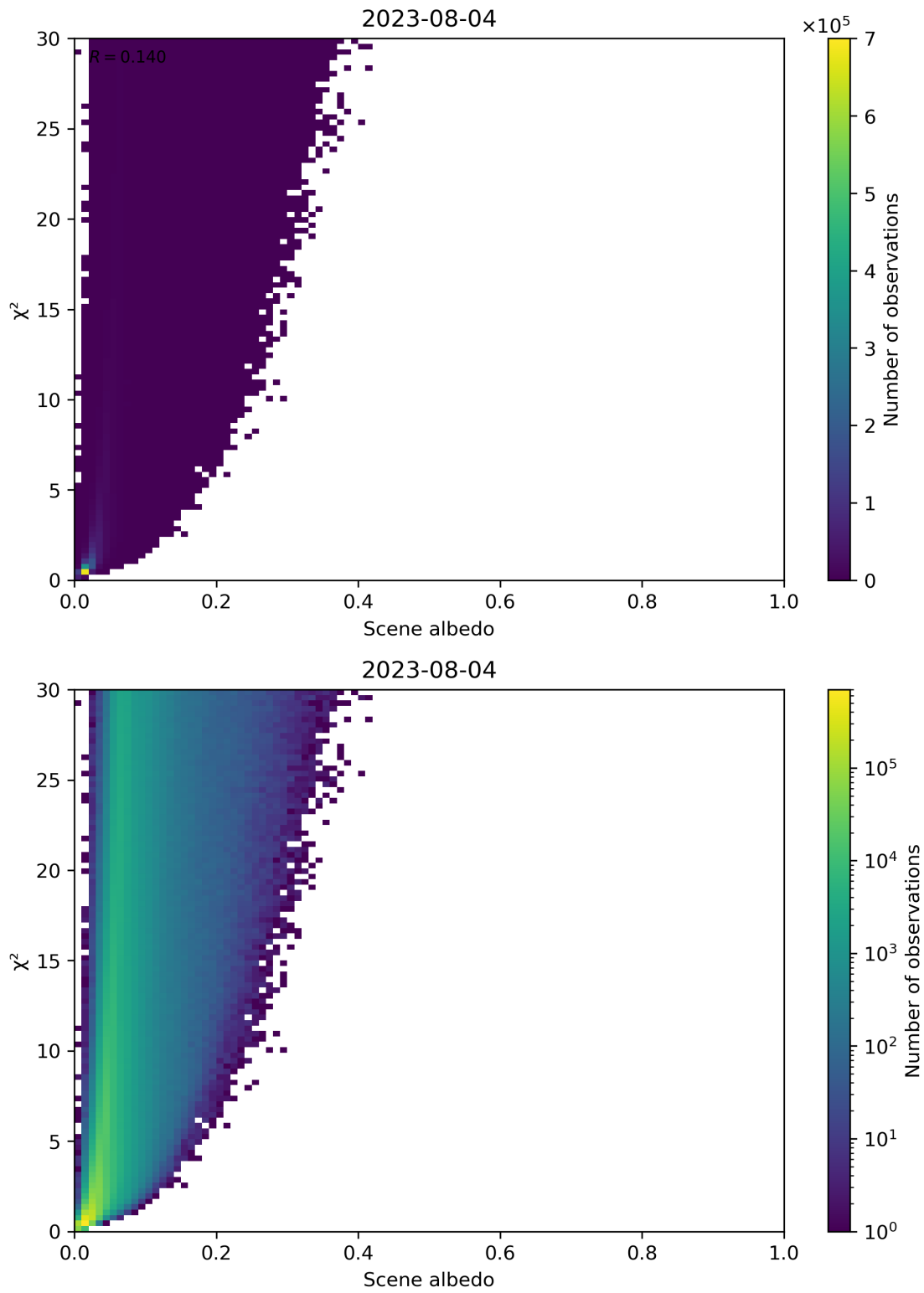
Figure 112: Scatter density plot of “Scene albedo” against “ \chi^2 ” for 2023-08-04 to 2023-08-05.
