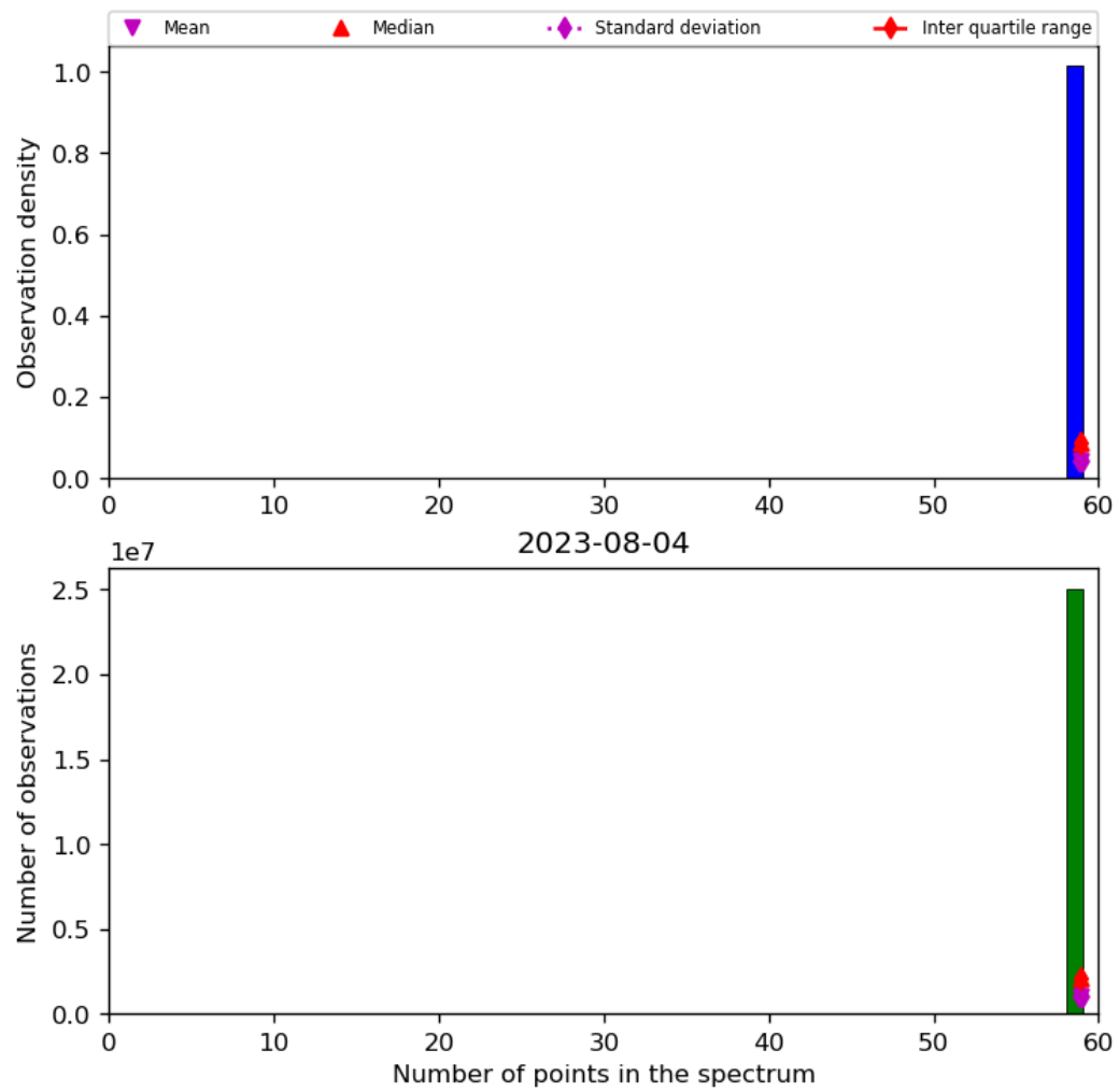
Figure 44: Histogram of “Number of points in the spectrum” for 2023-08-04 to 2023-08-05
