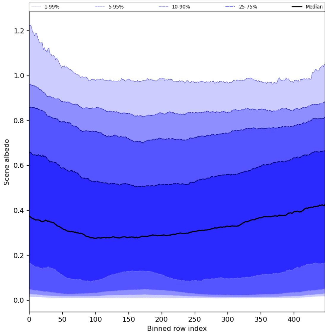
Figure 51: Along track statistics of “Scene albedo” for 2023-08-04 to 2023-08-05
