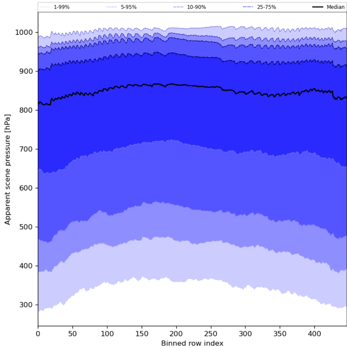
Figure 53: Along track statistics of “Apparent scene pressure” for 2023-08-04 to 2023-08-05
