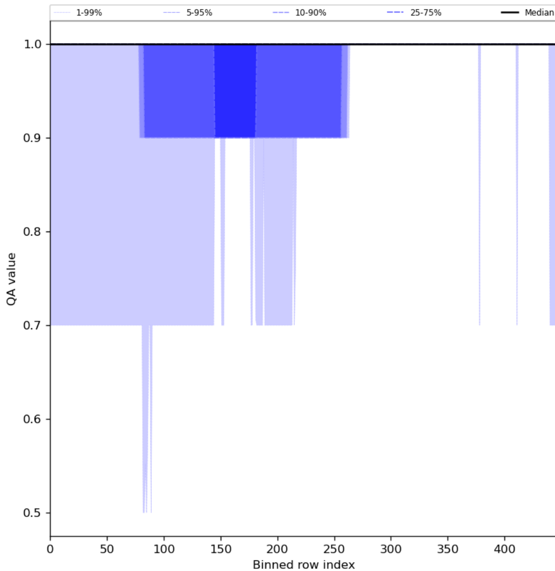
Figure 46: Along track statistics of “QA value” for 2023-08-04 to 2023-08-05
