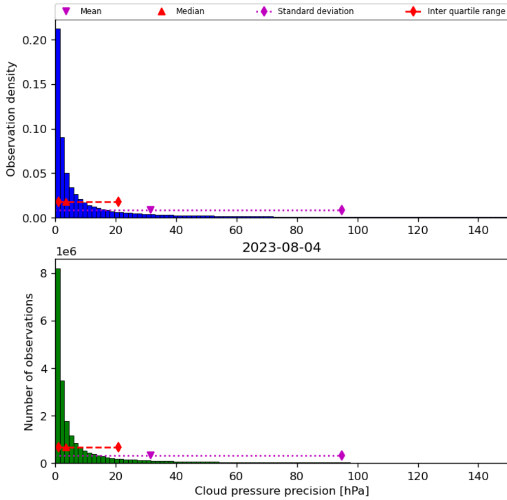
Figure 31: Histogram of “Cloud pressure precision” for 2023-08-04 to 2023-08-05
