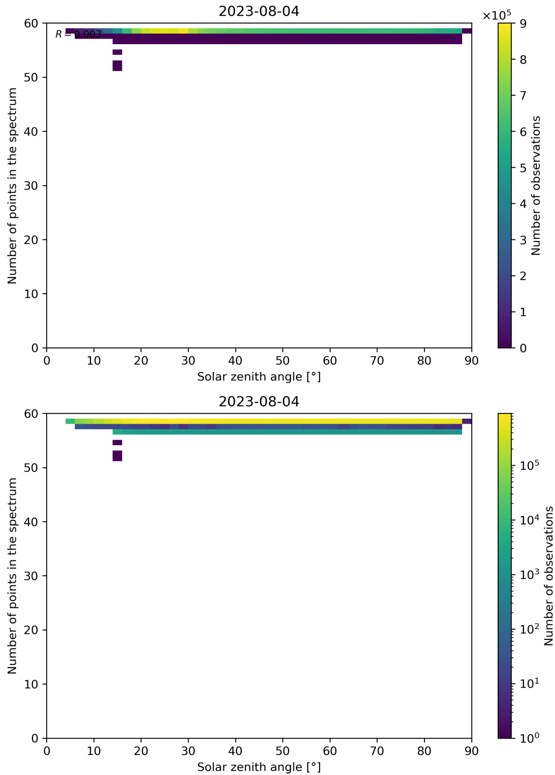
Figure 126: Scatter density plot of “Solar zenith angle” against “Number of points in the spectrum” for 2023-08-04 to 2023-08-05.
