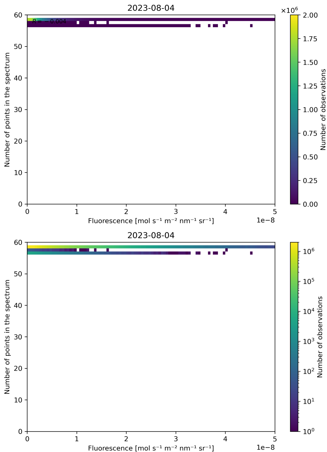
Figure 94: Scatter density plot of “Fluorescence” against “Number of points in the spectrum” for 2023-08-04 to 2023-08-05.
