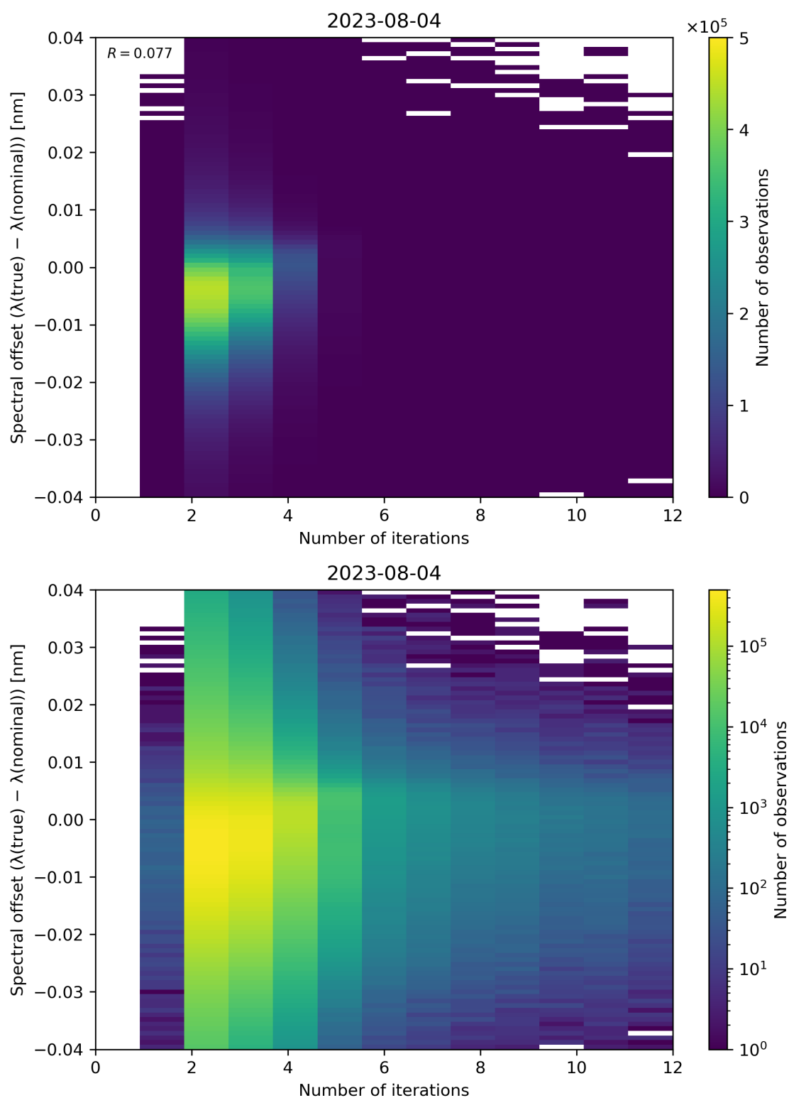
Figure 109: Scatter density plot of “Number of iterations” against “Spectral offset ( \lambda(\text{true}) - \lambda(\text{nominal}) )” for 2023-08-04 to 2023-08-05.
