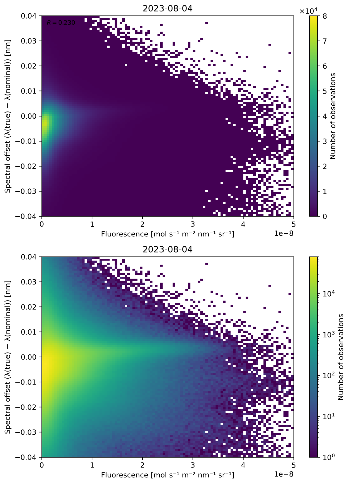
Figure 95: Scatter density plot of “Fluorescence” against “Spectral offset ( \lambda(\text{true}) - \lambda(\text{nominal}) )” for 2023-08-04 to 2023-08-05.
