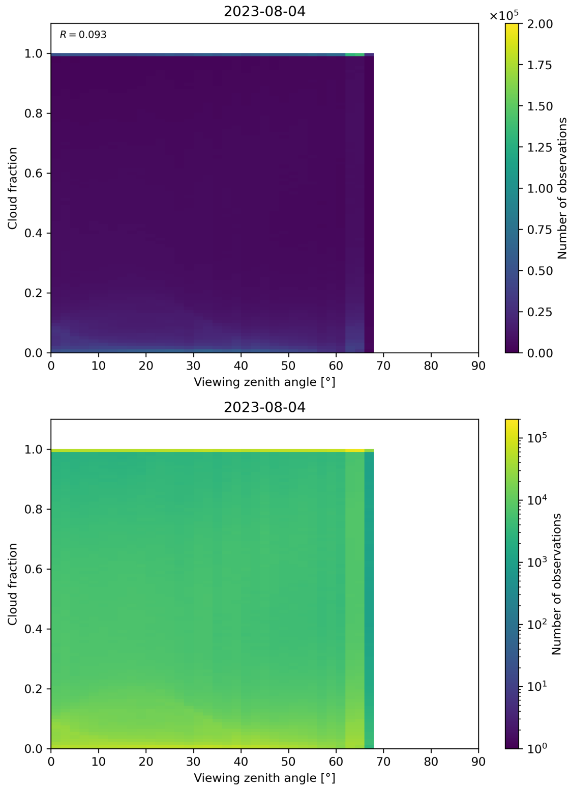
Figure 132: Scatter density plot of “Viewing zenith angle” against “Cloud fraction” for 2023-08-04 to 2023-08-05.
