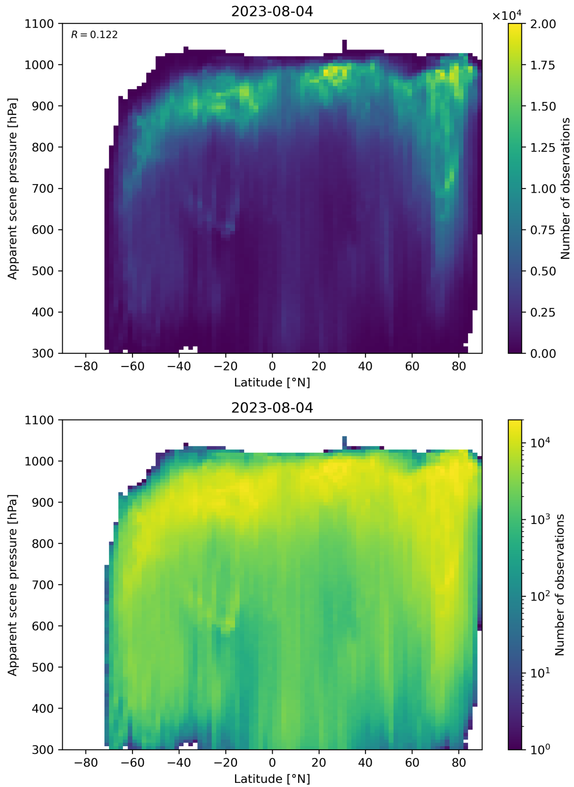
Figure 96: Scatter density plot of “Latitude” against “Apparent scene pressure” for 2023-08-04 to 2023-08-05.
