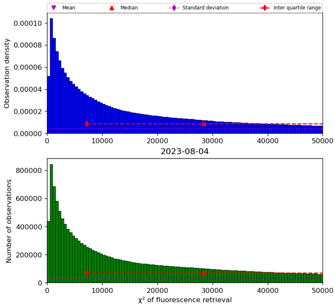
Figure 42: Histogram of “ \chi^2 of fluorescence retrieval” for 2023-08-04 to 2023-08-05
