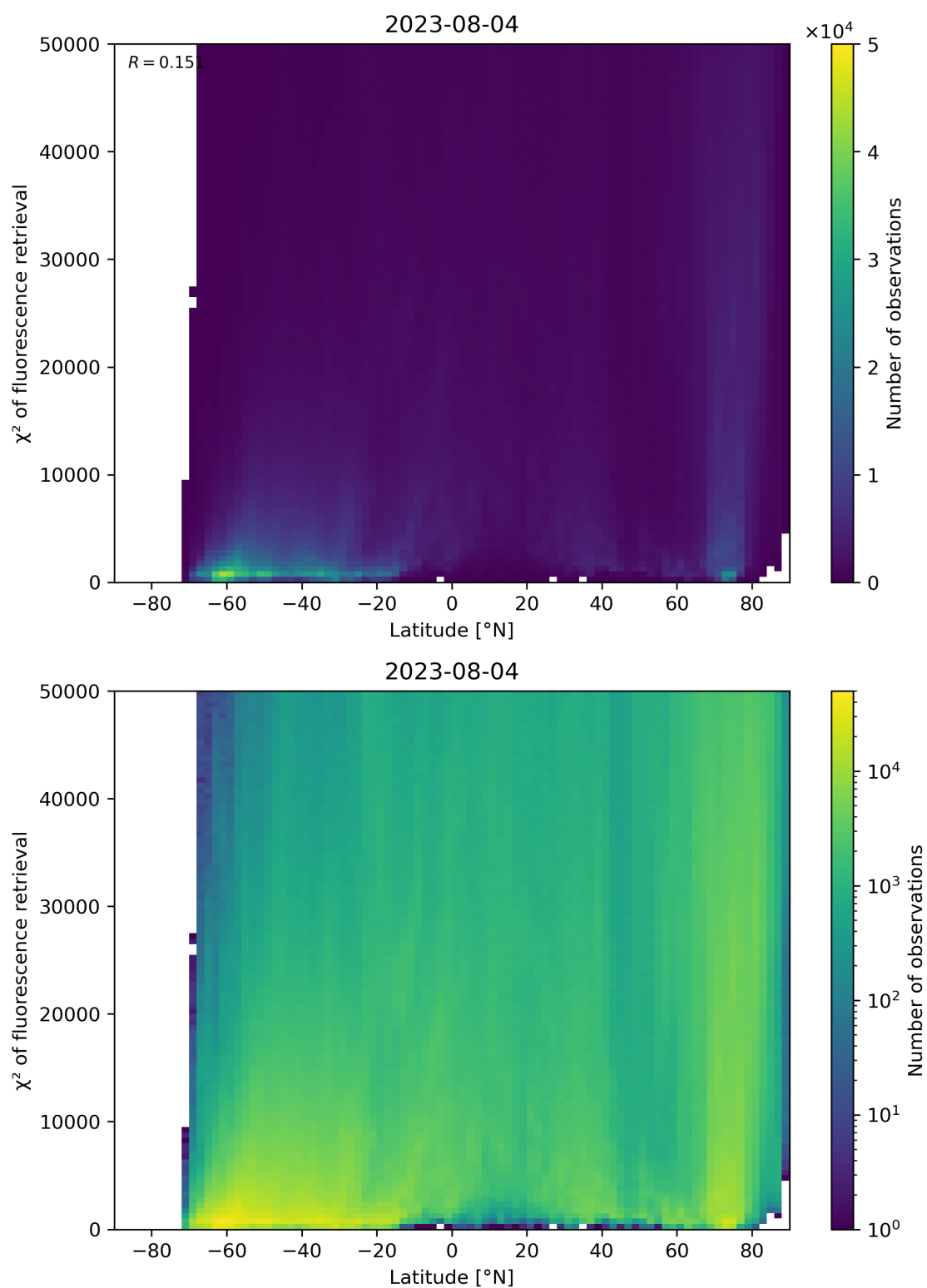
Figure 98: Scatter density plot of “Latitude” against “ \chi^2 of fluorescence retrieval” for 2023-08-04 to 2023-08-05.
