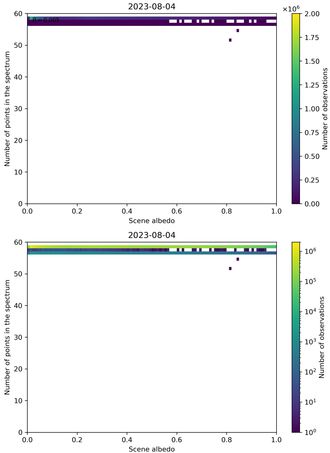
Figure 116: Scatter density plot of “Scene albedo” against “Number of points in the spectrum” for 2023-08-04 to 2023-08-05.
