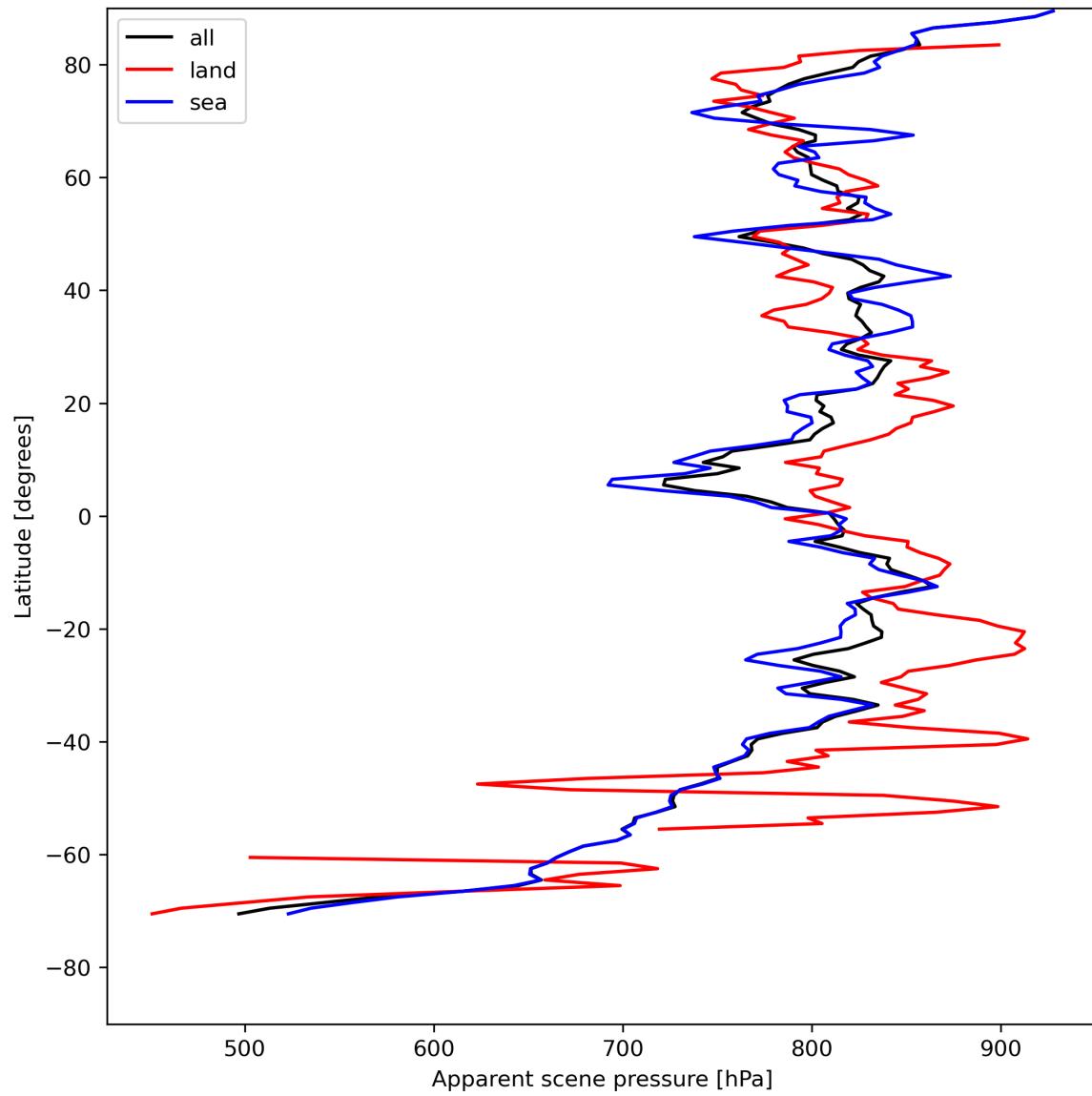
Figure 19: Zonal average of “Apparent scene pressure” for 2023-08-04 to 2023-08-05.
