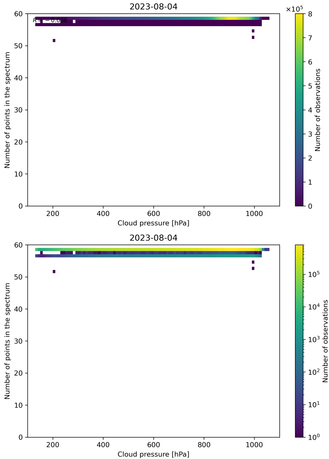
Figure 90: Scatter density plot of “Cloud pressure” against “Number of points in the spectrum” for 2023-08-04 to 2023-08-05.
