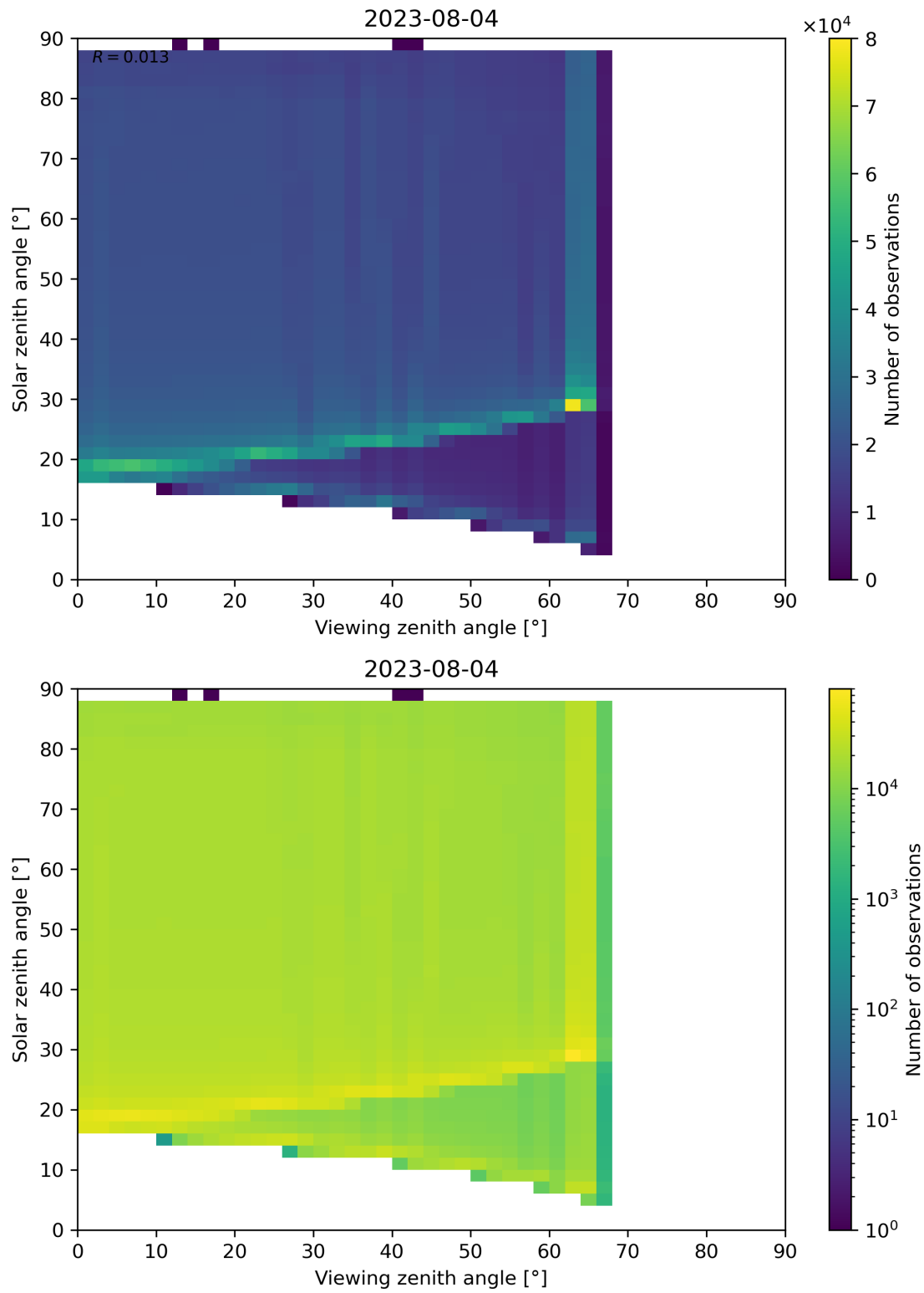
Figure 139: Scatter density plot of “Viewing zenith angle” against “Solar zenith angle” for 2023-08-04 to 2023-08-05.
