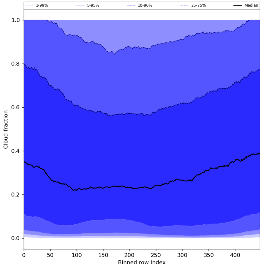
Figure 49: Along track statistics of “Cloud fraction” for 2023-08-04 to 2023-08-05
