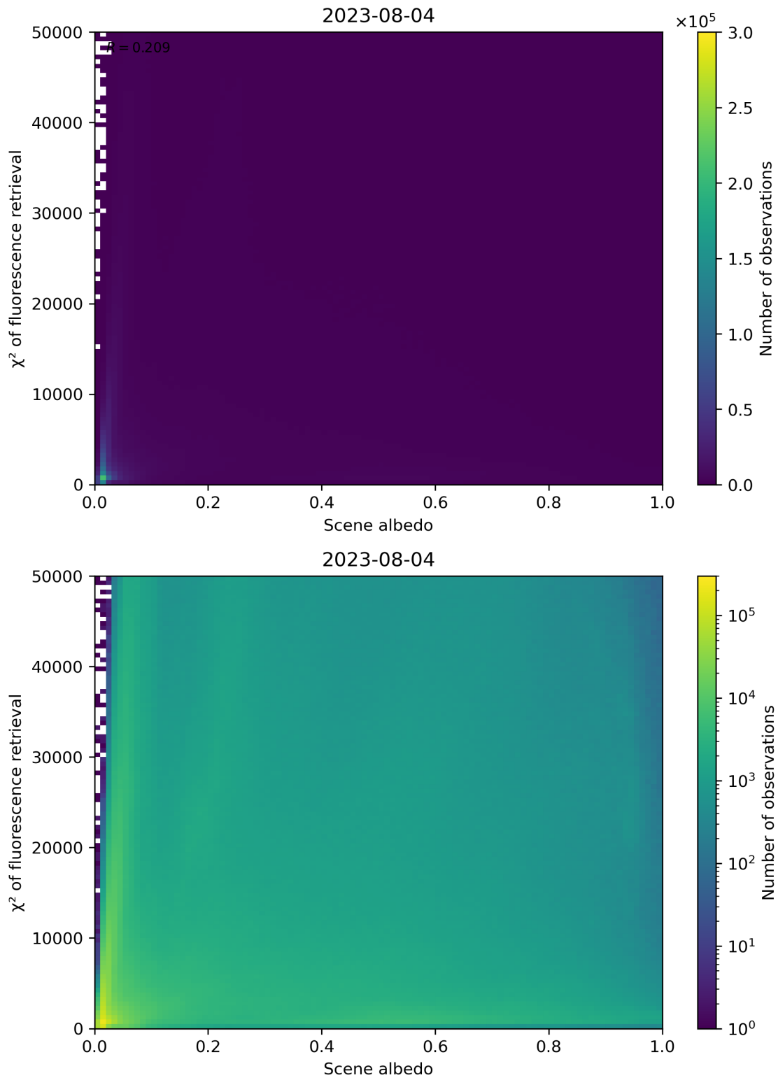
Figure 113: Scatter density plot of “Scene albedo” against “ \chi^2 of fluorescence retrieval” for 2023-08-04 to 2023-08-05.
