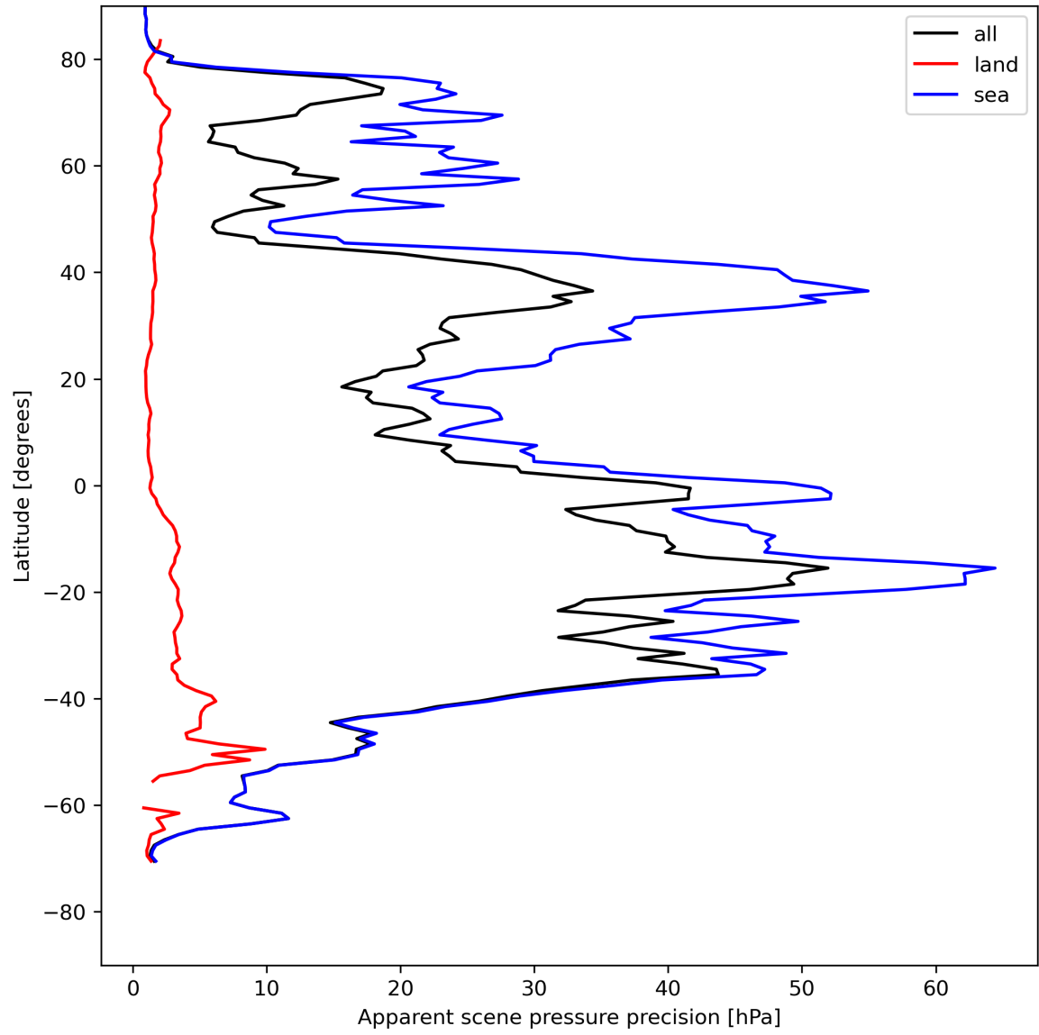
Figure 20: Zonal average of “Apparent scene pressure precision” for 2023-08-04 to 2023-08-05.
