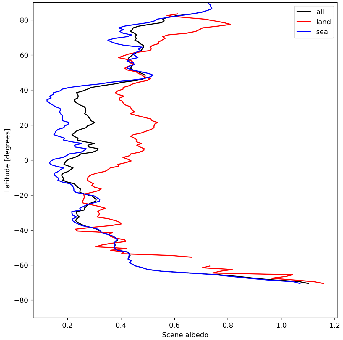
Figure 17: Zonal average of “Scene albedo” for 2023-08-04 to 2023-08-05.
