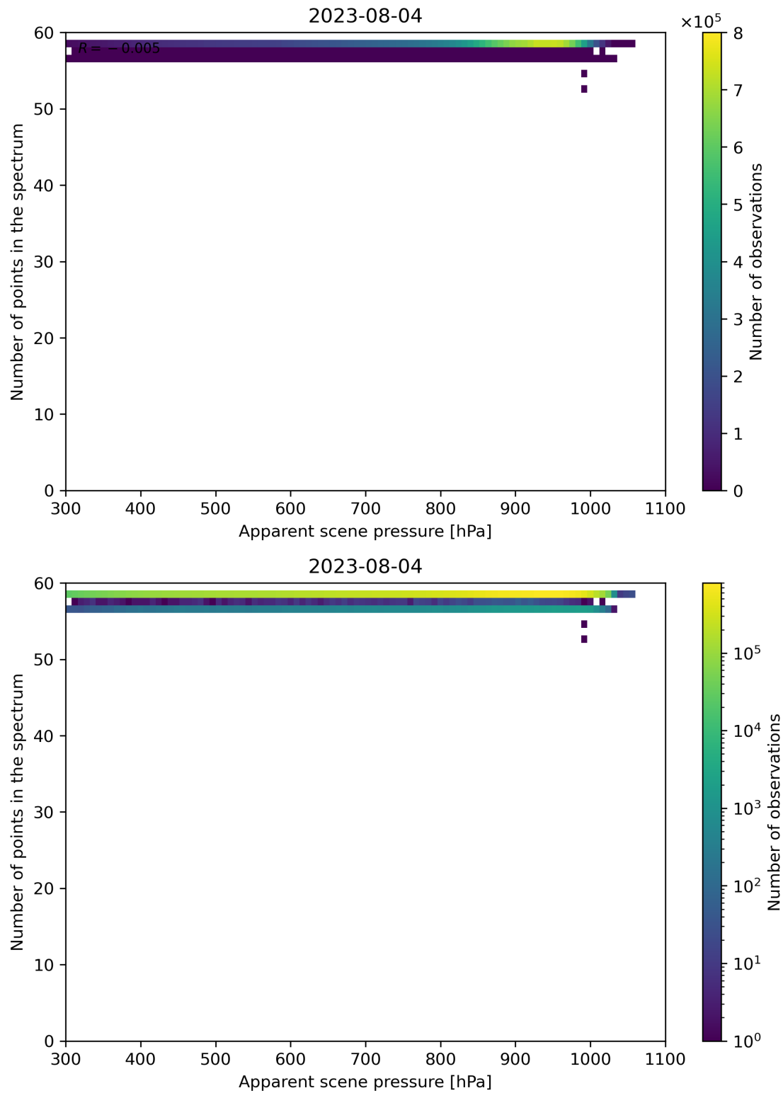
Figure 67: Scatter density plot of “Apparent scene pressure” against “Number of points in the spectrum” for 2023-08-04 to 2023-08-05.
