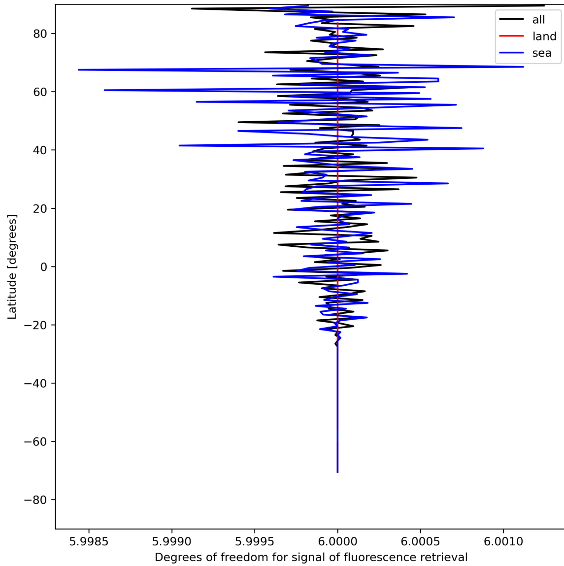
Figure 26: Zonal average of “Degrees of freedom for signal of fluorescence retrieval” for 2023-08-04 to 2023-08-05.
