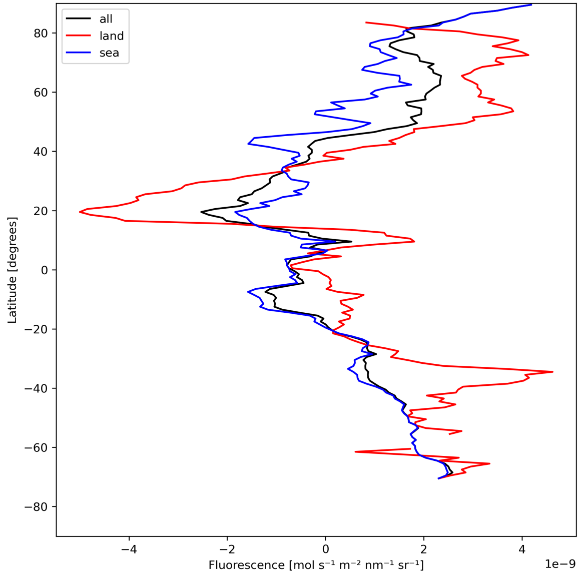
Figure 23: Zonal average of “Fluorescence” for 2023-08-04 to 2023-08-05.
