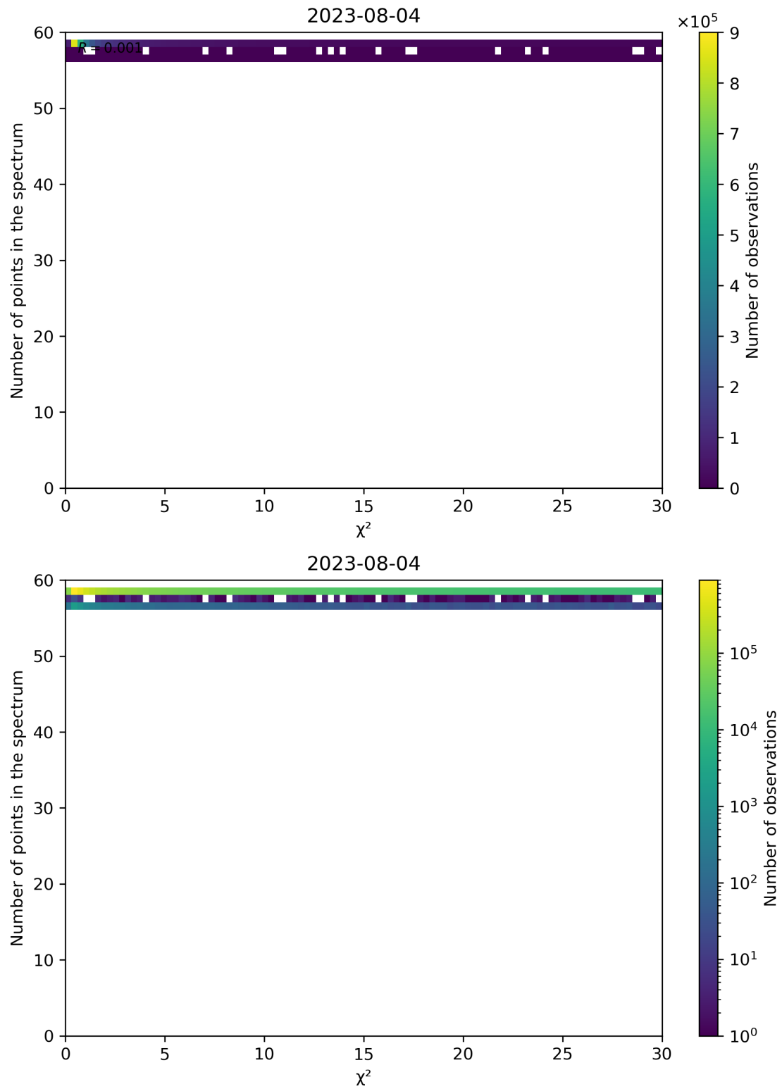
Figure 74: Scatter density plot of " \chi^2 " against "Number of points in the spectrum" for 2023-08-04 to 2023-08-05.
