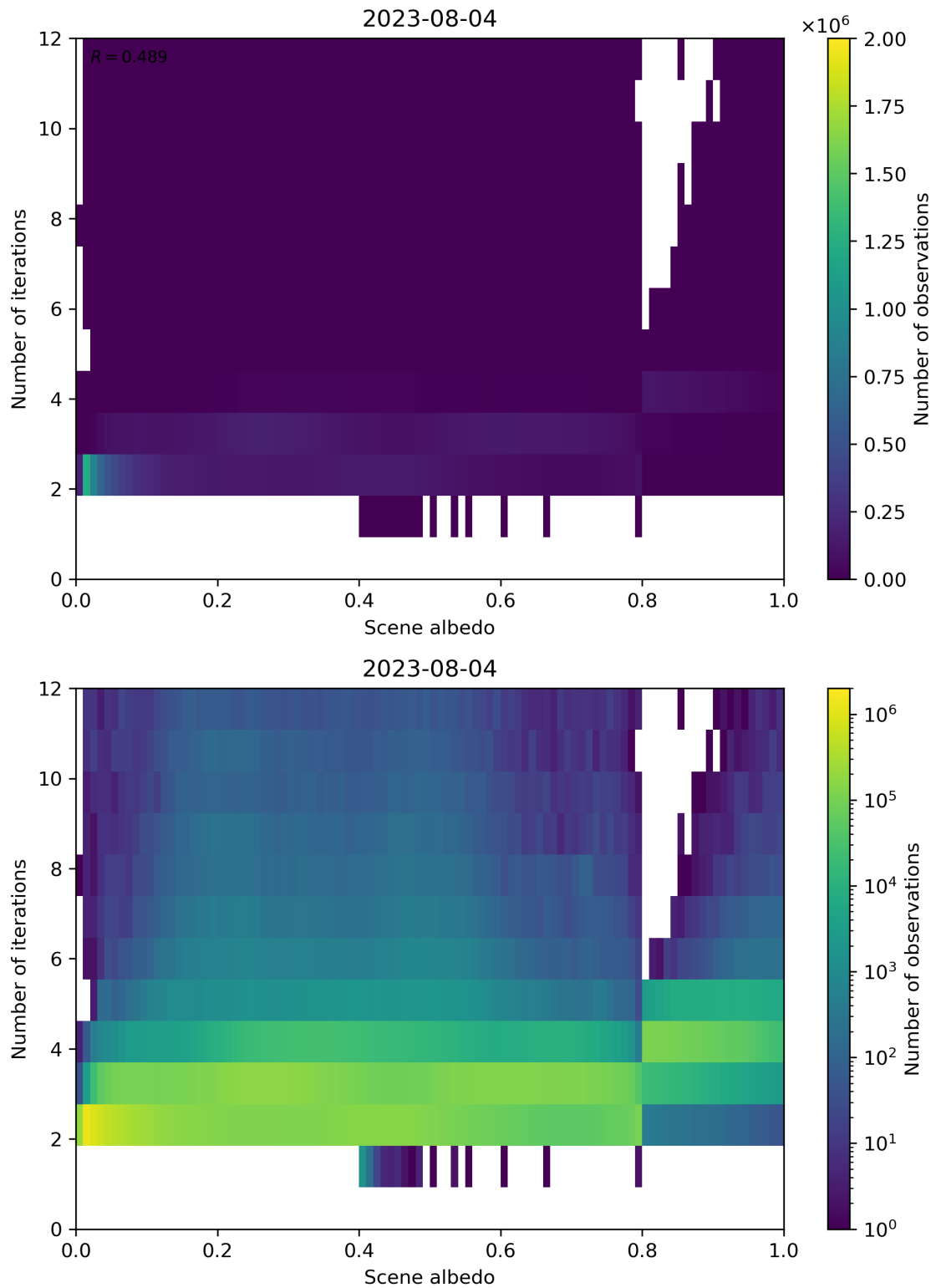
Figure 115: Scatter density plot of “Scene albedo” against “Number of iterations” for 2023-08-04 to 2023-08-05.
