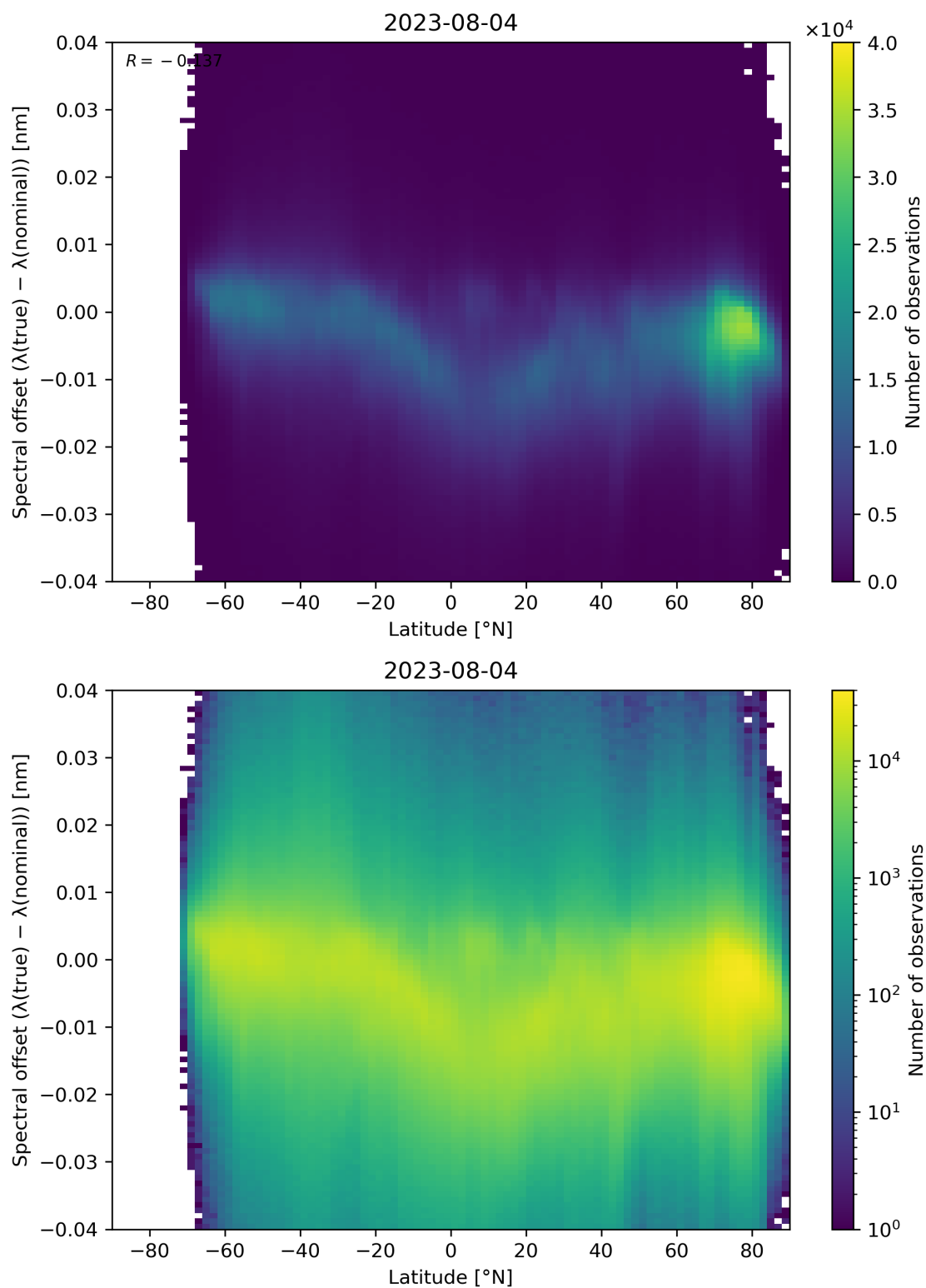
Figure 105: Scatter density plot of “Latitude” against “Spectral offset ( \lambda(\text{true}) - \lambda(\text{nominal}) )” for 2023-08-04 to 2023-08-05.
