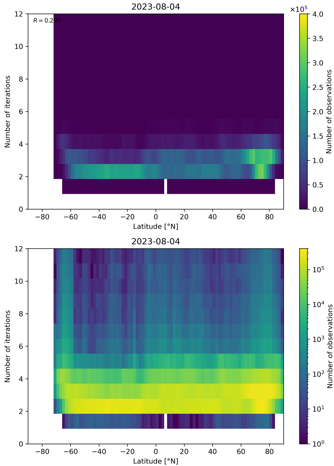
Figure 102: Scatter density plot of “Latitude” against “Number of iterations” for 2023-08-04 to 2023-08-05.
