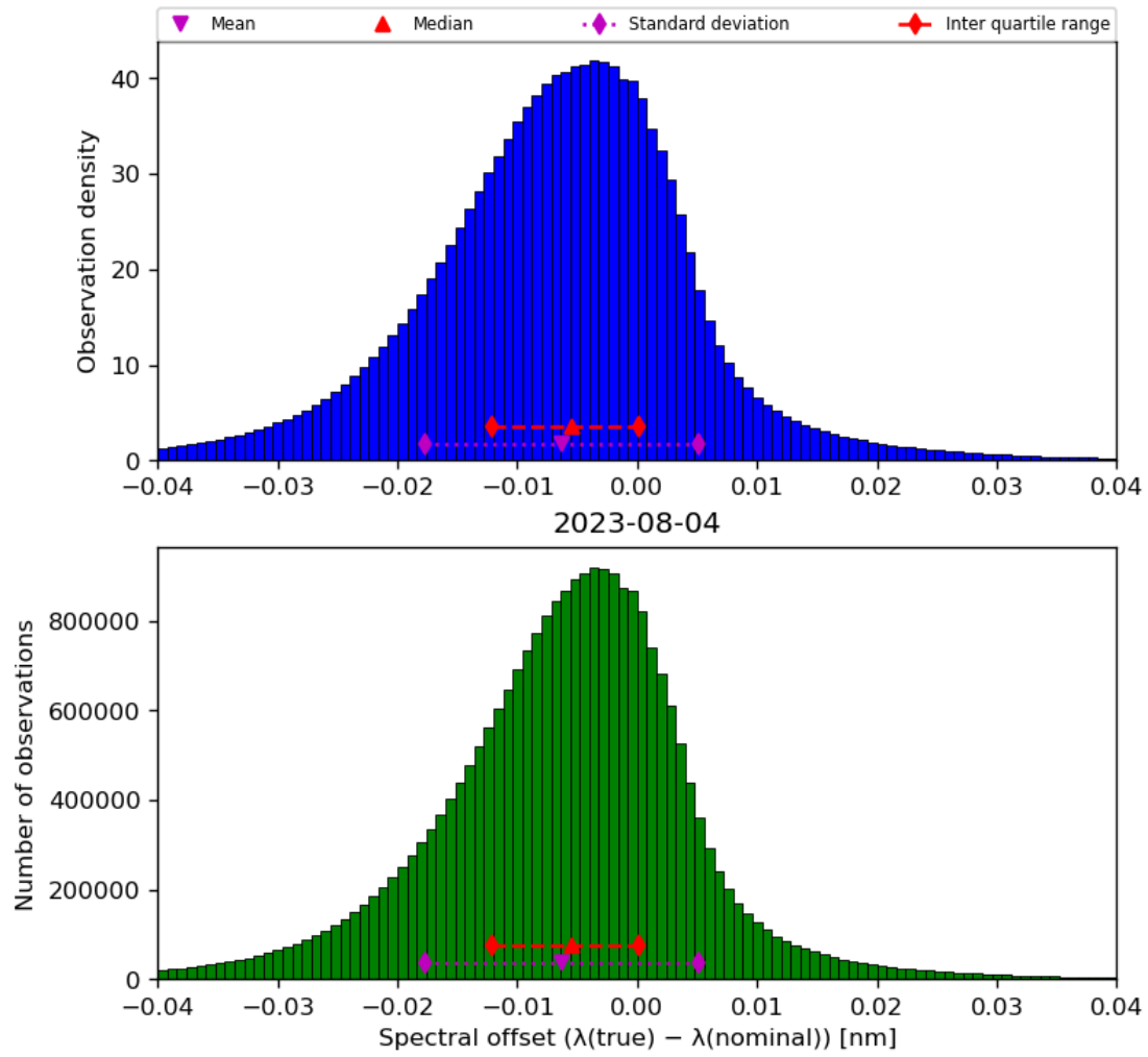
Figure 45: Histogram of “Spectral offset ( \lambda(\text{true}) - \lambda(\text{nominal}) )” for 2023-08-04 to 2023-08-05
