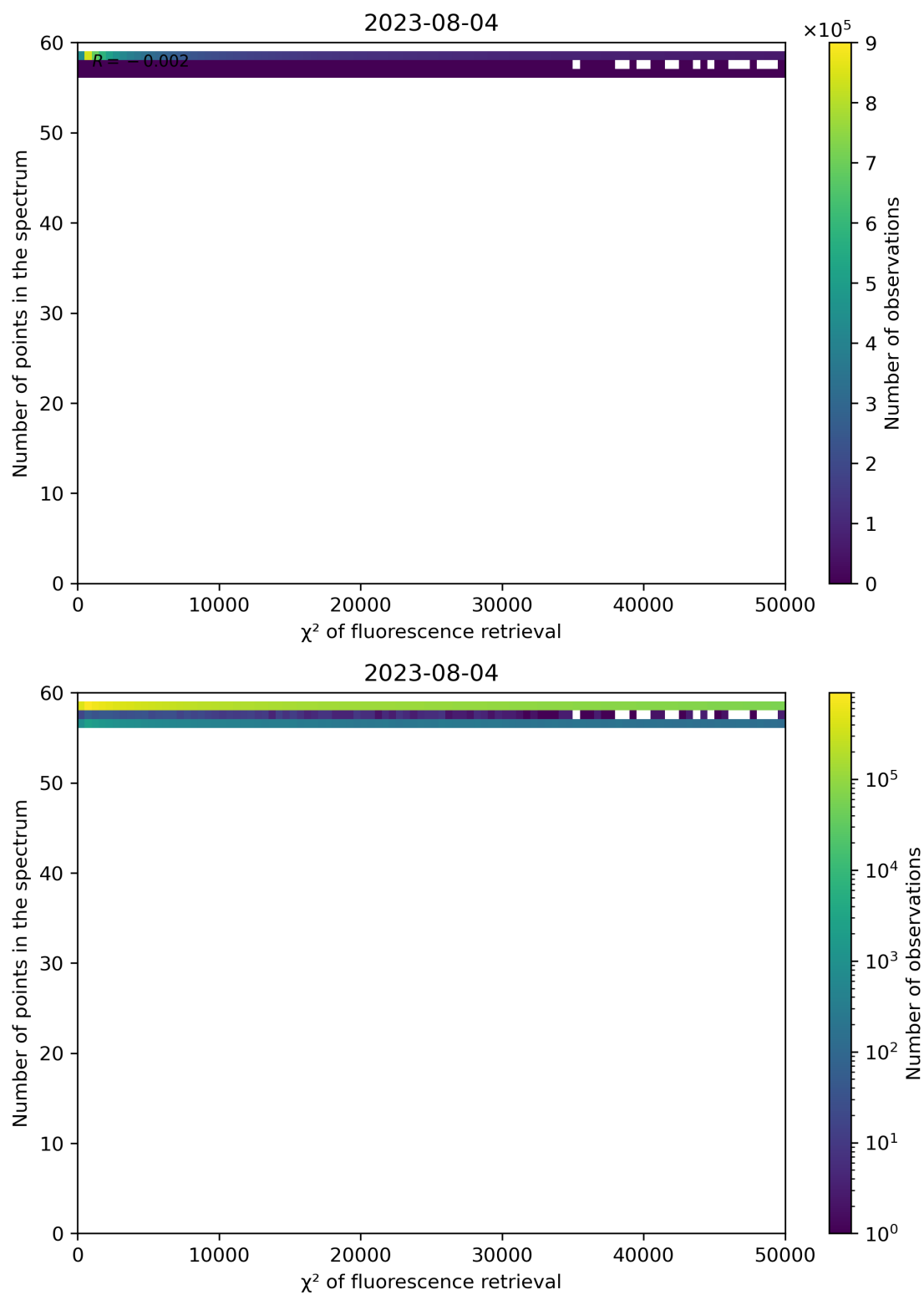
Figure 71: Scatter density plot of " \chi^2 of fluorescence retrieval" against "Number of points in the spectrum" for 2023-08-04 to 2023-08-05.
