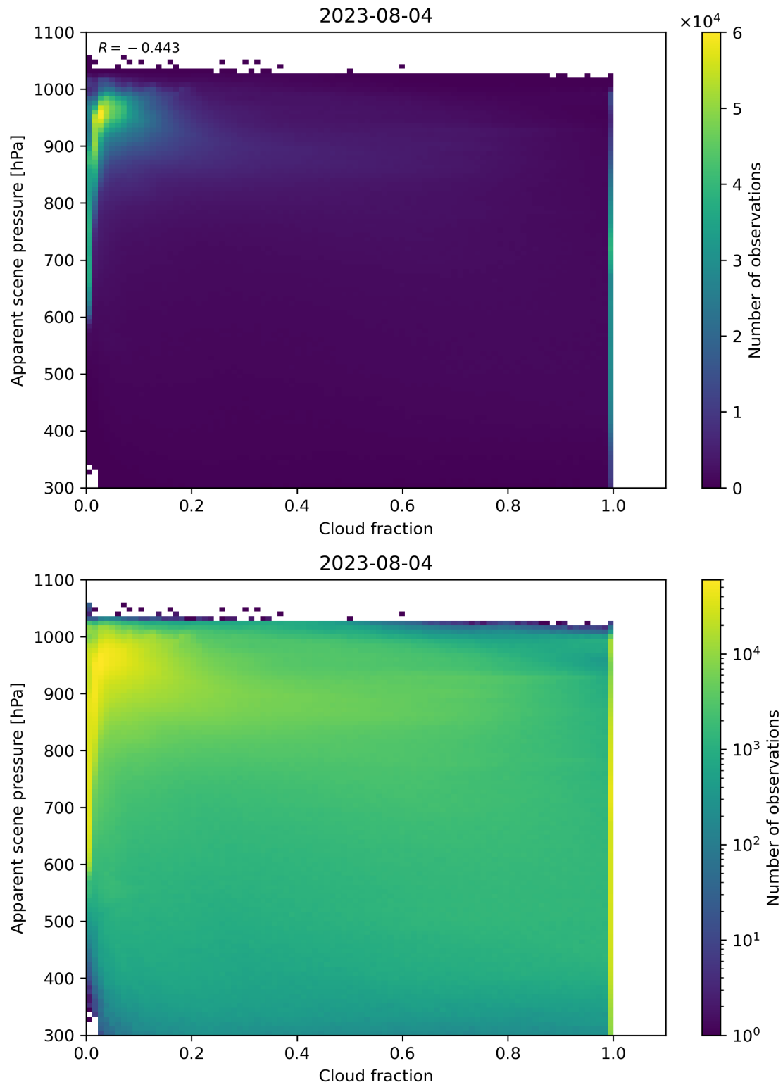
Figure 76: Scatter density plot of “Cloud fraction” against “Apparent scene pressure” for 2023-08-04 to 2023-08-05.
