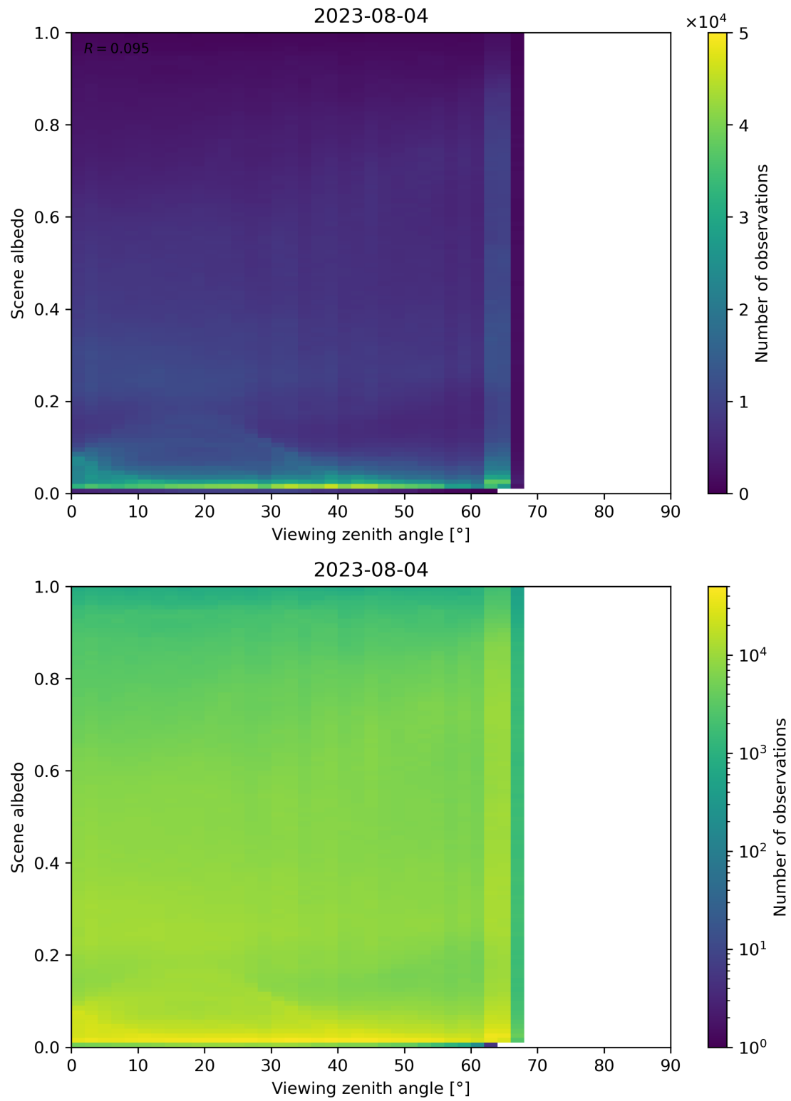
Figure 138: Scatter density plot of “Viewing zenith angle” against “Scene albedo” for 2023-08-04 to 2023-08-05.
