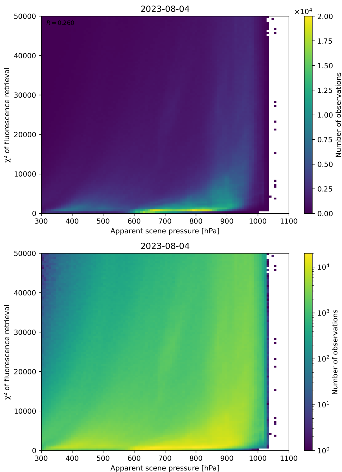
Figure 64: Scatter density plot of “Apparent scene pressure” against “ \chi^2 of fluorescence retrieval” for 2023-08-04 to 2023-08-05.
