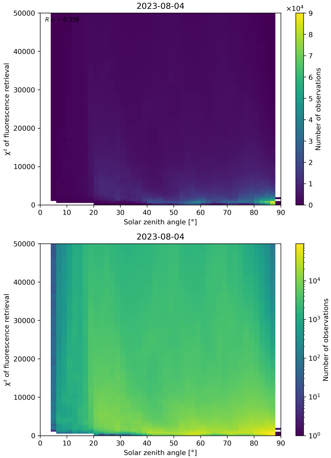
Figure 120: Scatter density plot of “Solar zenith angle” against “ \chi^2 of fluorescence retrieval” for 2023-08-04 to 2023-08-05.
