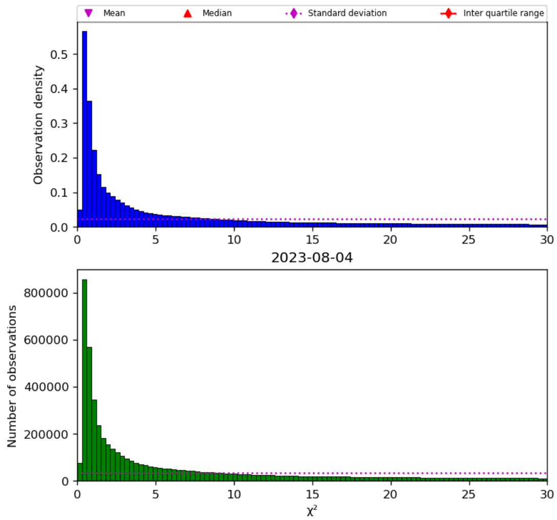
Figure 38: Histogram of “ \chi^2 ” for 2023-08-04 to 2023-08-05
