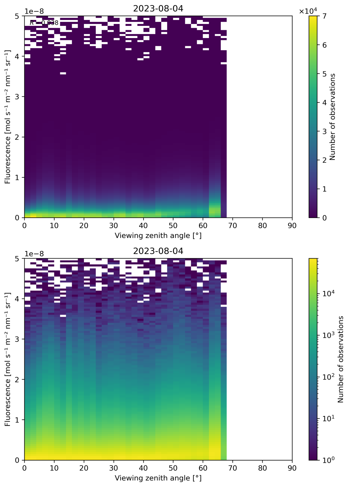
Figure 134: Scatter density plot of “Viewing zenith angle” against “Fluorescence” for 2023-08-04 to 2023-08-05.
