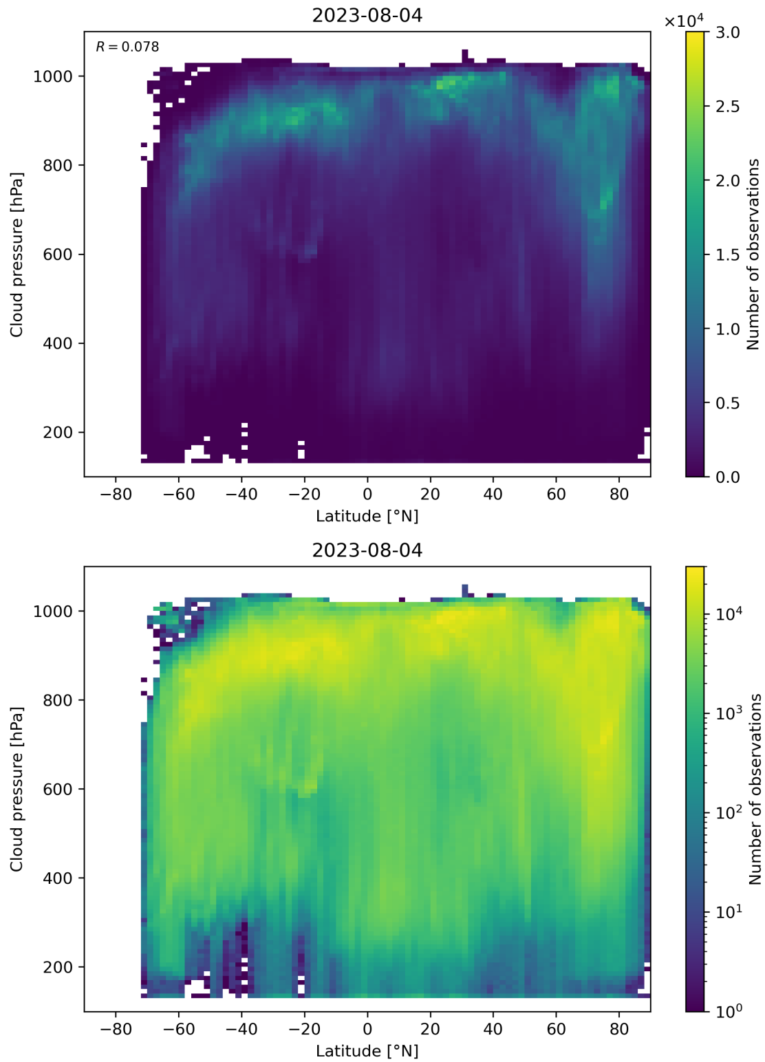
Figure 100: Scatter density plot of “Latitude” against “Cloud pressure” for 2023-08-04 to 2023-08-05.
