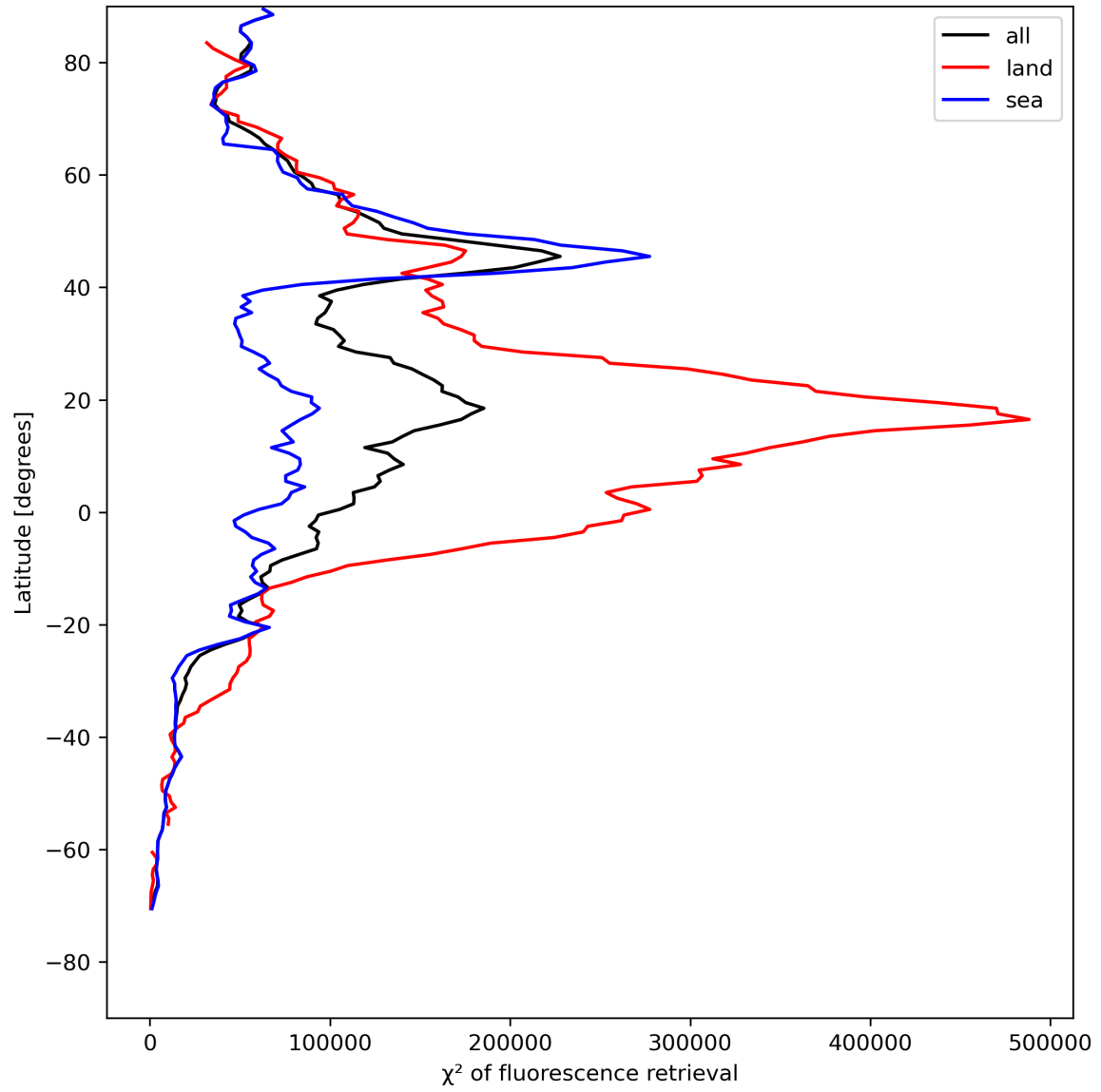
Figure 25: Zonal average of “ \chi^2 of fluorescence retrieval” for 2023-08-04 to 2023-08-05.
