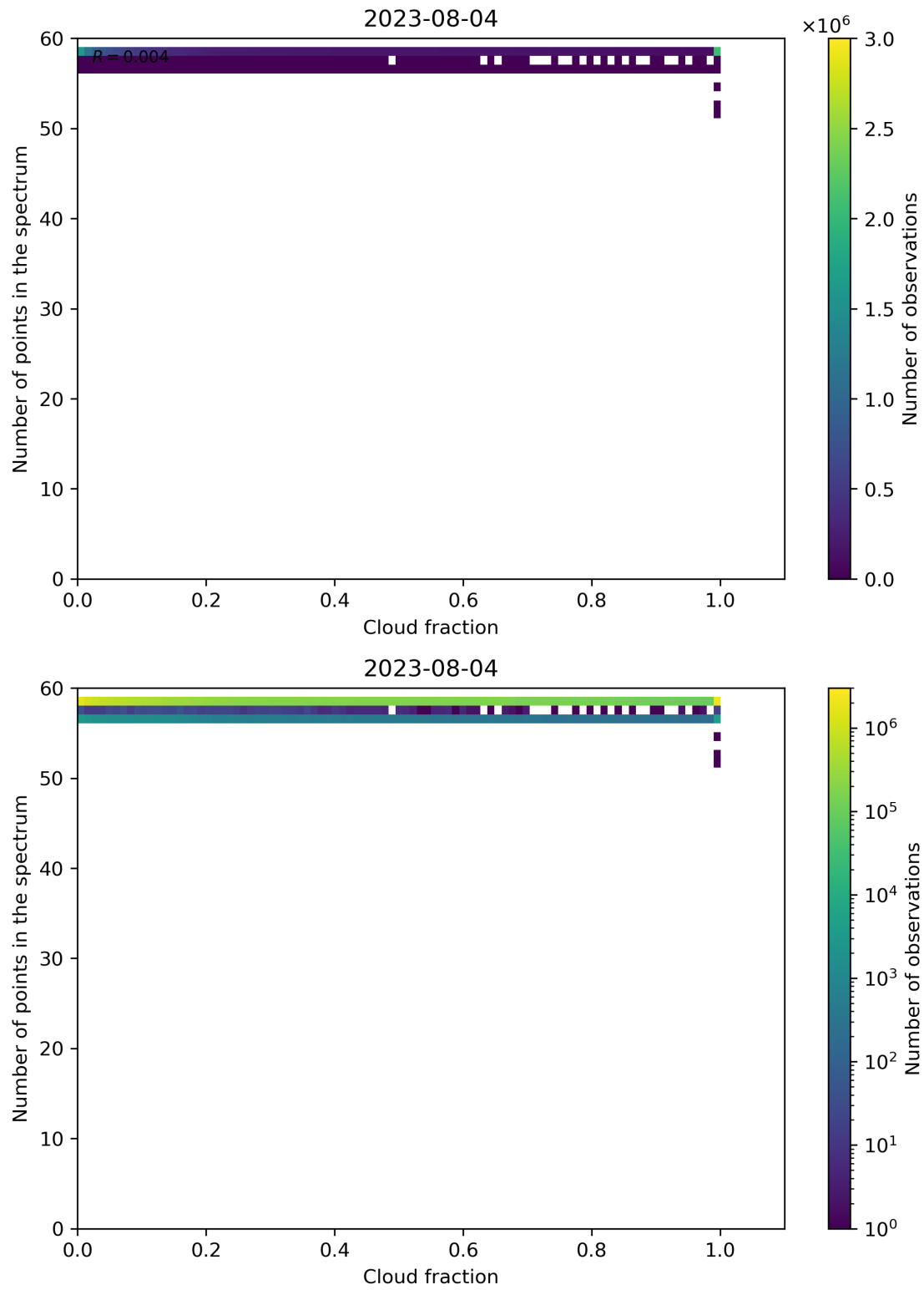
Figure 81: Scatter density plot of “Cloud fraction” against “Number of points in the spectrum” for 2023-08-04 to 2023-08-05.
