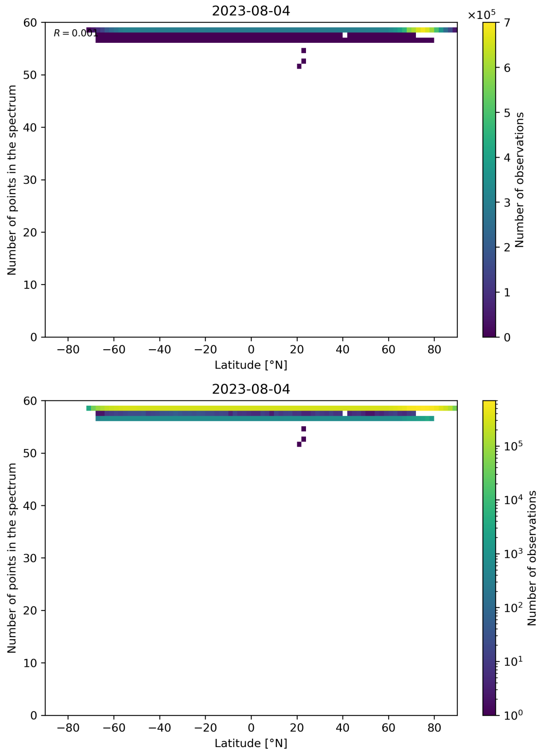
Figure 103: Scatter density plot of “Latitude” against “Number of points in the spectrum” for 2023-08-04 to 2023-08-05.
