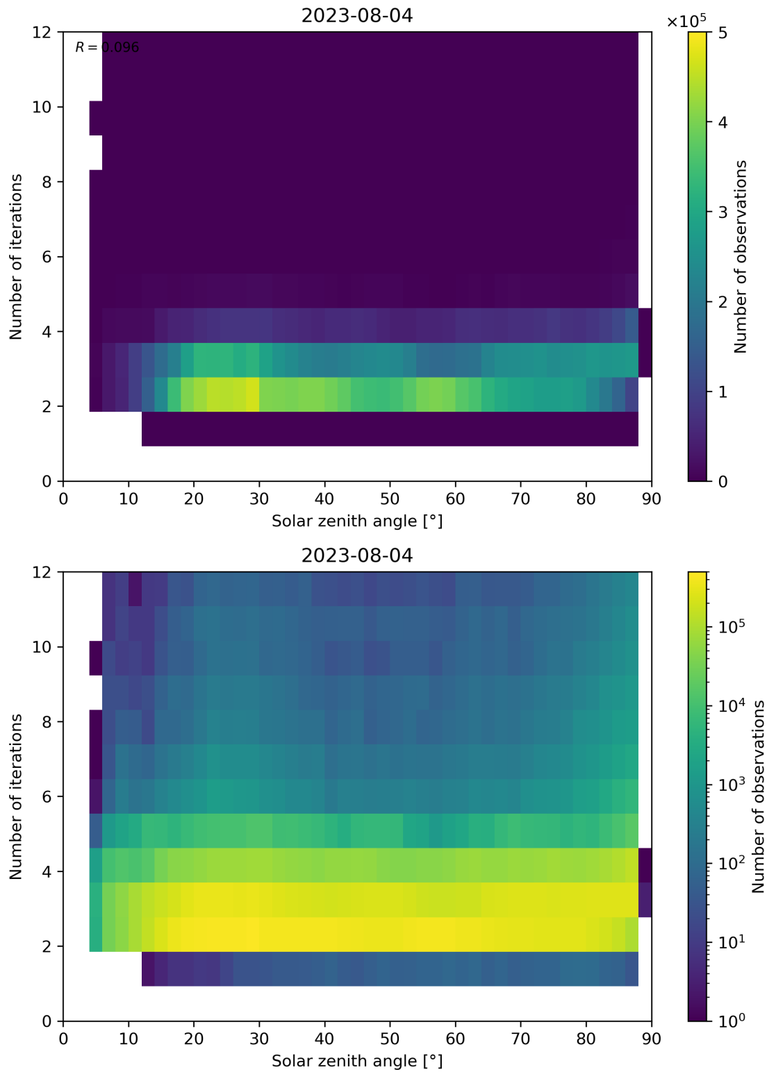
Figure 125: Scatter density plot of “Solar zenith angle” against “Number of iterations” for 2023-08-04 to 2023-08-05.
