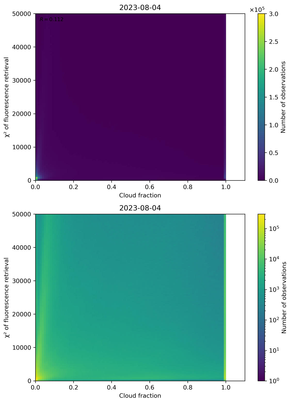
Figure 78: Scatter density plot of “Cloud fraction” against “ \chi^2 of fluorescence retrieval” for 2023-08-04 to 2023-08-05.
