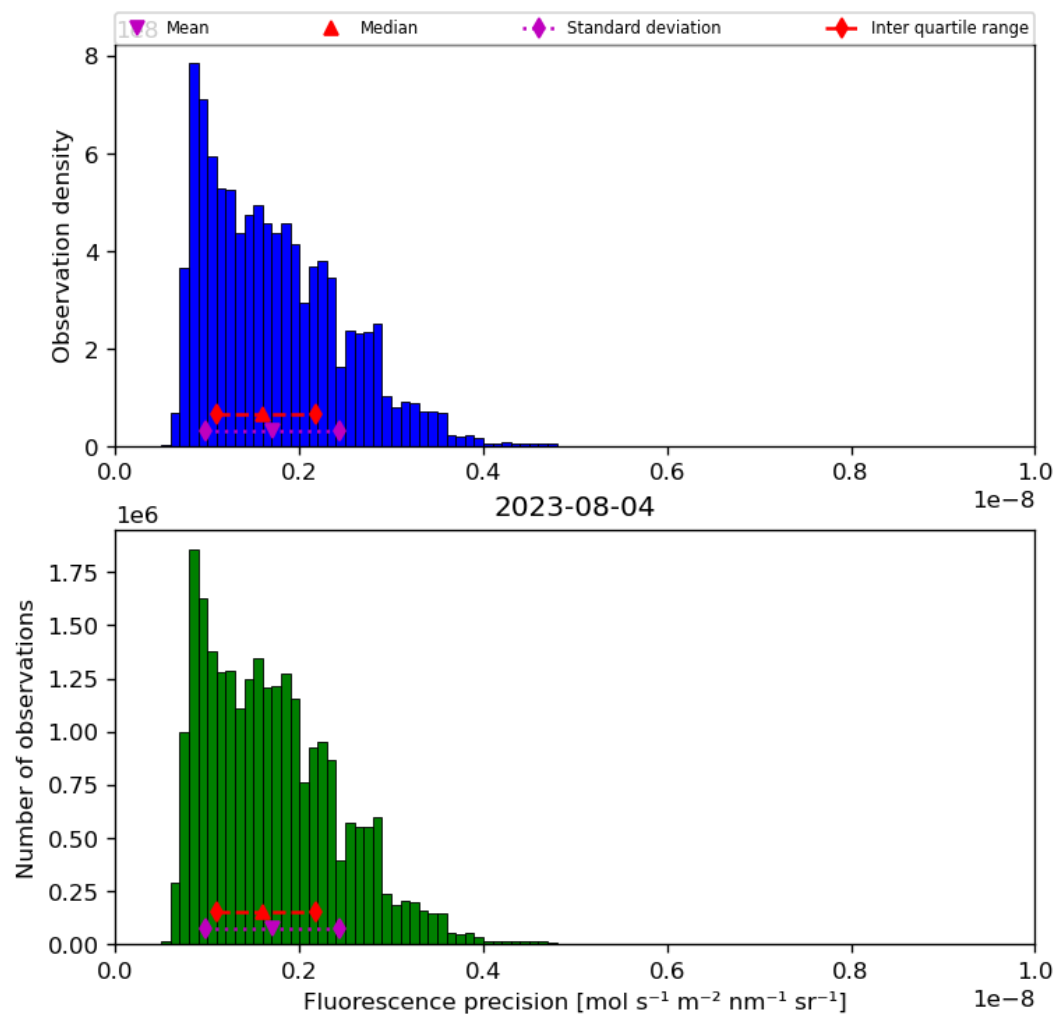
Figure 41: Histogram of “Fluorescence precision” for 2023-08-04 to 2023-08-05
