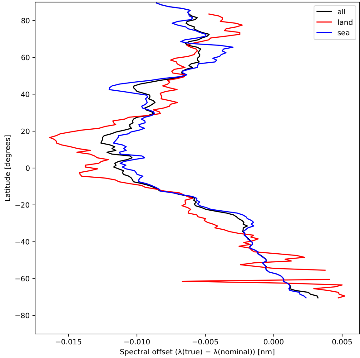
Figure 28: Zonal average of “Spectral offset ( \lambda(\text{true}) - \lambda(\text{nominal}) )” for 2023-08-04 to 2023-08-05.
