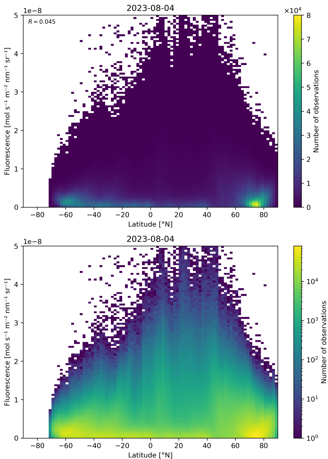
Figure 101: Scatter density plot of “Latitude” against “Fluorescence” for 2023-08-04 to 2023-08-05.
