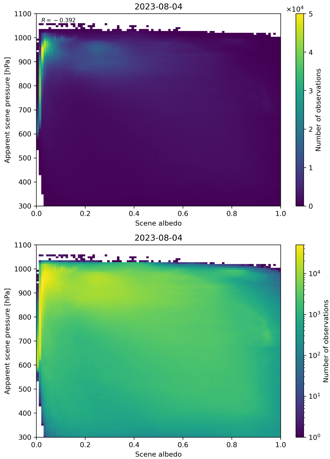
Figure 111: Scatter density plot of “Scene albedo” against “Apparent scene pressure” for 2023-08-04 to 2023-08-05.
