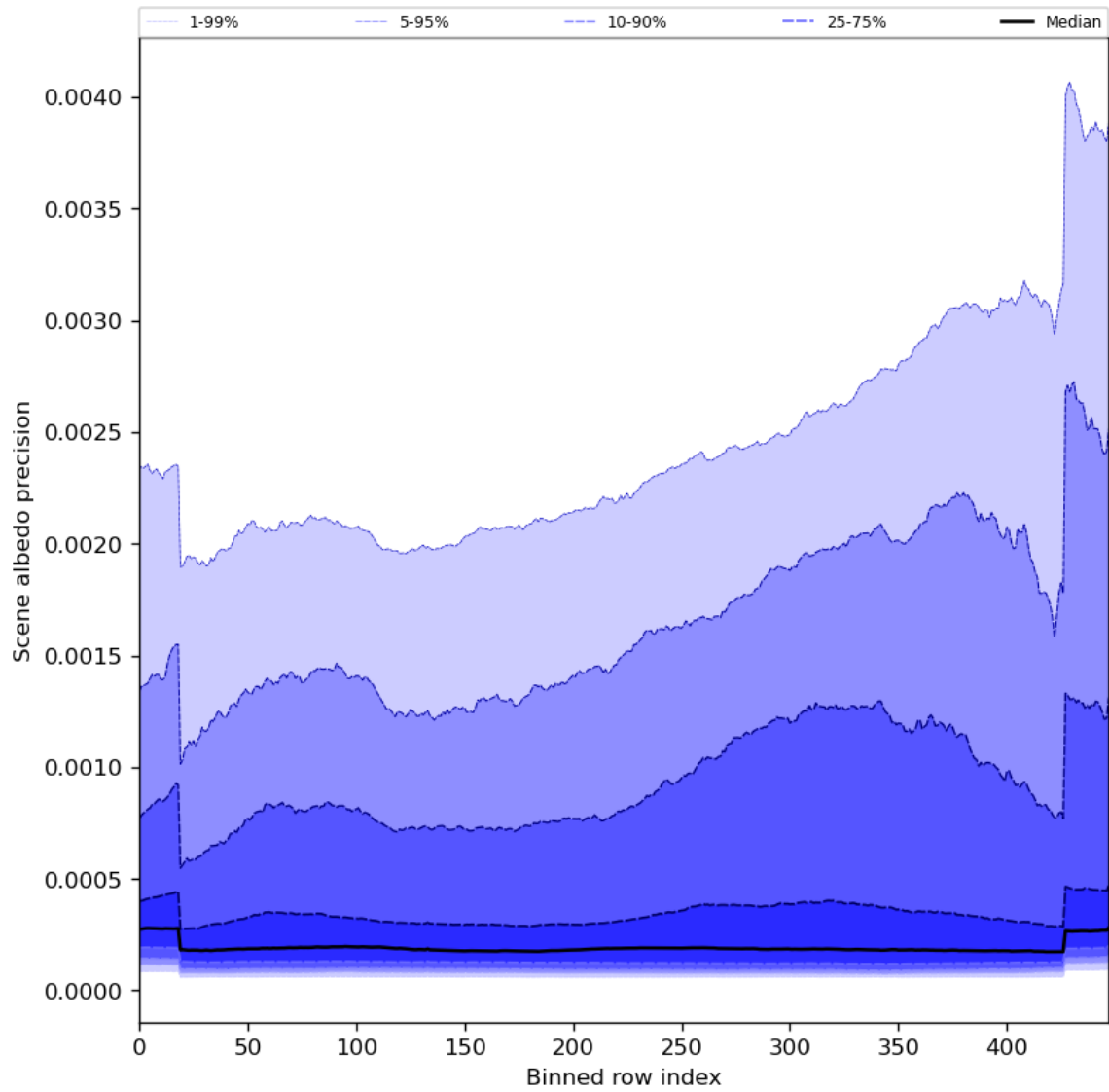
Figure 52: Along track statistics of “Scene albedo precision” for 2023-08-04 to 2023-08-05
