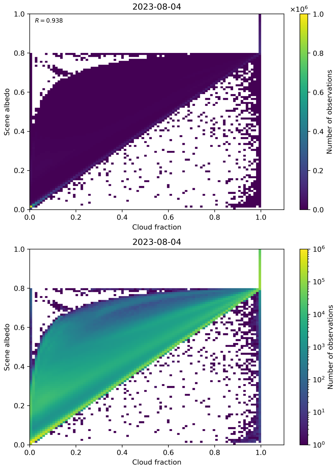
Figure 82: Scatter density plot of “Cloud fraction” against “Scene albedo” for 2023-08-04 to 2023-08-05.
