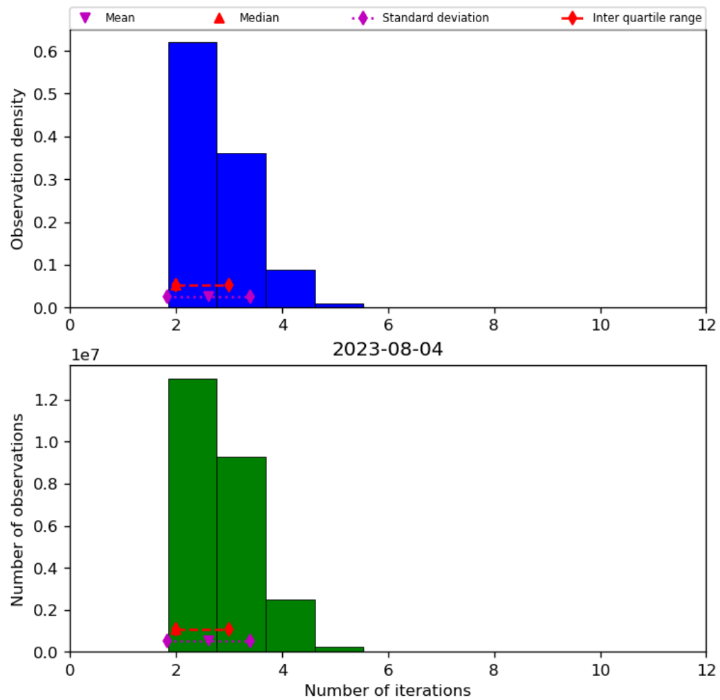
Figure 39: Histogram of “Number of iterations” for 2023-08-04 to 2023-08-05
