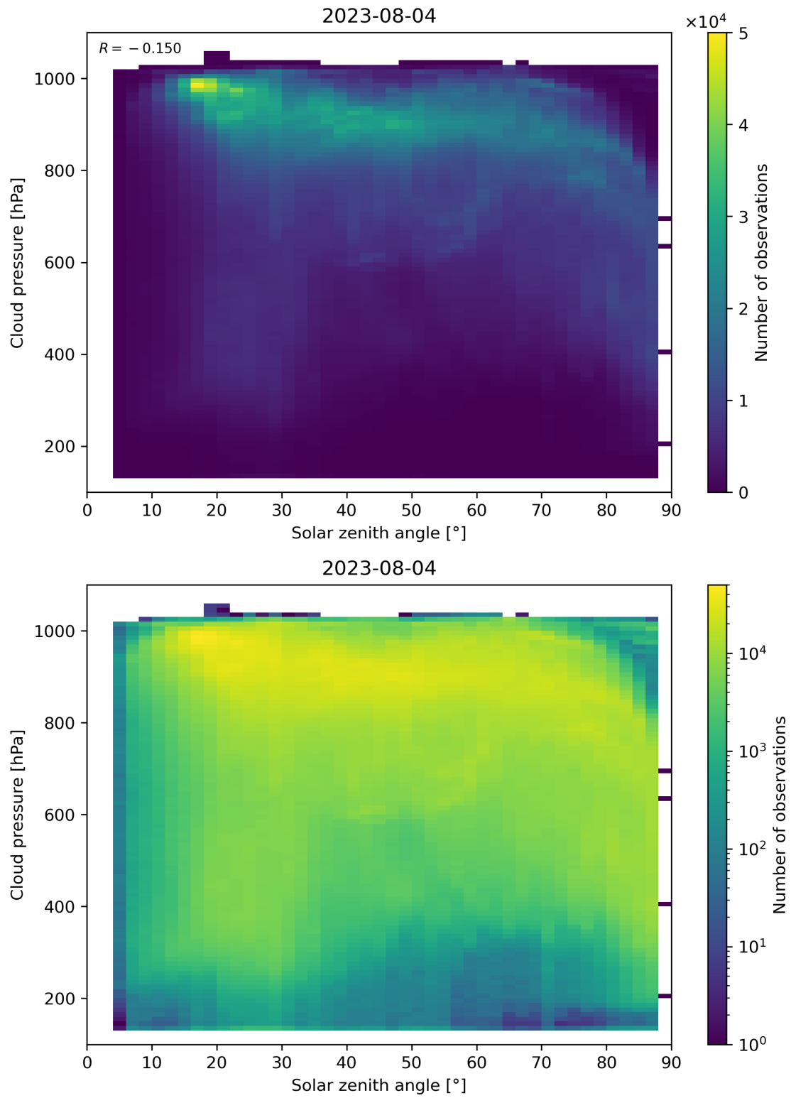
Figure 122: Scatter density plot of “Solar zenith angle” against “Cloud pressure” for 2023-08-04 to 2023-08-05.
