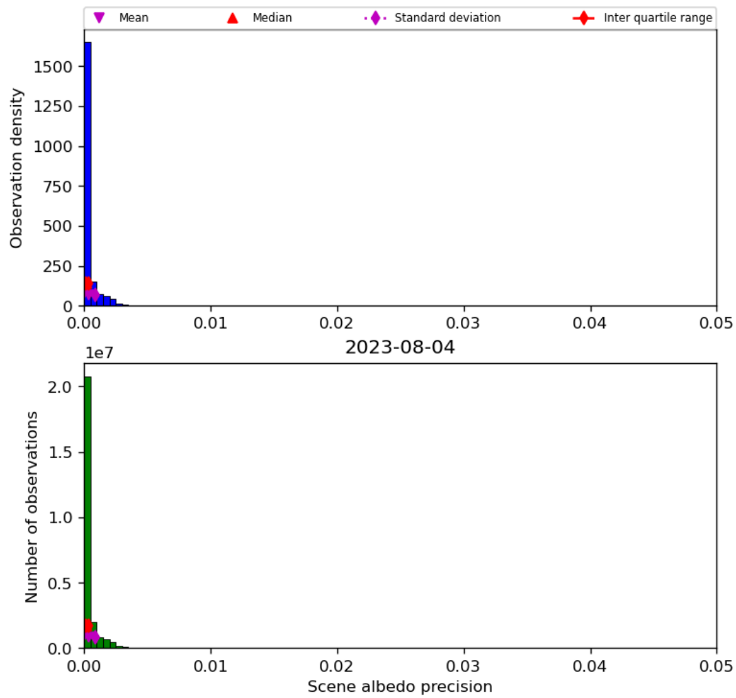
Figure 35: Histogram of “Scene albedo precision” for 2023-08-04 to 2023-08-05
