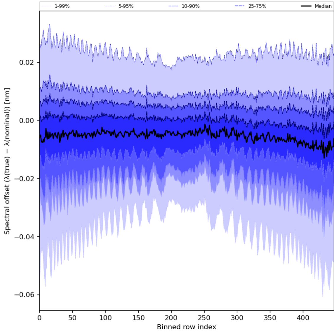
Figure 62: Along track statistics of “Spectral offset ( \lambda(\text{true}) - \lambda(\text{nominal}) )” for 2023-08-04 to 2023-08-05
