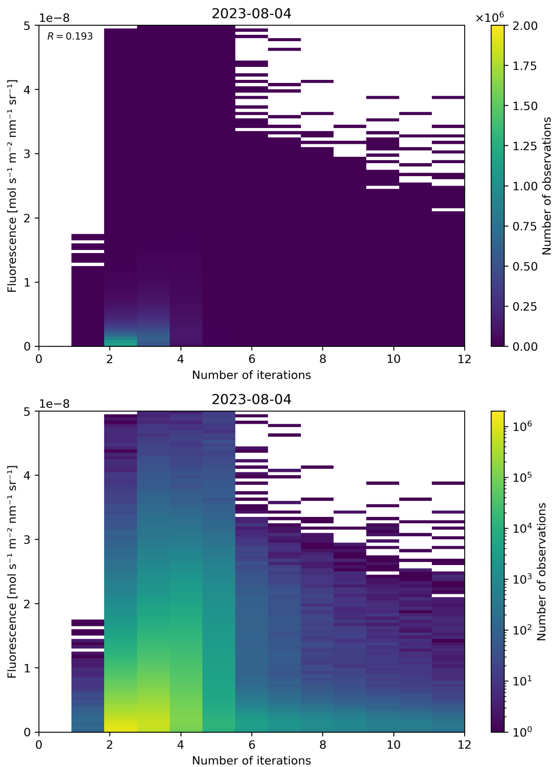
Figure 107: Scatter density plot of “Number of iterations” against “Fluorescence” for 2023-08-04 to 2023-08-05.
