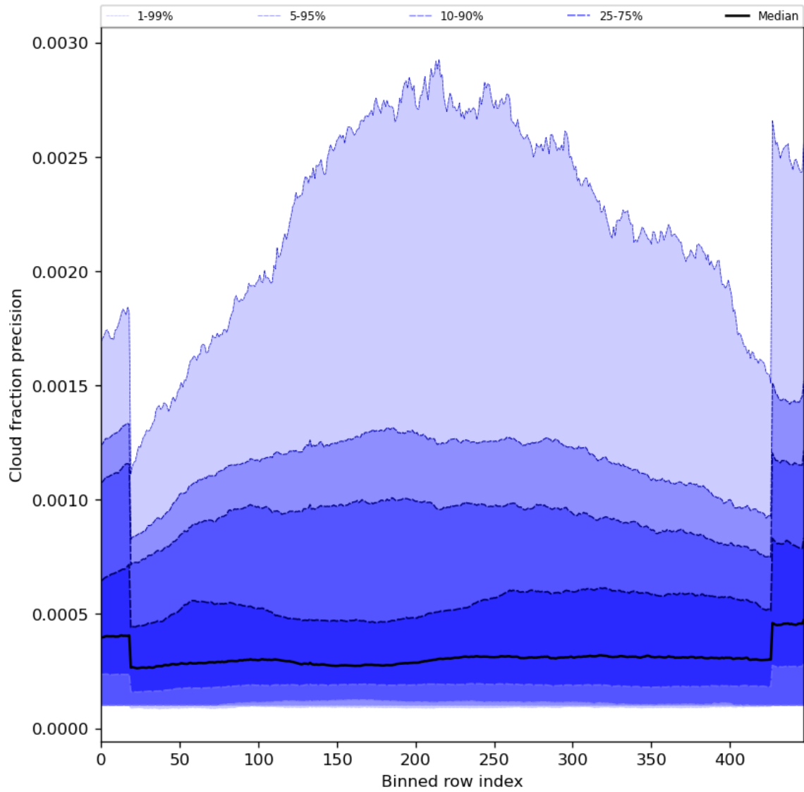
Figure 50: Along track statistics of “Cloud fraction precision” for 2023-08-04 to 2023-08-05
