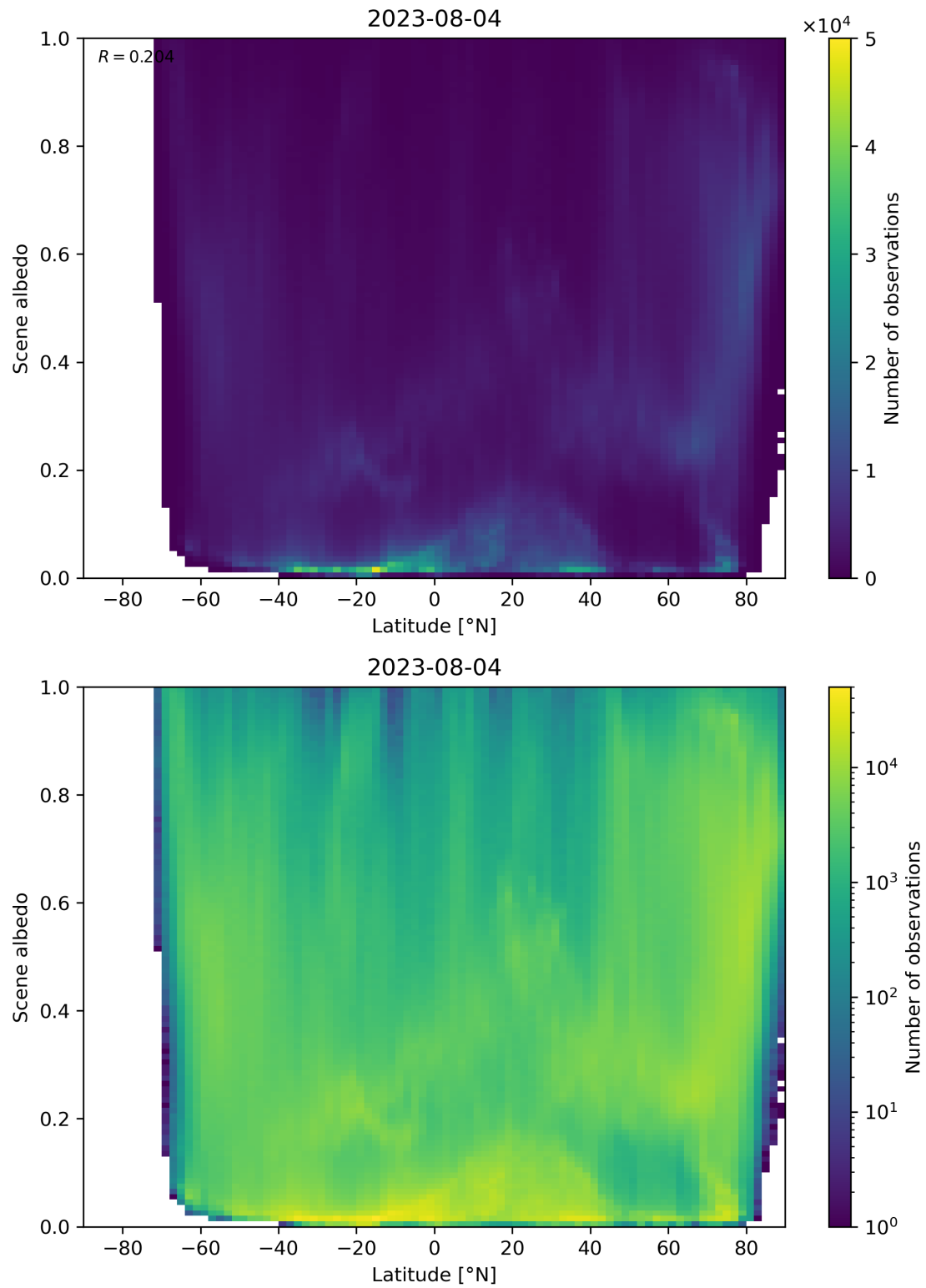
Figure 104: Scatter density plot of “Latitude” against “Scene albedo” for 2023-08-04 to 2023-08-05.
