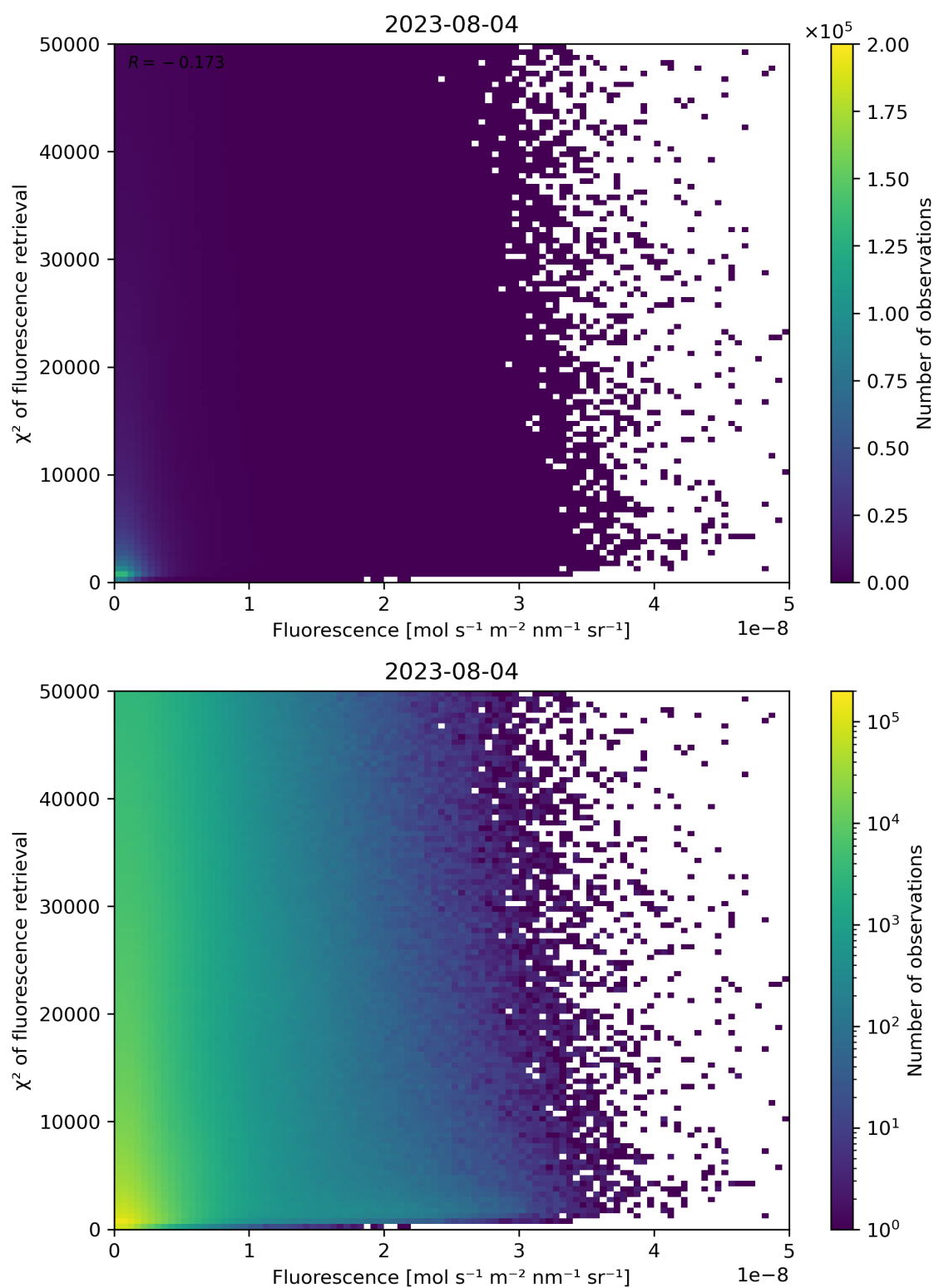
Figure 93: Scatter density plot of “Fluorescence” against “ \chi^2 of fluorescence retrieval” for 2023-08-04 to 2023-08-05.
