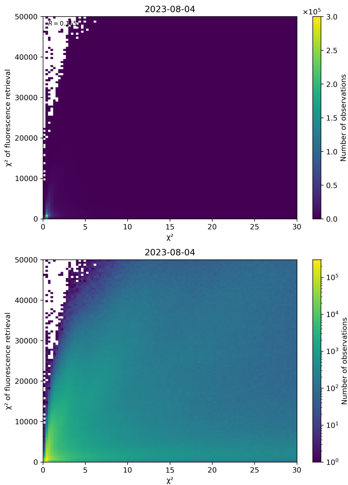
Figure 69: Scatter density plot of “ \chi^2 ” against “ \chi^2 of fluorescence retrieval” for 2023-08-04 to 2023-08-05.
