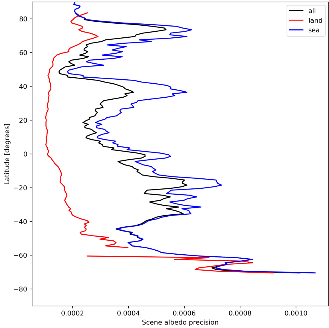
Figure 18: Zonal average of "Scene albedo precision" for 2023-08-04 to 2023-08-05.
