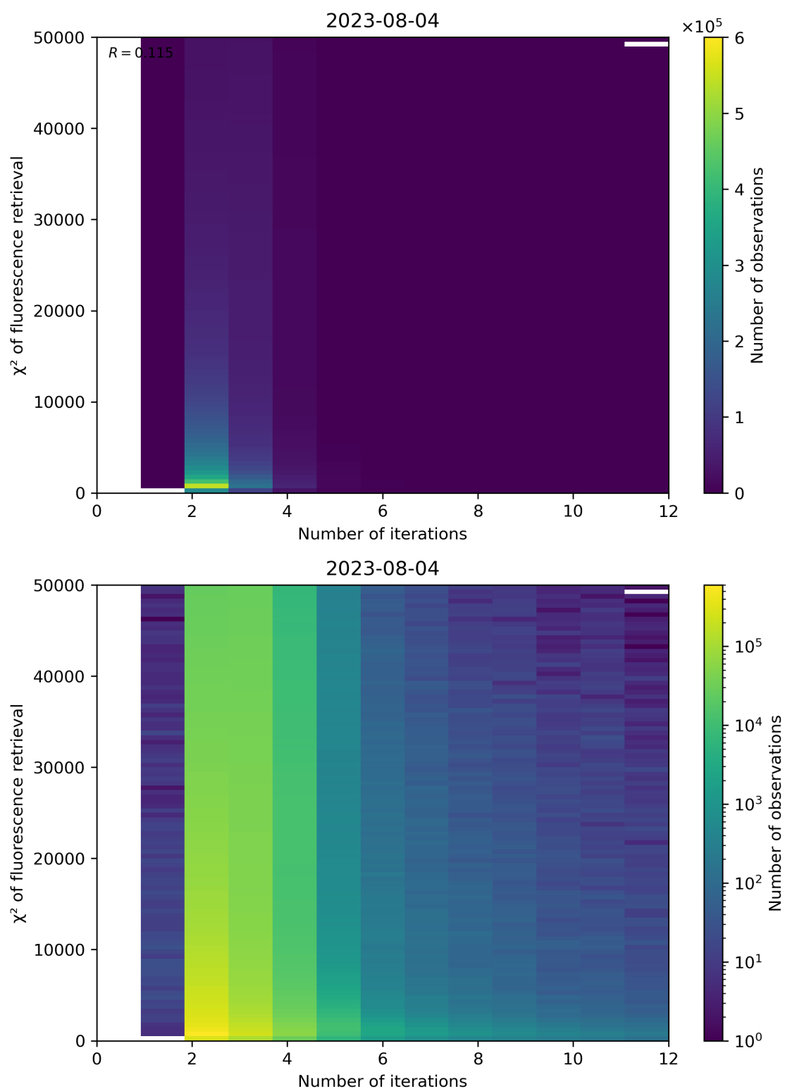
Figure 106: Scatter density plot of “Number of iterations” against “ \chi^2 of fluorescence retrieval” for 2023-08-04 to 2023-08-05.
