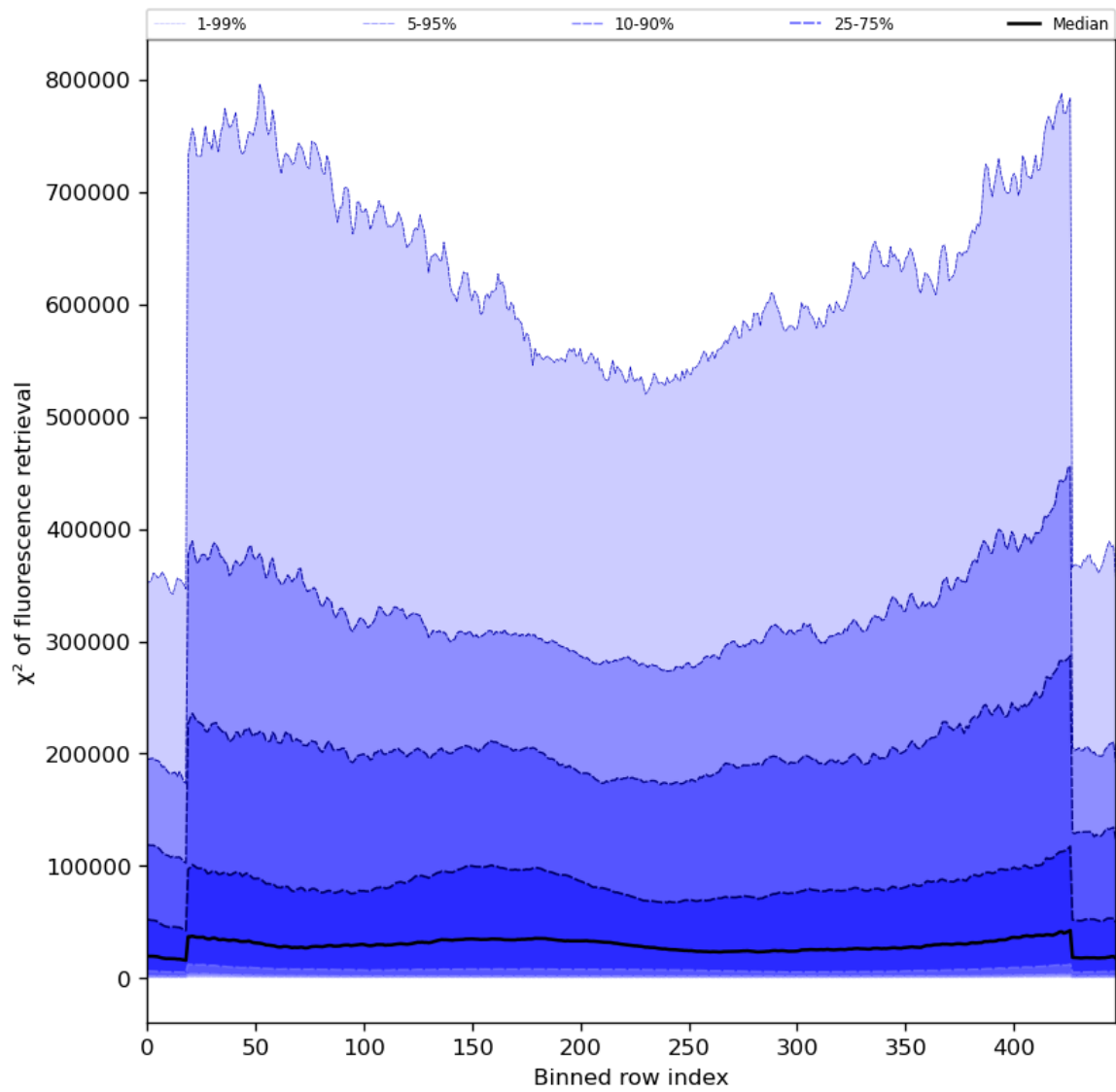
Figure 59: Along track statistics of “ \chi^2 of fluorescence retrieval” for 2023-08-04 to 2023-08-05
