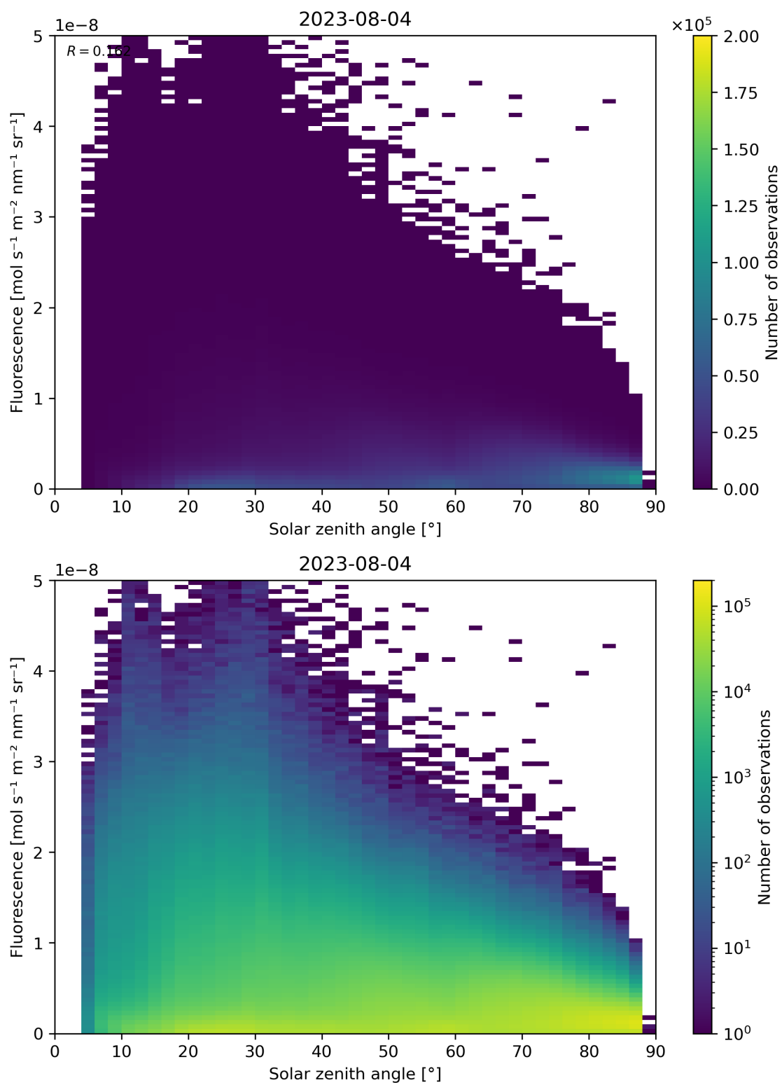
Figure 123: Scatter density plot of “Solar zenith angle” against “Fluorescence” for 2023-08-04 to 2023-08-05.
