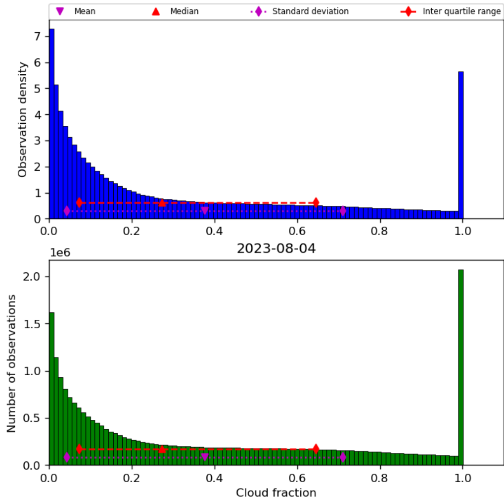
Figure 32: Histogram of “Cloud fraction” for 2023-08-04 to 2023-08-05
