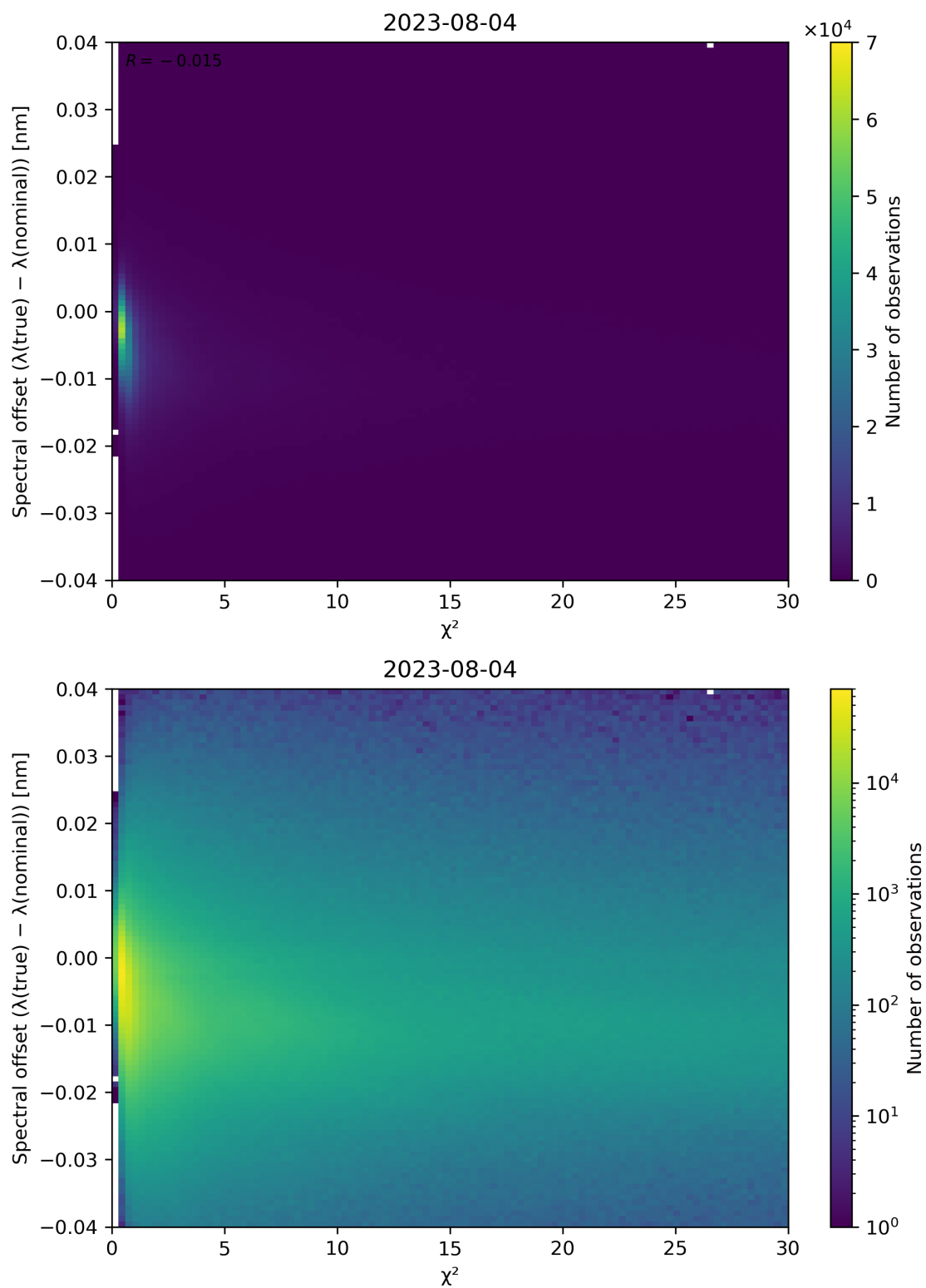
Figure 75: Scatter density plot of “ \chi^2 ” against “Spectral offset ( \lambda(\text{true}) - \lambda(\text{nominal}) )” for 2023-08-04 to 2023-08-05.
