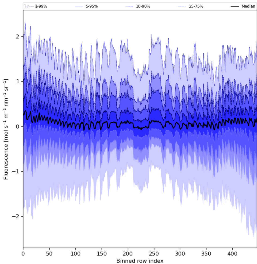
Figure 57: Along track statistics of “Fluorescence” for 2023-08-04 to 2023-08-05
