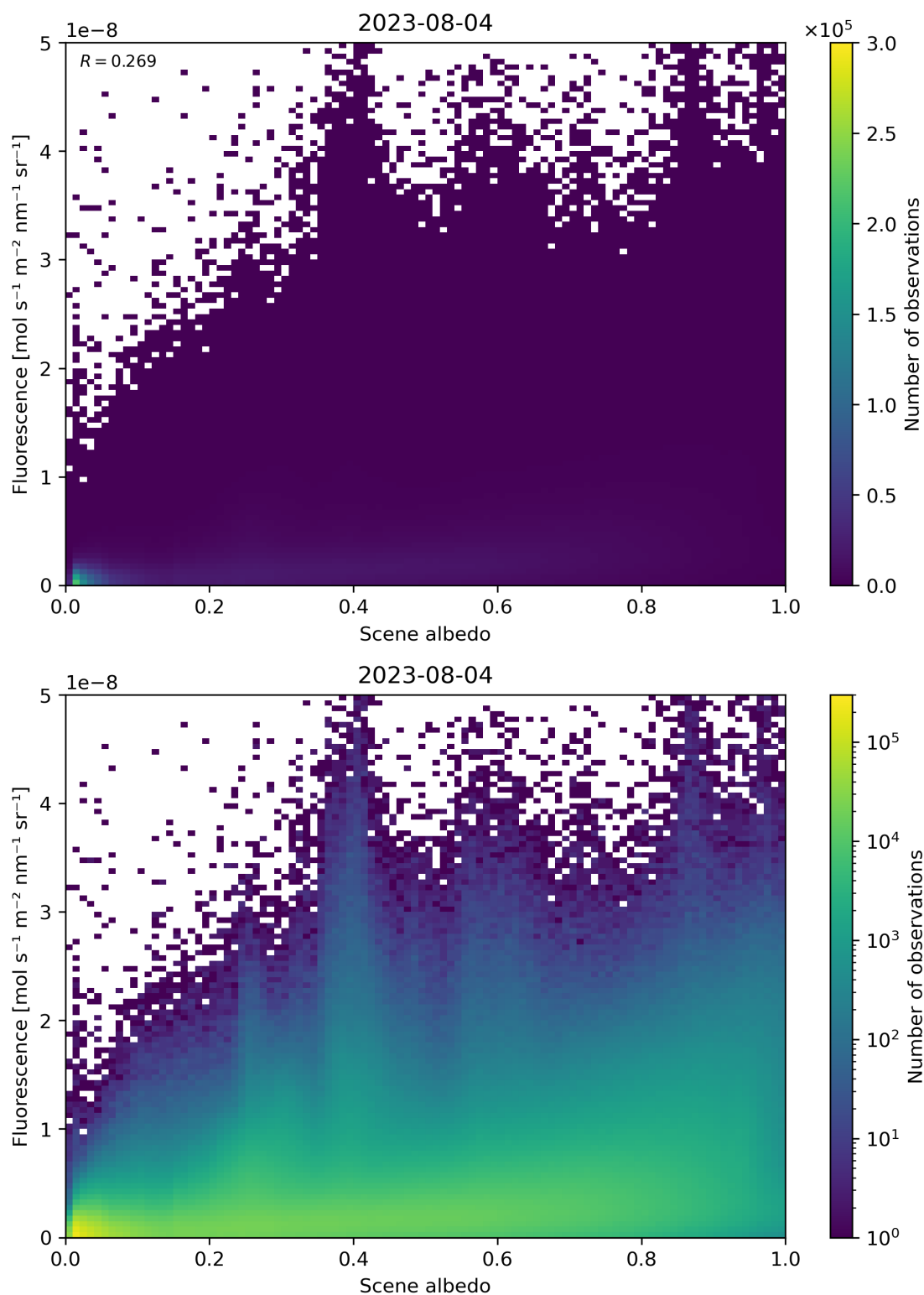
Figure 114: Scatter density plot of “Scene albedo” against “Fluorescence” for 2023-08-04 to 2023-08-05.
