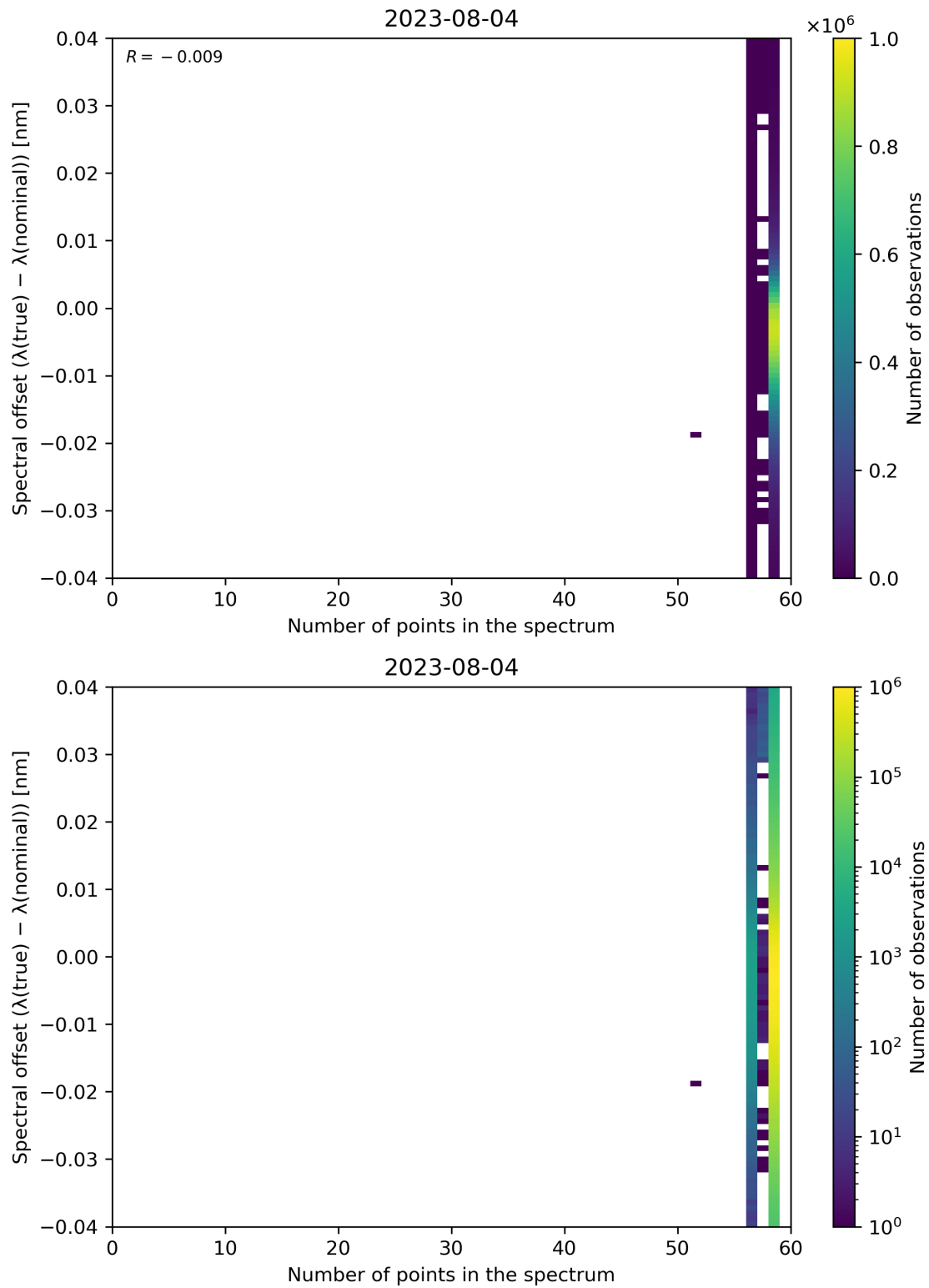
Figure 110: Scatter density plot of “Number of points in the spectrum” against “Spectral offset ( \lambda(\text{true}) - \lambda(\text{nominal}) )” for 2023-08-04 to 2023-08-05.
