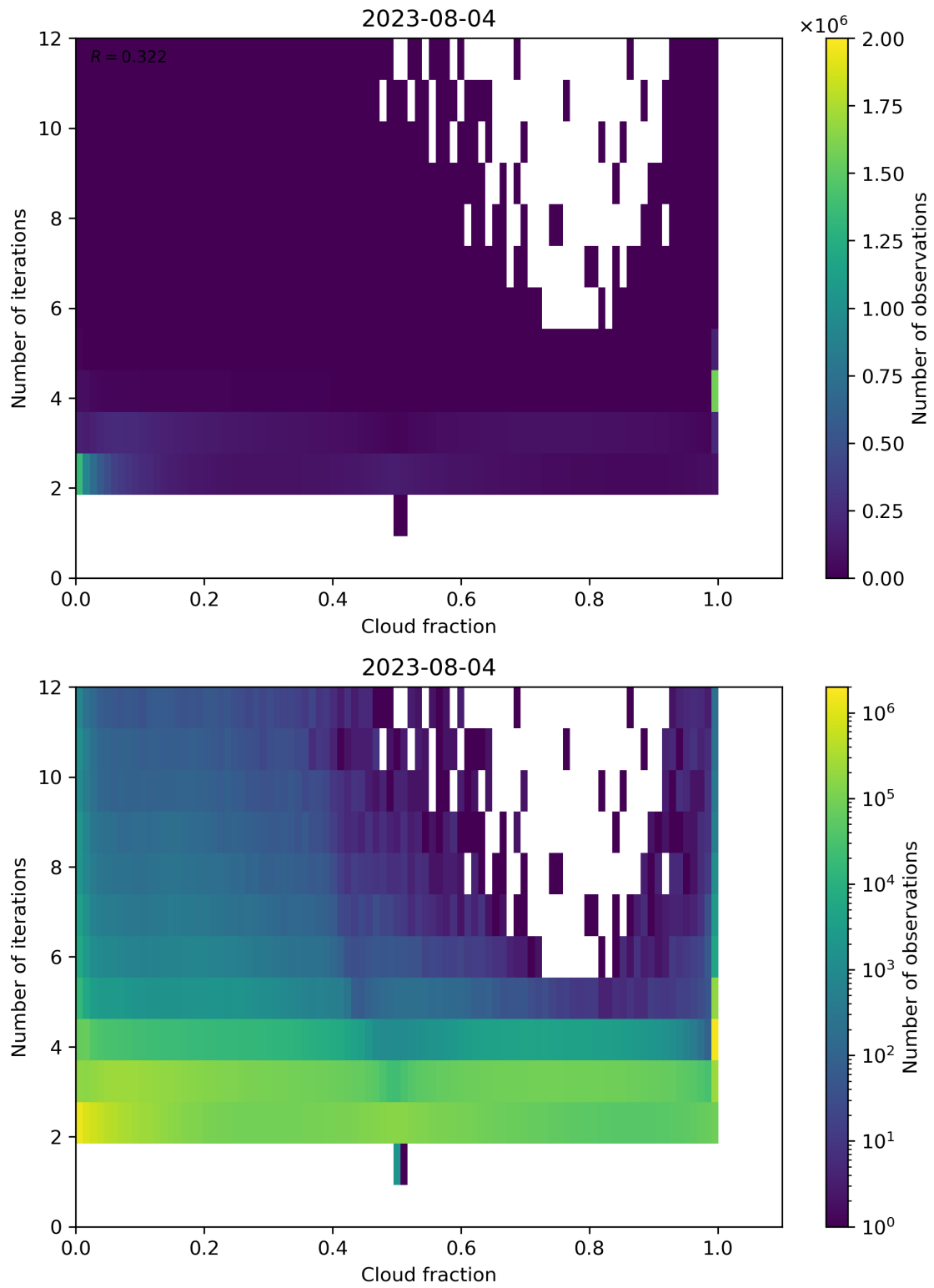
Figure 80: Scatter density plot of “Cloud fraction” against “Number of iterations” for 2023-08-04 to 2023-08-05.
