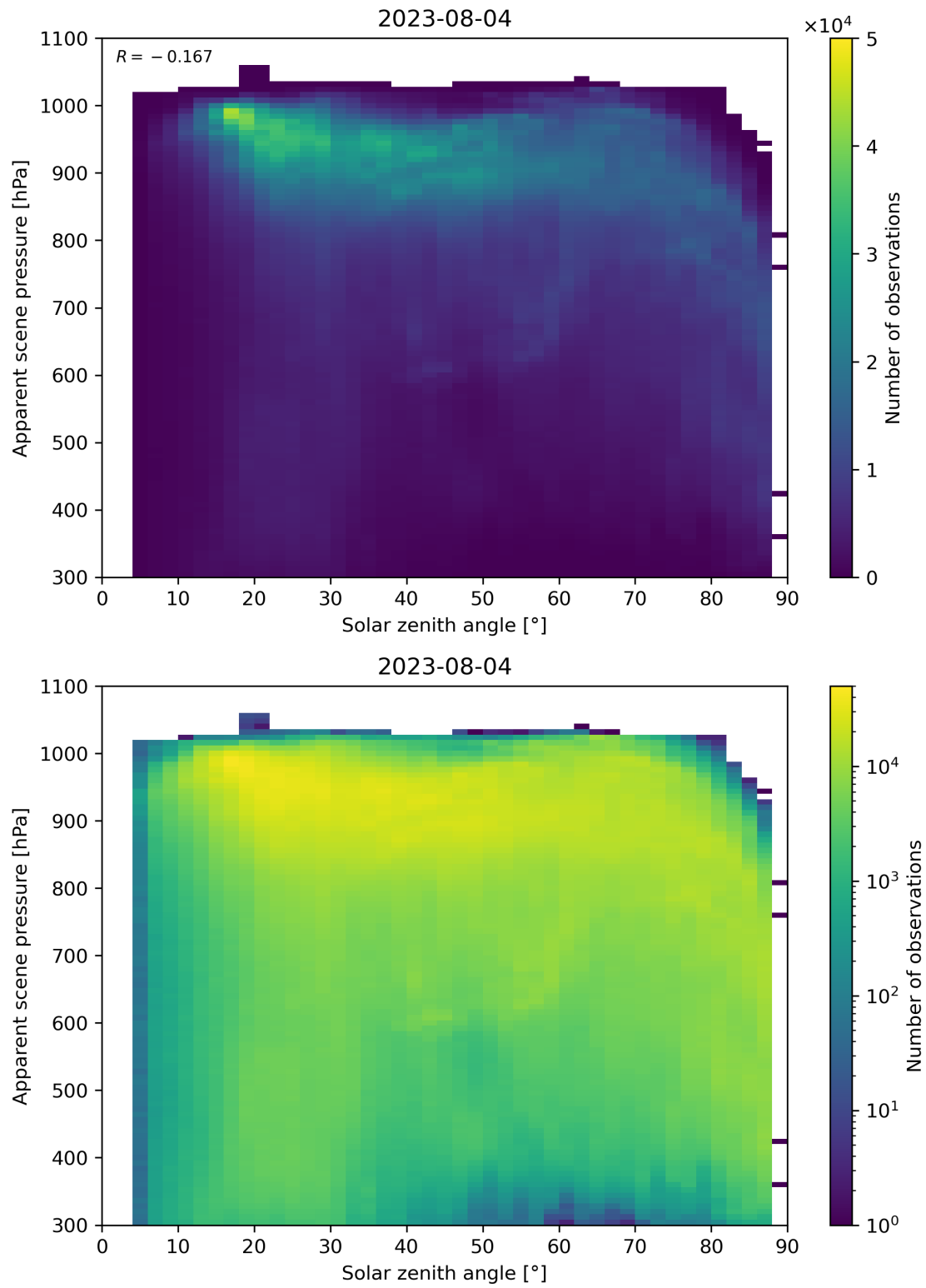
Figure 118: Scatter density plot of “Solar zenith angle” against “Apparent scene pressure” for 2023-08-04 to 2023-08-05.
