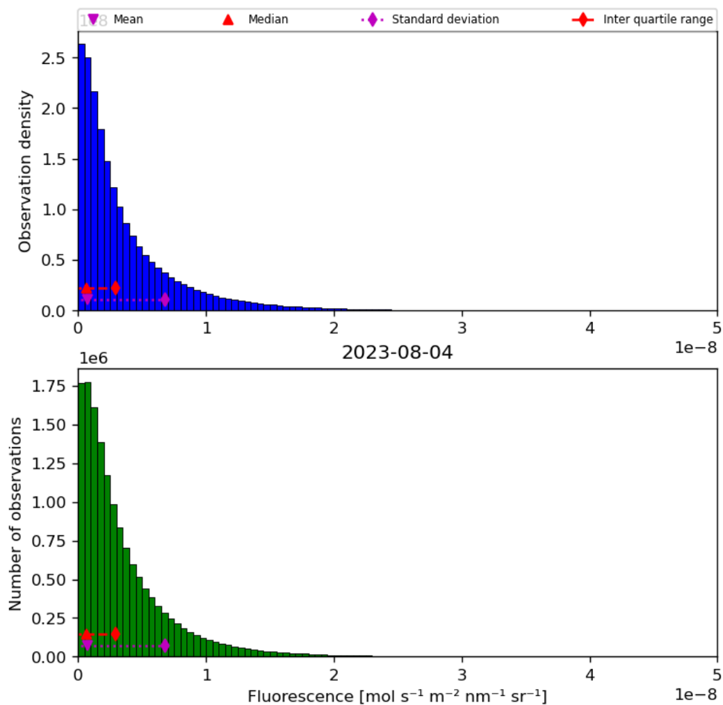
Figure 40: Histogram of “Fluorescence” for 2023-08-04 to 2023-08-05
