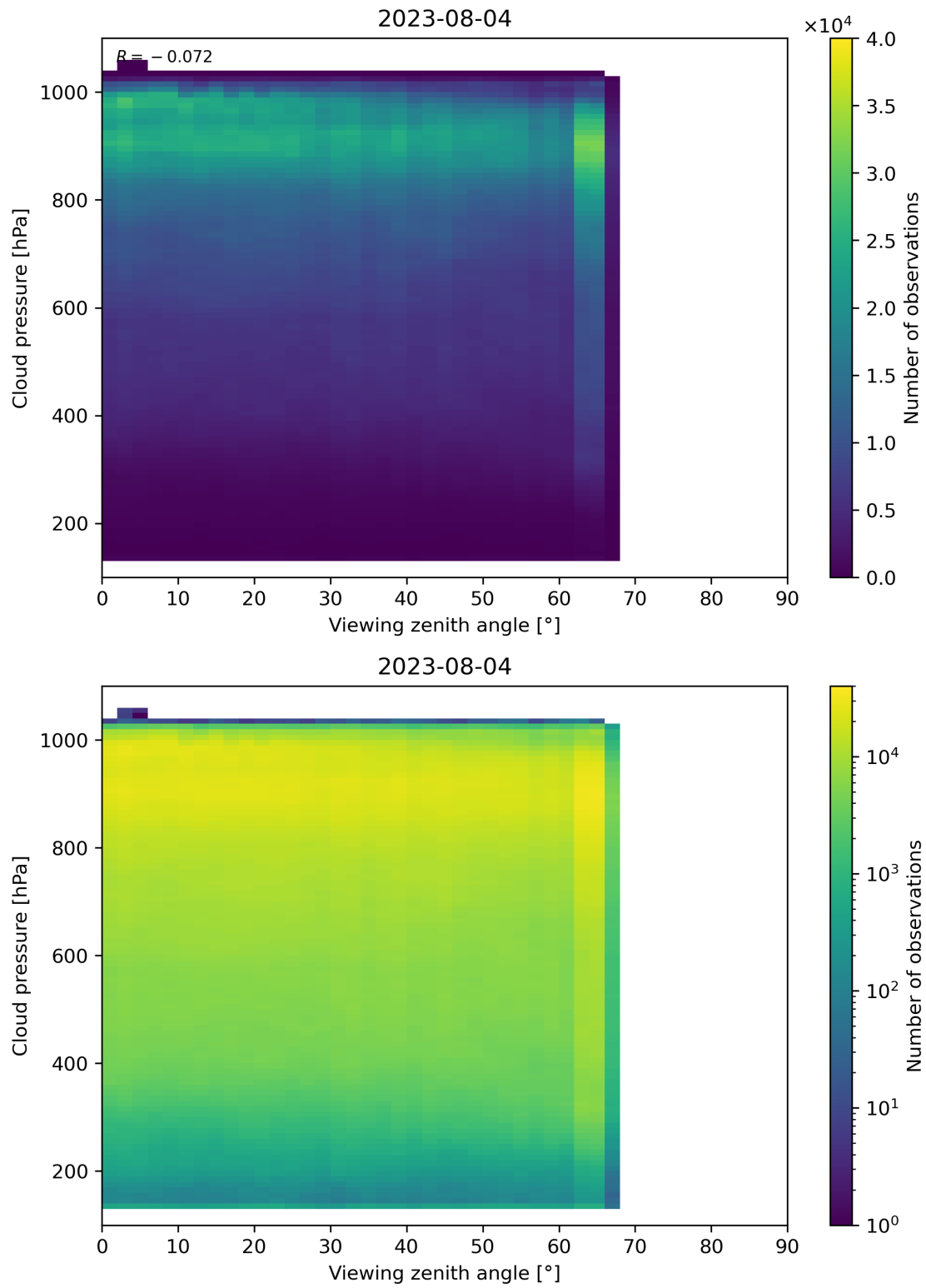
Figure 133: Scatter density plot of “Viewing zenith angle” against “Cloud pressure” for 2023-08-04 to 2023-08-05.
