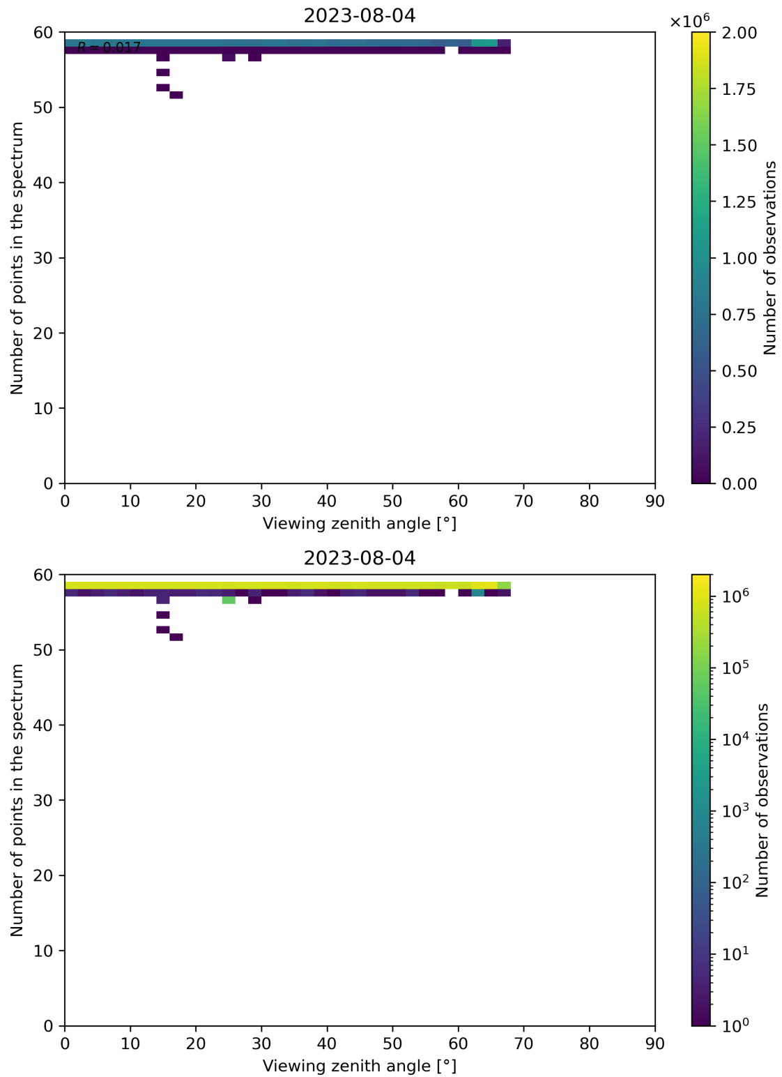
Figure 137: Scatter density plot of “Viewing zenith angle” against “Number of points in the spectrum” for 2023-08-04 to 2023-08-05.
