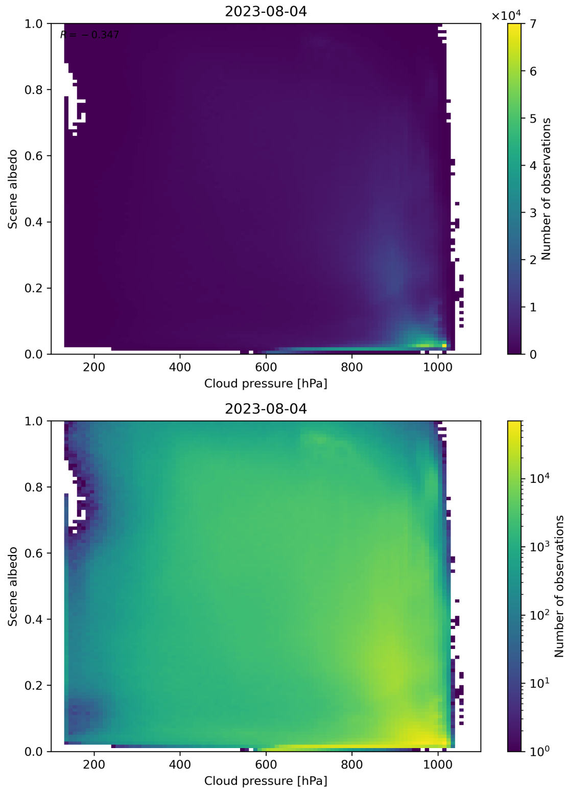
Figure 91: Scatter density plot of “Cloud pressure” against “Scene albedo” for 2023-08-04 to 2023-08-05.
