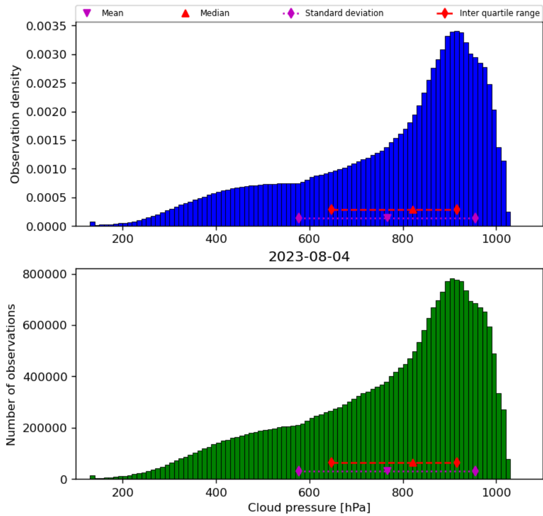
Figure 30: Histogram of “Cloud pressure” for 2023-08-04 to 2023-08-05
