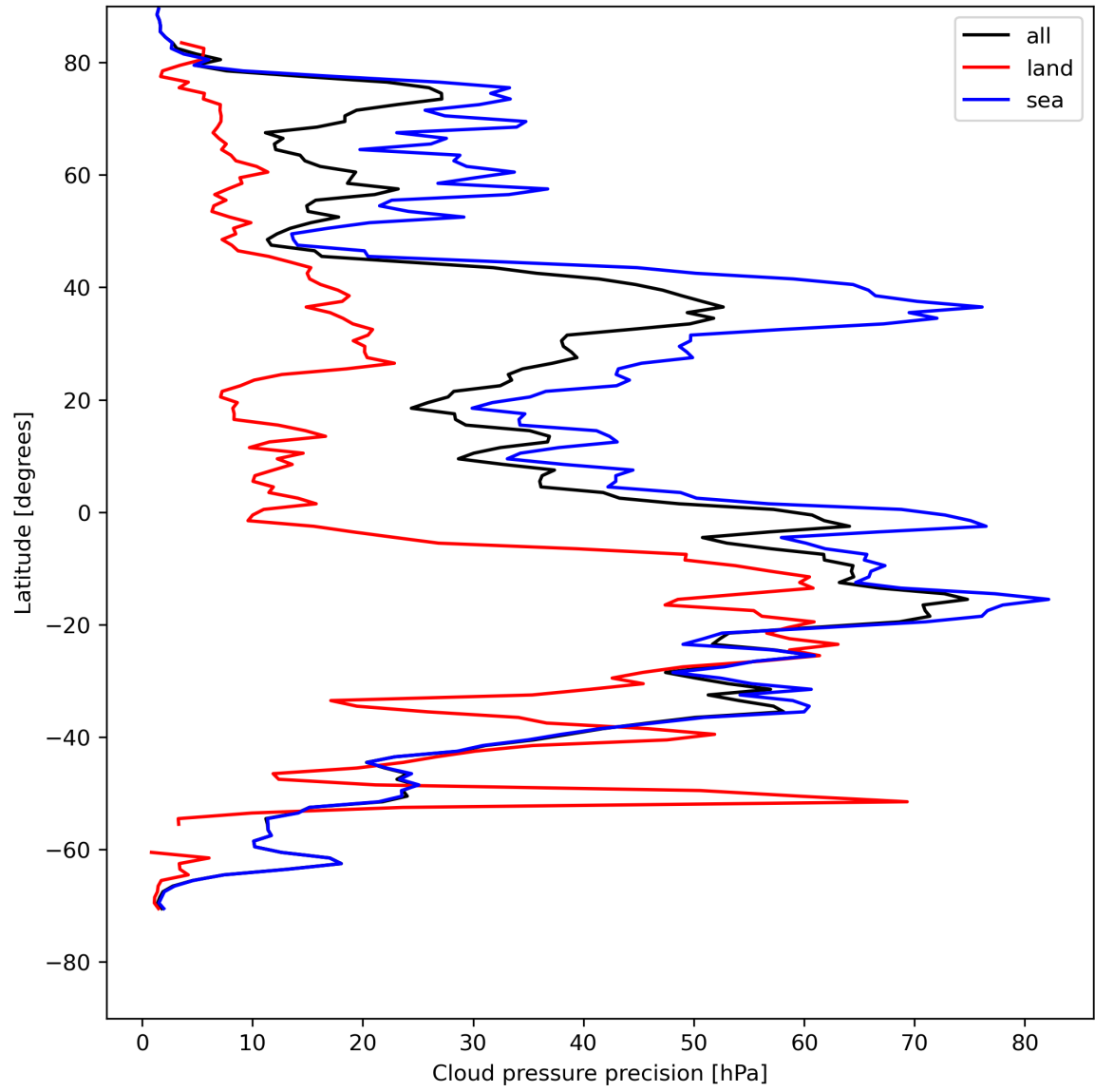
Figure 14: Zonal average of “Cloud pressure precision” for 2023-08-04 to 2023-08-05.
