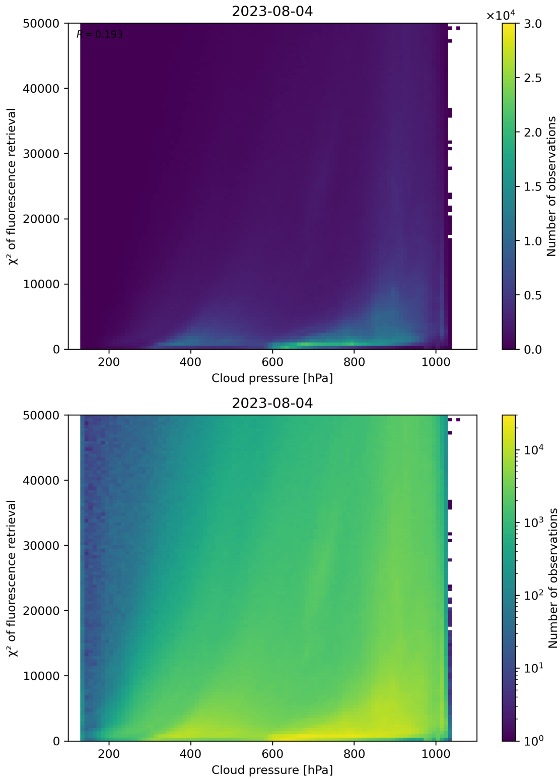
Figure 86: Scatter density plot of “Cloud pressure” against “ \chi^2 of fluorescence retrieval” for 2023-08-04 to 2023-08-05.
