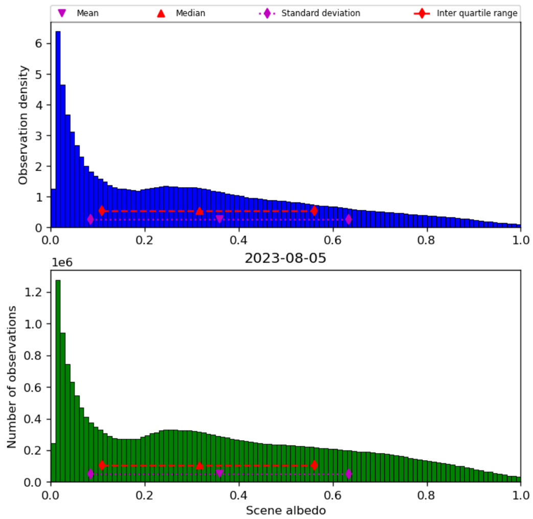
Figure 34: Histogram of “Scene albedo” for 2023-08-04 to 2023-08-06
