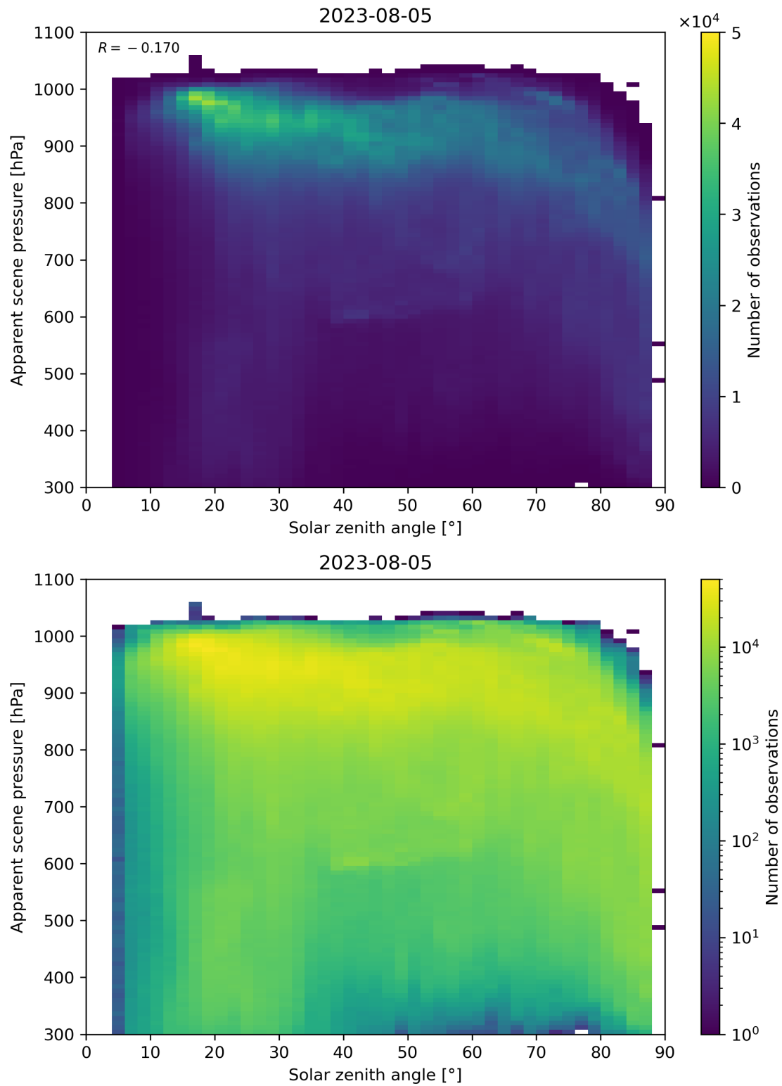
Figure 118: Scatter density plot of “Solar zenith angle” against “Apparent scene pressure” for 2023-08-04 to 2023-08-06.
