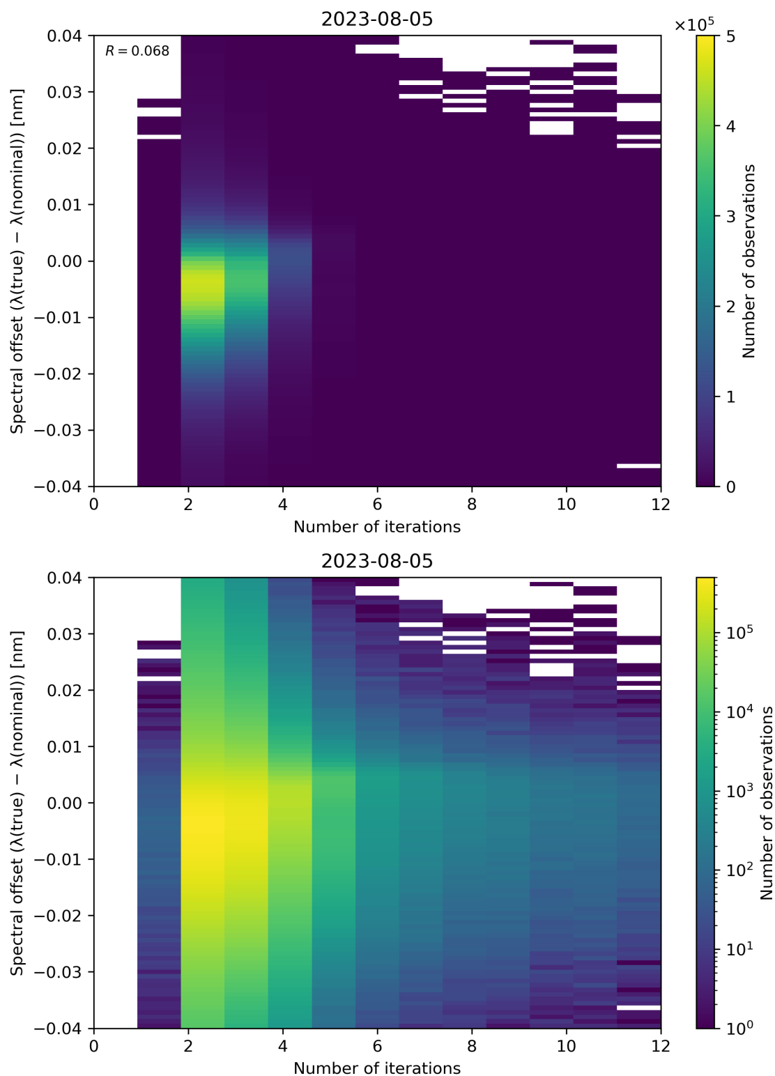
Figure 109: Scatter density plot of “Number of iterations” against “Spectral offset ( \lambda(\text{true}) - \lambda(\text{nominal}) )” for 2023-08-04 to 2023-08-06.
