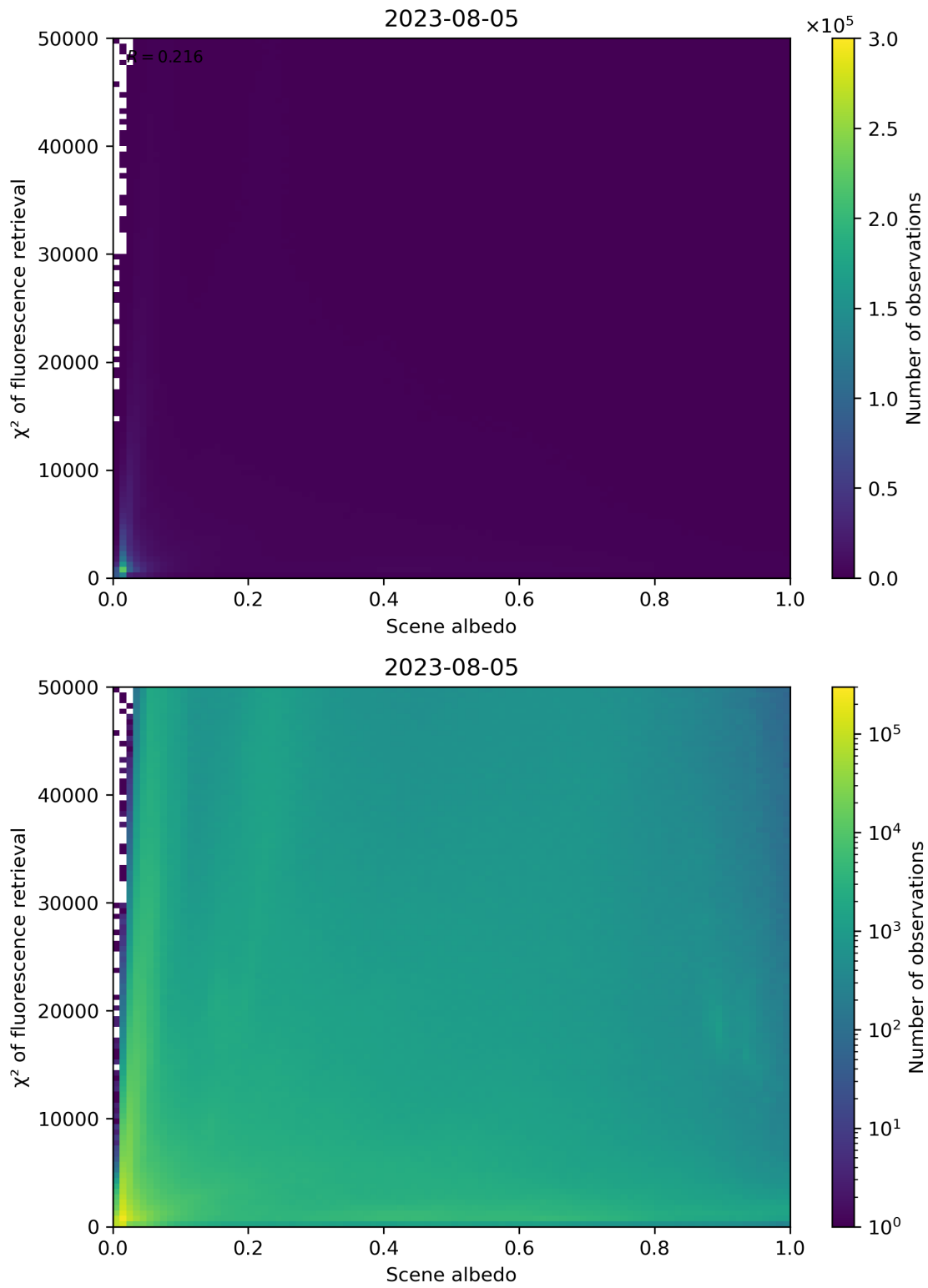
Figure 113: Scatter density plot of “Scene albedo” against “ \chi^2 of fluorescence retrieval” for 2023-08-04 to 2023-08-06.
