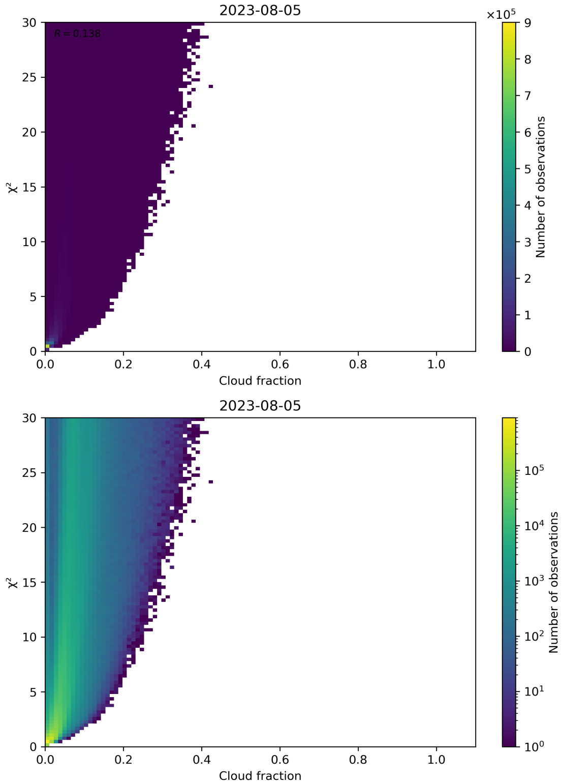
Figure 77: Scatter density plot of “Cloud fraction” against “ \chi^2 ” for 2023-08-04 to 2023-08-06.
