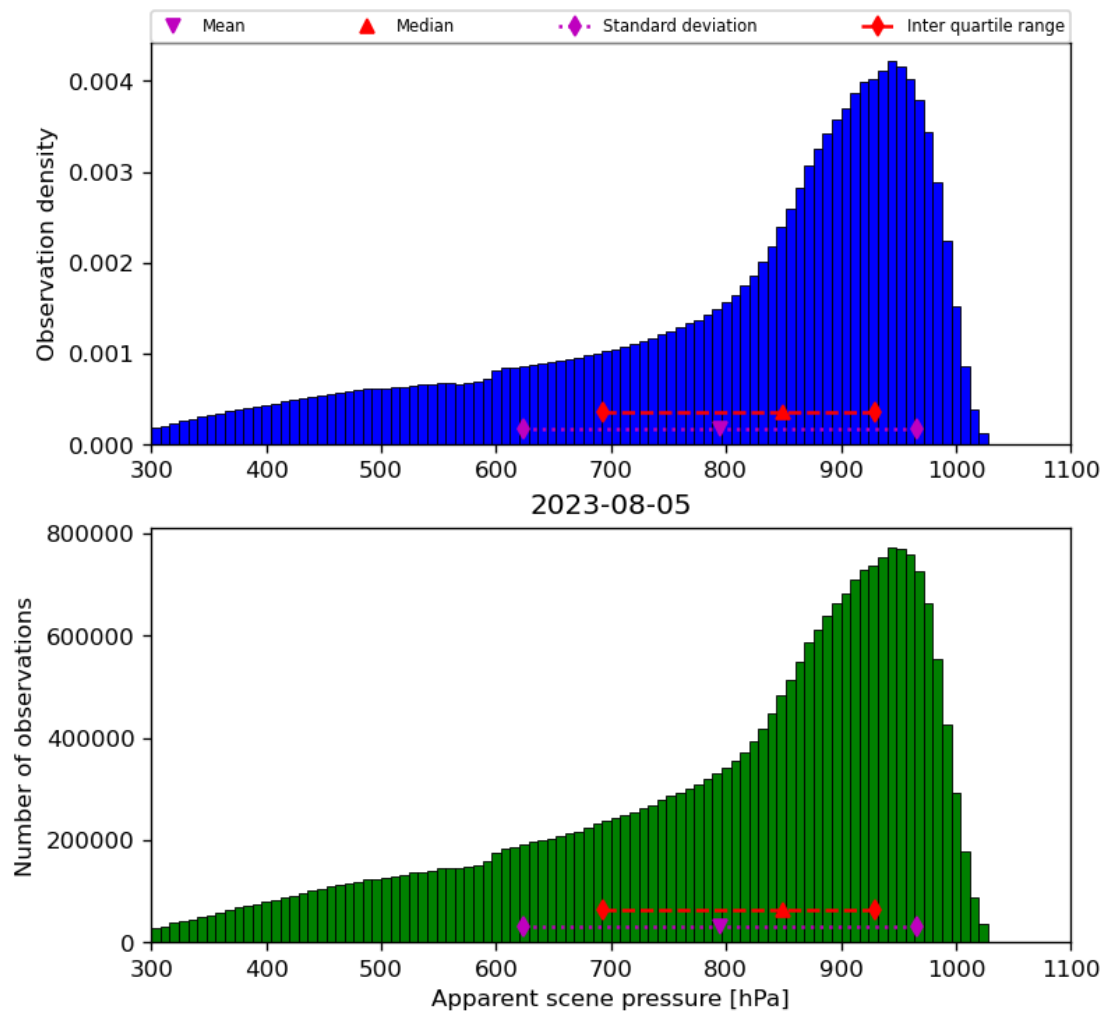
Figure 36: Histogram of “Apparent scene pressure” for 2023-08-04 to 2023-08-06
