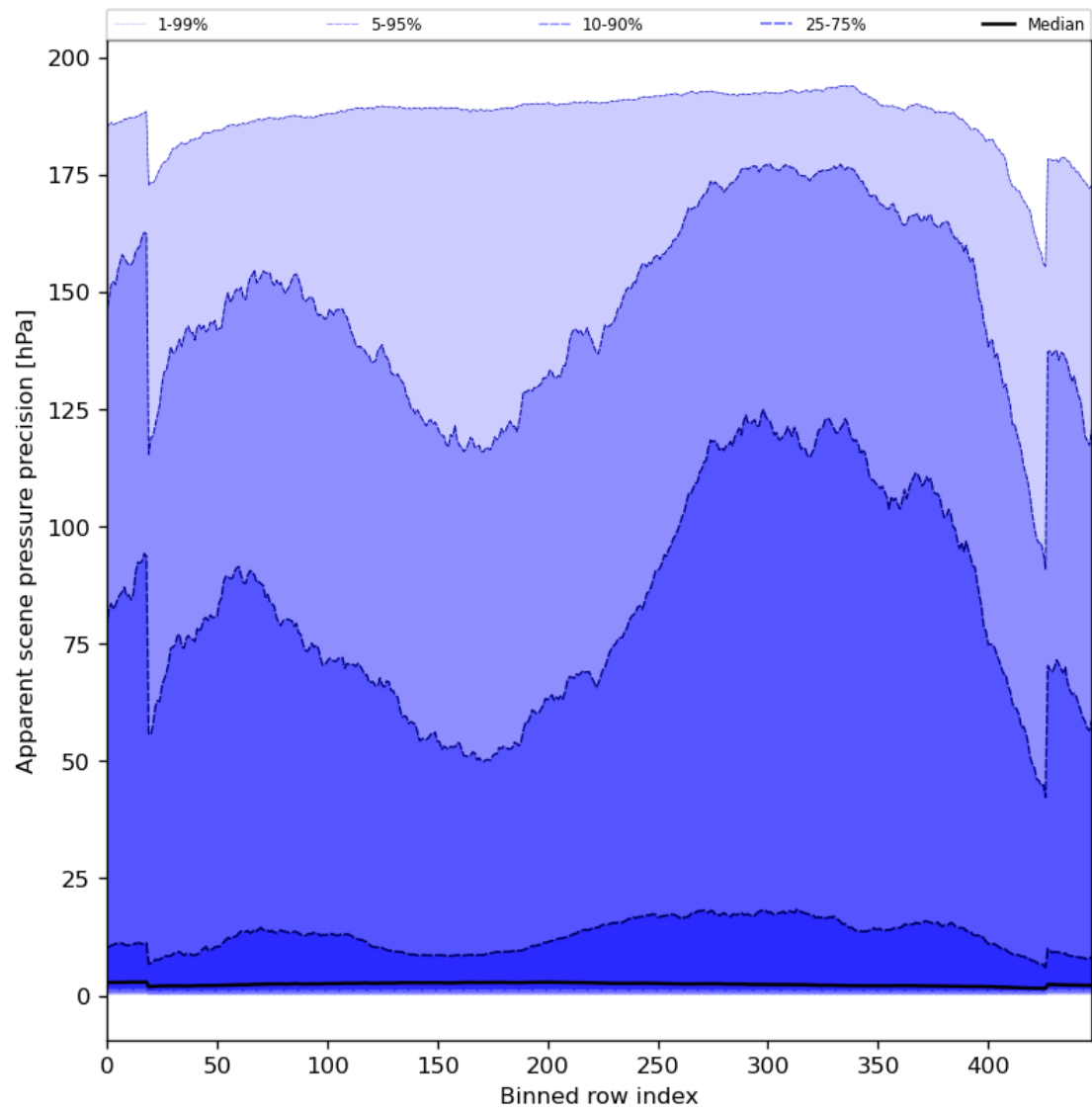
Figure 54: Along track statistics of “Apparent scene pressure precision” for 2023-08-04 to 2023-08-06
