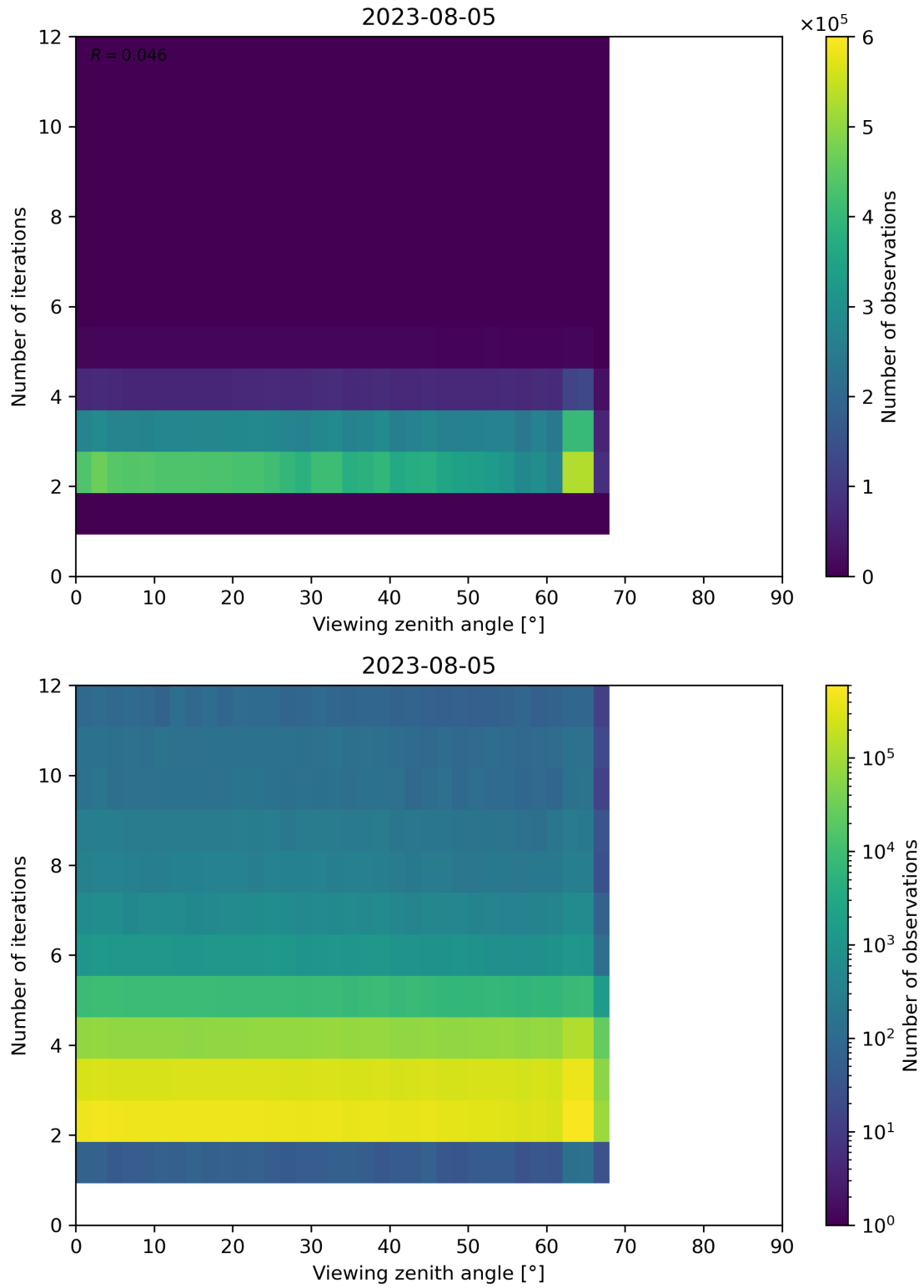
Figure 136: Scatter density plot of “Viewing zenith angle” against “Number of iterations” for 2023-08-04 to 2023-08-06.
