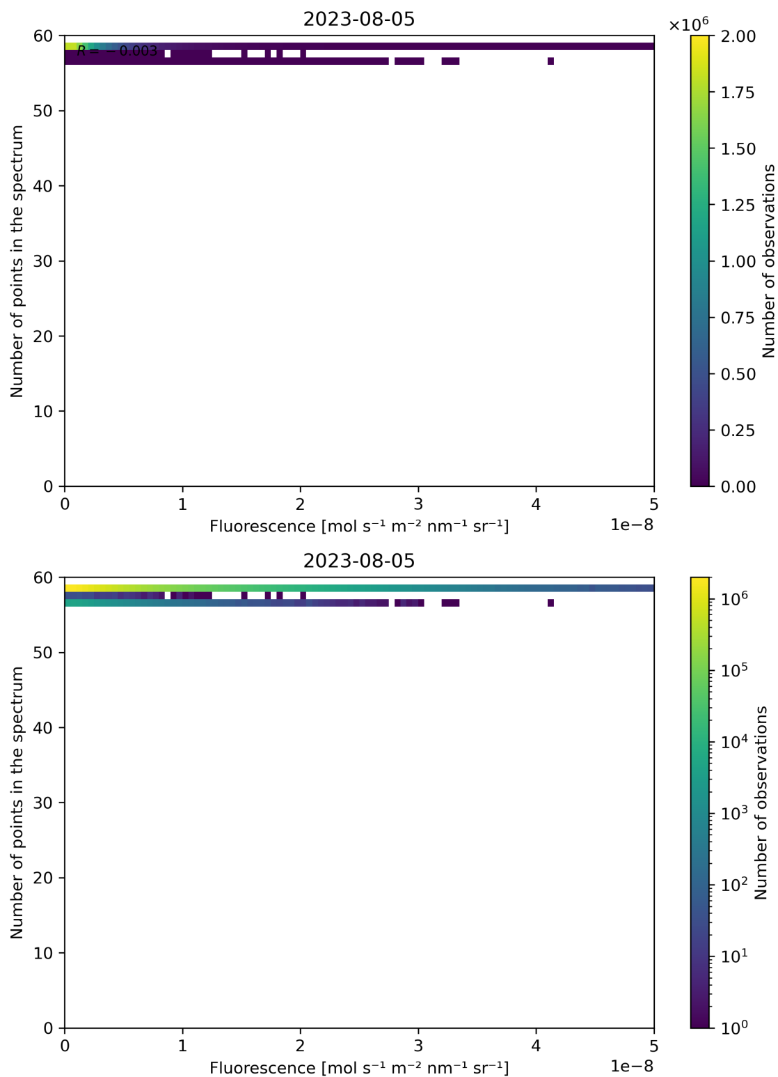
Figure 94: Scatter density plot of “Fluorescence” against “Number of points in the spectrum” for 2023-08-04 to 2023-08-06.
