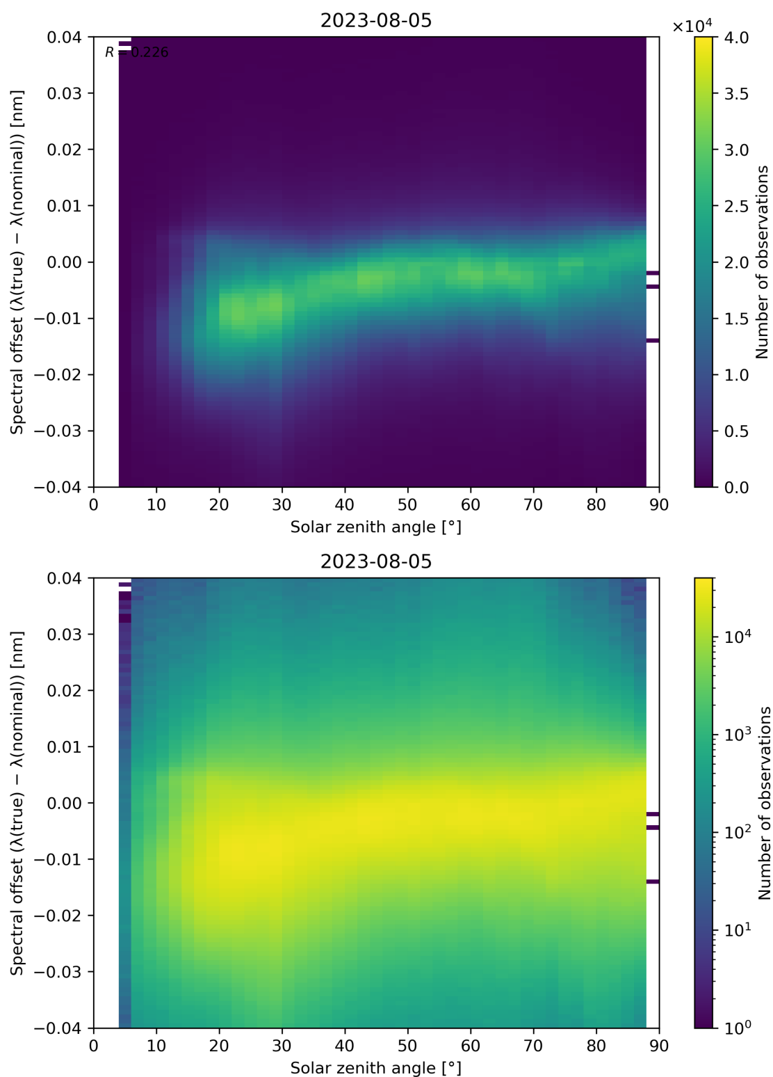
Figure 128: Scatter density plot of “Solar zenith angle” against “Spectral offset ( \lambda(\text{true}) - \lambda(\text{nominal}) )” for 2023-08-04 to 2023-08-06.
