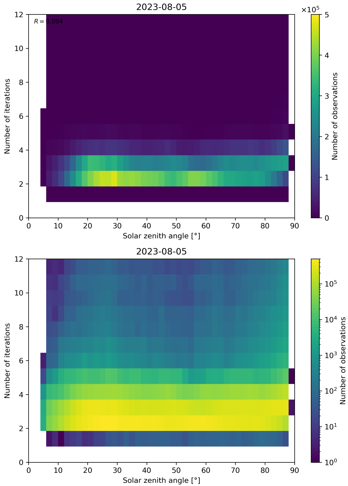
Figure 125: Scatter density plot of “Solar zenith angle” against “Number of iterations” for 2023-08-04 to 2023-08-06.
