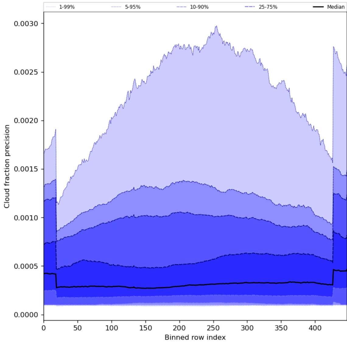
Figure 50: Along track statistics of “Cloud fraction precision” for 2023-08-04 to 2023-08-06
