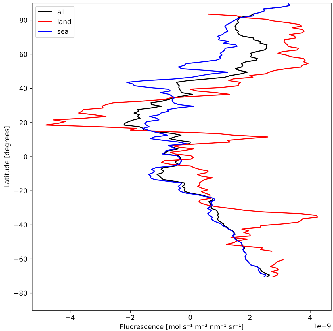
Figure 23: Zonal average of “Fluorescence” for 2023-08-04 to 2023-08-06.
