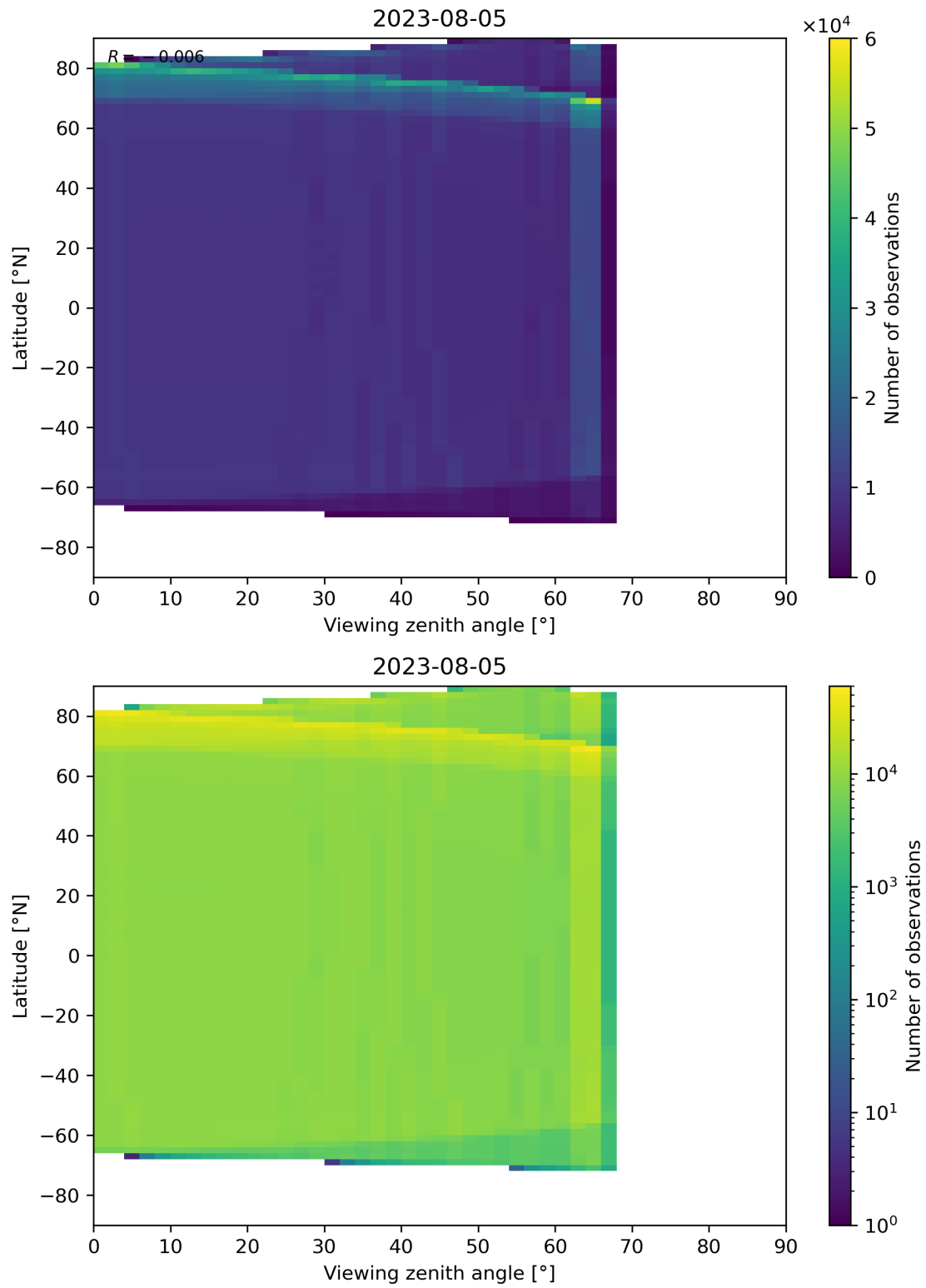
Figure 135: Scatter density plot of “Viewing zenith angle” against “Latitude” for 2023-08-04 to 2023-08-06.
