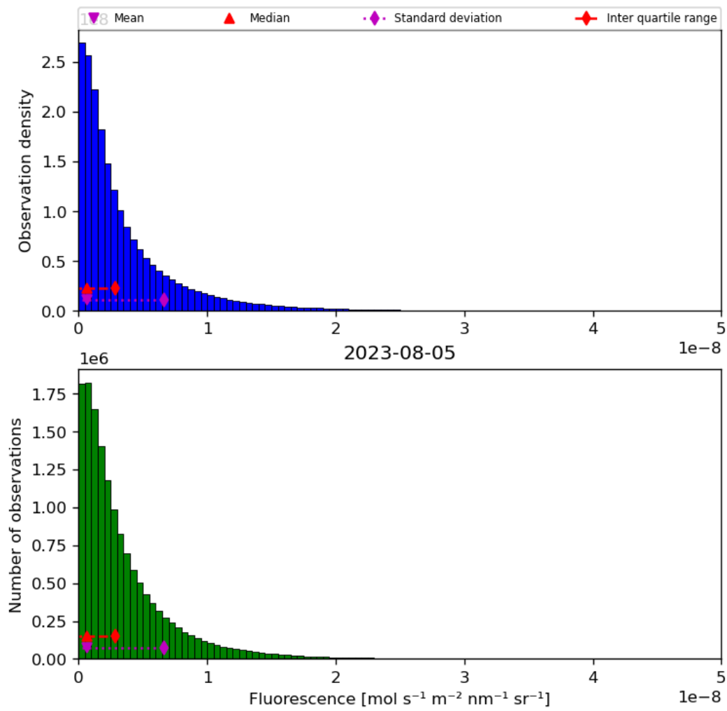
Figure 40: Histogram of “Fluorescence” for 2023-08-04 to 2023-08-06
