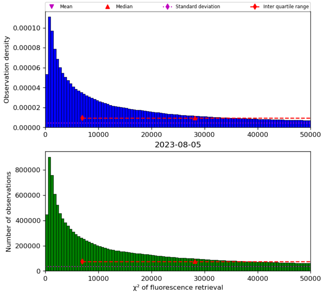
Figure 42: Histogram of “ \chi^2 of fluorescence retrieval” for 2023-08-04 to 2023-08-06
