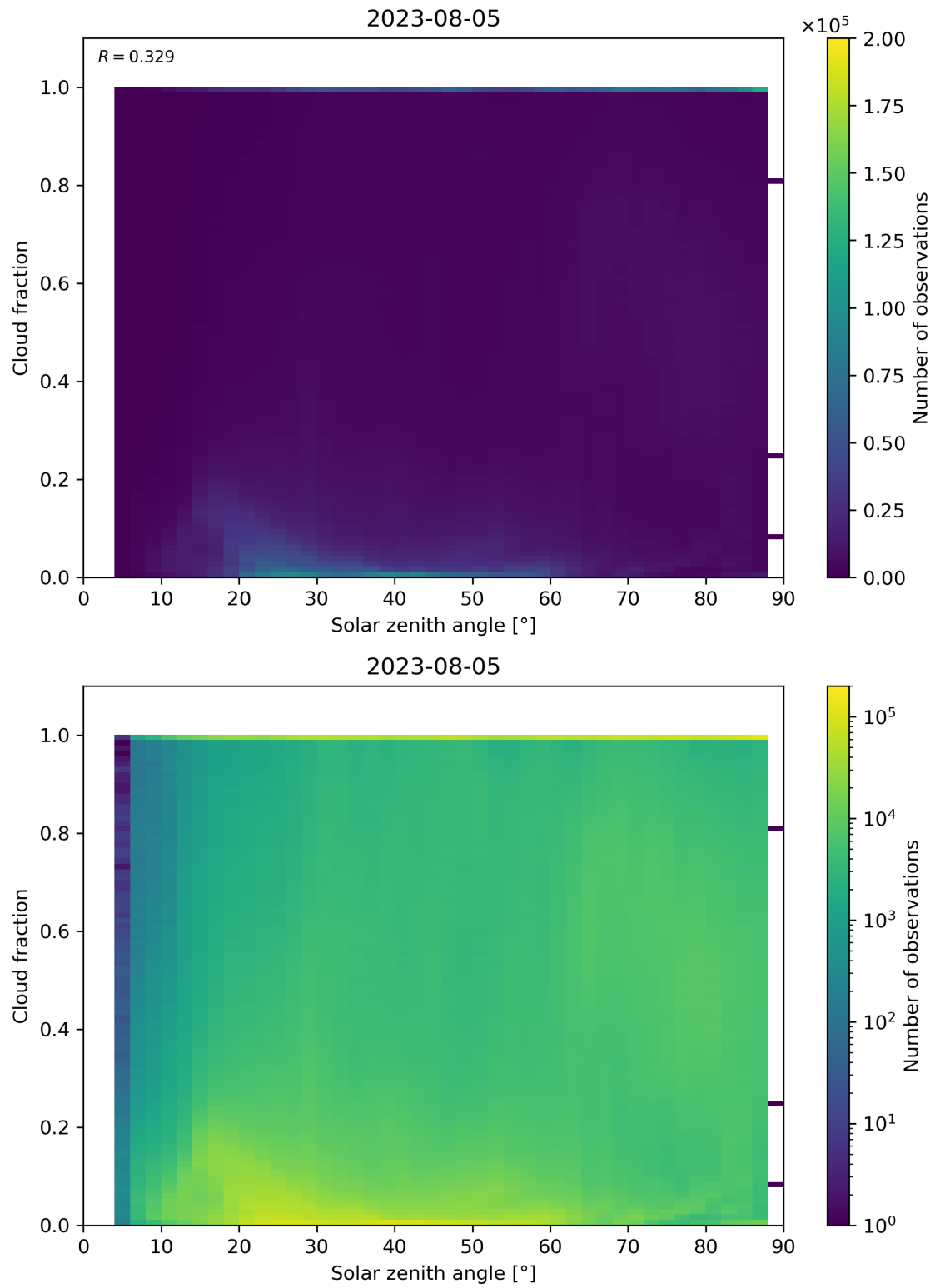
Figure 121: Scatter density plot of “Solar zenith angle” against “Cloud fraction” for 2023-08-04 to 2023-08-06.
