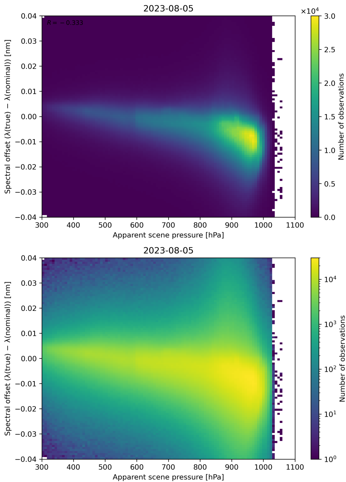
Figure 68: Scatter density plot of “Apparent scene pressure” against “Spectral offset ( \lambda(\text{true}) - \lambda(\text{nominal}) )” for 2023-08-04 to 2023-08-06.
