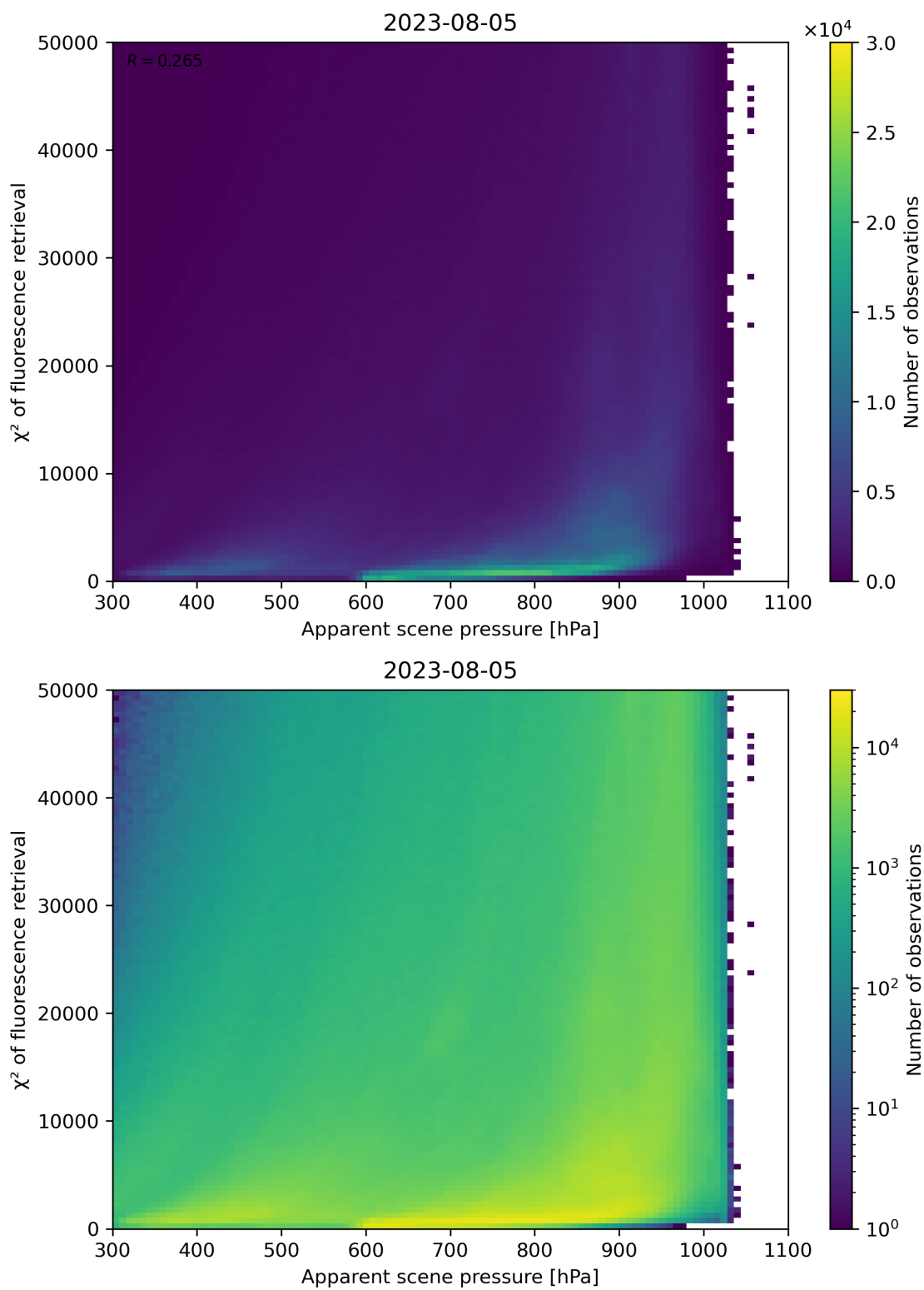
Figure 64: Scatter density plot of “Apparent scene pressure” against “ \chi^2 of fluorescence retrieval” for 2023-08-04 to 2023-08-06.
