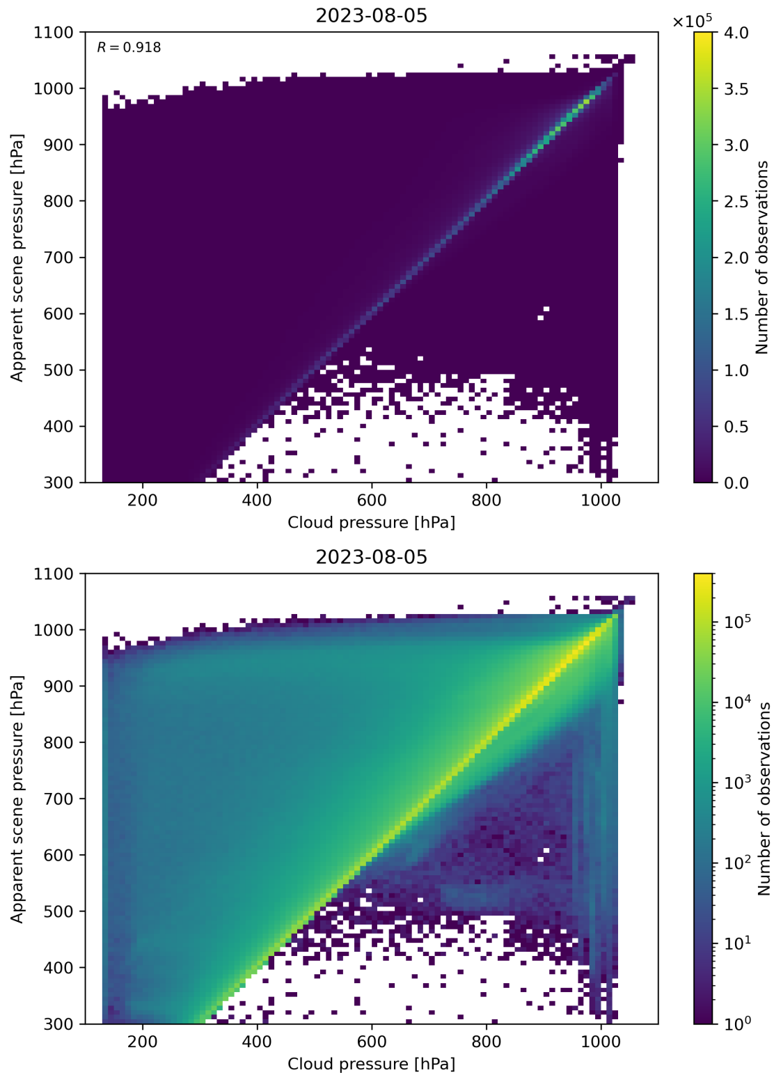
Figure 84: Scatter density plot of “Cloud pressure” against “Apparent scene pressure” for 2023-08-04 to 2023-08-06.
