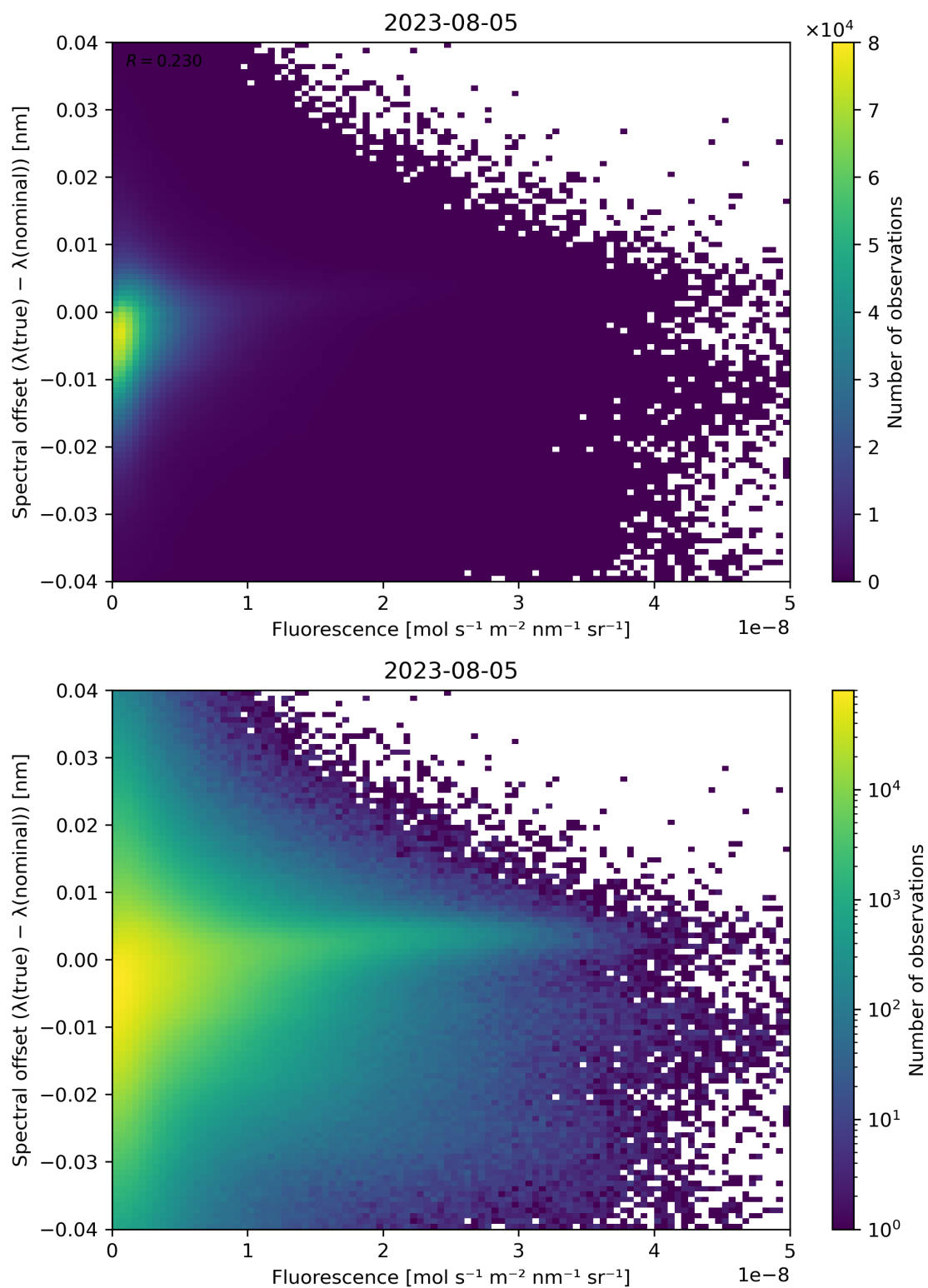
Figure 95: Scatter density plot of “Fluorescence” against “Spectral offset ( \lambda(\text{true}) - \lambda(\text{nominal}) )” for 2023-08-04 to 2023-08-06.
