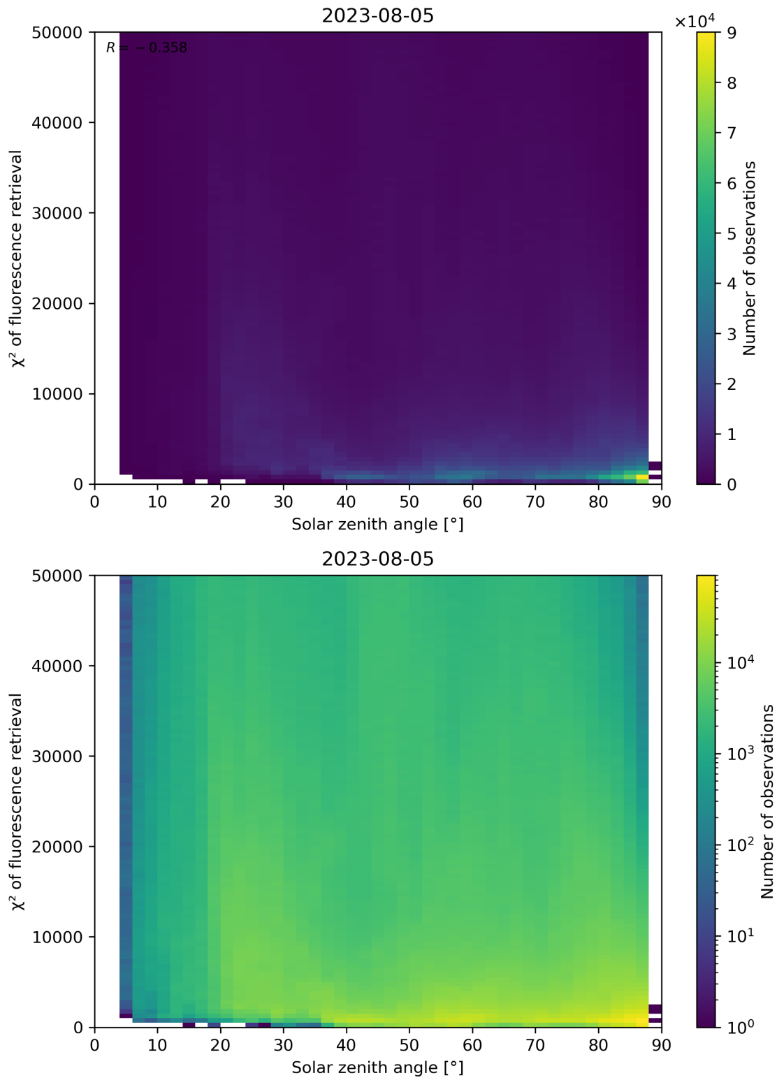
Figure 120: Scatter density plot of “Solar zenith angle” against “ \chi^2 of fluorescence retrieval” for 2023-08-04 to 2023-08-06.
