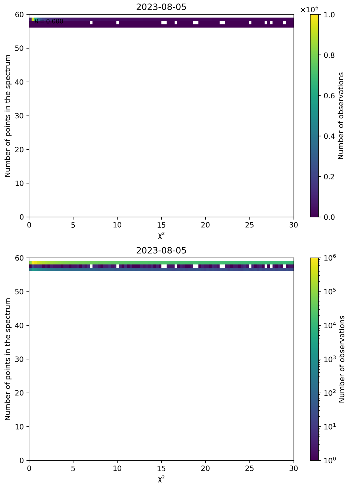
Figure 74: Scatter density plot of " \chi^2 " against "Number of points in the spectrum" for 2023-08-04 to 2023-08-06.
