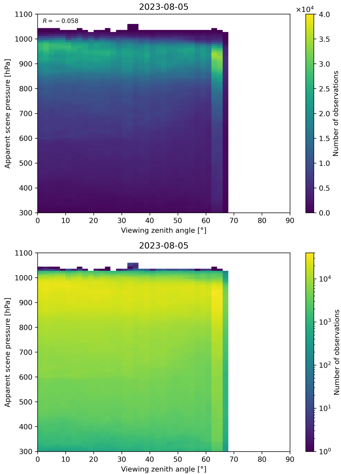
Figure 129: Scatter density plot of “Viewing zenith angle” against “Apparent scene pressure” for 2023-08-04 to 2023-08-06.
