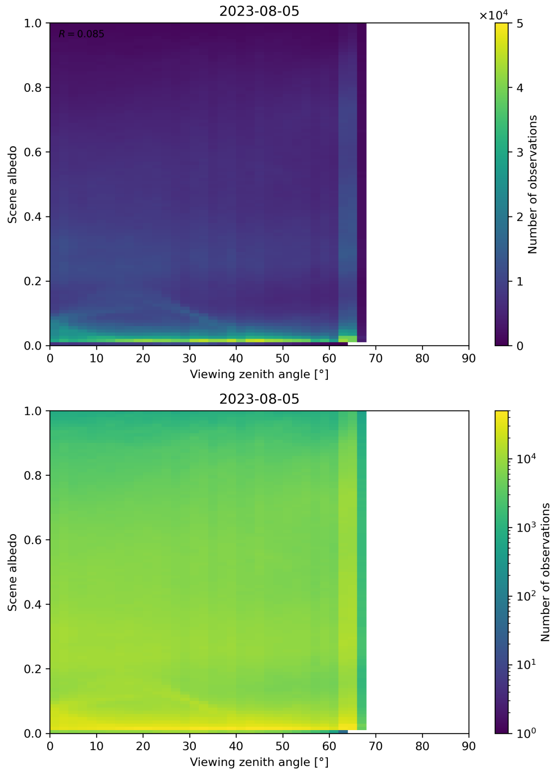
Figure 138: Scatter density plot of “Viewing zenith angle” against “Scene albedo” for 2023-08-04 to 2023-08-06.
