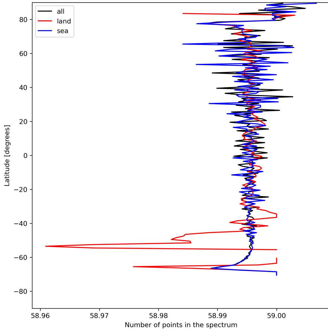
Figure 27: Zonal average of “Number of points in the spectrum” for 2023-08-04 to 2023-08-06.
