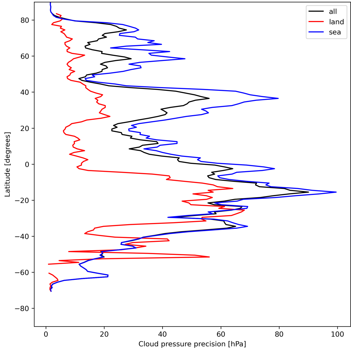
Figure 14: Zonal average of “Cloud pressure precision” for 2023-08-04 to 2023-08-06.
