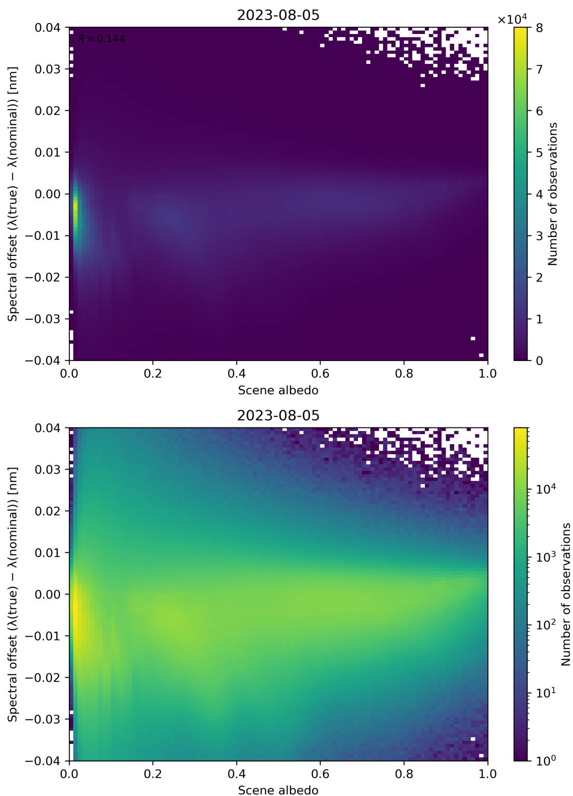
Figure 117: Scatter density plot of “Scene albedo” against “Spectral offset ( \lambda(\text{true}) - \lambda(\text{nominal}) )” for 2023-08-04 to 2023-08-06.
