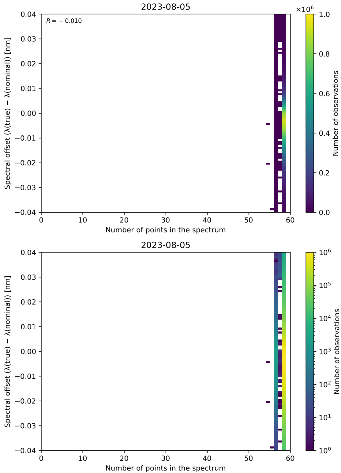
Figure 110: Scatter density plot of “Number of points in the spectrum” against “Spectral offset ( \lambda(\text{true}) - \lambda(\text{nominal}) )” for 2023-08-04 to 2023-08-06.
