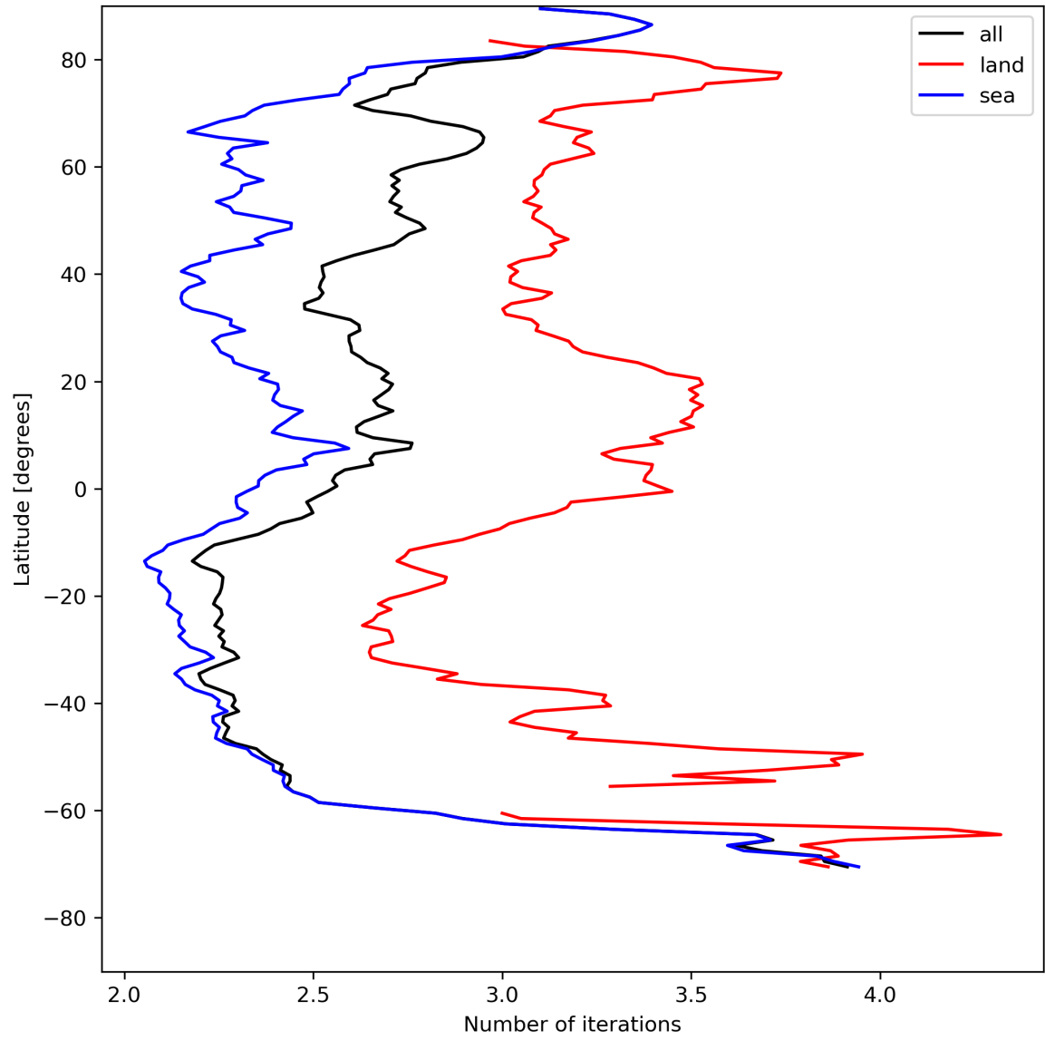
Figure 22: Zonal average of “Number of iterations” for 2023-08-04 to 2023-08-06.
