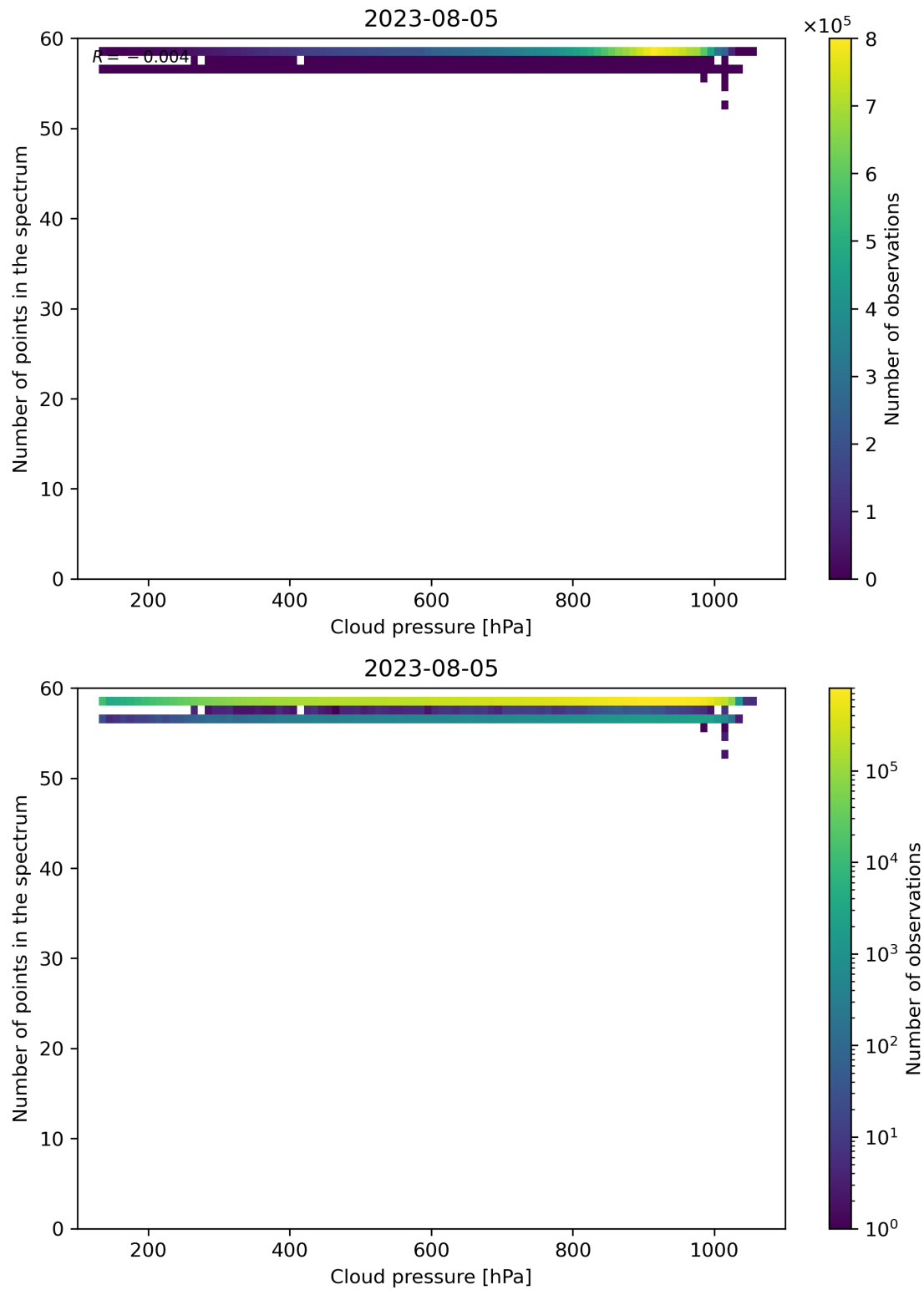
Figure 90: Scatter density plot of “Cloud pressure” against “Number of points in the spectrum” for 2023-08-04 to 2023-08-06.
