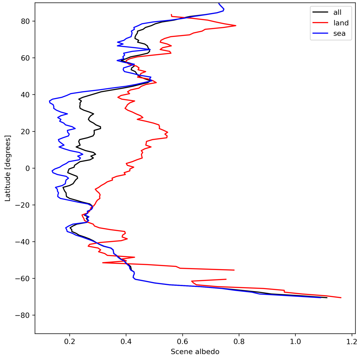
Figure 17: Zonal average of “Scene albedo” for 2023-08-04 to 2023-08-06.
