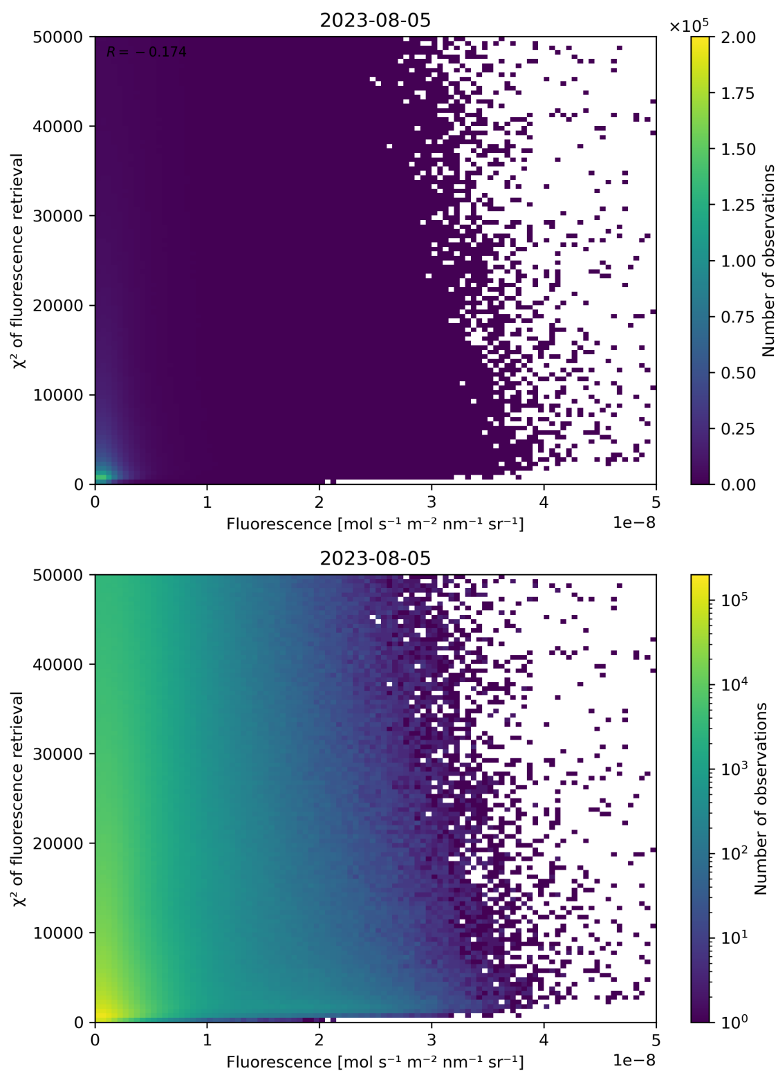
Figure 93: Scatter density plot of “Fluorescence” against “ \chi^2 of fluorescence retrieval” for 2023-08-04 to 2023-08-06.
