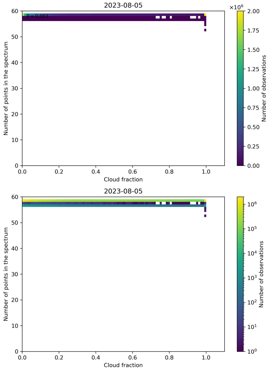
Figure 81: Scatter density plot of “Cloud fraction” against “Number of points in the spectrum” for 2023-08-04 to 2023-08-06.
