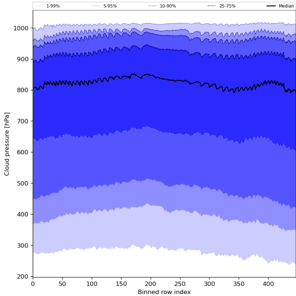
Figure 47: Along track statistics of “Cloud pressure” for 2023-08-04 to 2023-08-06
