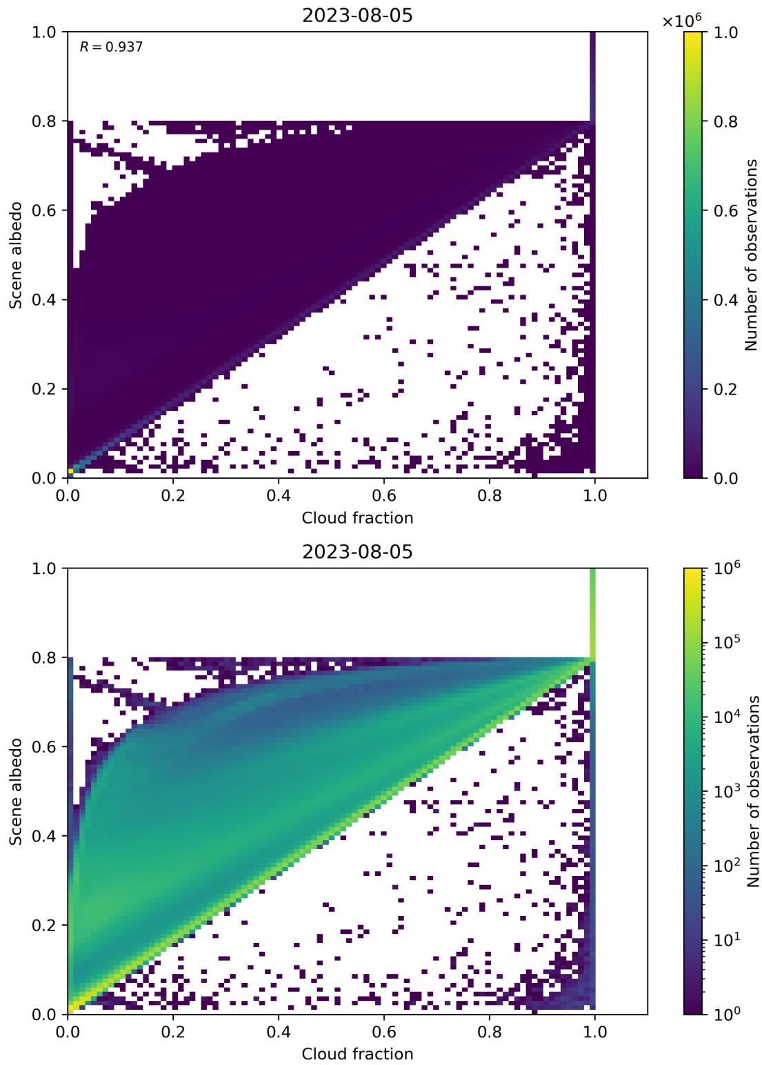
Figure 82: Scatter density plot of “Cloud fraction” against “Scene albedo” for 2023-08-04 to 2023-08-06.
