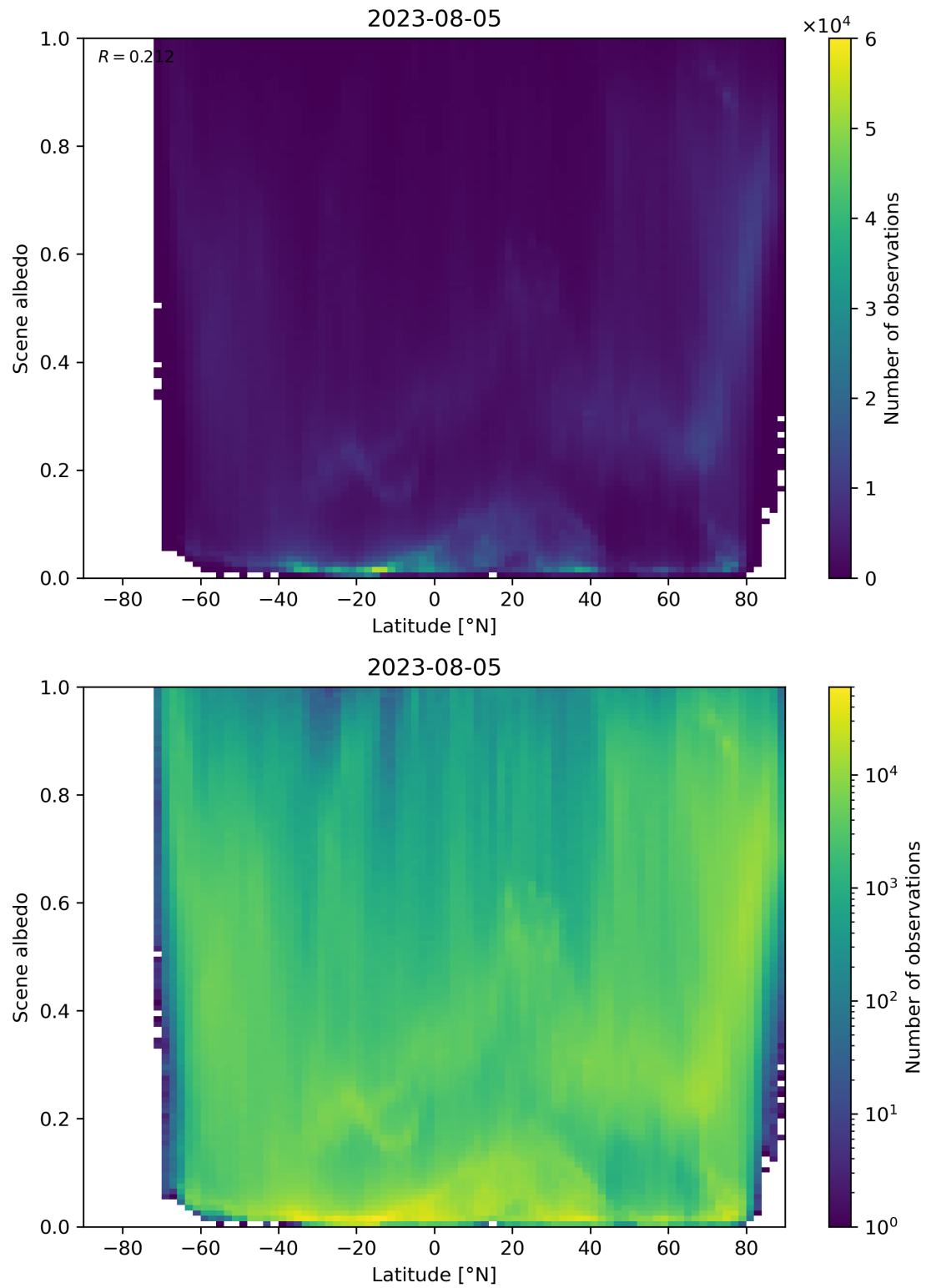
Figure 104: Scatter density plot of “Latitude” against “Scene albedo” for 2023-08-04 to 2023-08-06.
