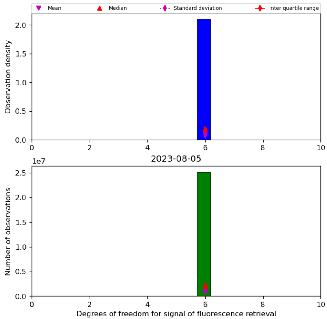
Figure 43: Histogram of “Degrees of freedom for signal of fluorescence retrieval” for 2023-08-04 to 2023-08-06
