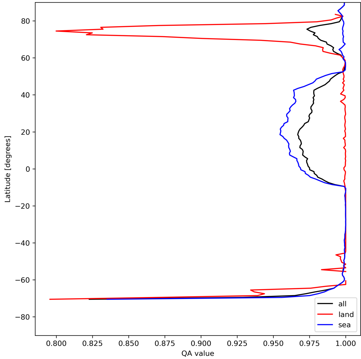
Figure 12: Zonal average of “QA value” for 2023-08-04 to 2023-08-06.
