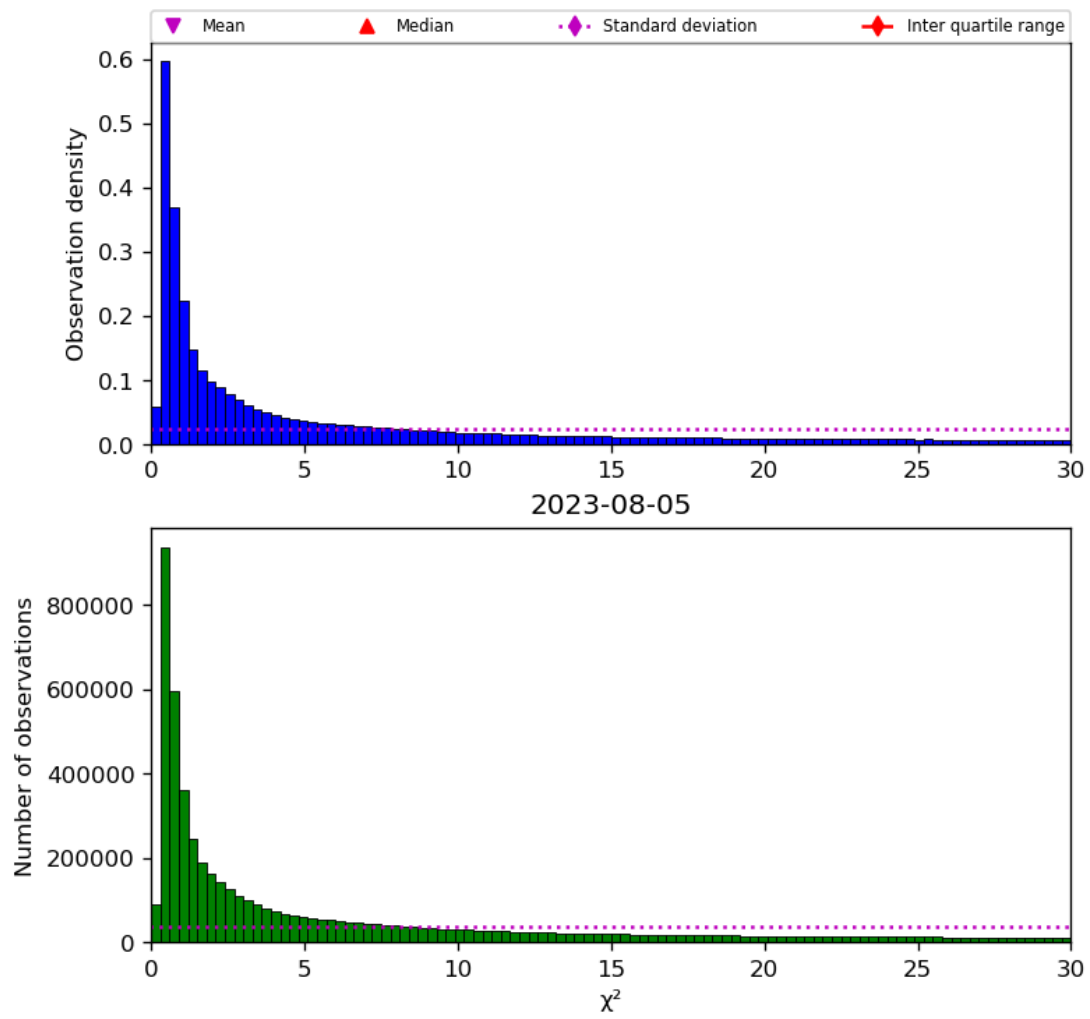
Figure 38: Histogram of “ \chi^2 ” for 2023-08-04 to 2023-08-06
