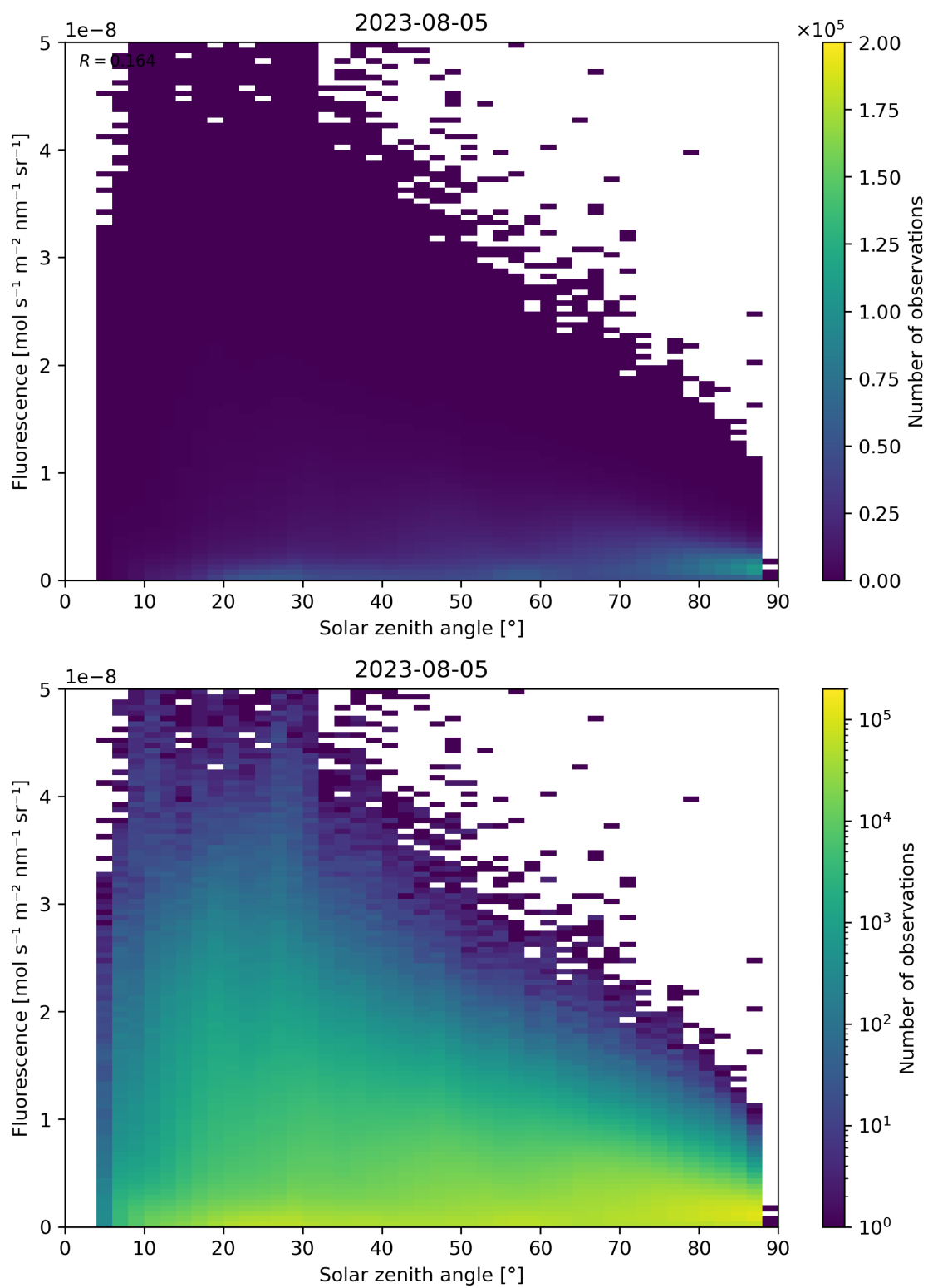
Figure 123: Scatter density plot of “Solar zenith angle” against “Fluorescence” for 2023-08-04 to 2023-08-06.
