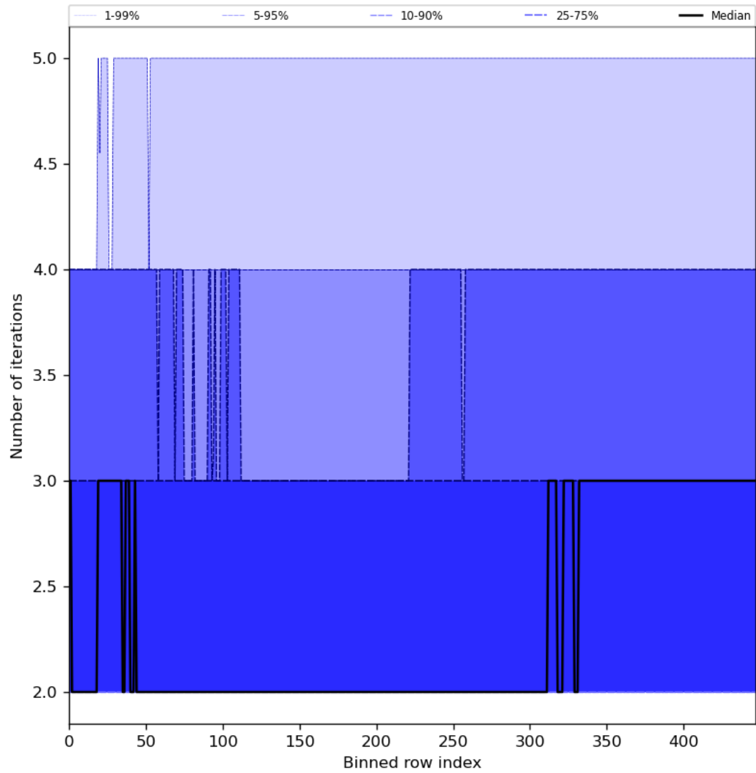
Figure 56: Along track statistics of “Number of iterations” for 2023-08-04 to 2023-08-06
