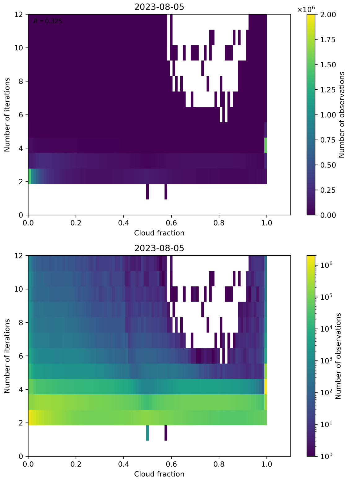
Figure 80: Scatter density plot of “Cloud fraction” against “Number of iterations” for 2023-08-04 to 2023-08-06.
