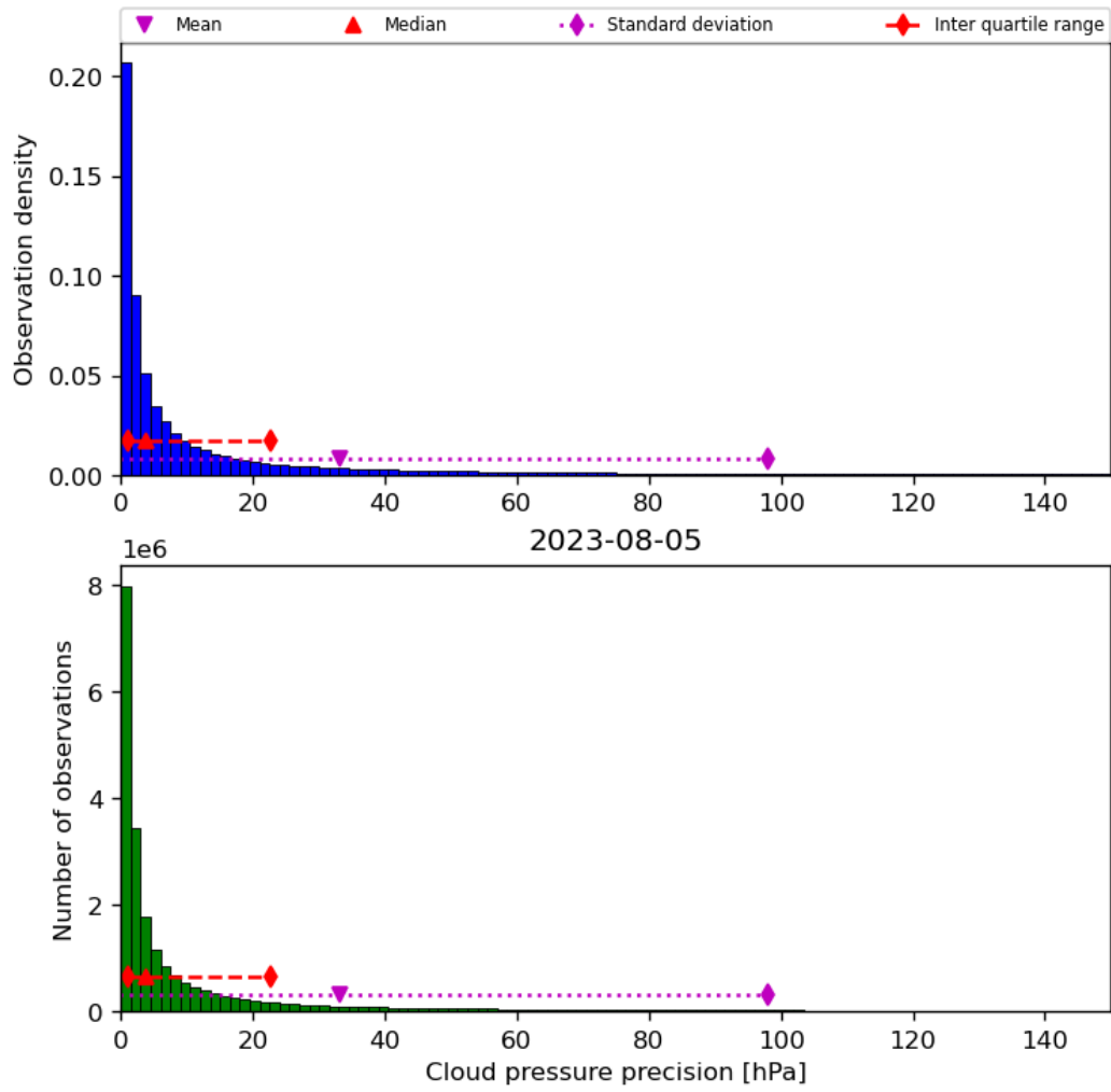
Figure 31: Histogram of “Cloud pressure precision” for 2023-08-04 to 2023-08-06
