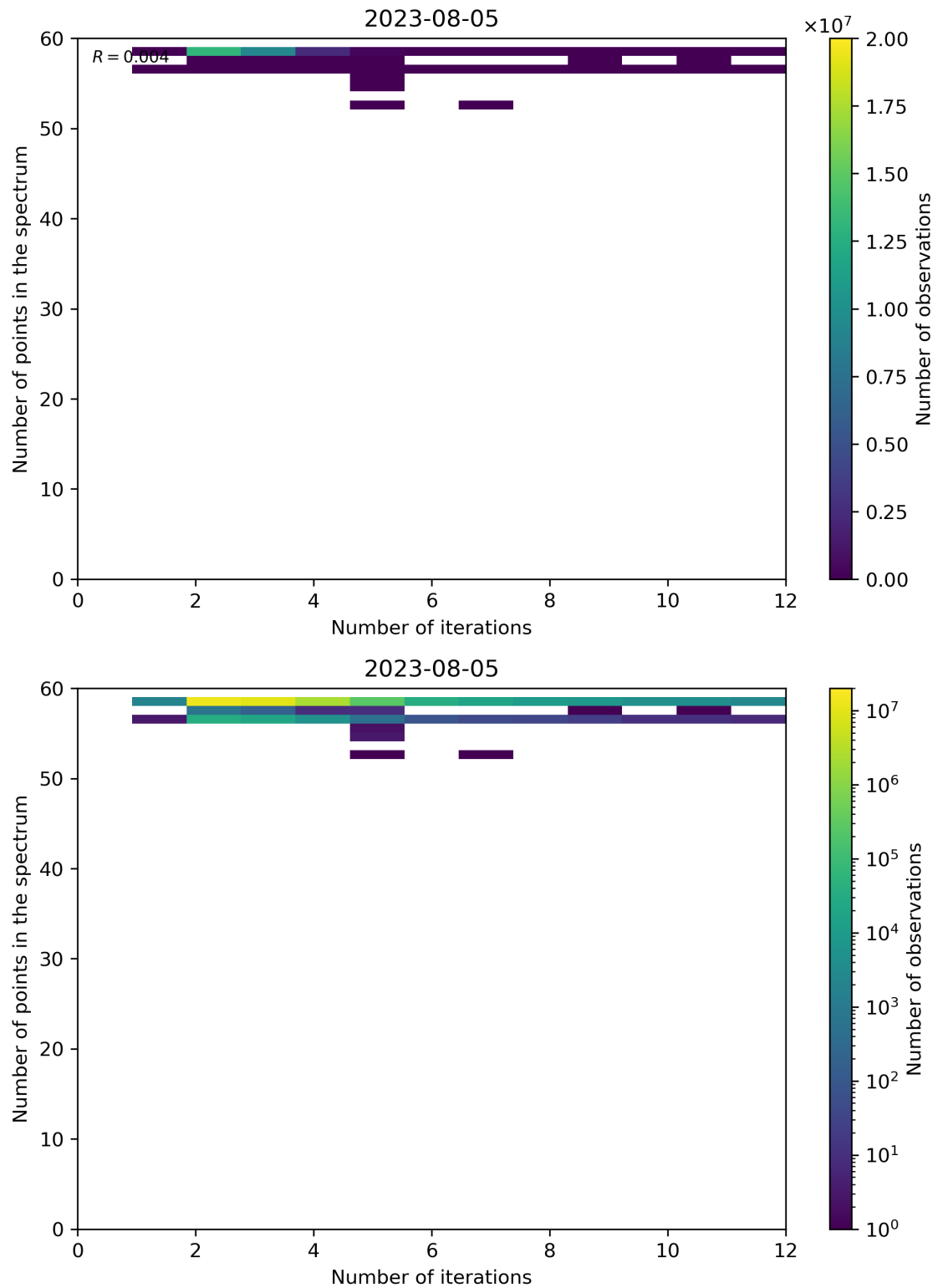
Figure 108: Scatter density plot of “Number of iterations” against “Number of points in the spectrum” for 2023-08-04 to 2023-08-06.
