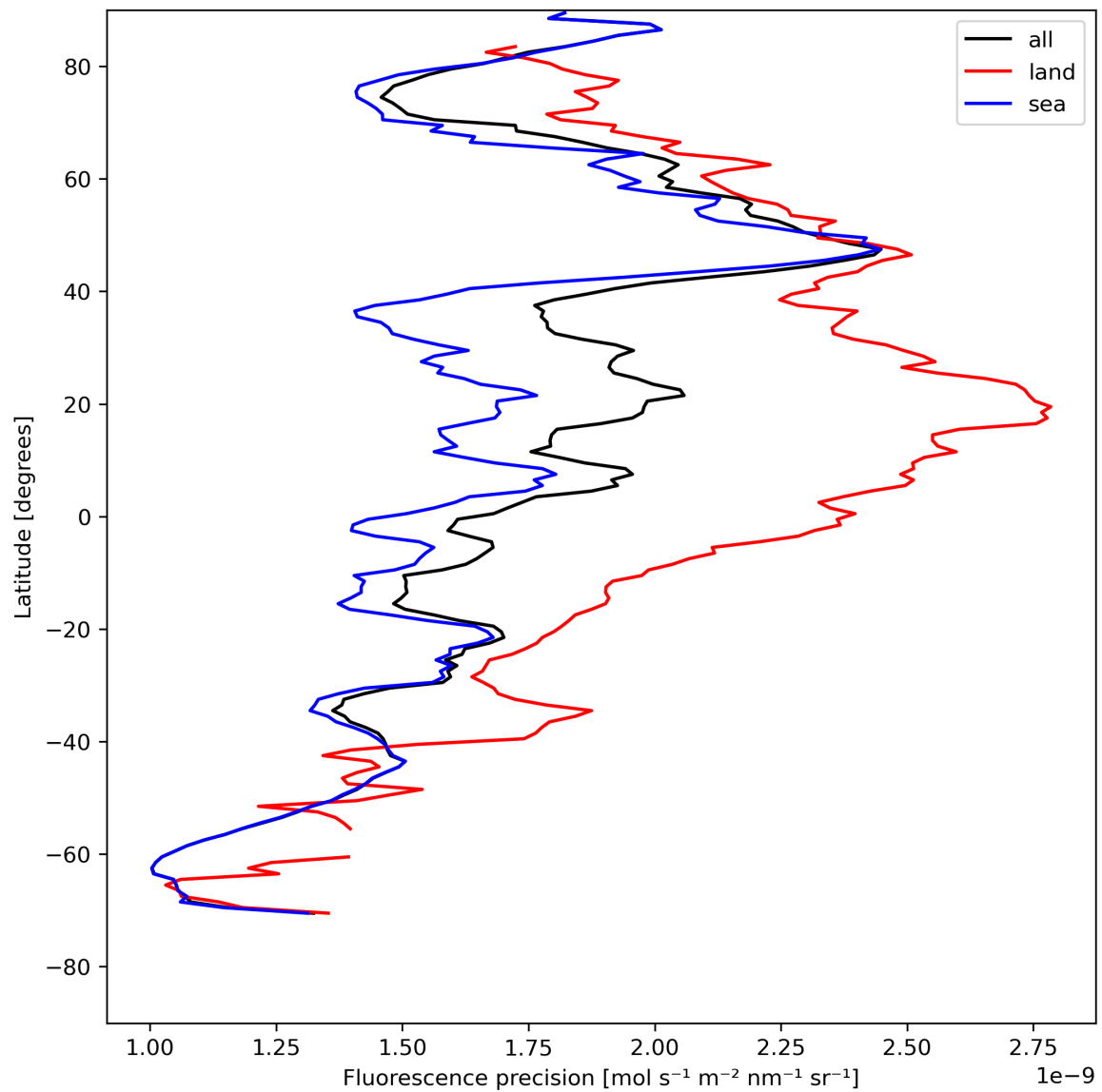
Figure 24: Zonal average of “Fluorescence precision” for 2023-08-04 to 2023-08-06.
