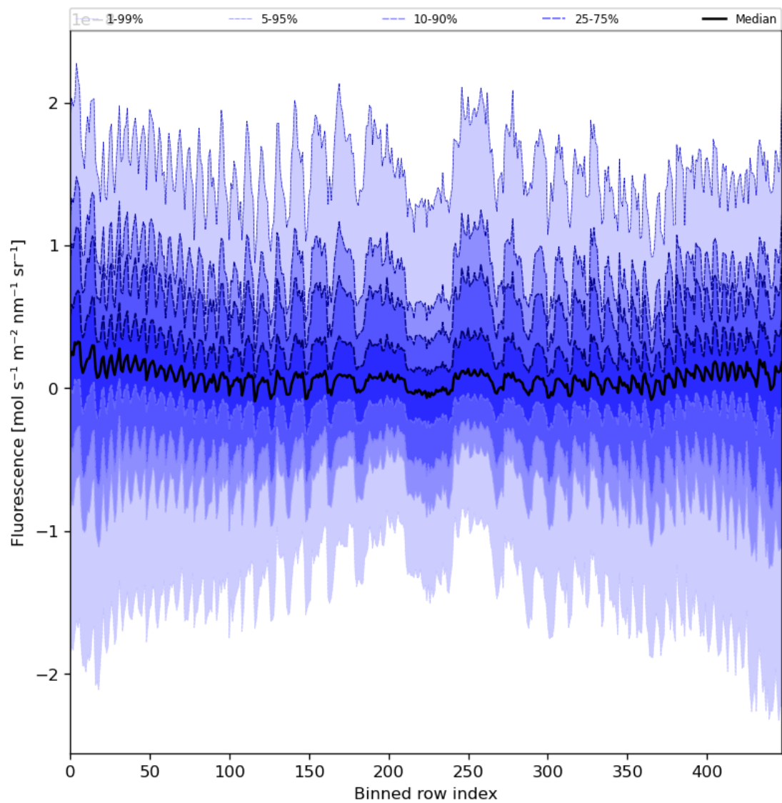
Figure 57: Along track statistics of “Fluorescence” for 2023-08-04 to 2023-08-06
