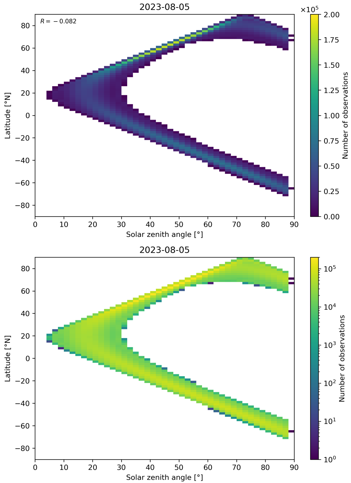
Figure 124: Scatter density plot of “Solar zenith angle” against “Latitude” for 2023-08-04 to 2023-08-06.
