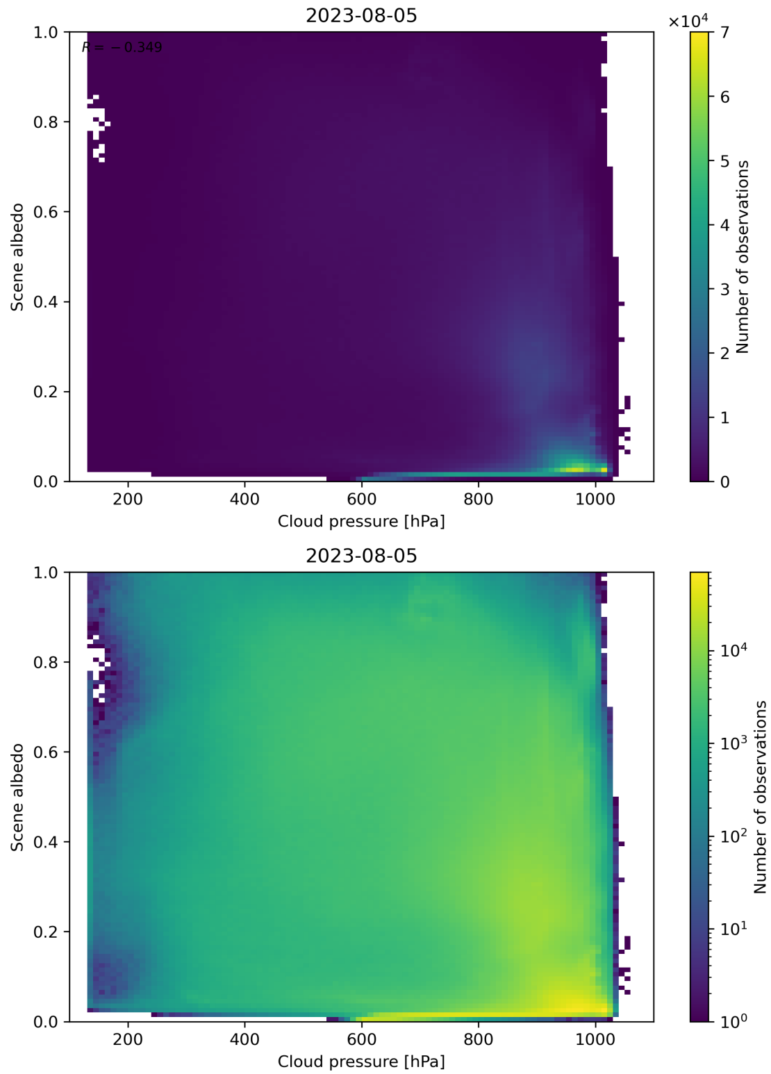
Figure 91: Scatter density plot of “Cloud pressure” against “Scene albedo” for 2023-08-04 to 2023-08-06.
