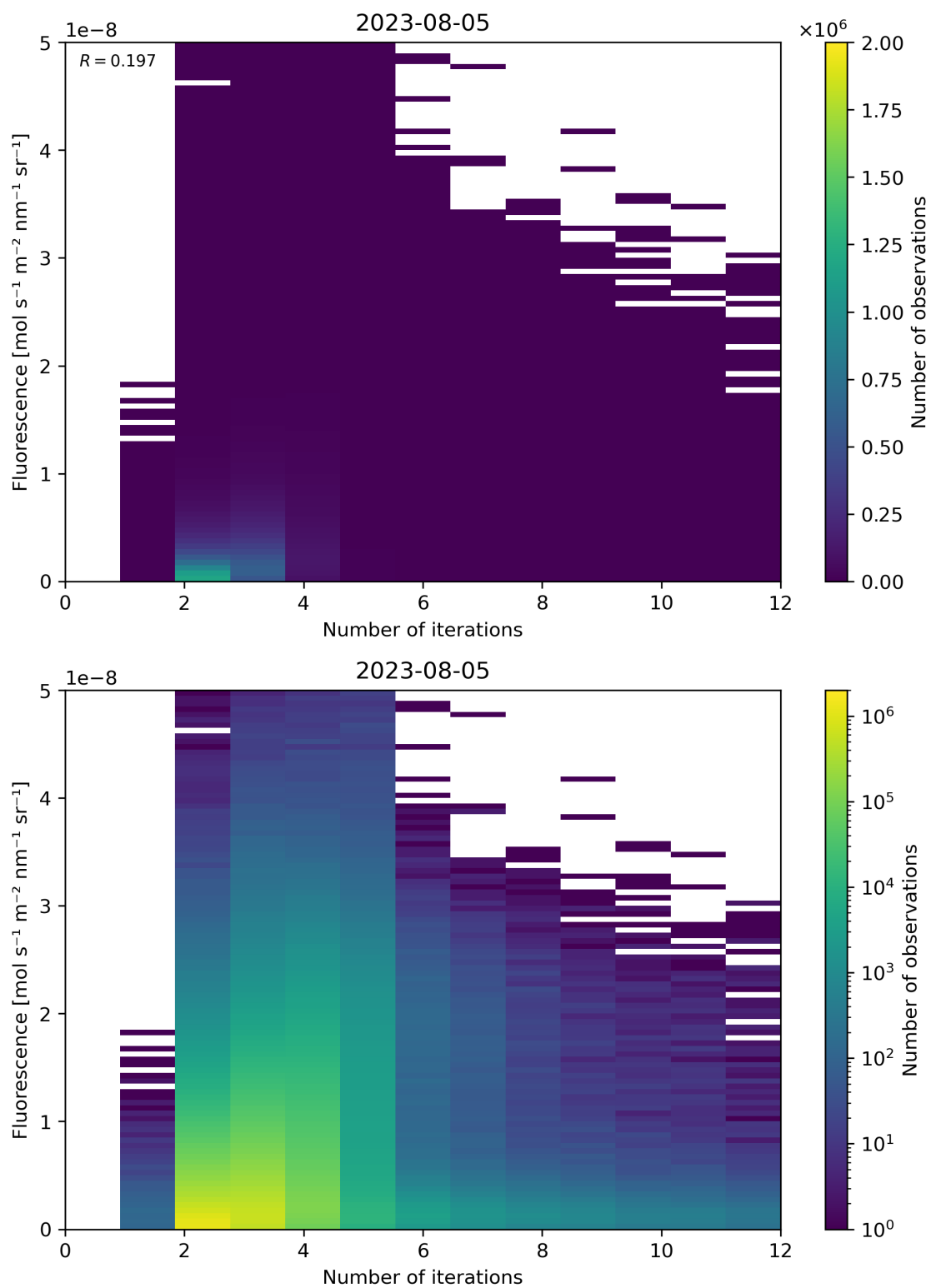
Figure 107: Scatter density plot of “Number of iterations” against “Fluorescence” for 2023-08-04 to 2023-08-06.
