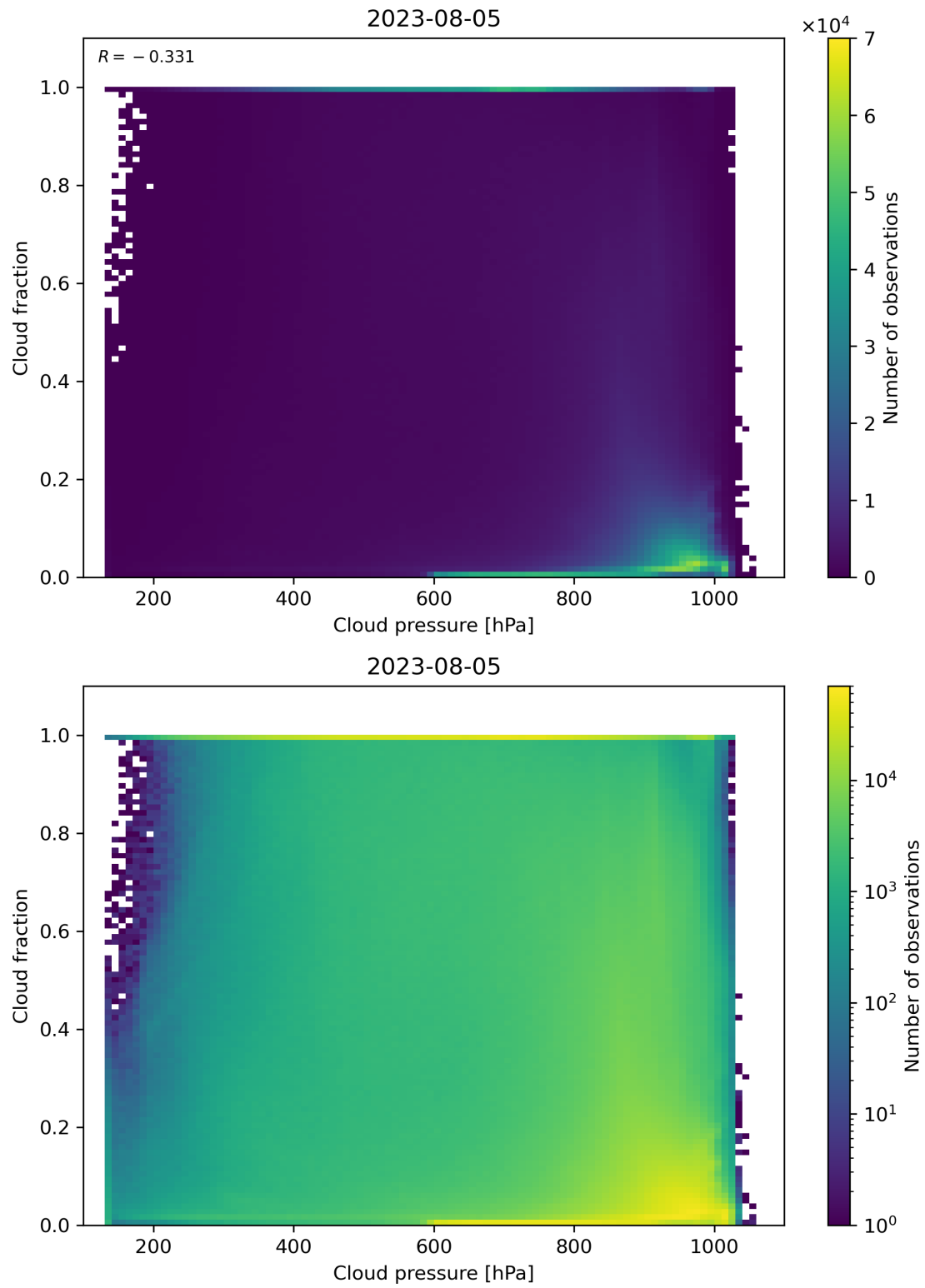
Figure 87: Scatter density plot of “Cloud pressure” against “Cloud fraction” for 2023-08-04 to 2023-08-06.
