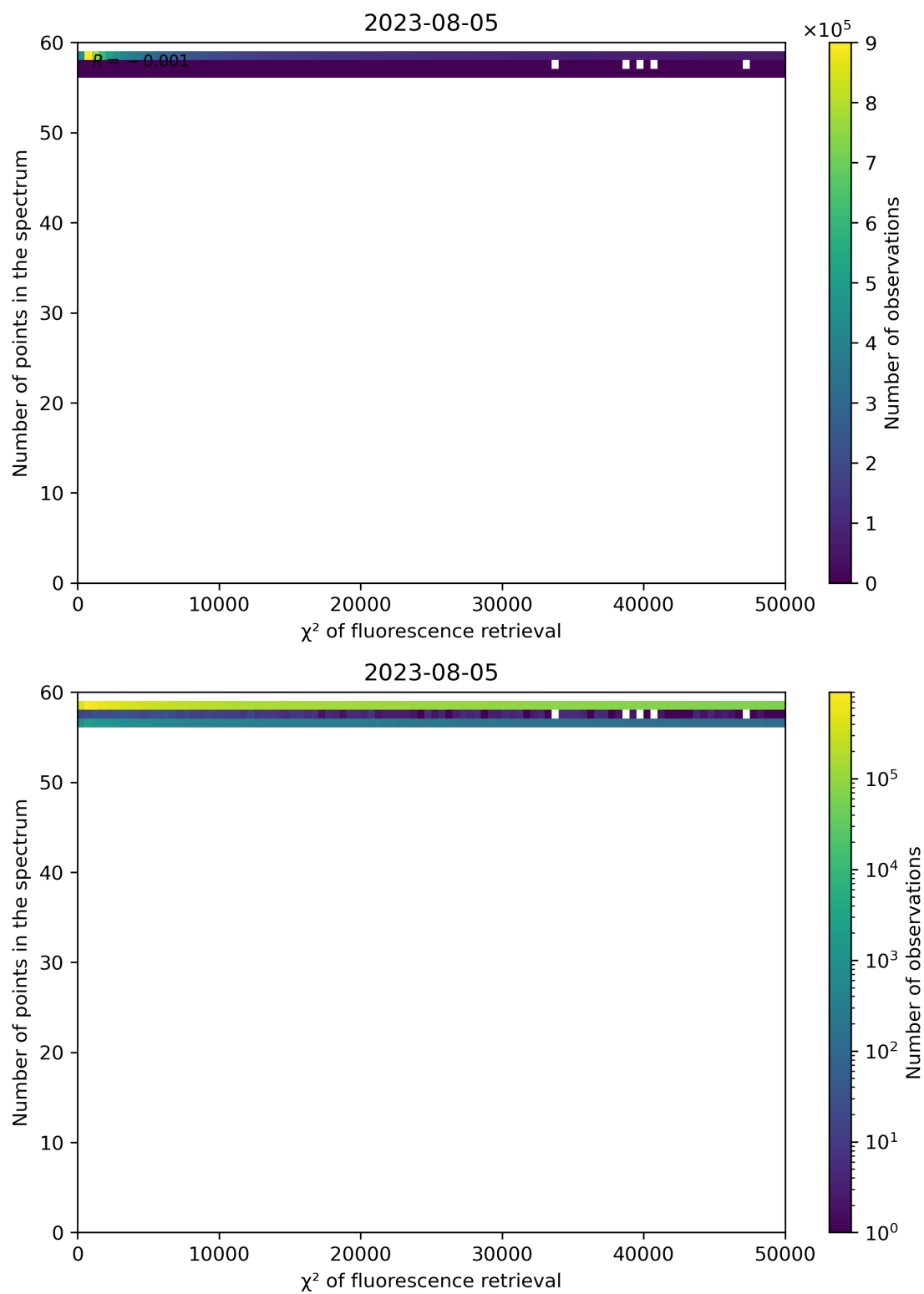
Figure 71: Scatter density plot of " \chi^2 of fluorescence retrieval" against "Number of points in the spectrum" for 2023-08-04 to 2023-08-06.
