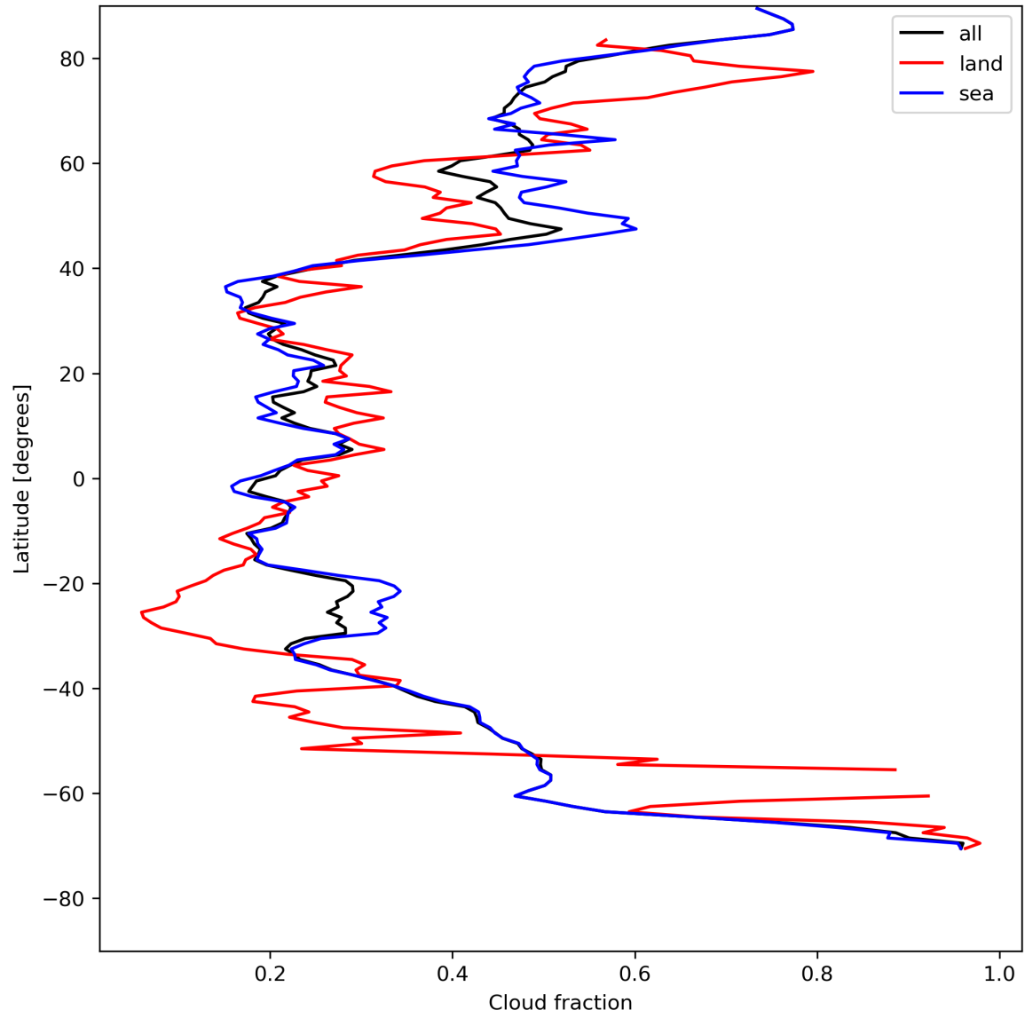
Figure 15: Zonal average of “Cloud fraction” for 2023-08-04 to 2023-08-06.
