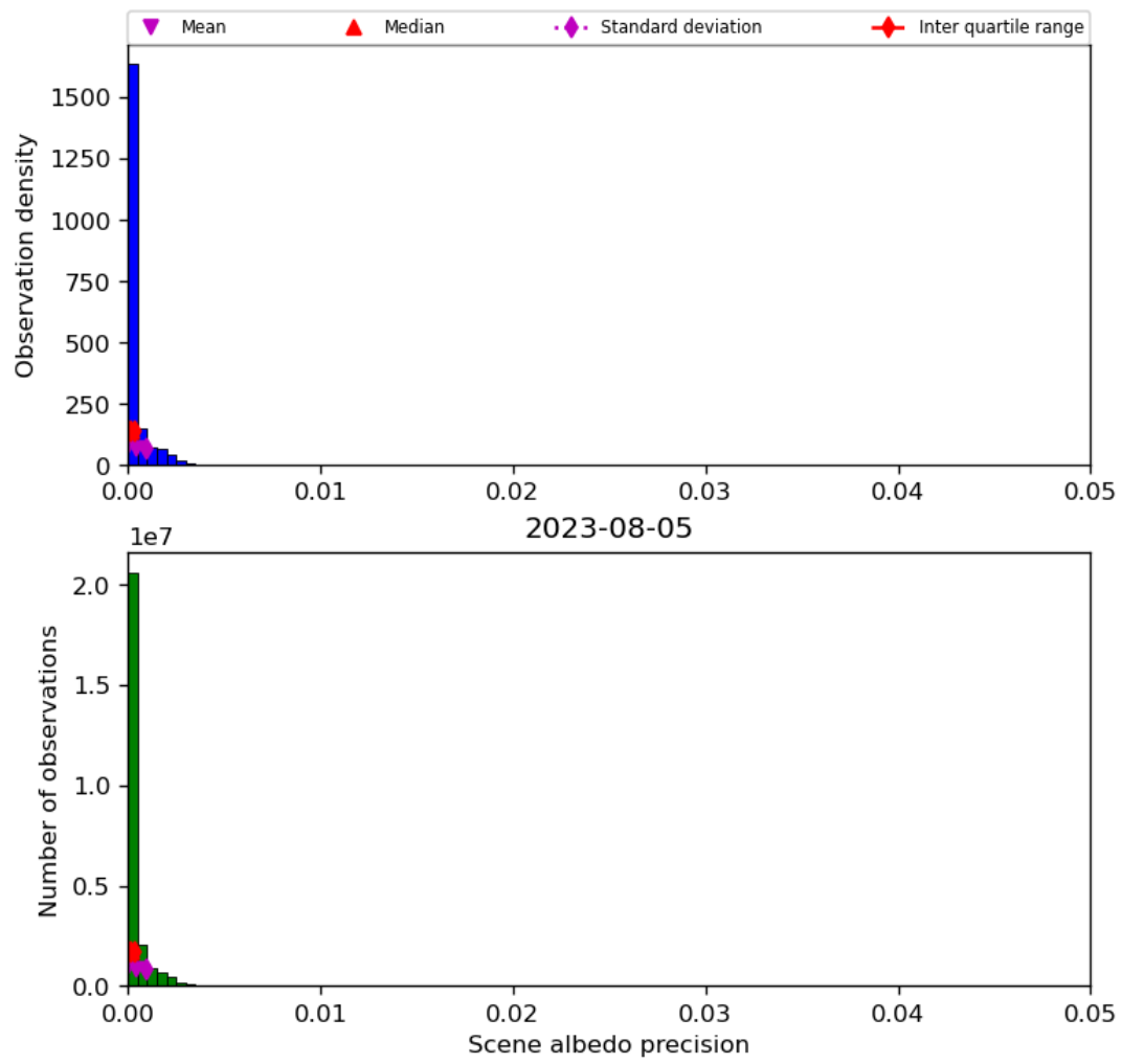
Figure 35: Histogram of “Scene albedo precision” for 2023-08-04 to 2023-08-06
