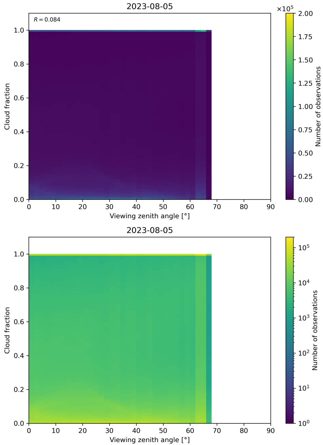
Figure 132: Scatter density plot of “Viewing zenith angle” against “Cloud fraction” for 2023-08-04 to 2023-08-06.
