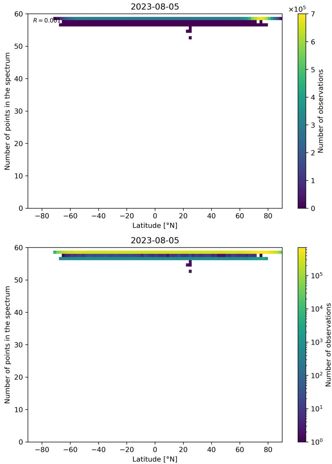
Figure 103: Scatter density plot of “Latitude” against “Number of points in the spectrum” for 2023-08-04 to 2023-08-06.
