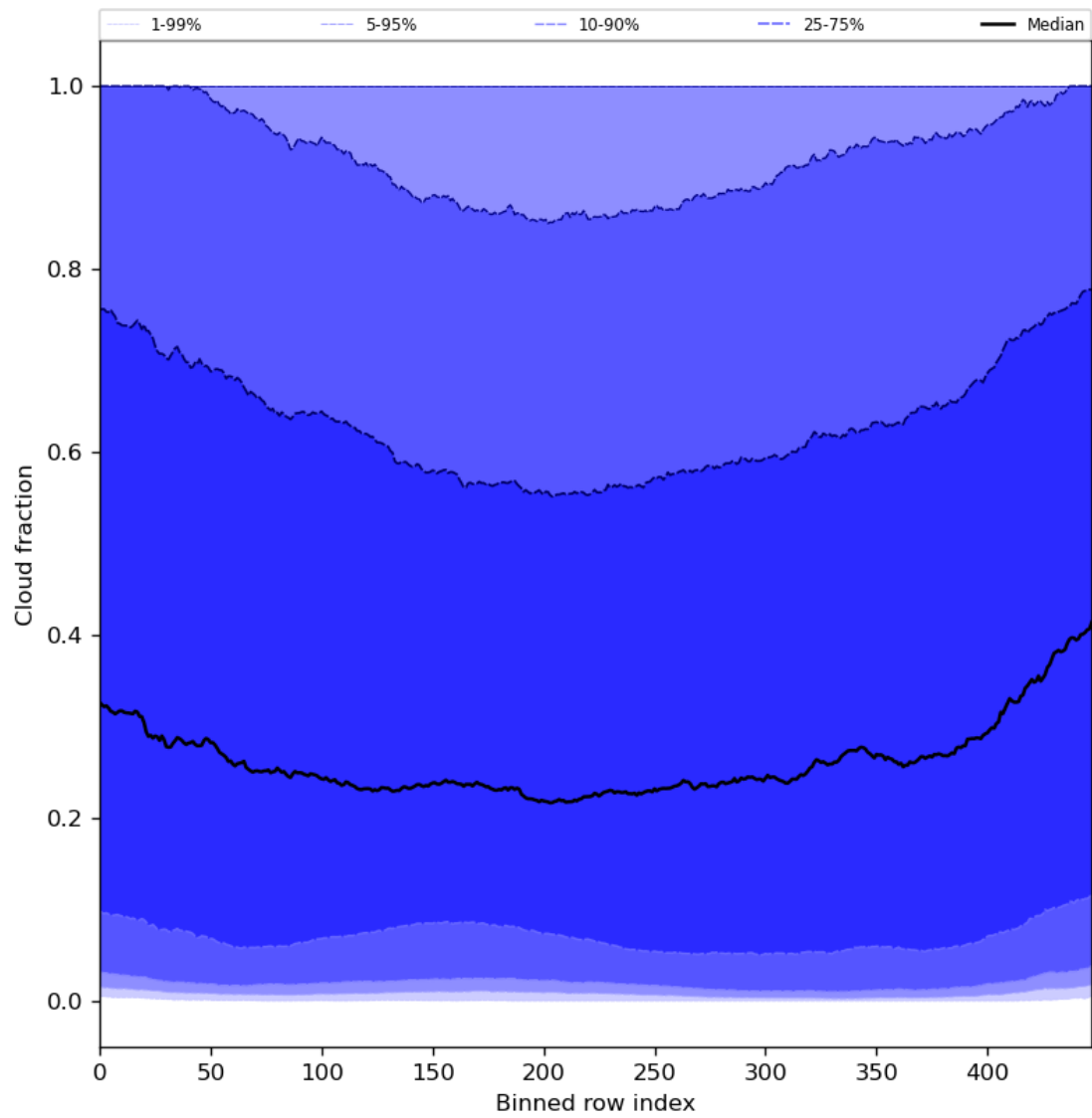
Figure 49: Along track statistics of “Cloud fraction” for 2023-08-04 to 2023-08-06
