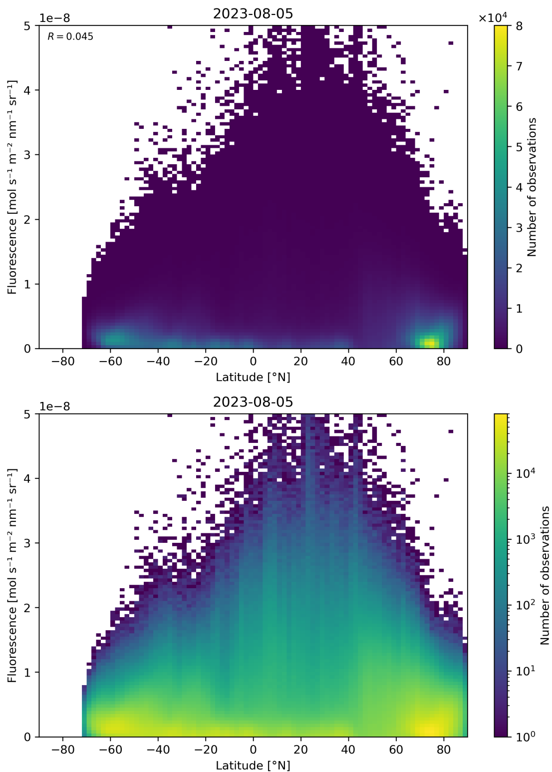
Figure 101: Scatter density plot of “Latitude” against “Fluorescence” for 2023-08-04 to 2023-08-06.
