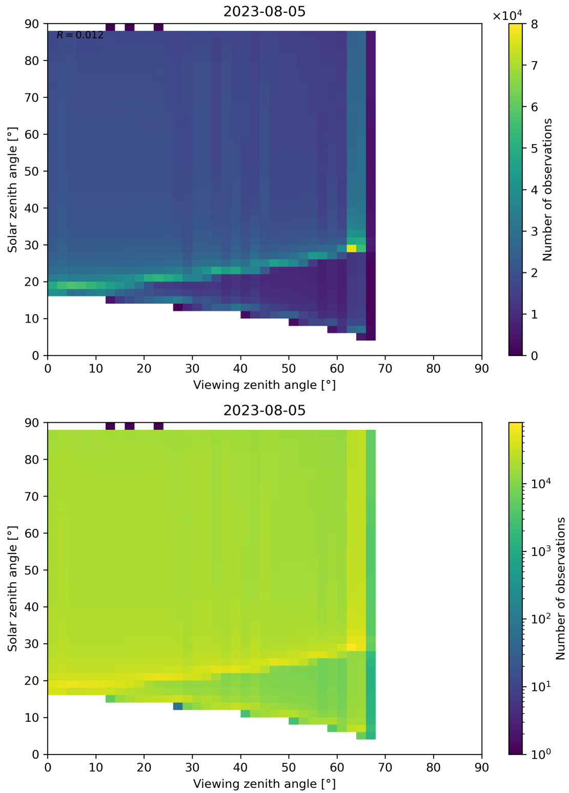
Figure 139: Scatter density plot of “Viewing zenith angle” against “Solar zenith angle” for 2023-08-04 to 2023-08-06.
