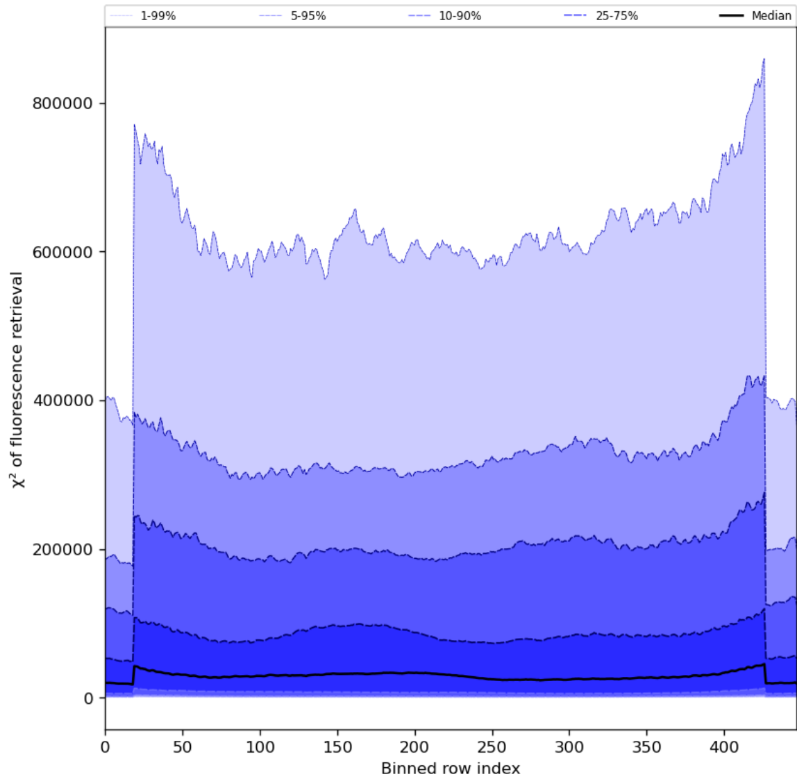
Figure 59: Along track statistics of “ \chi^2 of fluorescence retrieval” for 2023-08-04 to 2023-08-06
