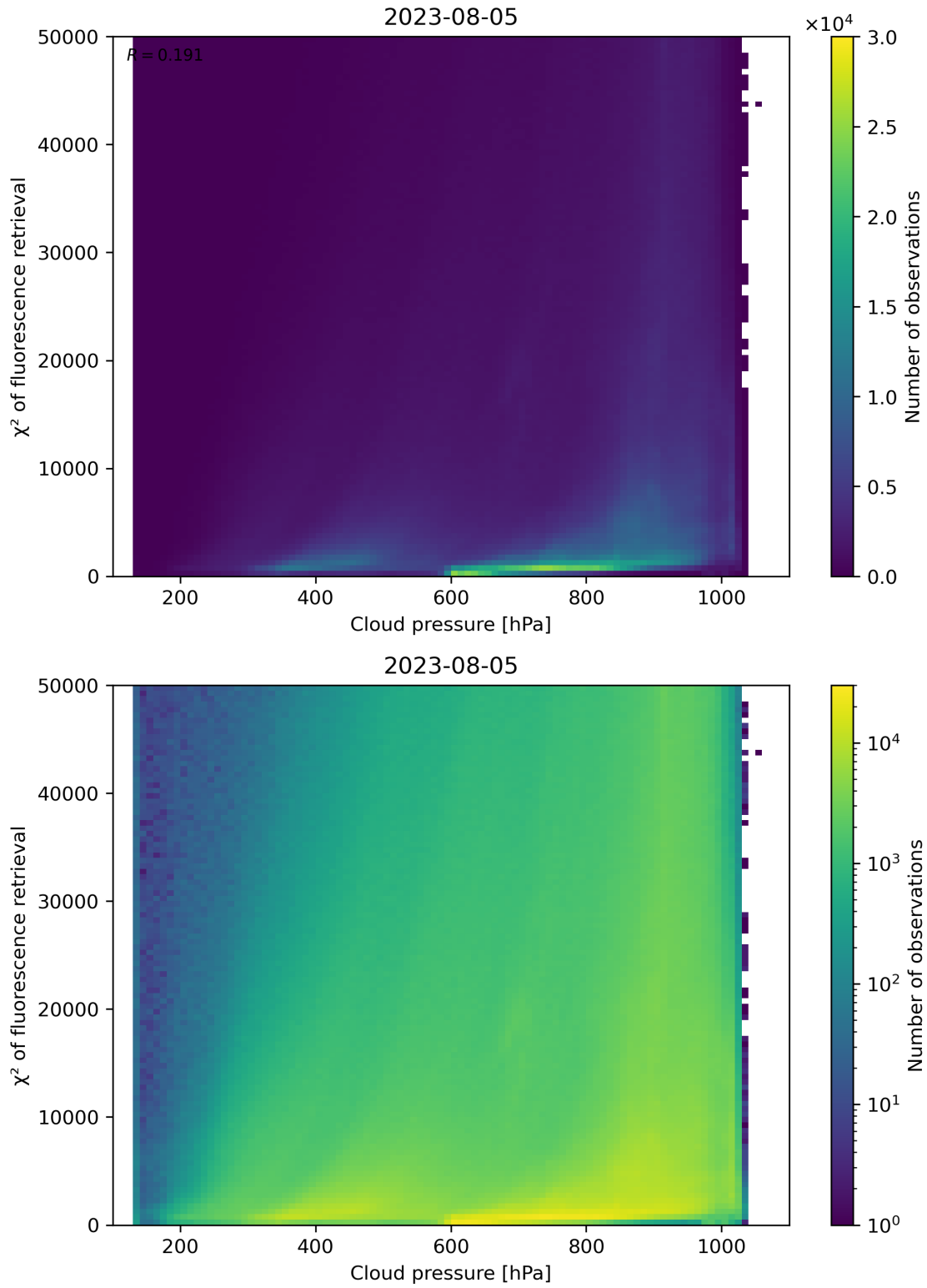
Figure 86: Scatter density plot of “Cloud pressure” against “ \chi^2 of fluorescence retrieval” for 2023-08-04 to 2023-08-06.
