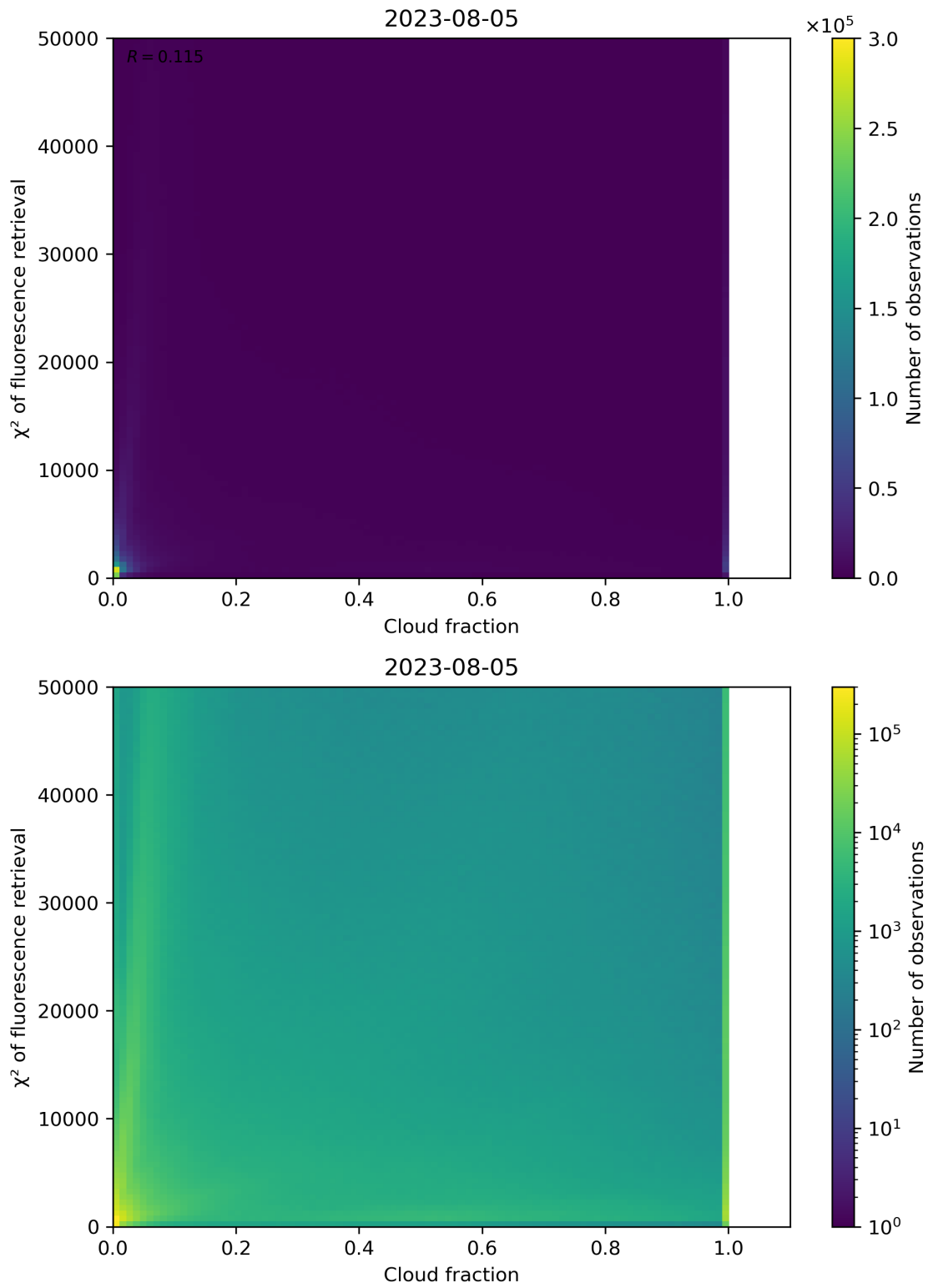
Figure 78: Scatter density plot of “Cloud fraction” against “ \chi^2 of fluorescence retrieval” for 2023-08-04 to 2023-08-06.
