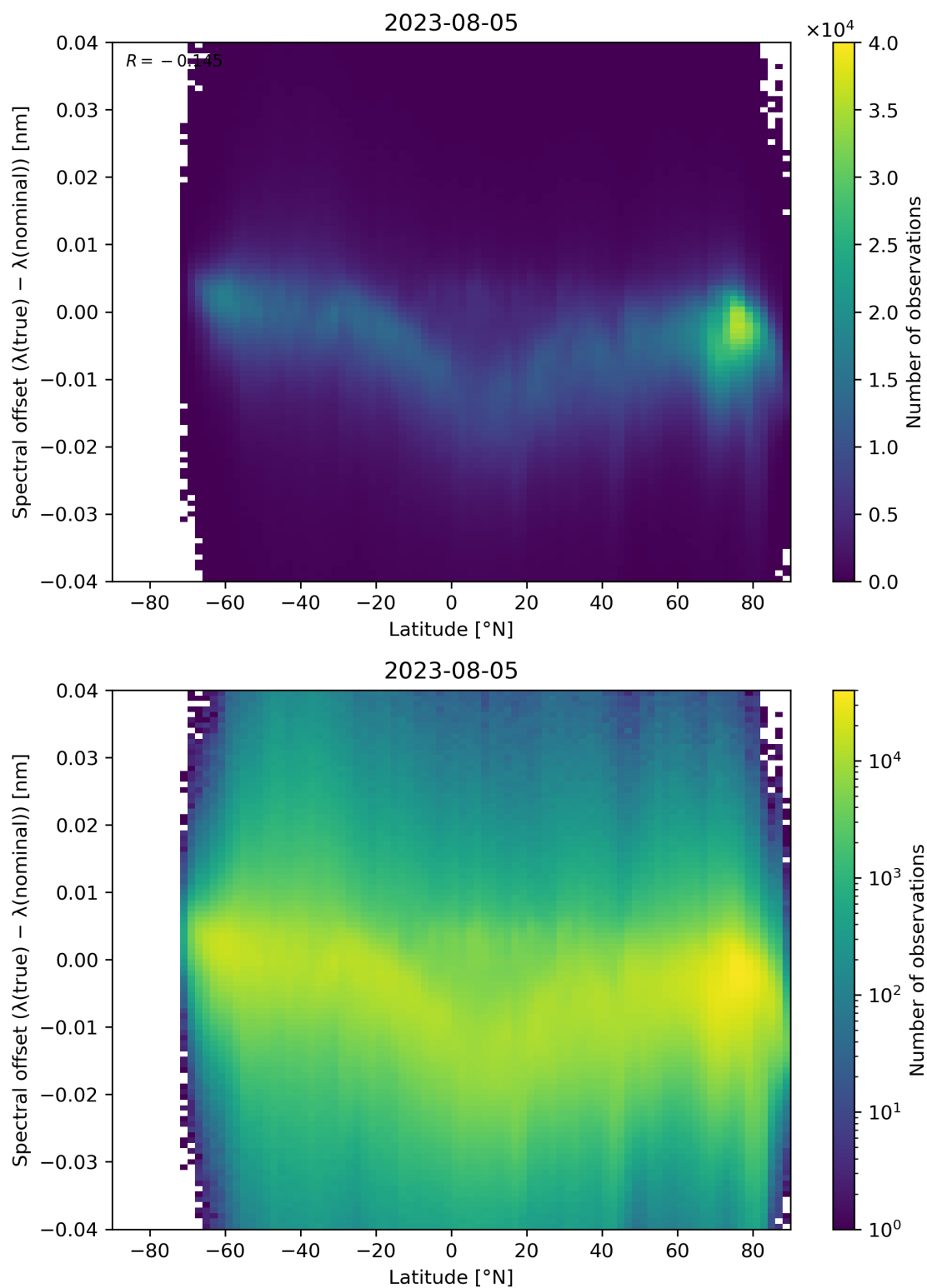
Figure 105: Scatter density plot of “Latitude” against “Spectral offset ( \lambda(\text{true}) - \lambda(\text{nominal}) )” for 2023-08-04 to 2023-08-06.
