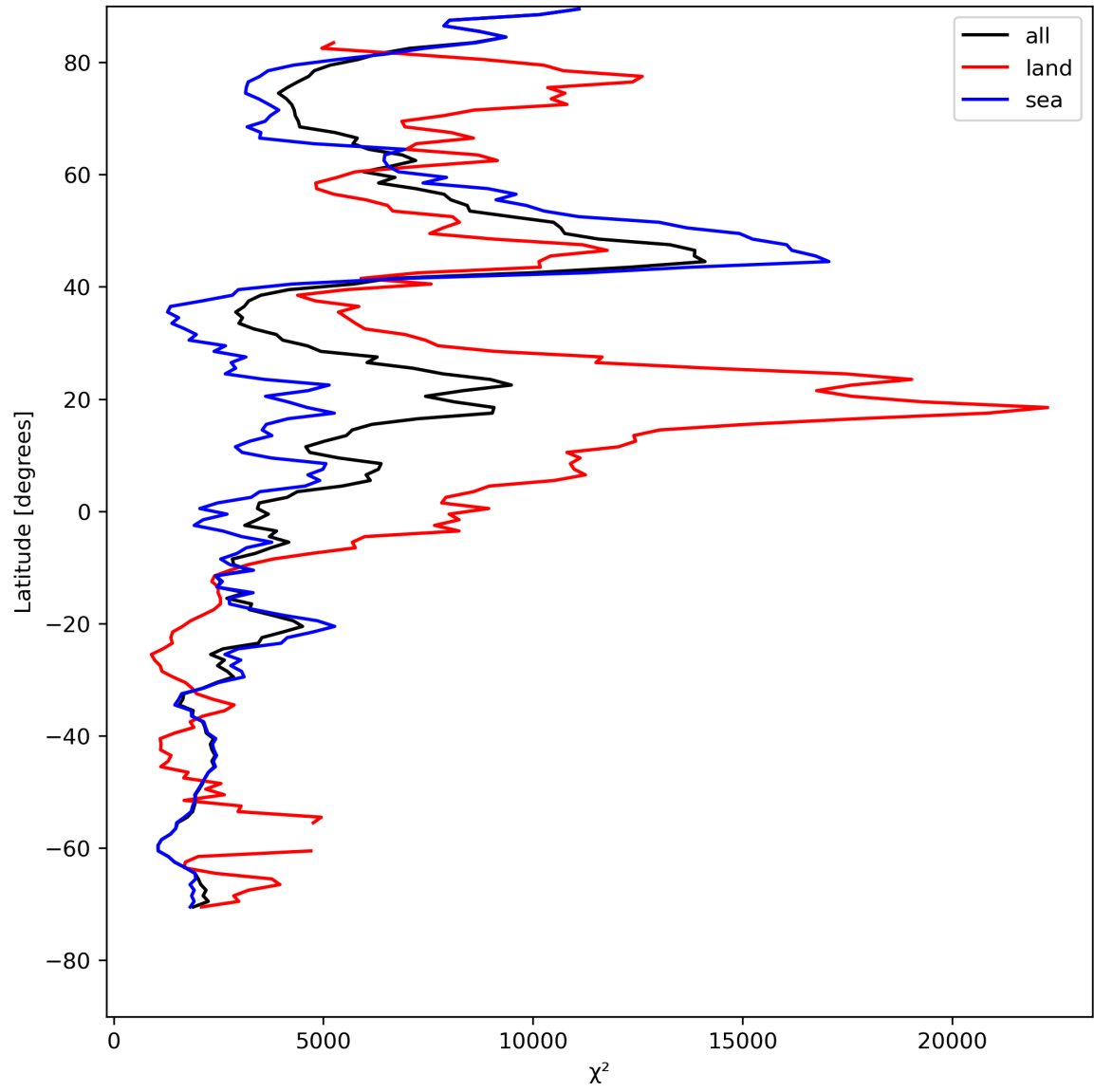
Figure 21: Zonal average of “ \chi^2 ” for 2023-08-04 to 2023-08-06.
