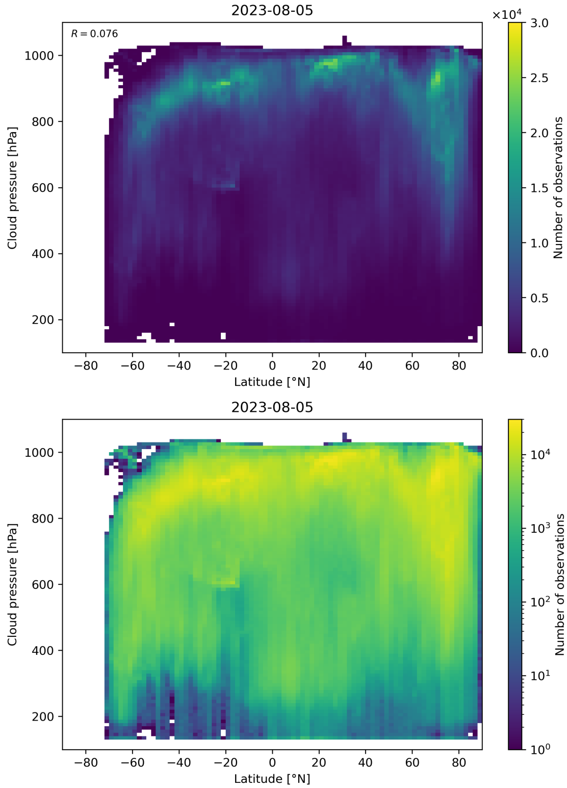
Figure 100: Scatter density plot of “Latitude” against “Cloud pressure” for 2023-08-04 to 2023-08-06.
