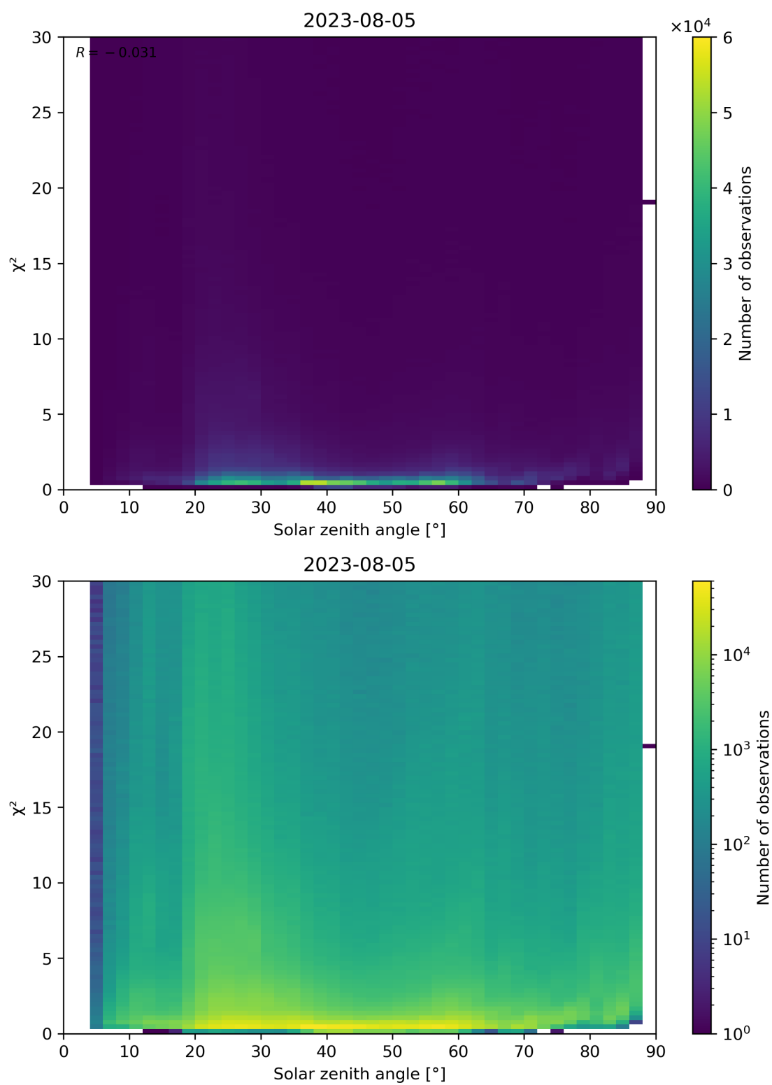
Figure 119: Scatter density plot of “Solar zenith angle” against “ \chi^2 ” for 2023-08-04 to 2023-08-06.
