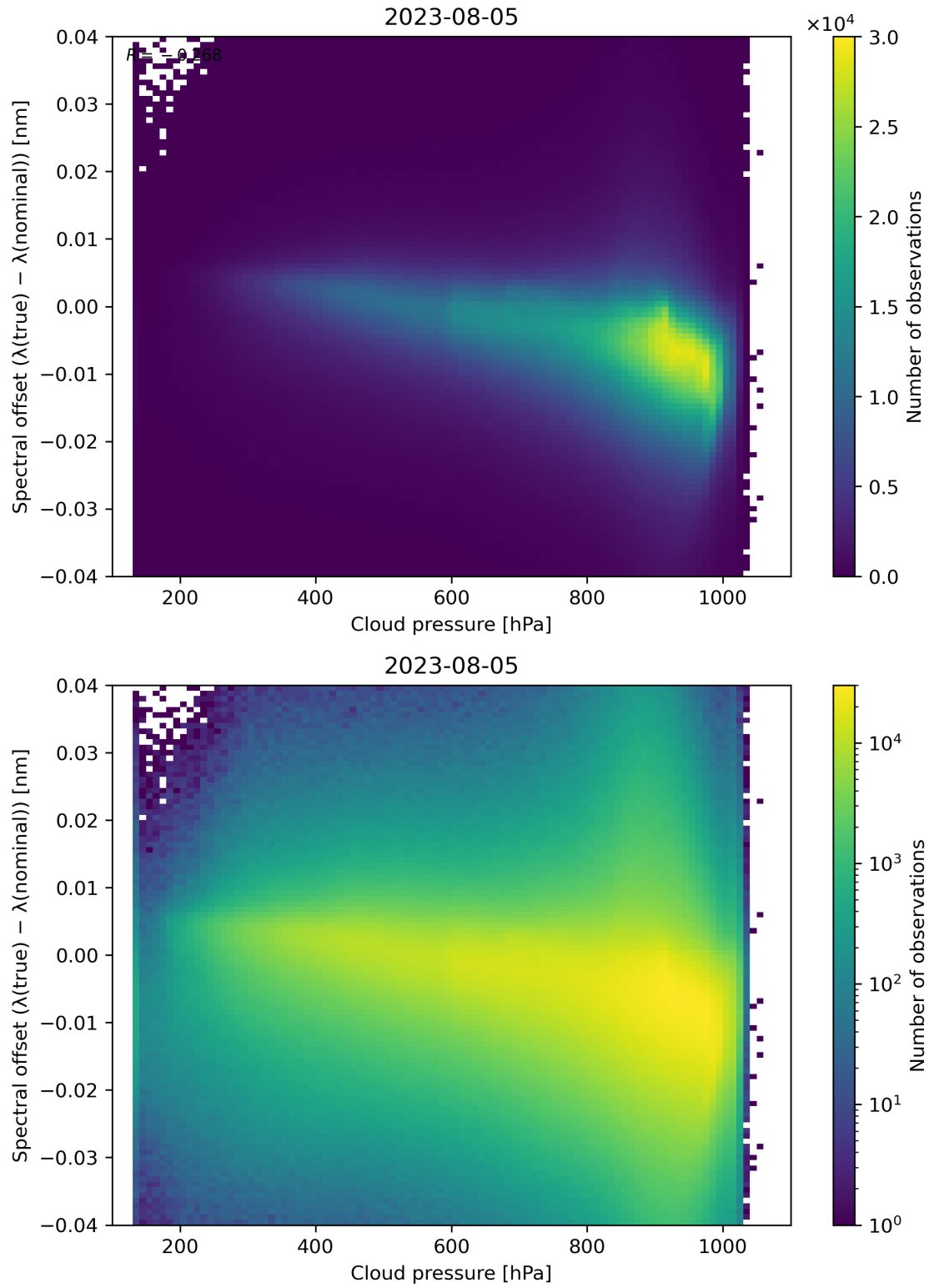
Figure 92: Scatter density plot of “Cloud pressure” against “Spectral offset ( \lambda(\text{true}) - \lambda(\text{nominal}) )” for 2023-08-04 to 2023-08-06.
