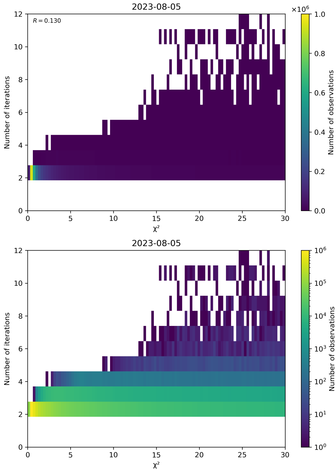
Figure 73: Scatter density plot of “ \chi^2 ” against “Number of iterations” for 2023-08-04 to 2023-08-06.
