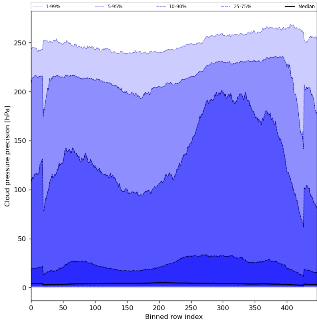
Figure 48: Along track statistics of “Cloud pressure precision” for 2023-08-04 to 2023-08-06
