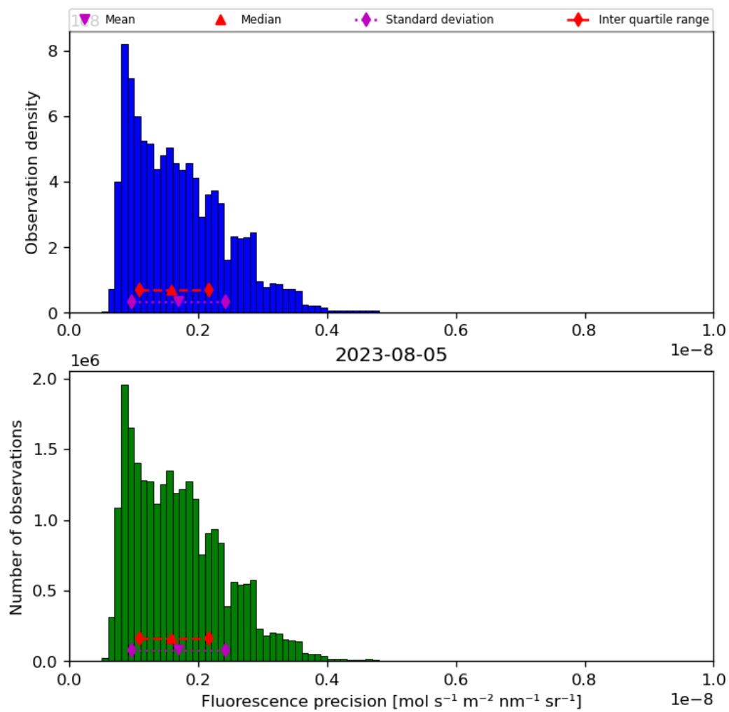
Figure 41: Histogram of “Fluorescence precision” for 2023-08-04 to 2023-08-06
