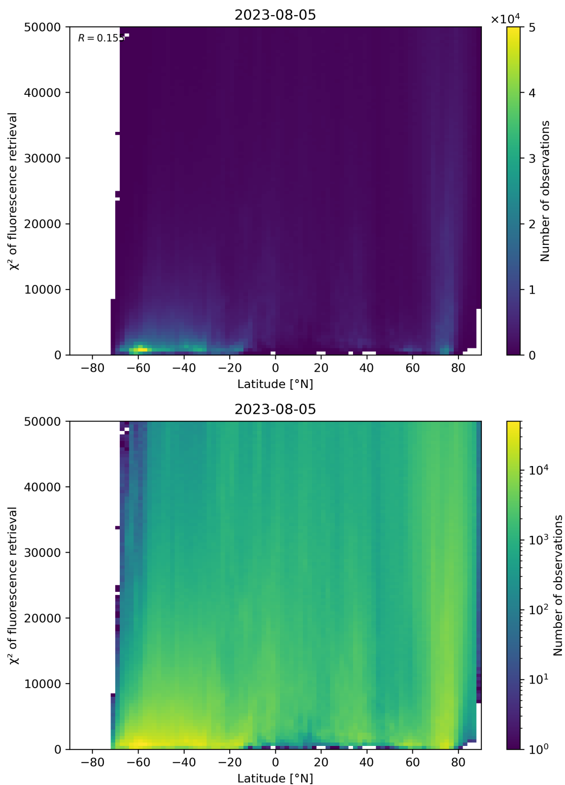
Figure 98: Scatter density plot of “Latitude” against “ \chi^2 of fluorescence retrieval” for 2023-08-04 to 2023-08-06.
