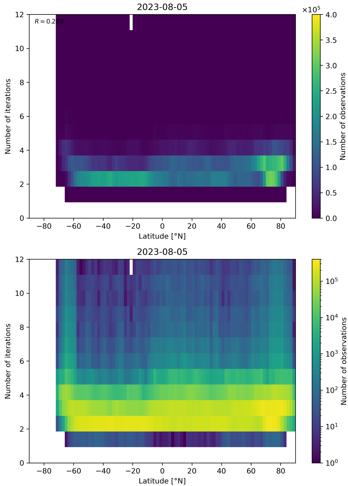
Figure 102: Scatter density plot of “Latitude” against “Number of iterations” for 2023-08-04 to 2023-08-06.
