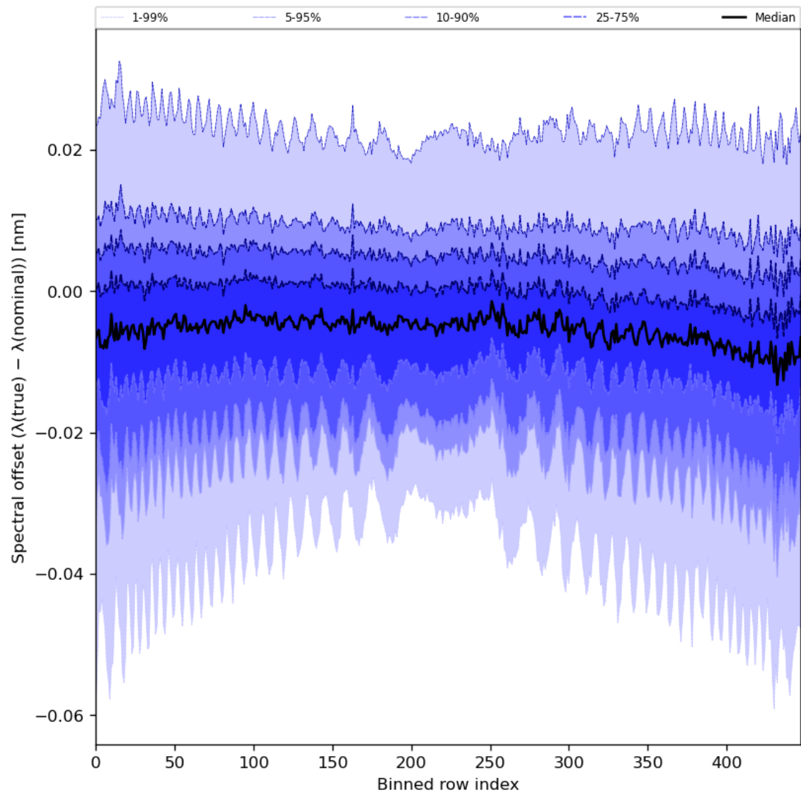
Figure 62: Along track statistics of “Spectral offset ( \lambda(\text{true}) - \lambda(\text{nominal}) )” for 2023-08-04 to 2023-08-06
