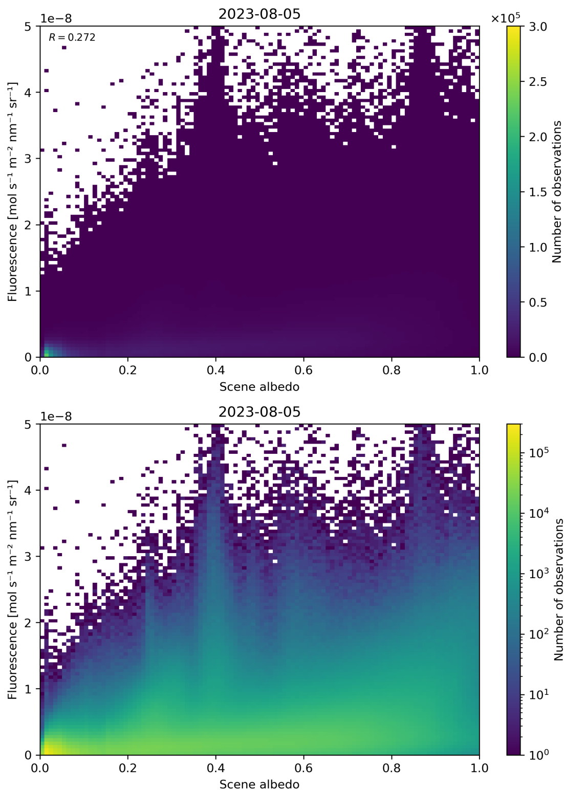
Figure 114: Scatter density plot of “Scene albedo” against “Fluorescence” for 2023-08-04 to 2023-08-06.
