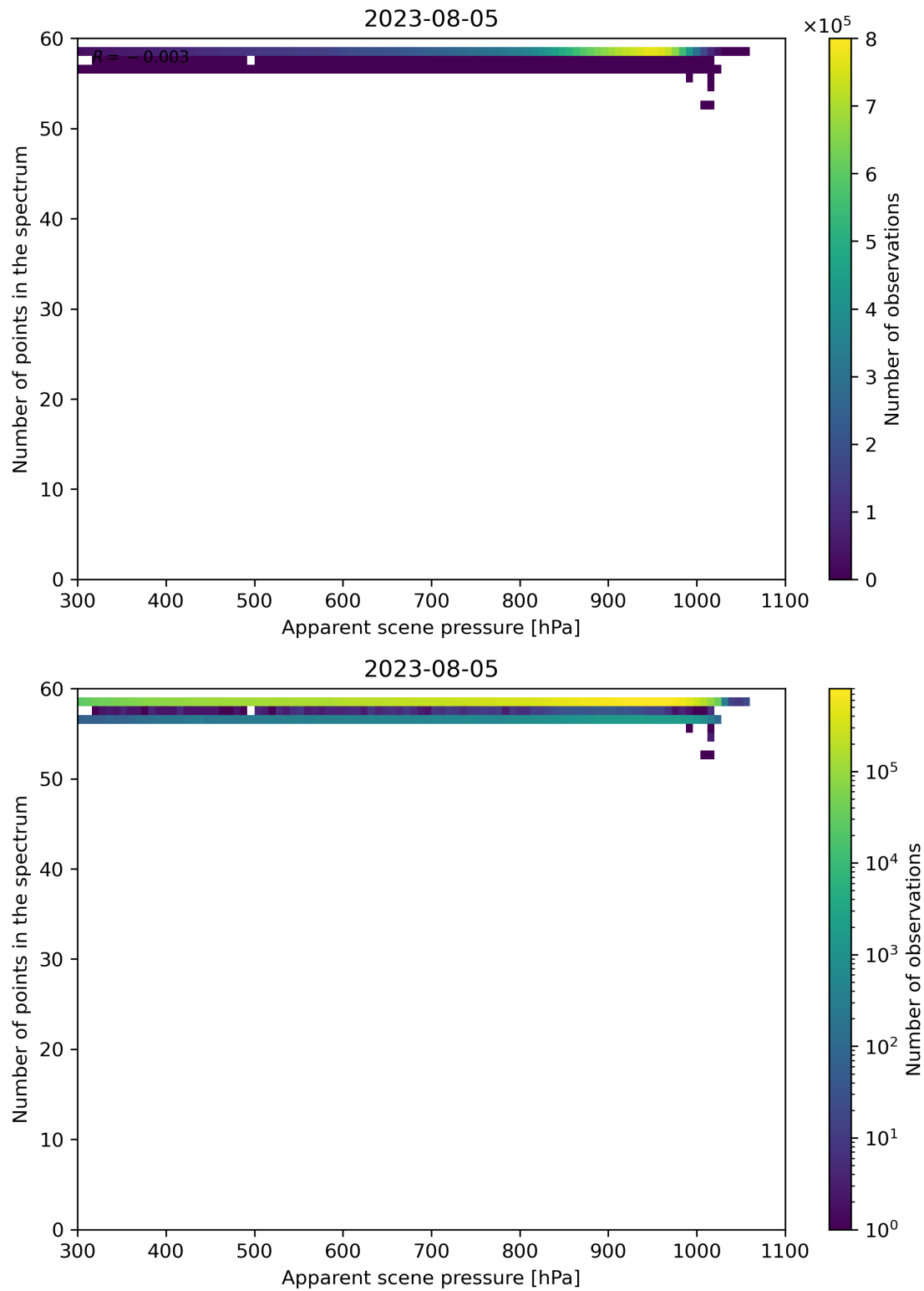
Figure 67: Scatter density plot of “Apparent scene pressure” against “Number of points in the spectrum” for 2023-08-04 to 2023-08-06.
