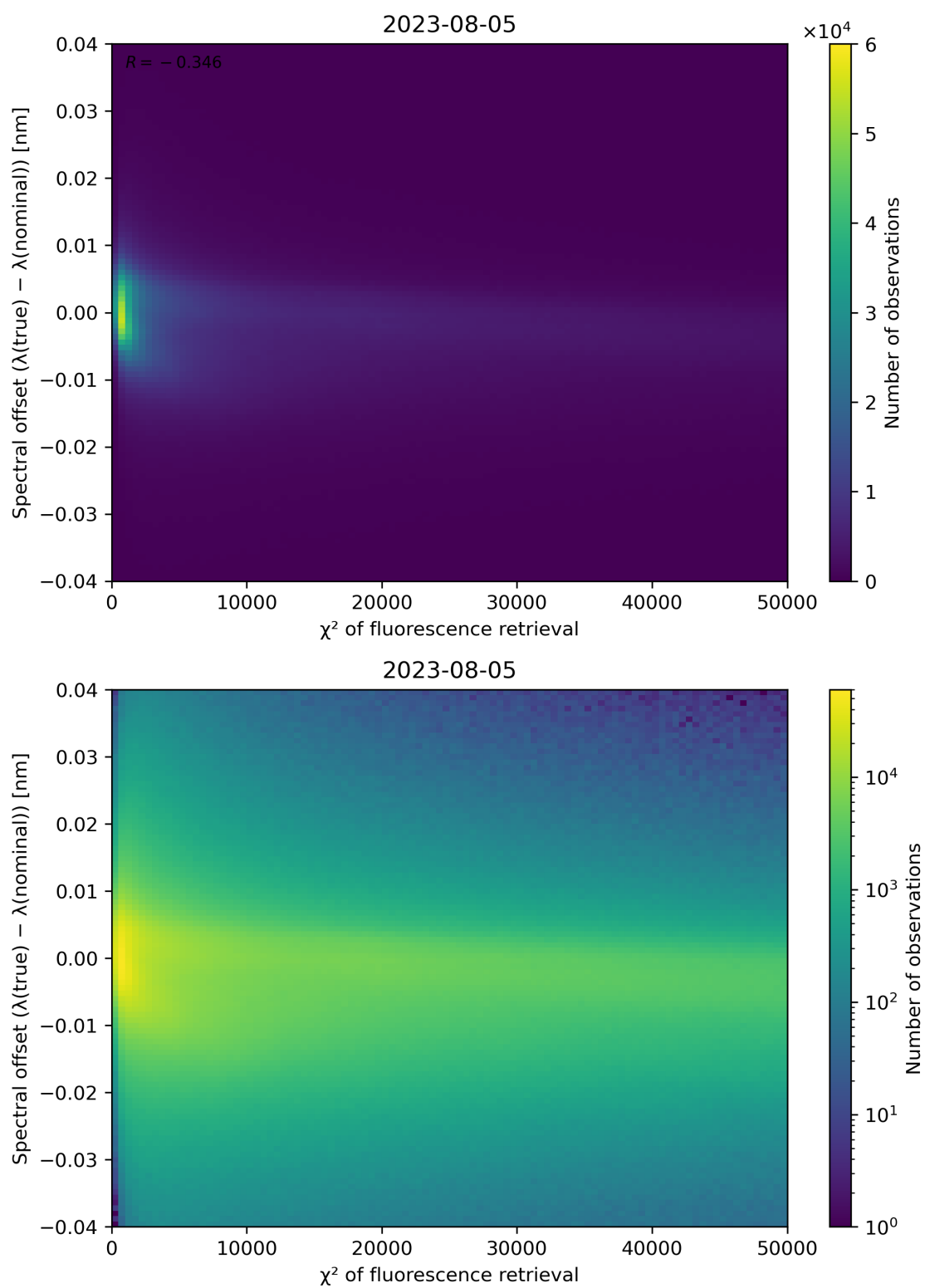
Figure 72: Scatter density plot of “ \chi^2 of fluorescence retrieval” against “Spectral offset ( \lambda(\text{true}) - \lambda(\text{nominal}) )” for 2023-08-04 to 2023-08-06.
