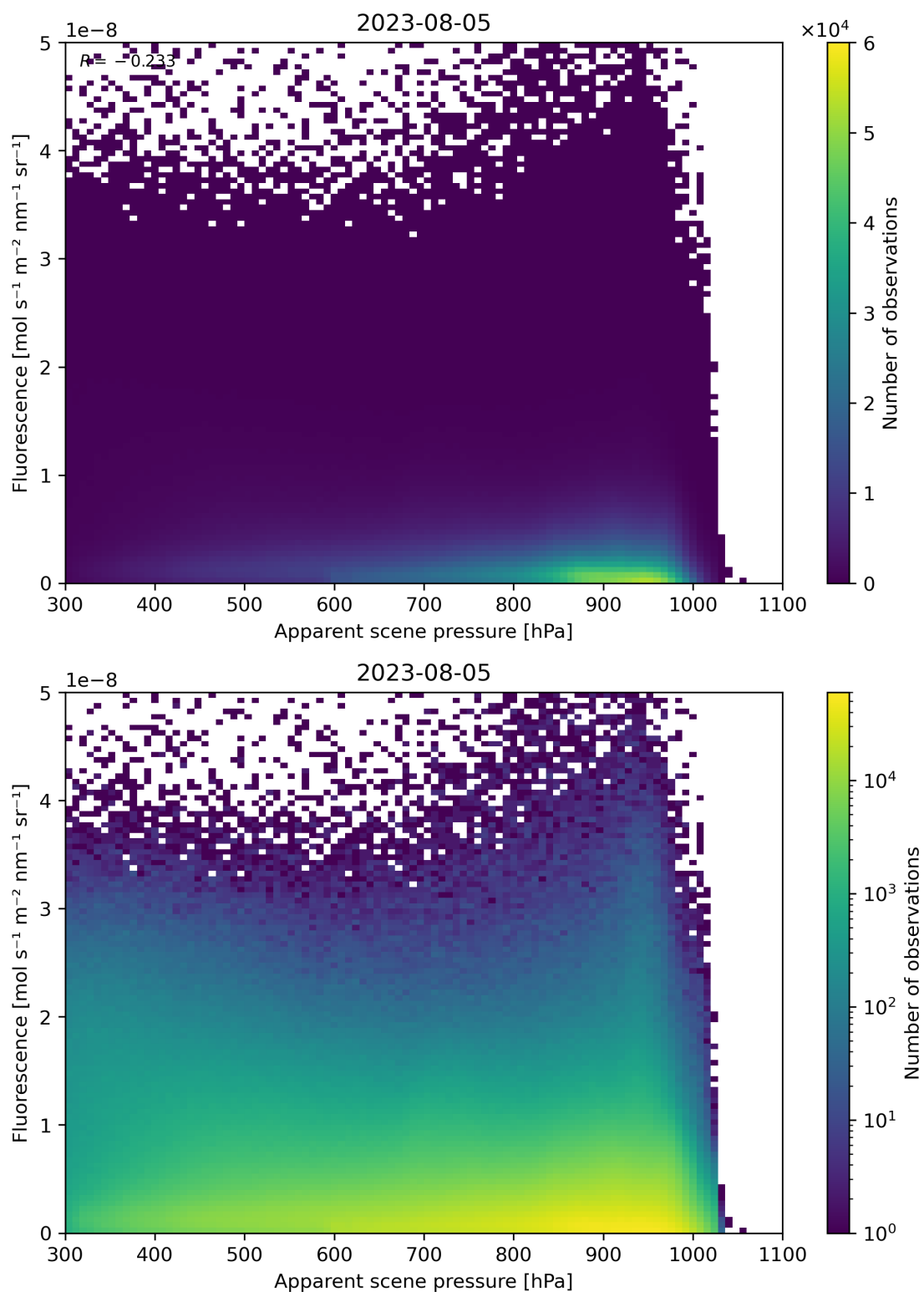
Figure 65: Scatter density plot of “Apparent scene pressure” against “Fluorescence” for 2023-08-04 to 2023-08-06.
