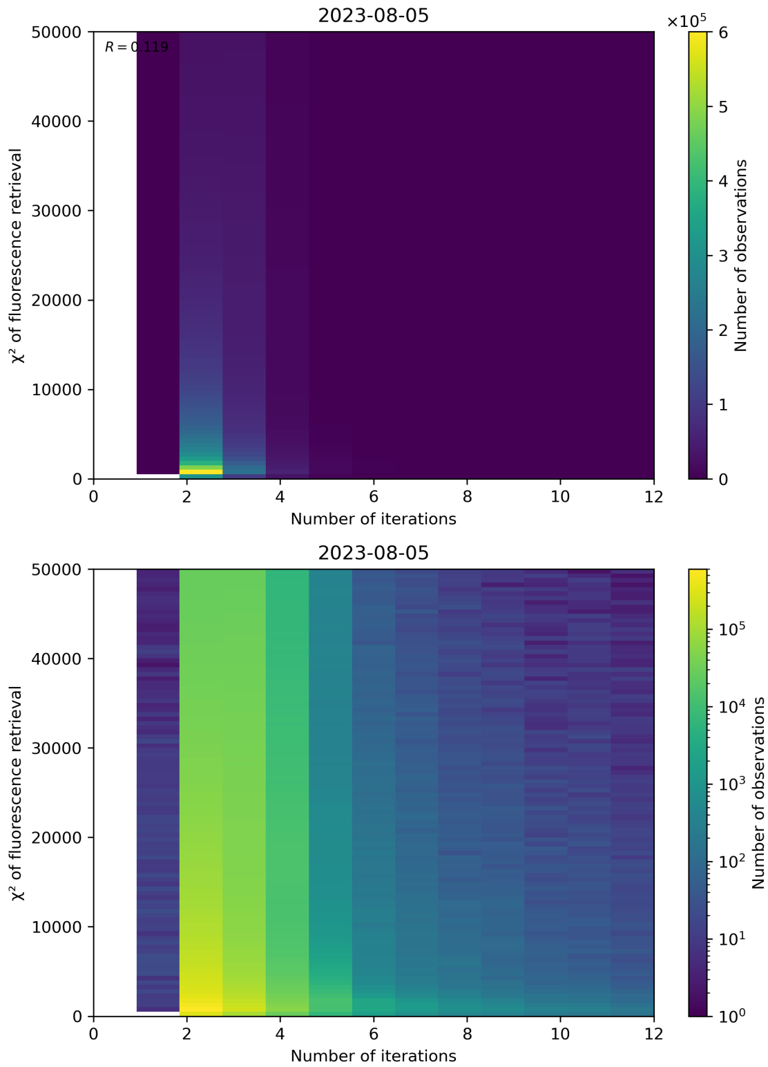
Figure 106: Scatter density plot of “Number of iterations” against “ \chi^2 of fluorescence retrieval” for 2023-08-04 to 2023-08-06.
