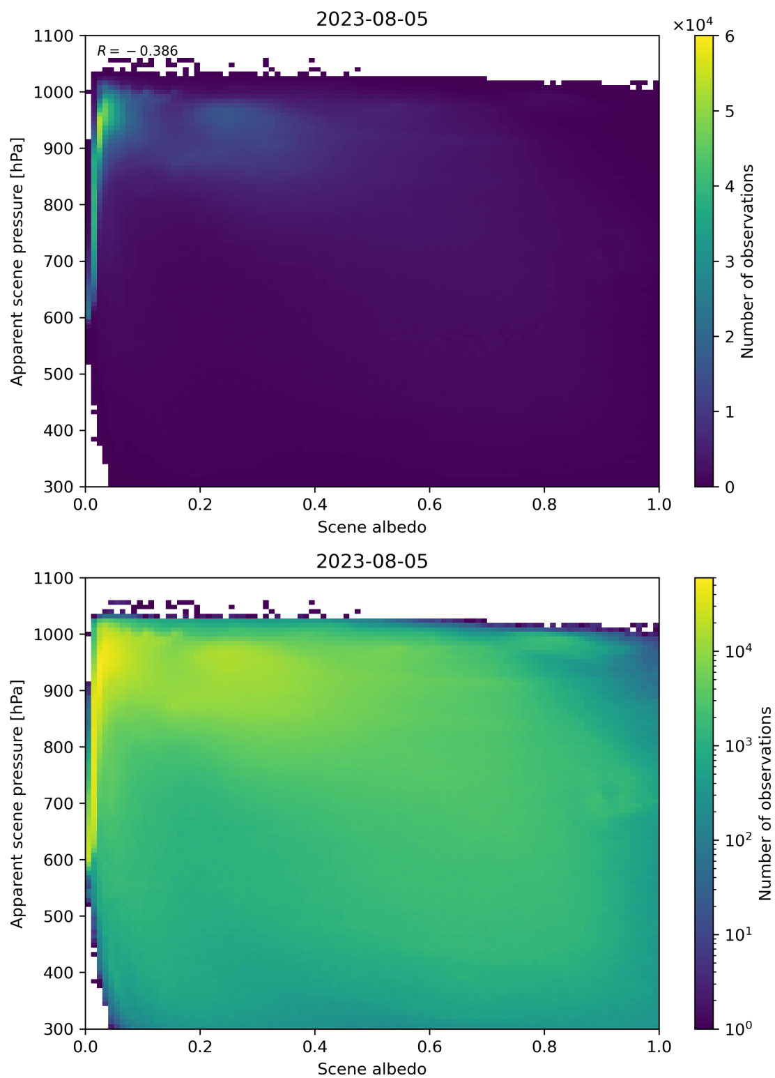
Figure 111: Scatter density plot of “Scene albedo” against “Apparent scene pressure” for 2023-08-04 to 2023-08-06.
