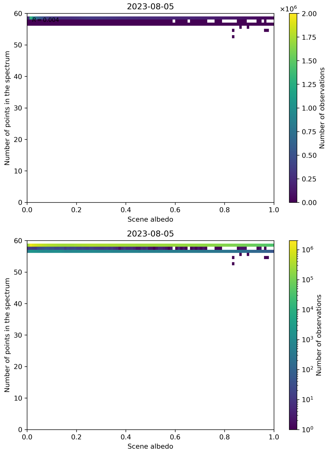
Figure 116: Scatter density plot of “Scene albedo” against “Number of points in the spectrum” for 2023-08-04 to 2023-08-06.
