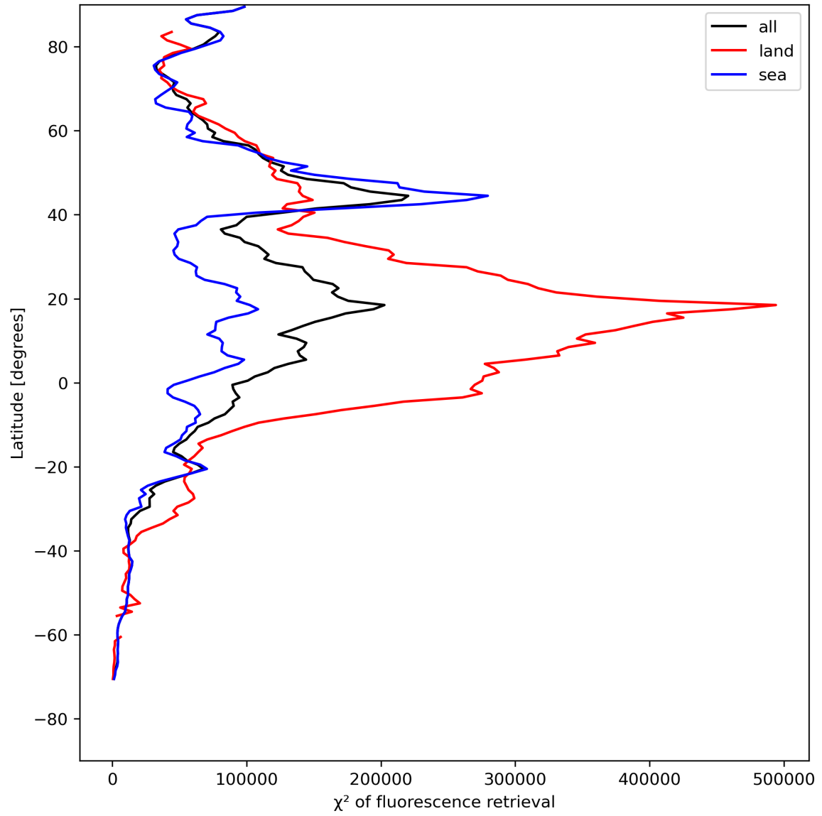
Figure 25: Zonal average of “ \chi^2 of fluorescence retrieval” for 2023-08-04 to 2023-08-06.
