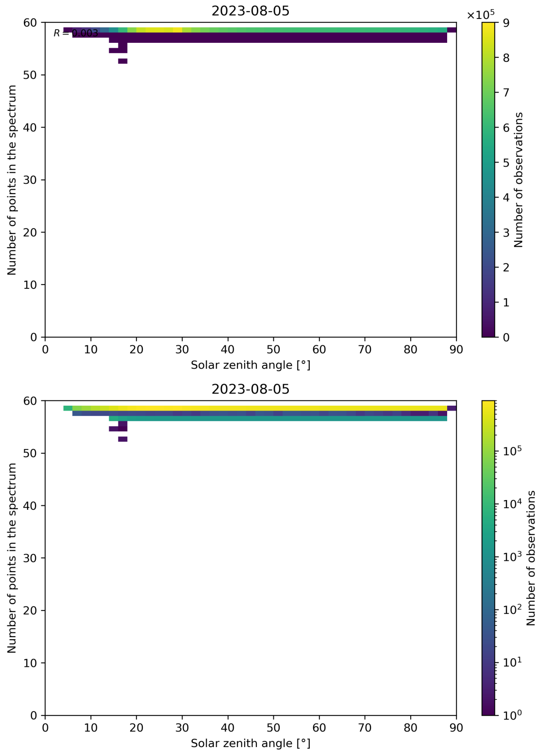
Figure 126: Scatter density plot of “Solar zenith angle” against “Number of points in the spectrum” for 2023-08-04 to 2023-08-06.
