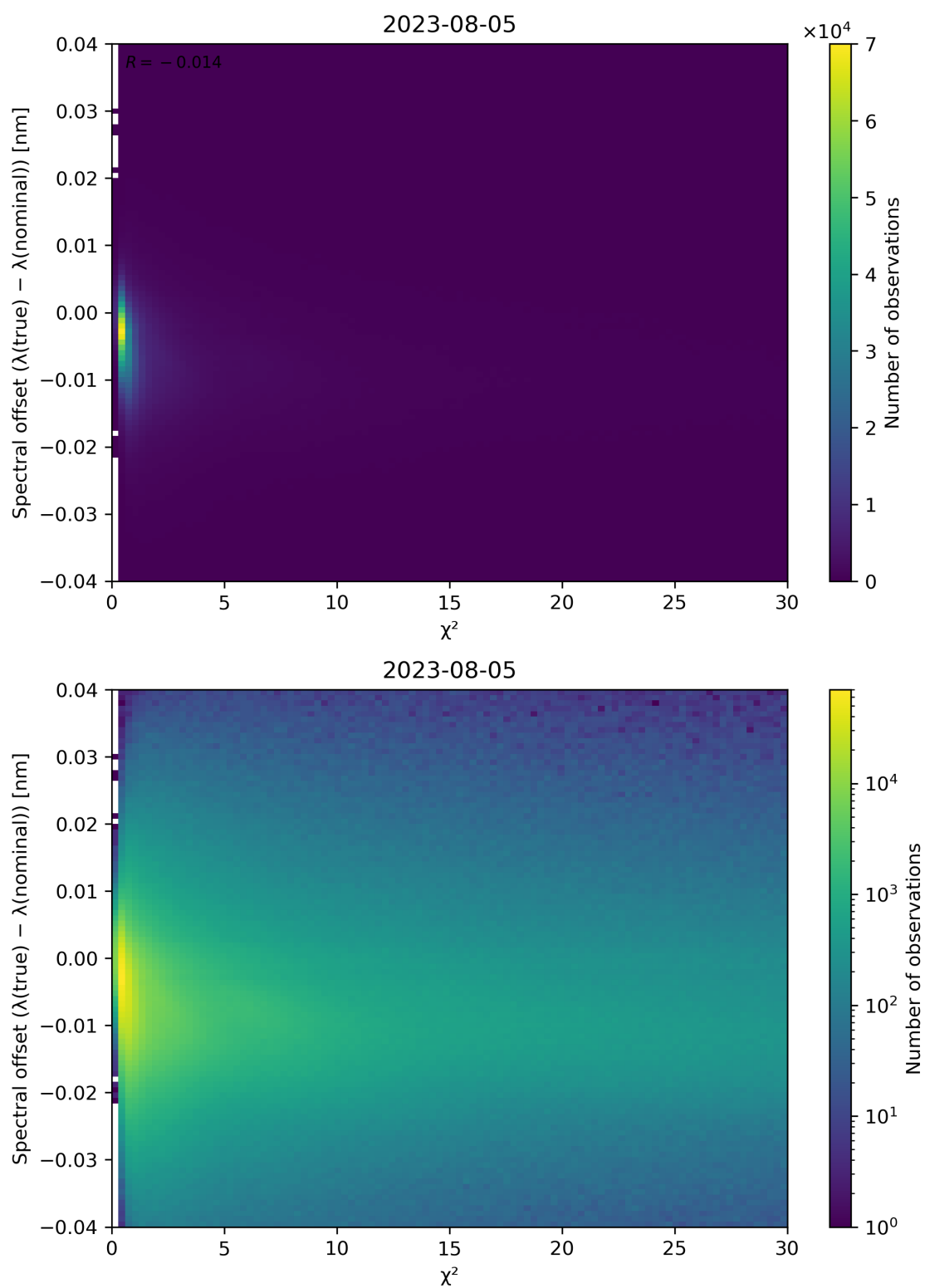
Figure 75: Scatter density plot of “ \chi^2 ” against “Spectral offset ( \lambda(\text{true}) - \lambda(\text{nominal}) )” for 2023-08-04 to 2023-08-06.
