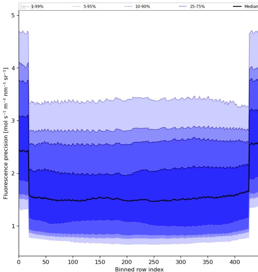
Figure 58: Along track statistics of “Fluorescence precision” for 2023-08-04 to 2023-08-06
