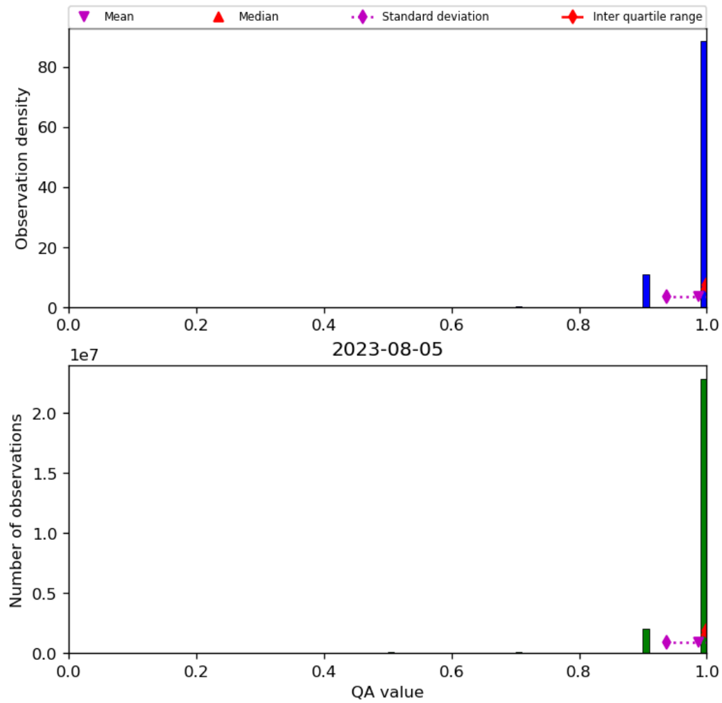
Figure 29: Histogram of “QA value” for 2023-08-04 to 2023-08-06
