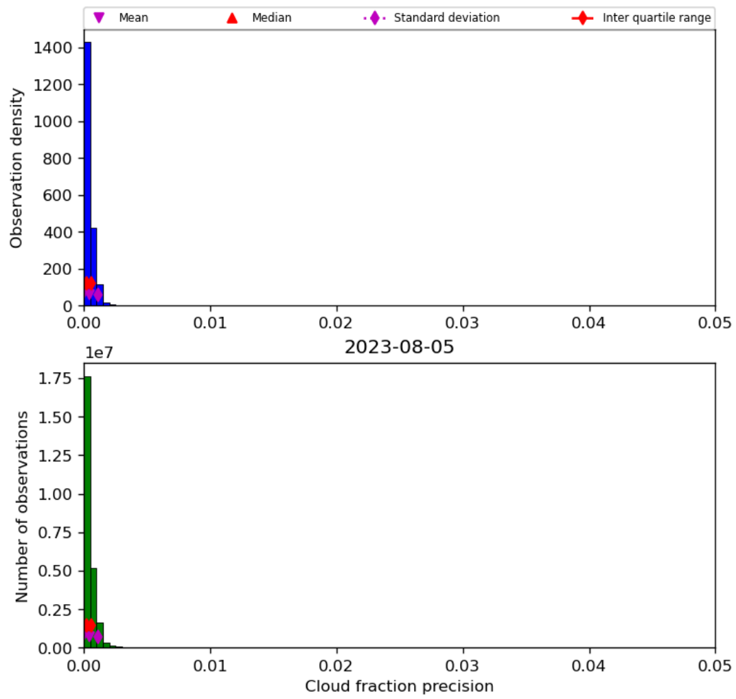
Figure 33: Histogram of “Cloud fraction precision” for 2023-08-04 to 2023-08-06
