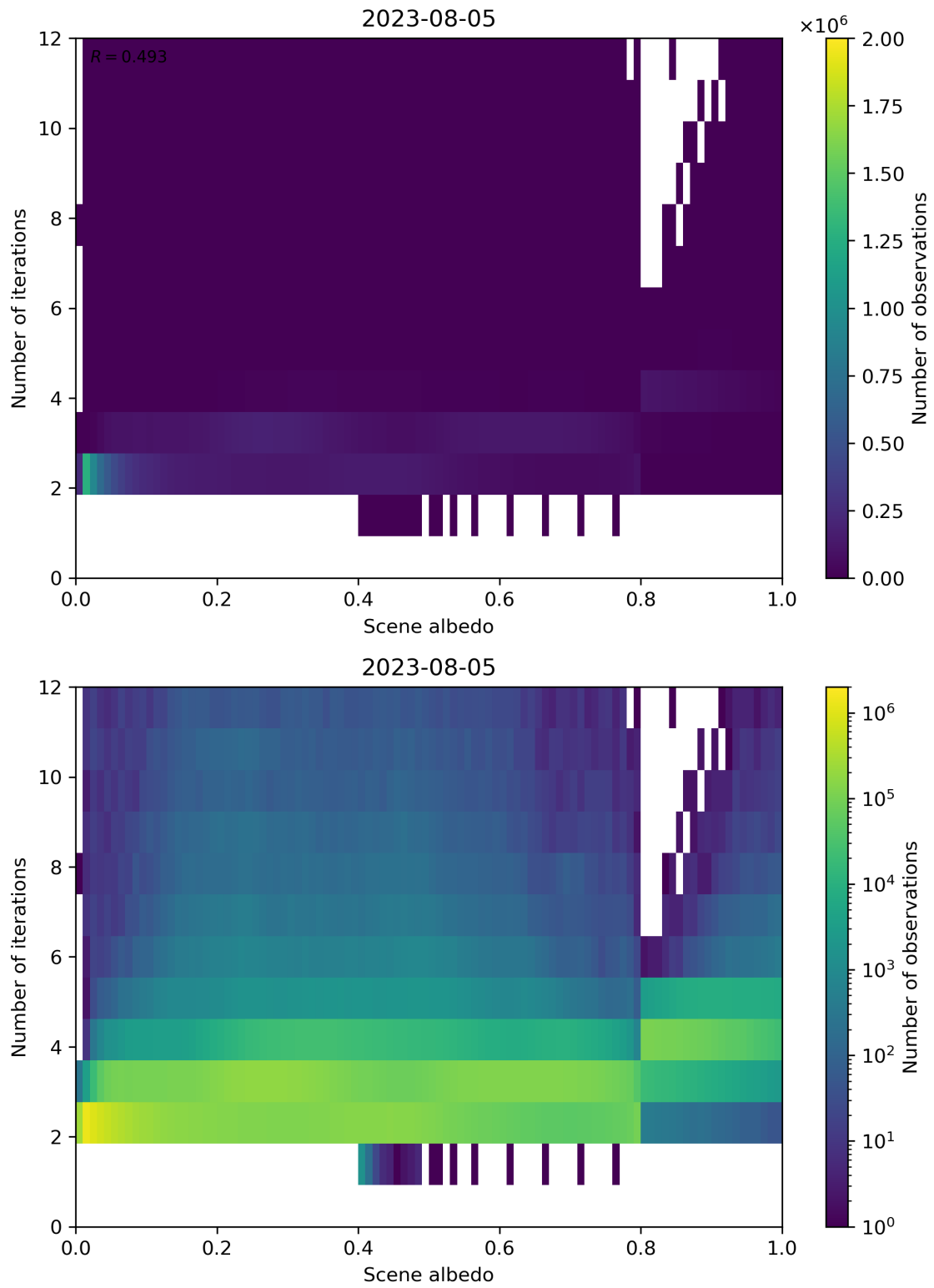
Figure 115: Scatter density plot of “Scene albedo” against “Number of iterations” for 2023-08-04 to 2023-08-06.
