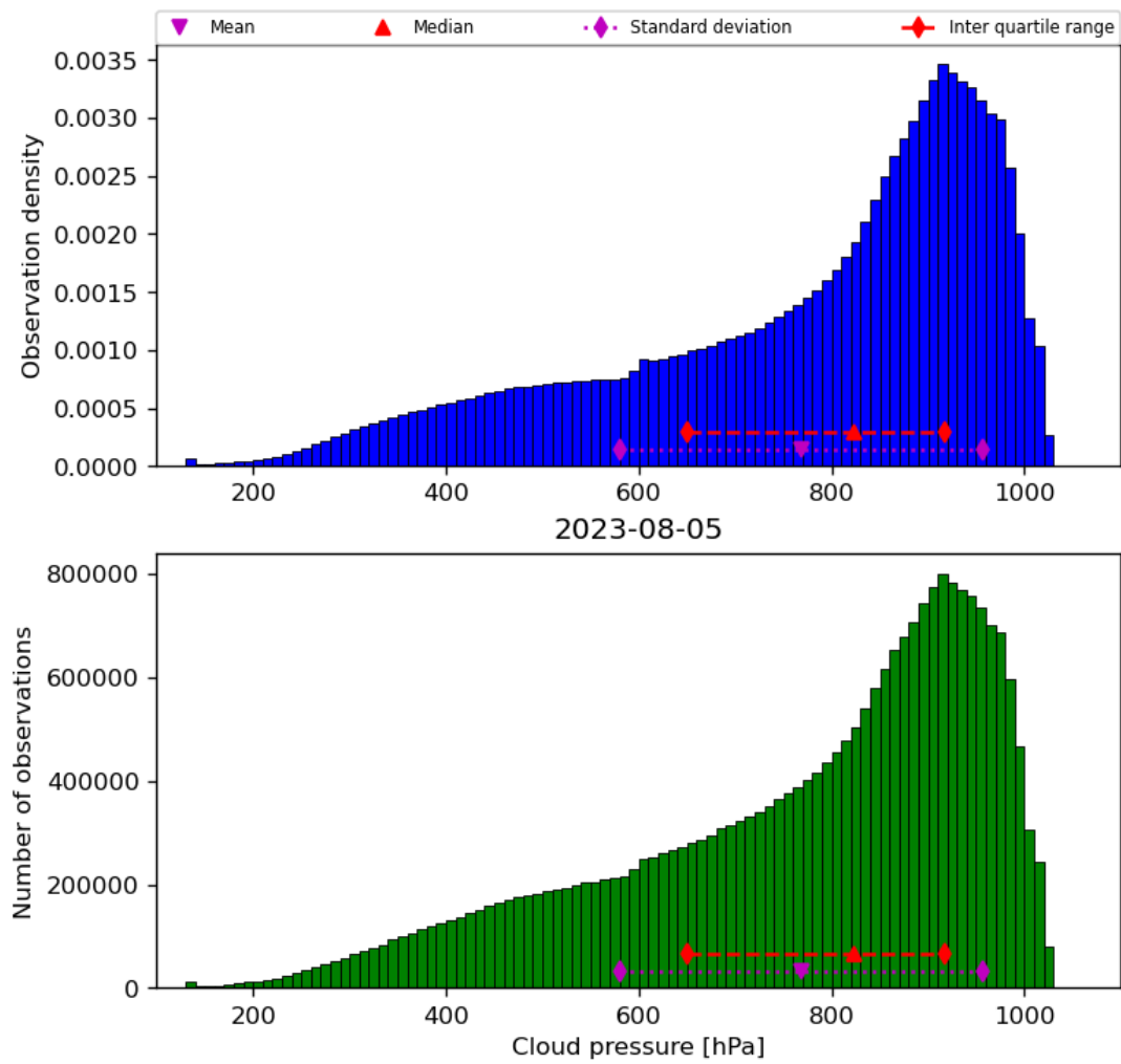
Figure 30: Histogram of “Cloud pressure” for 2023-08-04 to 2023-08-06
