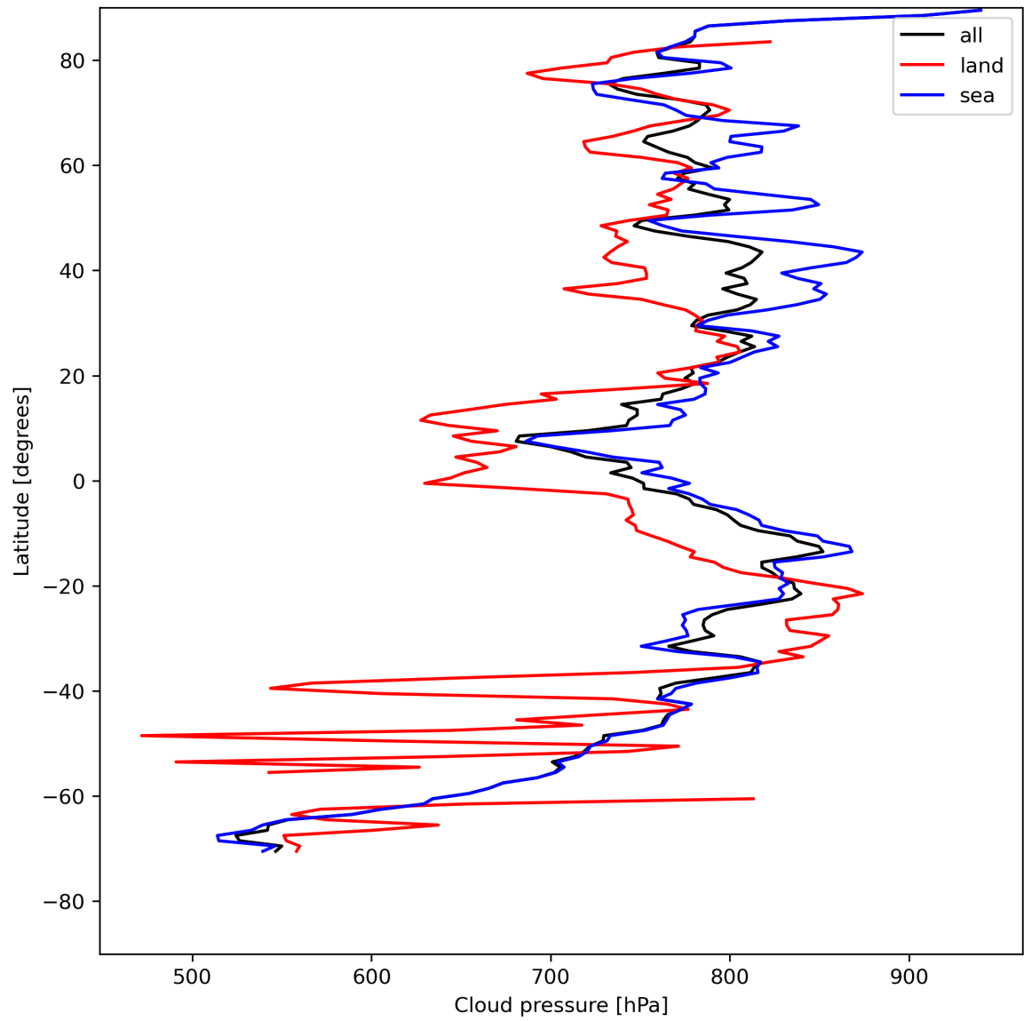
Figure 13: Zonal average of “Cloud pressure” for 2023-08-04 to 2023-08-06.
