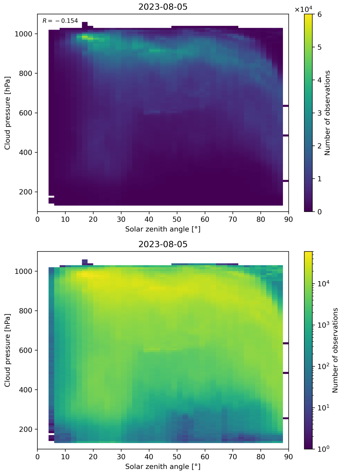
Figure 122: Scatter density plot of “Solar zenith angle” against “Cloud pressure” for 2023-08-04 to 2023-08-06.
