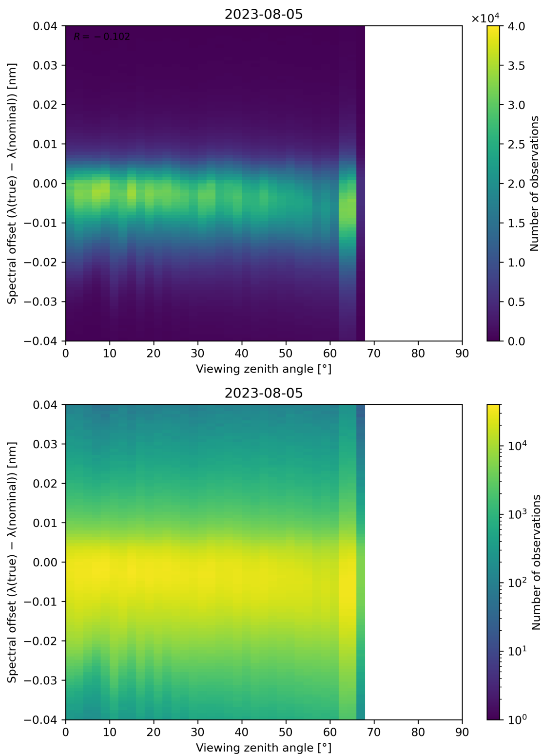
Figure 140: Scatter density plot of “Viewing zenith angle” against “Spectral offset ( \lambda(\text{true}) - \lambda(\text{nominal}) )” for 2023-08-04 to 2023-08-06.
