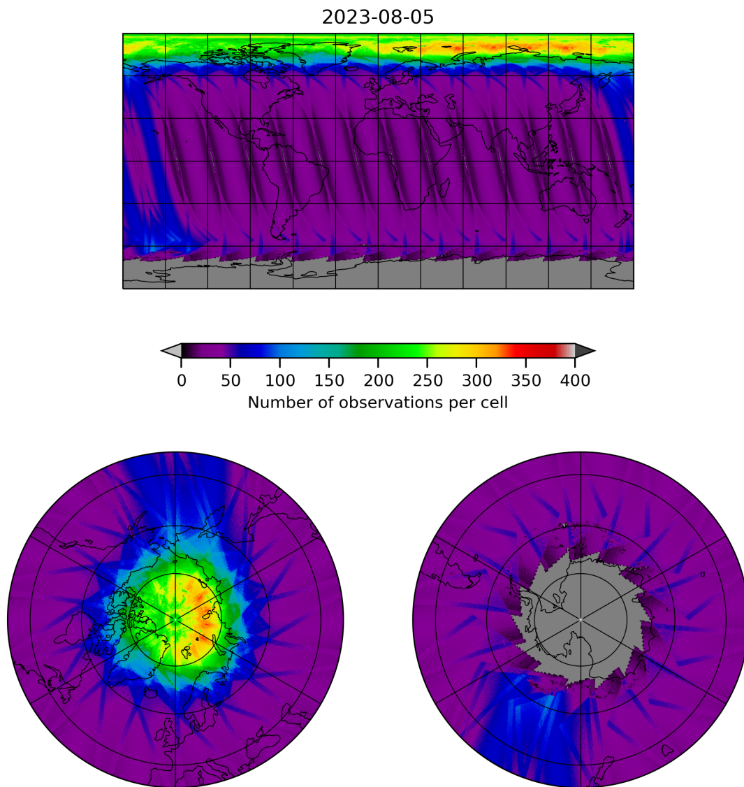
Figure 11: Map of the number of observations for 2023-08-04 to 2023-08-06
