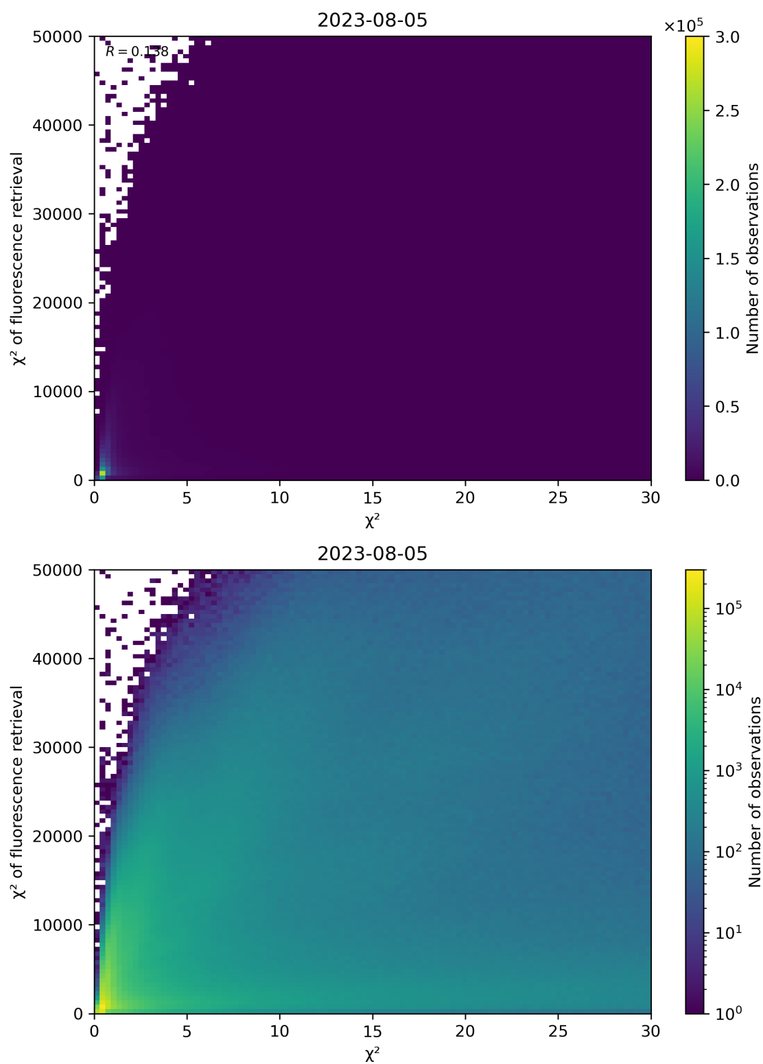
Figure 69: Scatter density plot of “ \chi^2 ” against “ \chi^2 of fluorescence retrieval” for 2023-08-04 to 2023-08-06.
