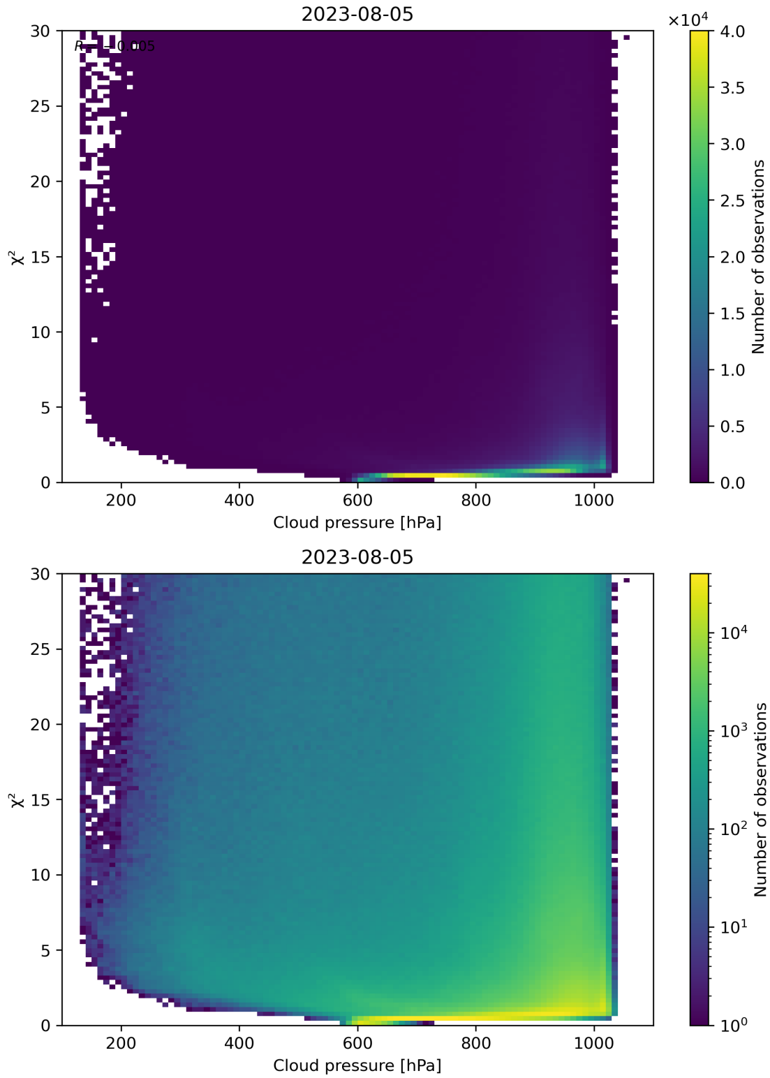
Figure 85: Scatter density plot of “Cloud pressure” against “ \chi^2 ” for 2023-08-04 to 2023-08-06.
