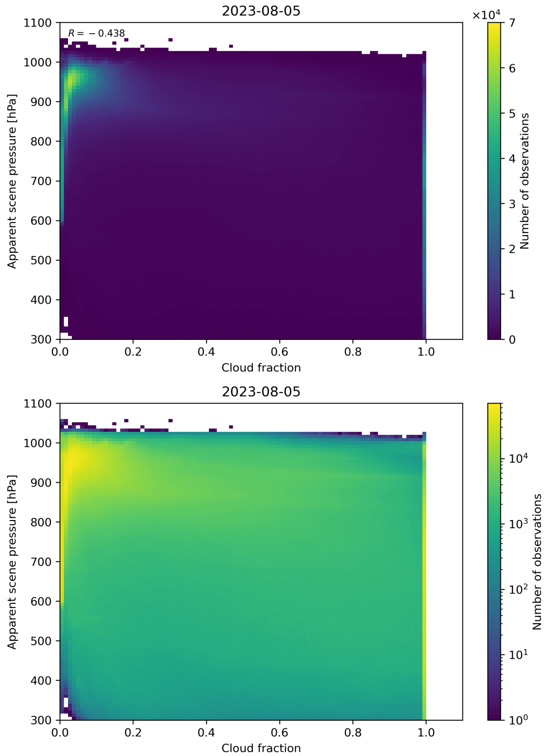
Figure 76: Scatter density plot of “Cloud fraction” against “Apparent scene pressure” for 2023-08-04 to 2023-08-06.
