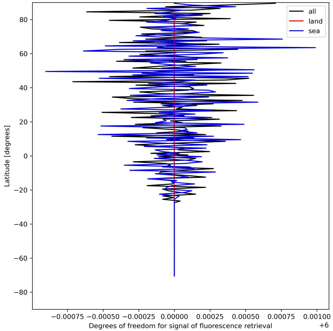
Figure 26: Zonal average of “Degrees of freedom for signal of fluorescence retrieval” for 2023-08-04 to 2023-08-06.
