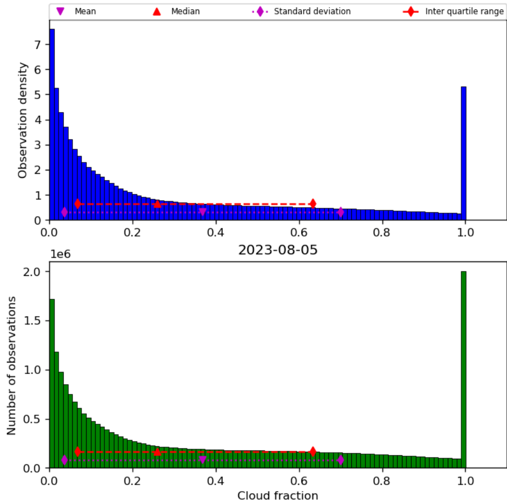
Figure 32: Histogram of “Cloud fraction” for 2023-08-04 to 2023-08-06
