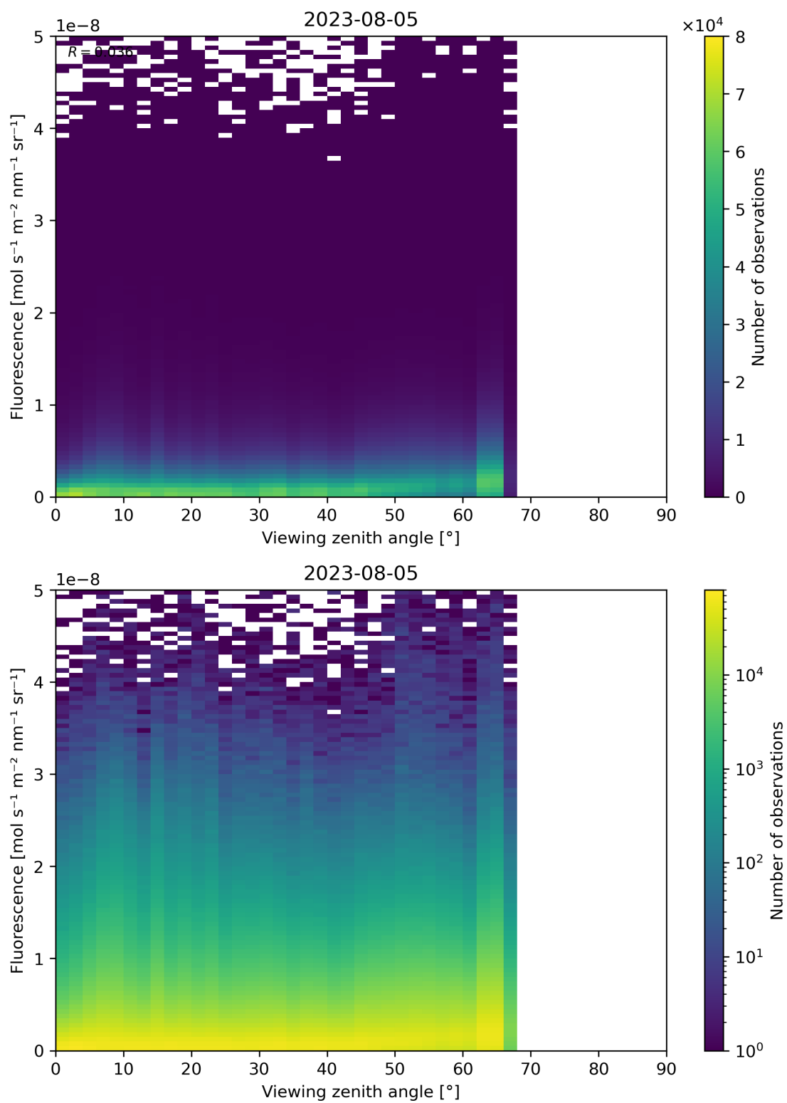
Figure 134: Scatter density plot of “Viewing zenith angle” against “Fluorescence” for 2023-08-04 to 2023-08-06.
