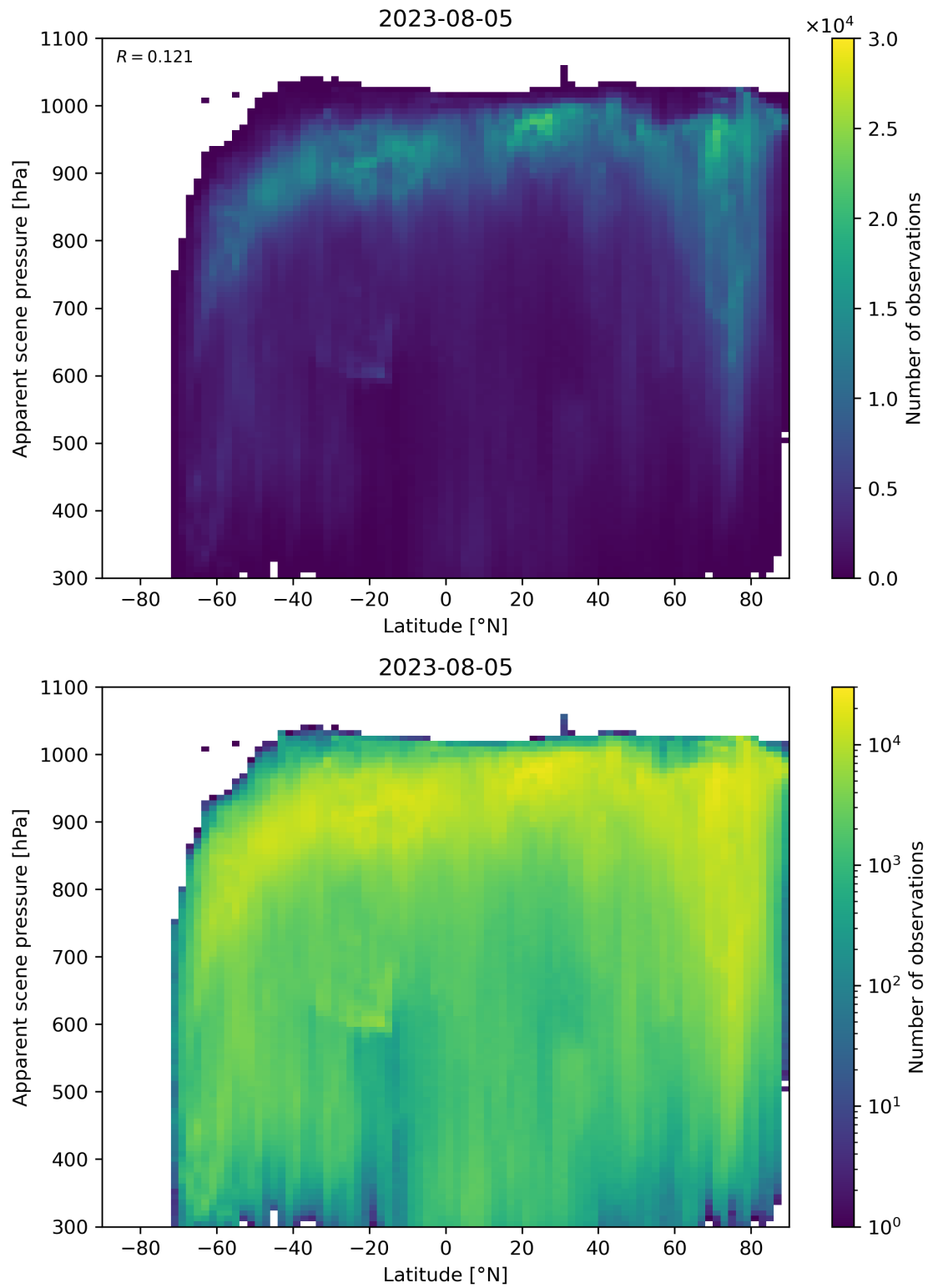
Figure 96: Scatter density plot of “Latitude” against “Apparent scene pressure” for 2023-08-04 to 2023-08-06.
