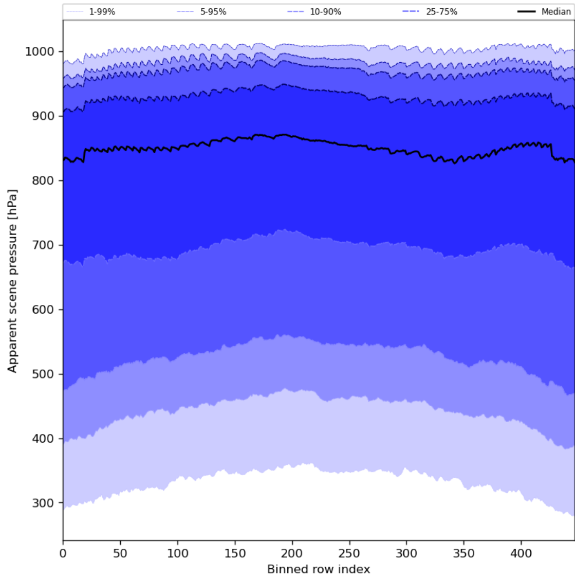
Figure 53: Along track statistics of “Apparent scene pressure” for 2023-08-04 to 2023-08-06
