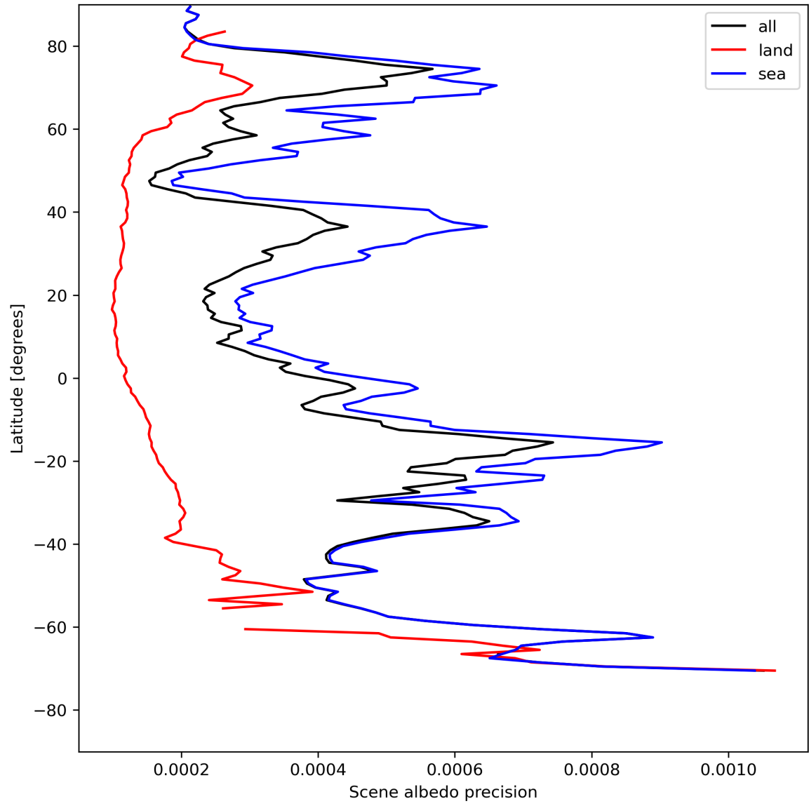
Figure 18: Zonal average of “Scene albedo precision” for 2023-08-04 to 2023-08-06.
