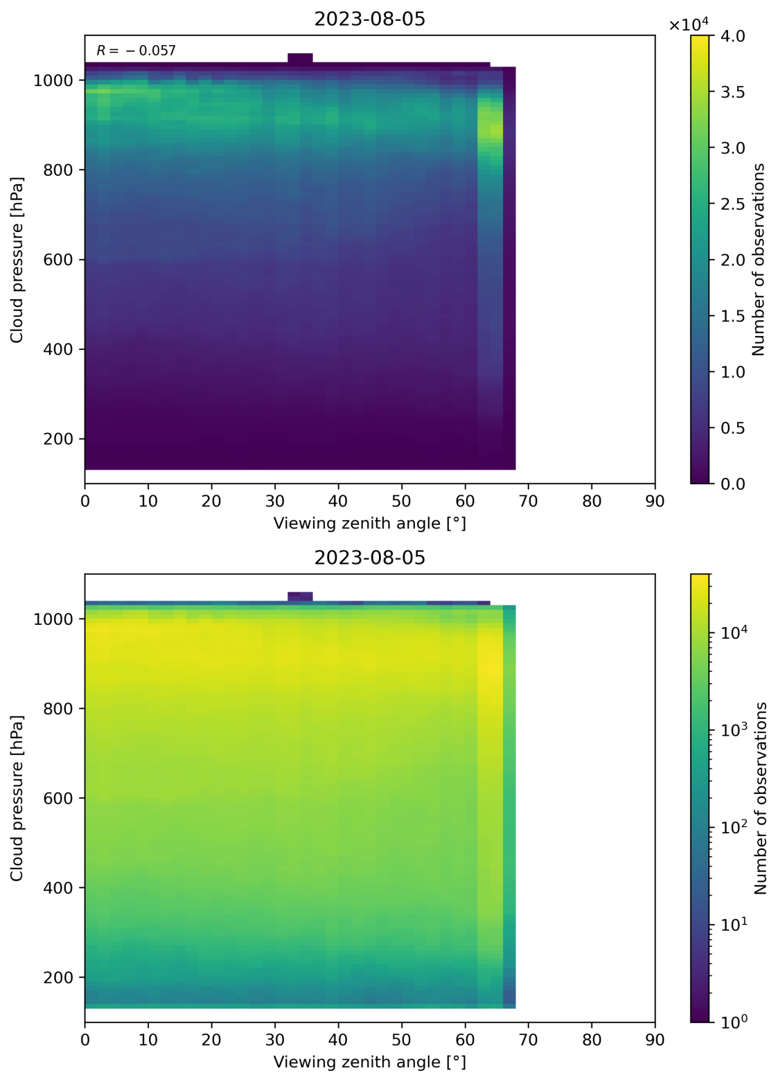
Figure 133: Scatter density plot of “Viewing zenith angle” against “Cloud pressure” for 2023-08-04 to 2023-08-06.
