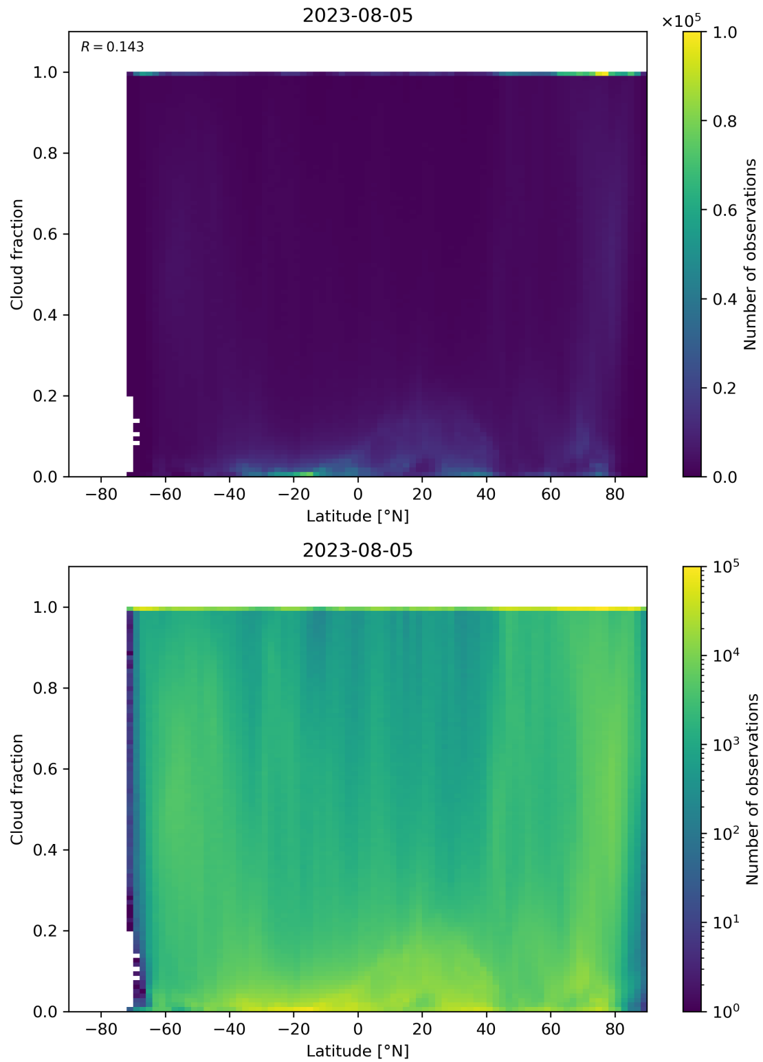
Figure 99: Scatter density plot of “Latitude” against “Cloud fraction” for 2023-08-04 to 2023-08-06.
