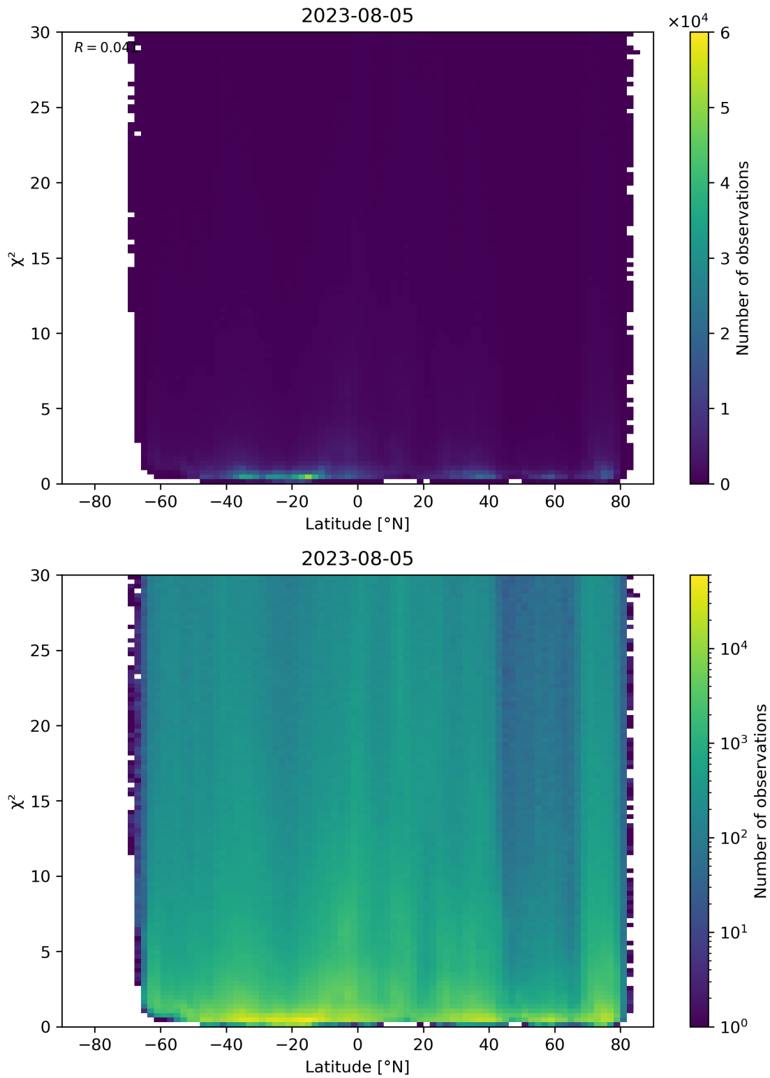
Figure 97: Scatter density plot of “Latitude” against “ \chi^2 ” for 2023-08-04 to 2023-08-06.
