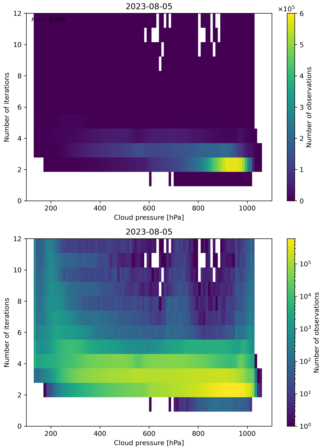
Figure 89: Scatter density plot of “Cloud pressure” against “Number of iterations” for 2023-08-04 to 2023-08-06.
