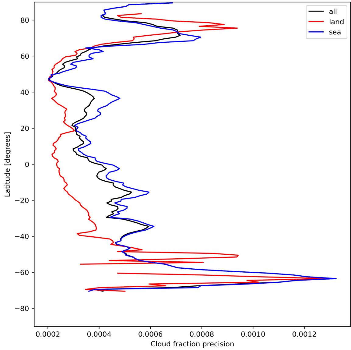
Figure 16: Zonal average of “Cloud fraction precision” for 2023-08-04 to 2023-08-06.
