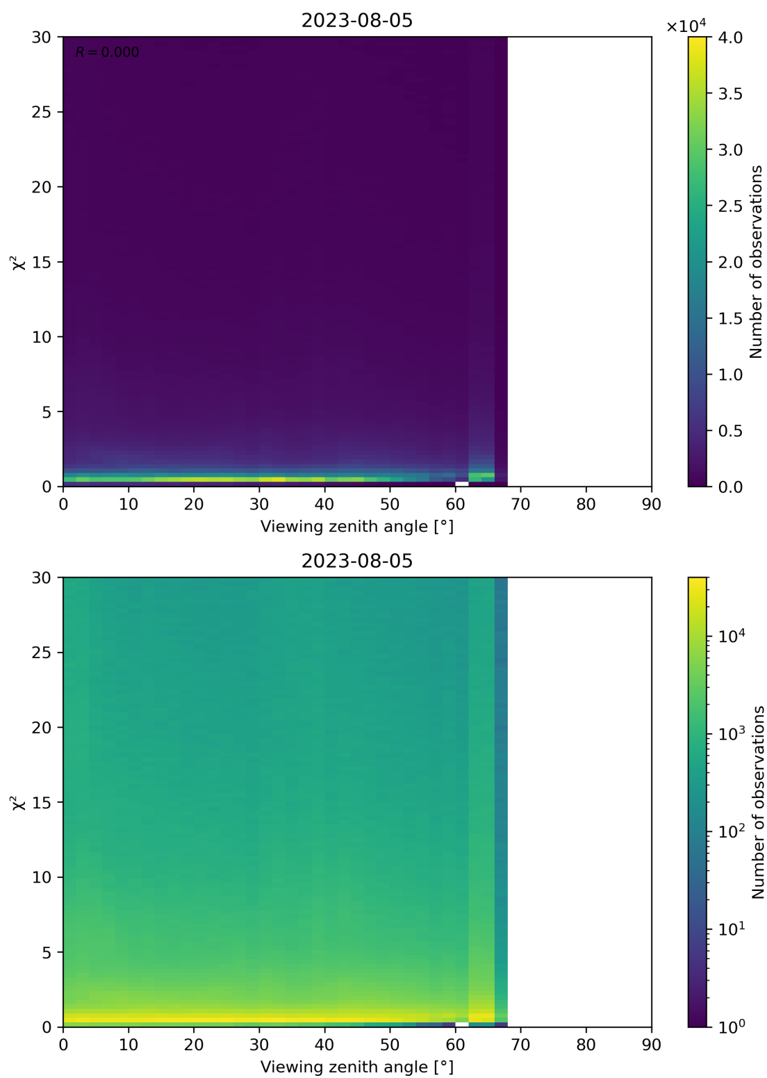
Figure 130: Scatter density plot of “Viewing zenith angle” against “ \chi^2 ” for 2023-08-04 to 2023-08-06.
