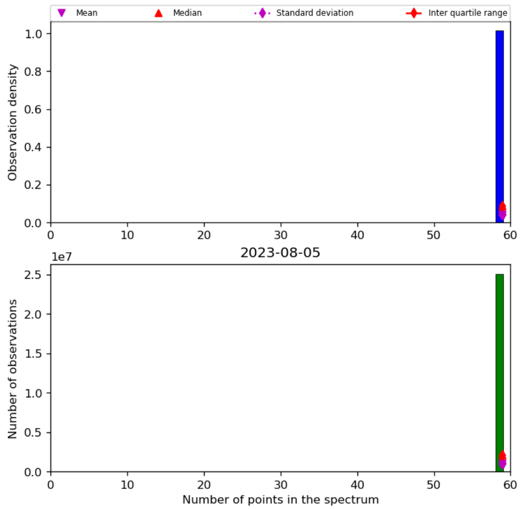
Figure 44: Histogram of "Number of points in the spectrum" for 2023-08-04 to 2023-08-06
