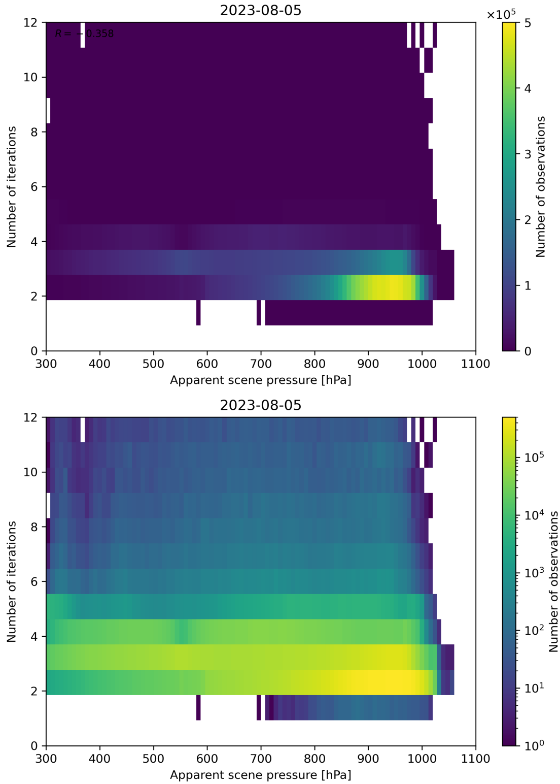
Figure 66: Scatter density plot of “Apparent scene pressure” against “Number of iterations” for 2023-08-04 to 2023-08-06.
