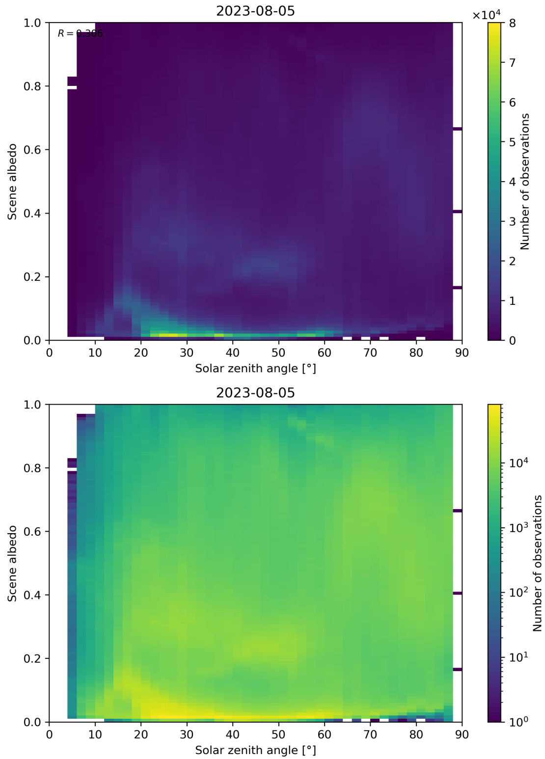
Figure 127: Scatter density plot of “Solar zenith angle” against “Scene albedo” for 2023-08-04 to 2023-08-06.
