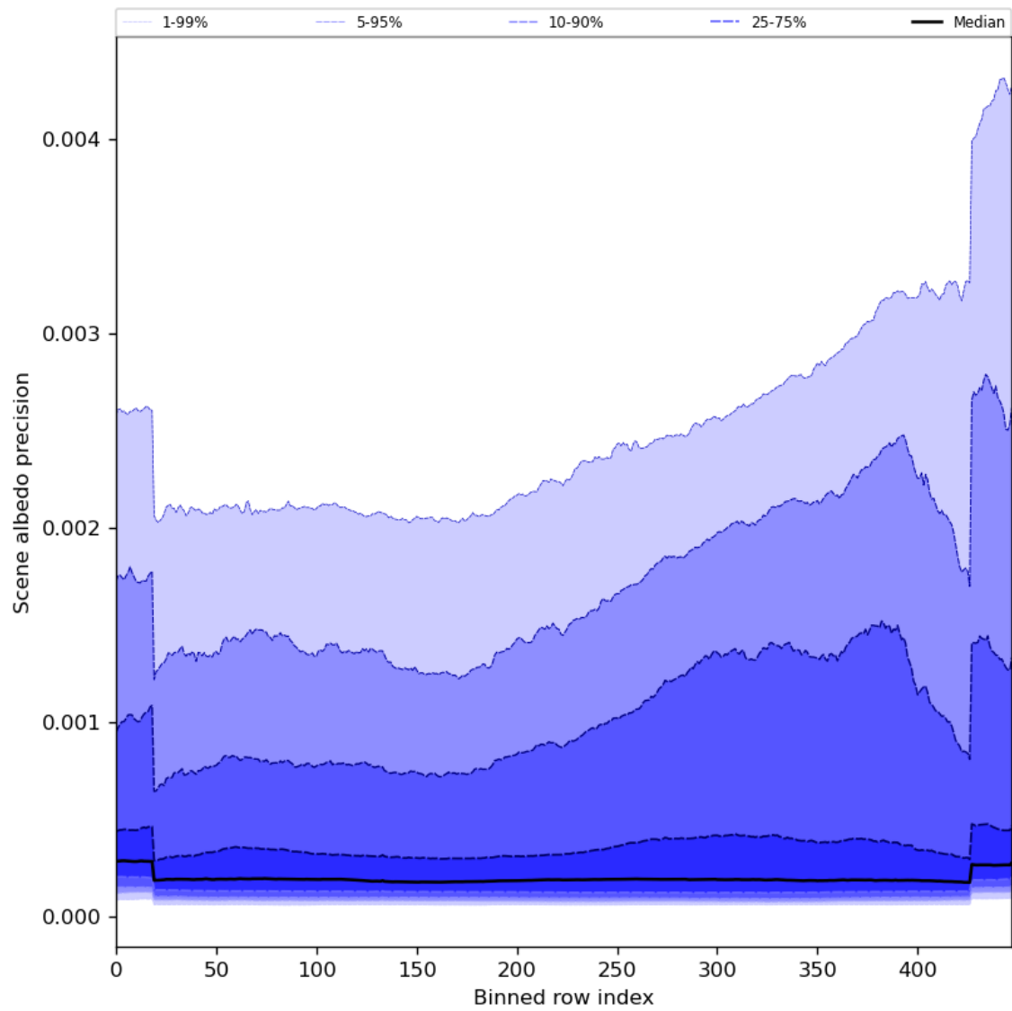
Figure 52: Along track statistics of “Scene albedo precision” for 2023-08-04 to 2023-08-06
