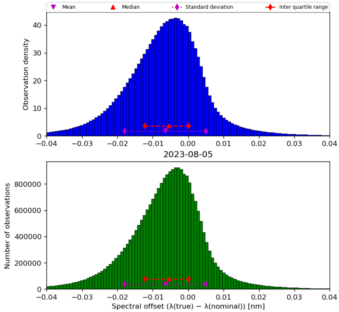
Figure 45: Histogram of “Spectral offset ( \lambda(\text{true}) - \lambda(\text{nominal}) )” for 2023-08-04 to 2023-08-06
