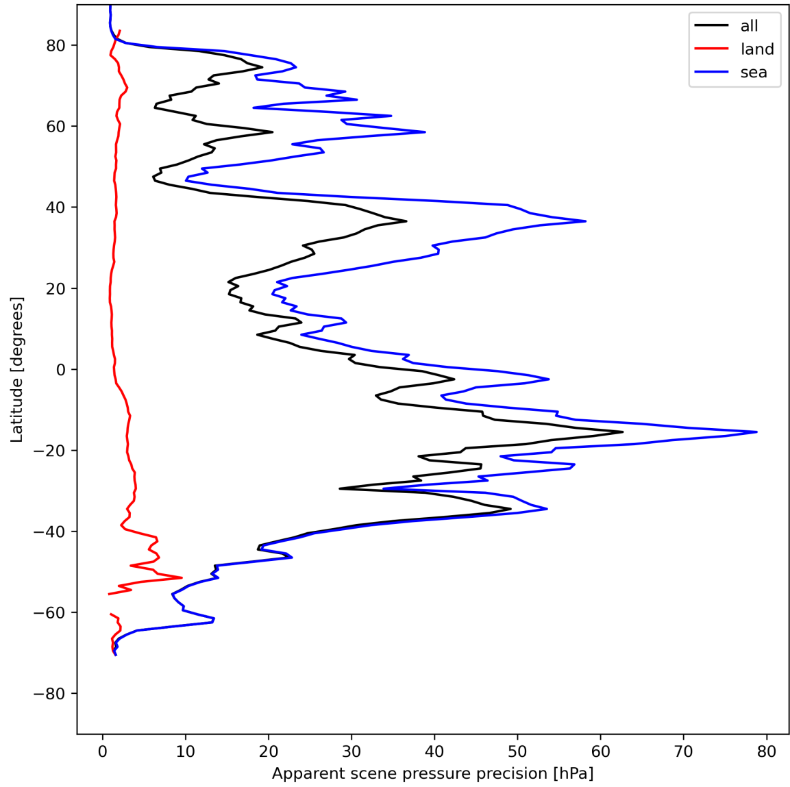
Figure 20: Zonal average of “Apparent scene pressure precision” for 2023-08-04 to 2023-08-06.
