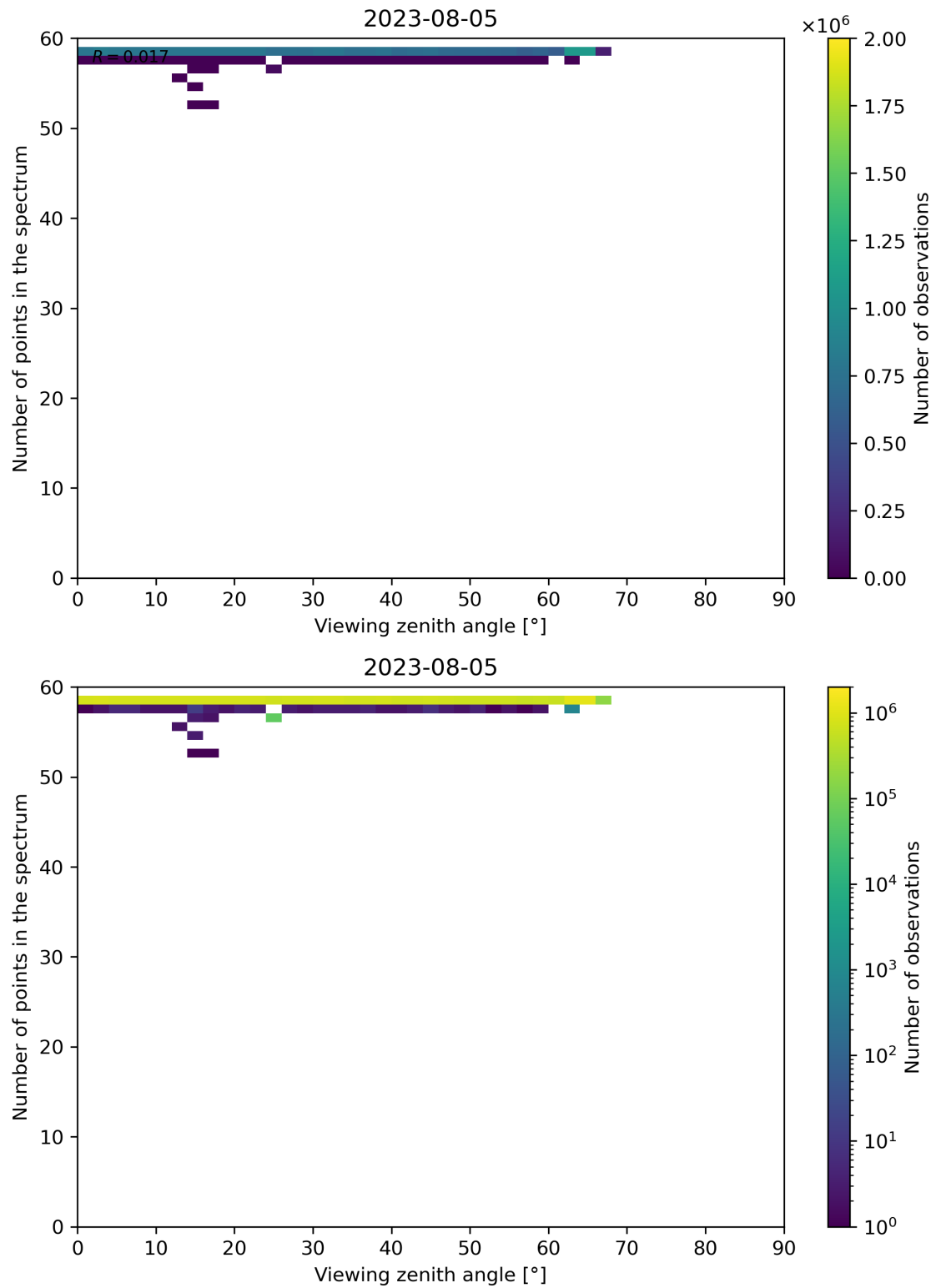
Figure 137: Scatter density plot of “Viewing zenith angle” against “Number of points in the spectrum” for 2023-08-04 to 2023-08-06.
