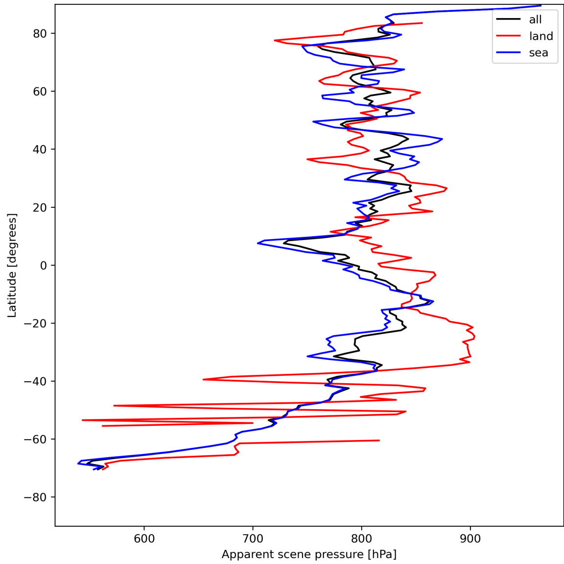
Figure 19: Zonal average of “Apparent scene pressure” for 2023-08-04 to 2023-08-06.
