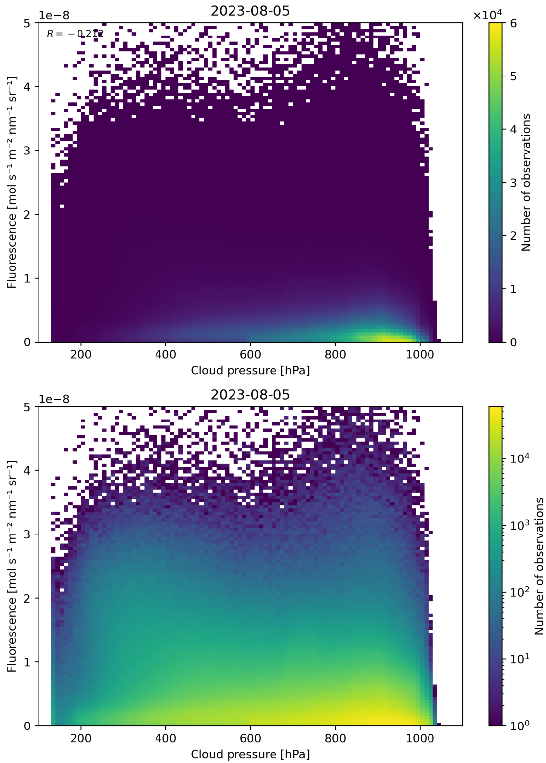
Figure 88: Scatter density plot of “Cloud pressure” against “Fluorescence” for 2023-08-04 to 2023-08-06.
