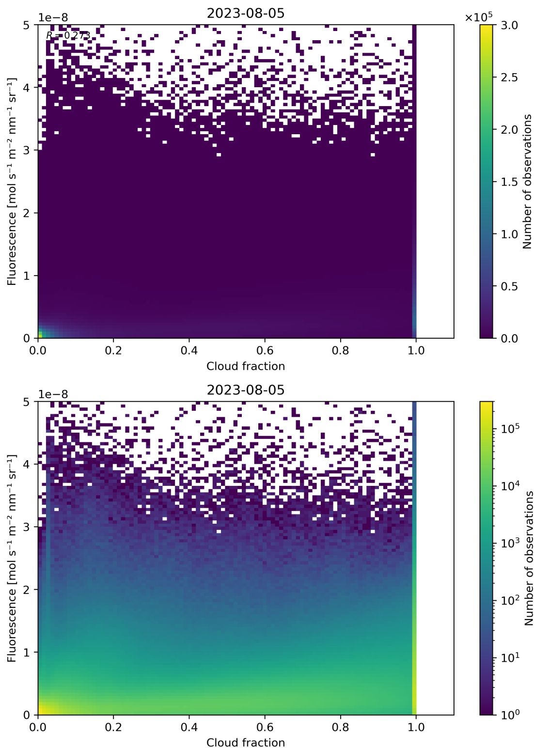
Figure 79: Scatter density plot of “Cloud fraction” against “Fluorescence” for 2023-08-04 to 2023-08-06.
