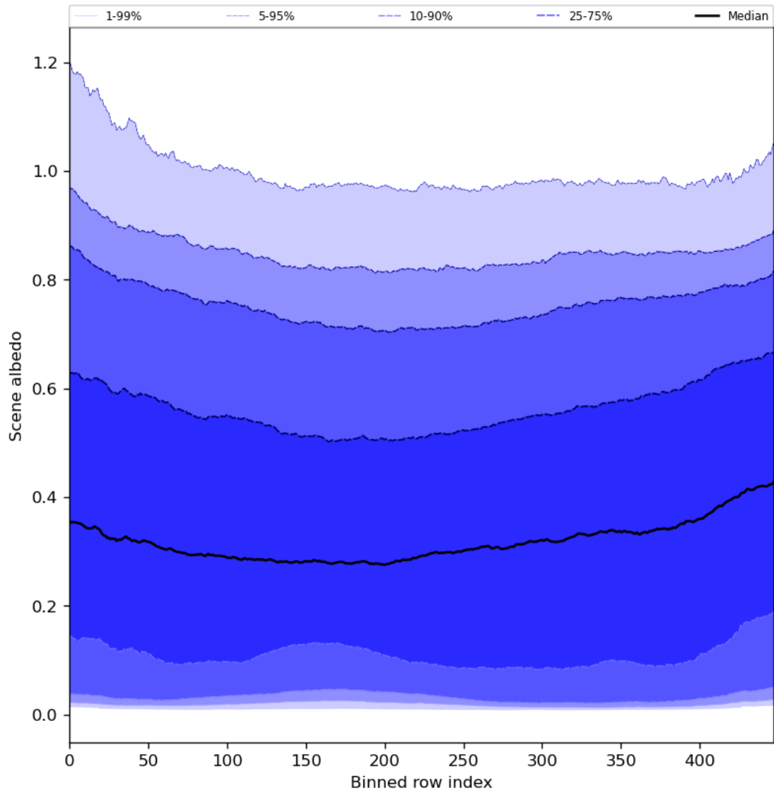
Figure 51: Along track statistics of “Scene albedo” for 2023-08-04 to 2023-08-06
