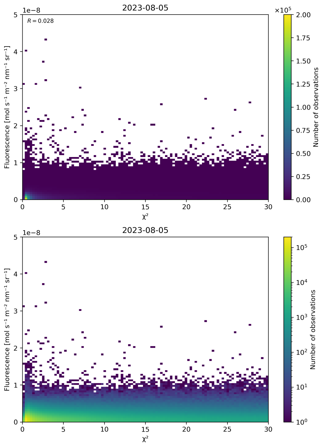
Figure 70: Scatter density plot of “ \chi^2 ” against “Fluorescence” for 2023-08-04 to 2023-08-06.
