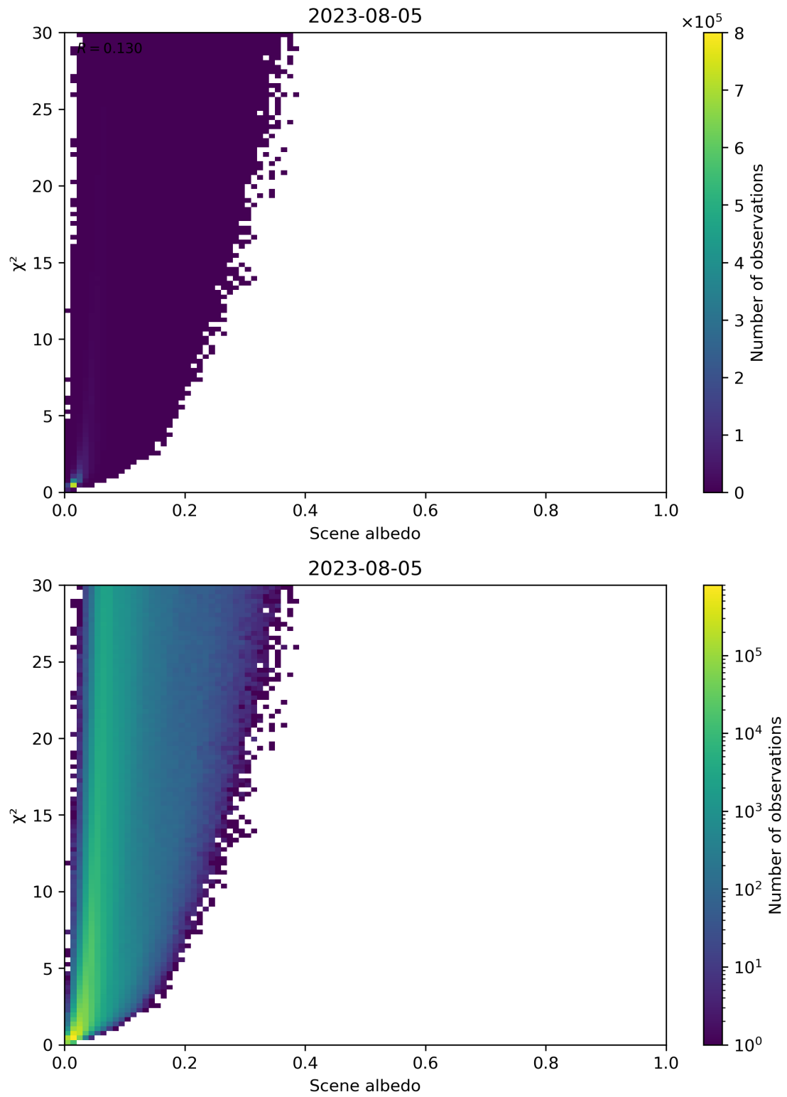
Figure 112: Scatter density plot of “Scene albedo” against “ \chi^2 ” for 2023-08-04 to 2023-08-06.
