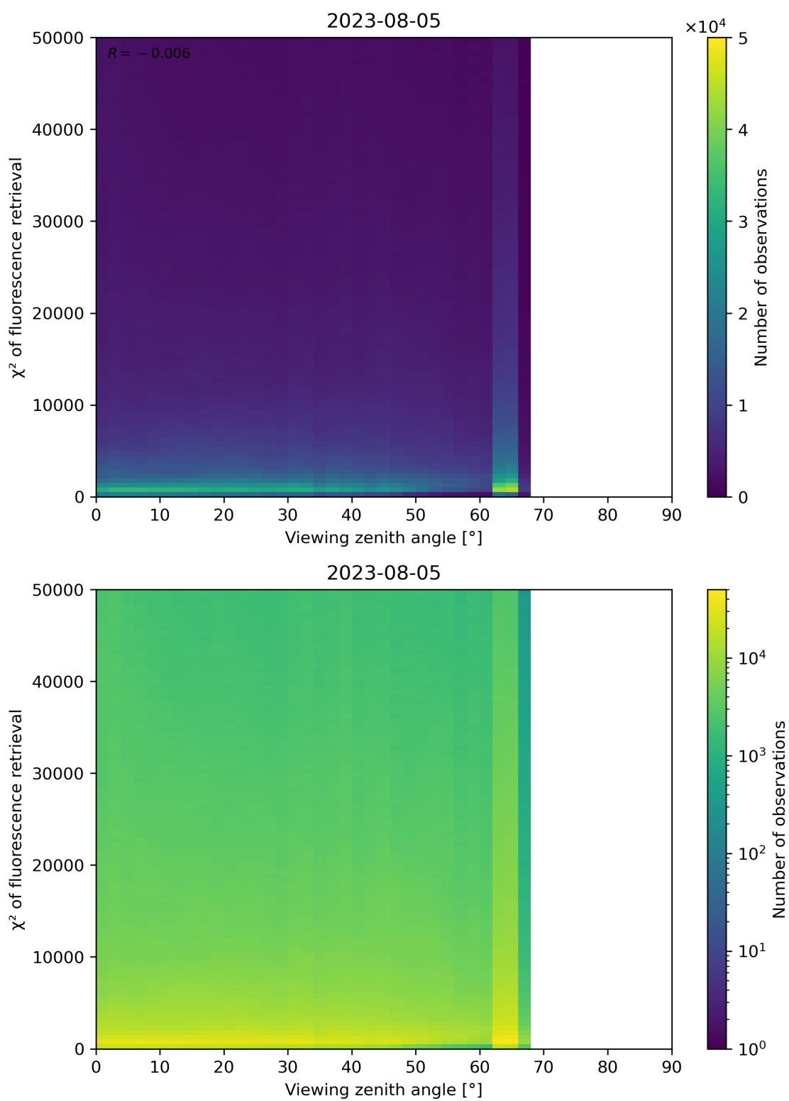
Figure 131: Scatter density plot of “Viewing zenith angle” against “ \chi^2 of fluorescence retrieval” for 2023-08-04 to 2023-08-06.
