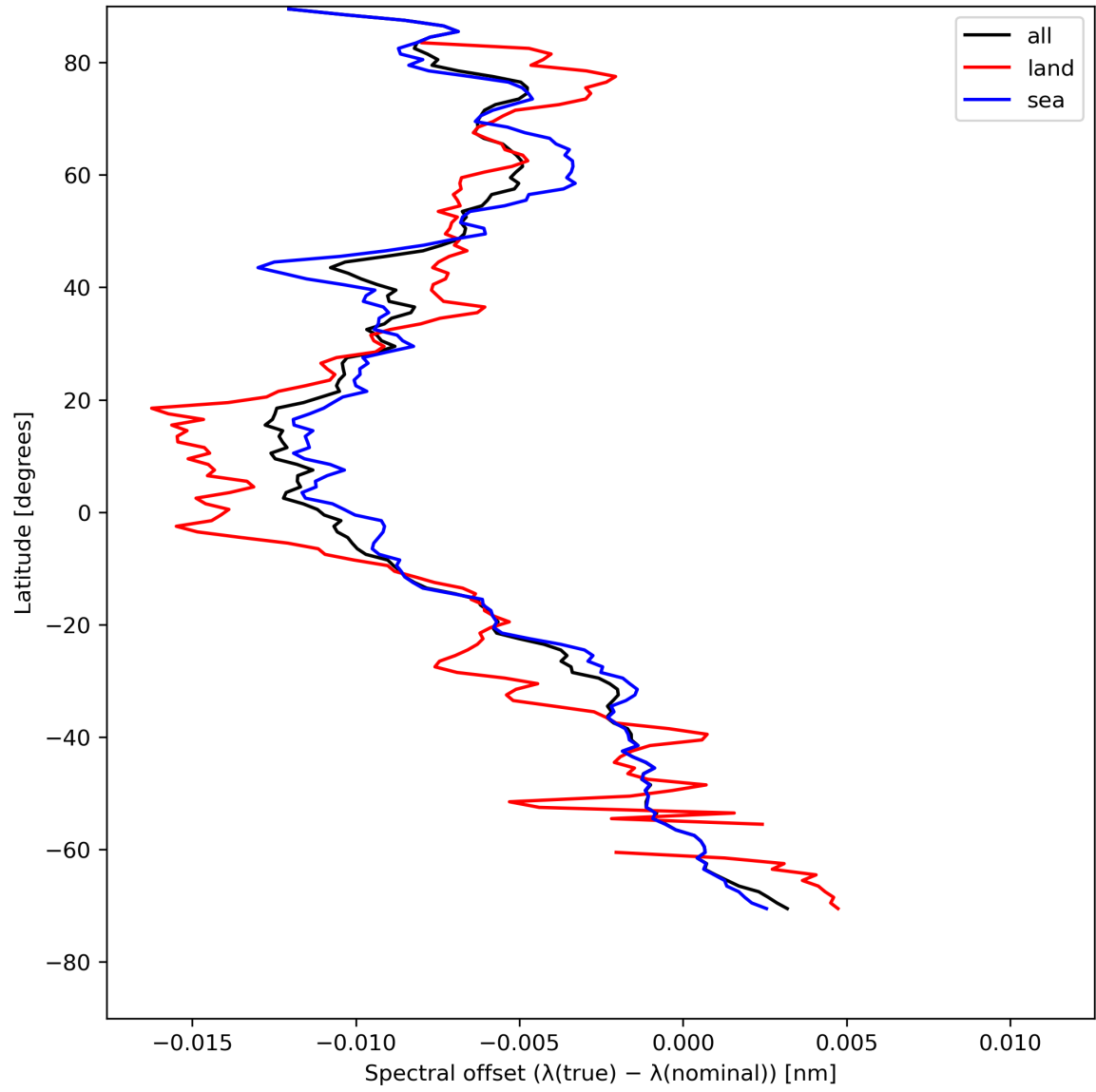
Figure 28: Zonal average of “Spectral offset ( \lambda(\text{true}) - \lambda(\text{nominal}) )” for 2023-08-04 to 2023-08-06.
