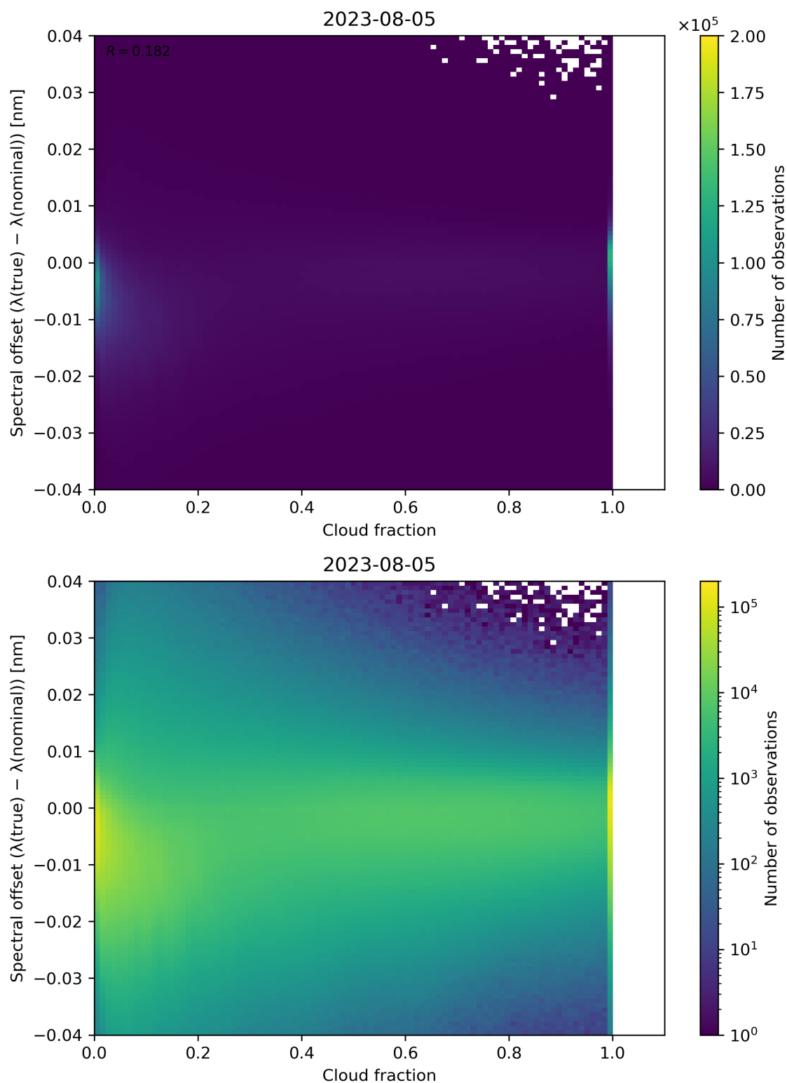
Figure 83: Scatter density plot of “Cloud fraction” against “Spectral offset ( \lambda(\text{true}) - \lambda(\text{nominal}) )” for 2023-08-04 to 2023-08-06.
