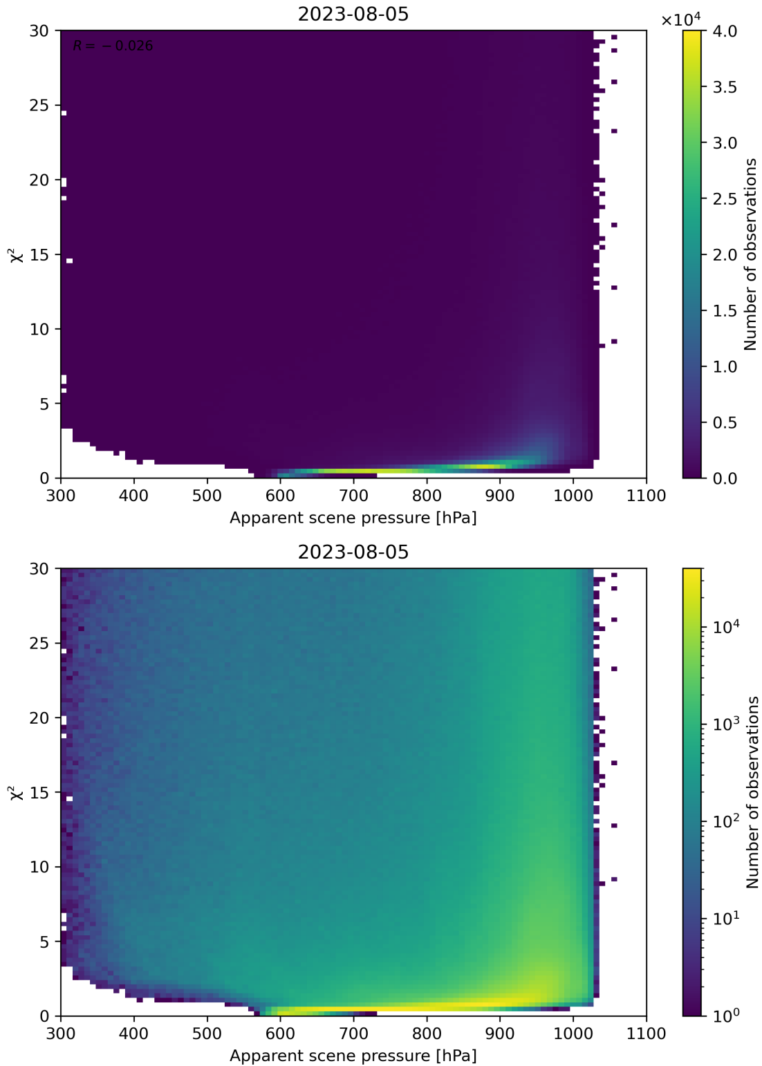
Figure 63: Scatter density plot of “Apparent scene pressure” against “ \chi^2 ” for 2023-08-04 to 2023-08-06.
