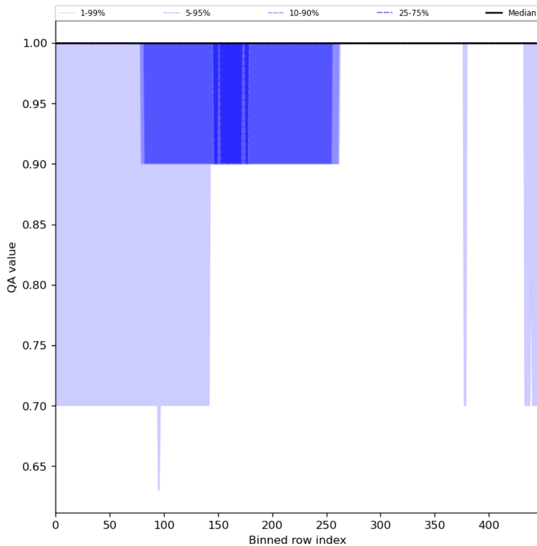
Figure 46: Along track statistics of “QA value” for 2023-08-04 to 2023-08-06
