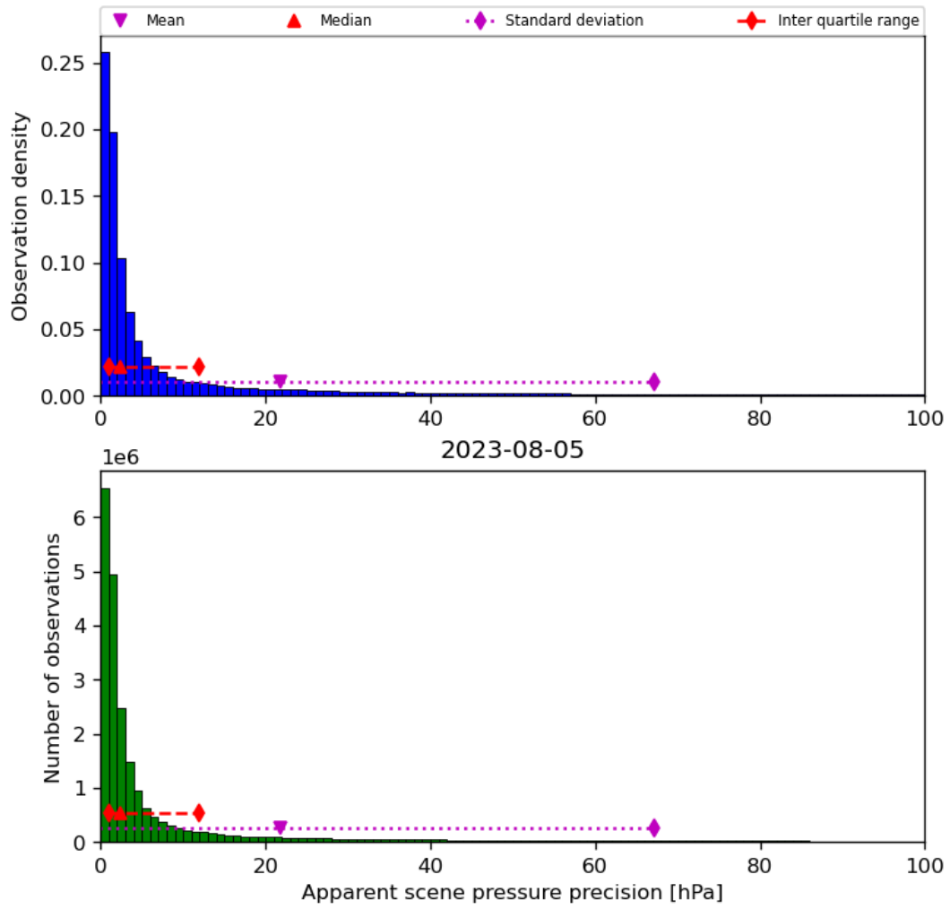
Figure 37: Histogram of “Apparent scene pressure precision” for 2023-08-04 to 2023-08-06
