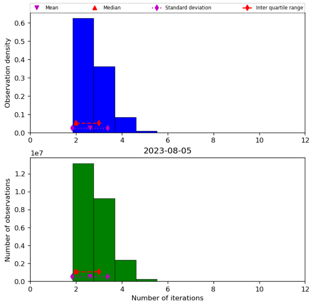
Figure 39: Histogram of “Number of iterations” for 2023-08-04 to 2023-08-06
