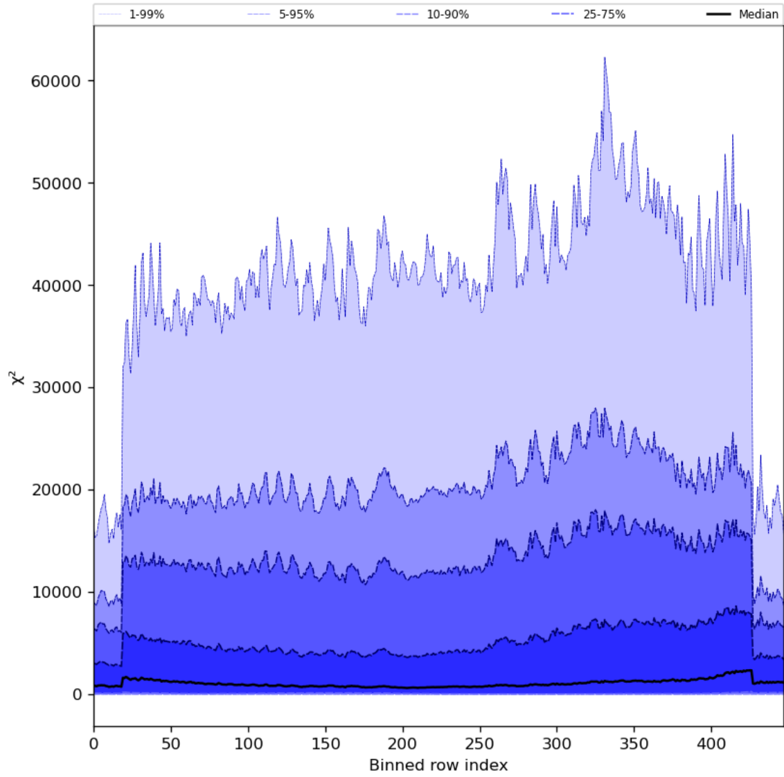
Figure 55: Along track statistics of “ \chi^2 ” for 2023-08-04 to 2023-08-06
