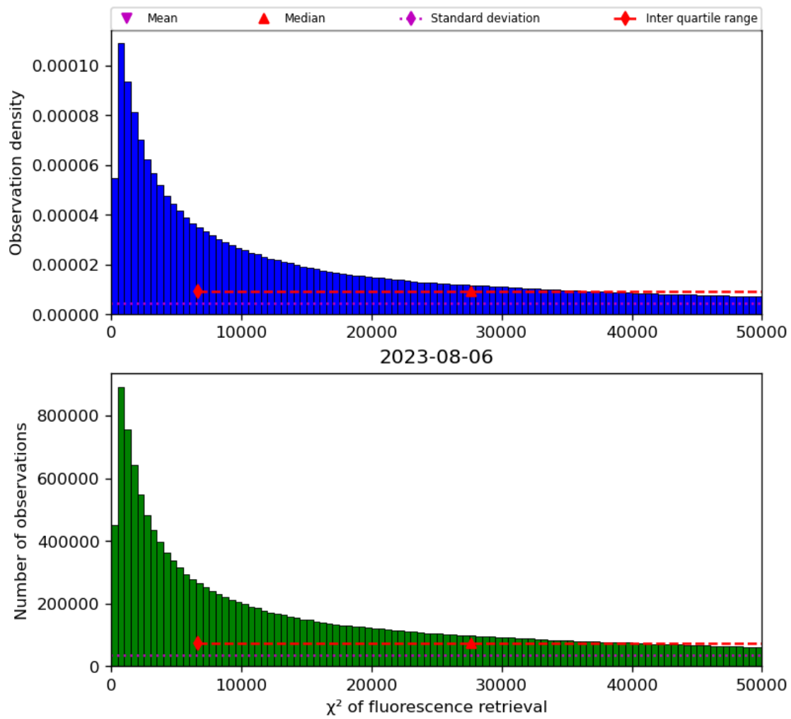
Figure 42: Histogram of “ \chi^2 of fluorescence retrieval” for 2023-08-05 to 2023-08-07
