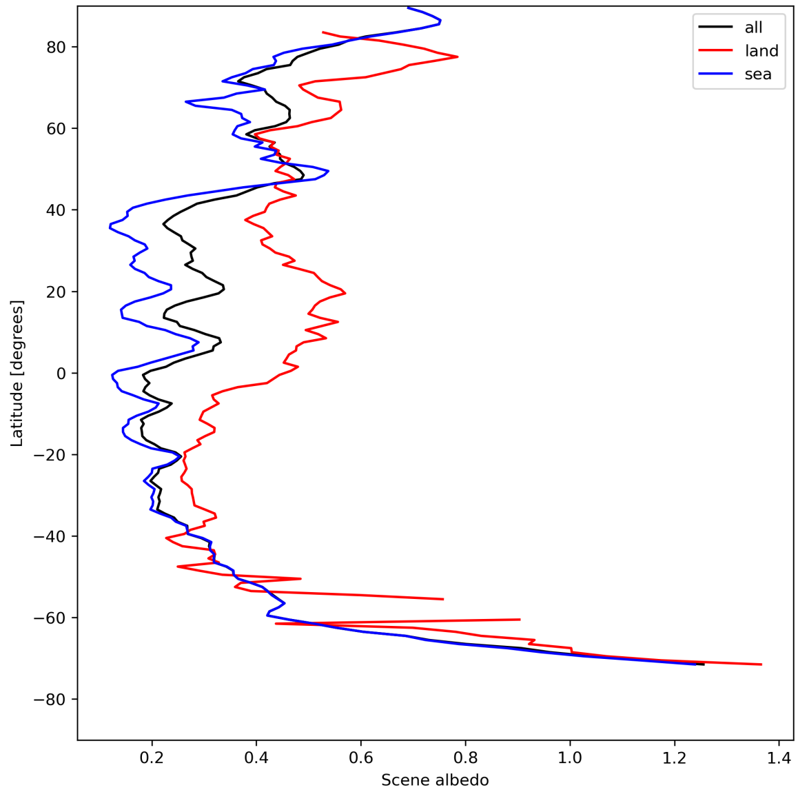
Figure 17: Zonal average of “Scene albedo” for 2023-08-05 to 2023-08-07.
