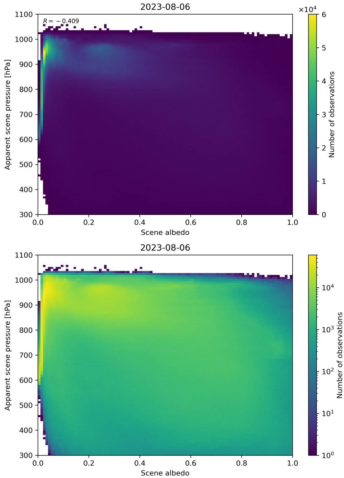
Figure 111: Scatter density plot of “Scene albedo” against “Apparent scene pressure” for 2023-08-05 to 2023-08-07.
