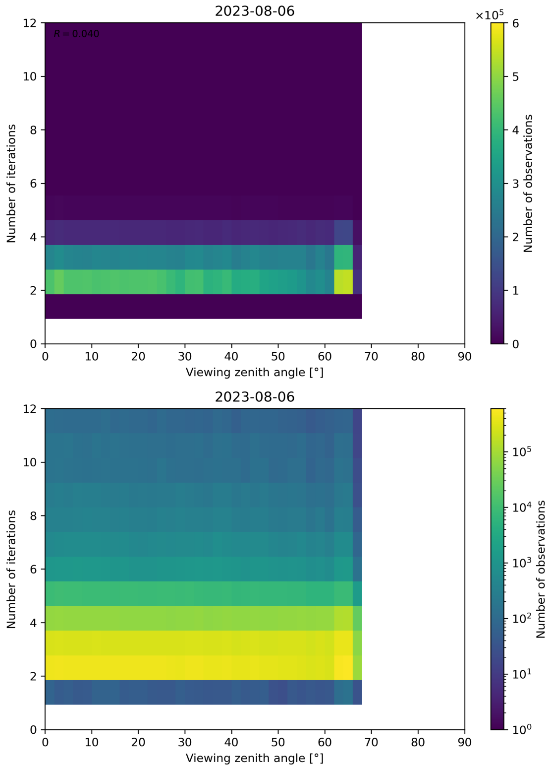
Figure 136: Scatter density plot of “Viewing zenith angle” against “Number of iterations” for 2023-08-05 to 2023-08-07.
