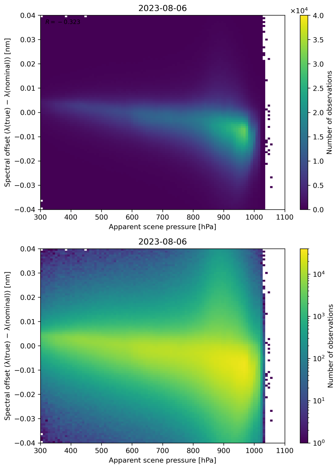
Figure 68: Scatter density plot of “Apparent scene pressure” against “Spectral offset ( \lambda(\text{true}) - \lambda(\text{nominal}) )” for 2023-08-05 to 2023-08-07.
