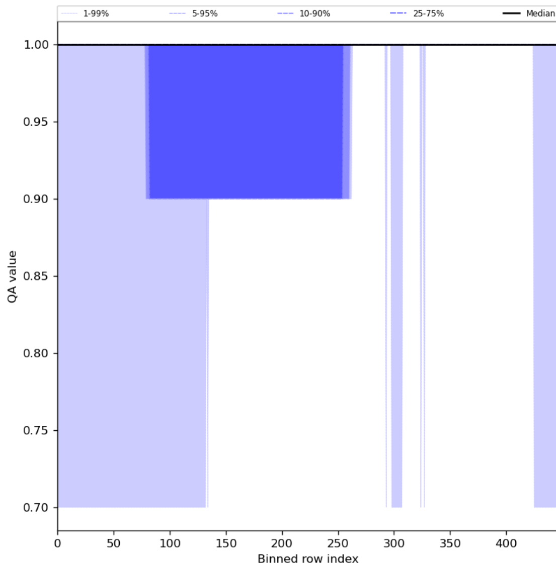
Figure 46: Along track statistics of “QA value” for 2023-08-05 to 2023-08-07
