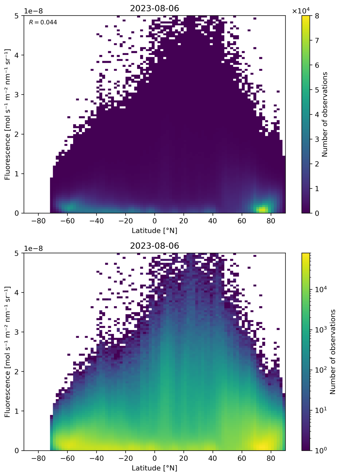
Figure 101: Scatter density plot of “Latitude” against “Fluorescence” for 2023-08-05 to 2023-08-07.
