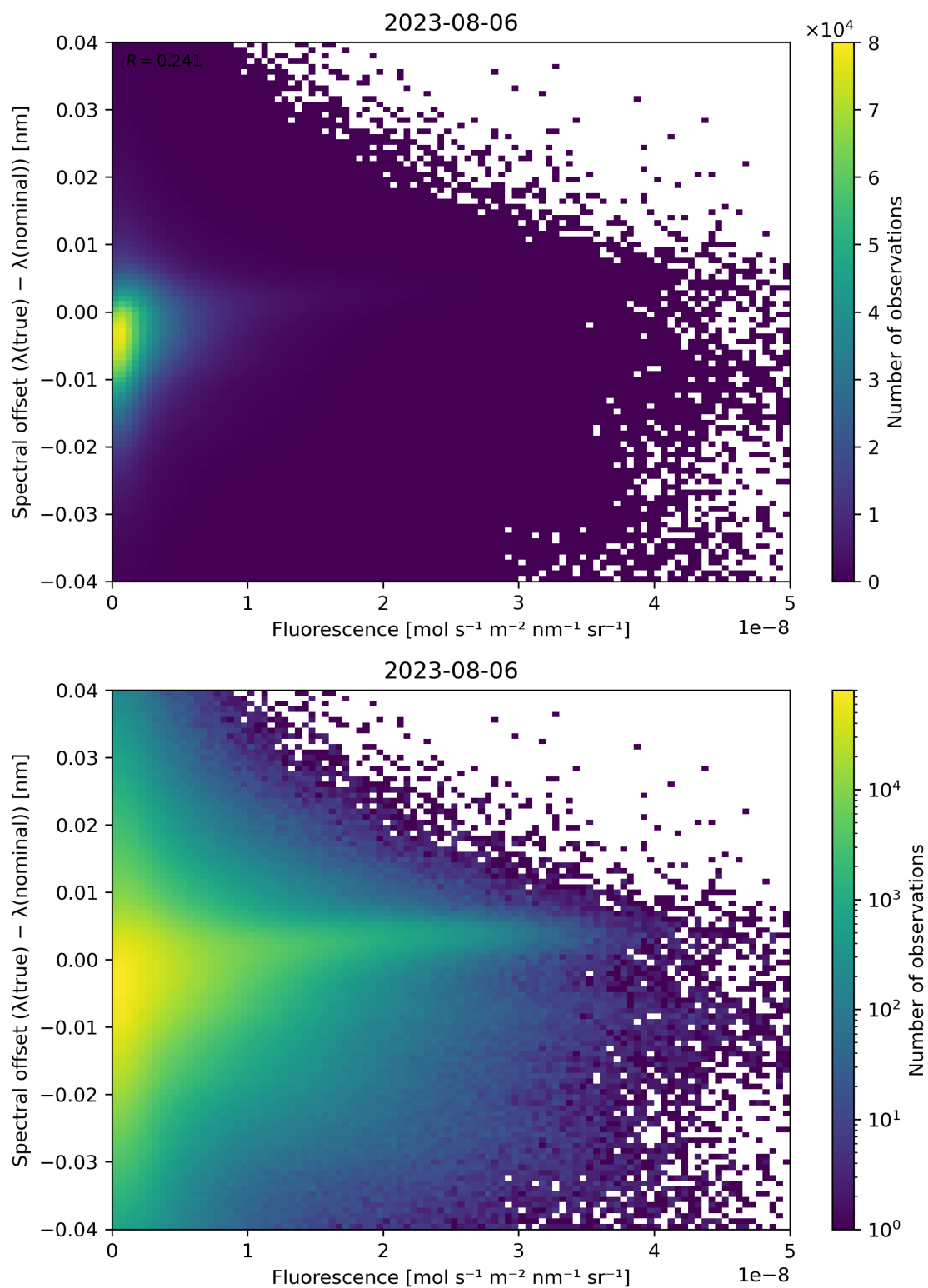
Figure 95: Scatter density plot of “Fluorescence” against “Spectral offset ( \lambda(\text{true}) - \lambda(\text{nominal}) )” for 2023-08-05 to 2023-08-07.
