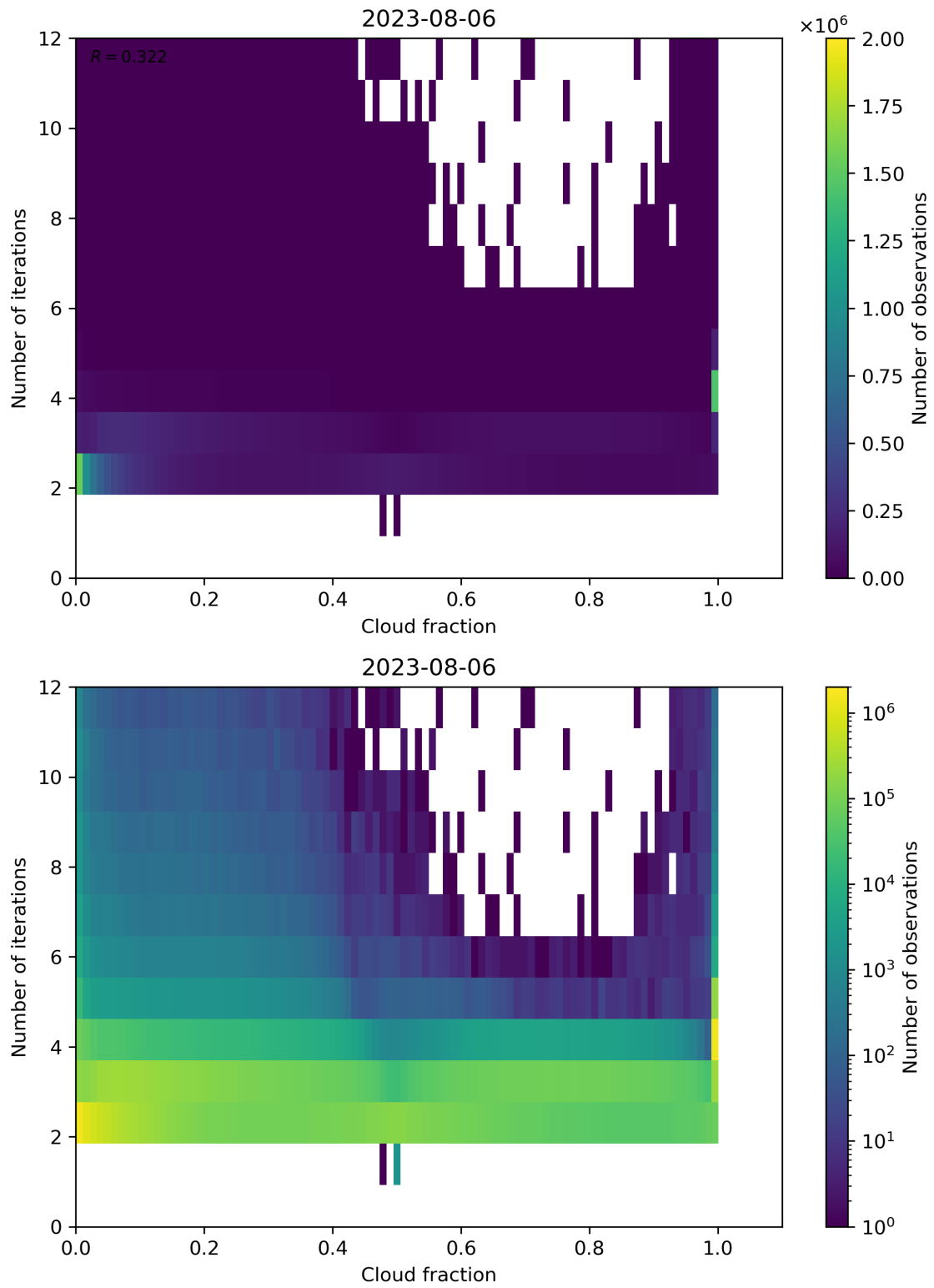
Figure 80: Scatter density plot of “Cloud fraction” against “Number of iterations” for 2023-08-05 to 2023-08-07.
