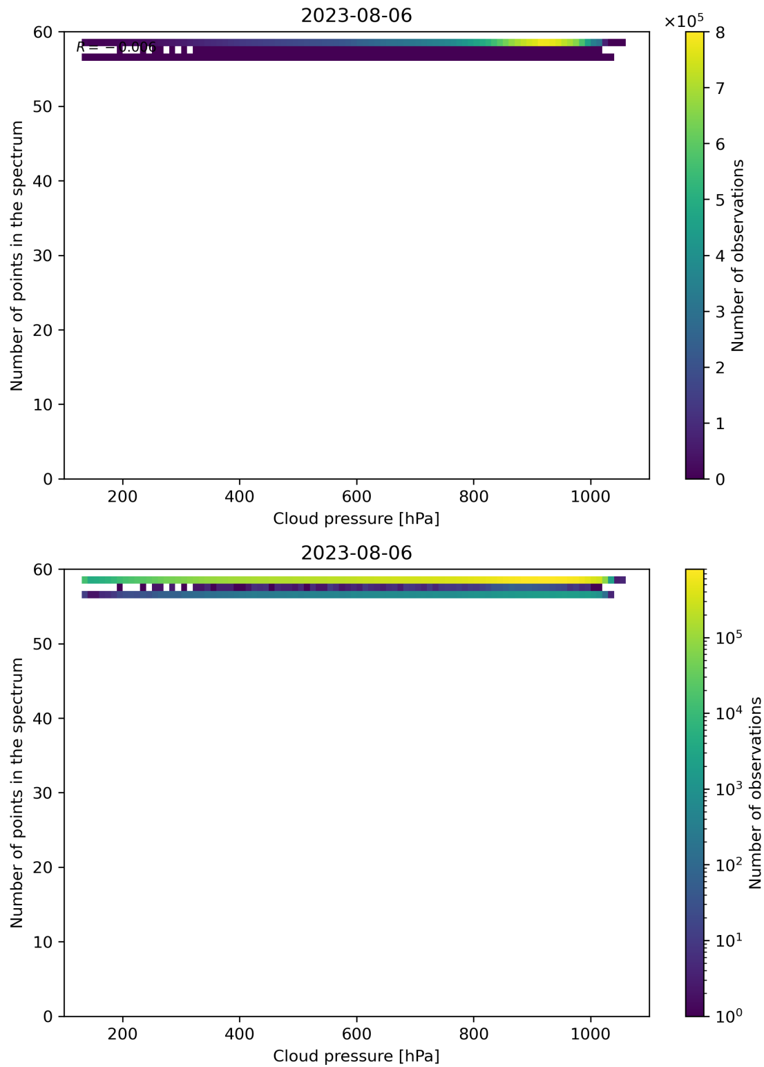
Figure 90: Scatter density plot of “Cloud pressure” against “Number of points in the spectrum” for 2023-08-05 to 2023-08-07.
