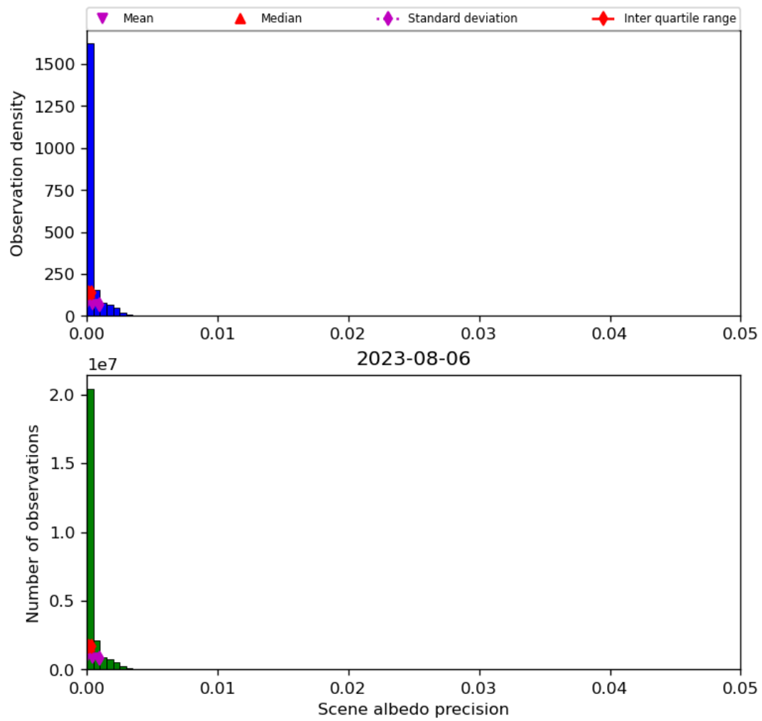
Figure 35: Histogram of “Scene albedo precision” for 2023-08-05 to 2023-08-07
