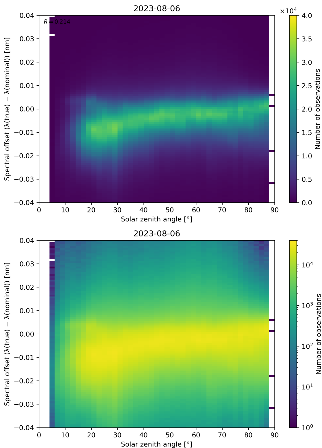
Figure 128: Scatter density plot of “Solar zenith angle” against “Spectral offset ( \lambda(\text{true}) - \lambda(\text{nominal}) )” for 2023-08-05 to 2023-08-07.
