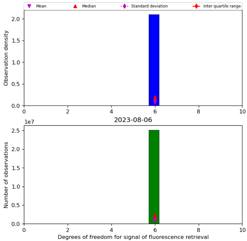
Figure 43: Histogram of “Degrees of freedom for signal of fluorescence retrieval” for 2023-08-05 to 2023-08-07
