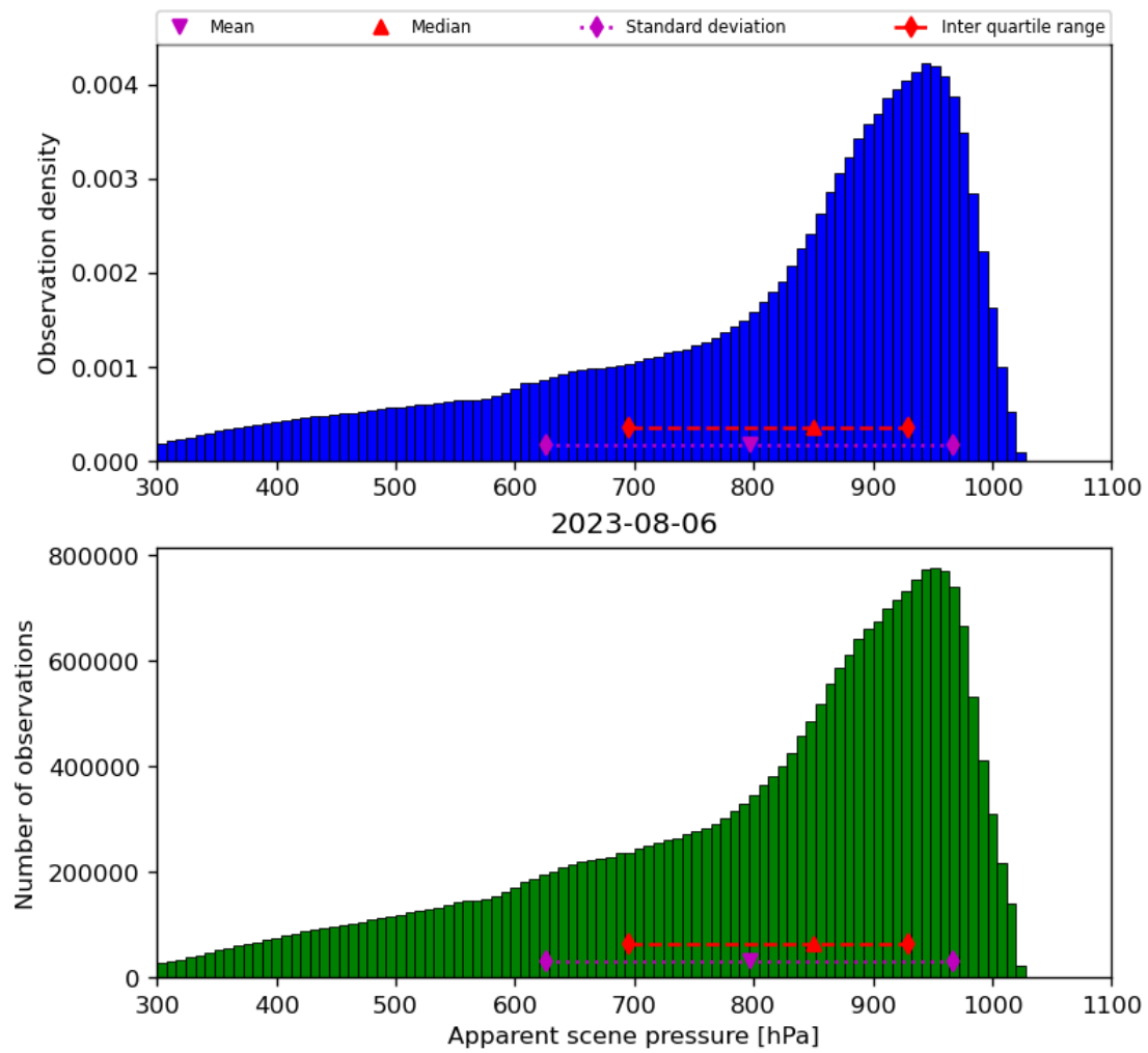
Figure 36: Histogram of “Apparent scene pressure” for 2023-08-05 to 2023-08-07
