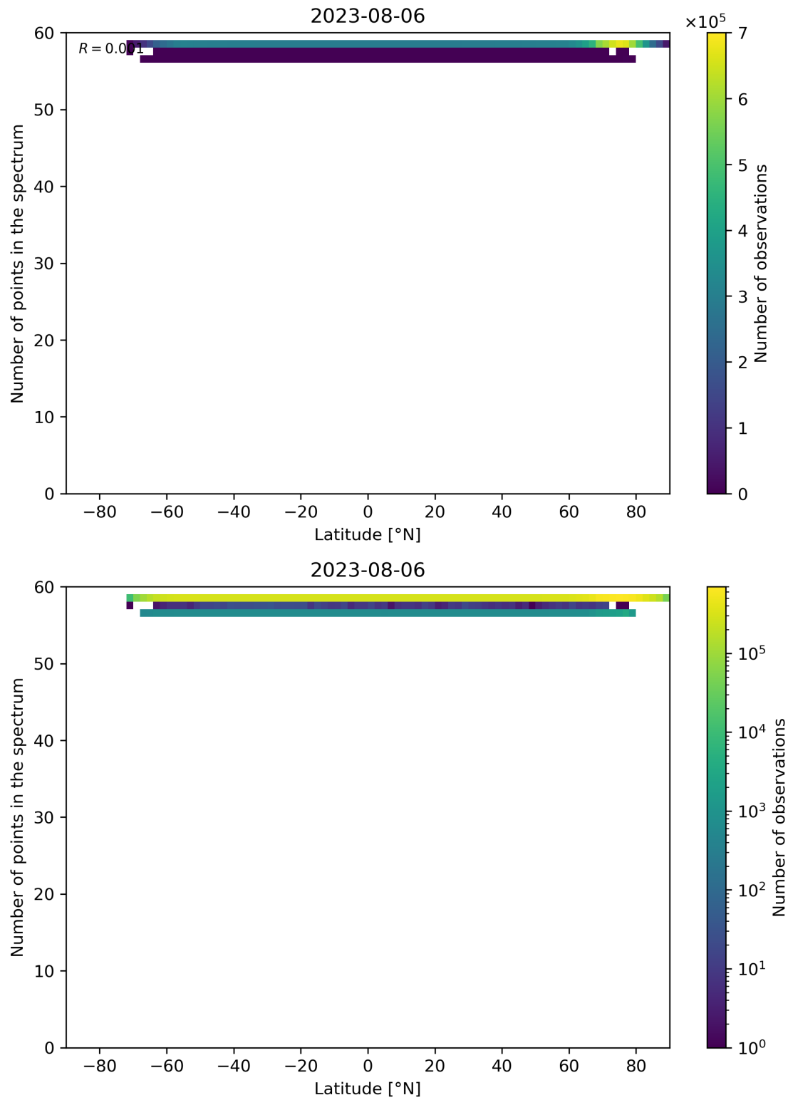
Figure 103: Scatter density plot of “Latitude” against “Number of points in the spectrum” for 2023-08-05 to 2023-08-07.
