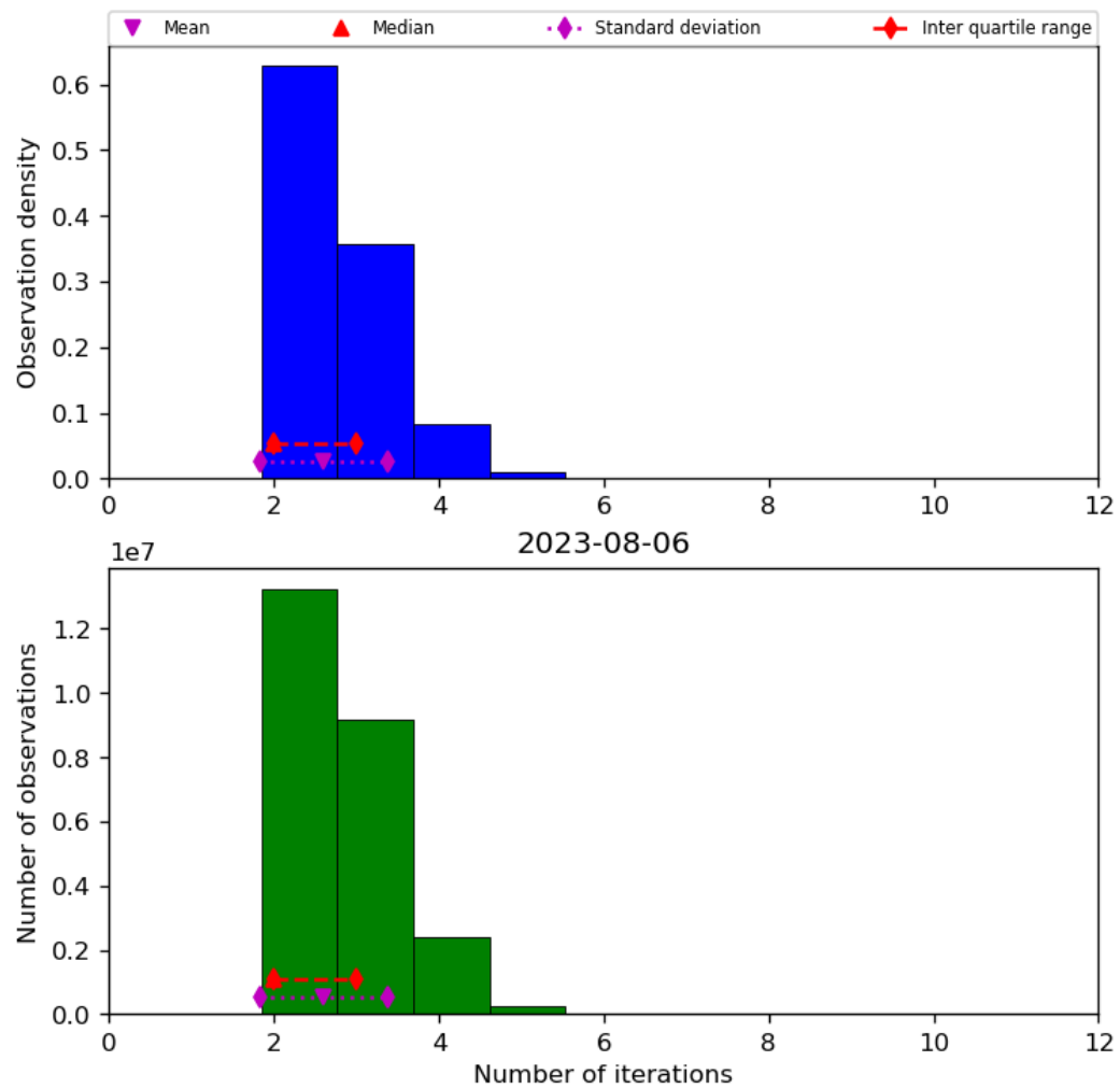
Figure 39: Histogram of “Number of iterations” for 2023-08-05 to 2023-08-07
