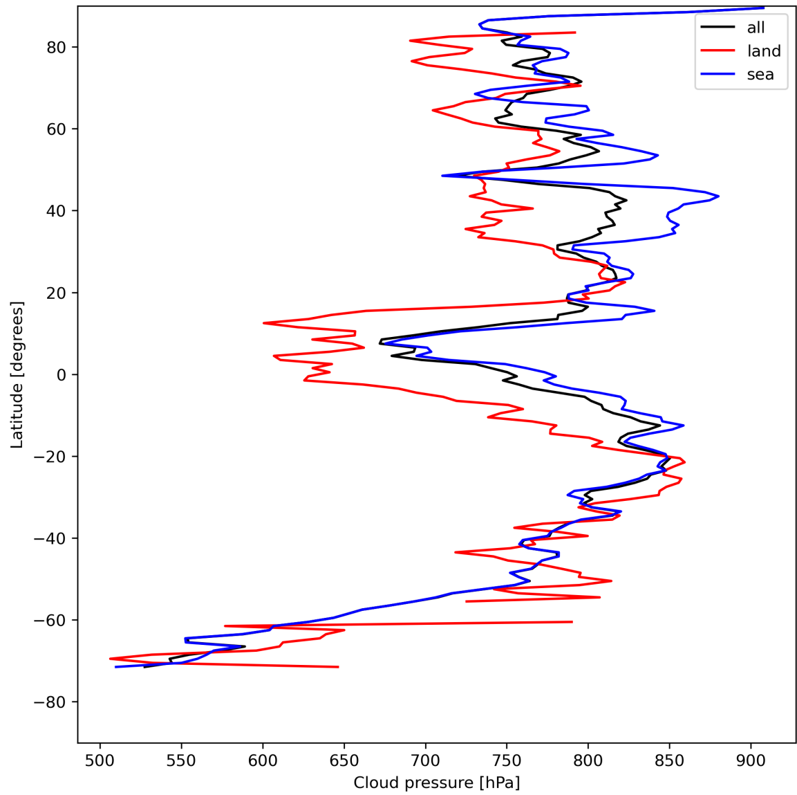
Figure 13: Zonal average of “Cloud pressure” for 2023-08-05 to 2023-08-07.
