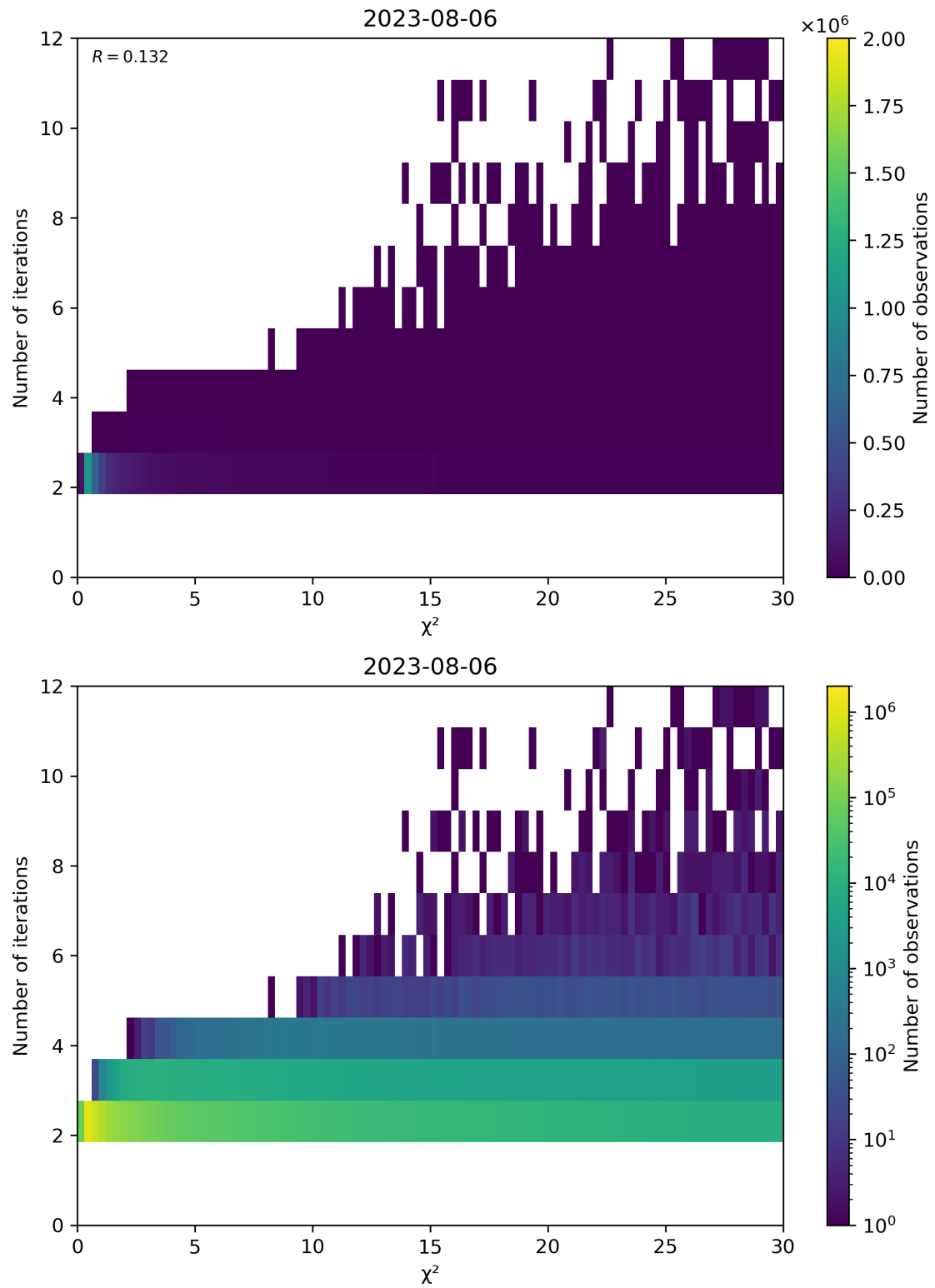
Figure 73: Scatter density plot of “ \chi^2 ” against “Number of iterations” for 2023-08-05 to 2023-08-07.
