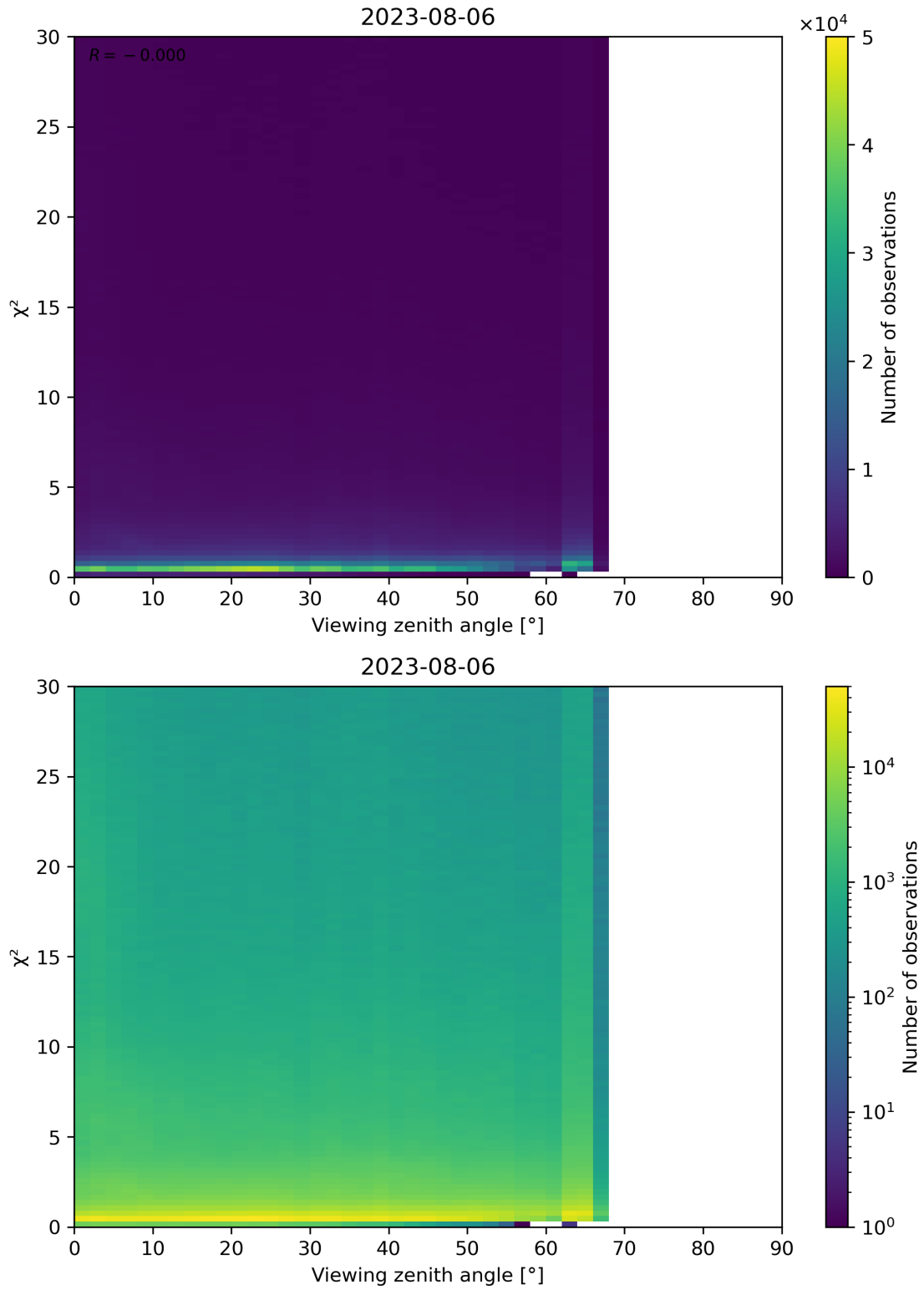
Figure 130: Scatter density plot of “Viewing zenith angle” against “ \chi^2 ” for 2023-08-05 to 2023-08-07.
