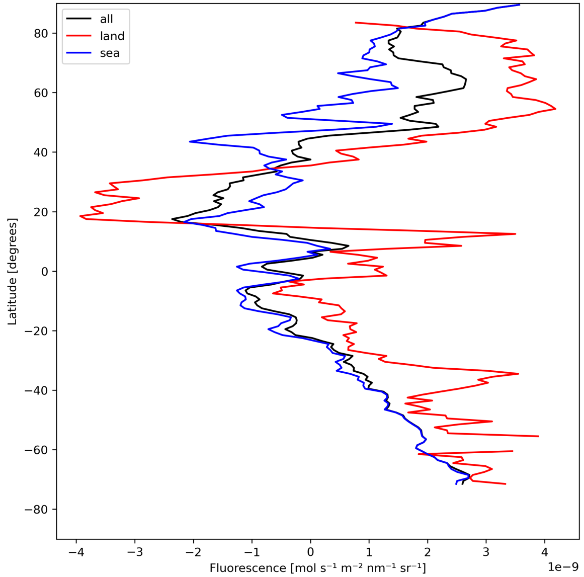
Figure 23: Zonal average of “Fluorescence” for 2023-08-05 to 2023-08-07.
