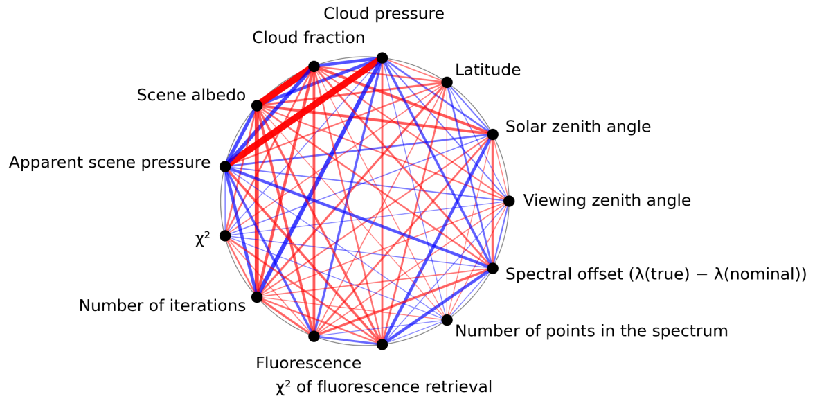
Figure 1: Map of correlation graph for 2023-08-05 to 2023-08-07.
