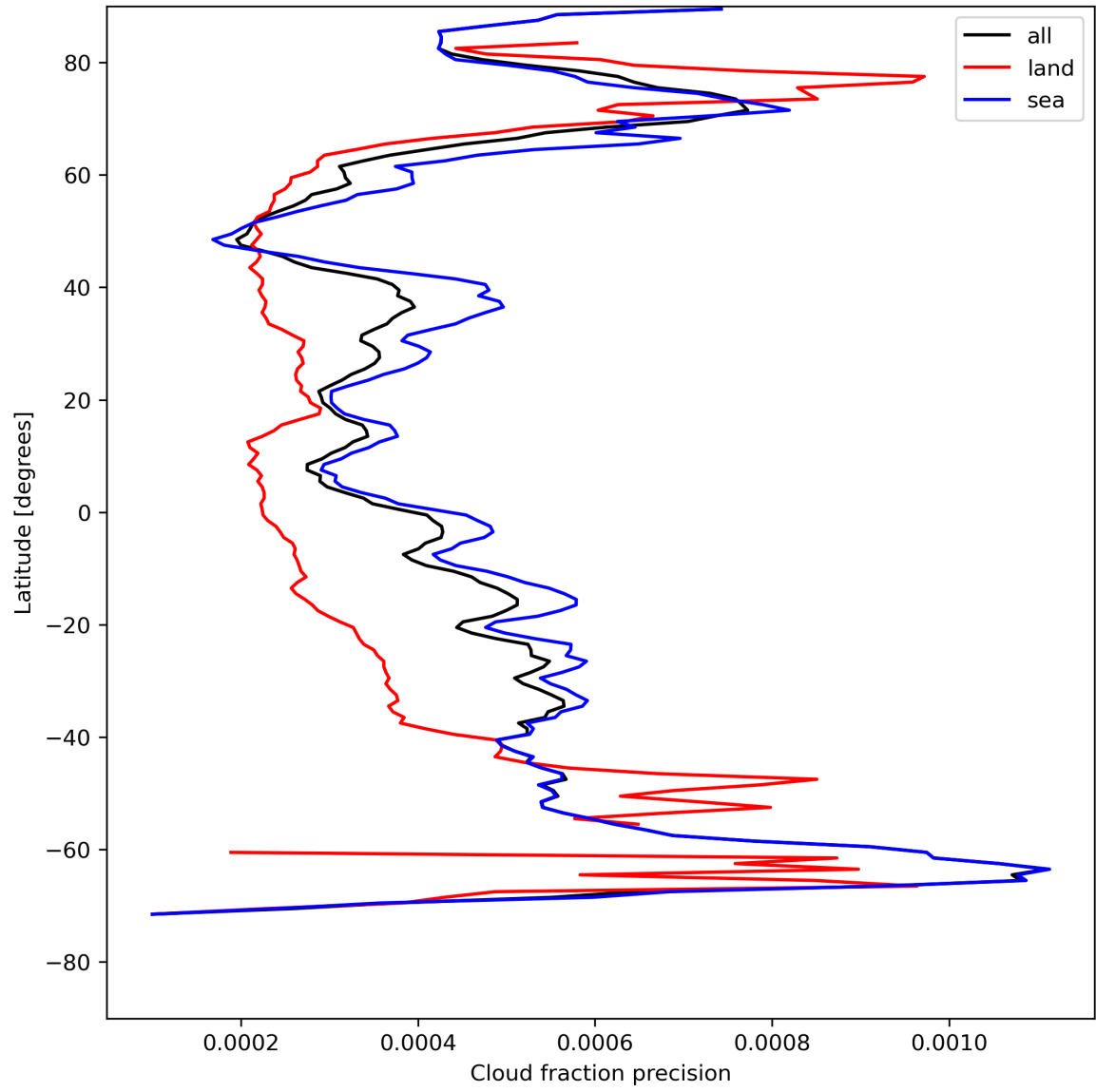
Figure 16: Zonal average of “Cloud fraction precision” for 2023-08-05 to 2023-08-07.
