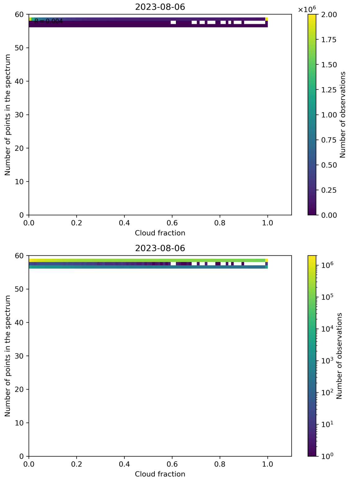
Figure 81: Scatter density plot of “Cloud fraction” against “Number of points in the spectrum” for 2023-08-05 to 2023-08-07.
