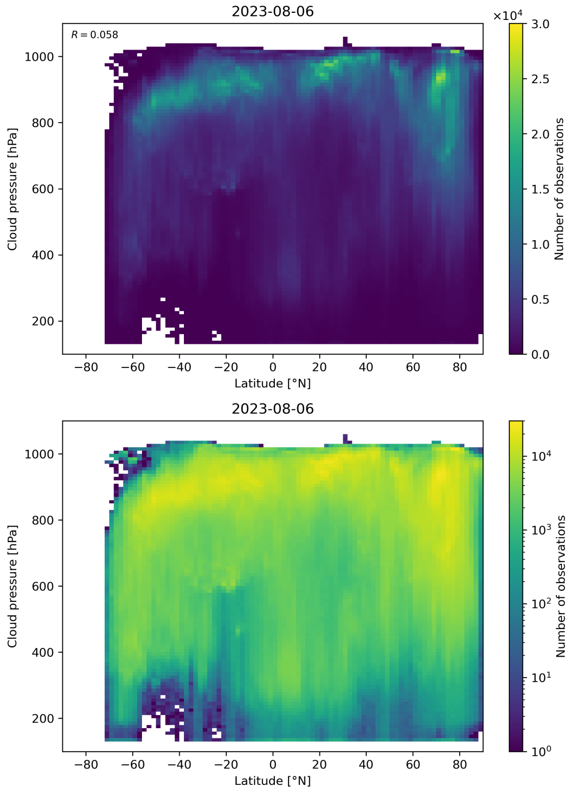
Figure 100: Scatter density plot of “Latitude” against “Cloud pressure” for 2023-08-05 to 2023-08-07.
