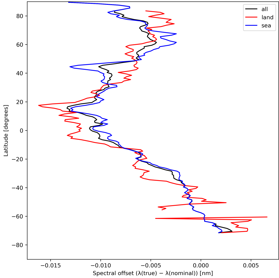
Figure 28: Zonal average of “Spectral offset ( \lambda(\text{true}) - \lambda(\text{nominal}) )” for 2023-08-05 to 2023-08-07.
