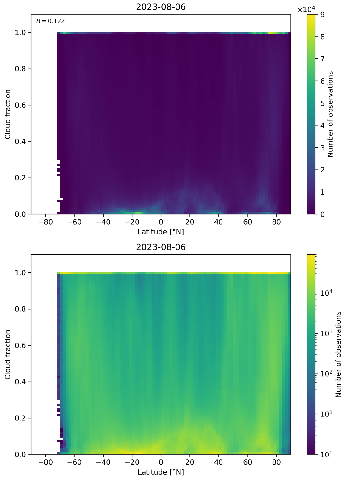
Figure 99: Scatter density plot of “Latitude” against “Cloud fraction” for 2023-08-05 to 2023-08-07.
