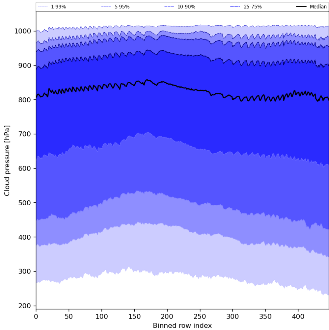
Figure 47: Along track statistics of “Cloud pressure” for 2023-08-05 to 2023-08-07
