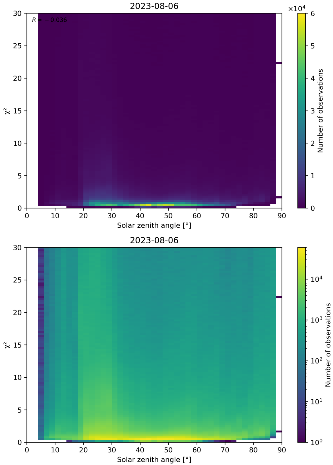
Figure 119: Scatter density plot of “Solar zenith angle” against “ \chi^2 ” for 2023-08-05 to 2023-08-07.
