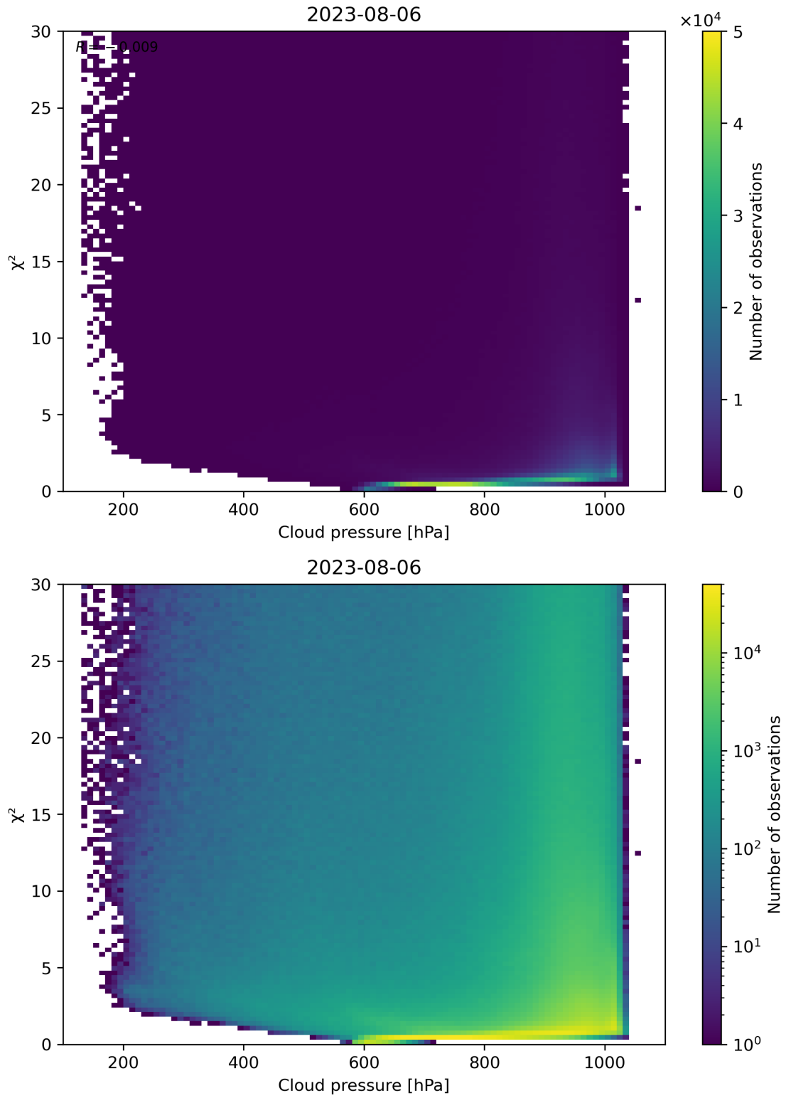
Figure 85: Scatter density plot of “Cloud pressure” against “ \chi^2 ” for 2023-08-05 to 2023-08-07.
