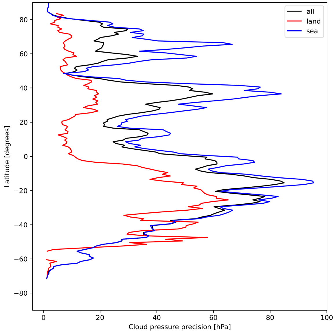
Figure 14: Zonal average of “Cloud pressure precision” for 2023-08-05 to 2023-08-07.
