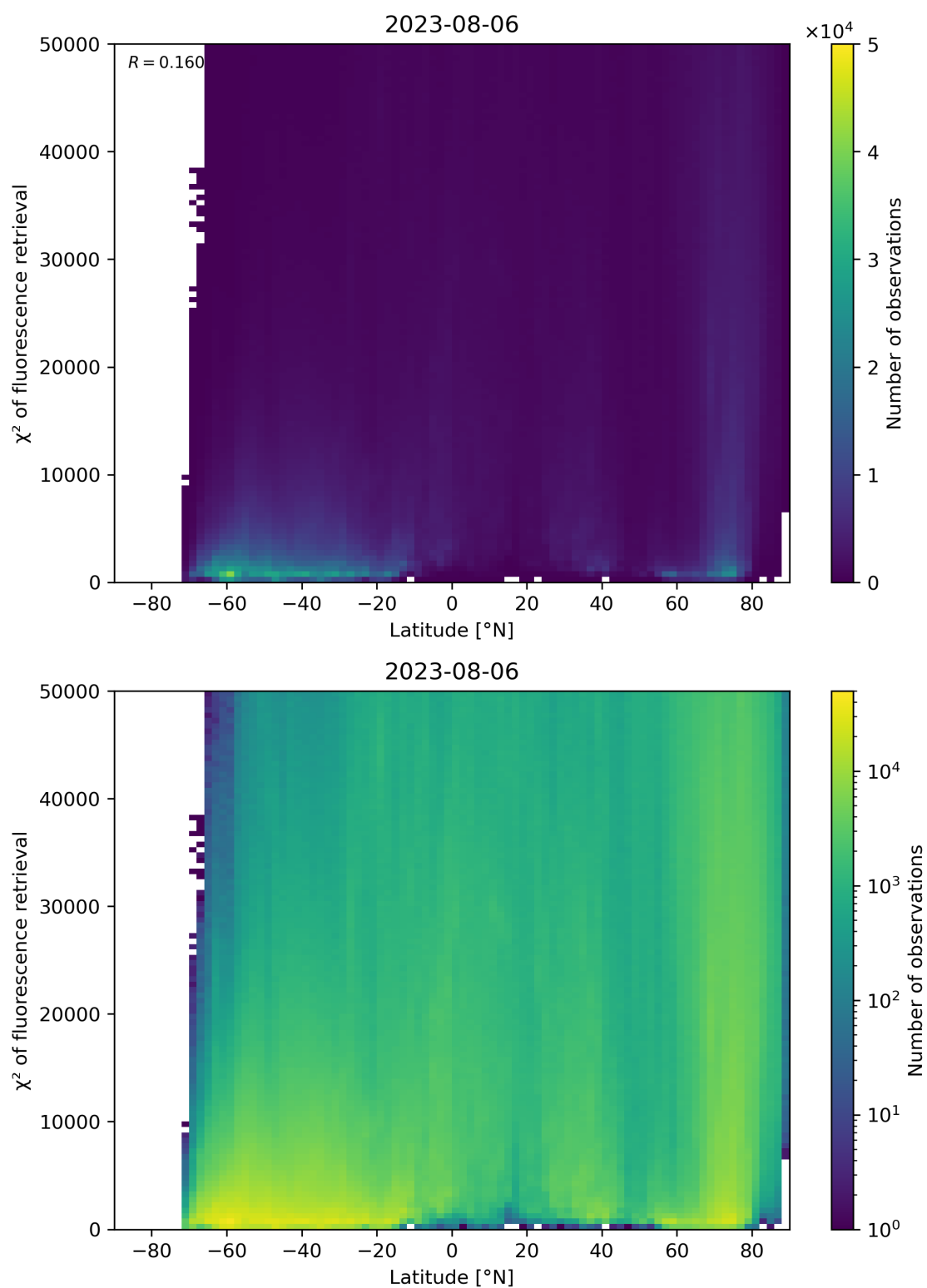
Figure 98: Scatter density plot of “Latitude” against “ \chi^2 of fluorescence retrieval” for 2023-08-05 to 2023-08-07.
