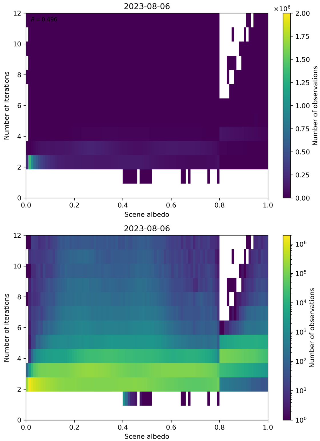
Figure 115: Scatter density plot of “Scene albedo” against “Number of iterations” for 2023-08-05 to 2023-08-07.
