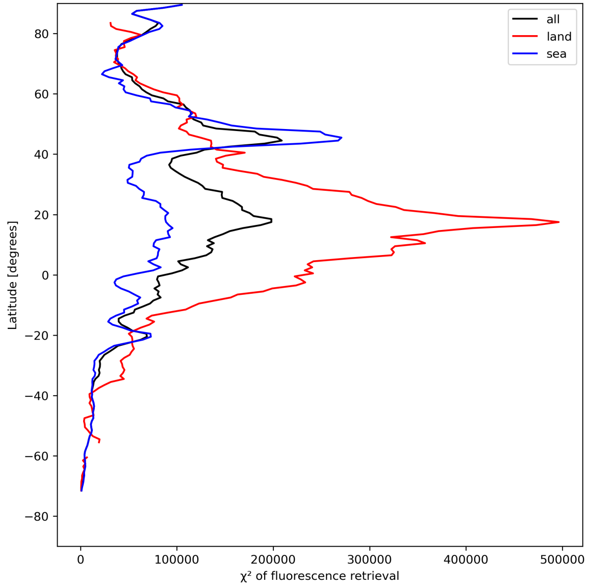
Figure 25: Zonal average of “ \chi^2 of fluorescence retrieval” for 2023-08-05 to 2023-08-07.
