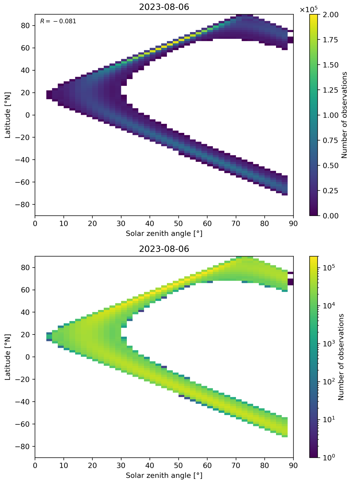
Figure 124: Scatter density plot of “Solar zenith angle” against “Latitude” for 2023-08-05 to 2023-08-07.
