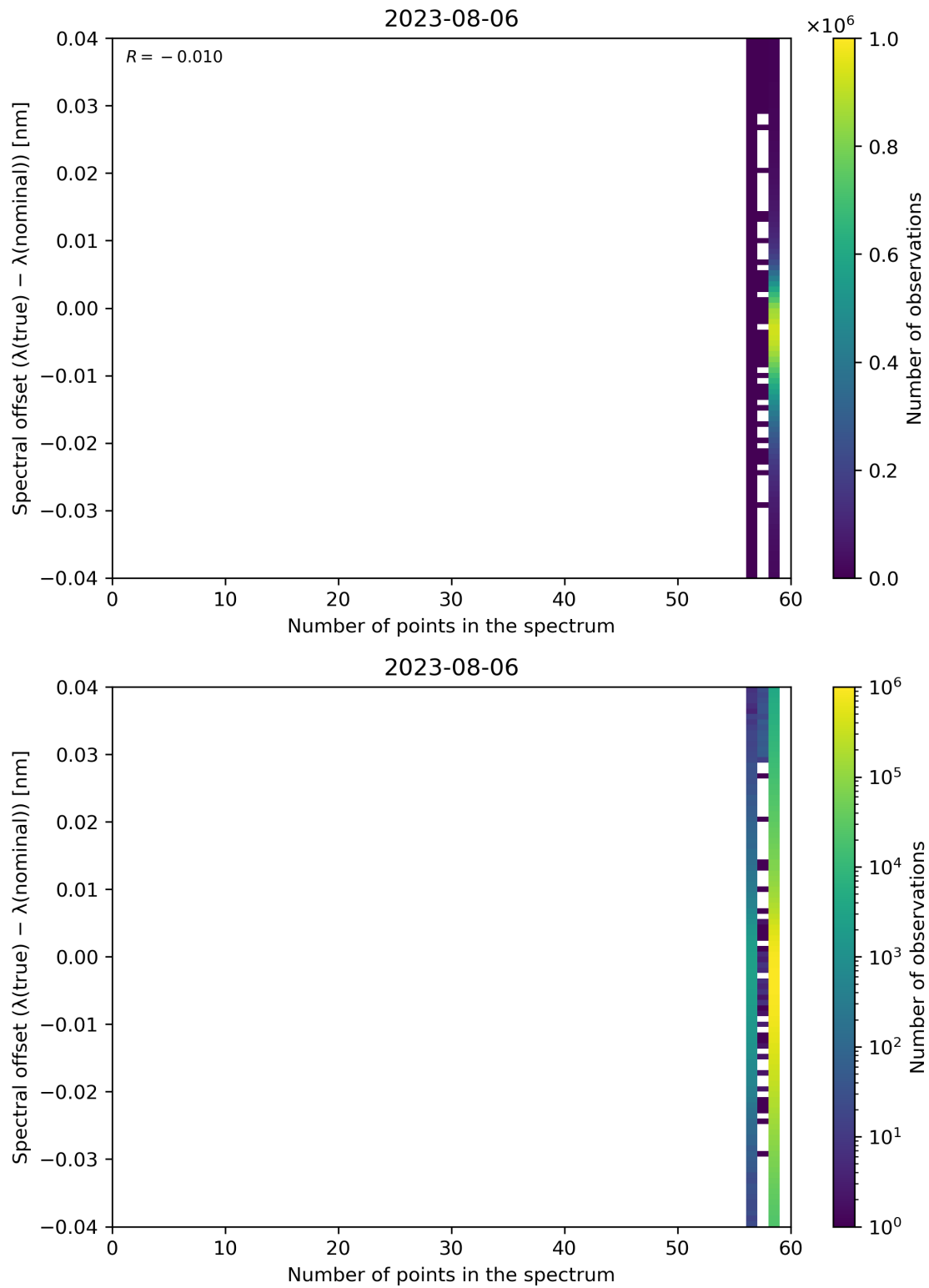
Figure 110: Scatter density plot of “Number of points in the spectrum” against “Spectral offset ( \lambda(\text{true}) - \lambda(\text{nominal}) )” for 2023-08-05 to 2023-08-07.
