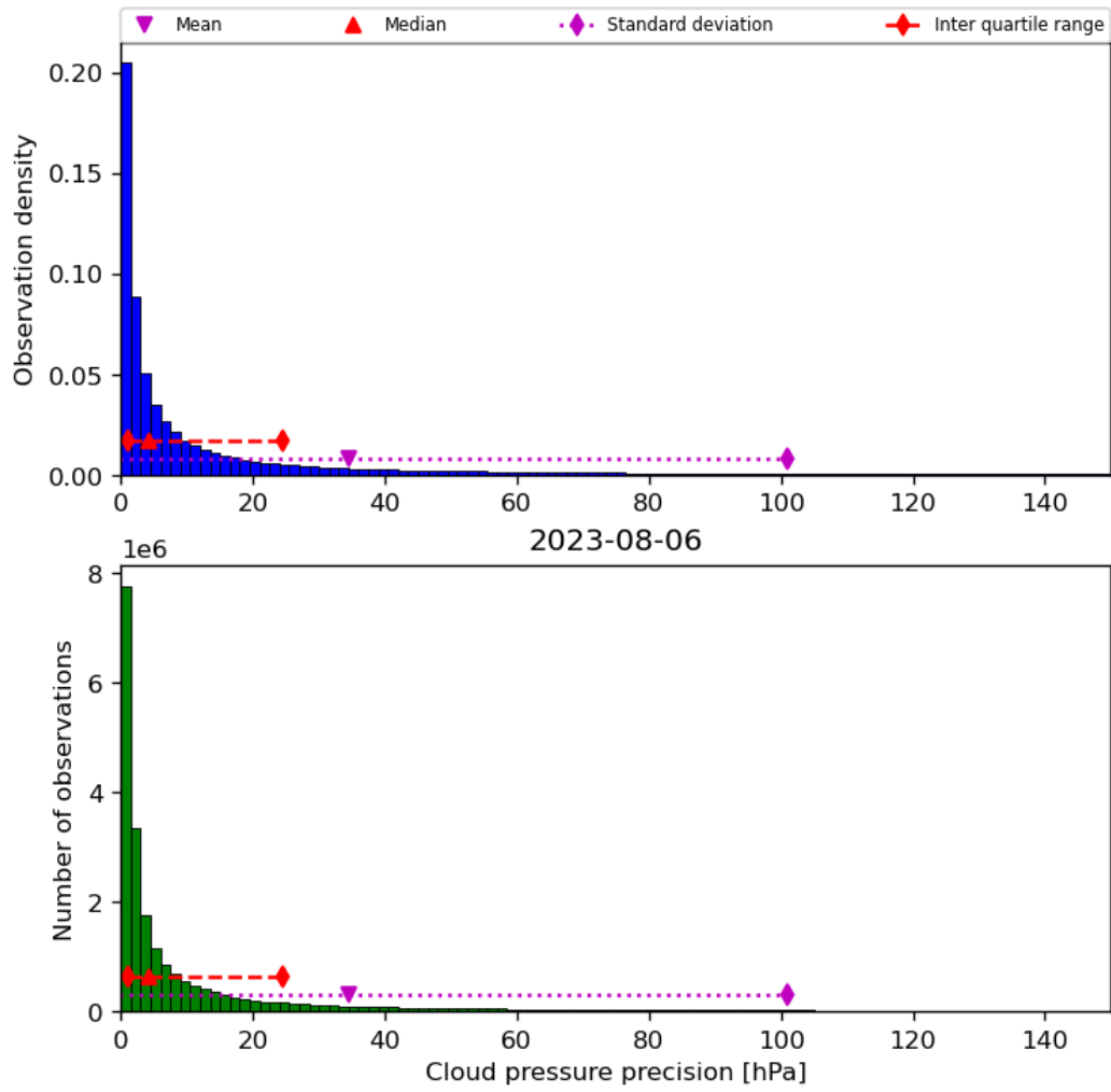
Figure 31: Histogram of “Cloud pressure precision” for 2023-08-05 to 2023-08-07
