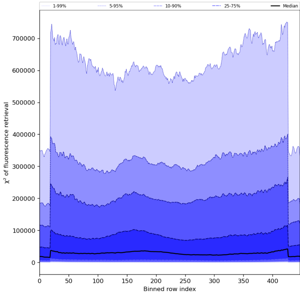
Figure 59: Along track statistics of “ \chi^2 of fluorescence retrieval” for 2023-08-05 to 2023-08-07
