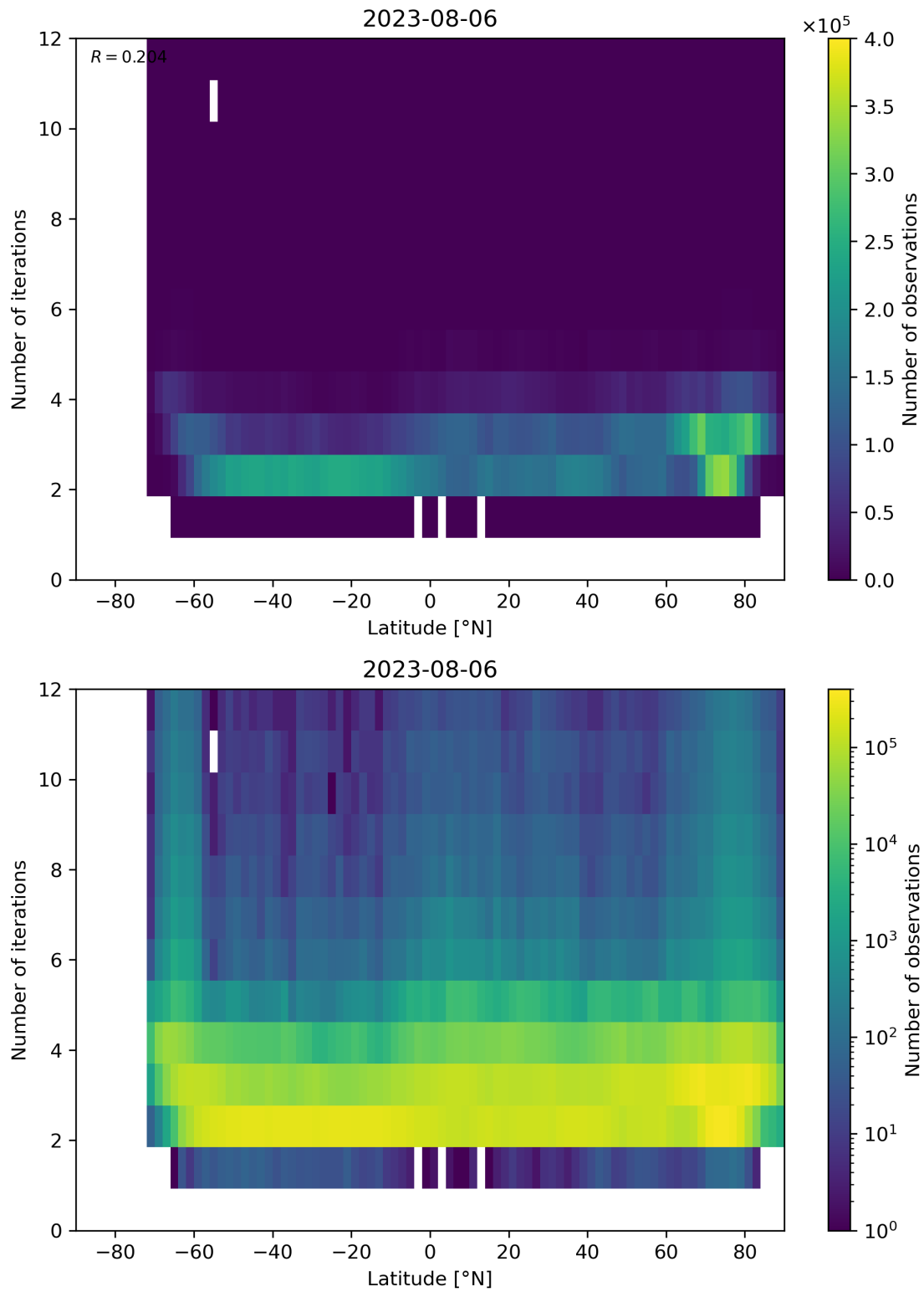
Figure 102: Scatter density plot of “Latitude” against “Number of iterations” for 2023-08-05 to 2023-08-07.
