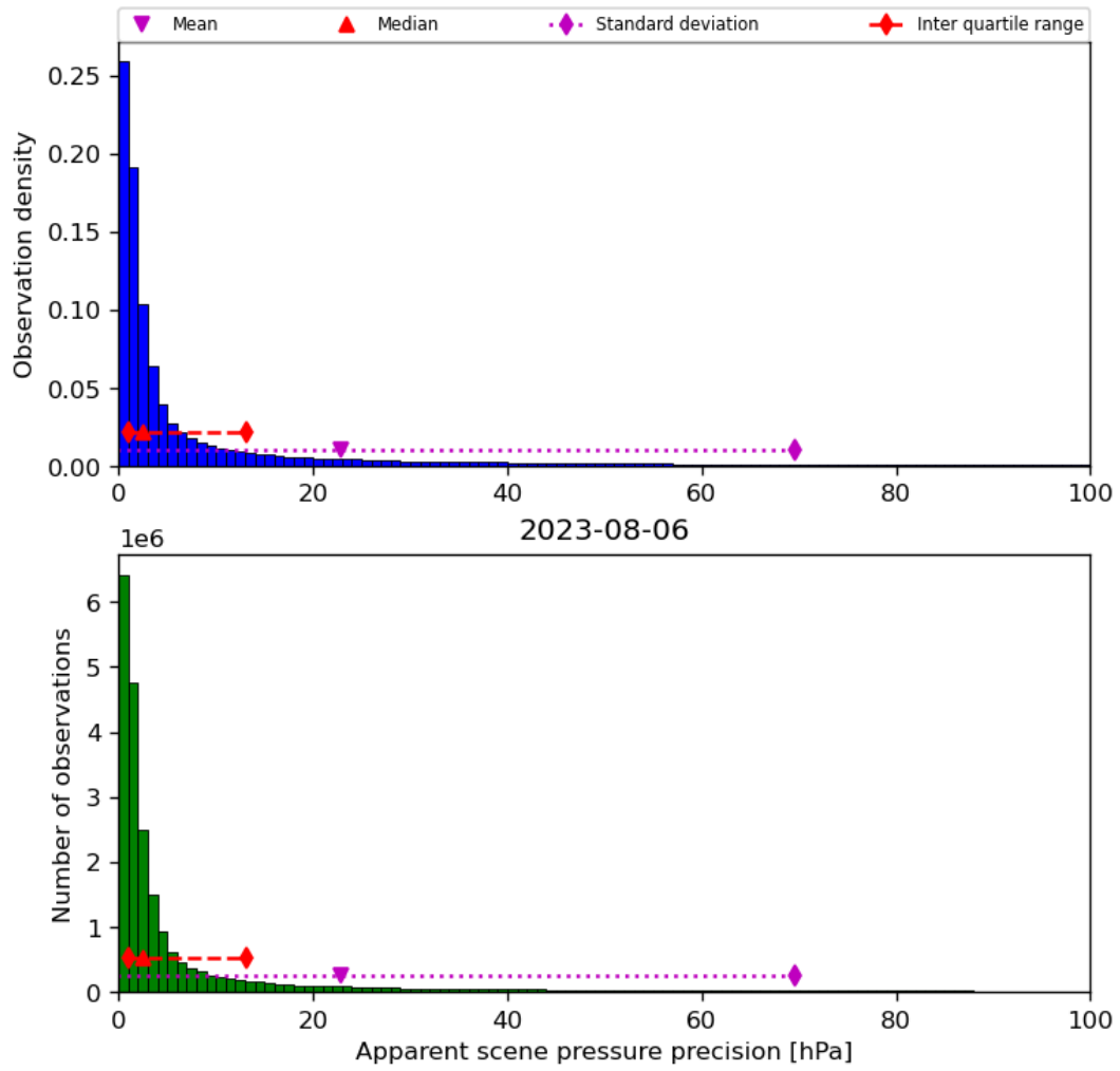
Figure 37: Histogram of “Apparent scene pressure precision” for 2023-08-05 to 2023-08-07
