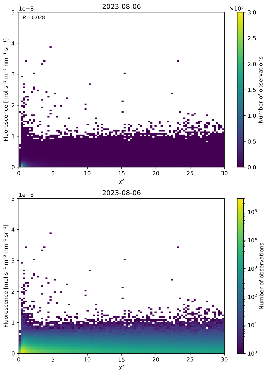
Figure 70: Scatter density plot of “ \chi^2 ” against “Fluorescence” for 2023-08-05 to 2023-08-07.
