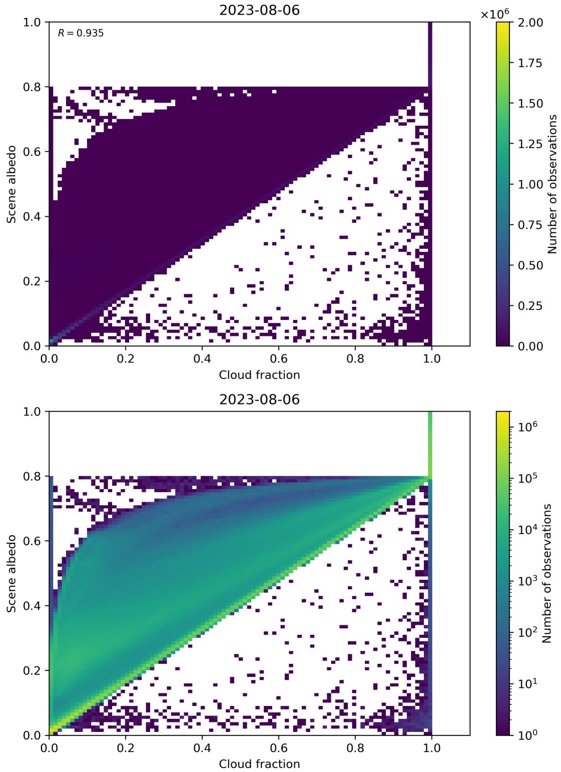
Figure 82: Scatter density plot of “Cloud fraction” against “Scene albedo” for 2023-08-05 to 2023-08-07.
