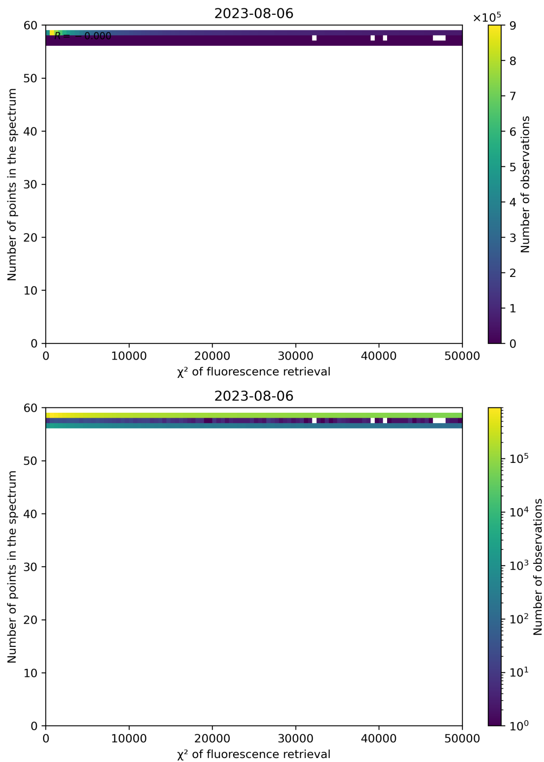
Figure 71: Scatter density plot of " \chi^2 of fluorescence retrieval" against "Number of points in the spectrum" for 2023-08-05 to 2023-08-07.
