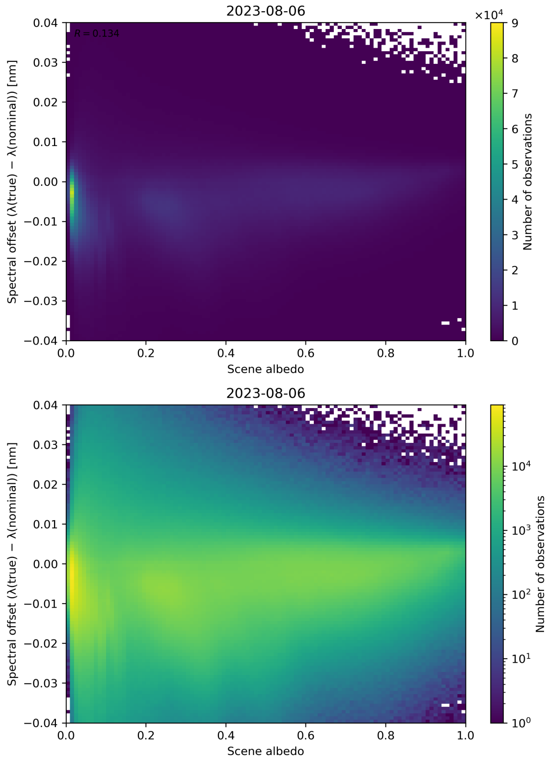
Figure 117: Scatter density plot of “Scene albedo” against “Spectral offset ( \lambda(\text{true}) - \lambda(\text{nominal}) )” for 2023-08-05 to 2023-08-07.
