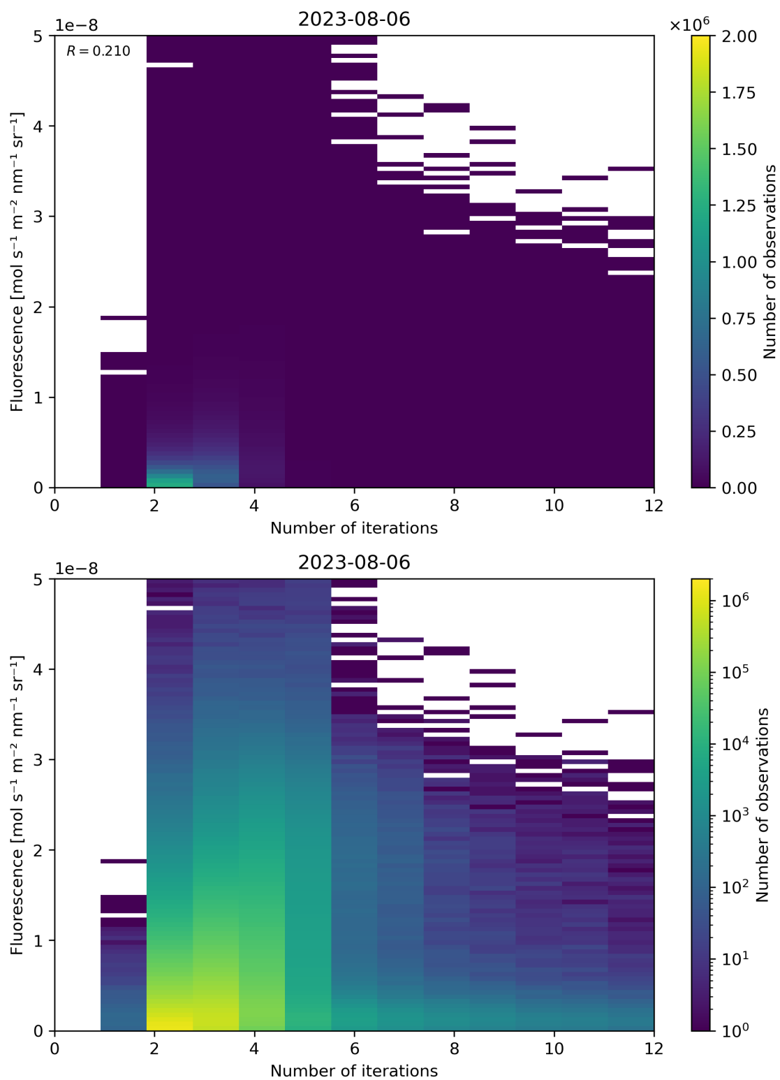
Figure 107: Scatter density plot of “Number of iterations” against “Fluorescence” for 2023-08-05 to 2023-08-07.
