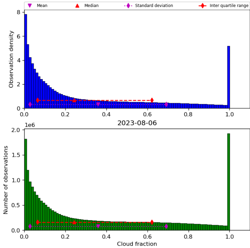
Figure 32: Histogram of “Cloud fraction” for 2023-08-05 to 2023-08-07
