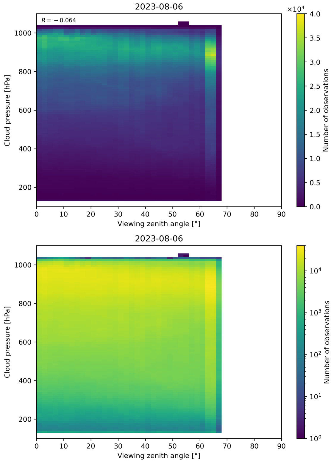
Figure 133: Scatter density plot of “Viewing zenith angle” against “Cloud pressure” for 2023-08-05 to 2023-08-07.
