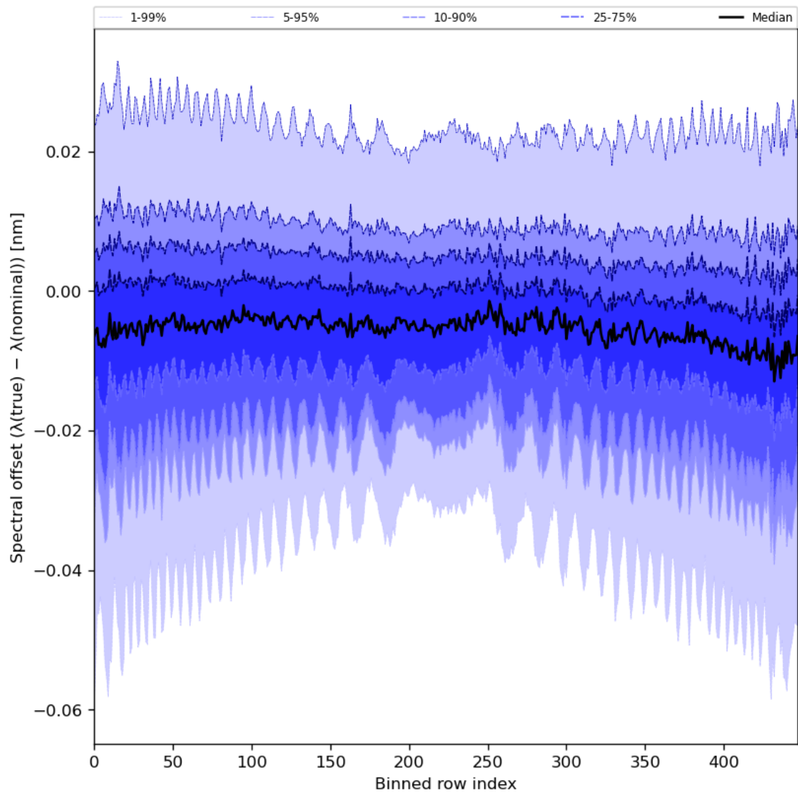
Figure 62: Along track statistics of “Spectral offset ( \lambda(\text{true}) - \lambda(\text{nominal}) )” for 2023-08-05 to 2023-08-07
