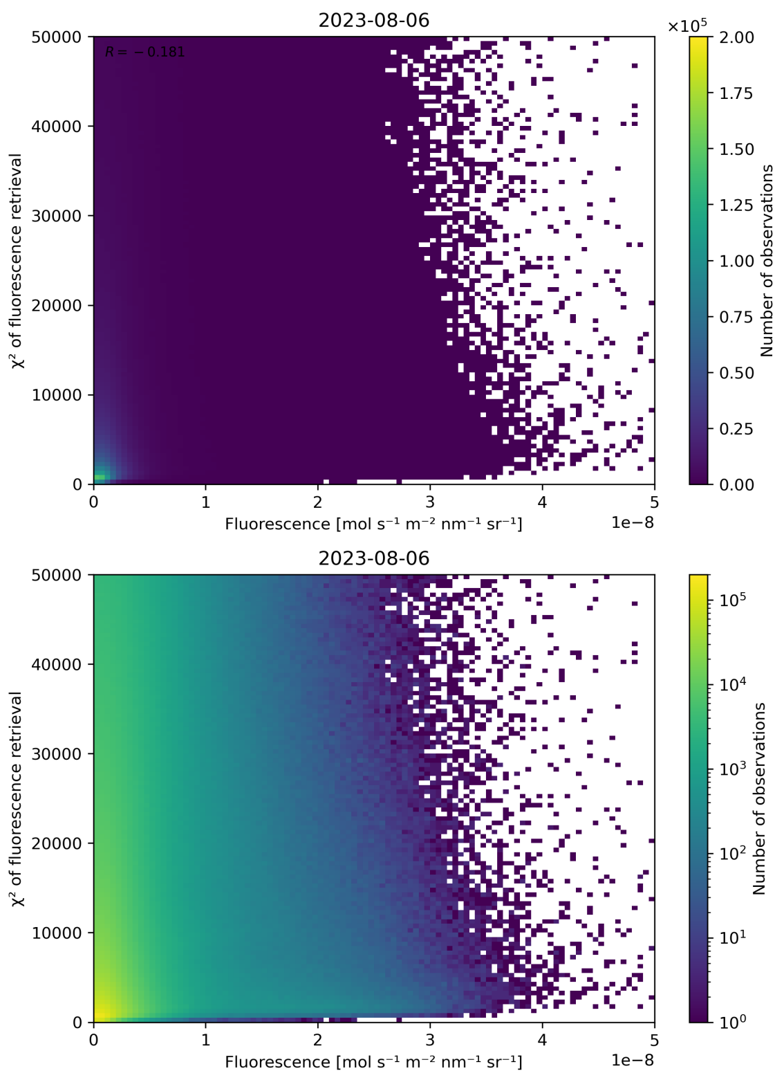
Figure 93: Scatter density plot of “Fluorescence” against “ \chi^2 of fluorescence retrieval” for 2023-08-05 to 2023-08-07.
