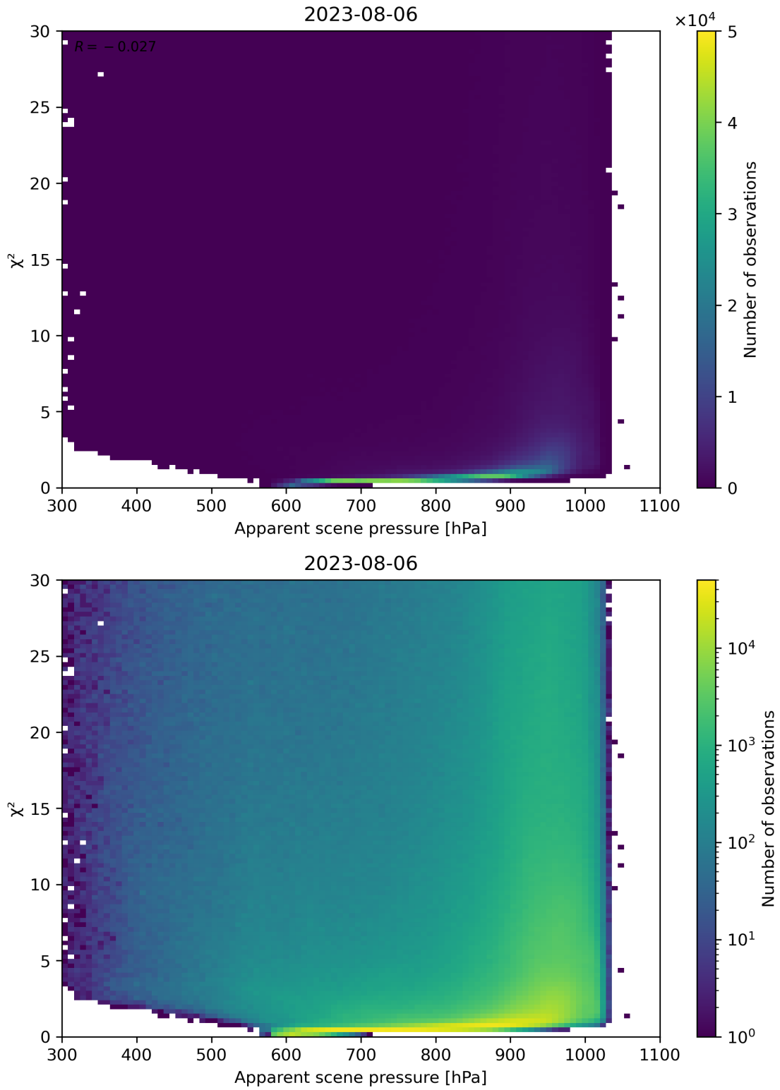
Figure 63: Scatter density plot of “Apparent scene pressure” against “ \chi^2 ” for 2023-08-05 to 2023-08-07.
