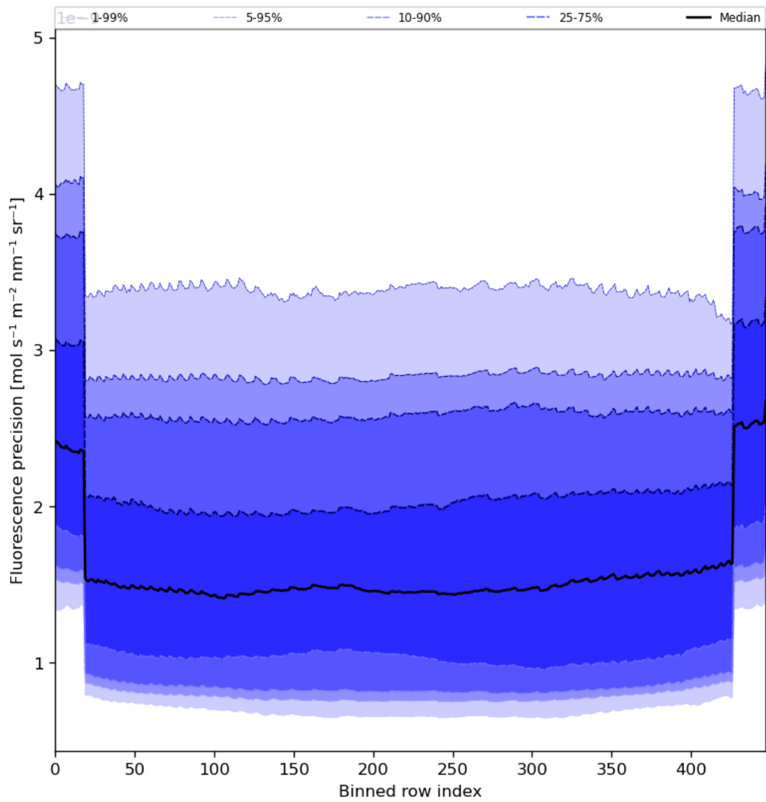
Figure 58: Along track statistics of “Fluorescence precision” for 2023-08-05 to 2023-08-07
