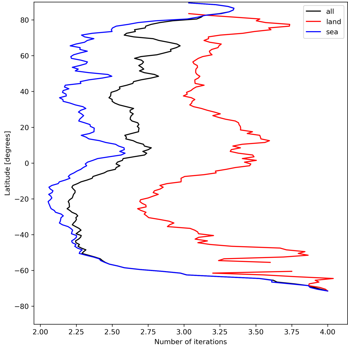
Figure 22: Zonal average of “Number of iterations” for 2023-08-05 to 2023-08-07.
