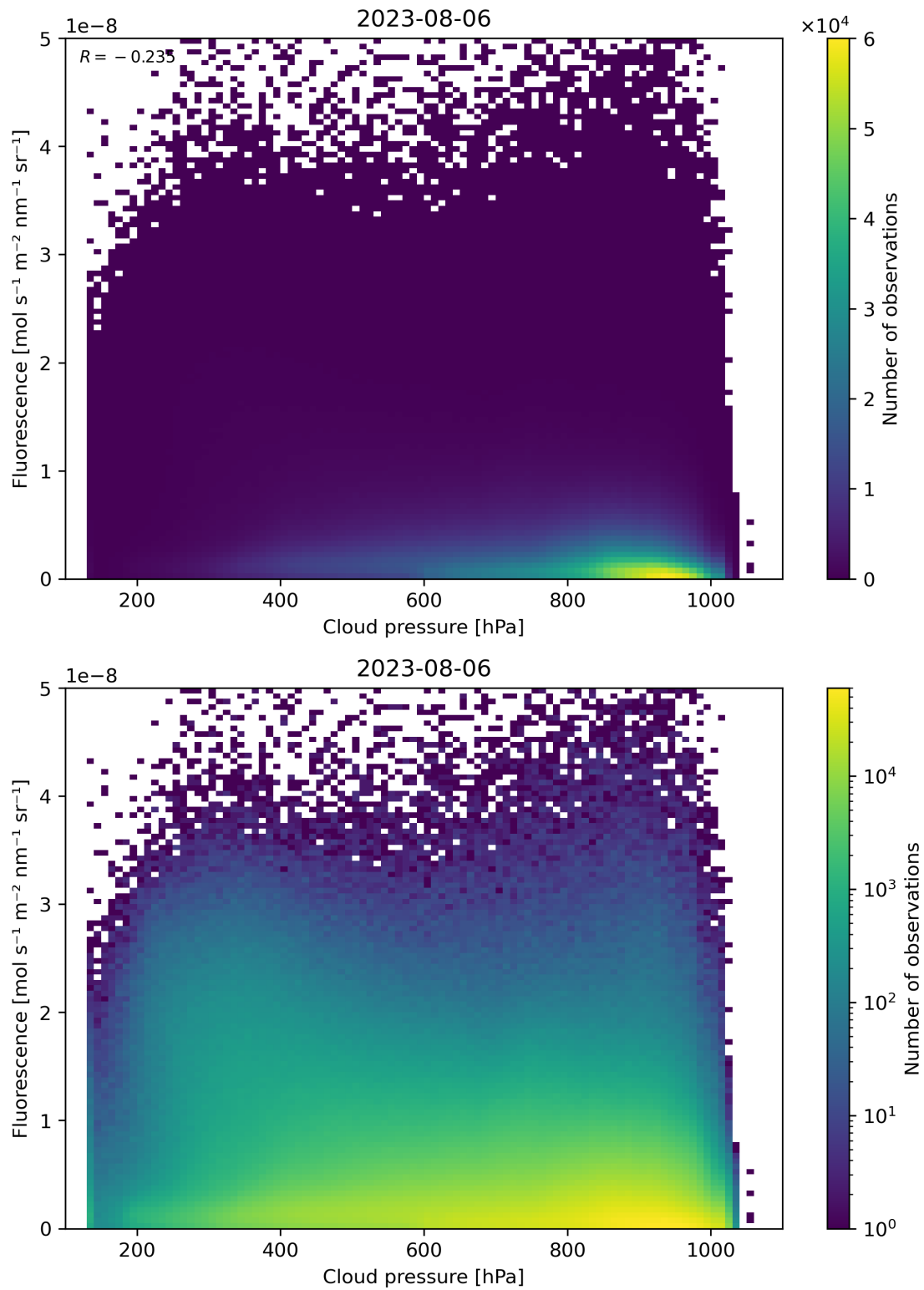
Figure 88: Scatter density plot of “Cloud pressure” against “Fluorescence” for 2023-08-05 to 2023-08-07.
