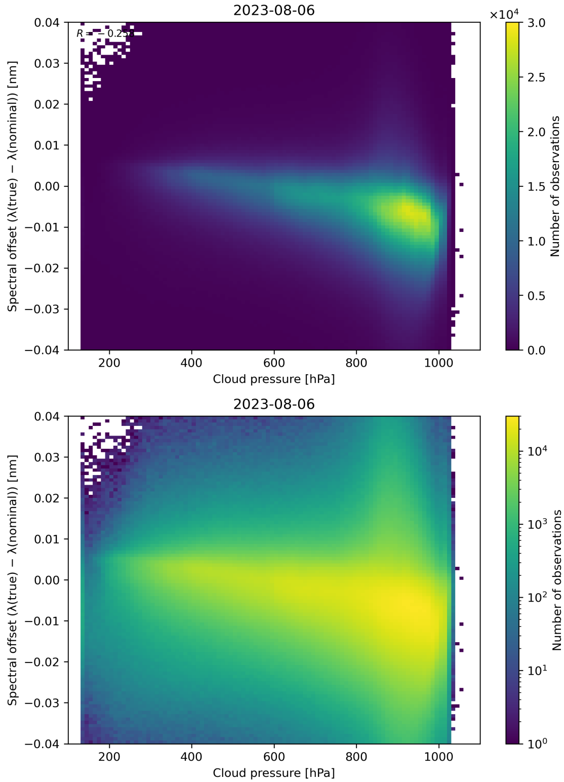
Figure 92: Scatter density plot of “Cloud pressure” against “Spectral offset ( \lambda(\text{true}) - \lambda(\text{nominal}) )” for 2023-08-05 to 2023-08-07.
