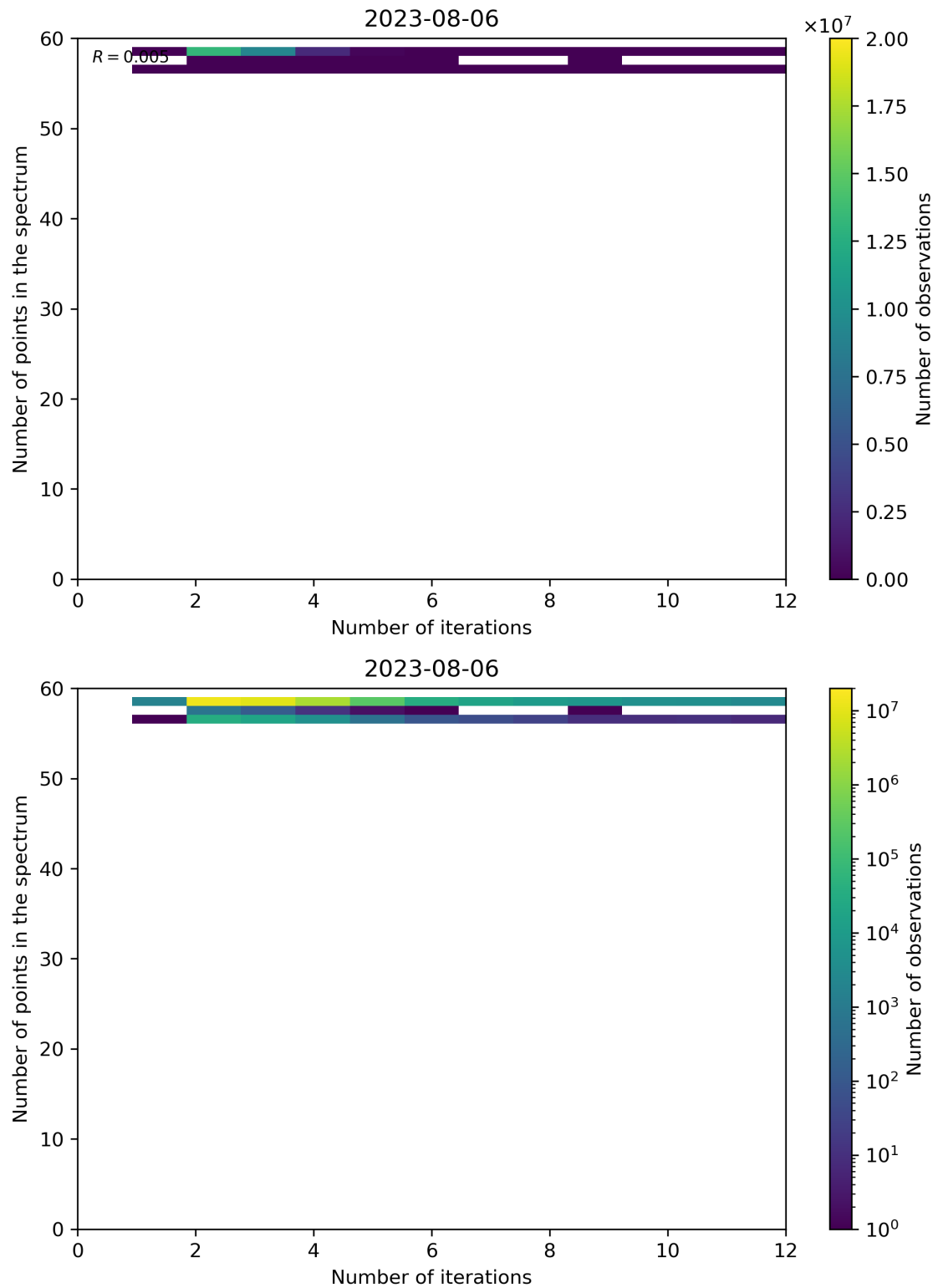
Figure 108: Scatter density plot of “Number of iterations” against “Number of points in the spectrum” for 2023-08-05 to 2023-08-07.
