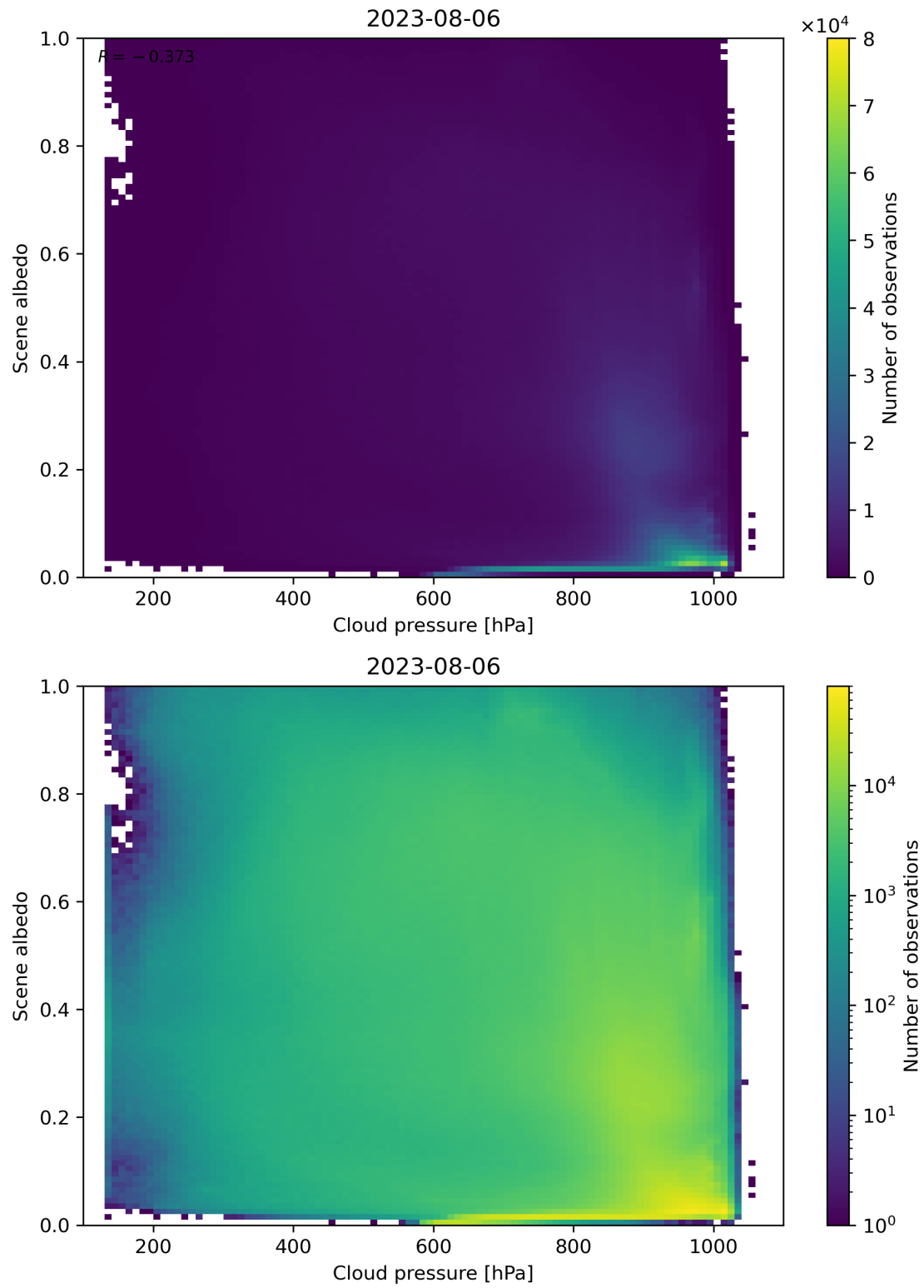
Figure 91: Scatter density plot of “Cloud pressure” against “Scene albedo” for 2023-08-05 to 2023-08-07.
