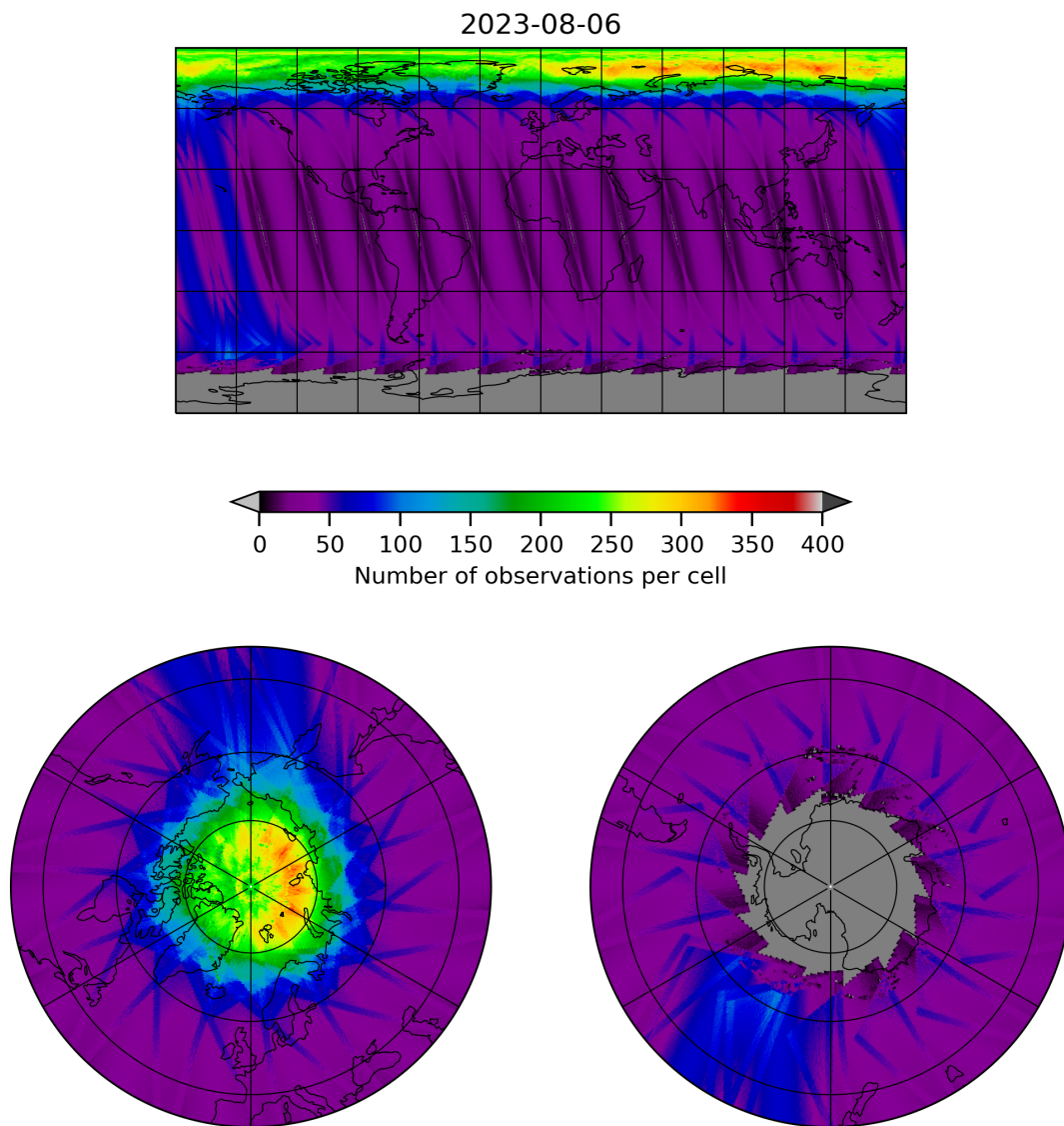
Figure 11: Map of the number of observations for 2023-08-05 to 2023-08-07
