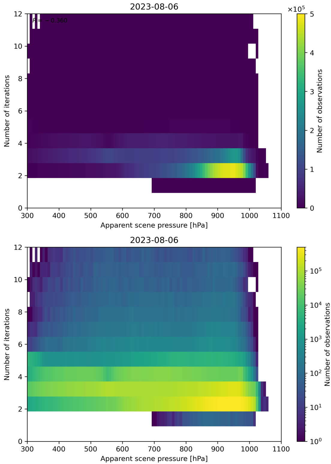
Figure 66: Scatter density plot of “Apparent scene pressure” against “Number of iterations” for 2023-08-05 to 2023-08-07.
