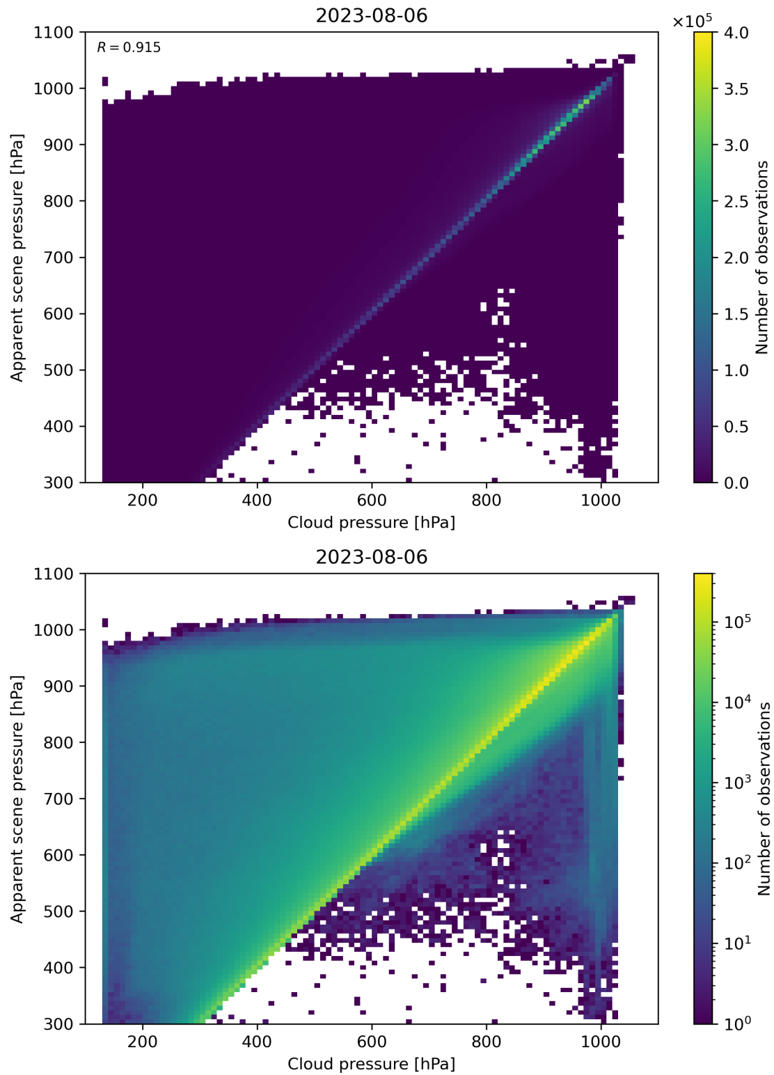
Figure 84: Scatter density plot of “Cloud pressure” against “Apparent scene pressure” for 2023-08-05 to 2023-08-07.
