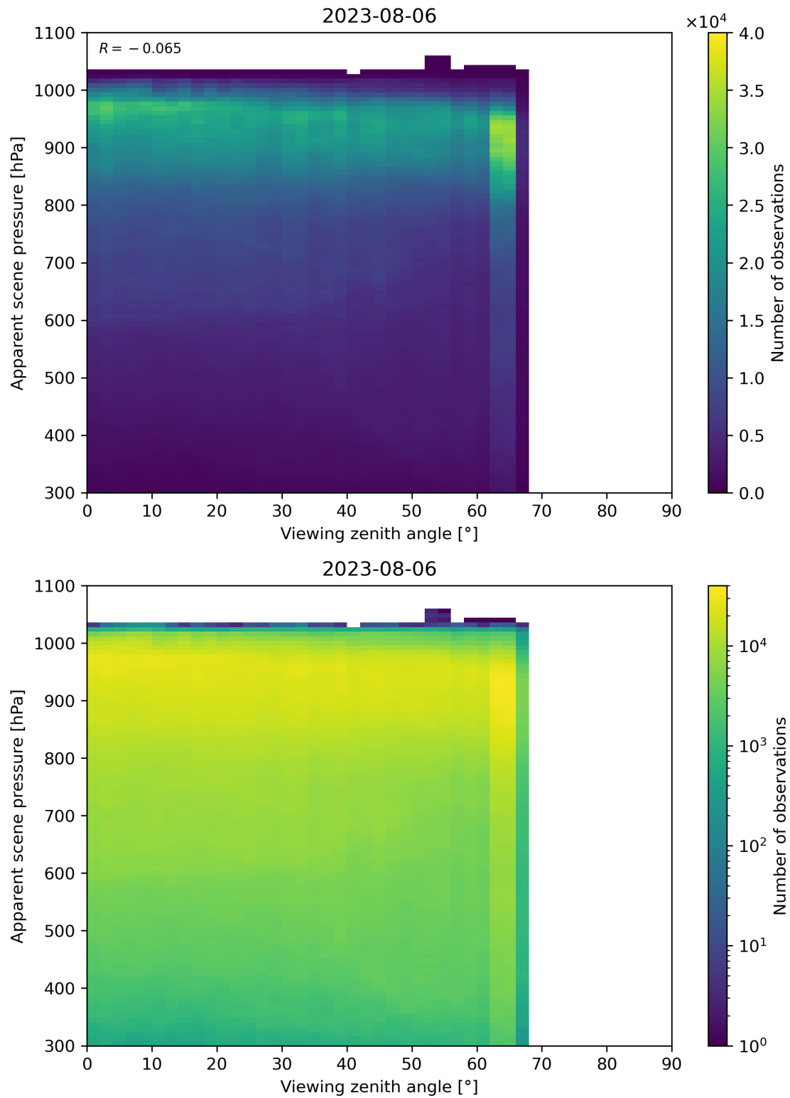
Figure 129: Scatter density plot of “Viewing zenith angle” against “Apparent scene pressure” for 2023-08-05 to 2023-08-07.
