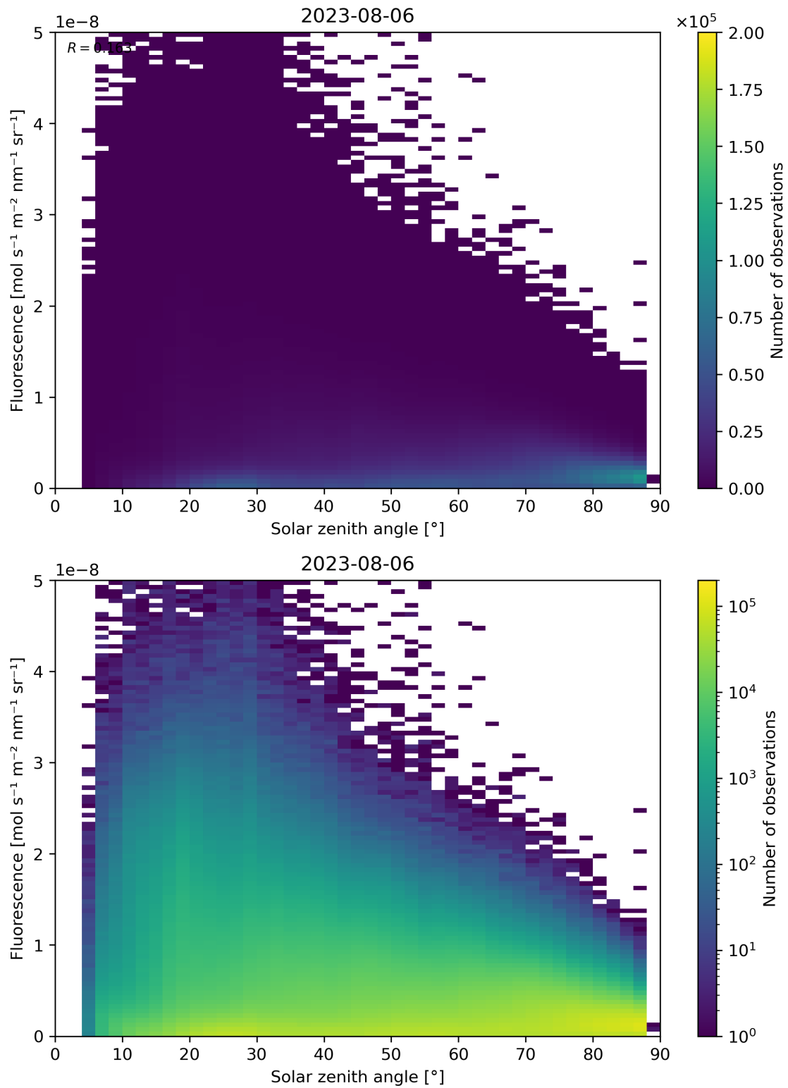
Figure 123: Scatter density plot of “Solar zenith angle” against “Fluorescence” for 2023-08-05 to 2023-08-07.
