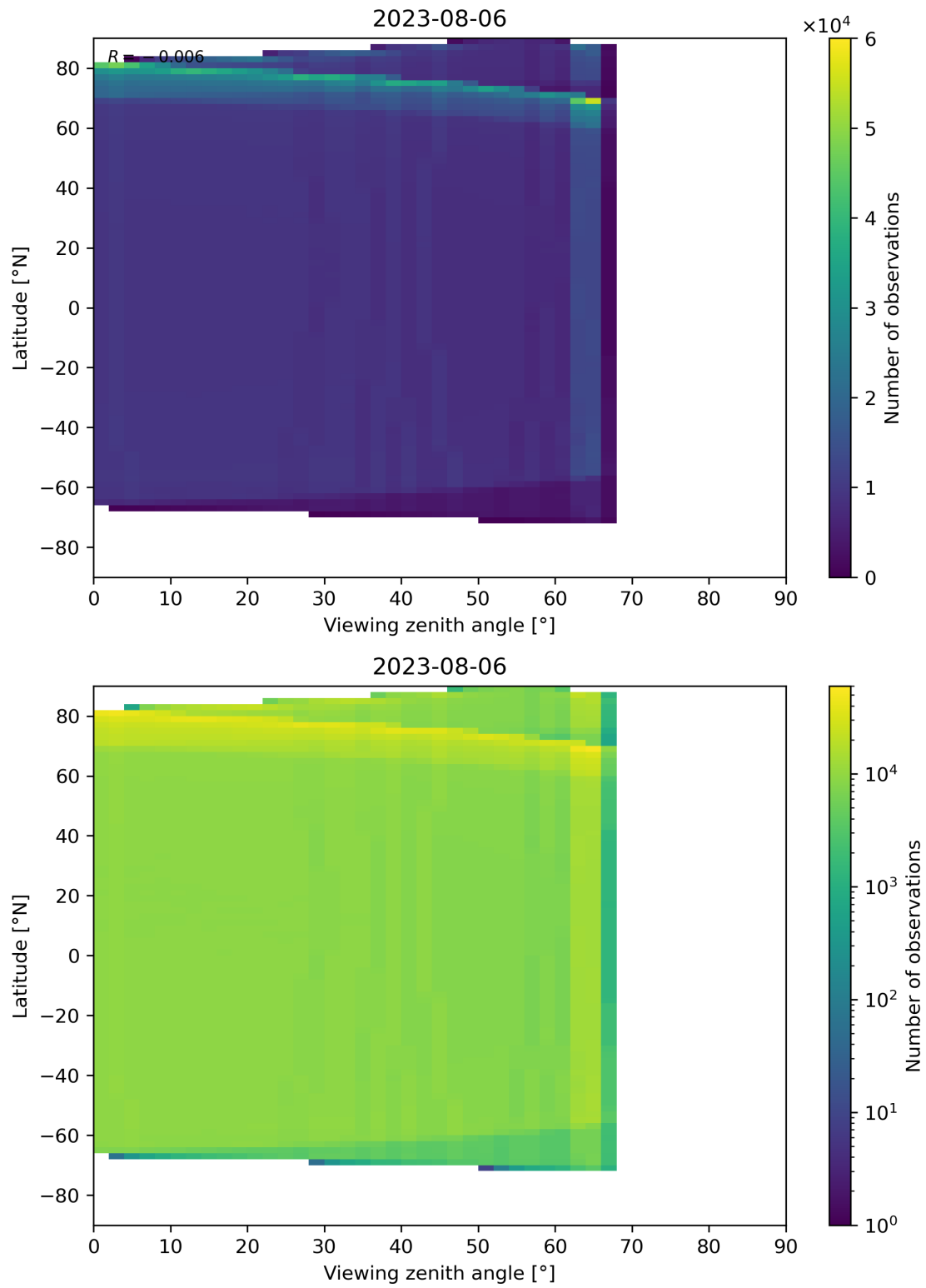
Figure 135: Scatter density plot of “Viewing zenith angle” against “Latitude” for 2023-08-05 to 2023-08-07.
