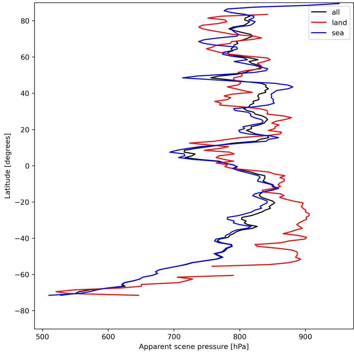
Figure 19: Zonal average of “Apparent scene pressure” for 2023-08-05 to 2023-08-07.
