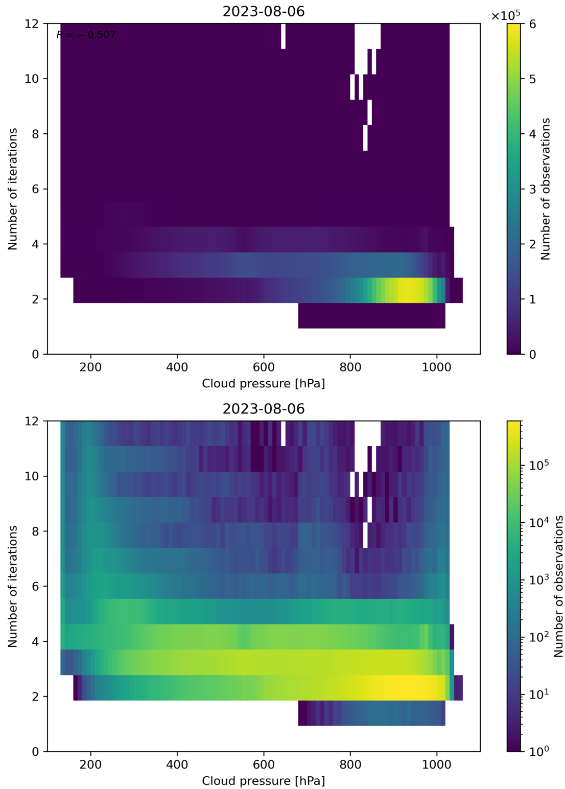
Figure 89: Scatter density plot of “Cloud pressure” against “Number of iterations” for 2023-08-05 to 2023-08-07.
