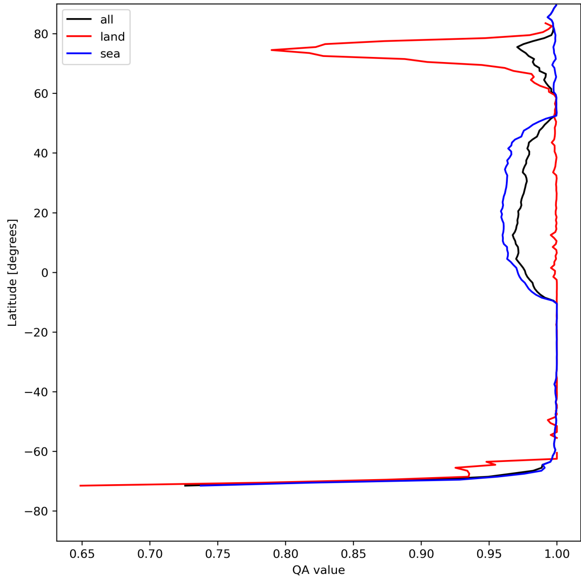
Figure 12: Zonal average of “QA value” for 2023-08-05 to 2023-08-07.
