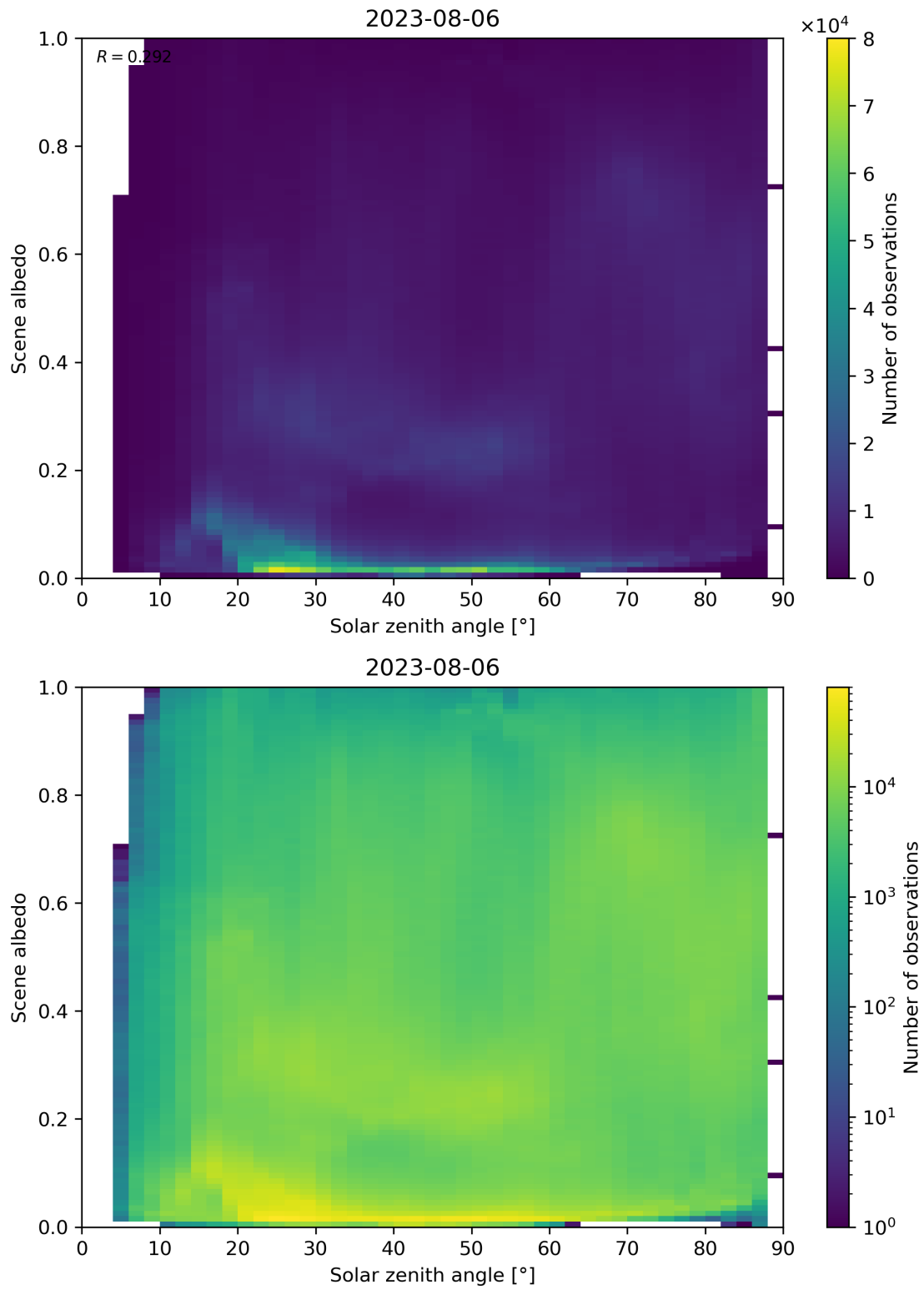
Figure 127: Scatter density plot of “Solar zenith angle” against “Scene albedo” for 2023-08-05 to 2023-08-07.
