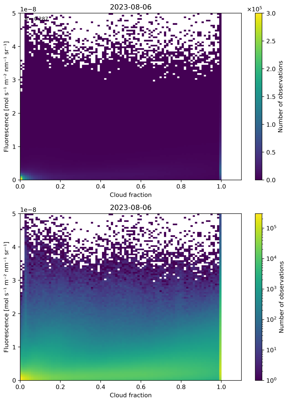
Figure 79: Scatter density plot of “Cloud fraction” against “Fluorescence” for 2023-08-05 to 2023-08-07.
