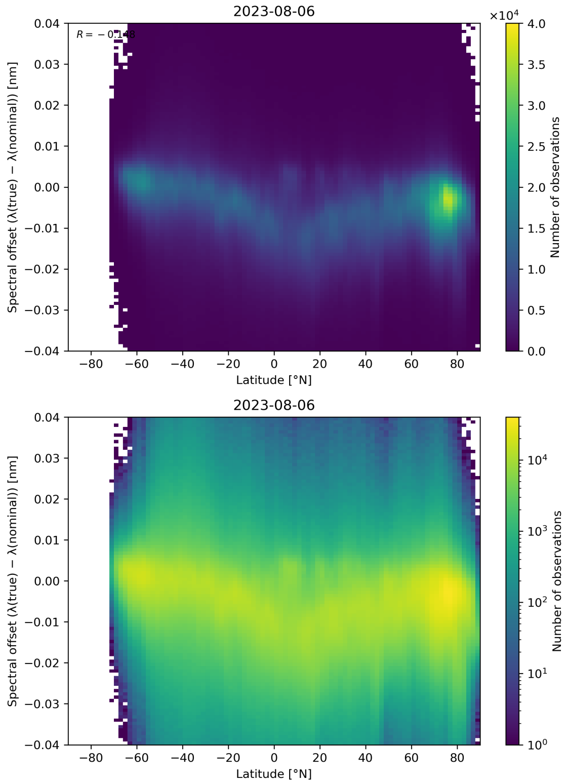
Figure 105: Scatter density plot of “Latitude” against “Spectral offset ( \lambda(\text{true}) - \lambda(\text{nominal}) )” for 2023-08-05 to 2023-08-07.
