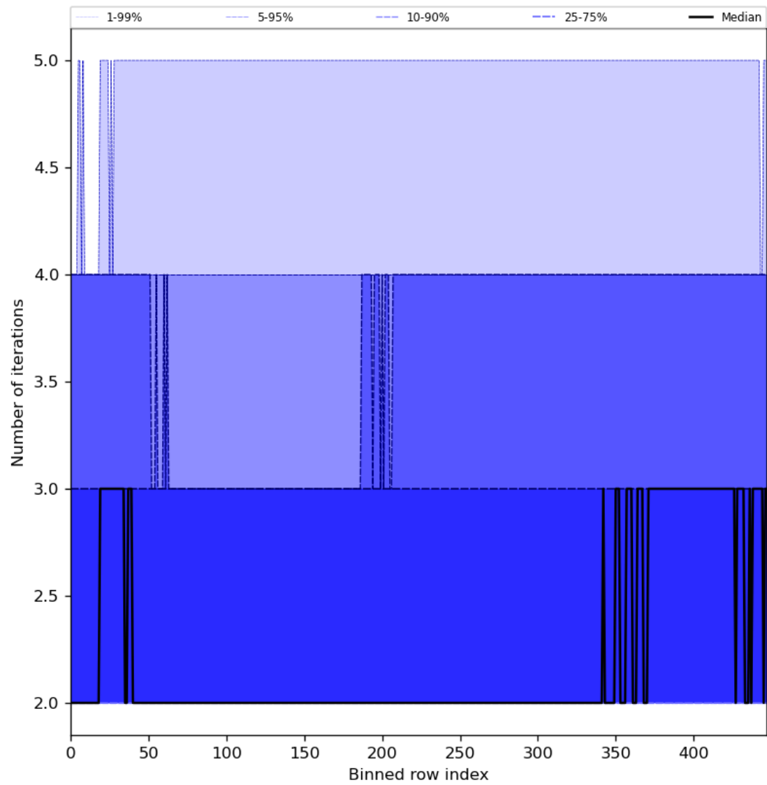
Figure 56: Along track statistics of “Number of iterations” for 2023-08-05 to 2023-08-07
