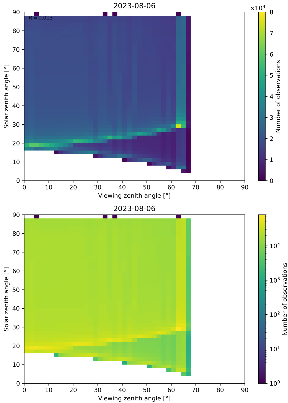
Figure 139: Scatter density plot of “Viewing zenith angle” against “Solar zenith angle” for 2023-08-05 to 2023-08-07.
