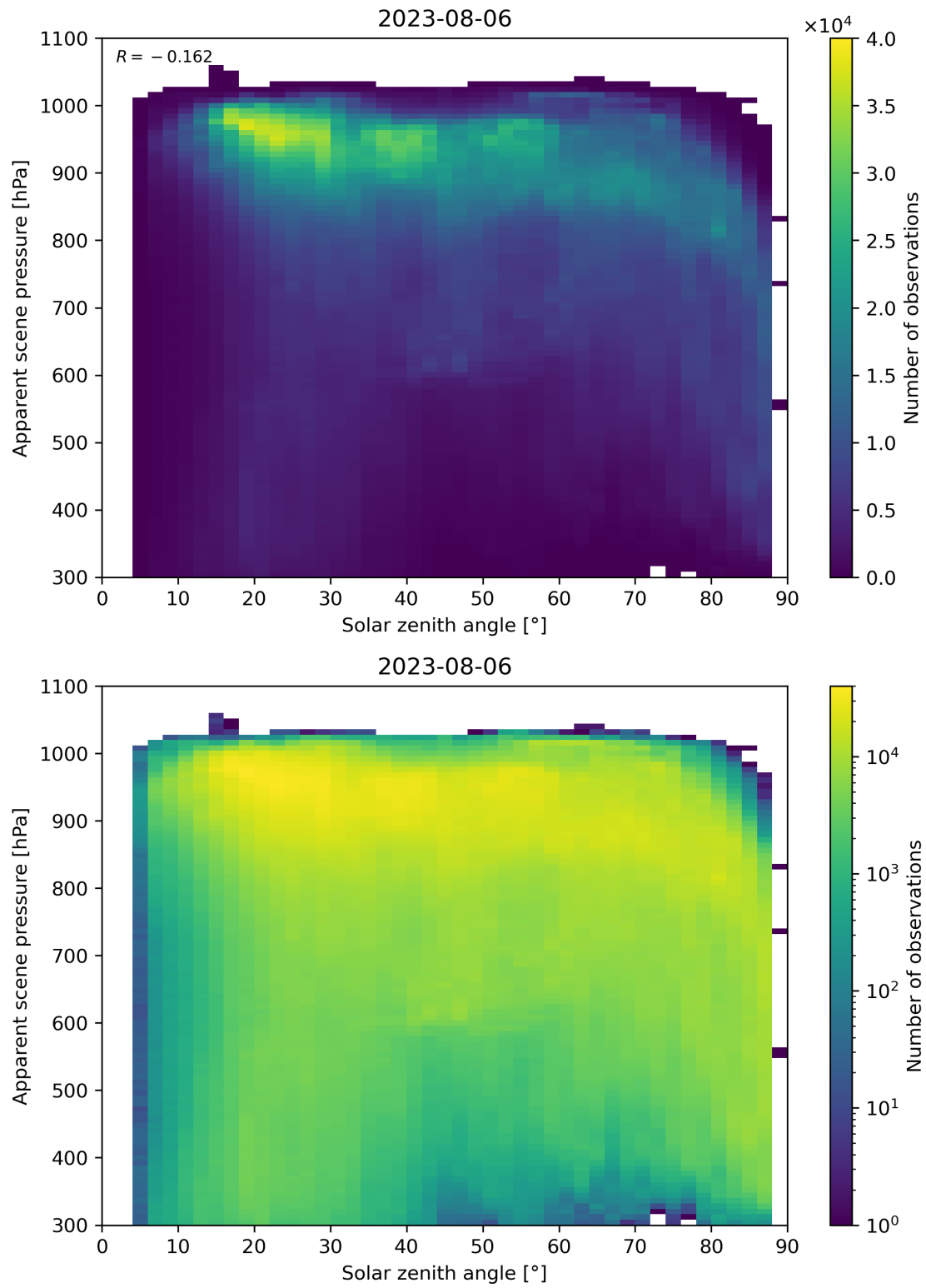
Figure 118: Scatter density plot of “Solar zenith angle” against “Apparent scene pressure” for 2023-08-05 to 2023-08-07.
