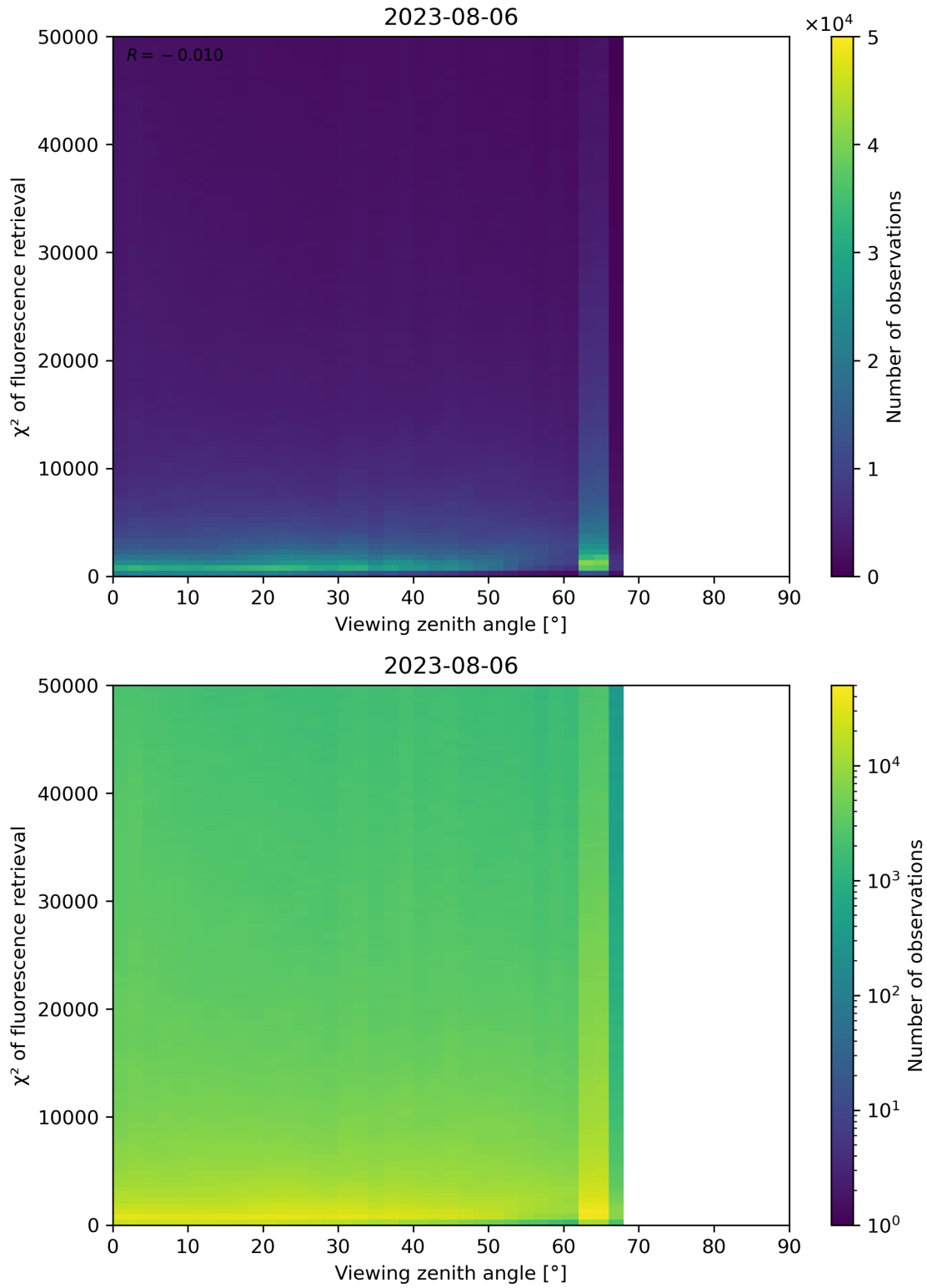
Figure 131: Scatter density plot of “Viewing zenith angle” against “ \chi^2 of fluorescence retrieval” for 2023-08-05 to 2023-08-07.
