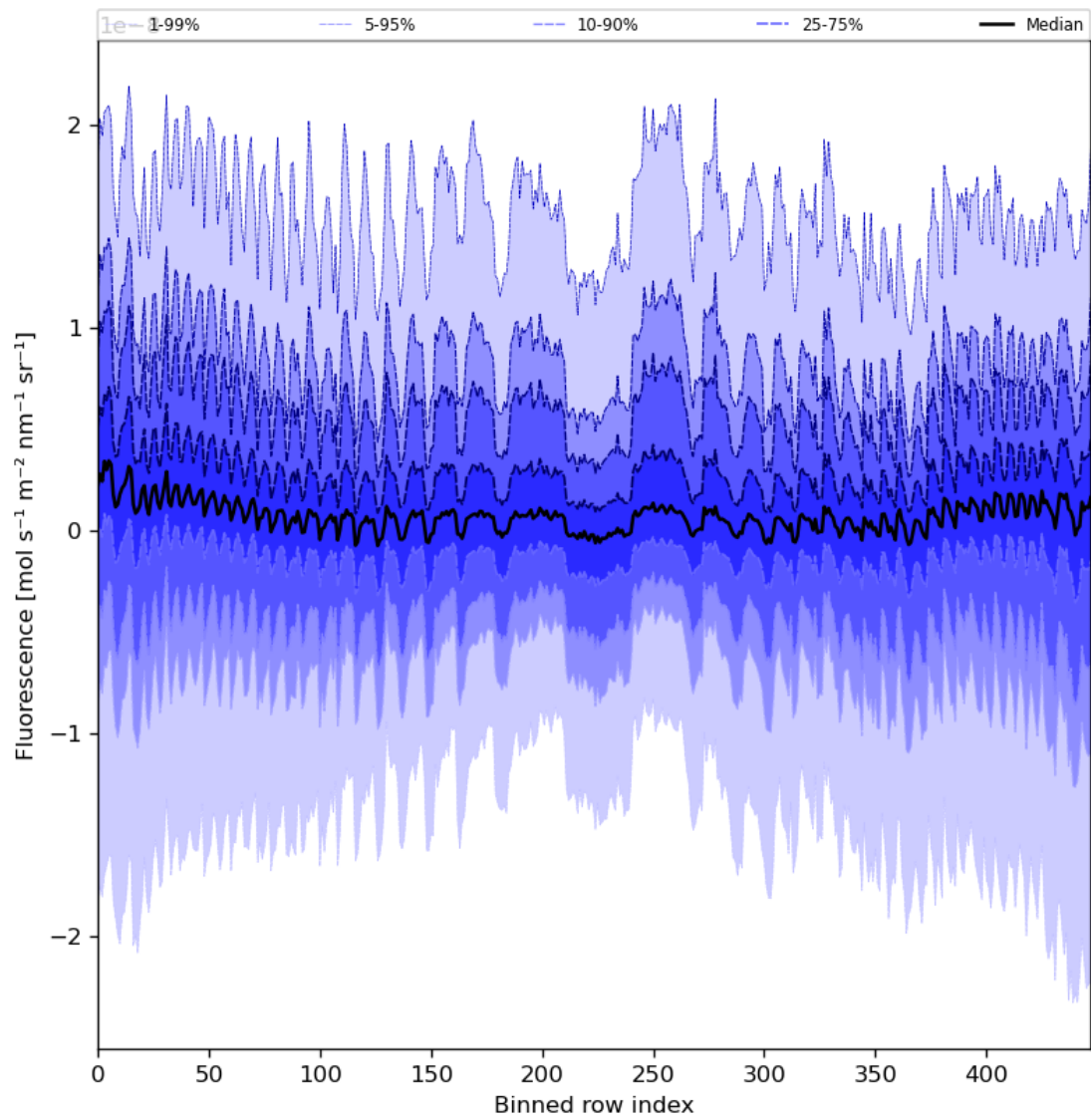
Figure 57: Along track statistics of “Fluorescence” for 2023-08-05 to 2023-08-07
