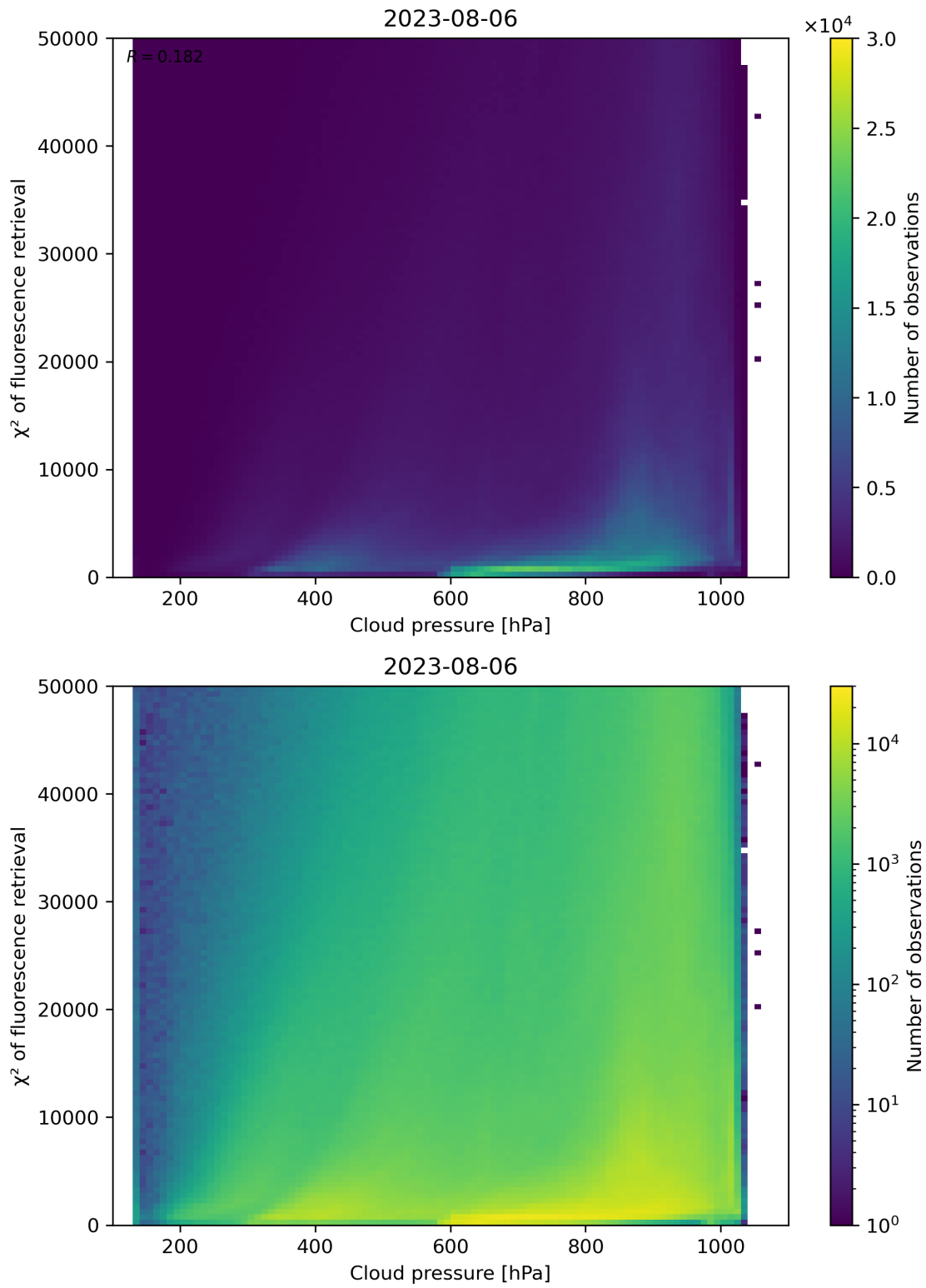
Figure 86: Scatter density plot of “Cloud pressure” against “ \chi^2 of fluorescence retrieval” for 2023-08-05 to 2023-08-07.
