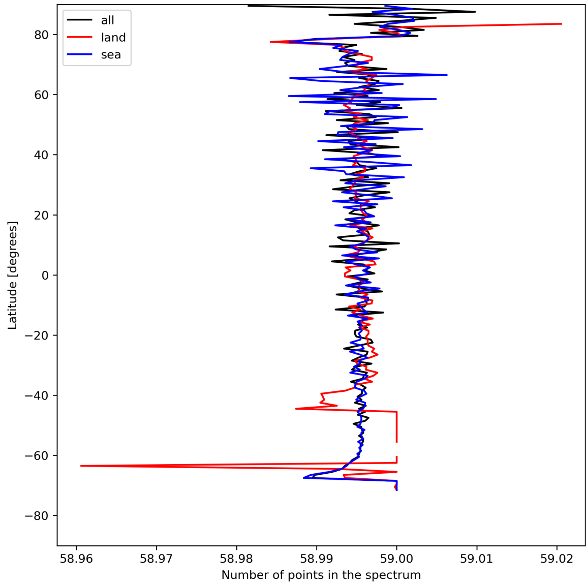
Figure 27: Zonal average of “Number of points in the spectrum” for 2023-08-05 to 2023-08-07.
