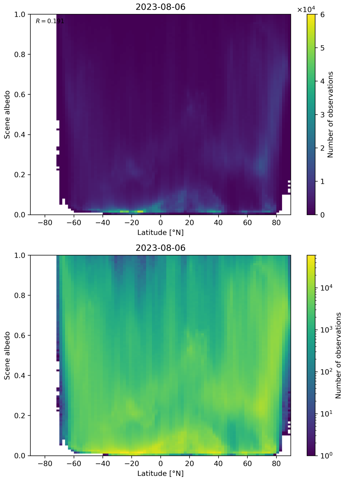
Figure 104: Scatter density plot of “Latitude” against “Scene albedo” for 2023-08-05 to 2023-08-07.
