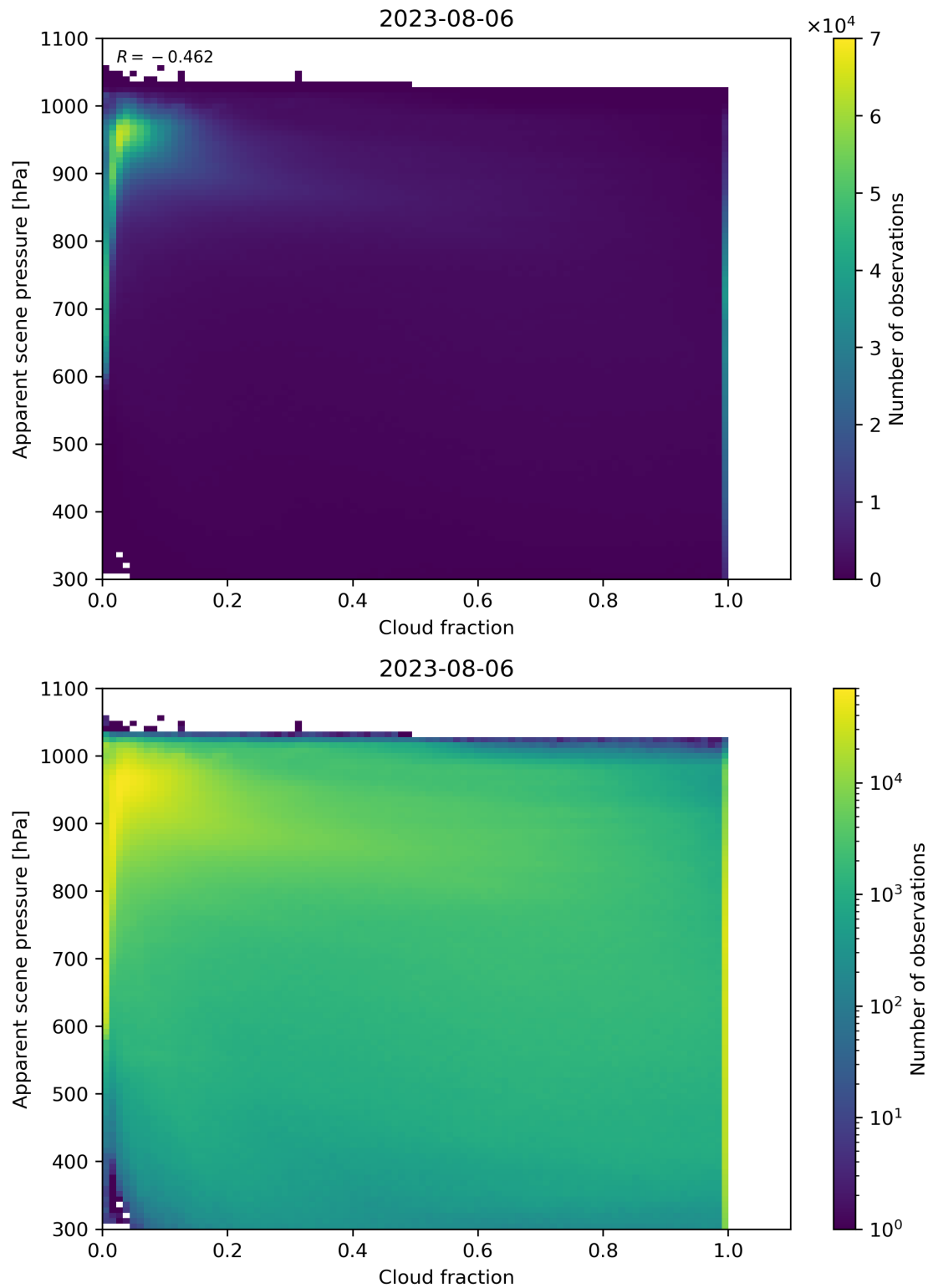
Figure 76: Scatter density plot of “Cloud fraction” against “Apparent scene pressure” for 2023-08-05 to 2023-08-07.
