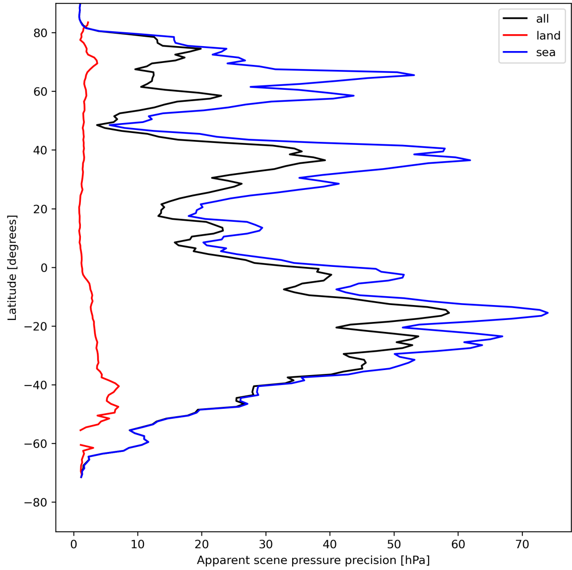
Figure 20: Zonal average of “Apparent scene pressure precision” for 2023-08-05 to 2023-08-07.
