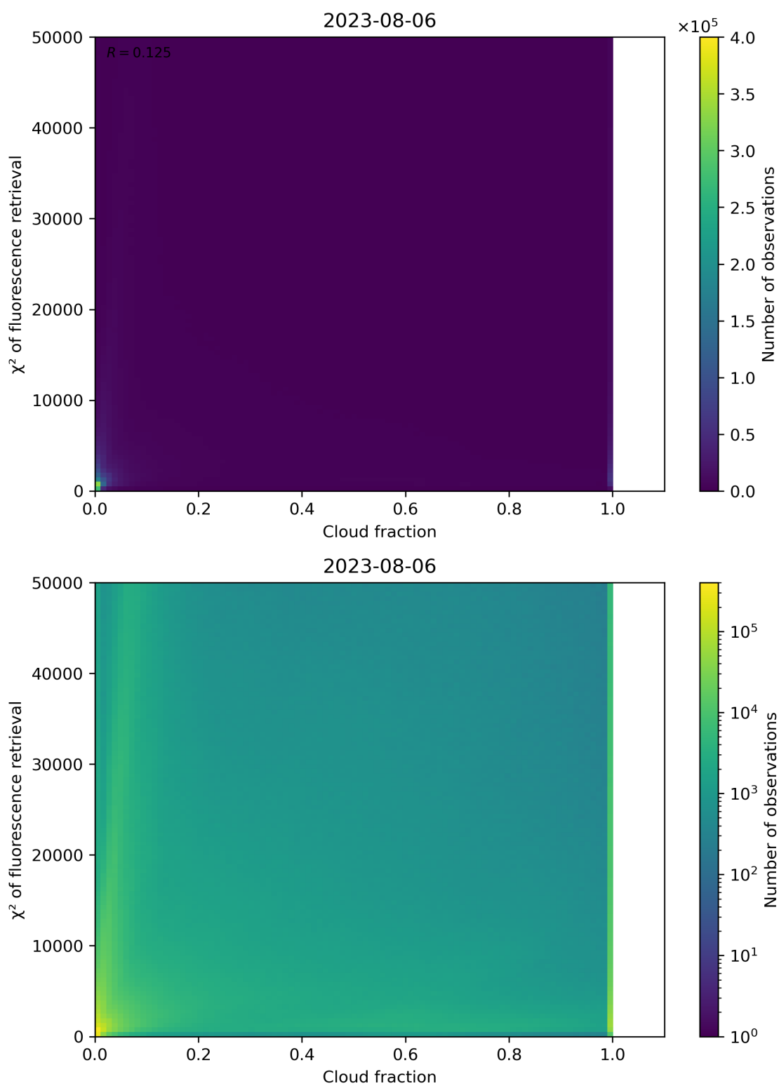
Figure 78: Scatter density plot of “Cloud fraction” against “ \chi^2 of fluorescence retrieval” for 2023-08-05 to 2023-08-07.
