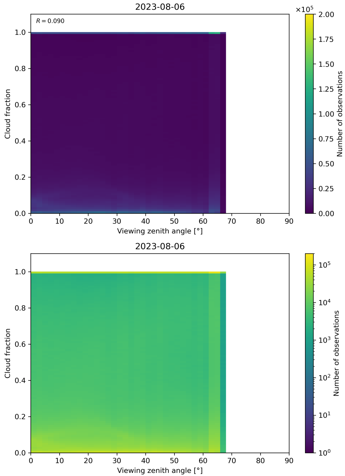
Figure 132: Scatter density plot of “Viewing zenith angle” against “Cloud fraction” for 2023-08-05 to 2023-08-07.
