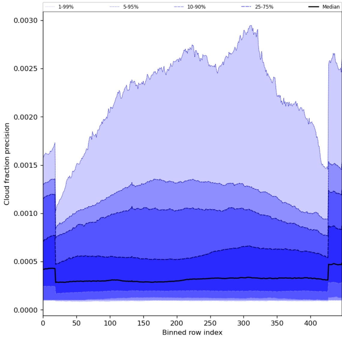
Figure 50: Along track statistics of “Cloud fraction precision” for 2023-08-05 to 2023-08-07
