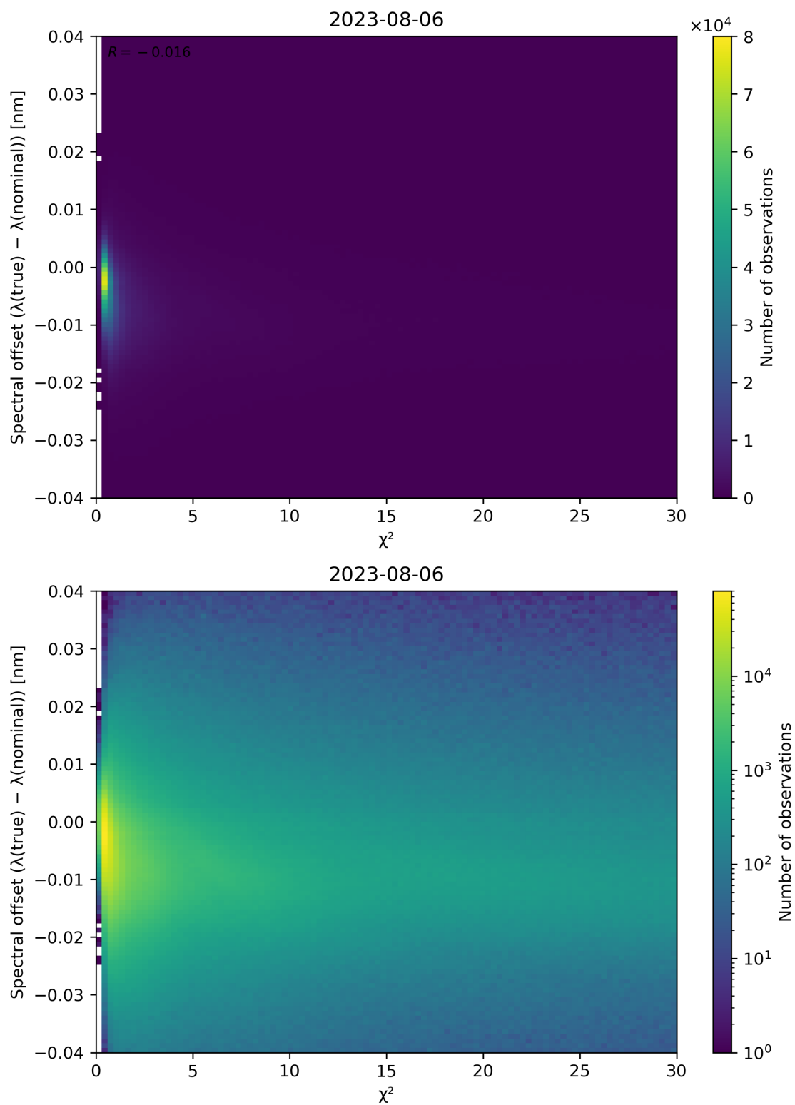
Figure 75: Scatter density plot of “ \chi^2 ” against “Spectral offset ( \lambda(\text{true}) - \lambda(\text{nominal}) )” for 2023-08-05 to 2023-08-07.
