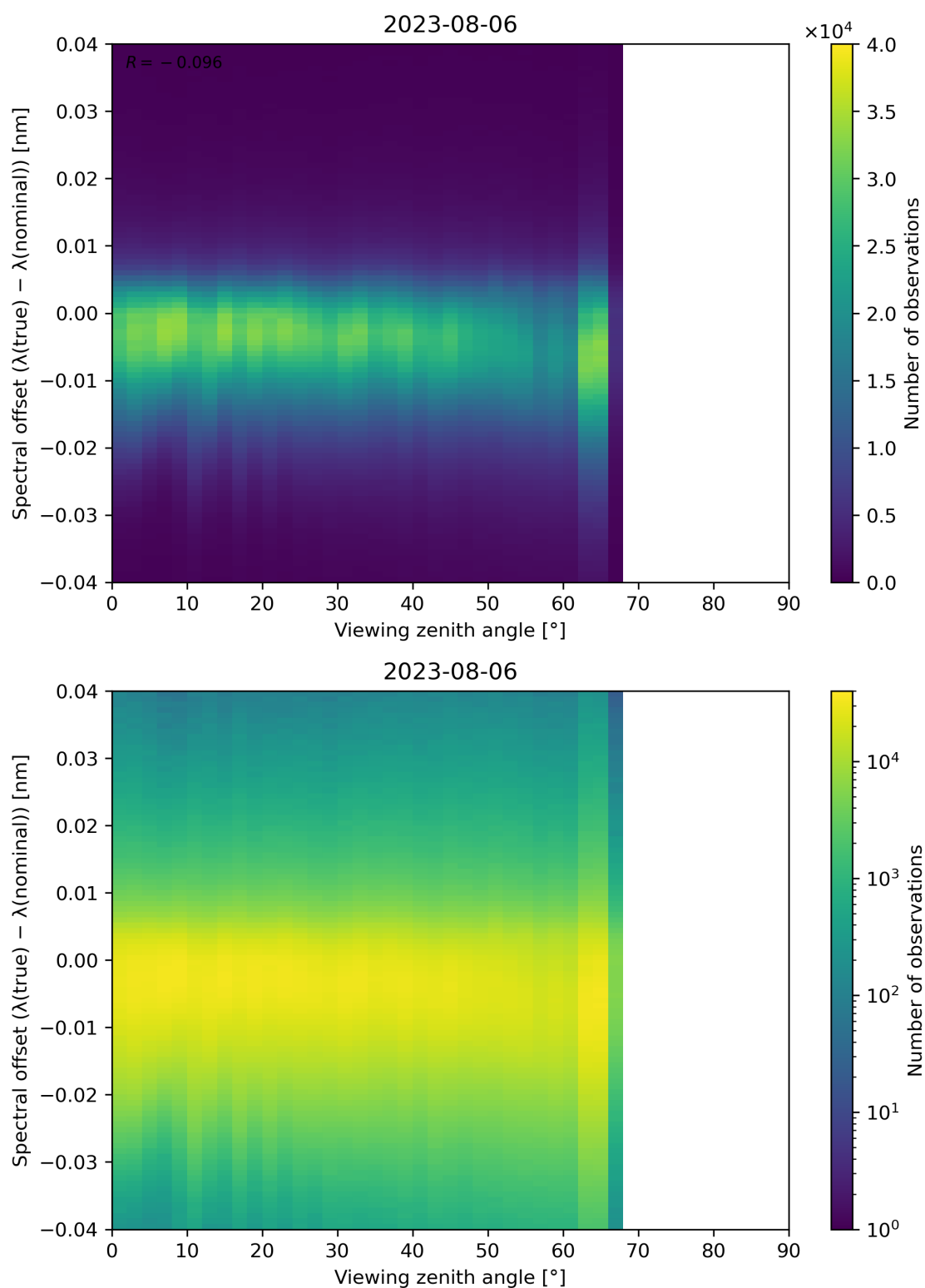
Figure 140: Scatter density plot of “Viewing zenith angle” against “Spectral offset ( \lambda(\text{true}) - \lambda(\text{nominal}) )” for 2023-08-05 to 2023-08-07.
