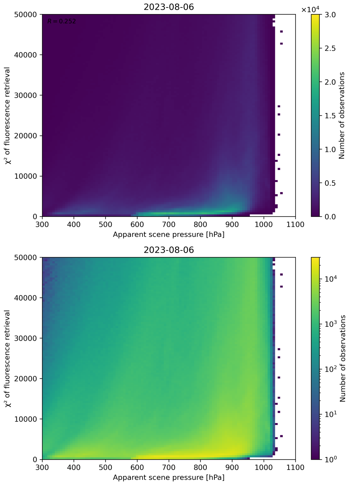
Figure 64: Scatter density plot of “Apparent scene pressure” against “ \chi^2 of fluorescence retrieval” for 2023-08-05 to 2023-08-07.
