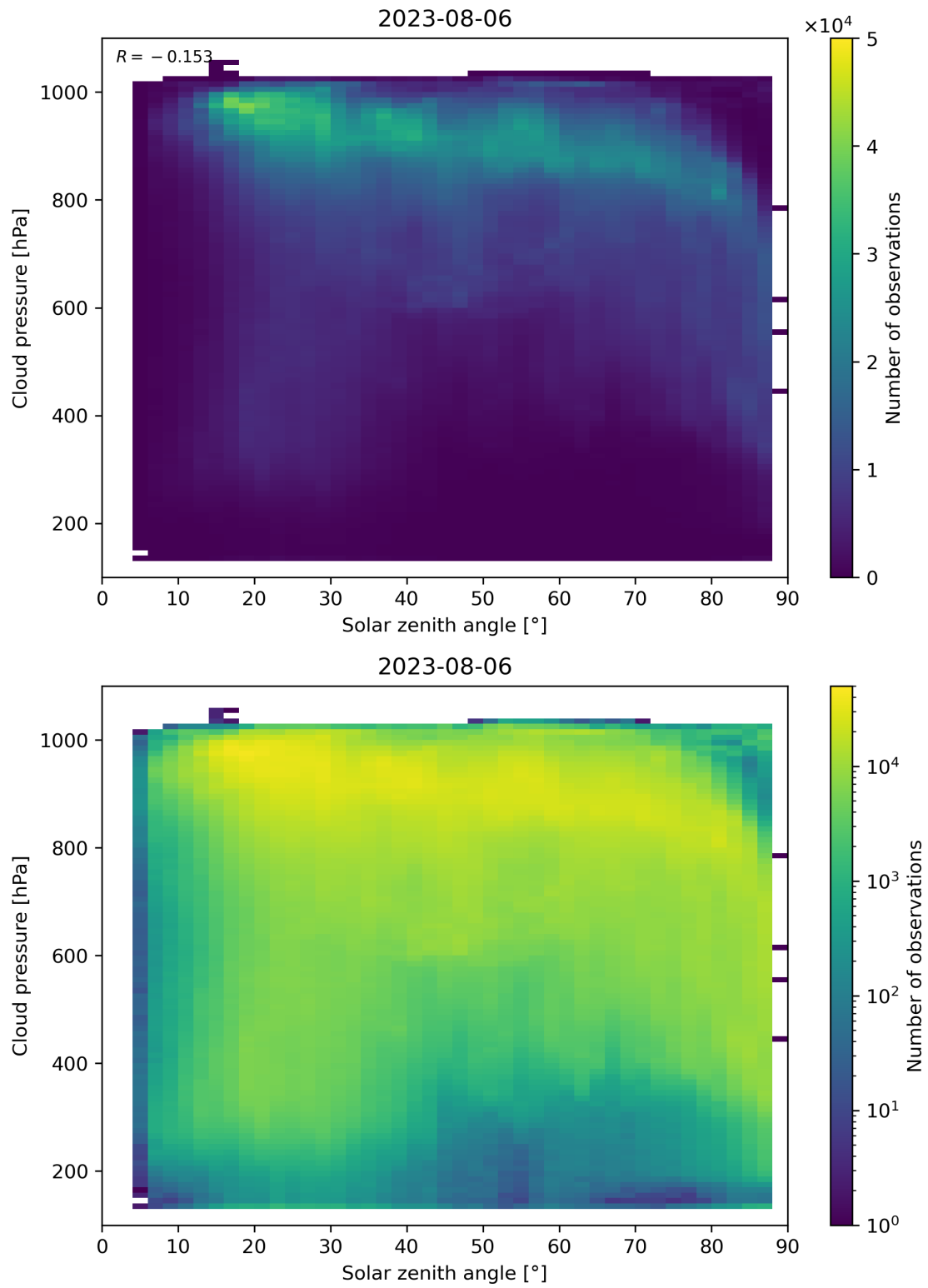
Figure 122: Scatter density plot of “Solar zenith angle” against “Cloud pressure” for 2023-08-05 to 2023-08-07.
