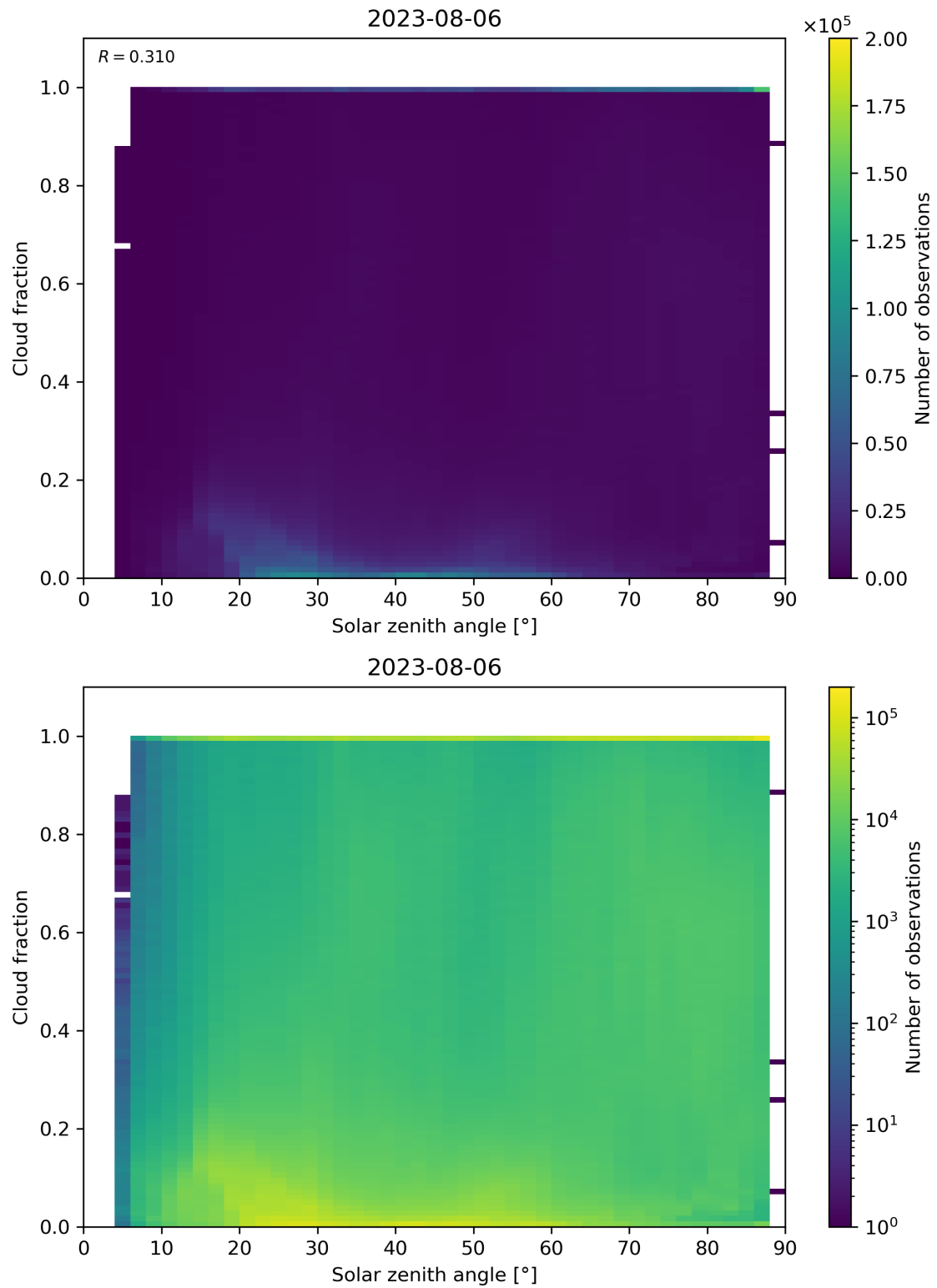
Figure 121: Scatter density plot of “Solar zenith angle” against “Cloud fraction” for 2023-08-05 to 2023-08-07.
