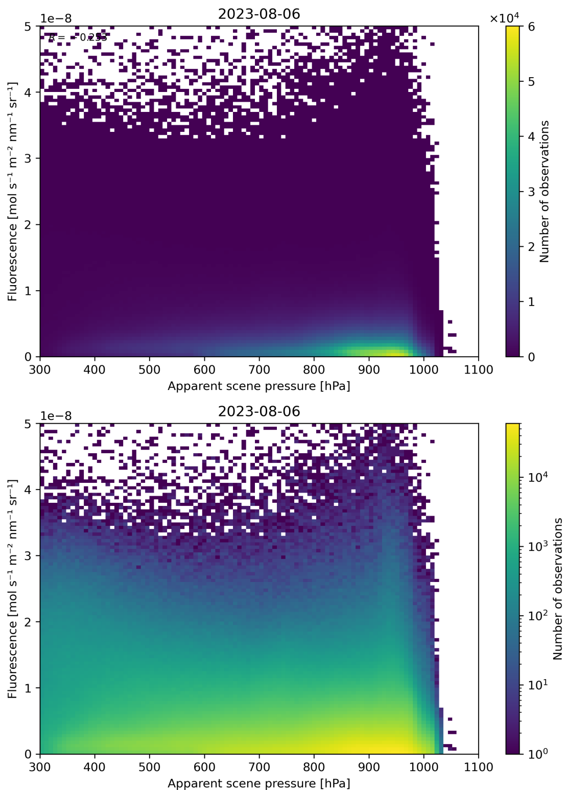
Figure 65: Scatter density plot of “Apparent scene pressure” against “Fluorescence” for 2023-08-05 to 2023-08-07.
