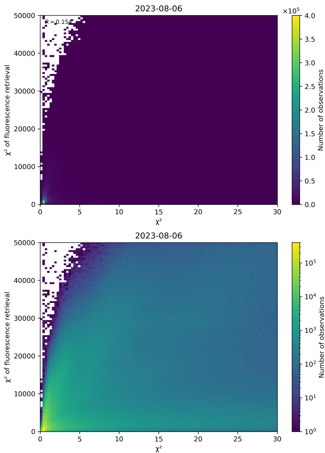
Figure 69: Scatter density plot of “ \chi^2 ” against “ \chi^2 of fluorescence retrieval” for 2023-08-05 to 2023-08-07.
