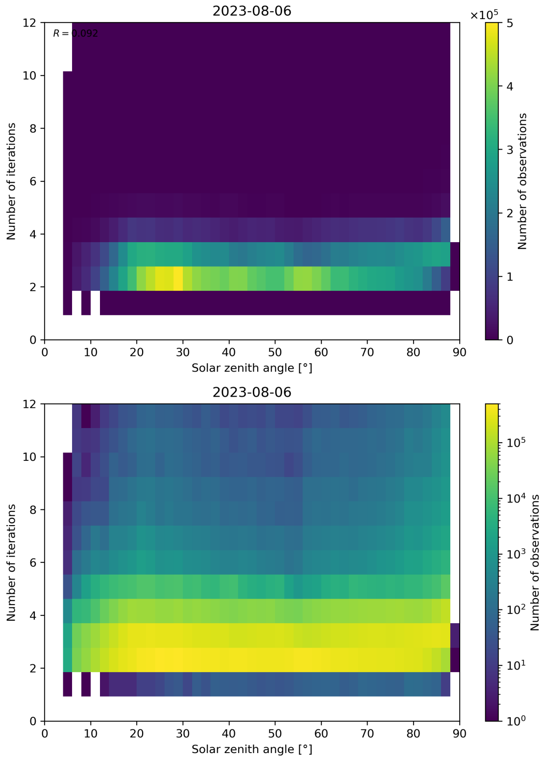
Figure 125: Scatter density plot of “Solar zenith angle” against “Number of iterations” for 2023-08-05 to 2023-08-07.
