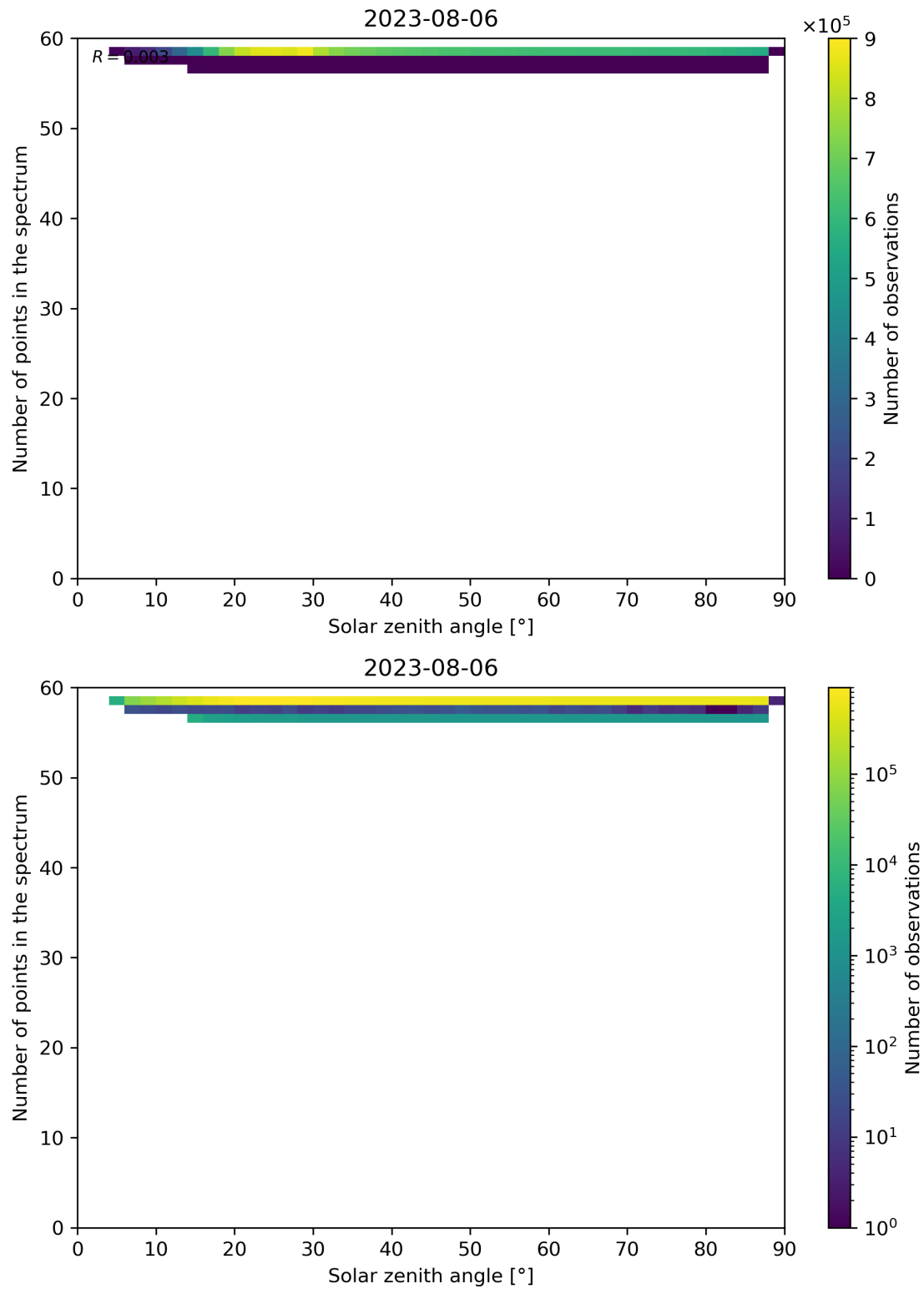
Figure 126: Scatter density plot of “Solar zenith angle” against “Number of points in the spectrum” for 2023-08-05 to 2023-08-07.
