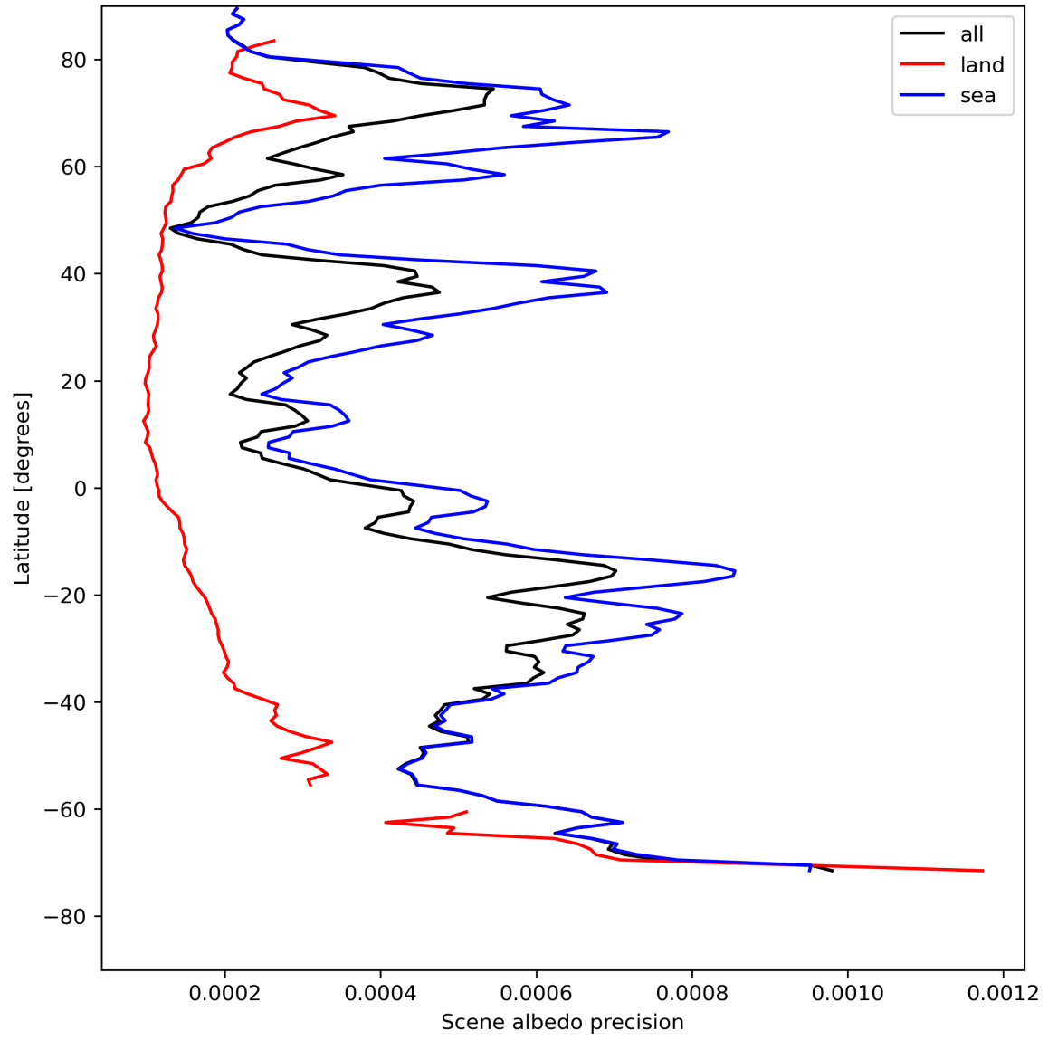
Figure 18: Zonal average of “Scene albedo precision” for 2023-08-05 to 2023-08-07.
