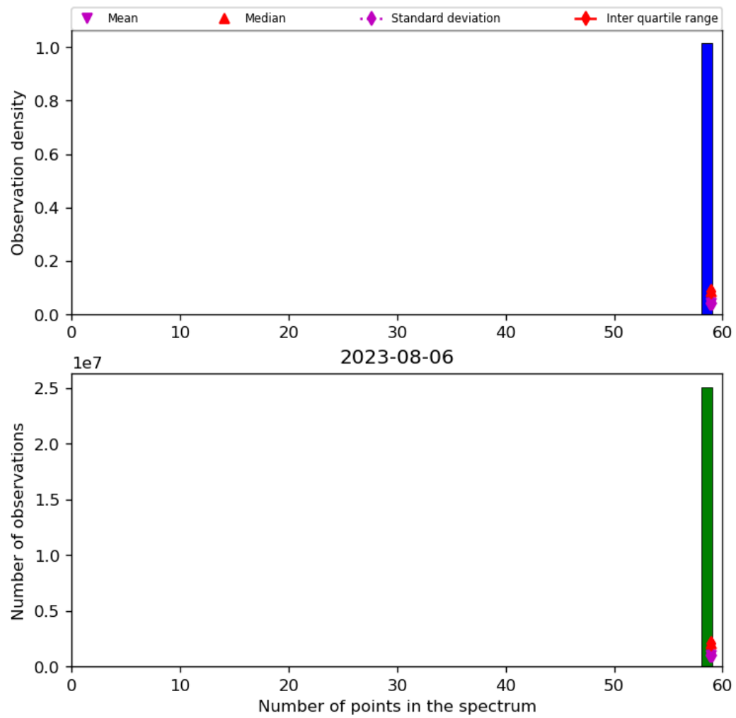
Figure 44: Histogram of “Number of points in the spectrum” for 2023-08-05 to 2023-08-07
