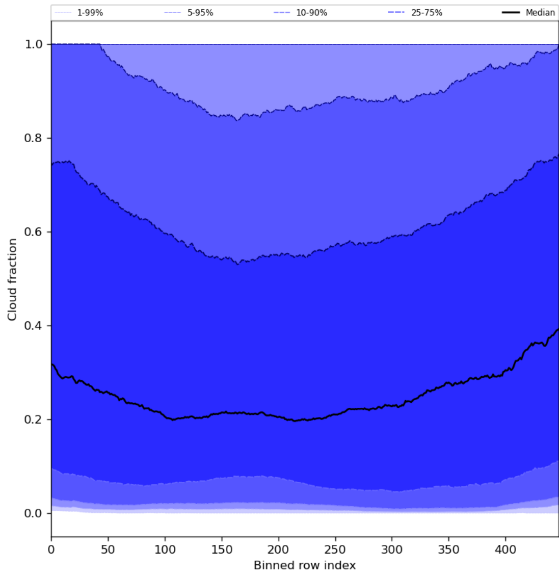
Figure 49: Along track statistics of “Cloud fraction” for 2023-08-05 to 2023-08-07
