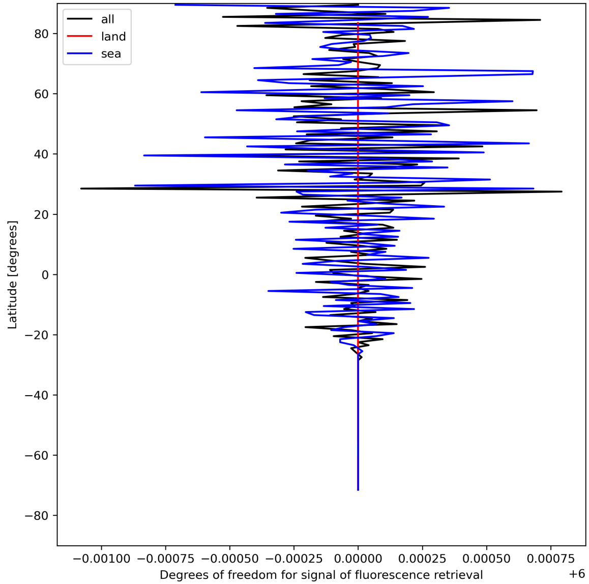
Figure 26: Zonal average of “Degrees of freedom for signal of fluorescence retrieval” for 2023-08-05 to 2023-08-07.
