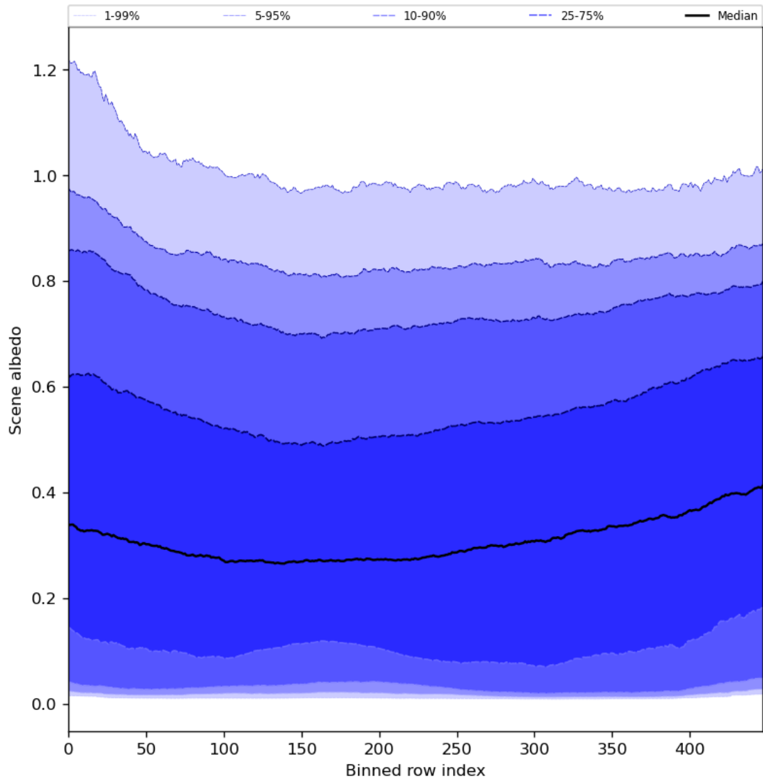
Figure 51: Along track statistics of “Scene albedo” for 2023-08-05 to 2023-08-07
