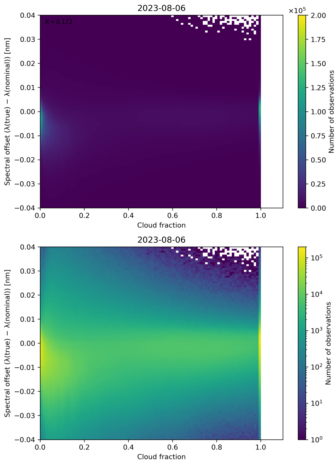
Figure 83: Scatter density plot of “Cloud fraction” against “Spectral offset ( \lambda(\text{true}) - \lambda(\text{nominal}) )” for 2023-08-05 to 2023-08-07.
