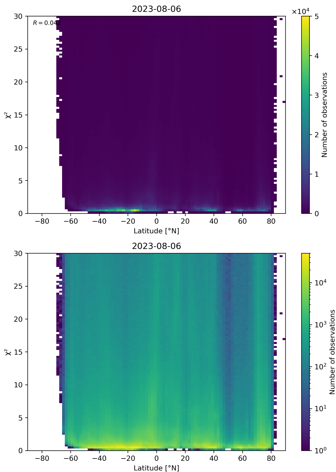
Figure 97: Scatter density plot of “Latitude” against “ \chi^2 ” for 2023-08-05 to 2023-08-07.
