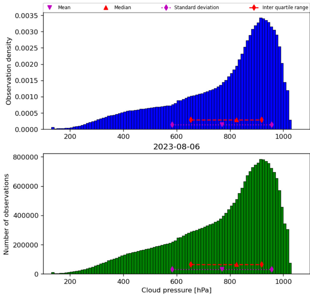
Figure 30: Histogram of “Cloud pressure” for 2023-08-05 to 2023-08-07
