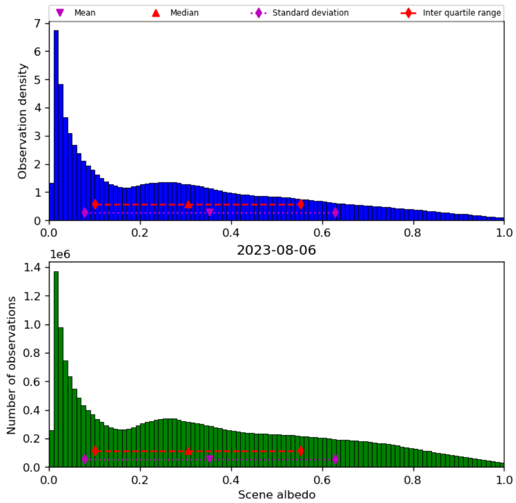
Figure 34: Histogram of “Scene albedo” for 2023-08-05 to 2023-08-07
