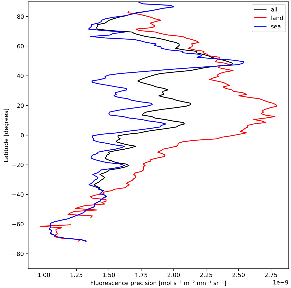
Figure 24: Zonal average of “Fluorescence precision” for 2023-08-05 to 2023-08-07.
