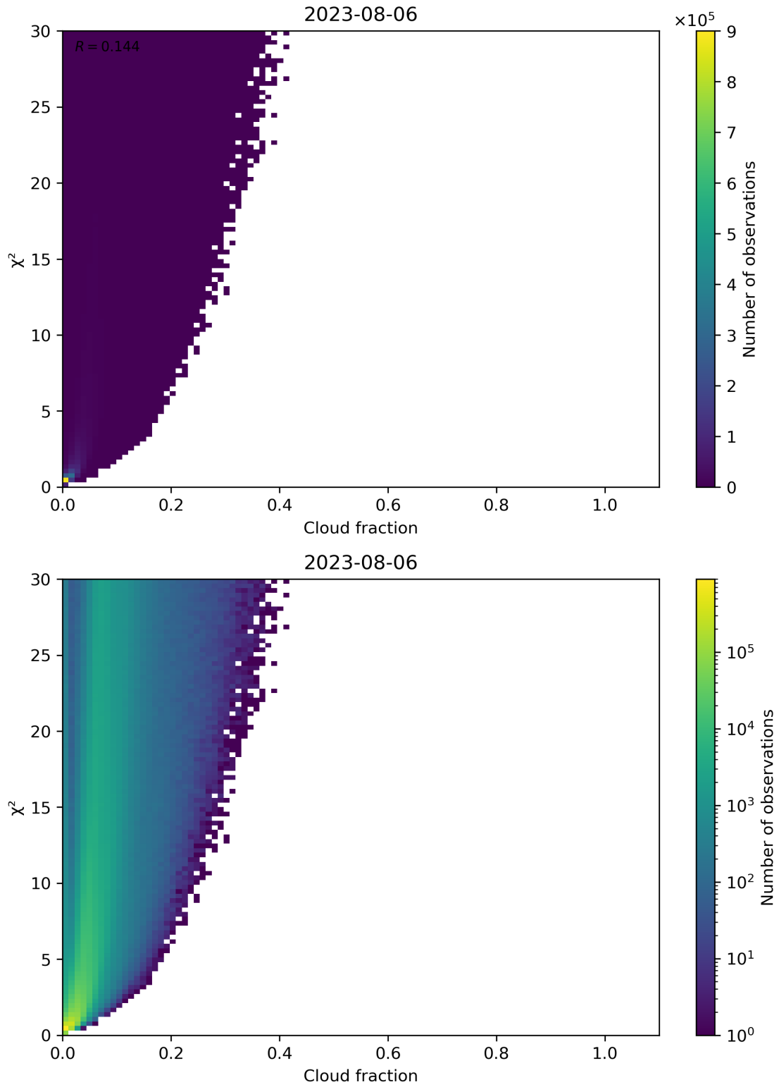
Figure 77: Scatter density plot of “Cloud fraction” against “ \chi^2 ” for 2023-08-05 to 2023-08-07.
