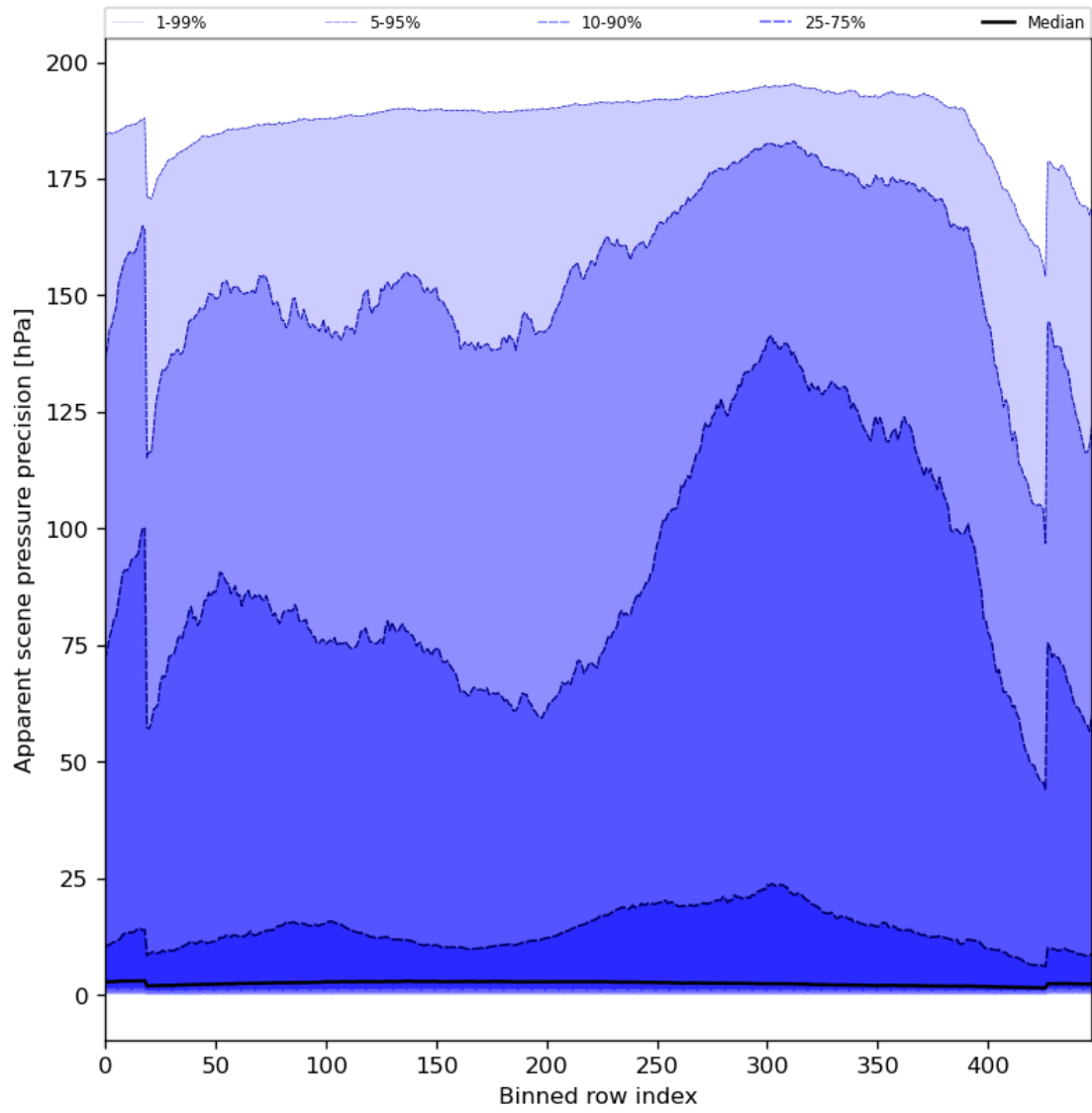
Figure 54: Along track statistics of “Apparent scene pressure precision” for 2023-08-05 to 2023-08-07
