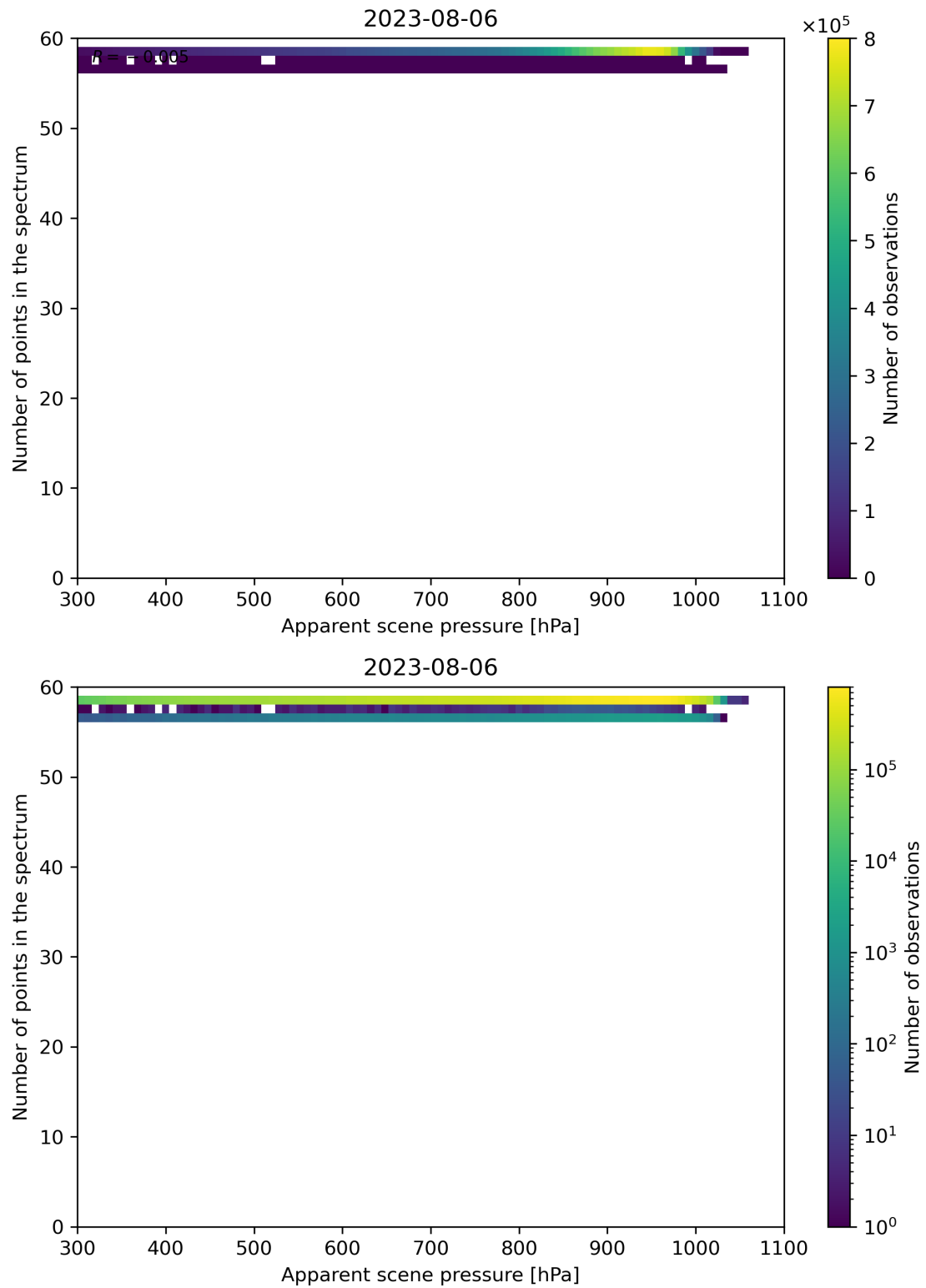
Figure 67: Scatter density plot of “Apparent scene pressure” against “Number of points in the spectrum” for 2023-08-05 to 2023-08-07.
