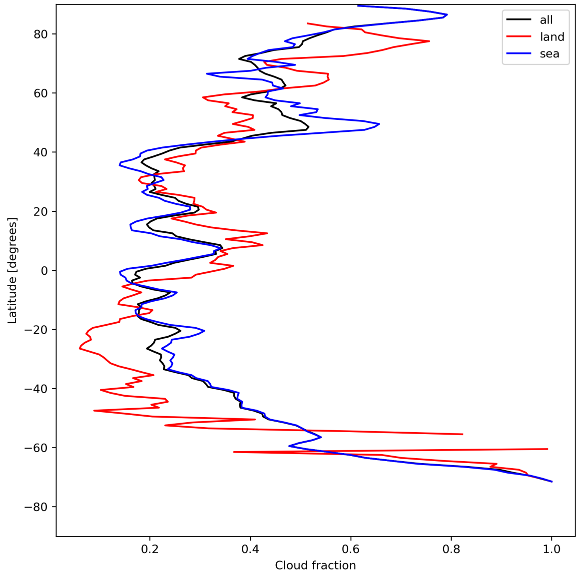
Figure 15: Zonal average of “Cloud fraction” for 2023-08-05 to 2023-08-07.
