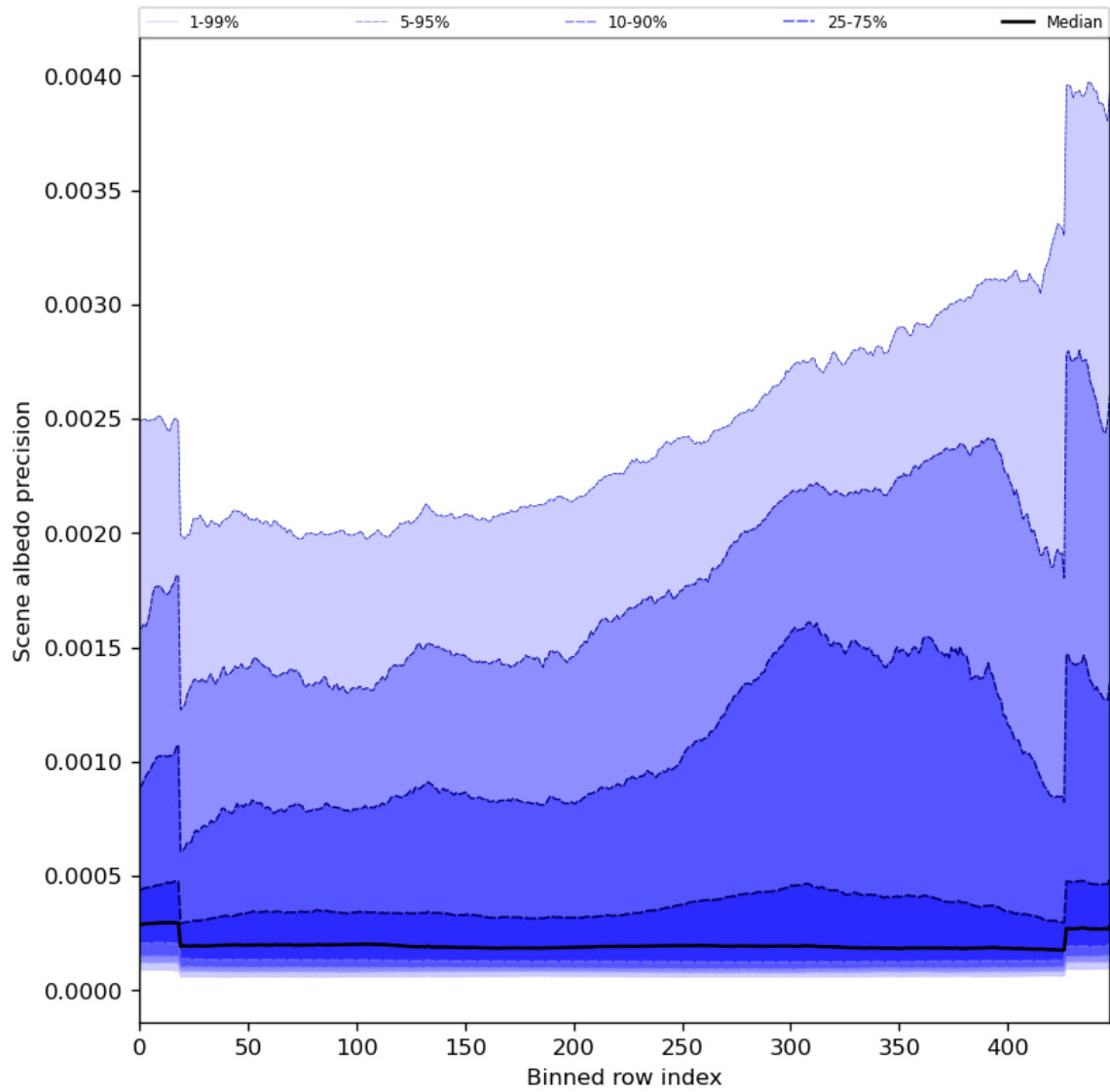
Figure 52: Along track statistics of “Scene albedo precision” for 2023-08-05 to 2023-08-07
