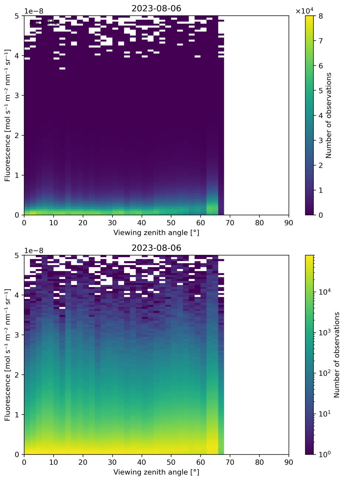
Figure 134: Scatter density plot of “Viewing zenith angle” against “Fluorescence” for 2023-08-05 to 2023-08-07.
