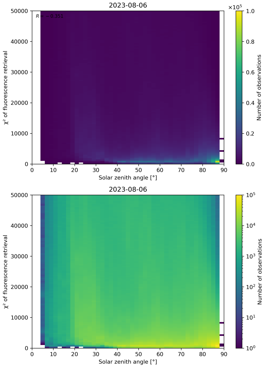
Figure 120: Scatter density plot of “Solar zenith angle” against “ \chi^2 of fluorescence retrieval” for 2023-08-05 to 2023-08-07.
