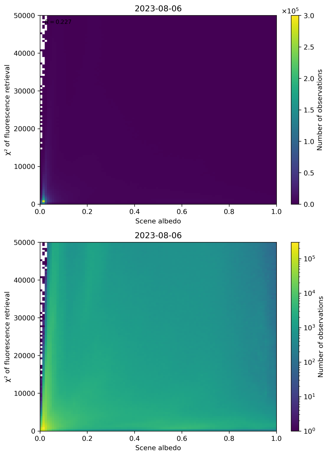
Figure 113: Scatter density plot of “Scene albedo” against “ \chi^2 of fluorescence retrieval” for 2023-08-05 to 2023-08-07.
