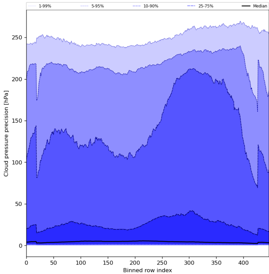
Figure 48: Along track statistics of “Cloud pressure precision” for 2023-08-05 to 2023-08-07
