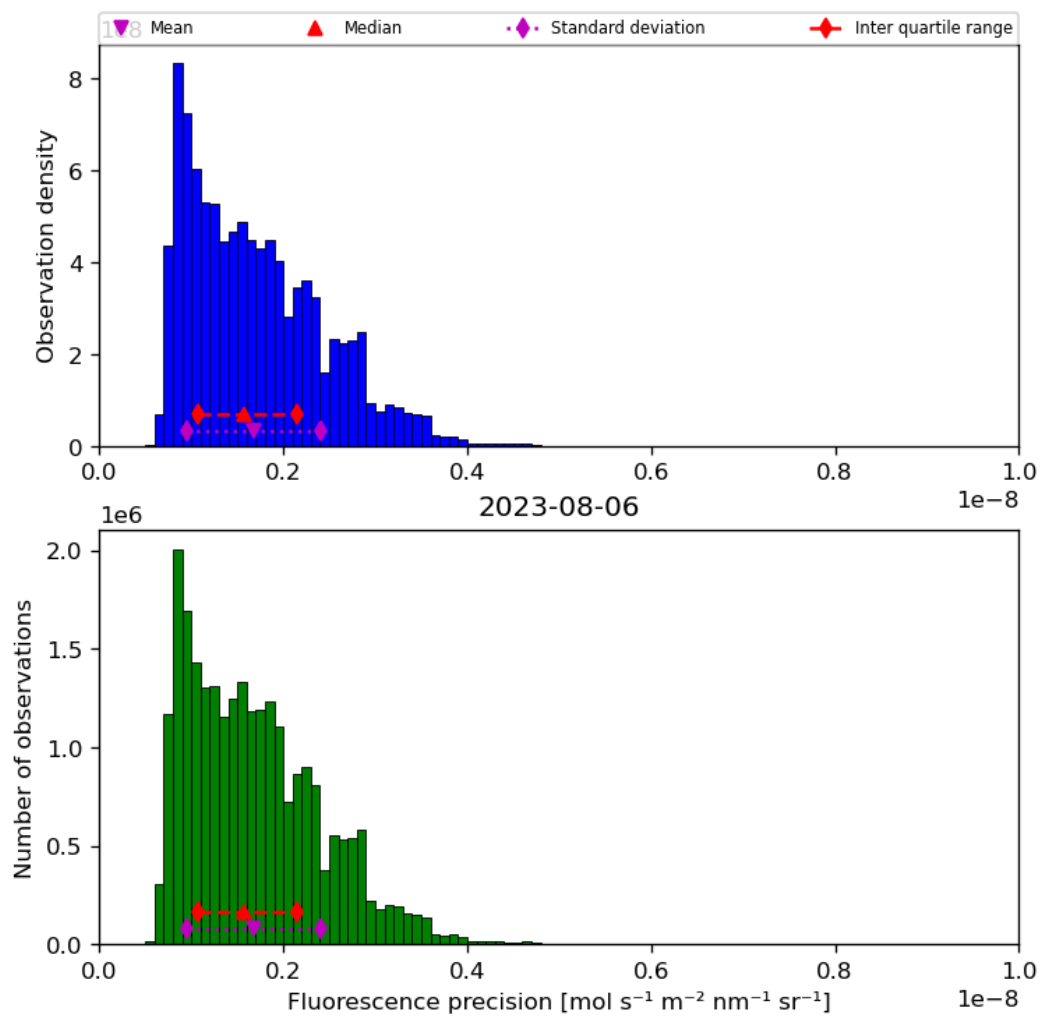
Figure 41: Histogram of “Fluorescence precision” for 2023-08-05 to 2023-08-07
