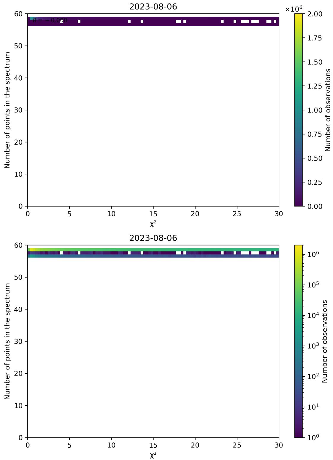
Figure 74: Scatter density plot of " \chi^2 " against "Number of points in the spectrum" for 2023-08-05 to 2023-08-07.
