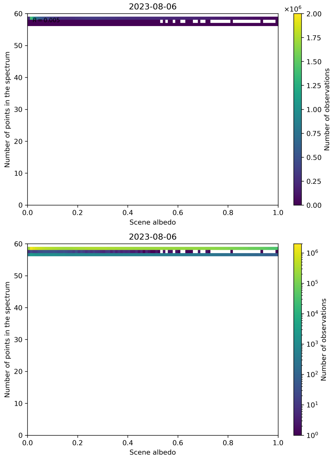
Figure 116: Scatter density plot of “Scene albedo” against “Number of points in the spectrum” for 2023-08-05 to 2023-08-07.
