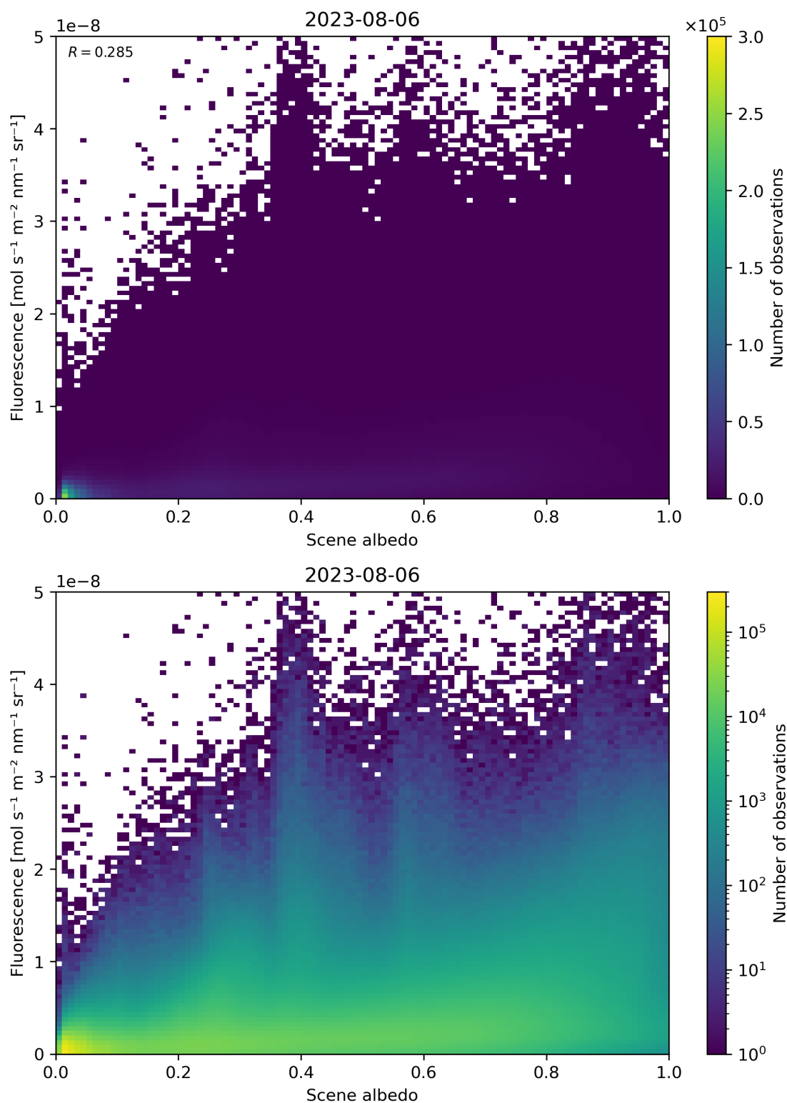
Figure 114: Scatter density plot of “Scene albedo” against “Fluorescence” for 2023-08-05 to 2023-08-07.
