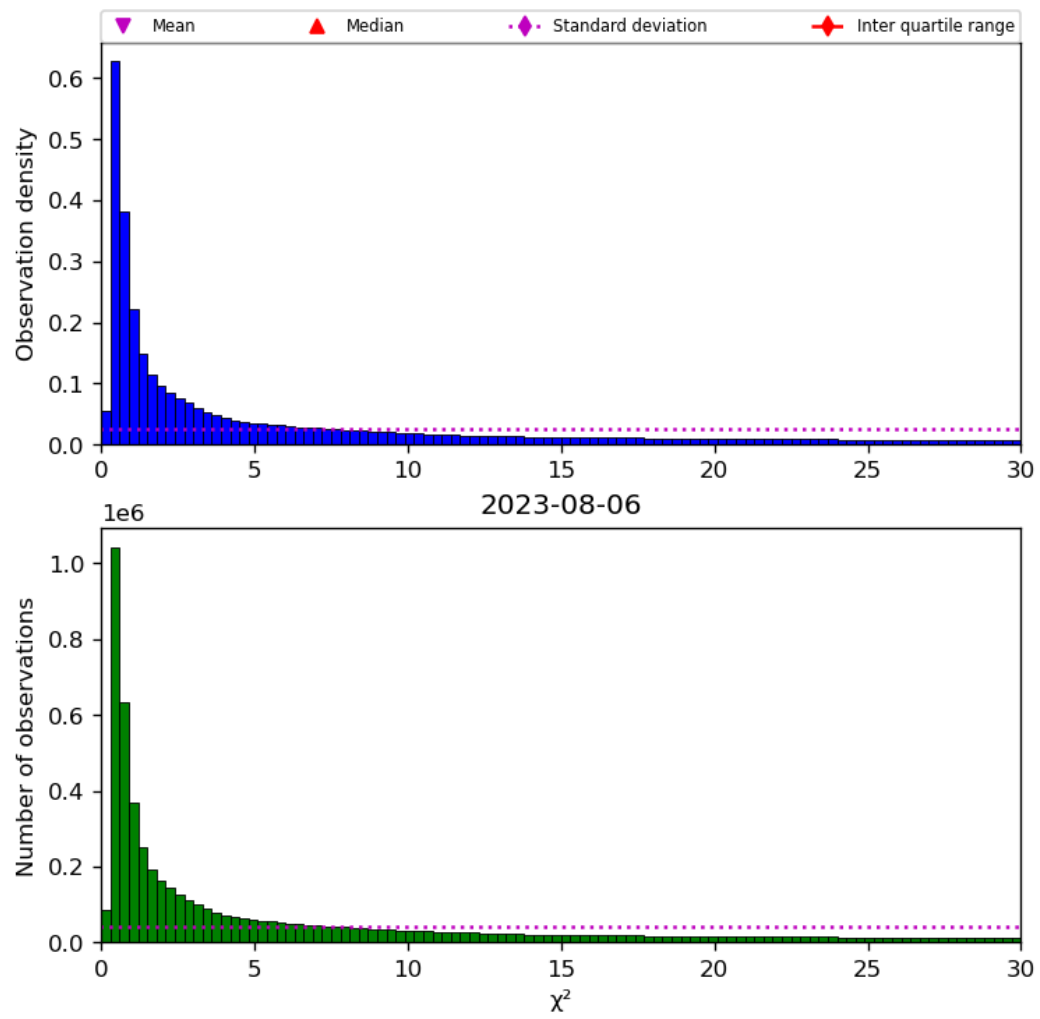
Figure 38: Histogram of “ \chi^2 ” for 2023-08-05 to 2023-08-07
