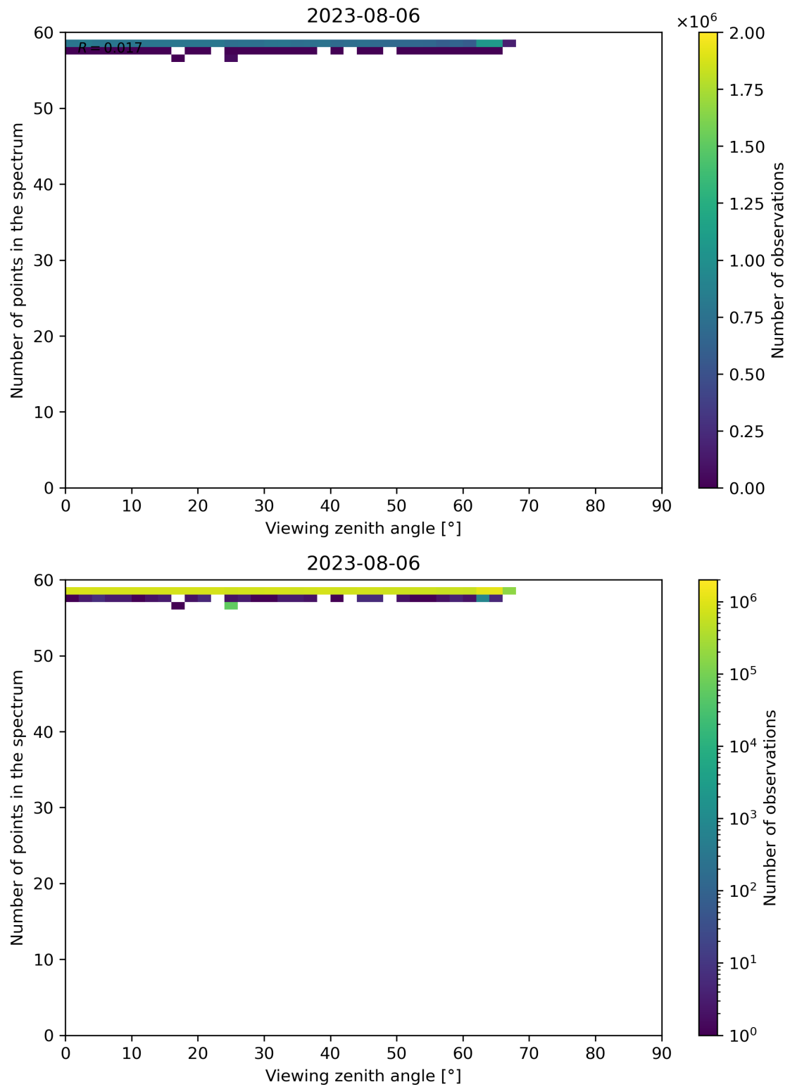
Figure 137: Scatter density plot of “Viewing zenith angle” against “Number of points in the spectrum” for 2023-08-05 to 2023-08-07.
