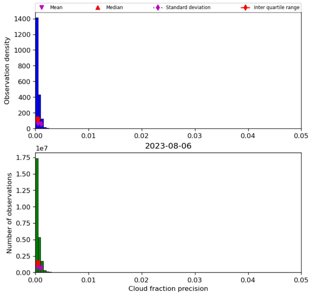
Figure 33: Histogram of “Cloud fraction precision” for 2023-08-05 to 2023-08-07
