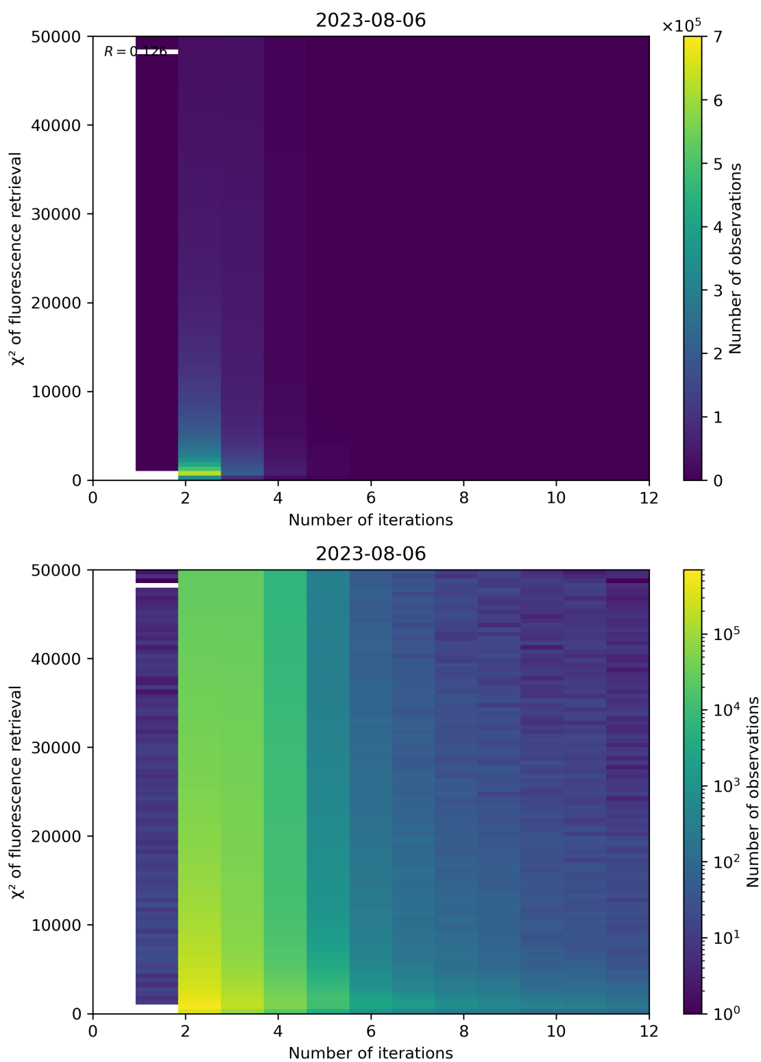
Figure 106: Scatter density plot of “Number of iterations” against “ \chi^2 of fluorescence retrieval” for 2023-08-05 to 2023-08-07.
