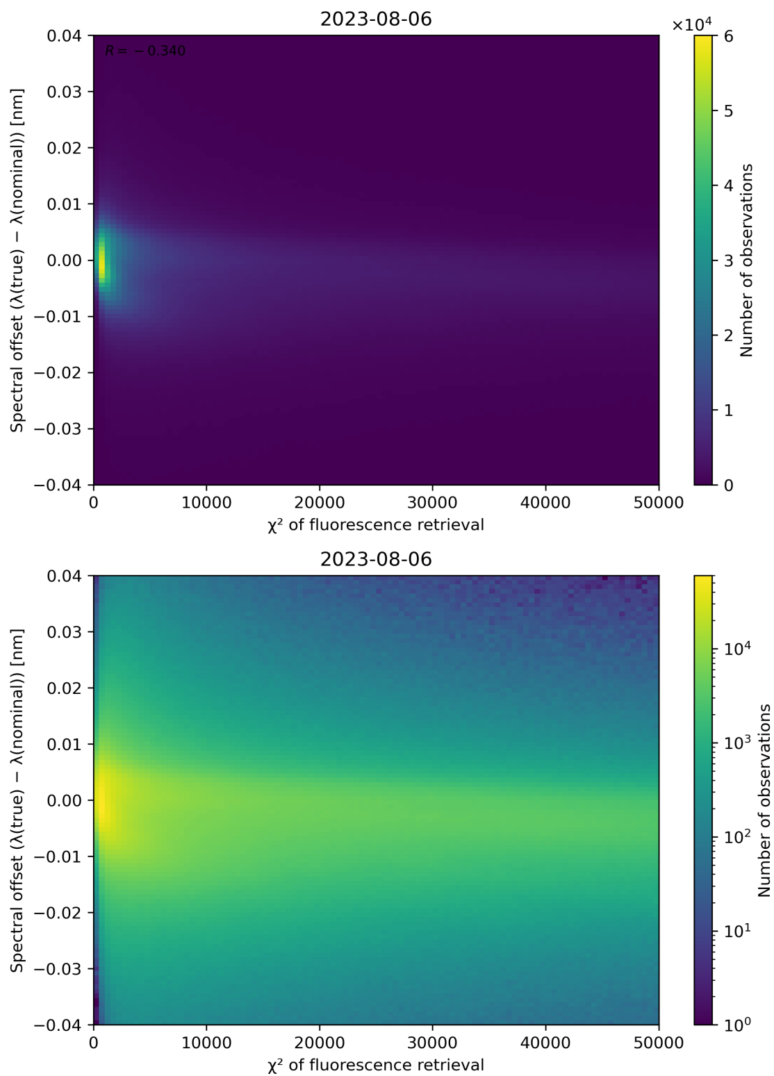
Figure 72: Scatter density plot of " \chi^2 of fluorescence retrieval" against "Spectral offset ( \lambda(\text{true}) - \lambda(\text{nominal})) " for 2023-08-05 to 2023-08-07.
