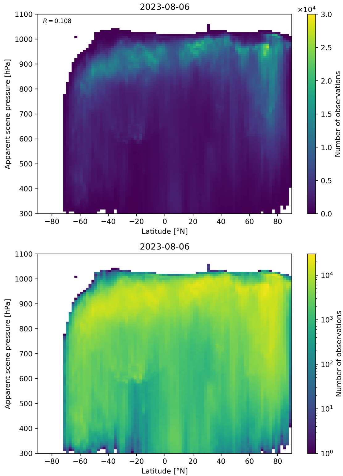
Figure 96: Scatter density plot of “Latitude” against “Apparent scene pressure” for 2023-08-05 to 2023-08-07.
