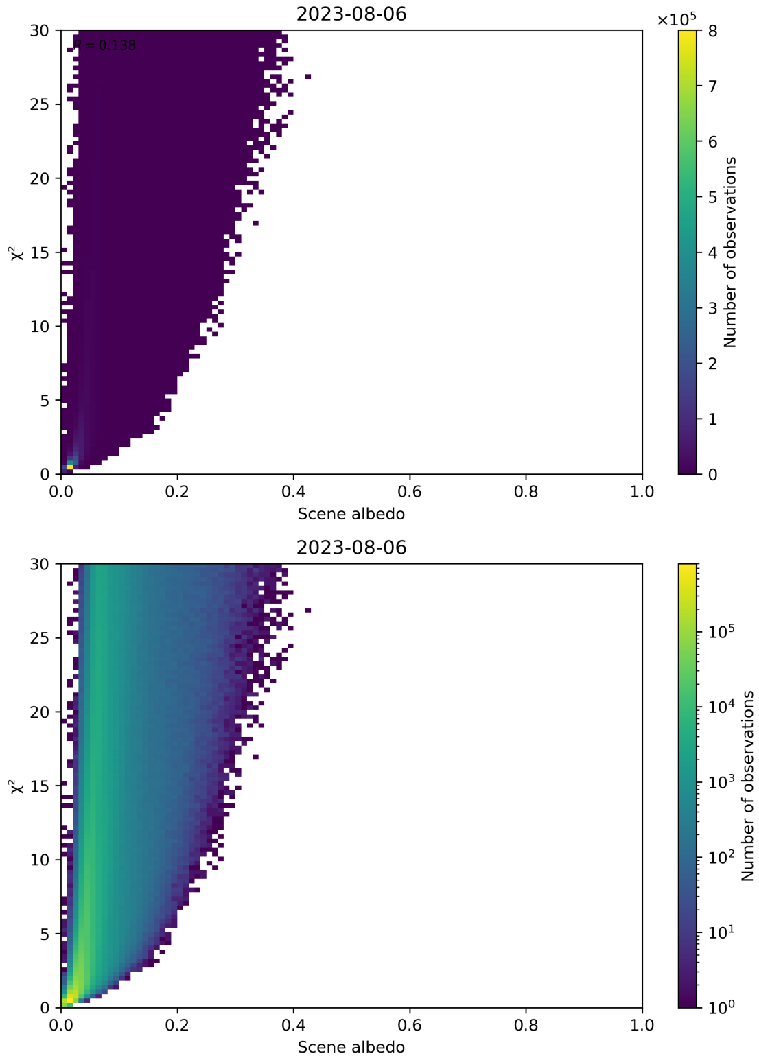
Figure 112: Scatter density plot of “Scene albedo” against “ \chi^2 ” for 2023-08-05 to 2023-08-07.
