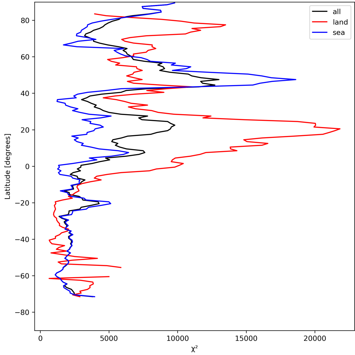
Figure 21: Zonal average of “ \chi^2 ” for 2023-08-05 to 2023-08-07.
