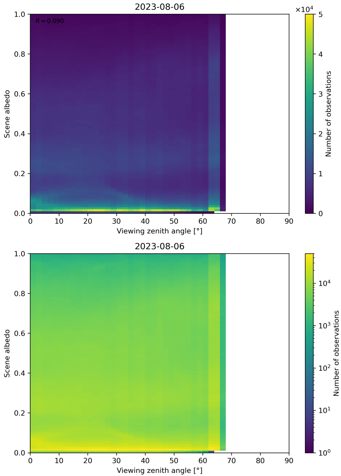
Figure 138: Scatter density plot of “Viewing zenith angle” against “Scene albedo” for 2023-08-05 to 2023-08-07.
