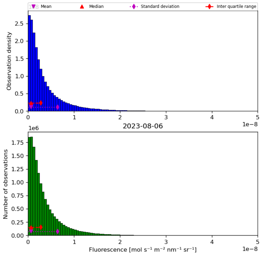
Figure 40: Histogram of “Fluorescence” for 2023-08-05 to 2023-08-07
