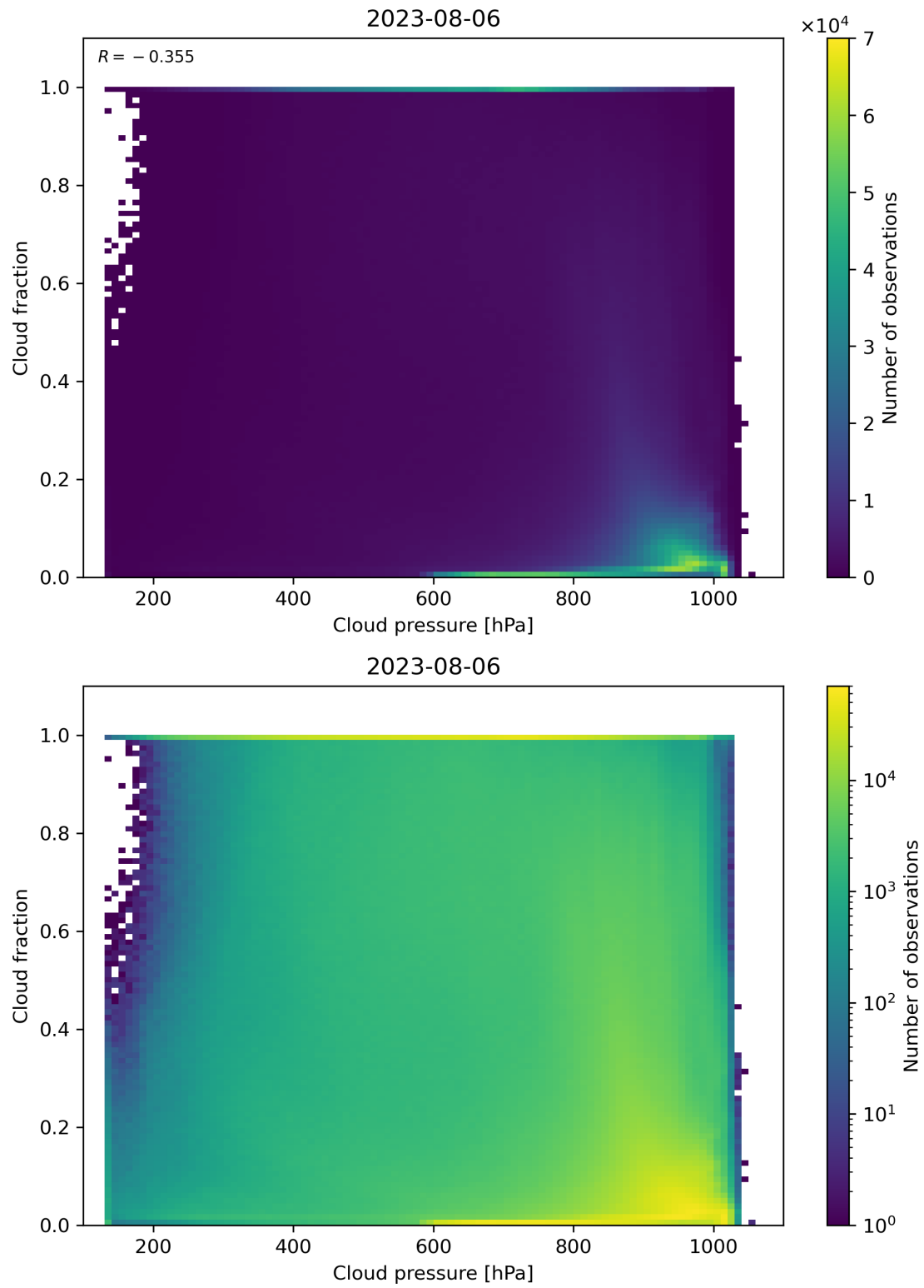
Figure 87: Scatter density plot of “Cloud pressure” against “Cloud fraction” for 2023-08-05 to 2023-08-07.
