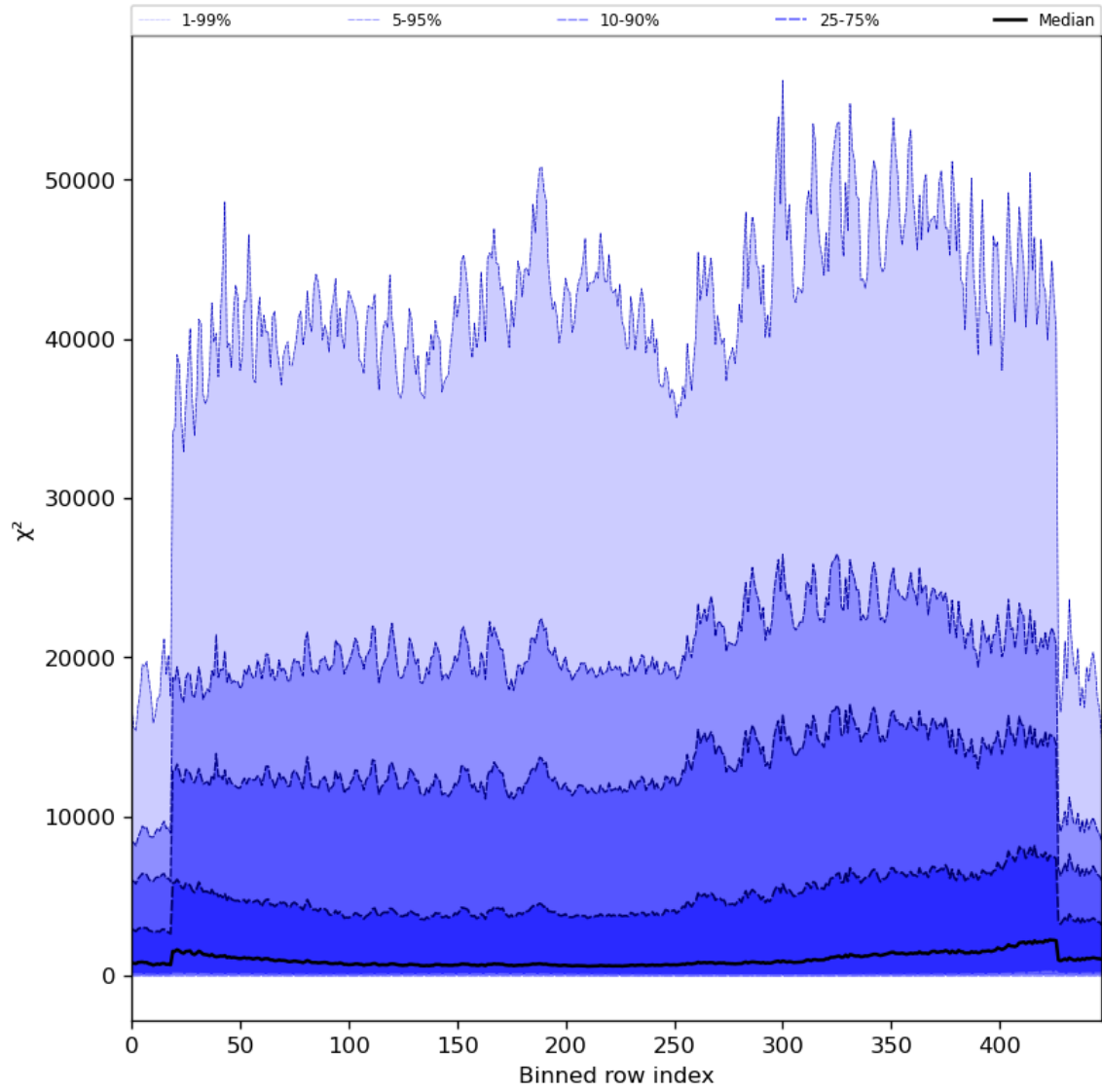
Figure 55: Along track statistics of “ \chi^2 ” for 2023-08-05 to 2023-08-07
