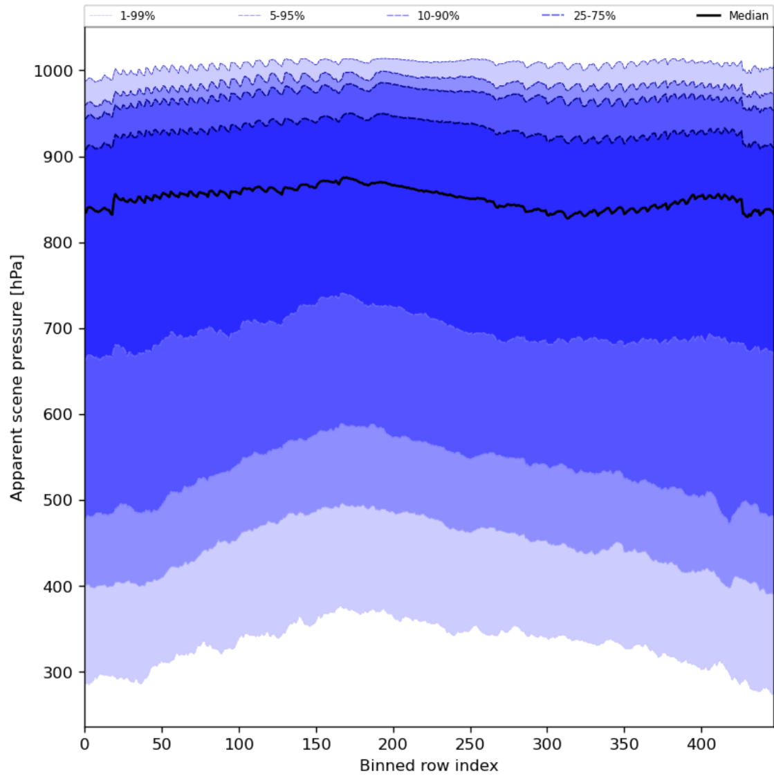
Figure 53: Along track statistics of “Apparent scene pressure” for 2023-08-05 to 2023-08-07
