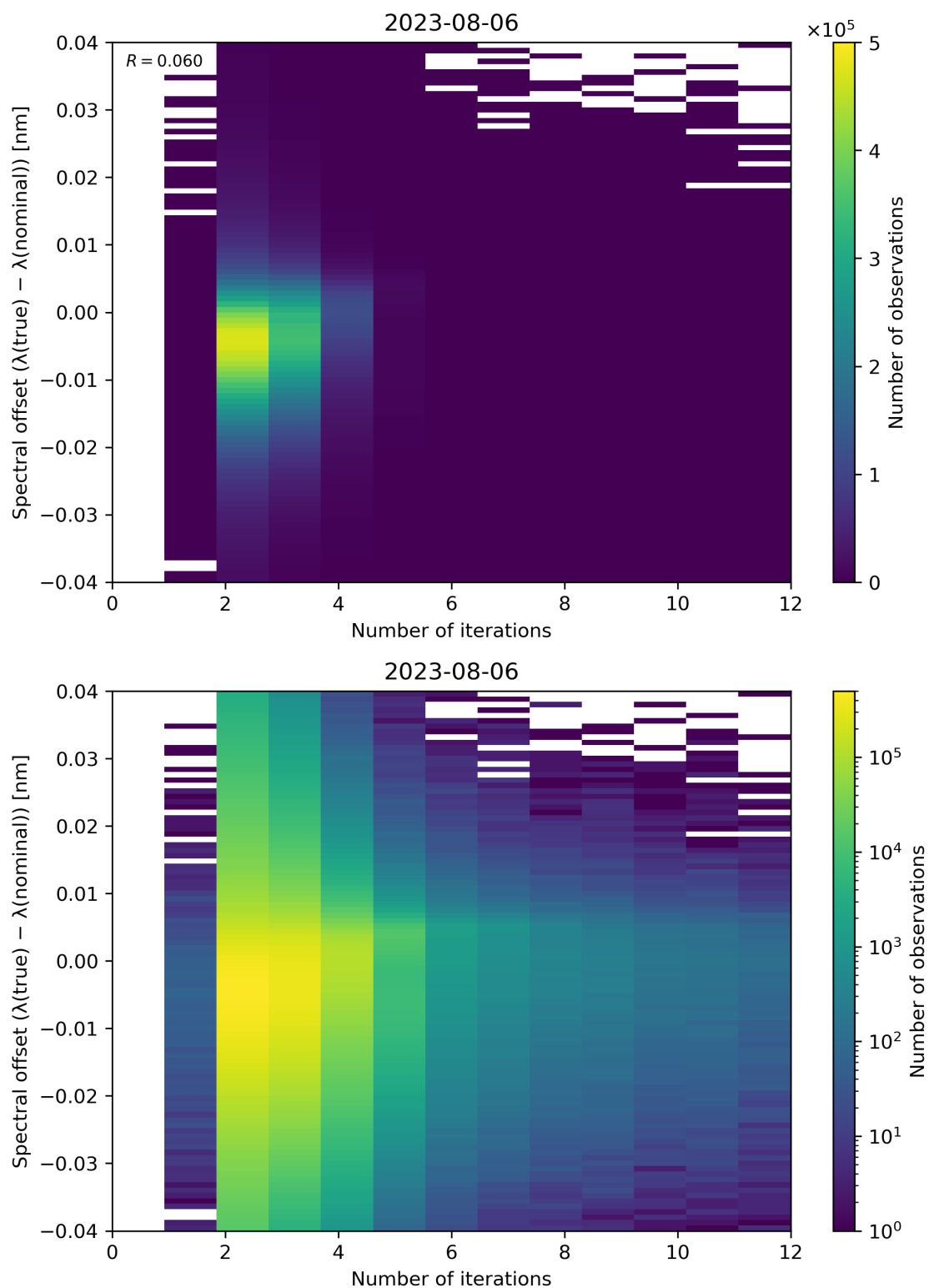
Figure 109: Scatter density plot of “Number of iterations” against “Spectral offset ( \lambda(\text{true}) - \lambda(\text{nominal}) )” for 2023-08-05 to 2023-08-07.
