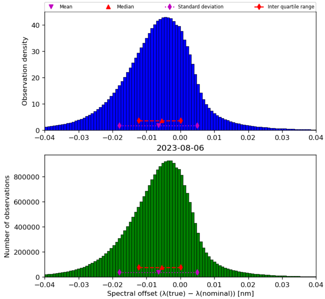
Figure 45: Histogram of “Spectral offset ( \lambda(\text{true}) - \lambda(\text{nominal}) )” for 2023-08-05 to 2023-08-07
