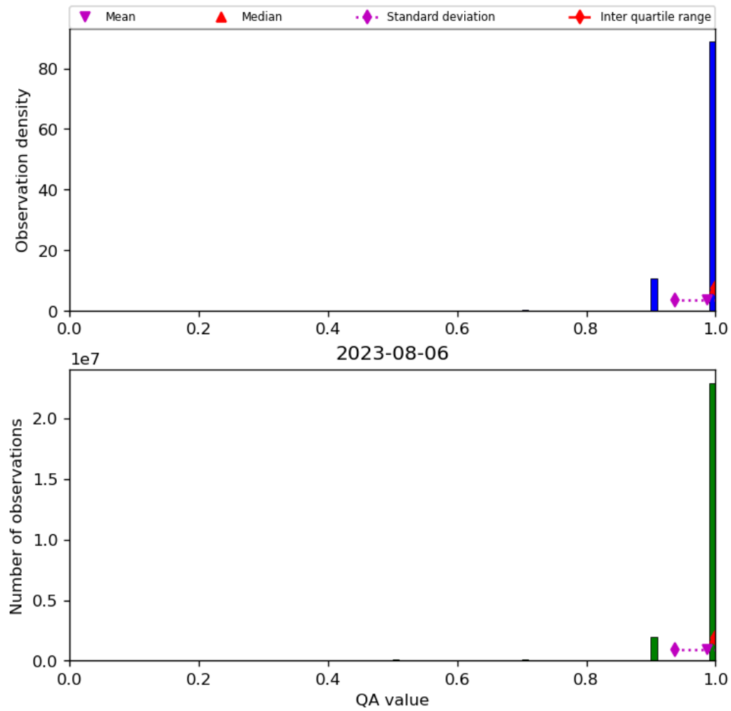
Figure 29: Histogram of “QA value” for 2023-08-05 to 2023-08-07
