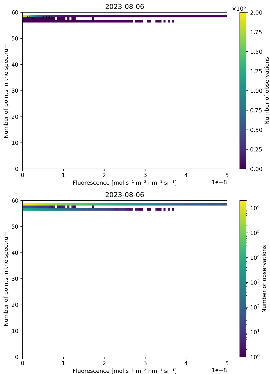
Figure 94: Scatter density plot of “Fluorescence” against “Number of points in the spectrum” for 2023-08-05 to 2023-08-07.
